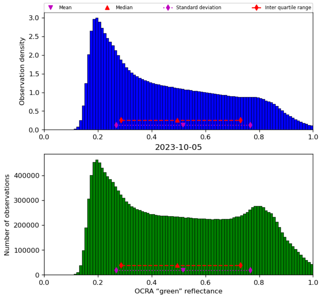
Figure 52: Histogram of “OCRA “green” reflectance” for 2023-10-04 to 2023-10-06
