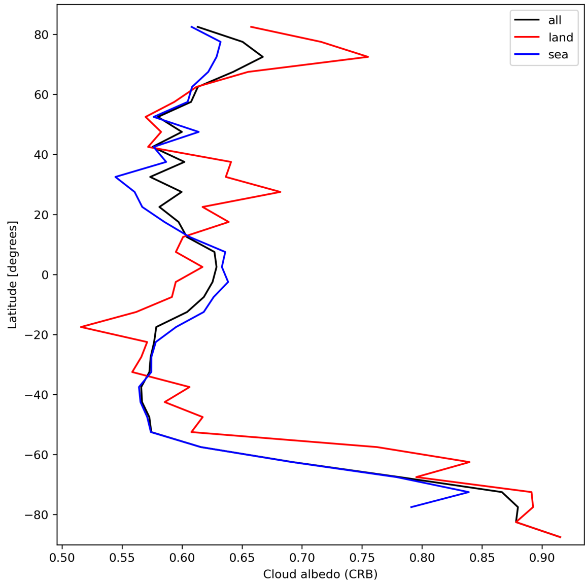
Figure 28: Zonal average of “Cloud albedo (CRB)” for 2023-10-04 to 2023-10-06.
