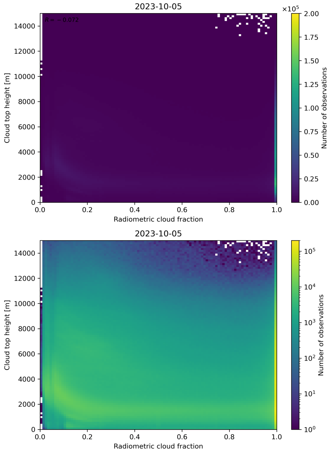
Figure 76: Scatter density plot of “Radiometric cloud fraction” against “Cloud top height” for 2023-10-04 to 2023-10-06.
