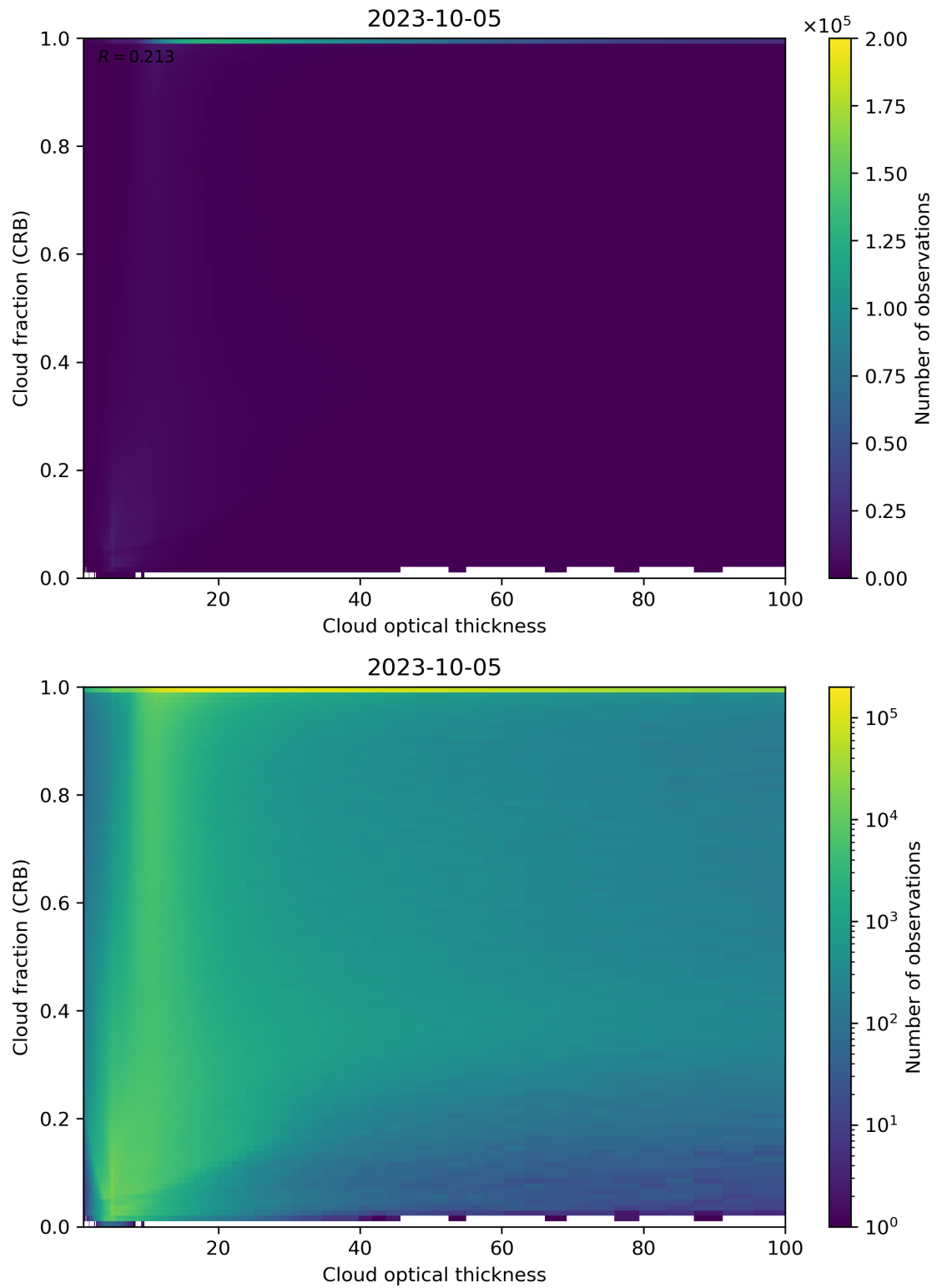
Figure 84: Scatter density plot of “Cloud optical thickness” against “Cloud fraction (CRB)” for 2023-10-04 to 2023-10-06.
