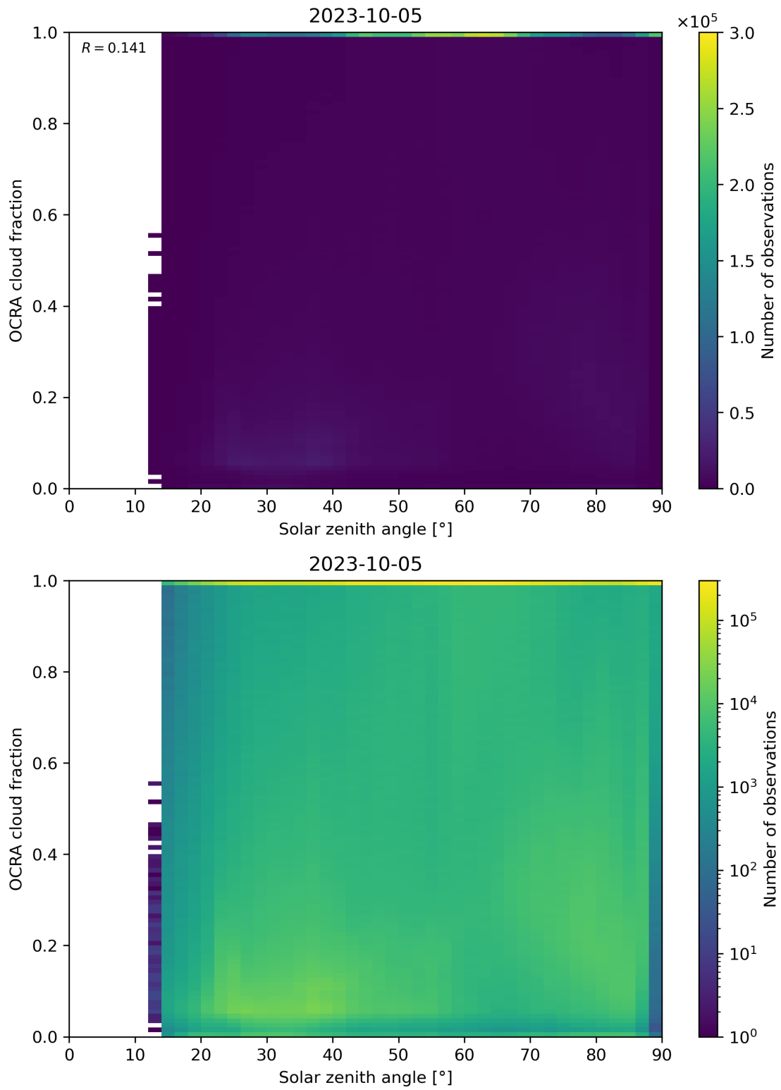
Figure 100: Scatter density plot of “Solar zenith angle” against “OCRA cloud fraction” for 2023-10-04 to 2023-10-06.
