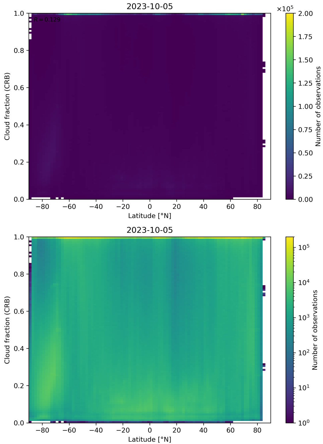
Figure 94: Scatter density plot of “Latitude” against “Cloud fraction (CRB)” for 2023-10-04 to 2023-10-06.
