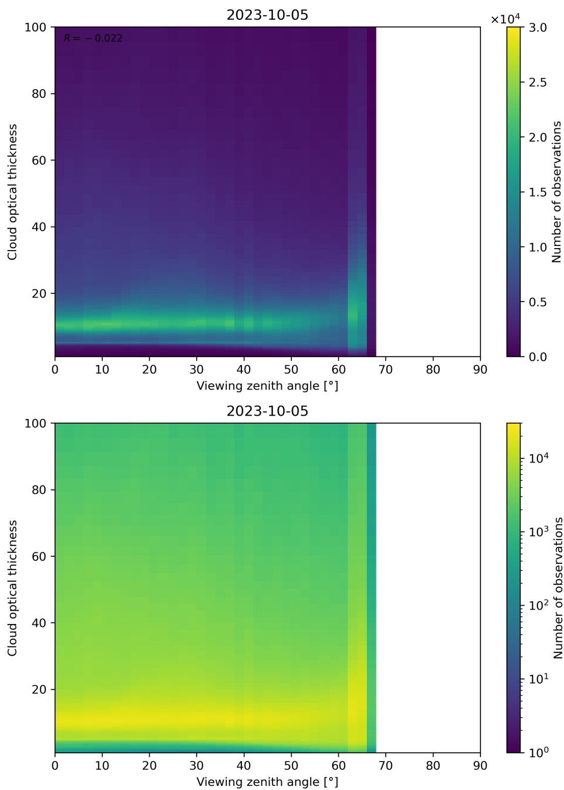
Figure 111: Scatter density plot of “Viewing zenith angle” against “Cloud optical thickness” for 2023-10-04 to 2023-10-06.
