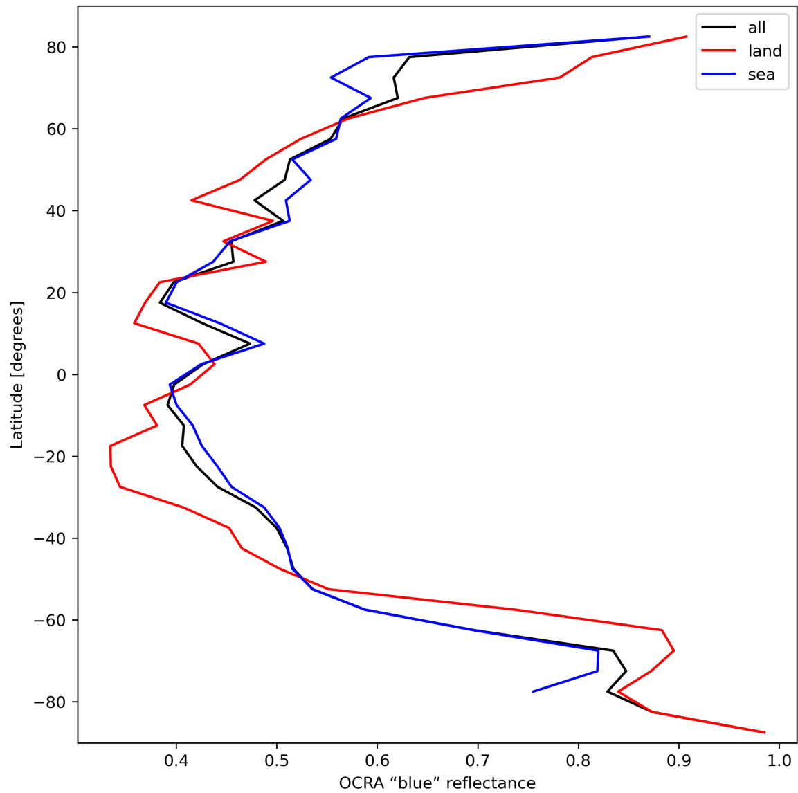
Figure 35: Zonal average of “OCRA “blue” reflectance” for 2023-10-04 to 2023-10-06.
