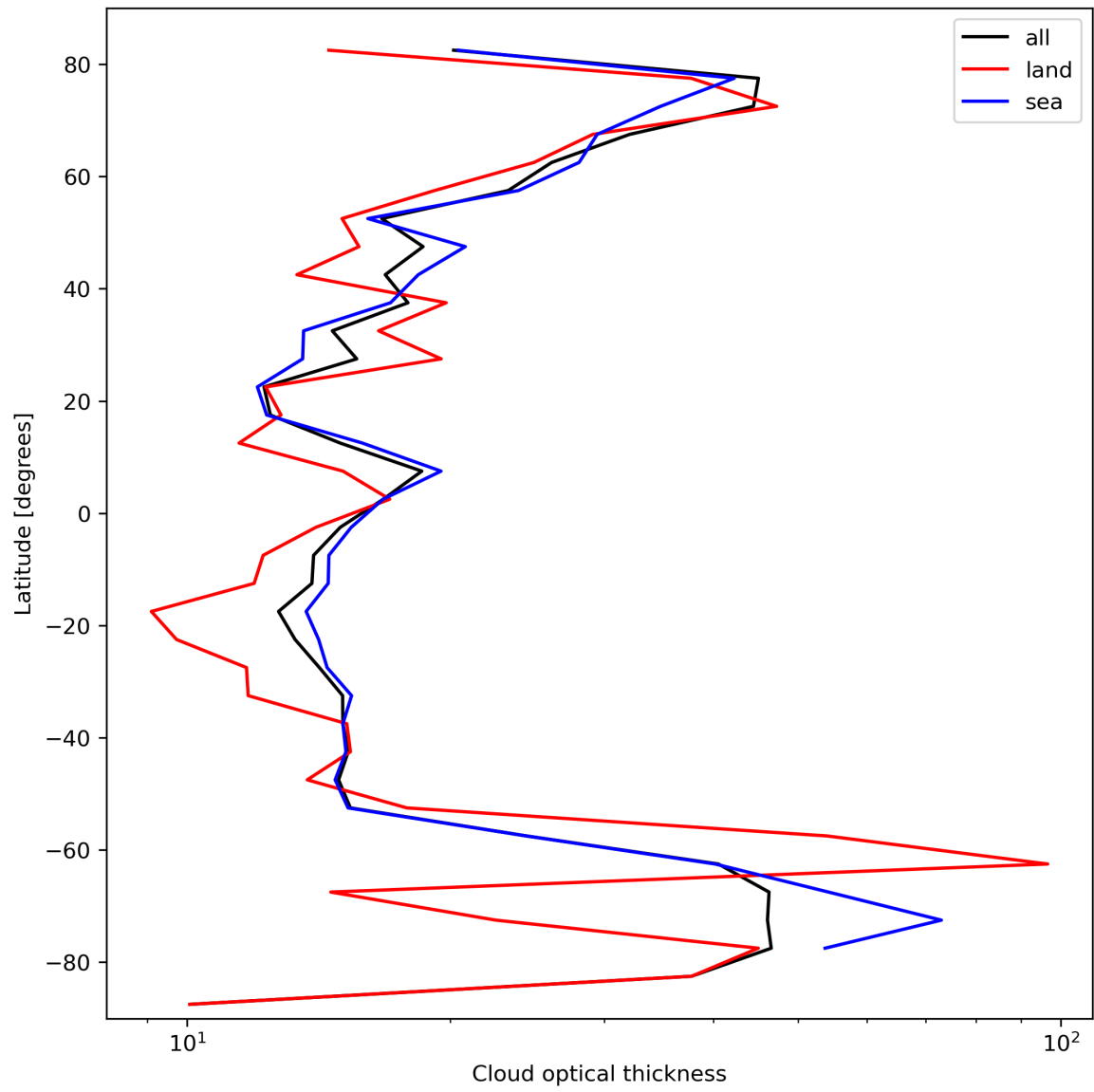
Figure 25: Zonal average of “Cloud optical thickness” for 2023-10-04 to 2023-10-06.
