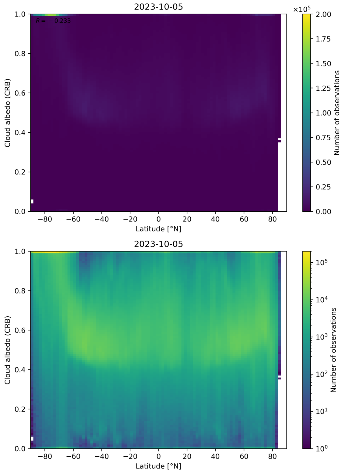
Figure 91: Scatter density plot of “Latitude” against “Cloud albedo (CRB)” for 2023-10-04 to 2023-10-06.
