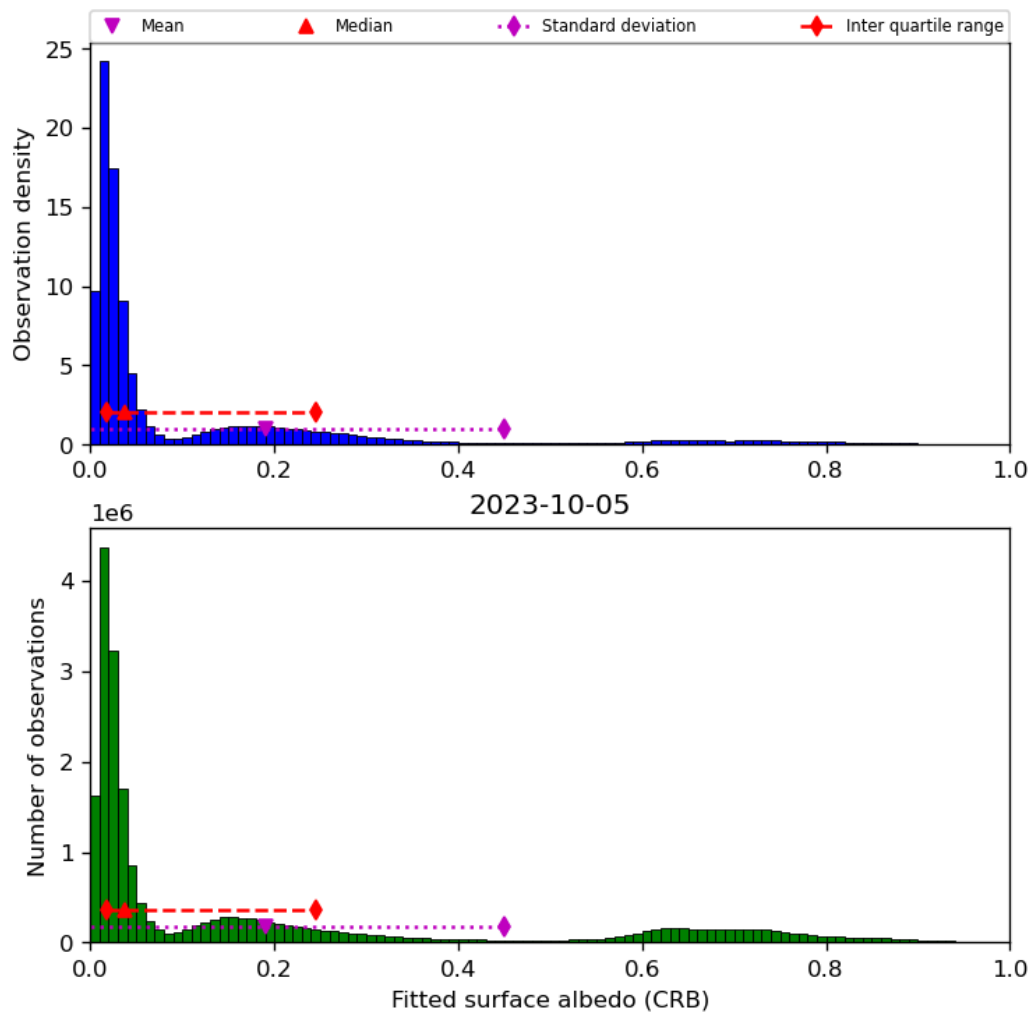
Figure 46: Histogram of “Fitted surface albedo (CRB)” for 2023-10-04 to 2023-10-06
