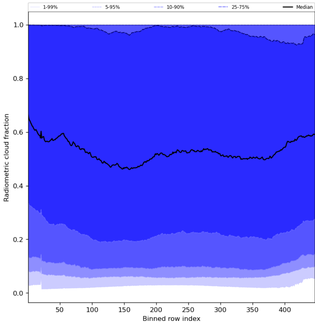
Figure 55: Along track statistics of “Radiometric cloud fraction” for 2023-10-04 to 2023-10-06
