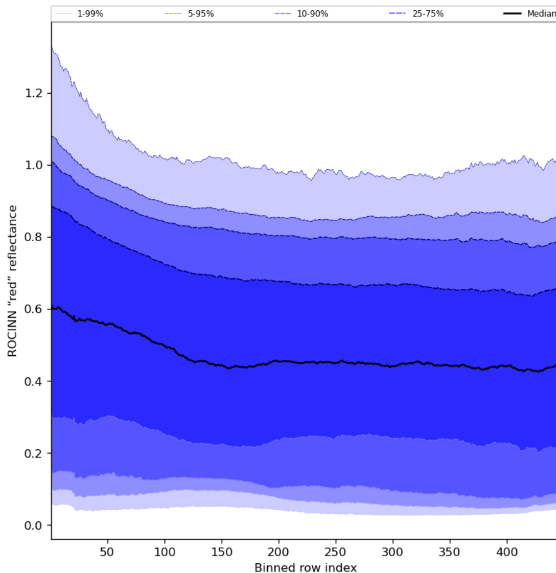
Figure 69: Along track statistics of “ROCINN “red” reflectance” for 2023-10-04 to 2023-10-06
