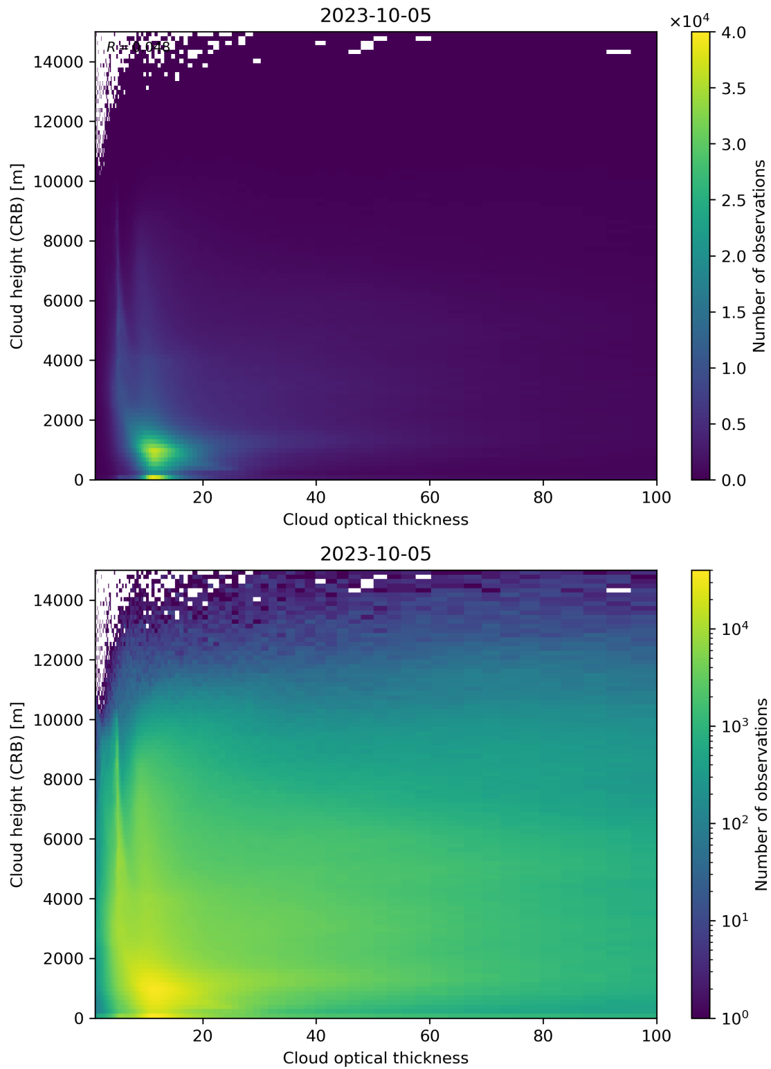
Figure 85: Scatter density plot of “Cloud optical thickness” against “Cloud height (CRB)” for 2023-10-04 to 2023-10-06.
