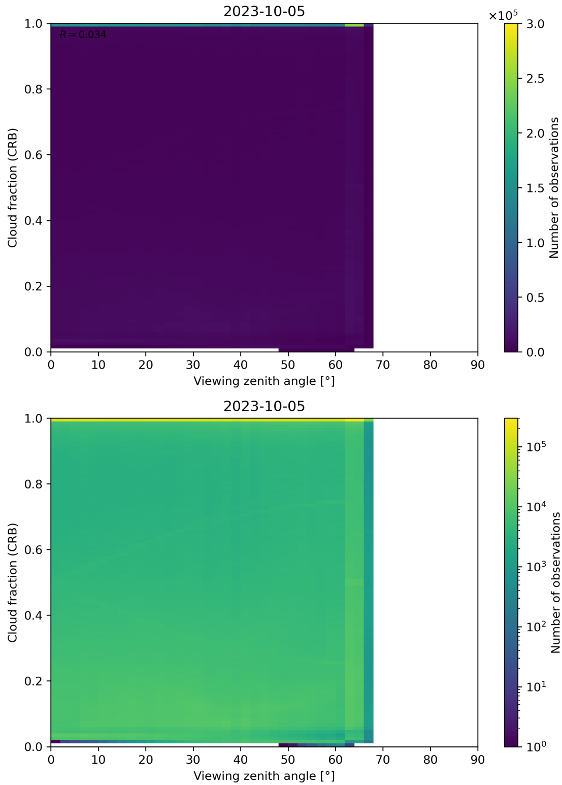
Figure 109: Scatter density plot of “Viewing zenith angle” against “Cloud fraction (CRB)” for 2023-10-04 to 2023-10-06.
