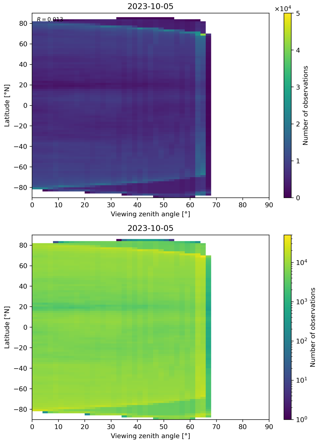
Figure 113: Scatter density plot of “Viewing zenith angle” against “Latitude” for 2023-10-04 to 2023-10-06.
