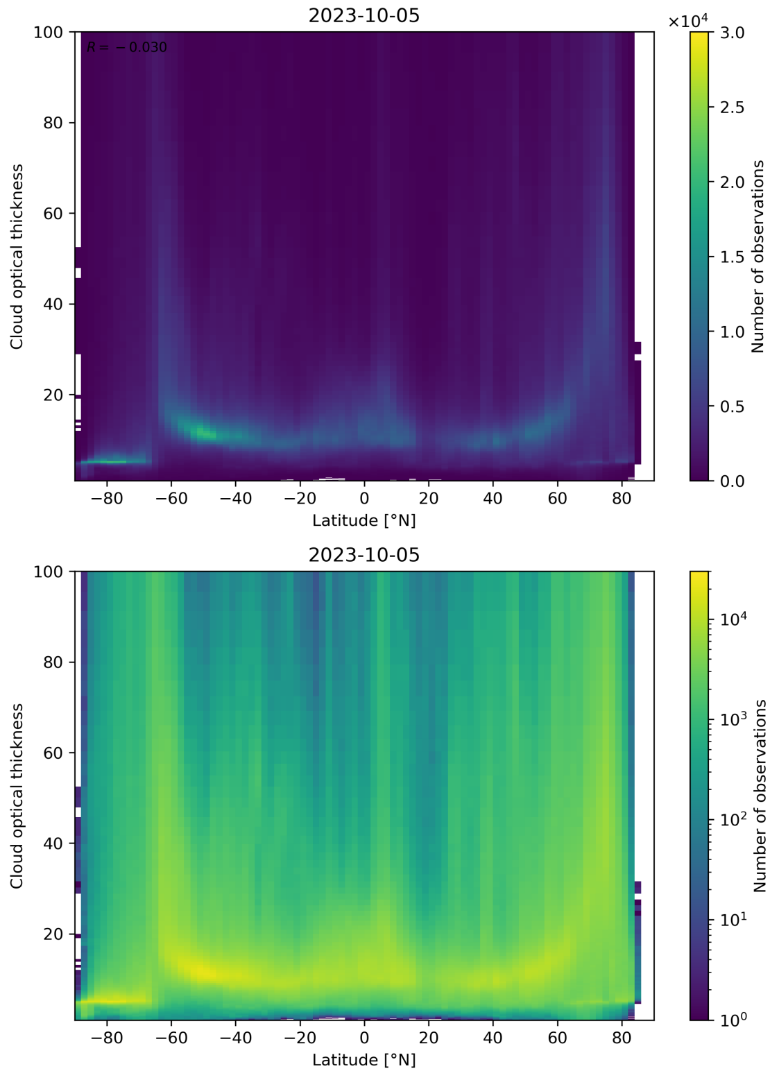
Figure 96: Scatter density plot of “Latitude” against “Cloud optical thickness” for 2023-10-04 to 2023-10-06.
