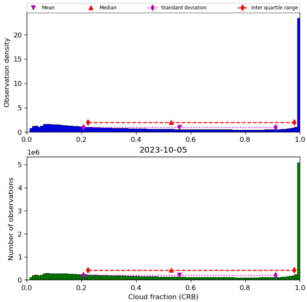
Figure 42: Histogram of “Cloud fraction (CRB)” for 2023-10-04 to 2023-10-06
