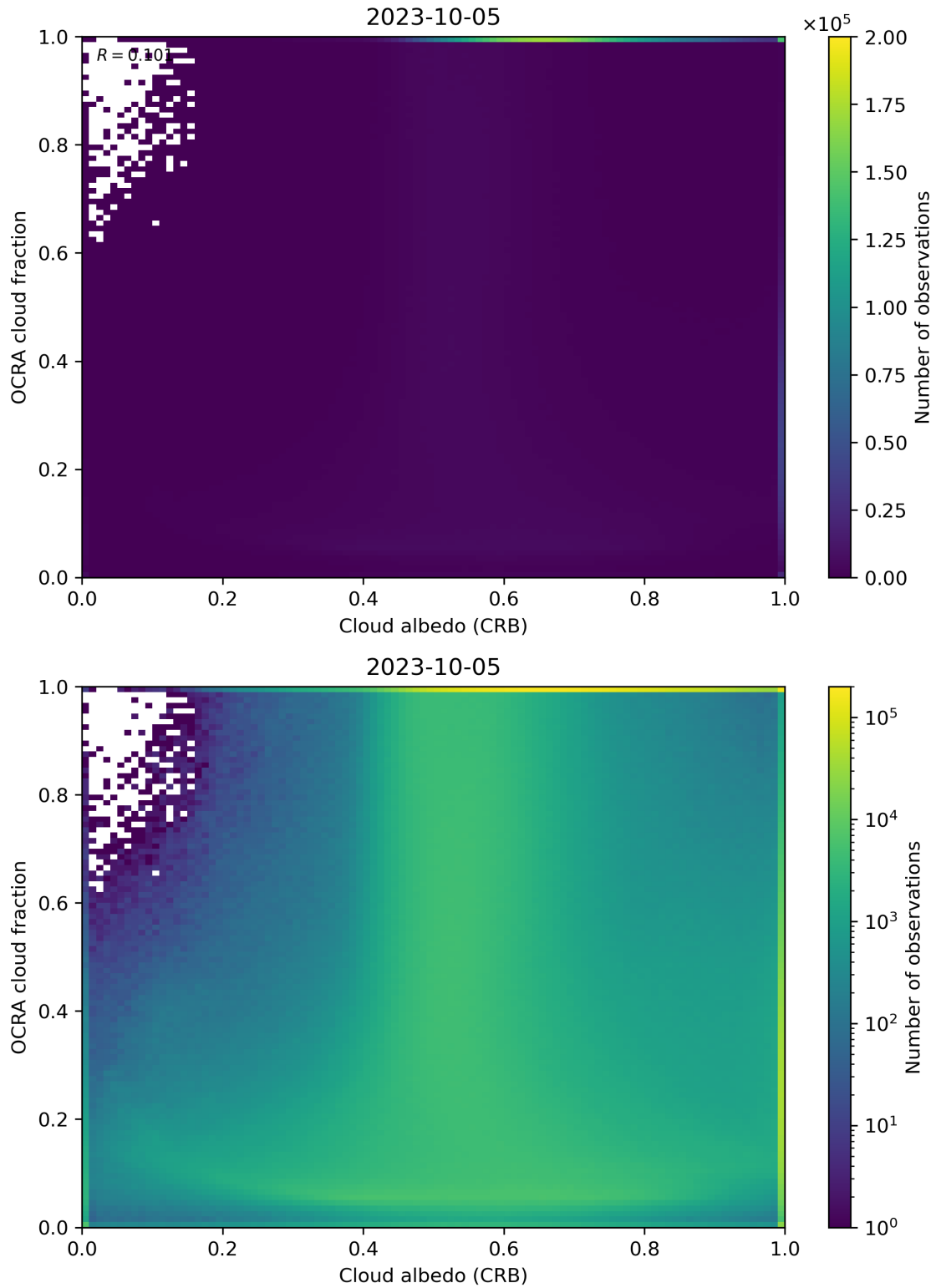
Figure 70: Scatter density plot of “Cloud albedo (CRB)” against “OCRA cloud fraction” for 2023-10-04 to 2023-10-06.
