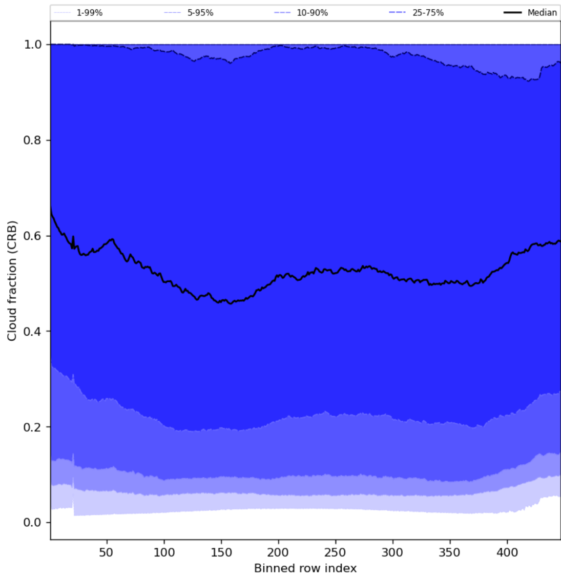
Figure 58: Along track statistics of “Cloud fraction (CRB)” for 2023-10-04 to 2023-10-06
