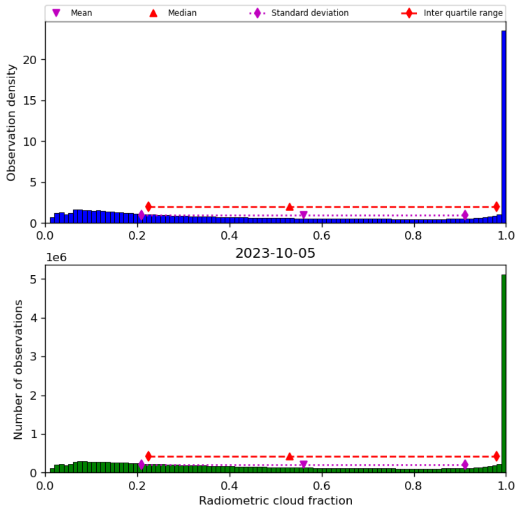
Figure 39: Histogram of “Radiometric cloud fraction” for 2023-10-04 to 2023-10-06
