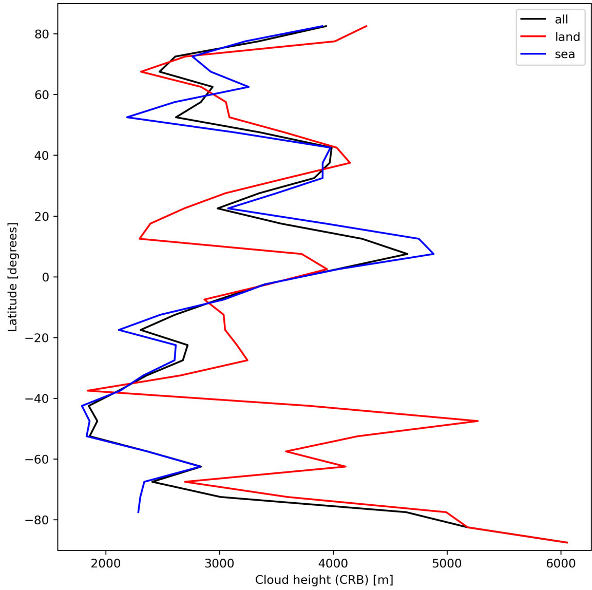
Figure 27: Zonal average of “Cloud height (CRB)” for 2023-10-04 to 2023-10-06.
