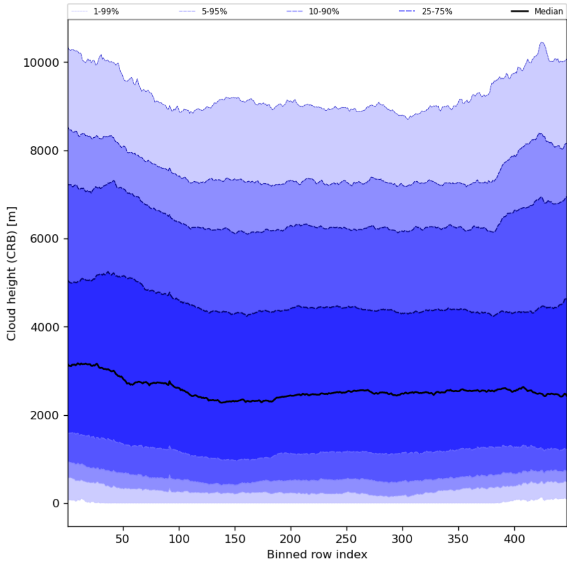
Figure 59: Along track statistics of “Cloud height (CRB)” for 2023-10-04 to 2023-10-06
