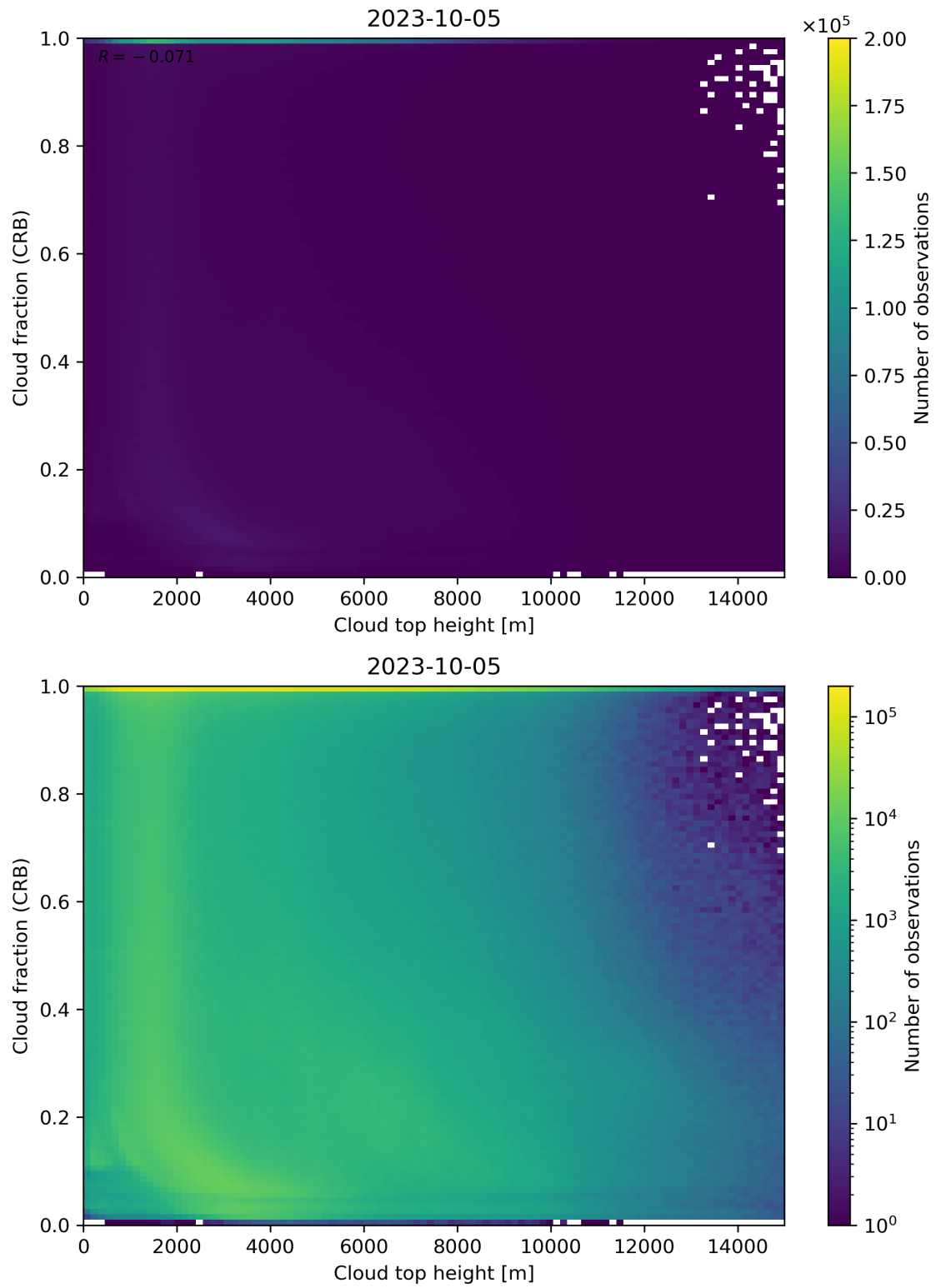
Figure 88: Scatter density plot of “Cloud top height” against “Cloud fraction (CRB)” for 2023-10-04 to 2023-10-06.
