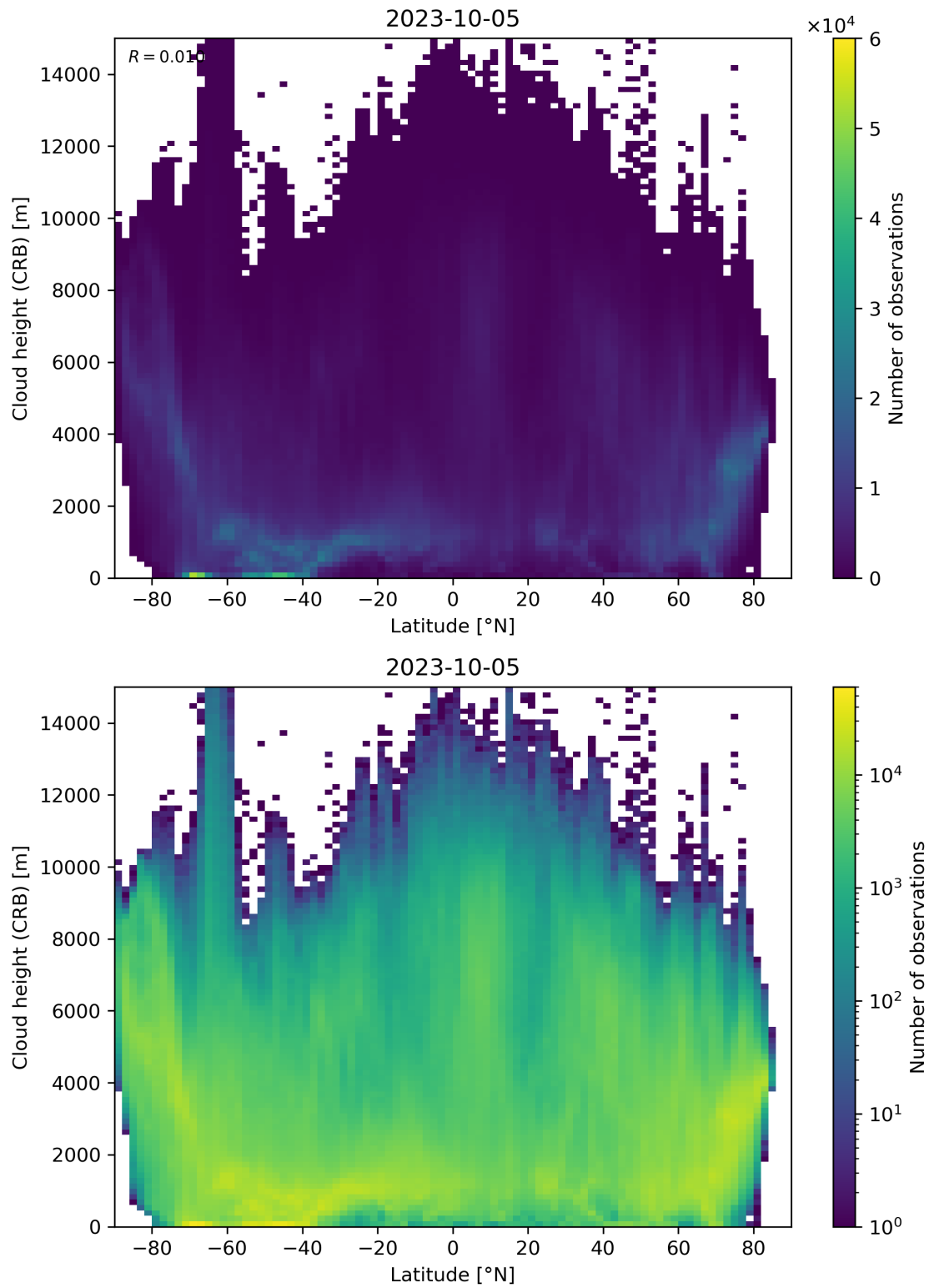
Figure 95: Scatter density plot of “Latitude” against “Cloud height (CRB)” for 2023-10-04 to 2023-10-06.
