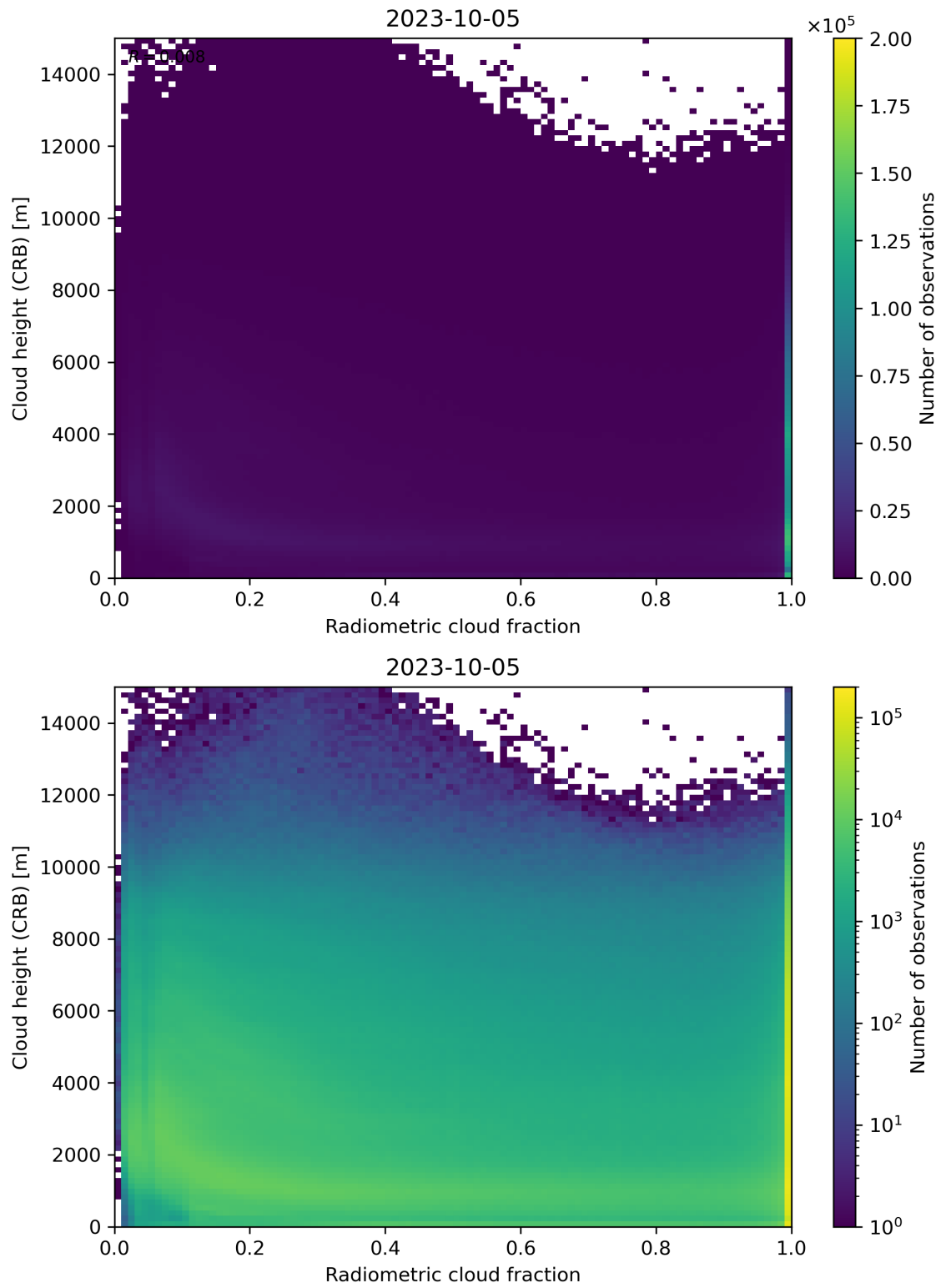
Figure 74: Scatter density plot of “Radiometric cloud fraction” against “Cloud height (CRB)” for 2023-10-04 to 2023-10-06.
