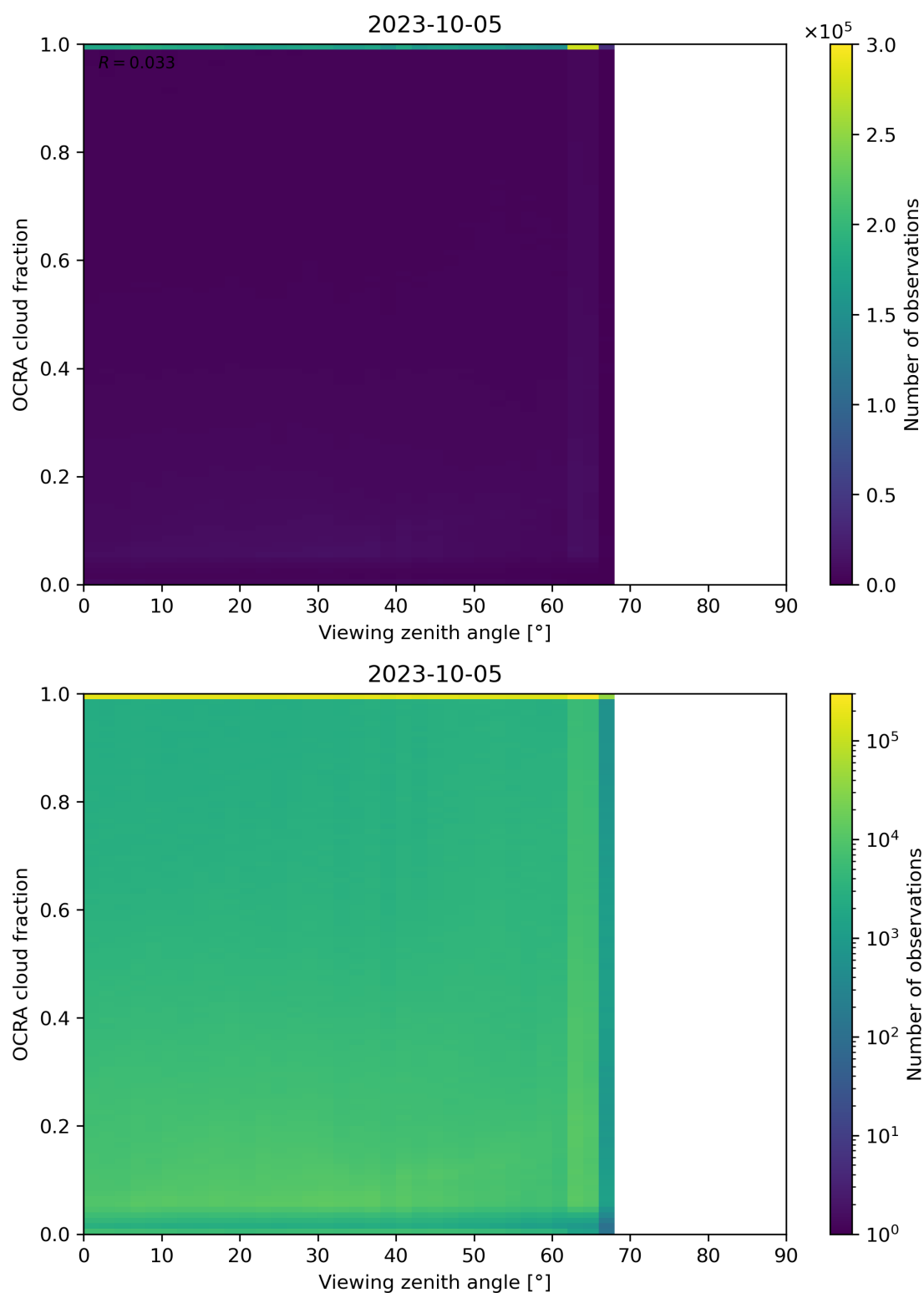
Figure 108: Scatter density plot of “Viewing zenith angle” against “OCRA cloud fraction” for 2023-10-04 to 2023-10-06.
