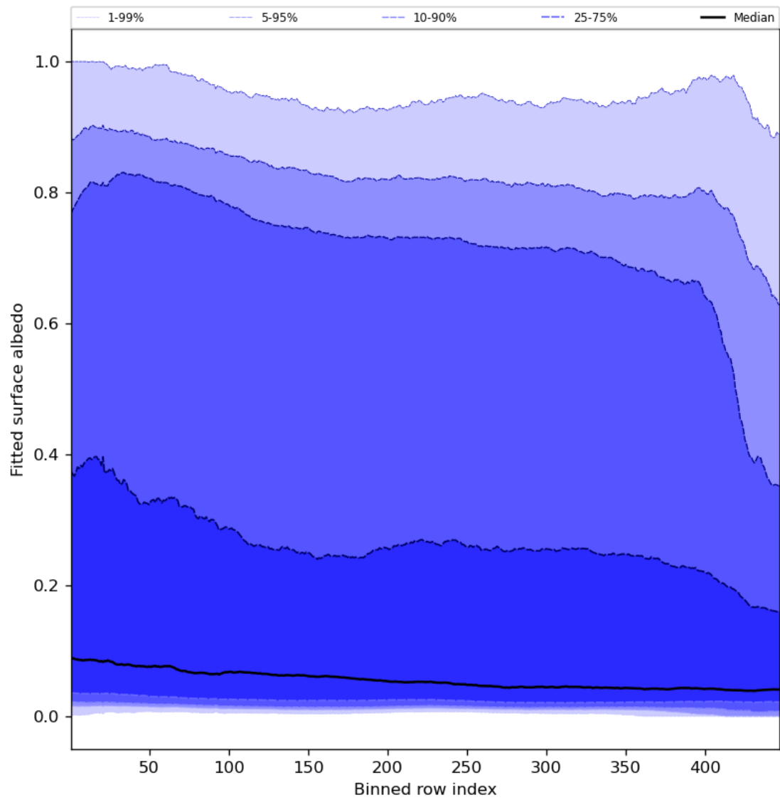
Figure 61: Along track statistics of “Fitted surface albedo” for 2023-10-04 to 2023-10-06
