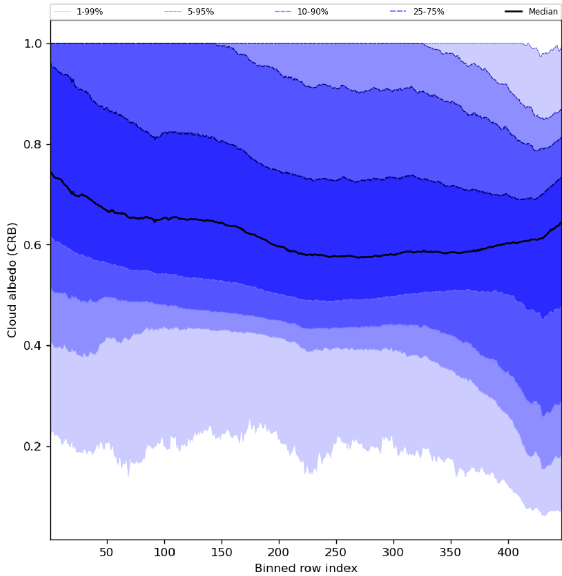
Figure 60: Along track statistics of “Cloud albedo (CRB)” for 2023-10-04 to 2023-10-06
