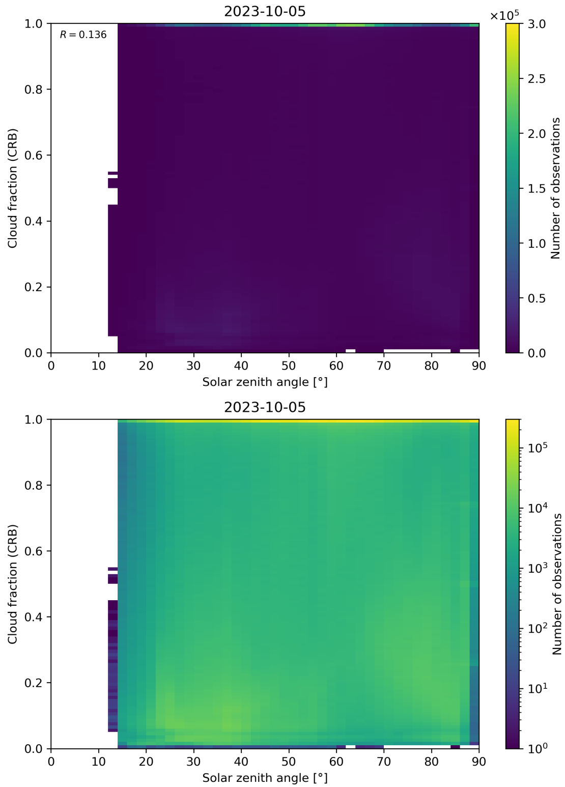
Figure 101: Scatter density plot of “Solar zenith angle” against “Cloud fraction (CRB)” for 2023-10-04 to 2023-10-06.
