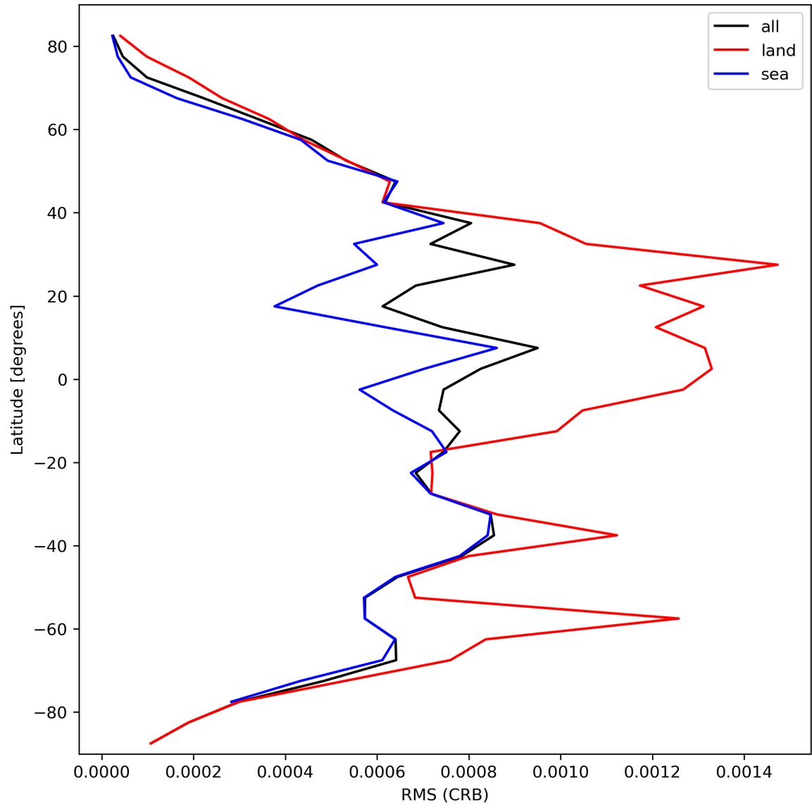
Figure 32: Zonal average of “RMS (CRB)” for 2023-10-04 to 2023-10-06.
