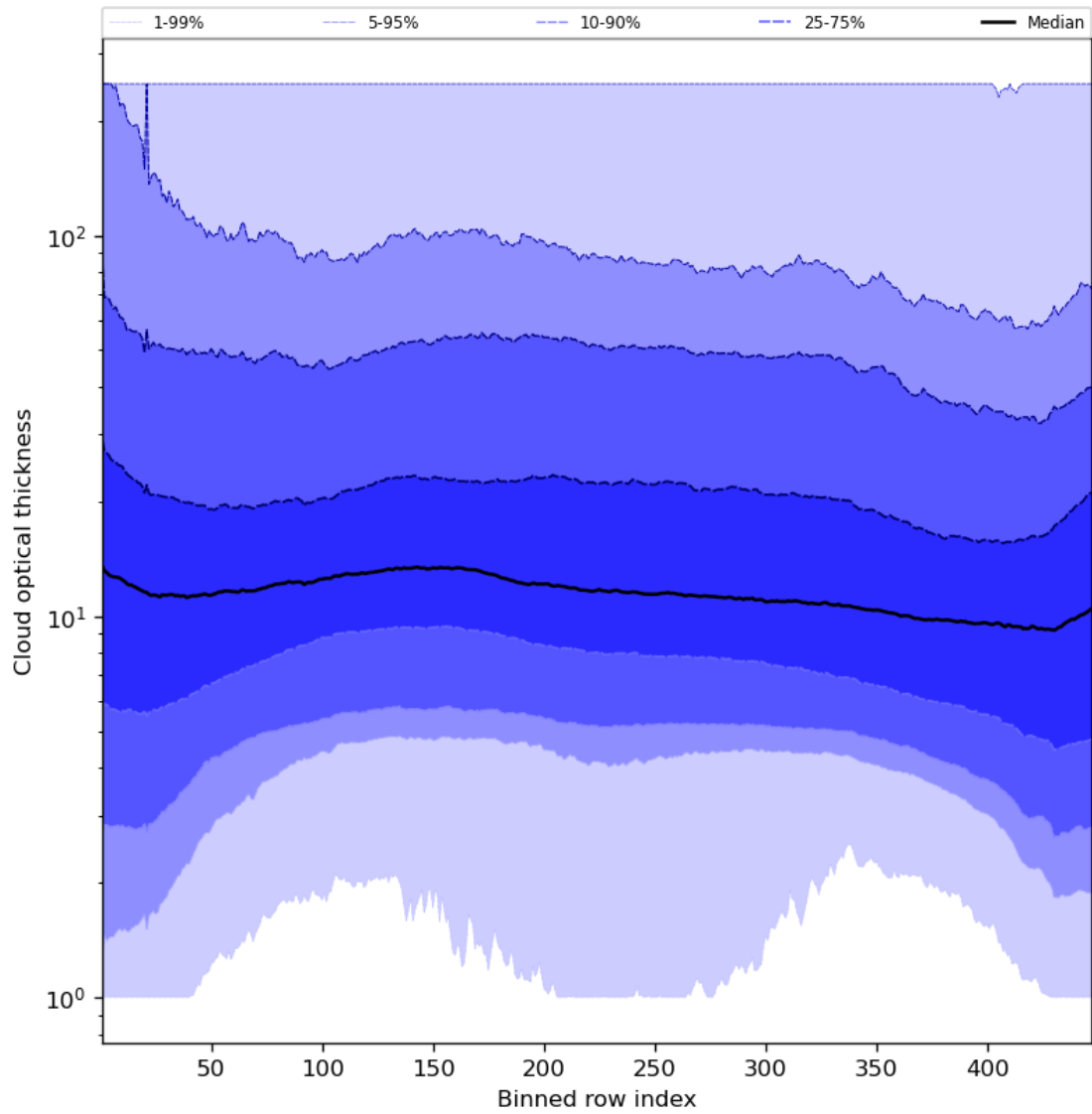
Figure 57: Along track statistics of “Cloud optical thickness” for 2023-10-04 to 2023-10-06
