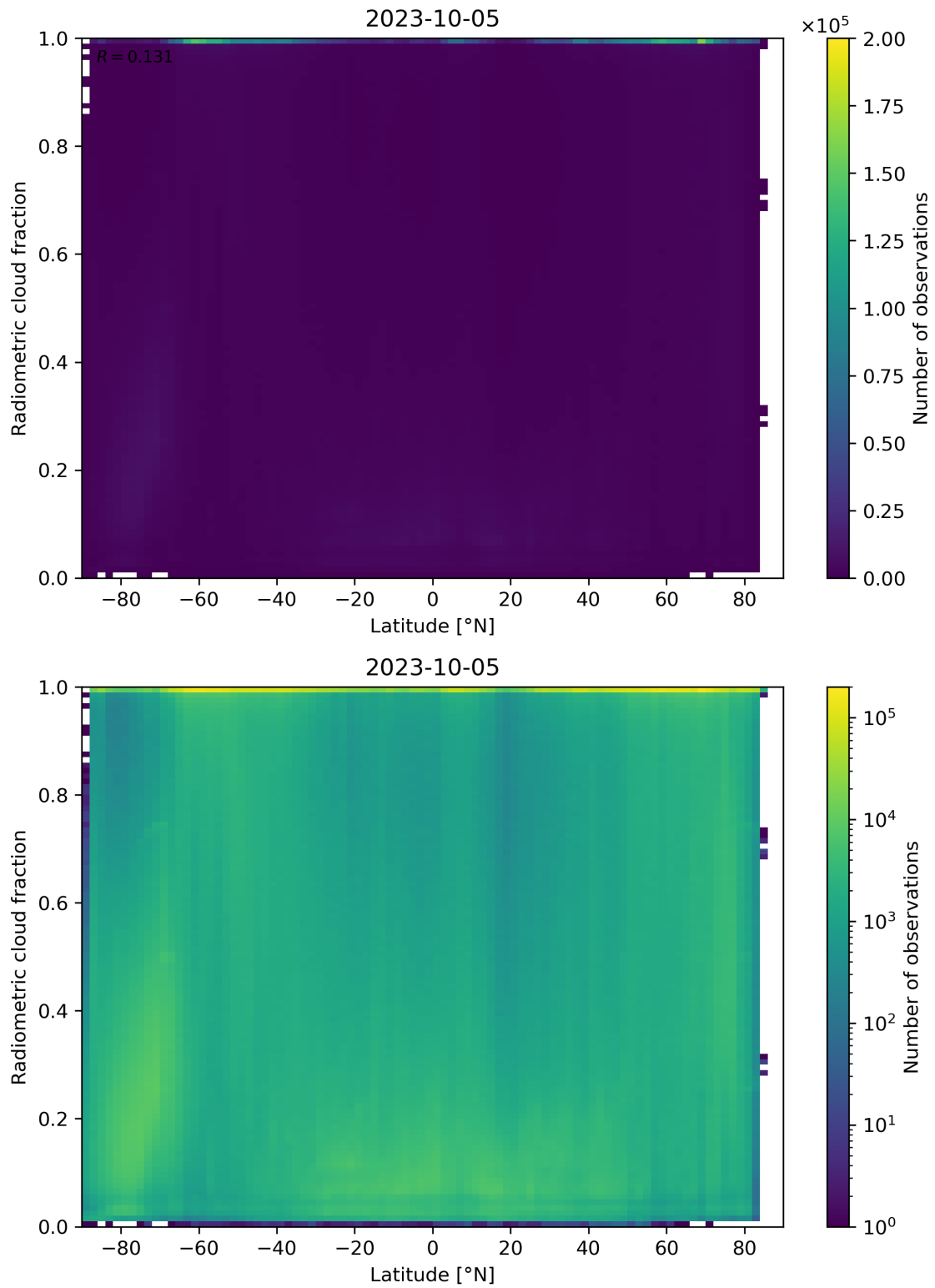
Figure 92: Scatter density plot of “Latitude” against “Radiometric cloud fraction” for 2023-10-04 to 2023-10-06.
