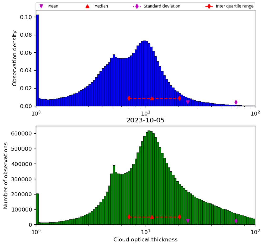
Figure 41: Histogram of “Cloud optical thickness” for 2023-10-04 to 2023-10-06
