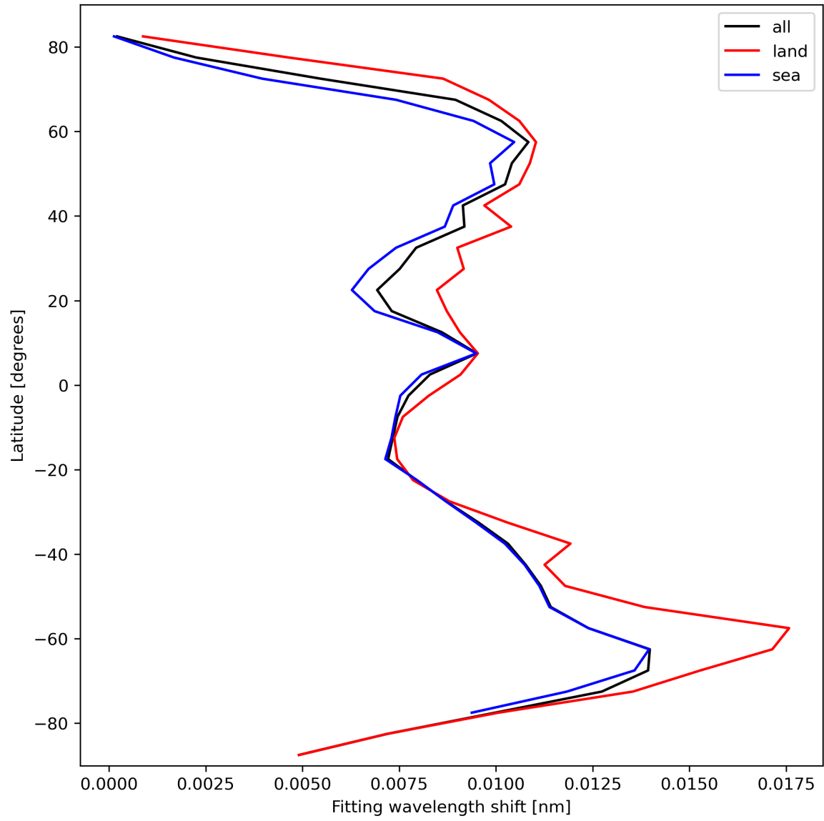
Figure 33: Zonal average of “Fitting wavelength shift” for 2023-10-04 to 2023-10-06.
