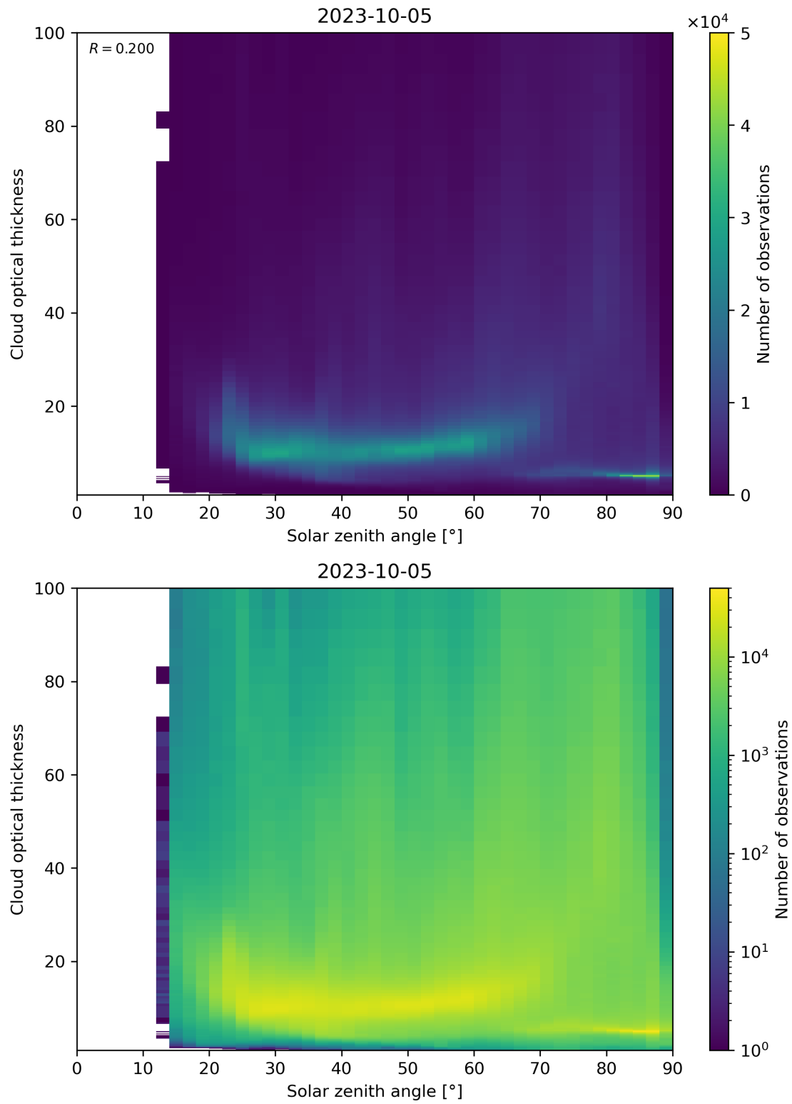
Figure 103: Scatter density plot of “Solar zenith angle” against “Cloud optical thickness” for 2023-10-04 to 2023-10-06.
