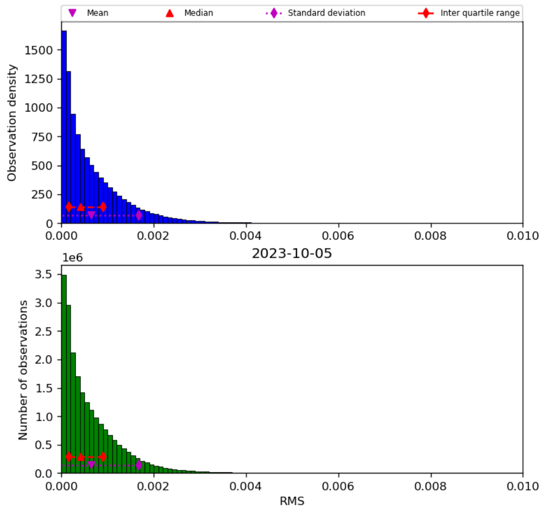
Figure 47: Histogram of “RMS” for 2023-10-04 to 2023-10-06
