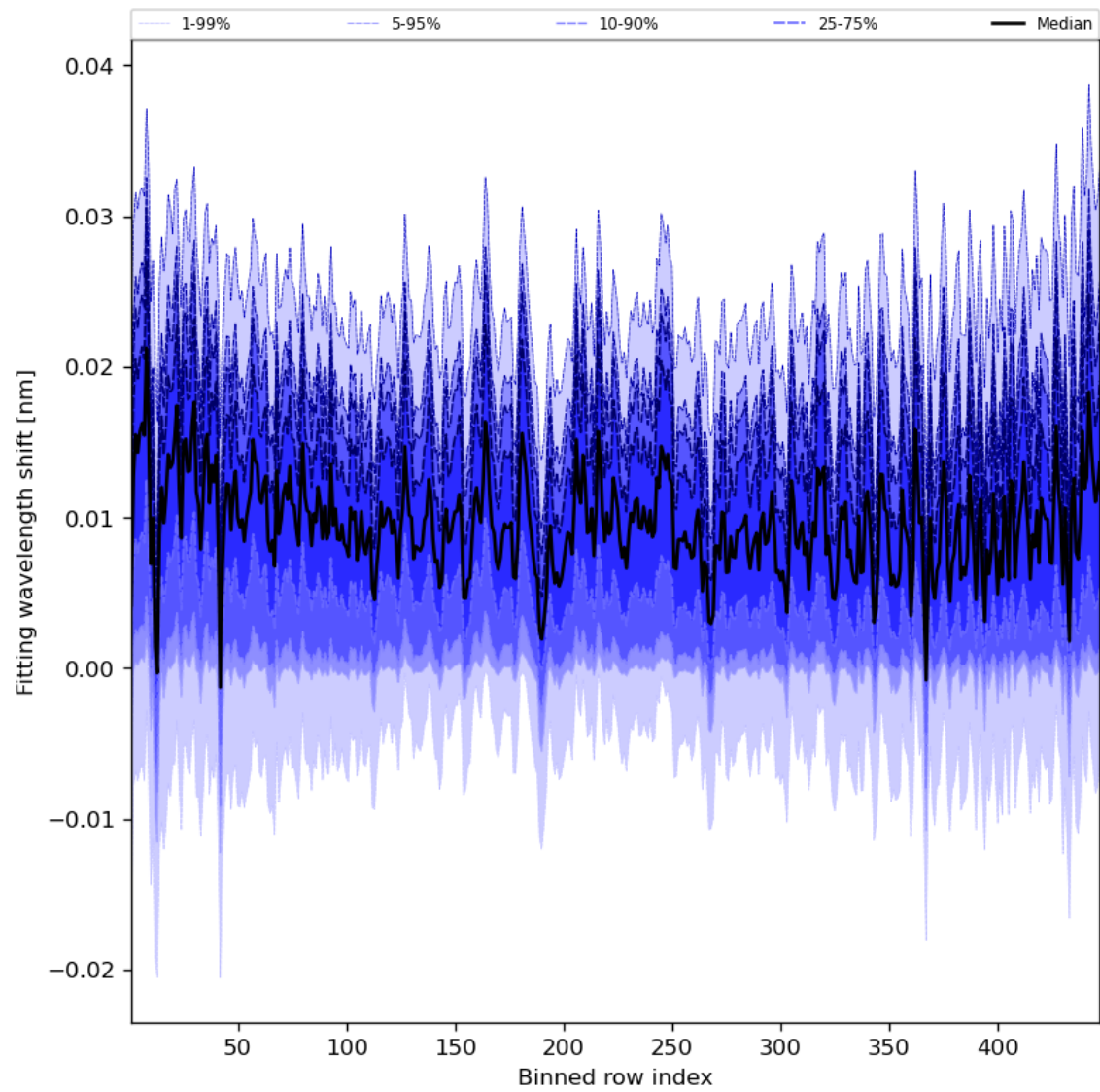
Figure 65: Along track statistics of “Fitting wavelength shift” for 2023-10-04 to 2023-10-06
