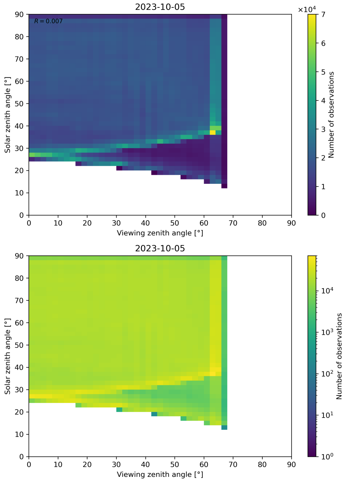
Figure 114: Scatter density plot of “Viewing zenith angle” against “Solar zenith angle” for 2023-10-04 to 2023-10-06.
