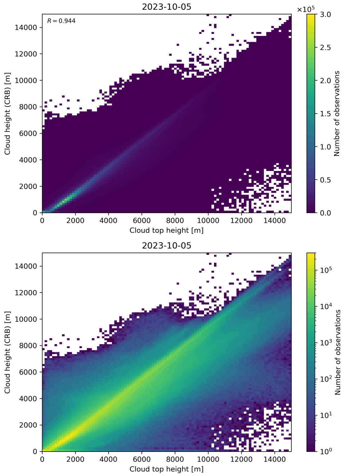
Figure 89: Scatter density plot of “Cloud top height” against “Cloud height (CRB)” for 2023-10-04 to 2023-10-06.
