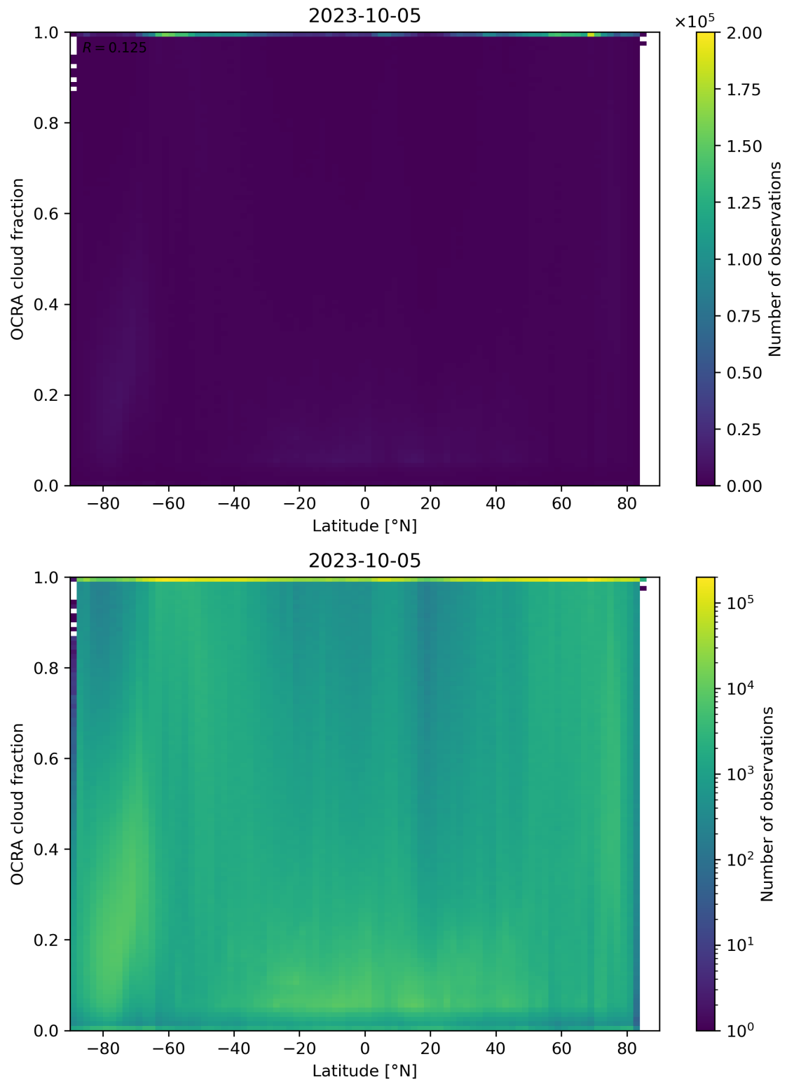
Figure 93: Scatter density plot of “Latitude” against “OCRA cloud fraction” for 2023-10-04 to 2023-10-06.
