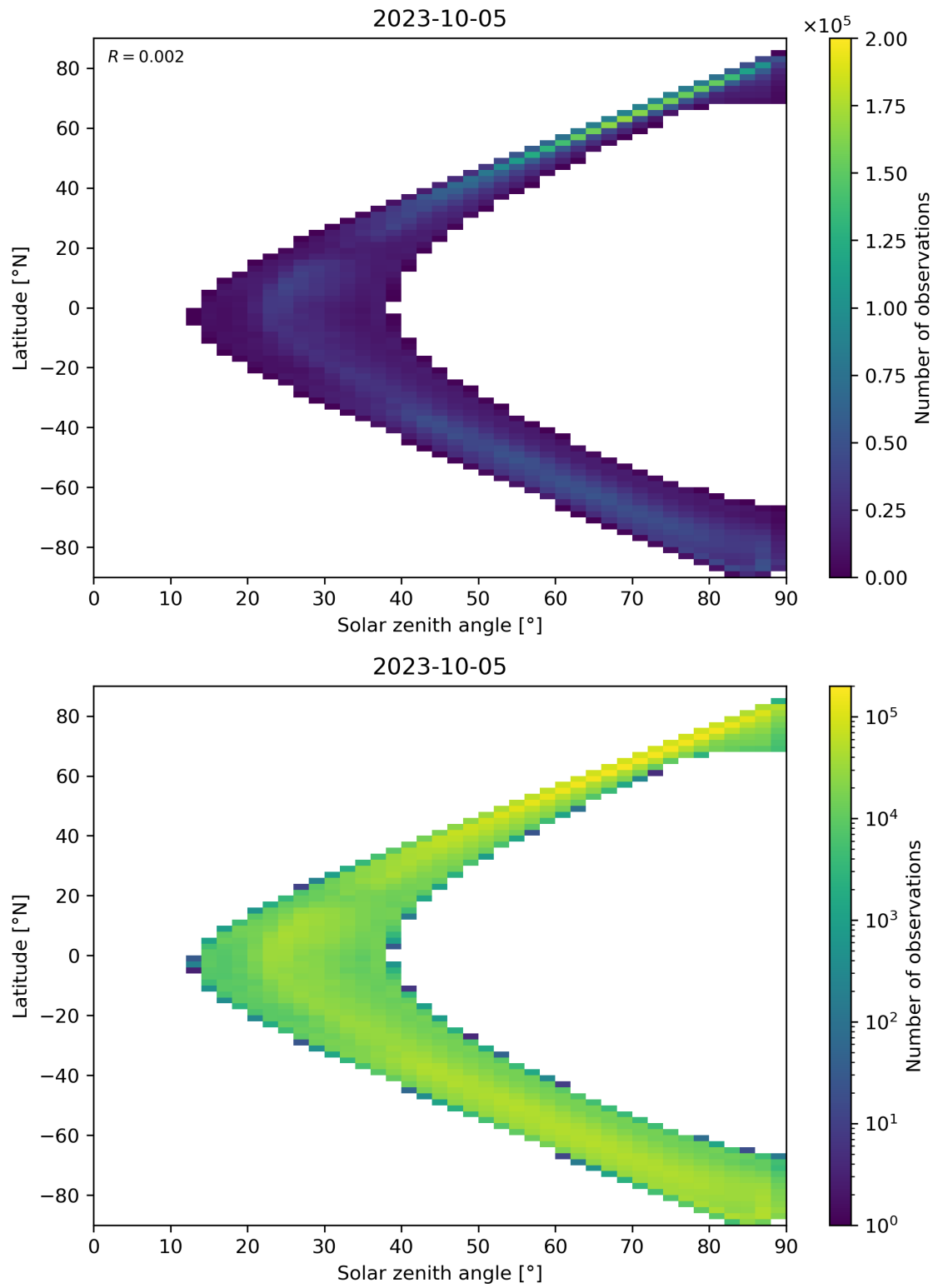
Figure 105: Scatter density plot of “Solar zenith angle” against “Latitude” for 2023-10-04 to 2023-10-06.
