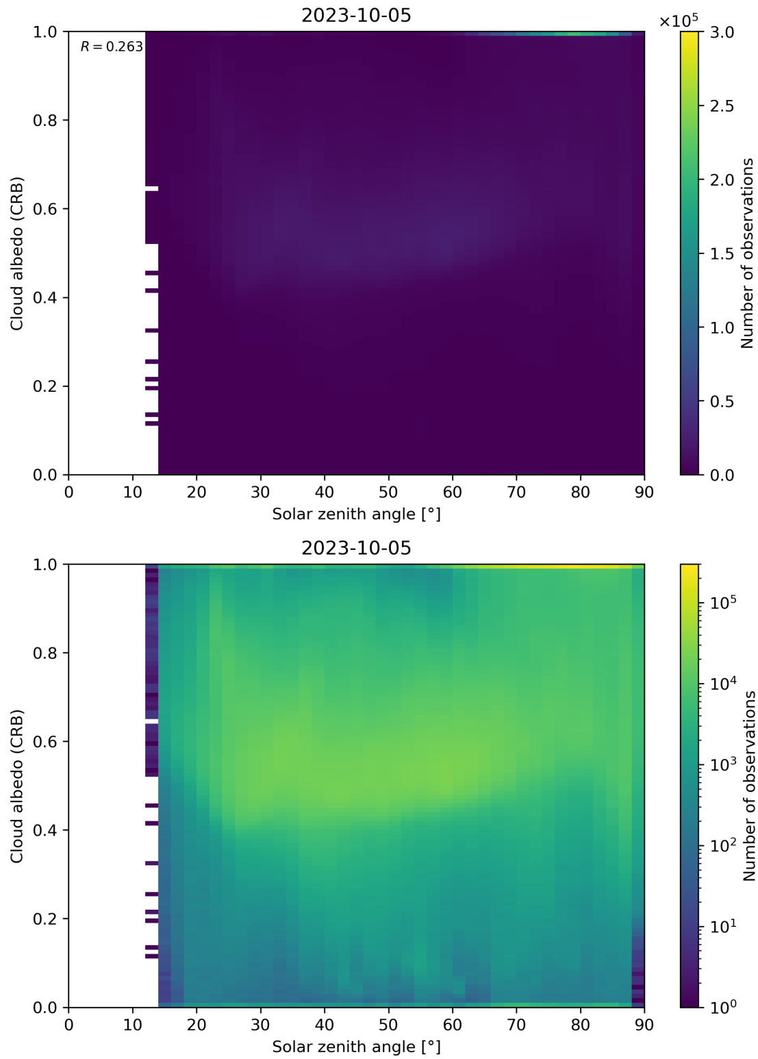
Figure 98: Scatter density plot of “Solar zenith angle” against “Cloud albedo (CRB)” for 2023-10-04 to 2023-10-06.
