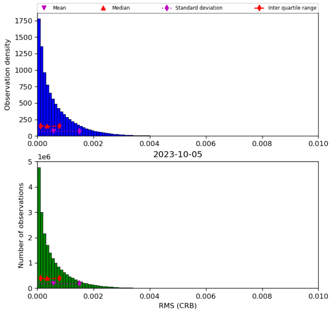
Figure 48: Histogram of “RMS (CRB)” for 2023-10-04 to 2023-10-06
