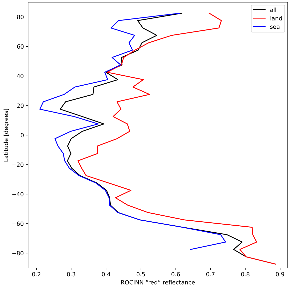
Figure 37: Zonal average of “ROCINN “red” reflectance” for 2023-10-04 to 2023-10-06.
