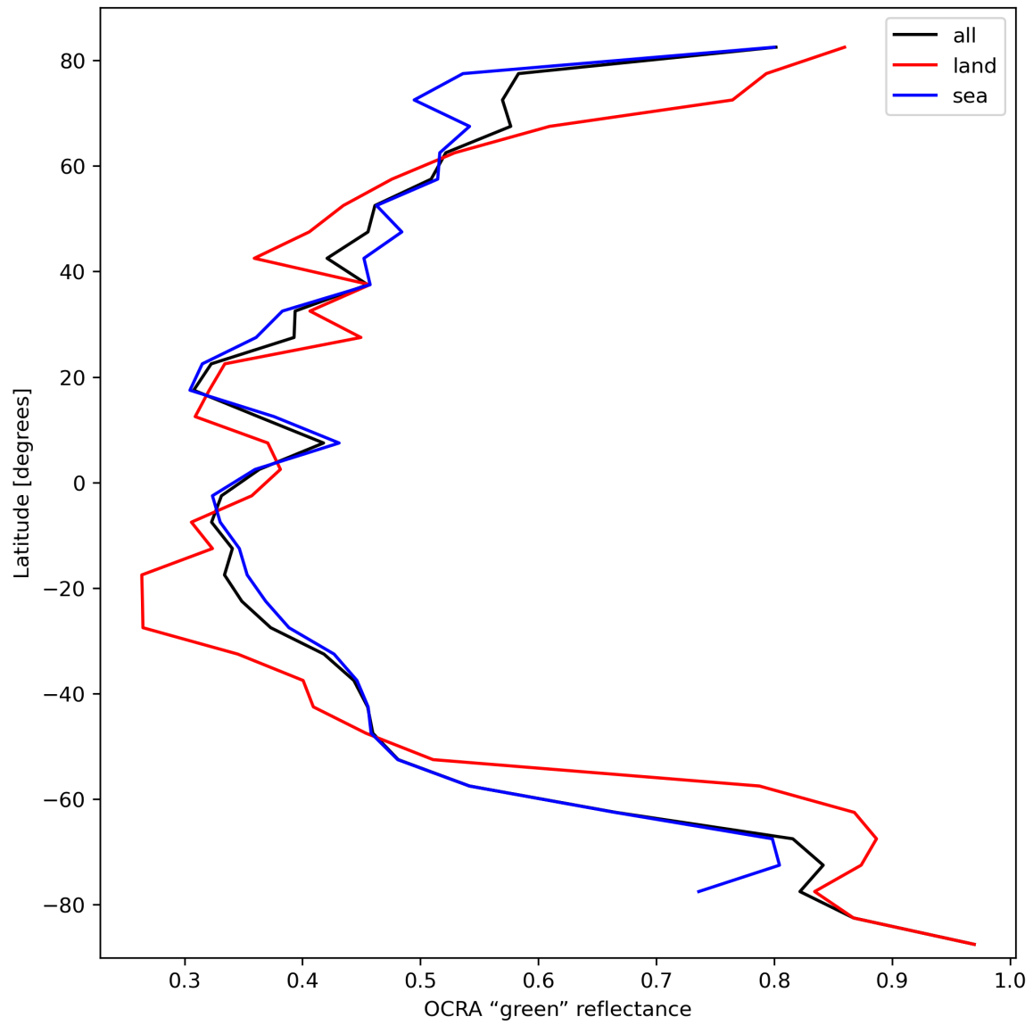
Figure 36: Zonal average of “OCRA “green” reflectance” for 2023-10-04 to 2023-10-06.
