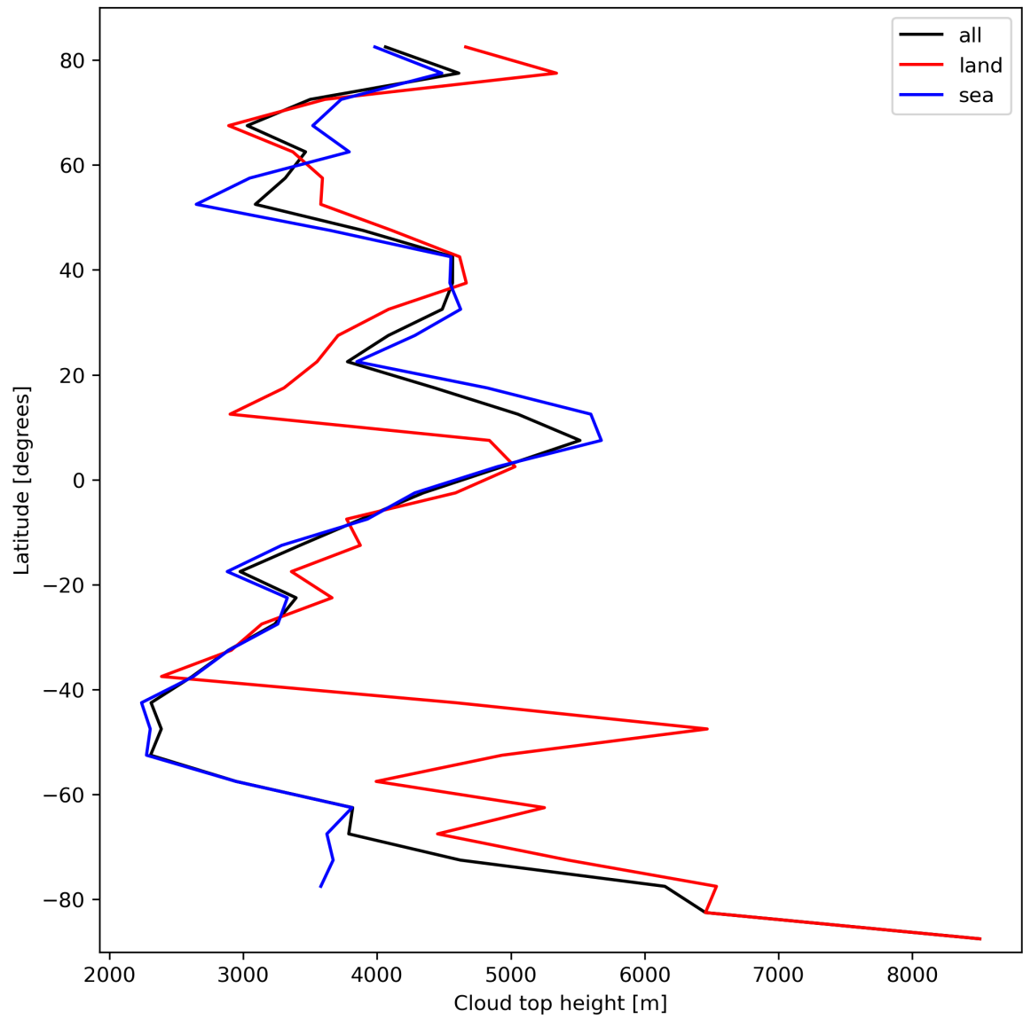
Figure 24: Zonal average of “Cloud top height” for 2023-10-04 to 2023-10-06.
