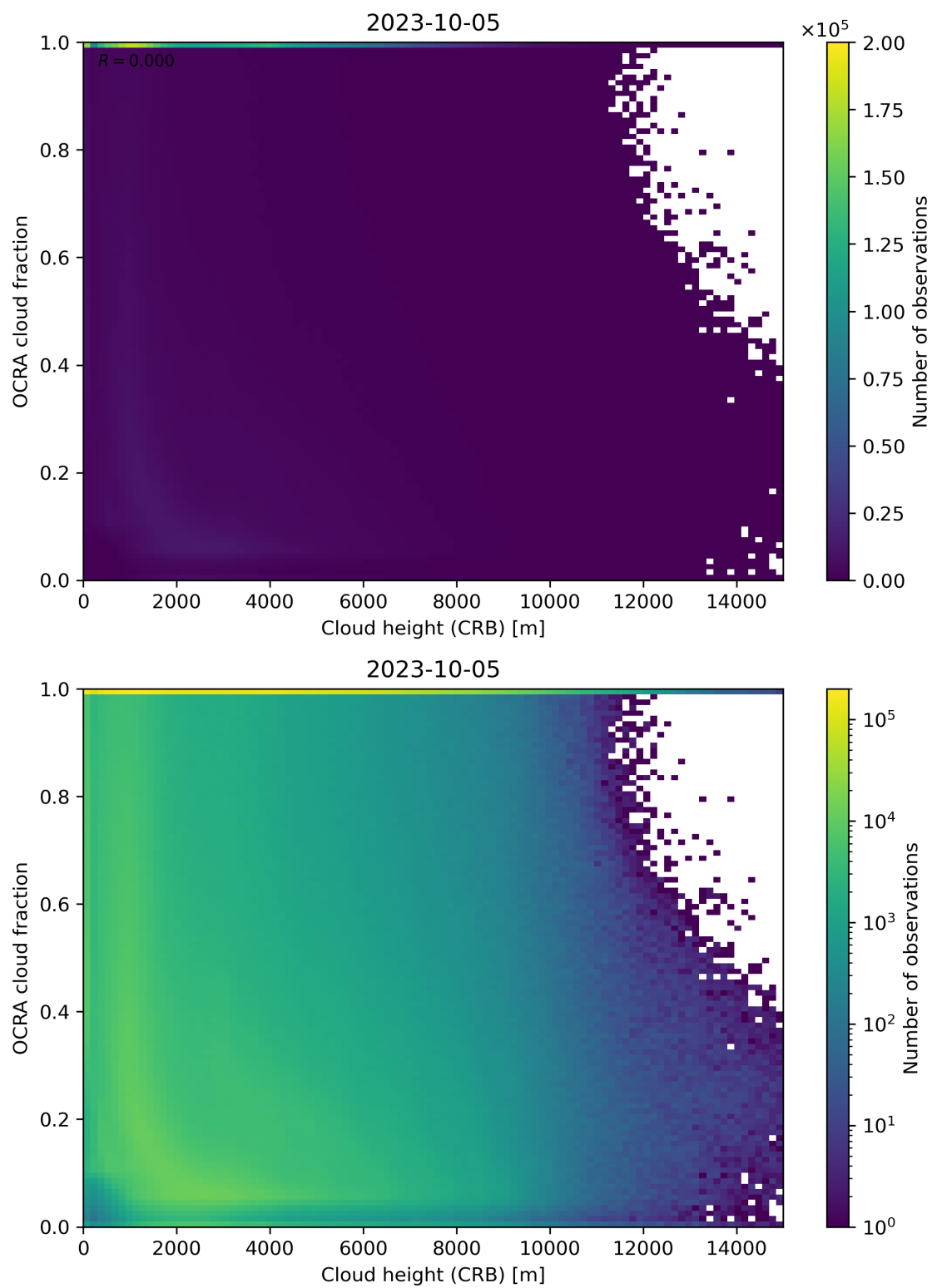
Figure 81: Scatter density plot of “Cloud height (CRB)” against “OCRA cloud fraction” for 2023-10-04 to 2023-10-06.
