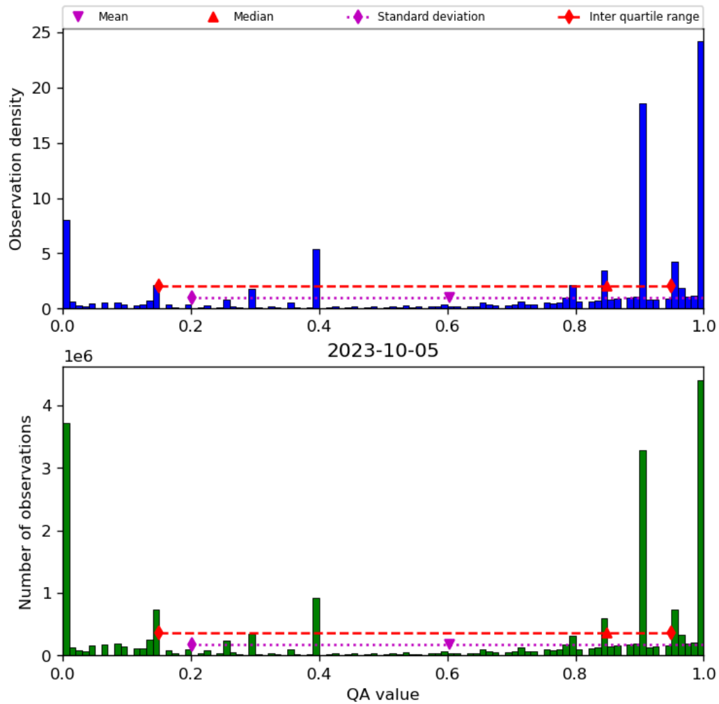
Figure 38: Histogram of “QA value” for 2023-10-04 to 2023-10-06
