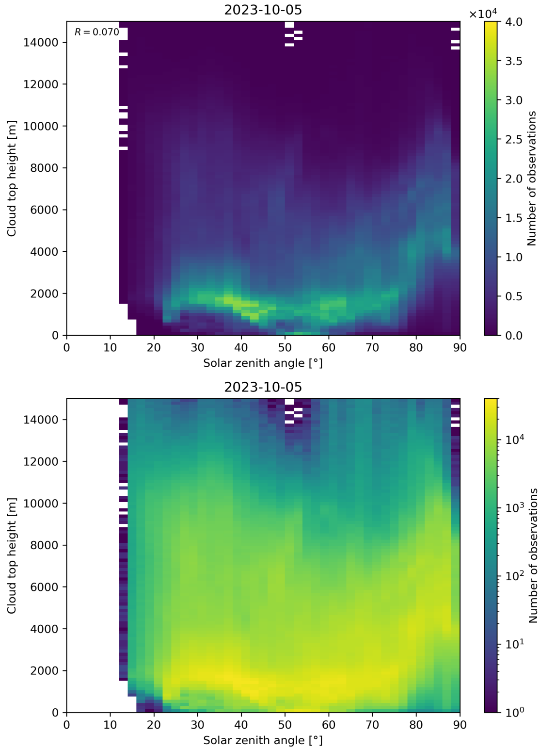
Figure 104: Scatter density plot of “Solar zenith angle” against “Cloud top height” for 2023-10-04 to 2023-10-06.
