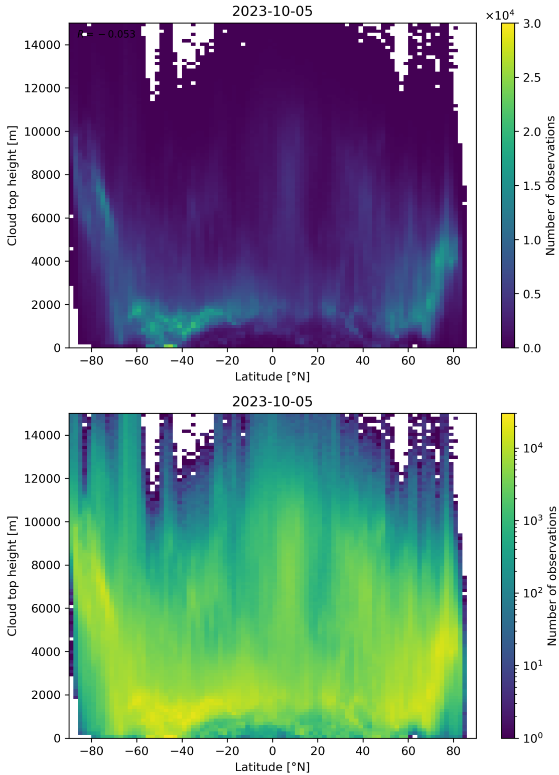
Figure 97: Scatter density plot of “Latitude” against “Cloud top height” for 2023-10-04 to 2023-10-06.
