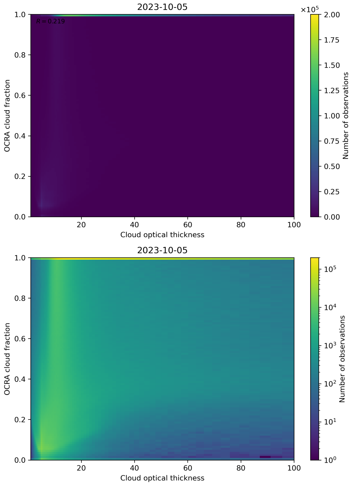
Figure 83: Scatter density plot of “Cloud optical thickness” against “OCRA cloud fraction” for 2023-10-04 to 2023-10-06.
