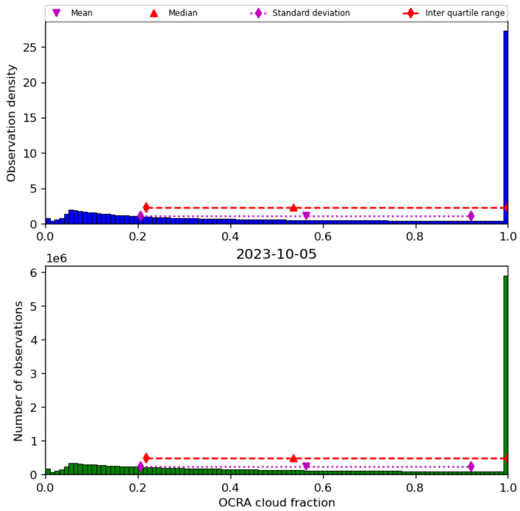
Figure 50: Histogram of “OCRA cloud fraction” for 2023-10-04 to 2023-10-06
