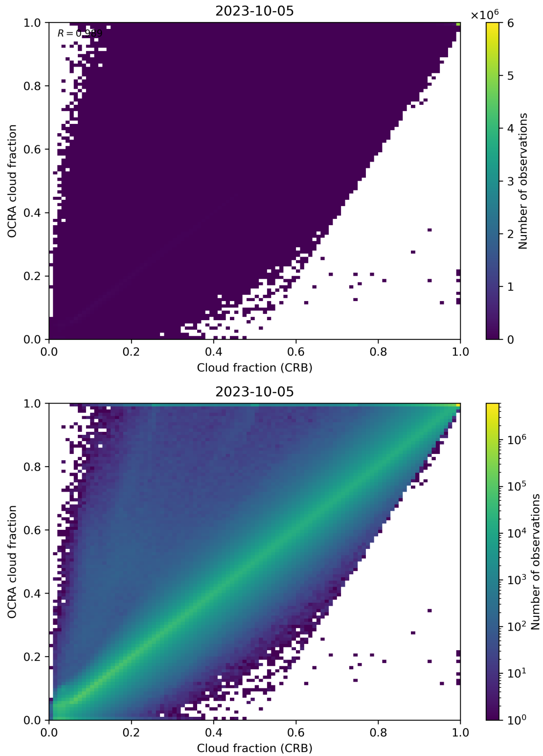
Figure 78: Scatter density plot of “Cloud fraction (CRB)” against “OCRA cloud fraction” for 2023-10-04 to 2023-10-06.
