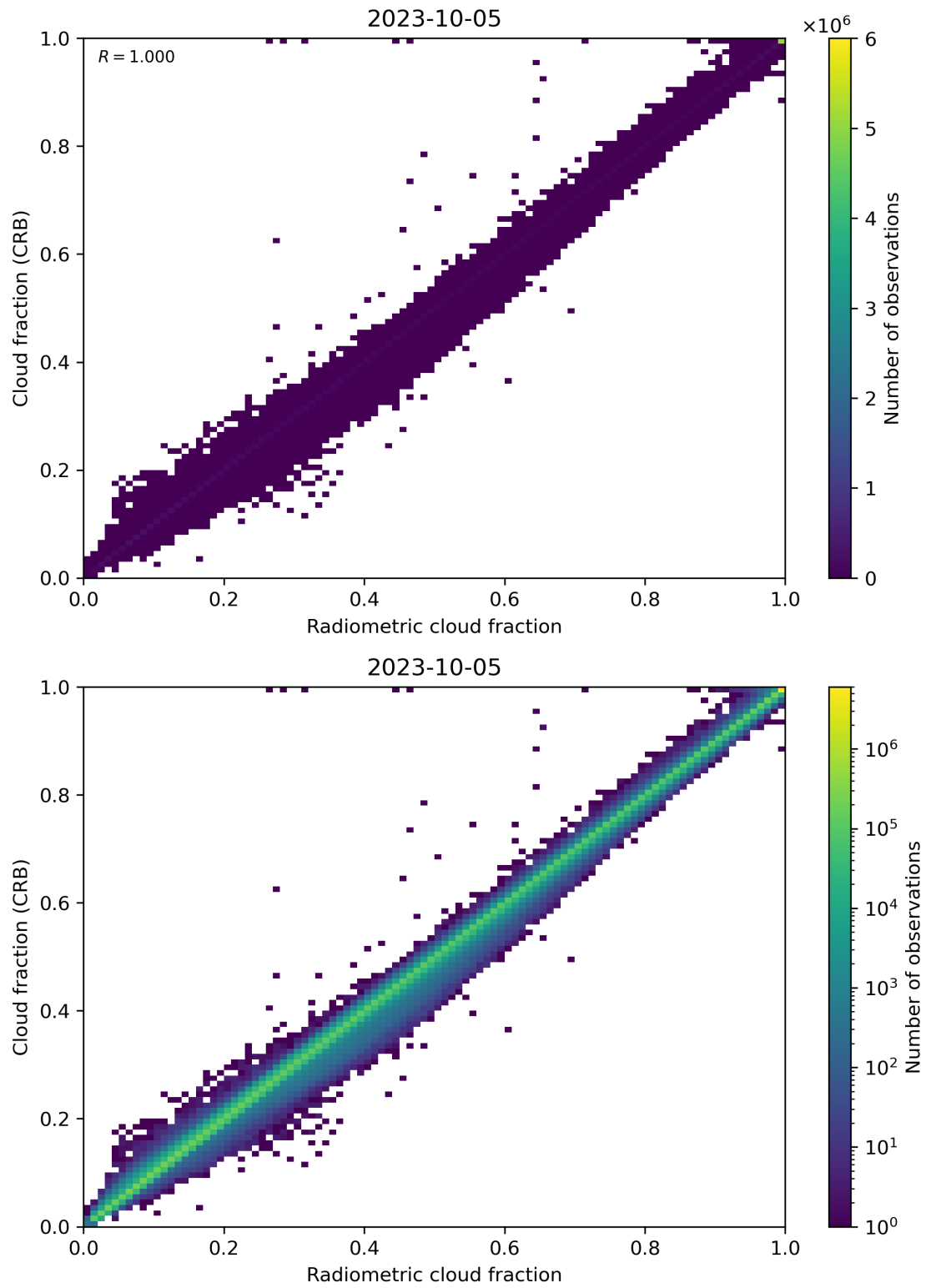
Figure 73: Scatter density plot of “Radiometric cloud fraction” against “Cloud fraction (CRB)” for 2023-10-04 to 2023-10-06.
