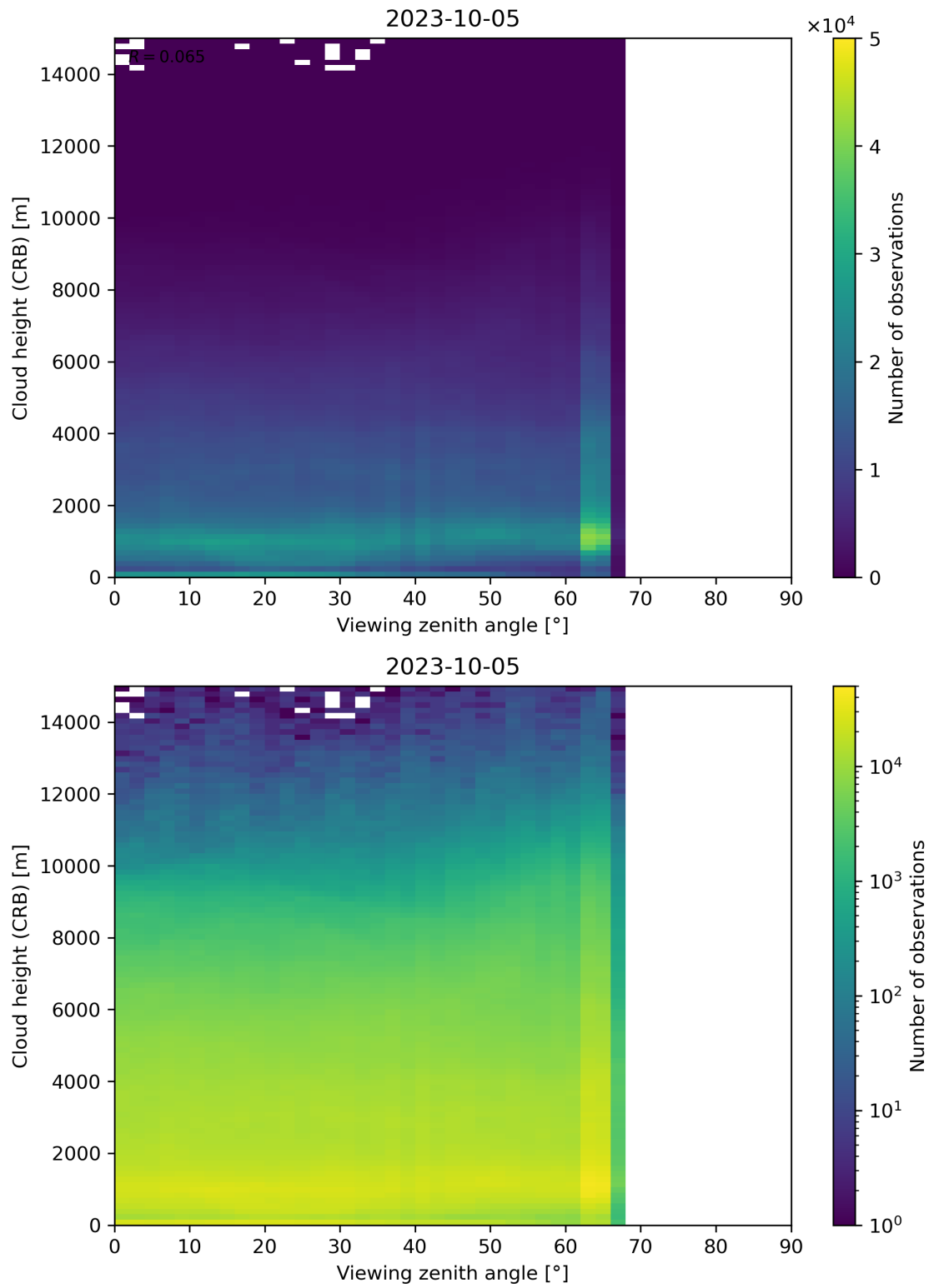
Figure 110: Scatter density plot of “Viewing zenith angle” against “Cloud height (CRB)” for 2023-10-04 to 2023-10-06.
