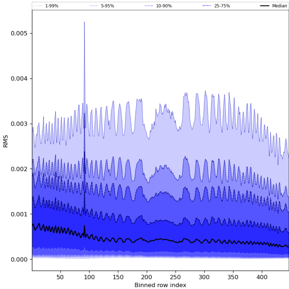
Figure 63: Along track statistics of “RMS” for 2023-10-04 to 2023-10-06
