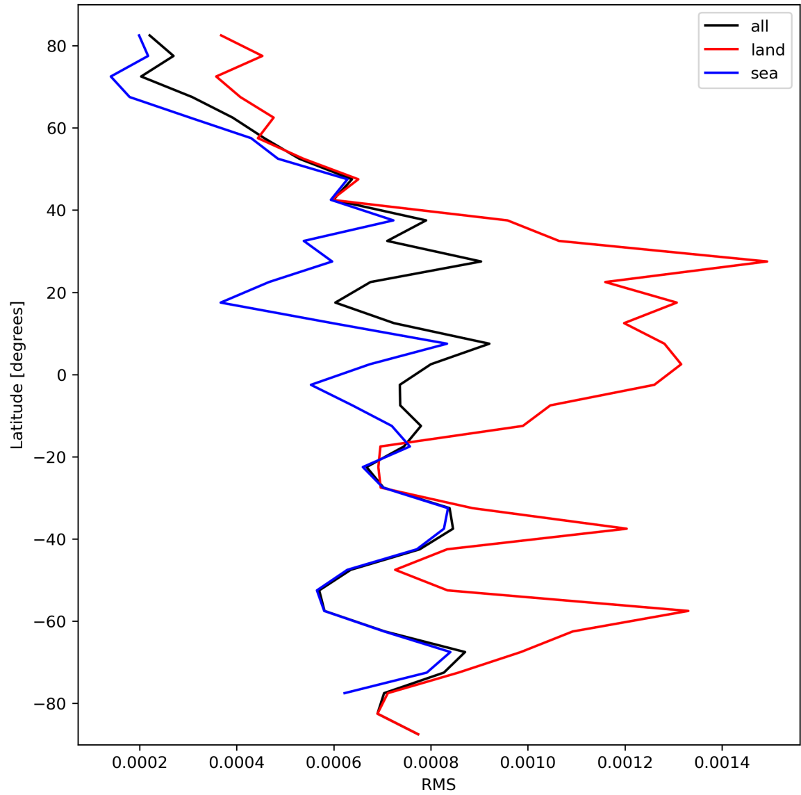
Figure 31: Zonal average of “RMS” for 2023-10-04 to 2023-10-06.
