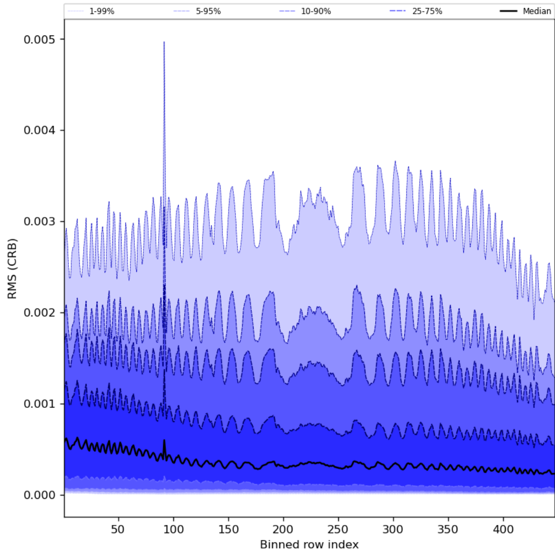
Figure 64: Along track statistics of "RMS (CRB)" for 2023-10-04 to 2023-10-06
