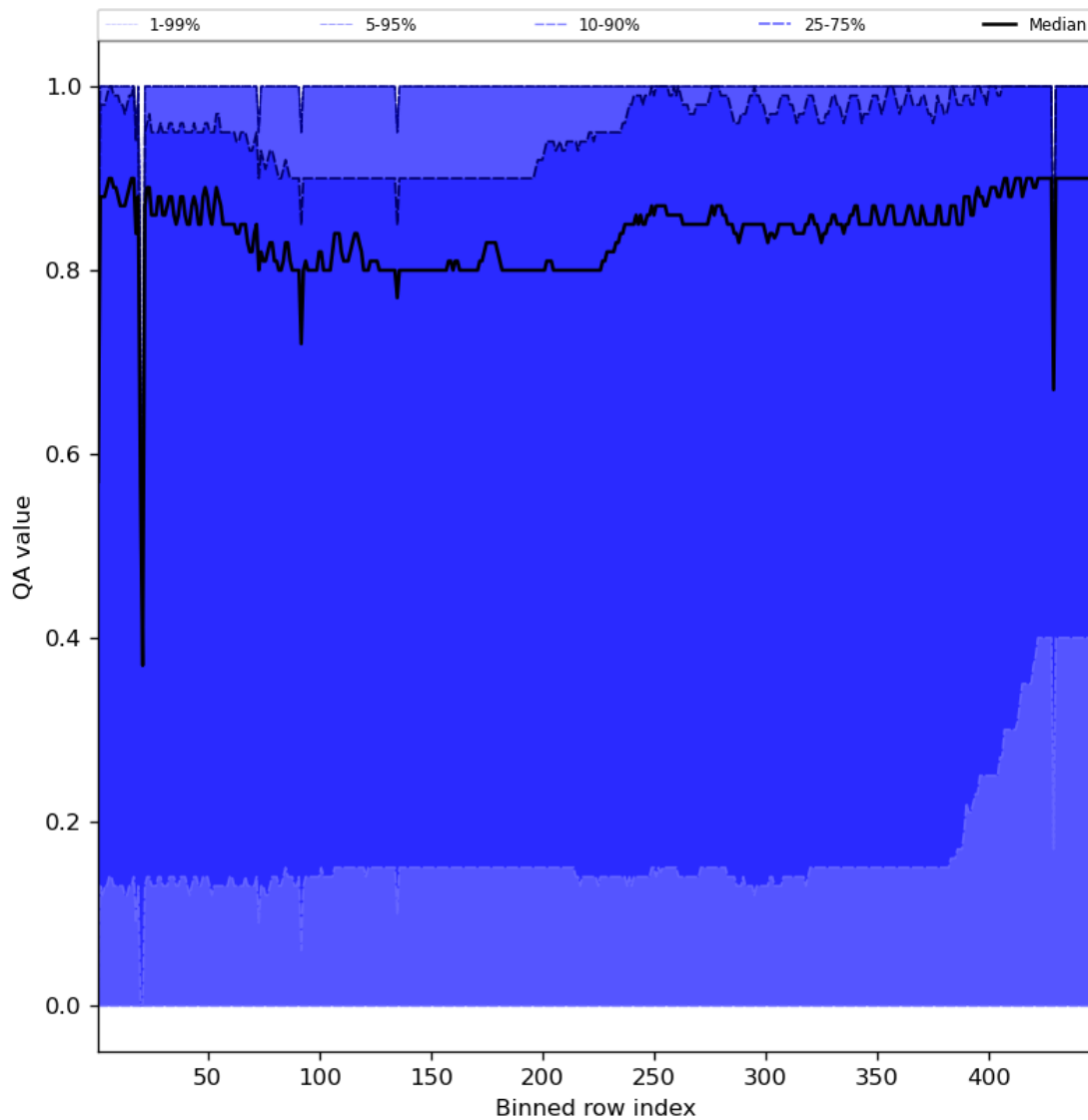
Figure 54: Along track statistics of “QA value” for 2023-10-04 to 2023-10-06
