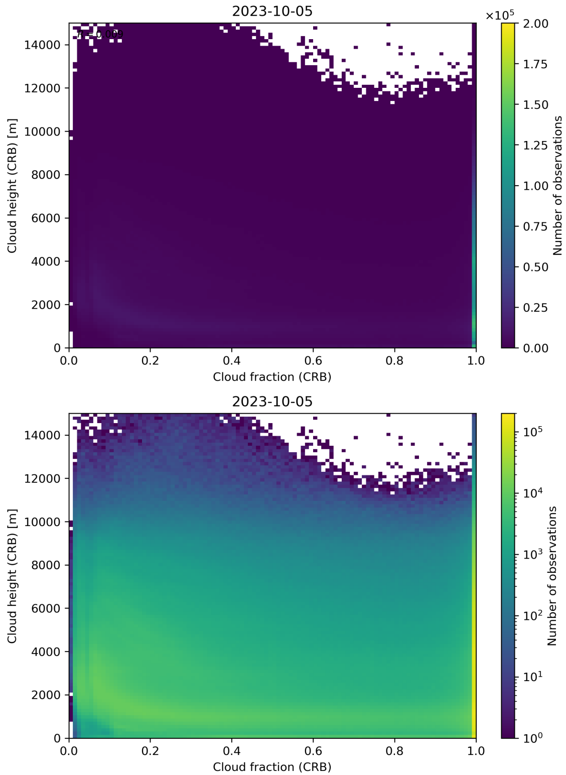
Figure 79: Scatter density plot of “Cloud fraction (CRB)” against “Cloud height (CRB)” for 2023-10-04 to 2023-10-06.
