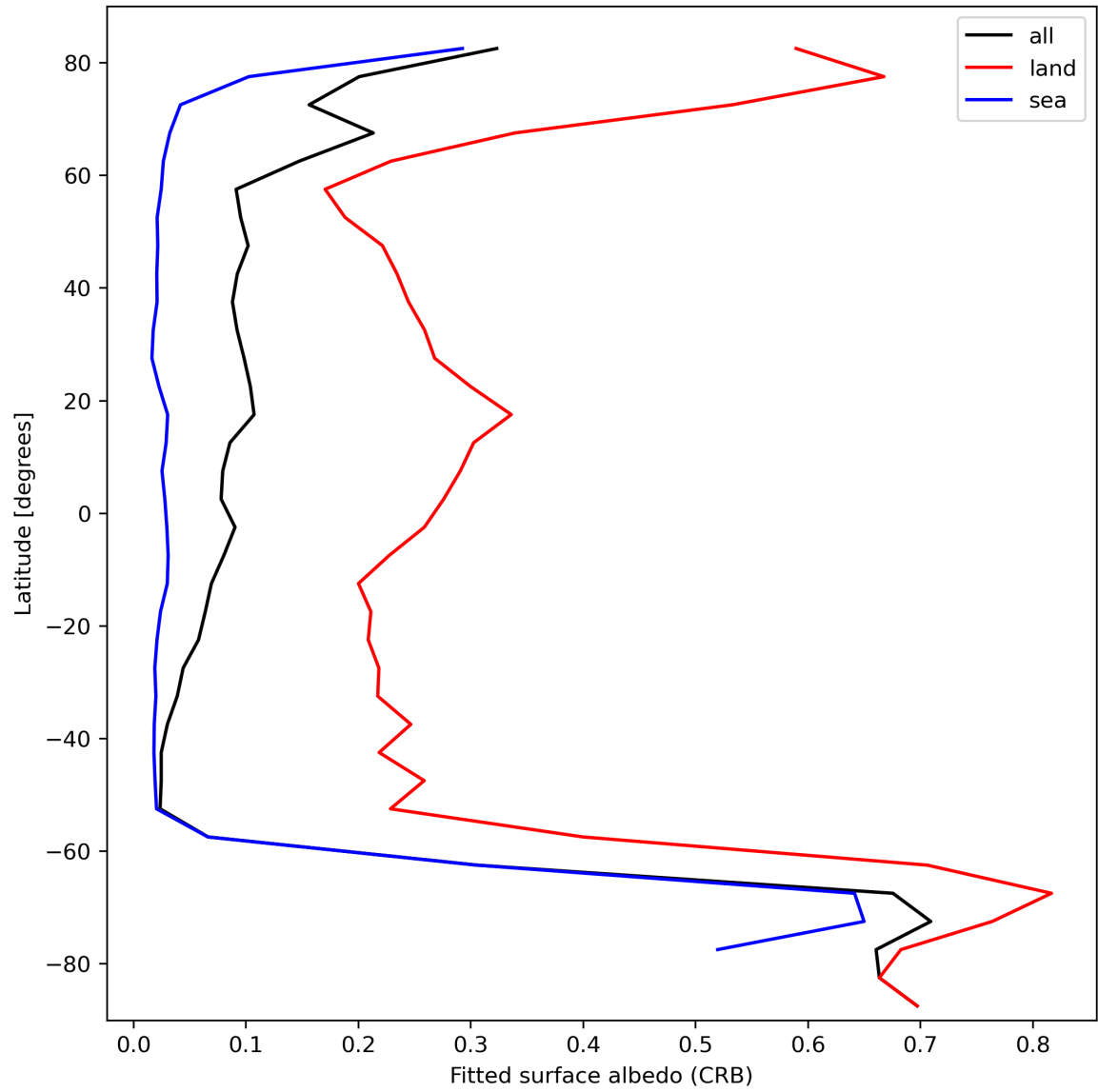
Figure 30: Zonal average of “Fitted surface albedo (CRB)” for 2023-10-04 to 2023-10-06.
