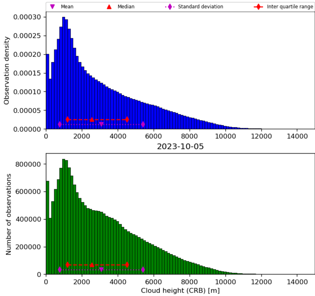
Figure 43: Histogram of “Cloud height (CRB)” for 2023-10-04 to 2023-10-06
