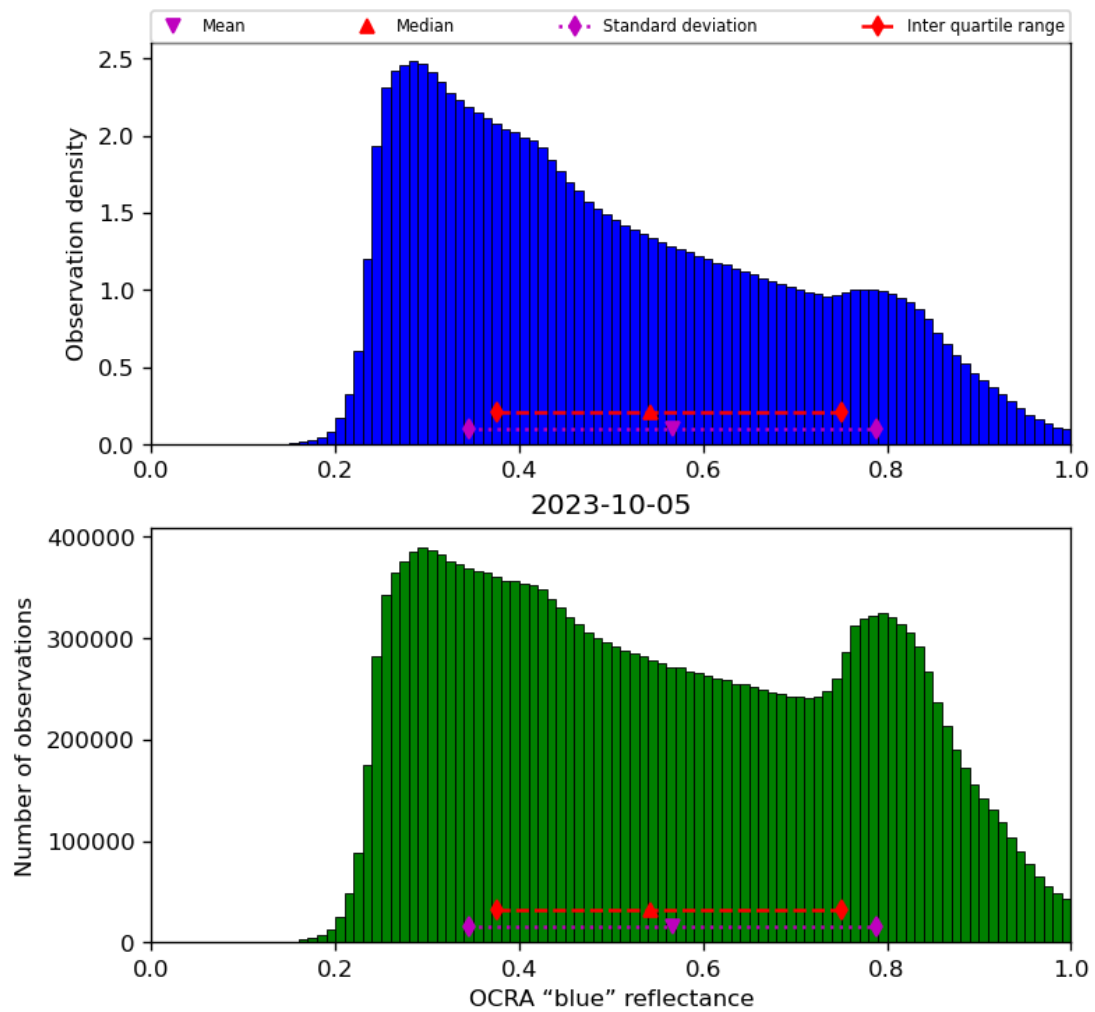
Figure 51: Histogram of “OCRA “blue” reflectance” for 2023-10-04 to 2023-10-06
