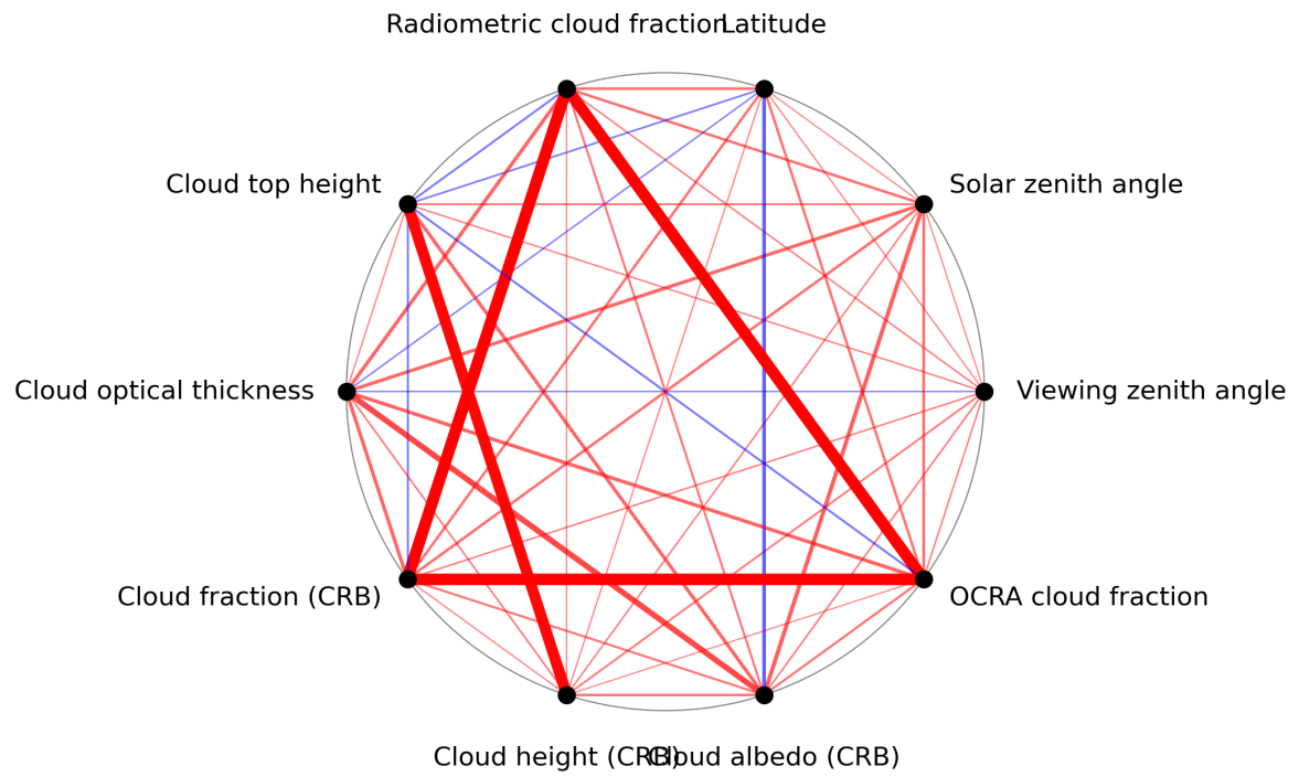
Figure 1: Map of correlation graph for 2023-10-04 to 2023-10-06.
