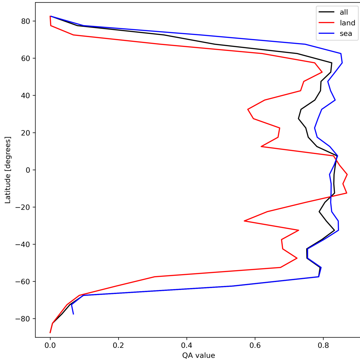
Figure 22: Zonal average of “QA value” for 2023-10-04 to 2023-10-06.
