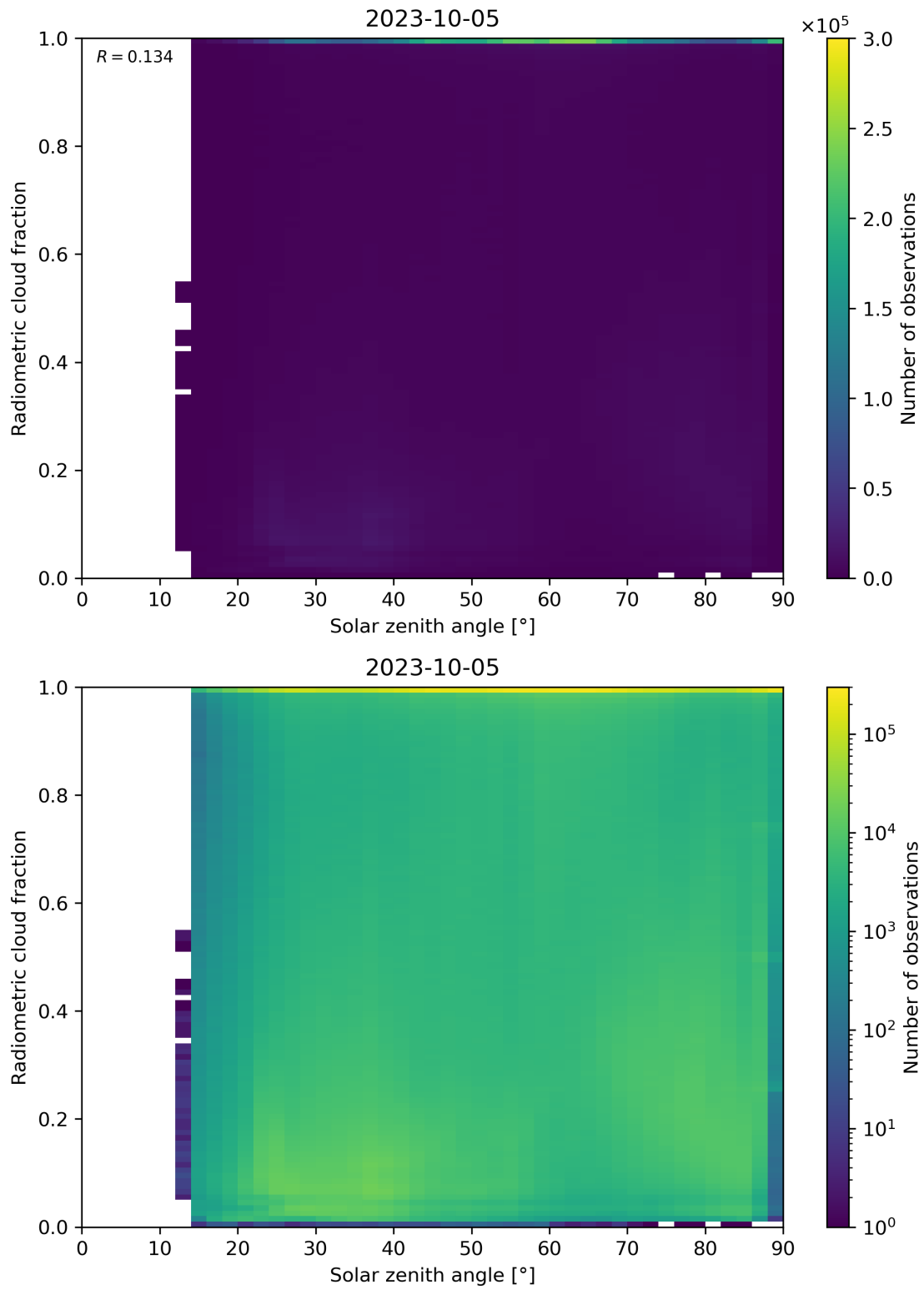
Figure 99: Scatter density plot of “Solar zenith angle” against “Radiometric cloud fraction” for 2023-10-04 to 2023-10-06.
