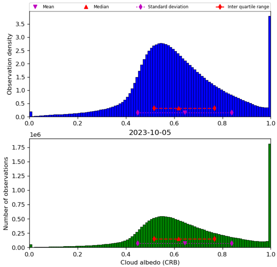
Figure 44: Histogram of “Cloud albedo (CRB)” for 2023-10-04 to 2023-10-06
