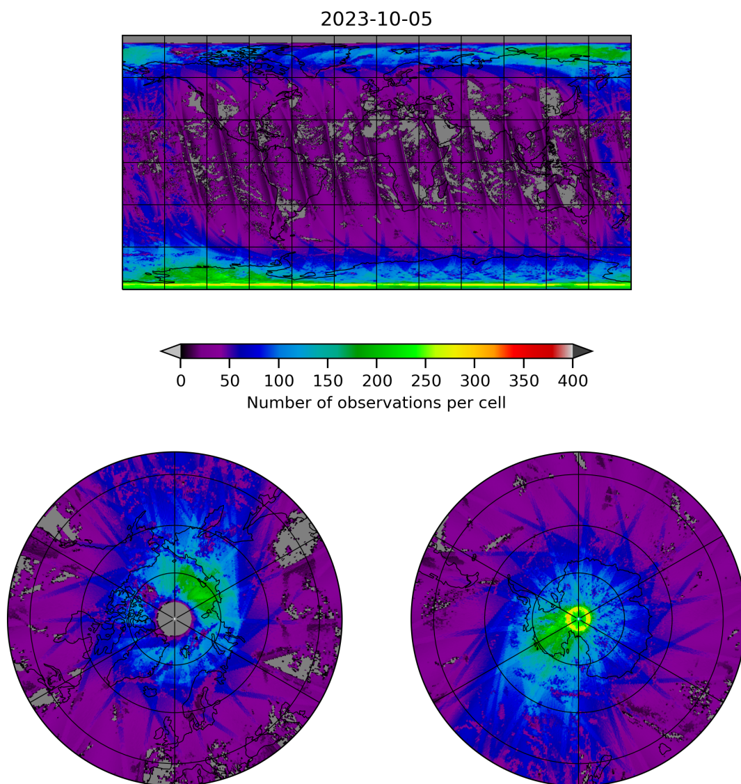
Figure 21: Map of the number of observations for 2023-10-04 to 2023-10-06
