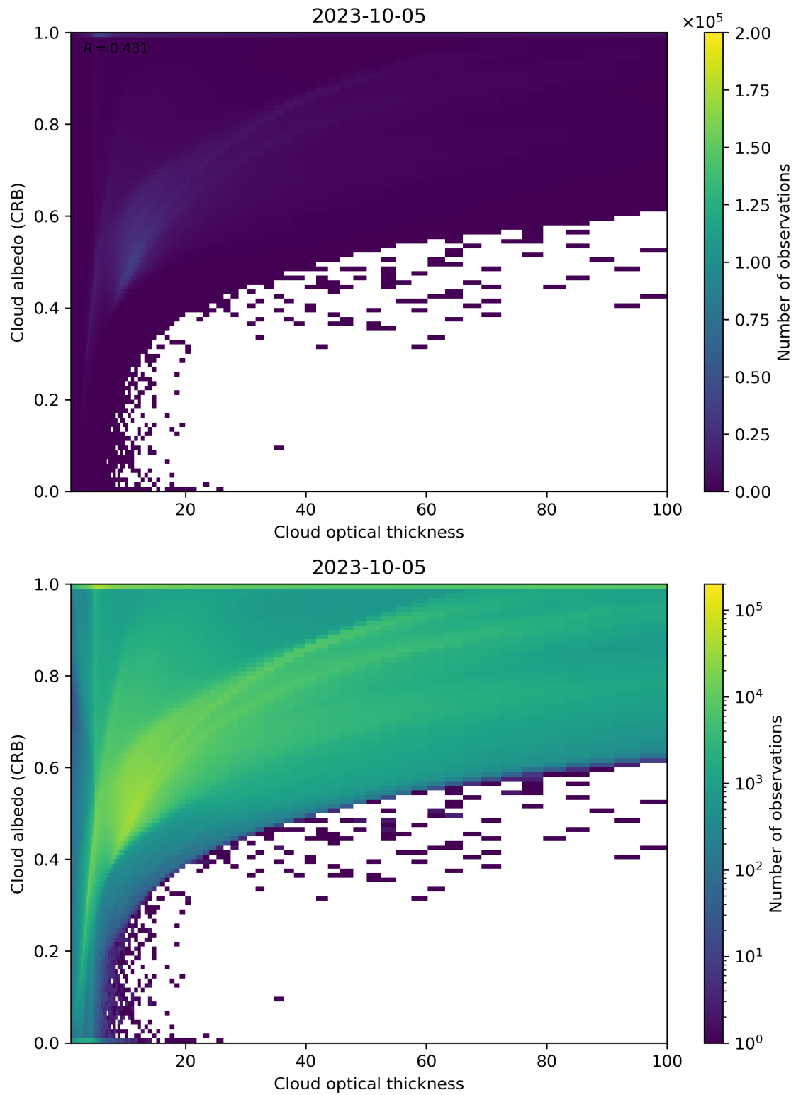
Figure 82: Scatter density plot of “Cloud optical thickness” against “Cloud albedo (CRB)” for 2023-10-04 to 2023-10-06.
