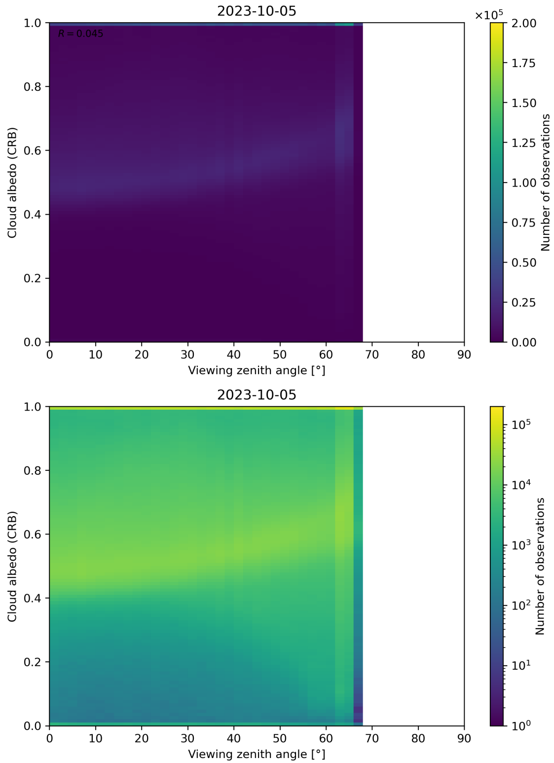
Figure 106: Scatter density plot of “Viewing zenith angle” against “Cloud albedo (CRB)” for 2023-10-04 to 2023-10-06.
