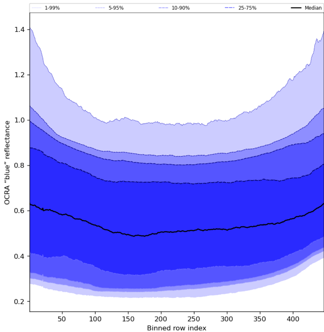
Figure 67: Along track statistics of "OCRA "blue" reflectance" for 2023-10-04 to 2023-10-06
