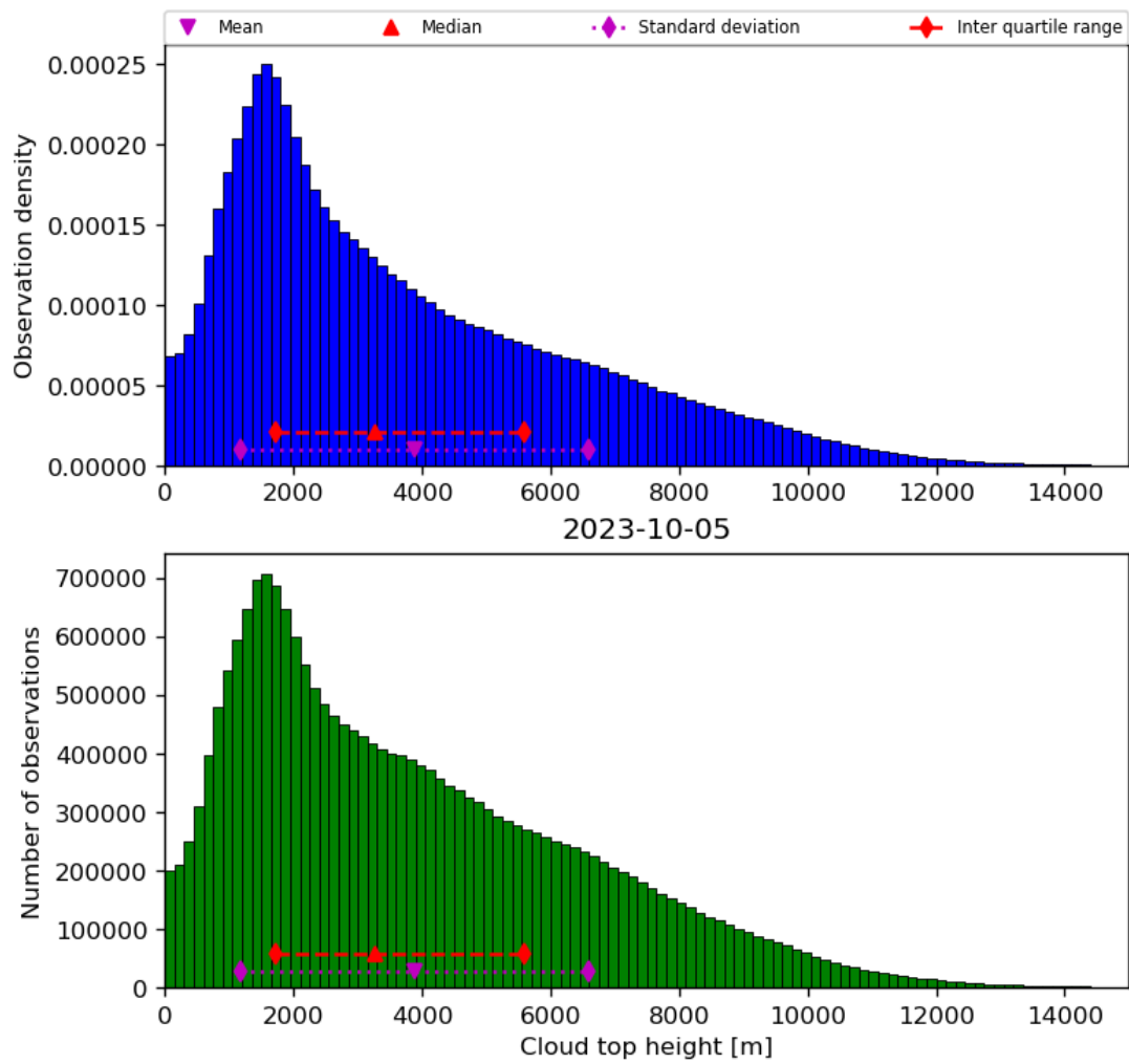
Figure 40: Histogram of “Cloud top height” for 2023-10-04 to 2023-10-06
