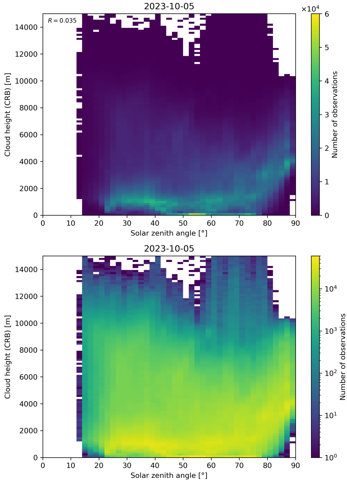
Figure 102: Scatter density plot of “Solar zenith angle” against “Cloud height (CRB)” for 2023-10-04 to 2023-10-06.
