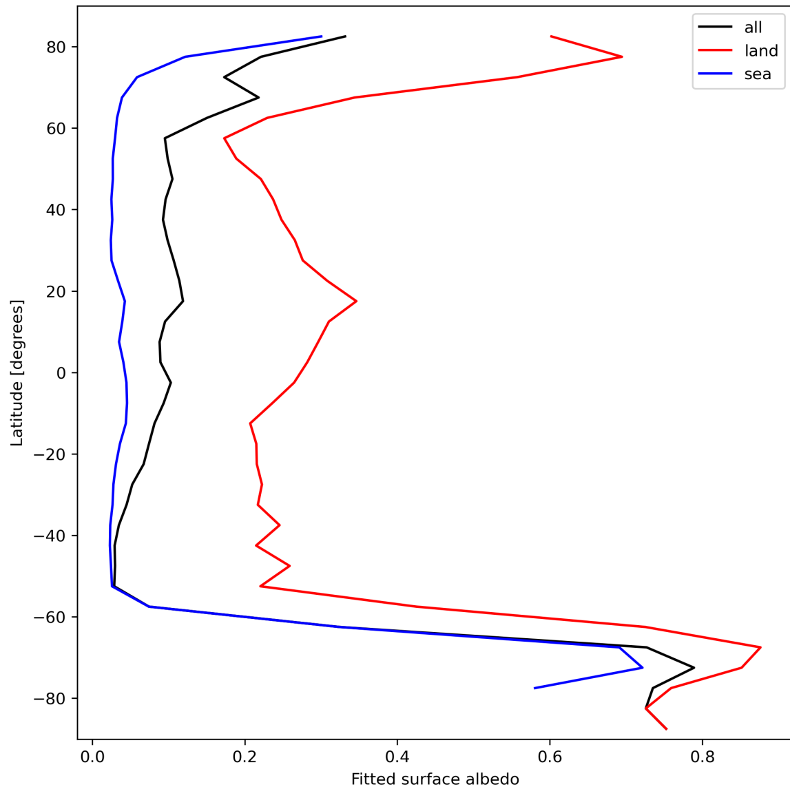
Figure 29: Zonal average of “Fitted surface albedo” for 2023-10-04 to 2023-10-06.
