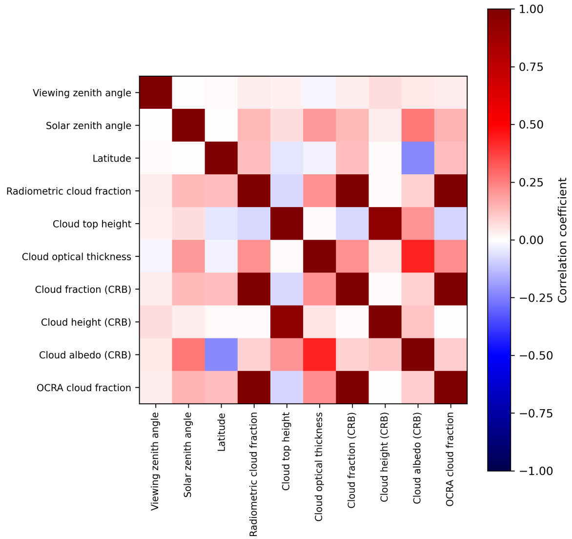
Figure 2: Map of correlation matrix for 2023-10-04 to 2023-10-06.
