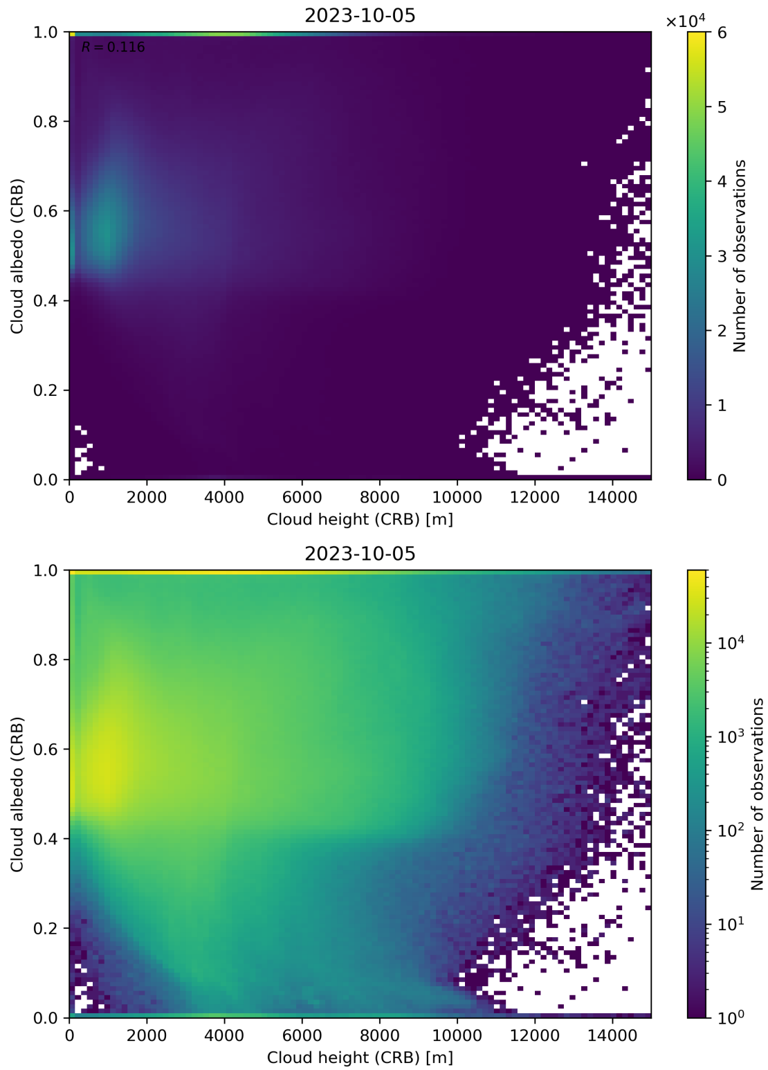
Figure 80: Scatter density plot of “Cloud height (CRB)” against “Cloud albedo (CRB)” for 2023-10-04 to 2023-10-06.
