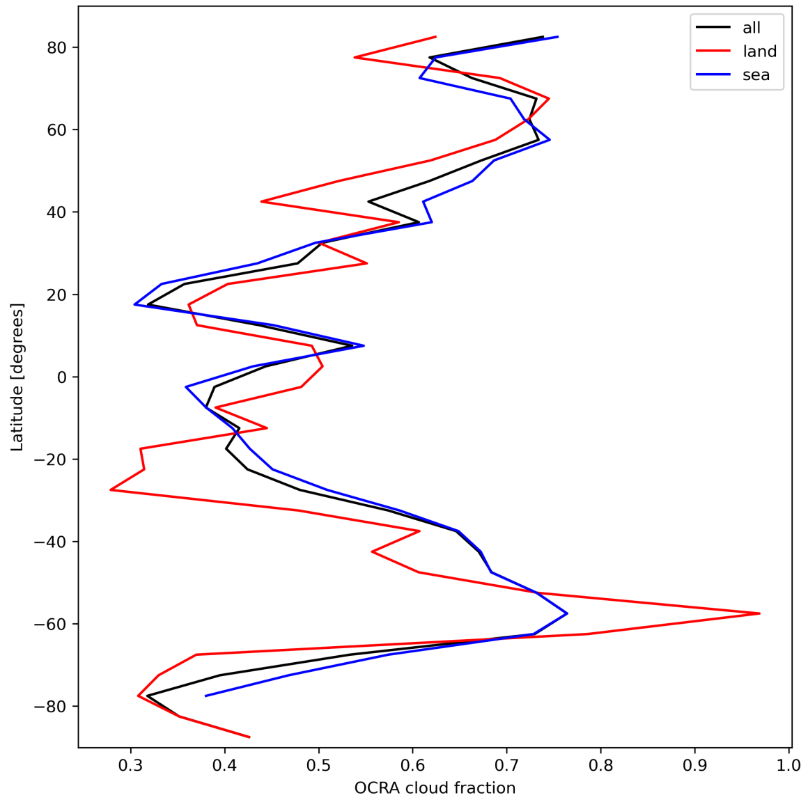
Figure 34: Zonal average of “OCRA cloud fraction” for 2023-10-04 to 2023-10-06.
