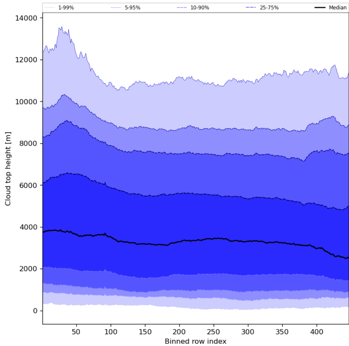
Figure 56: Along track statistics of “Cloud top height” for 2023-10-04 to 2023-10-06
