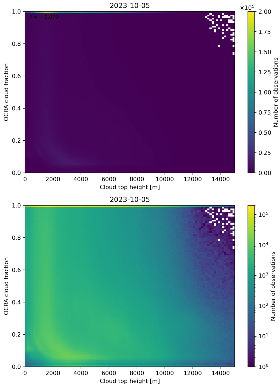
Figure 87: Scatter density plot of “Cloud top height” against “OCRA cloud fraction” for 2023-10-04 to 2023-10-06.
