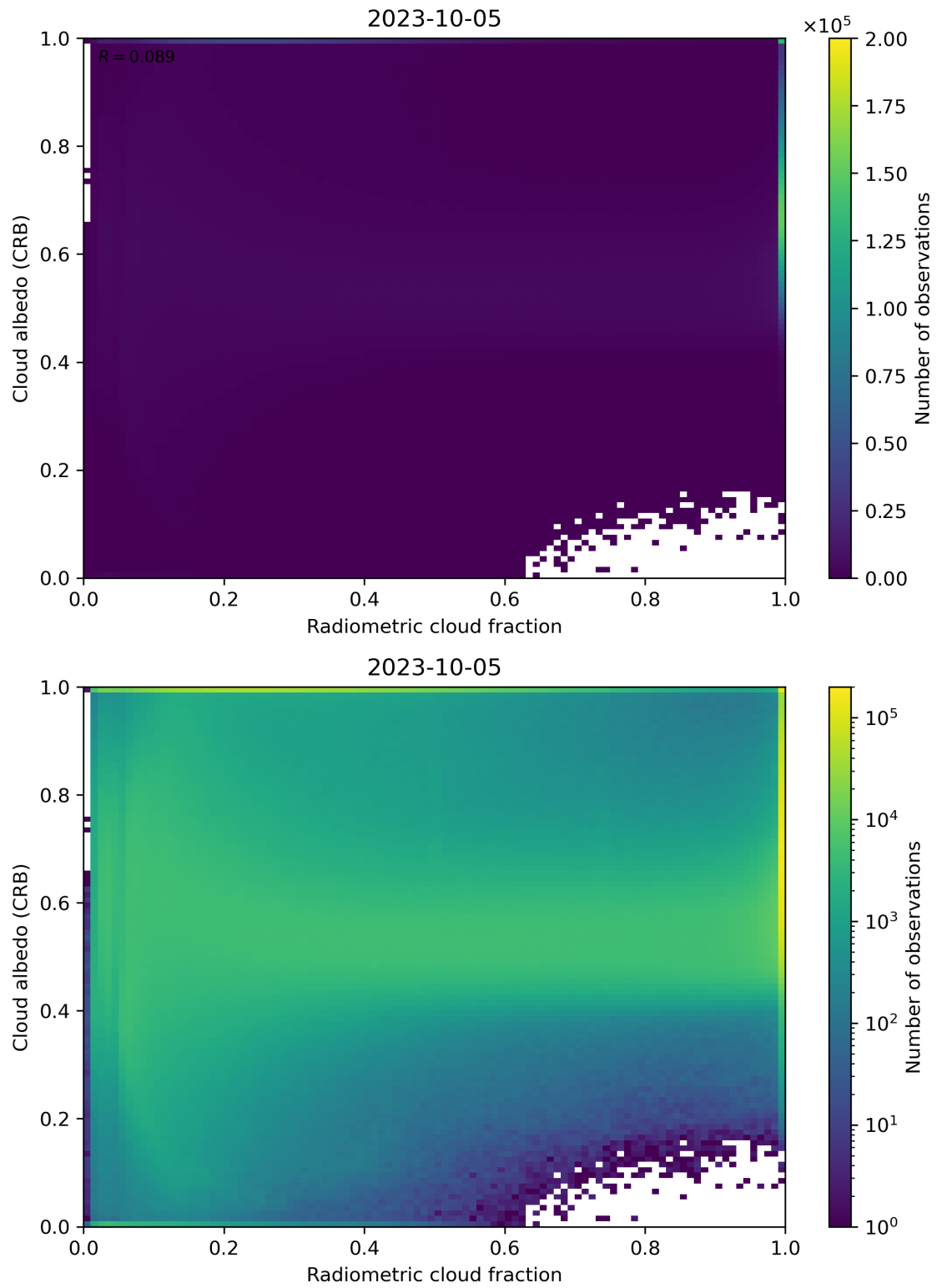
Figure 71: Scatter density plot of “Radiometric cloud fraction” against “Cloud albedo (CRB)” for 2023-10-04 to 2023-10-06.
