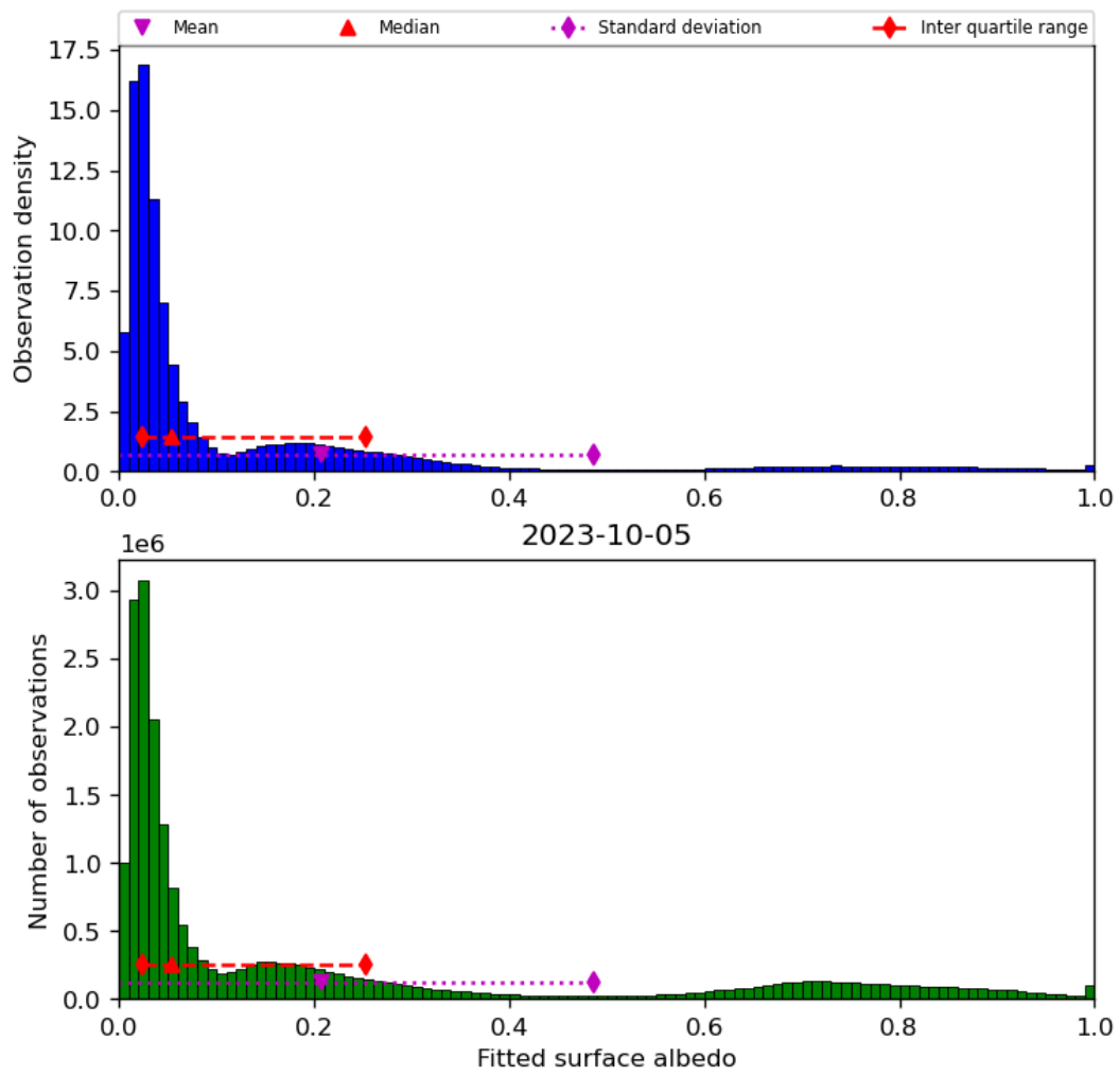
Figure 45: Histogram of “Fitted surface albedo” for 2023-10-04 to 2023-10-06
