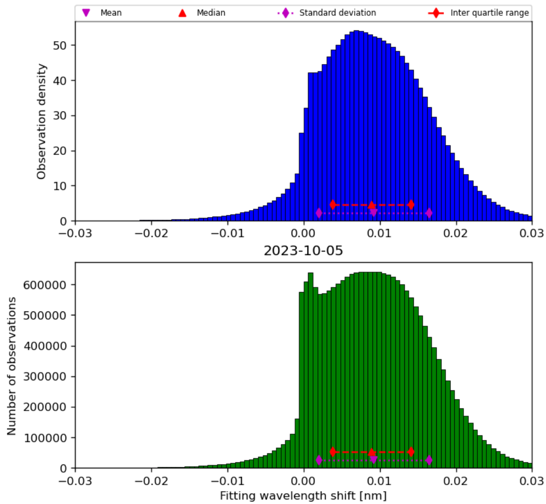
Figure 49: Histogram of “Fitting wavelength shift” for 2023-10-04 to 2023-10-06
