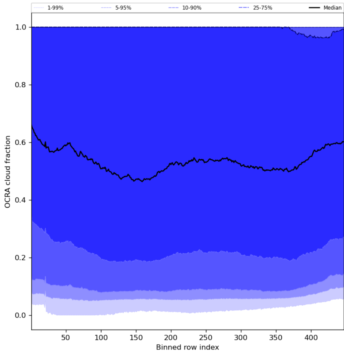
Figure 66: Along track statistics of “OCRA cloud fraction” for 2023-10-04 to 2023-10-06
