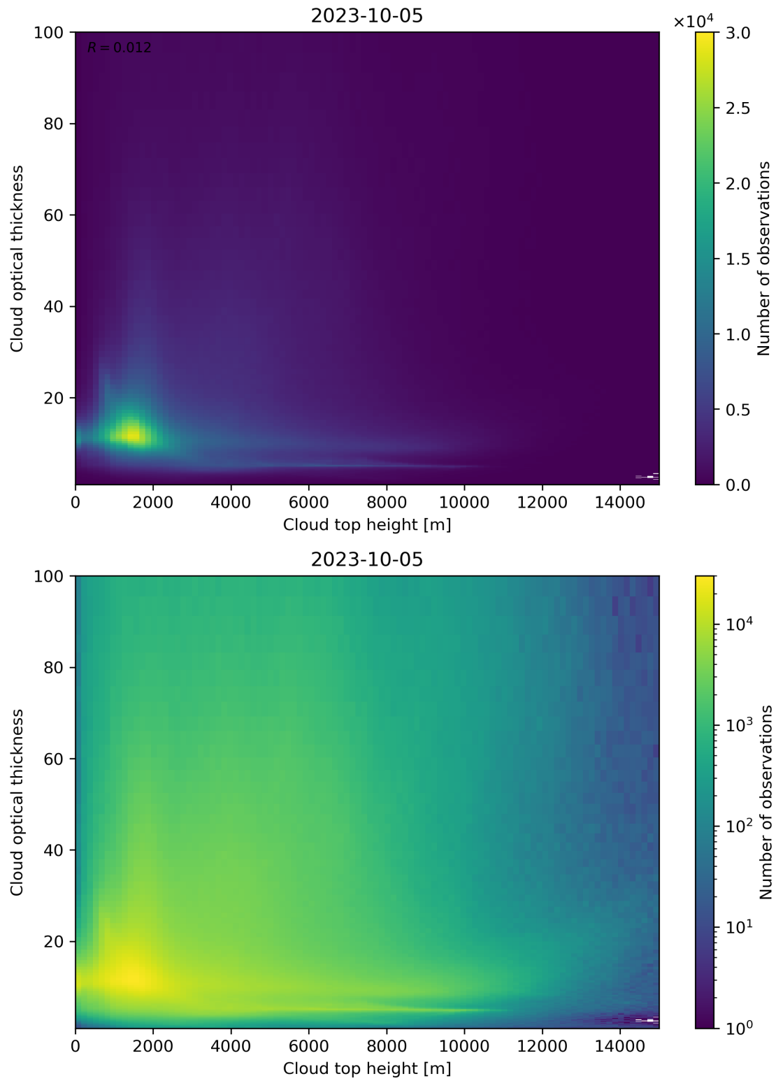
Figure 90: Scatter density plot of “Cloud top height” against “Cloud optical thickness” for 2023-10-04 to 2023-10-06.
