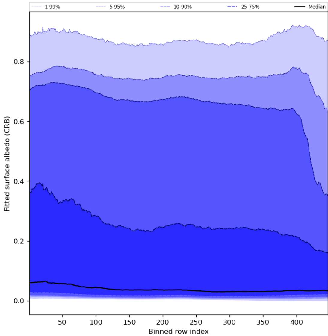
Figure 62: Along track statistics of “Fitted surface albedo (CRB)” for 2023-10-04 to 2023-10-06
