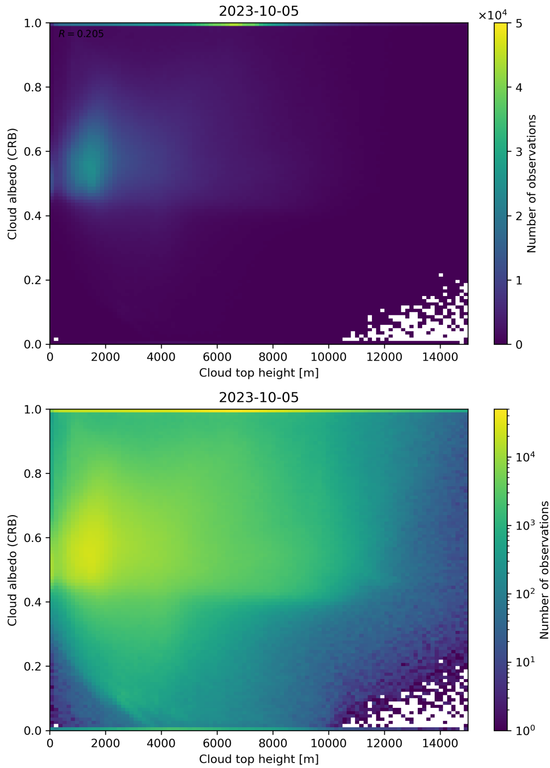
Figure 86: Scatter density plot of “Cloud top height” against “Cloud albedo (CRB)” for 2023-10-04 to 2023-10-06.
