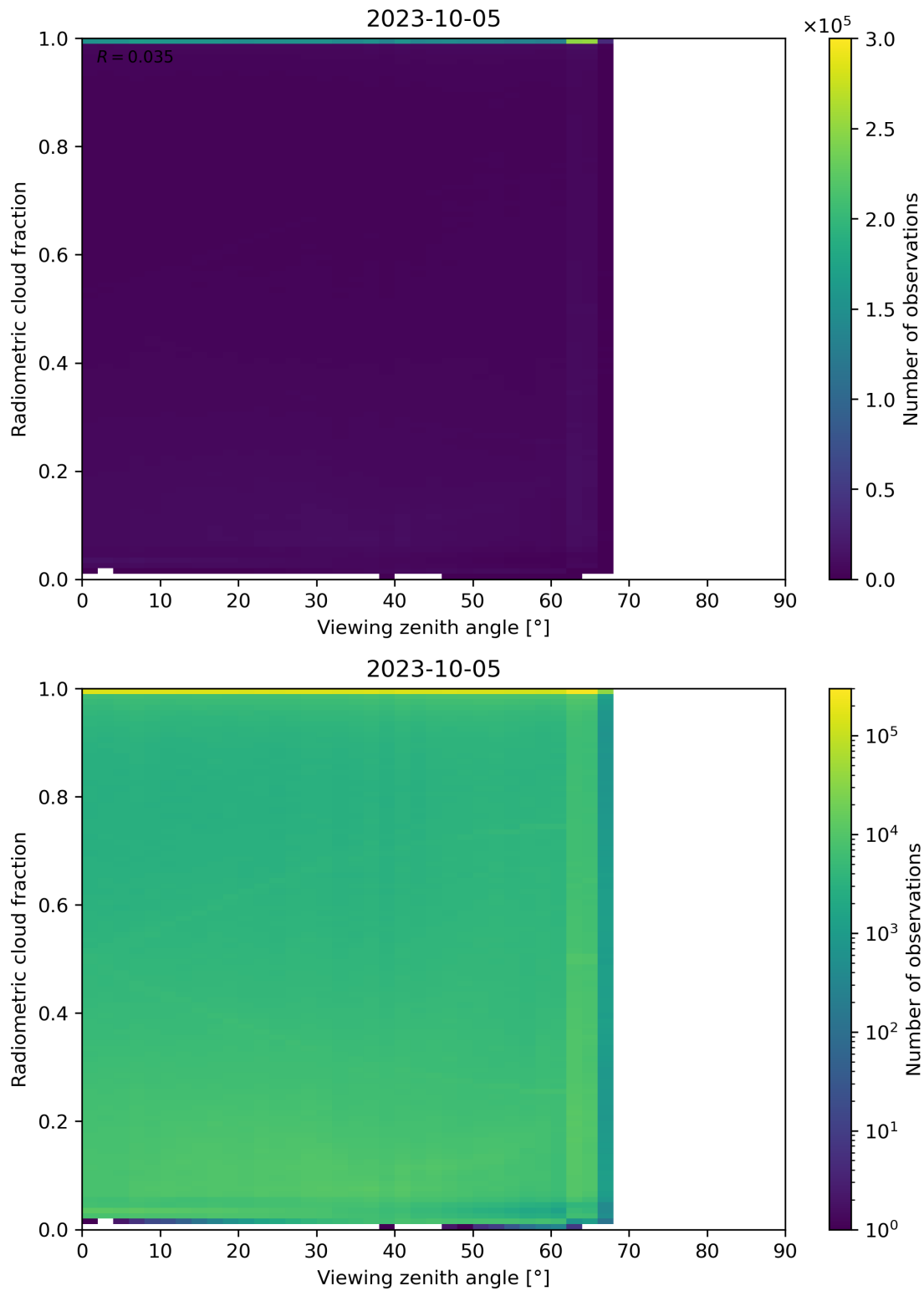
Figure 107: Scatter density plot of “Viewing zenith angle” against “Radiometric cloud fraction” for 2023-10-04 to 2023-10-06.
