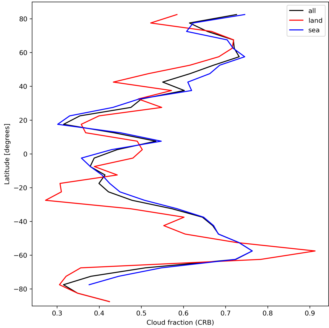
Figure 26: Zonal average of “Cloud fraction (CRB)” for 2023-10-04 to 2023-10-06.
