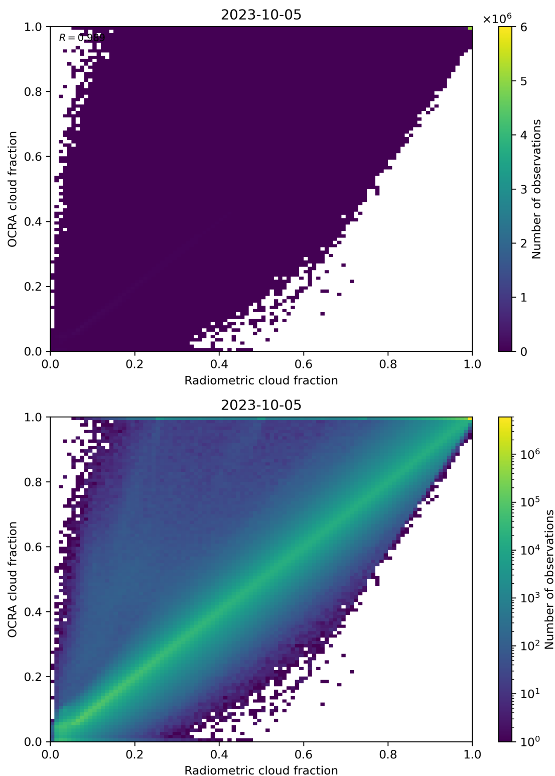
Figure 72: Scatter density plot of “Radiometric cloud fraction” against “OCRA cloud fraction” for 2023-10-04 to 2023-10-06.
