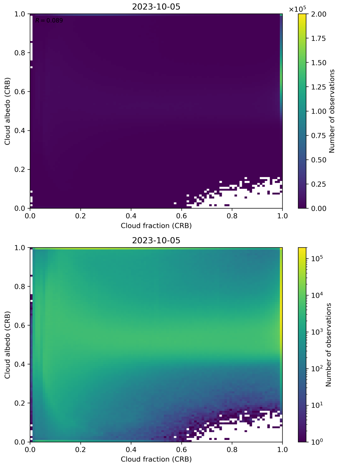
Figure 77: Scatter density plot of “Cloud fraction (CRB)” against “Cloud albedo (CRB)” for 2023-10-04 to 2023-10-06.
