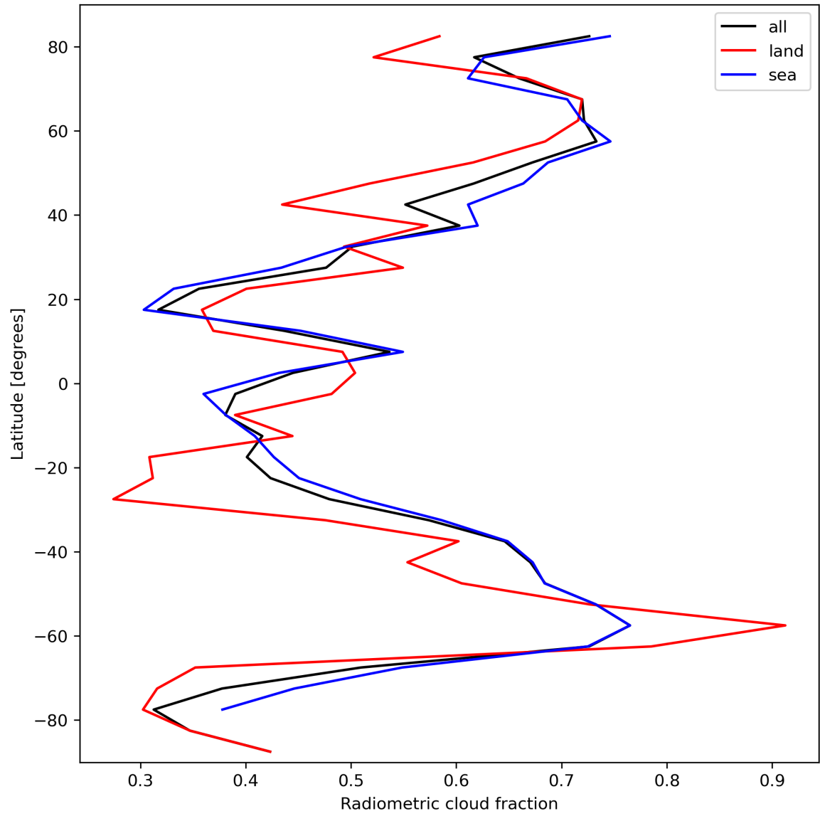
Figure 23: Zonal average of “Radiometric cloud fraction” for 2023-10-04 to 2023-10-06.
