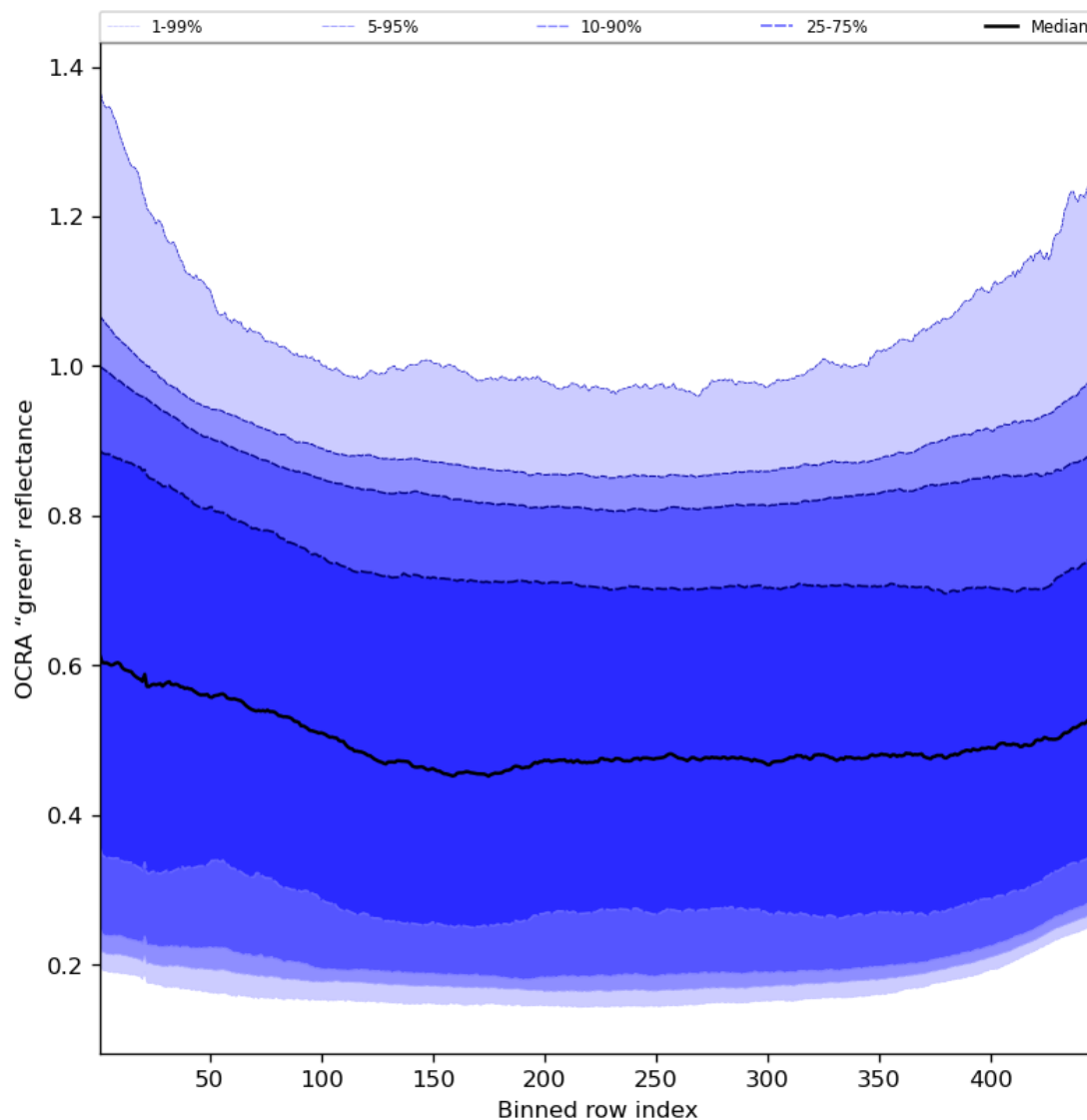
Figure 68: Along track statistics of “OCRA “green” reflectance” for 2023-10-04 to 2023-10-06
