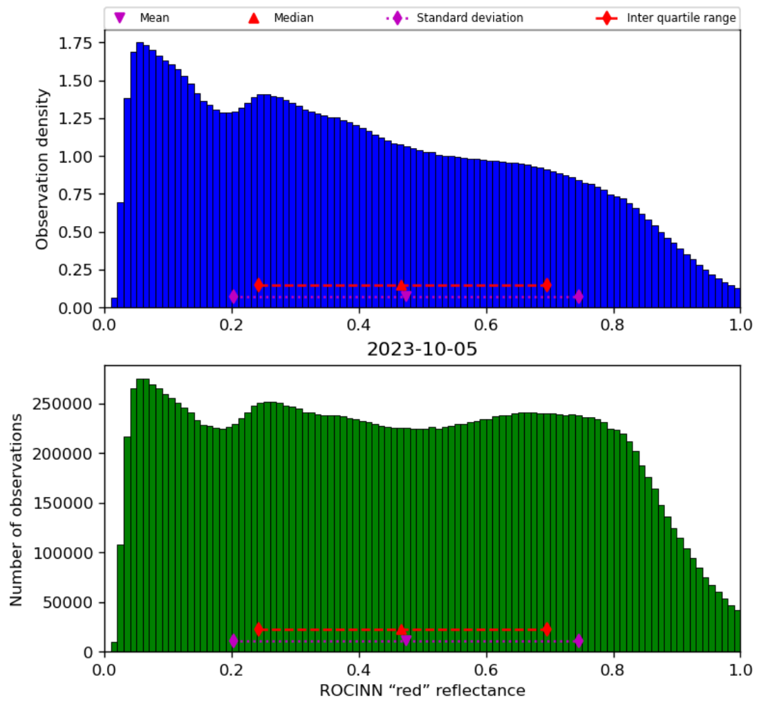
Figure 53: Histogram of “ROCINN “red” reflectance” for 2023-10-04 to 2023-10-06
