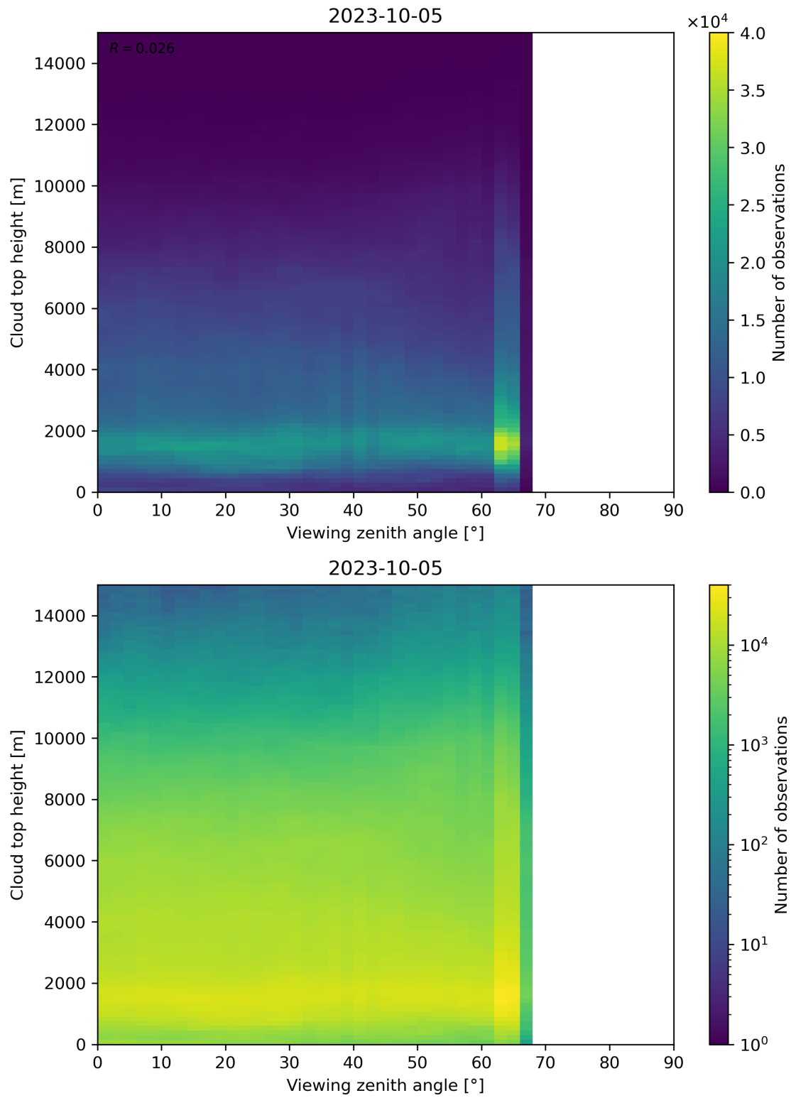
Figure 112: Scatter density plot of “Viewing zenith angle” against “Cloud top height” for 2023-10-04 to 2023-10-06.
