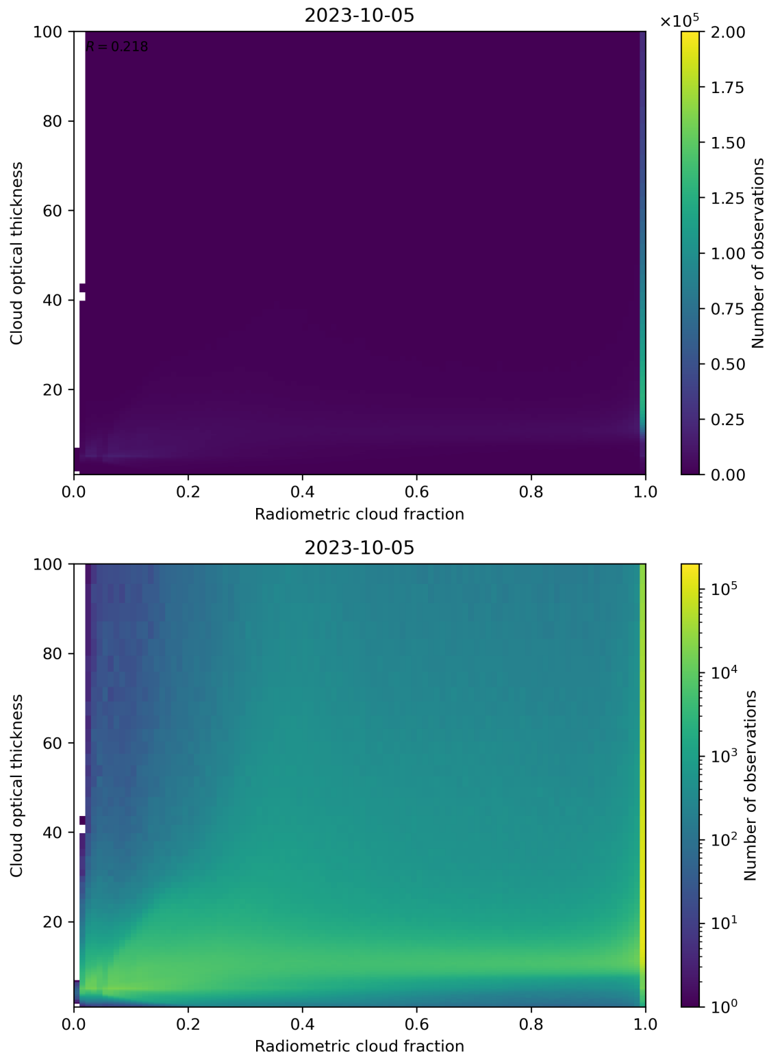
Figure 75: Scatter density plot of “Radiometric cloud fraction” against “Cloud optical thickness” for 2023-10-04 to 2023-10-06.
