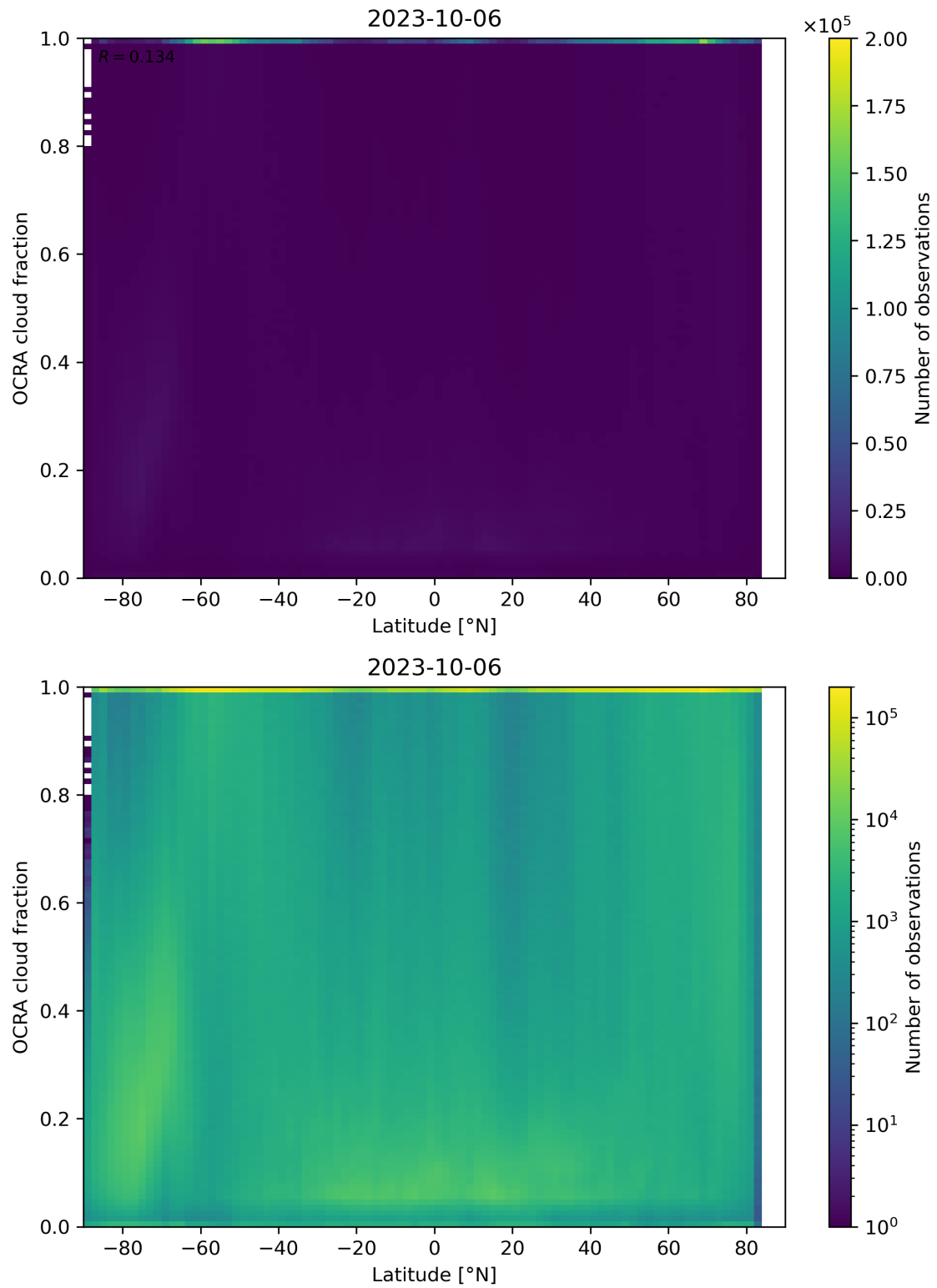
Figure 93: Scatter density plot of “Latitude” against “OCRA cloud fraction” for 2023-10-06 to 2023-10-07.
