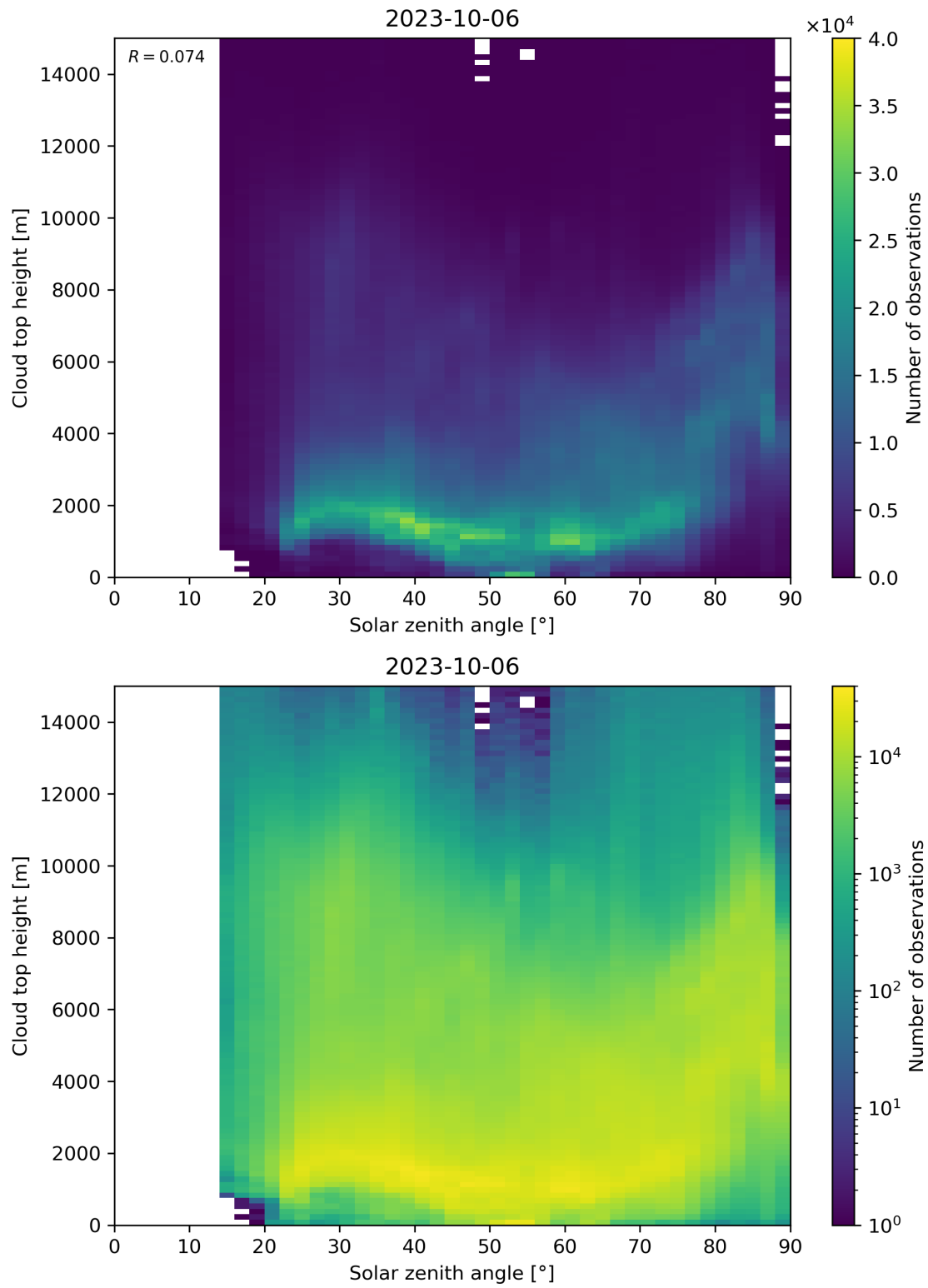
Figure 104: Scatter density plot of “Solar zenith angle” against “Cloud top height” for 2023-10-06 to 2023-10-07.
