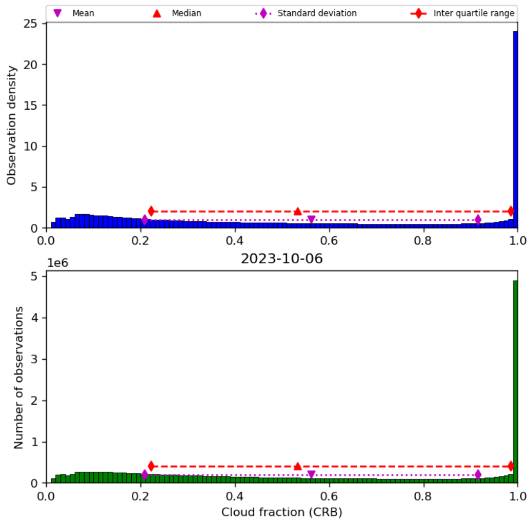
Figure 42: Histogram of “Cloud fraction (CRB)” for 2023-10-06 to 2023-10-07
