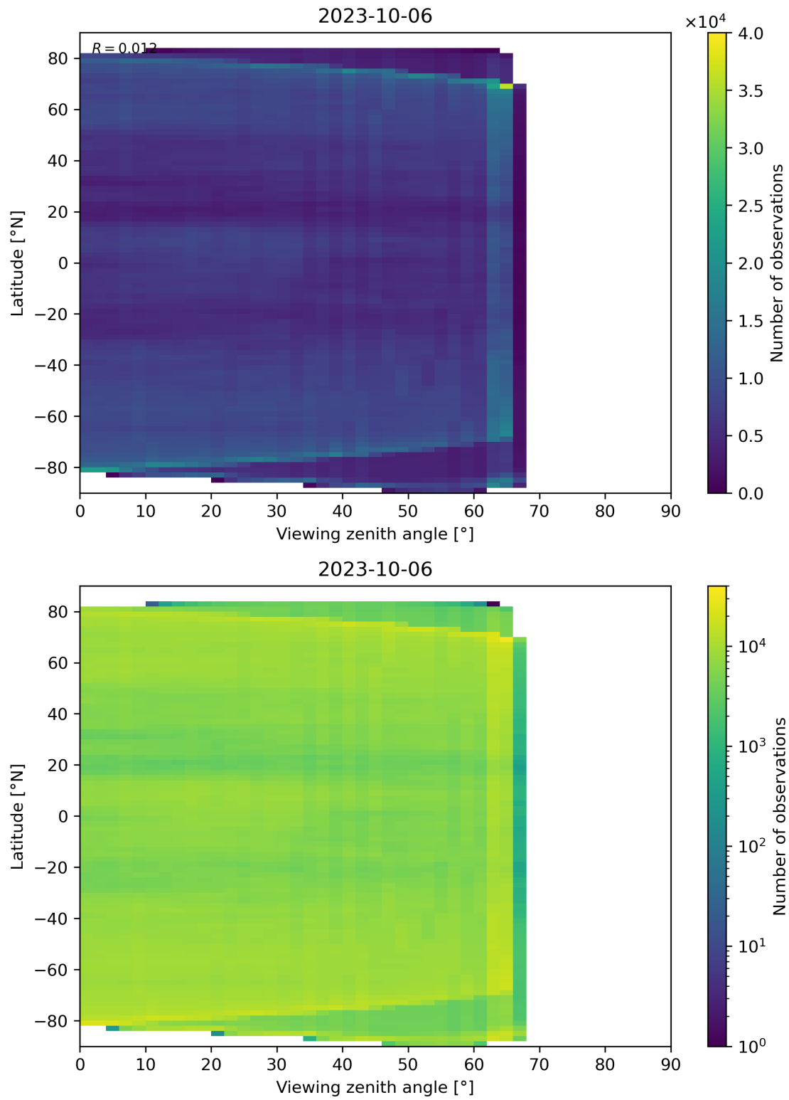
Figure 113: Scatter density plot of “Viewing zenith angle” against “Latitude” for 2023-10-06 to 2023-10-07.
