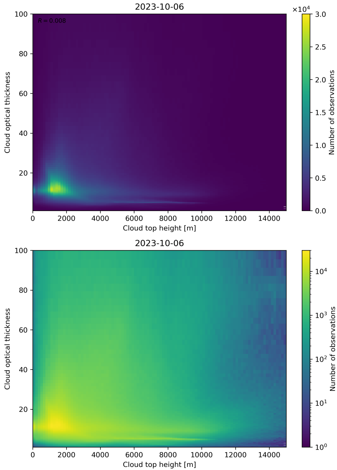
Figure 90: Scatter density plot of “Cloud top height” against “Cloud optical thickness” for 2023-10-06 to 2023-10-07.
