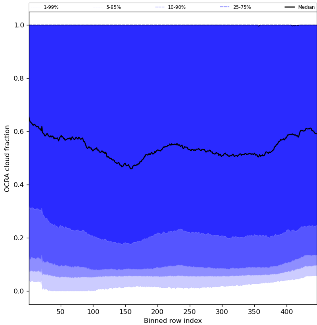
Figure 66: Along track statistics of “OCRA cloud fraction” for 2023-10-06 to 2023-10-07
