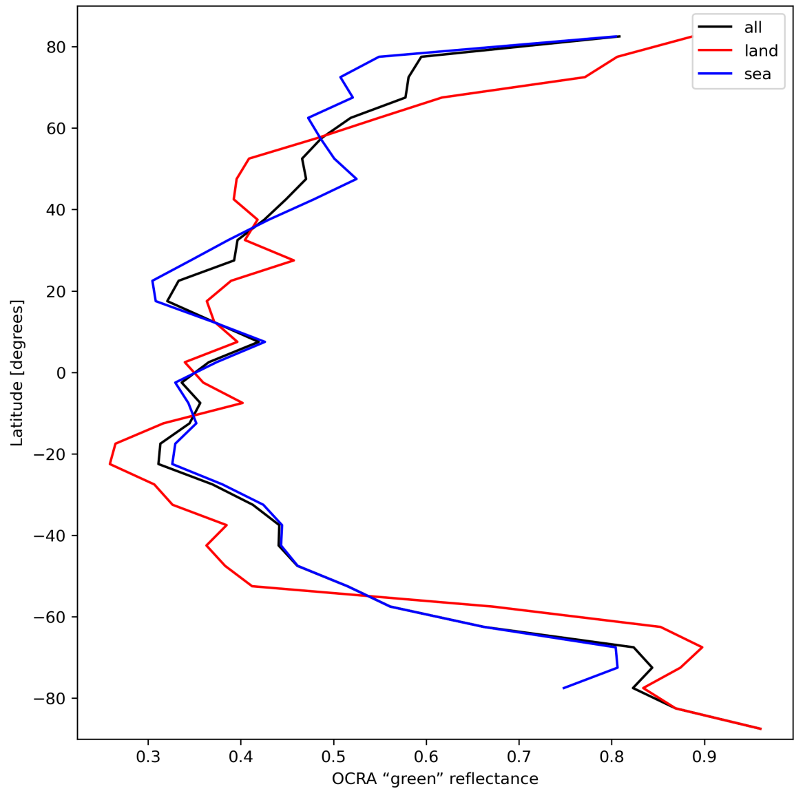
Figure 36: Zonal average of “OCRA “green” reflectance” for 2023-10-06 to 2023-10-07.
