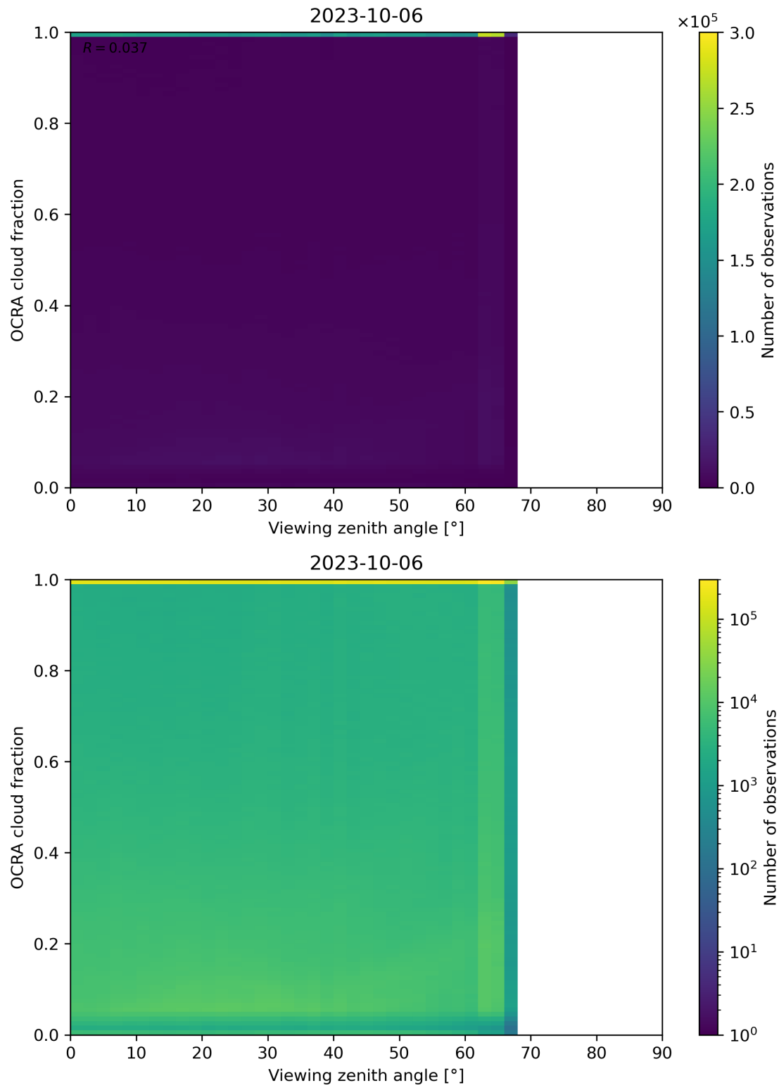
Figure 108: Scatter density plot of “Viewing zenith angle” against “OCRA cloud fraction” for 2023-10-06 to 2023-10-07.
