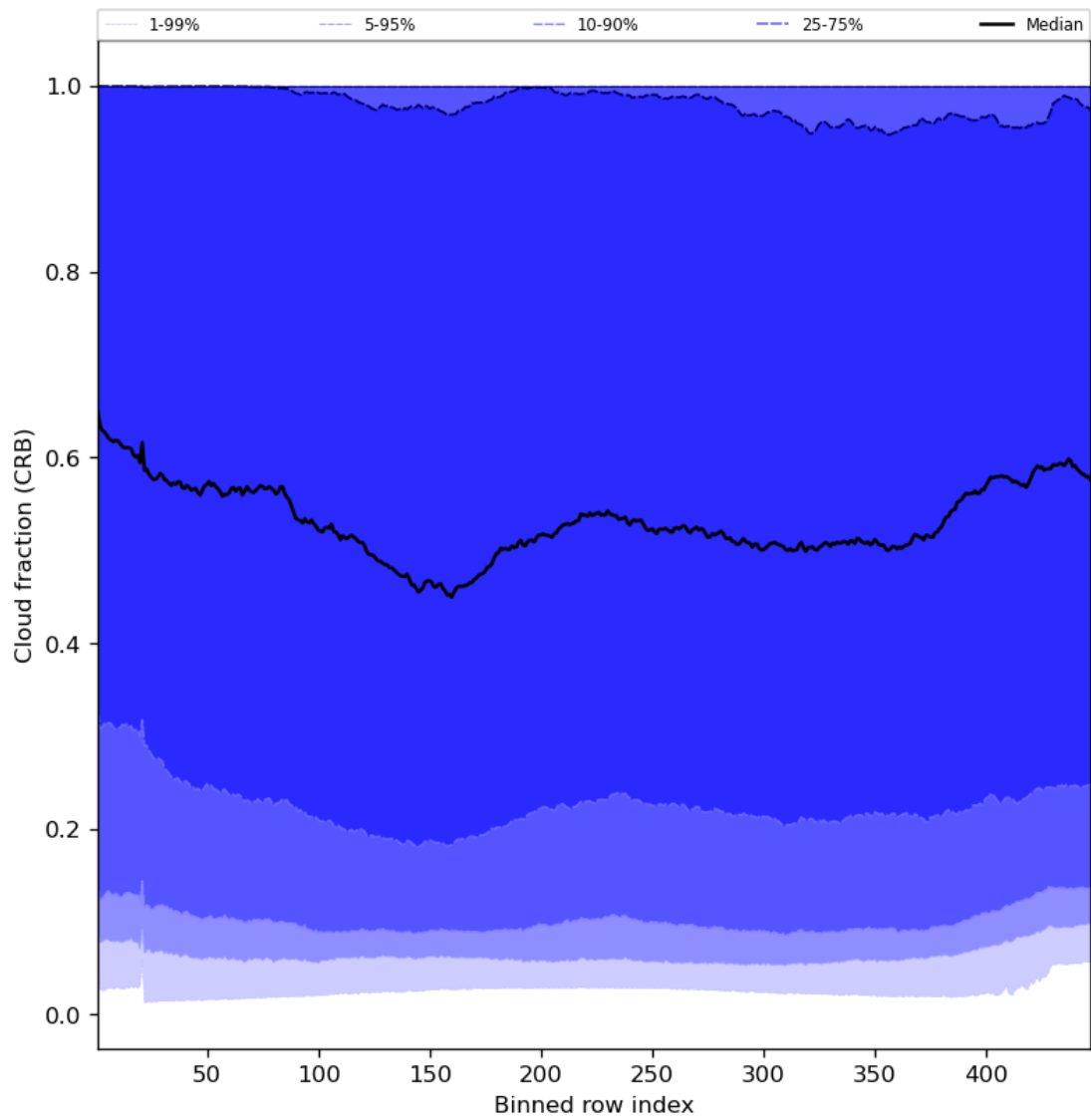
Figure 58: Along track statistics of “Cloud fraction (CRB)” for 2023-10-06 to 2023-10-07
