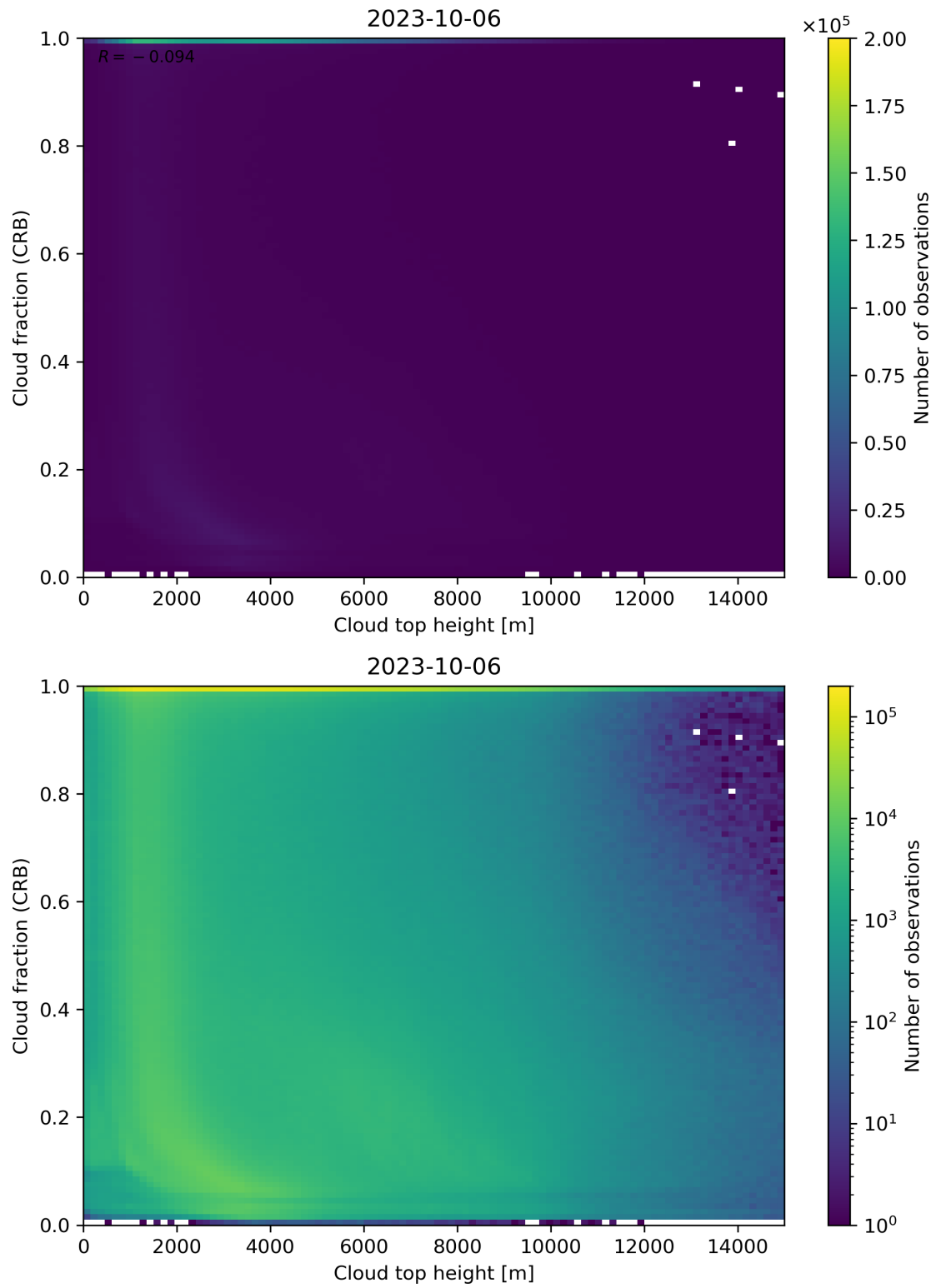
Figure 88: Scatter density plot of “Cloud top height” against “Cloud fraction (CRB)” for 2023-10-06 to 2023-10-07.
