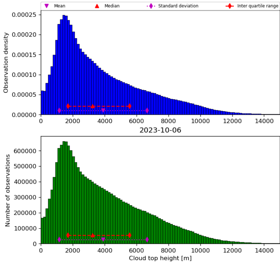
Figure 40: Histogram of “Cloud top height” for 2023-10-06 to 2023-10-07
