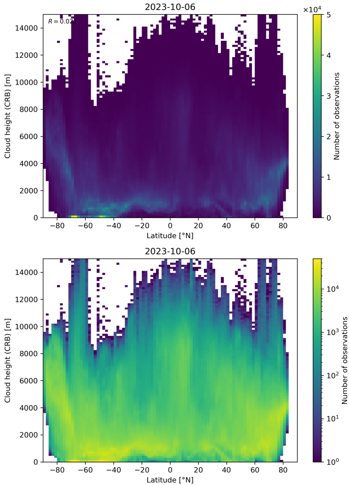
Figure 95: Scatter density plot of “Latitude” against “Cloud height (CRB)” for 2023-10-06 to 2023-10-07.
