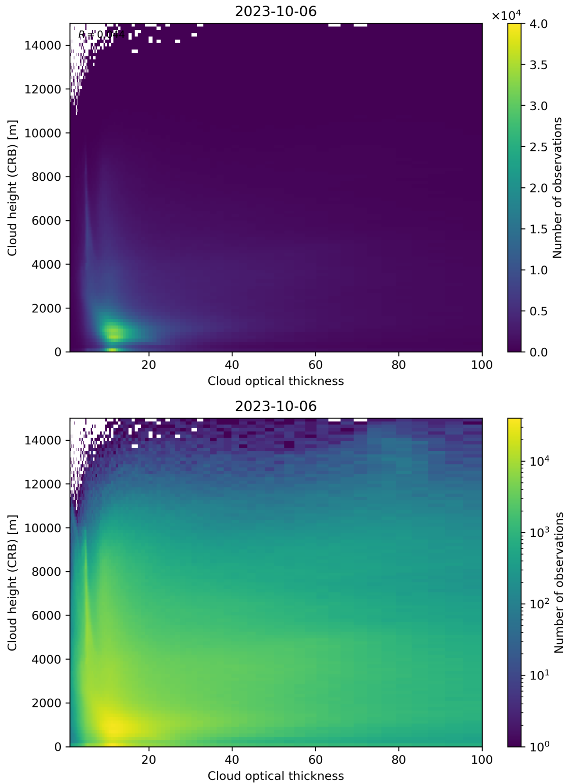
Figure 85: Scatter density plot of “Cloud optical thickness” against “Cloud height (CRB)” for 2023-10-06 to 2023-10-07.
