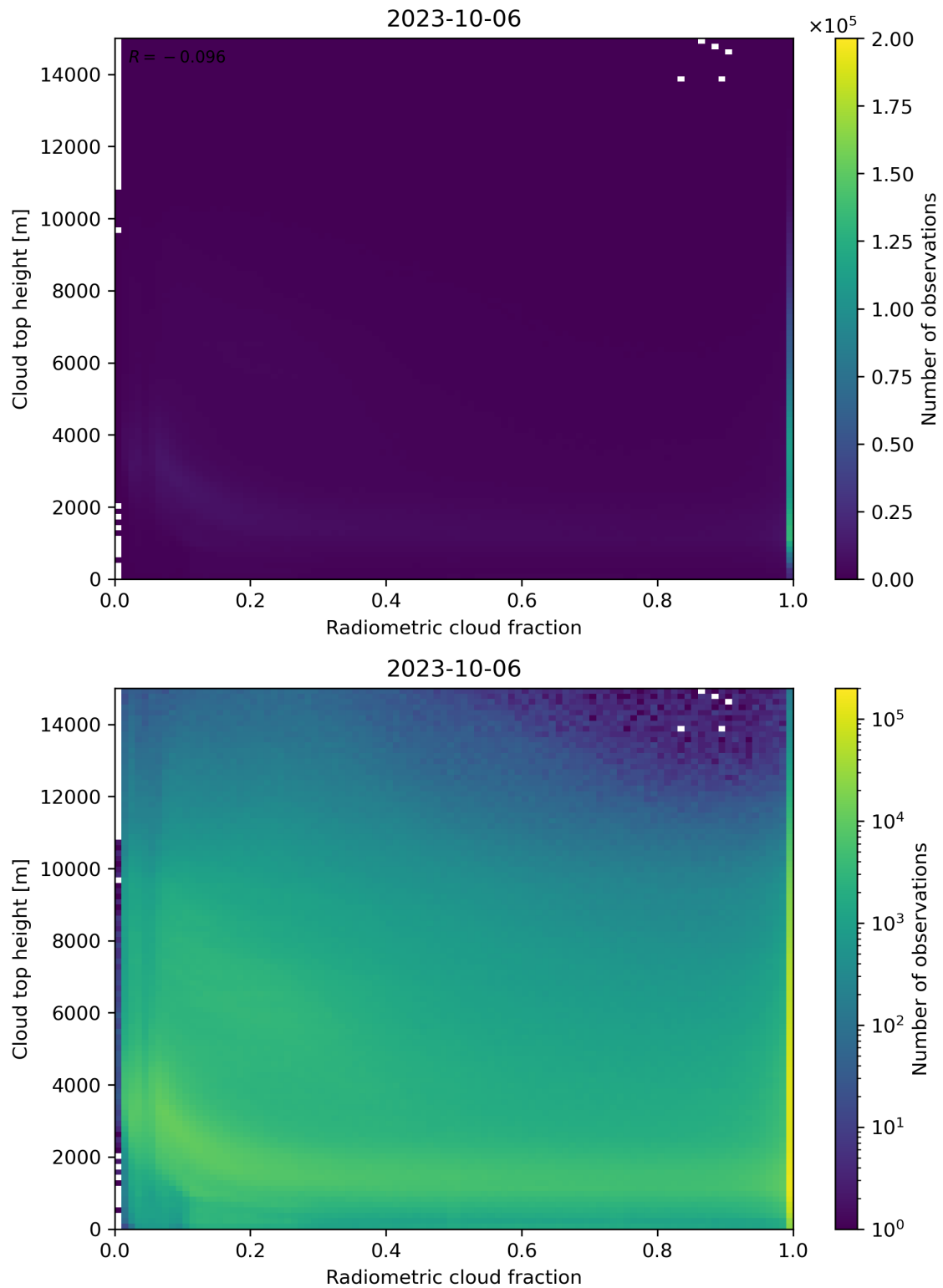
Figure 76: Scatter density plot of “Radiometric cloud fraction” against “Cloud top height” for 2023-10-06 to 2023-10-07.
