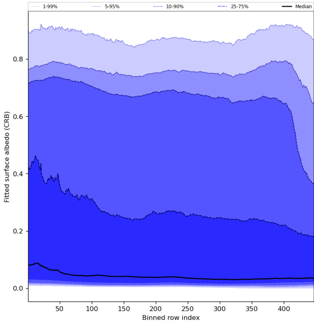
Figure 62: Along track statistics of “Fitted surface albedo (CRB)” for 2023-10-06 to 2023-10-07
