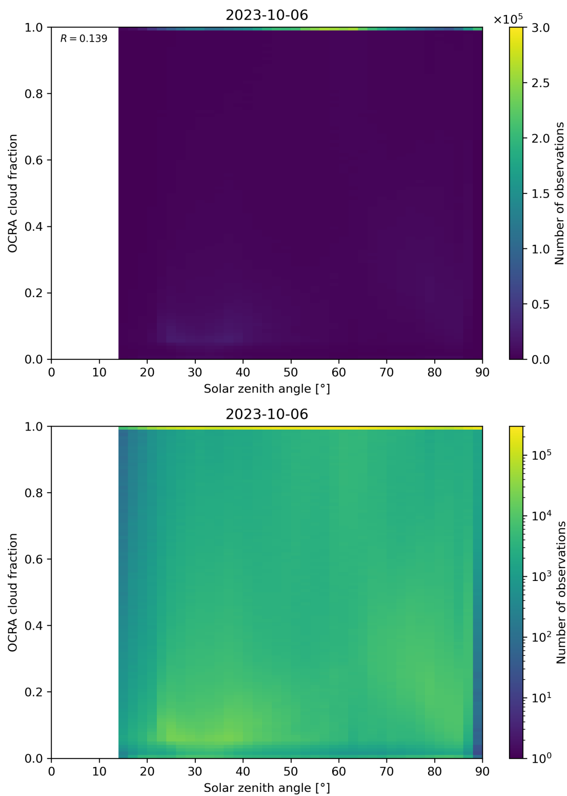
Figure 100: Scatter density plot of “Solar zenith angle” against “OCRA cloud fraction” for 2023-10-06 to 2023-10-07.
