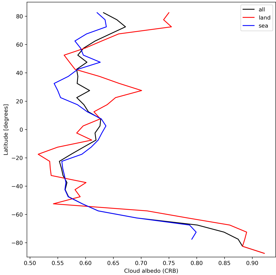
Figure 28: Zonal average of “Cloud albedo (CRB)” for 2023-10-06 to 2023-10-07.
