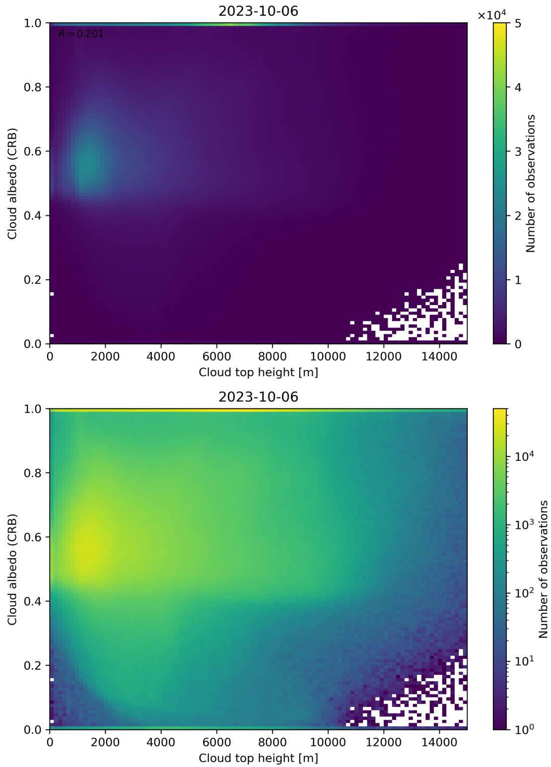
Figure 86: Scatter density plot of “Cloud top height” against “Cloud albedo (CRB)” for 2023-10-06 to 2023-10-07.
