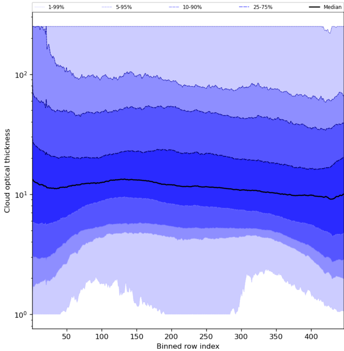
Figure 57: Along track statistics of “Cloud optical thickness” for 2023-10-06 to 2023-10-07
