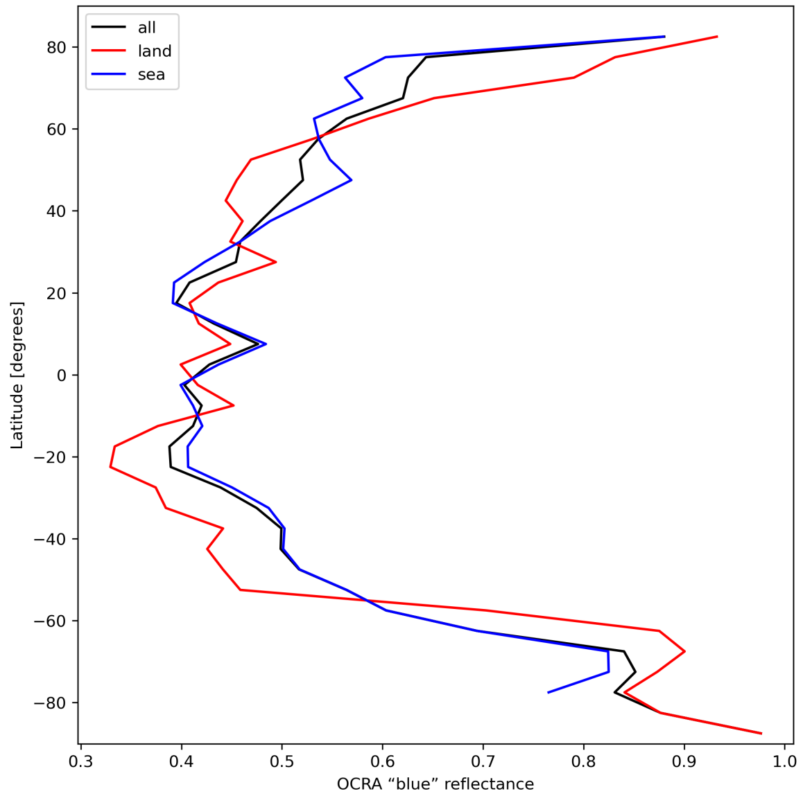
Figure 35: Zonal average of “OCRA “blue” reflectance” for 2023-10-06 to 2023-10-07.
