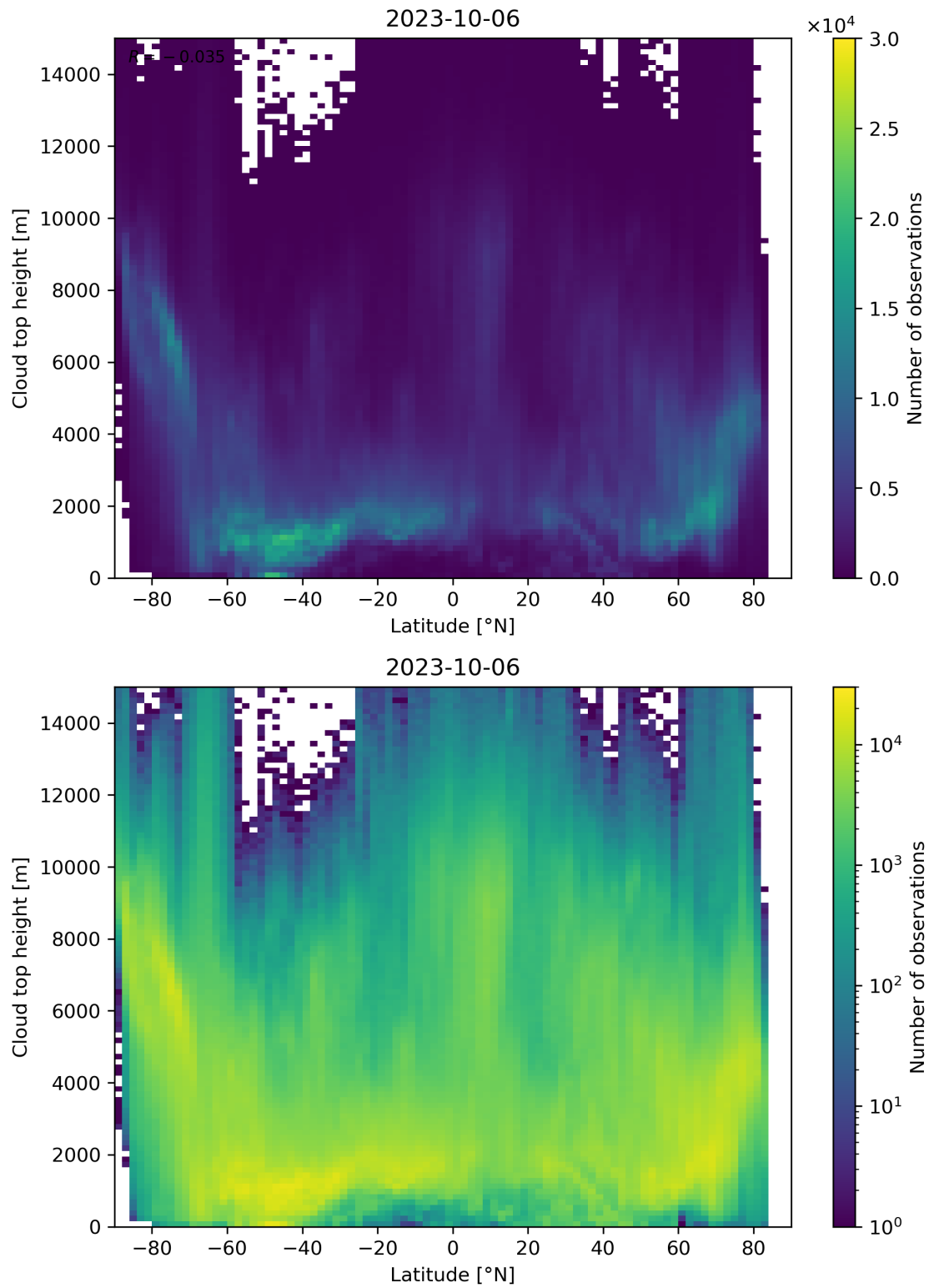
Figure 97: Scatter density plot of “Latitude” against “Cloud top height” for 2023-10-06 to 2023-10-07.
