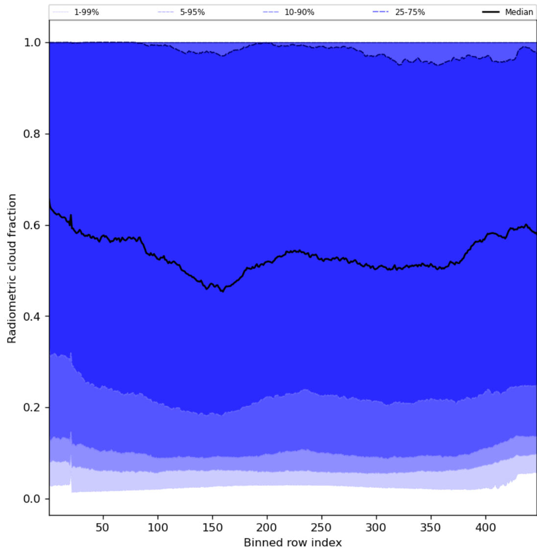
Figure 55: Along track statistics of “Radiometric cloud fraction” for 2023-10-06 to 2023-10-07
