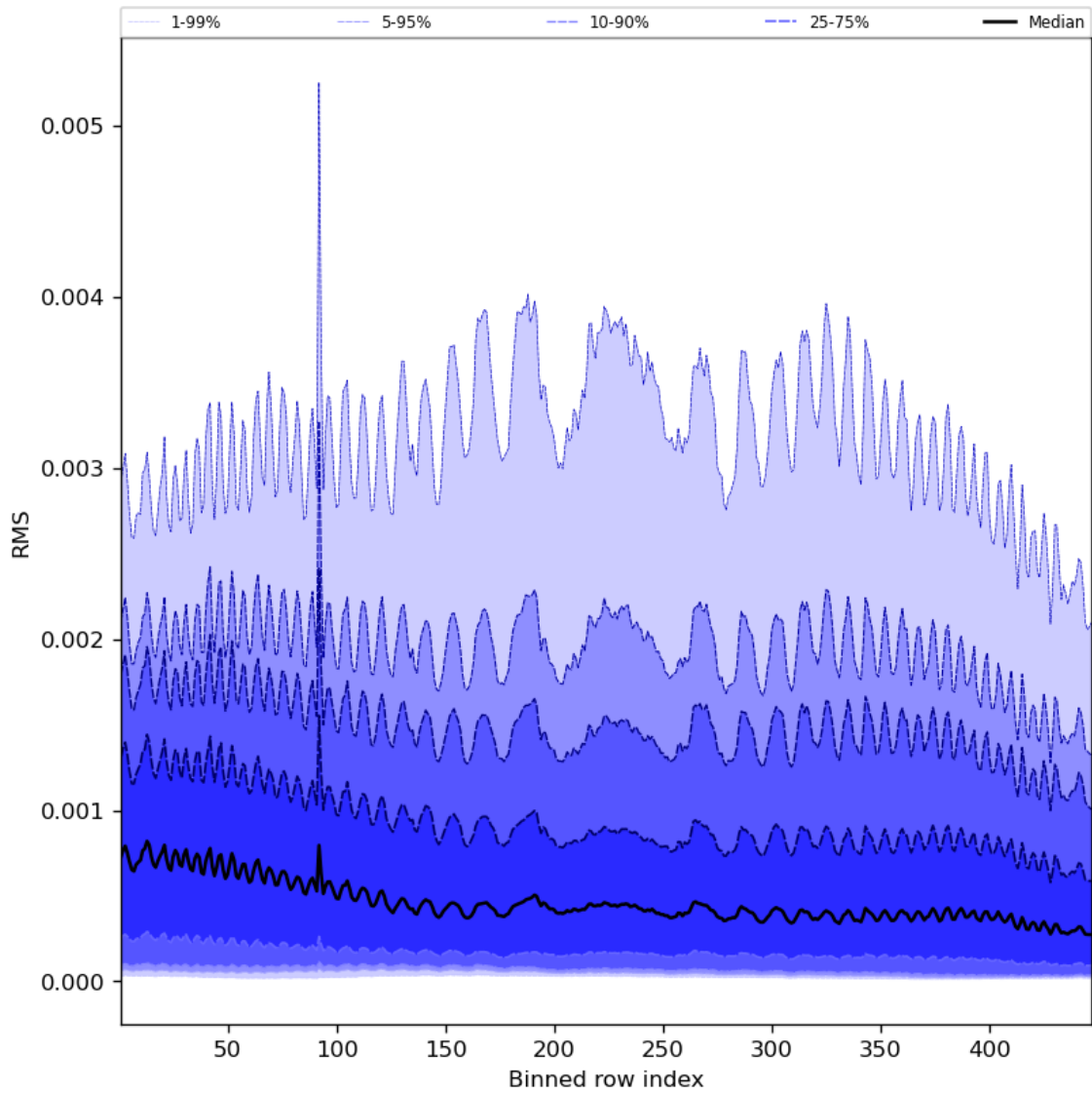
Figure 63: Along track statistics of “RMS” for 2023-10-06 to 2023-10-07
