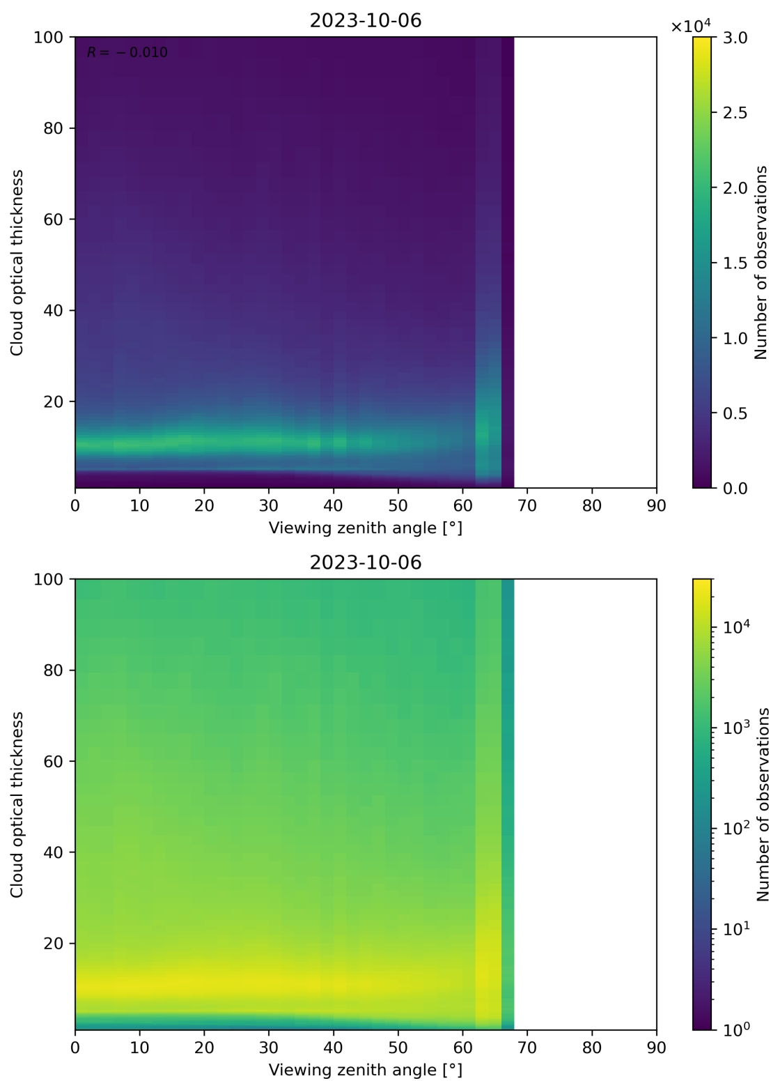
Figure 111: Scatter density plot of “Viewing zenith angle” against “Cloud optical thickness” for 2023-10-06 to 2023-10-07.
