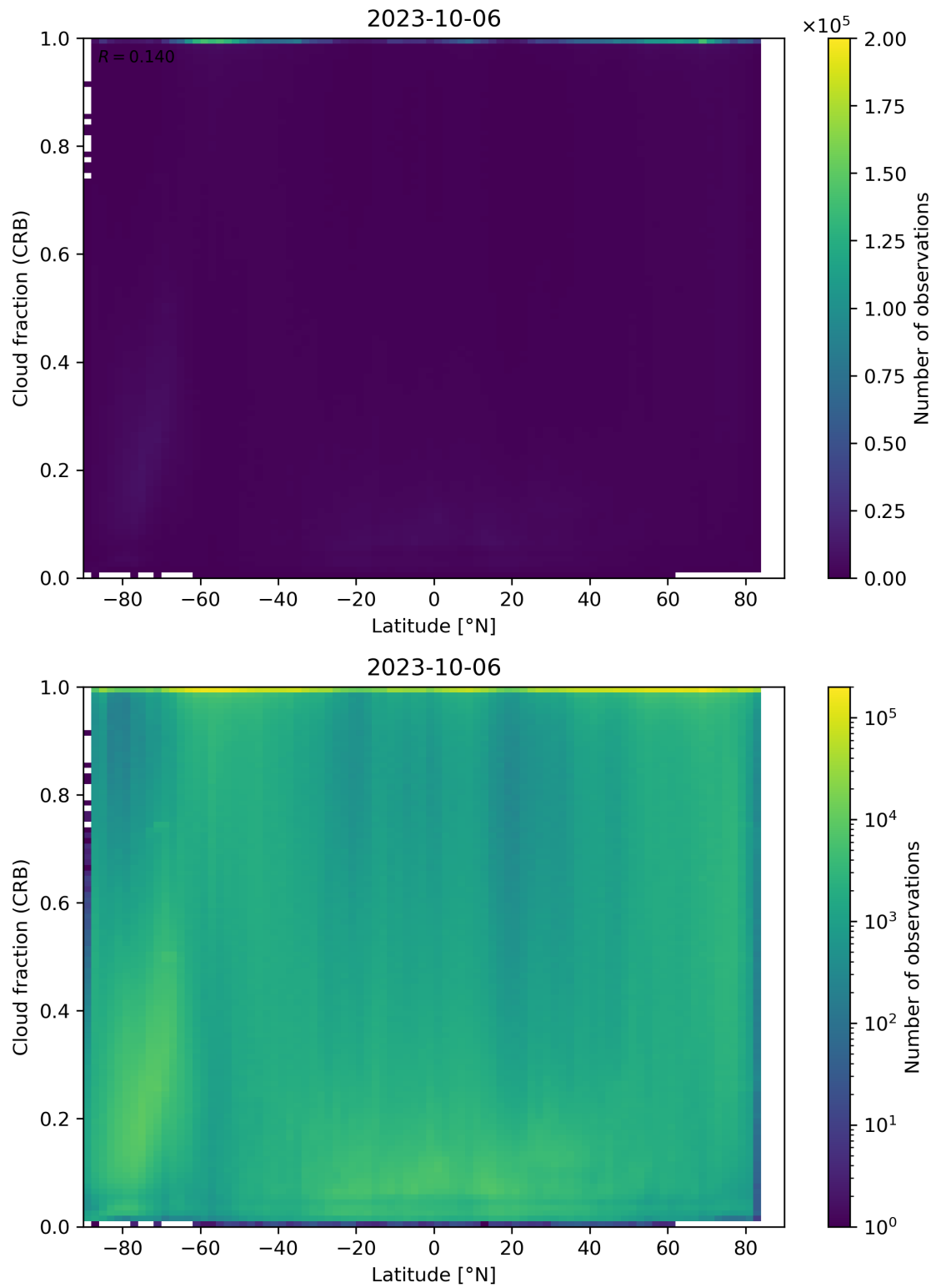
Figure 94: Scatter density plot of “Latitude” against “Cloud fraction (CRB)” for 2023-10-06 to 2023-10-07.
