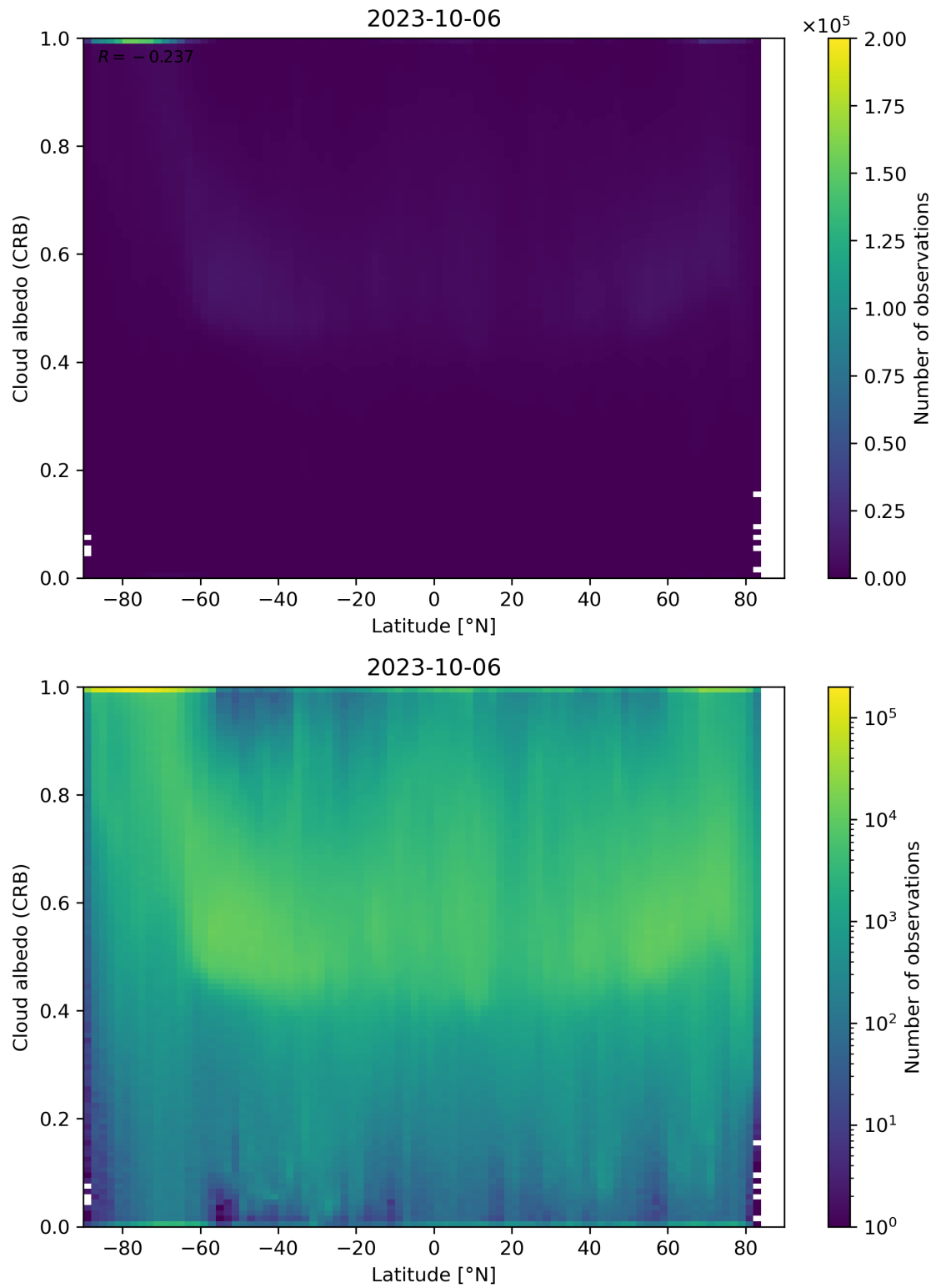
Figure 91: Scatter density plot of “Latitude” against “Cloud albedo (CRB)” for 2023-10-06 to 2023-10-07.
