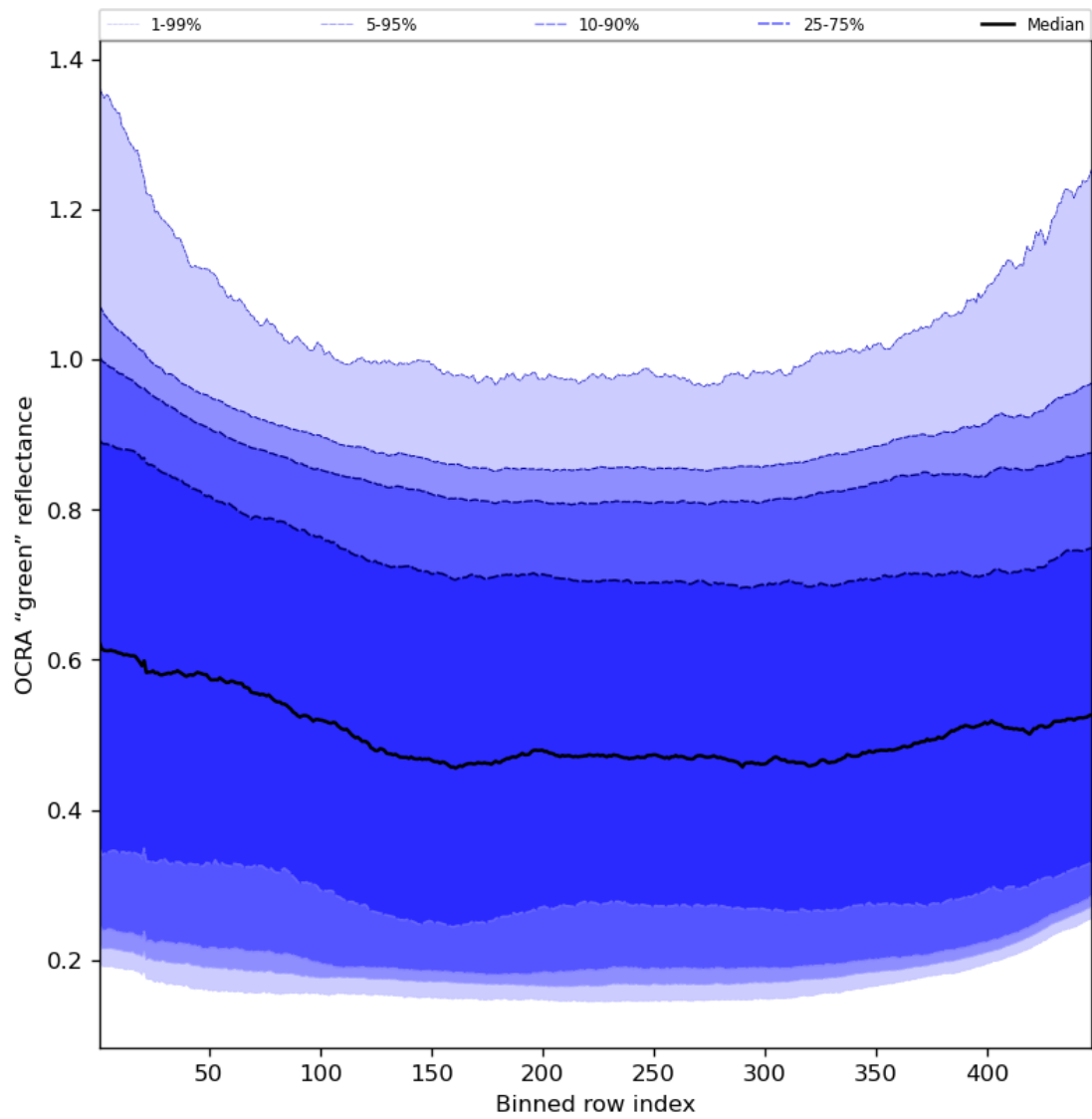
Figure 68: Along track statistics of “OCRA “green” reflectance” for 2023-10-06 to 2023-10-07
