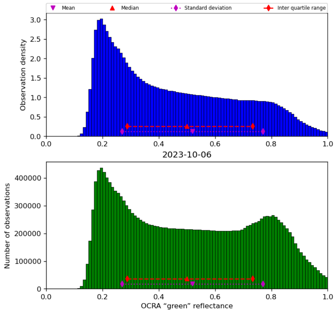
Figure 52: Histogram of “OCRA “green” reflectance” for 2023-10-06 to 2023-10-07
