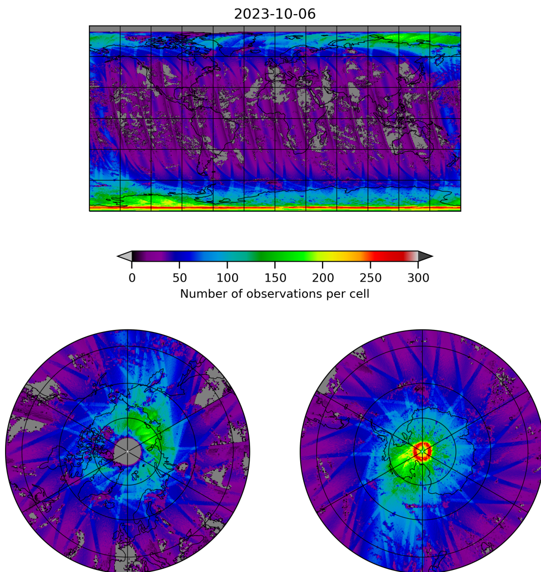
Figure 21: Map of the number of observations for 2023-10-06 to 2023-10-07
