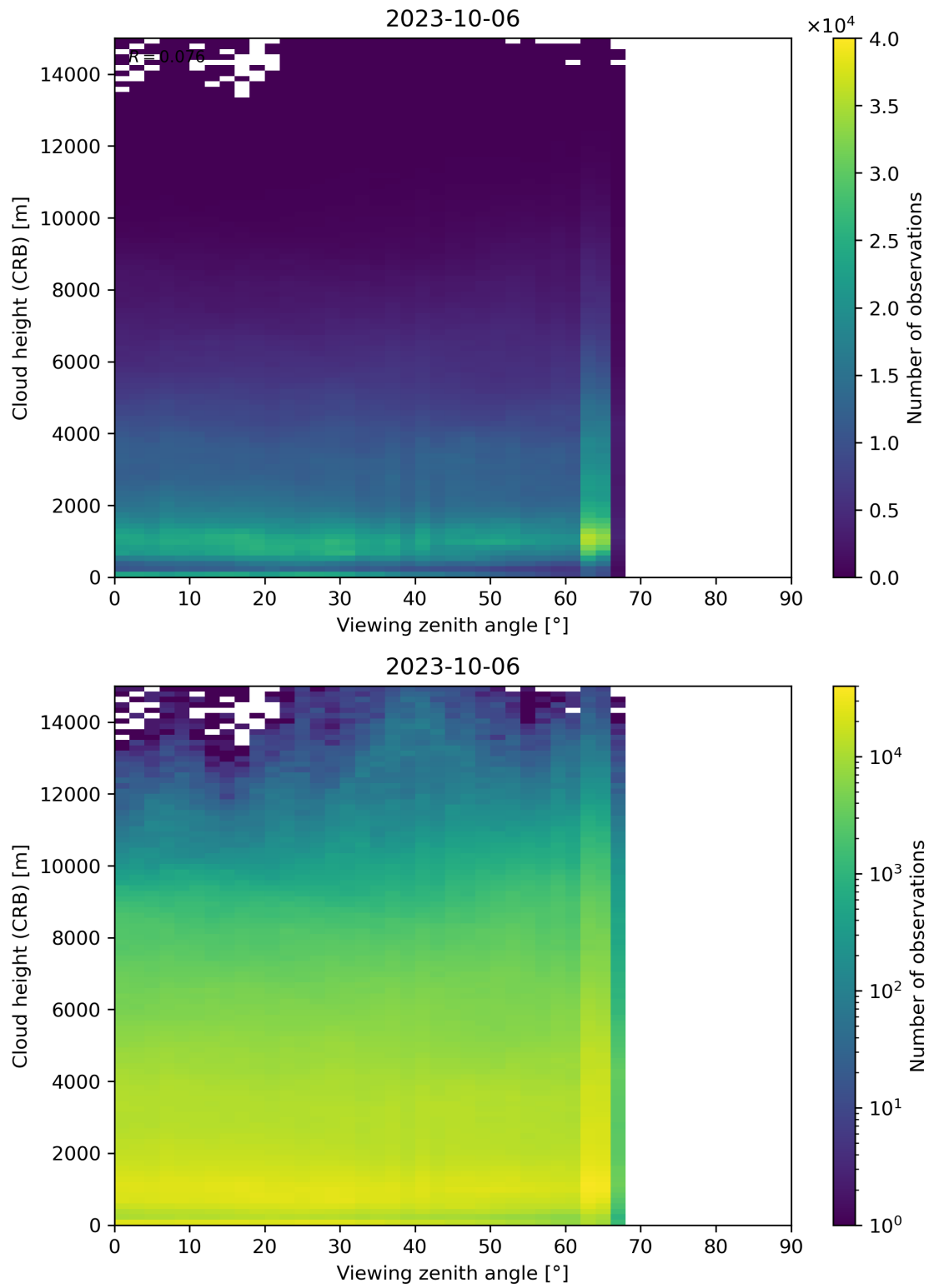
Figure 110: Scatter density plot of “Viewing zenith angle” against “Cloud height (CRB)” for 2023-10-06 to 2023-10-07.
