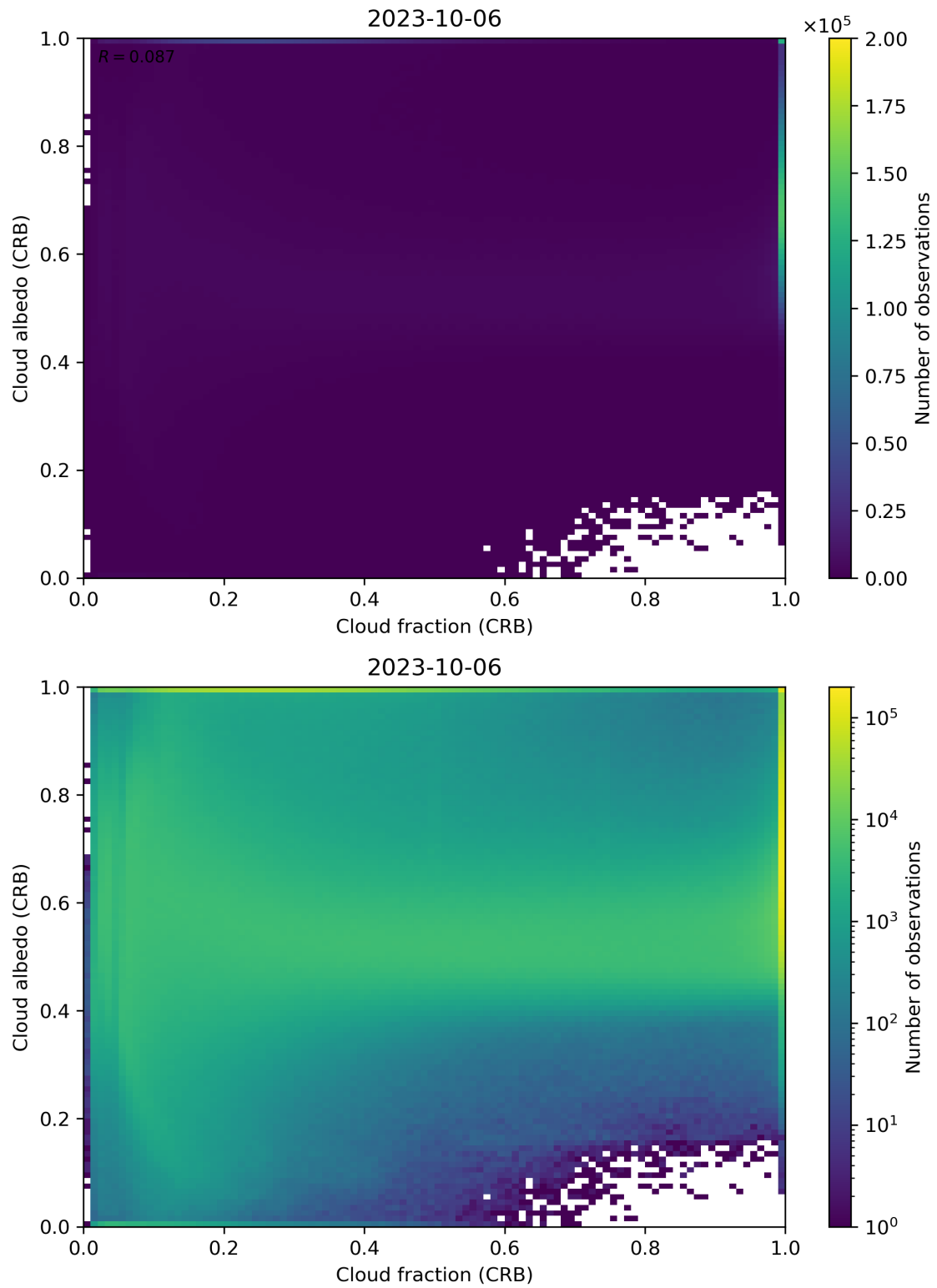
Figure 77: Scatter density plot of “Cloud fraction (CRB)” against “Cloud albedo (CRB)” for 2023-10-06 to 2023-10-07.
