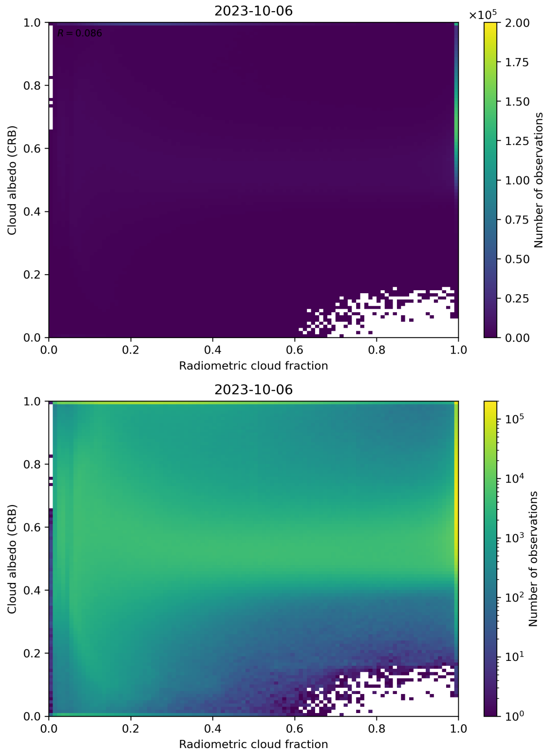
Figure 71: Scatter density plot of “Radiometric cloud fraction” against “Cloud albedo (CRB)” for 2023-10-06 to 2023-10-07.
