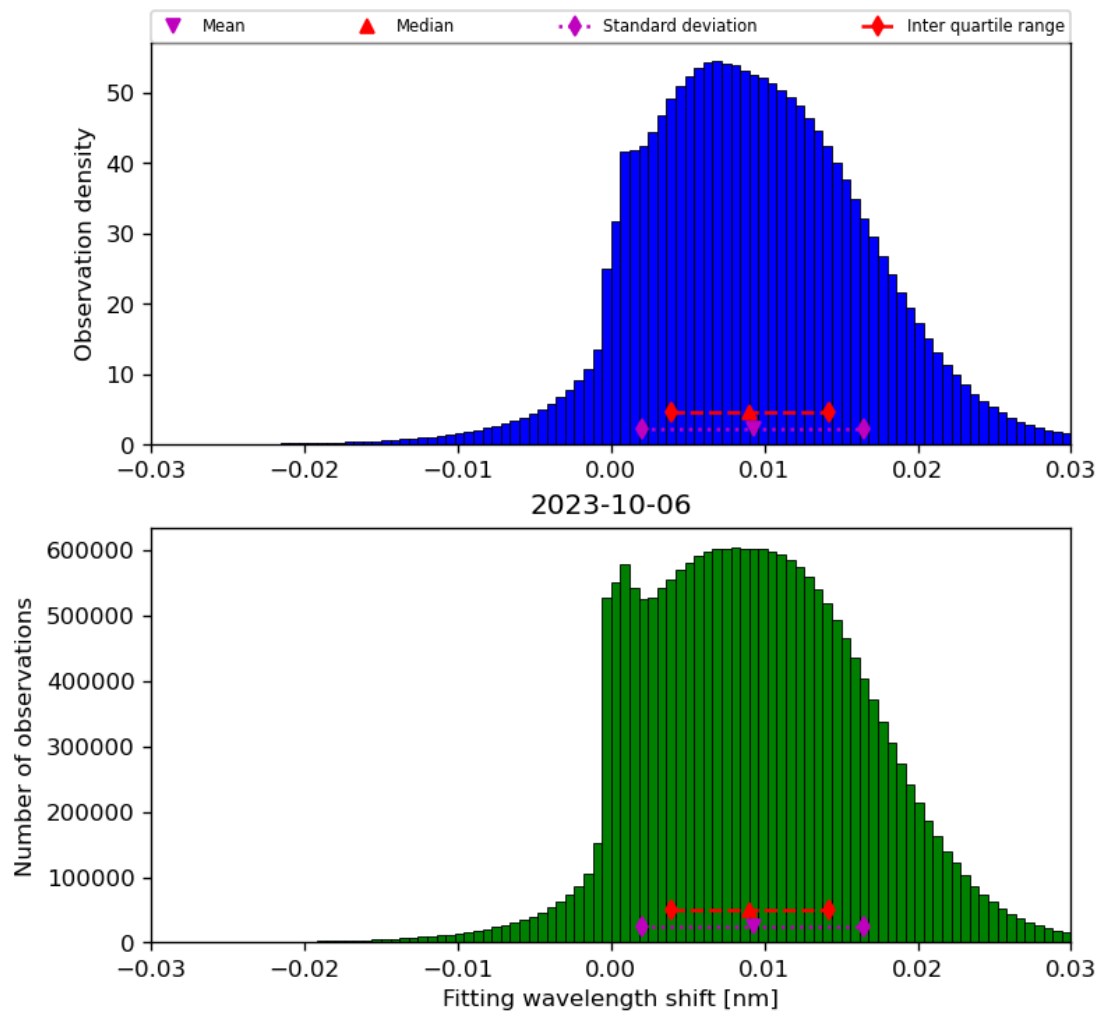
Figure 49: Histogram of “Fitting wavelength shift” for 2023-10-06 to 2023-10-07
