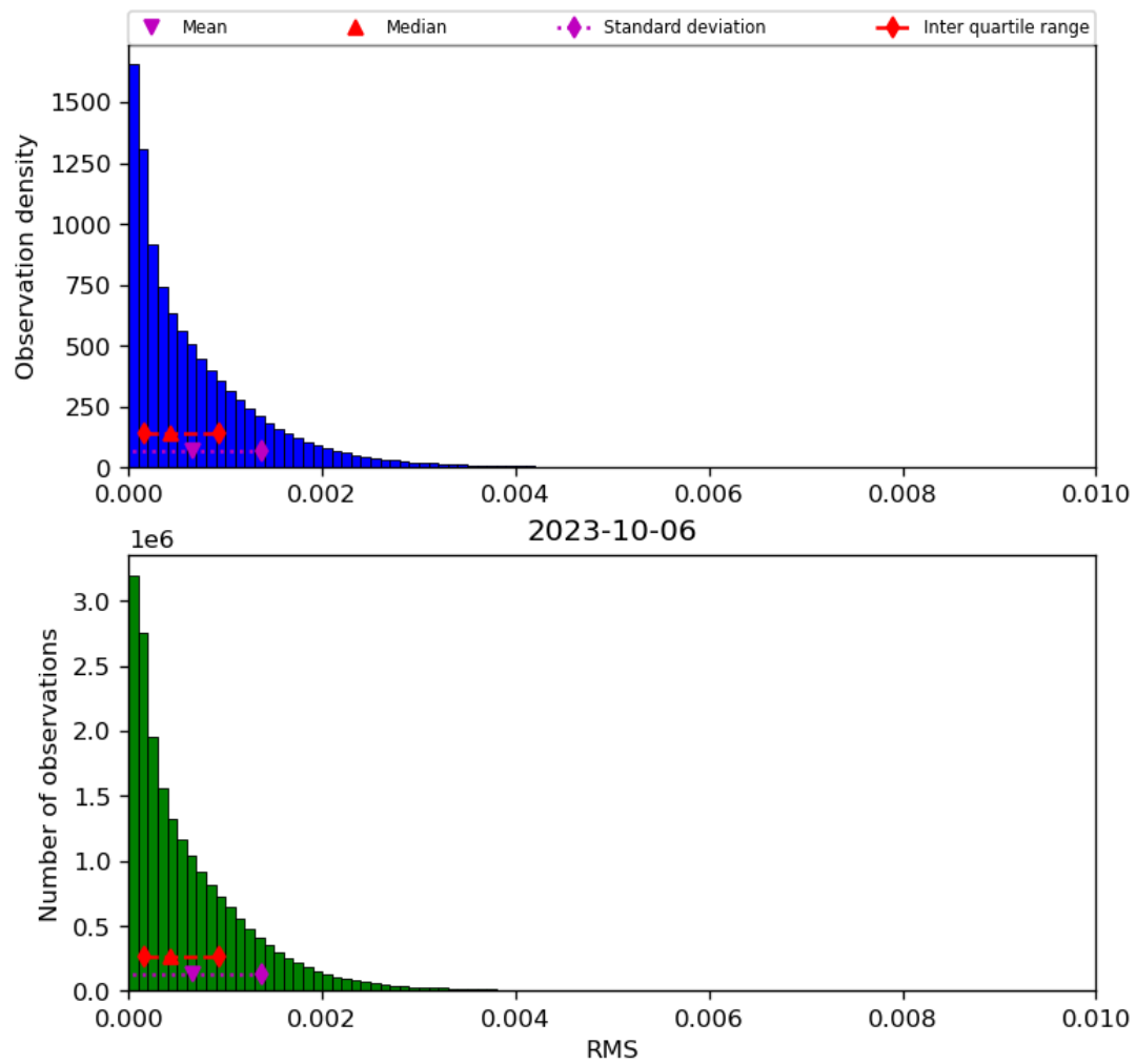
Figure 47: Histogram of “RMS” for 2023-10-06 to 2023-10-07
