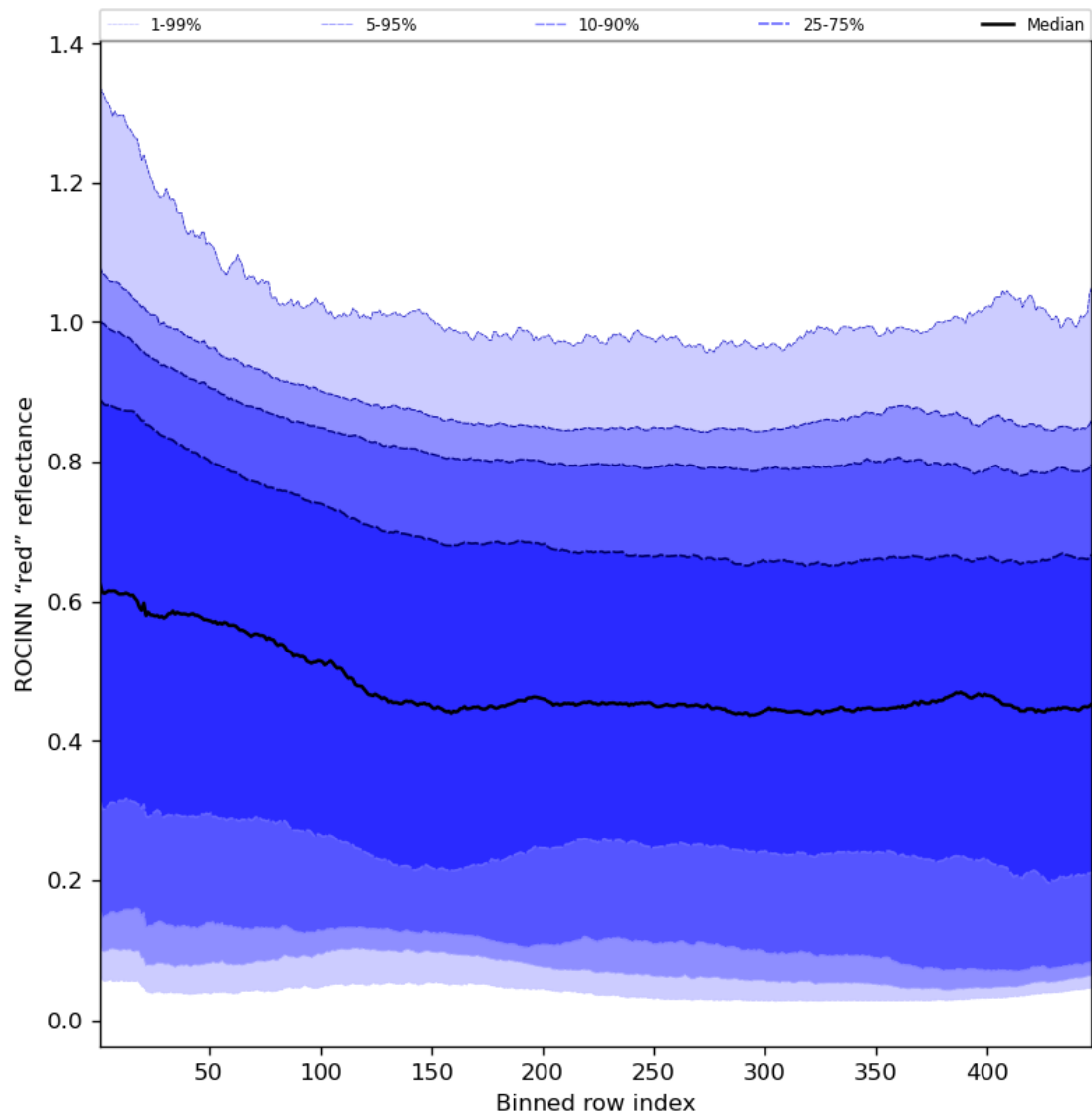
Figure 69: Along track statistics of “ROCINN “red” reflectance” for 2023-10-06 to 2023-10-07
