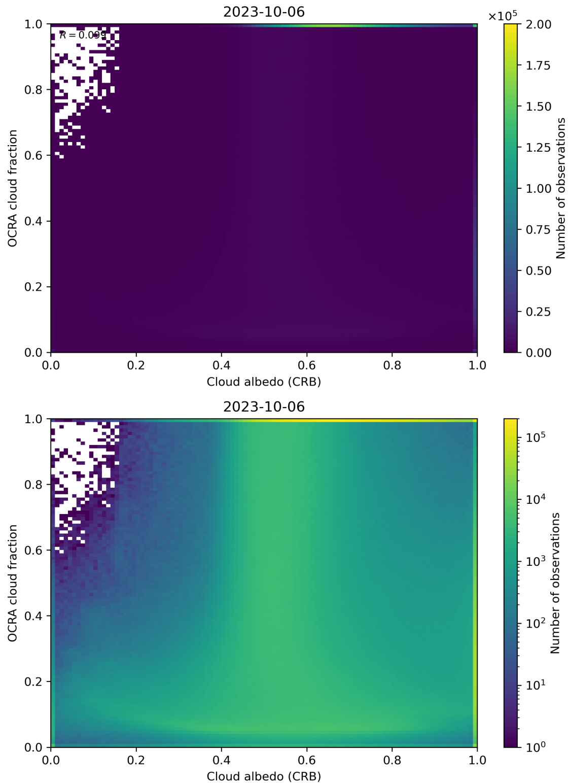
Figure 70: Scatter density plot of “Cloud albedo (CRB)” against “OCRA cloud fraction” for 2023-10-06 to 2023-10-07.
