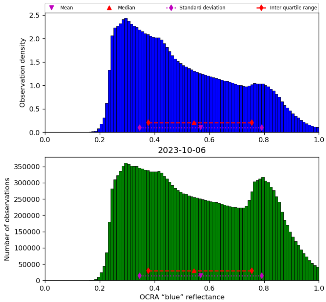
Figure 51: Histogram of “OCRA “blue” reflectance” for 2023-10-06 to 2023-10-07
