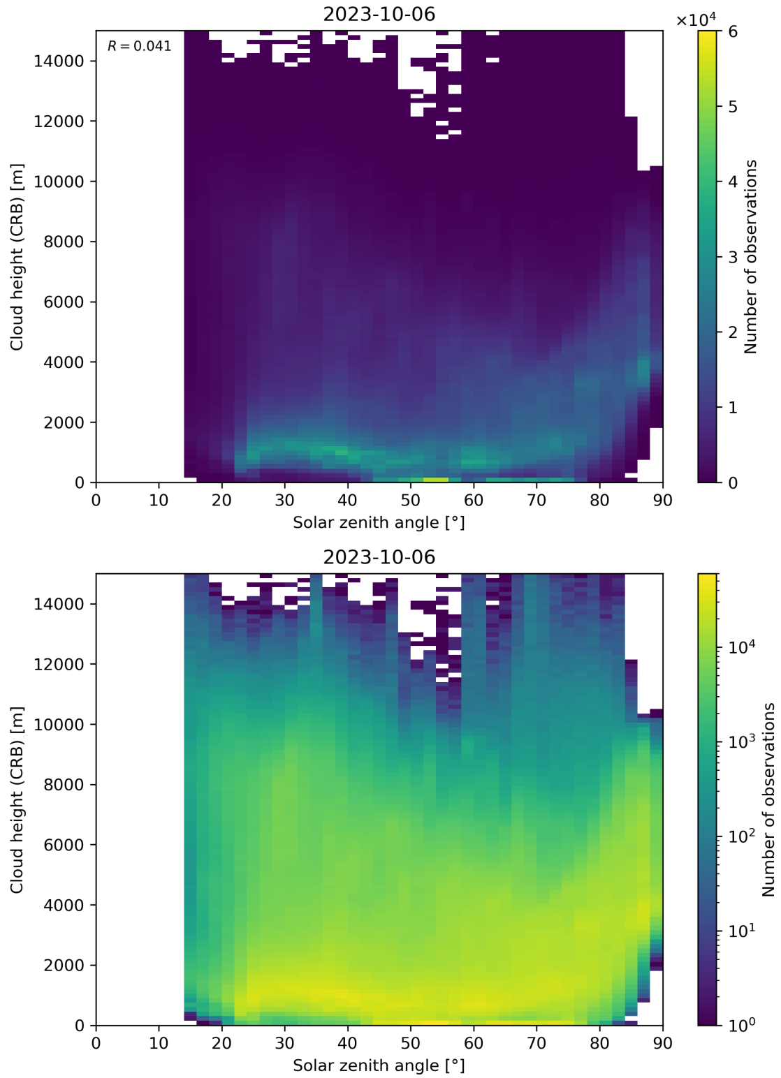
Figure 102: Scatter density plot of “Solar zenith angle” against “Cloud height (CRB)” for 2023-10-06 to 2023-10-07.
