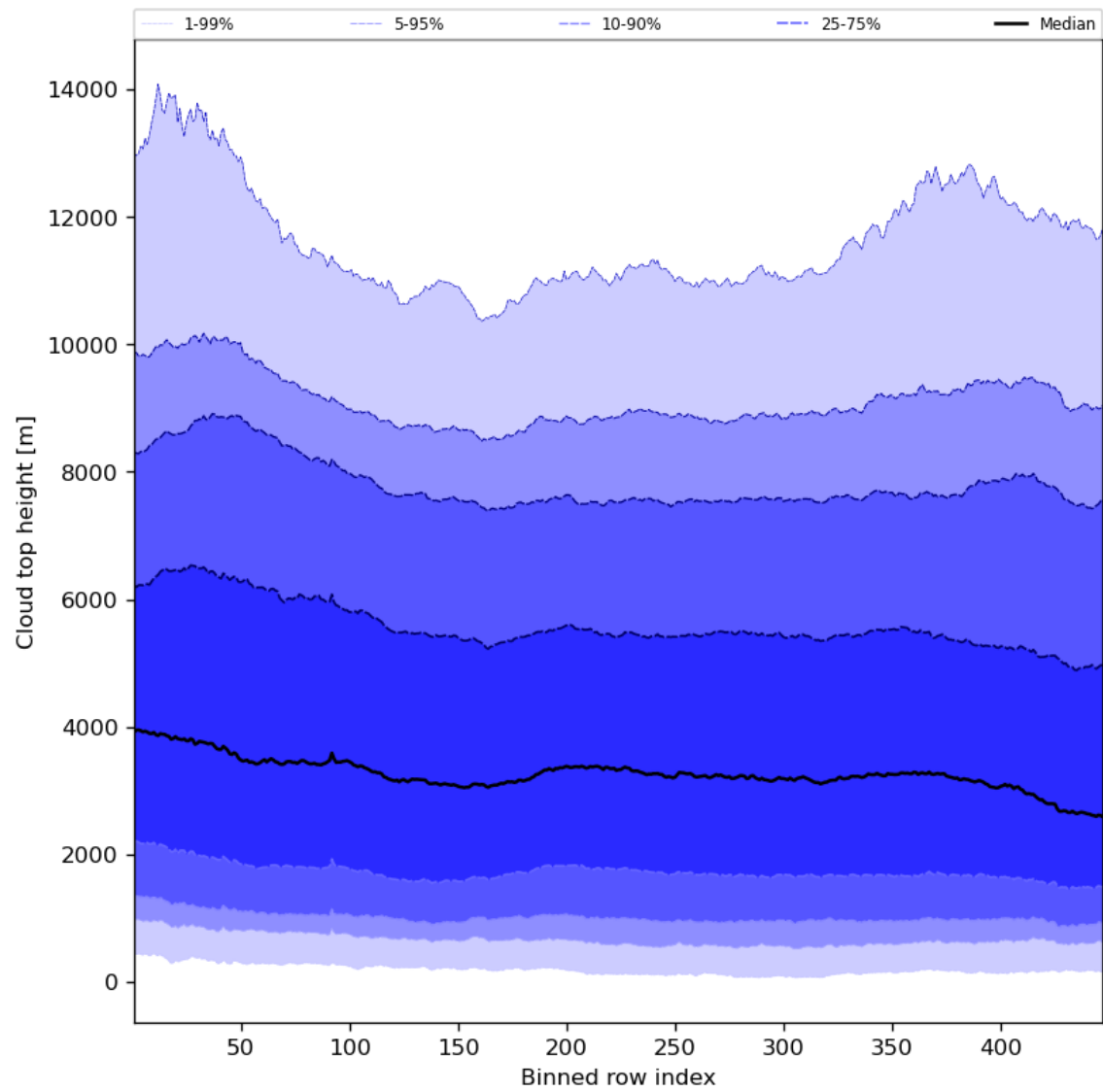
Figure 56: Along track statistics of “Cloud top height” for 2023-10-06 to 2023-10-07
