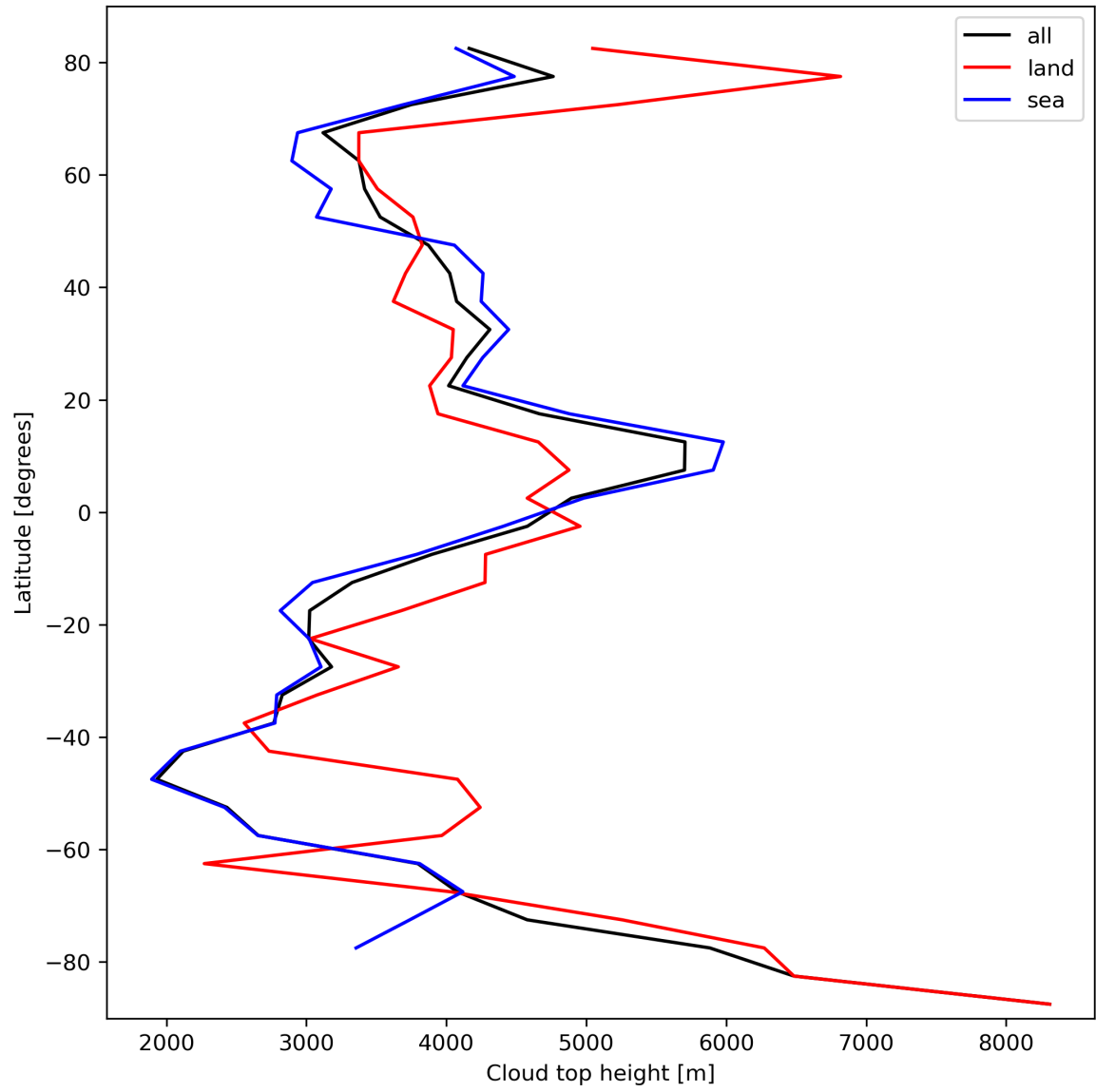
Figure 24: Zonal average of “Cloud top height” for 2023-10-06 to 2023-10-07.
