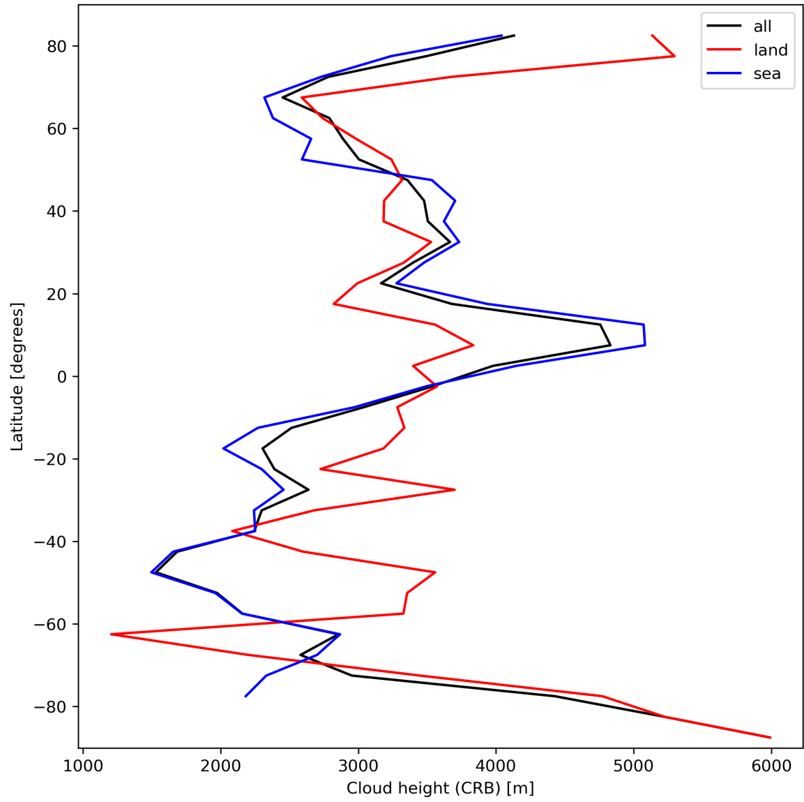
Figure 27: Zonal average of “Cloud height (CRB)” for 2023-10-06 to 2023-10-07.
