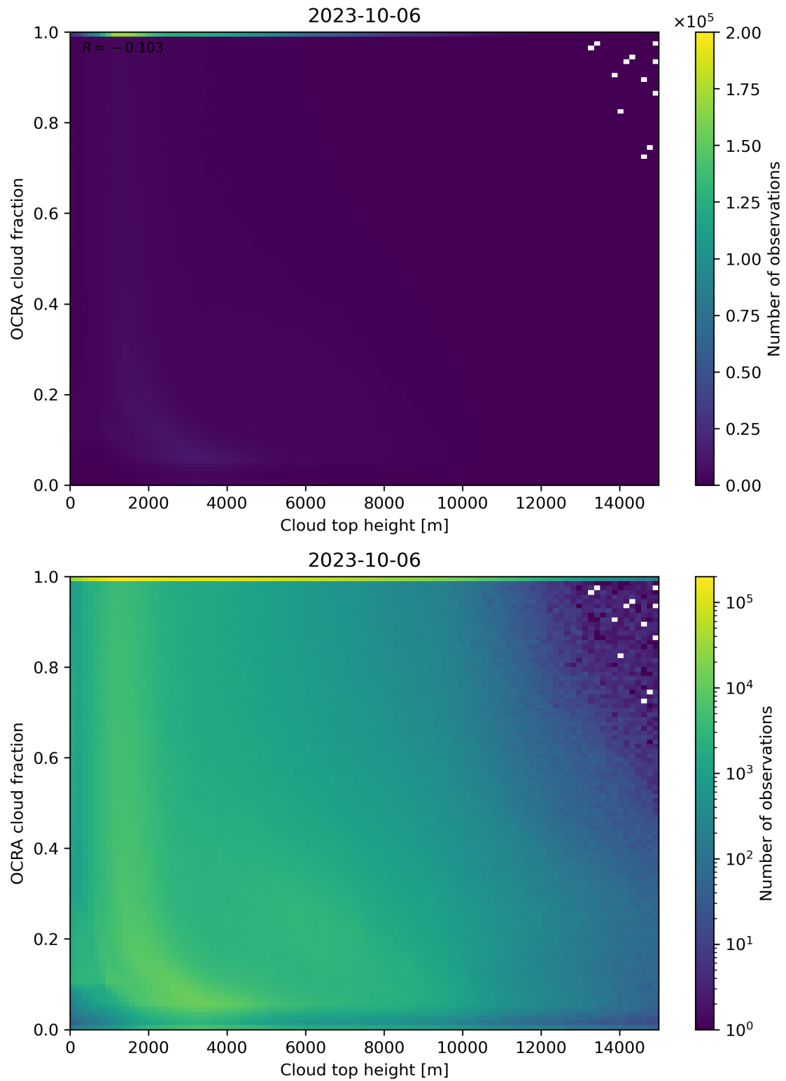
Figure 87: Scatter density plot of “Cloud top height” against “OCRA cloud fraction” for 2023-10-06 to 2023-10-07.
