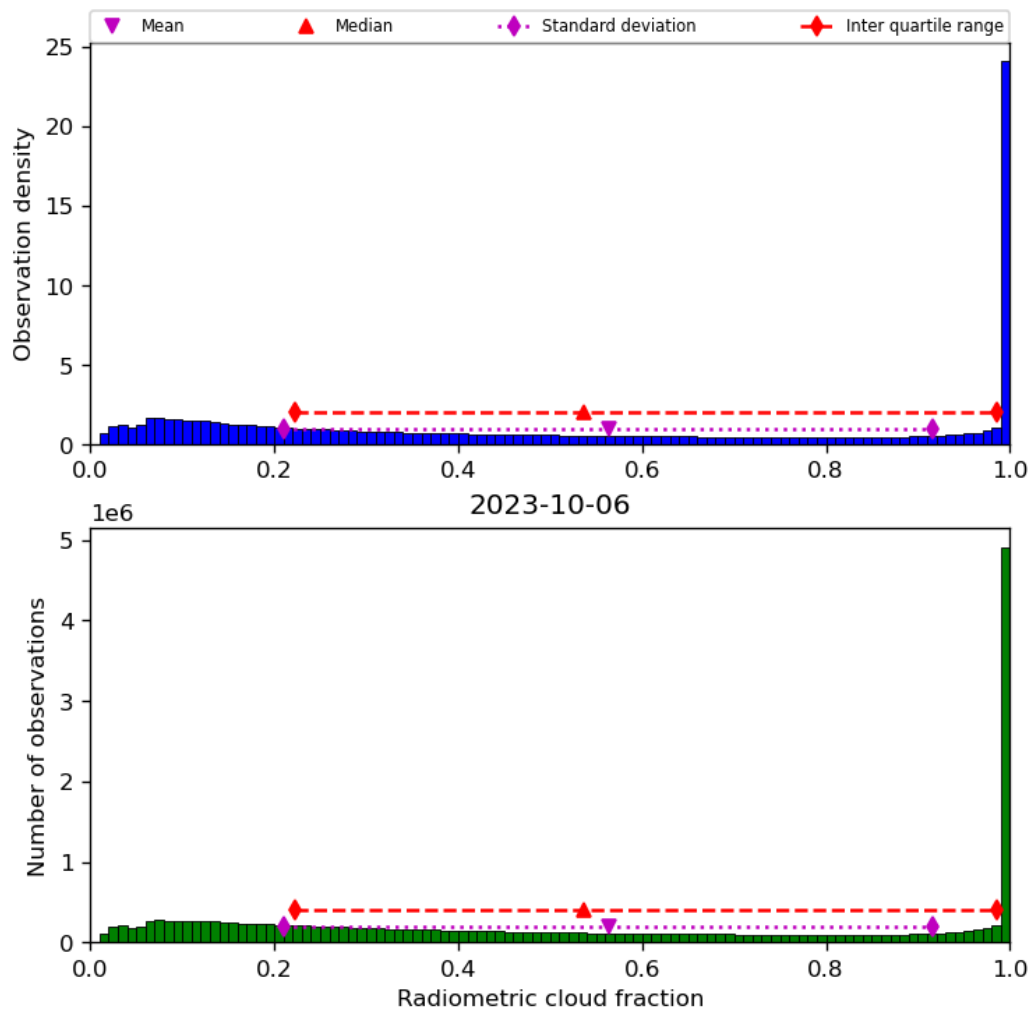
Figure 39: Histogram of “Radiometric cloud fraction” for 2023-10-06 to 2023-10-07
