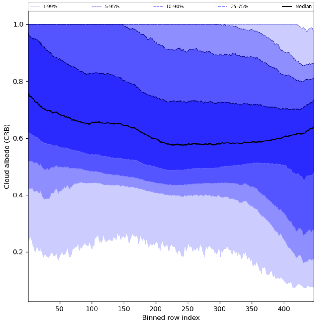
Figure 60: Along track statistics of “Cloud albedo (CRB)” for 2023-10-06 to 2023-10-07
