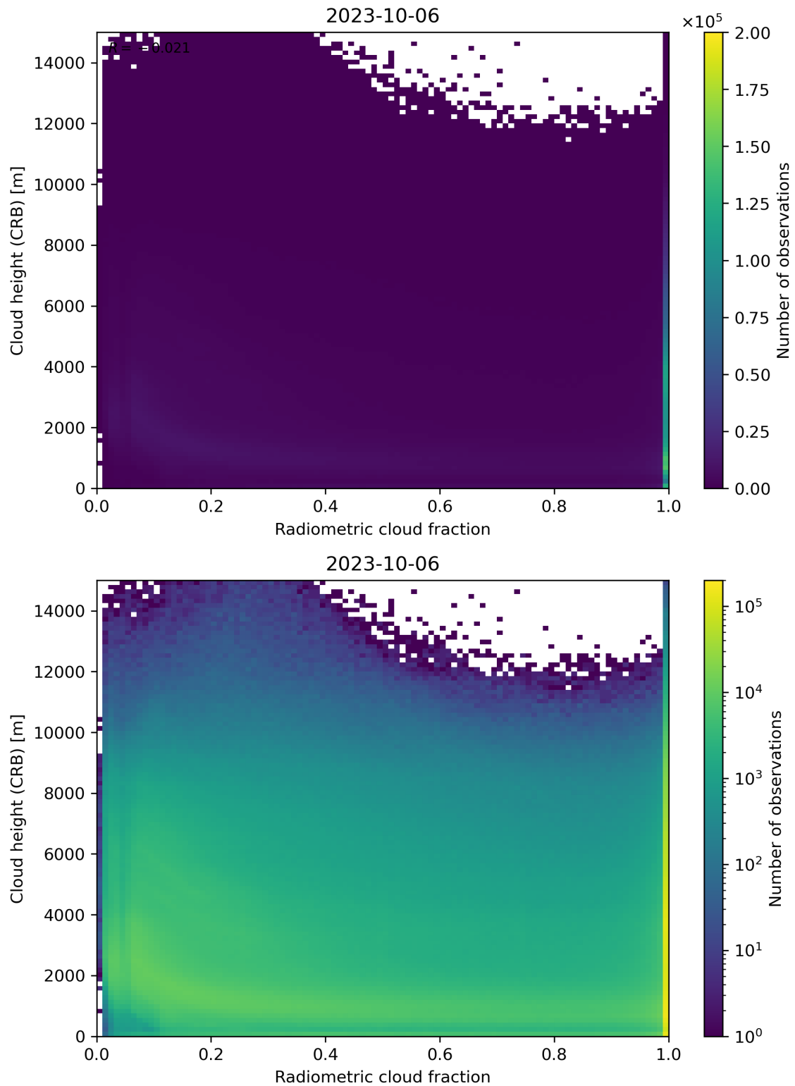
Figure 74: Scatter density plot of “Radiometric cloud fraction” against “Cloud height (CRB)” for 2023-10-06 to 2023-10-07.
