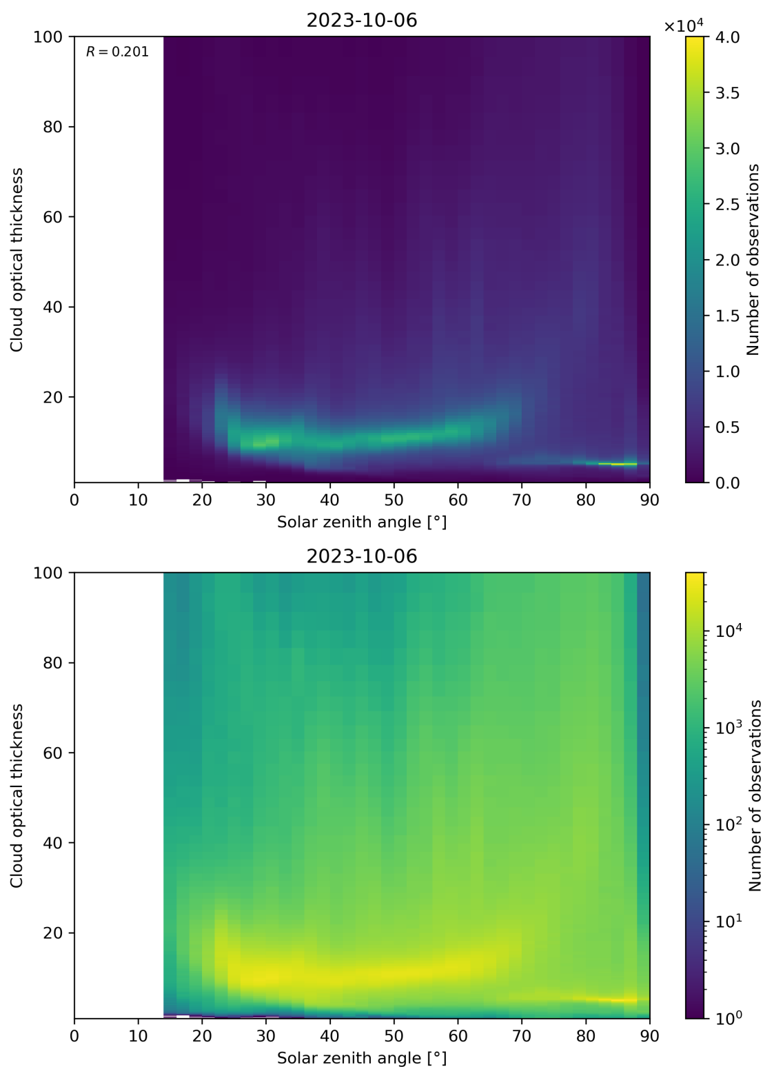
Figure 103: Scatter density plot of “Solar zenith angle” against “Cloud optical thickness” for 2023-10-06 to 2023-10-07.
