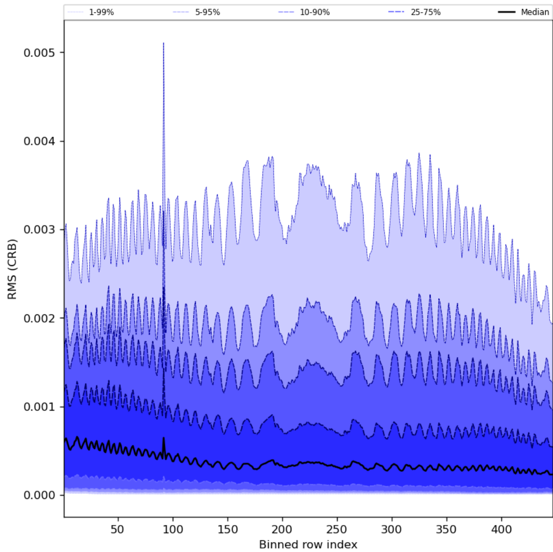
Figure 64: Along track statistics of “RMS (CRB)” for 2023-10-06 to 2023-10-07
