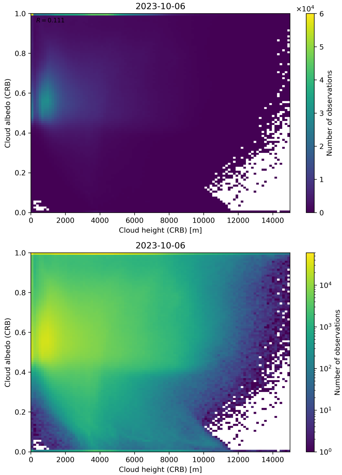
Figure 80: Scatter density plot of “Cloud height (CRB)” against “Cloud albedo (CRB)” for 2023-10-06 to 2023-10-07.
