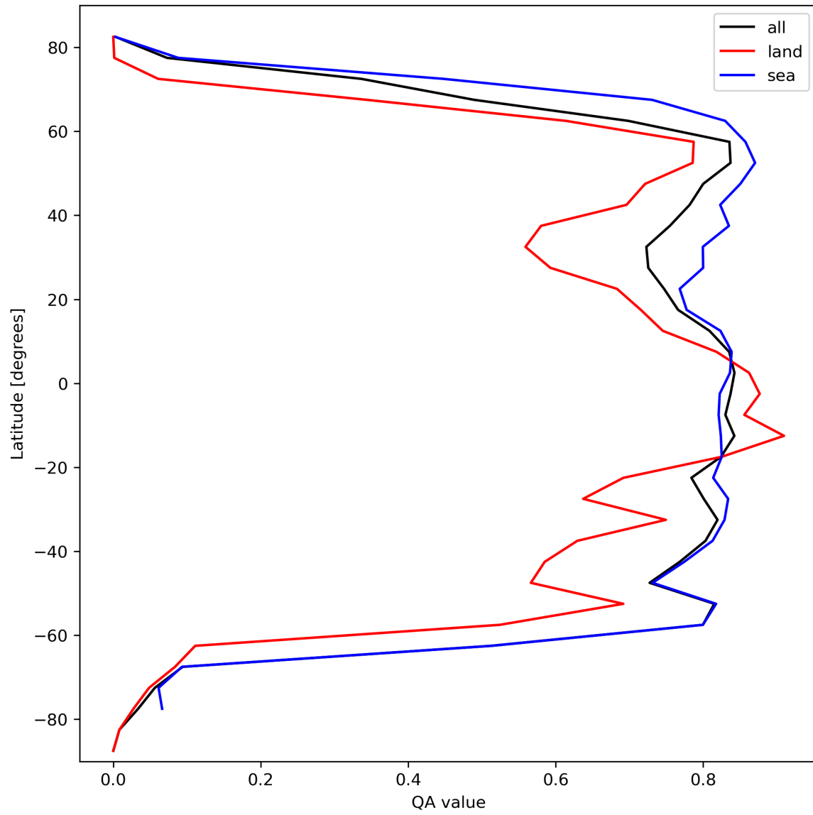
Figure 22: Zonal average of “QA value” for 2023-10-06 to 2023-10-07.
