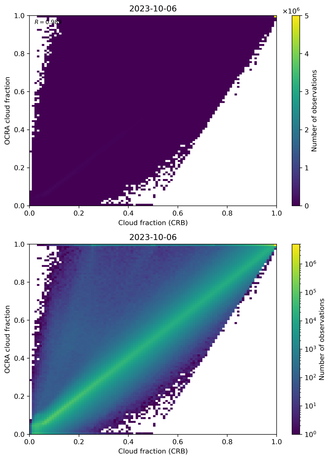
Figure 78: Scatter density plot of “Cloud fraction (CRB)” against “OCRA cloud fraction” for 2023-10-06 to 2023-10-07.
