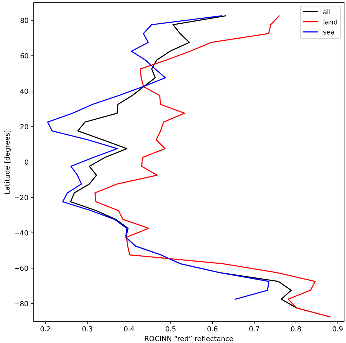
Figure 37: Zonal average of “ROCINN “red” reflectance” for 2023-10-06 to 2023-10-07.
