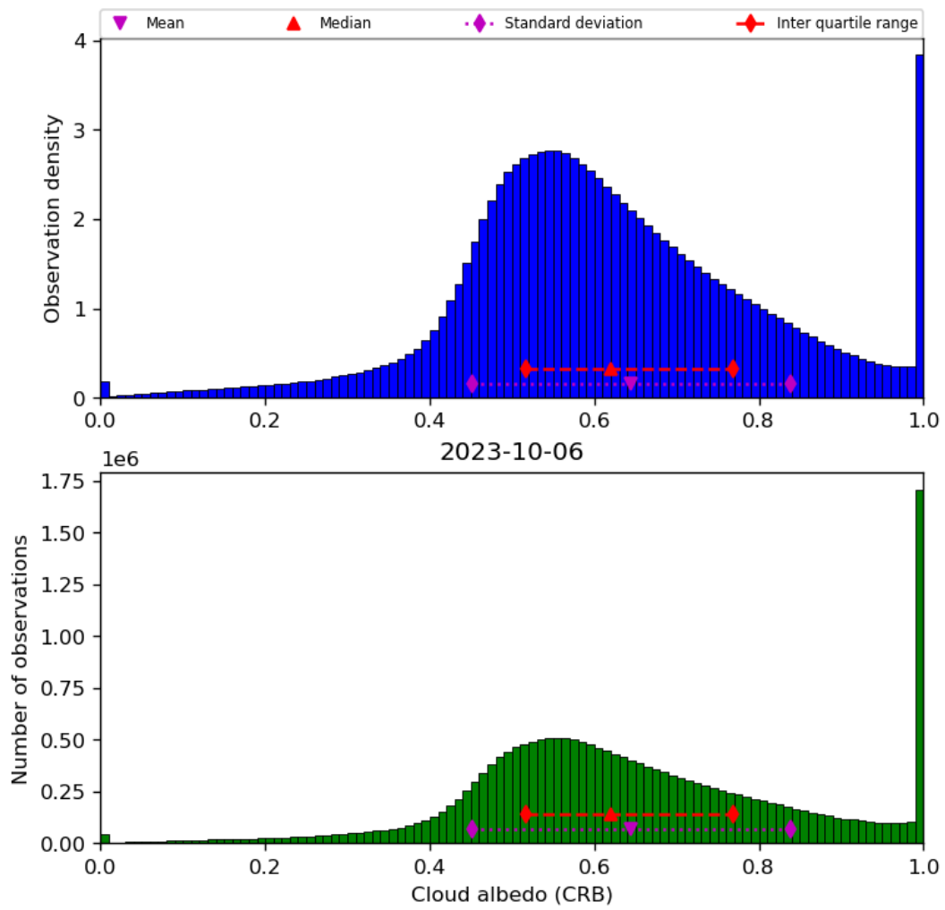
Figure 44: Histogram of “Cloud albedo (CRB)” for 2023-10-06 to 2023-10-07
