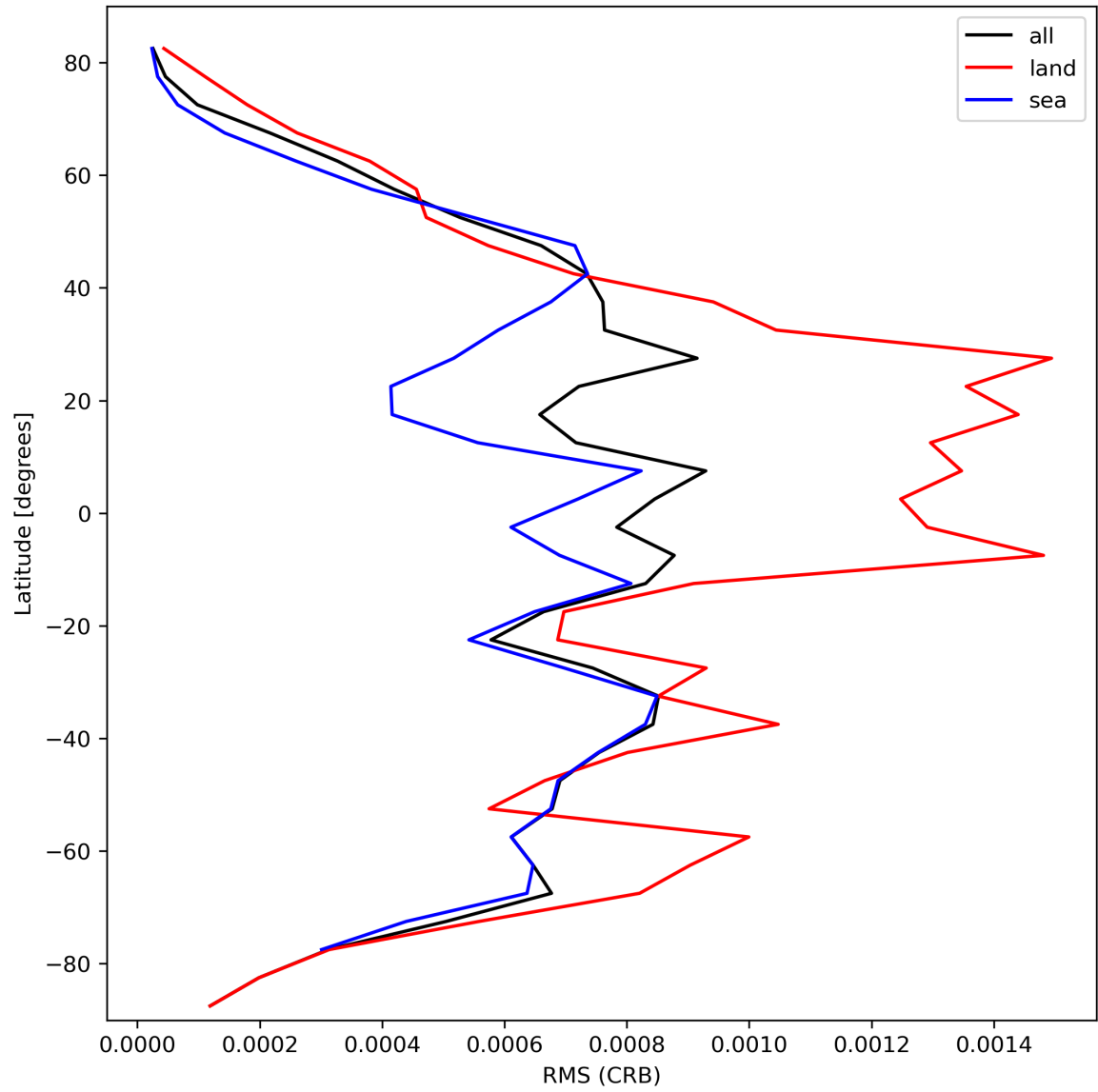
Figure 32: Zonal average of “RMS (CRB)” for 2023-10-06 to 2023-10-07.
