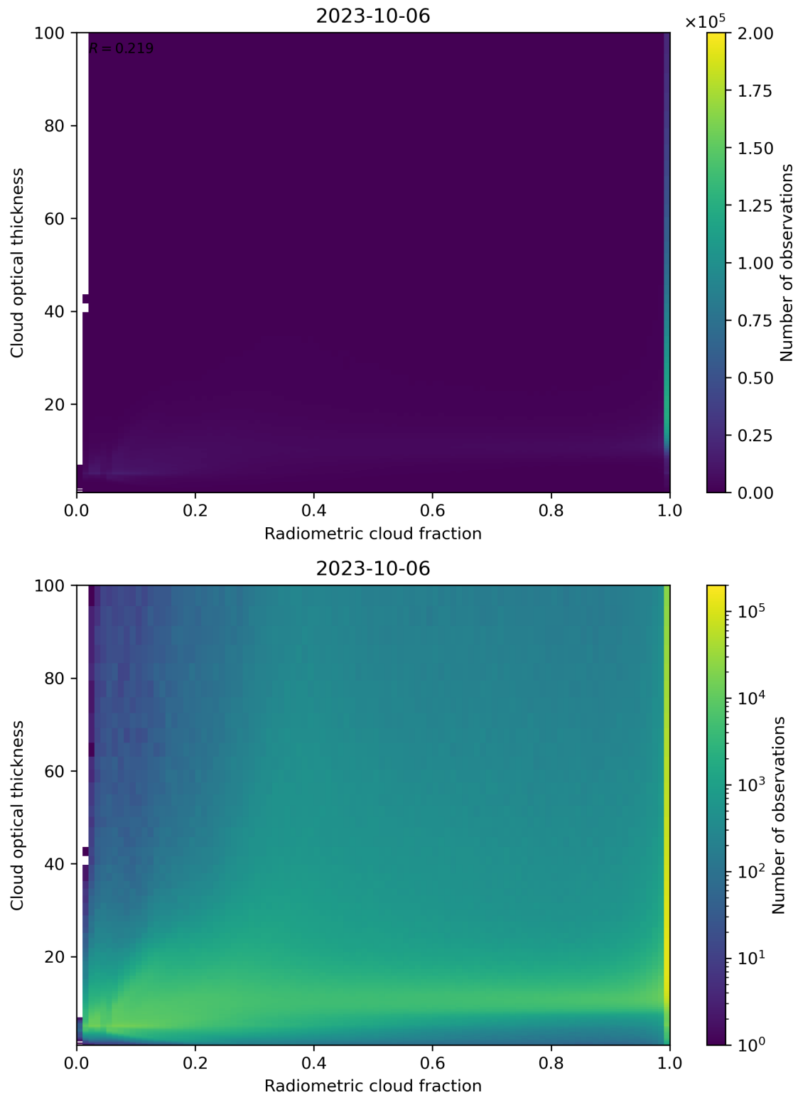
Figure 75: Scatter density plot of “Radiometric cloud fraction” against “Cloud optical thickness” for 2023-10-06 to 2023-10-07.
