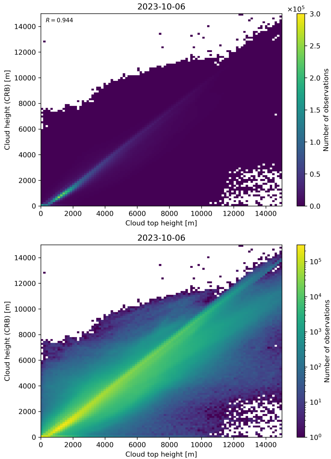
Figure 89: Scatter density plot of “Cloud top height” against “Cloud height (CRB)” for 2023-10-06 to 2023-10-07.
