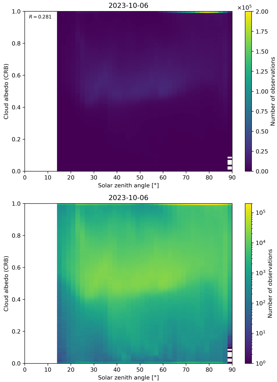
Figure 98: Scatter density plot of “Solar zenith angle” against “Cloud albedo (CRB)” for 2023-10-06 to 2023-10-07.
