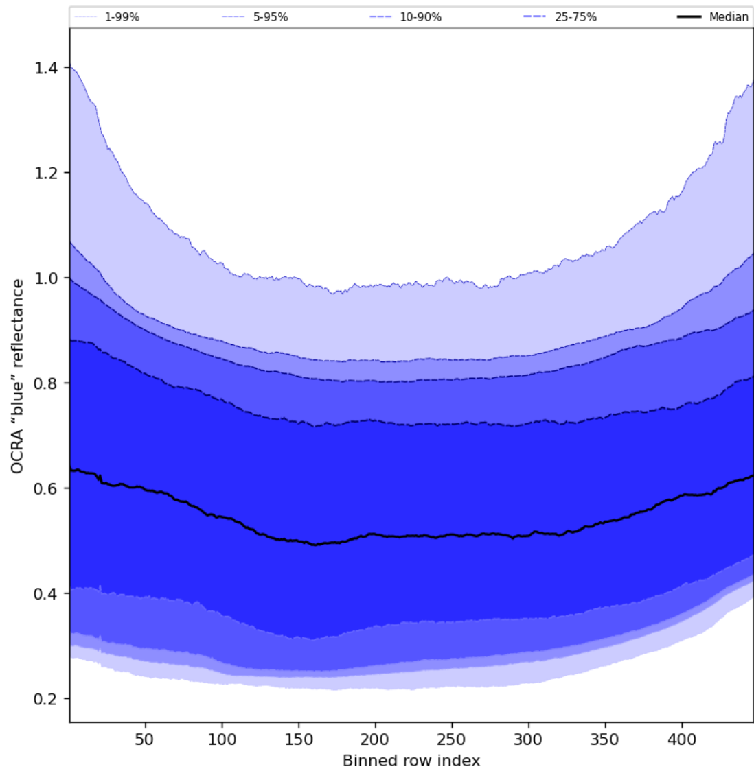
Figure 67: Along track statistics of “OCRA “blue” reflectance” for 2023-10-06 to 2023-10-07
