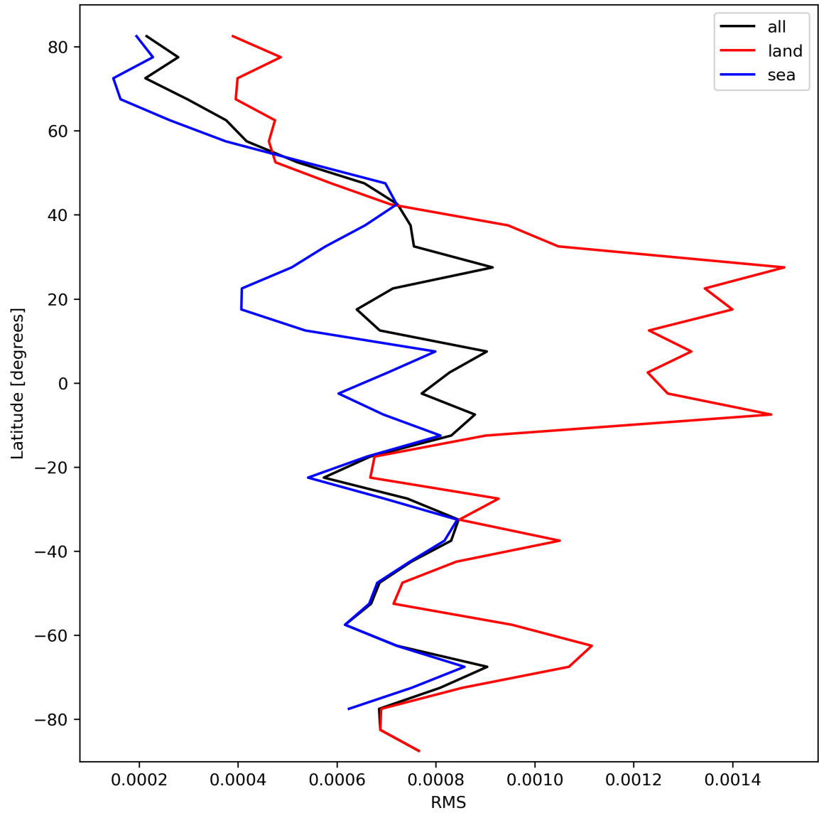
Figure 31: Zonal average of “RMS” for 2023-10-06 to 2023-10-07.
