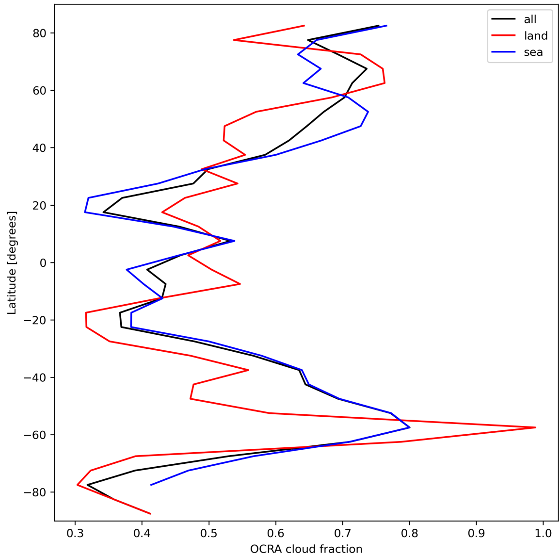
Figure 34: Zonal average of “OCRA cloud fraction” for 2023-10-06 to 2023-10-07.
