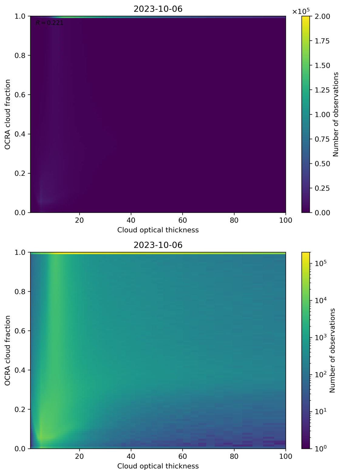
Figure 83: Scatter density plot of “Cloud optical thickness” against “OCRA cloud fraction” for 2023-10-06 to 2023-10-07.
