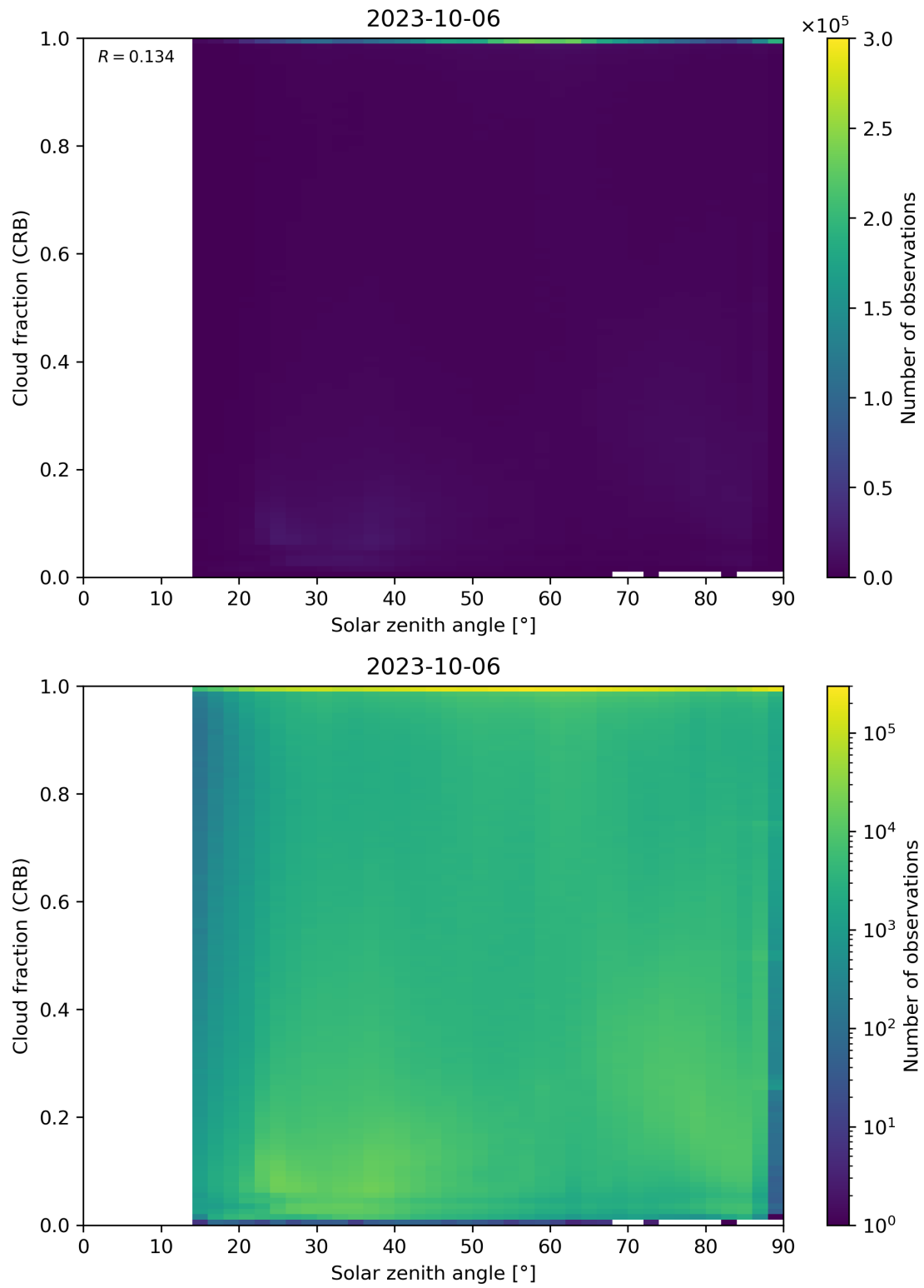
Figure 101: Scatter density plot of “Solar zenith angle” against “Cloud fraction (CRB)” for 2023-10-06 to 2023-10-07.
