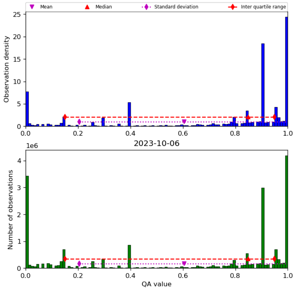
Figure 38: Histogram of “QA value” for 2023-10-06 to 2023-10-07
