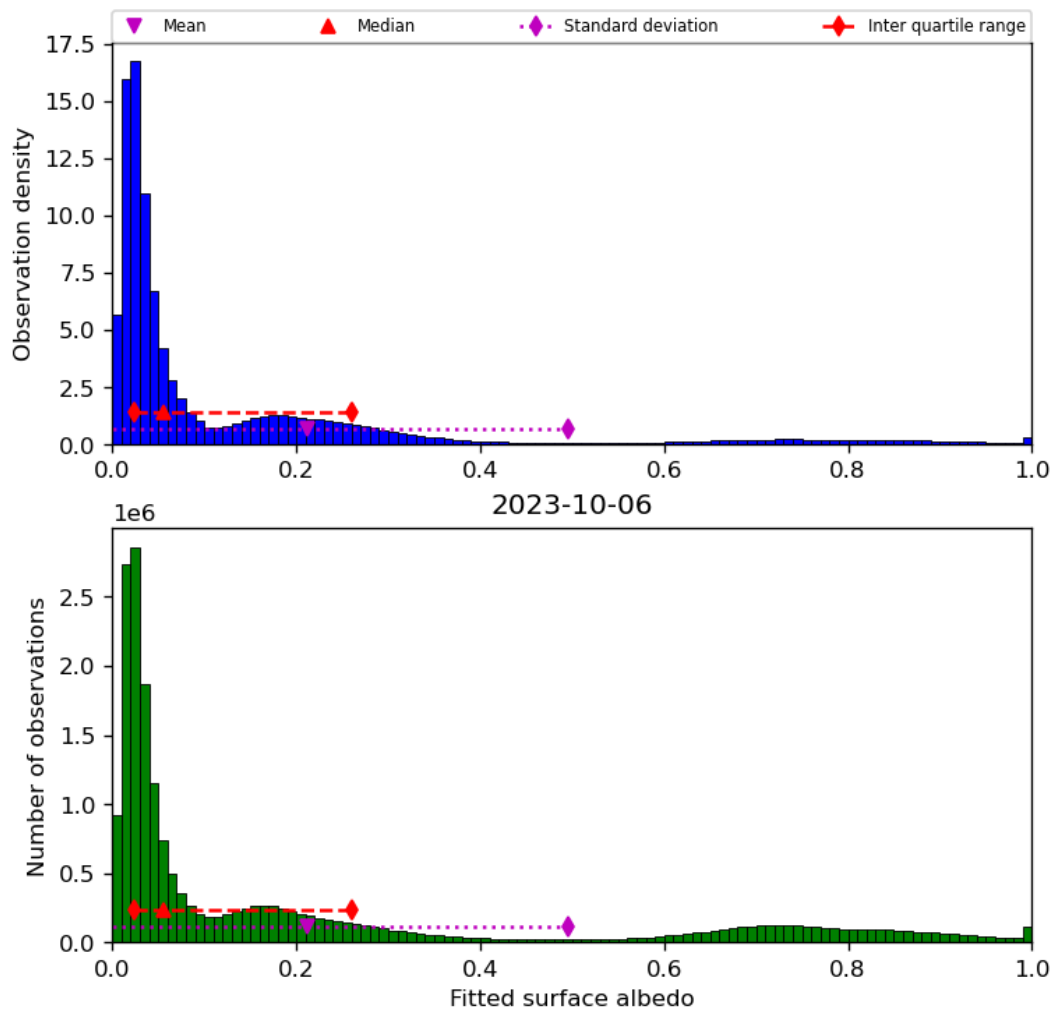
Figure 45: Histogram of “Fitted surface albedo” for 2023-10-06 to 2023-10-07
