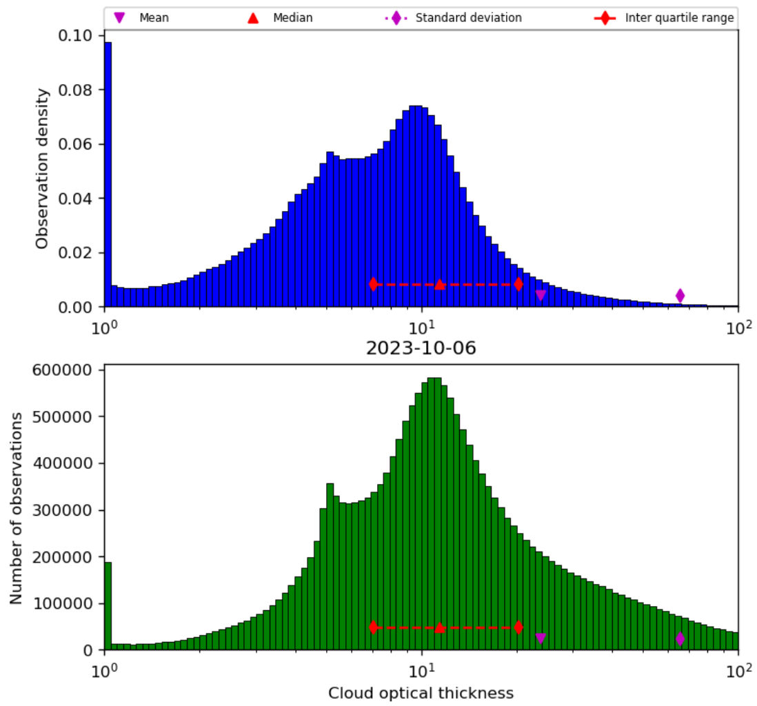
Figure 41: Histogram of “Cloud optical thickness” for 2023-10-06 to 2023-10-07
