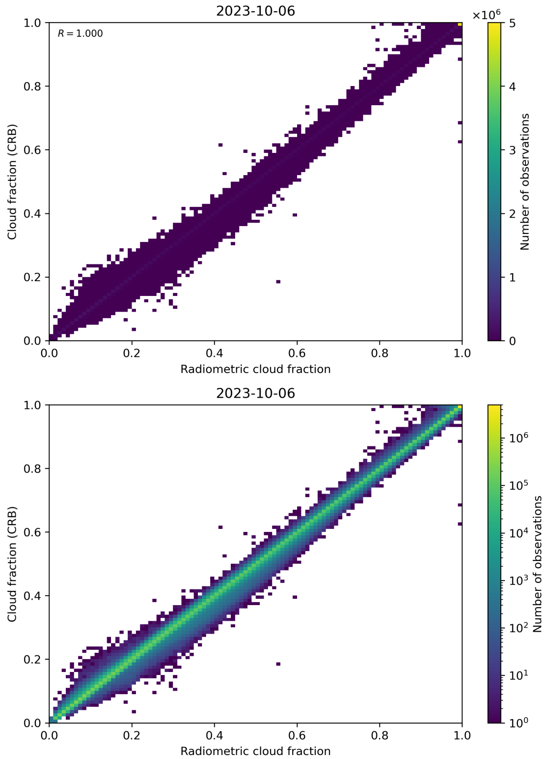
Figure 73: Scatter density plot of “Radiometric cloud fraction” against “Cloud fraction (CRB)” for 2023-10-06 to 2023-10-07.
