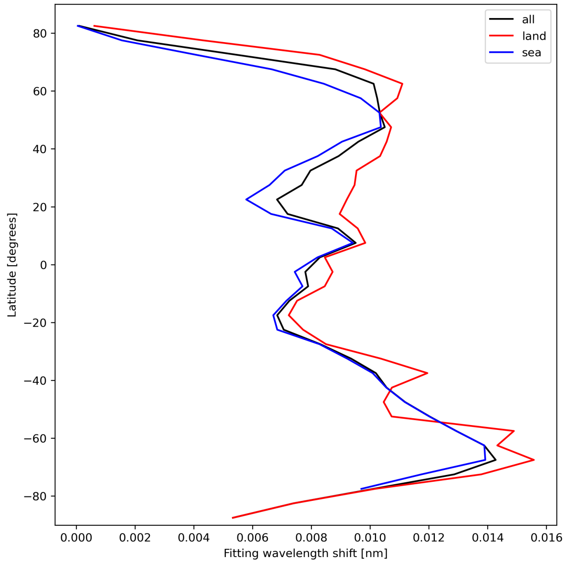
Figure 33: Zonal average of “Fitting wavelength shift” for 2023-10-06 to 2023-10-07.
