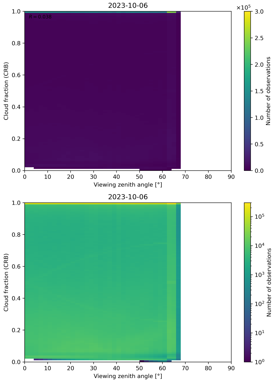
Figure 109: Scatter density plot of “Viewing zenith angle” against “Cloud fraction (CRB)” for 2023-10-06 to 2023-10-07.
