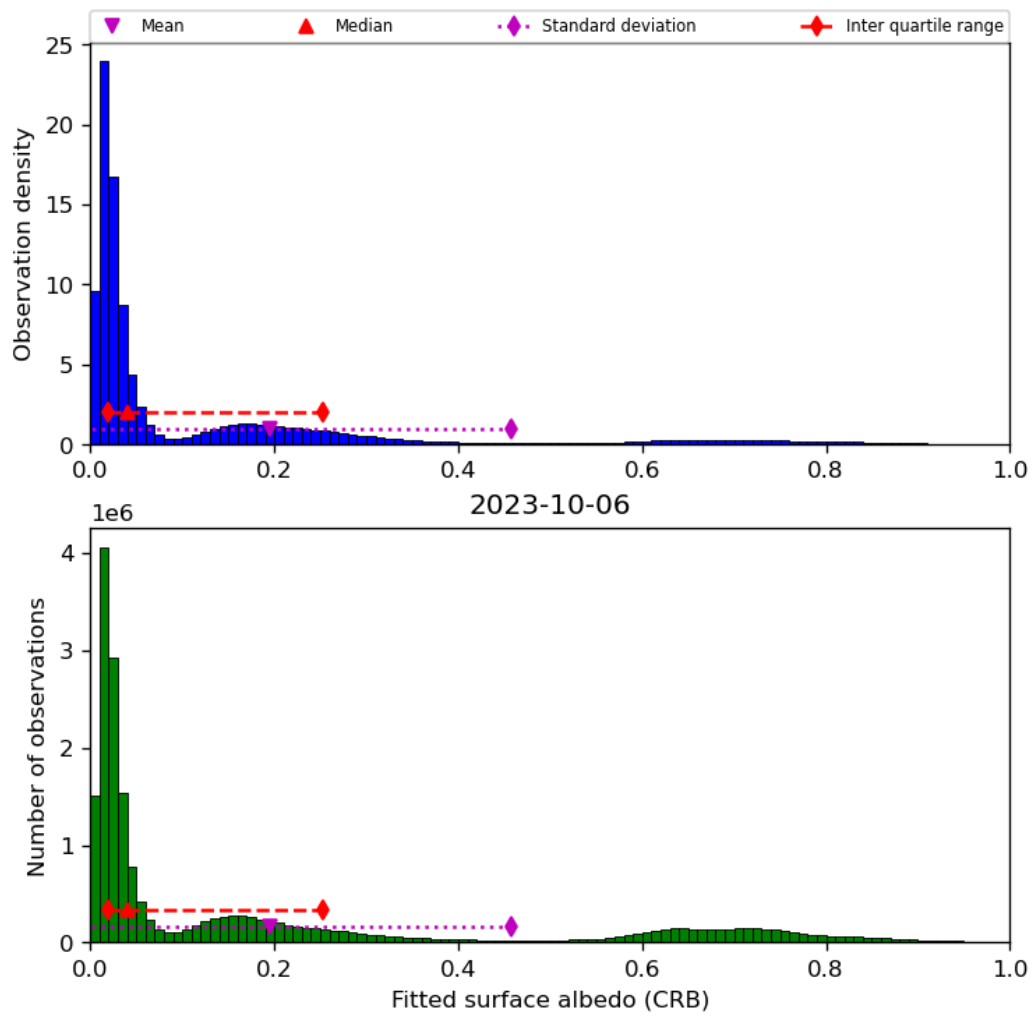
Figure 46: Histogram of “Fitted surface albedo (CRB)” for 2023-10-06 to 2023-10-07
