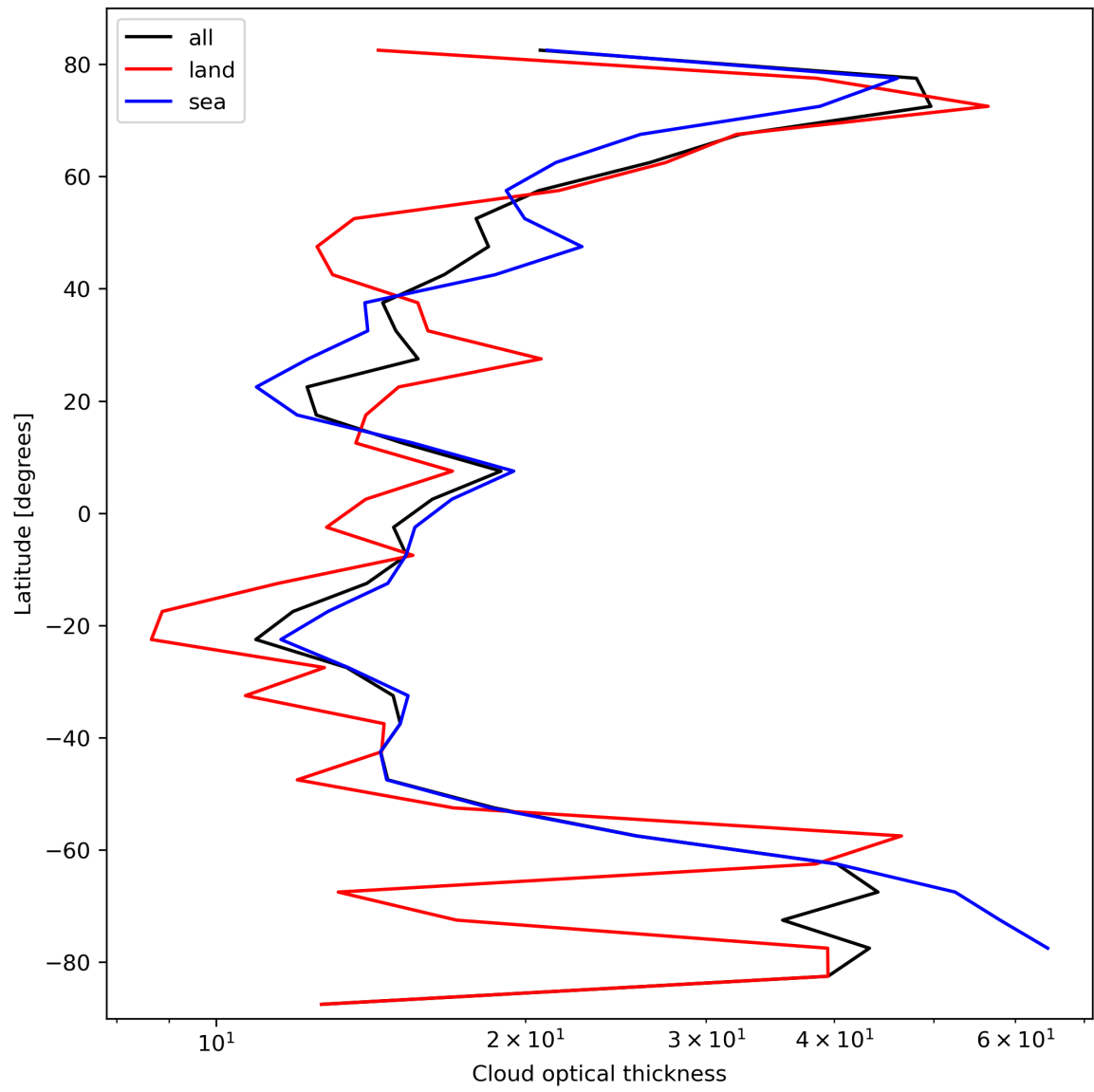
Figure 25: Zonal average of “Cloud optical thickness” for 2023-10-06 to 2023-10-07.
