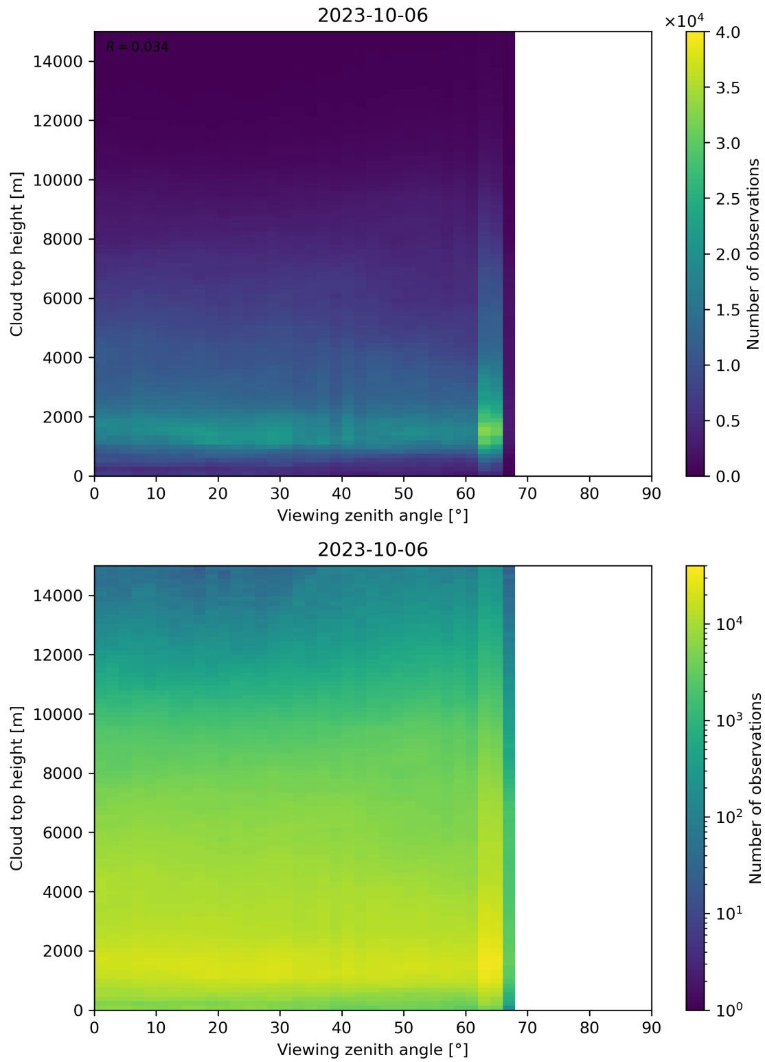
Figure 112: Scatter density plot of “Viewing zenith angle” against “Cloud top height” for 2023-10-06 to 2023-10-07.
