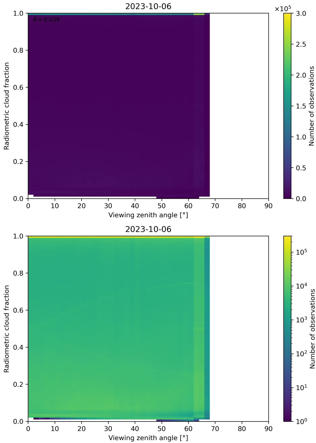
Figure 107: Scatter density plot of “Viewing zenith angle” against “Radiometric cloud fraction” for 2023-10-06 to 2023-10-07.
