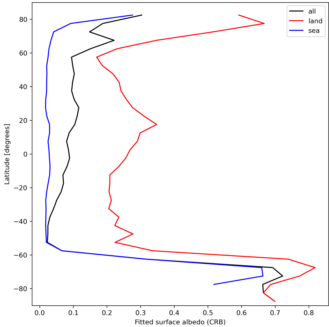
Figure 30: Zonal average of “Fitted surface albedo (CRB)” for 2023-10-06 to 2023-10-07.
