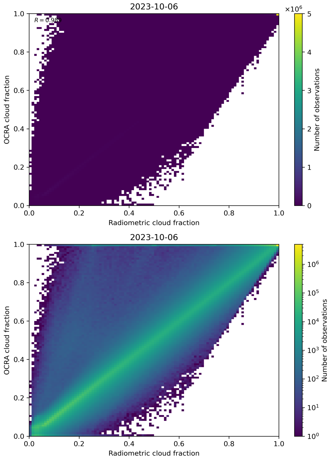
Figure 72: Scatter density plot of “Radiometric cloud fraction” against “OCRA cloud fraction” for 2023-10-06 to 2023-10-07.
