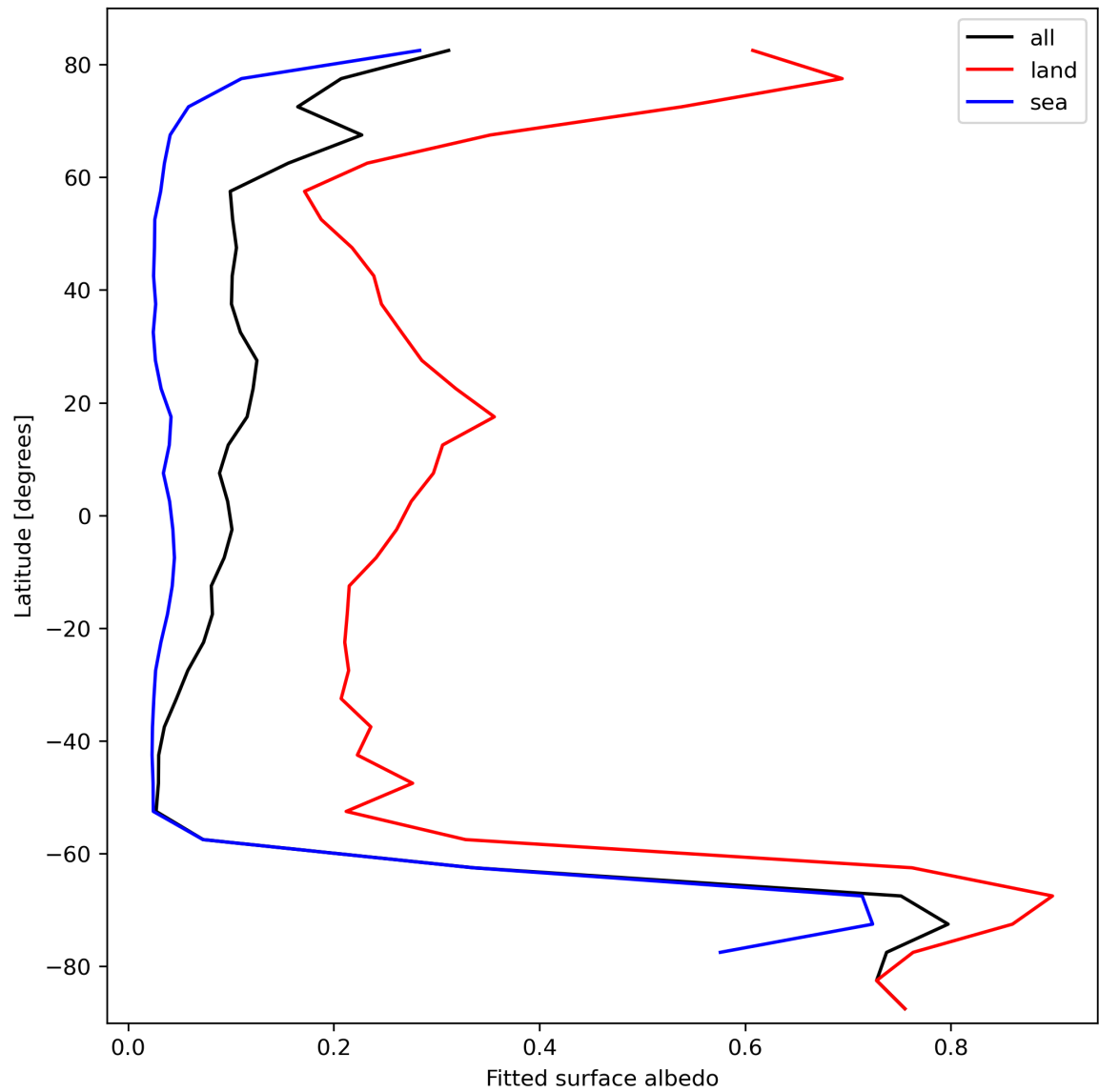
Figure 29: Zonal average of “Fitted surface albedo” for 2023-10-06 to 2023-10-07.
