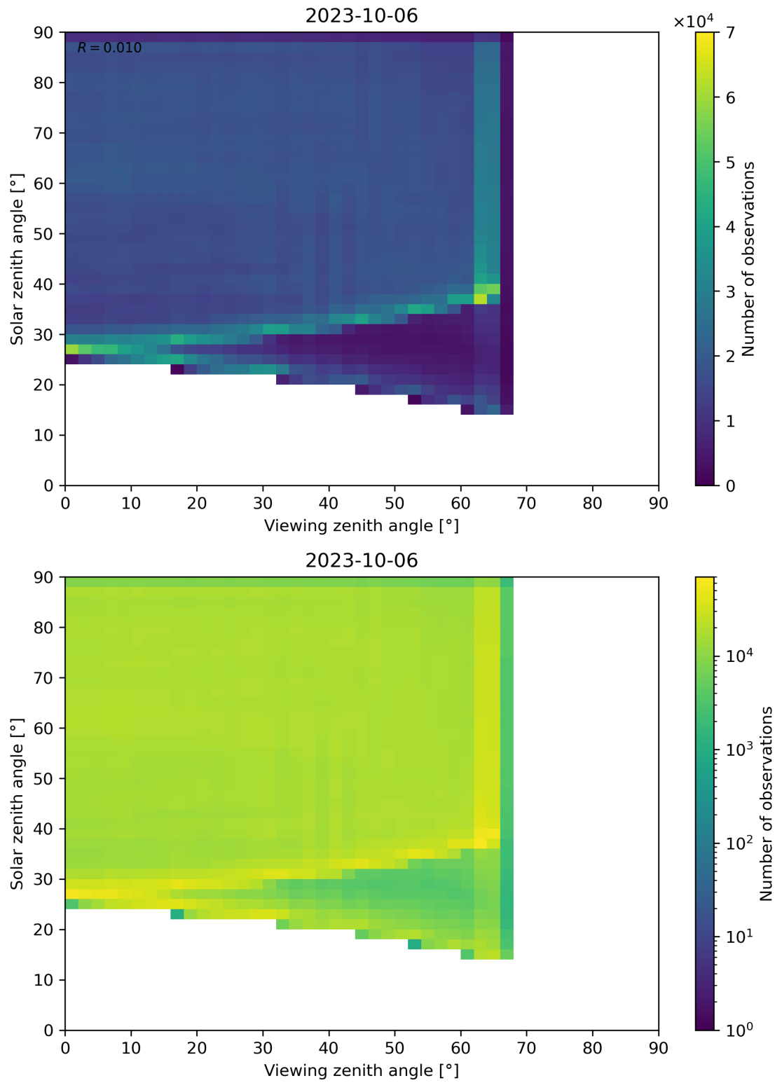
Figure 114: Scatter density plot of “Viewing zenith angle” against “Solar zenith angle” for 2023-10-06 to 2023-10-07.
