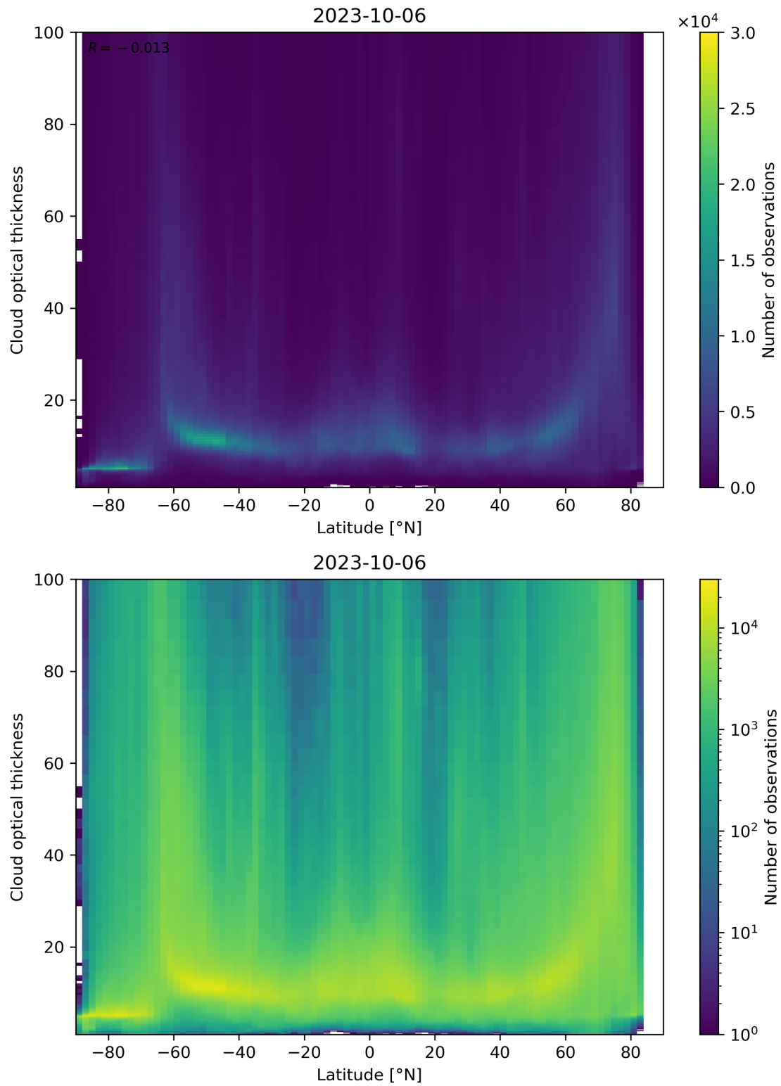
Figure 96: Scatter density plot of “Latitude” against “Cloud optical thickness” for 2023-10-06 to 2023-10-07.
