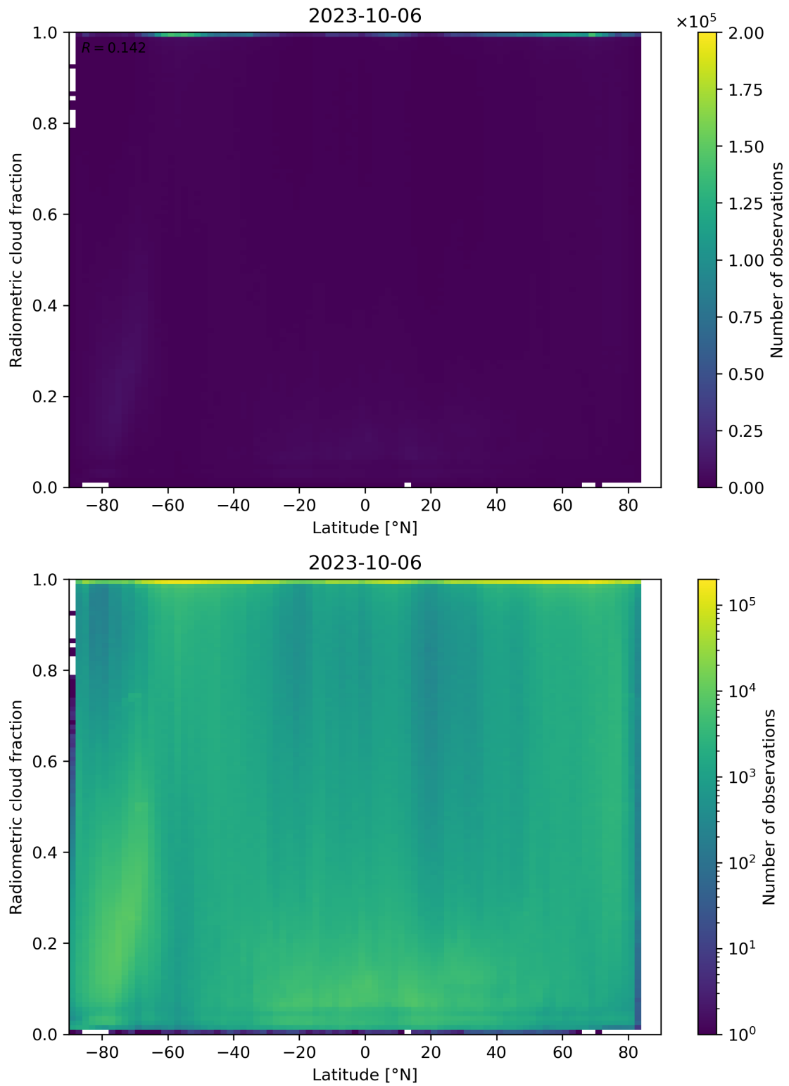
Figure 92: Scatter density plot of “Latitude” against “Radiometric cloud fraction” for 2023-10-06 to 2023-10-07.
