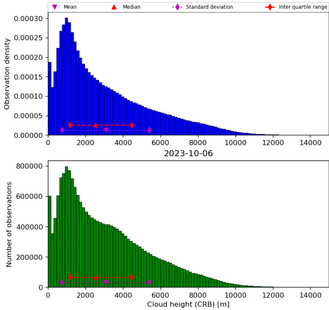
Figure 43: Histogram of “Cloud height (CRB)” for 2023-10-06 to 2023-10-07
