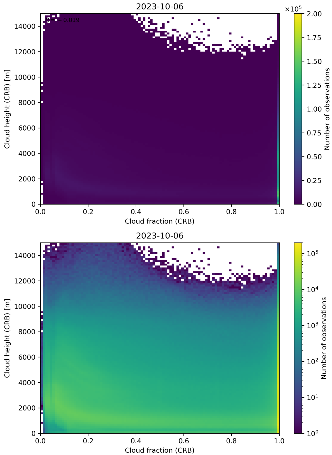
Figure 79: Scatter density plot of “Cloud fraction (CRB)” against “Cloud height (CRB)” for 2023-10-06 to 2023-10-07.
