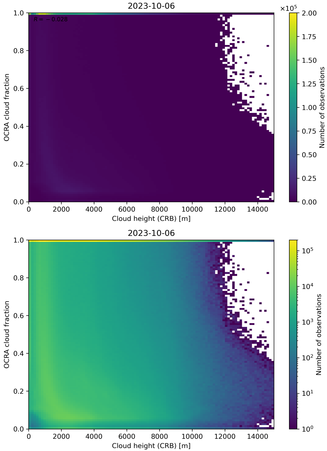
Figure 81: Scatter density plot of “Cloud height (CRB)” against “OCRA cloud fraction” for 2023-10-06 to 2023-10-07.
