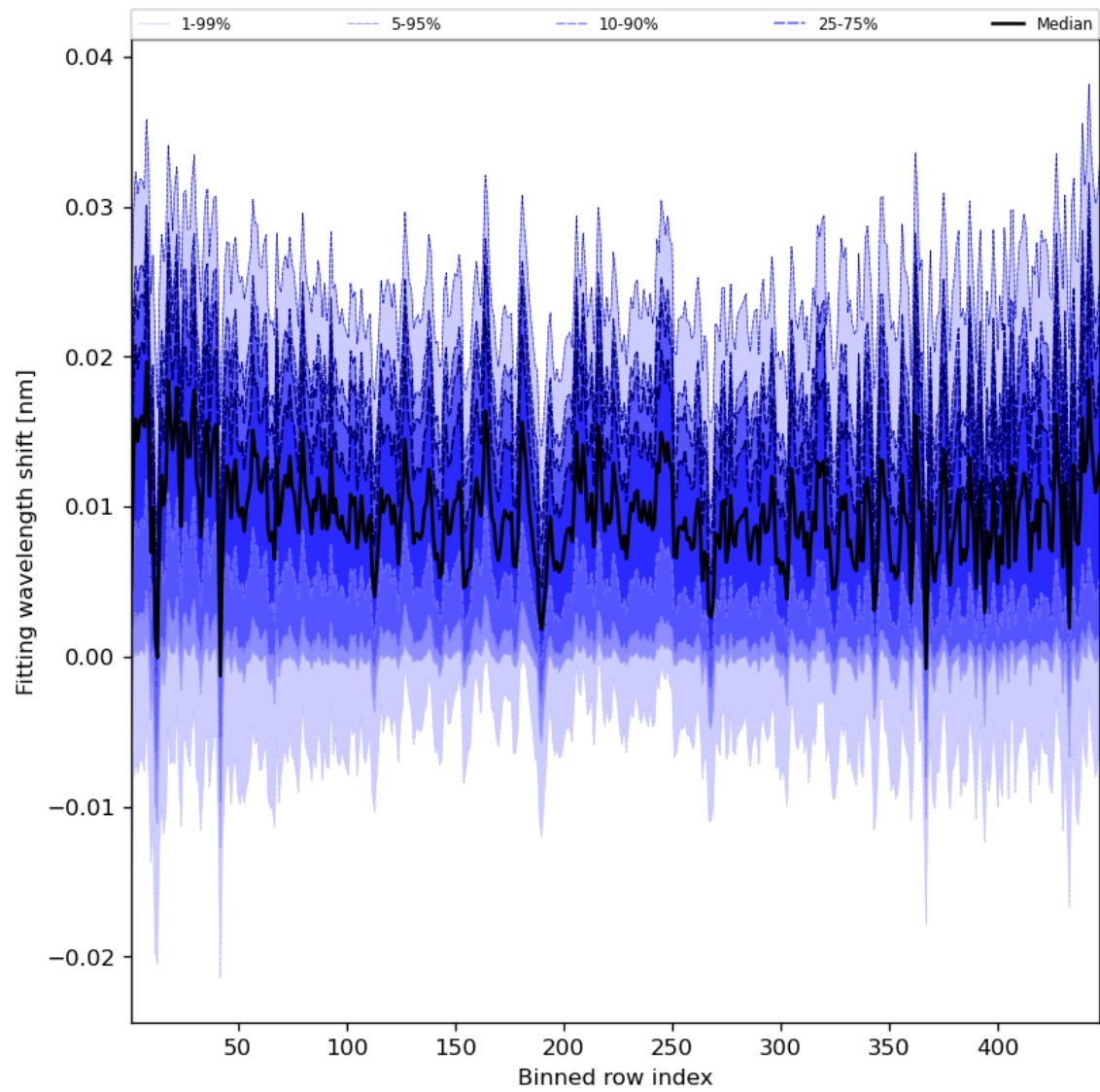
Figure 65: Along track statistics of “Fitting wavelength shift” for 2023-10-06 to 2023-10-07
