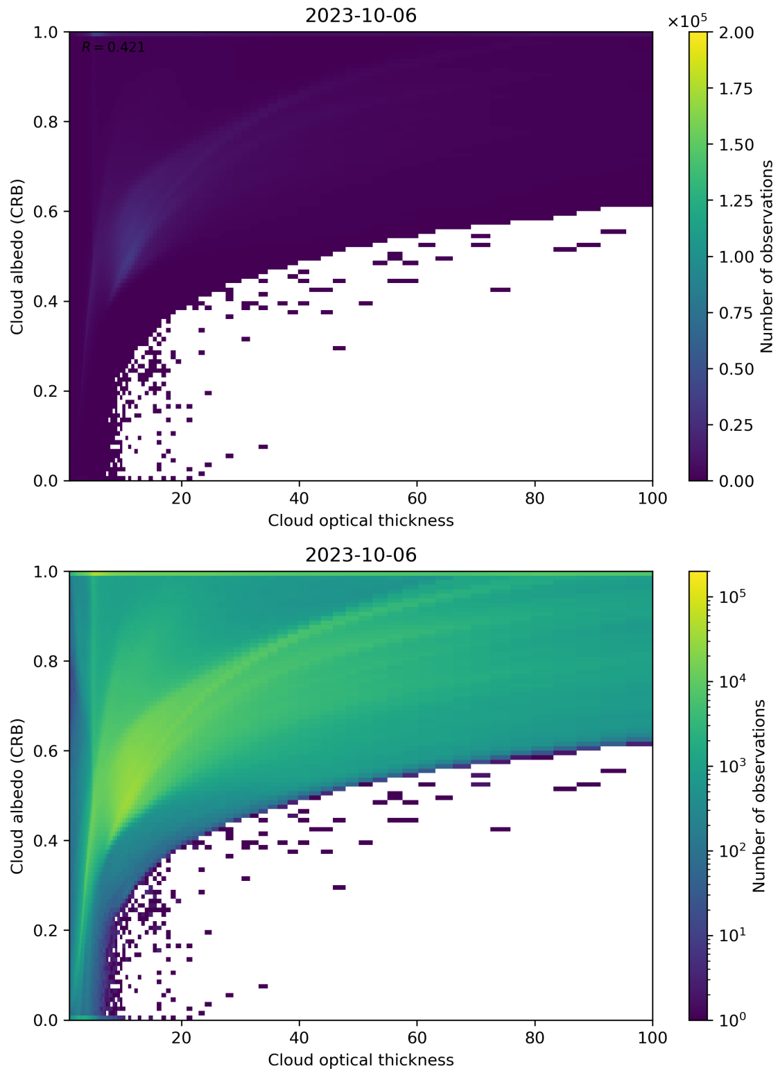
Figure 82: Scatter density plot of “Cloud optical thickness” against “Cloud albedo (CRB)” for 2023-10-06 to 2023-10-07.
