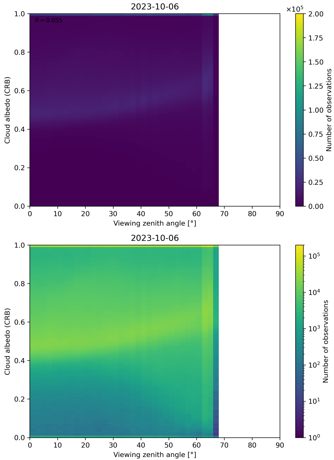
Figure 106: Scatter density plot of “Viewing zenith angle” against “Cloud albedo (CRB)” for 2023-10-06 to 2023-10-07.
