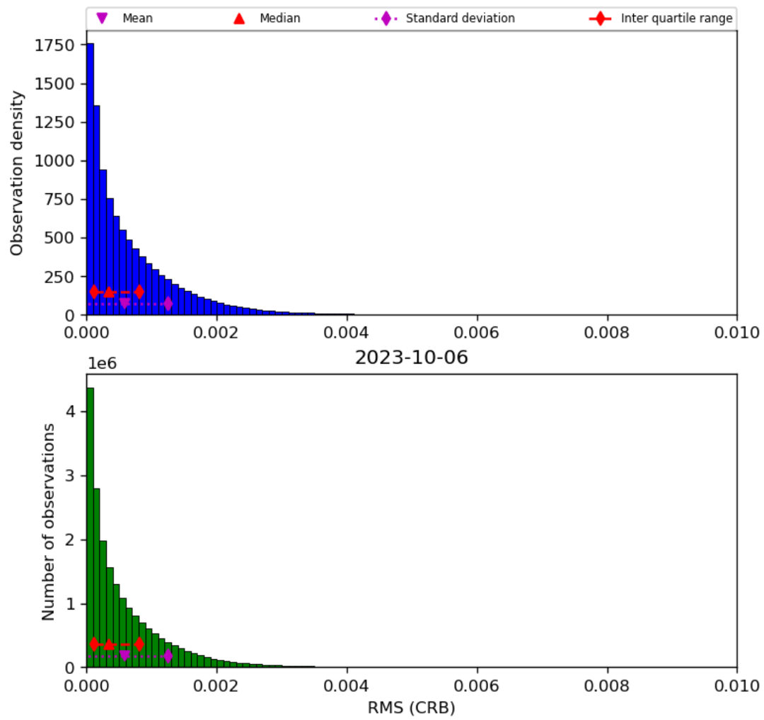
Figure 48: Histogram of “RMS (CRB)” for 2023-10-06 to 2023-10-07
