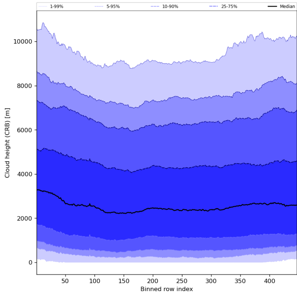
Figure 59: Along track statistics of “Cloud height (CRB)” for 2023-10-06 to 2023-10-07
