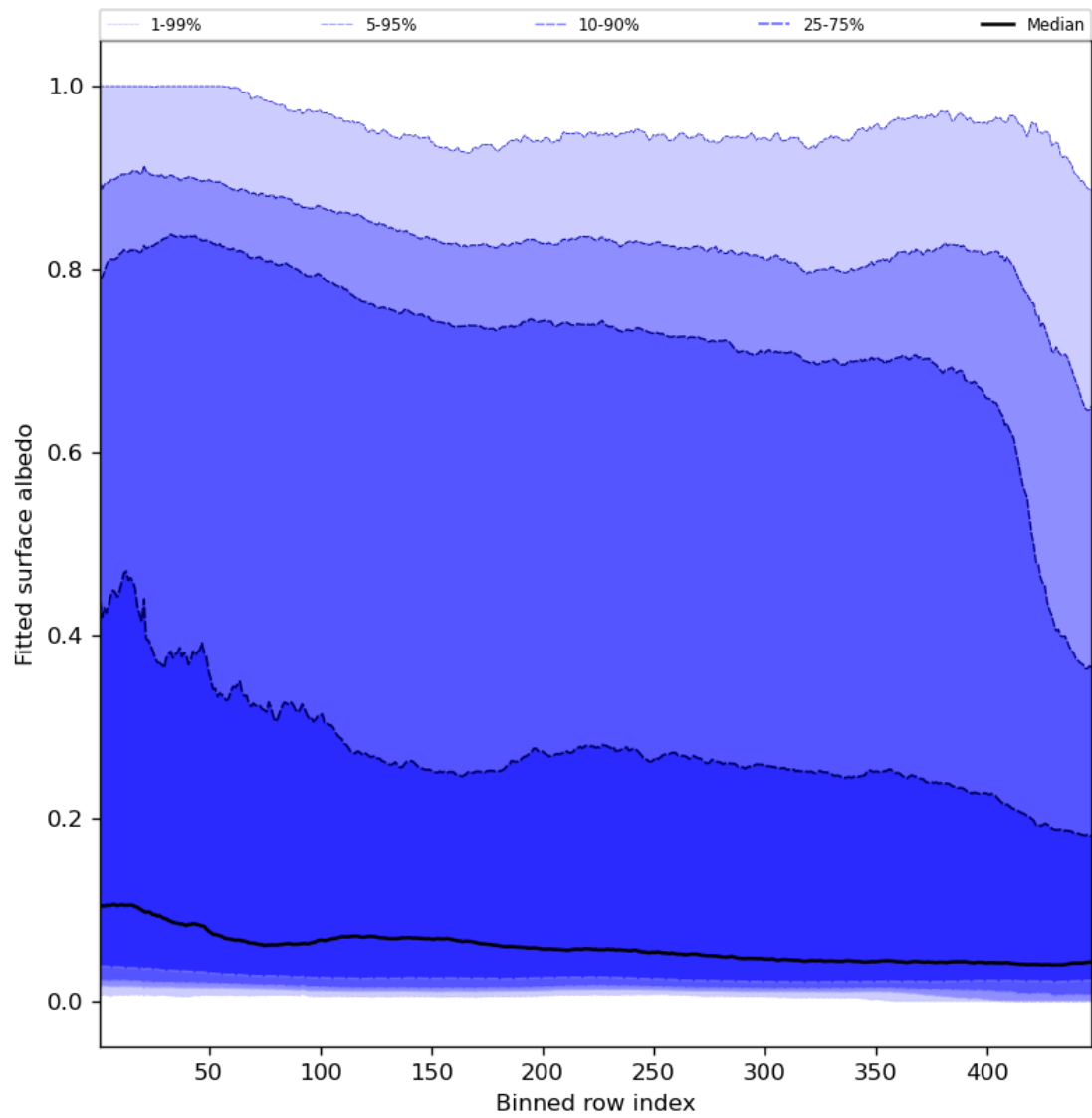
Figure 61: Along track statistics of “Fitted surface albedo” for 2023-10-06 to 2023-10-07
