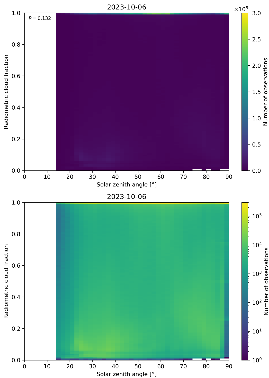
Figure 99: Scatter density plot of “Solar zenith angle” against “Radiometric cloud fraction” for 2023-10-06 to 2023-10-07.
