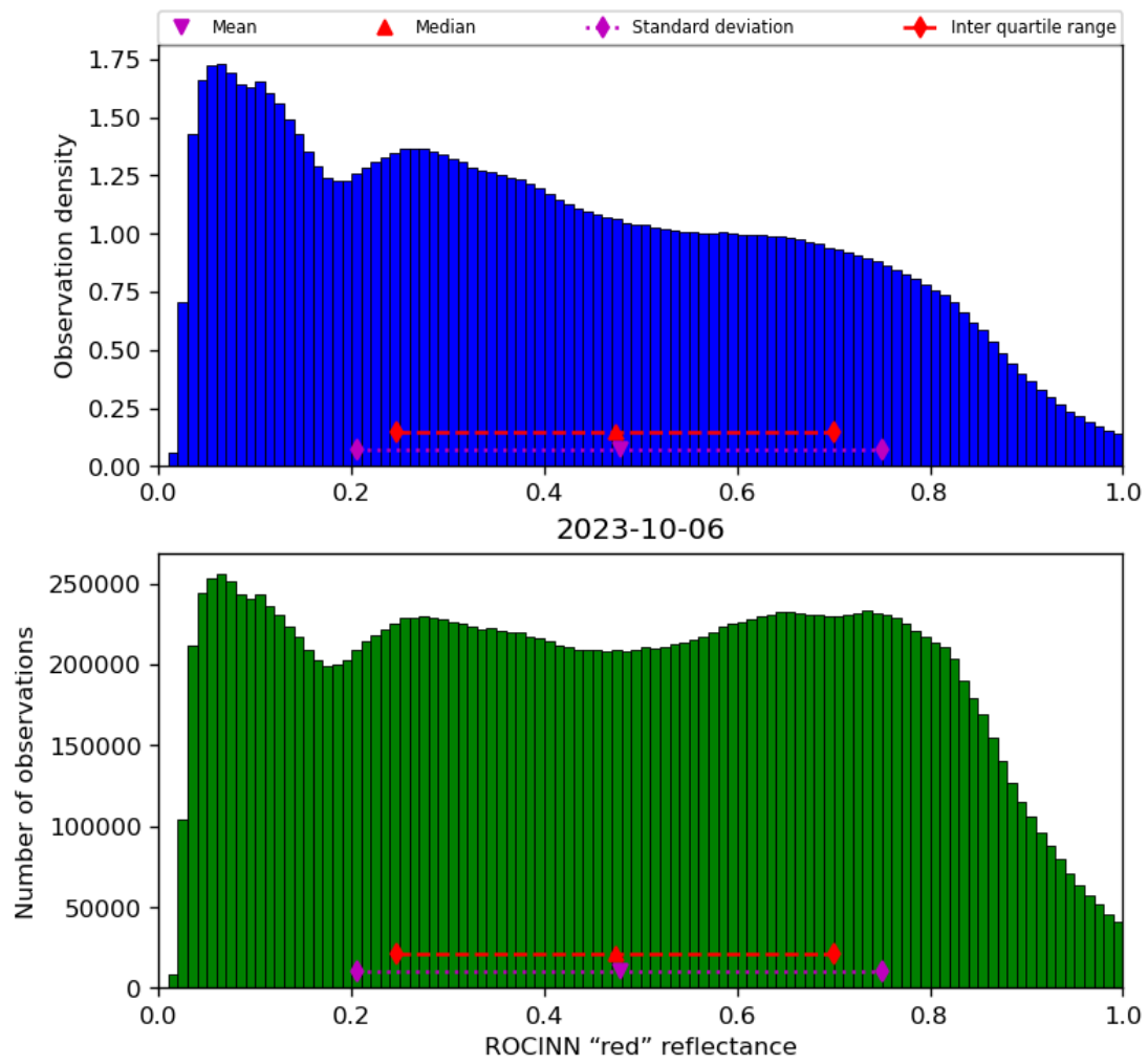
Figure 53: Histogram of “ROCINN “red” reflectance” for 2023-10-06 to 2023-10-07
