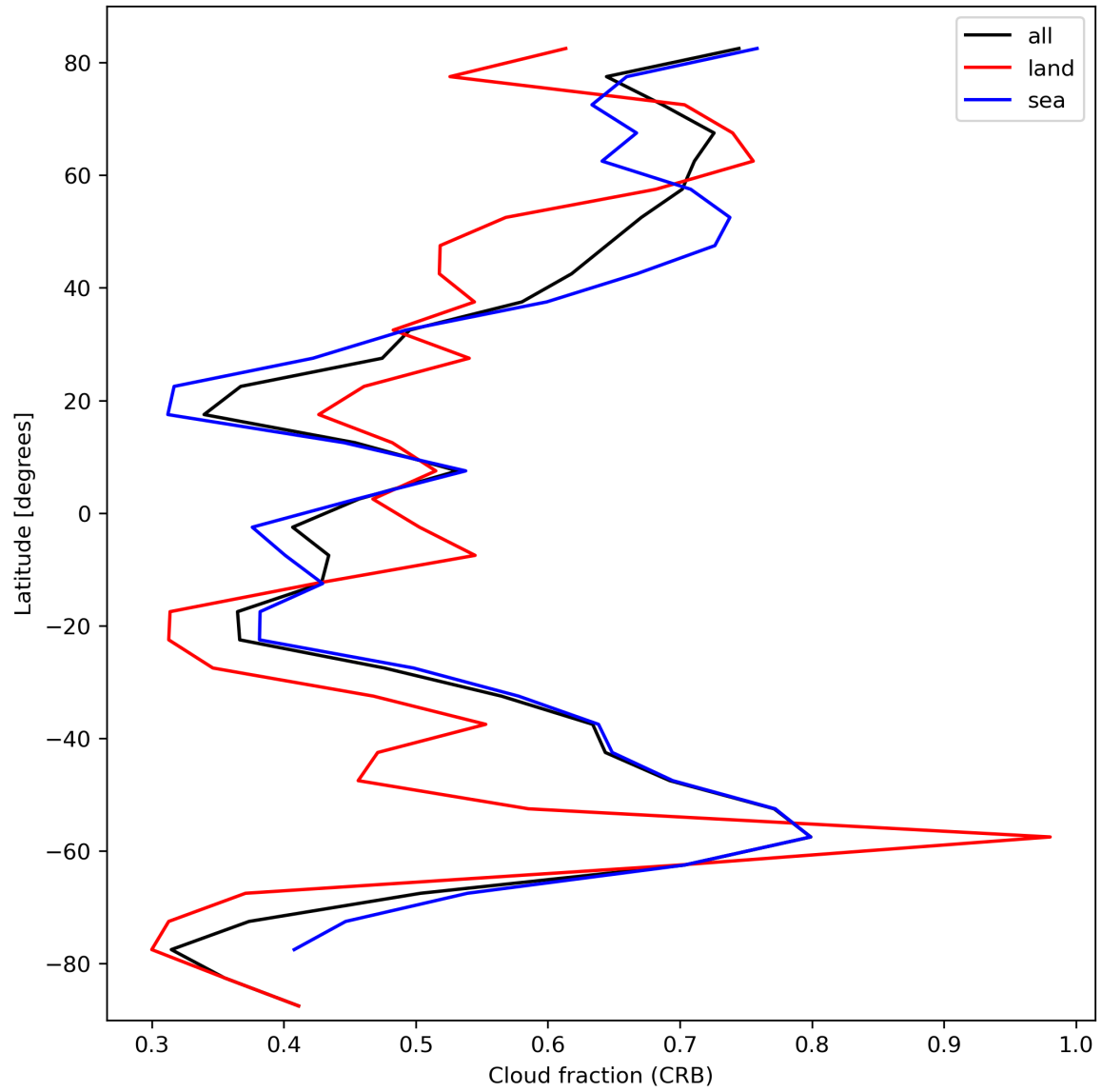
Figure 26: Zonal average of “Cloud fraction (CRB)” for 2023-10-06 to 2023-10-07.
