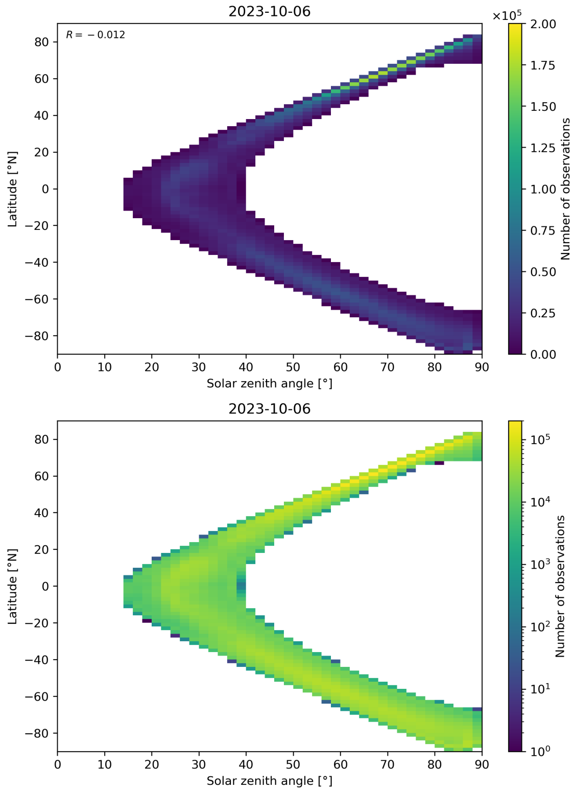
Figure 105: Scatter density plot of “Solar zenith angle” against “Latitude” for 2023-10-06 to 2023-10-07.
