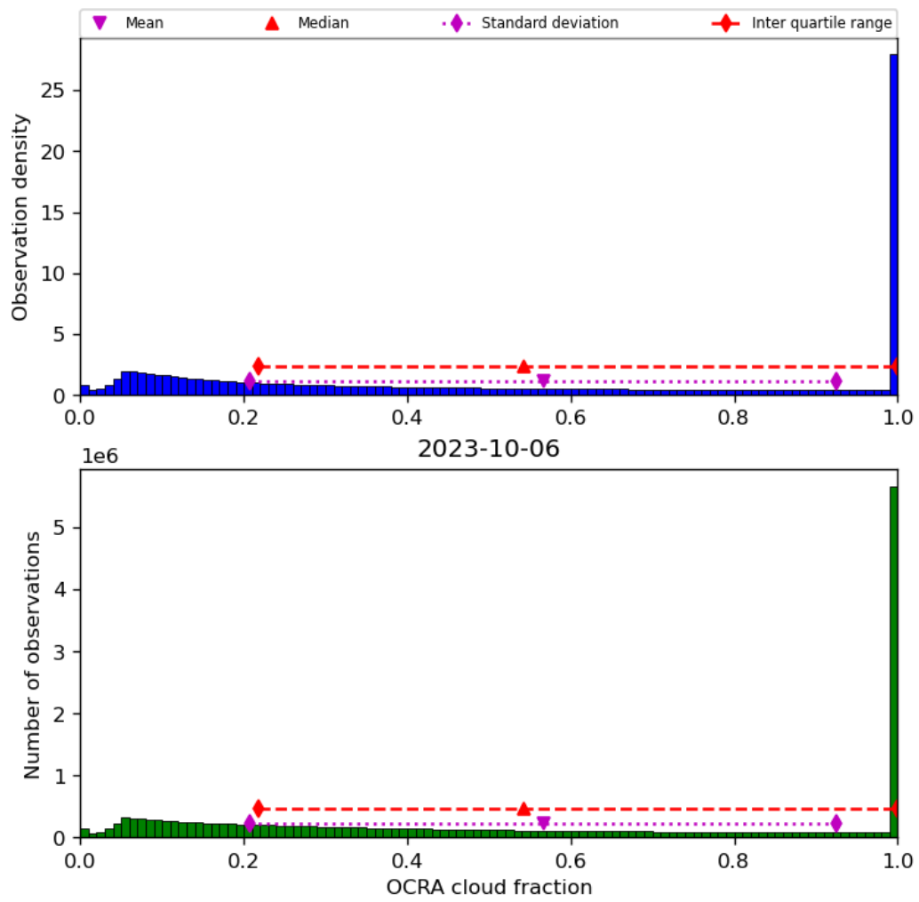
Figure 50: Histogram of “OCRA cloud fraction” for 2023-10-06 to 2023-10-07
