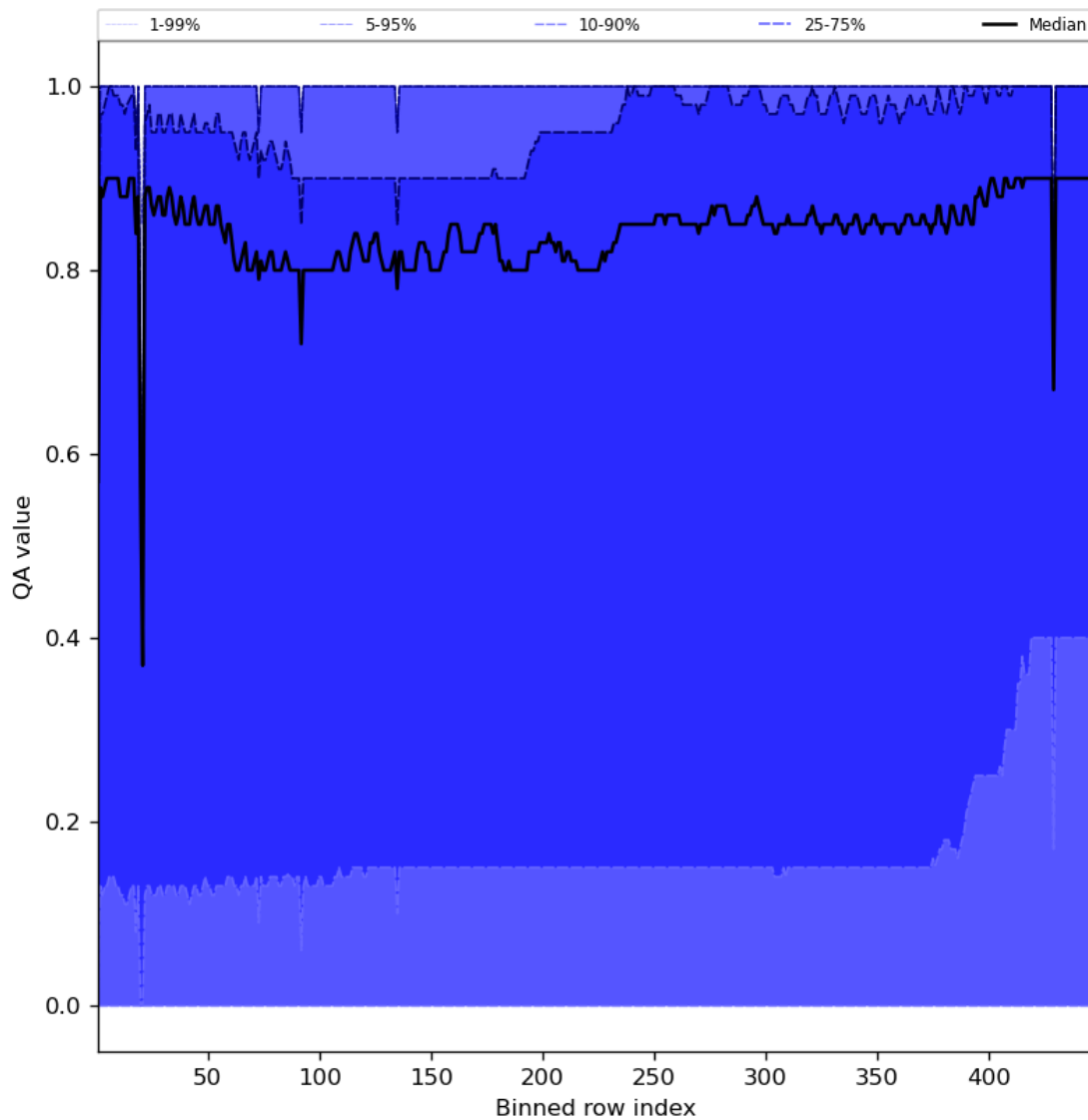
Figure 54: Along track statistics of “QA value” for 2023-10-06 to 2023-10-07
