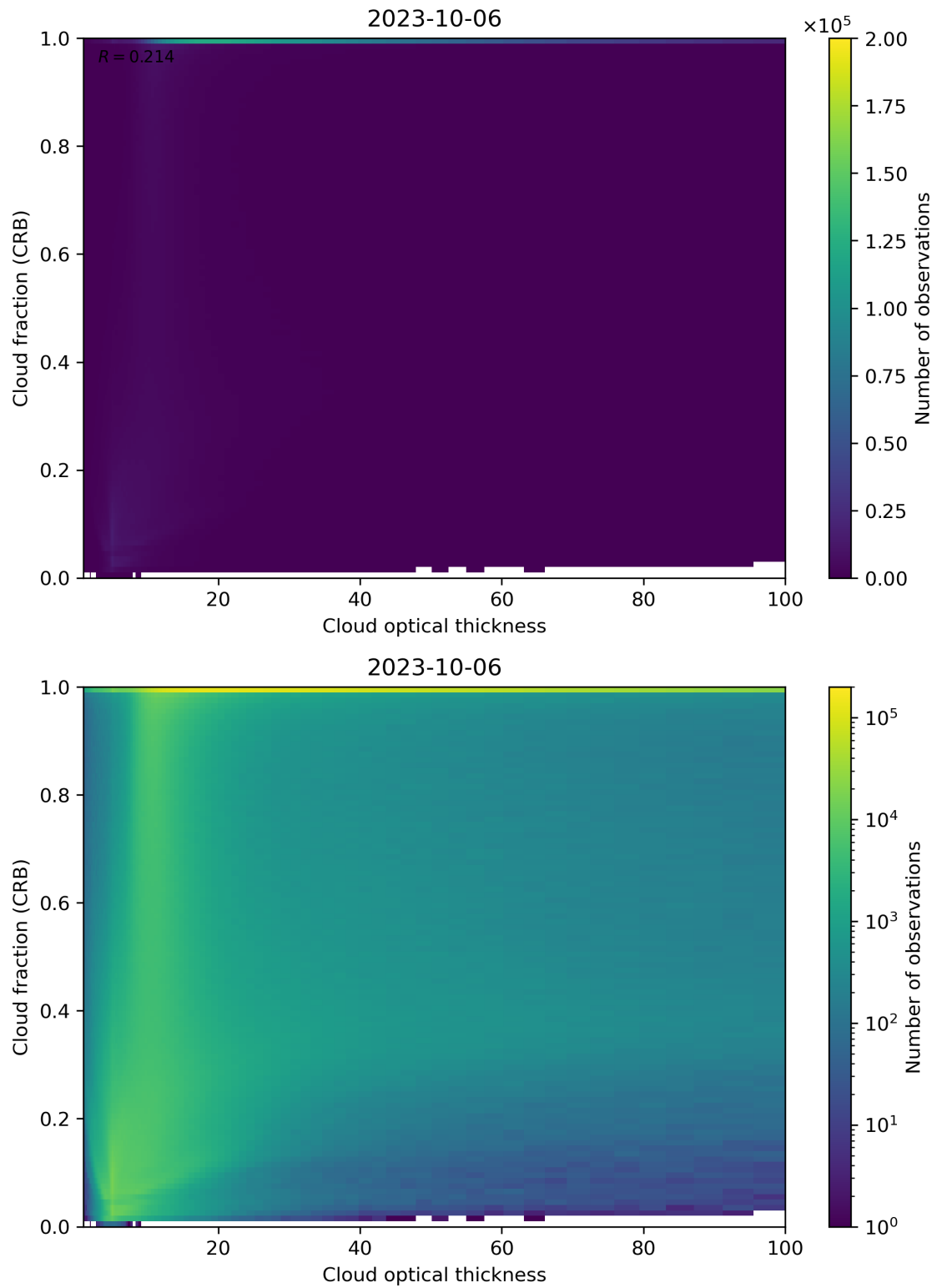
Figure 84: Scatter density plot of “Cloud optical thickness” against “Cloud fraction (CRB)” for 2023-10-06 to 2023-10-07.
