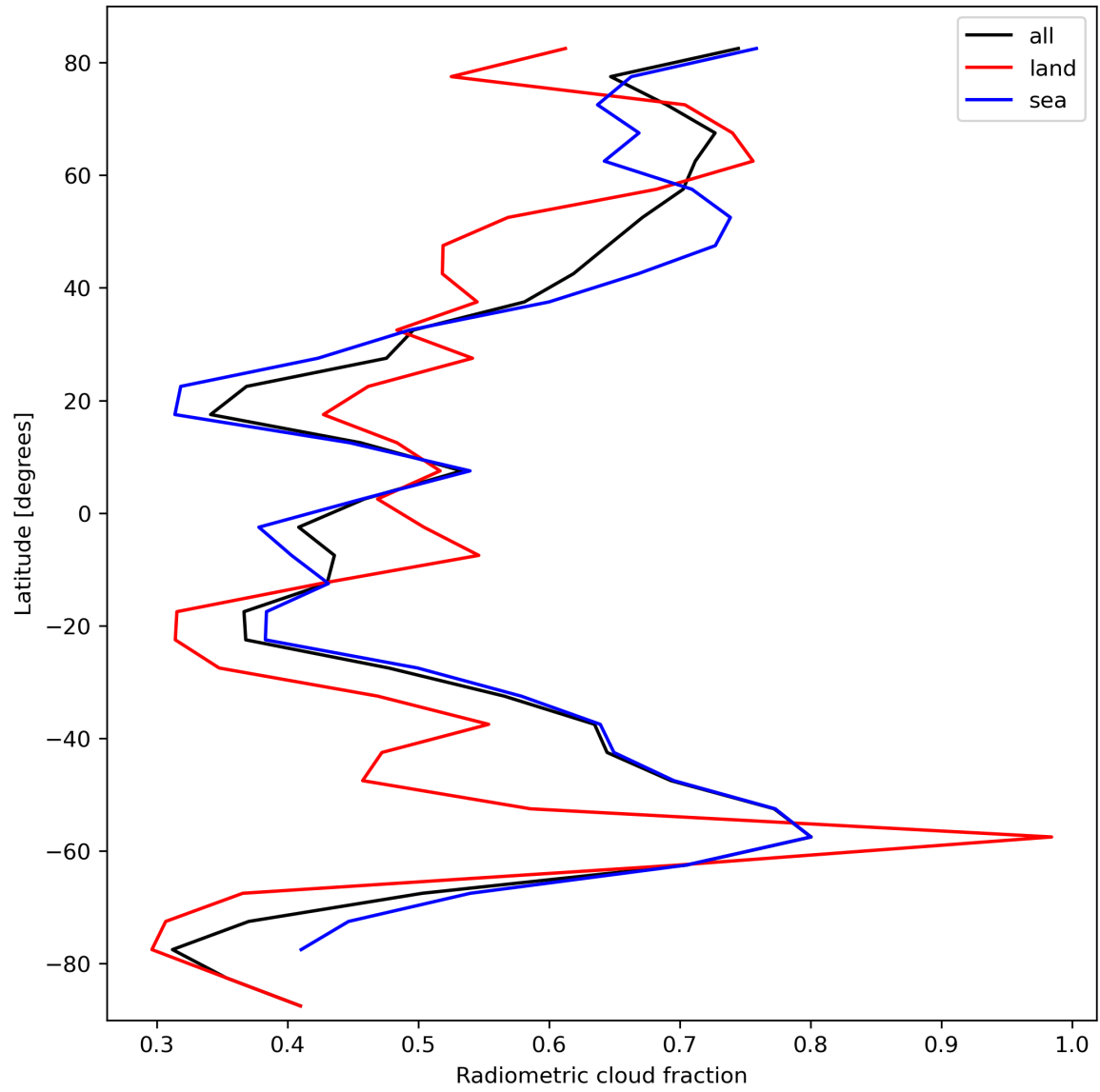
Figure 23: Zonal average of “Radiometric cloud fraction” for 2023-10-06 to 2023-10-07.
