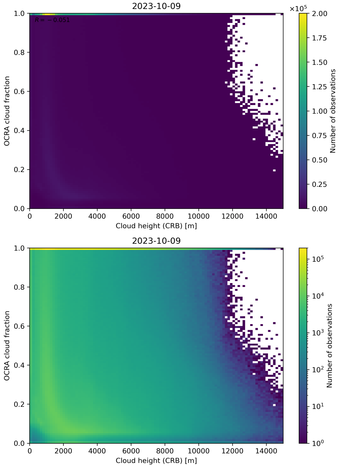
Figure 81: Scatter density plot of “Cloud height (CRB)” against “OCRA cloud fraction” for 2023-10-08 to 2023-10-10.
