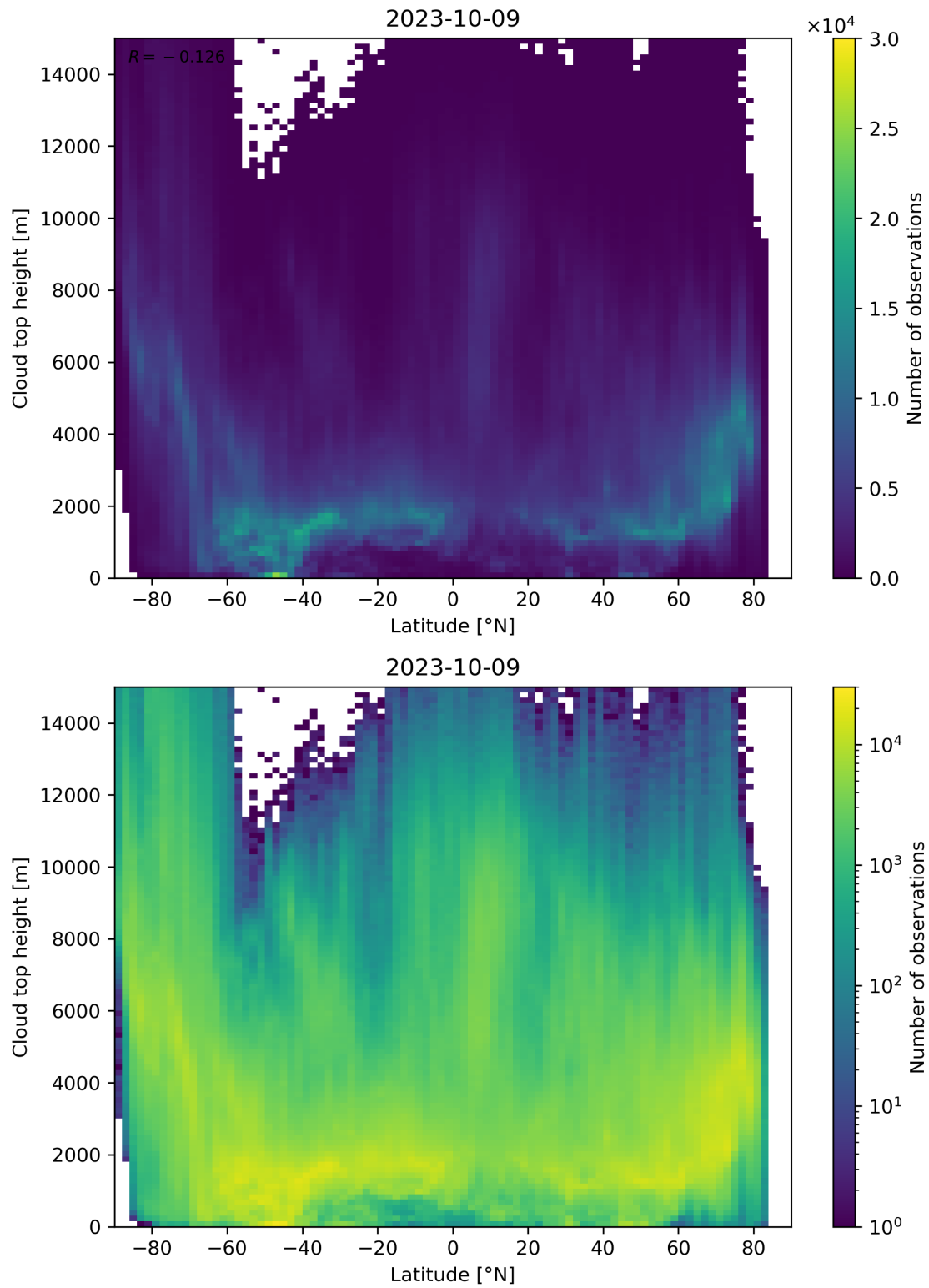
Figure 97: Scatter density plot of “Latitude” against “Cloud top height” for 2023-10-08 to 2023-10-10.
