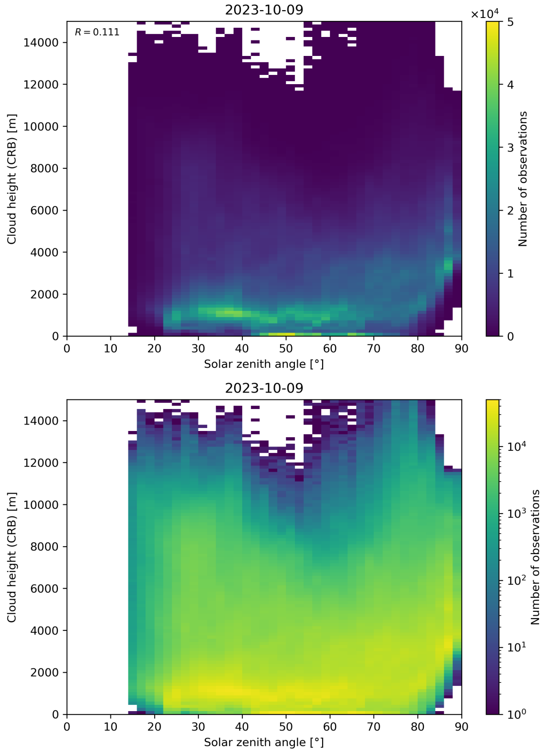
Figure 102: Scatter density plot of “Solar zenith angle” against “Cloud height (CRB)” for 2023-10-08 to 2023-10-10.
