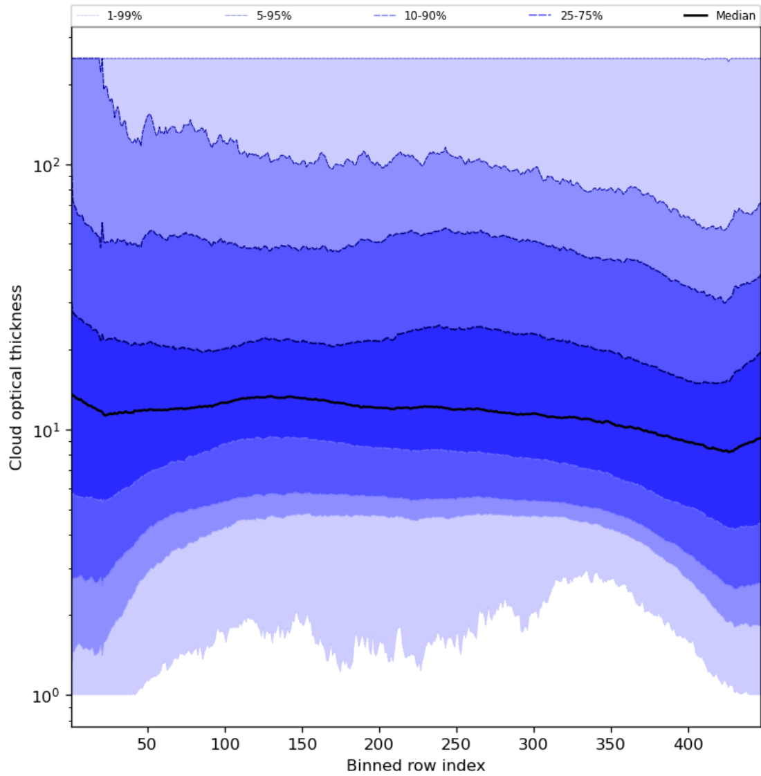
Figure 57: Along track statistics of “Cloud optical thickness” for 2023-10-08 to 2023-10-10
