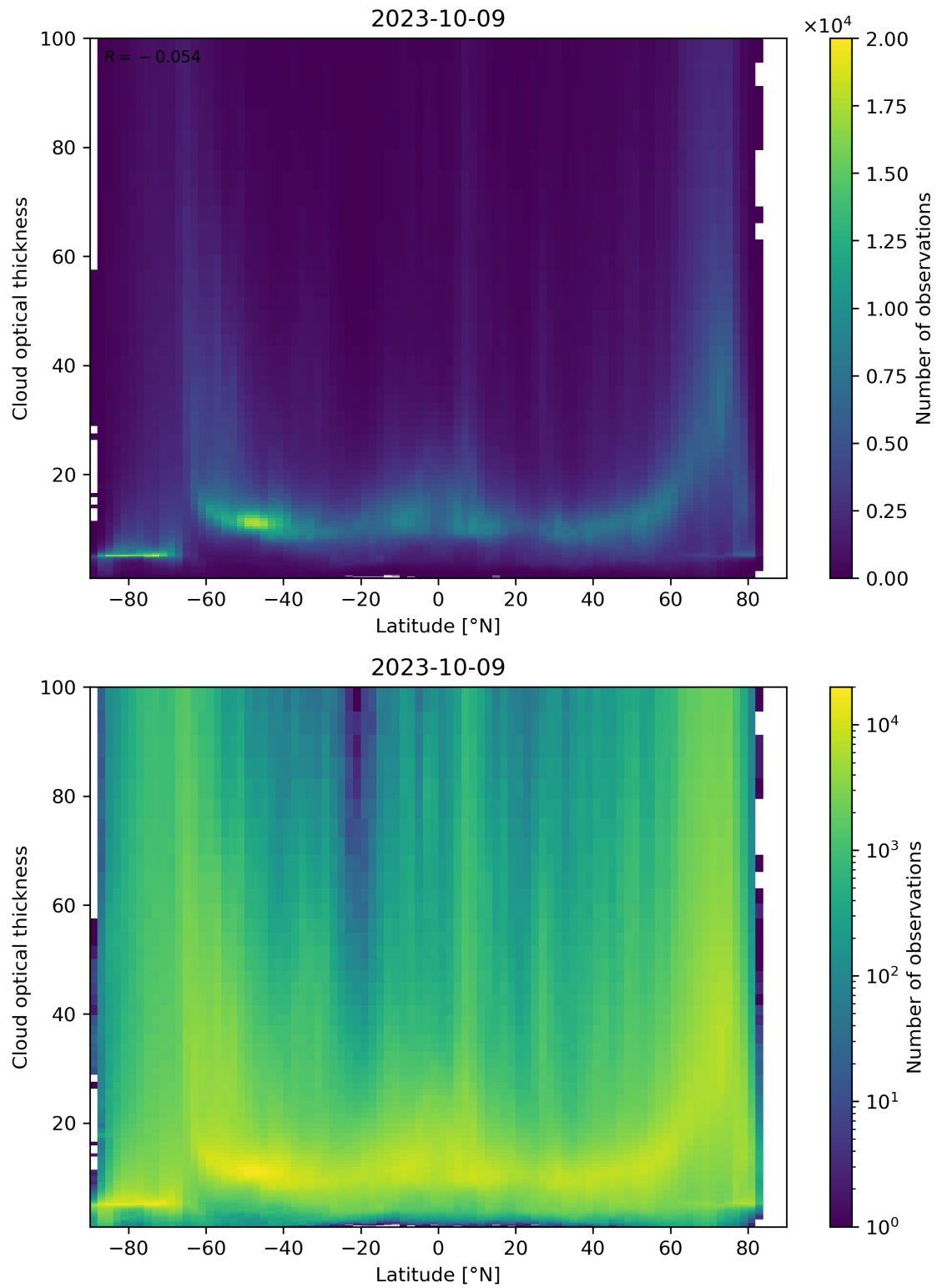
Figure 96: Scatter density plot of “Latitude” against “Cloud optical thickness” for 2023-10-08 to 2023-10-10.
