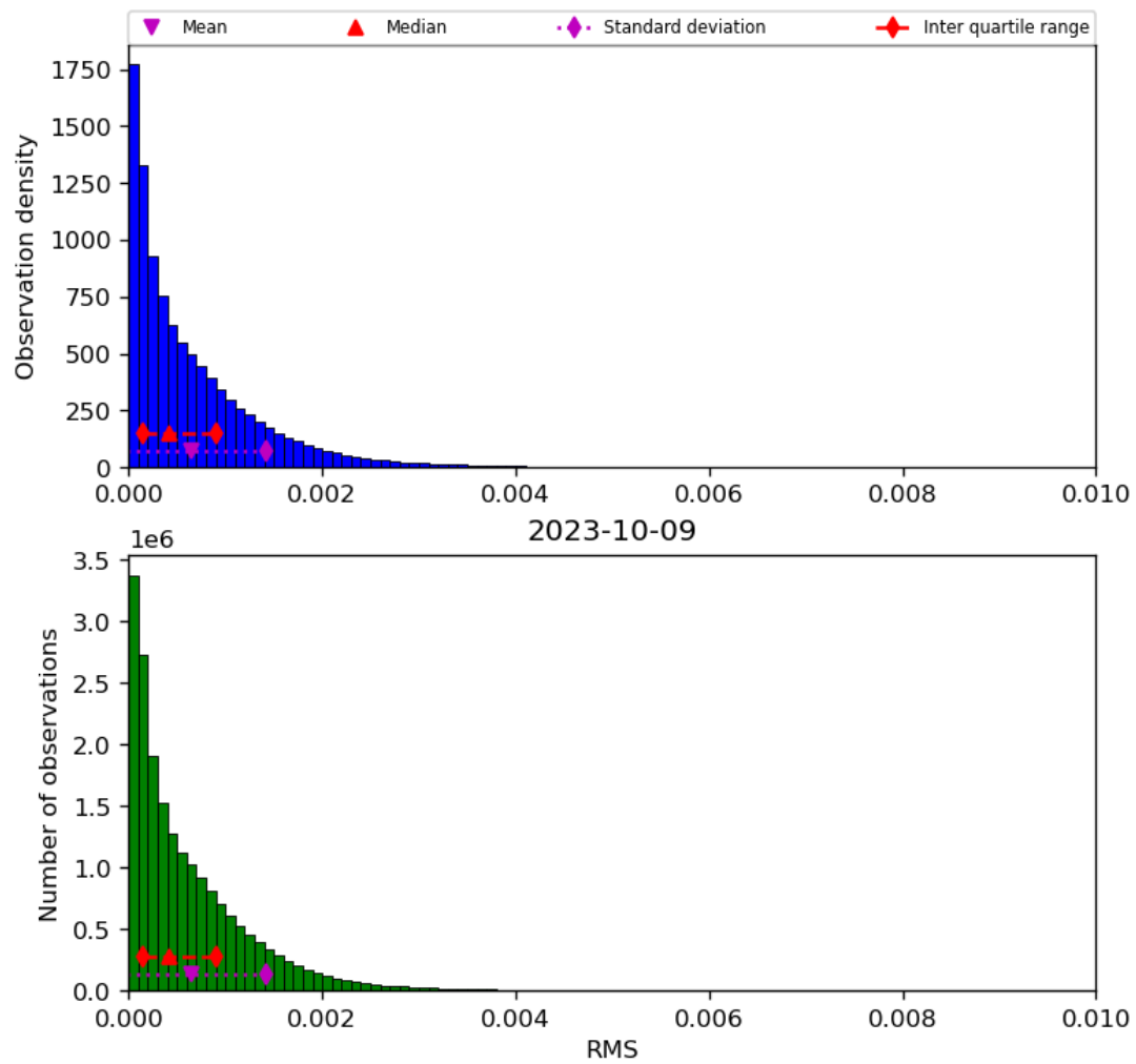
Figure 47: Histogram of “RMS” for 2023-10-08 to 2023-10-10
