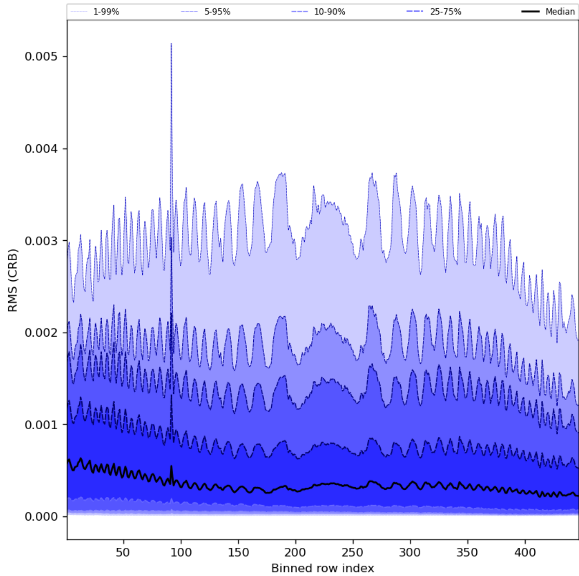
Figure 64: Along track statistics of “RMS (CRB)” for 2023-10-08 to 2023-10-10
