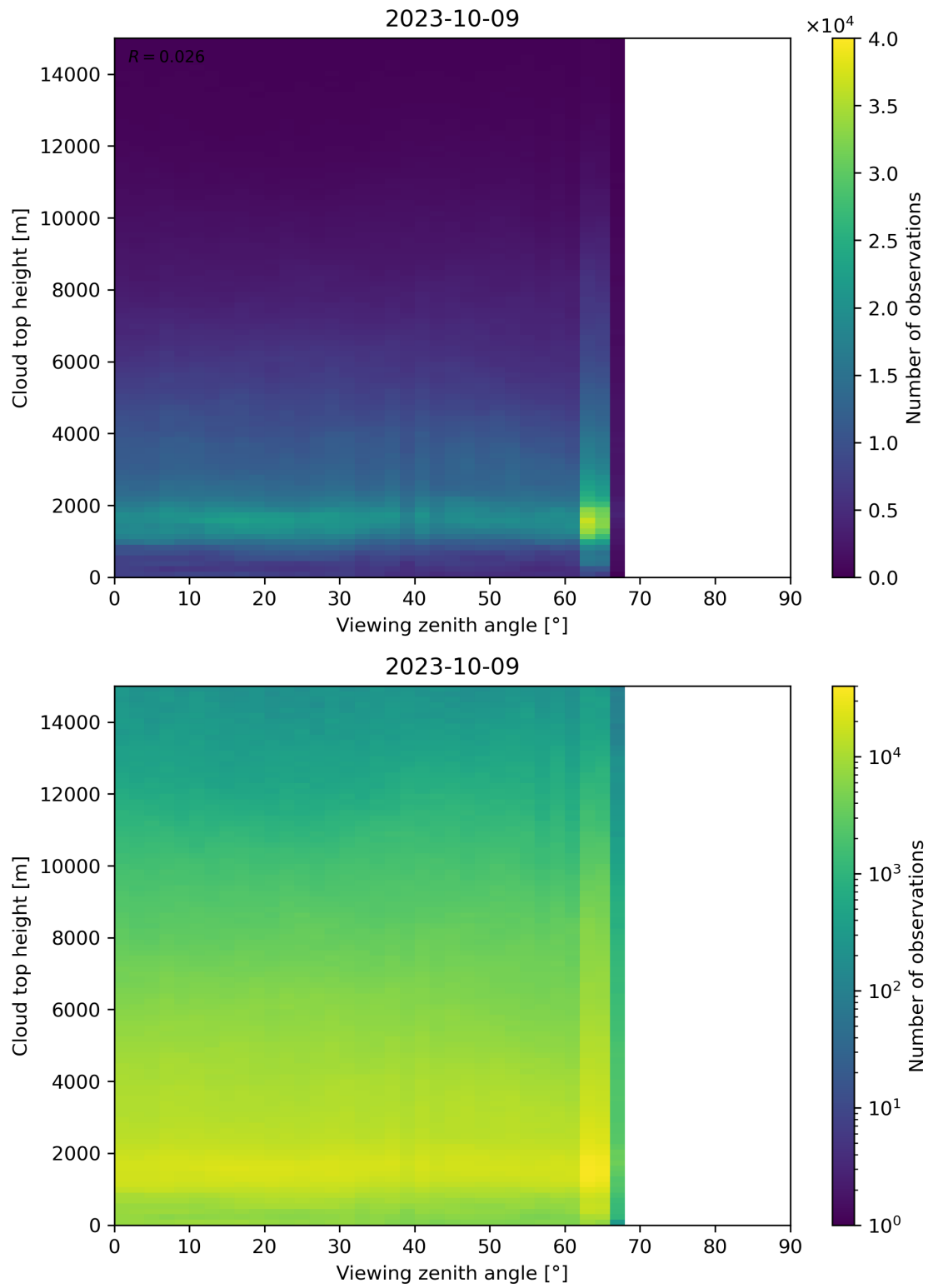
Figure 112: Scatter density plot of “Viewing zenith angle” against “Cloud top height” for 2023-10-08 to 2023-10-10.
