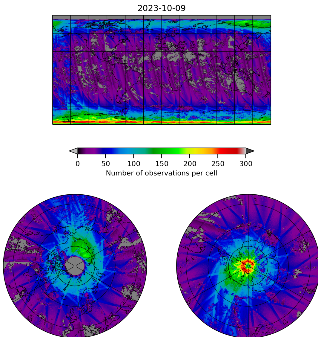
Figure 21: Map of the number of observations for 2023-10-08 to 2023-10-10
