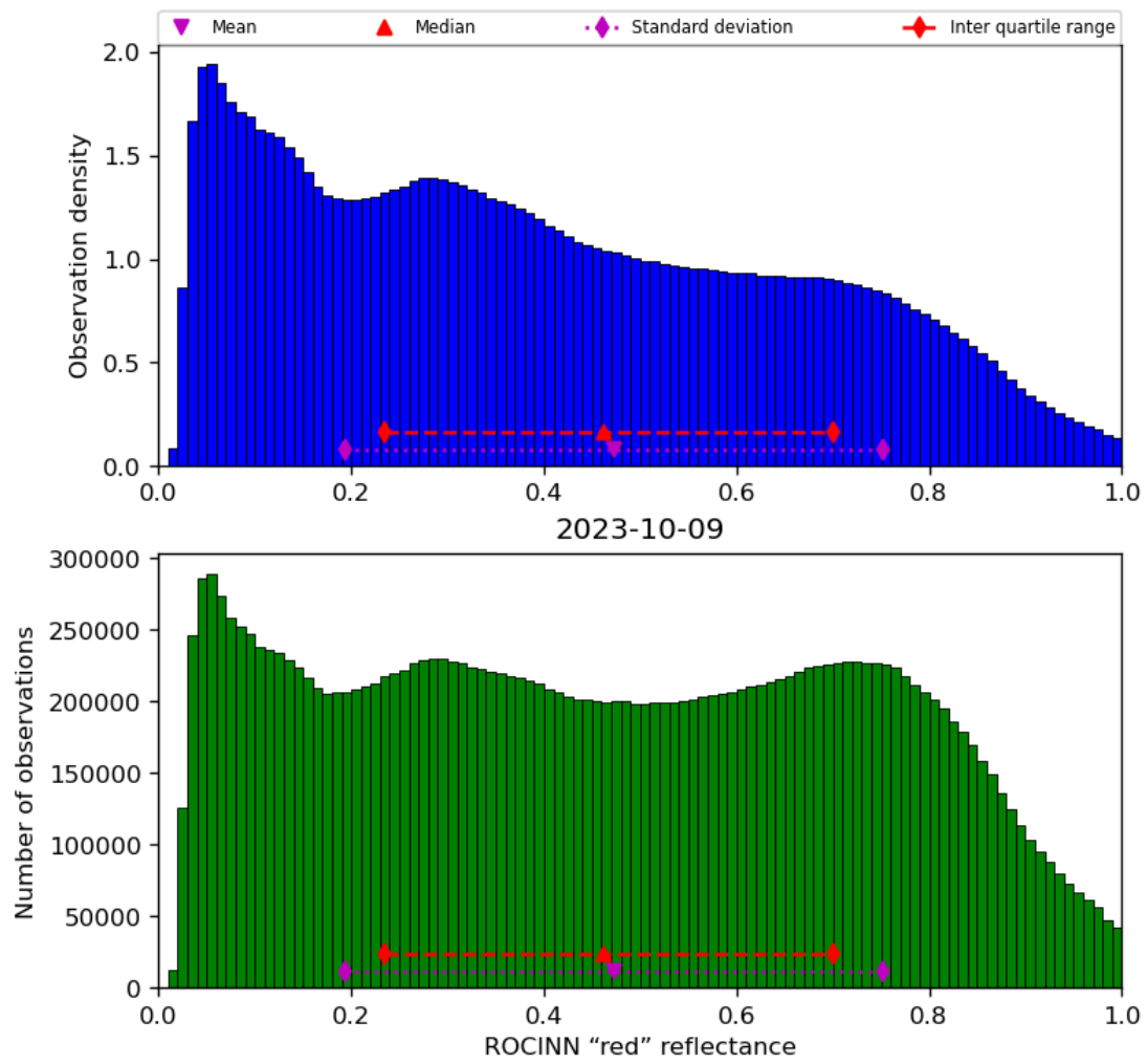
Figure 53: Histogram of “ROCINN “red” reflectance” for 2023-10-08 to 2023-10-10
