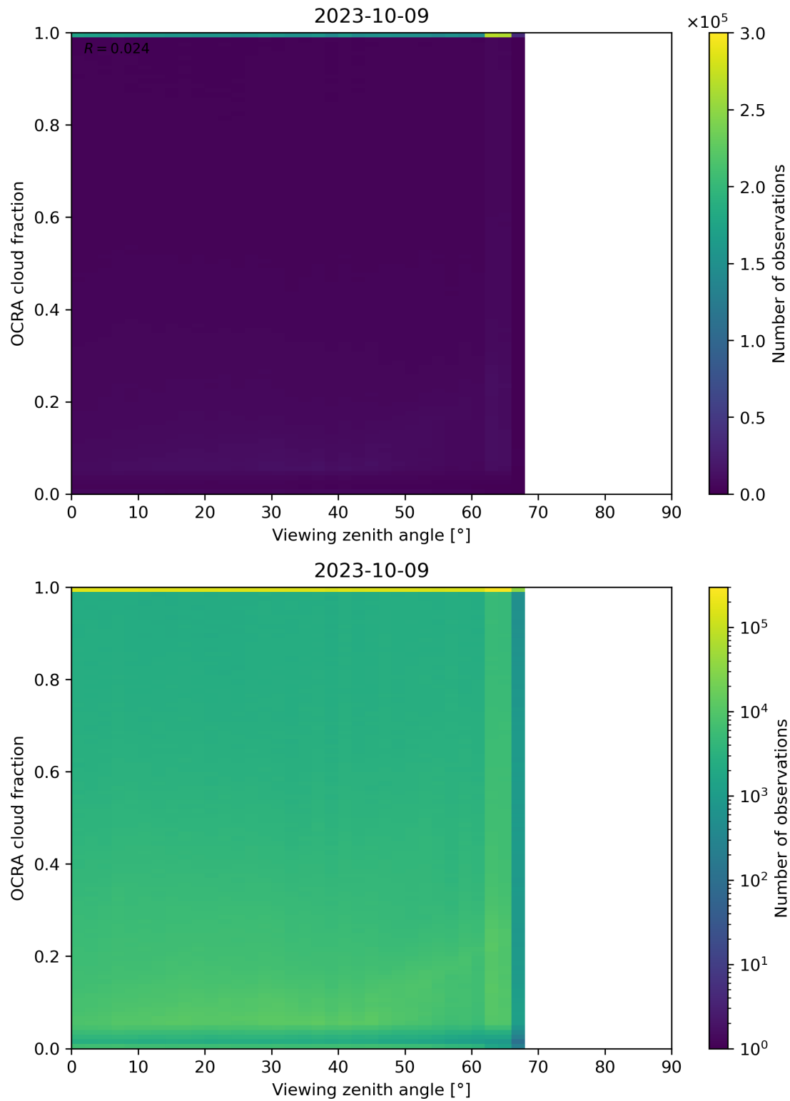
Figure 108: Scatter density plot of “Viewing zenith angle” against “OCRA cloud fraction” for 2023-10-08 to 2023-10-10.
