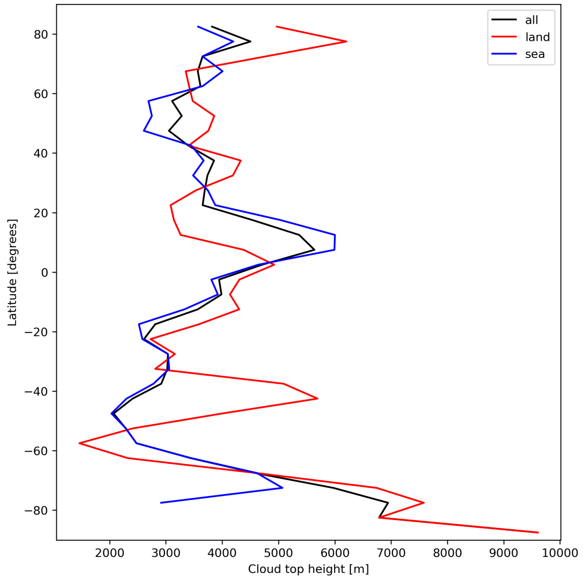
Figure 24: Zonal average of “Cloud top height” for 2023-10-08 to 2023-10-10.
