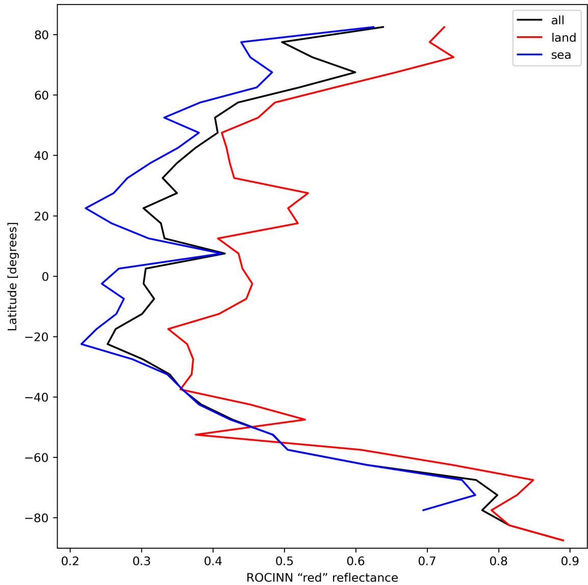
Figure 37: Zonal average of “ROCINN “red” reflectance” for 2023-10-08 to 2023-10-10.
