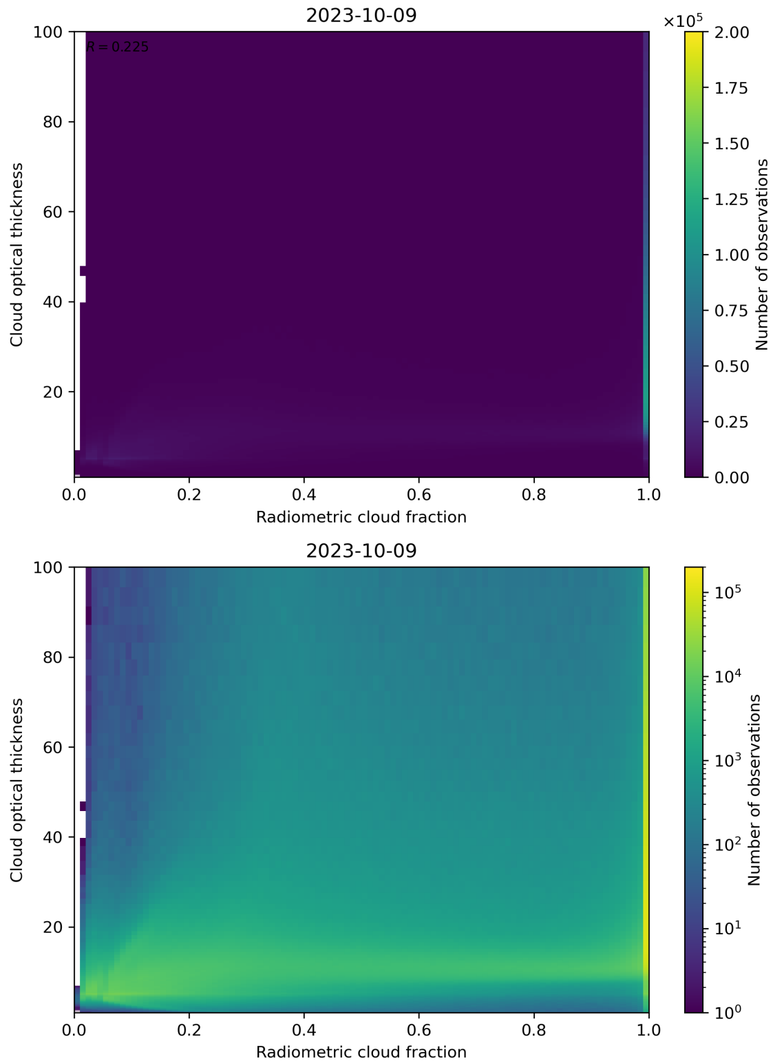
Figure 75: Scatter density plot of “Radiometric cloud fraction” against “Cloud optical thickness” for 2023-10-08 to 2023-10-10.
