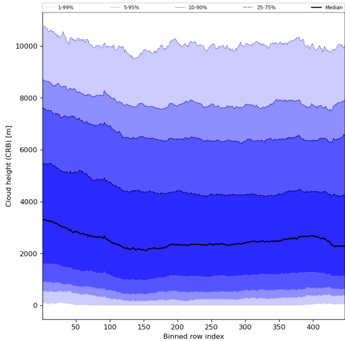
Figure 59: Along track statistics of “Cloud height (CRB)” for 2023-10-08 to 2023-10-10
