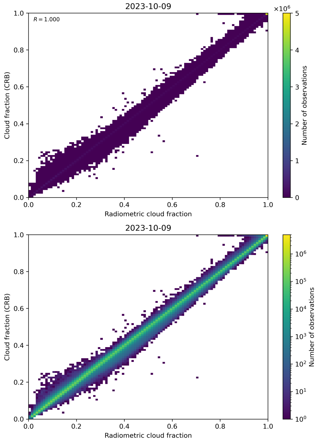
Figure 73: Scatter density plot of “Radiometric cloud fraction” against “Cloud fraction (CRB)” for 2023-10-08 to 2023-10-10.
