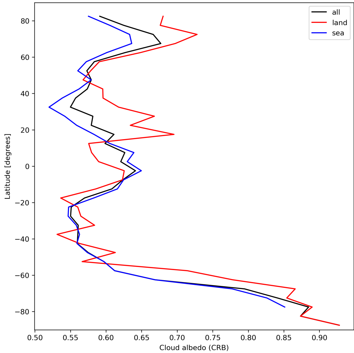
Figure 28: Zonal average of “Cloud albedo (CRB)” for 2023-10-08 to 2023-10-10.
