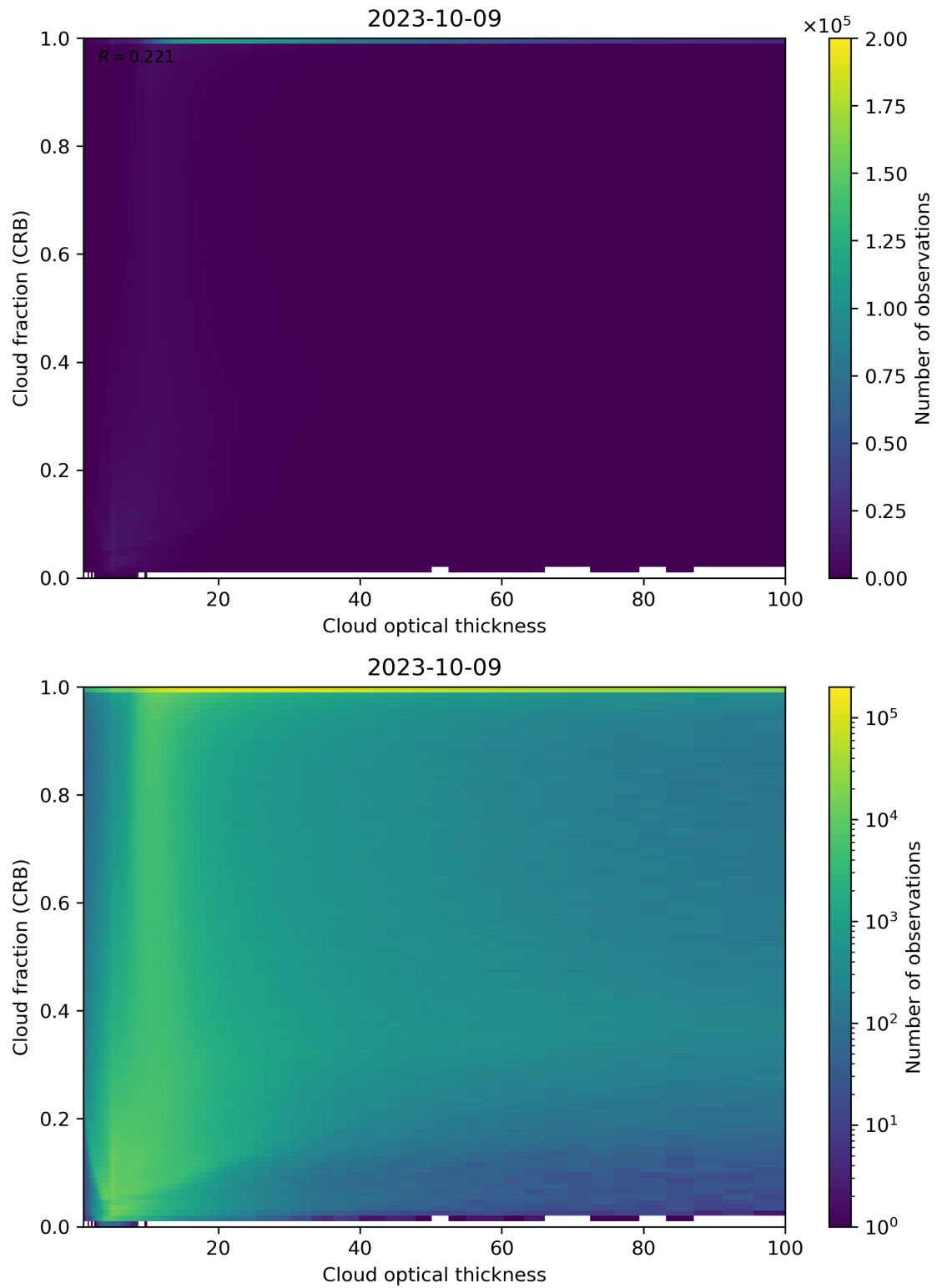
Figure 84: Scatter density plot of “Cloud optical thickness” against “Cloud fraction (CRB)” for 2023-10-08 to 2023-10-10.
