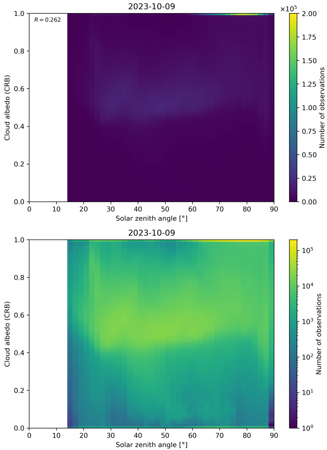
Figure 98: Scatter density plot of “Solar zenith angle” against “Cloud albedo (CRB)” for 2023-10-08 to 2023-10-10.
