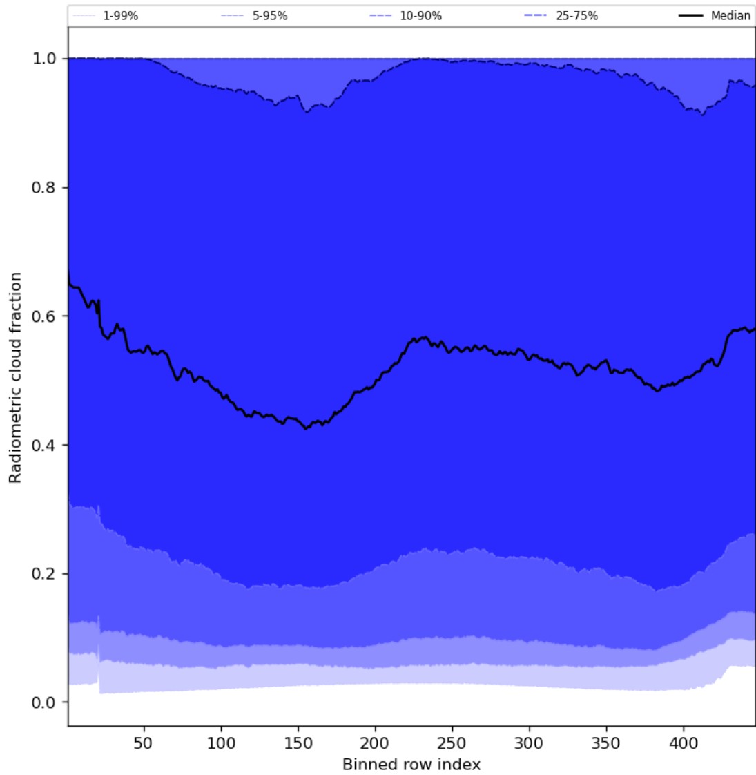
Figure 55: Along track statistics of “Radiometric cloud fraction” for 2023-10-08 to 2023-10-10
