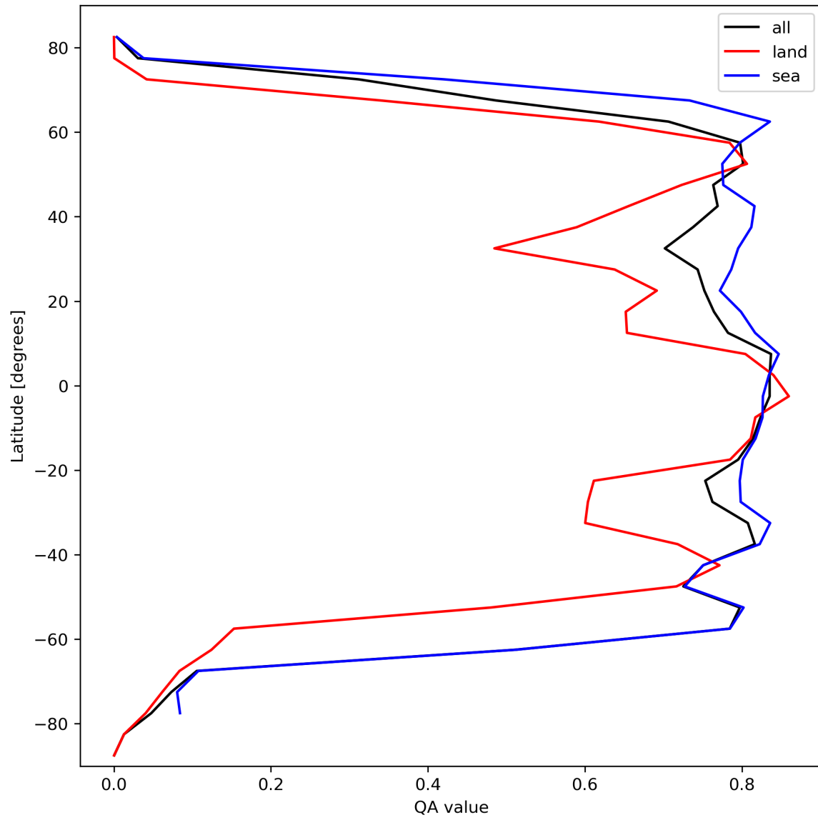
Figure 22: Zonal average of “QA value” for 2023-10-08 to 2023-10-10.
