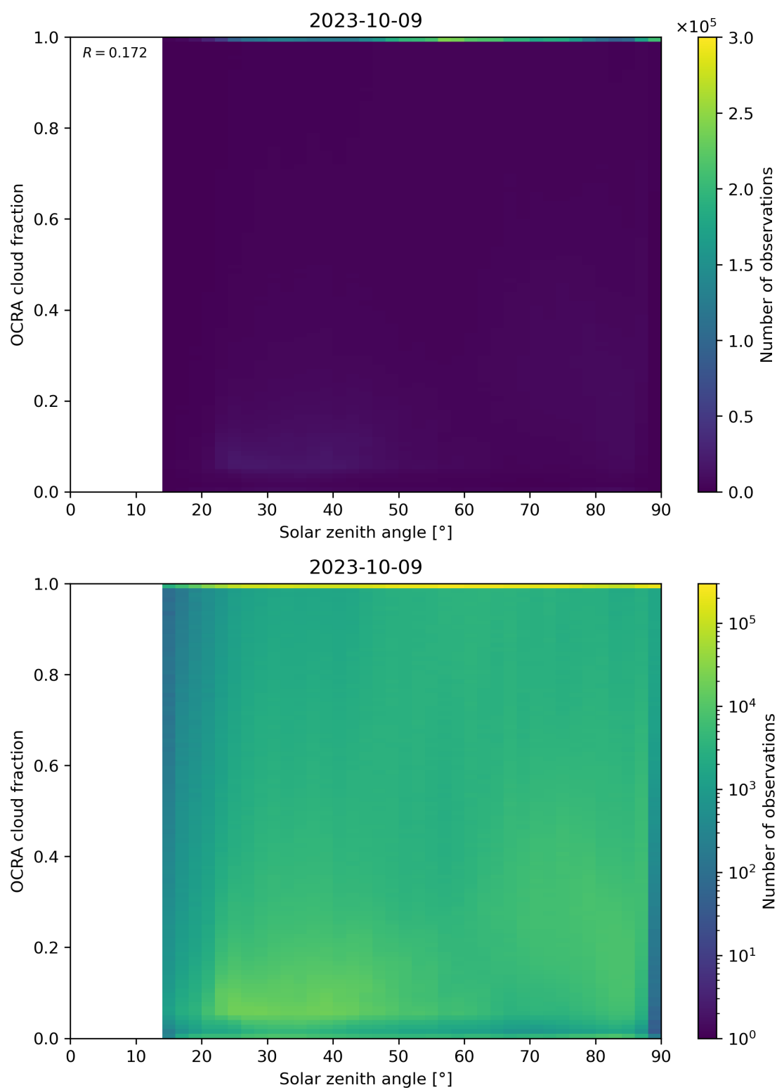
Figure 100: Scatter density plot of “Solar zenith angle” against “OCRA cloud fraction” for 2023-10-08 to 2023-10-10.
