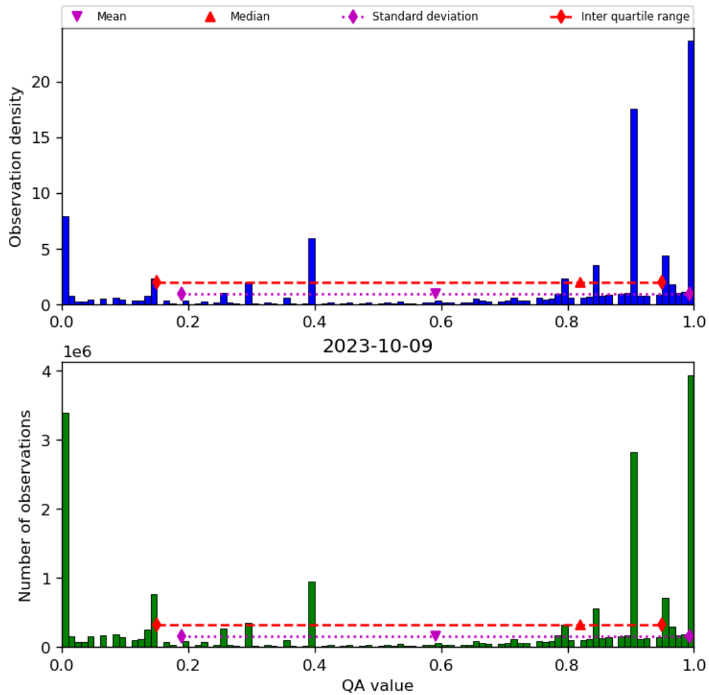
Figure 38: Histogram of “QA value” for 2023-10-08 to 2023-10-10
