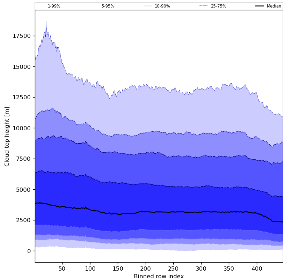
Figure 56: Along track statistics of “Cloud top height” for 2023-10-08 to 2023-10-10
