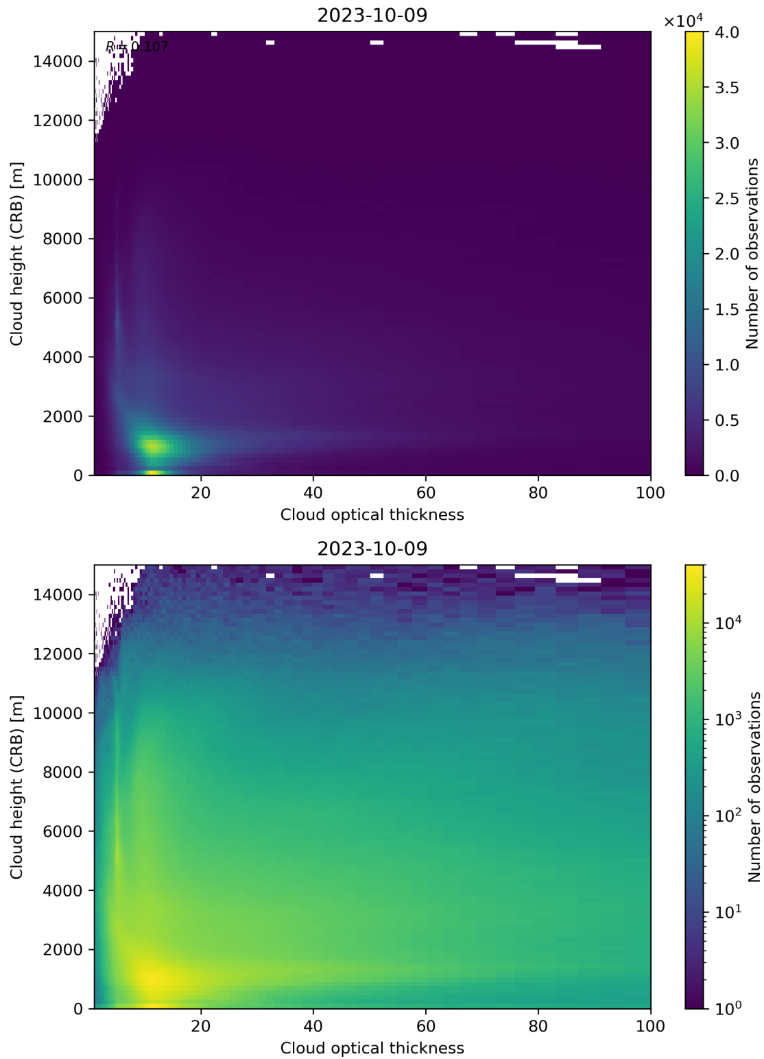
Figure 85: Scatter density plot of “Cloud optical thickness” against “Cloud height (CRB)” for 2023-10-08 to 2023-10-10.
