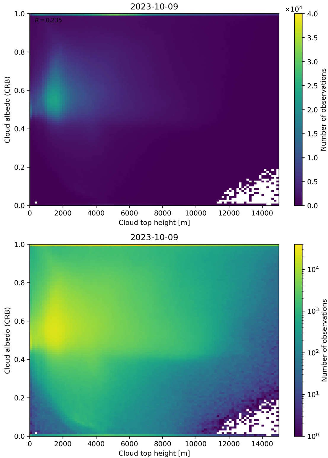
Figure 86: Scatter density plot of “Cloud top height” against “Cloud albedo (CRB)” for 2023-10-08 to 2023-10-10.
