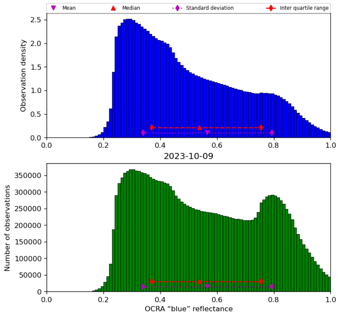
Figure 51: Histogram of “OCRA “blue” reflectance” for 2023-10-08 to 2023-10-10
