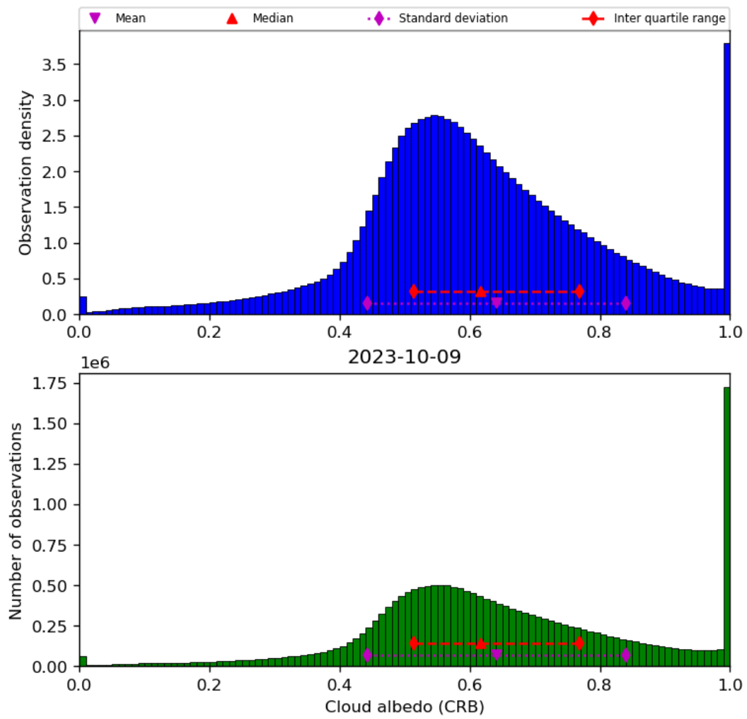
Figure 44: Histogram of “Cloud albedo (CRB)” for 2023-10-08 to 2023-10-10
