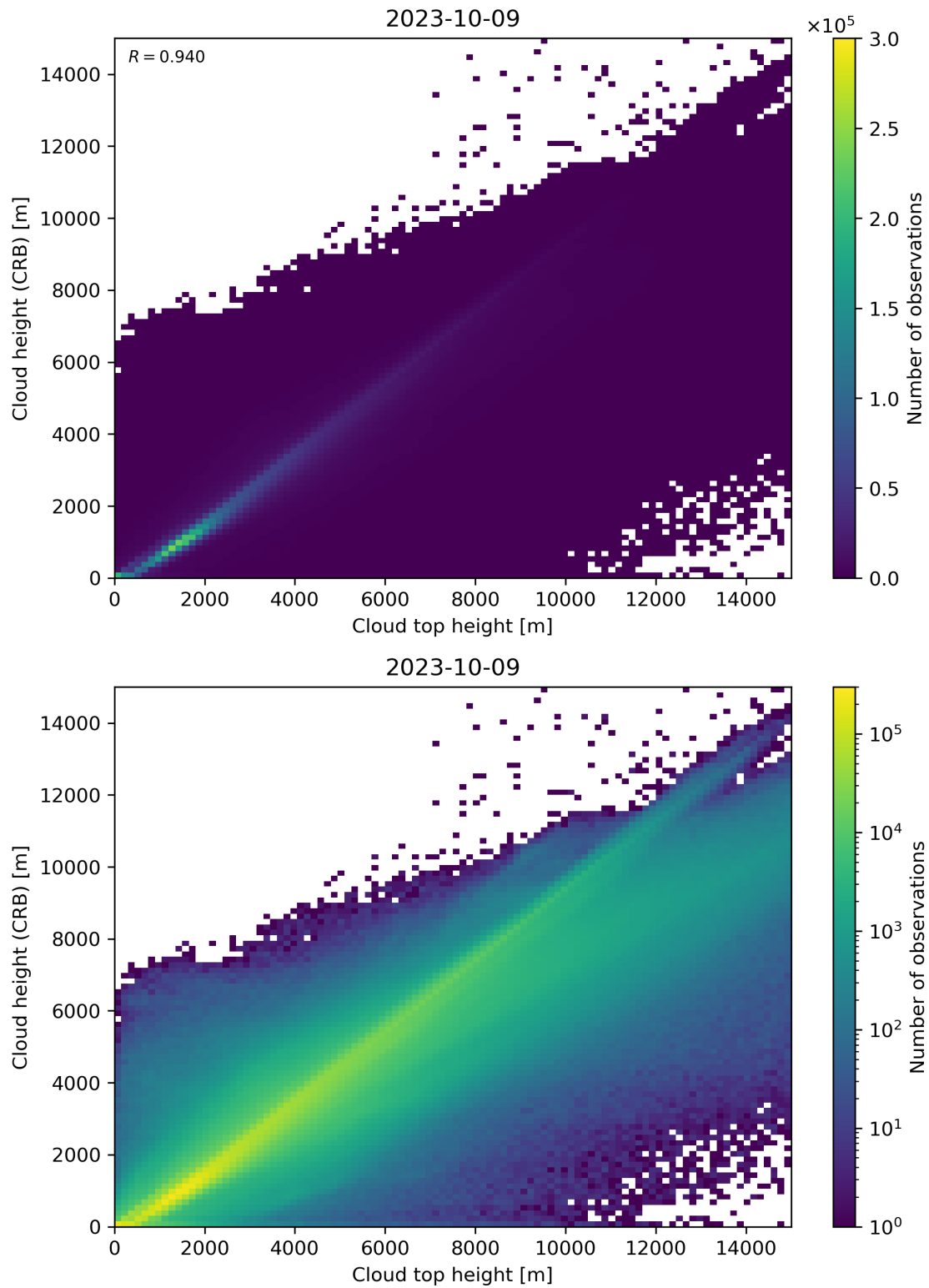
Figure 89: Scatter density plot of “Cloud top height” against “Cloud height (CRB)” for 2023-10-08 to 2023-10-10.
