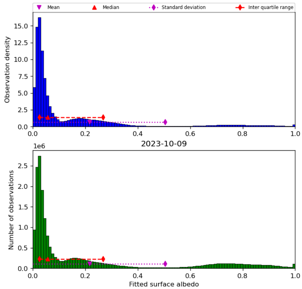
Figure 45: Histogram of “Fitted surface albedo” for 2023-10-08 to 2023-10-10
