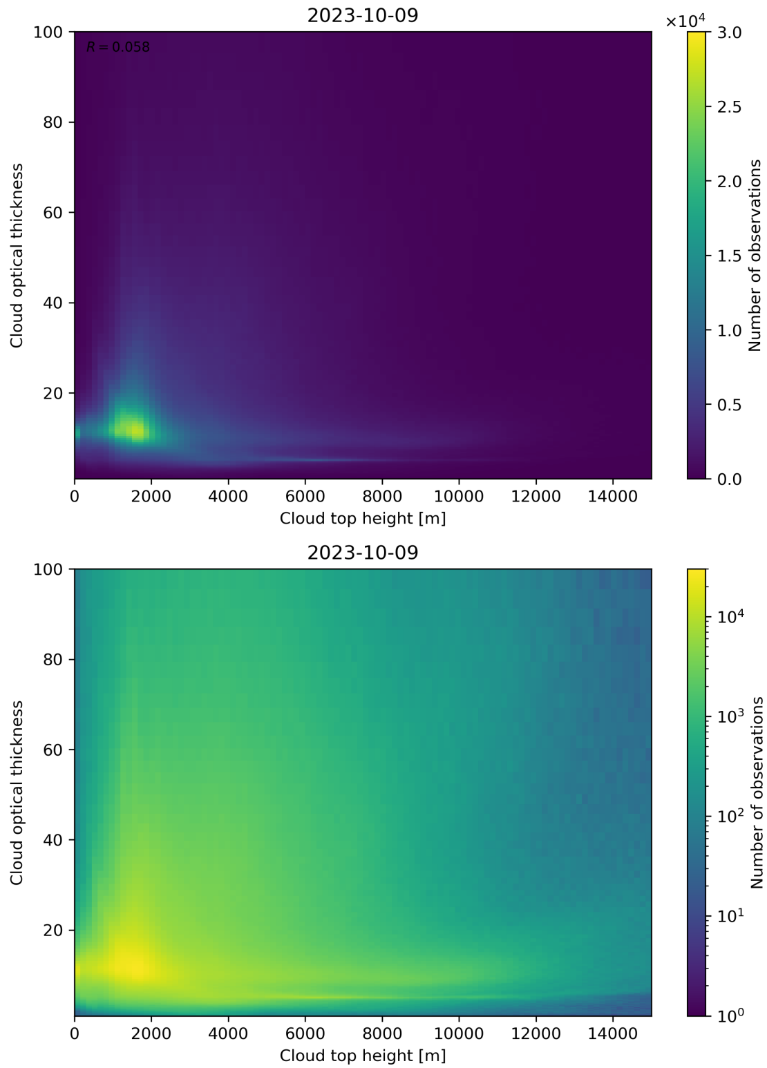
Figure 90: Scatter density plot of “Cloud top height” against “Cloud optical thickness” for 2023-10-08 to 2023-10-10.
