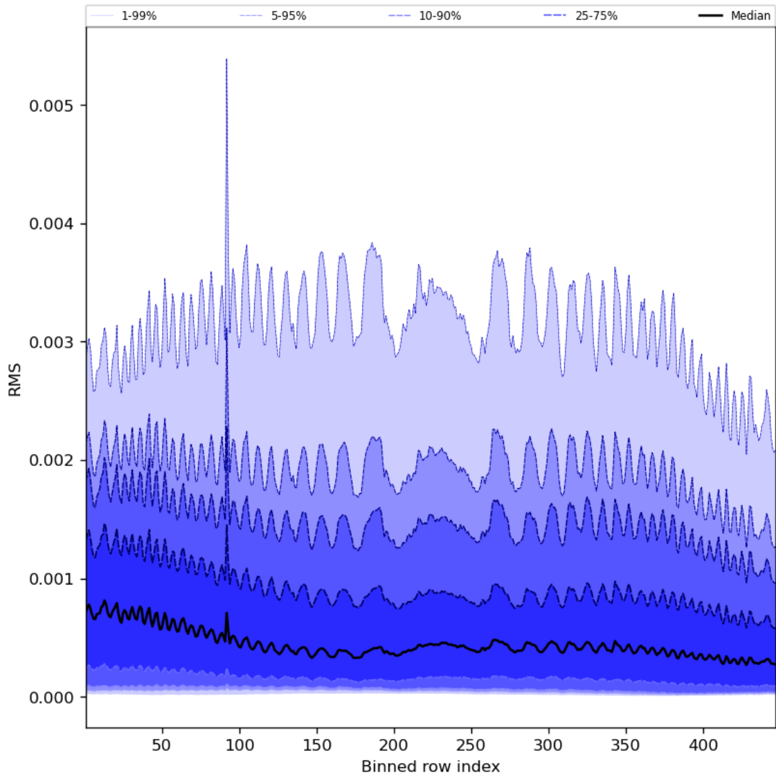
Figure 63: Along track statistics of “RMS” for 2023-10-08 to 2023-10-10
