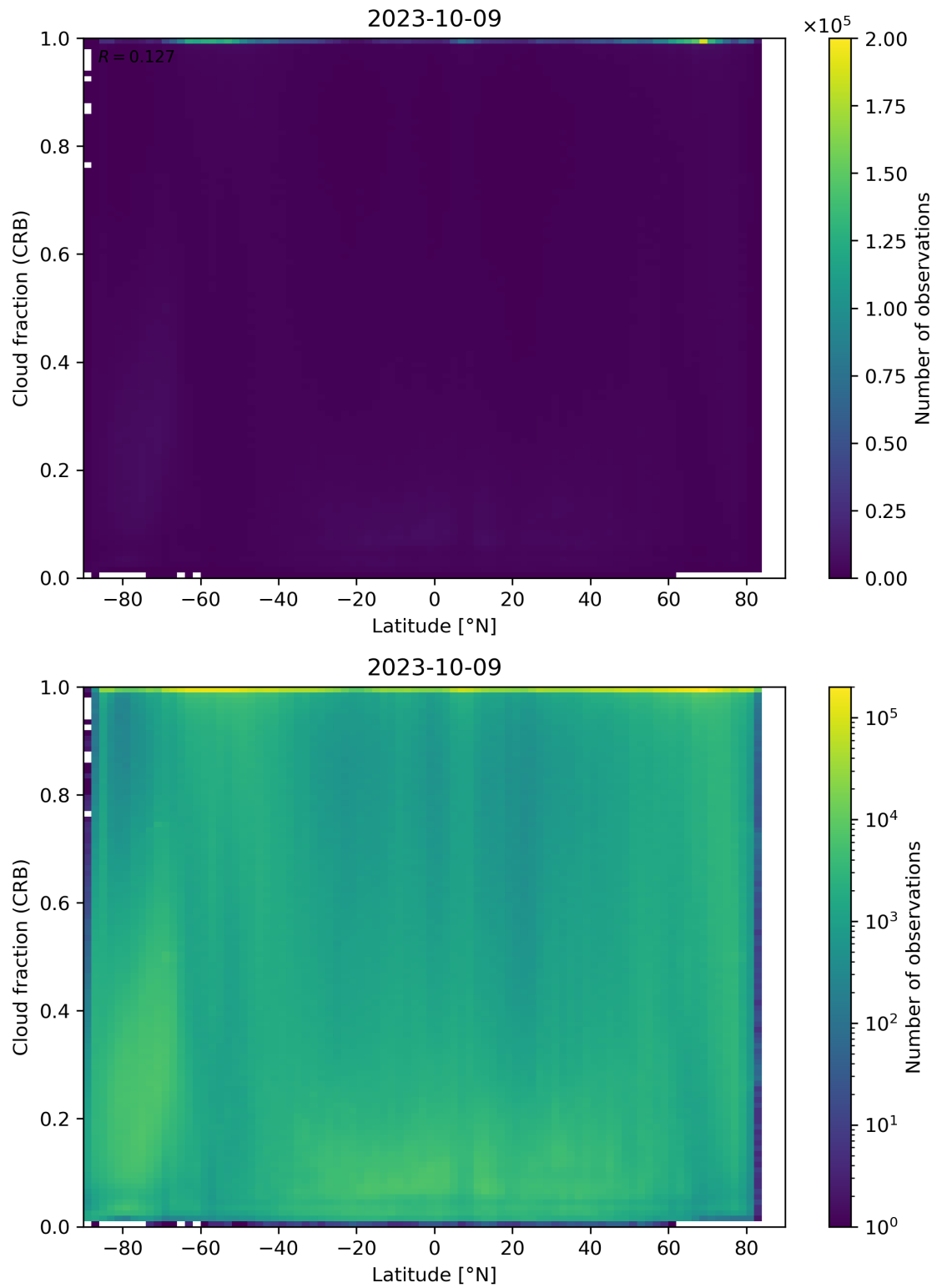
Figure 94: Scatter density plot of “Latitude” against “Cloud fraction (CRB)” for 2023-10-08 to 2023-10-10.
