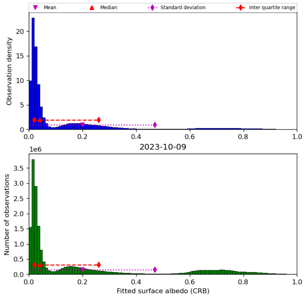
Figure 46: Histogram of “Fitted surface albedo (CRB)” for 2023-10-08 to 2023-10-10
