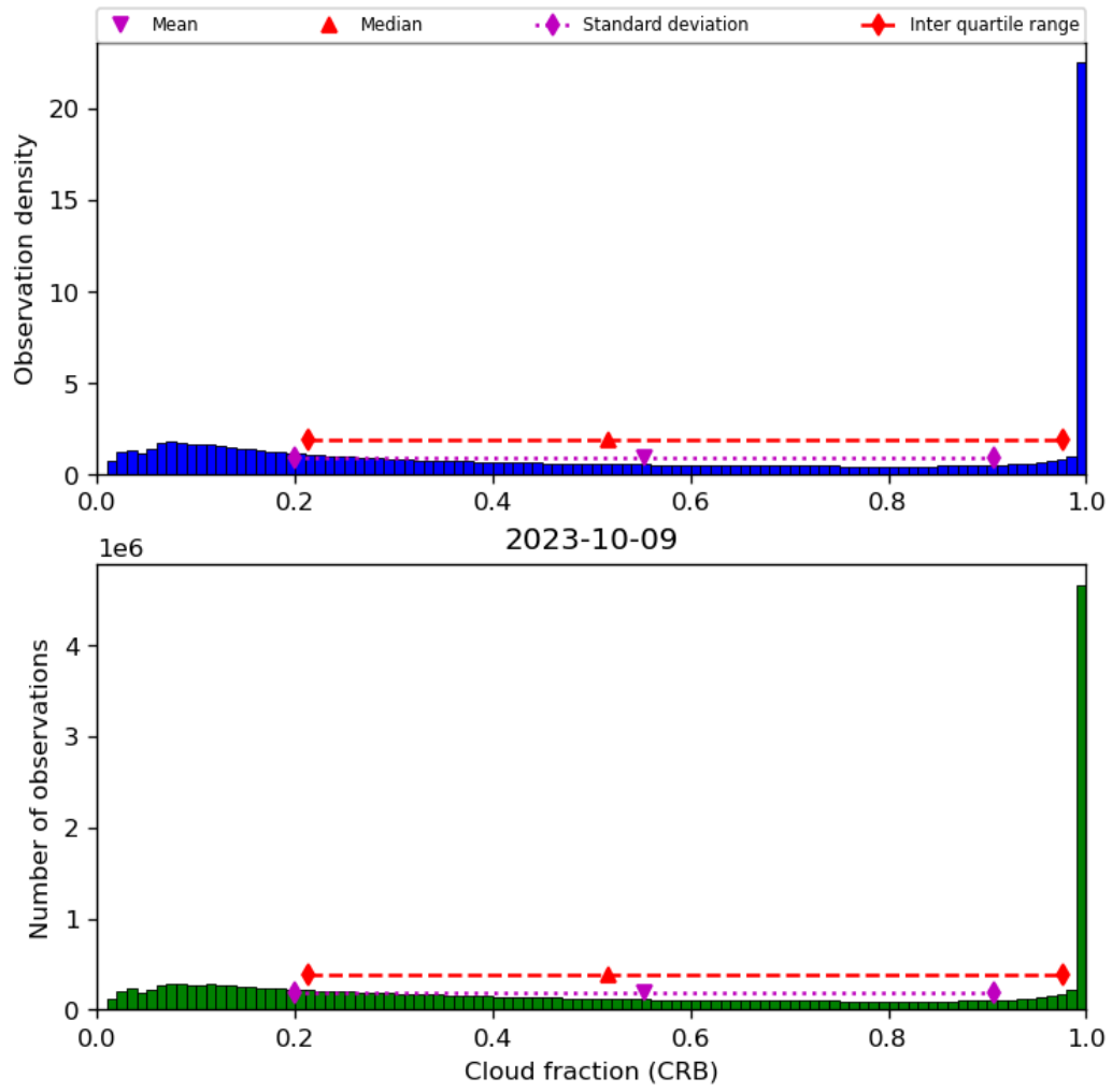
Figure 42: Histogram of “Cloud fraction (CRB)” for 2023-10-08 to 2023-10-10
