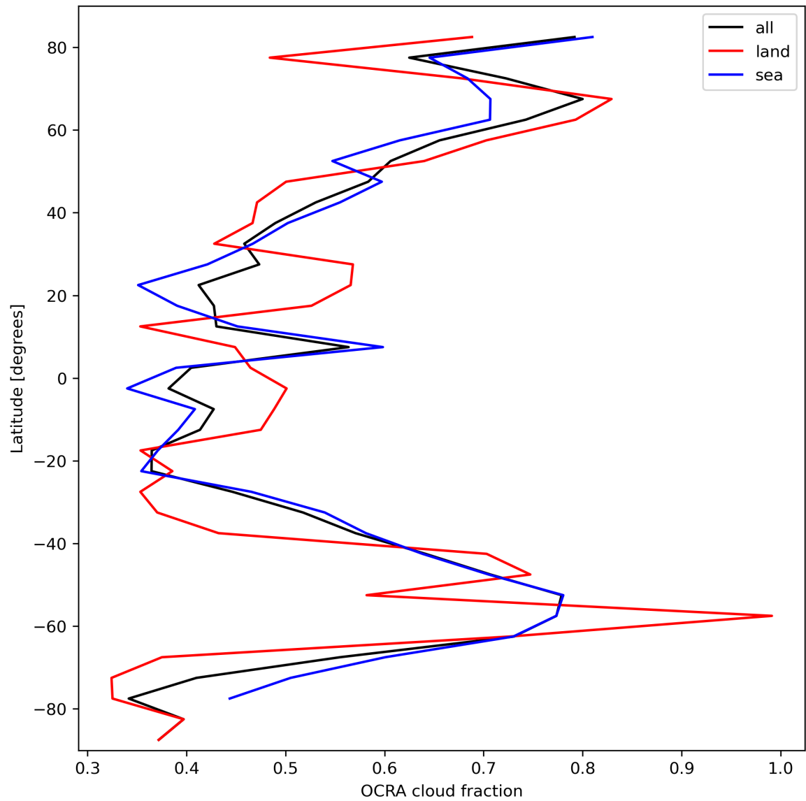
Figure 34: Zonal average of “OCRA cloud fraction” for 2023-10-08 to 2023-10-10.
