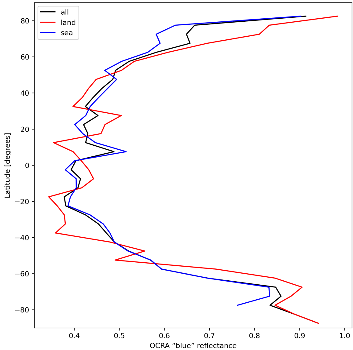
Figure 35: Zonal average of "OCRA "blue" reflectance" for 2023-10-08 to 2023-10-10.
