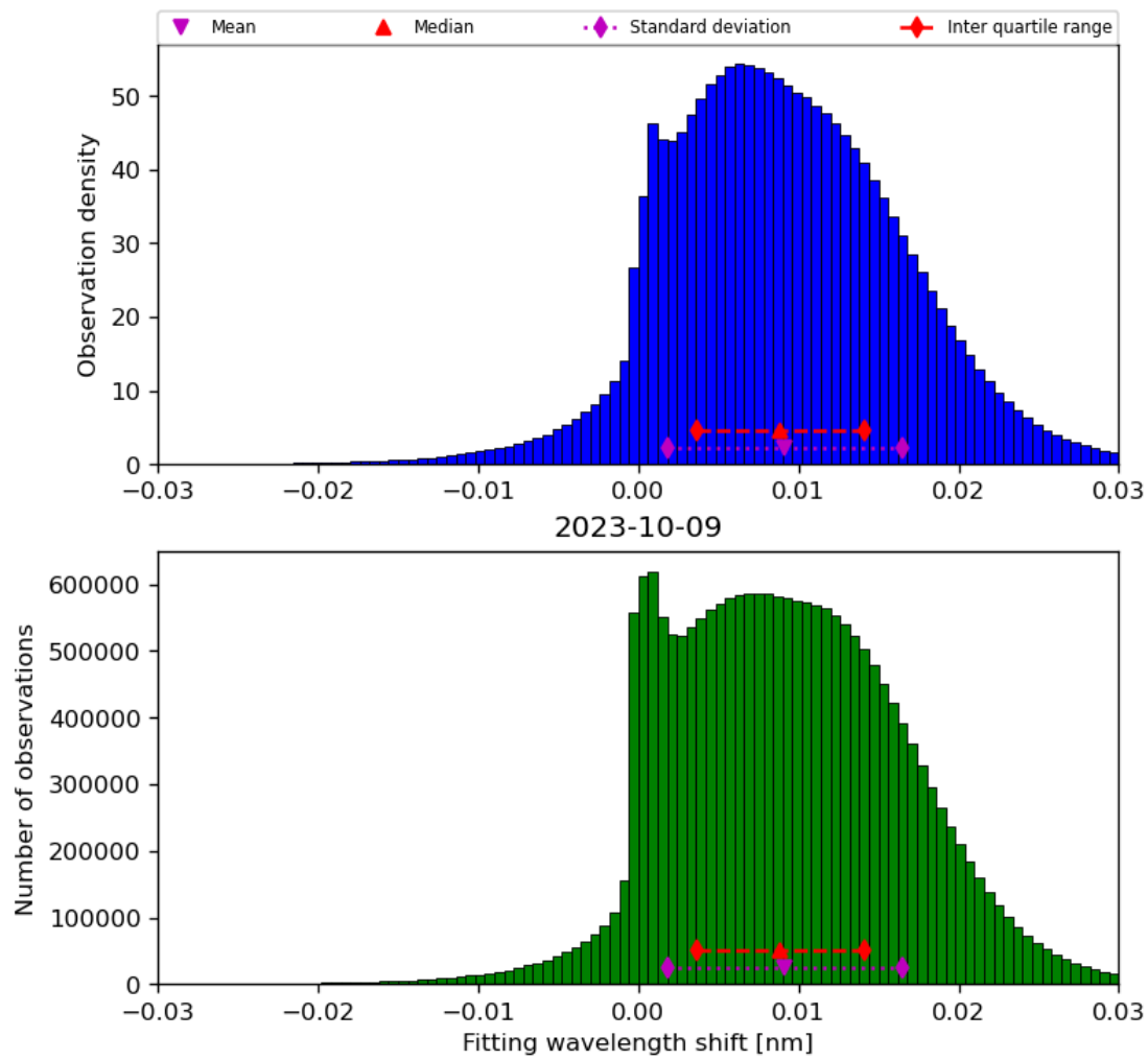
Figure 49: Histogram of “Fitting wavelength shift” for 2023-10-08 to 2023-10-10
