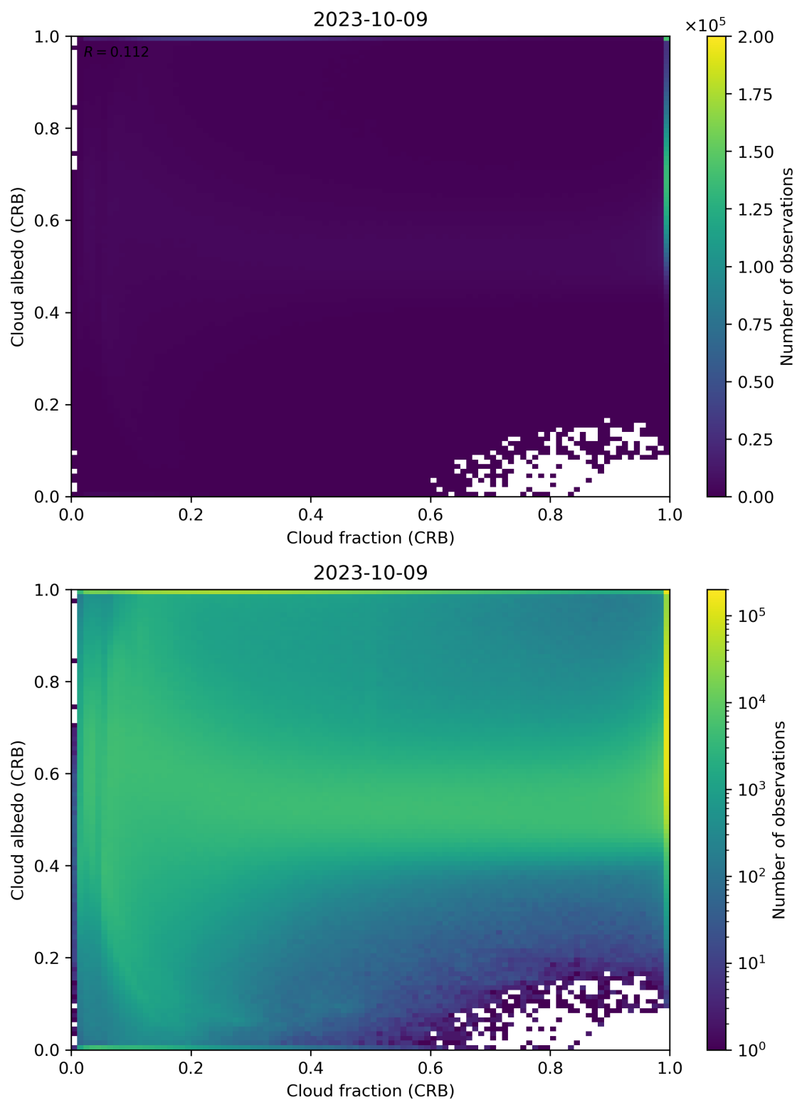
Figure 77: Scatter density plot of “Cloud fraction (CRB)” against “Cloud albedo (CRB)” for 2023-10-08 to 2023-10-10.
