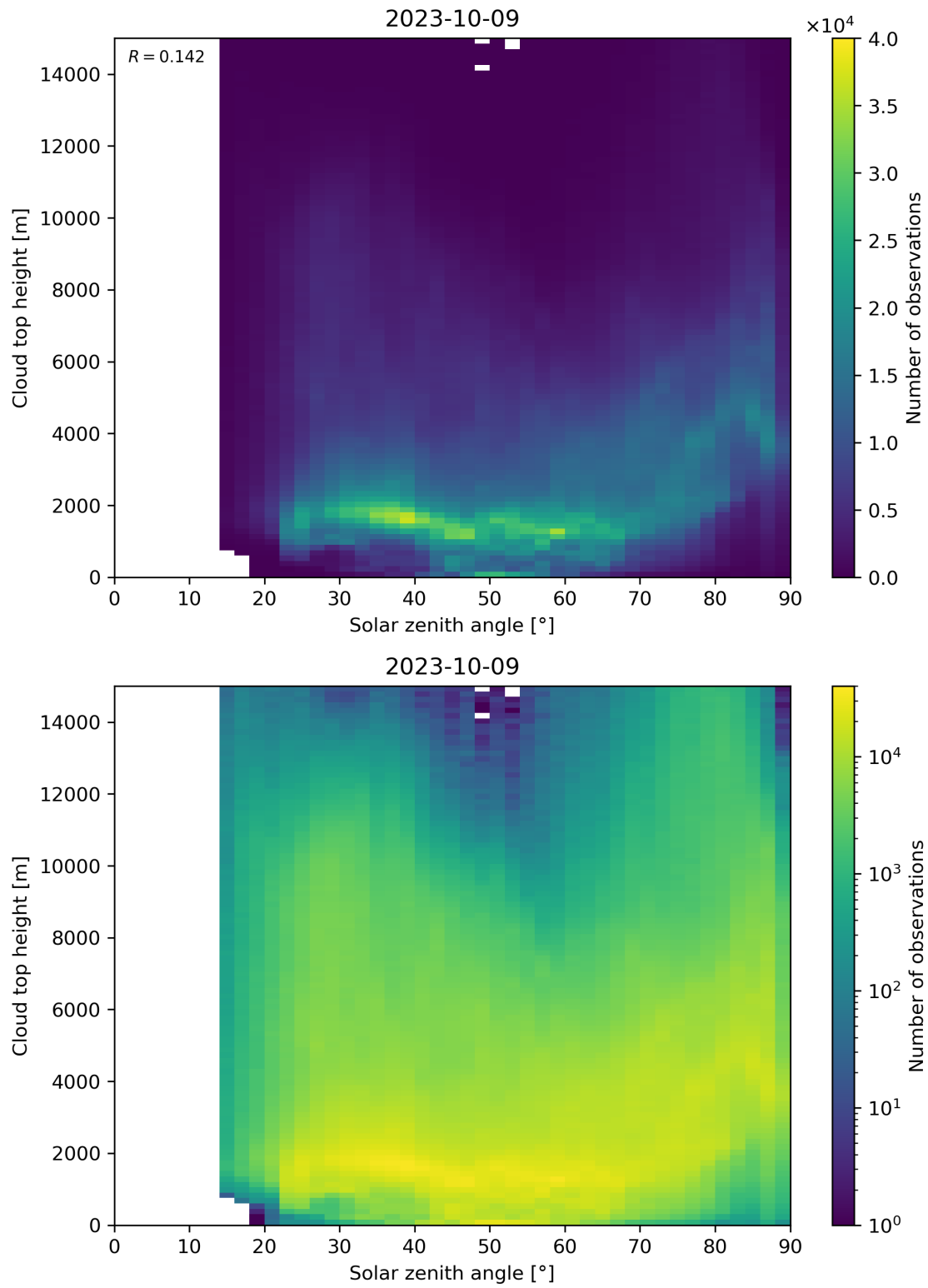
Figure 104: Scatter density plot of “Solar zenith angle” against “Cloud top height” for 2023-10-08 to 2023-10-10.
