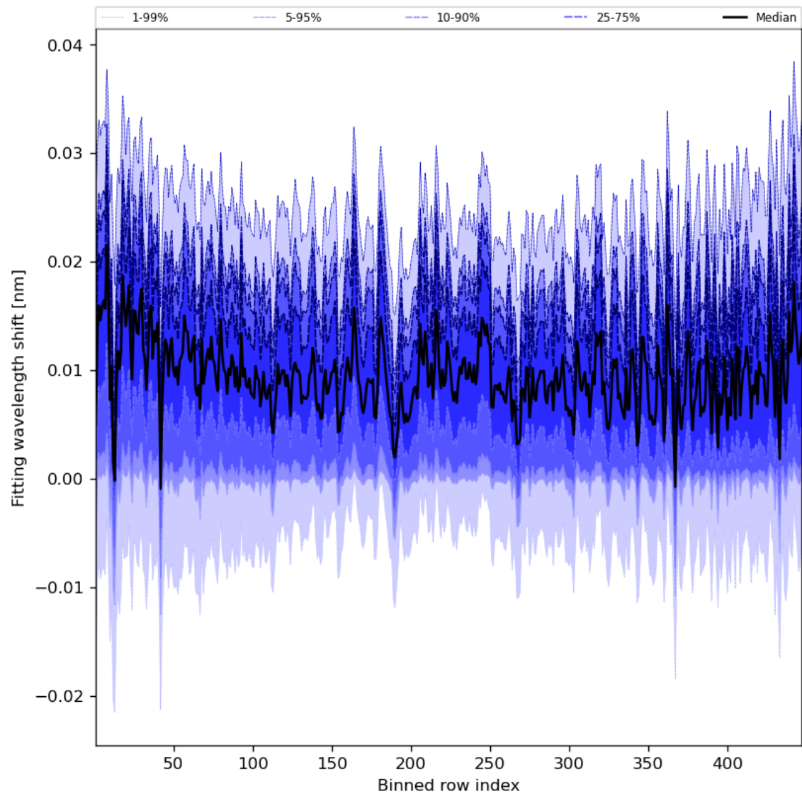
Figure 65: Along track statistics of “Fitting wavelength shift” for 2023-10-08 to 2023-10-10
