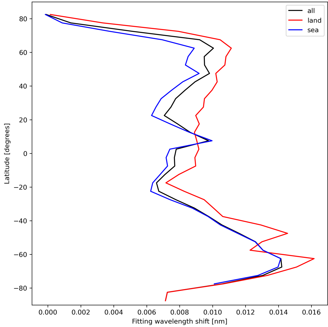
Figure 33: Zonal average of “Fitting wavelength shift” for 2023-10-08 to 2023-10-10.
