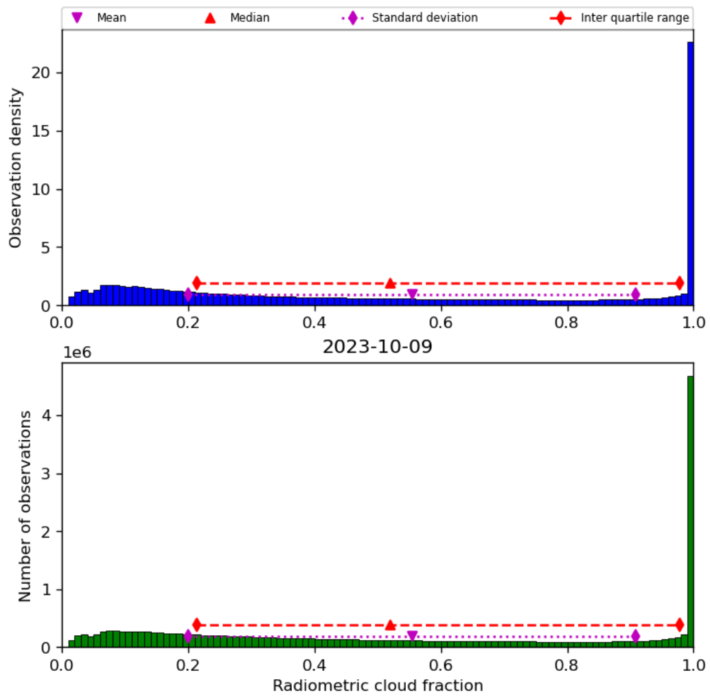
Figure 39: Histogram of “Radiometric cloud fraction” for 2023-10-08 to 2023-10-10
