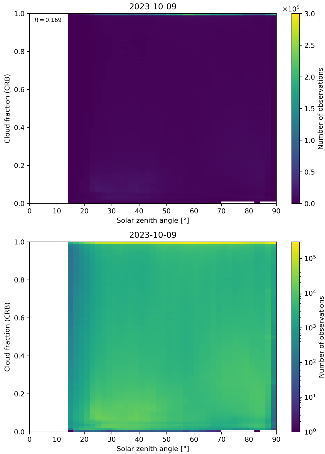
Figure 101: Scatter density plot of “Solar zenith angle” against “Cloud fraction (CRB)” for 2023-10-08 to 2023-10-10.
