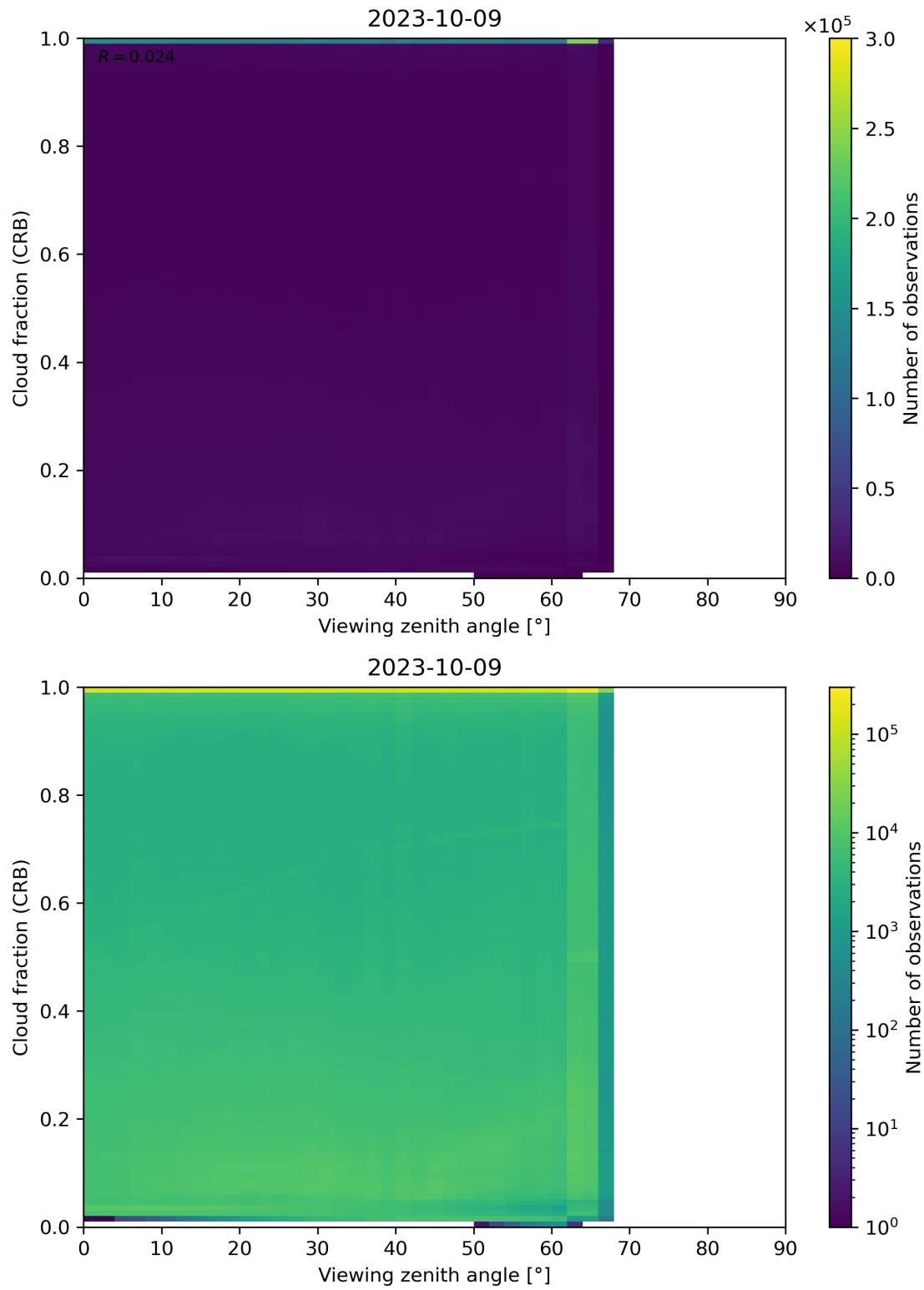
Figure 109: Scatter density plot of “Viewing zenith angle” against “Cloud fraction (CRB)” for 2023-10-08 to 2023-10-10.
