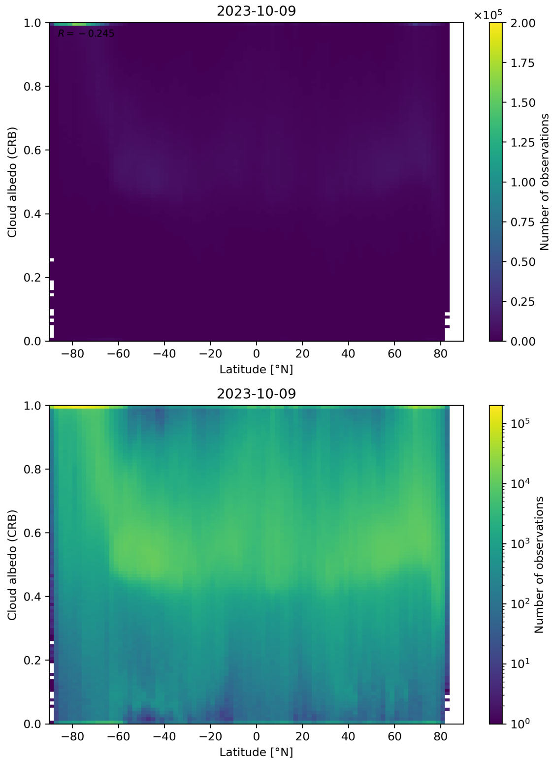
Figure 91: Scatter density plot of “Latitude” against “Cloud albedo (CRB)” for 2023-10-08 to 2023-10-10.
