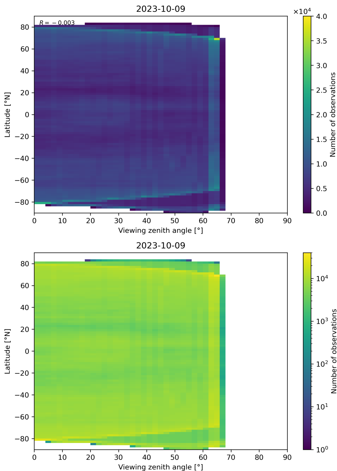
Figure 113: Scatter density plot of “Viewing zenith angle” against “Latitude” for 2023-10-08 to 2023-10-10.
