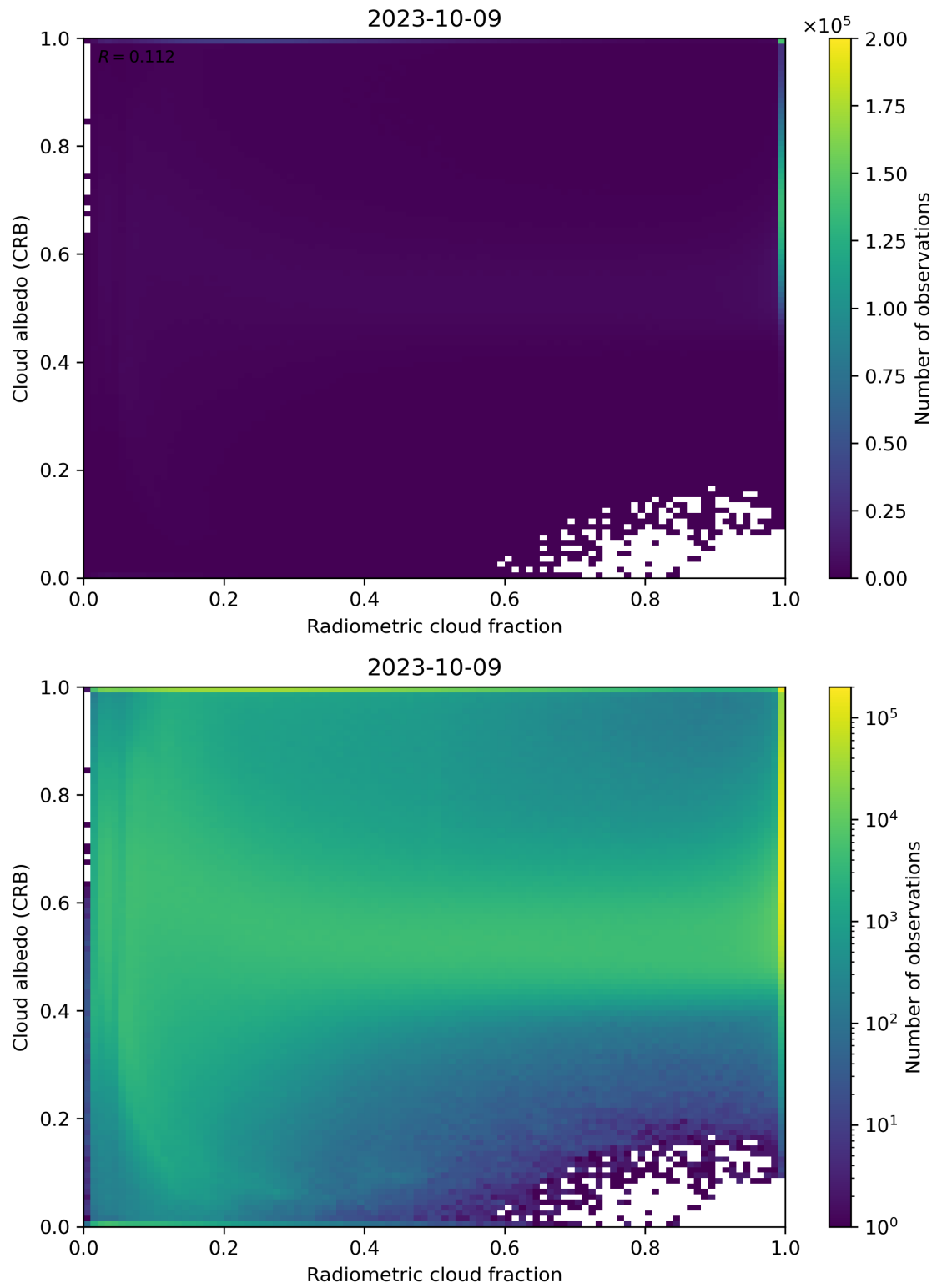
Figure 71: Scatter density plot of “Radiometric cloud fraction” against “Cloud albedo (CRB)” for 2023-10-08 to 2023-10-10.
