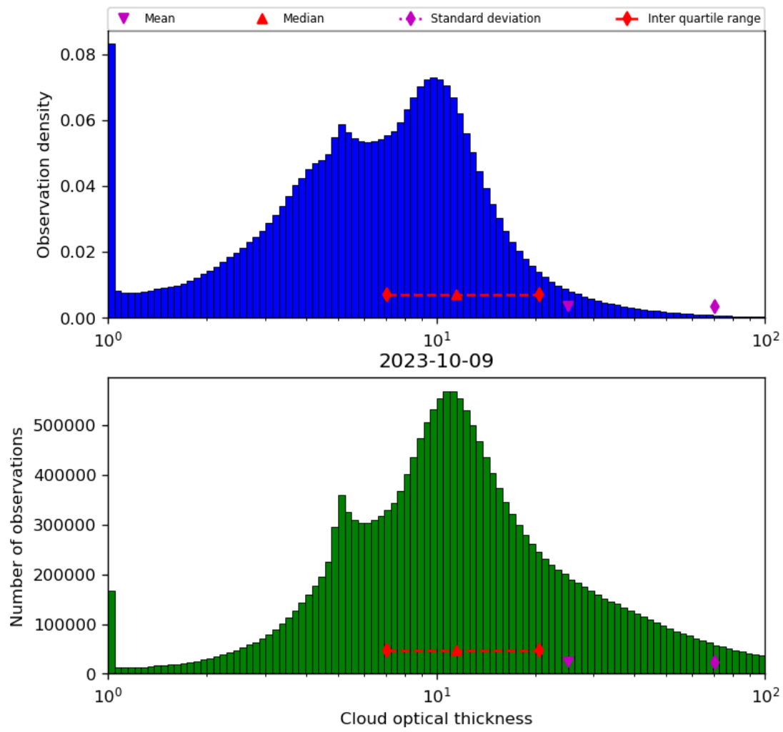
Figure 41: Histogram of “Cloud optical thickness” for 2023-10-08 to 2023-10-10
