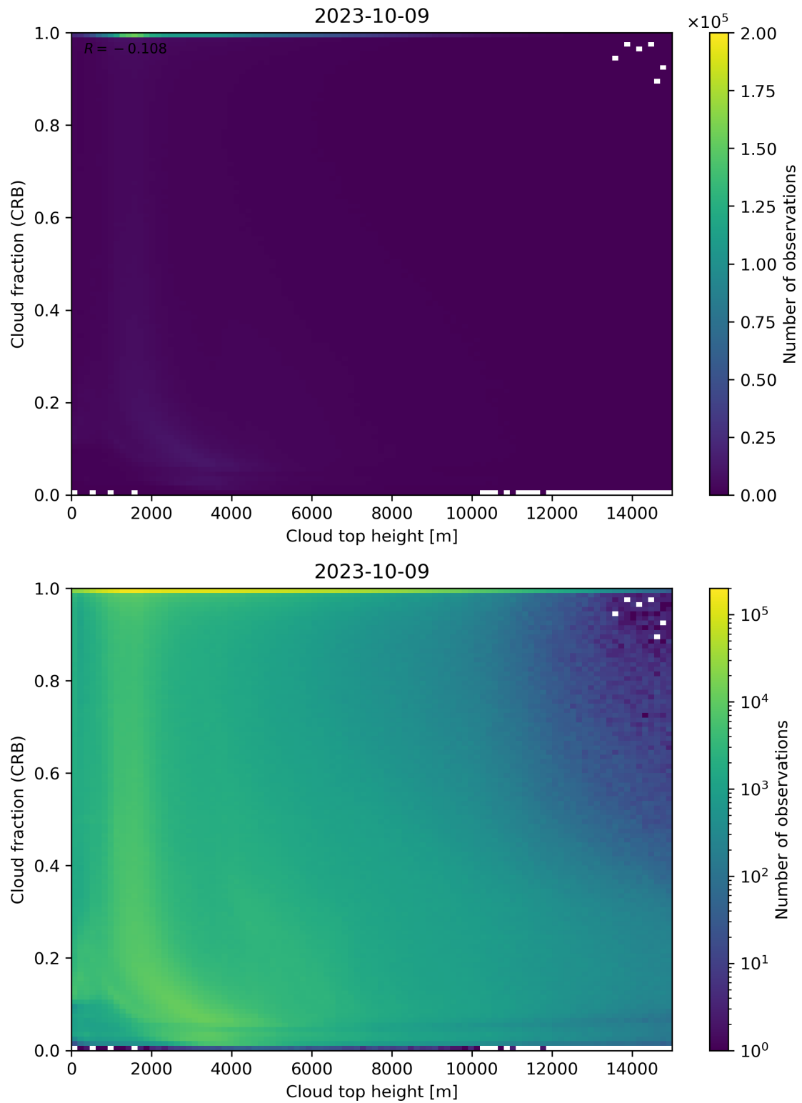
Figure 88: Scatter density plot of “Cloud top height” against “Cloud fraction (CRB)” for 2023-10-08 to 2023-10-10.
