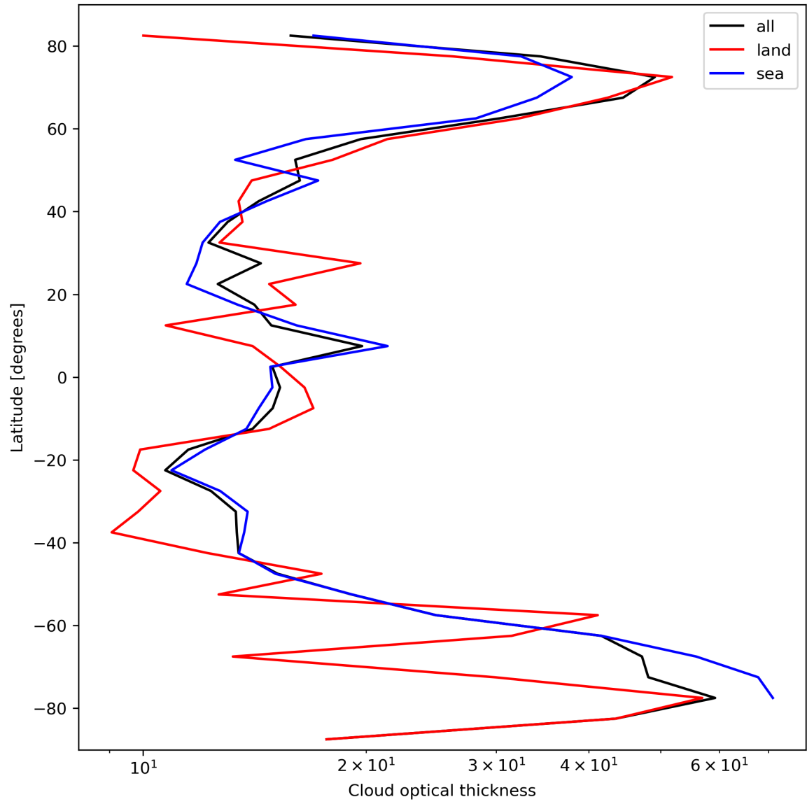
Figure 25: Zonal average of “Cloud optical thickness” for 2023-10-08 to 2023-10-10.
