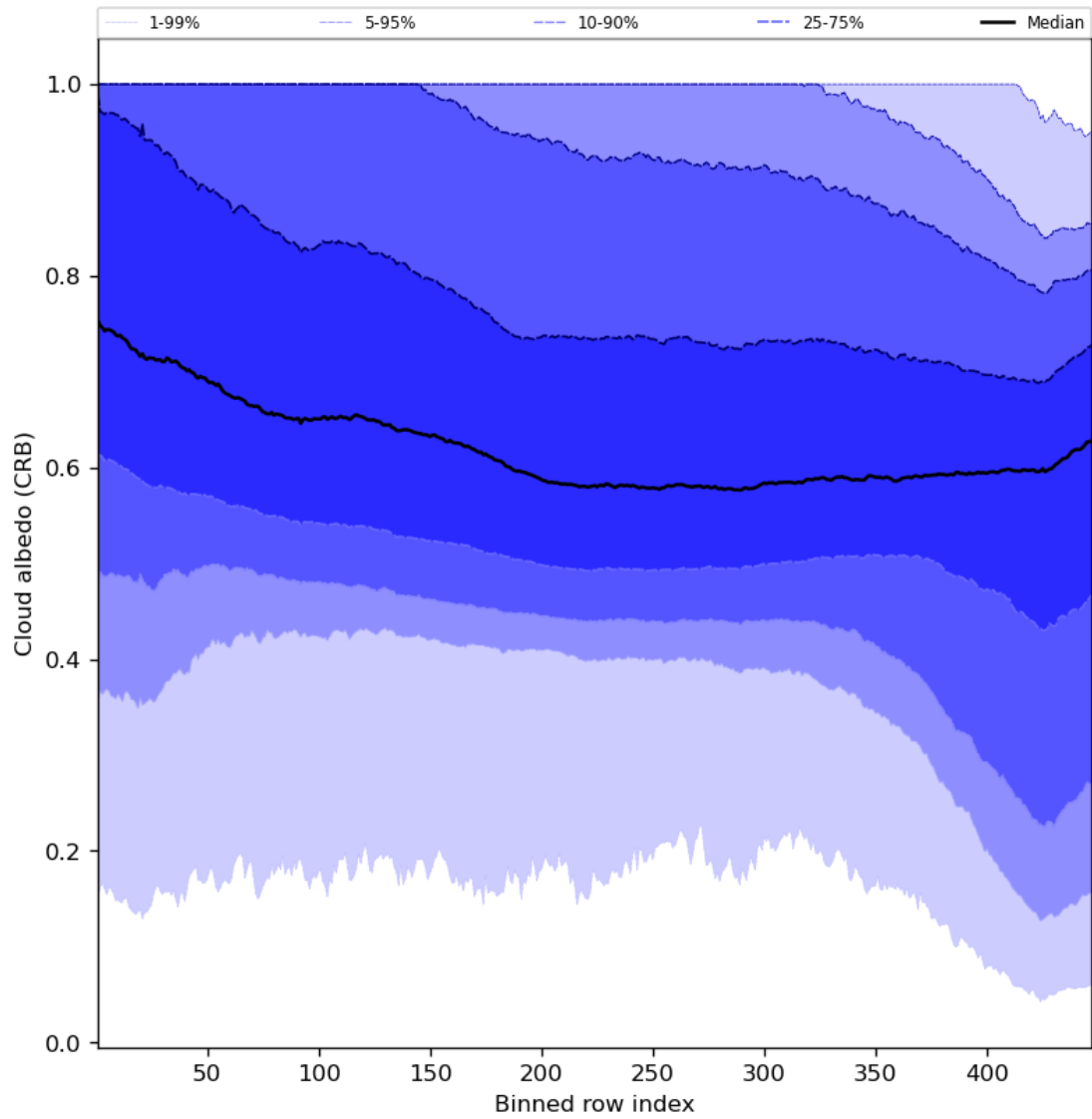
Figure 60: Along track statistics of “Cloud albedo (CRB)” for 2023-10-08 to 2023-10-10
