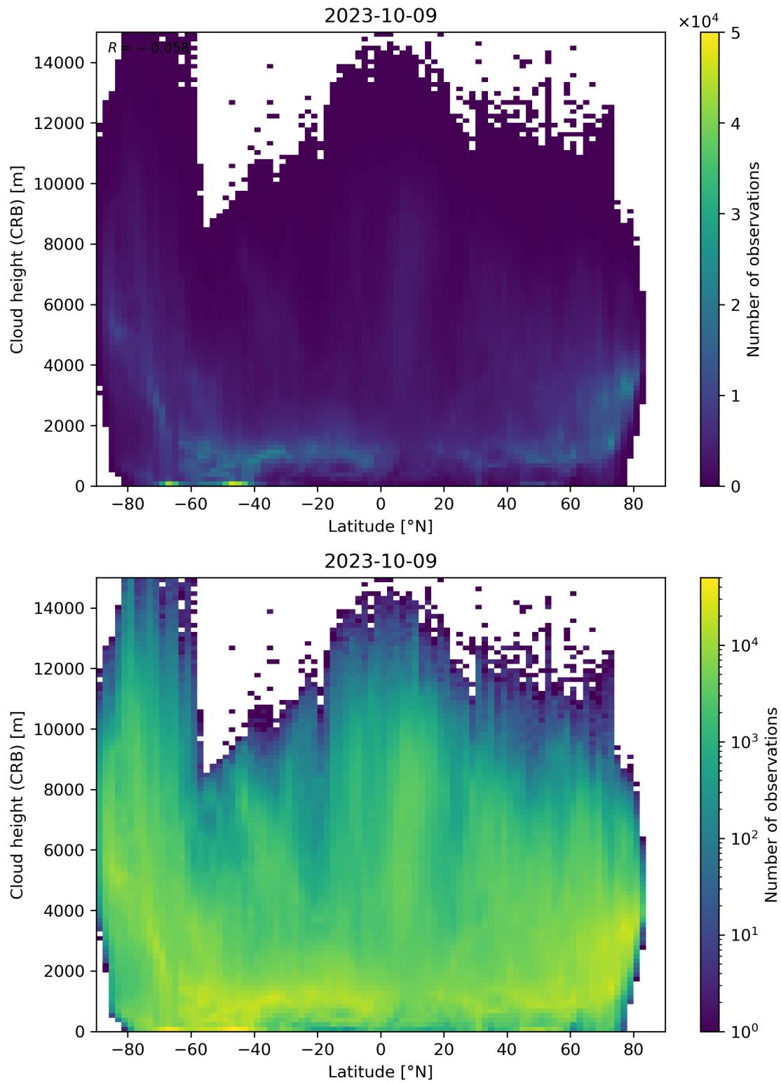
Figure 95: Scatter density plot of “Latitude” against “Cloud height (CRB)” for 2023-10-08 to 2023-10-10.
