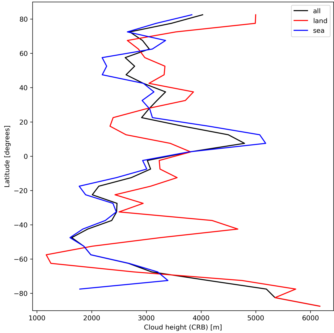
Figure 27: Zonal average of “Cloud height (CRB)” for 2023-10-08 to 2023-10-10.
