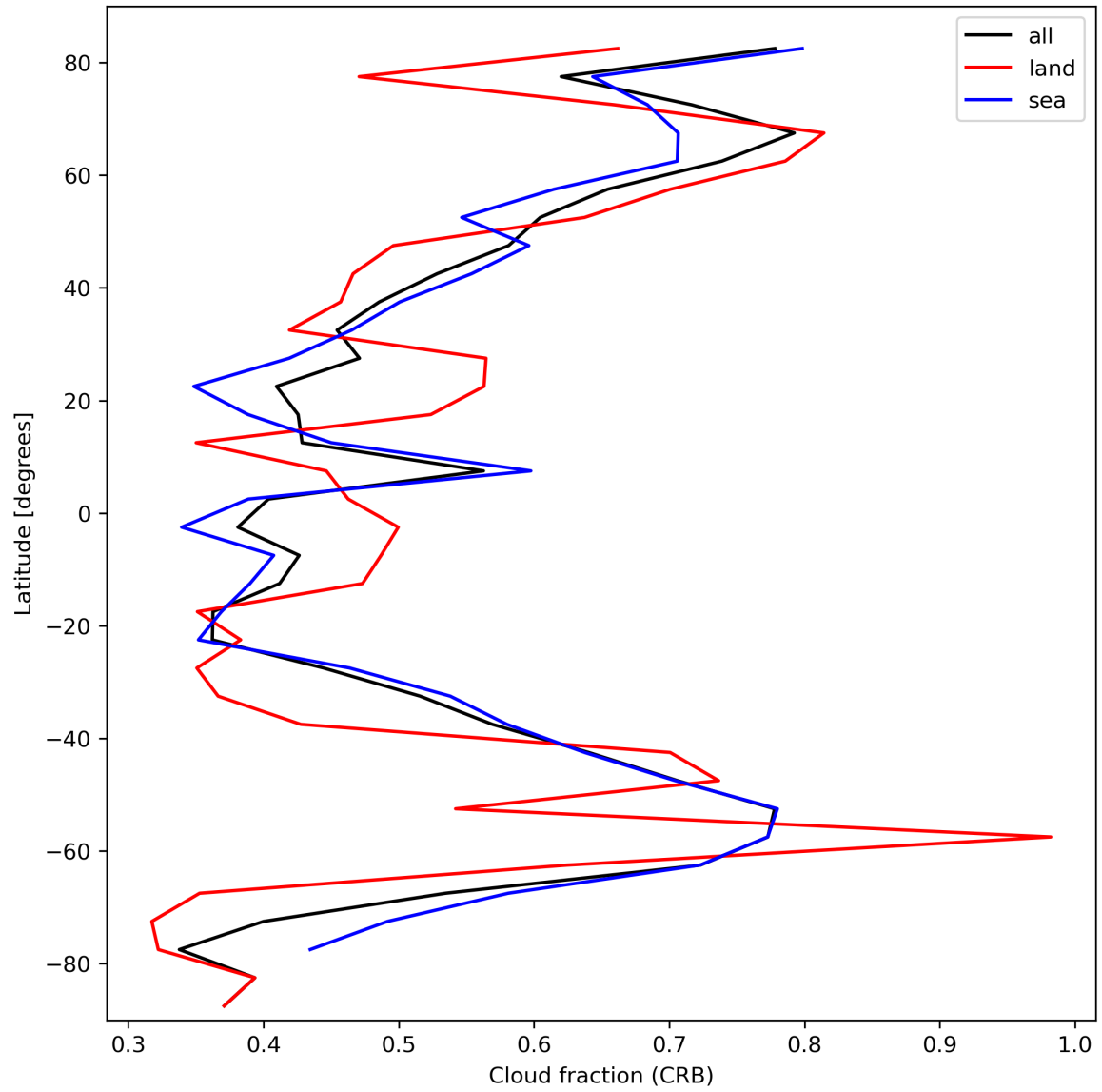
Figure 26: Zonal average of “Cloud fraction (CRB)” for 2023-10-08 to 2023-10-10.
