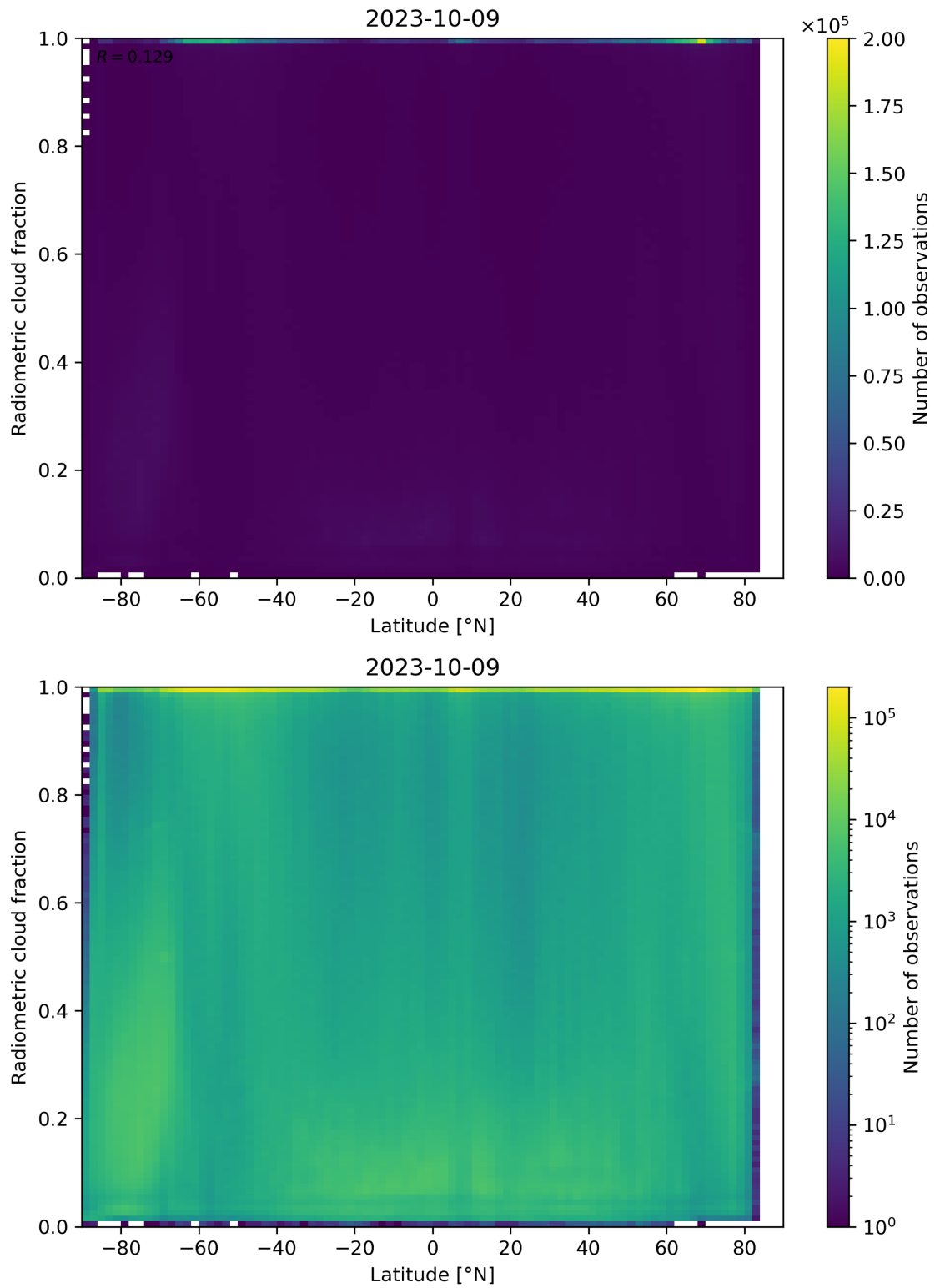
Figure 92: Scatter density plot of “Latitude” against “Radiometric cloud fraction” for 2023-10-08 to 2023-10-10.
