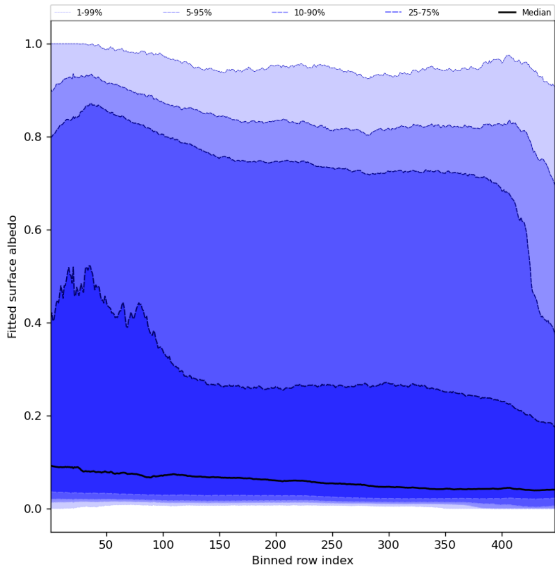
Figure 61: Along track statistics of “Fitted surface albedo” for 2023-10-08 to 2023-10-10
