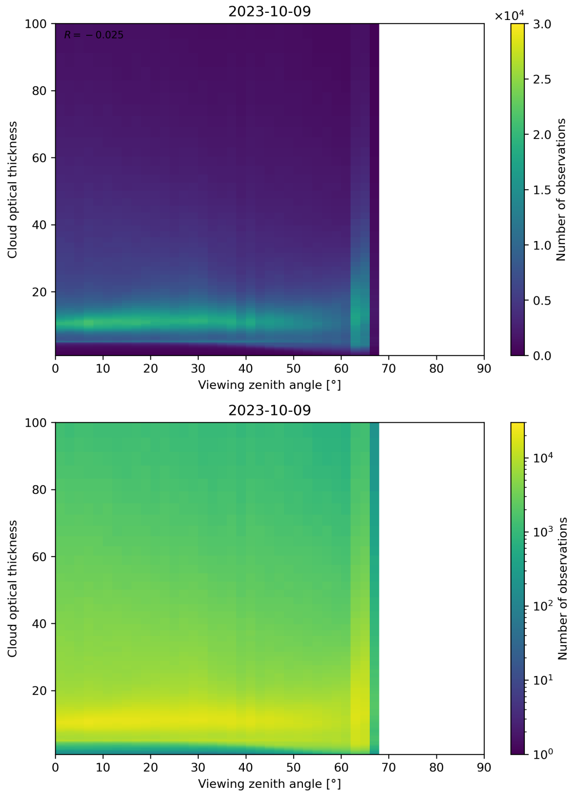
Figure 111: Scatter density plot of “Viewing zenith angle” against “Cloud optical thickness” for 2023-10-08 to 2023-10-10.
