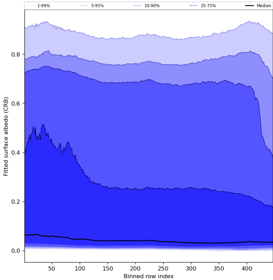
Figure 62: Along track statistics of “Fitted surface albedo (CRB)” for 2023-10-08 to 2023-10-10
