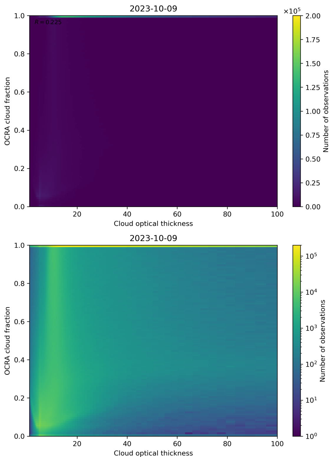
Figure 83: Scatter density plot of “Cloud optical thickness” against “OCRA cloud fraction” for 2023-10-08 to 2023-10-10.
