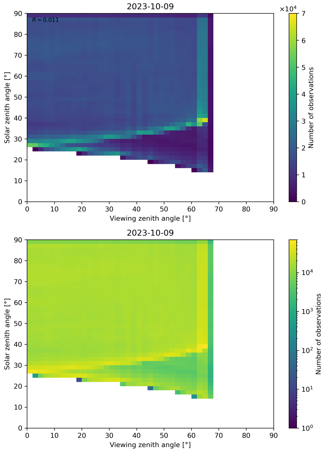
Figure 114: Scatter density plot of “Viewing zenith angle” against “Solar zenith angle” for 2023-10-08 to 2023-10-10.
