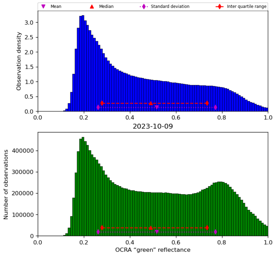
Figure 52: Histogram of “OCRA “green” reflectance” for 2023-10-08 to 2023-10-10
