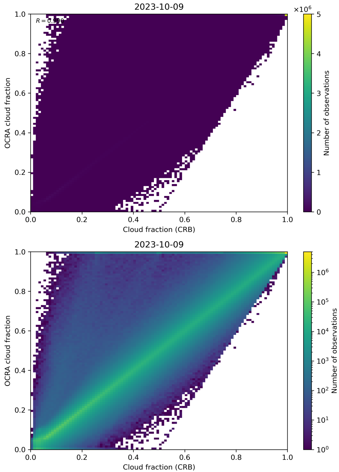
Figure 78: Scatter density plot of “Cloud fraction (CRB)” against “OCRA cloud fraction” for 2023-10-08 to 2023-10-10.
