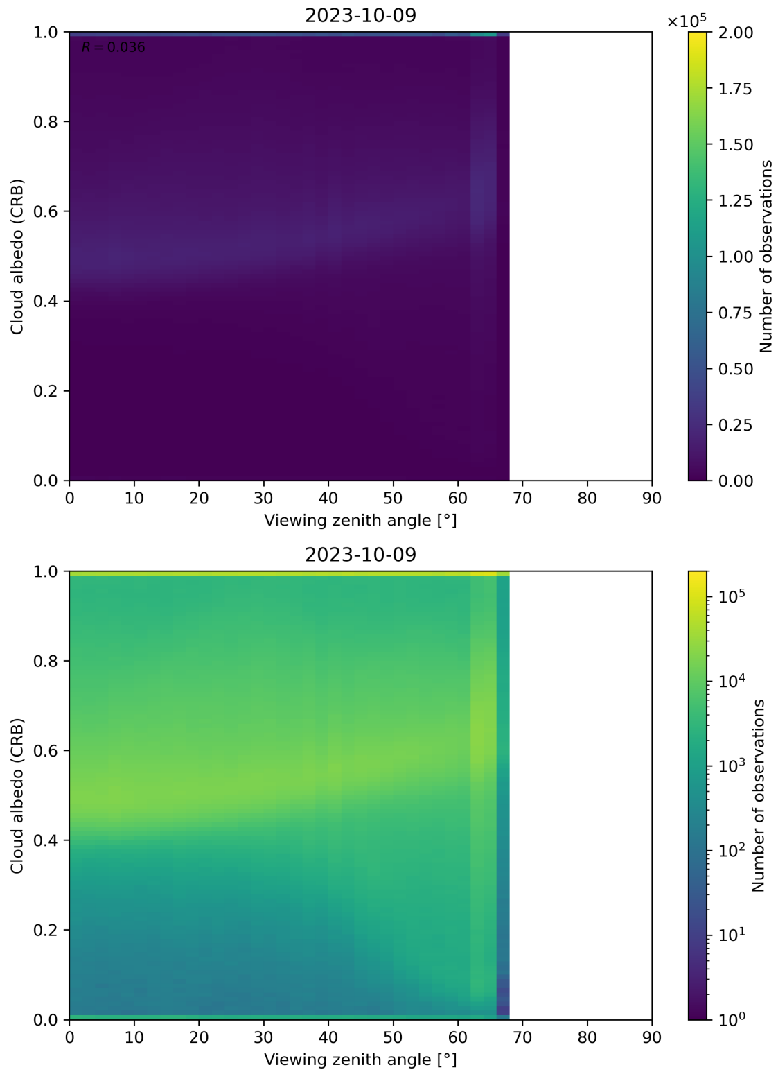
Figure 106: Scatter density plot of “Viewing zenith angle” against “Cloud albedo (CRB)” for 2023-10-08 to 2023-10-10.
