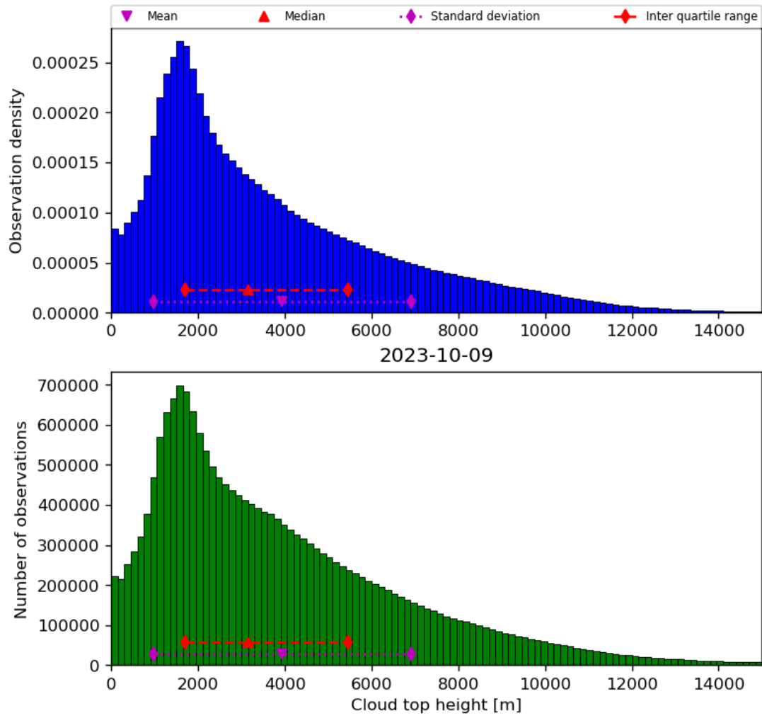
Figure 40: Histogram of “Cloud top height” for 2023-10-08 to 2023-10-10
