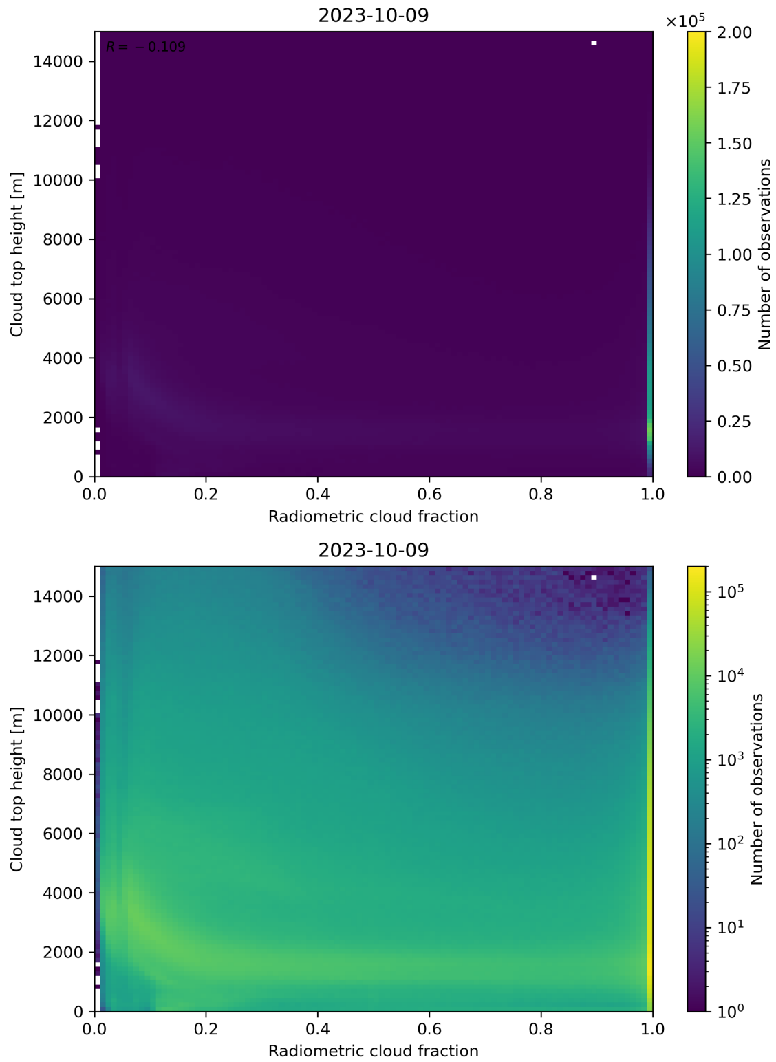
Figure 76: Scatter density plot of “Radiometric cloud fraction” against “Cloud top height” for 2023-10-08 to 2023-10-10.
