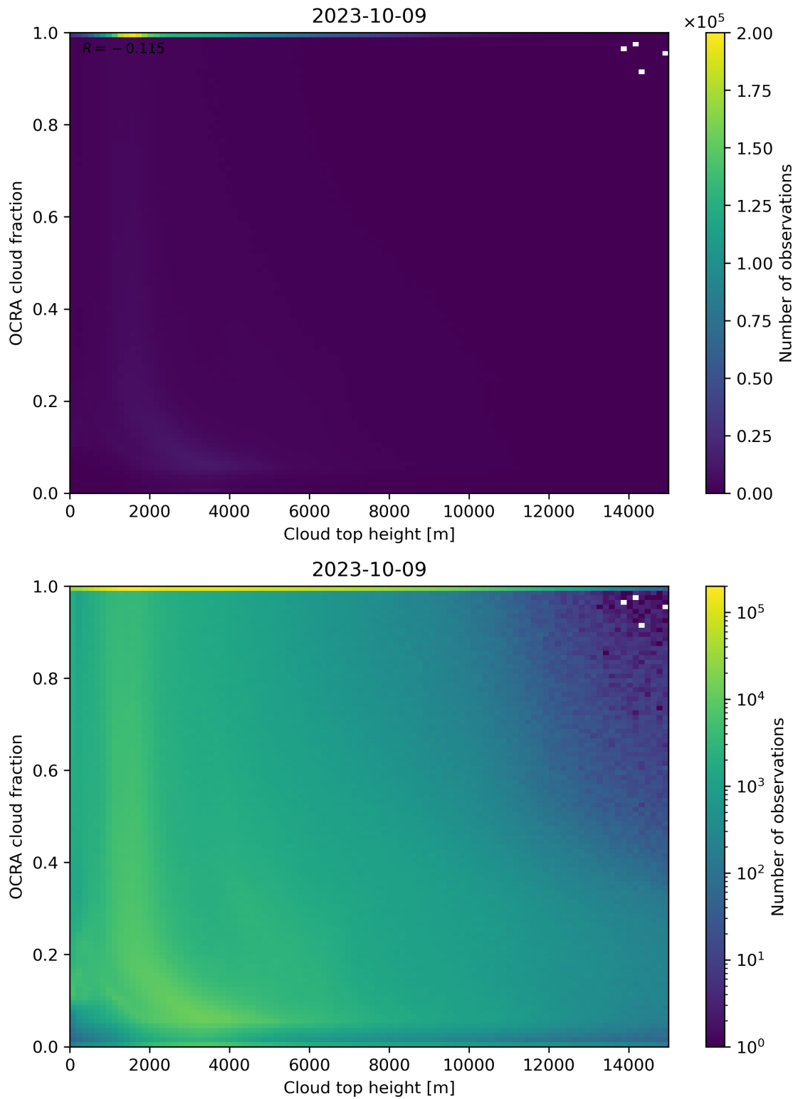
Figure 87: Scatter density plot of “Cloud top height” against “OCRA cloud fraction” for 2023-10-08 to 2023-10-10.
