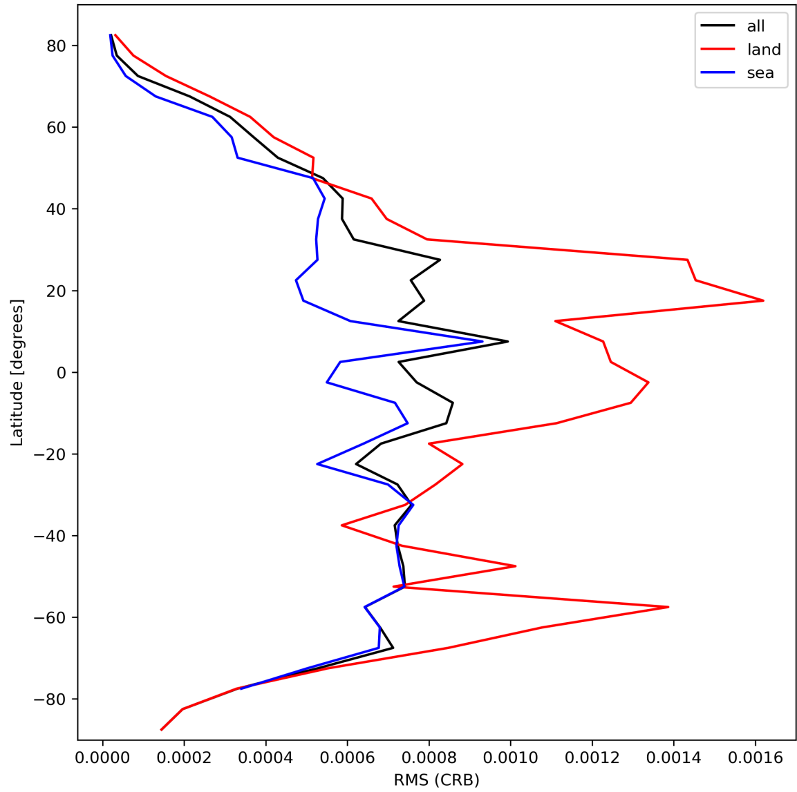
Figure 32: Zonal average of “RMS (CRB)” for 2023-10-08 to 2023-10-10.
