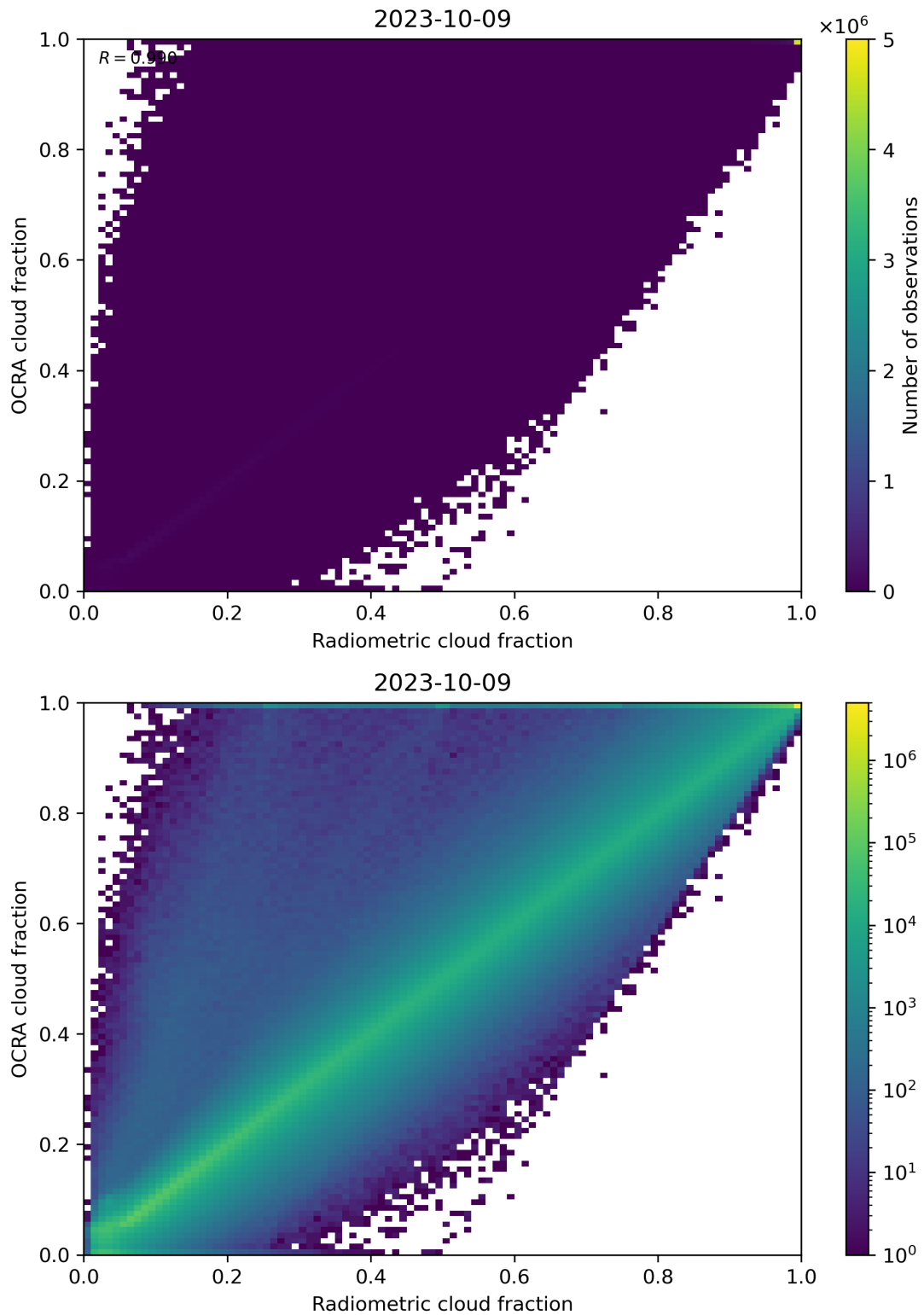
Figure 72: Scatter density plot of “Radiometric cloud fraction” against “OCRA cloud fraction” for 2023-10-08 to 2023-10-10.
