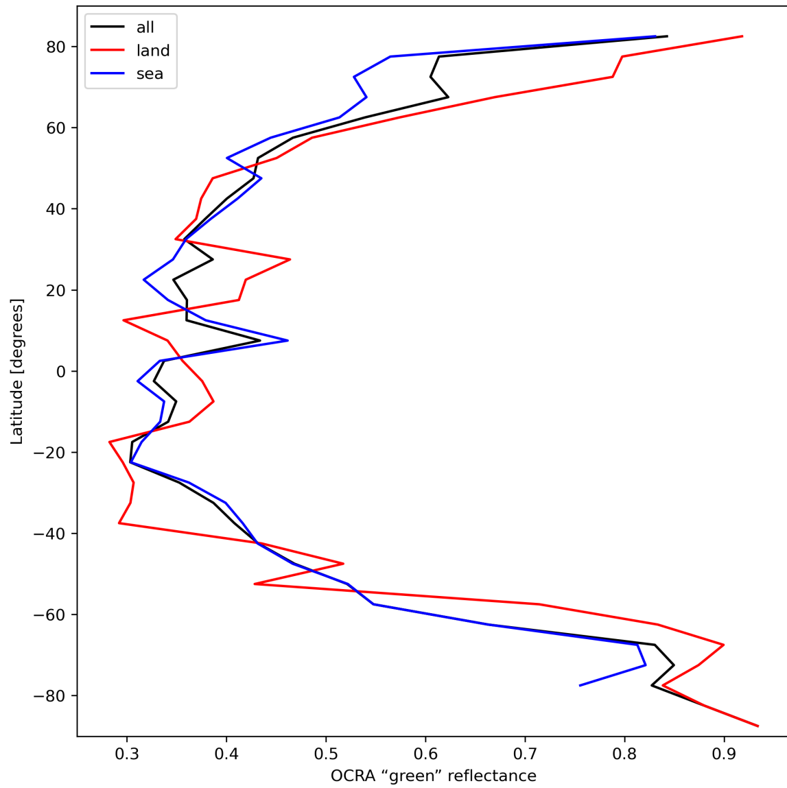
Figure 36: Zonal average of “OCRA “green” reflectance” for 2023-10-08 to 2023-10-10.
