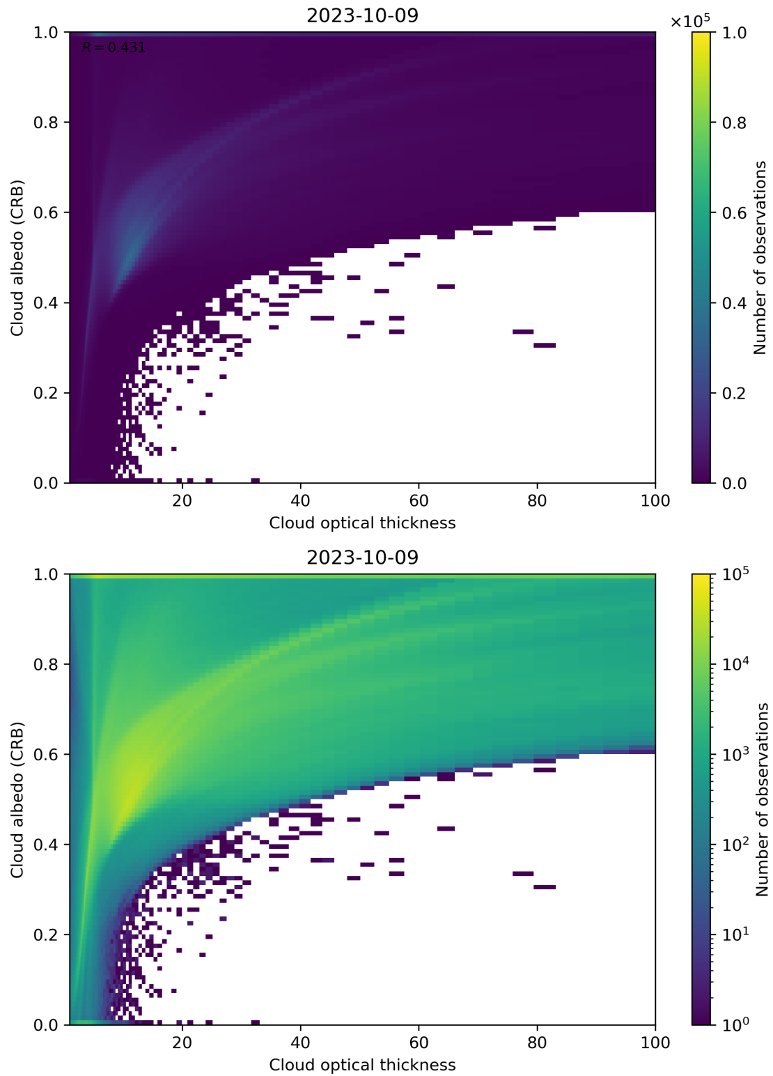
Figure 82: Scatter density plot of “Cloud optical thickness” against “Cloud albedo (CRB)” for 2023-10-08 to 2023-10-10.
