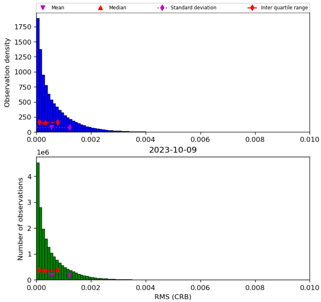
Figure 48: Histogram of “RMS (CRB)” for 2023-10-08 to 2023-10-10
