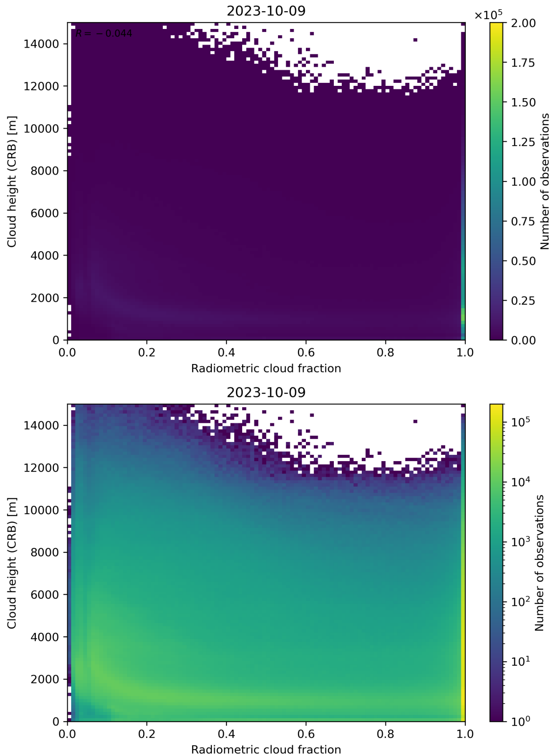
Figure 74: Scatter density plot of “Radiometric cloud fraction” against “Cloud height (CRB)” for 2023-10-08 to 2023-10-10.
