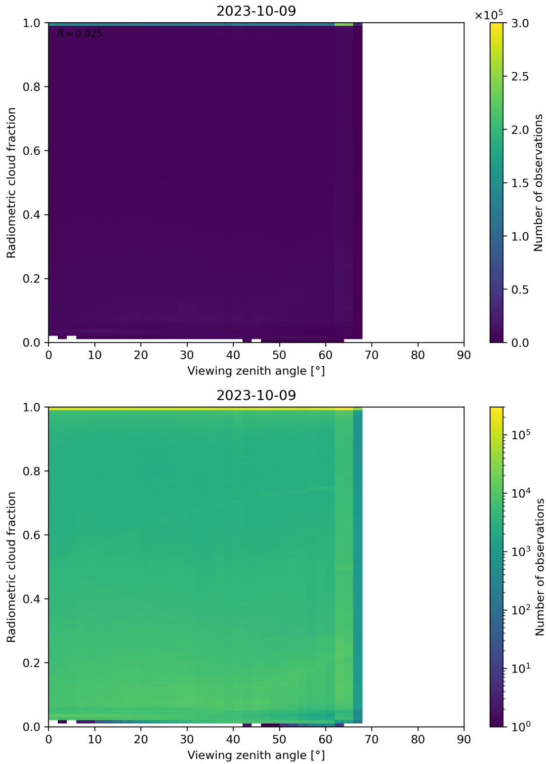
Figure 107: Scatter density plot of “Viewing zenith angle” against “Radiometric cloud fraction” for 2023-10-08 to 2023-10-10.
