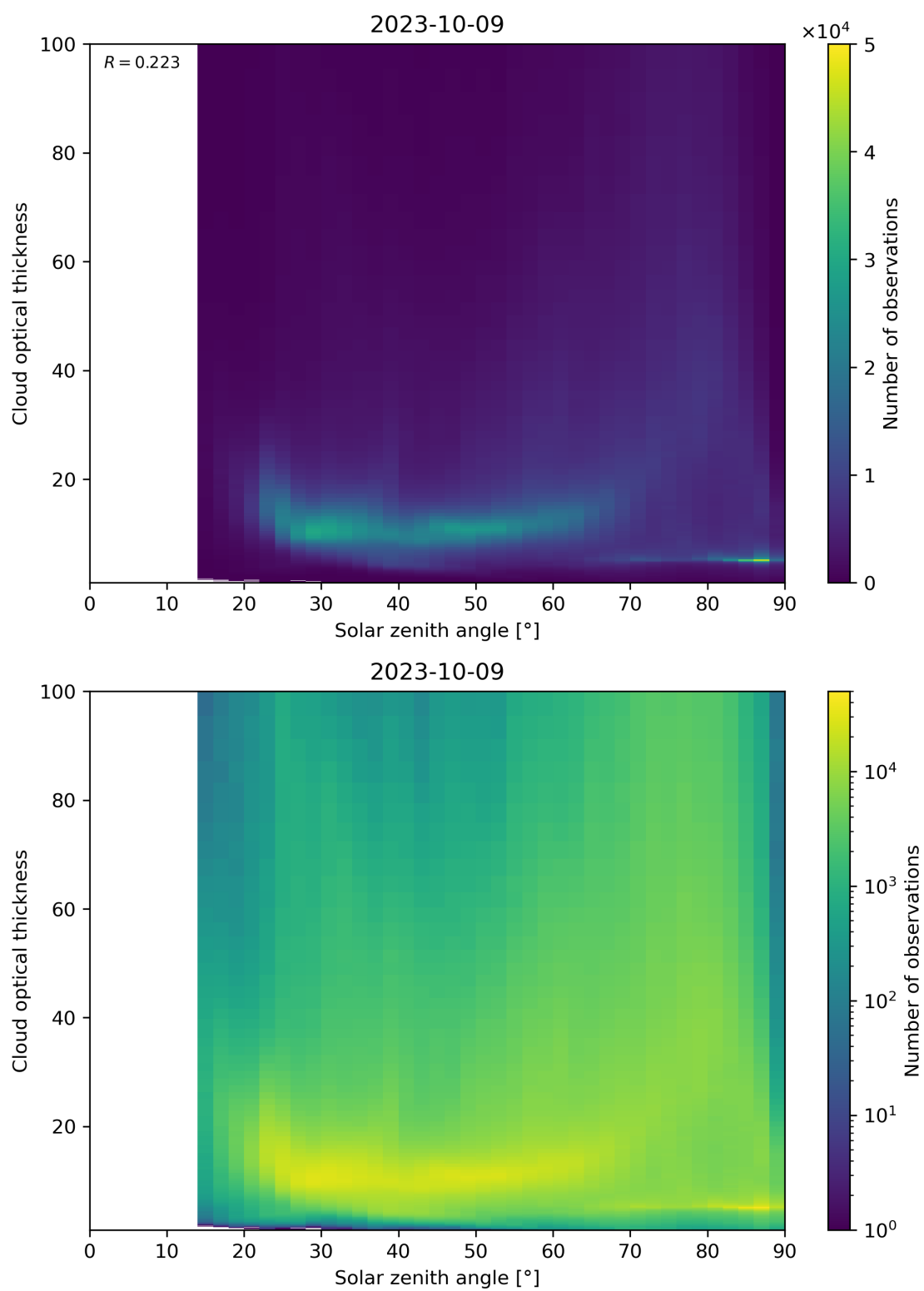
Figure 103: Scatter density plot of “Solar zenith angle” against “Cloud optical thickness” for 2023-10-08 to 2023-10-10.
