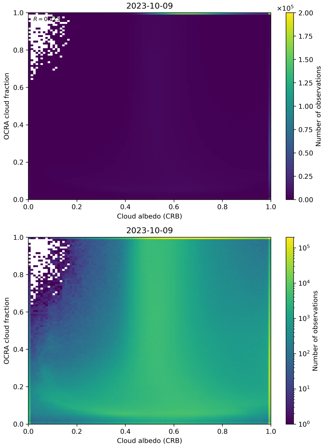
Figure 70: Scatter density plot of “Cloud albedo (CRB)” against “OCRA cloud fraction” for 2023-10-08 to 2023-10-10.
