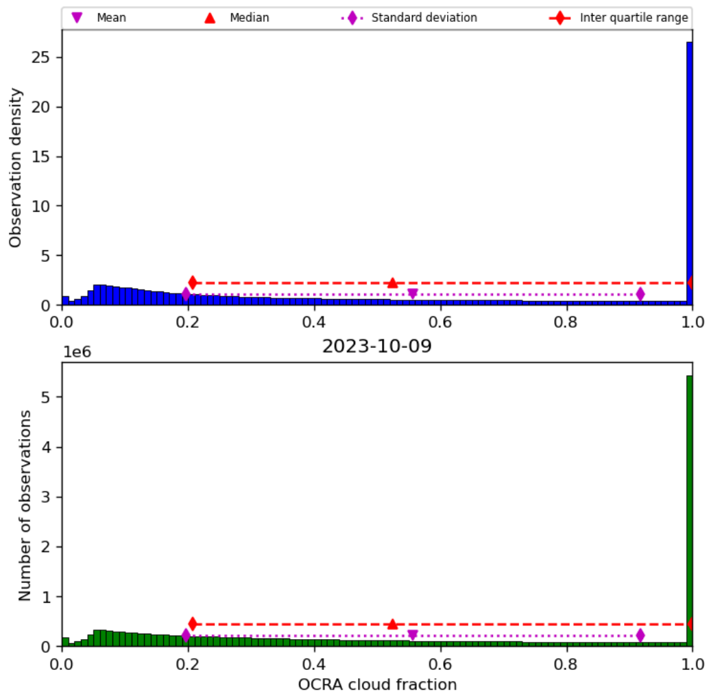
Figure 50: Histogram of “OCRA cloud fraction” for 2023-10-08 to 2023-10-10
