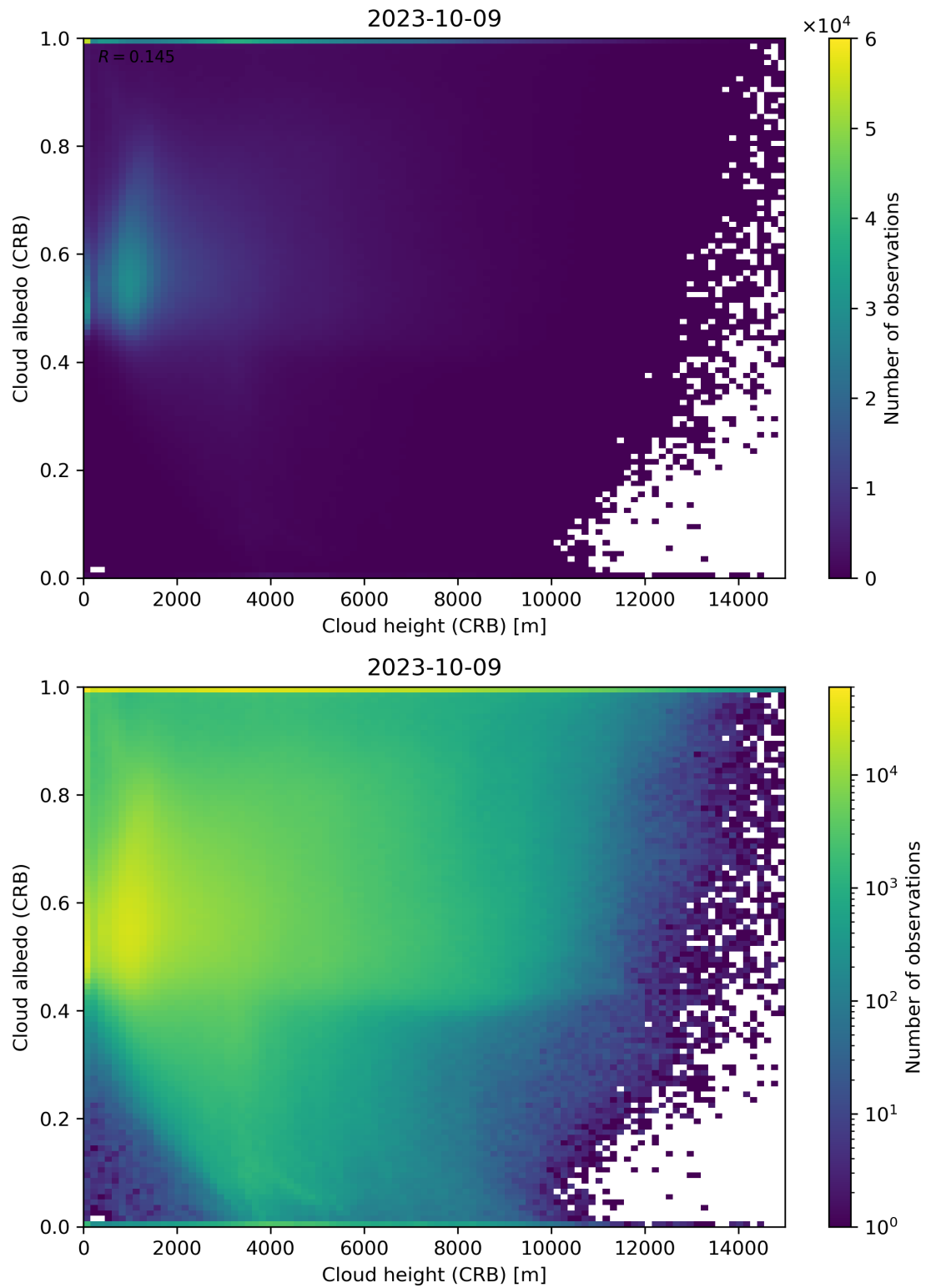
Figure 80: Scatter density plot of “Cloud height (CRB)” against “Cloud albedo (CRB)” for 2023-10-08 to 2023-10-10.
