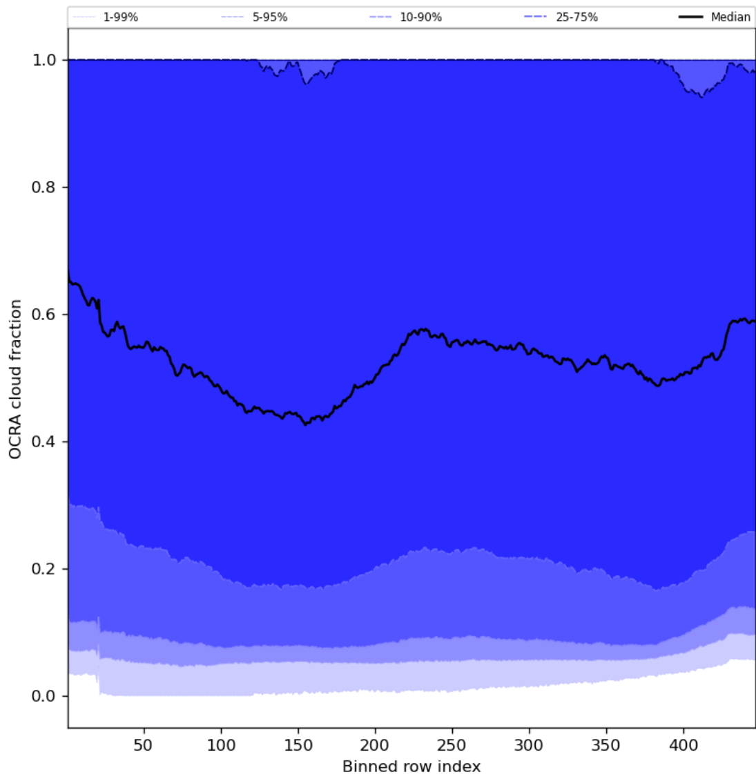
Figure 66: Along track statistics of “OCRA cloud fraction” for 2023-10-08 to 2023-10-10
