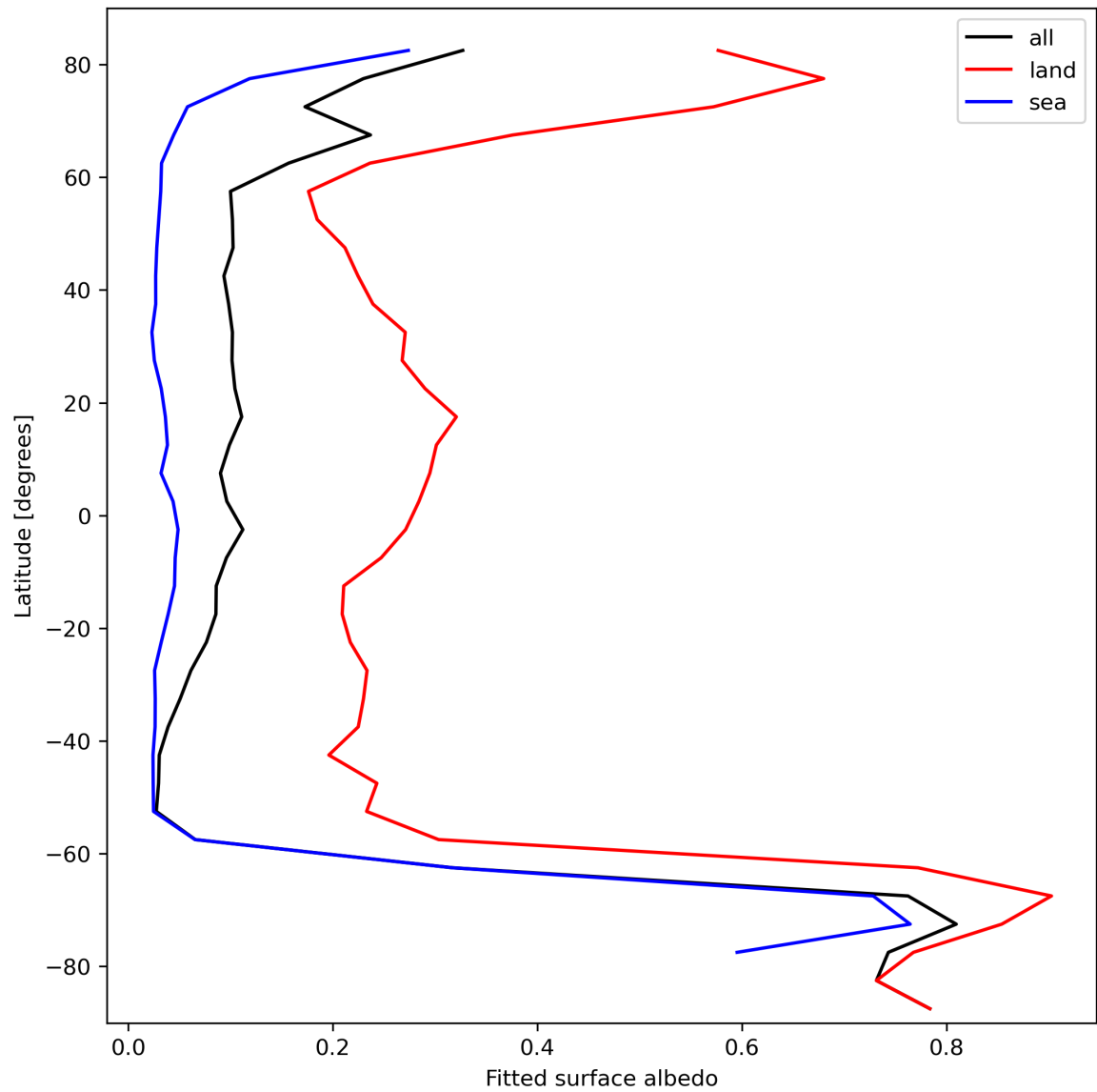
Figure 29: Zonal average of “Fitted surface albedo” for 2023-10-08 to 2023-10-10.
