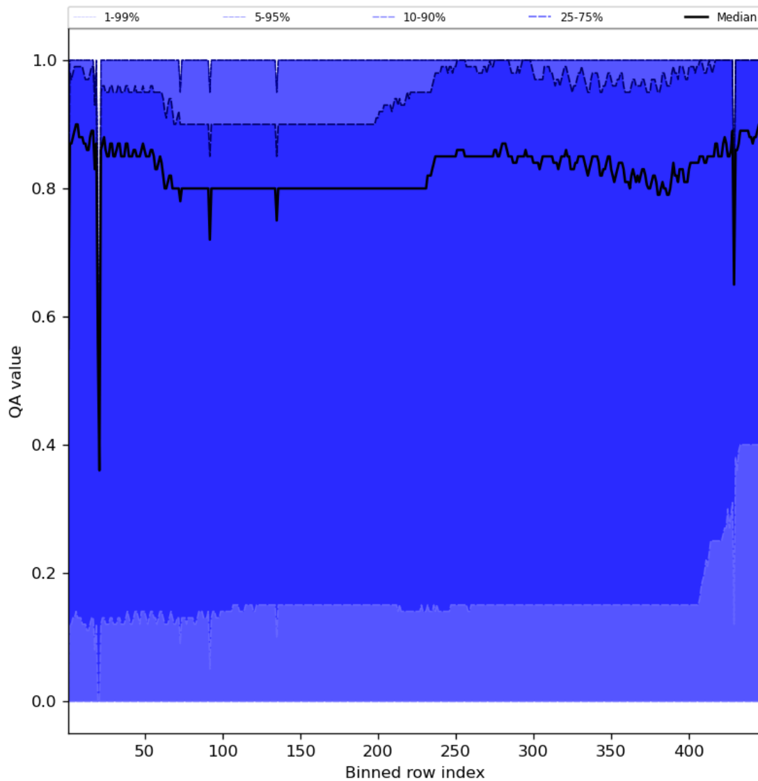
Figure 54: Along track statistics of “QA value” for 2023-10-08 to 2023-10-10
