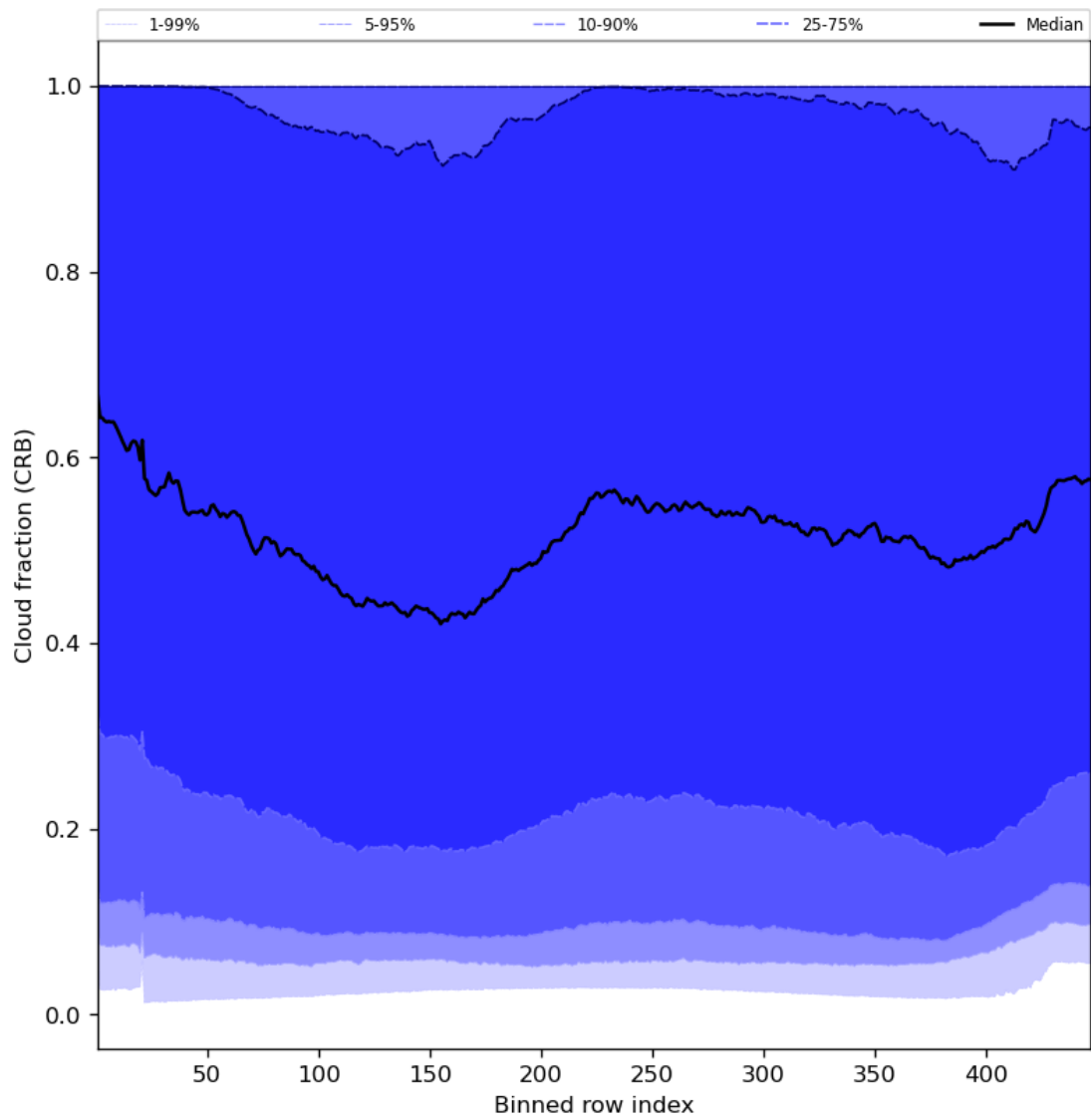
Figure 58: Along track statistics of “Cloud fraction (CRB)” for 2023-10-08 to 2023-10-10
