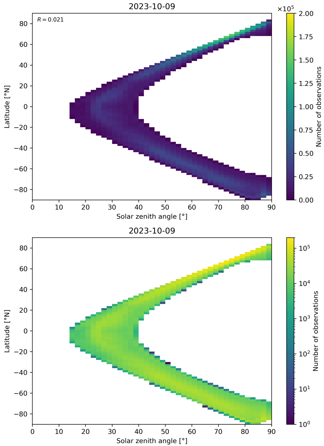
Figure 105: Scatter density plot of “Solar zenith angle” against “Latitude” for 2023-10-08 to 2023-10-10.
