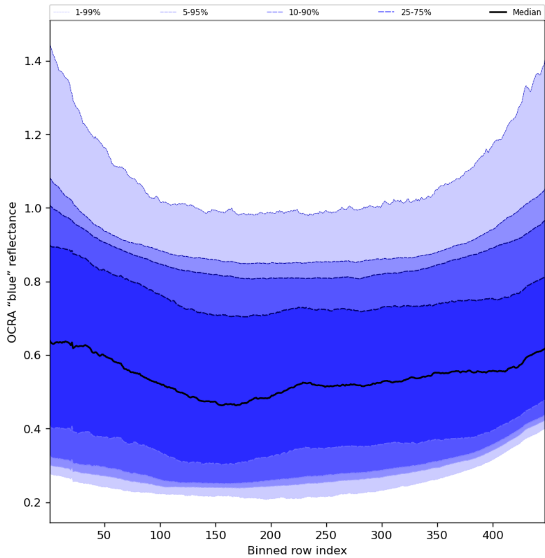
Figure 67: Along track statistics of “OCRA “blue” reflectance” for 2023-10-08 to 2023-10-10
