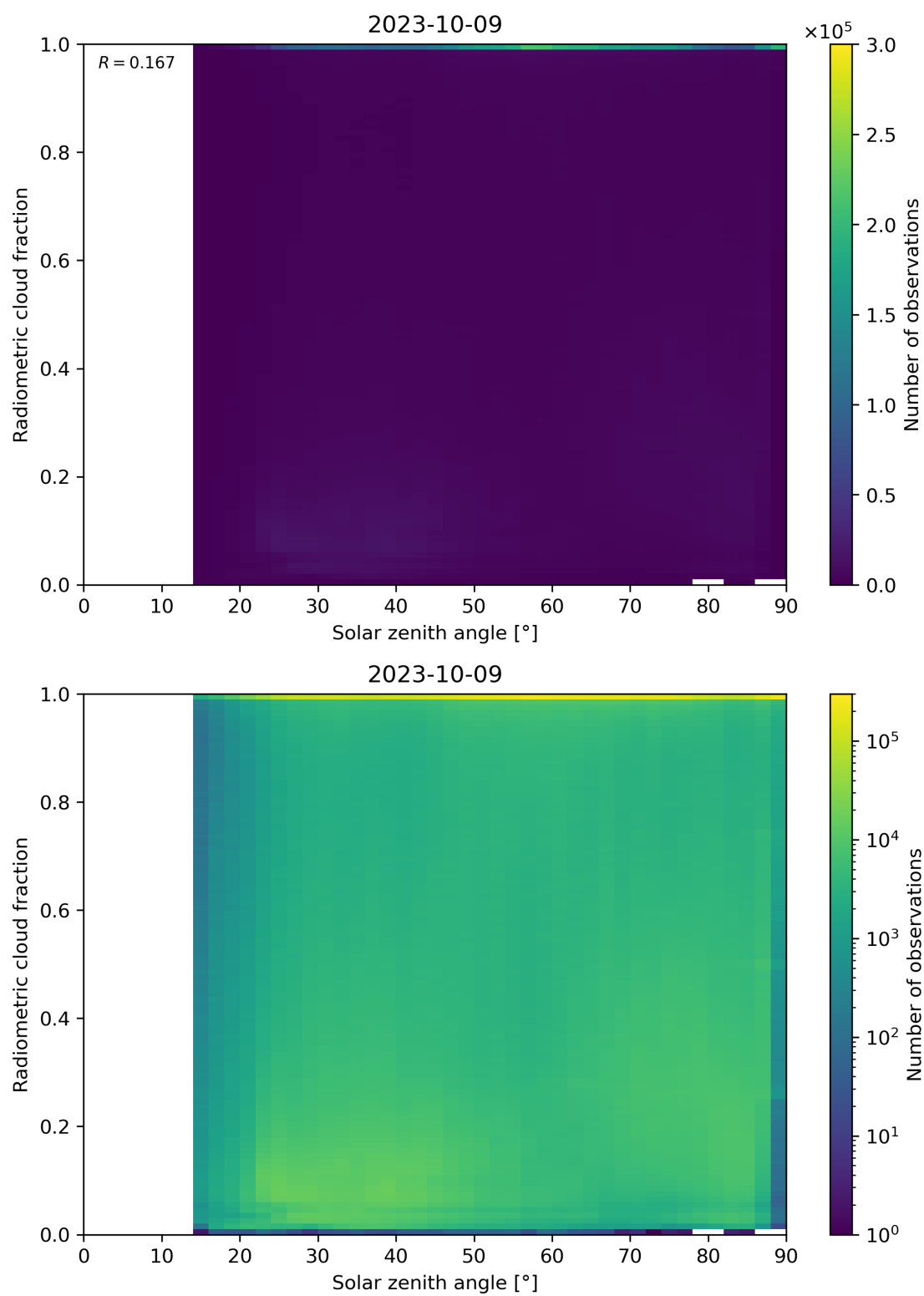
Figure 99: Scatter density plot of “Solar zenith angle” against “Radiometric cloud fraction” for 2023-10-08 to 2023-10-10.
