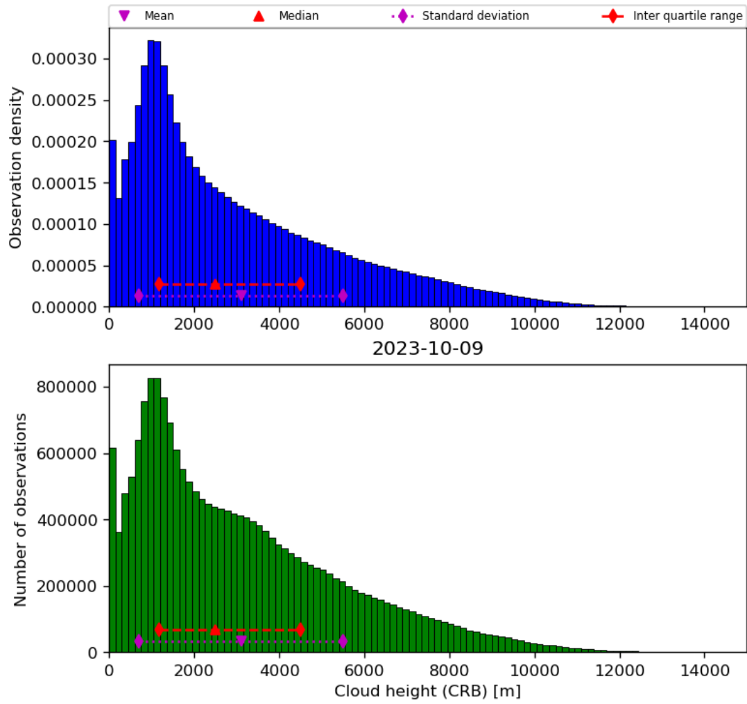
Figure 43: Histogram of “Cloud height (CRB)” for 2023-10-08 to 2023-10-10
