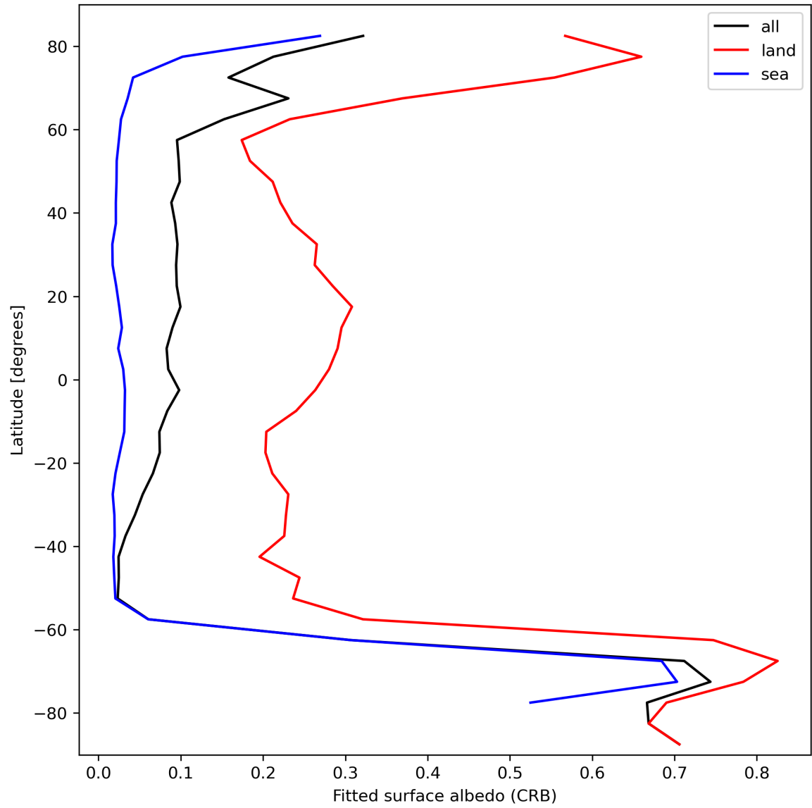
Figure 30: Zonal average of “Fitted surface albedo (CRB)” for 2023-10-08 to 2023-10-10.
