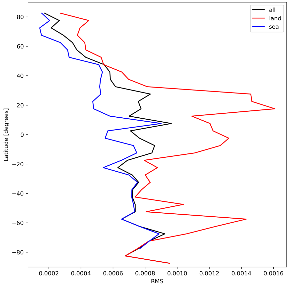
Figure 31: Zonal average of “RMS” for 2023-10-08 to 2023-10-10.
