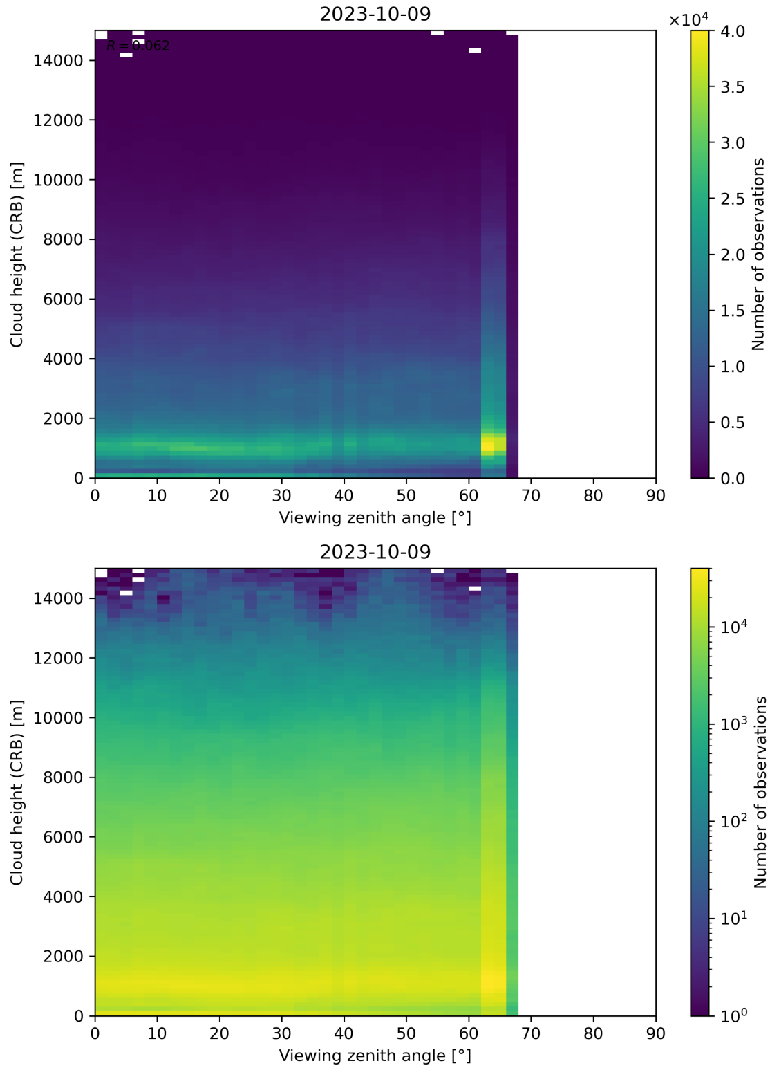
Figure 110: Scatter density plot of “Viewing zenith angle” against “Cloud height (CRB)” for 2023-10-08 to 2023-10-10.
