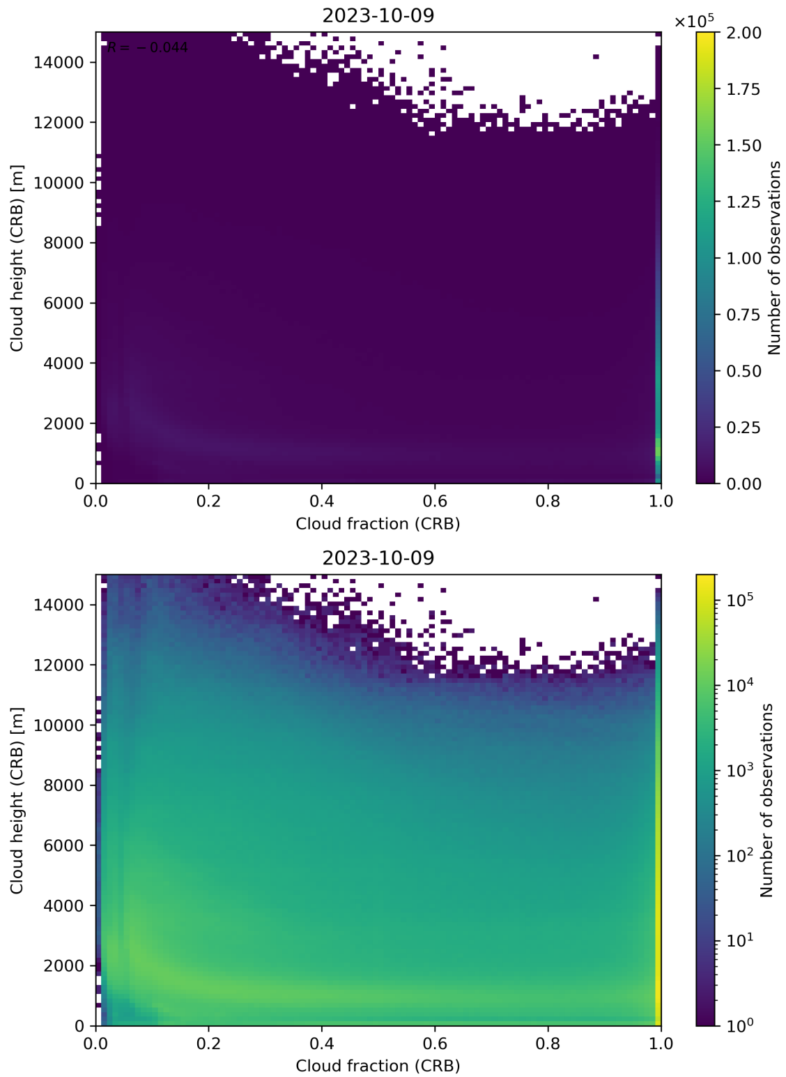
Figure 79: Scatter density plot of “Cloud fraction (CRB)” against “Cloud height (CRB)” for 2023-10-08 to 2023-10-10.
