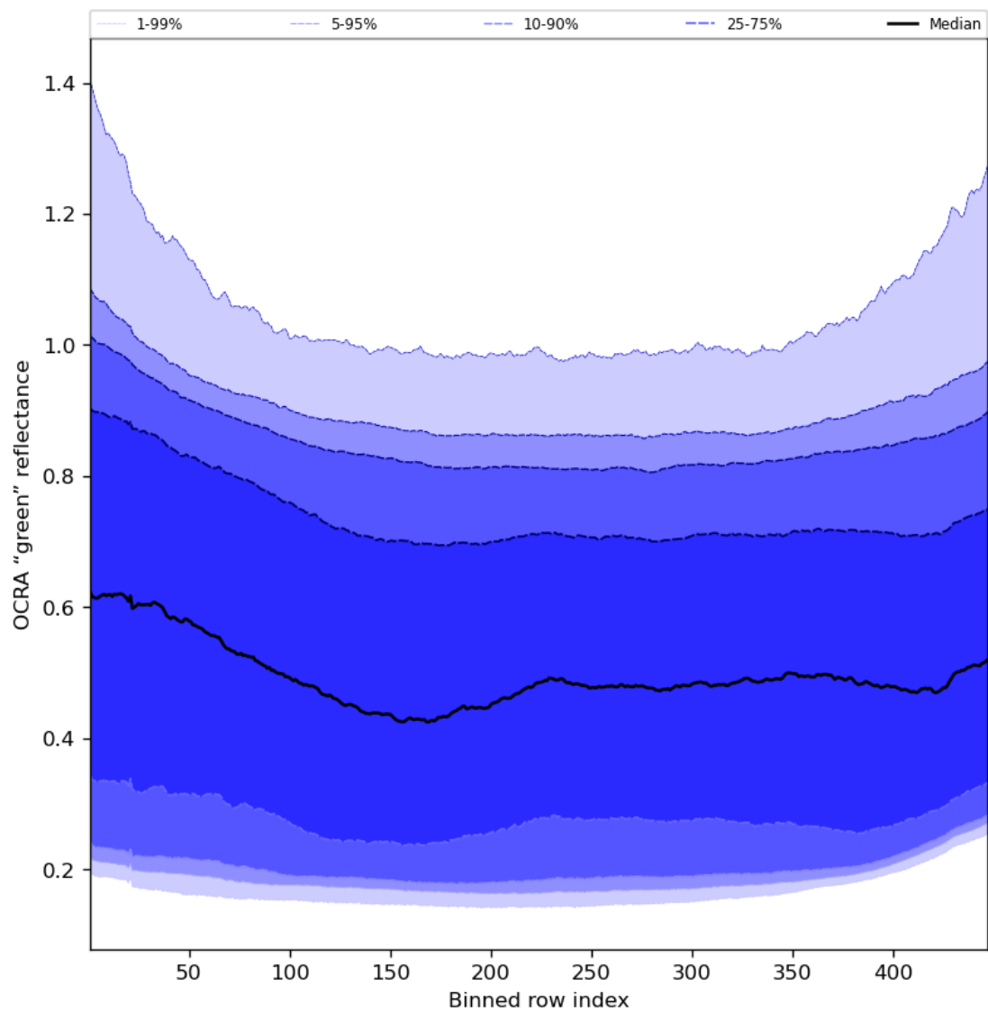
Figure 68: Along track statistics of “OCRA “green” reflectance” for 2023-10-08 to 2023-10-10
