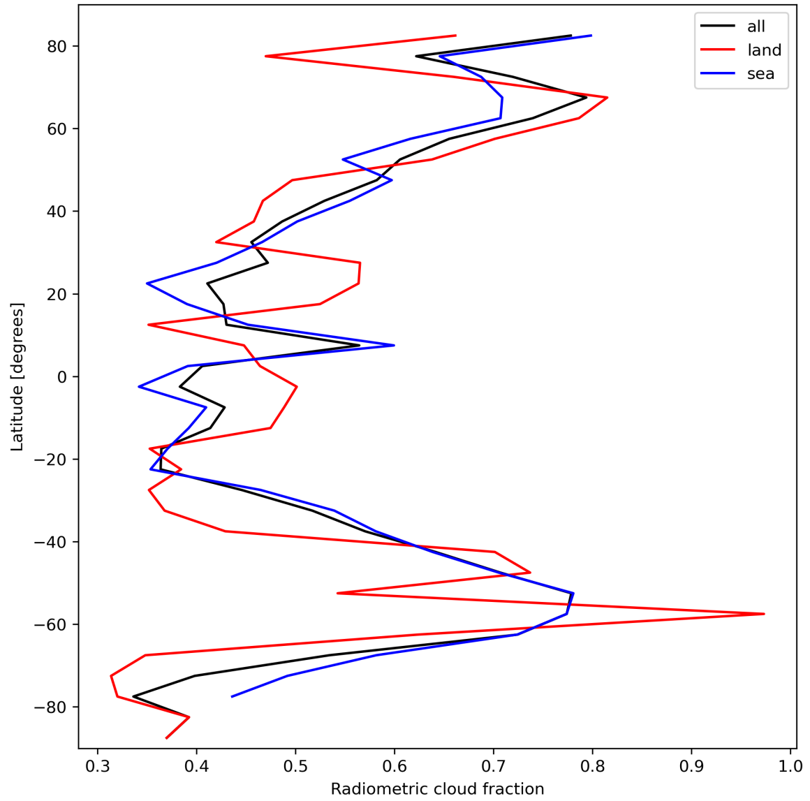
Figure 23: Zonal average of “Radiometric cloud fraction” for 2023-10-08 to 2023-10-10.
