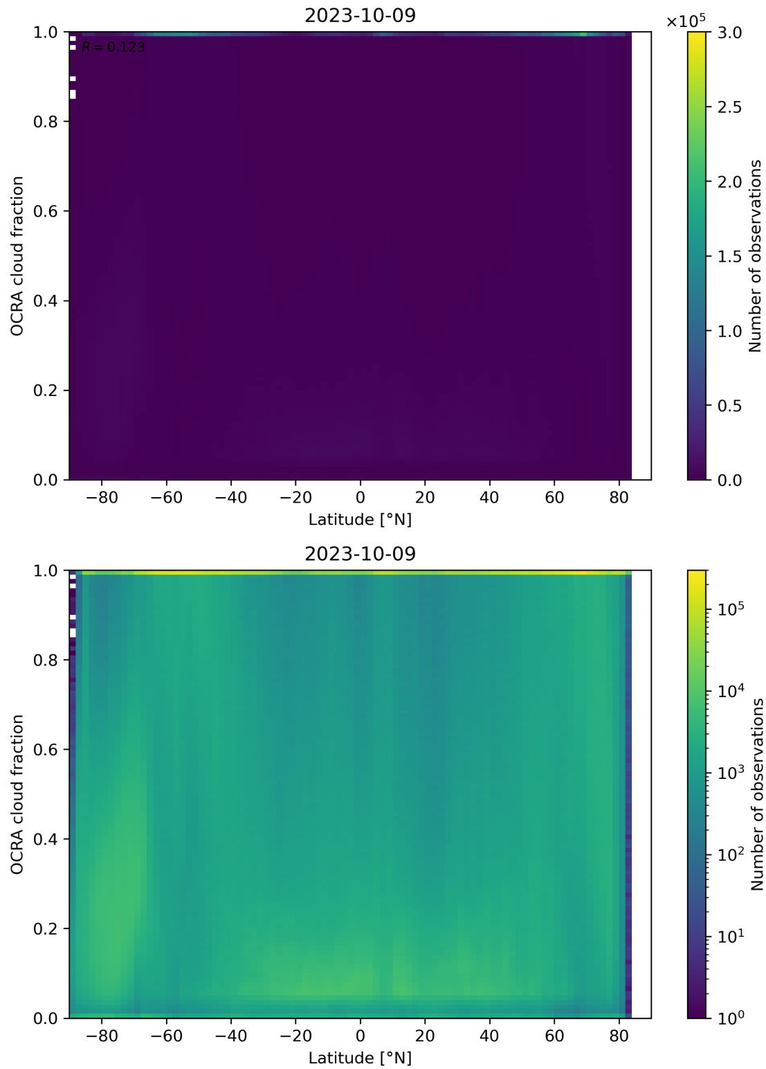
Figure 93: Scatter density plot of “Latitude” against “OCRA cloud fraction” for 2023-10-08 to 2023-10-10.
