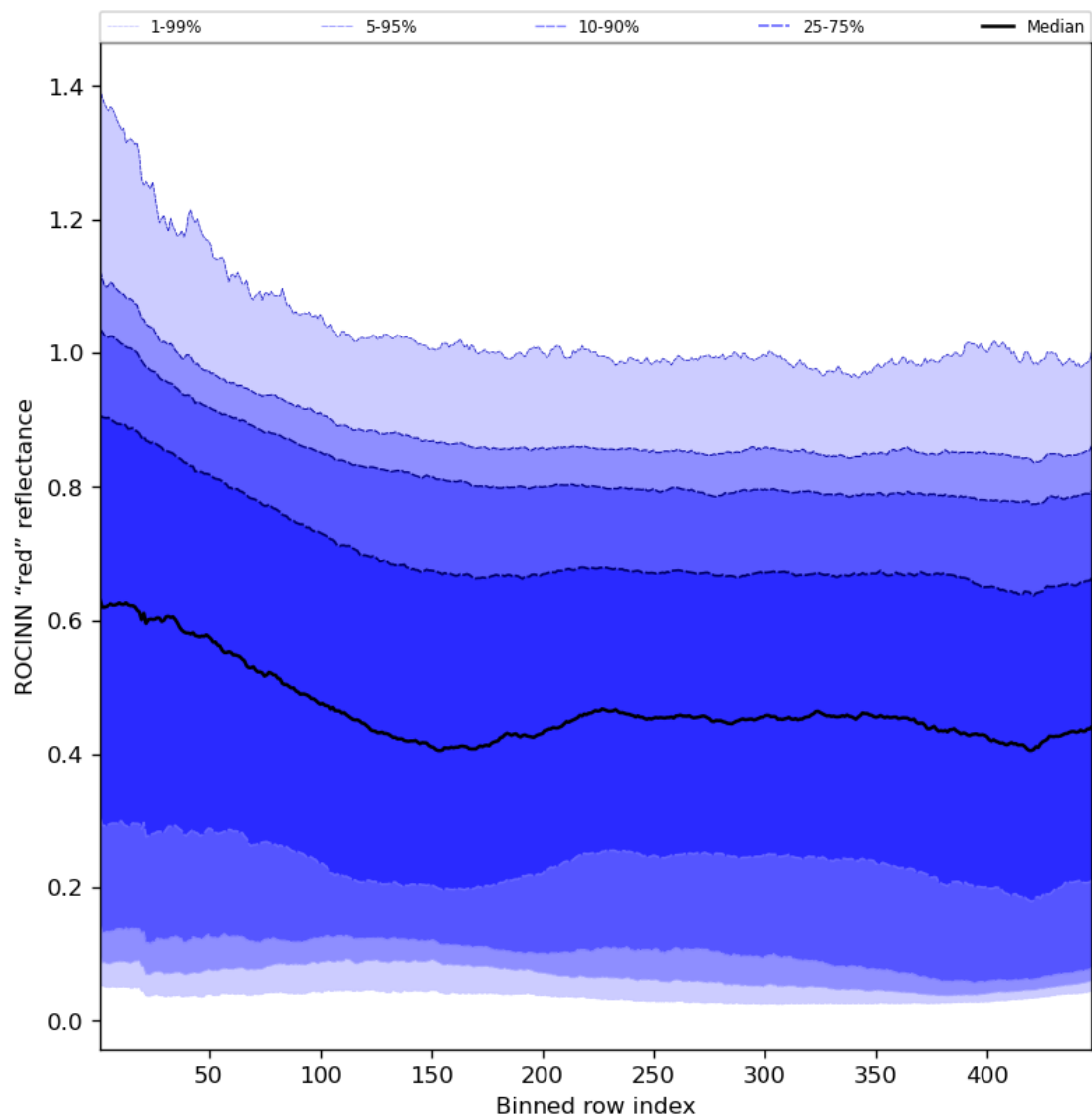
Figure 69: Along track statistics of “ROCINN “red” reflectance” for 2023-10-08 to 2023-10-10
