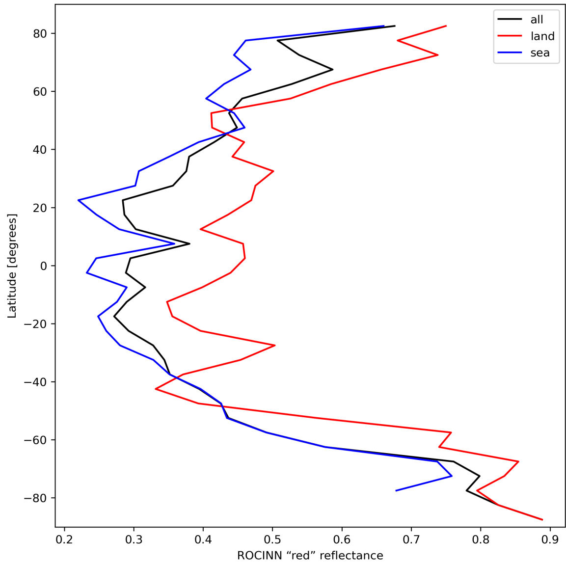
Figure 37: Zonal average of "ROCINN "red" reflectance" for 2023-10-10 to 2023-10-12.
