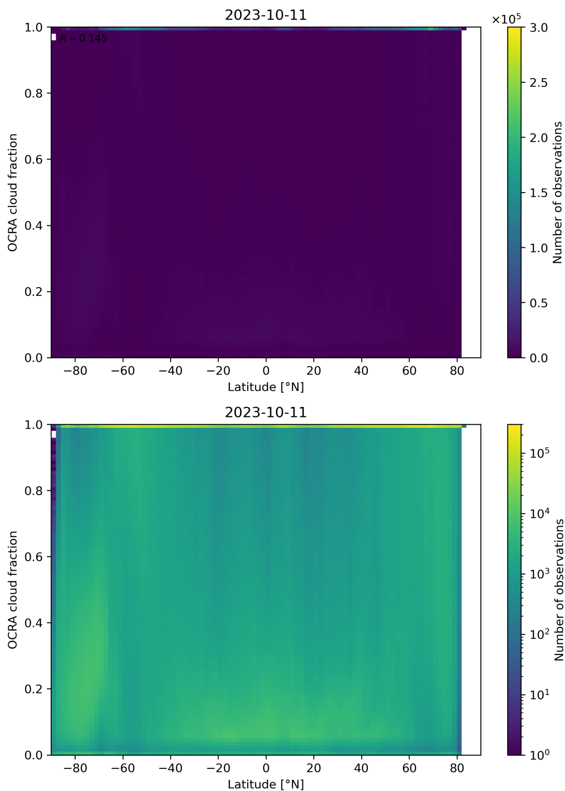
Figure 93: Scatter density plot of “Latitude” against “OCRA cloud fraction” for 2023-10-10 to 2023-10-12.
