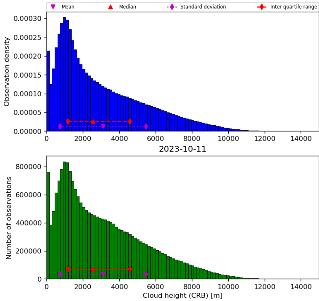
Figure 43: Histogram of “Cloud height (CRB)” for 2023-10-10 to 2023-10-12
