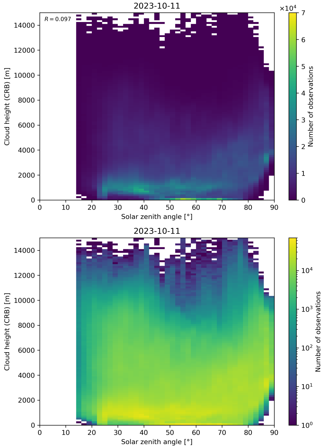
Figure 102: Scatter density plot of “Solar zenith angle” against “Cloud height (CRB)” for 2023-10-10 to 2023-10-12.
