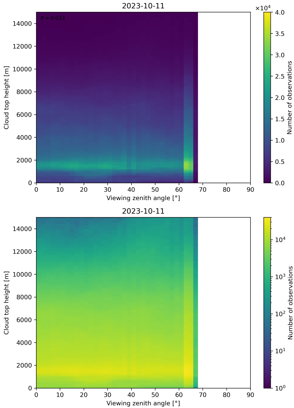
Figure 112: Scatter density plot of “Viewing zenith angle” against “Cloud top height” for 2023-10-10 to 2023-10-12.
