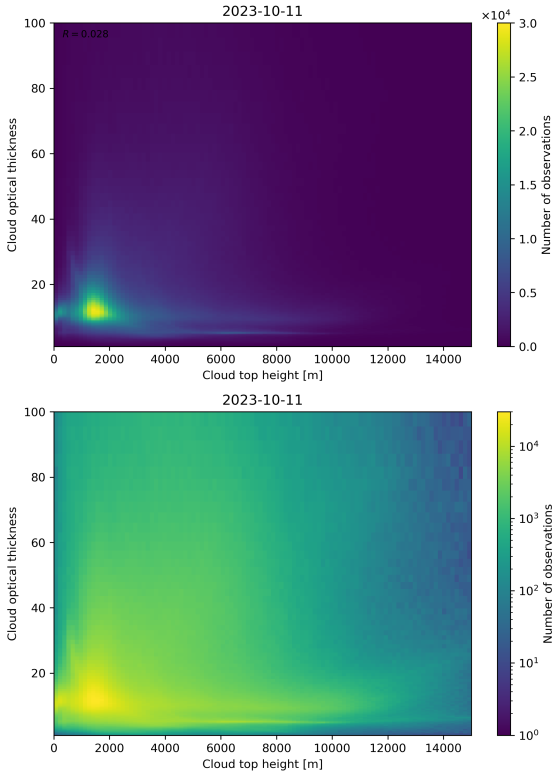
Figure 90: Scatter density plot of “Cloud top height” against “Cloud optical thickness” for 2023-10-10 to 2023-10-12.
