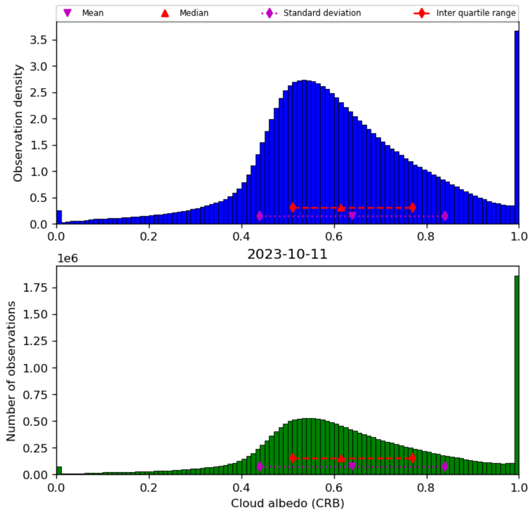
Figure 44: Histogram of “Cloud albedo (CRB)” for 2023-10-10 to 2023-10-12
