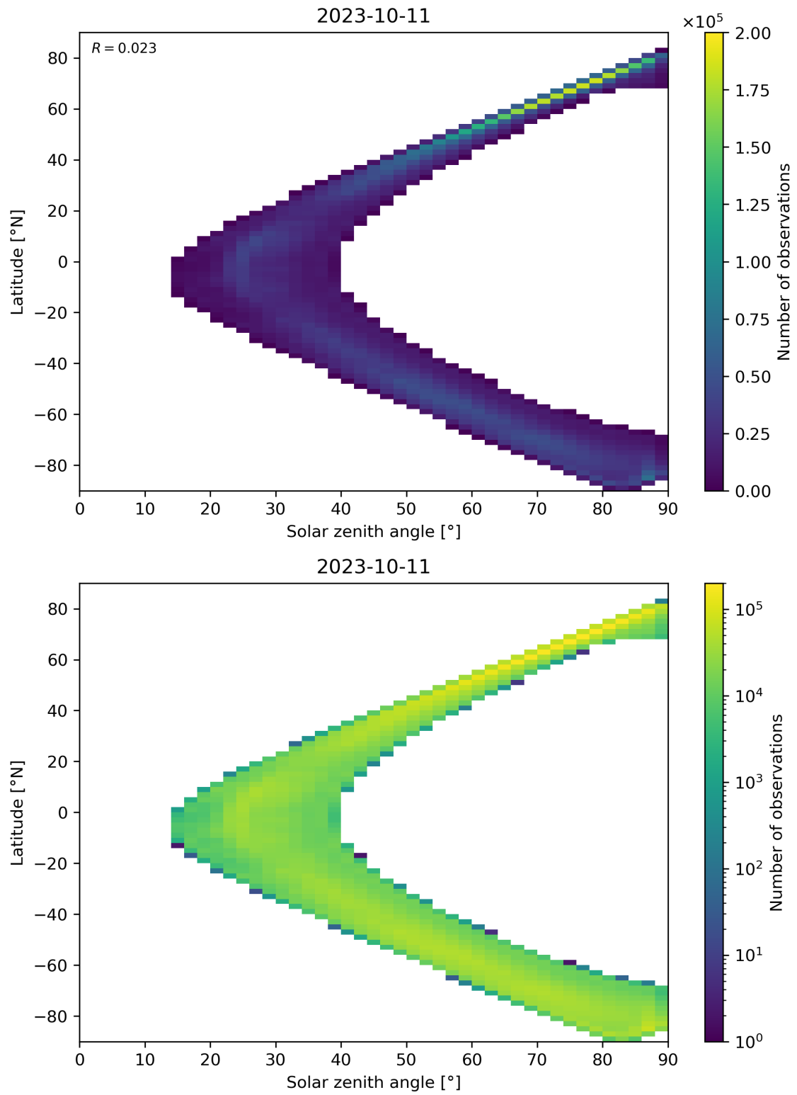
Figure 105: Scatter density plot of “Solar zenith angle” against “Latitude” for 2023-10-10 to 2023-10-12.
