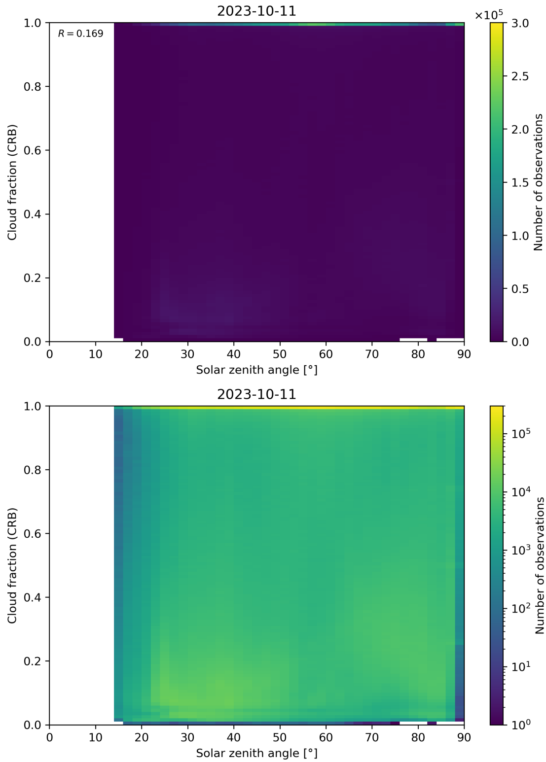
Figure 101: Scatter density plot of “Solar zenith angle” against “Cloud fraction (CRB)” for 2023-10-10 to 2023-10-12.
