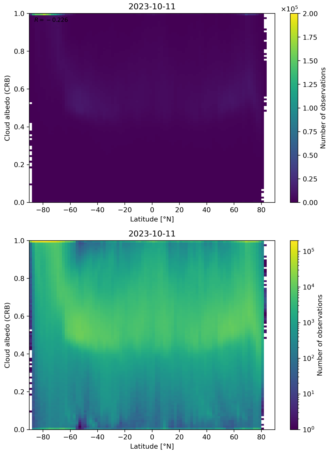
Figure 91: Scatter density plot of “Latitude” against “Cloud albedo (CRB)” for 2023-10-10 to 2023-10-12.
