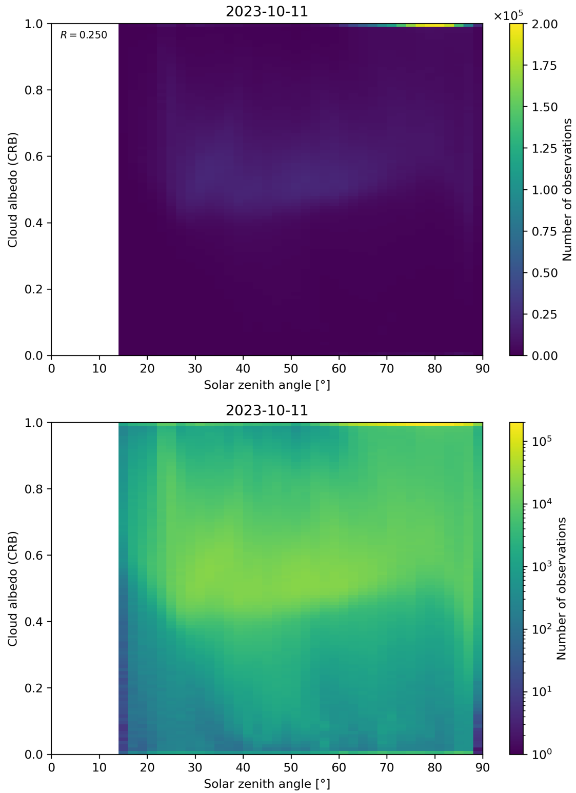
Figure 98: Scatter density plot of “Solar zenith angle” against “Cloud albedo (CRB)” for 2023-10-10 to 2023-10-12.
