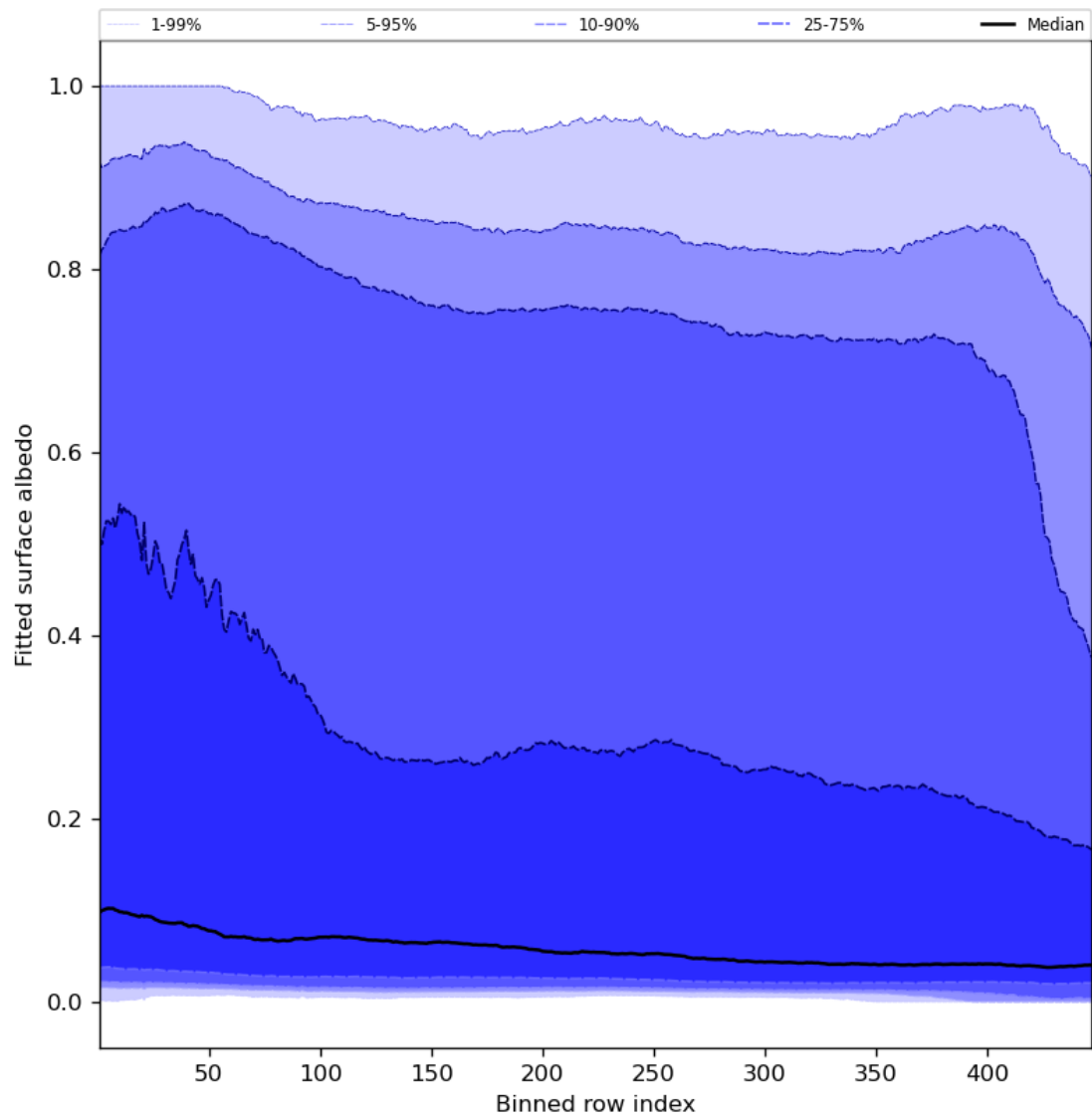
Figure 61: Along track statistics of “Fitted surface albedo” for 2023-10-10 to 2023-10-12
