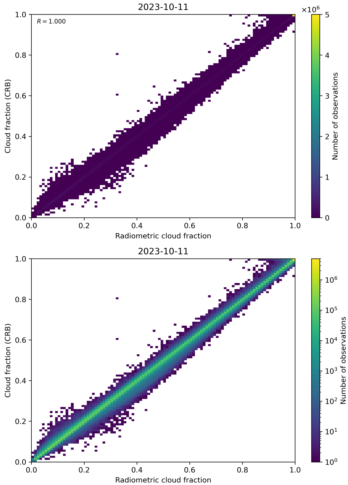
Figure 73: Scatter density plot of “Radiometric cloud fraction” against “Cloud fraction (CRB)” for 2023-10-10 to 2023-10-12.
