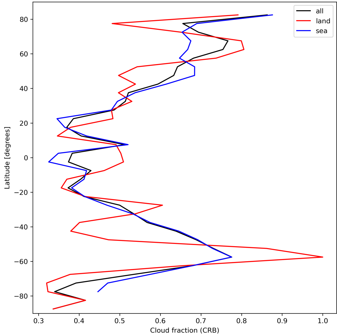
Figure 26: Zonal average of “Cloud fraction (CRB)” for 2023-10-10 to 2023-10-12.
