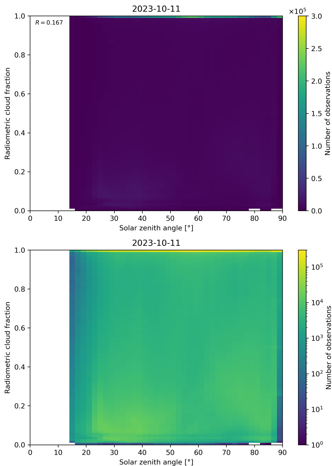
Figure 99: Scatter density plot of “Solar zenith angle” against “Radiometric cloud fraction” for 2023-10-10 to 2023-10-12.
