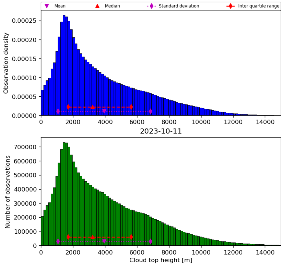
Figure 40: Histogram of “Cloud top height” for 2023-10-10 to 2023-10-12
