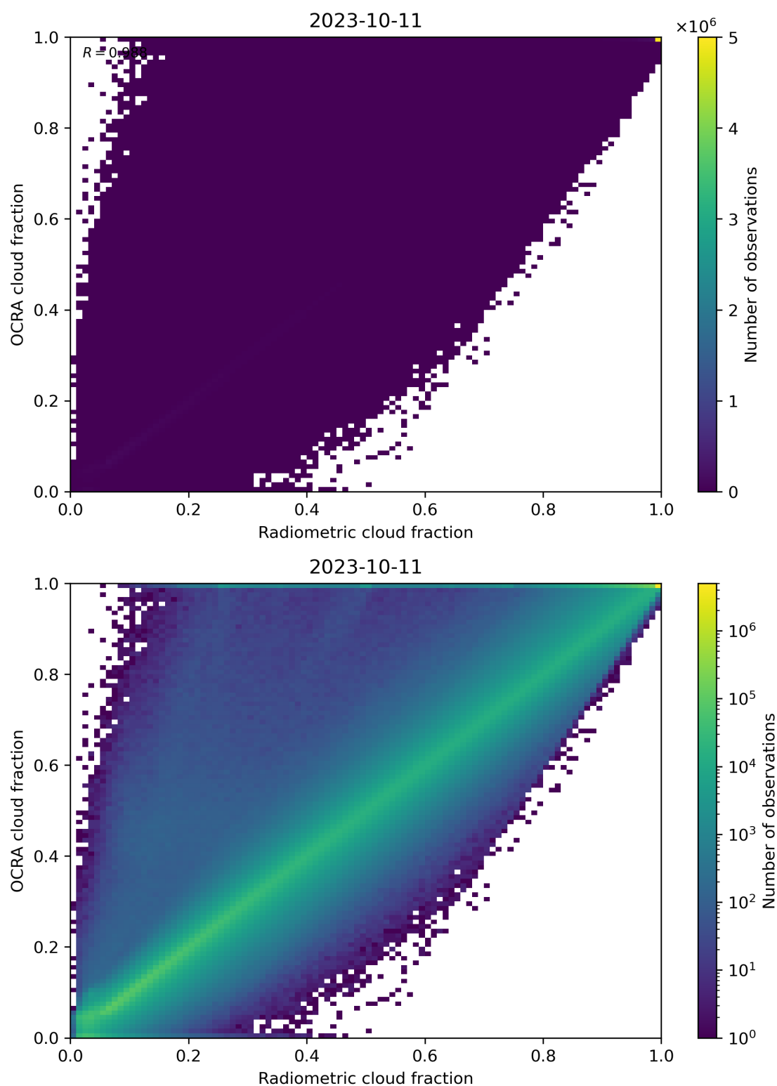
Figure 72: Scatter density plot of “Radiometric cloud fraction” against “OCRA cloud fraction” for 2023-10-10 to 2023-10-12.
