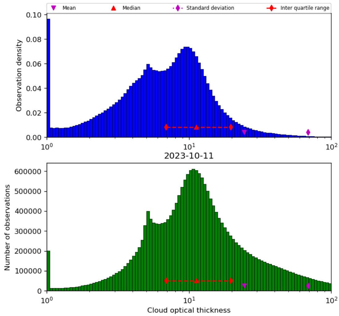
Figure 41: Histogram of “Cloud optical thickness” for 2023-10-10 to 2023-10-12
