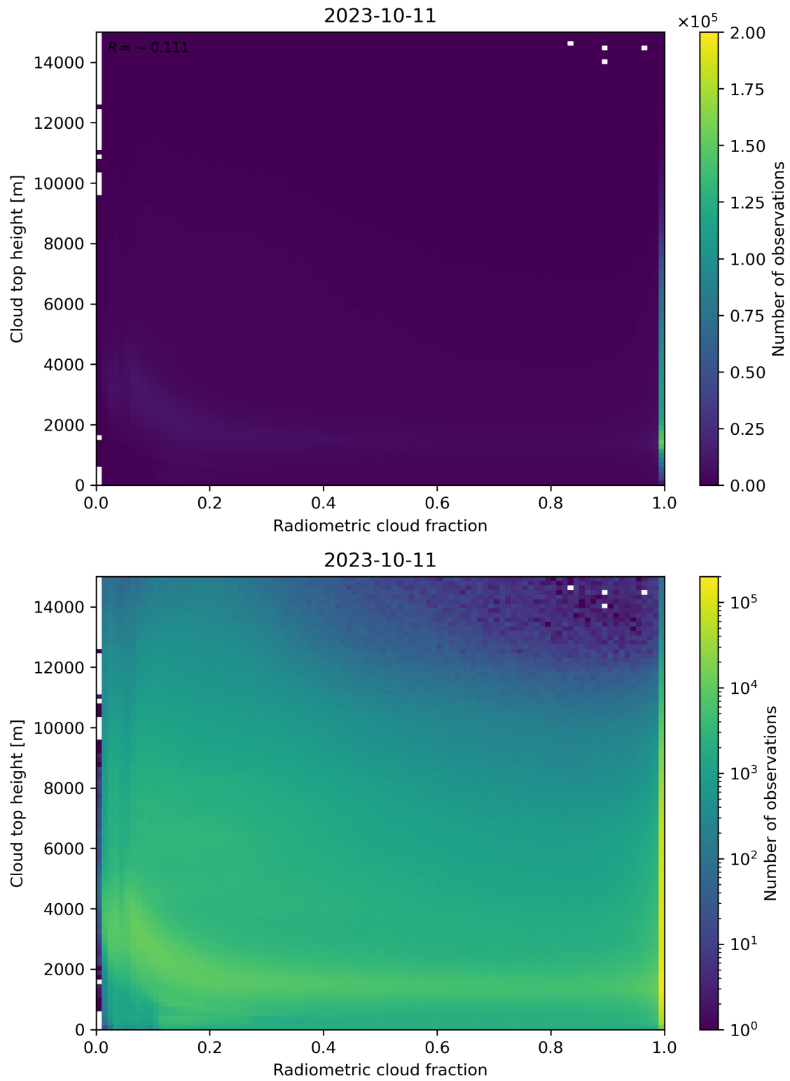
Figure 76: Scatter density plot of “Radiometric cloud fraction” against “Cloud top height” for 2023-10-10 to 2023-10-12.
