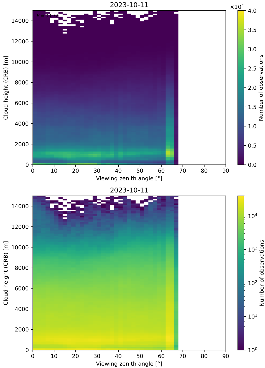
Figure 110: Scatter density plot of “Viewing zenith angle” against “Cloud height (CRB)” for 2023-10-10 to 2023-10-12.
