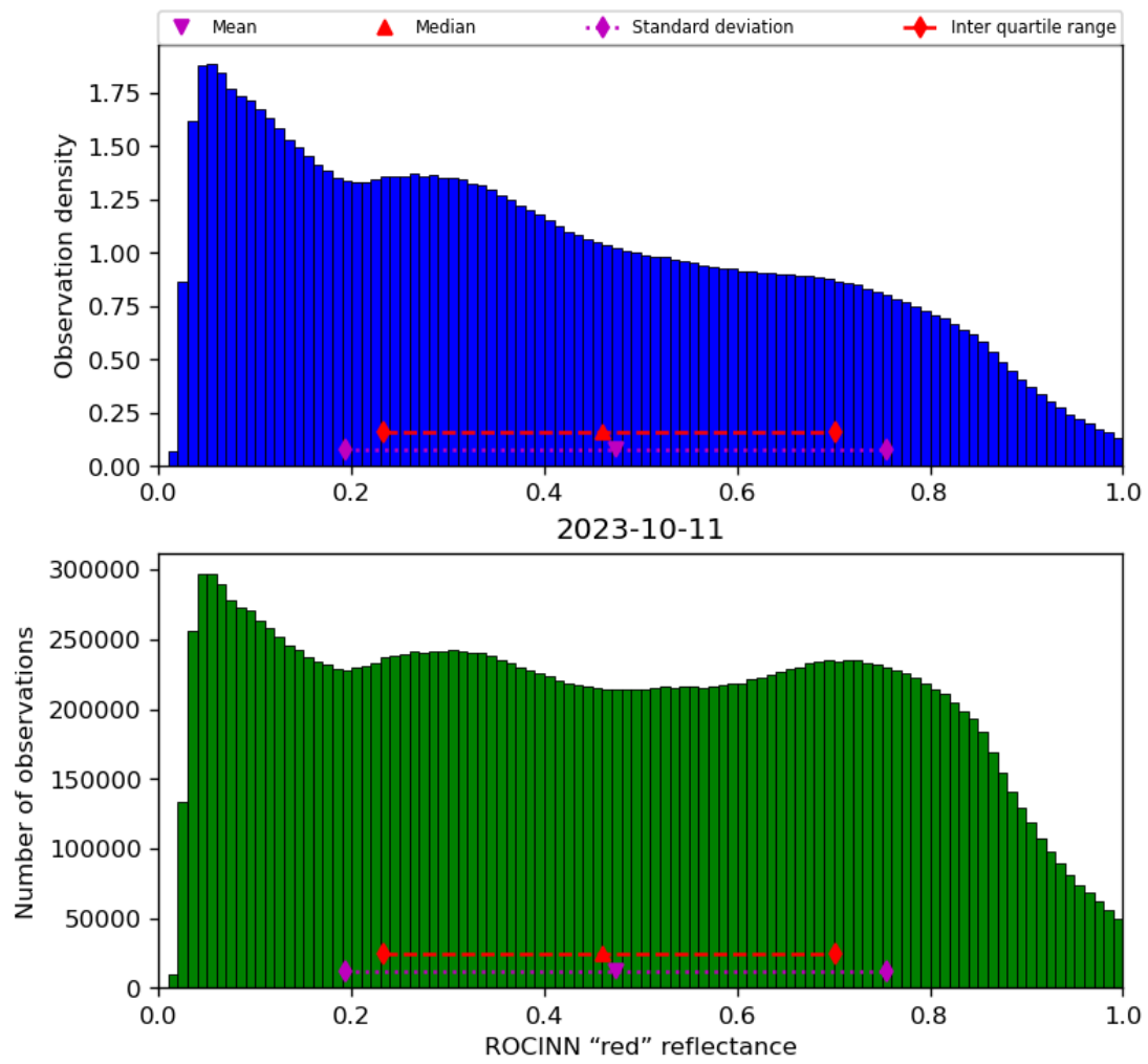
Figure 53: Histogram of “ROCINN “red” reflectance” for 2023-10-10 to 2023-10-12
