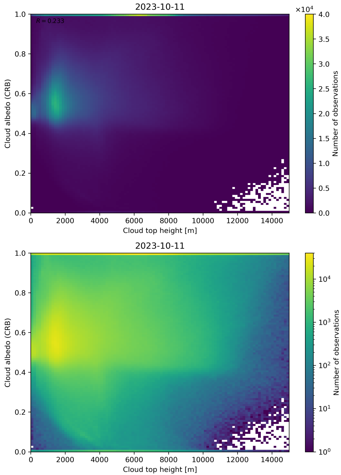
Figure 86: Scatter density plot of “Cloud top height” against “Cloud albedo (CRB)” for 2023-10-10 to 2023-10-12.
