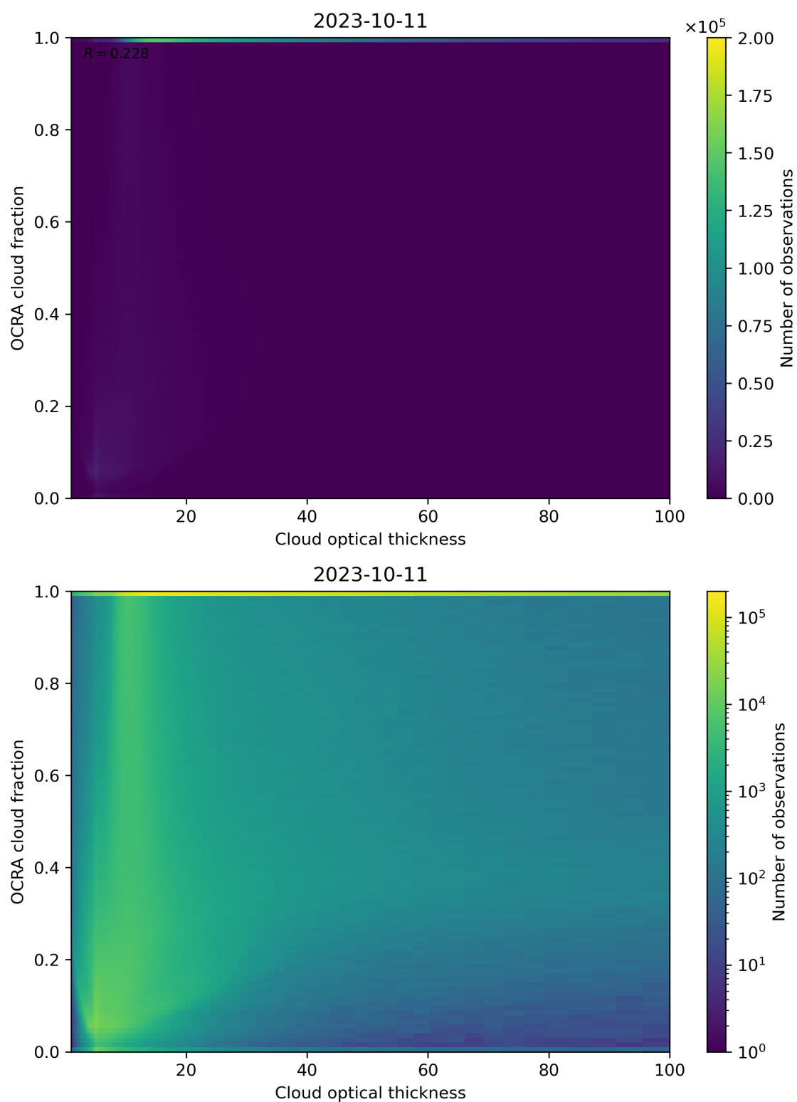
Figure 83: Scatter density plot of “Cloud optical thickness” against “OCRA cloud fraction” for 2023-10-10 to 2023-10-12.
