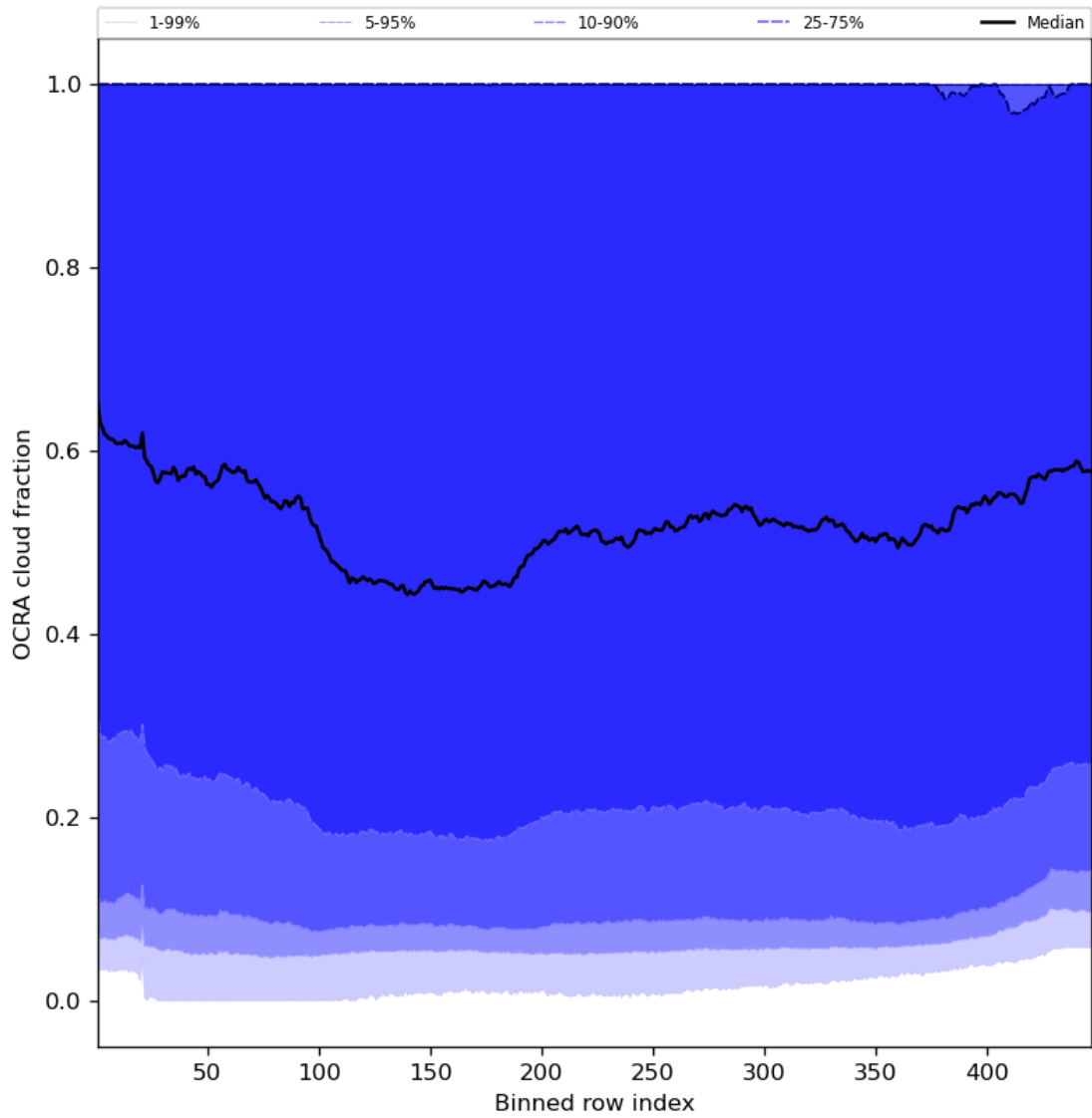
Figure 66: Along track statistics of “OCRA cloud fraction” for 2023-10-10 to 2023-10-12
