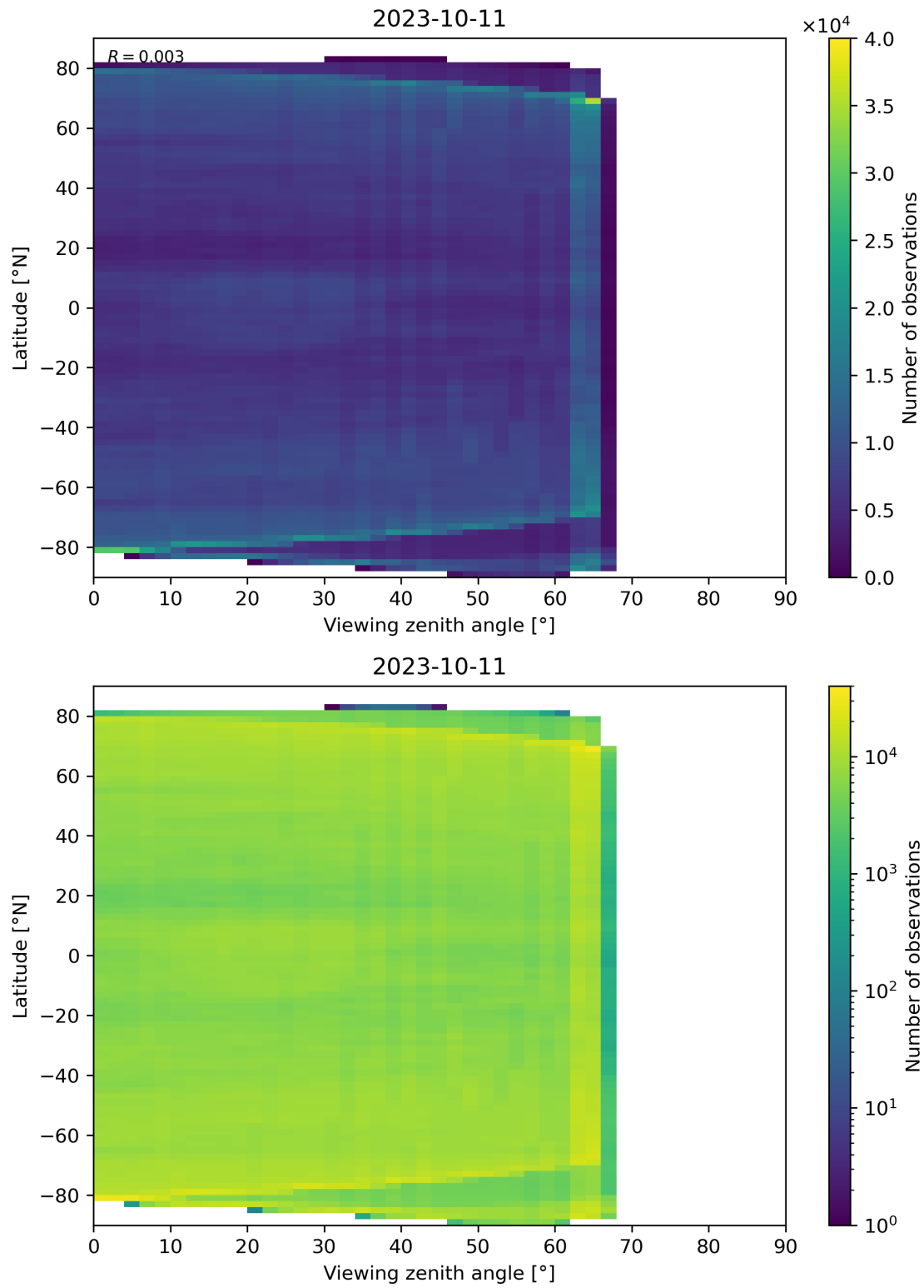
Figure 113: Scatter density plot of “Viewing zenith angle” against “Latitude” for 2023-10-10 to 2023-10-12.
