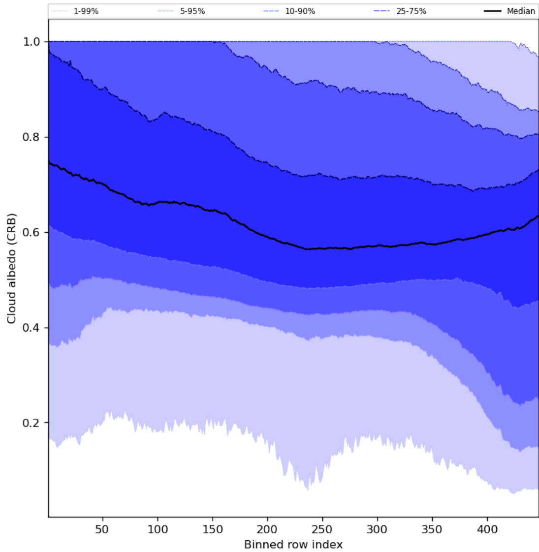
Figure 60: Along track statistics of “Cloud albedo (CRB)” for 2023-10-10 to 2023-10-12
