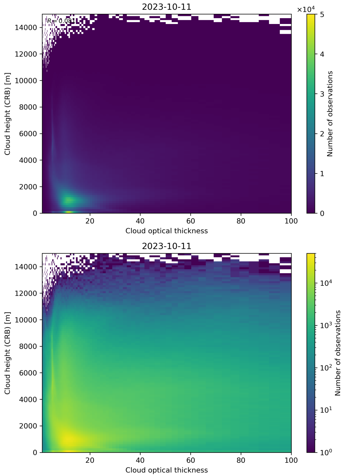
Figure 85: Scatter density plot of “Cloud optical thickness” against “Cloud height (CRB)” for 2023-10-10 to 2023-10-12.
