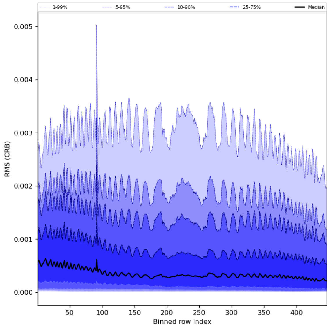
Figure 64: Along track statistics of “RMS (CRB)” for 2023-10-10 to 2023-10-12
