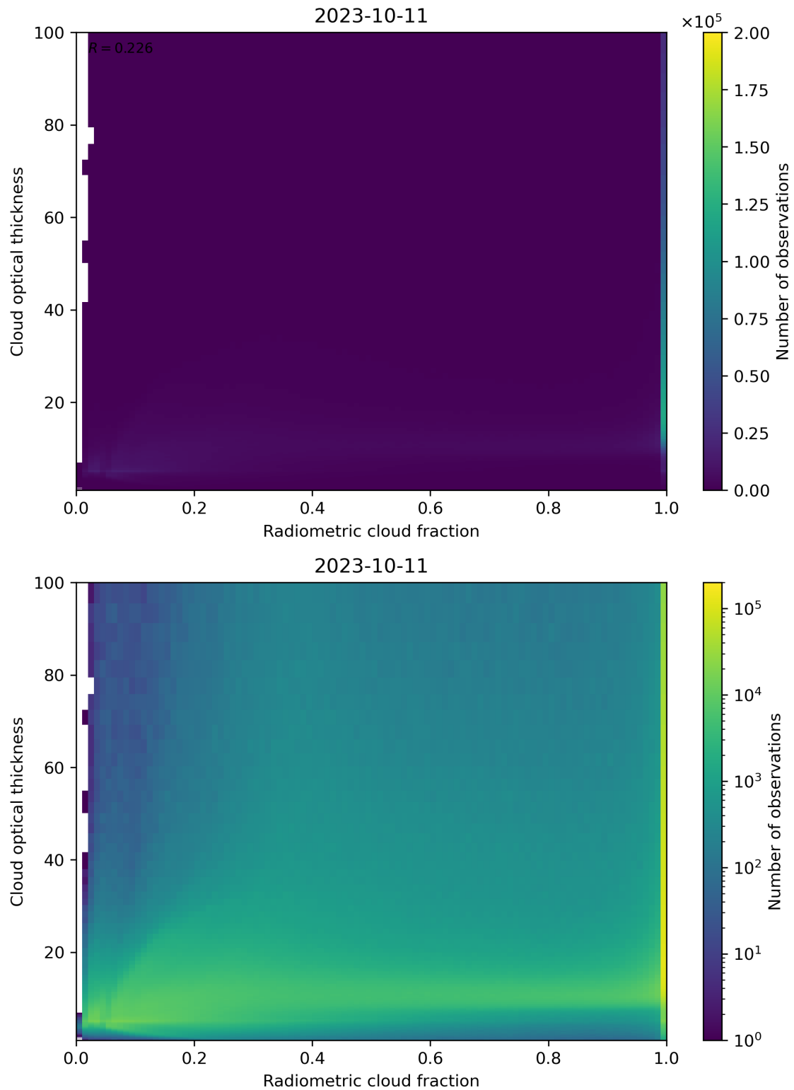
Figure 75: Scatter density plot of “Radiometric cloud fraction” against “Cloud optical thickness” for 2023-10-10 to 2023-10-12.
