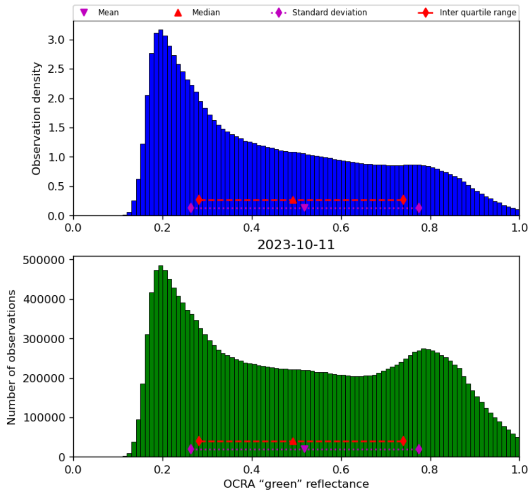
Figure 52: Histogram of “OCRA “green” reflectance” for 2023-10-10 to 2023-10-12
