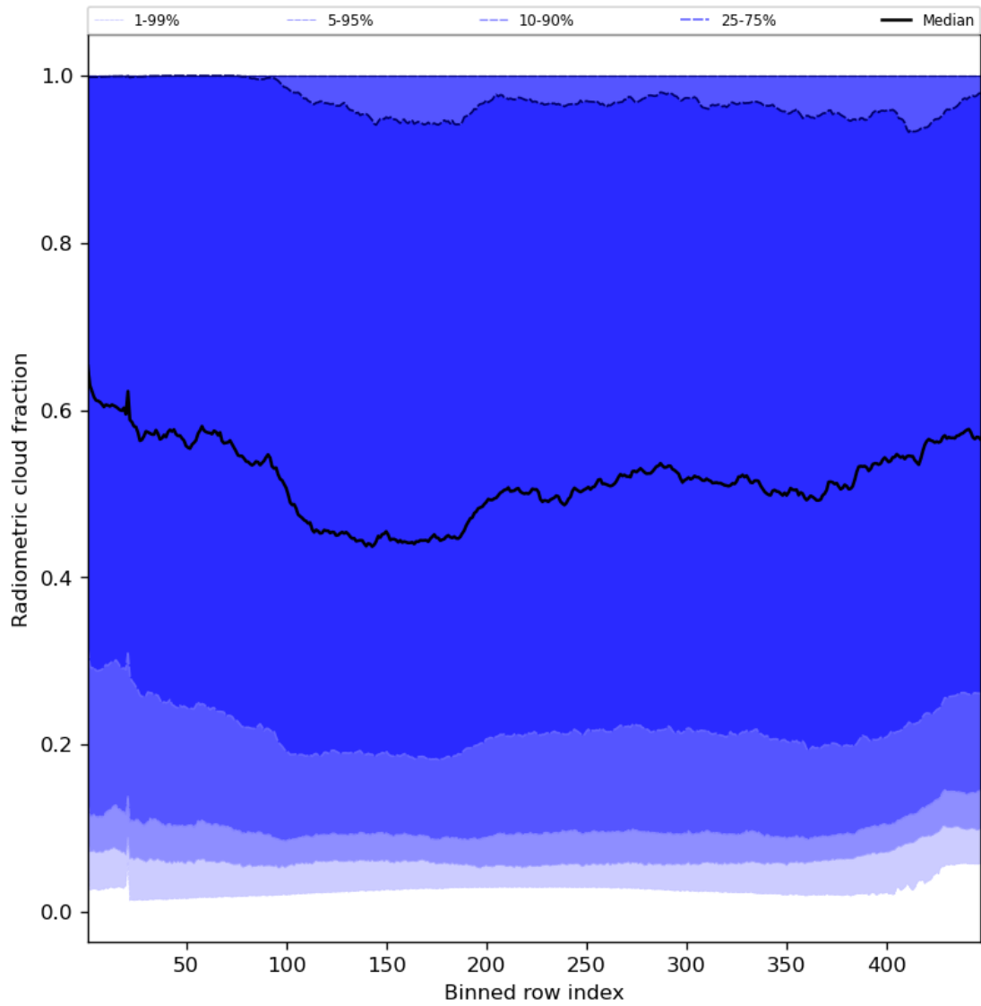
Figure 55: Along track statistics of “Radiometric cloud fraction” for 2023-10-10 to 2023-10-12
