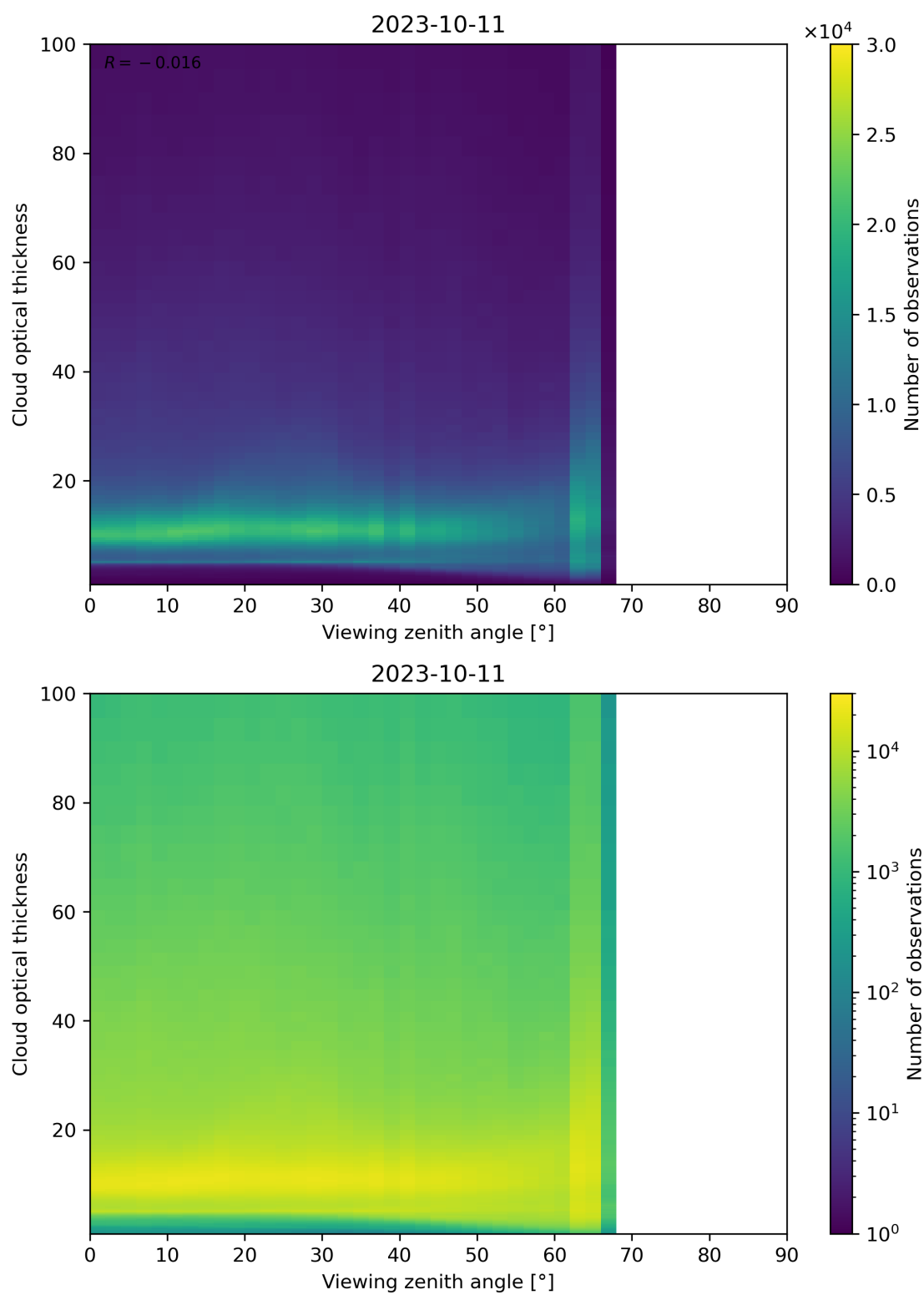
Figure 111: Scatter density plot of “Viewing zenith angle” against “Cloud optical thickness” for 2023-10-10 to 2023-10-12.
