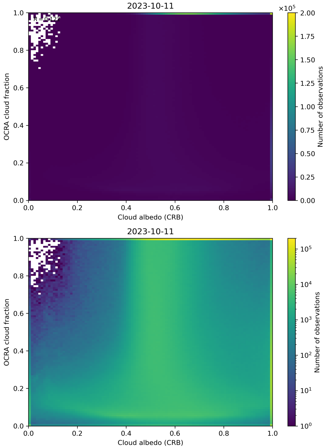
Figure 70: Scatter density plot of “Cloud albedo (CRB)” against “OCRA cloud fraction” for 2023-10-10 to 2023-10-12.
