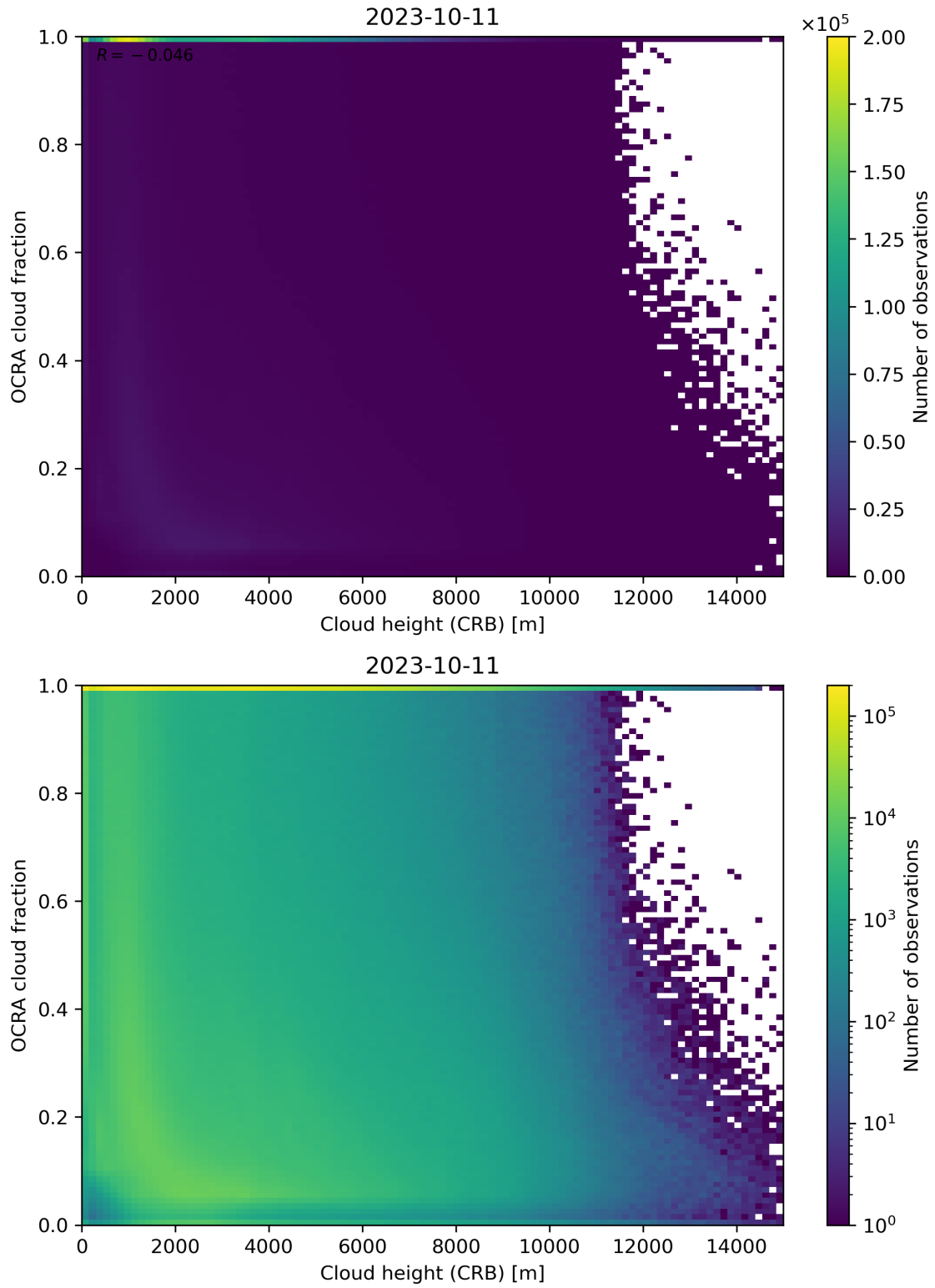
Figure 81: Scatter density plot of “Cloud height (CRB)” against “OCRA cloud fraction” for 2023-10-10 to 2023-10-12.
