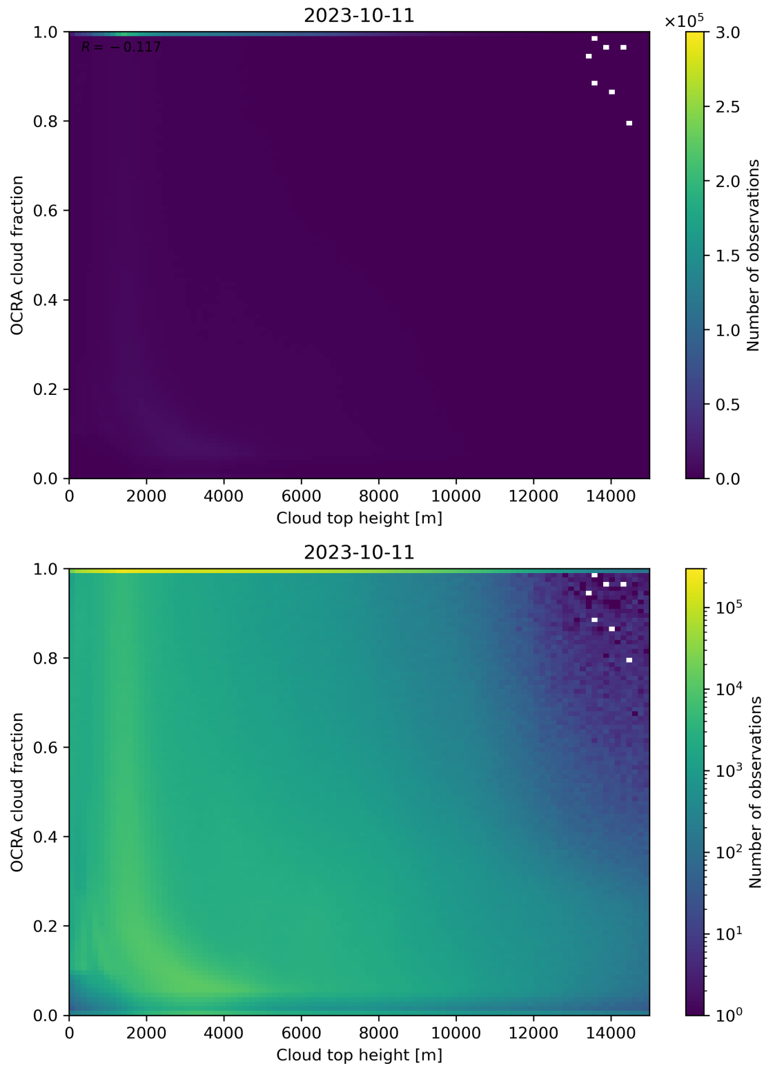
Figure 87: Scatter density plot of “Cloud top height” against “OCRA cloud fraction” for 2023-10-10 to 2023-10-12.
