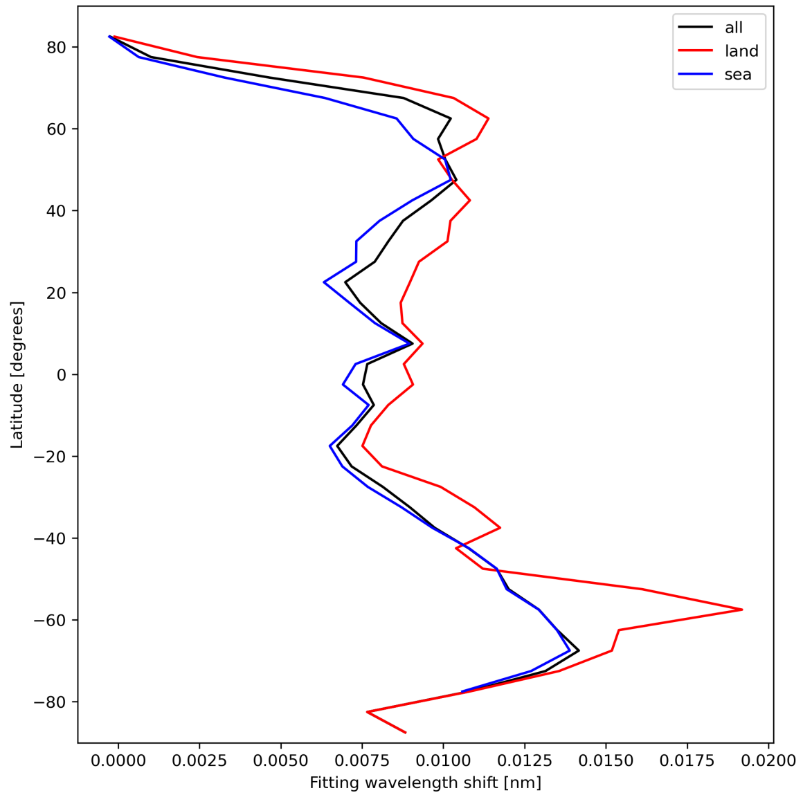
Figure 33: Zonal average of “Fitting wavelength shift” for 2023-10-10 to 2023-10-12.
