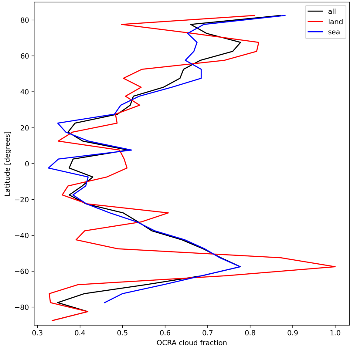
Figure 34: Zonal average of “OCRA cloud fraction” for 2023-10-10 to 2023-10-12.
