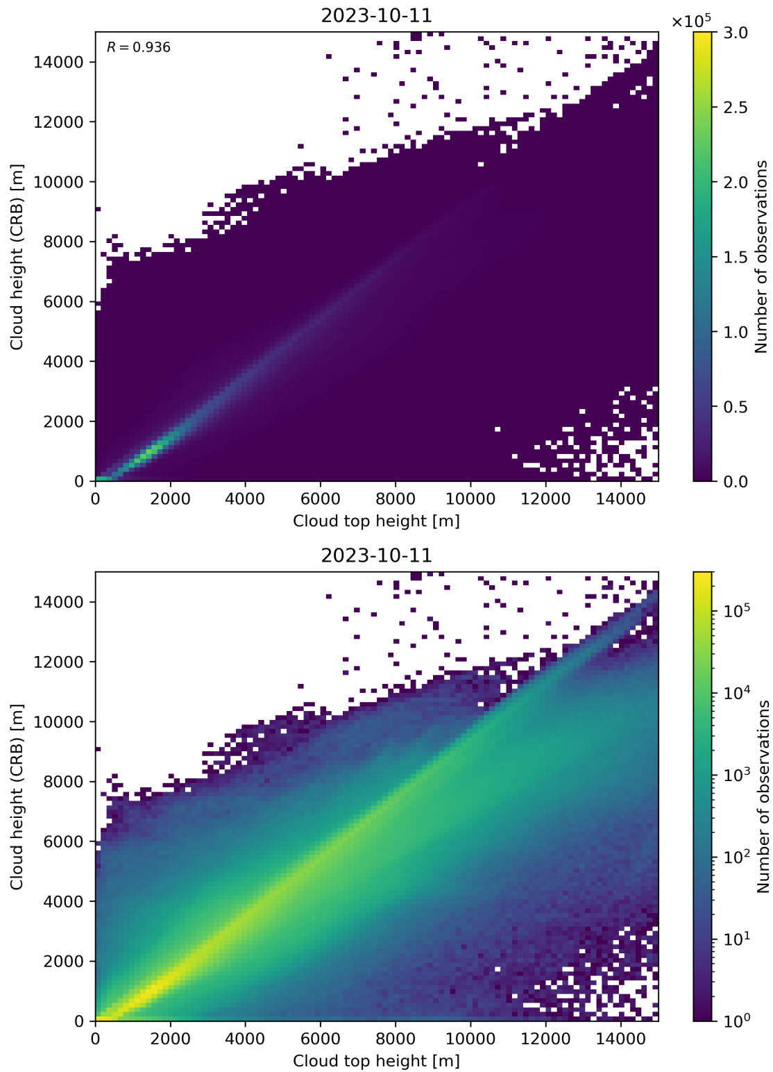
Figure 89: Scatter density plot of “Cloud top height” against “Cloud height (CRB)” for 2023-10-10 to 2023-10-12.
