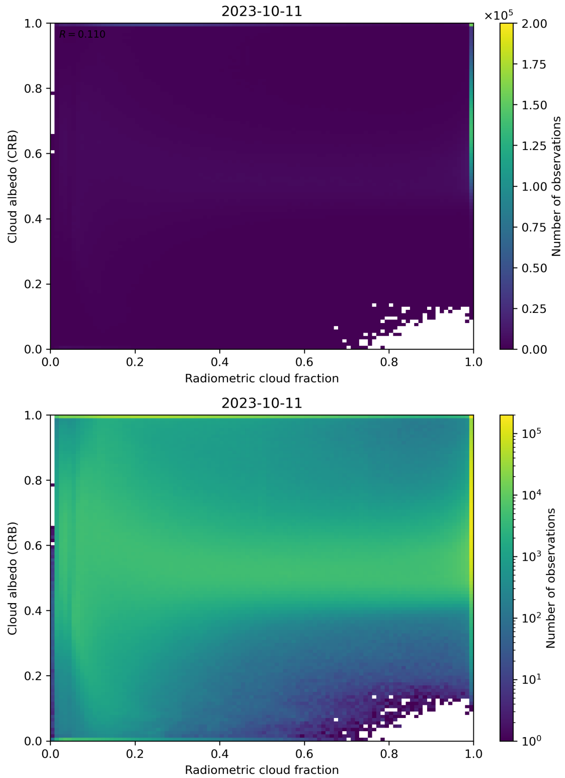
Figure 71: Scatter density plot of “Radiometric cloud fraction” against “Cloud albedo (CRB)” for 2023-10-10 to 2023-10-12.
