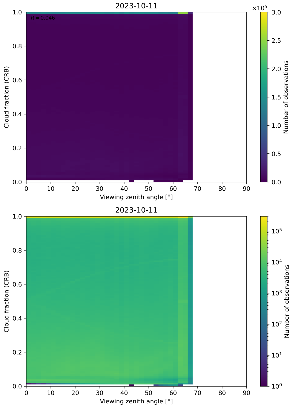
Figure 109: Scatter density plot of “Viewing zenith angle” against “Cloud fraction (CRB)” for 2023-10-10 to 2023-10-12.
