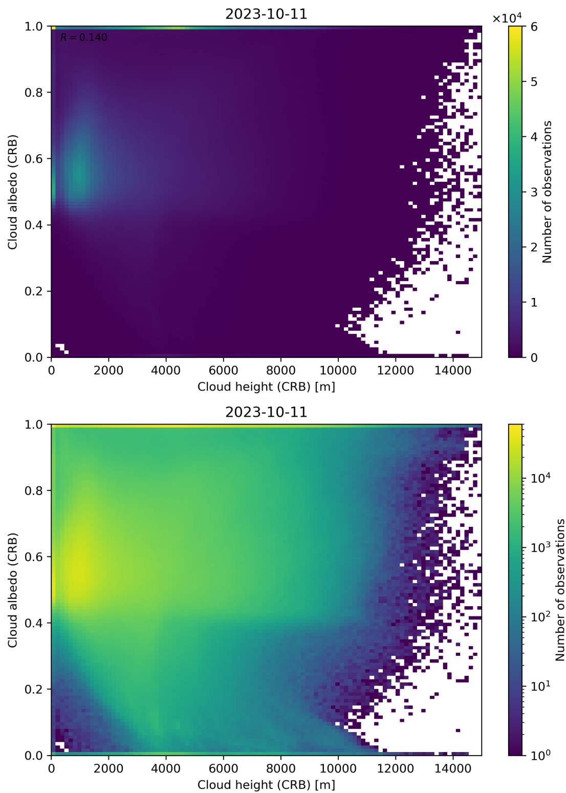
Figure 80: Scatter density plot of “Cloud height (CRB)” against “Cloud albedo (CRB)” for 2023-10-10 to 2023-10-12.
