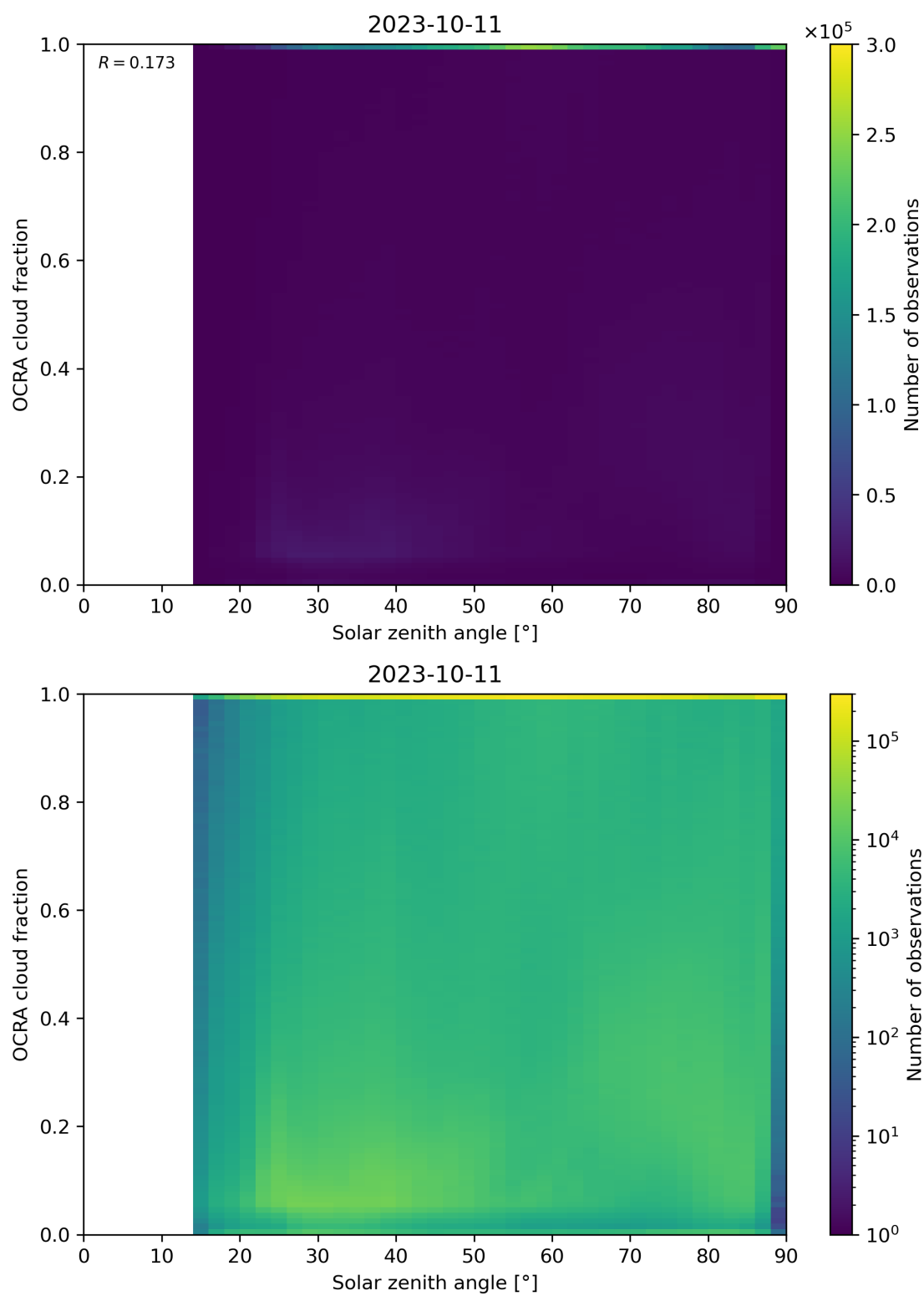
Figure 100: Scatter density plot of “Solar zenith angle” against “OCRA cloud fraction” for 2023-10-10 to 2023-10-12.
