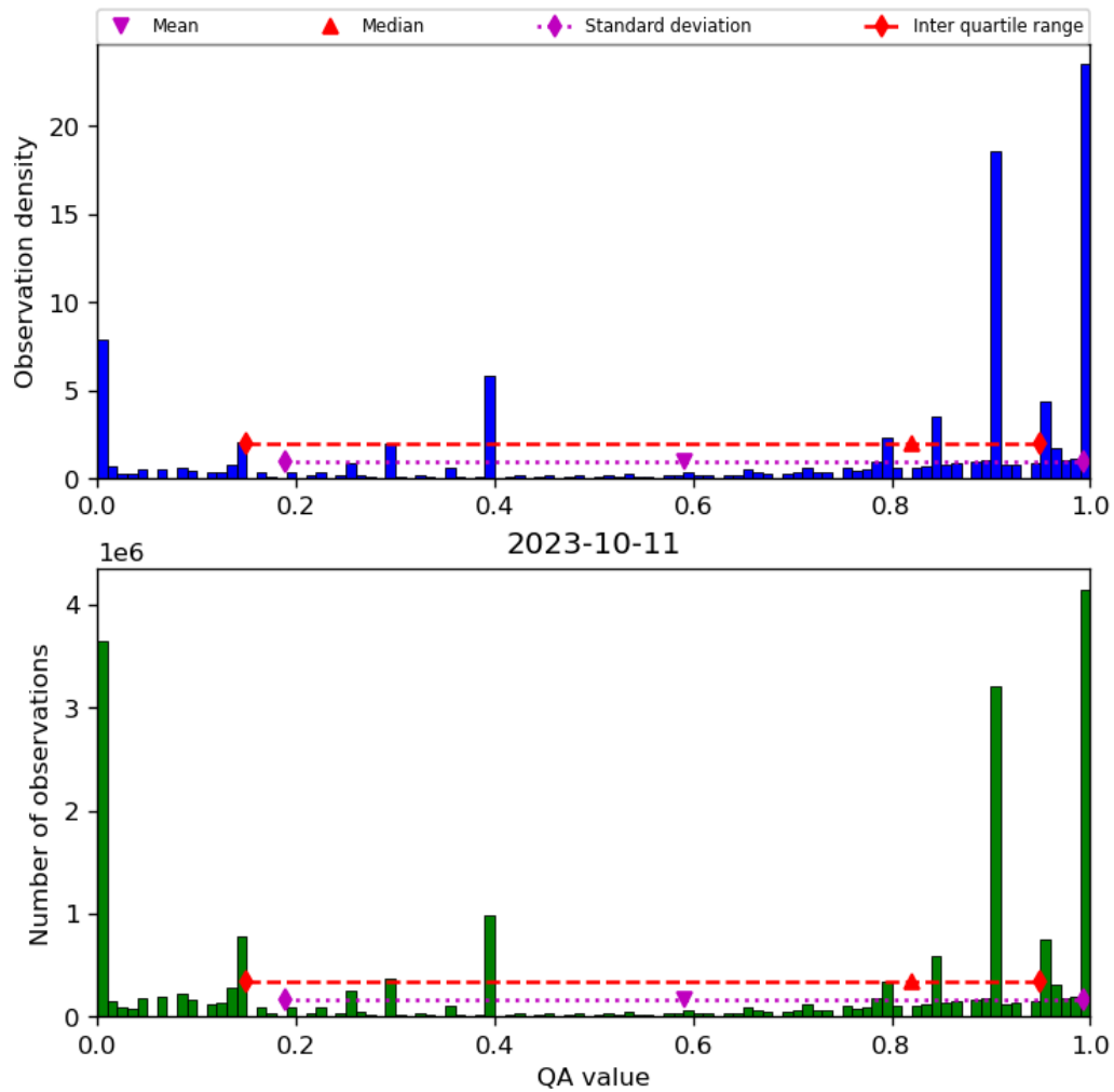
Figure 38: Histogram of “QA value” for 2023-10-10 to 2023-10-12
