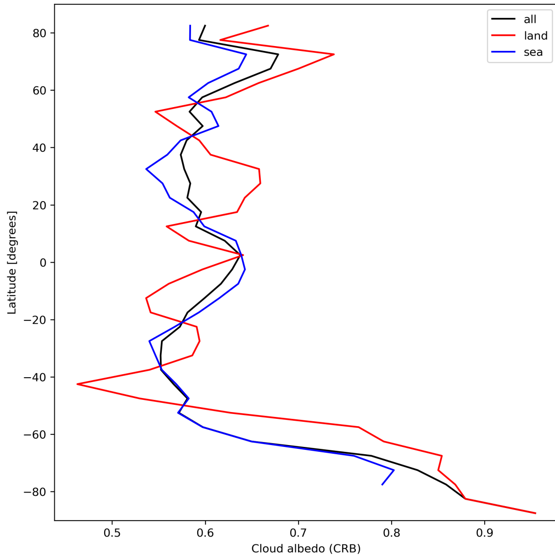
Figure 28: Zonal average of “Cloud albedo (CRB)” for 2023-10-10 to 2023-10-12.
