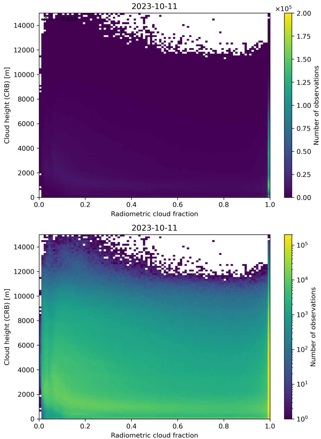
Figure 74: Scatter density plot of “Radiometric cloud fraction” against “Cloud height (CRB)” for 2023-10-10 to 2023-10-12.
