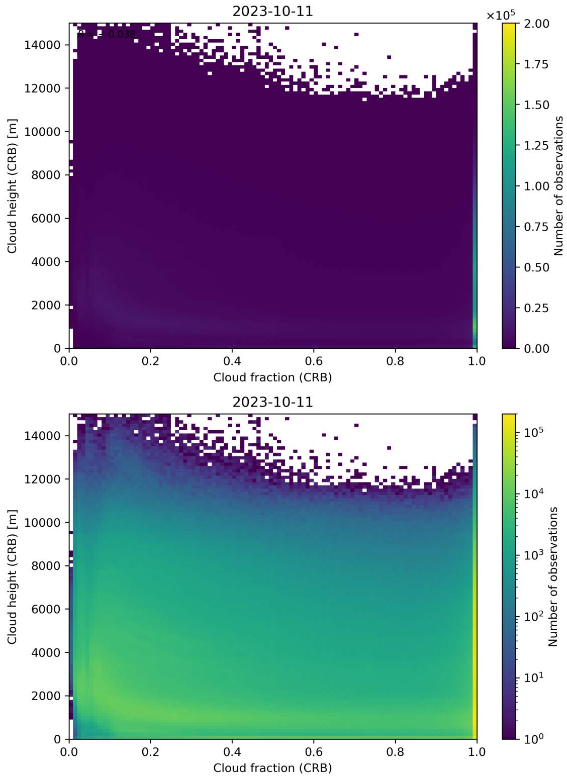
Figure 79: Scatter density plot of “Cloud fraction (CRB)” against “Cloud height (CRB)” for 2023-10-10 to 2023-10-12.
