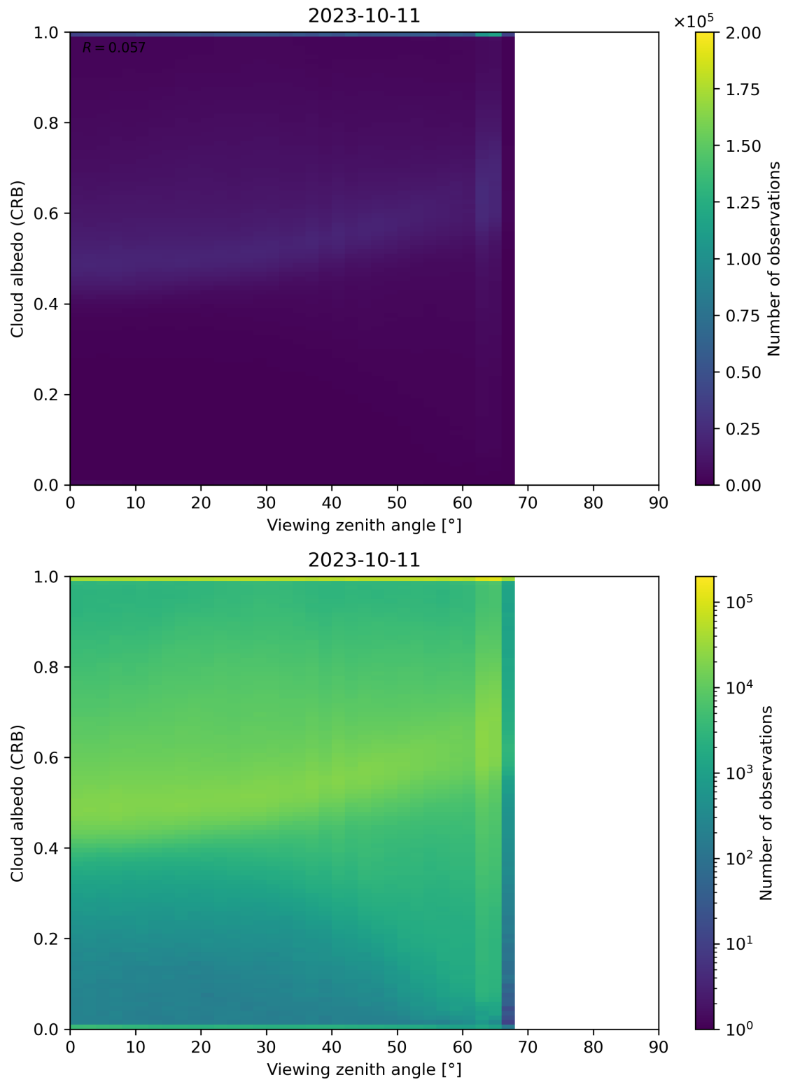
Figure 106: Scatter density plot of “Viewing zenith angle” against “Cloud albedo (CRB)” for 2023-10-10 to 2023-10-12.
