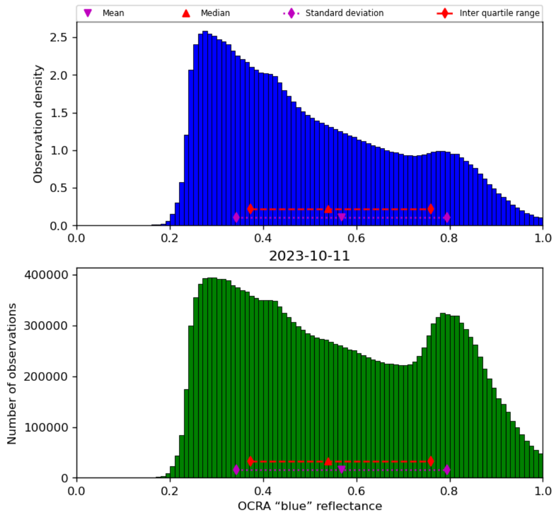
Figure 51: Histogram of “OCRA “blue” reflectance” for 2023-10-10 to 2023-10-12
