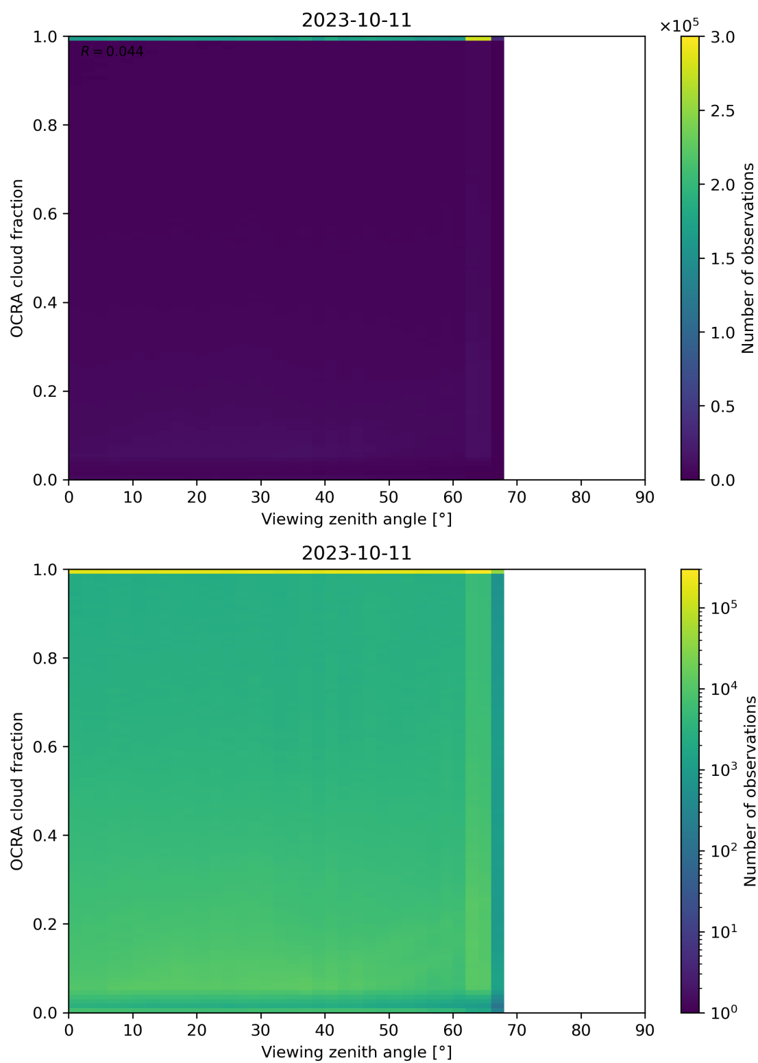
Figure 108: Scatter density plot of “Viewing zenith angle” against “OCRA cloud fraction” for 2023-10-10 to 2023-10-12.
