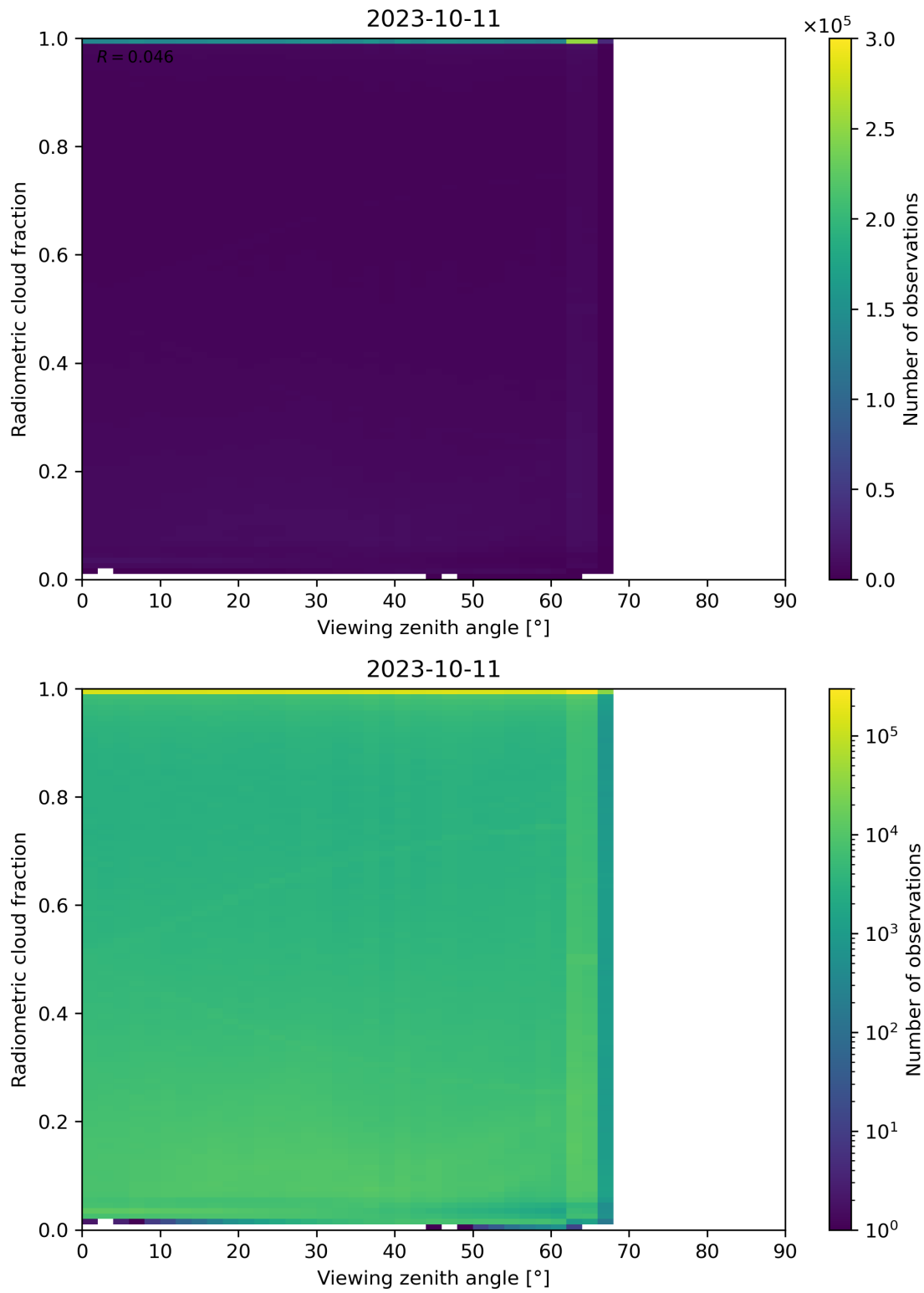
Figure 107: Scatter density plot of “Viewing zenith angle” against “Radiometric cloud fraction” for 2023-10-10 to 2023-10-12.
