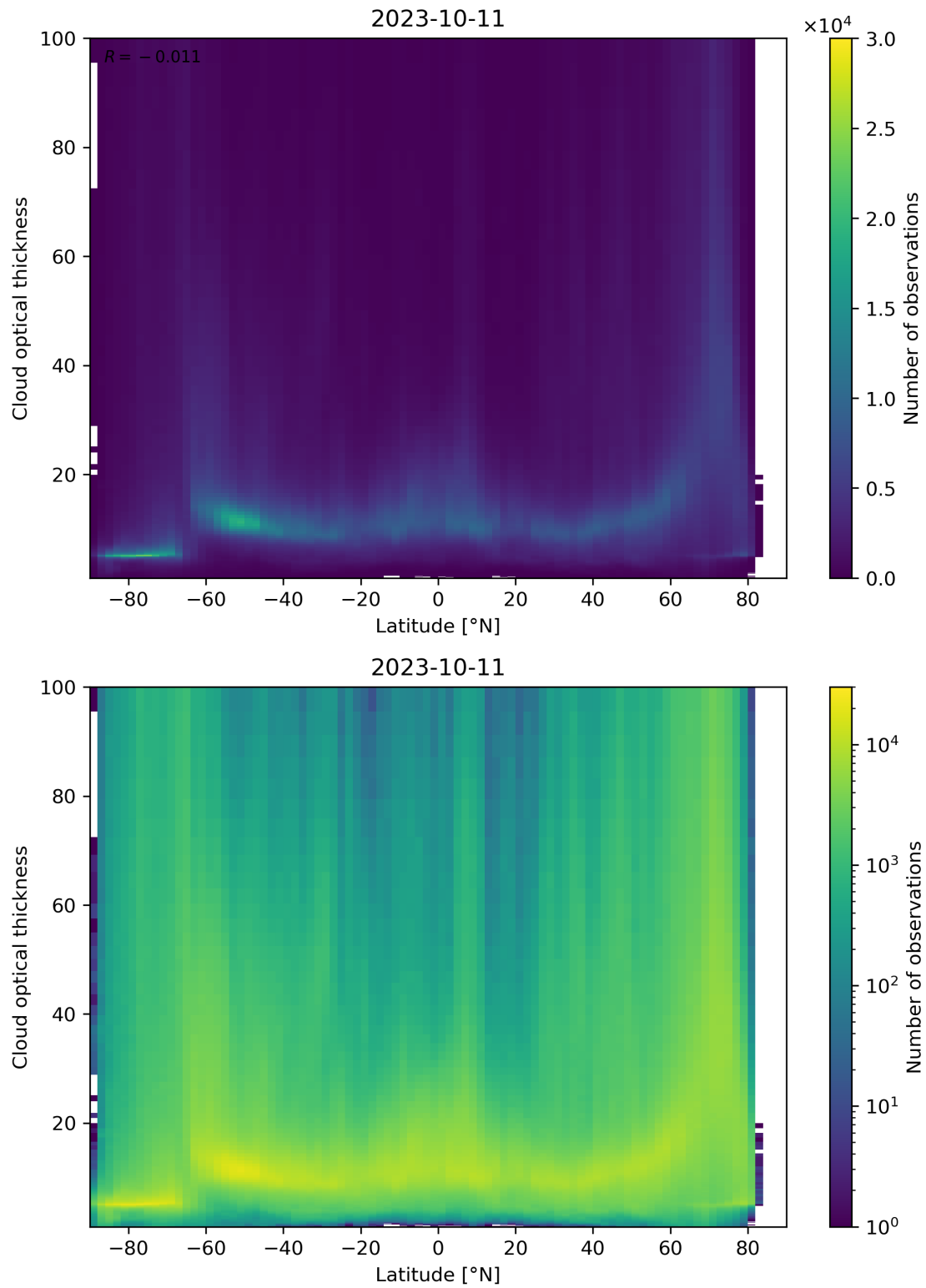
Figure 96: Scatter density plot of “Latitude” against “Cloud optical thickness” for 2023-10-10 to 2023-10-12.
