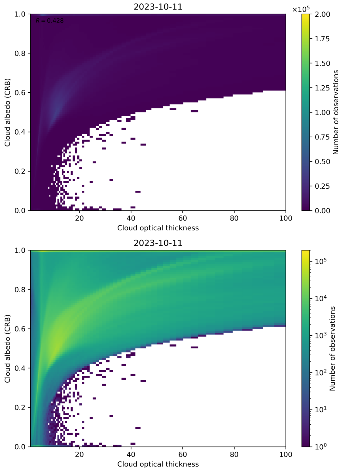
Figure 82: Scatter density plot of “Cloud optical thickness” against “Cloud albedo (CRB)” for 2023-10-10 to 2023-10-12.
