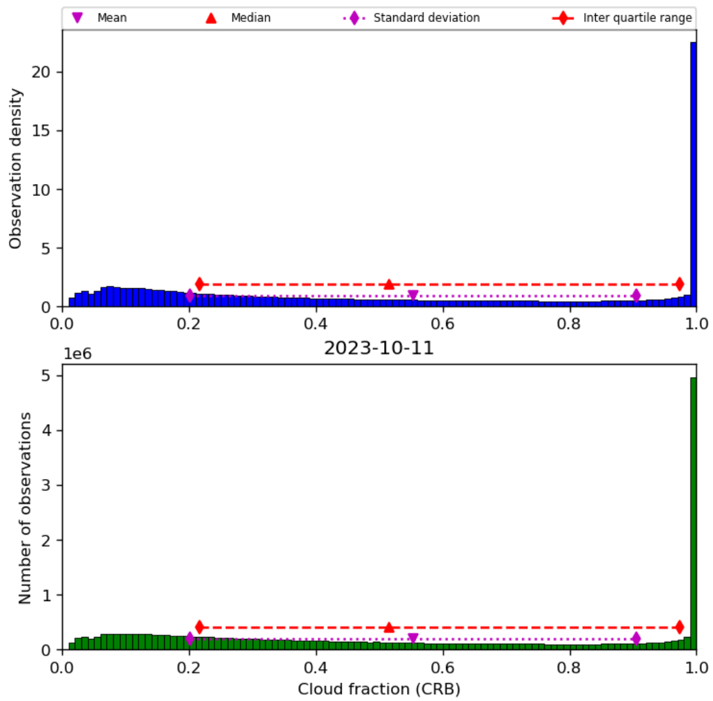
Figure 42: Histogram of “Cloud fraction (CRB)” for 2023-10-10 to 2023-10-12
