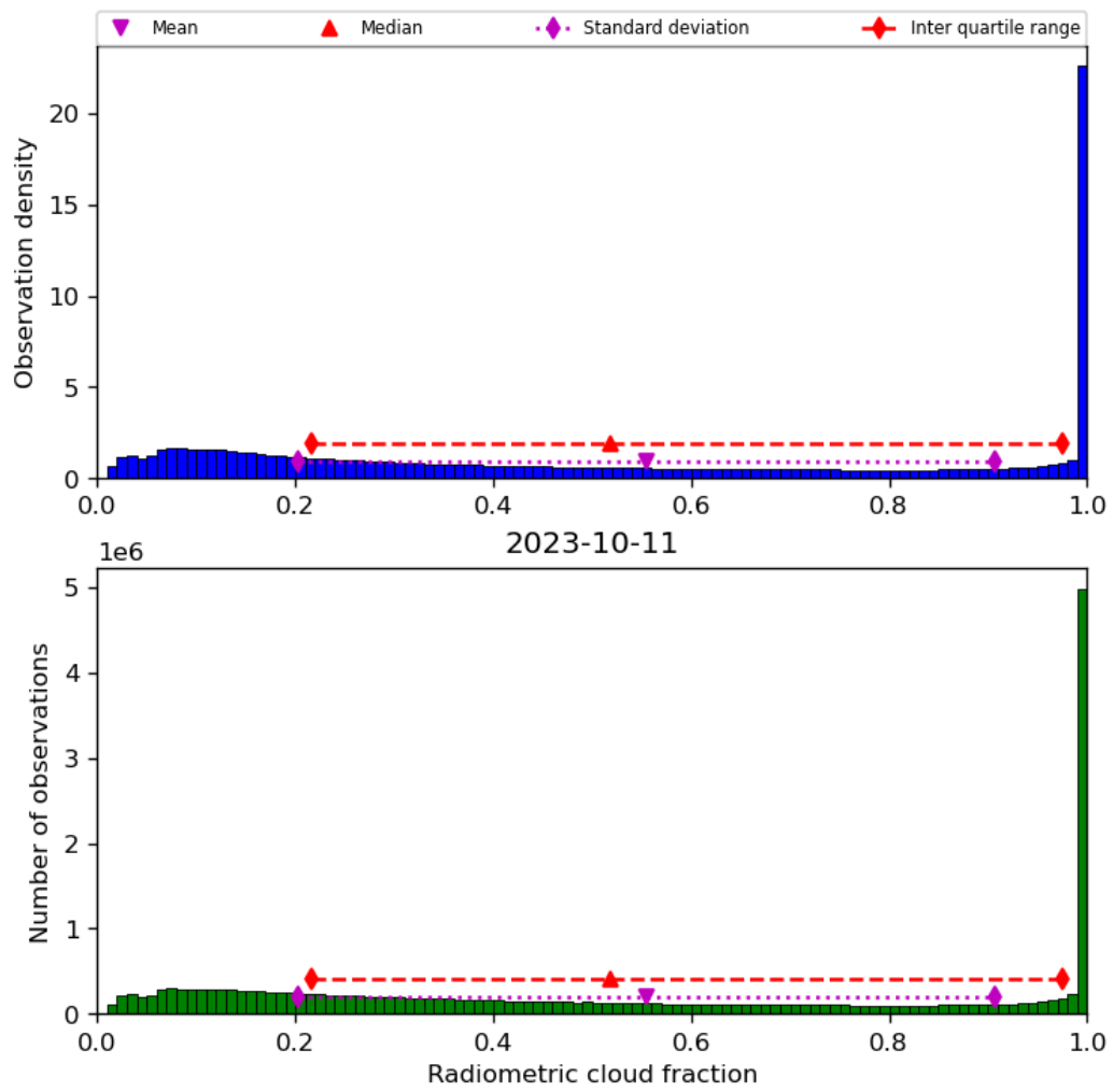
Figure 39: Histogram of “Radiometric cloud fraction” for 2023-10-10 to 2023-10-12
