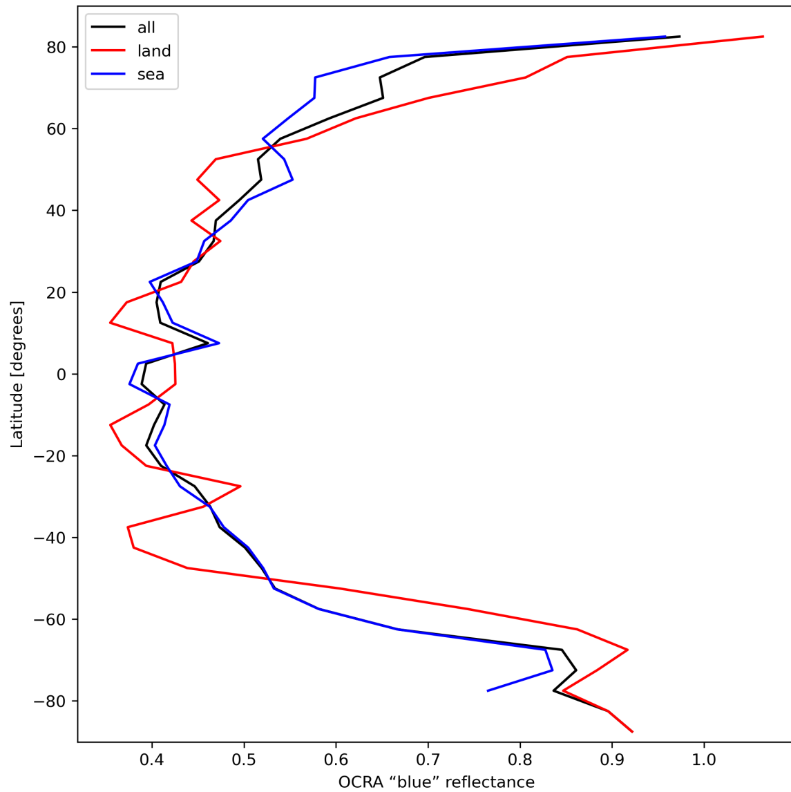
Figure 35: Zonal average of “OCRA “blue” reflectance” for 2023-10-10 to 2023-10-12.
