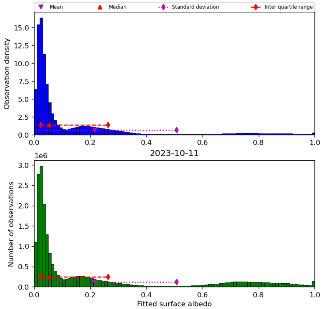
Figure 45: Histogram of “Fitted surface albedo” for 2023-10-10 to 2023-10-12
