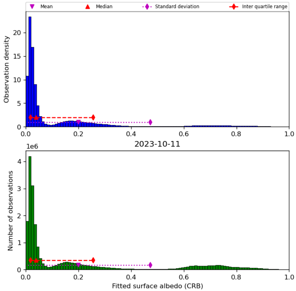
Figure 46: Histogram of “Fitted surface albedo (CRB)” for 2023-10-10 to 2023-10-12
