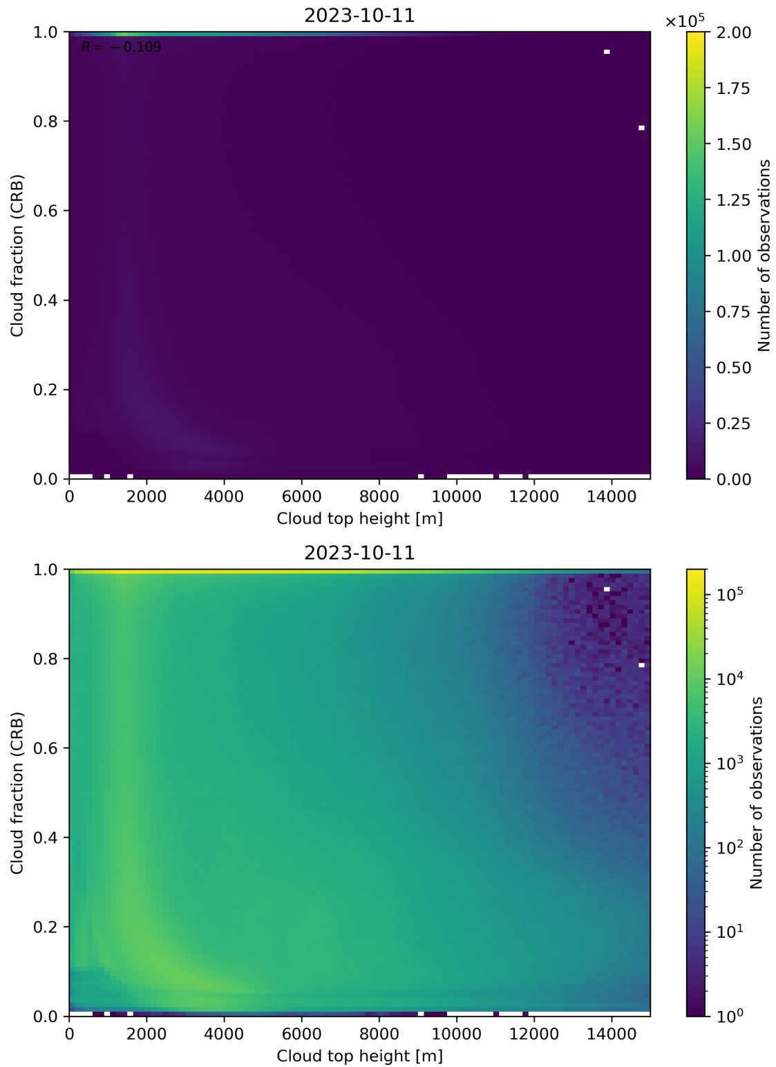
Figure 88: Scatter density plot of “Cloud top height” against “Cloud fraction (CRB)” for 2023-10-10 to 2023-10-12.
