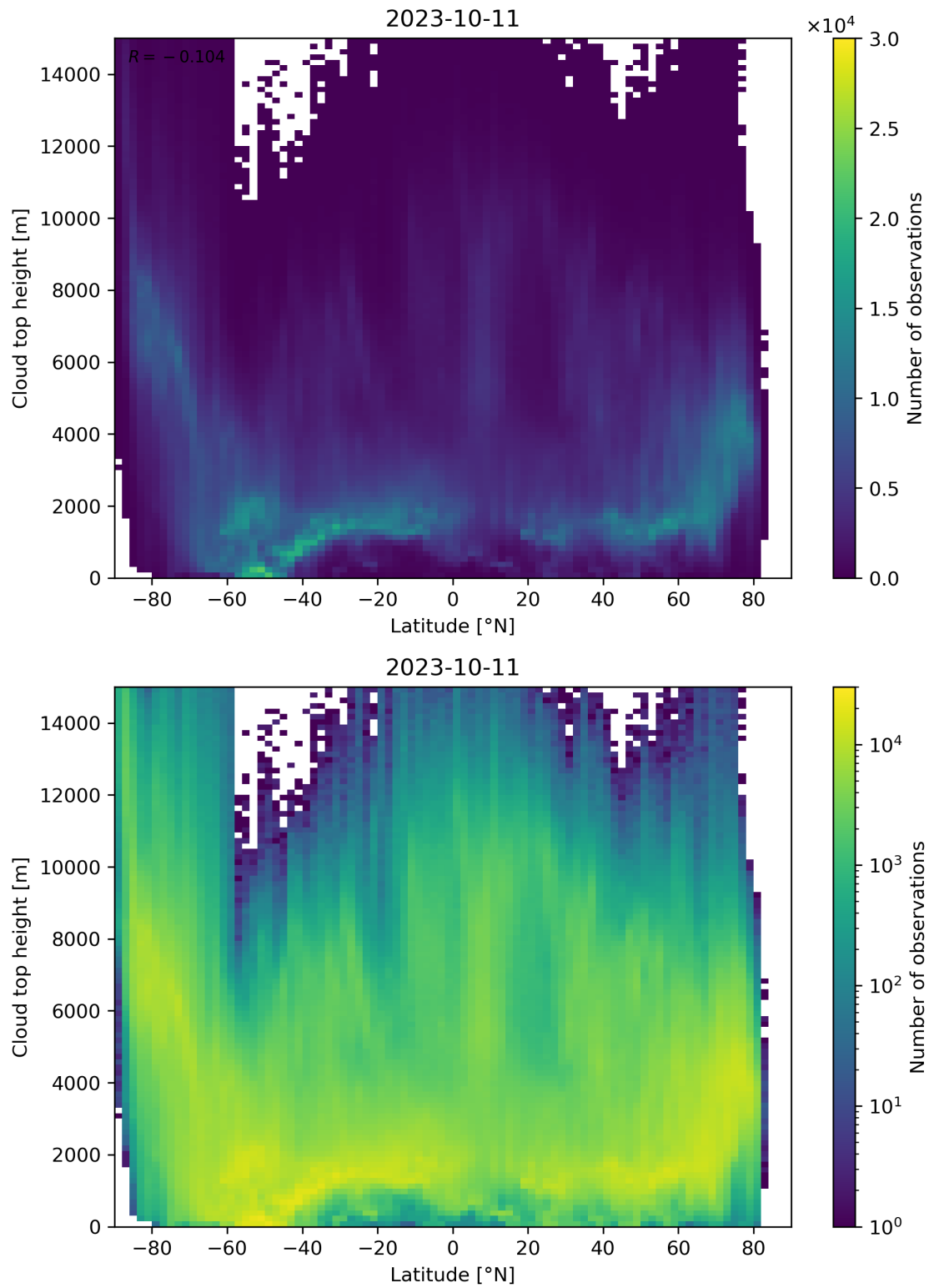
Figure 97: Scatter density plot of “Latitude” against “Cloud top height” for 2023-10-10 to 2023-10-12.
