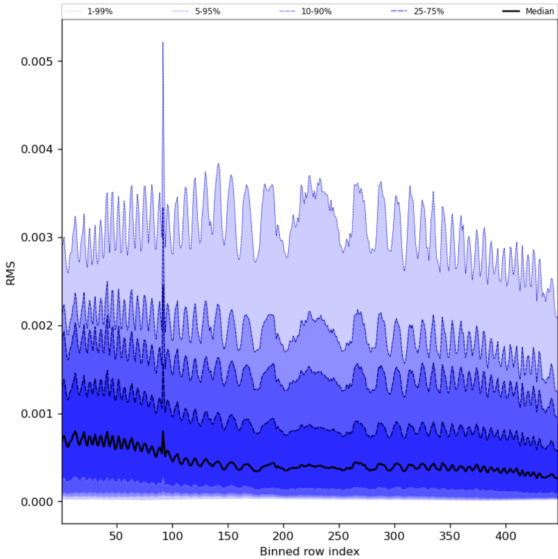
Figure 63: Along track statistics of “RMS” for 2023-10-10 to 2023-10-12
