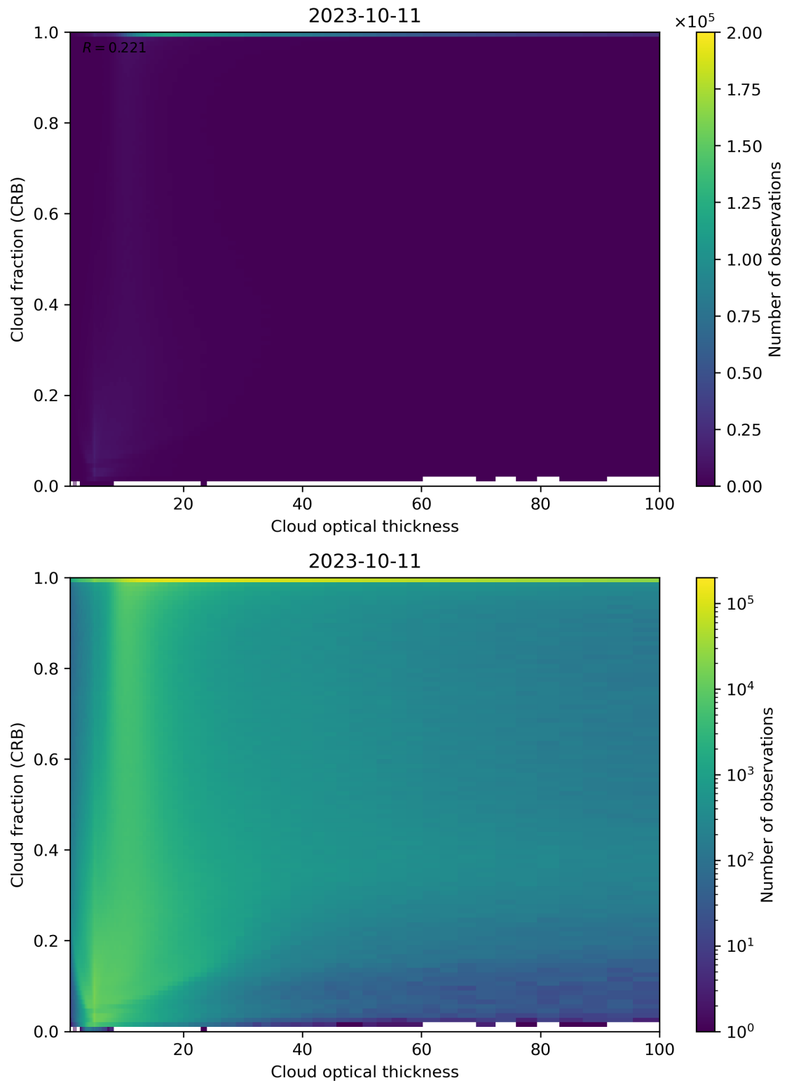
Figure 84: Scatter density plot of “Cloud optical thickness” against “Cloud fraction (CRB)” for 2023-10-10 to 2023-10-12.
