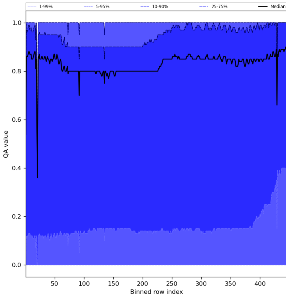
Figure 54: Along track statistics of “QA value” for 2023-10-10 to 2023-10-12
