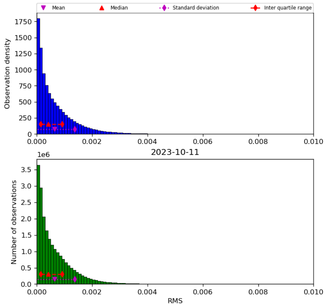
Figure 47: Histogram of “RMS” for 2023-10-10 to 2023-10-12
