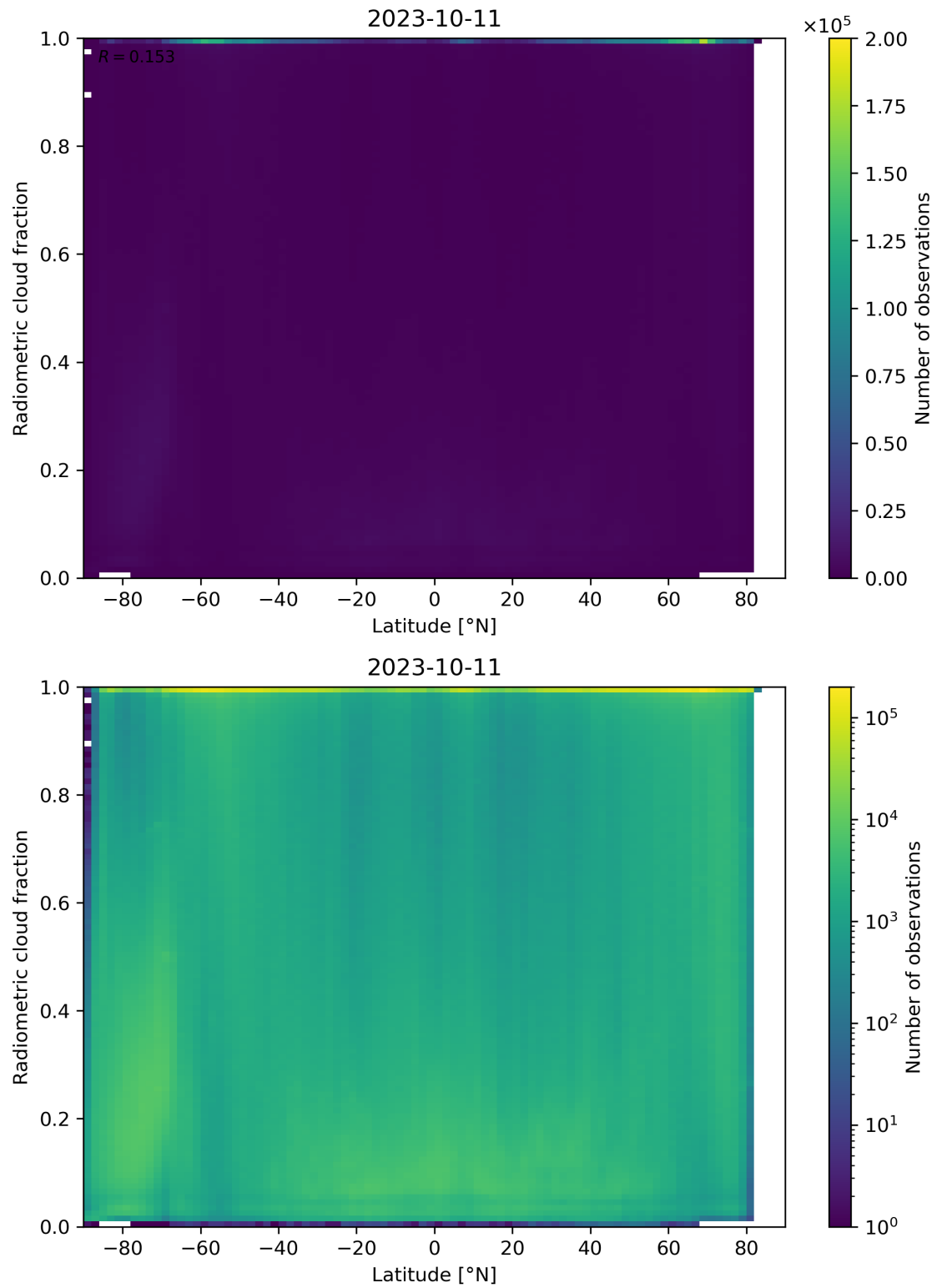
Figure 92: Scatter density plot of “Latitude” against “Radiometric cloud fraction” for 2023-10-10 to 2023-10-12.
