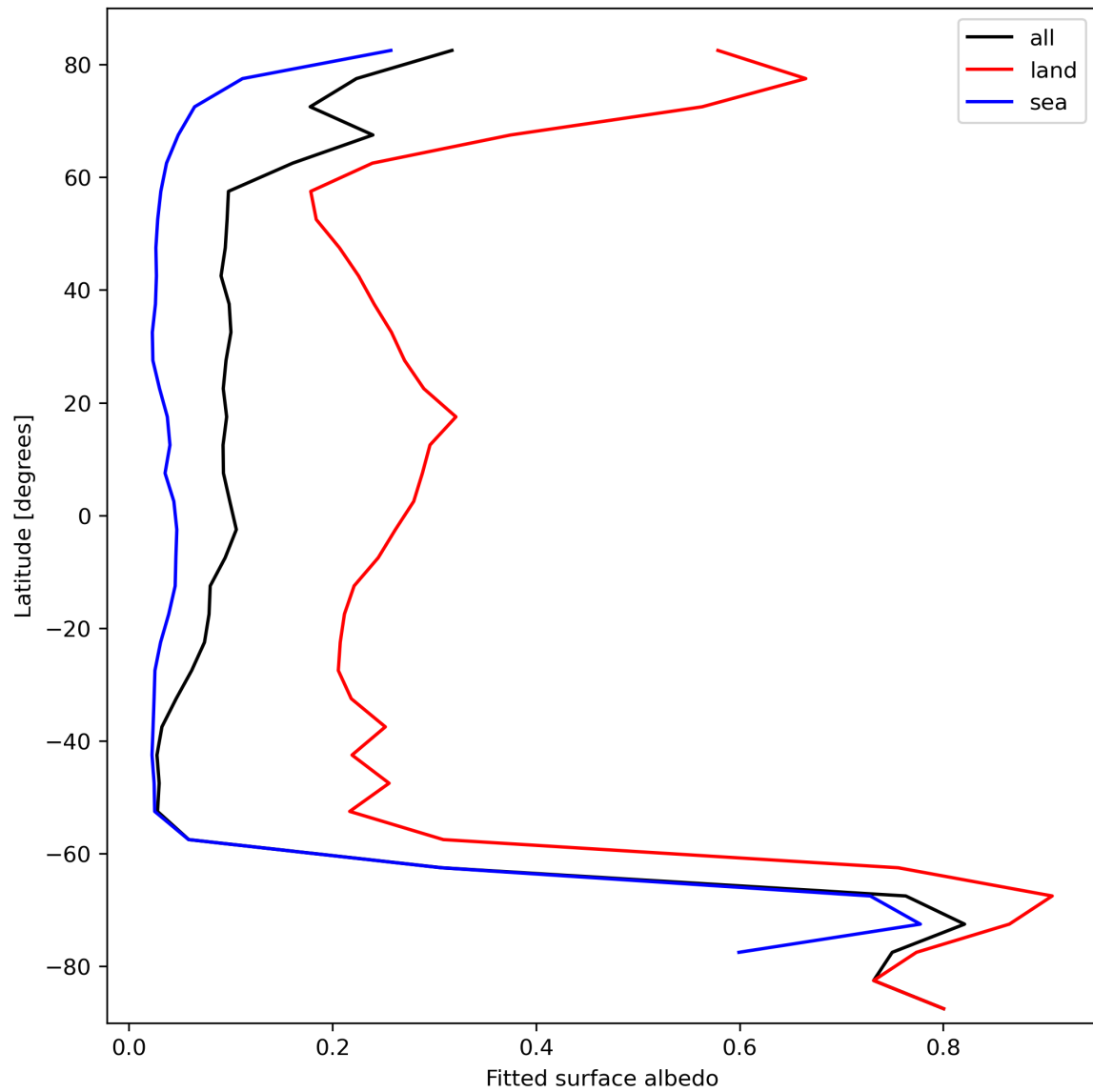
Figure 29: Zonal average of “Fitted surface albedo” for 2023-10-10 to 2023-10-12.
