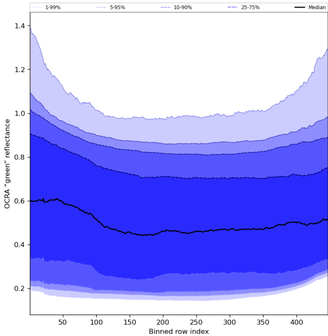
Figure 68: Along track statistics of “OCRA “green” reflectance” for 2023-10-10 to 2023-10-12
