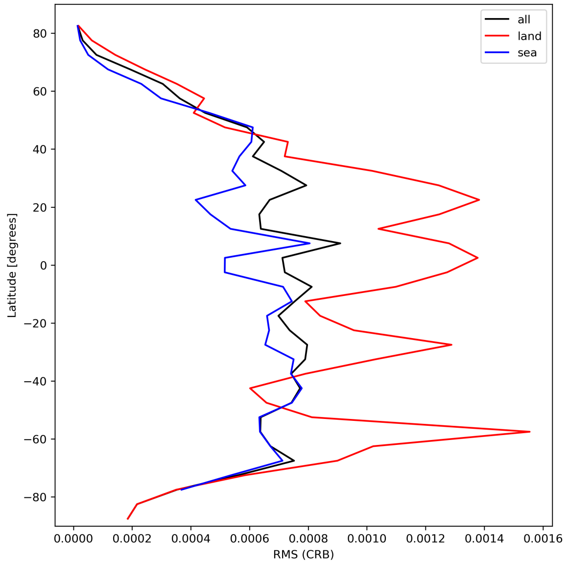
Figure 32: Zonal average of “RMS (CRB)” for 2023-10-10 to 2023-10-12.
