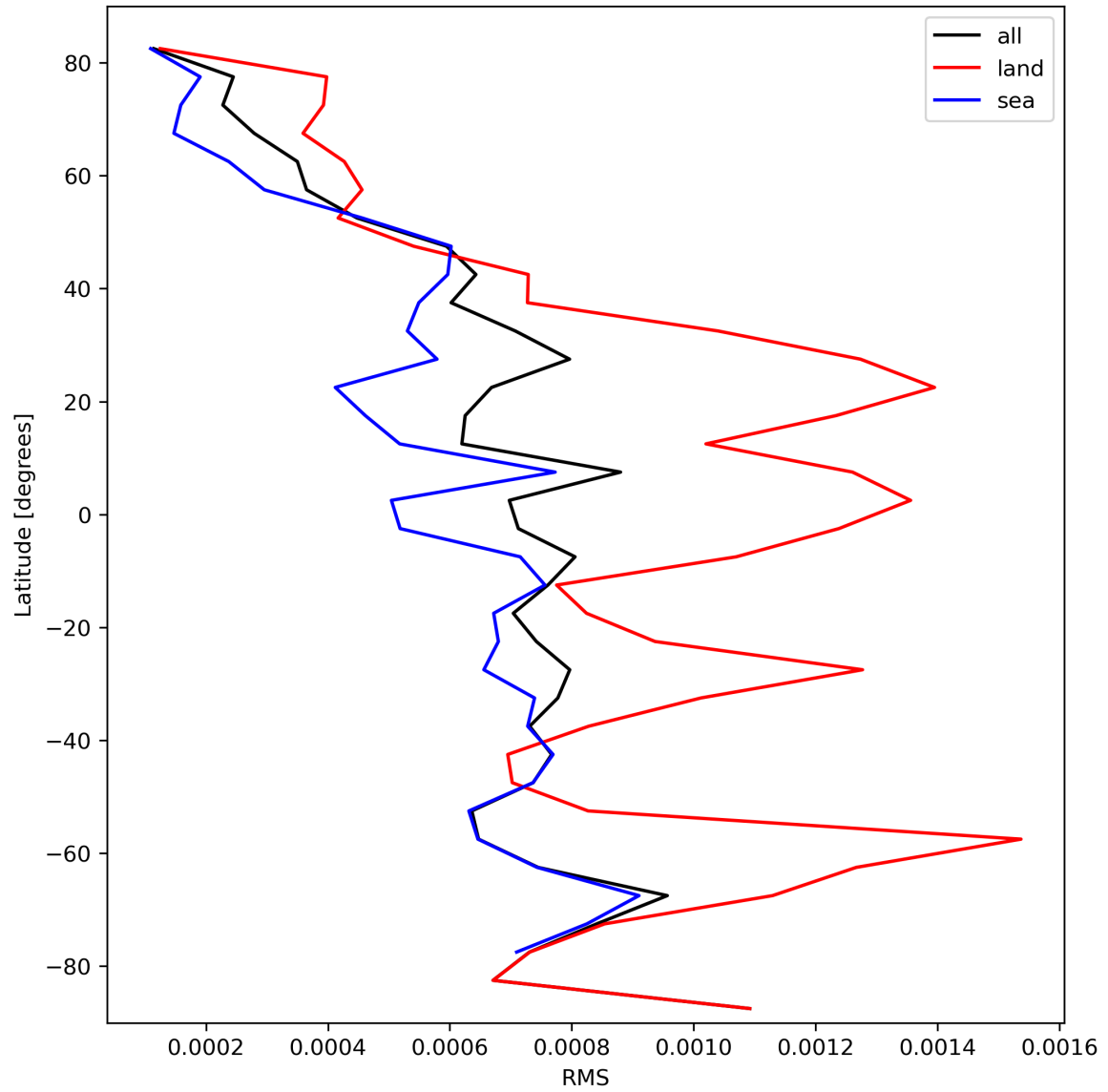
Figure 31: Zonal average of “RMS” for 2023-10-10 to 2023-10-12.
