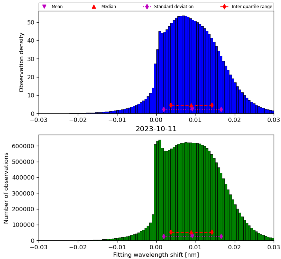
Figure 49: Histogram of “Fitting wavelength shift” for 2023-10-10 to 2023-10-12
