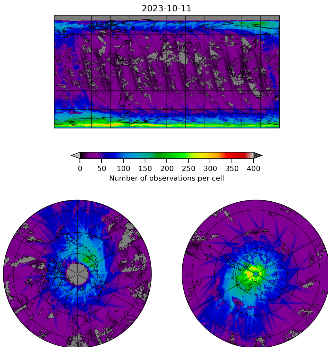
Figure 21: Map of the number of observations for 2023-10-10 to 2023-10-12
