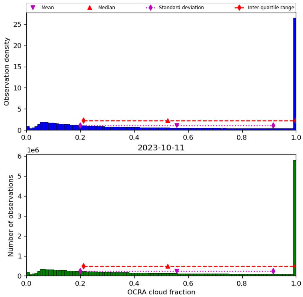
Figure 50: Histogram of “OCRA cloud fraction” for 2023-10-10 to 2023-10-12
