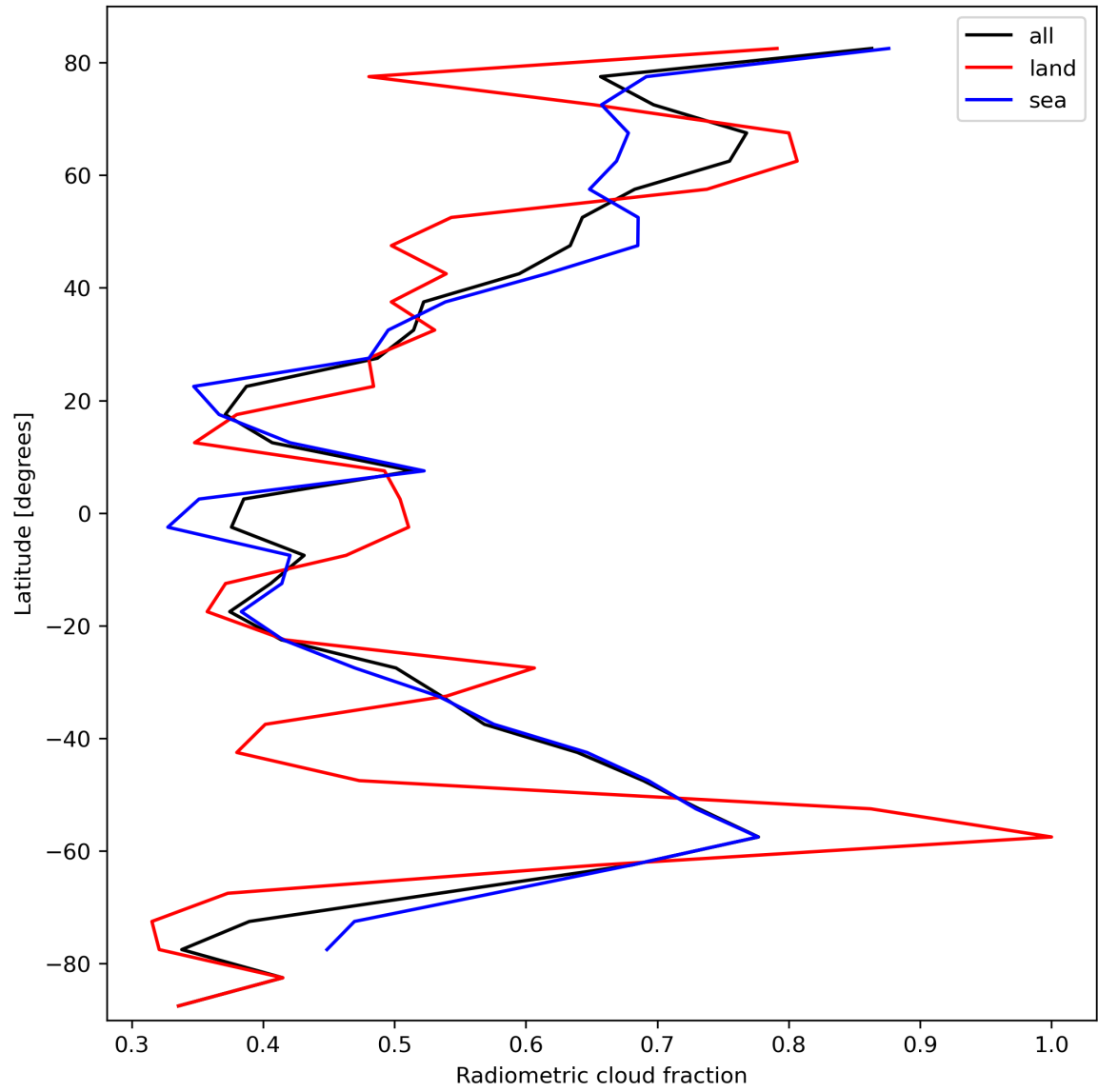
Figure 23: Zonal average of “Radiometric cloud fraction” for 2023-10-10 to 2023-10-12.
