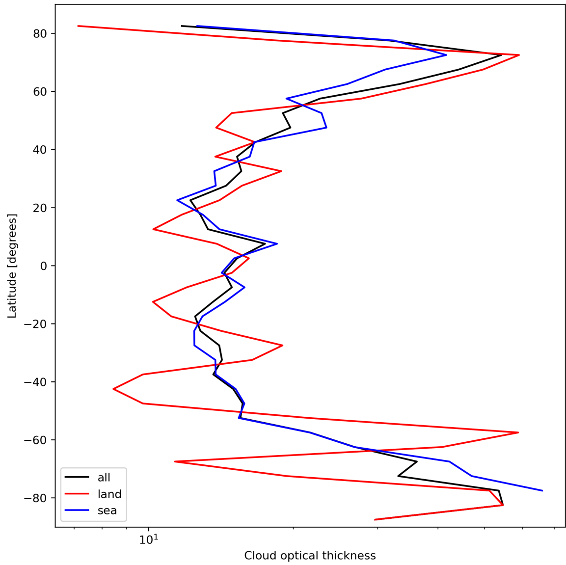
Figure 25: Zonal average of “Cloud optical thickness” for 2023-10-10 to 2023-10-12.
