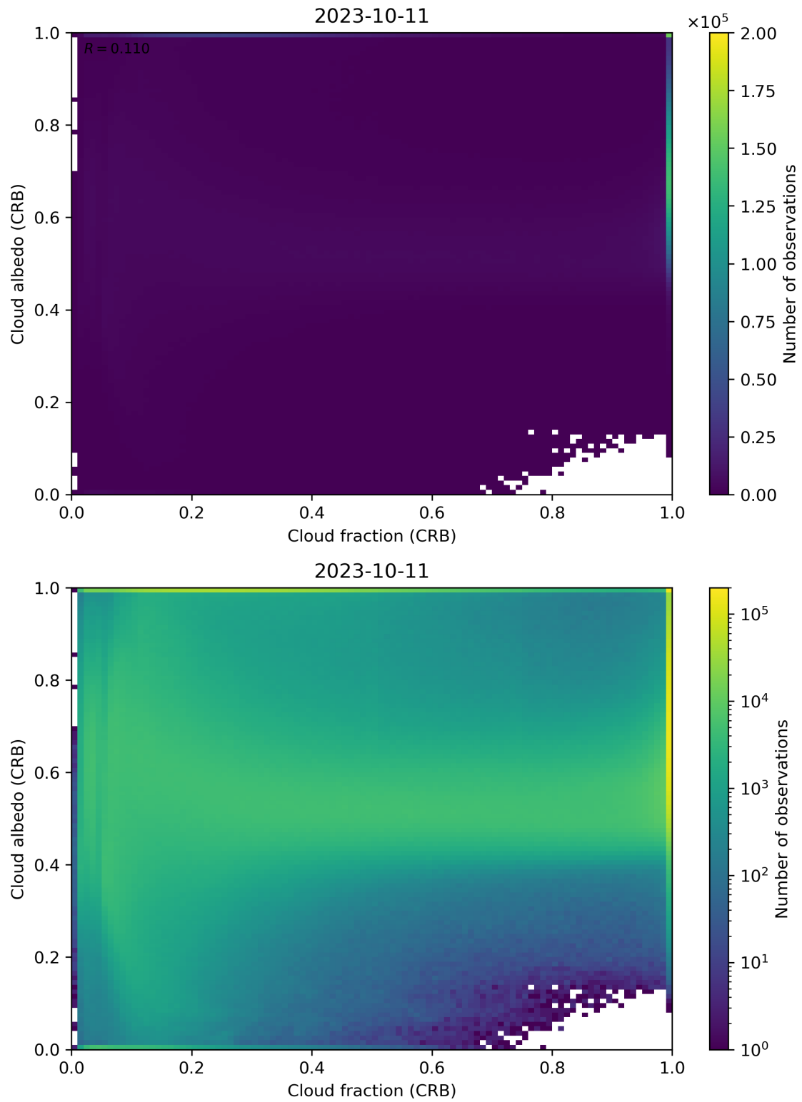
Figure 77: Scatter density plot of “Cloud fraction (CRB)” against “Cloud albedo (CRB)” for 2023-10-10 to 2023-10-12.
