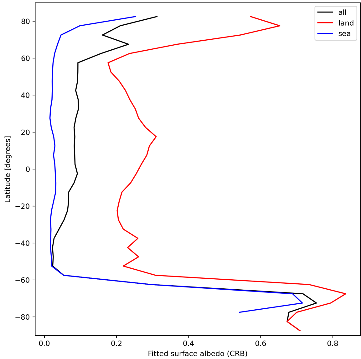
Figure 30: Zonal average of “Fitted surface albedo (CRB)” for 2023-10-10 to 2023-10-12.
