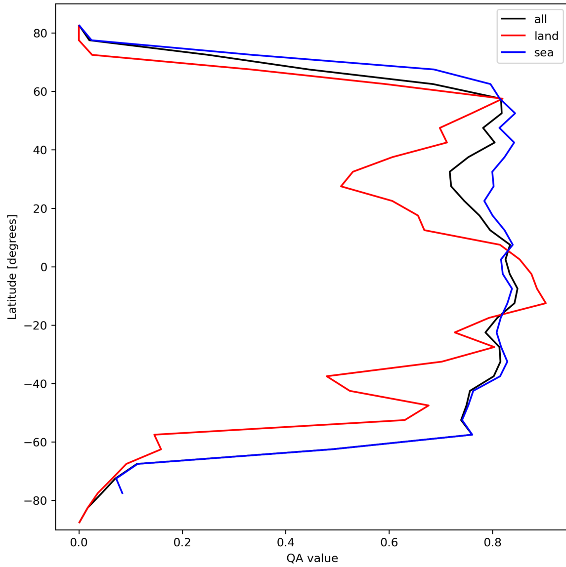
Figure 22: Zonal average of “QA value” for 2023-10-10 to 2023-10-12.
