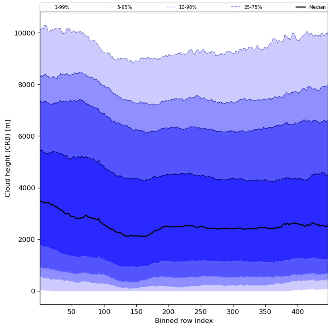
Figure 59: Along track statistics of “Cloud height (CRB)” for 2023-10-10 to 2023-10-12
