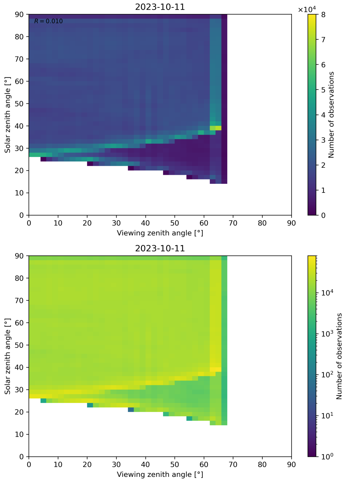
Figure 114: Scatter density plot of “Viewing zenith angle” against “Solar zenith angle” for 2023-10-10 to 2023-10-12.
