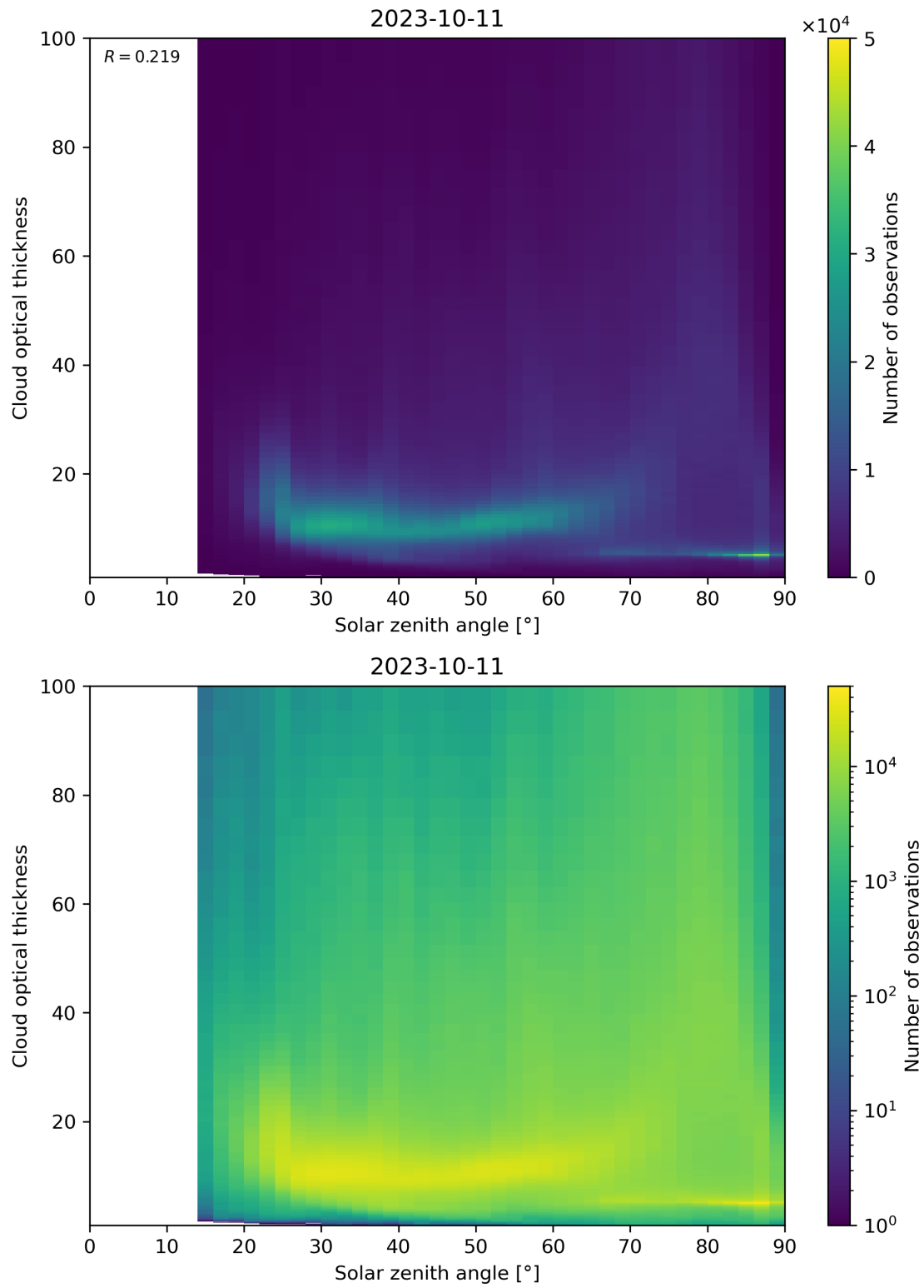
Figure 103: Scatter density plot of “Solar zenith angle” against “Cloud optical thickness” for 2023-10-10 to 2023-10-12.
