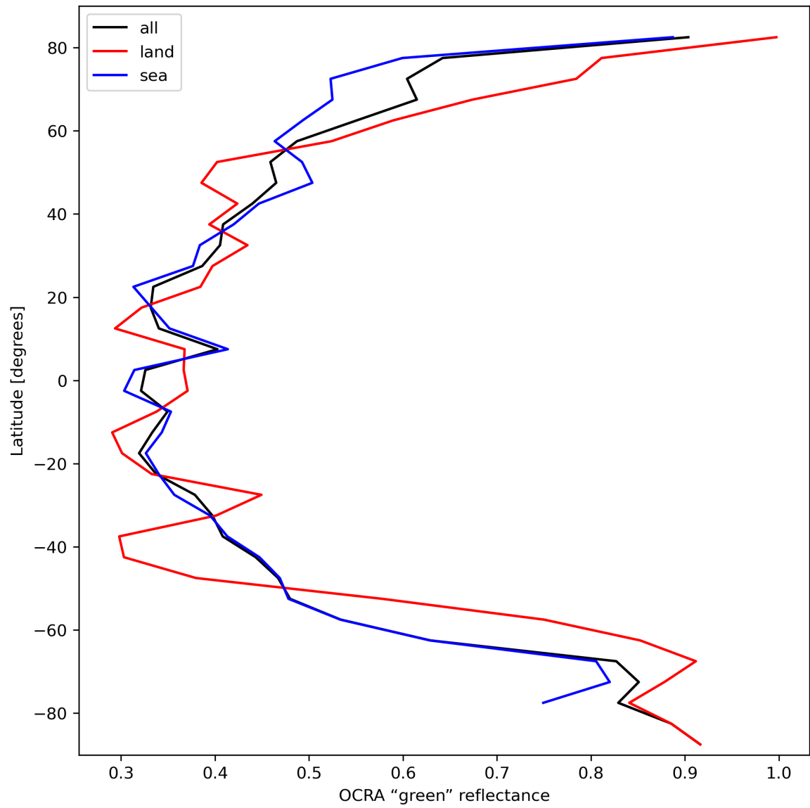
Figure 36: Zonal average of “OCRA “green” reflectance” for 2023-10-10 to 2023-10-12.
