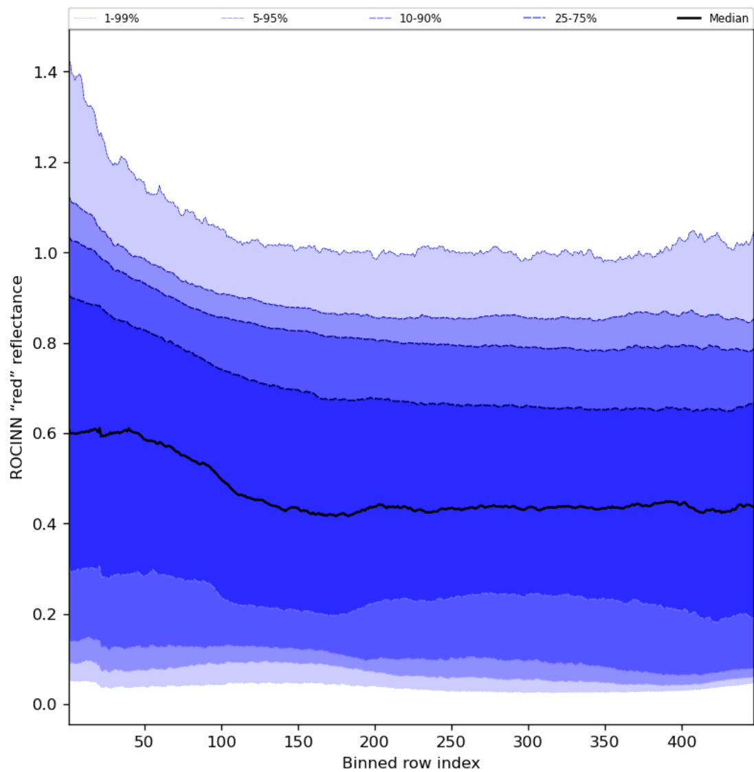
Figure 69: Along track statistics of "ROCINN "red" reflectance" for 2023-10-10 to 2023-10-12
