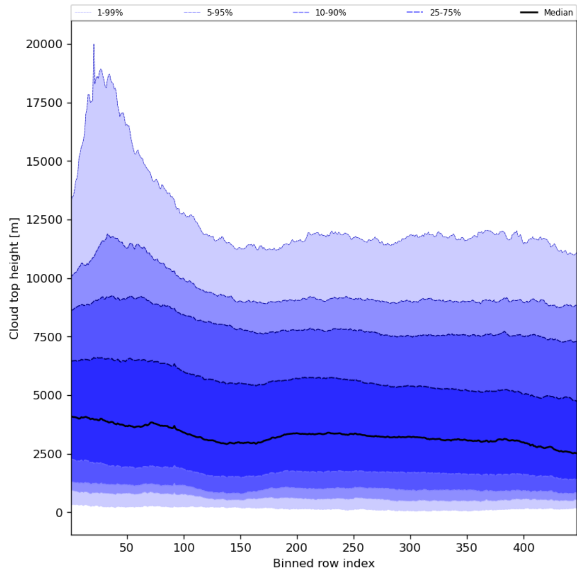
Figure 56: Along track statistics of “Cloud top height” for 2023-10-10 to 2023-10-12
