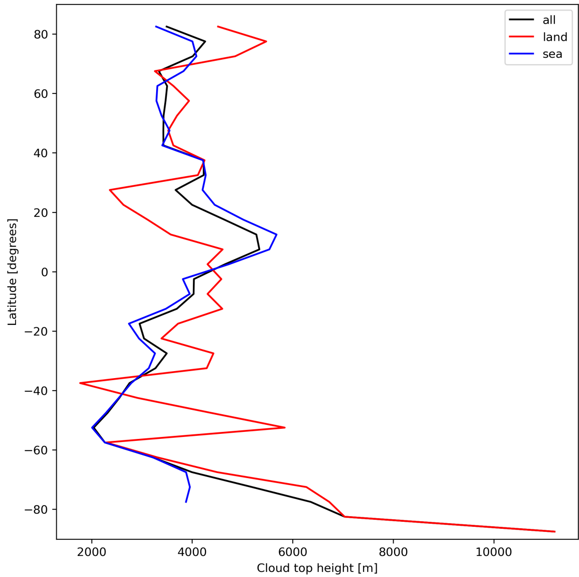
Figure 24: Zonal average of “Cloud top height” for 2023-10-10 to 2023-10-12.
