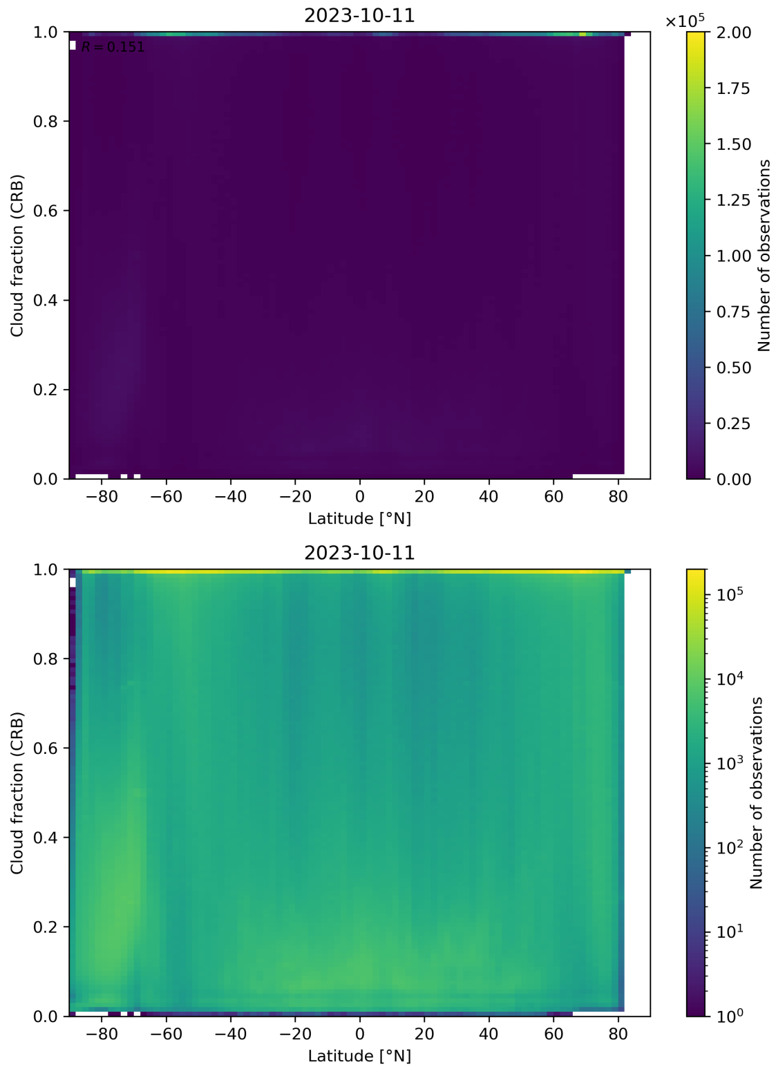
Figure 94: Scatter density plot of “Latitude” against “Cloud fraction (CRB)” for 2023-10-10 to 2023-10-12.
