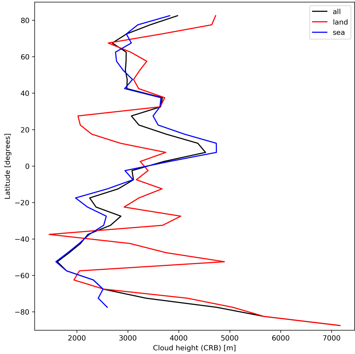
Figure 27: Zonal average of “Cloud height (CRB)” for 2023-10-10 to 2023-10-12.
