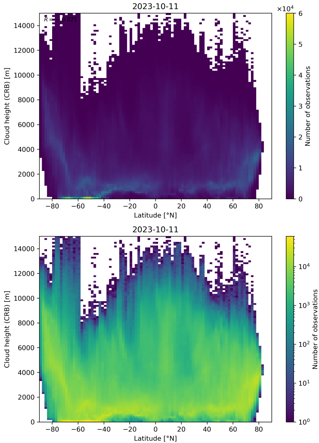
Figure 95: Scatter density plot of “Latitude” against “Cloud height (CRB)” for 2023-10-10 to 2023-10-12.
