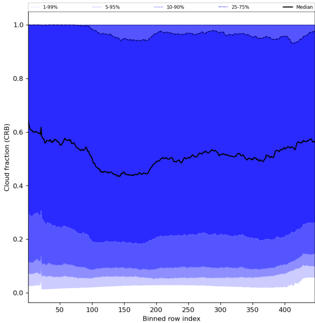
Figure 58: Along track statistics of “Cloud fraction (CRB)” for 2023-10-10 to 2023-10-12
