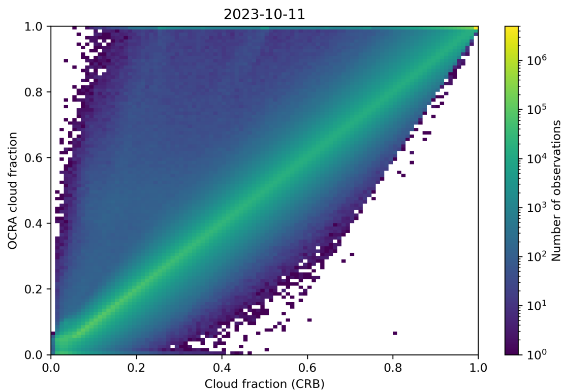
Figure 78: Scatter density plot of “Cloud fraction (CRB)” against “OCRA cloud fraction” for 2023-10-10 to 2023-10-12.
