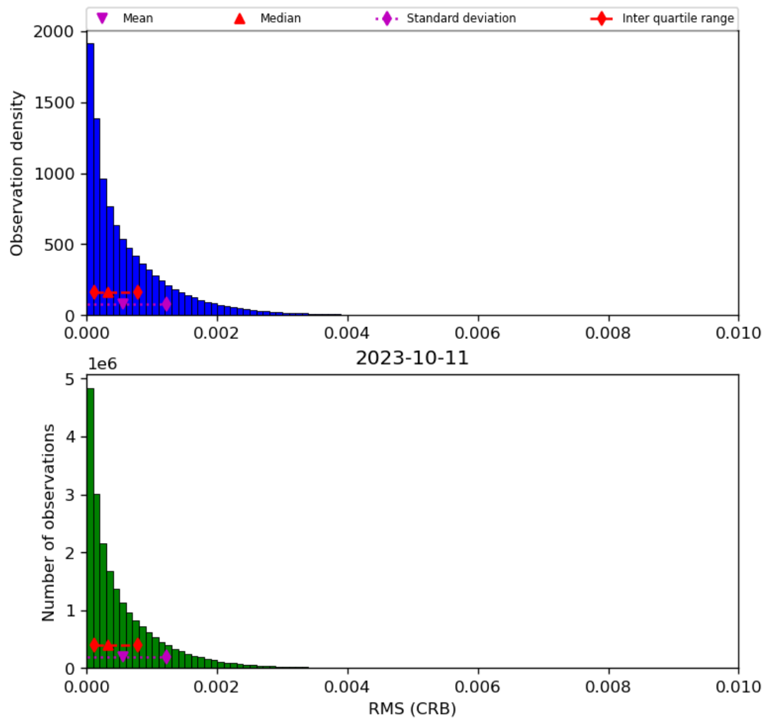
Figure 48: Histogram of “RMS (CRB)” for 2023-10-10 to 2023-10-12
