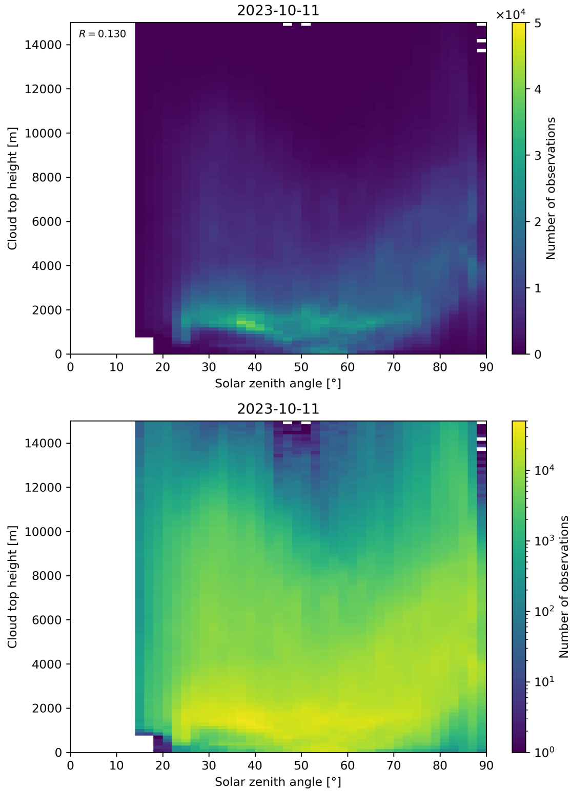
Figure 104: Scatter density plot of “Solar zenith angle” against “Cloud top height” for 2023-10-10 to 2023-10-12.
