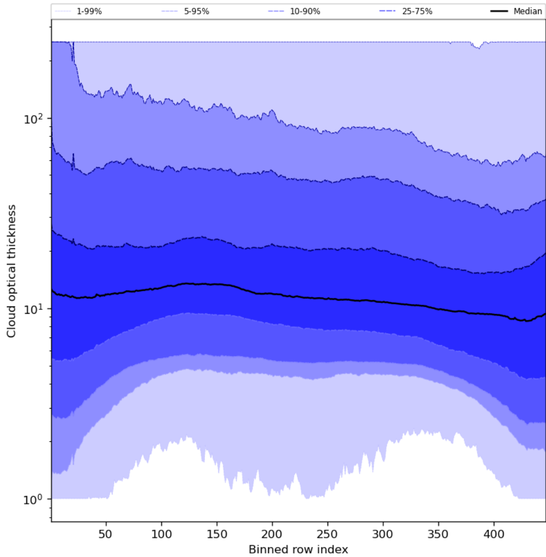
Figure 57: Along track statistics of “Cloud optical thickness” for 2023-10-10 to 2023-10-12
