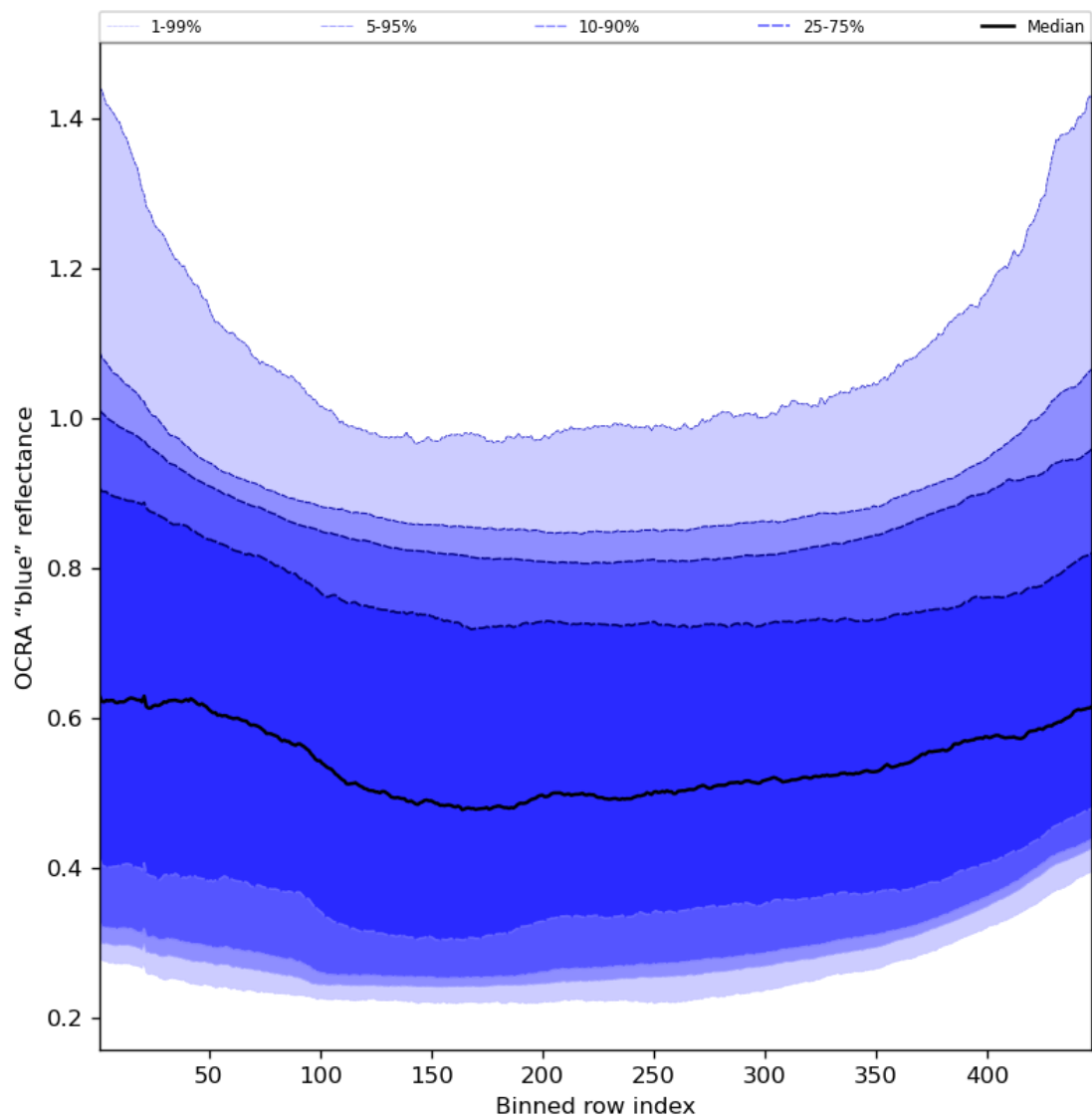
Figure 67: Along track statistics of “OCRA “blue” reflectance” for 2023-10-10 to 2023-10-12
