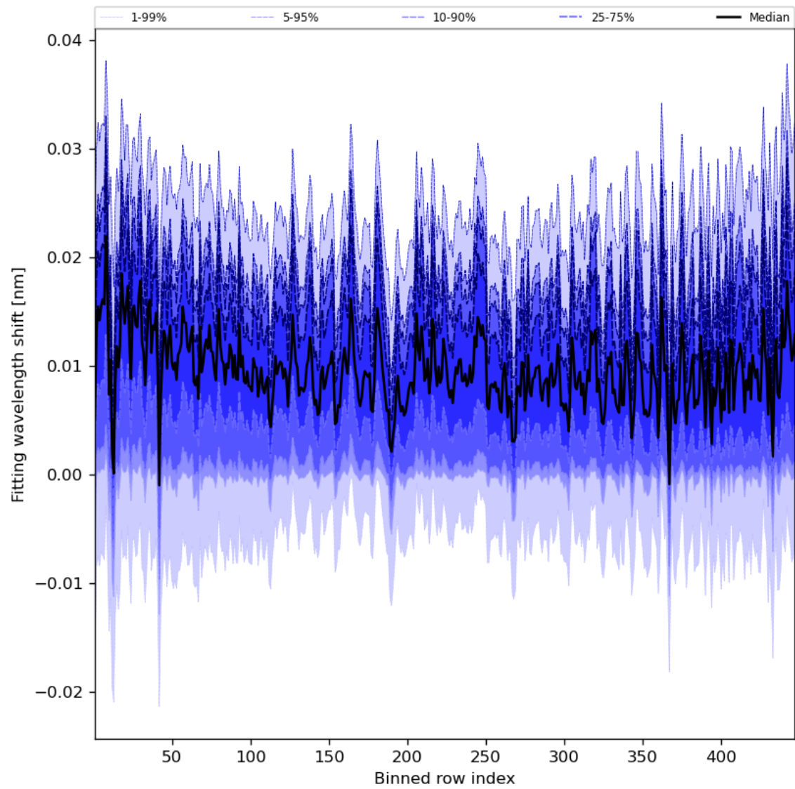
Figure 65: Along track statistics of “Fitting wavelength shift” for 2023-10-10 to 2023-10-12
