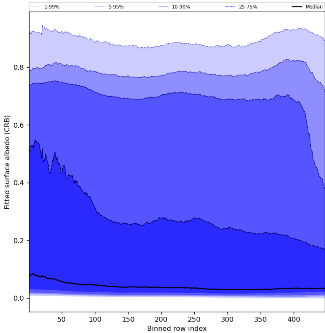
Figure 62: Along track statistics of “Fitted surface albedo (CRB)” for 2023-10-10 to 2023-10-12
