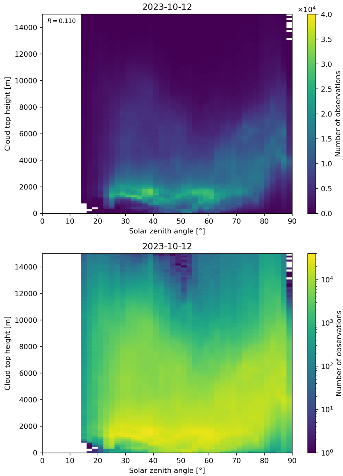
Figure 104: Scatter density plot of “Solar zenith angle” against “Cloud top height” for 2023-10-12 to 2023-10-13.
