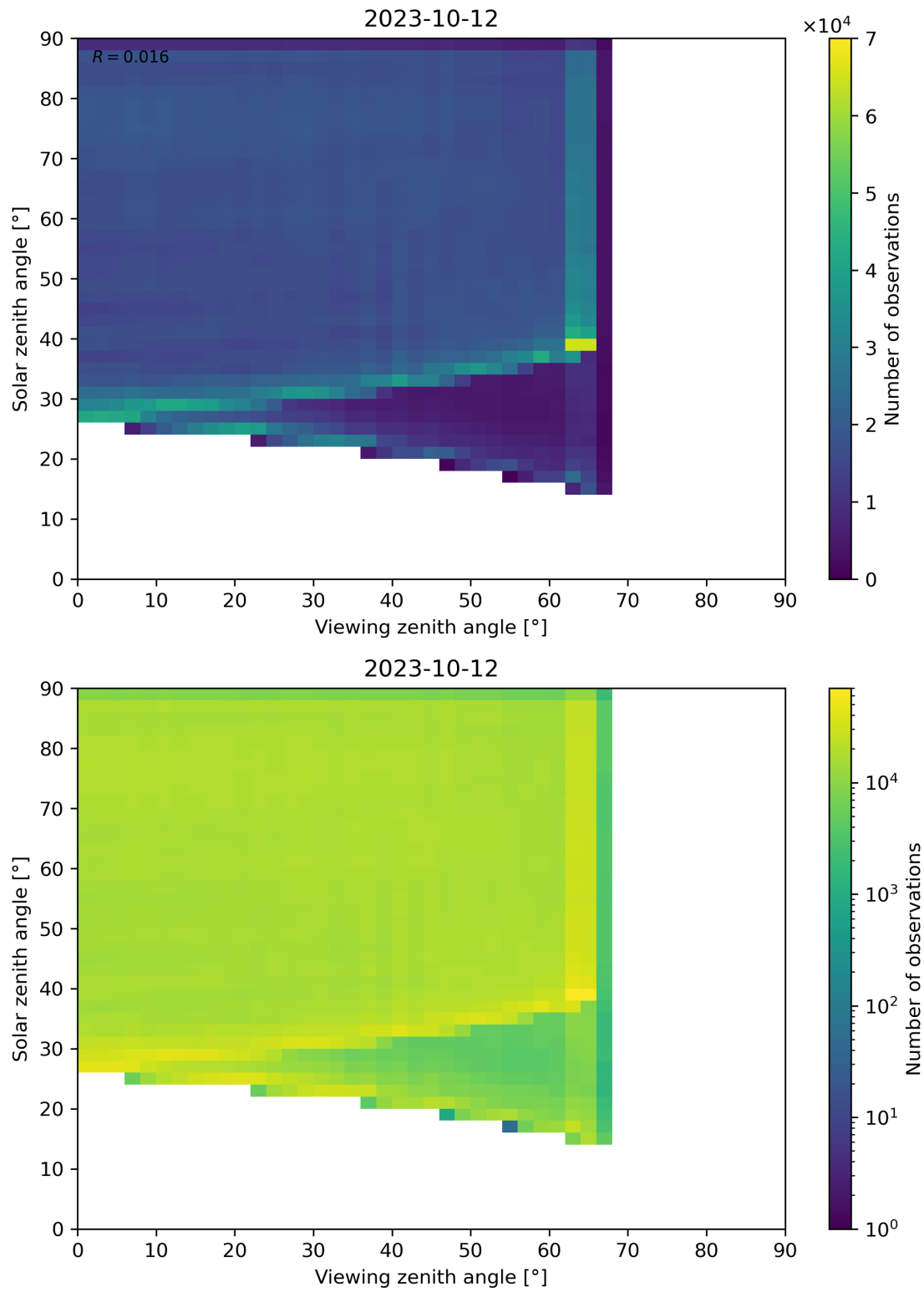
Figure 114: Scatter density plot of “Viewing zenith angle” against “Solar zenith angle” for 2023-10-12 to 2023-10-13.
