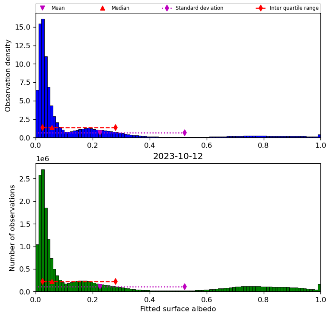
Figure 45: Histogram of “Fitted surface albedo” for 2023-10-12 to 2023-10-13
