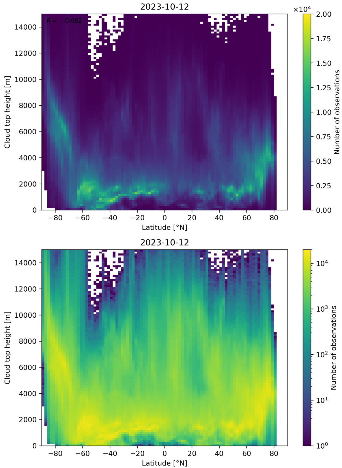
Figure 97: Scatter density plot of “Latitude” against “Cloud top height” for 2023-10-12 to 2023-10-13.
