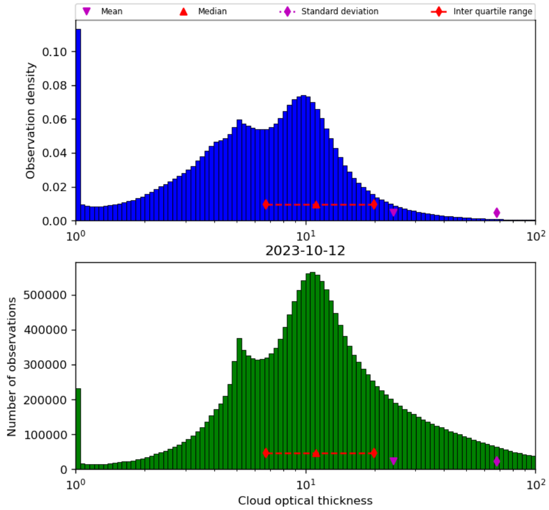
Figure 41: Histogram of “Cloud optical thickness” for 2023-10-12 to 2023-10-13
