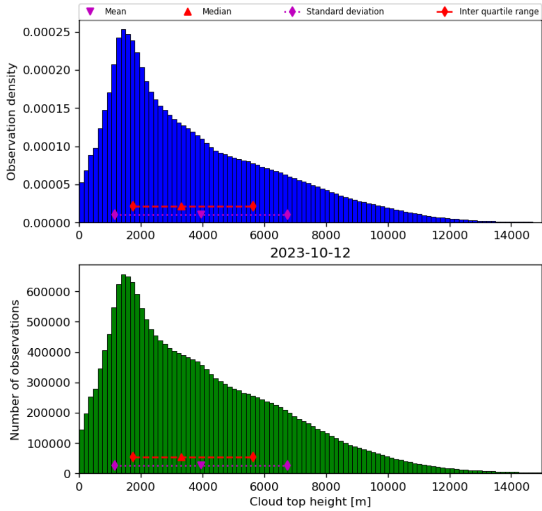
Figure 40: Histogram of “Cloud top height” for 2023-10-12 to 2023-10-13
