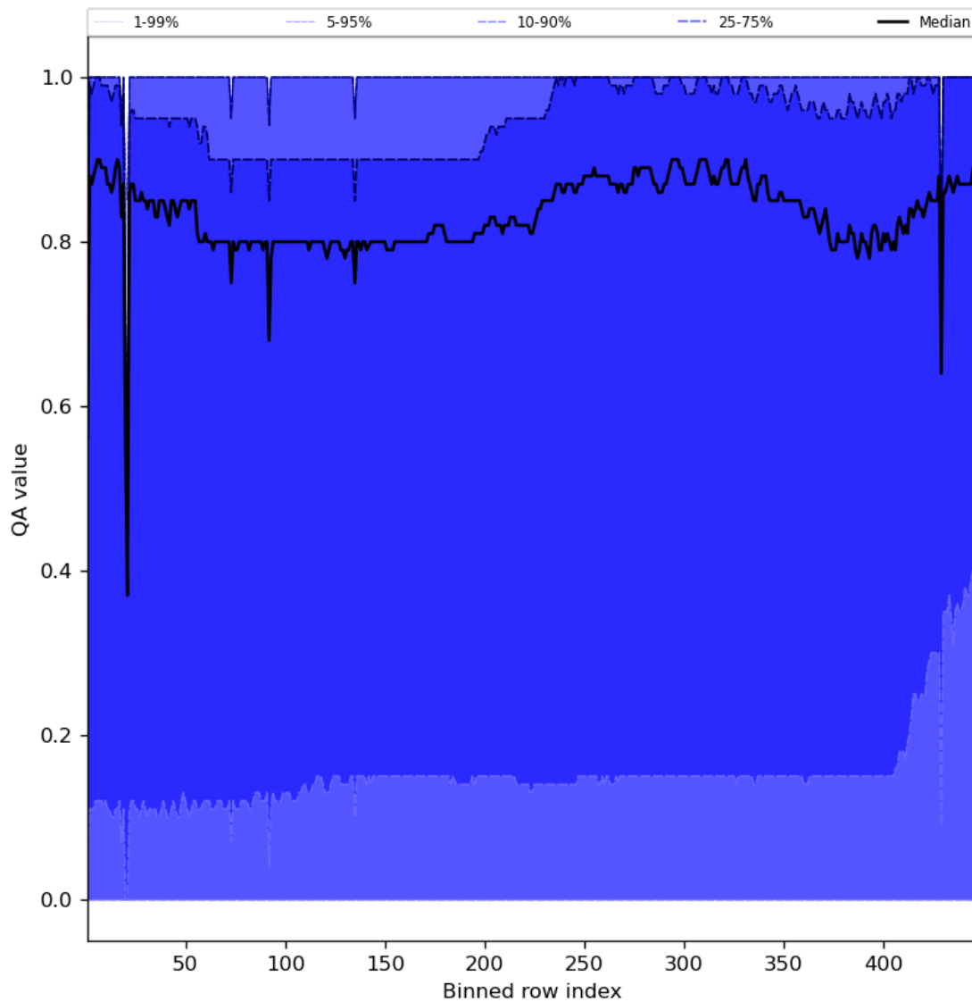
Figure 54: Along track statistics of “QA value” for 2023-10-12 to 2023-10-13
