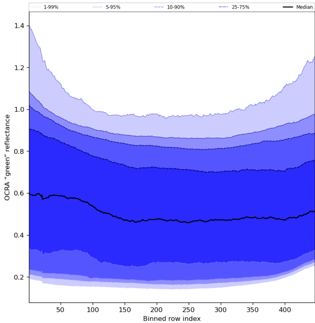
Figure 68: Along track statistics of “OCRA “green” reflectance” for 2023-10-12 to 2023-10-13
