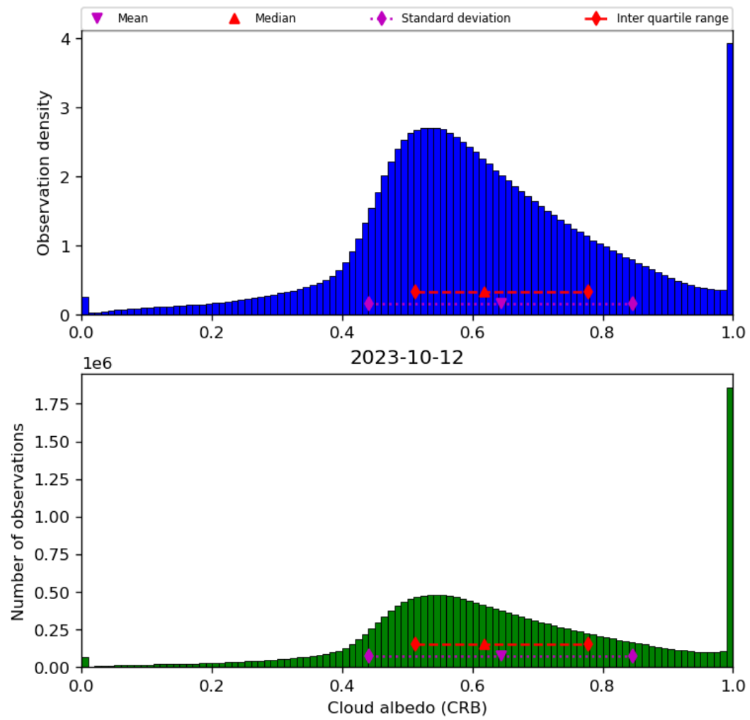
Figure 44: Histogram of “Cloud albedo (CRB)” for 2023-10-12 to 2023-10-13
