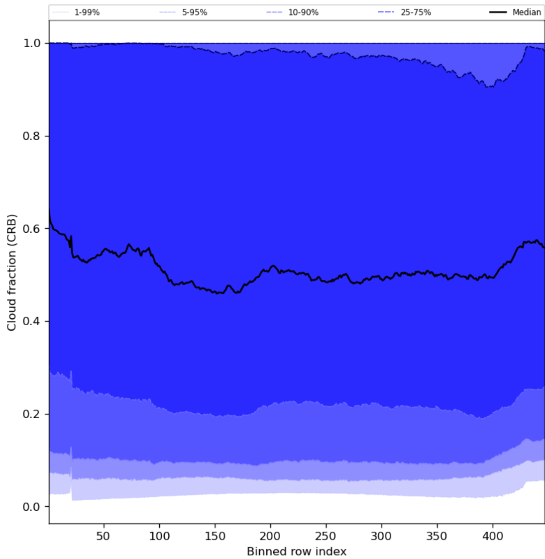
Figure 58: Along track statistics of “Cloud fraction (CRB)” for 2023-10-12 to 2023-10-13
