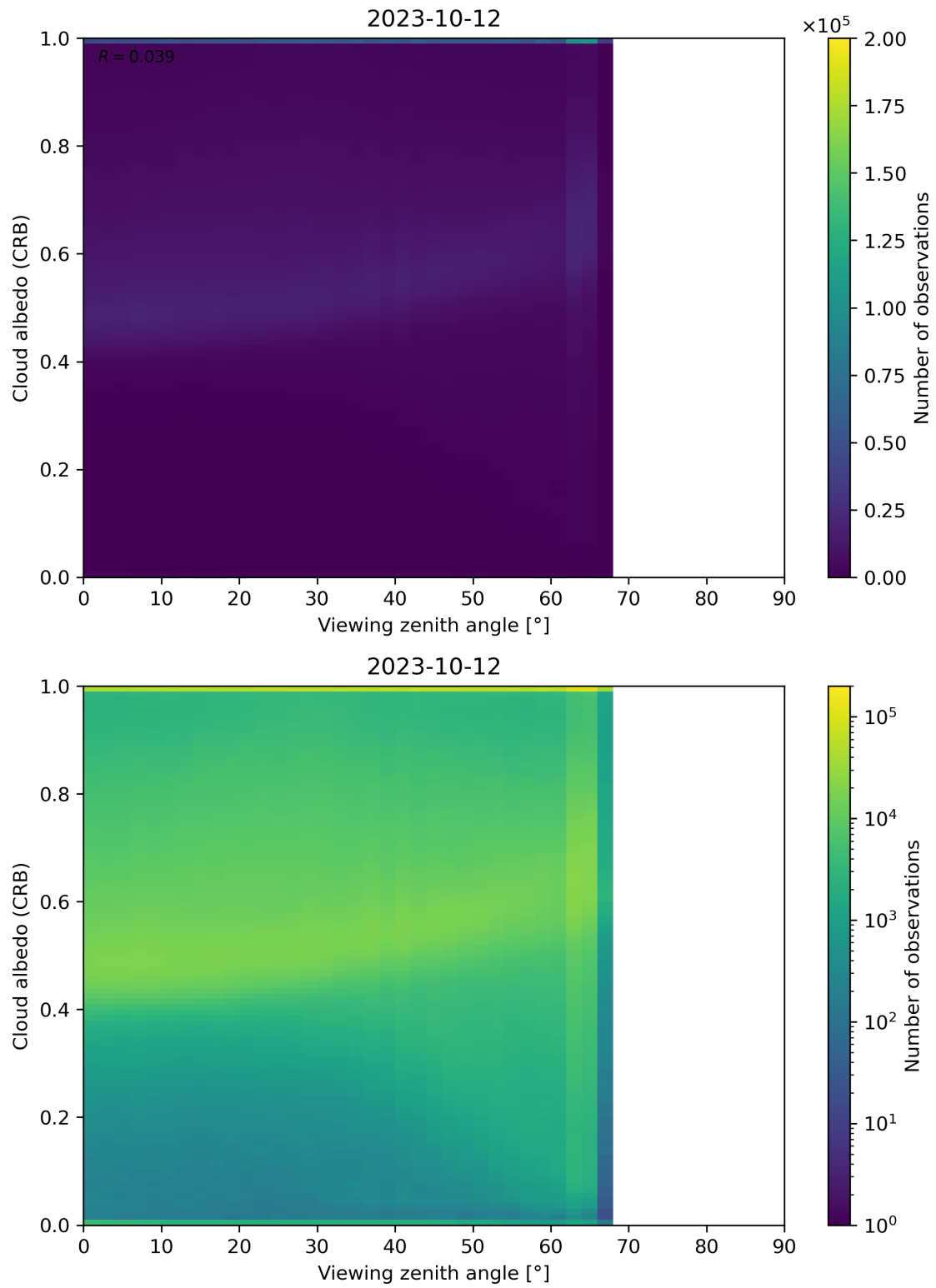
Figure 106: Scatter density plot of “Viewing zenith angle” against “Cloud albedo (CRB)” for 2023-10-12 to 2023-10-13.
