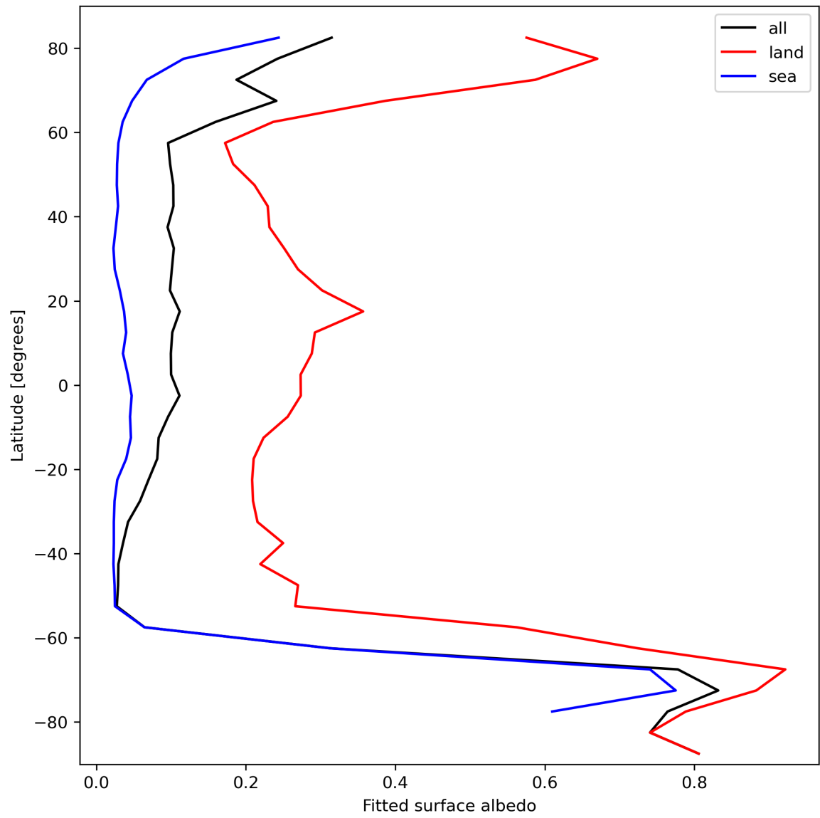
Figure 29: Zonal average of “Fitted surface albedo” for 2023-10-12 to 2023-10-13.
