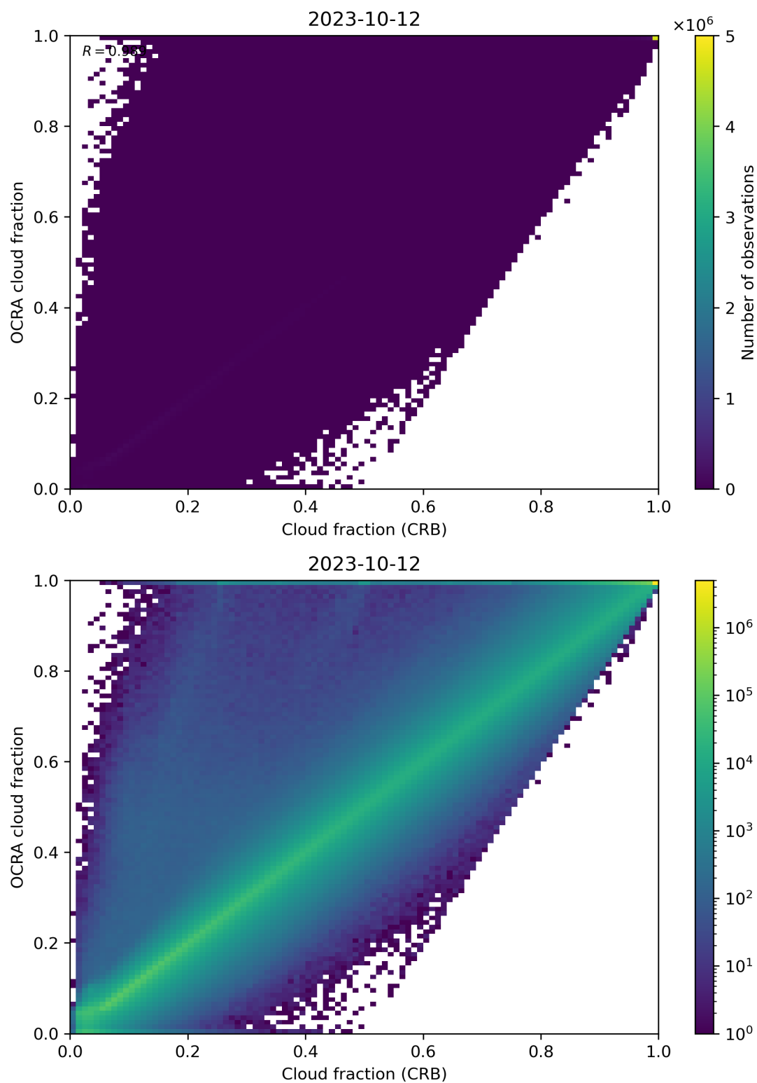
Figure 78: Scatter density plot of “Cloud fraction (CRB)” against “OCRA cloud fraction” for 2023-10-12 to 2023-10-13.
