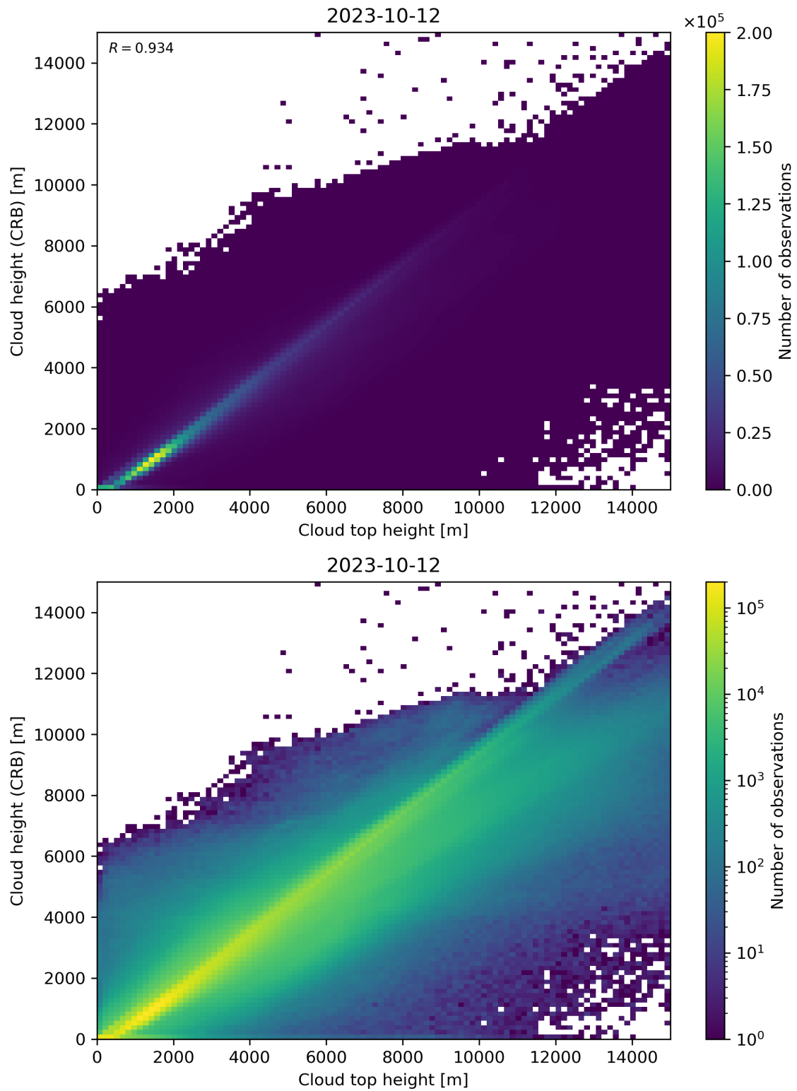
Figure 89: Scatter density plot of “Cloud top height” against “Cloud height (CRB)” for 2023-10-12 to 2023-10-13.
