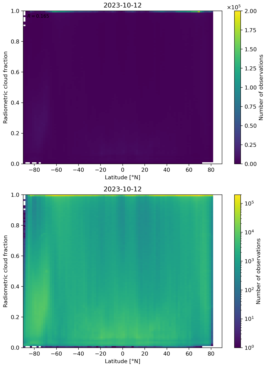
Figure 92: Scatter density plot of “Latitude” against “Radiometric cloud fraction” for 2023-10-12 to 2023-10-13.
