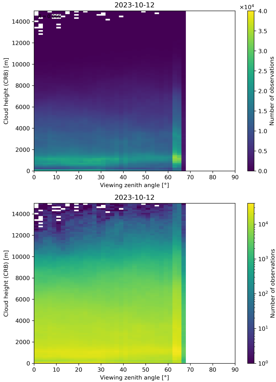
Figure 110: Scatter density plot of “Viewing zenith angle” against “Cloud height (CRB)” for 2023-10-12 to 2023-10-13.
