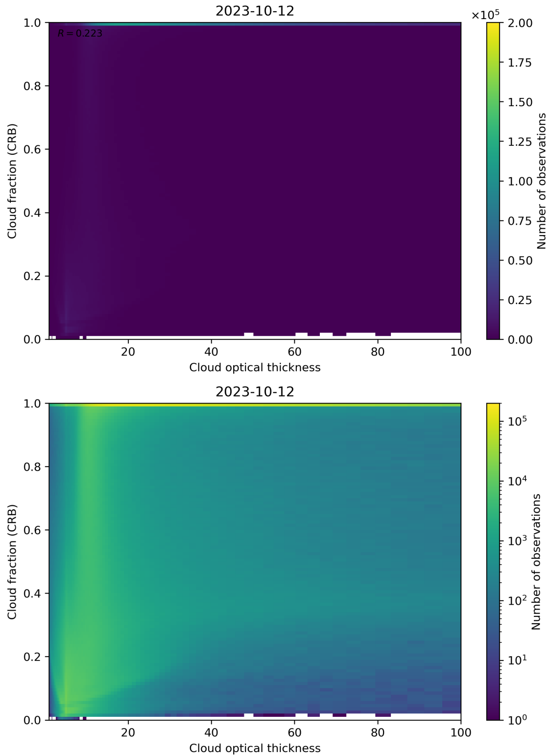
Figure 84: Scatter density plot of “Cloud optical thickness” against “Cloud fraction (CRB)” for 2023-10-12 to 2023-10-13.
