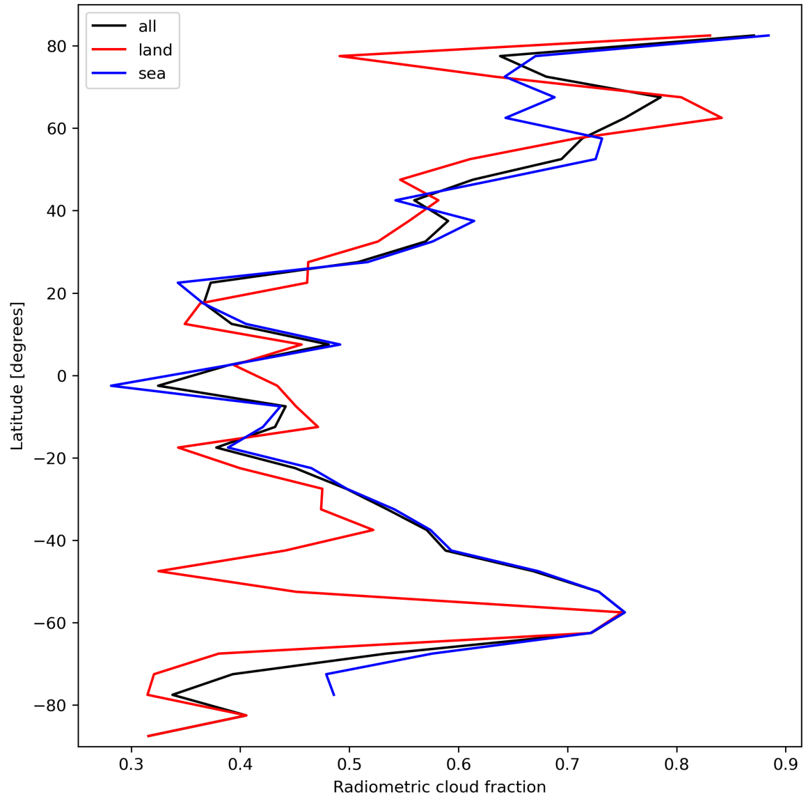
Figure 23: Zonal average of “Radiometric cloud fraction” for 2023-10-12 to 2023-10-13.
