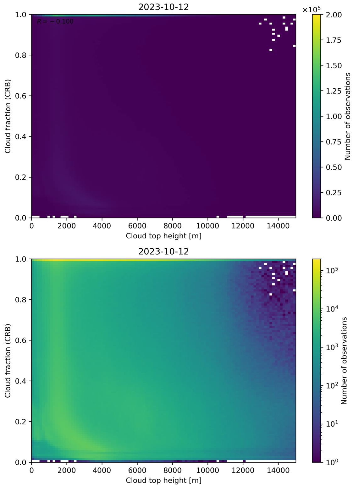
Figure 88: Scatter density plot of “Cloud top height” against “Cloud fraction (CRB)” for 2023-10-12 to 2023-10-13.
