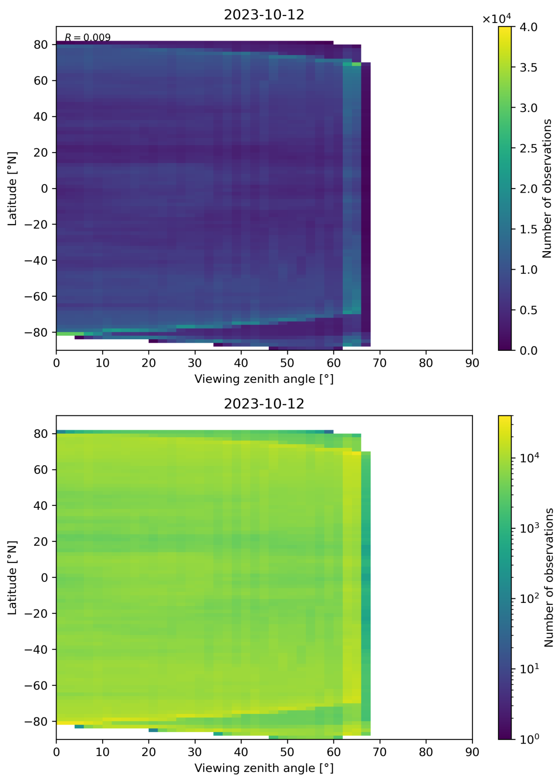
Figure 113: Scatter density plot of “Viewing zenith angle” against “Latitude” for 2023-10-12 to 2023-10-13.
