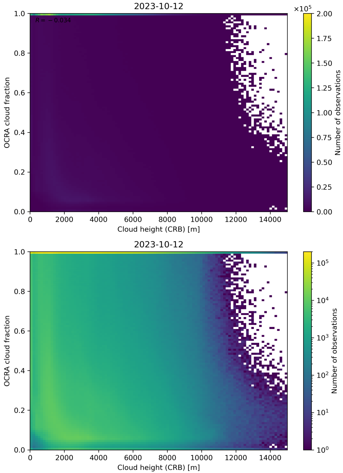
Figure 81: Scatter density plot of “Cloud height (CRB)” against “OCRA cloud fraction” for 2023-10-12 to 2023-10-13.
