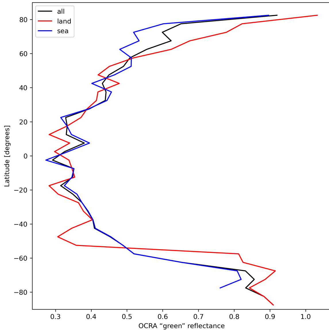
Figure 36: Zonal average of “OCRA “green” reflectance” for 2023-10-12 to 2023-10-13.
