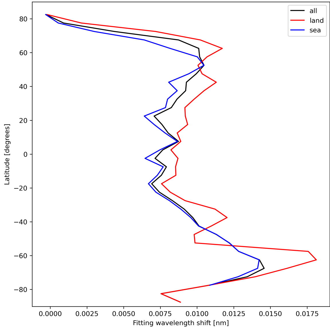
Figure 33: Zonal average of “Fitting wavelength shift” for 2023-10-12 to 2023-10-13.
