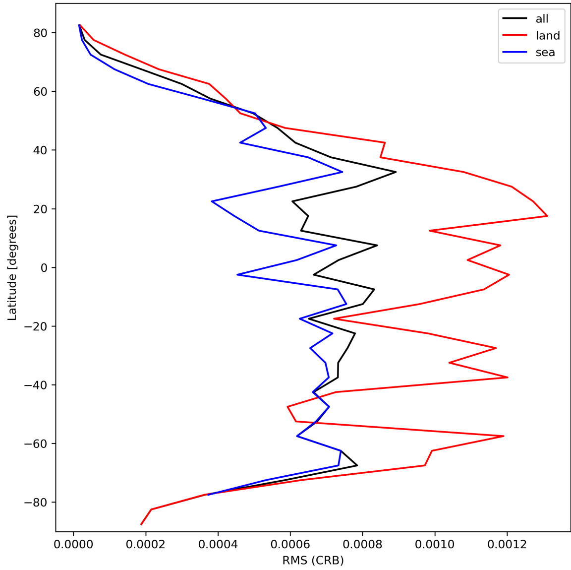
Figure 32: Zonal average of “RMS (CRB)” for 2023-10-12 to 2023-10-13.
