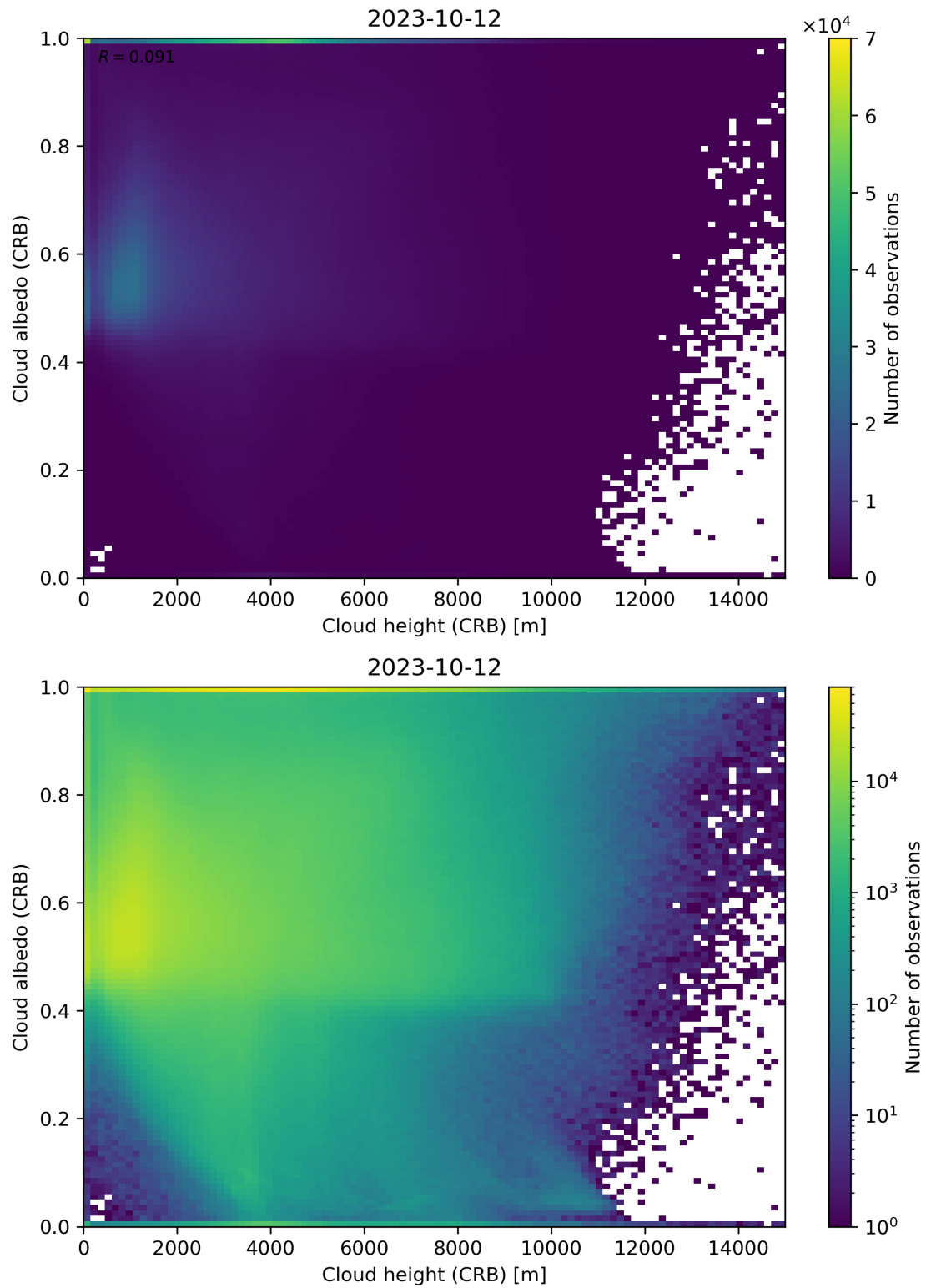
Figure 80: Scatter density plot of “Cloud height (CRB)” against “Cloud albedo (CRB)” for 2023-10-12 to 2023-10-13.
