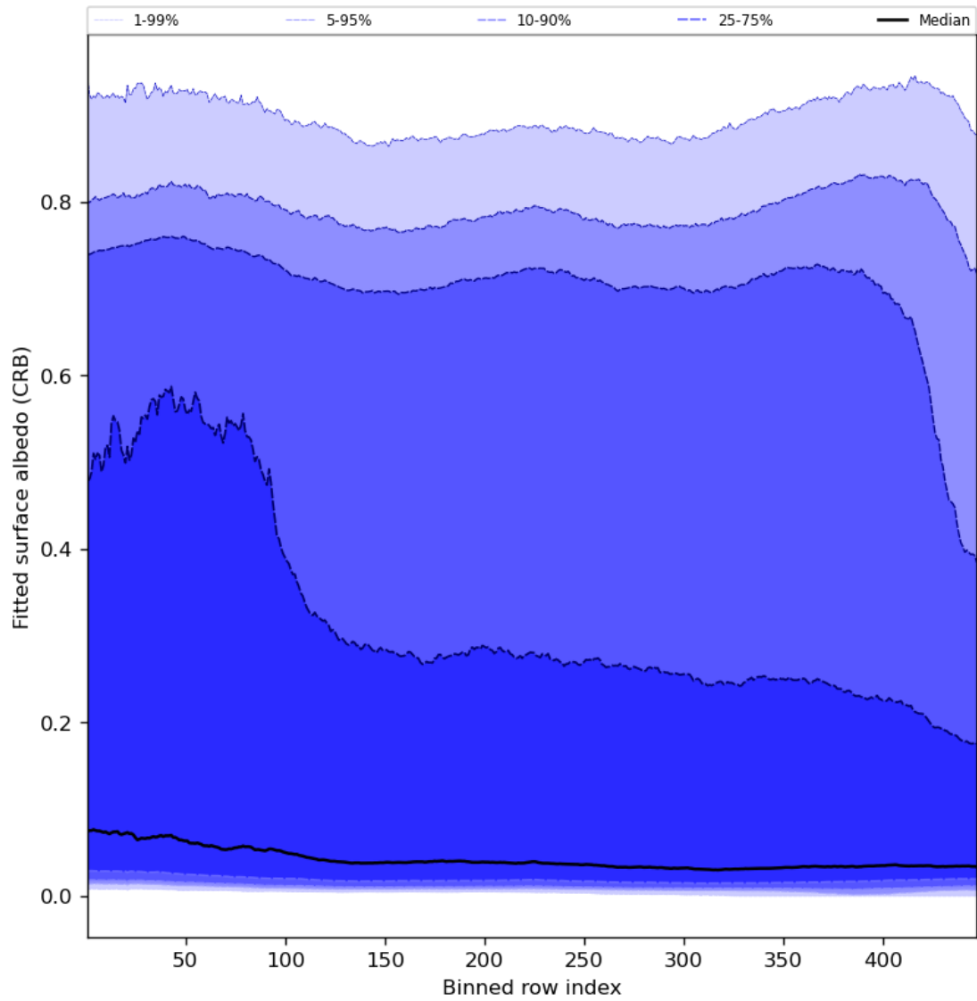
Figure 62: Along track statistics of “Fitted surface albedo (CRB)” for 2023-10-12 to 2023-10-13
