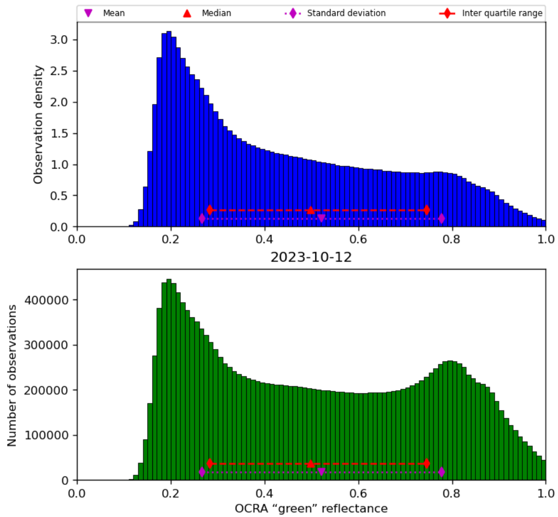
Figure 52: Histogram of “OCRA “green” reflectance” for 2023-10-12 to 2023-10-13
