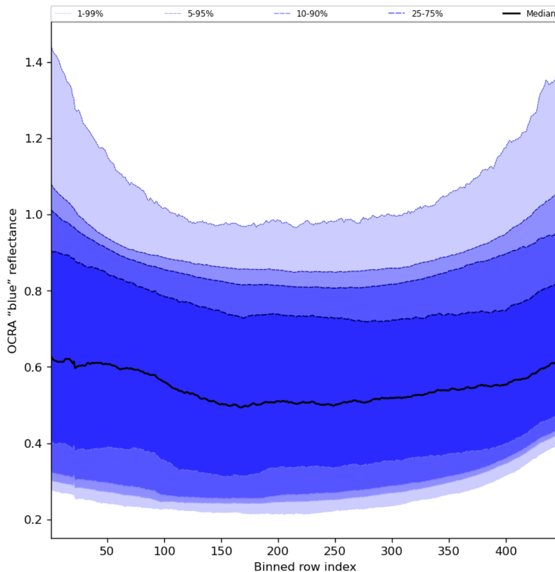
Figure 67: Along track statistics of “OCRA “blue” reflectance” for 2023-10-12 to 2023-10-13
