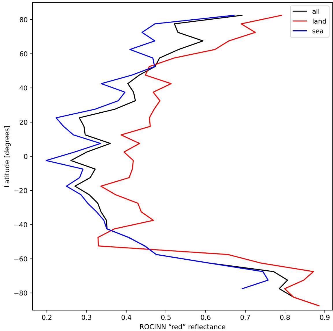
Figure 37: Zonal average of “ROCINN “red” reflectance” for 2023-10-12 to 2023-10-13.
