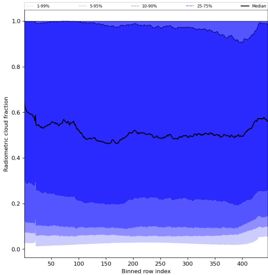
Figure 55: Along track statistics of “Radiometric cloud fraction” for 2023-10-12 to 2023-10-13
