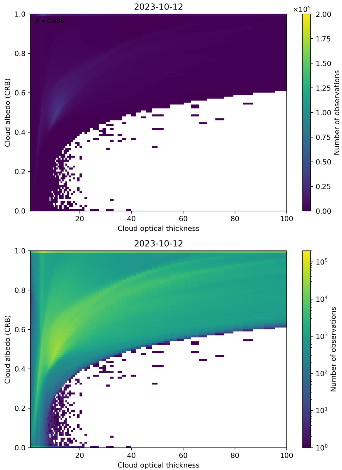
Figure 82: Scatter density plot of “Cloud optical thickness” against “Cloud albedo (CRB)” for 2023-10-12 to 2023-10-13.
