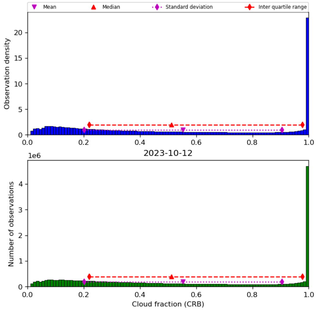
Figure 42: Histogram of “Cloud fraction (CRB)” for 2023-10-12 to 2023-10-13
