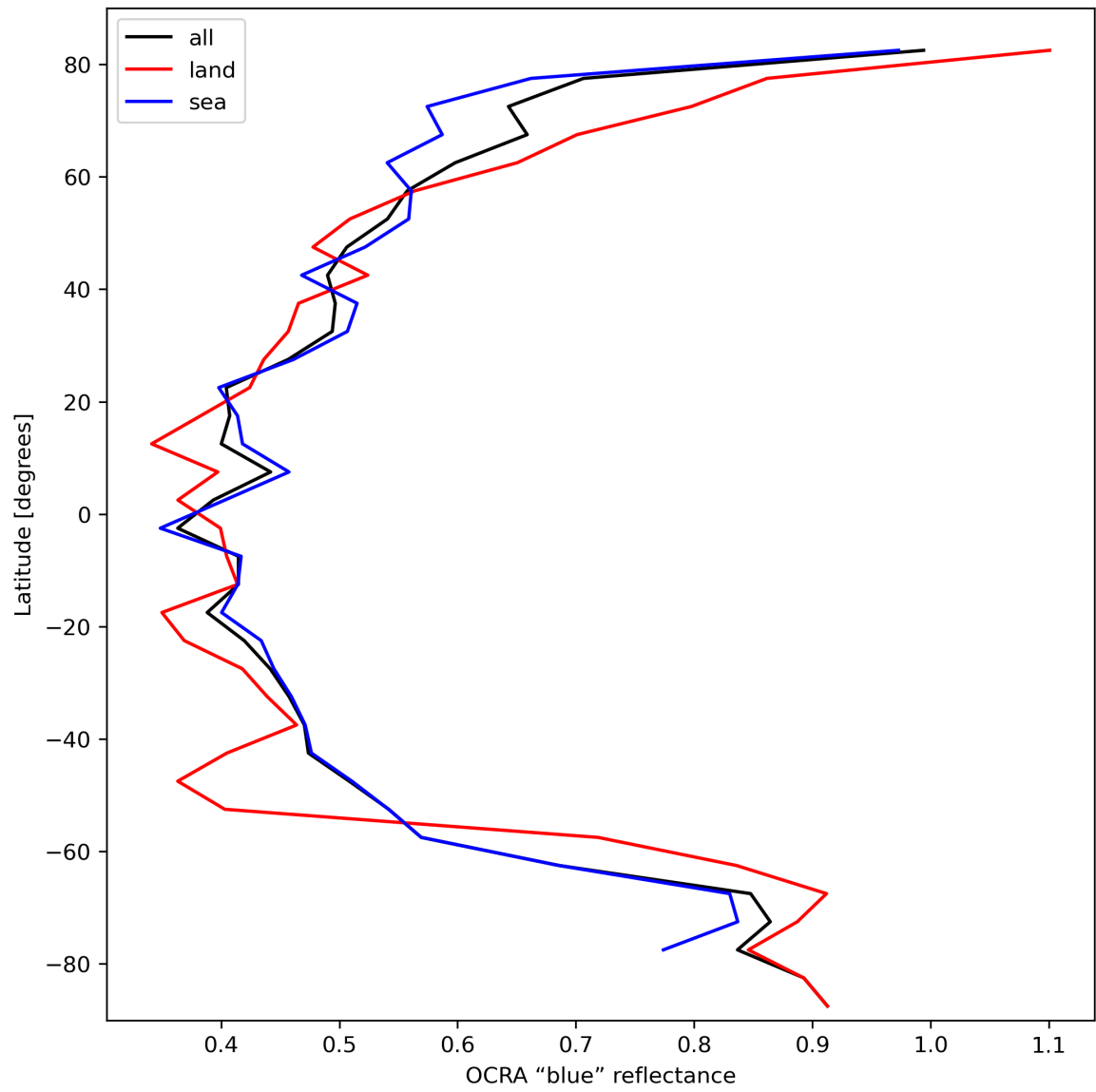
Figure 35: Zonal average of “OCRA “blue” reflectance” for 2023-10-12 to 2023-10-13.
