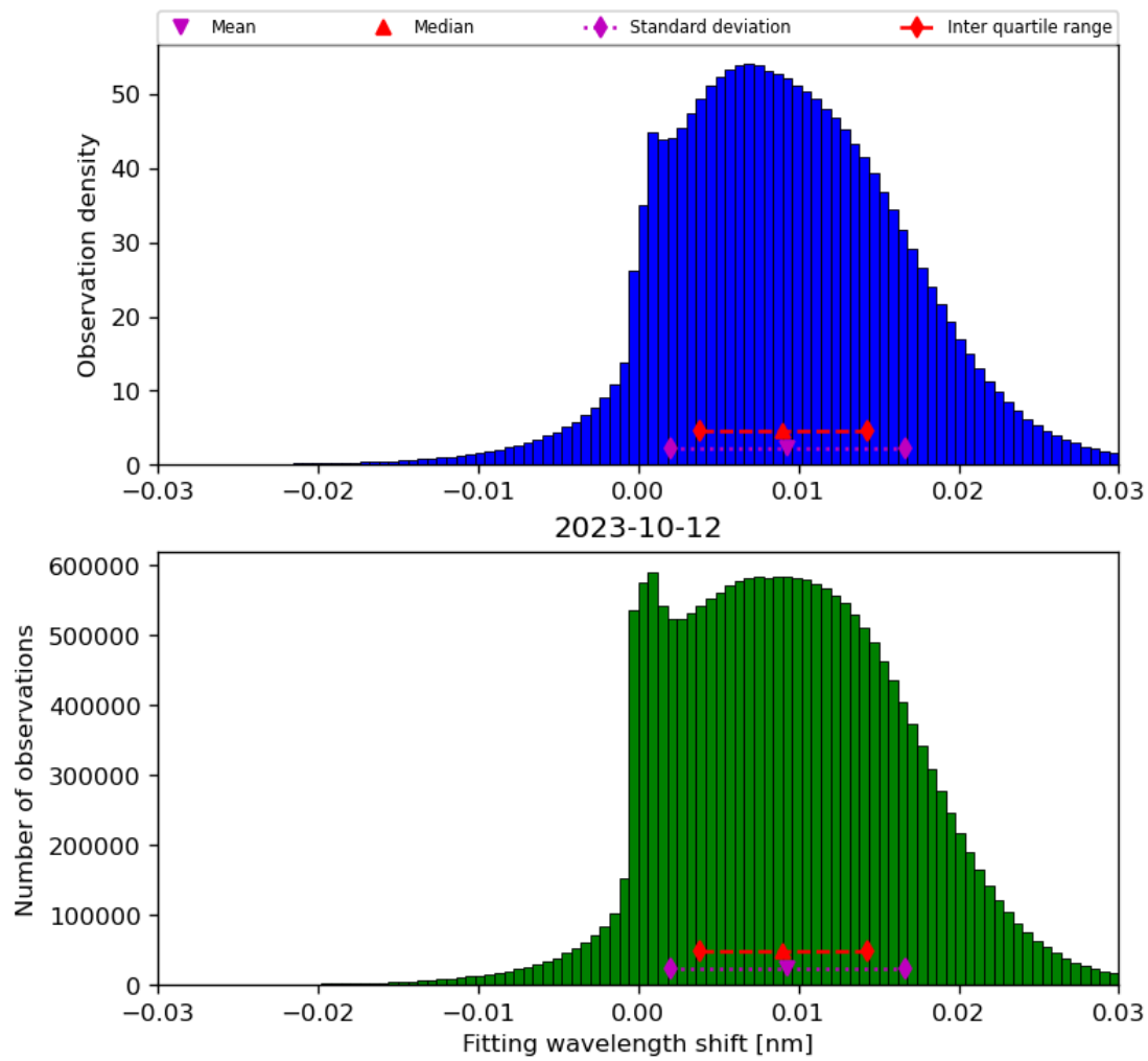
Figure 49: Histogram of “Fitting wavelength shift” for 2023-10-12 to 2023-10-13
