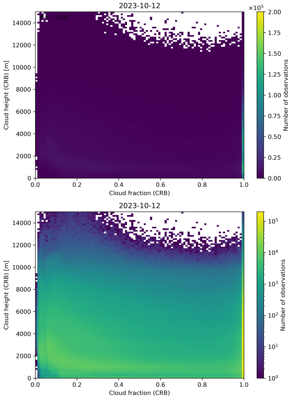
Figure 79: Scatter density plot of “Cloud fraction (CRB)” against “Cloud height (CRB)” for 2023-10-12 to 2023-10-13.
