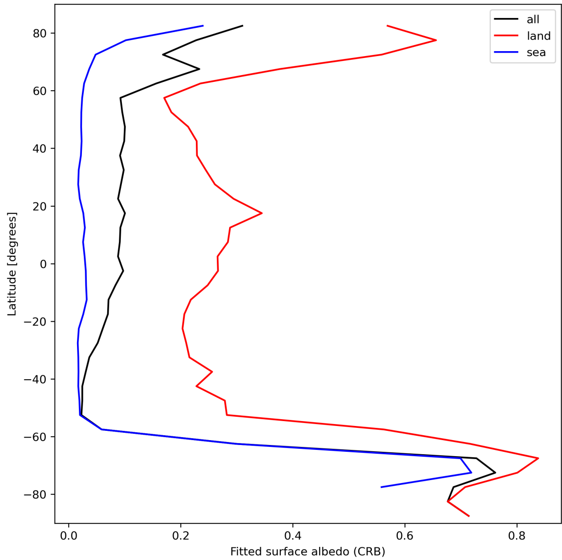
Figure 30: Zonal average of “Fitted surface albedo (CRB)” for 2023-10-12 to 2023-10-13.
