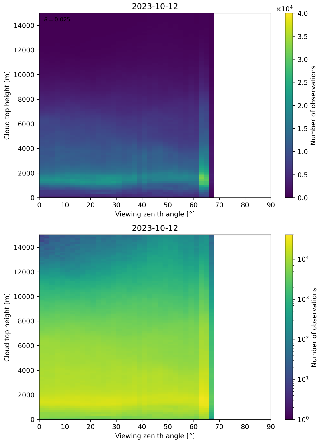
Figure 112: Scatter density plot of “Viewing zenith angle” against “Cloud top height” for 2023-10-12 to 2023-10-13.
