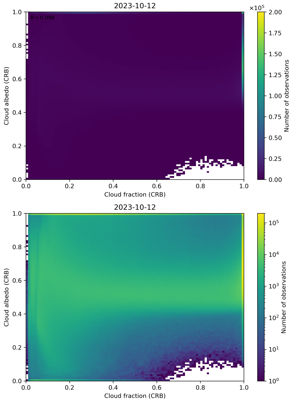
Figure 77: Scatter density plot of “Cloud fraction (CRB)” against “Cloud albedo (CRB)” for 2023-10-12 to 2023-10-13.
