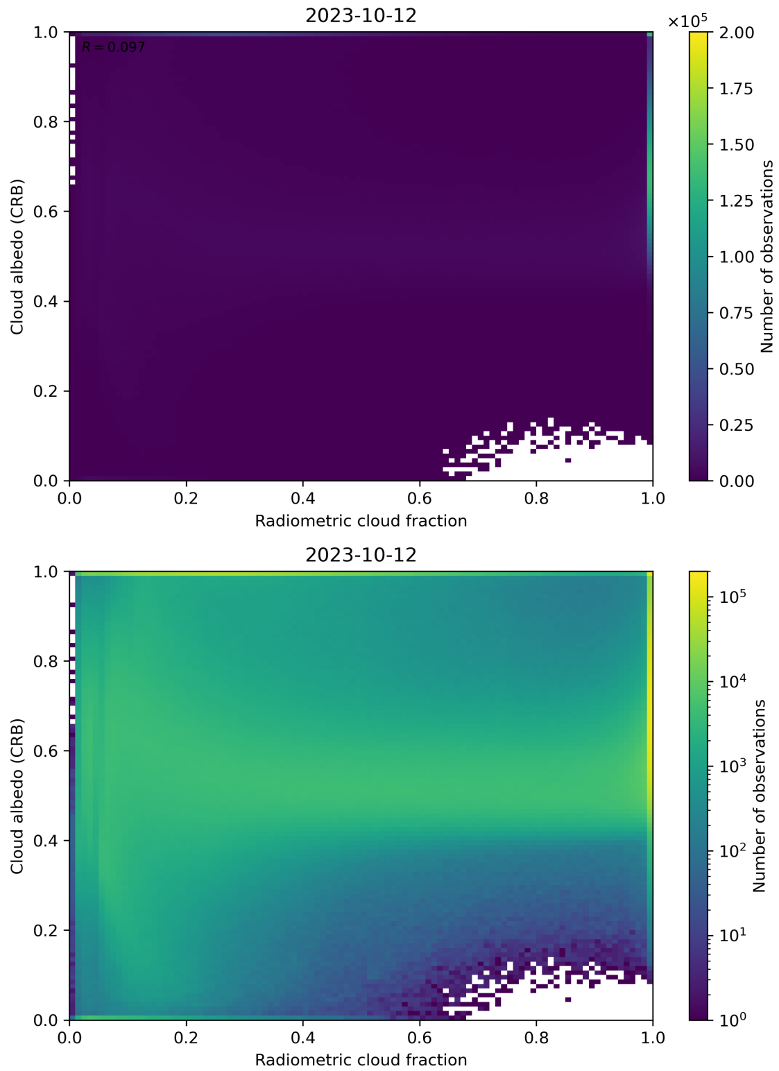
Figure 71: Scatter density plot of “Radiometric cloud fraction” against “Cloud albedo (CRB)” for 2023-10-12 to 2023-10-13.
