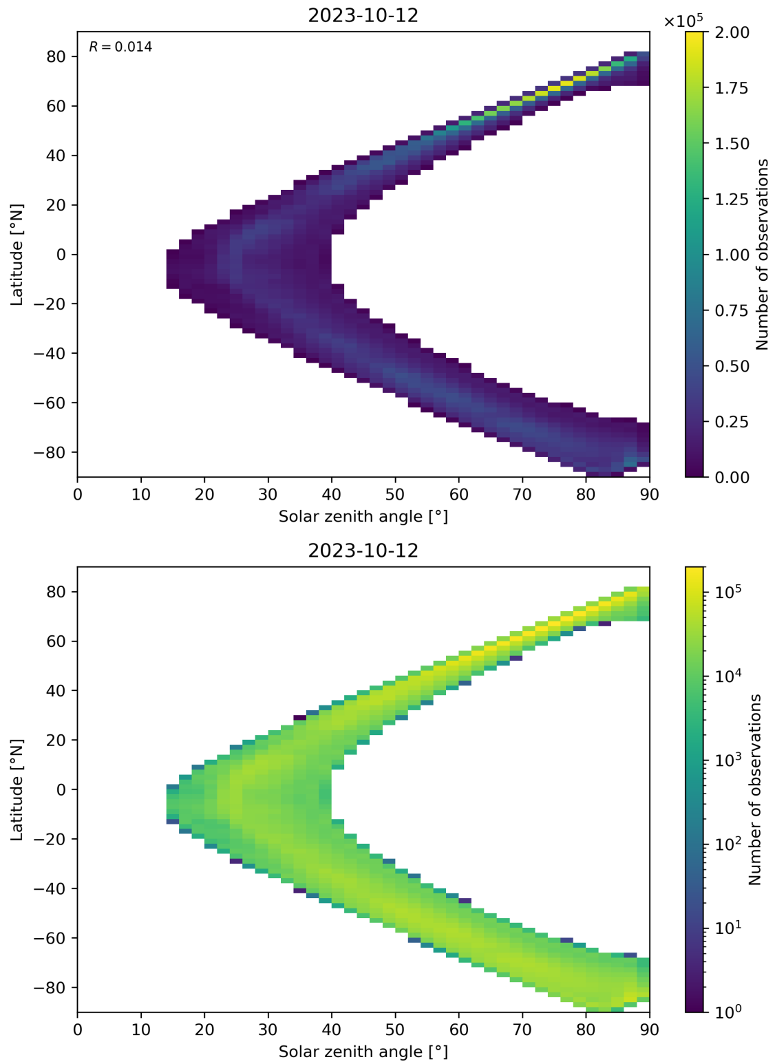
Figure 105: Scatter density plot of “Solar zenith angle” against “Latitude” for 2023-10-12 to 2023-10-13.
