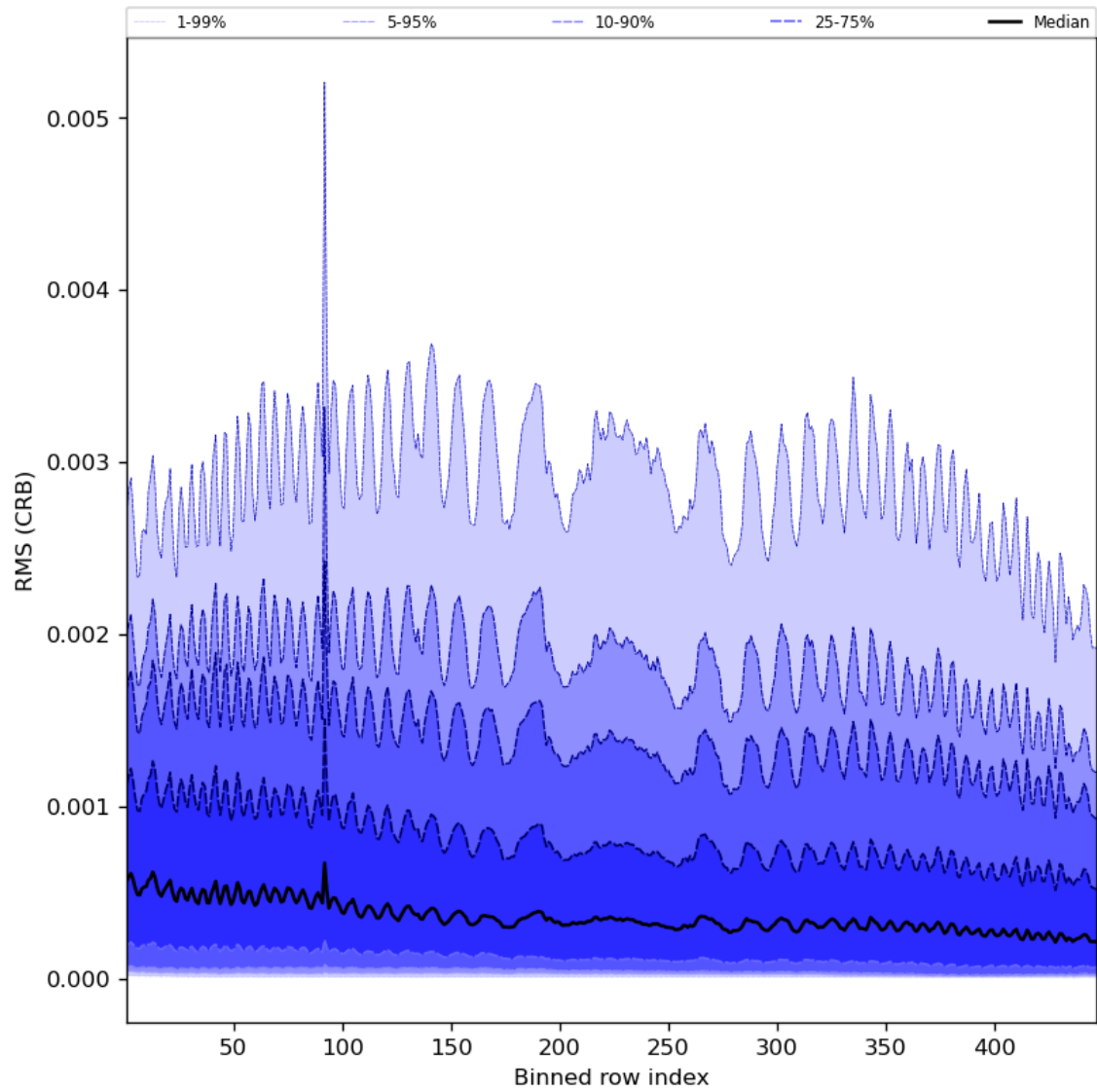
Figure 64: Along track statistics of “RMS (CRB)” for 2023-10-12 to 2023-10-13
