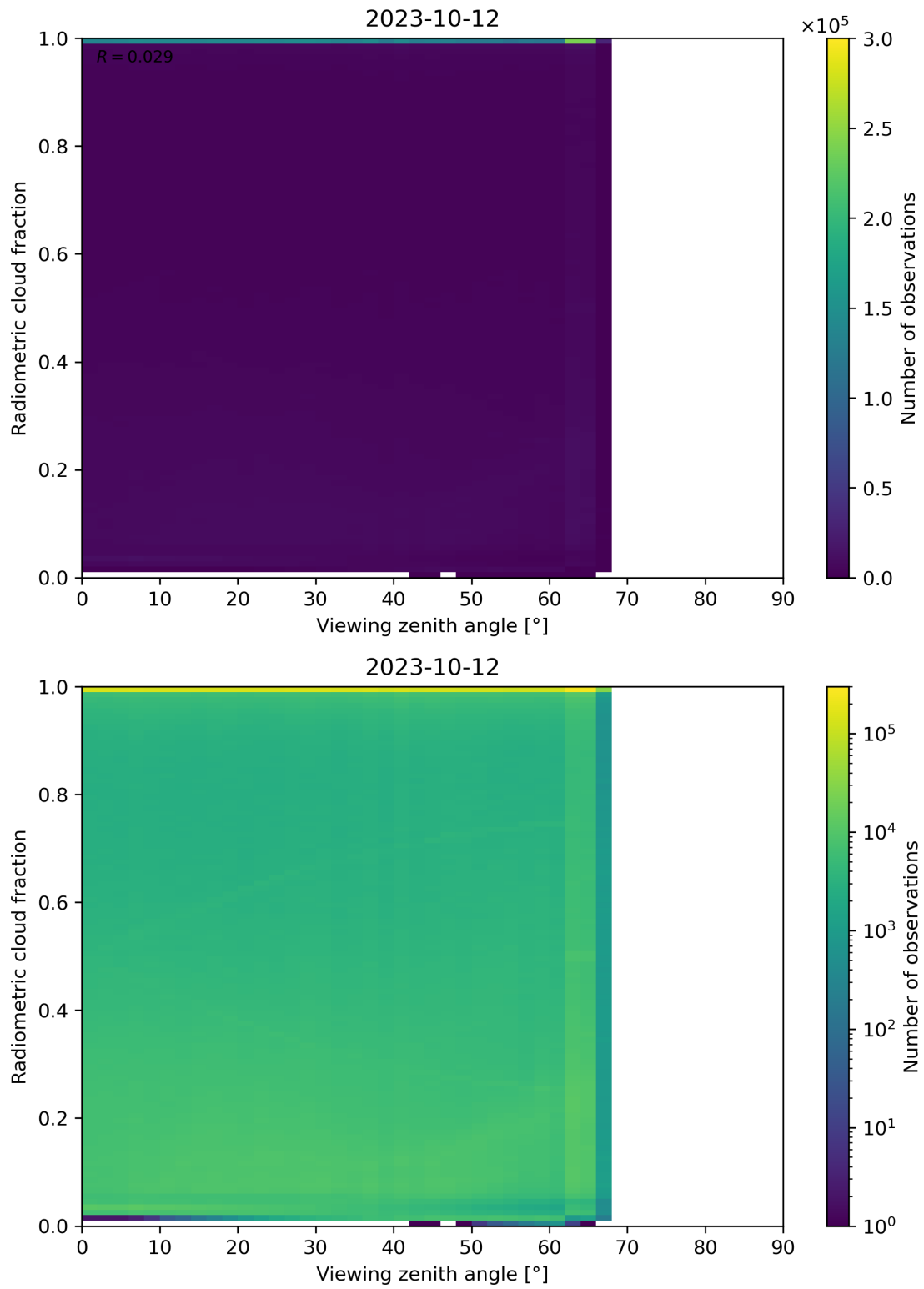
Figure 107: Scatter density plot of “Viewing zenith angle” against “Radiometric cloud fraction” for 2023-10-12 to 2023-10-13.
