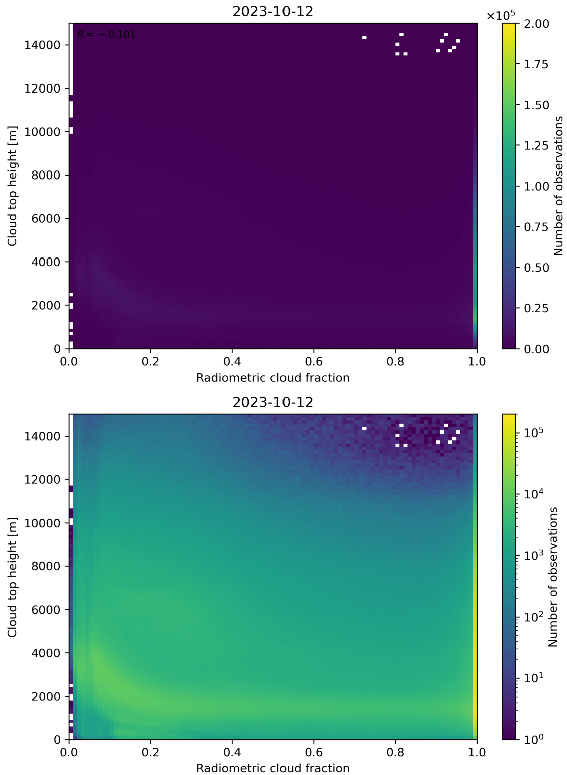
Figure 76: Scatter density plot of “Radiometric cloud fraction” against “Cloud top height” for 2023-10-12 to 2023-10-13.
