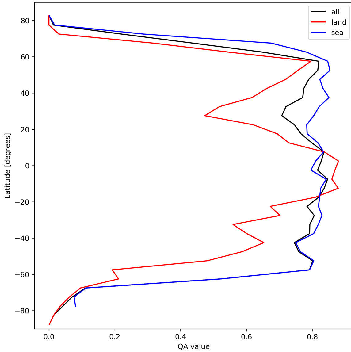
Figure 22: Zonal average of “QA value” for 2023-10-12 to 2023-10-13.
