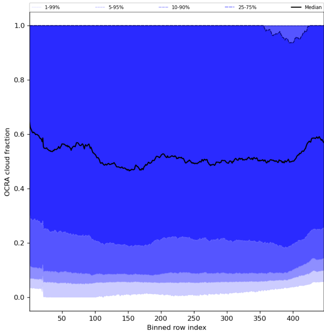
Figure 66: Along track statistics of “OCRA cloud fraction” for 2023-10-12 to 2023-10-13
