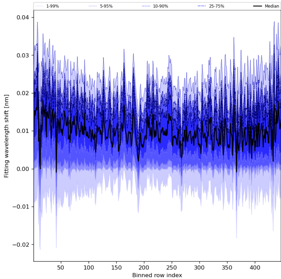
Figure 65: Along track statistics of “Fitting wavelength shift” for 2023-10-12 to 2023-10-13
