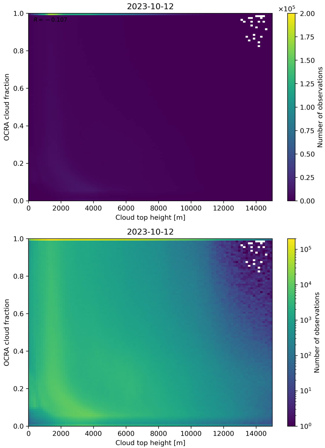
Figure 87: Scatter density plot of “Cloud top height” against “OCRA cloud fraction” for 2023-10-12 to 2023-10-13.
