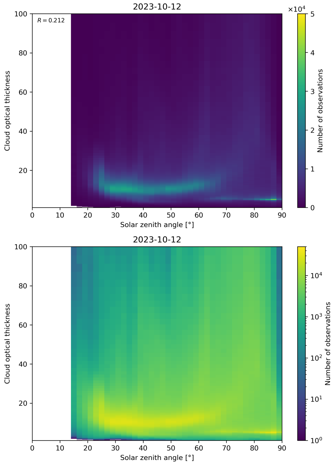
Figure 103: Scatter density plot of “Solar zenith angle” against “Cloud optical thickness” for 2023-10-12 to 2023-10-13.
