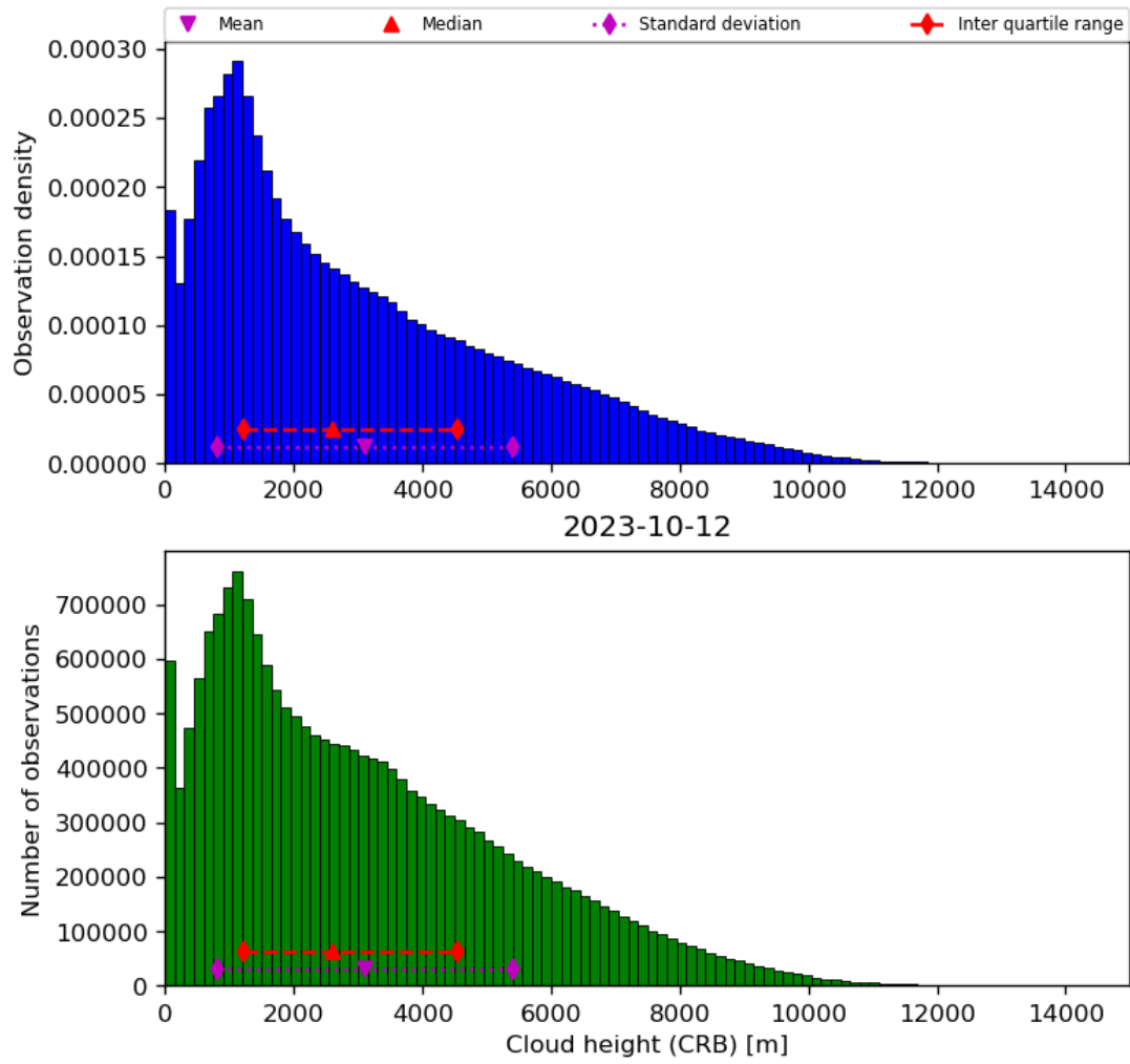
Figure 43: Histogram of “Cloud height (CRB)” for 2023-10-12 to 2023-10-13
