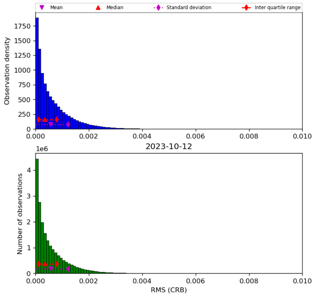
Figure 48: Histogram of “RMS (CRB)” for 2023-10-12 to 2023-10-13
