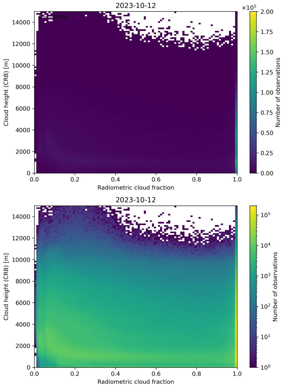
Figure 74: Scatter density plot of “Radiometric cloud fraction” against “Cloud height (CRB)” for 2023-10-12 to 2023-10-13.
