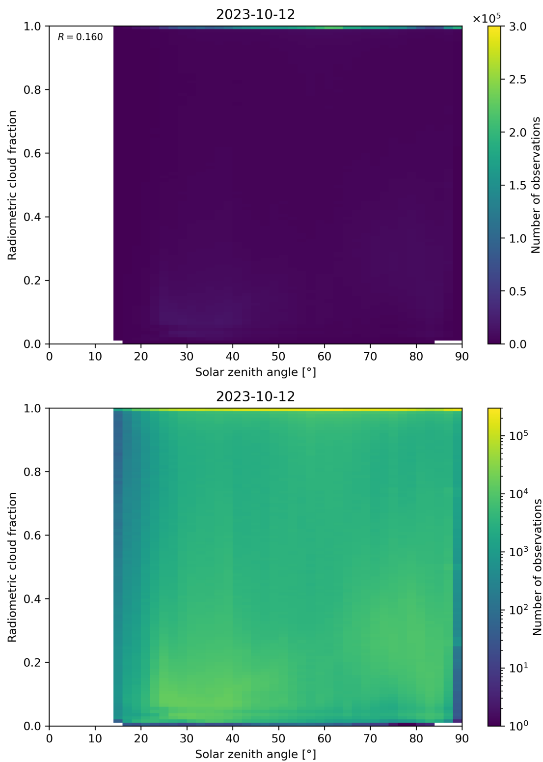
Figure 99: Scatter density plot of “Solar zenith angle” against “Radiometric cloud fraction” for 2023-10-12 to 2023-10-13.
