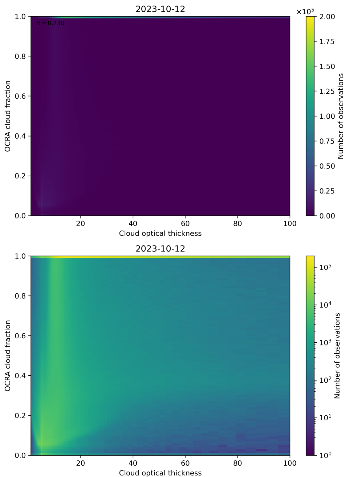
Figure 83: Scatter density plot of “Cloud optical thickness” against “OCRA cloud fraction” for 2023-10-12 to 2023-10-13.
