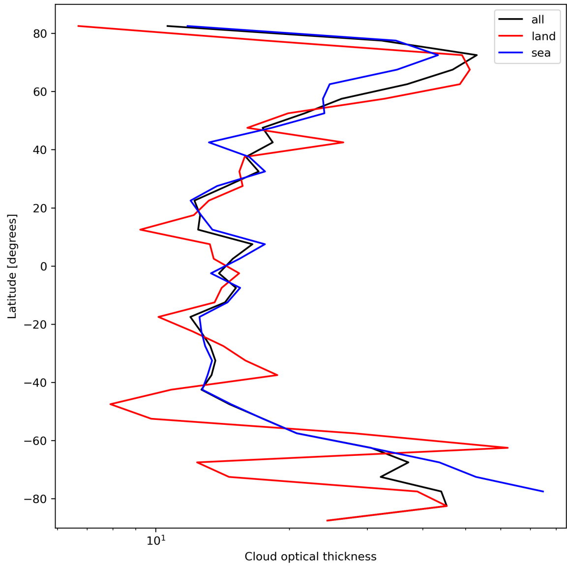
Figure 25: Zonal average of “Cloud optical thickness” for 2023-10-12 to 2023-10-13.
