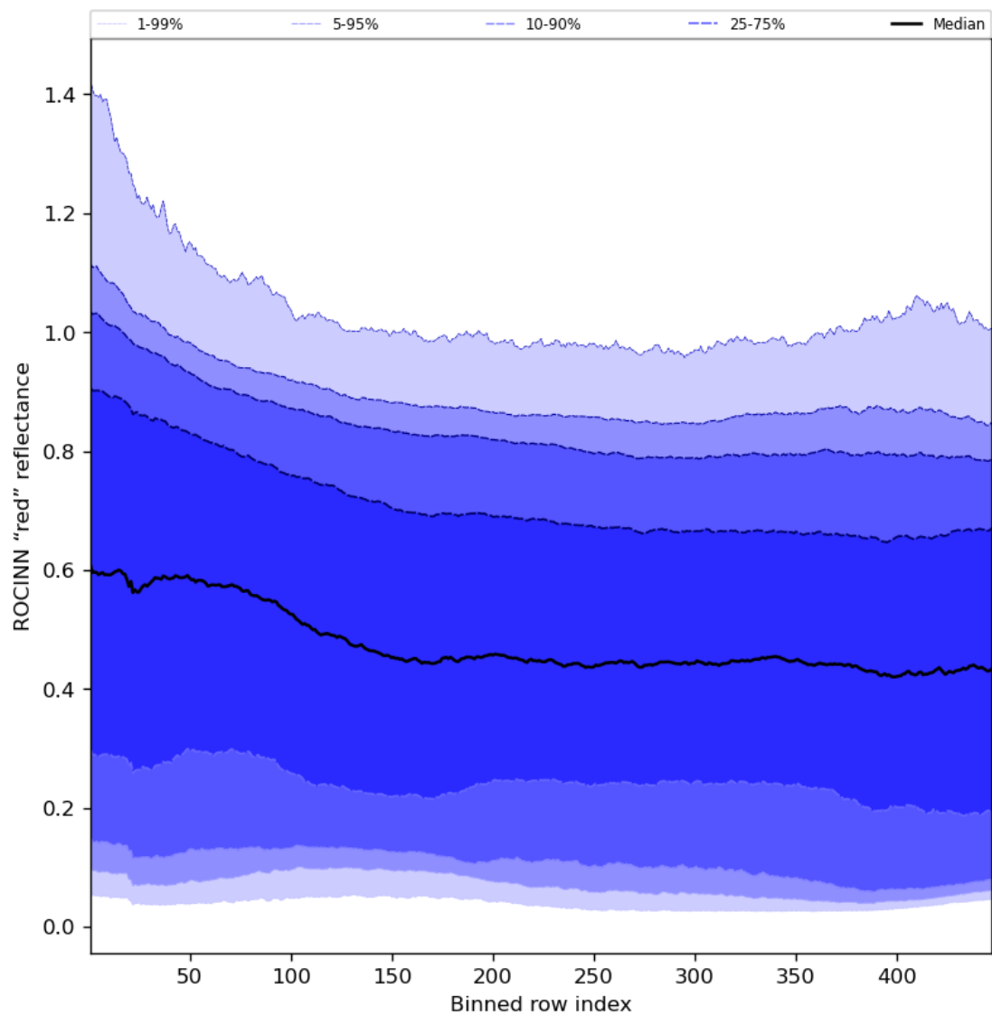
Figure 69: Along track statistics of “ROCINN “red” reflectance” for 2023-10-12 to 2023-10-13
