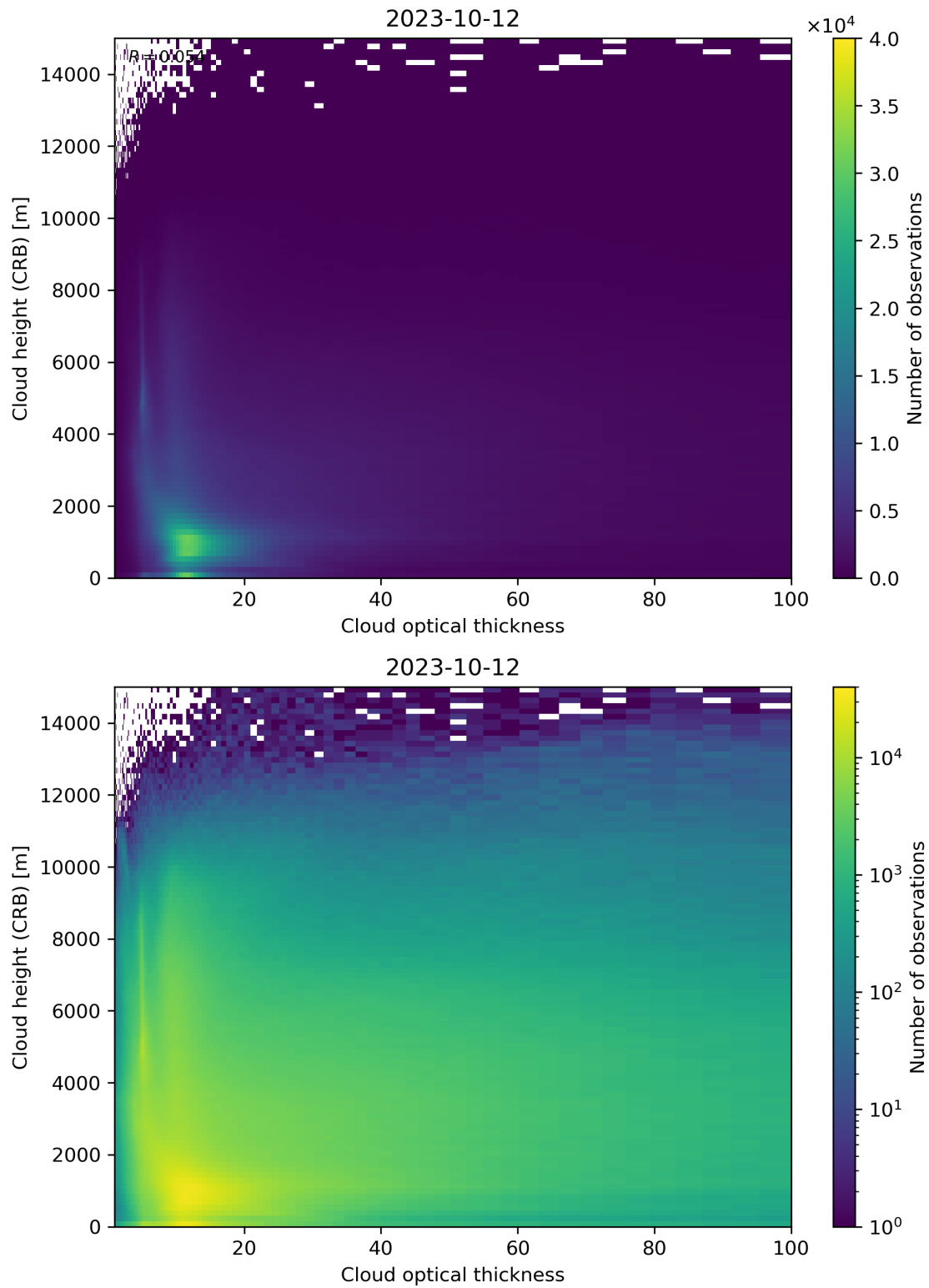
Figure 85: Scatter density plot of “Cloud optical thickness” against “Cloud height (CRB)” for 2023-10-12 to 2023-10-13.
