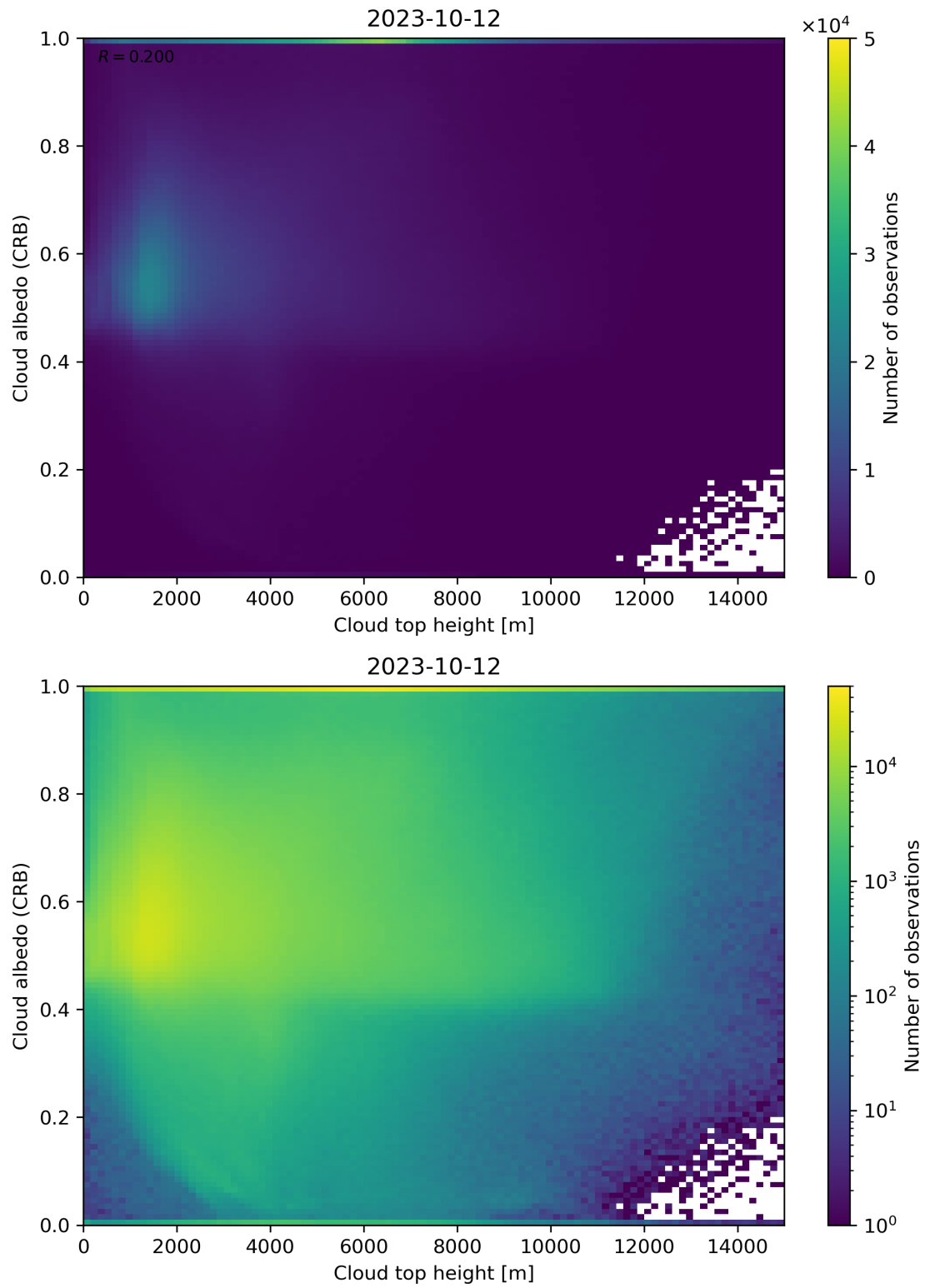
Figure 86: Scatter density plot of “Cloud top height” against “Cloud albedo (CRB)” for 2023-10-12 to 2023-10-13.
