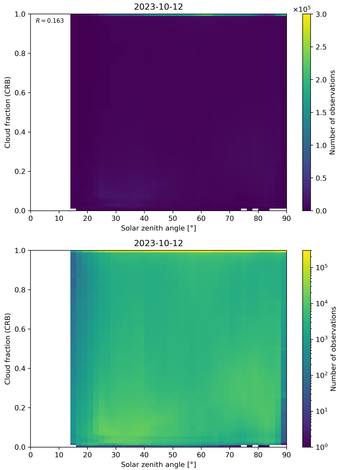
Figure 101: Scatter density plot of “Solar zenith angle” against “Cloud fraction (CRB)” for 2023-10-12 to 2023-10-13.
