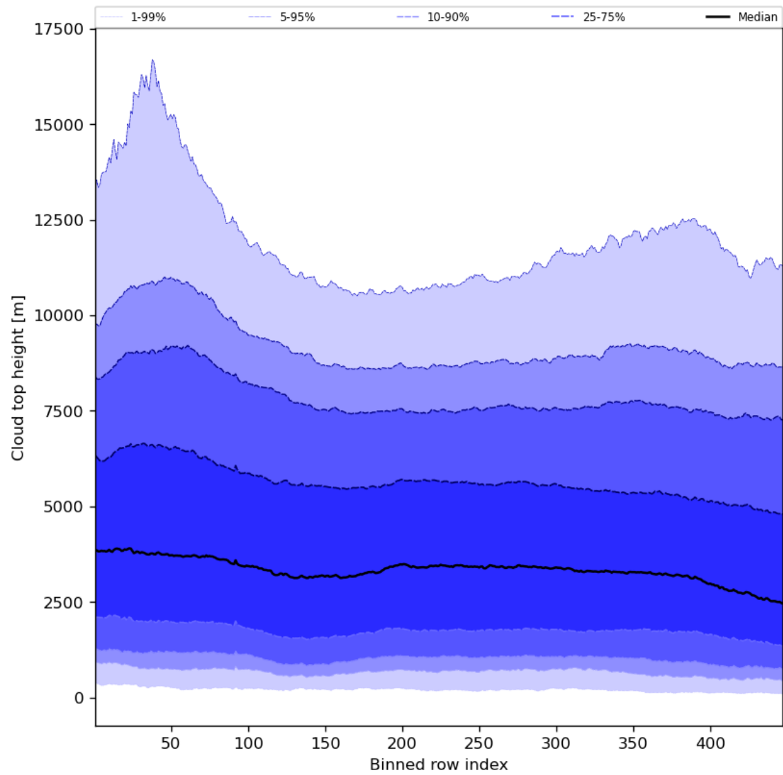
Figure 56: Along track statistics of “Cloud top height” for 2023-10-12 to 2023-10-13
