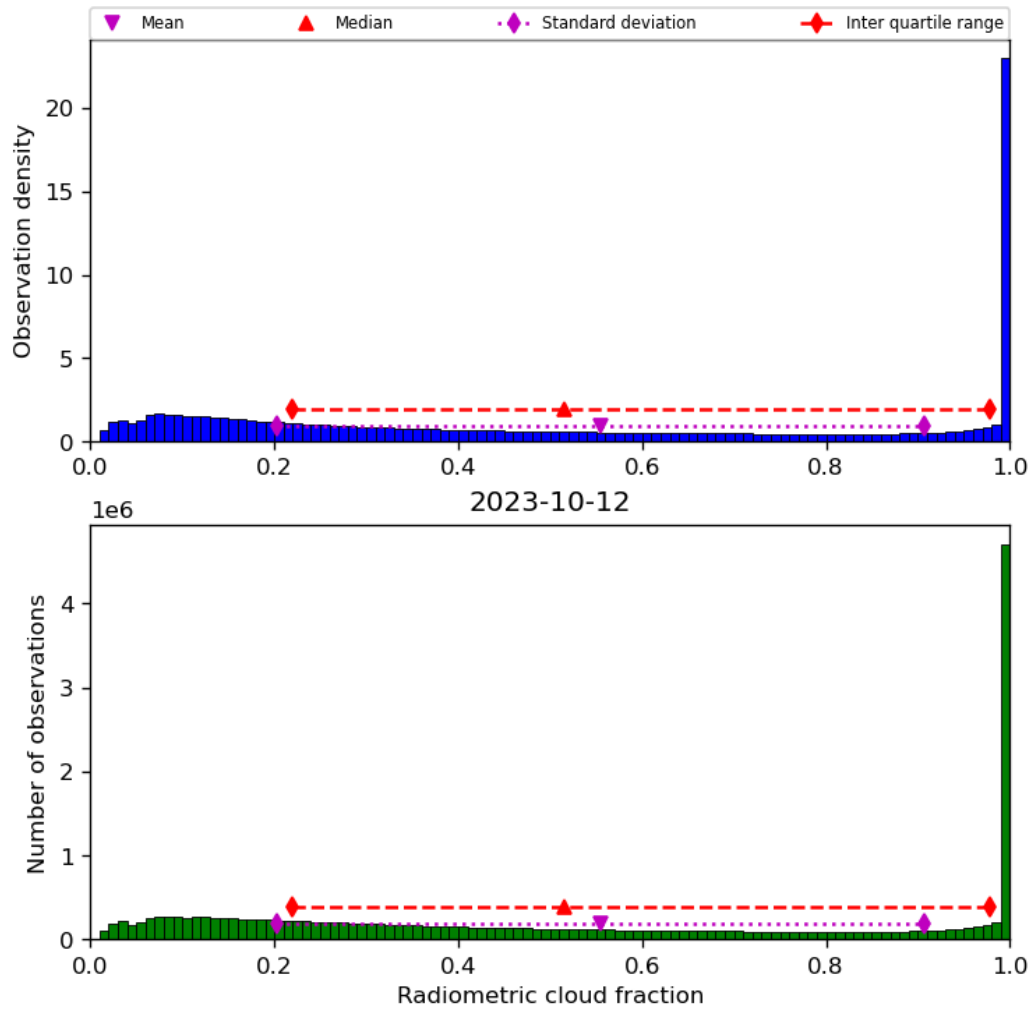
Figure 39: Histogram of “Radiometric cloud fraction” for 2023-10-12 to 2023-10-13
