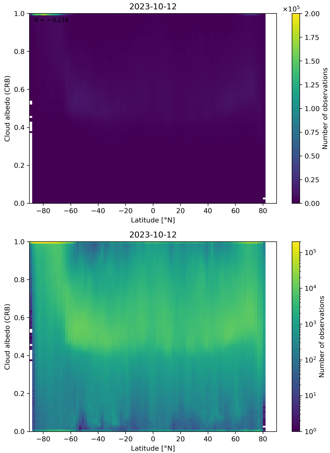
Figure 91: Scatter density plot of “Latitude” against “Cloud albedo (CRB)” for 2023-10-12 to 2023-10-13.
