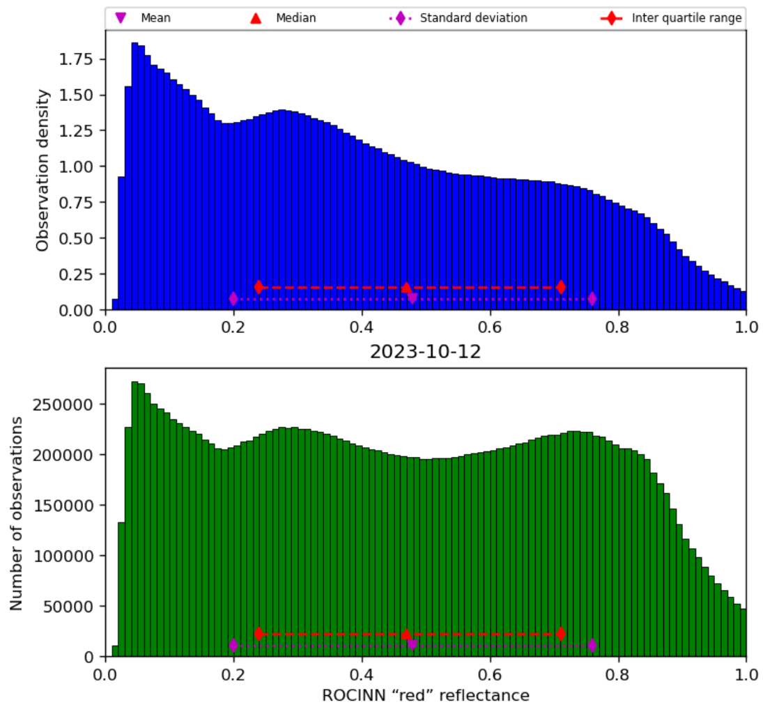
Figure 53: Histogram of “ROCINN “red” reflectance” for 2023-10-12 to 2023-10-13
