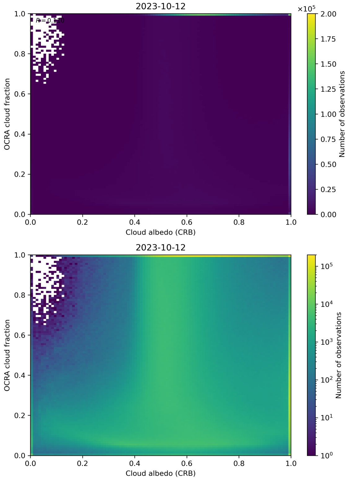
Figure 70: Scatter density plot of “Cloud albedo (CRB)” against “OCRA cloud fraction” for 2023-10-12 to 2023-10-13.
