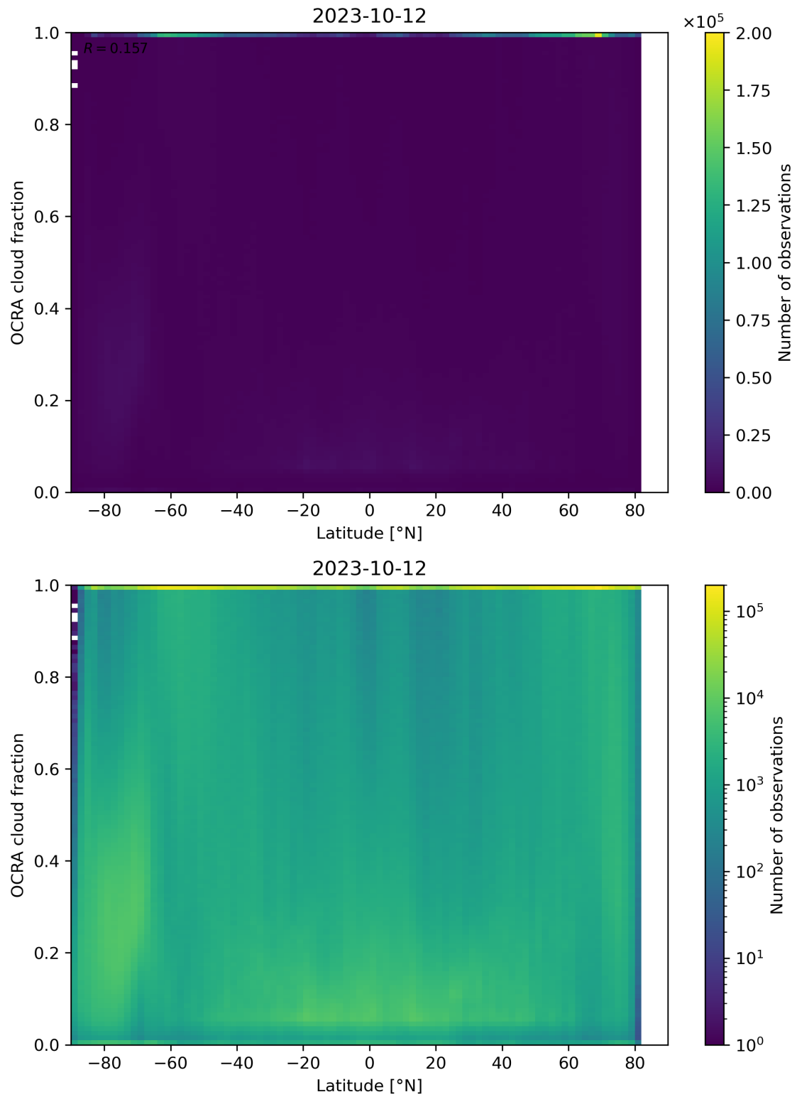
Figure 93: Scatter density plot of “Latitude” against “OCRA cloud fraction” for 2023-10-12 to 2023-10-13.
