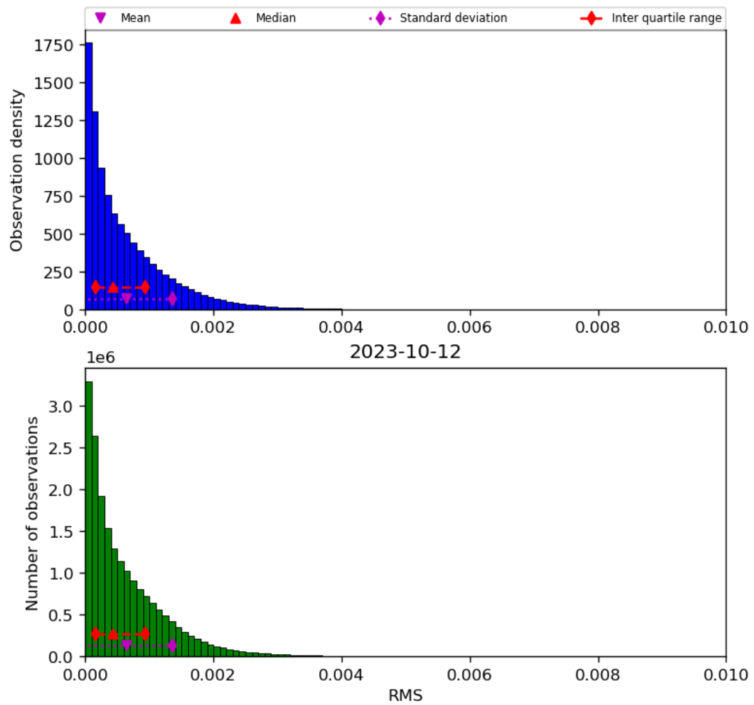
Figure 47: Histogram of “RMS” for 2023-10-12 to 2023-10-13
