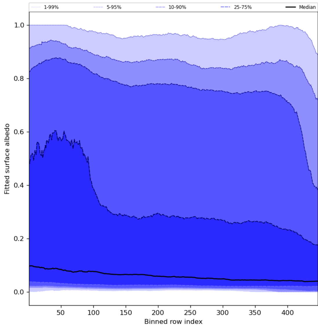
Figure 61: Along track statistics of “Fitted surface albedo” for 2023-10-12 to 2023-10-13
