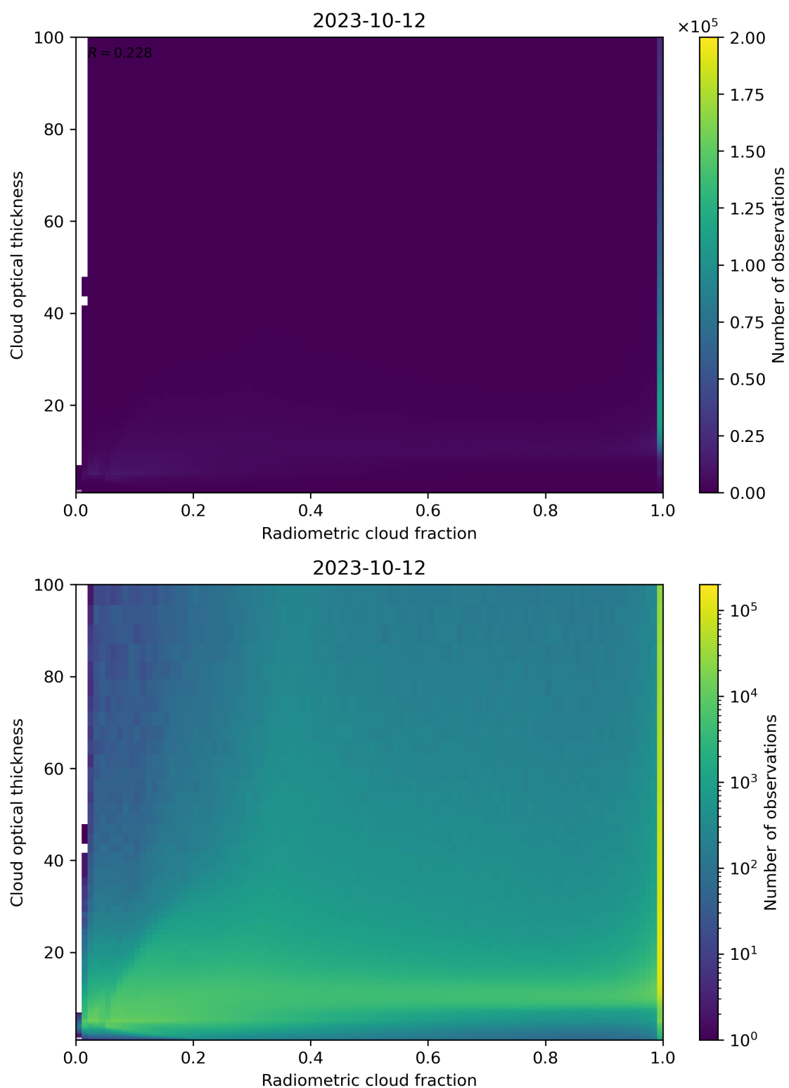
Figure 75: Scatter density plot of “Radiometric cloud fraction” against “Cloud optical thickness” for 2023-10-12 to 2023-10-13.
