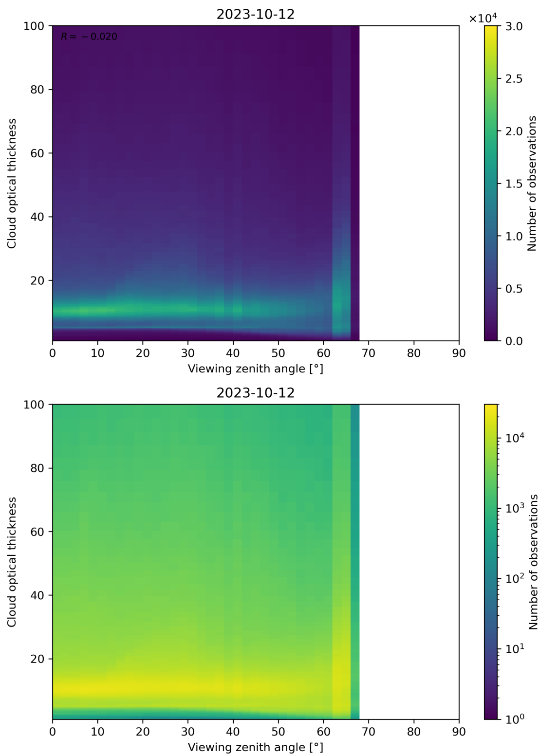
Figure 111: Scatter density plot of “Viewing zenith angle” against “Cloud optical thickness” for 2023-10-12 to 2023-10-13.
