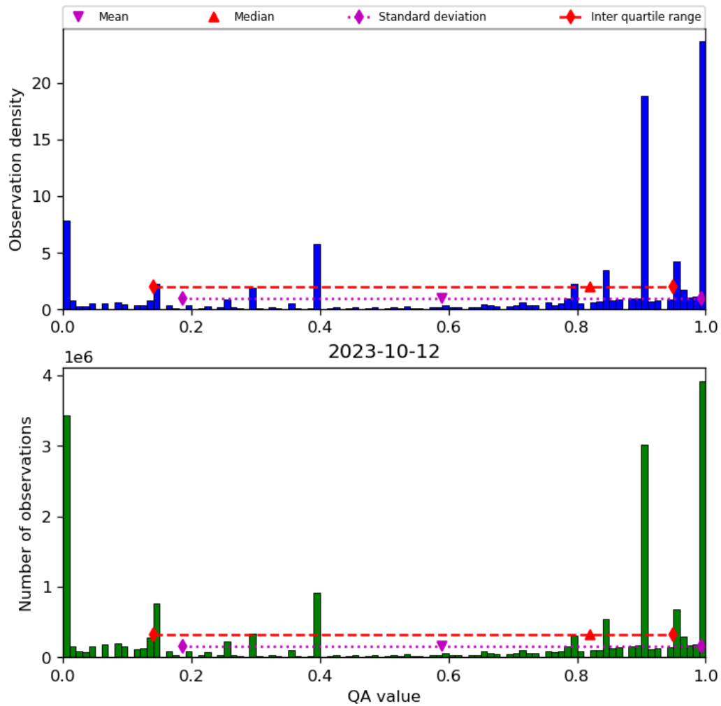
Figure 38: Histogram of “QA value” for 2023-10-12 to 2023-10-13
