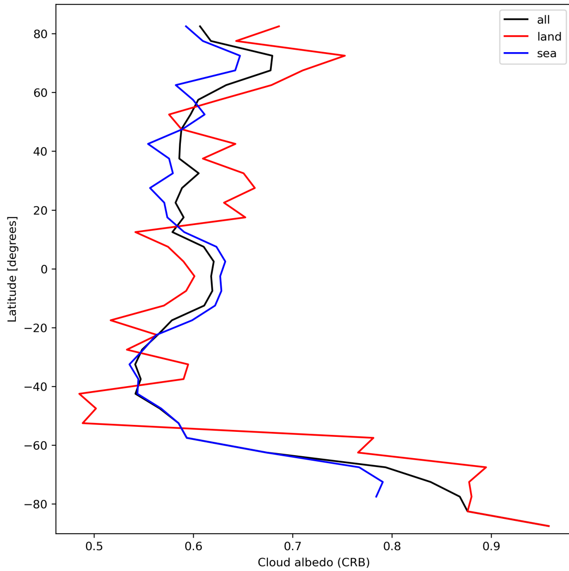
Figure 28: Zonal average of “Cloud albedo (CRB)” for 2023-10-12 to 2023-10-13.
