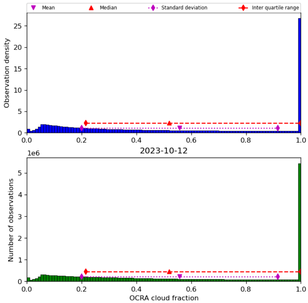
Figure 50: Histogram of “OCRA cloud fraction” for 2023-10-12 to 2023-10-13
