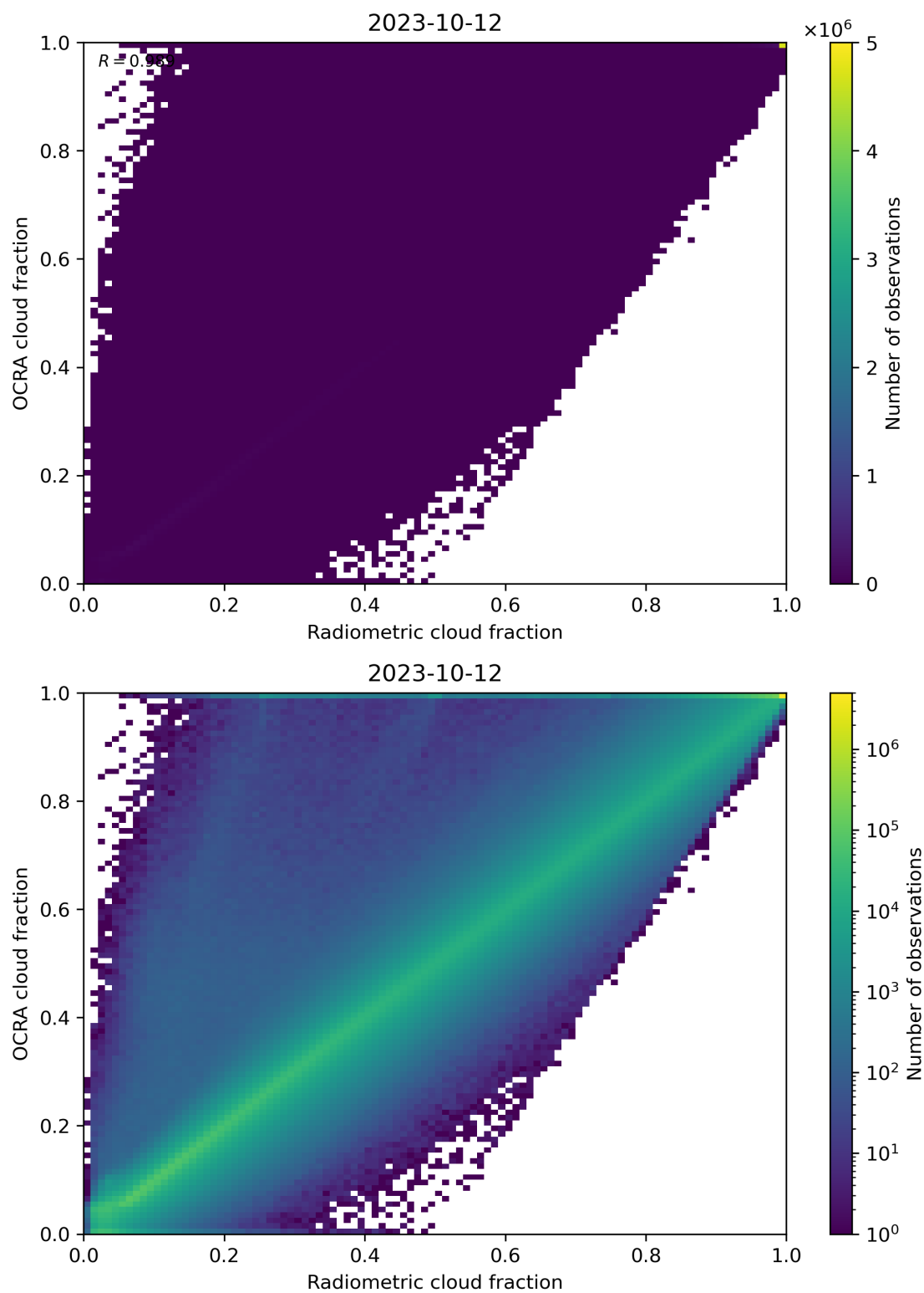
Figure 72: Scatter density plot of “Radiometric cloud fraction” against “OCRA cloud fraction” for 2023-10-12 to 2023-10-13.
