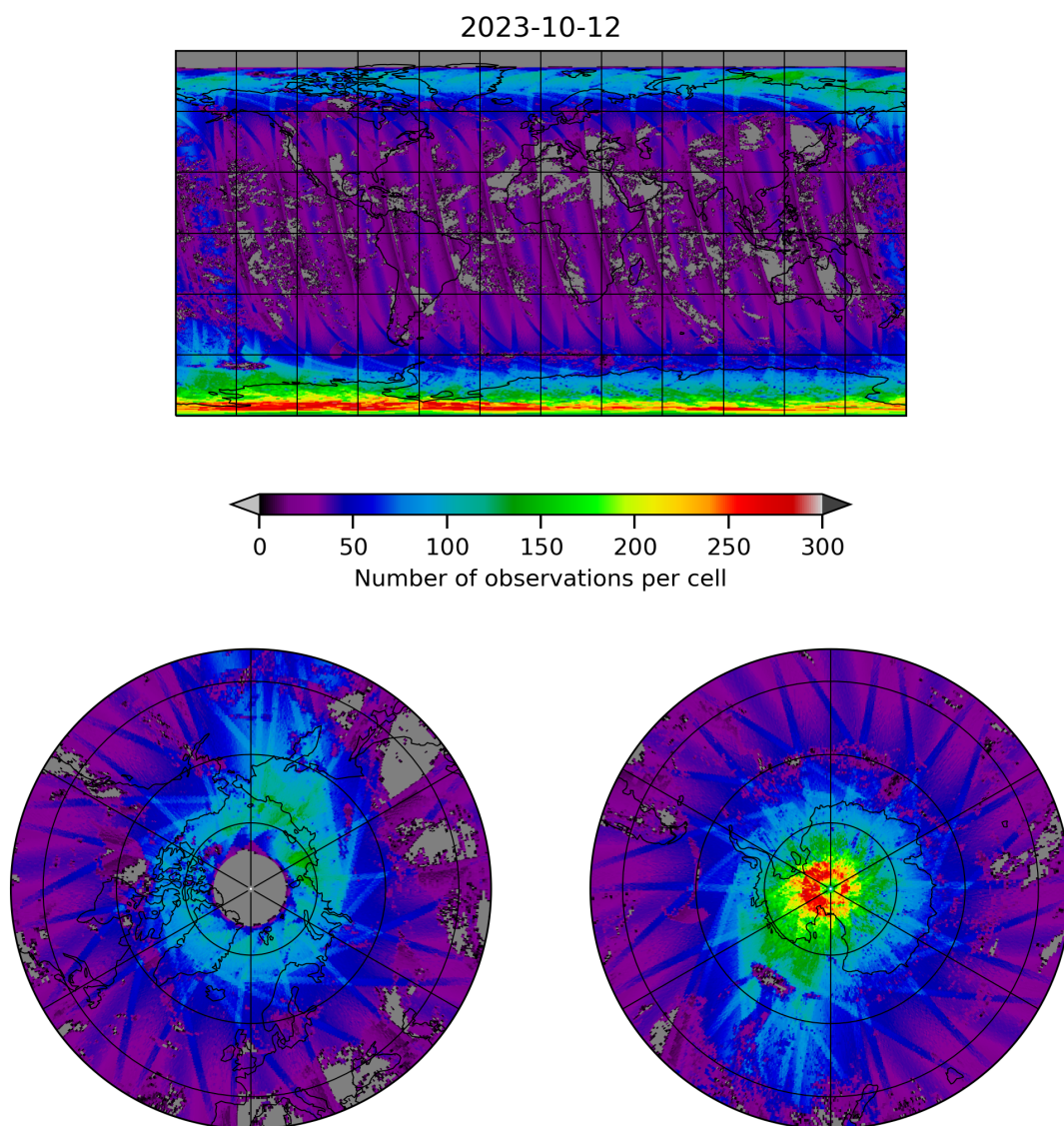
Figure 21: Map of the number of observations for 2023-10-12 to 2023-10-13
