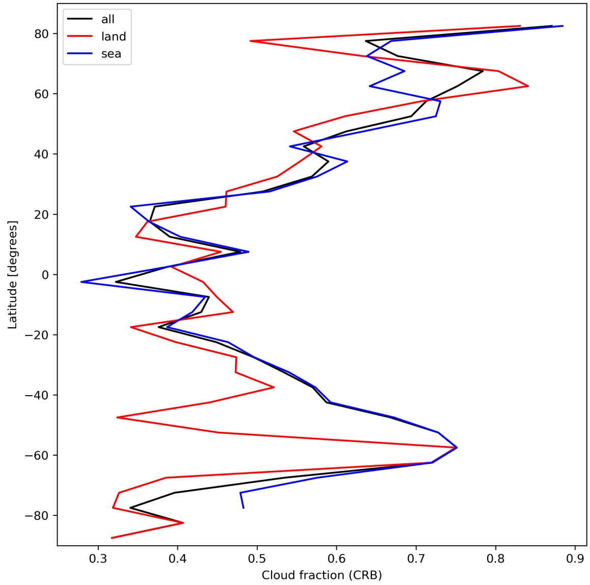
Figure 26: Zonal average of “Cloud fraction (CRB)” for 2023-10-12 to 2023-10-13.
