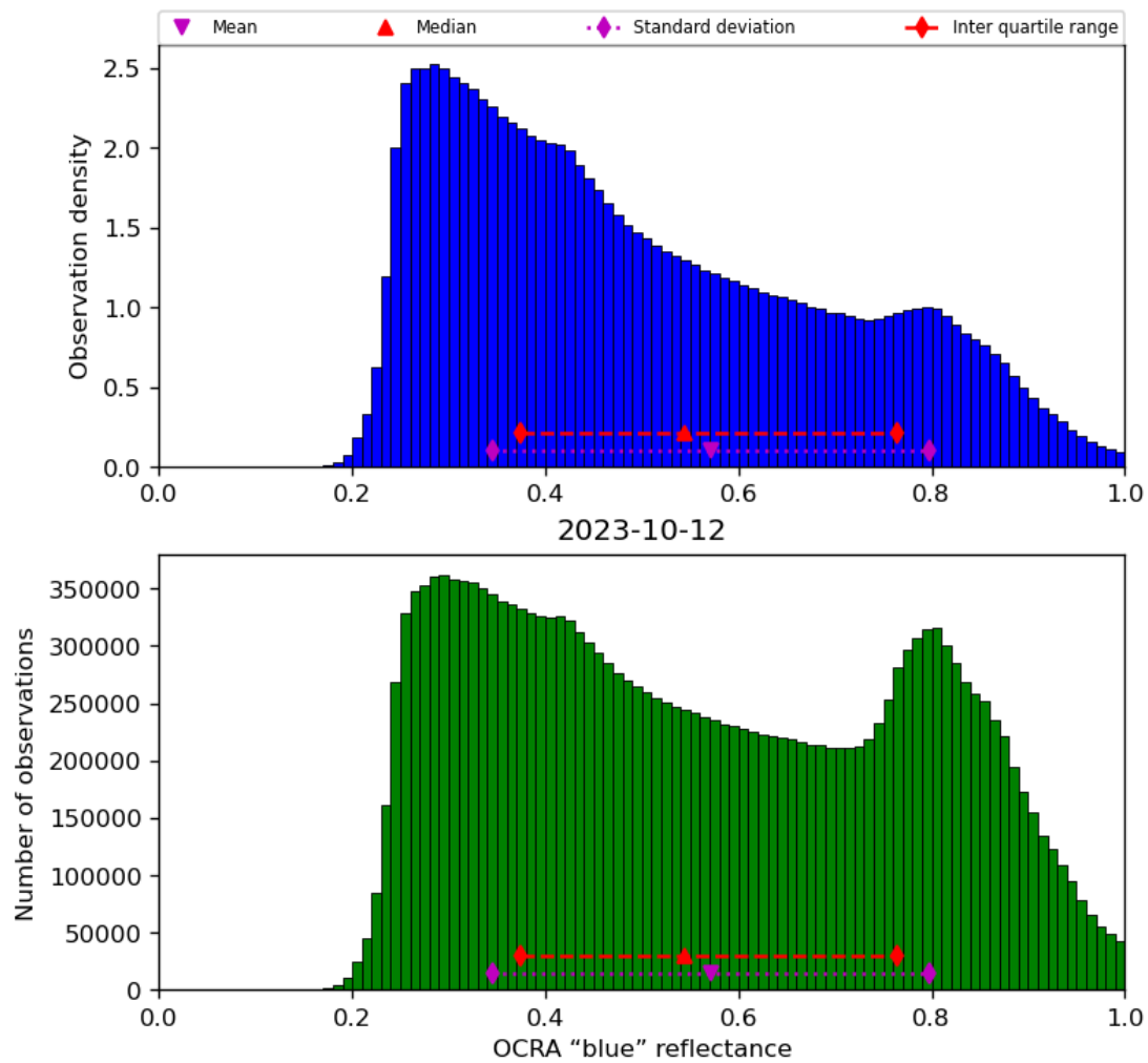
Figure 51: Histogram of “OCRA “blue” reflectance” for 2023-10-12 to 2023-10-13
