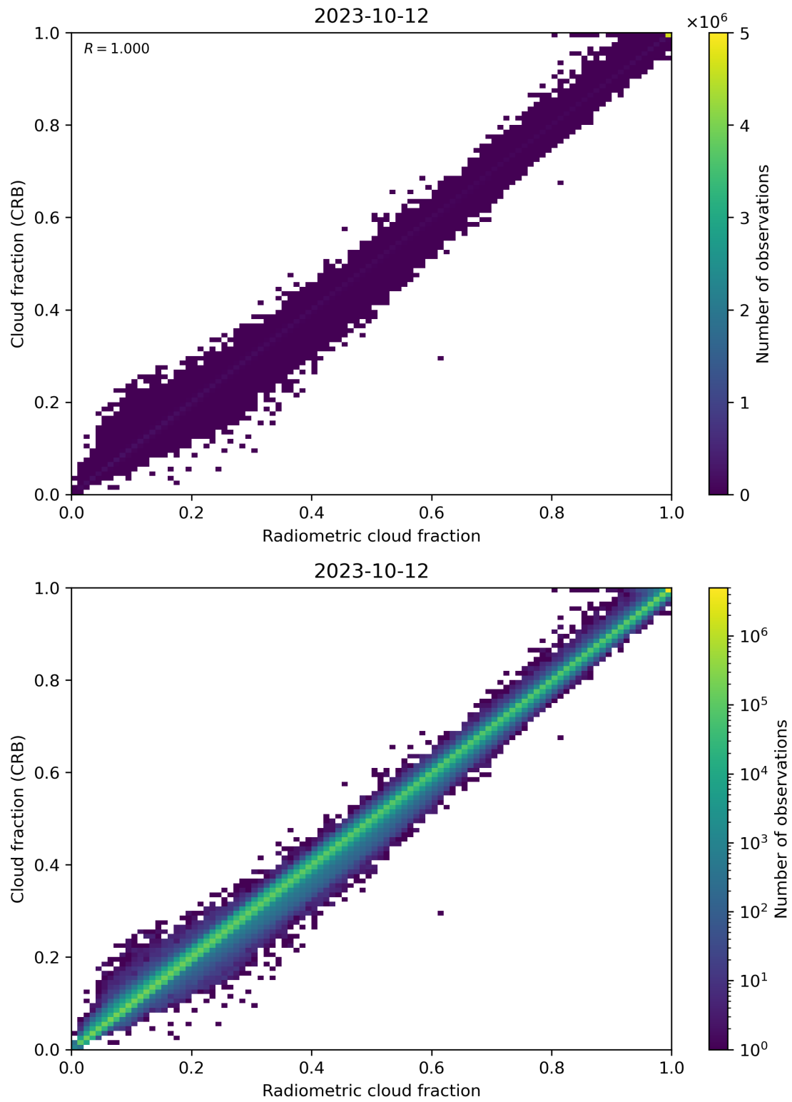
Figure 73: Scatter density plot of “Radiometric cloud fraction” against “Cloud fraction (CRB)” for 2023-10-12 to 2023-10-13.
