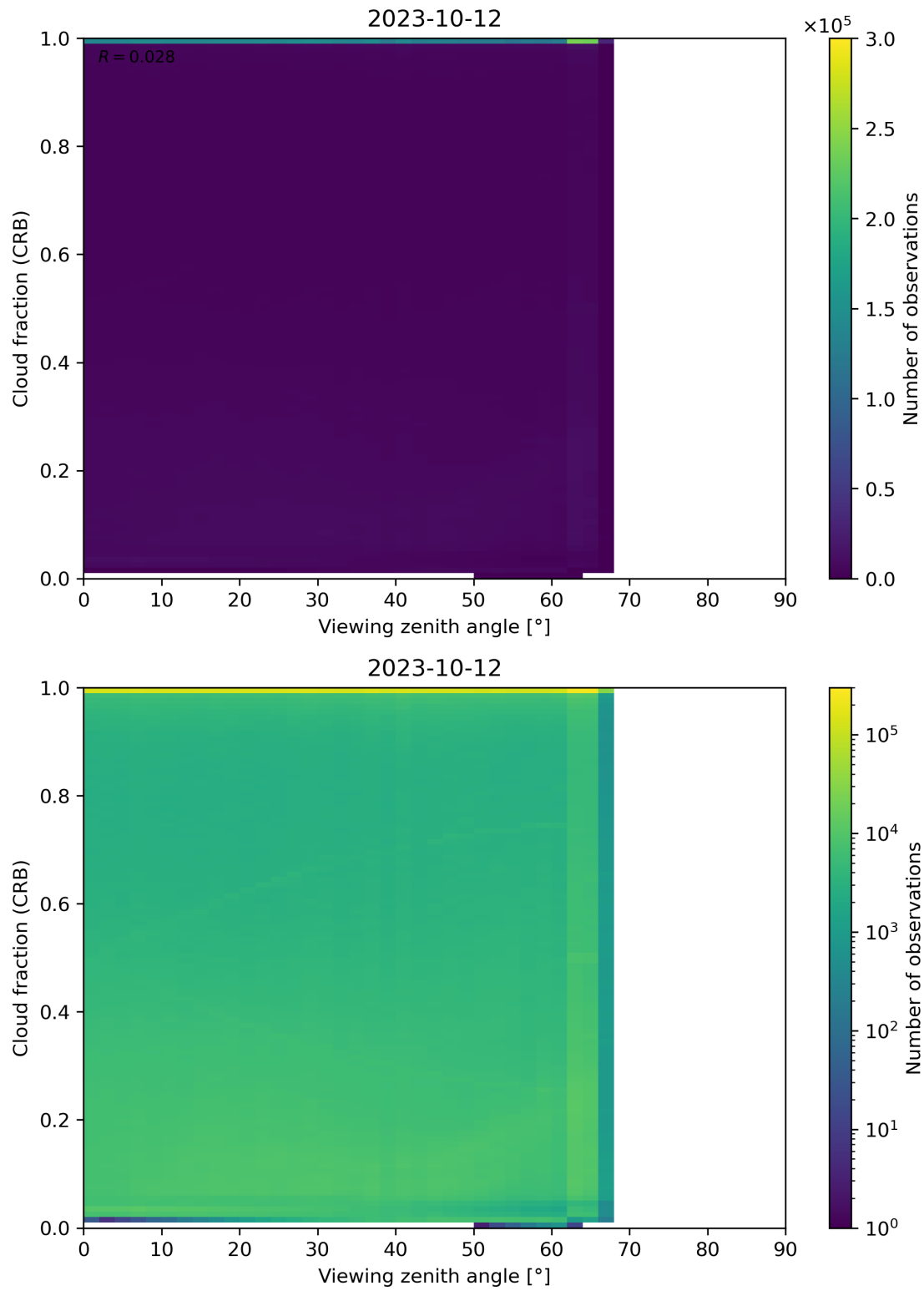
Figure 109: Scatter density plot of “Viewing zenith angle” against “Cloud fraction (CRB)” for 2023-10-12 to 2023-10-13.
