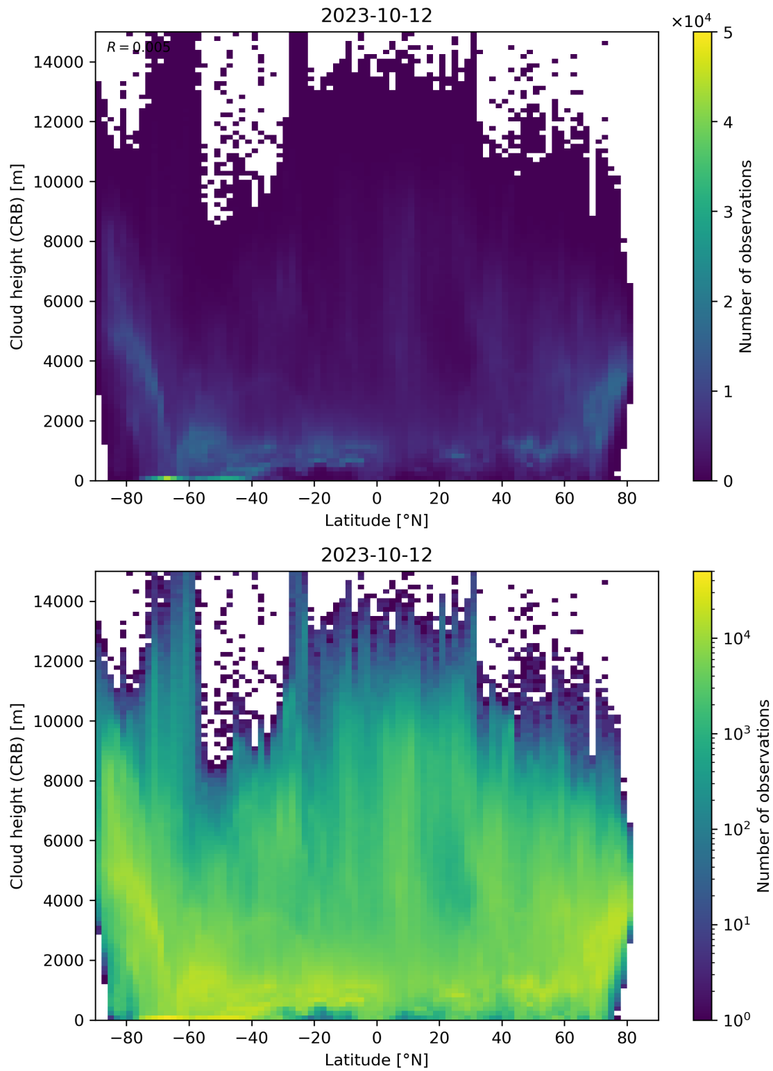
Figure 95: Scatter density plot of “Latitude” against “Cloud height (CRB)” for 2023-10-12 to 2023-10-13.
