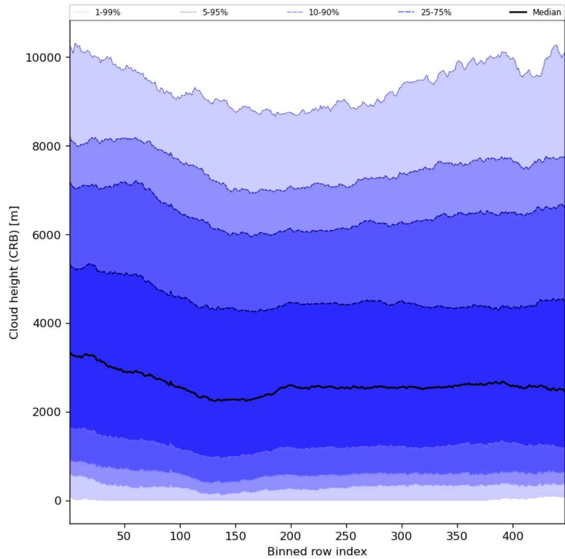
Figure 59: Along track statistics of “Cloud height (CRB)” for 2023-10-12 to 2023-10-13
