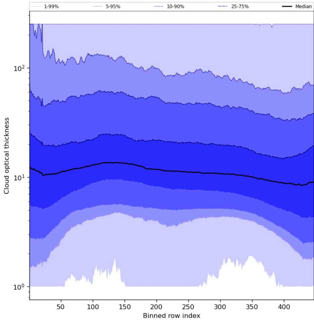
Figure 57: Along track statistics of “Cloud optical thickness” for 2023-10-12 to 2023-10-13
