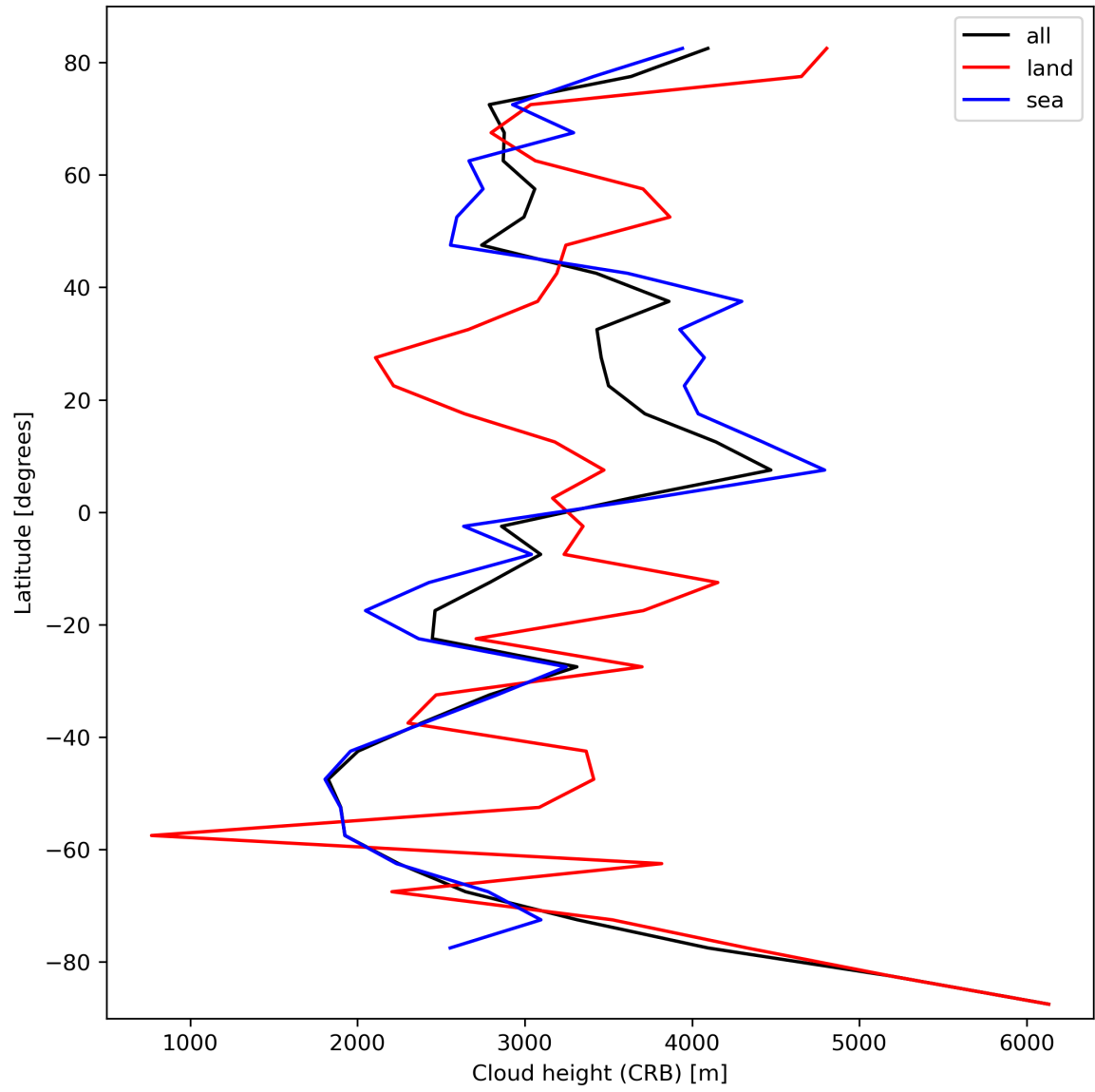
Figure 27: Zonal average of “Cloud height (CRB)” for 2023-10-12 to 2023-10-13.
