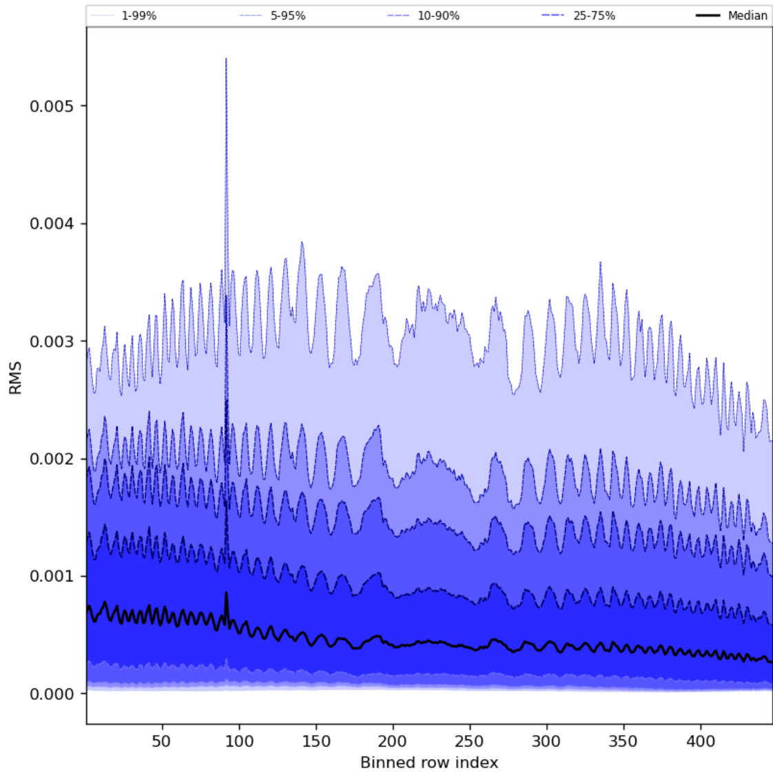
Figure 63: Along track statistics of “RMS” for 2023-10-12 to 2023-10-13
