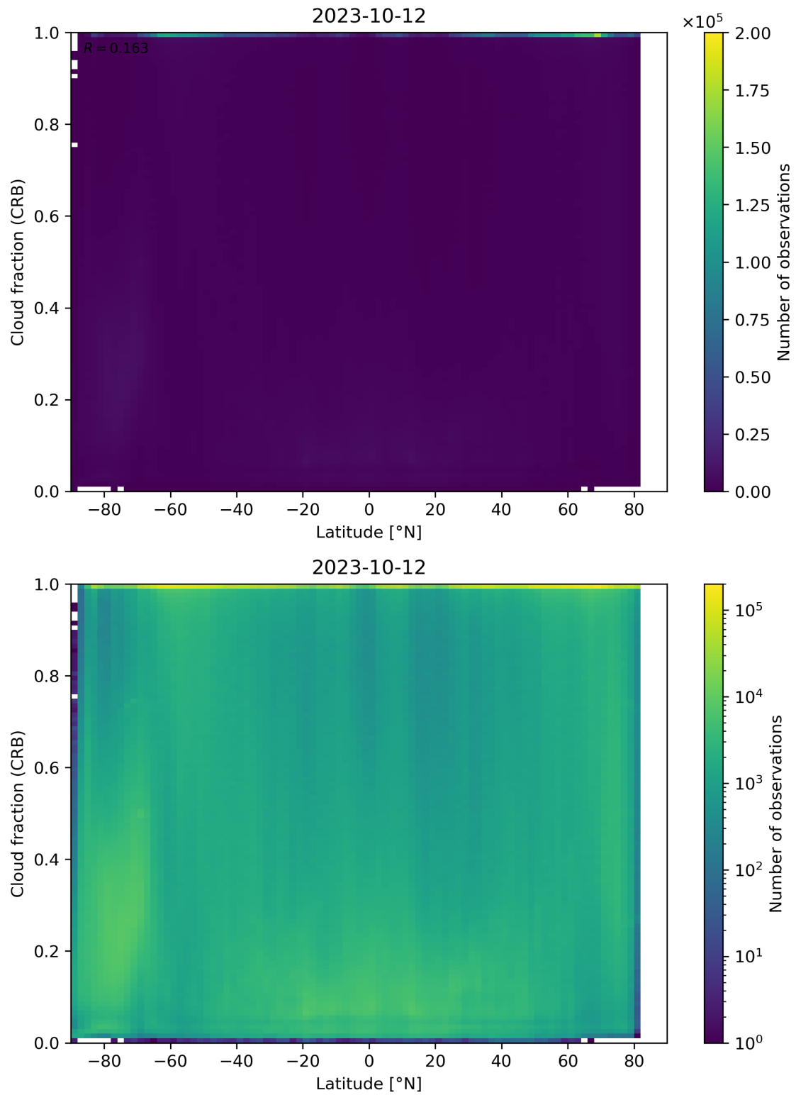
Figure 94: Scatter density plot of “Latitude” against “Cloud fraction (CRB)” for 2023-10-12 to 2023-10-13.
