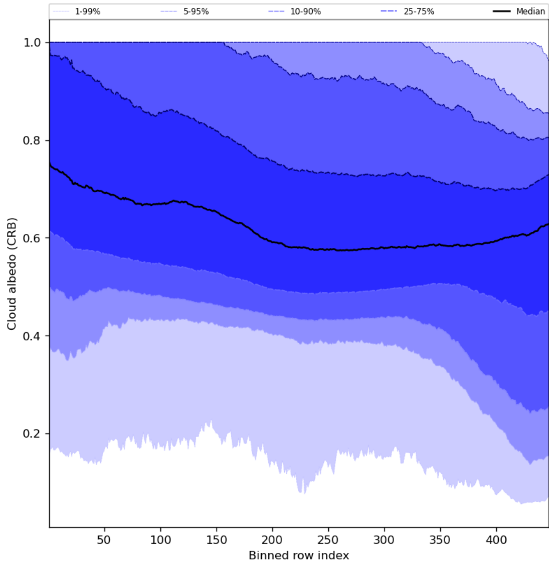
Figure 60: Along track statistics of “Cloud albedo (CRB)” for 2023-10-12 to 2023-10-13
