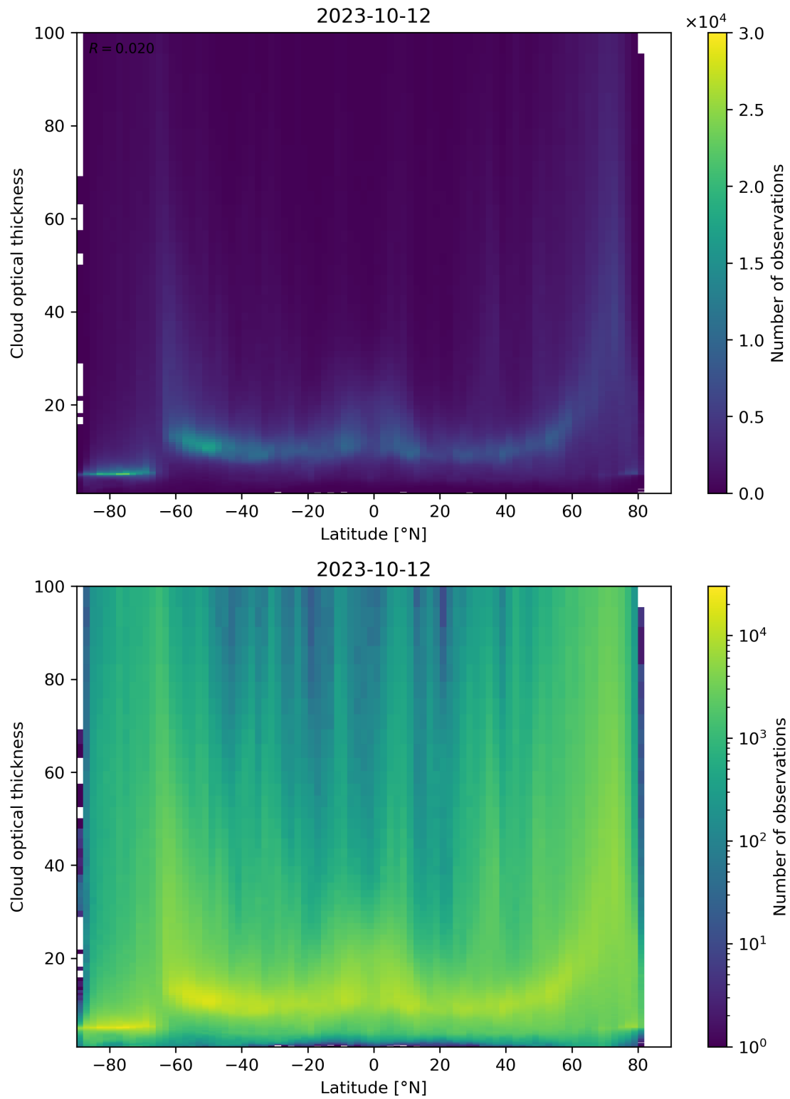
Figure 96: Scatter density plot of “Latitude” against “Cloud optical thickness” for 2023-10-12 to 2023-10-13.
