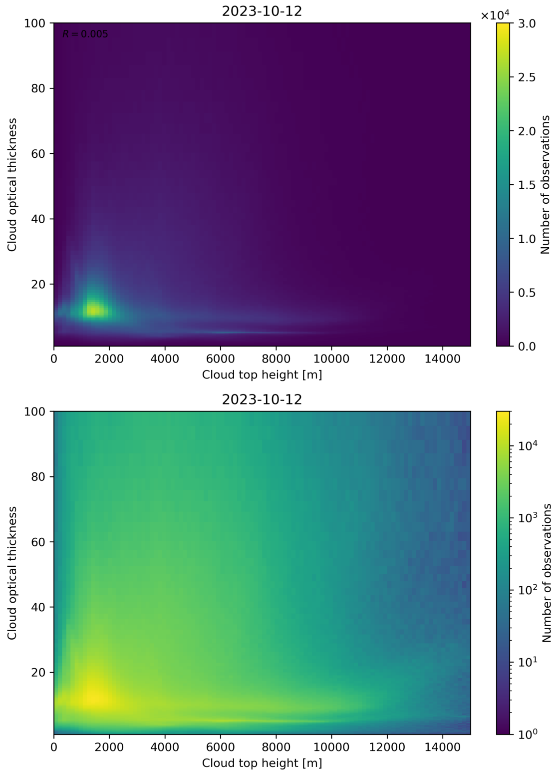
Figure 90: Scatter density plot of “Cloud top height” against “Cloud optical thickness” for 2023-10-12 to 2023-10-13.
