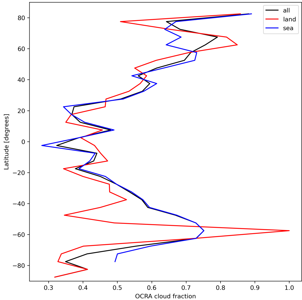
Figure 34: Zonal average of “OCRA cloud fraction” for 2023-10-12 to 2023-10-13.
