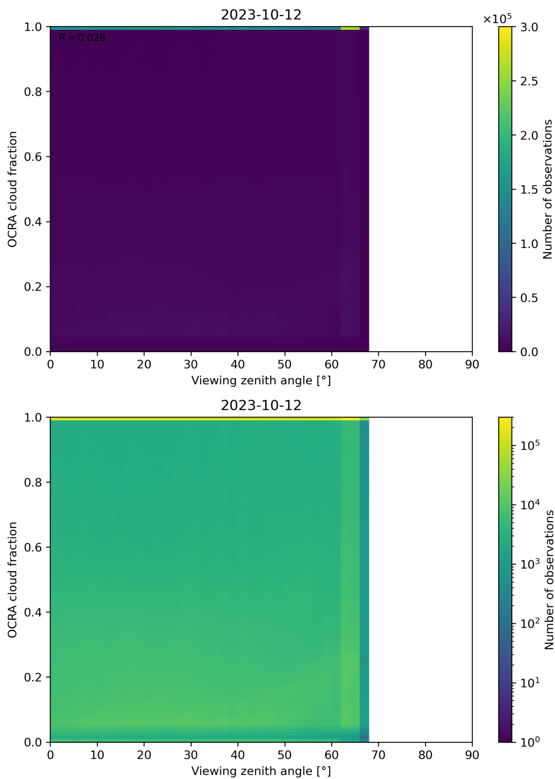
Figure 108: Scatter density plot of “Viewing zenith angle” against “OCRA cloud fraction” for 2023-10-12 to 2023-10-13.
