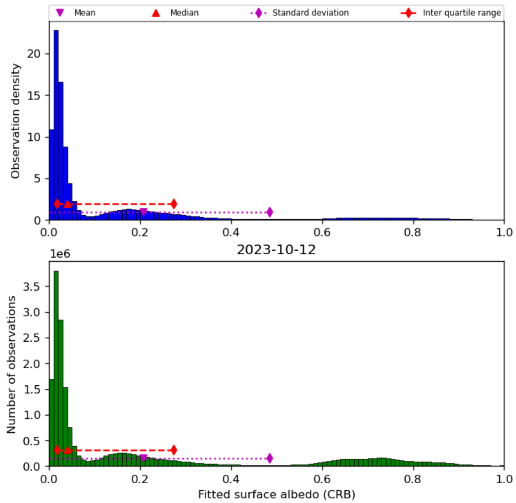
Figure 46: Histogram of “Fitted surface albedo (CRB)” for 2023-10-12 to 2023-10-13
