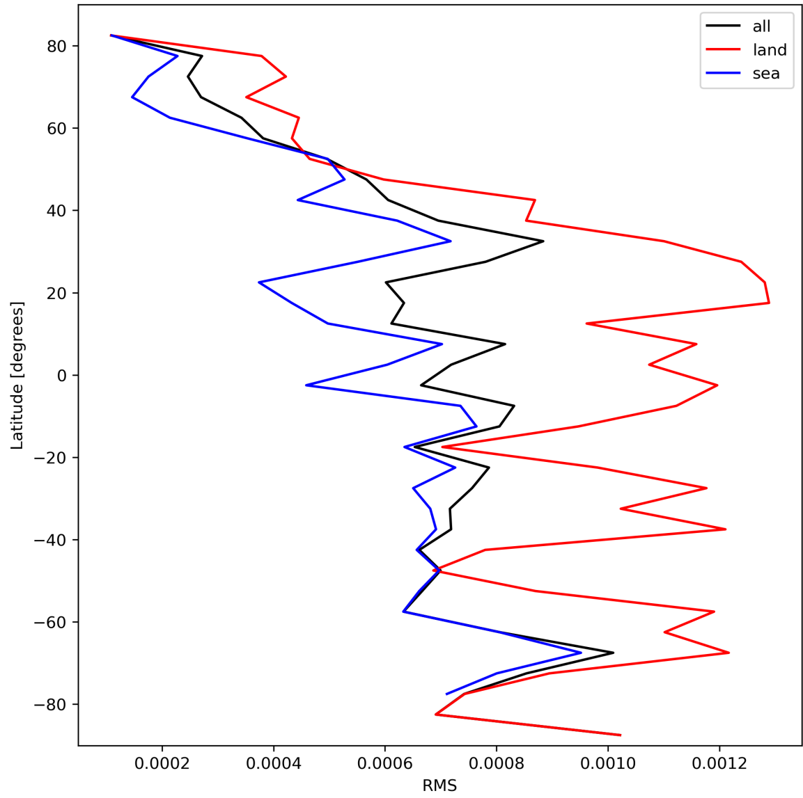
Figure 31: Zonal average of “RMS” for 2023-10-12 to 2023-10-13.
