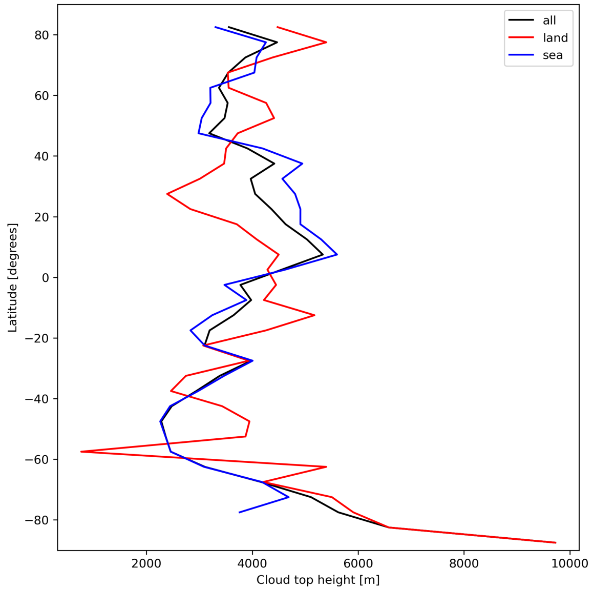
Figure 24: Zonal average of “Cloud top height” for 2023-10-12 to 2023-10-13.
