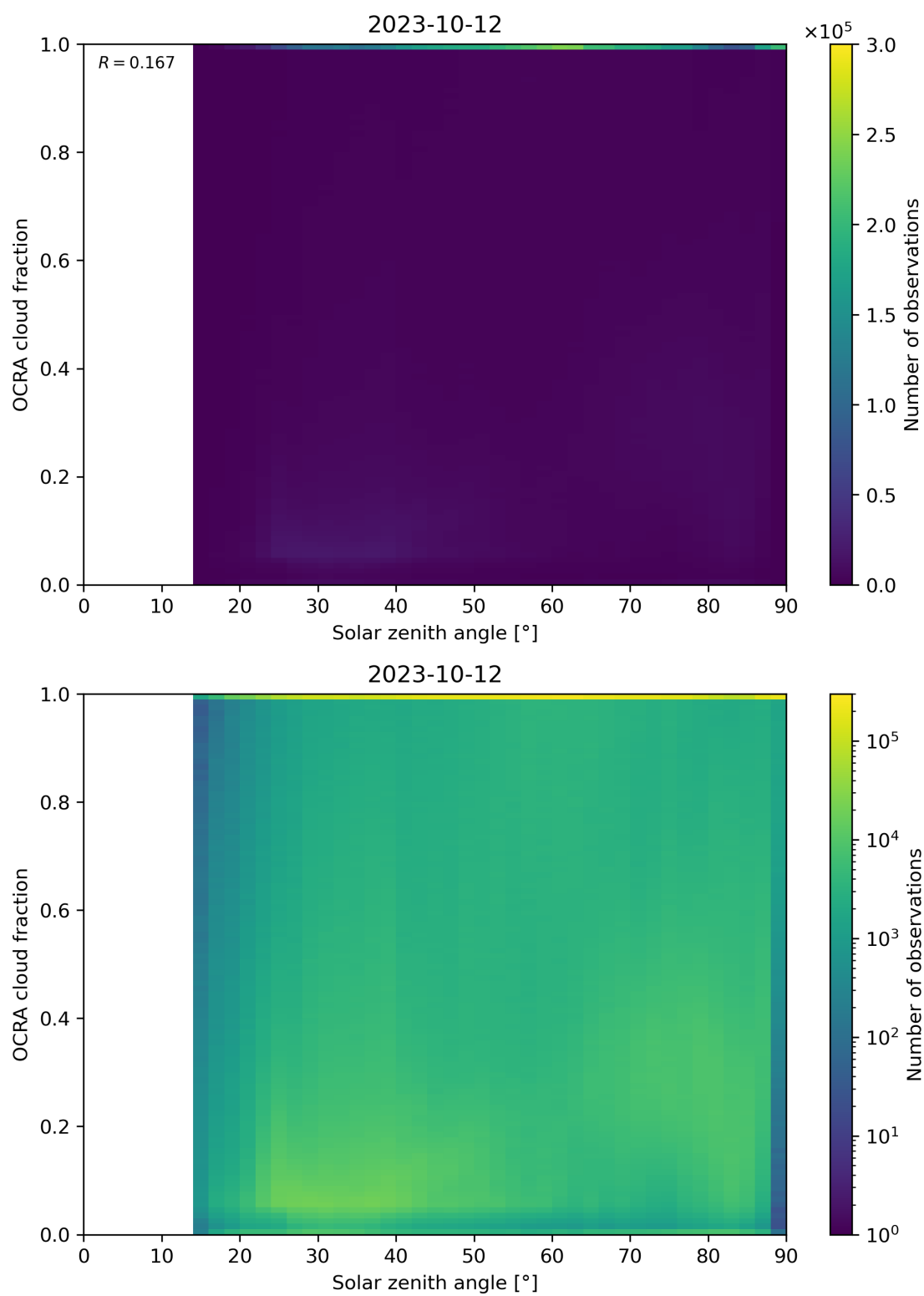
Figure 100: Scatter density plot of “Solar zenith angle” against “OCRA cloud fraction” for 2023-10-12 to 2023-10-13.
