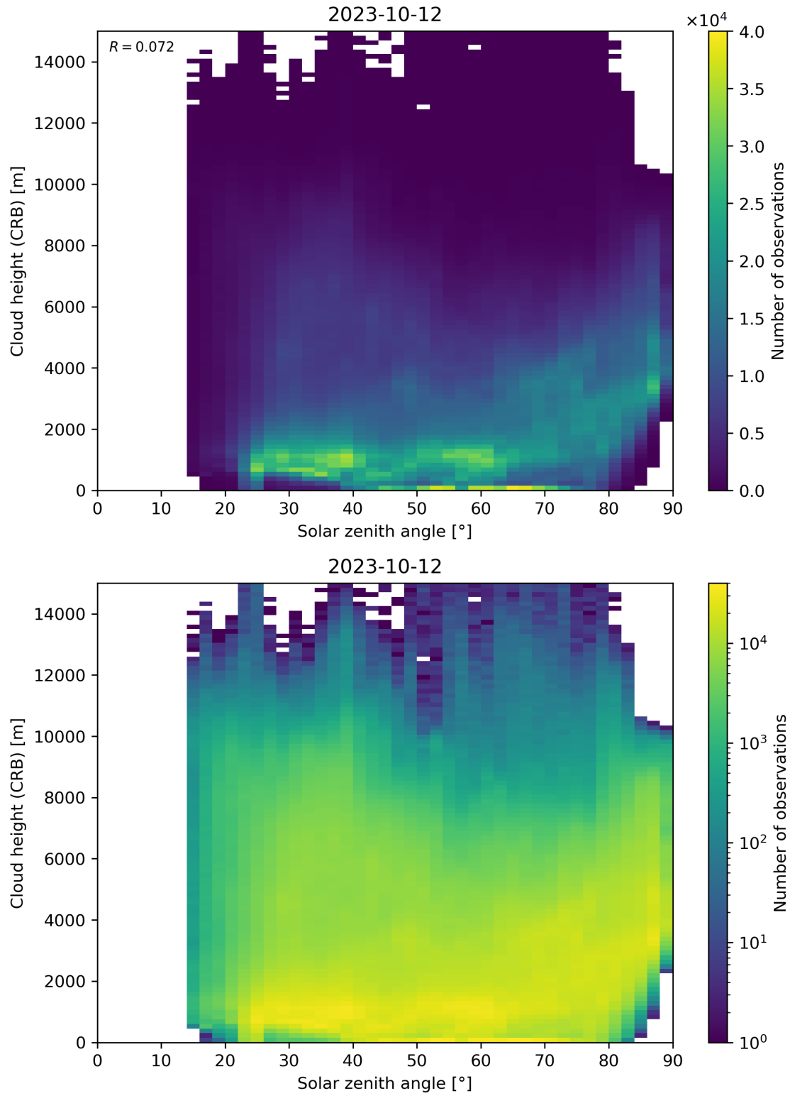
Figure 102: Scatter density plot of “Solar zenith angle” against “Cloud height (CRB)” for 2023-10-12 to 2023-10-13.
