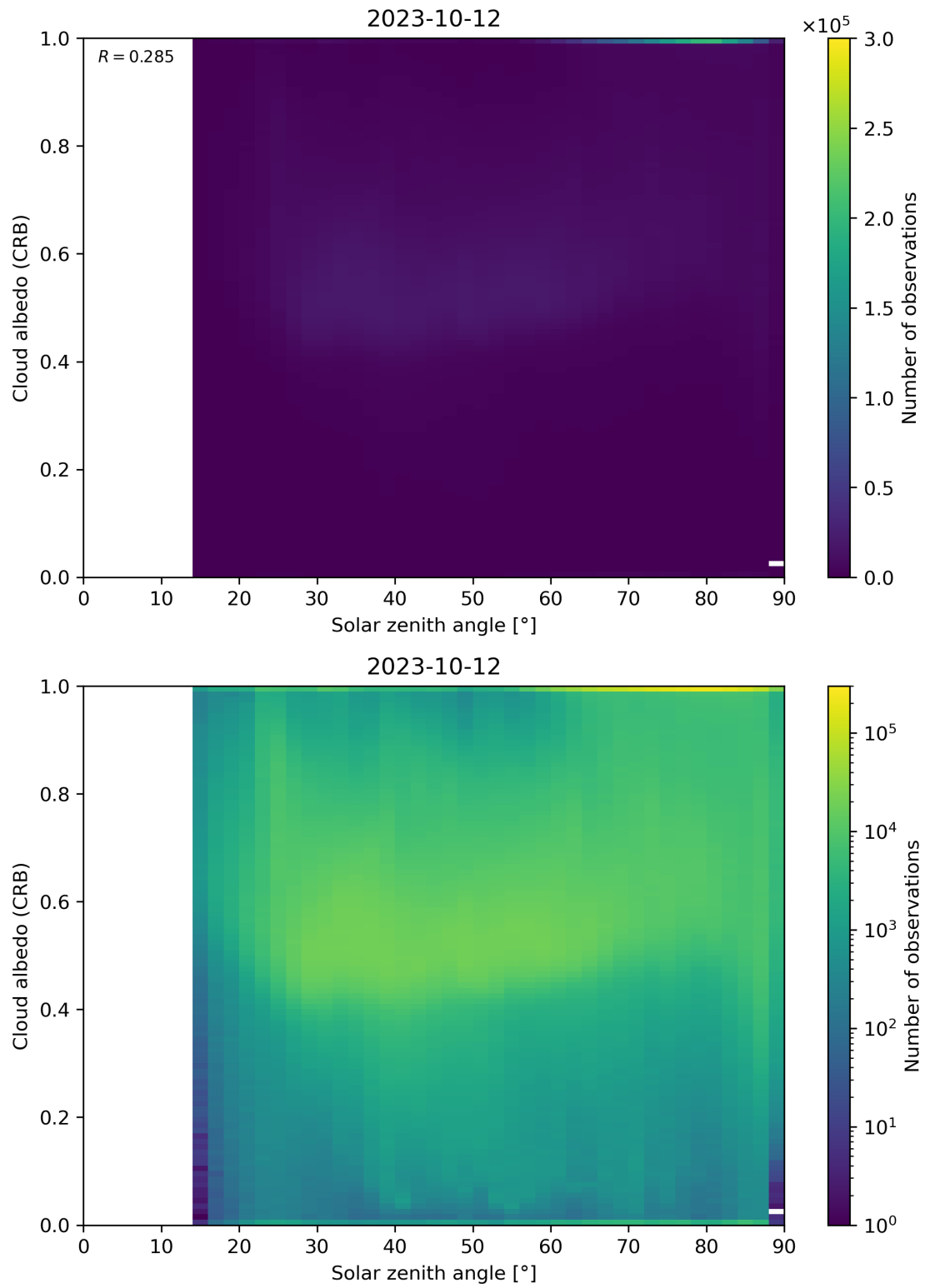
Figure 98: Scatter density plot of “Solar zenith angle” against “Cloud albedo (CRB)” for 2023-10-12 to 2023-10-13.
