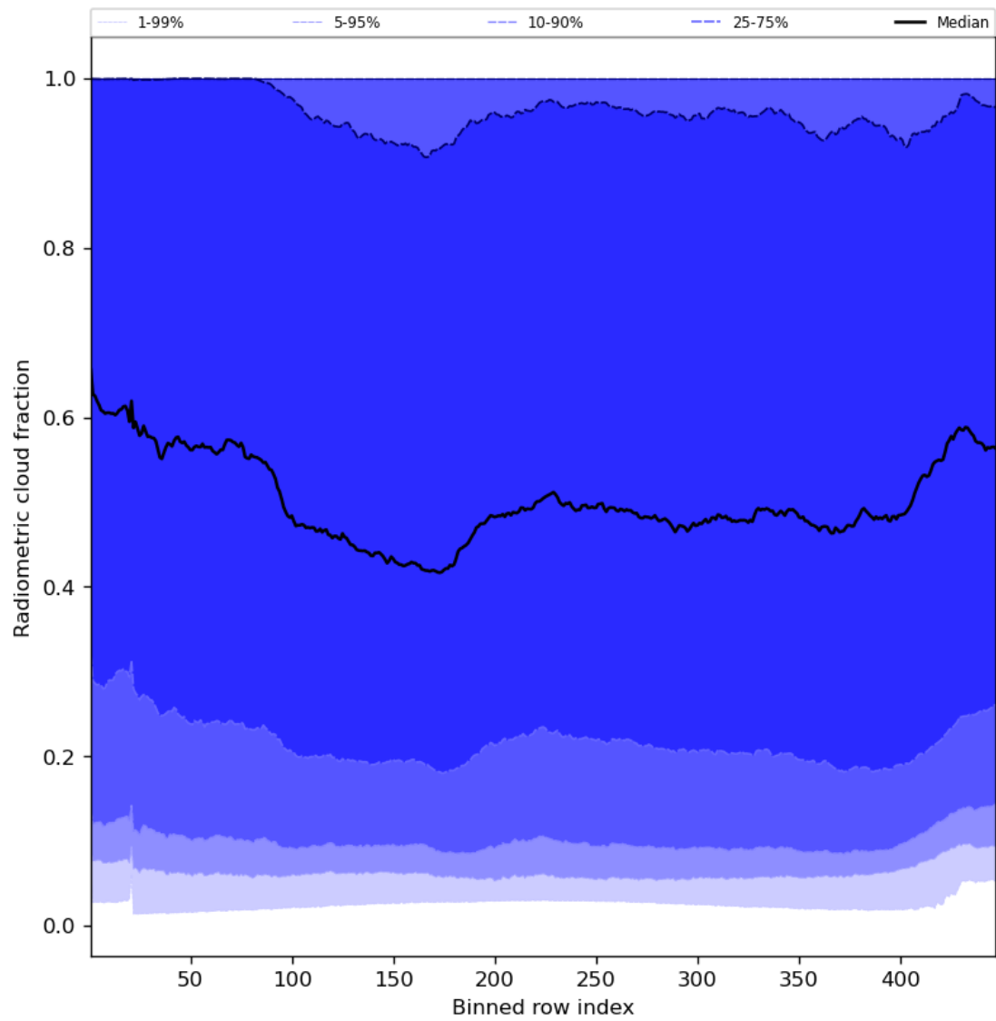
Figure 55: Along track statistics of “Radiometric cloud fraction” for 2023-10-12 to 2023-10-14
