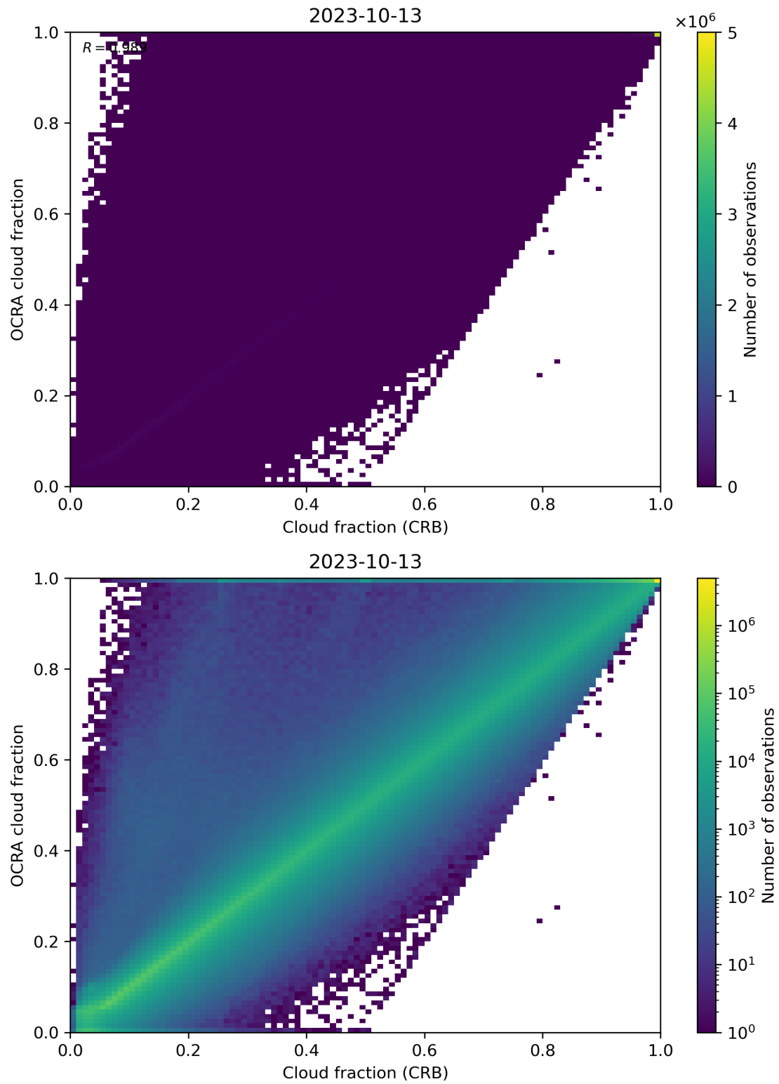
Figure 78: Scatter density plot of “Cloud fraction (CRB)” against “OCRA cloud fraction” for 2023-10-12 to 2023-10-14.
