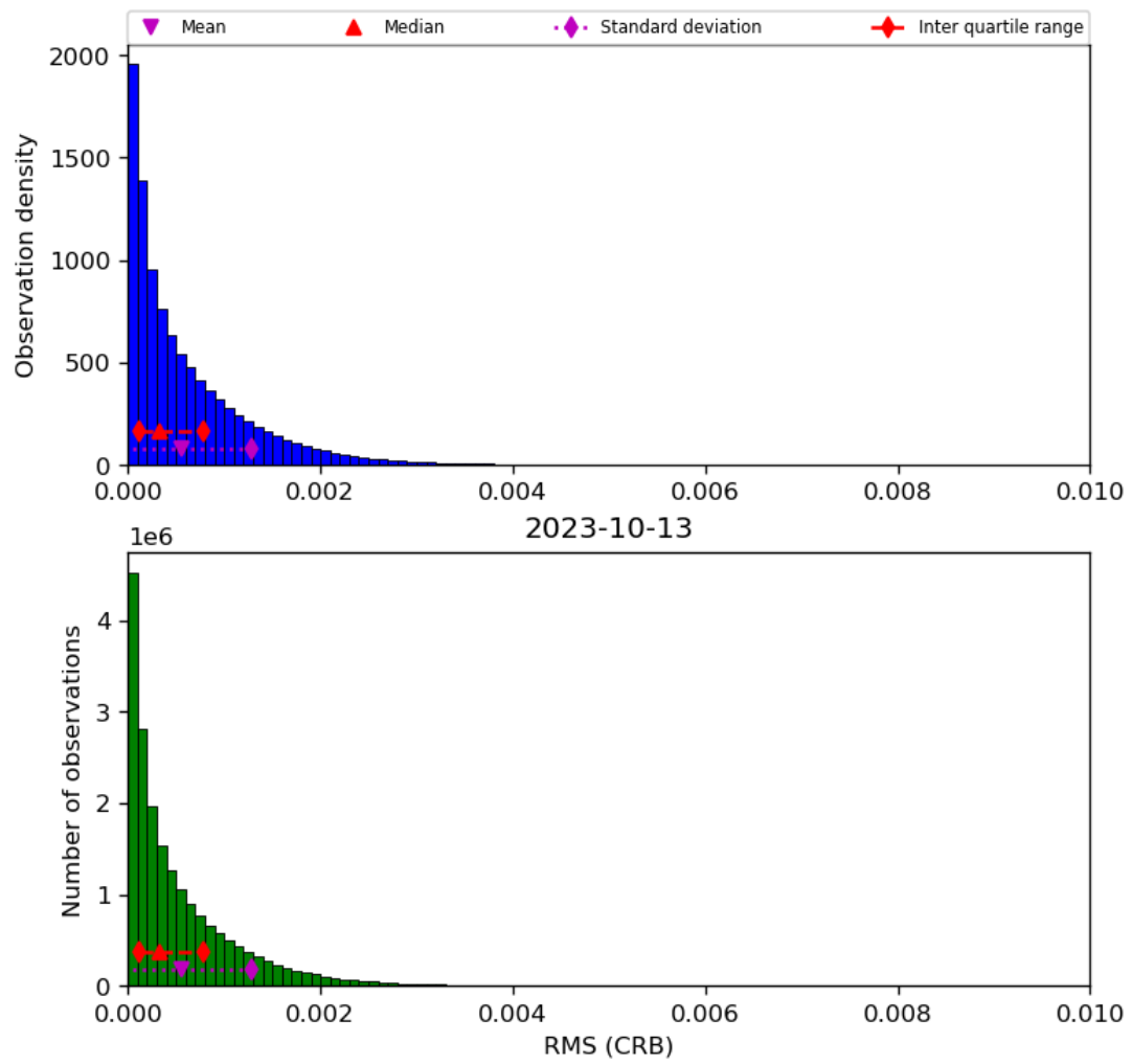
Figure 48: Histogram of “RMS (CRB)” for 2023-10-12 to 2023-10-14
