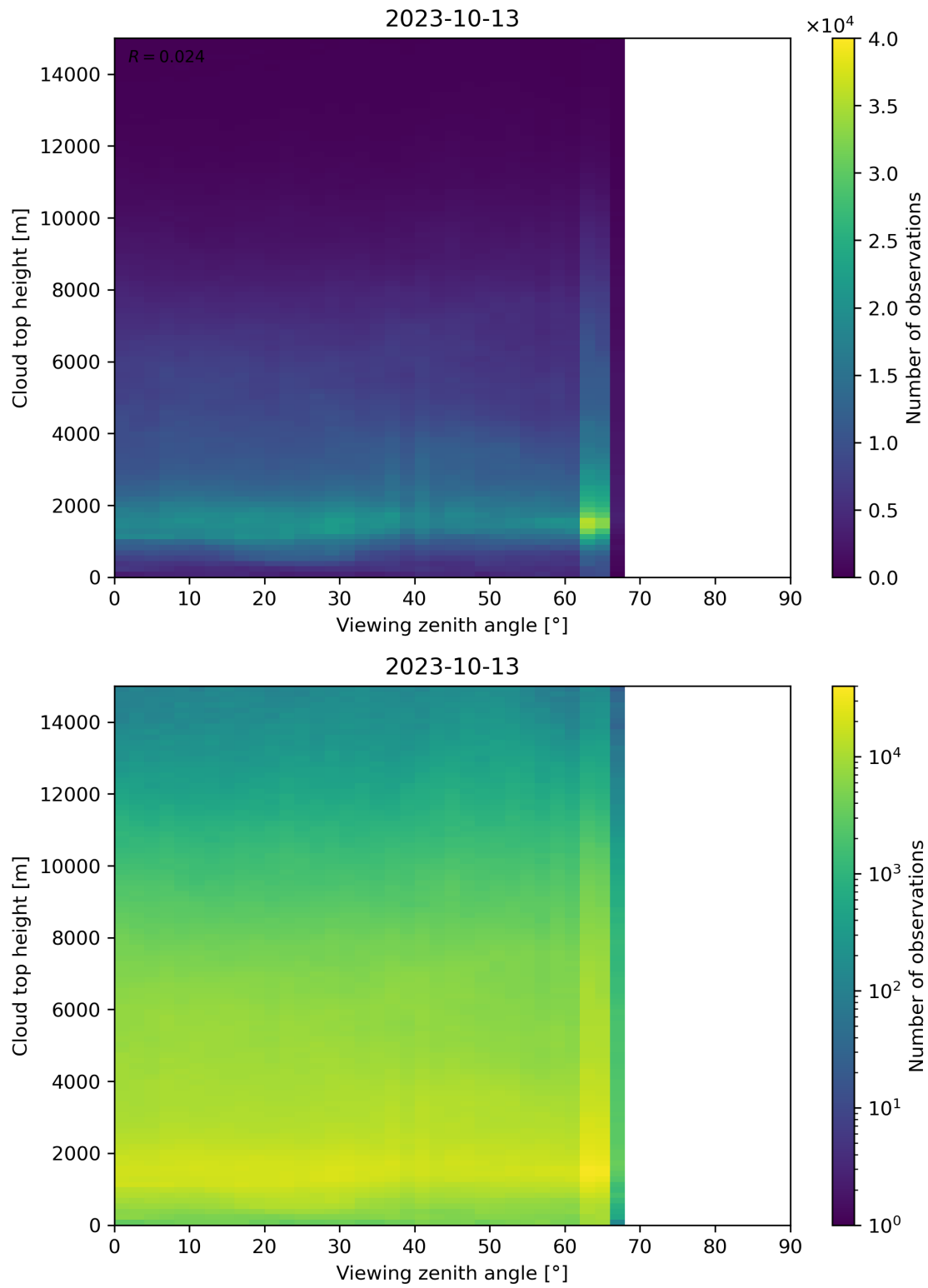
Figure 112: Scatter density plot of “Viewing zenith angle” against “Cloud top height” for 2023-10-12 to 2023-10-14.
