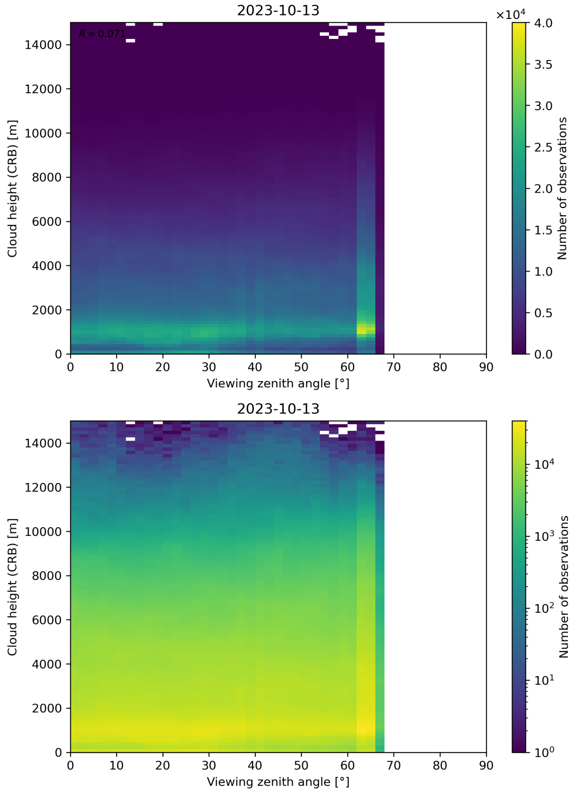
Figure 110: Scatter density plot of “Viewing zenith angle” against “Cloud height (CRB)” for 2023-10-12 to 2023-10-14.
