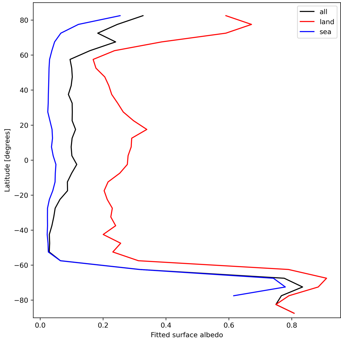
Figure 29: Zonal average of “Fitted surface albedo” for 2023-10-12 to 2023-10-14.
