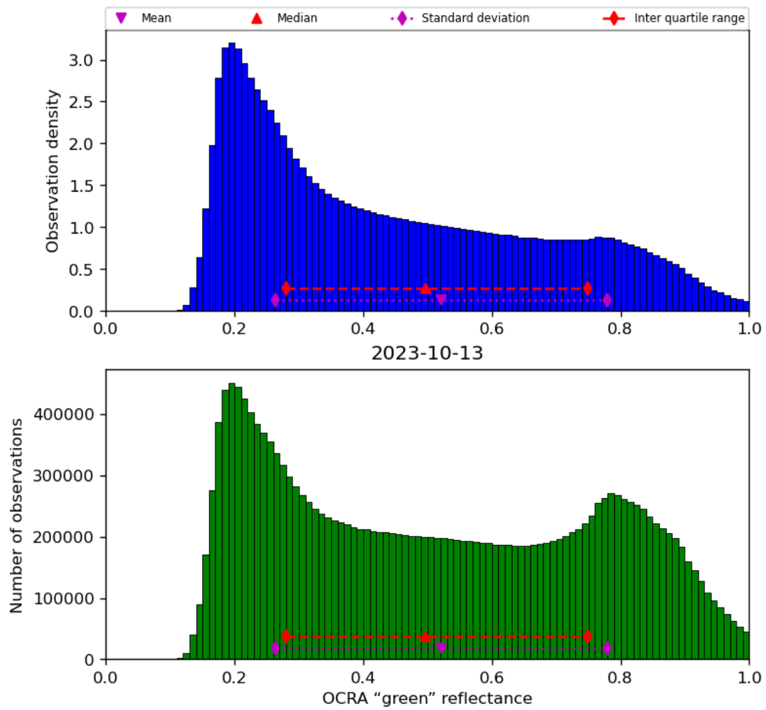
Figure 52: Histogram of “OCRA “green” reflectance” for 2023-10-12 to 2023-10-14
