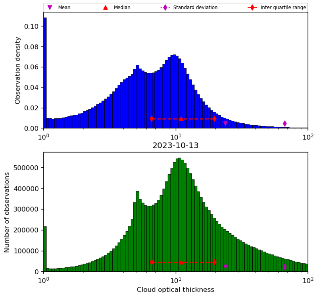
Figure 41: Histogram of “Cloud optical thickness” for 2023-10-12 to 2023-10-14
