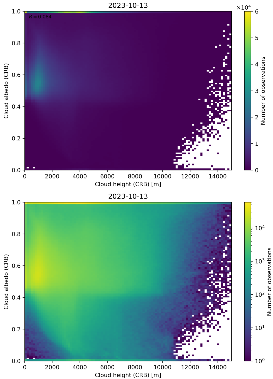
Figure 80: Scatter density plot of “Cloud height (CRB)” against “Cloud albedo (CRB)” for 2023-10-12 to 2023-10-14.
