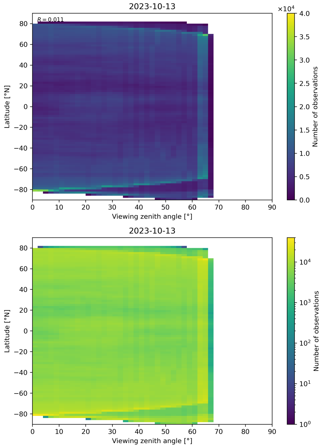
Figure 113: Scatter density plot of “Viewing zenith angle” against “Latitude” for 2023-10-12 to 2023-10-14.
