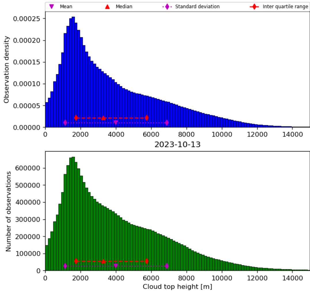
Figure 40: Histogram of “Cloud top height” for 2023-10-12 to 2023-10-14
