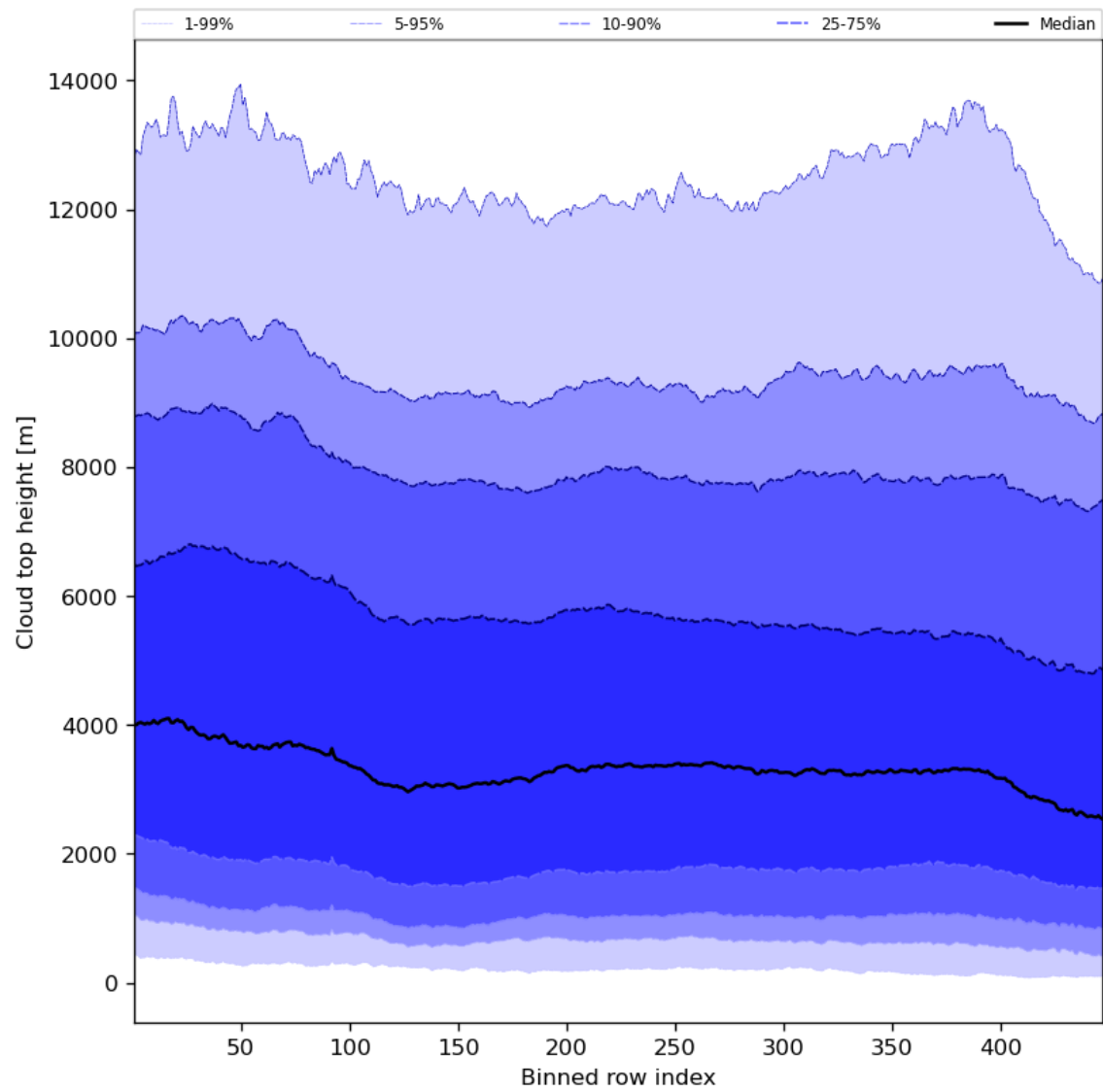
Figure 56: Along track statistics of “Cloud top height” for 2023-10-12 to 2023-10-14
