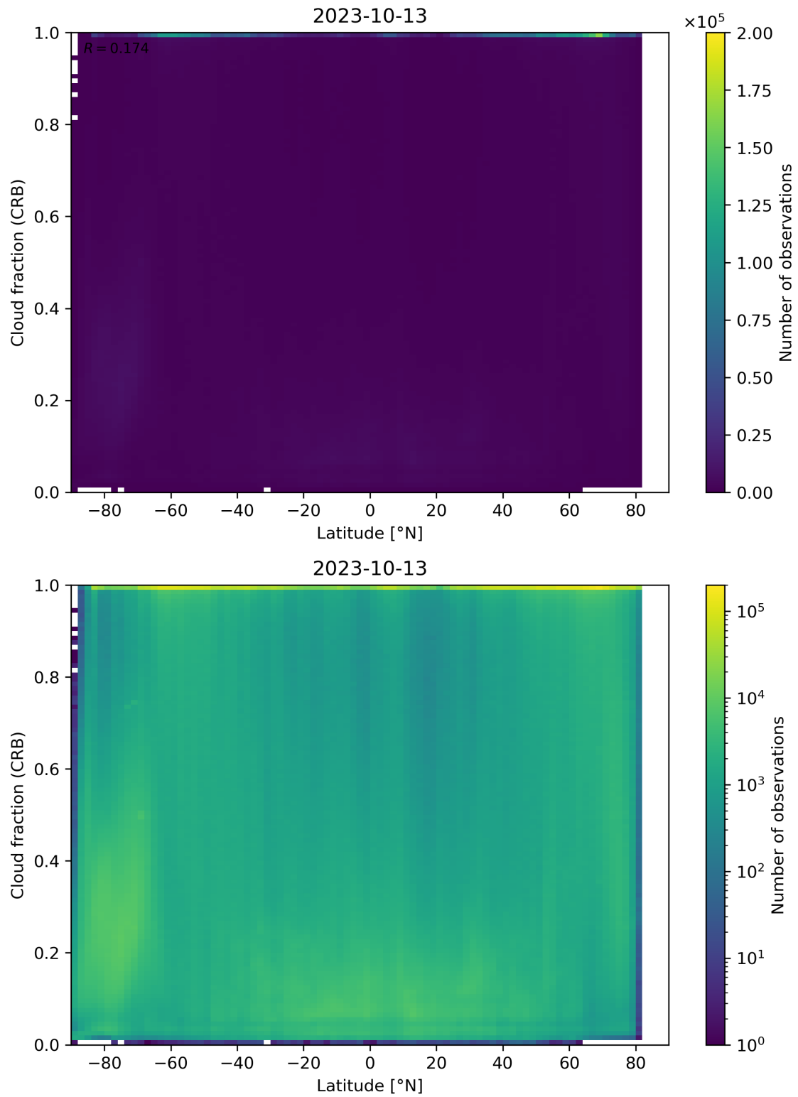
Figure 94: Scatter density plot of “Latitude” against “Cloud fraction (CRB)” for 2023-10-12 to 2023-10-14.
