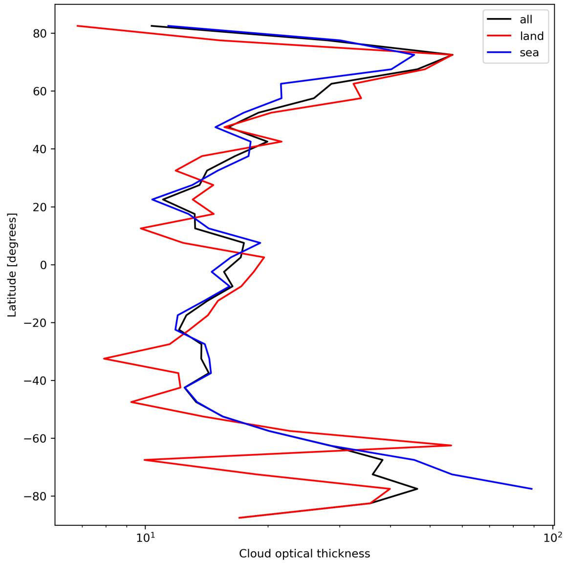
Figure 25: Zonal average of “Cloud optical thickness” for 2023-10-12 to 2023-10-14.
