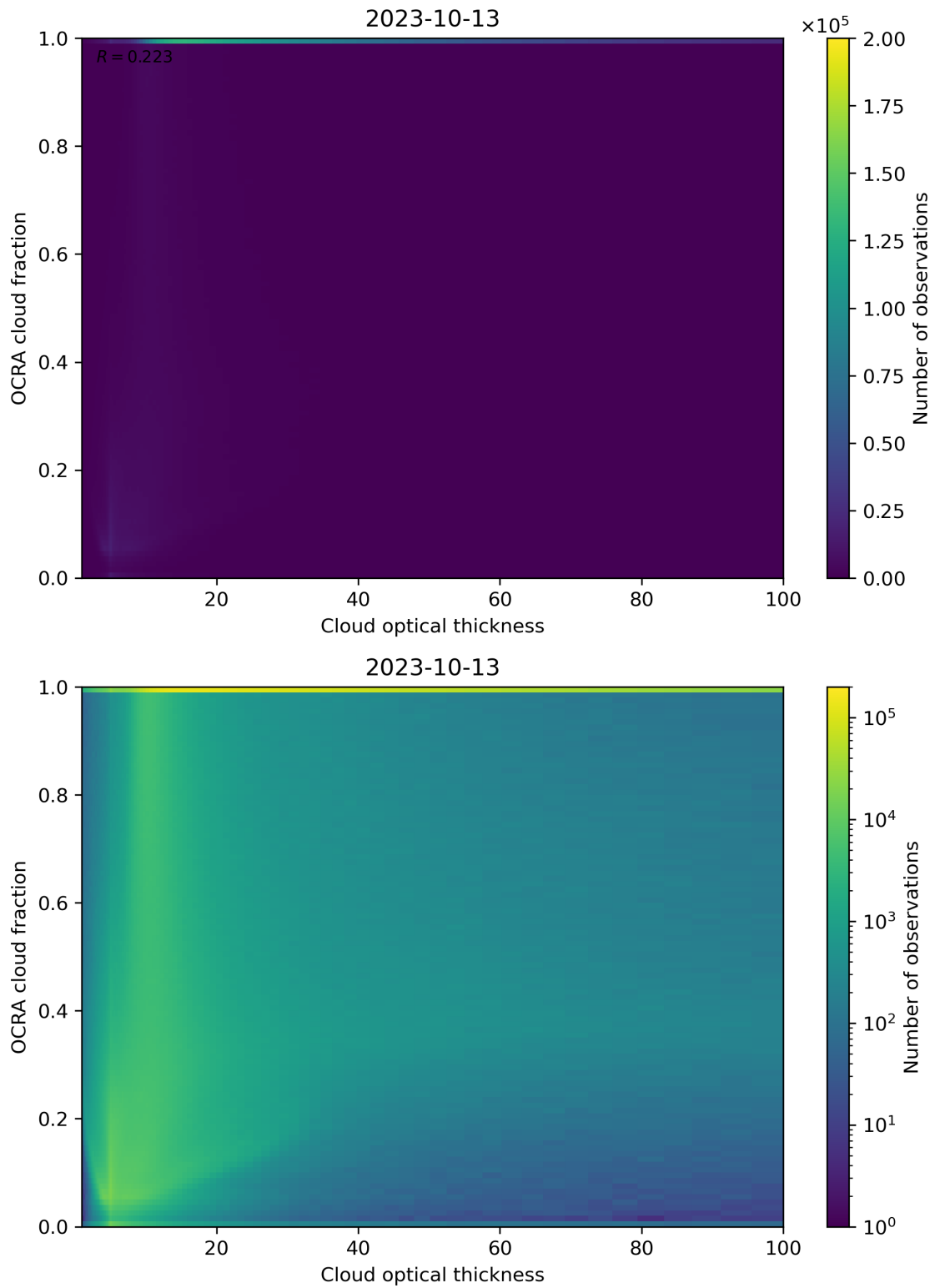
Figure 83: Scatter density plot of “Cloud optical thickness” against “OCRA cloud fraction” for 2023-10-12 to 2023-10-14.
