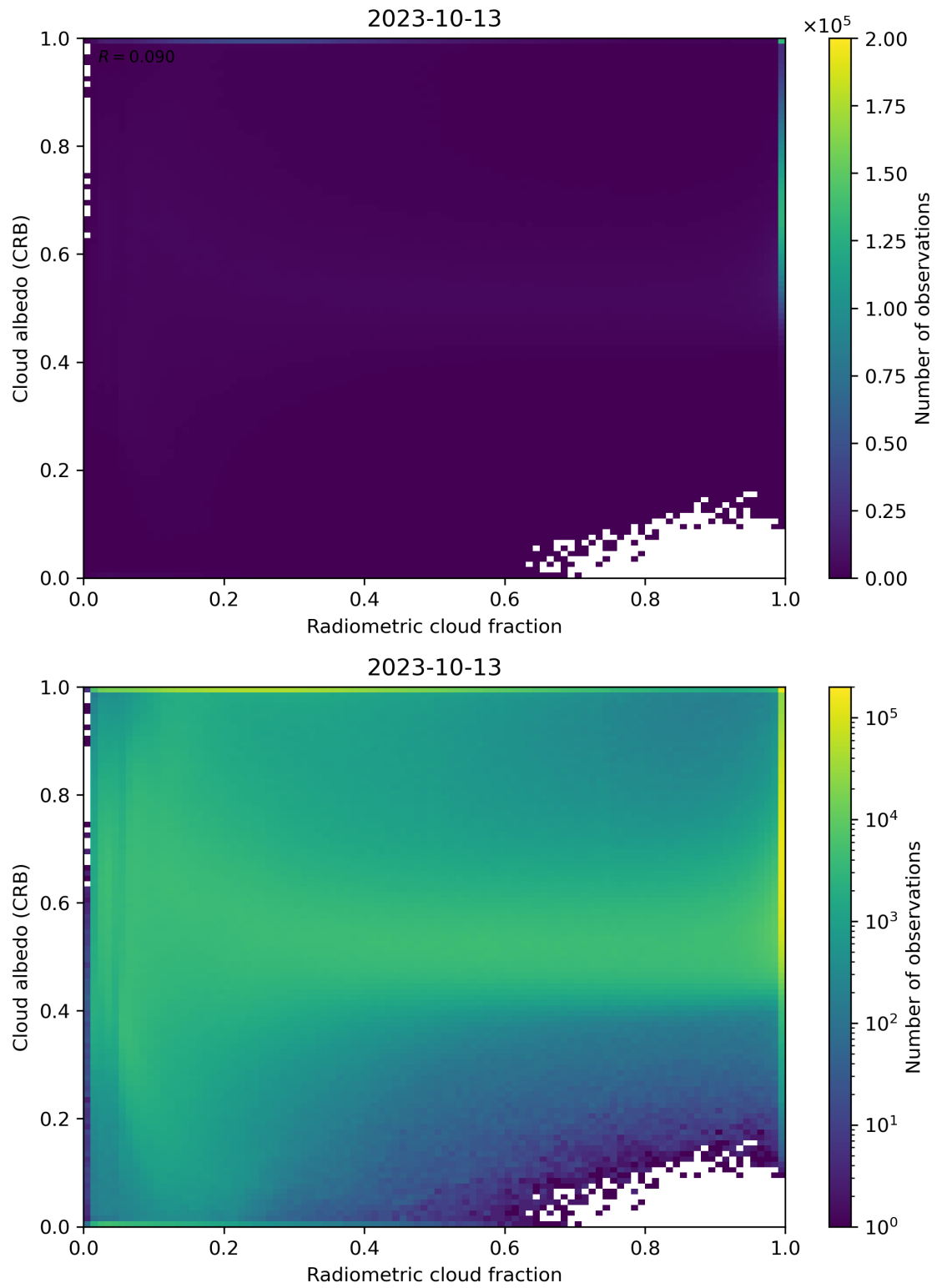
Figure 71: Scatter density plot of “Radiometric cloud fraction” against “Cloud albedo (CRB)” for 2023-10-12 to 2023-10-14.
