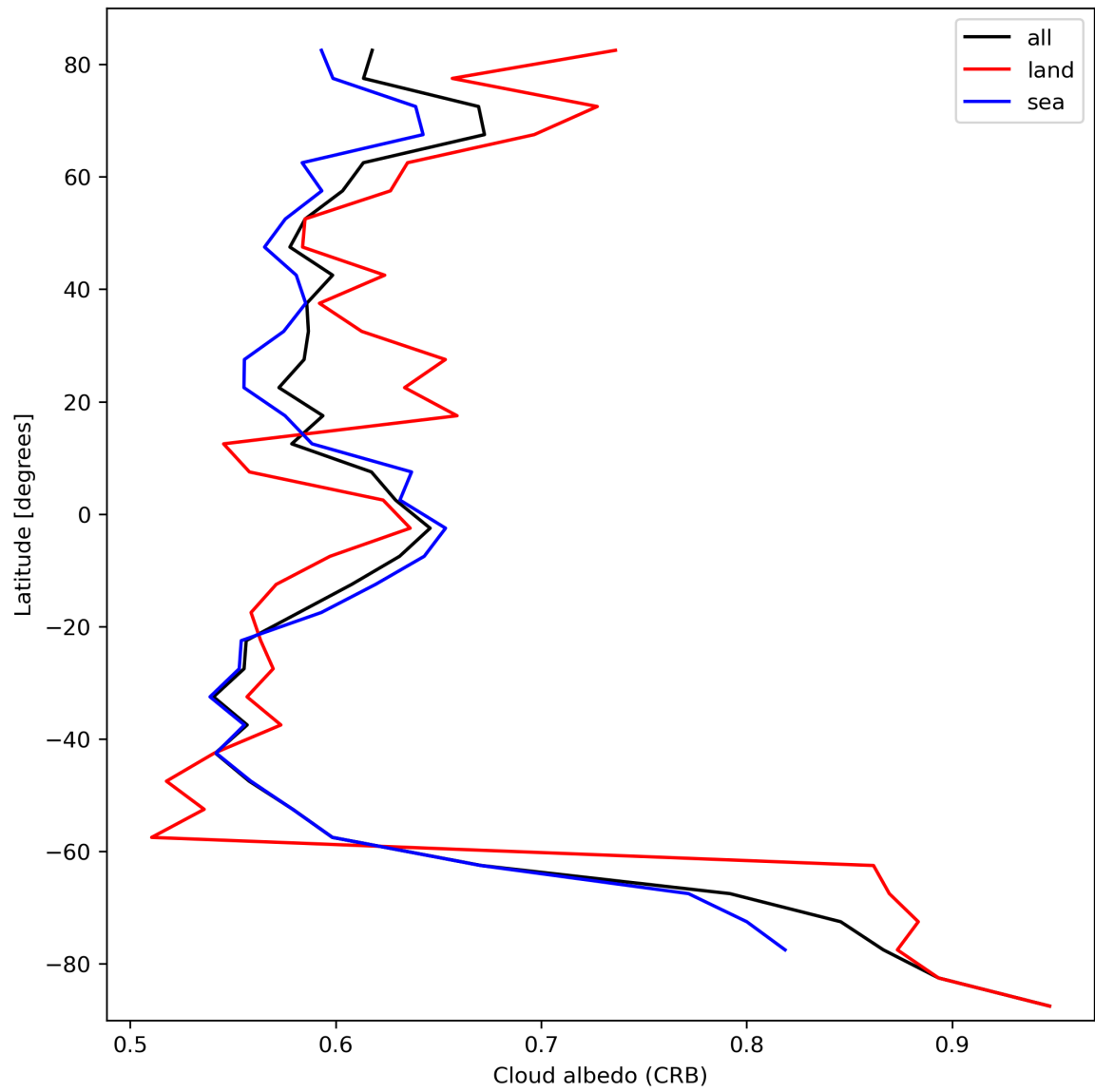
Figure 28: Zonal average of “Cloud albedo (CRB)” for 2023-10-12 to 2023-10-14.
