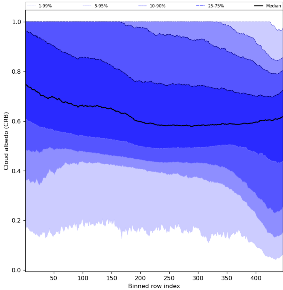
Figure 60: Along track statistics of “Cloud albedo (CRB)” for 2023-10-12 to 2023-10-14
