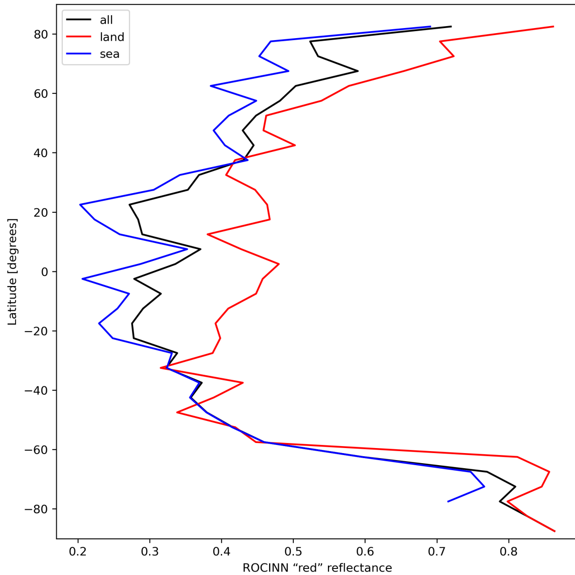
Figure 37: Zonal average of “ROCINN “red” reflectance” for 2023-10-12 to 2023-10-14.
