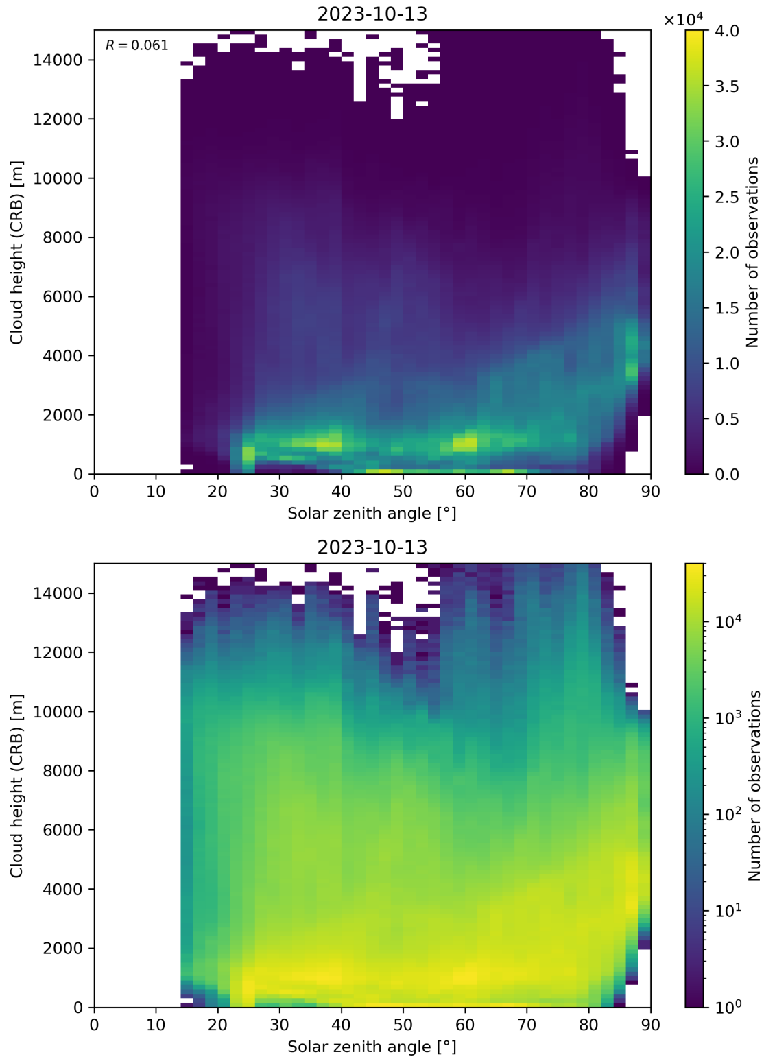
Figure 102: Scatter density plot of “Solar zenith angle” against “Cloud height (CRB)” for 2023-10-12 to 2023-10-14.
