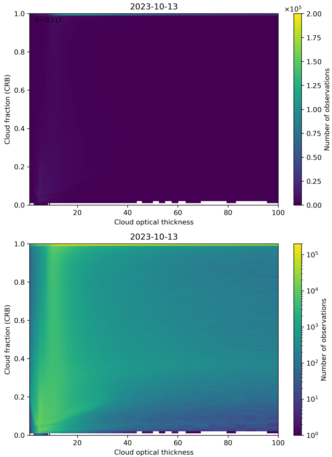
Figure 84: Scatter density plot of “Cloud optical thickness” against “Cloud fraction (CRB)” for 2023-10-12 to 2023-10-14.
