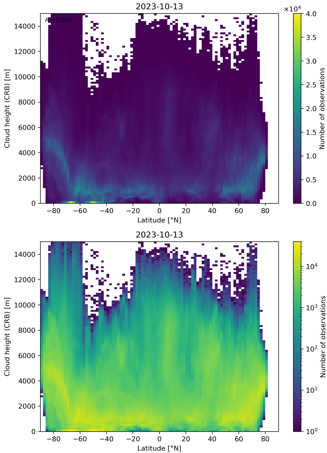
Figure 95: Scatter density plot of “Latitude” against “Cloud height (CRB)” for 2023-10-12 to 2023-10-14.
