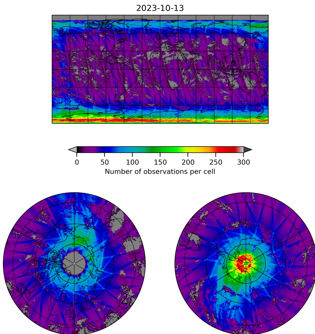
Figure 21: Map of the number of observations for 2023-10-12 to 2023-10-14
