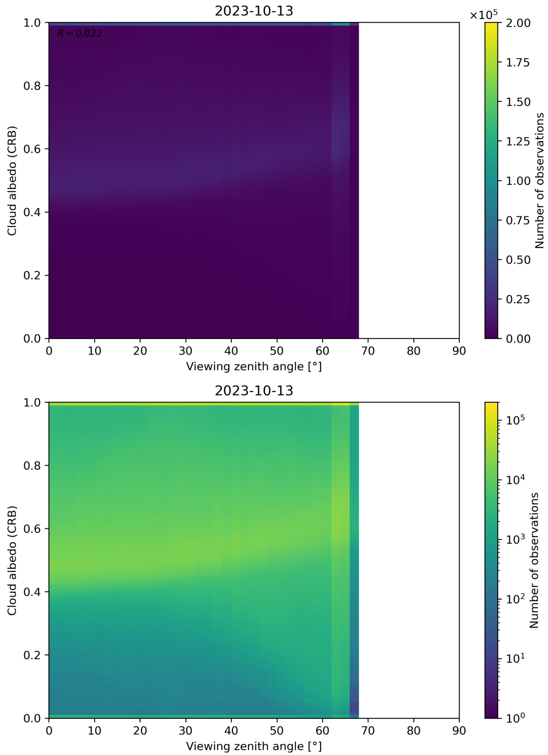
Figure 106: Scatter density plot of “Viewing zenith angle” against “Cloud albedo (CRB)” for 2023-10-12 to 2023-10-14.
