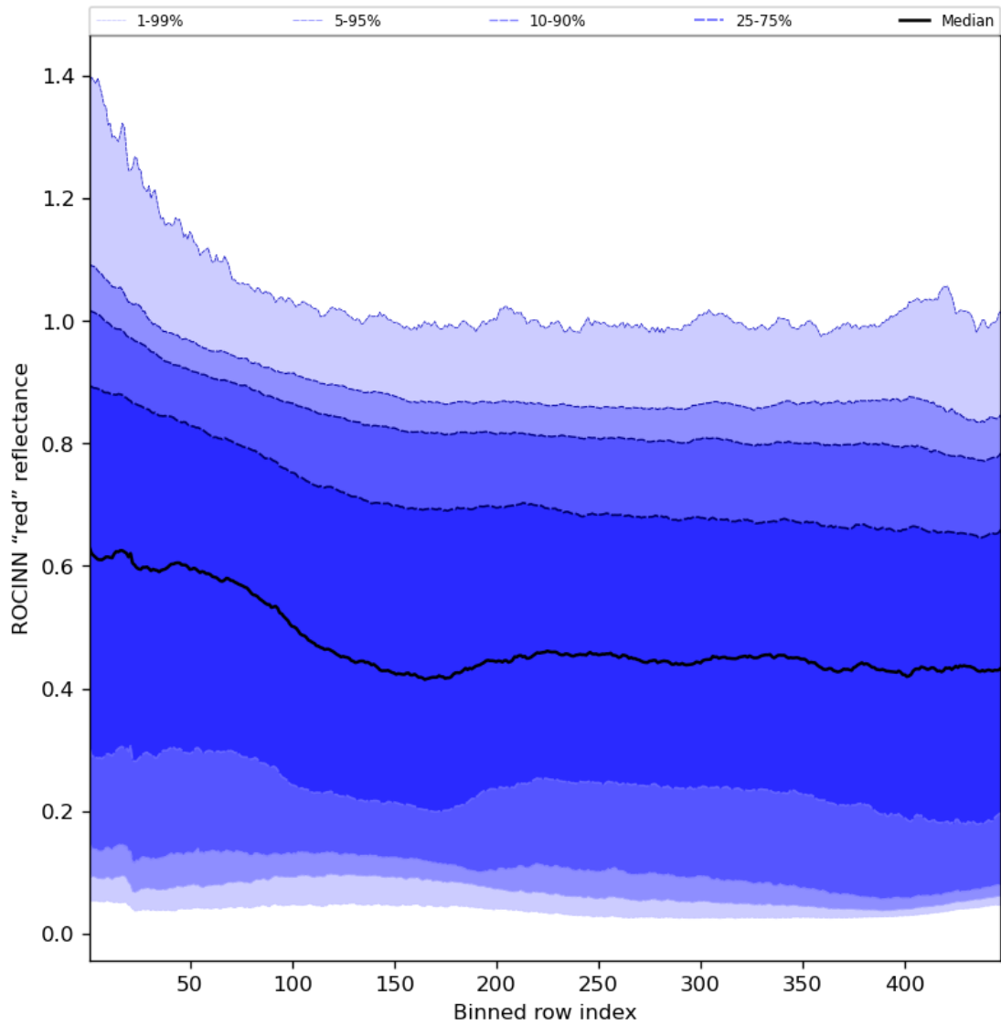
Figure 69: Along track statistics of “ROCINN “red” reflectance” for 2023-10-12 to 2023-10-14
