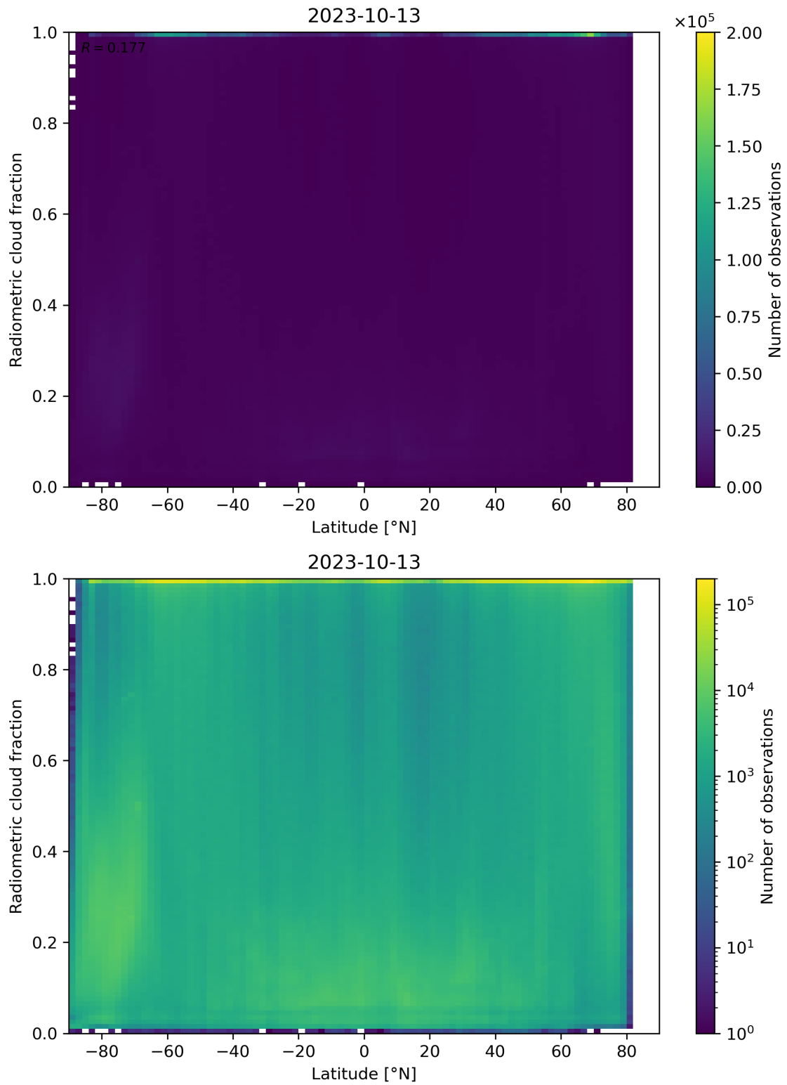
Figure 92: Scatter density plot of “Latitude” against “Radiometric cloud fraction” for 2023-10-12 to 2023-10-14.
