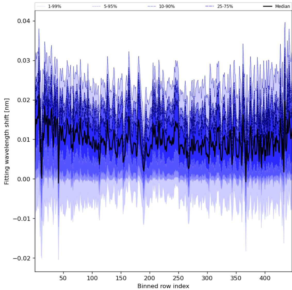
Figure 65: Along track statistics of “Fitting wavelength shift” for 2023-10-12 to 2023-10-14
