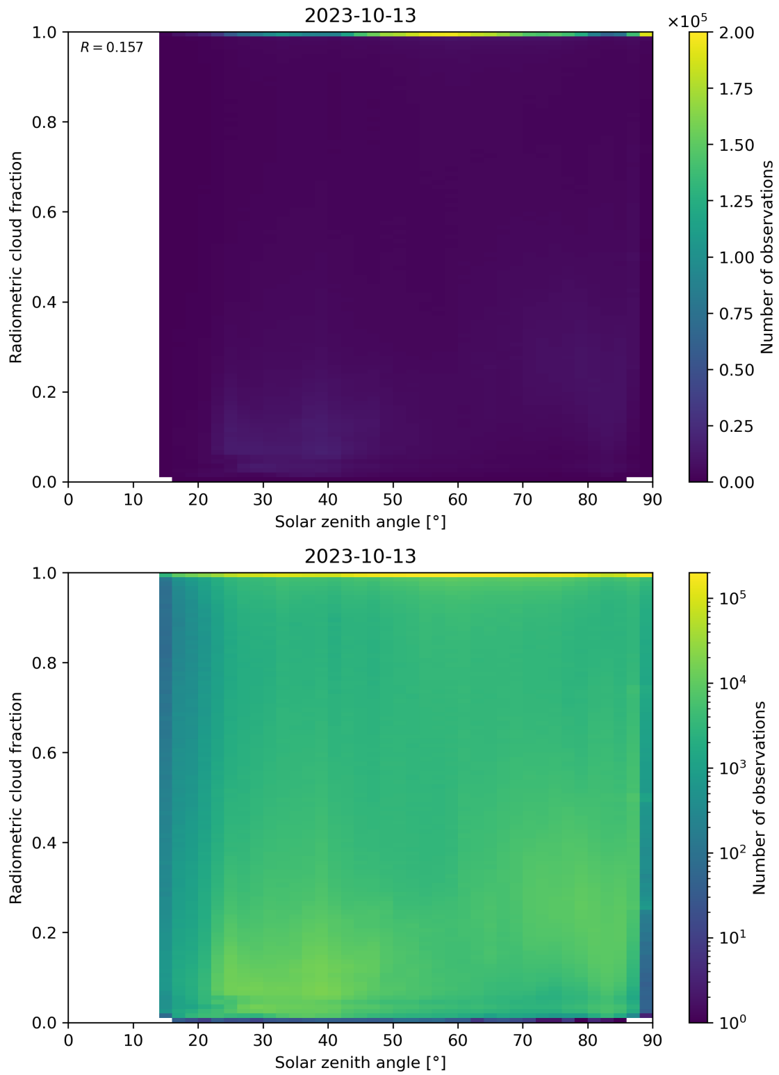
Figure 99: Scatter density plot of “Solar zenith angle” against “Radiometric cloud fraction” for 2023-10-12 to 2023-10-14.
