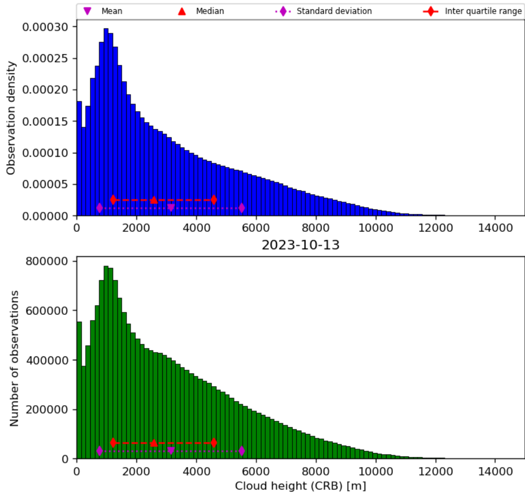
Figure 43: Histogram of “Cloud height (CRB)” for 2023-10-12 to 2023-10-14
