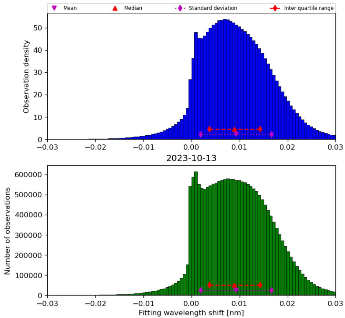
Figure 49: Histogram of “Fitting wavelength shift” for 2023-10-12 to 2023-10-14
