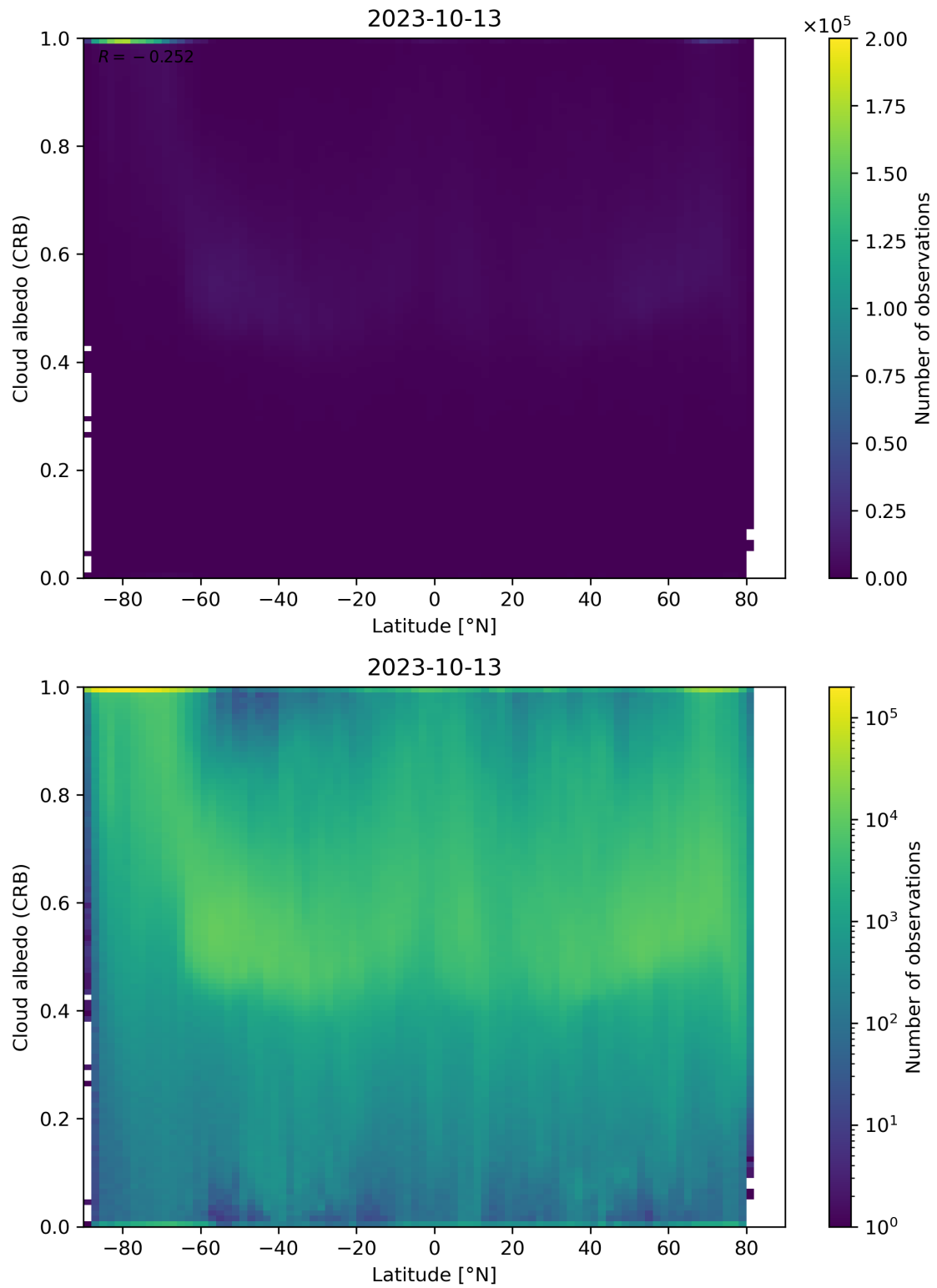
Figure 91: Scatter density plot of “Latitude” against “Cloud albedo (CRB)” for 2023-10-12 to 2023-10-14.
