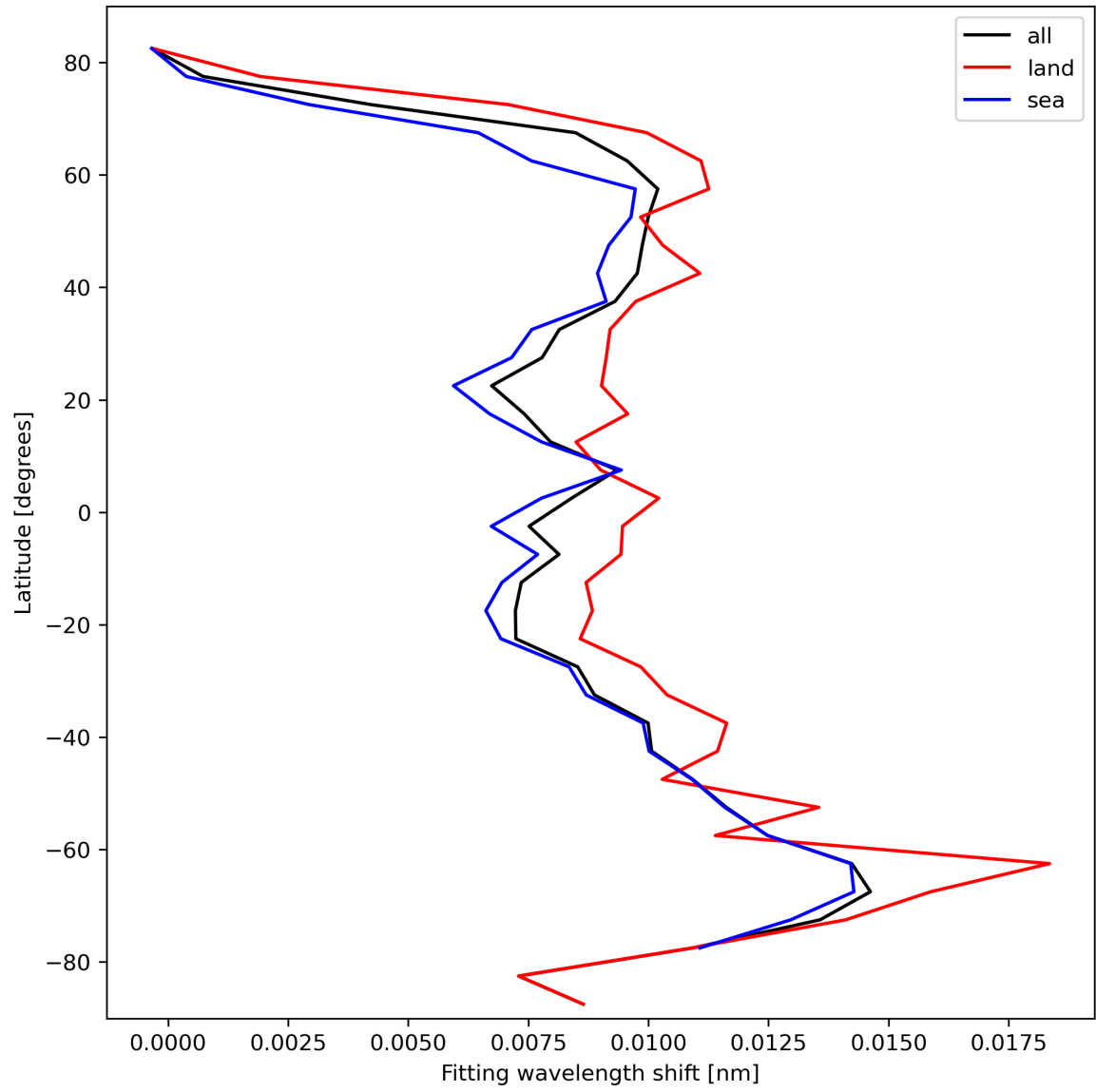
Figure 33: Zonal average of “Fitting wavelength shift” for 2023-10-12 to 2023-10-14.
