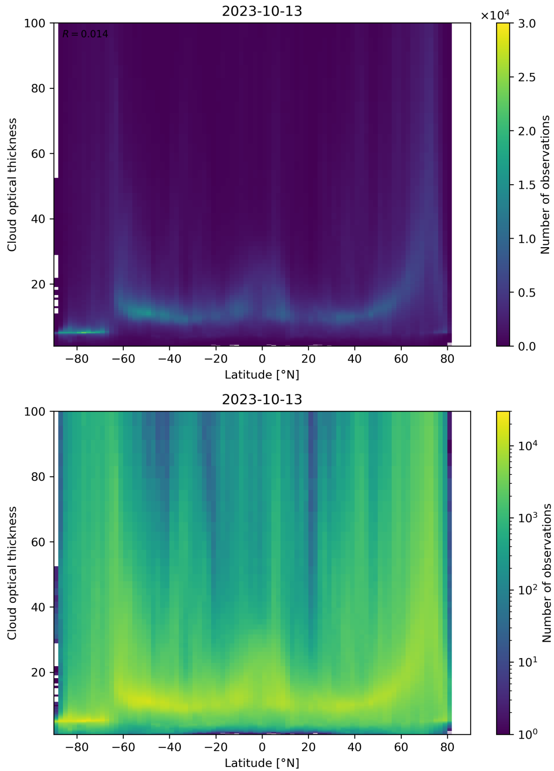
Figure 96: Scatter density plot of “Latitude” against “Cloud optical thickness” for 2023-10-12 to 2023-10-14.
