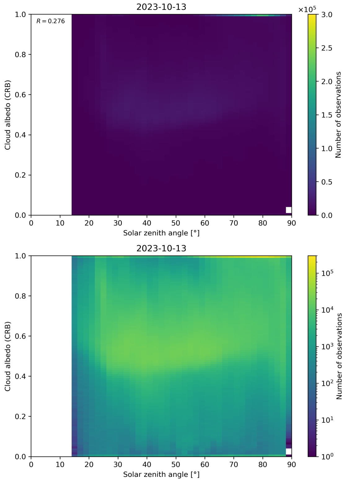
Figure 98: Scatter density plot of “Solar zenith angle” against “Cloud albedo (CRB)” for 2023-10-12 to 2023-10-14.
