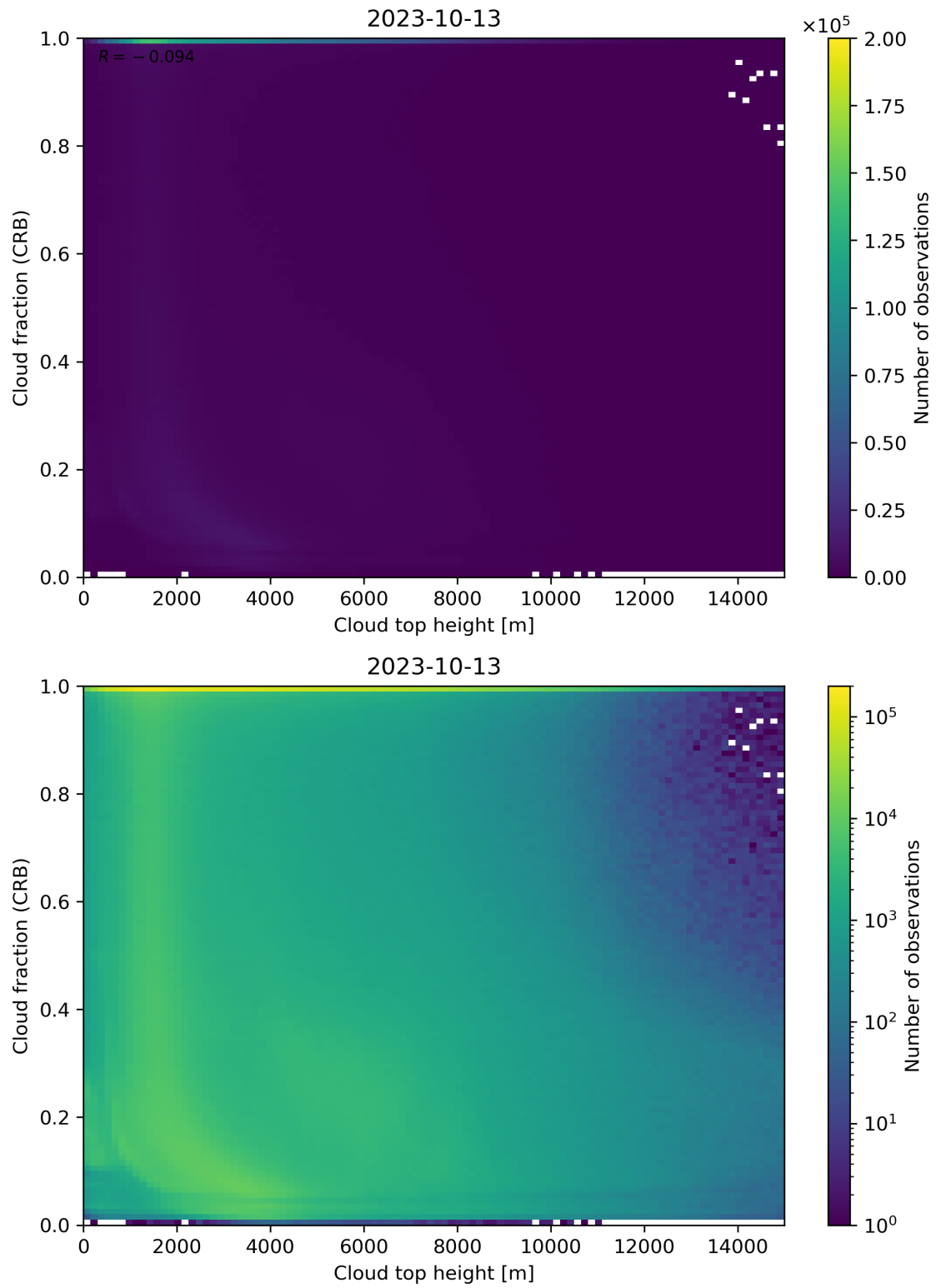
Figure 88: Scatter density plot of “Cloud top height” against “Cloud fraction (CRB)” for 2023-10-12 to 2023-10-14.
