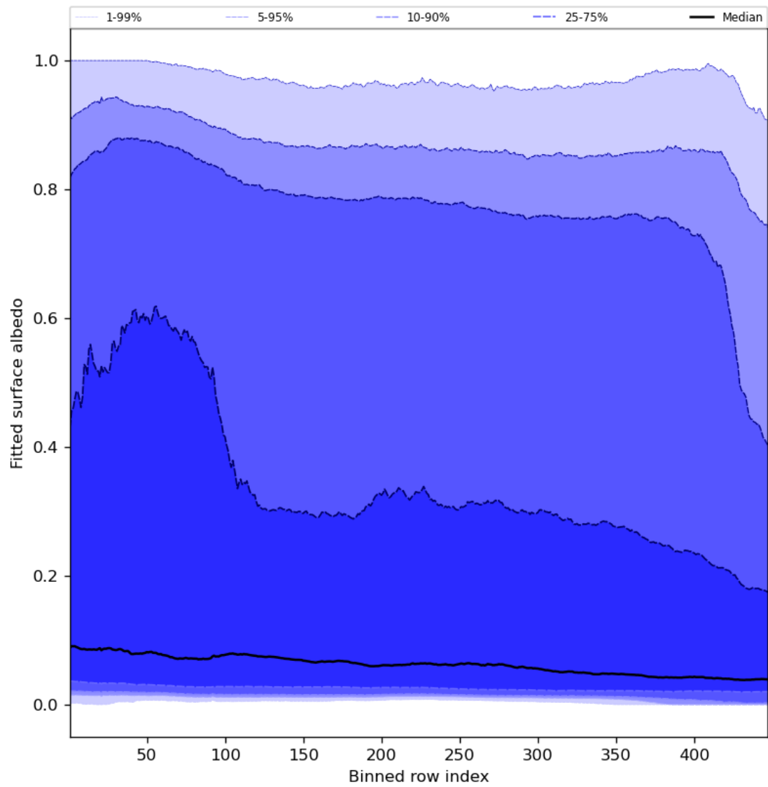
Figure 61: Along track statistics of “Fitted surface albedo” for 2023-10-12 to 2023-10-14
