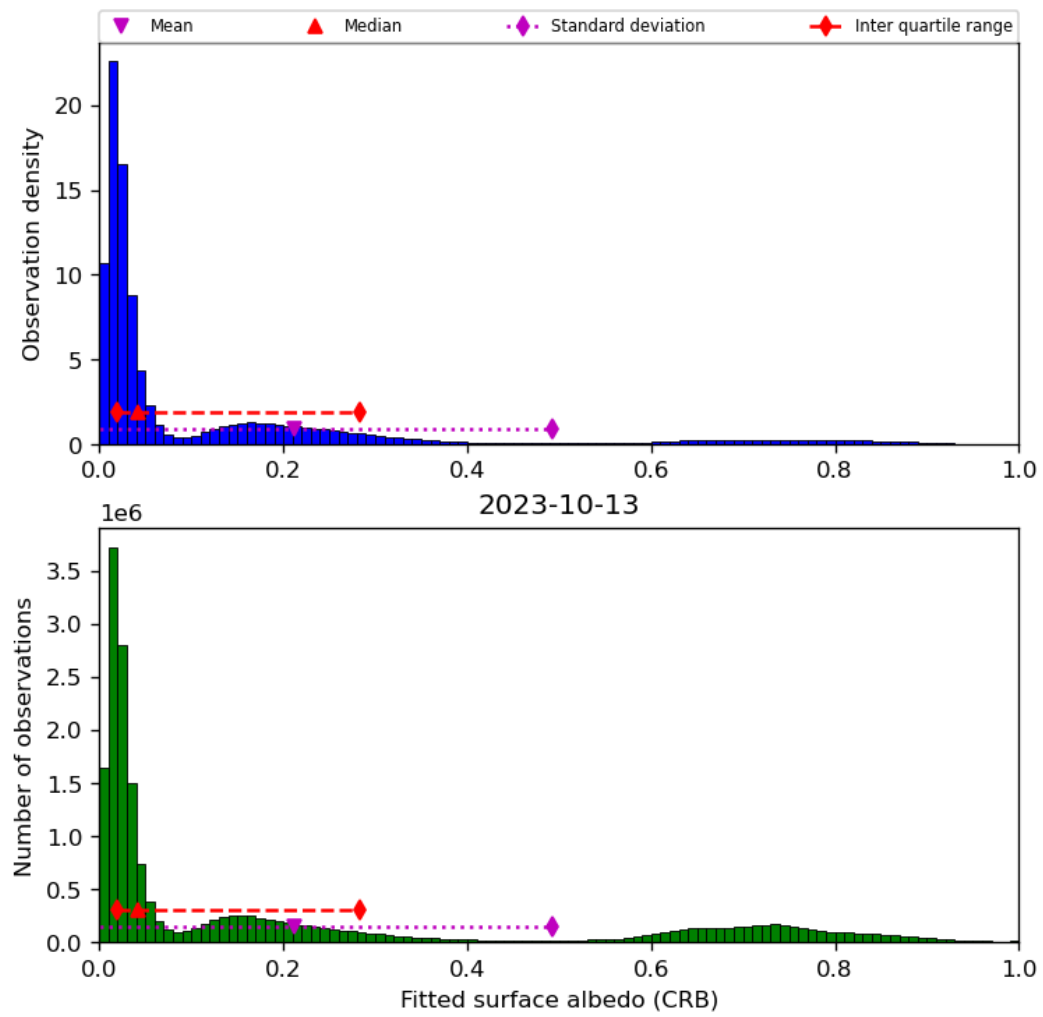
Figure 46: Histogram of “Fitted surface albedo (CRB)” for 2023-10-12 to 2023-10-14
