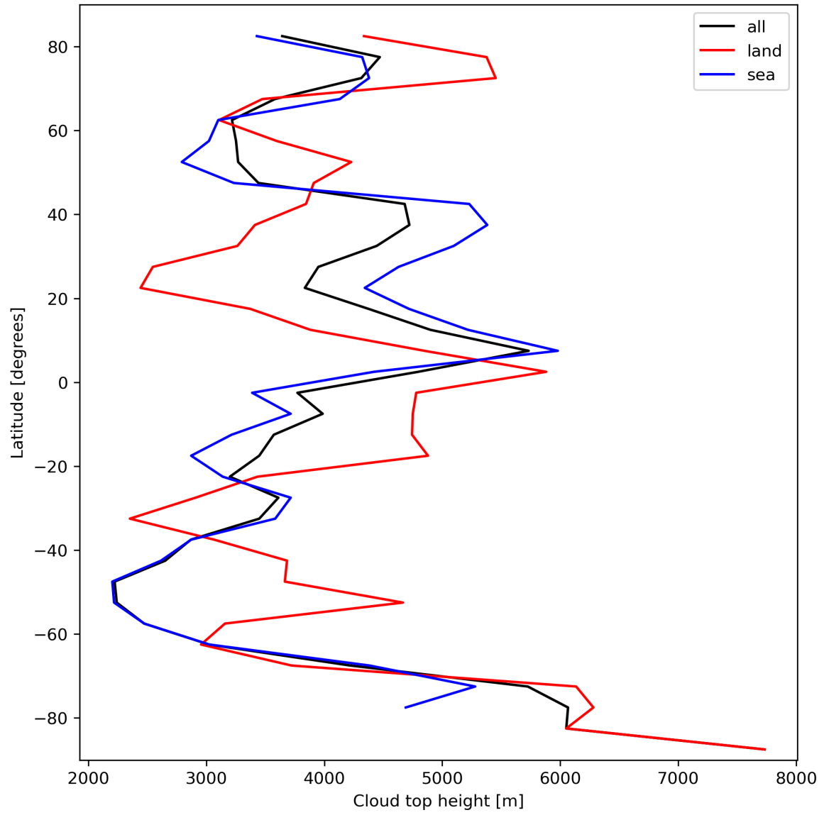
Figure 24: Zonal average of “Cloud top height” for 2023-10-12 to 2023-10-14.
