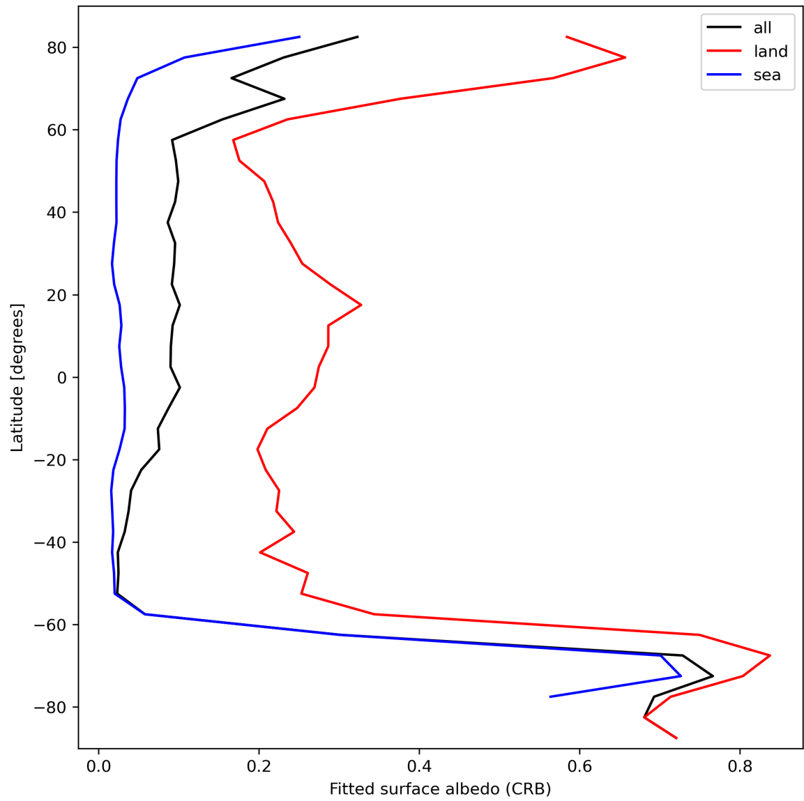
Figure 30: Zonal average of “Fitted surface albedo (CRB)” for 2023-10-12 to 2023-10-14.
