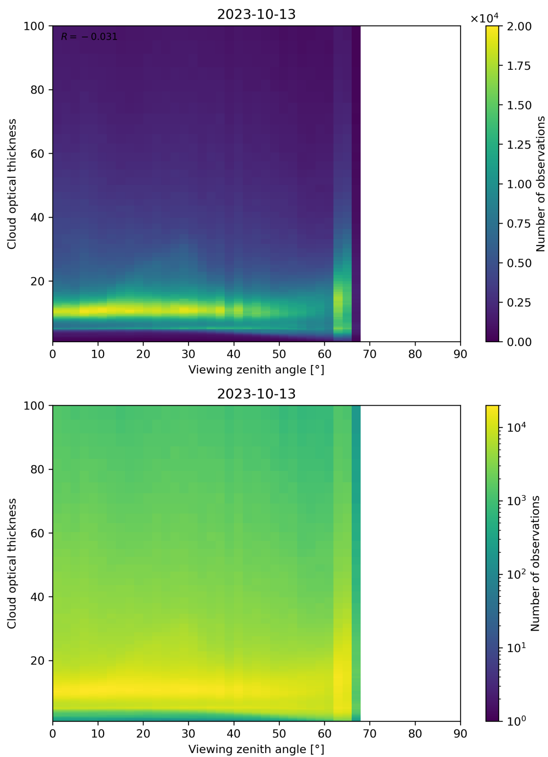
Figure 111: Scatter density plot of “Viewing zenith angle” against “Cloud optical thickness” for 2023-10-12 to 2023-10-14.
