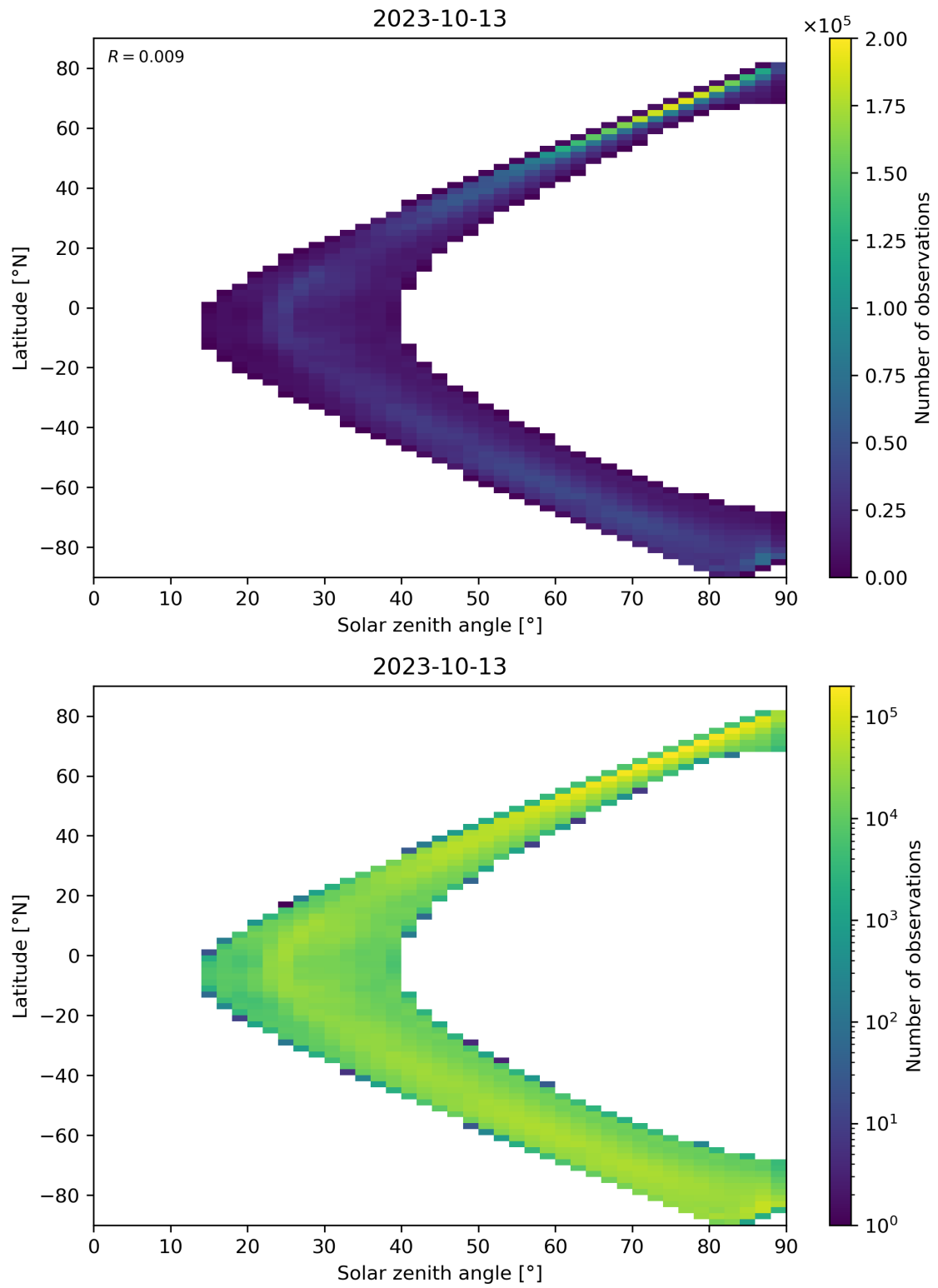
Figure 105: Scatter density plot of “Solar zenith angle” against “Latitude” for 2023-10-12 to 2023-10-14.
