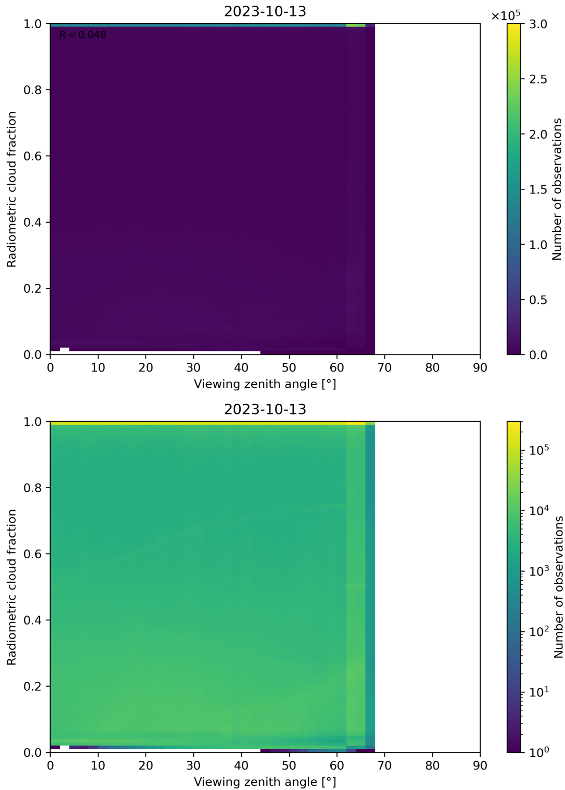
Figure 107: Scatter density plot of “Viewing zenith angle” against “Radiometric cloud fraction” for 2023-10-12 to 2023-10-14.
