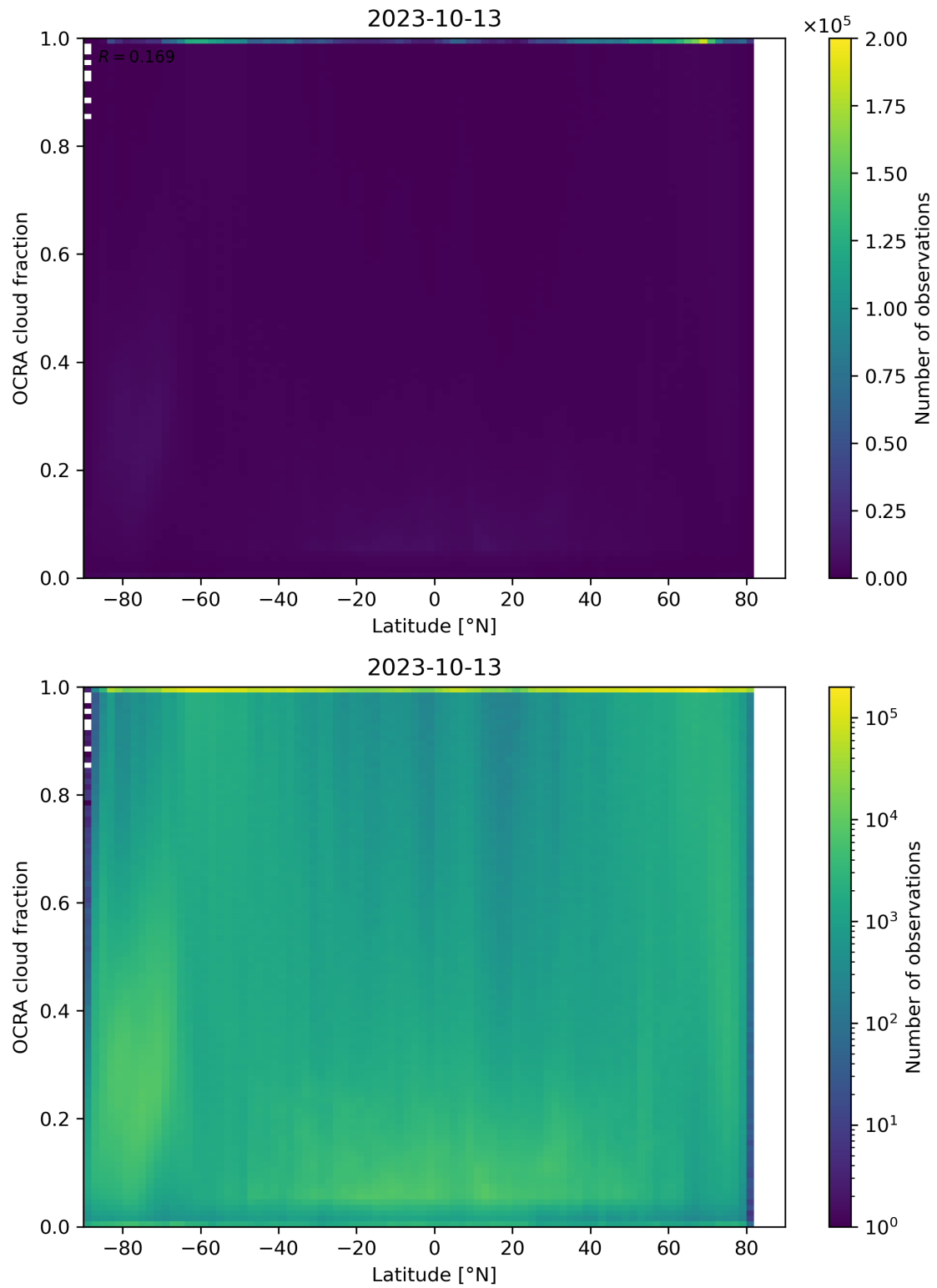
Figure 93: Scatter density plot of “Latitude” against “OCRA cloud fraction” for 2023-10-12 to 2023-10-14.
