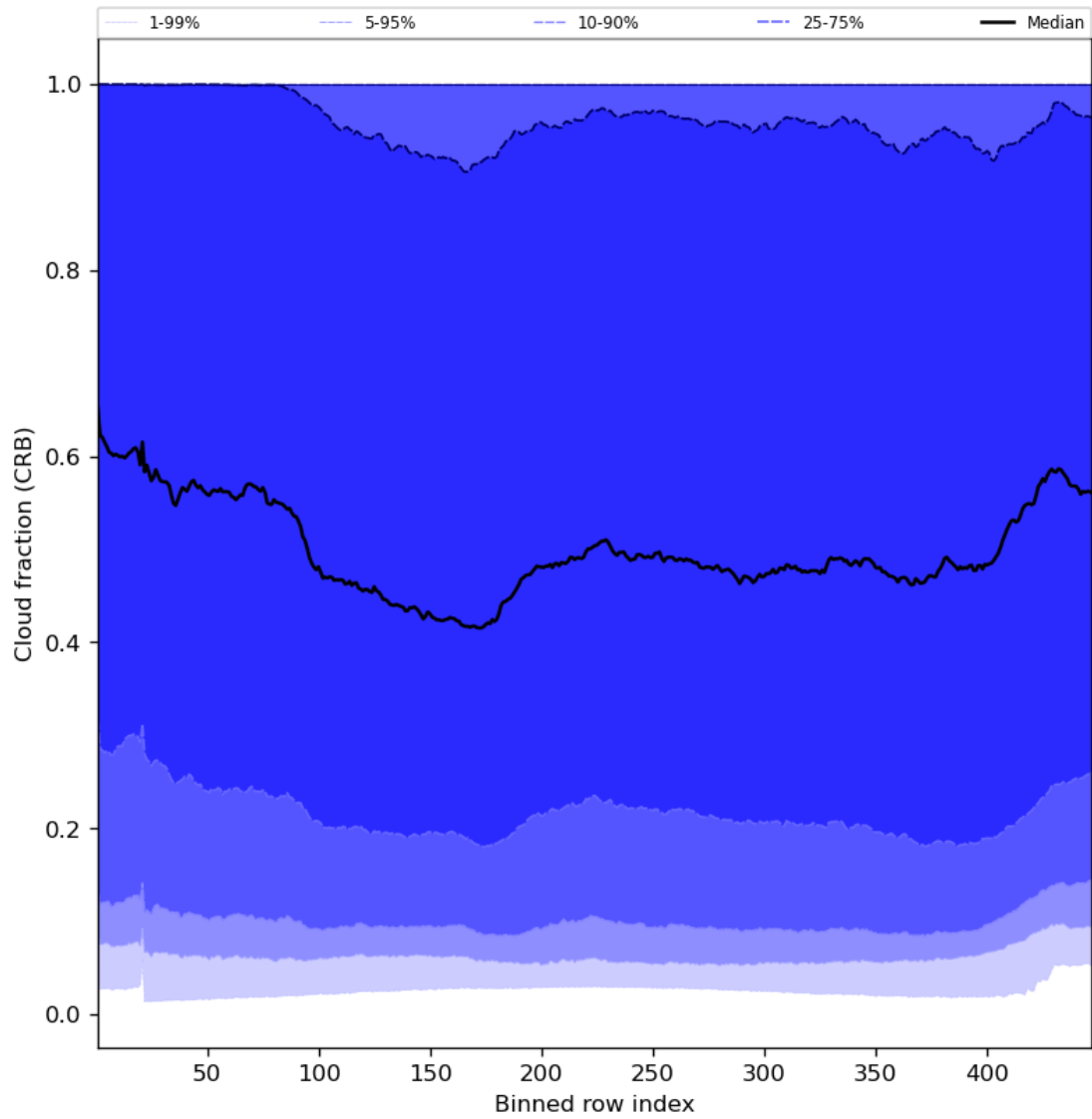
Figure 58: Along track statistics of “Cloud fraction (CRB)” for 2023-10-12 to 2023-10-14
