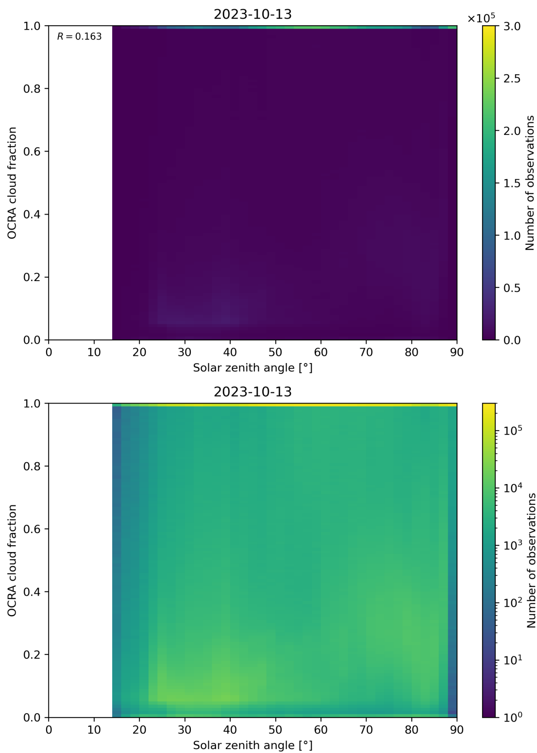
Figure 100: Scatter density plot of “Solar zenith angle” against “OCRA cloud fraction” for 2023-10-12 to 2023-10-14.
