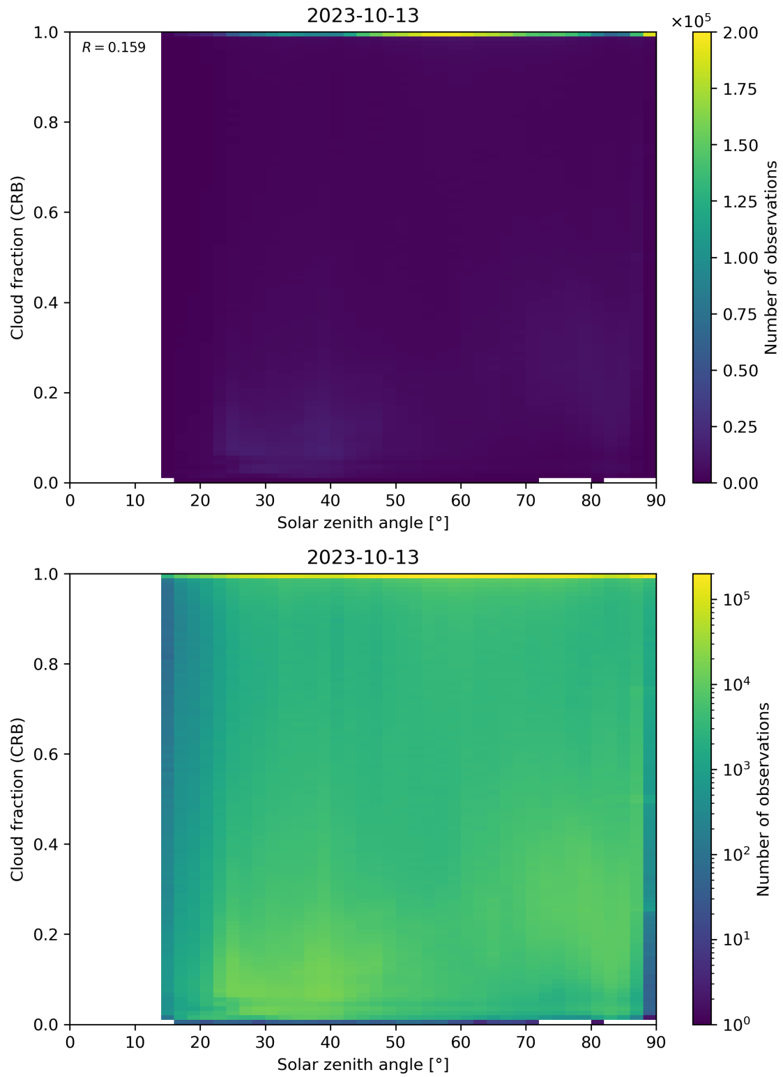
Figure 101: Scatter density plot of “Solar zenith angle” against “Cloud fraction (CRB)” for 2023-10-12 to 2023-10-14.
