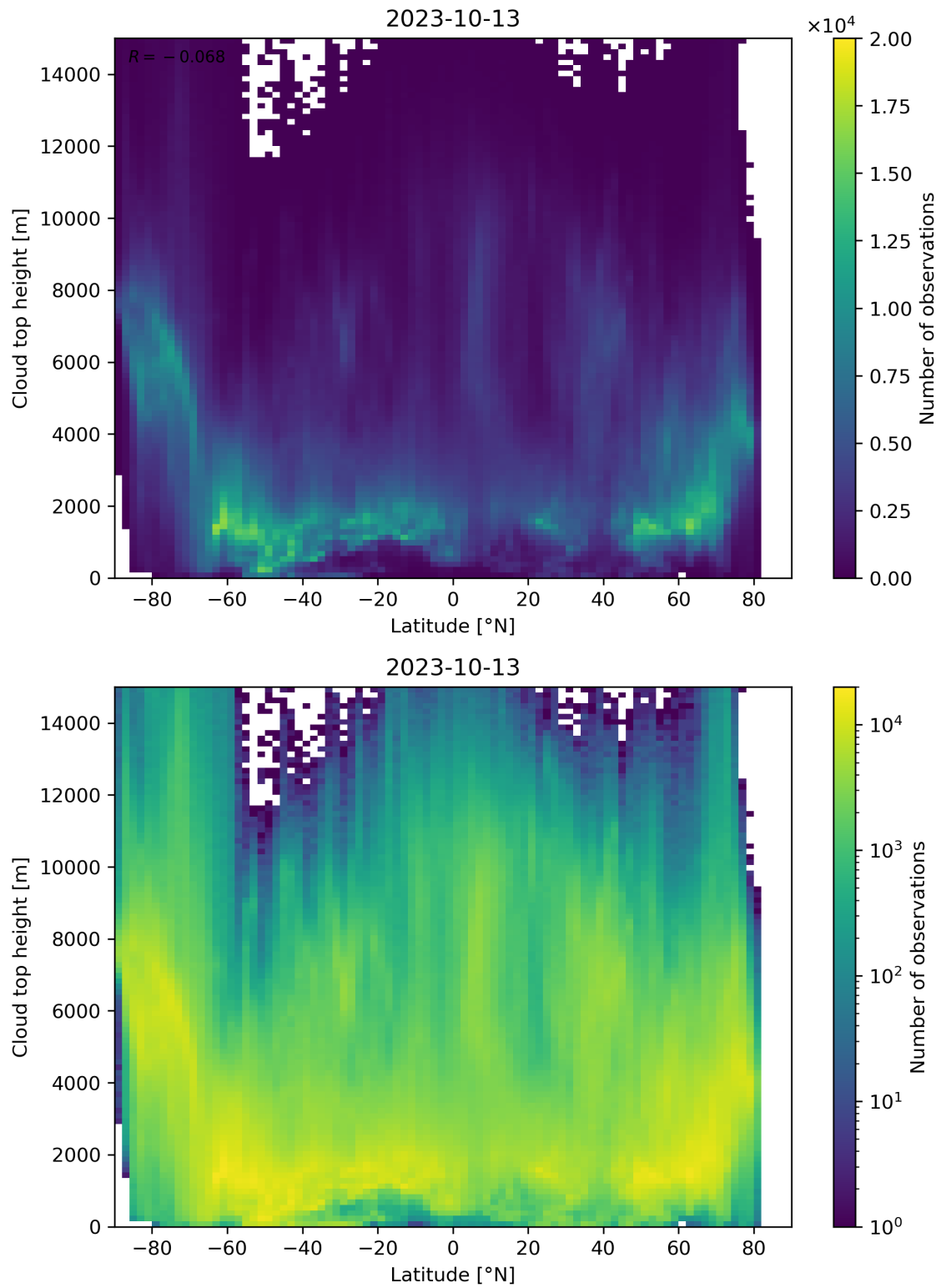
Figure 97: Scatter density plot of “Latitude” against “Cloud top height” for 2023-10-12 to 2023-10-14.
