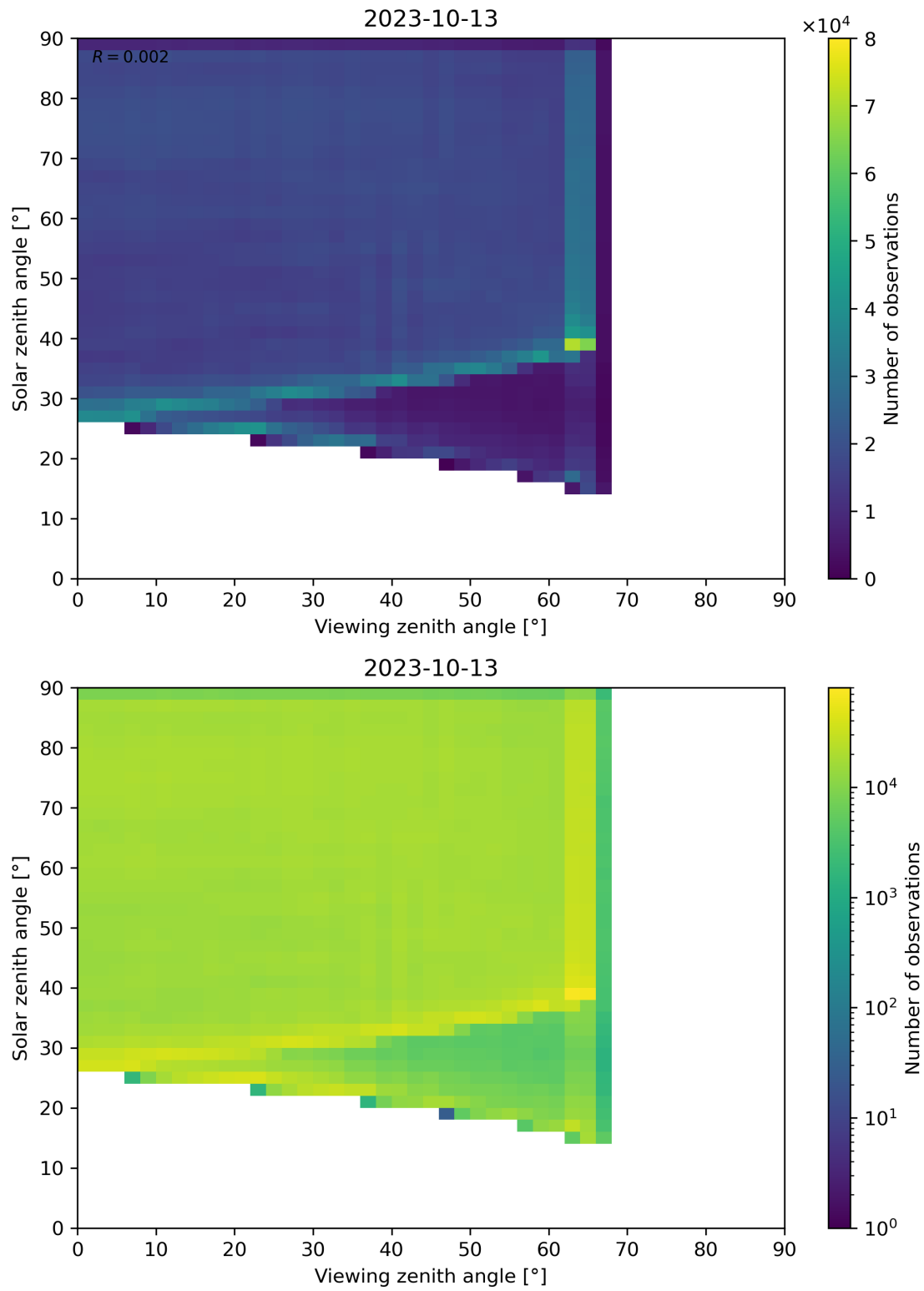
Figure 114: Scatter density plot of “Viewing zenith angle” against “Solar zenith angle” for 2023-10-12 to 2023-10-14.
