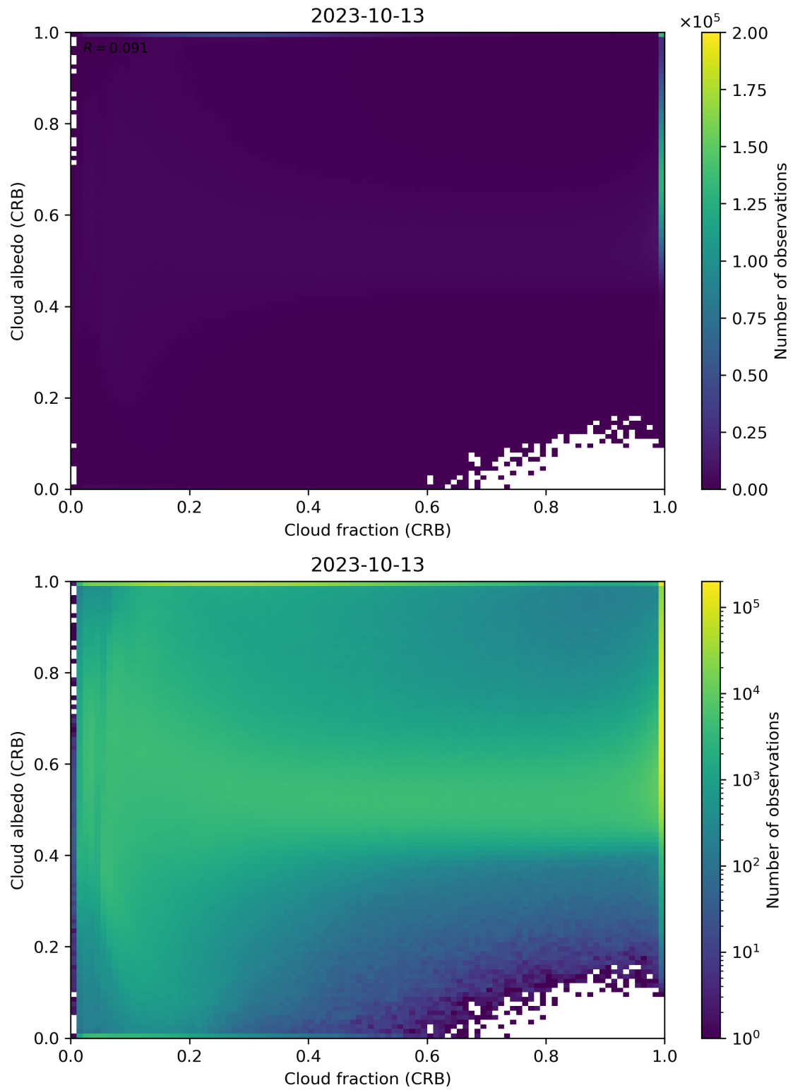
Figure 77: Scatter density plot of “Cloud fraction (CRB)” against “Cloud albedo (CRB)” for 2023-10-12 to 2023-10-14.
