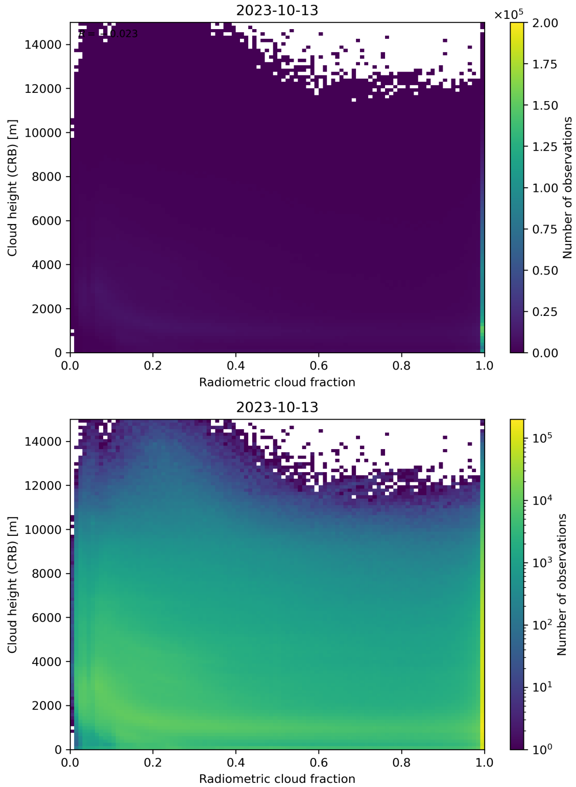
Figure 74: Scatter density plot of “Radiometric cloud fraction” against “Cloud height (CRB)” for 2023-10-12 to 2023-10-14.
