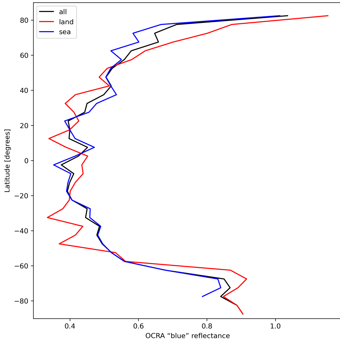
Figure 35: Zonal average of “OCRA “blue” reflectance” for 2023-10-12 to 2023-10-14.
