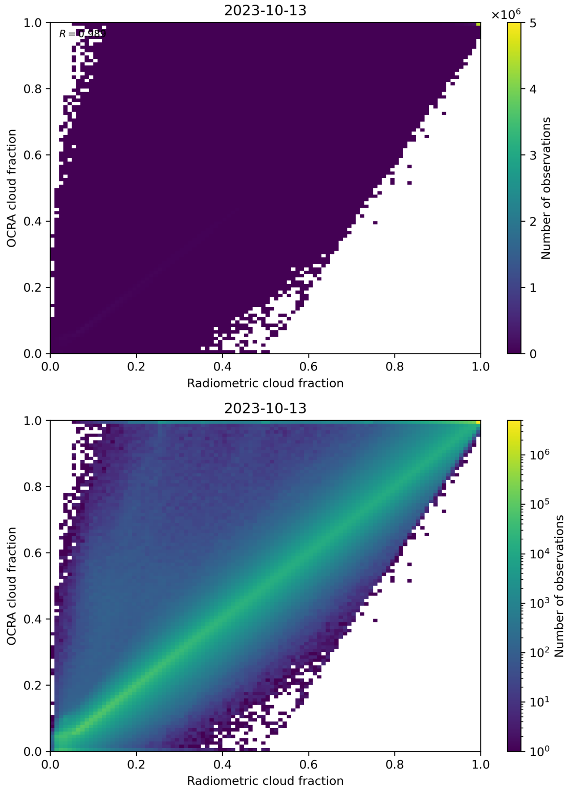
Figure 72: Scatter density plot of “Radiometric cloud fraction” against “OCRA cloud fraction” for 2023-10-12 to 2023-10-14.
