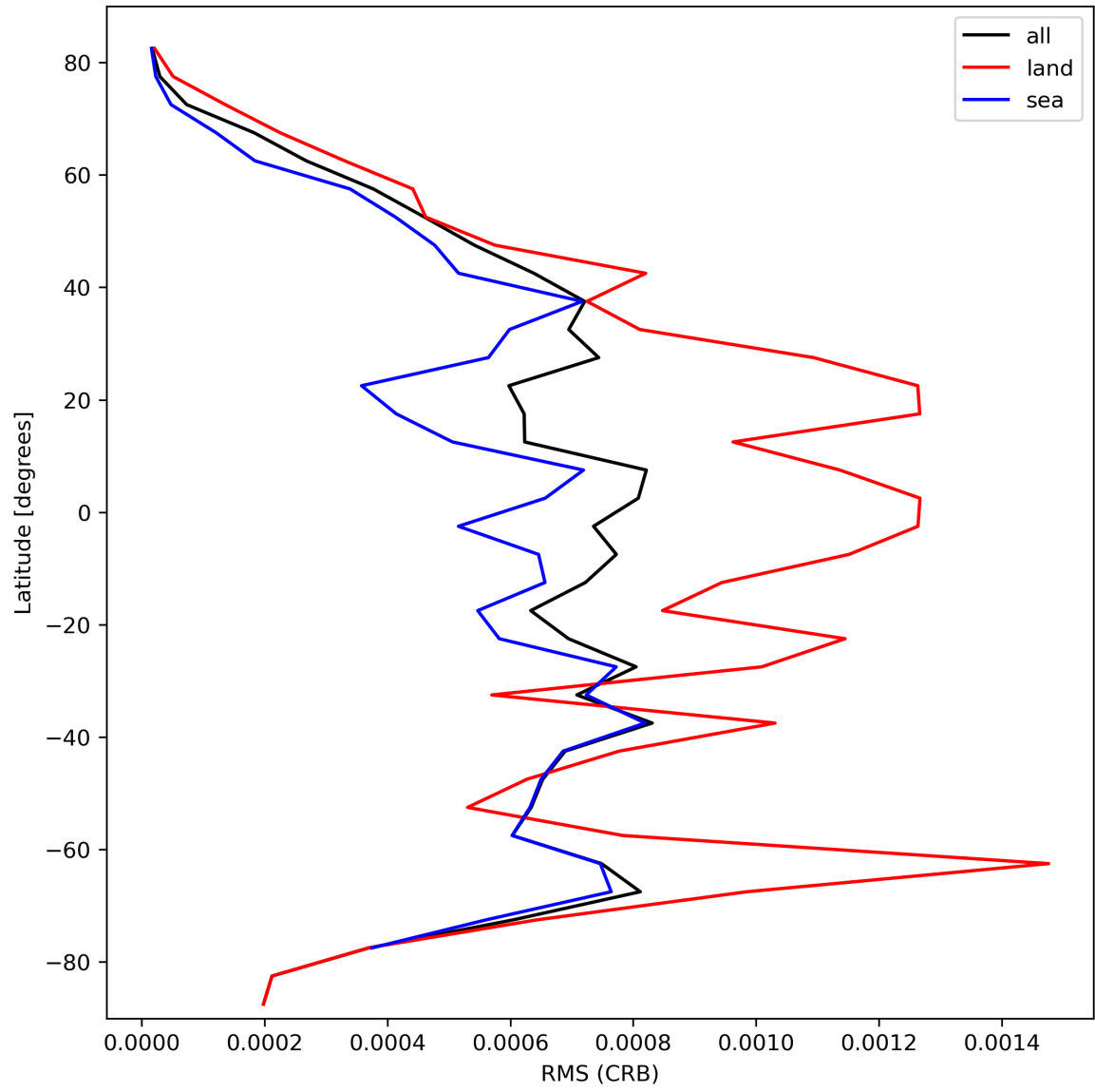
Figure 32: Zonal average of “RMS (CRB)” for 2023-10-12 to 2023-10-14.
