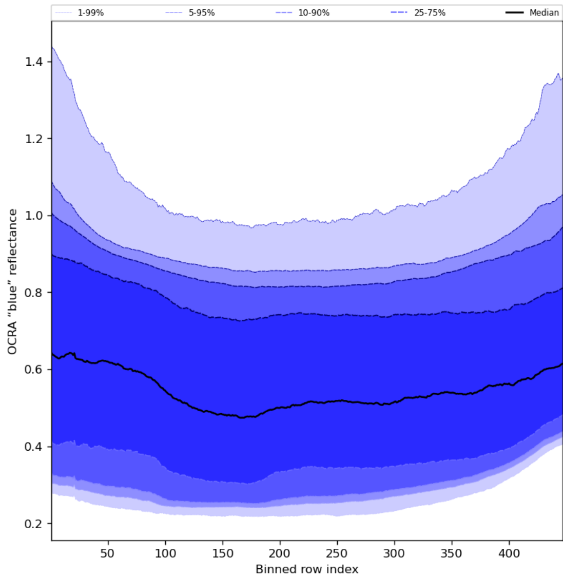
Figure 67: Along track statistics of "OCRA "blue" reflectance" for 2023-10-12 to 2023-10-14
