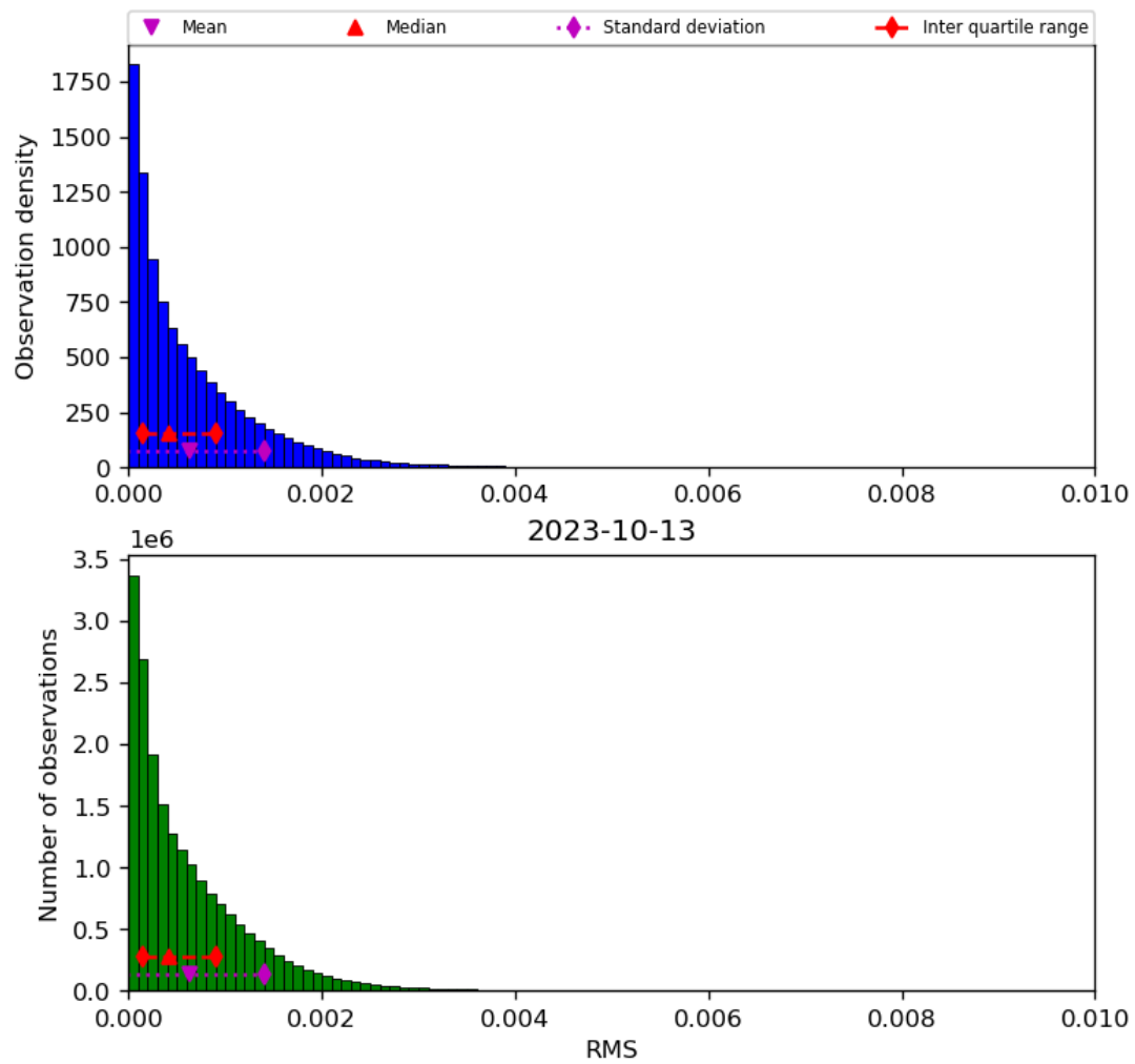
Figure 47: Histogram of “RMS” for 2023-10-12 to 2023-10-14
