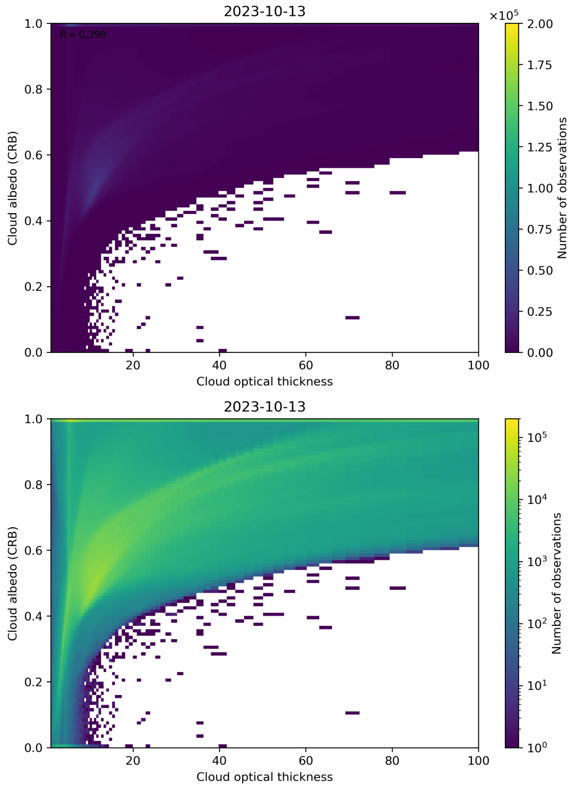
Figure 82: Scatter density plot of “Cloud optical thickness” against “Cloud albedo (CRB)” for 2023-10-12 to 2023-10-14.
