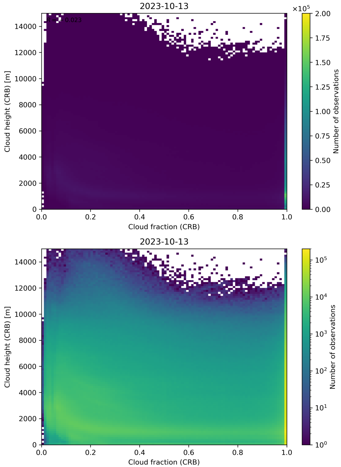
Figure 79: Scatter density plot of “Cloud fraction (CRB)” against “Cloud height (CRB)” for 2023-10-12 to 2023-10-14.
