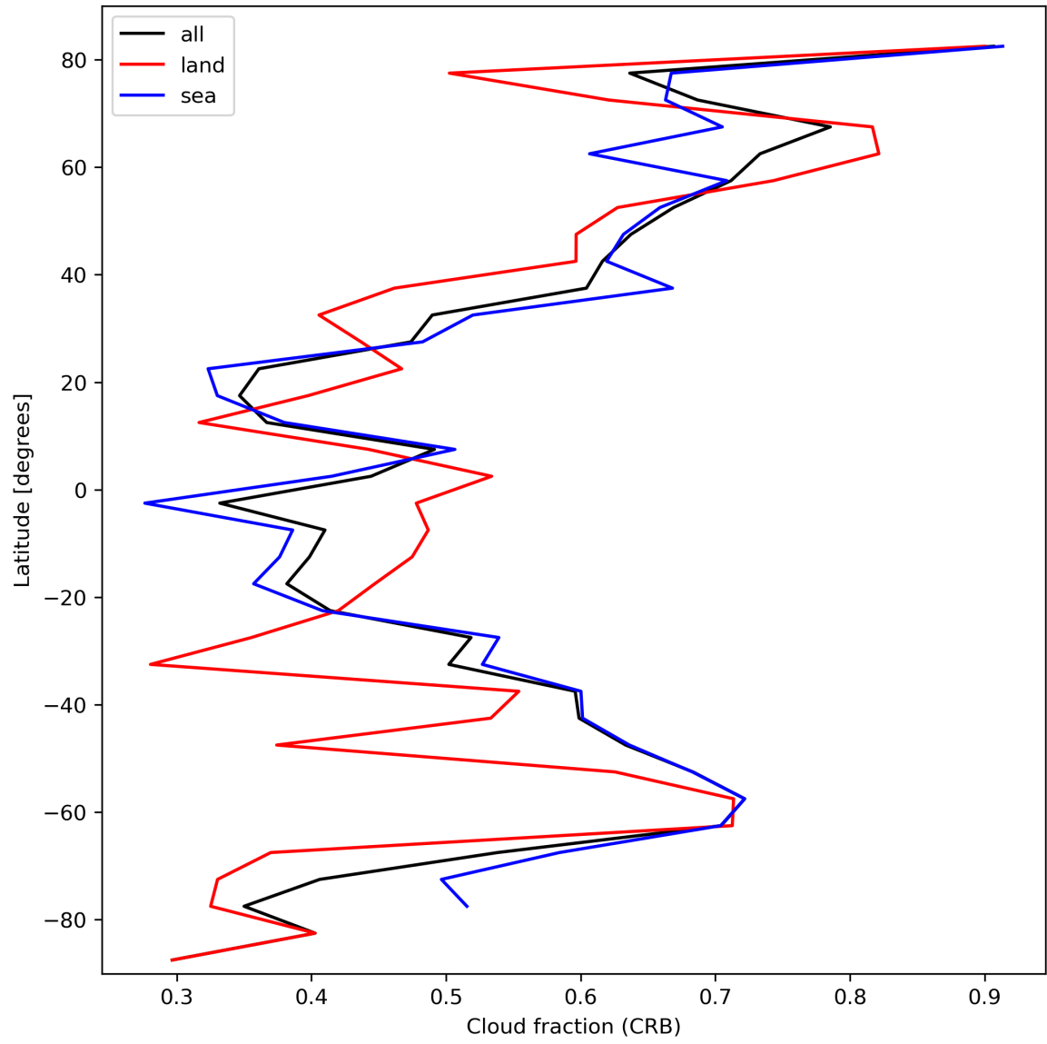
Figure 26: Zonal average of “Cloud fraction (CRB)” for 2023-10-12 to 2023-10-14.
