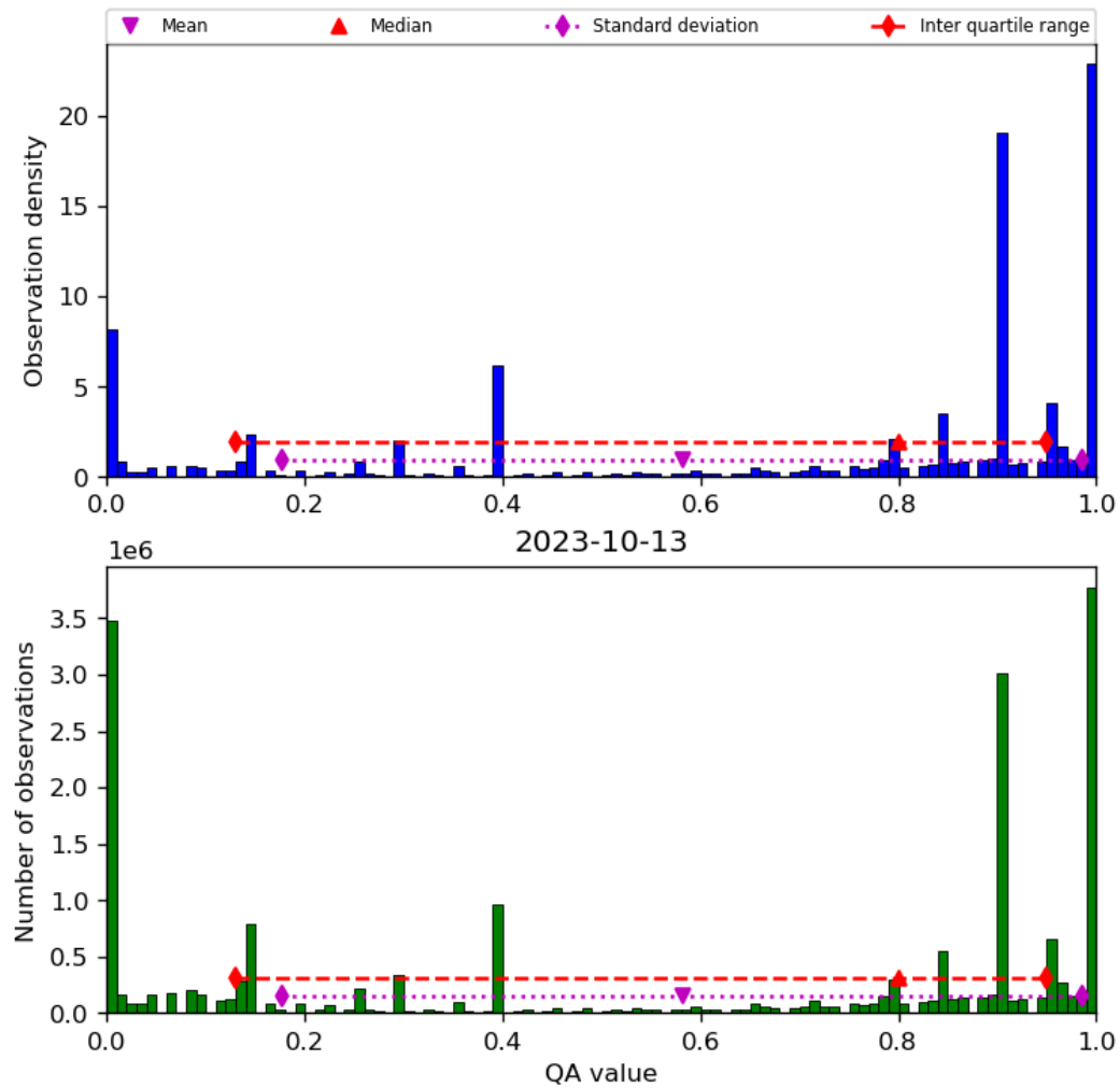
Figure 38: Histogram of “QA value” for 2023-10-12 to 2023-10-14
