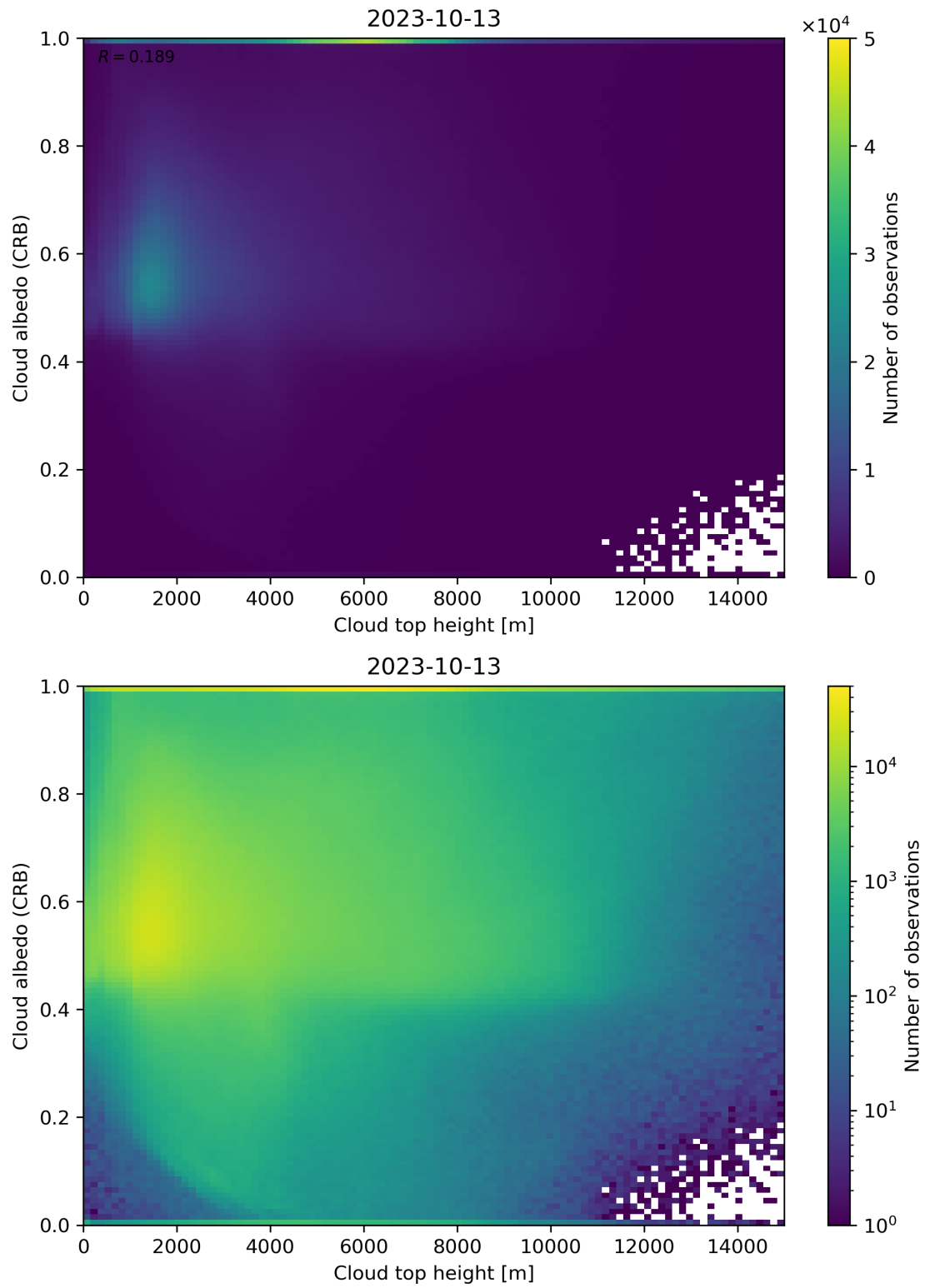
Figure 86: Scatter density plot of “Cloud top height” against “Cloud albedo (CRB)” for 2023-10-12 to 2023-10-14.
