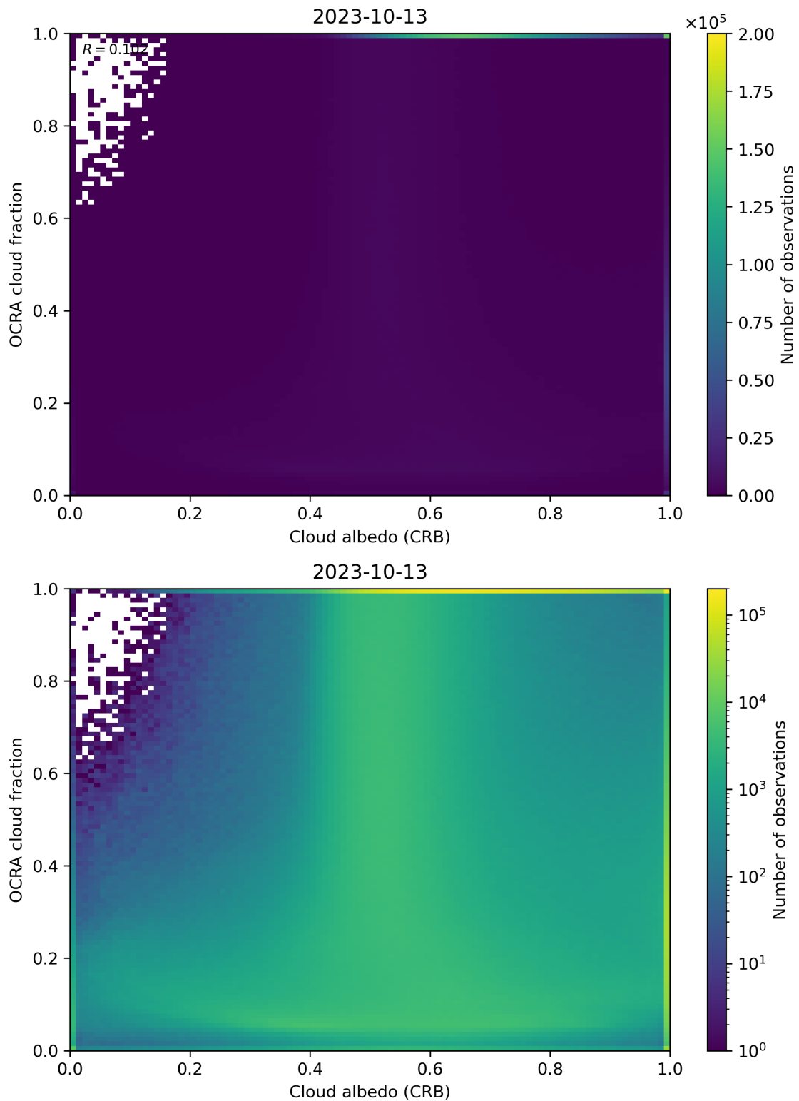
Figure 70: Scatter density plot of “Cloud albedo (CRB)” against “OCRA cloud fraction” for 2023-10-12 to 2023-10-14.
