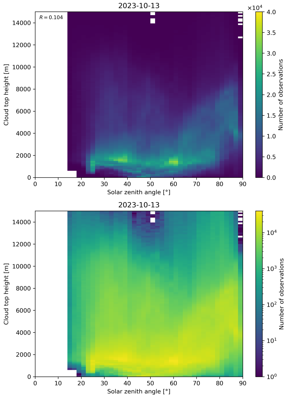
Figure 104: Scatter density plot of “Solar zenith angle” against “Cloud top height” for 2023-10-12 to 2023-10-14.
