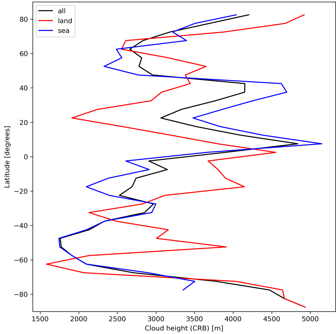
Figure 27: Zonal average of “Cloud height (CRB)” for 2023-10-12 to 2023-10-14.
