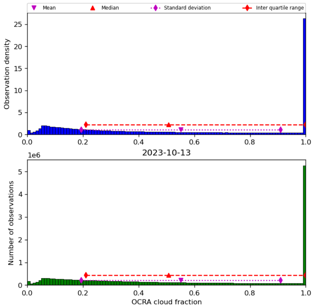
Figure 50: Histogram of “OCRA cloud fraction” for 2023-10-12 to 2023-10-14
