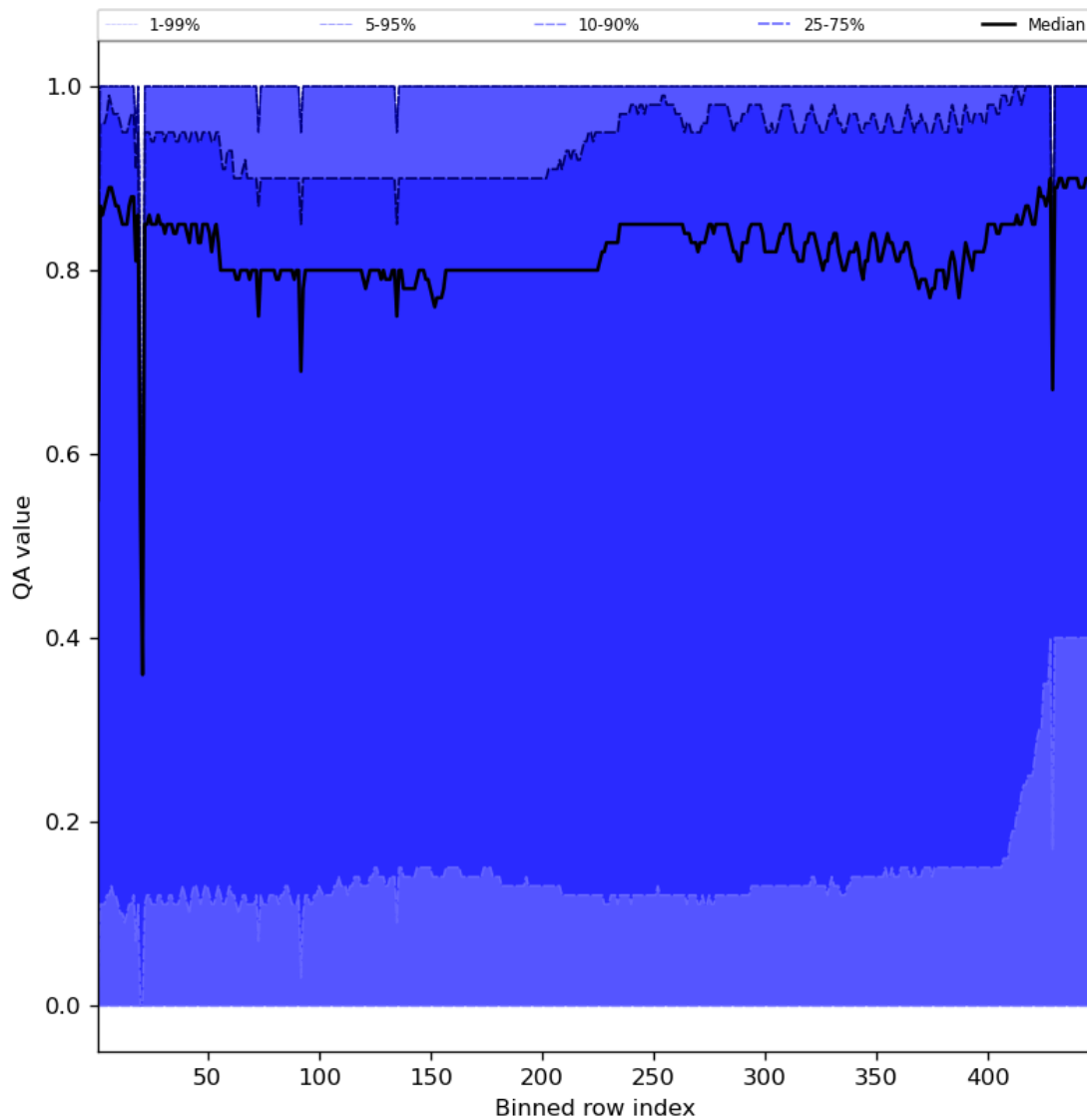
Figure 54: Along track statistics of “QA value” for 2023-10-12 to 2023-10-14
