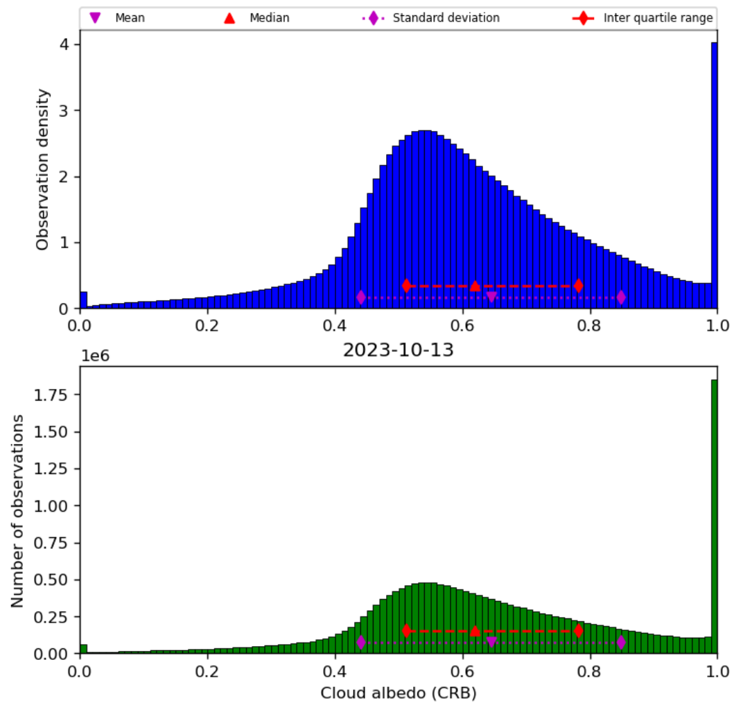
Figure 44: Histogram of “Cloud albedo (CRB)” for 2023-10-12 to 2023-10-14
