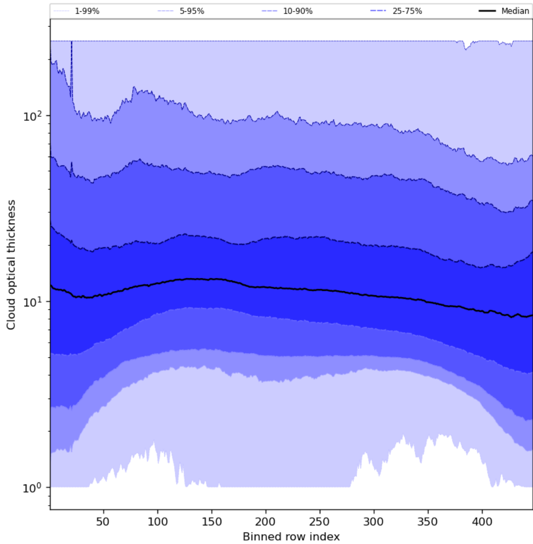
Figure 57: Along track statistics of “Cloud optical thickness” for 2023-10-12 to 2023-10-14
