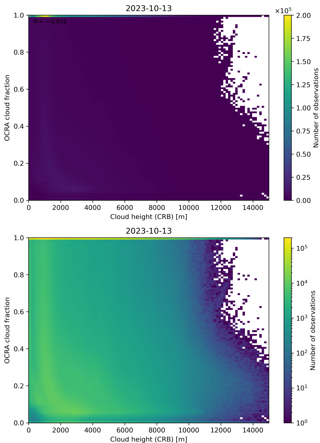
Figure 81: Scatter density plot of “Cloud height (CRB)” against “OCRA cloud fraction” for 2023-10-12 to 2023-10-14.
