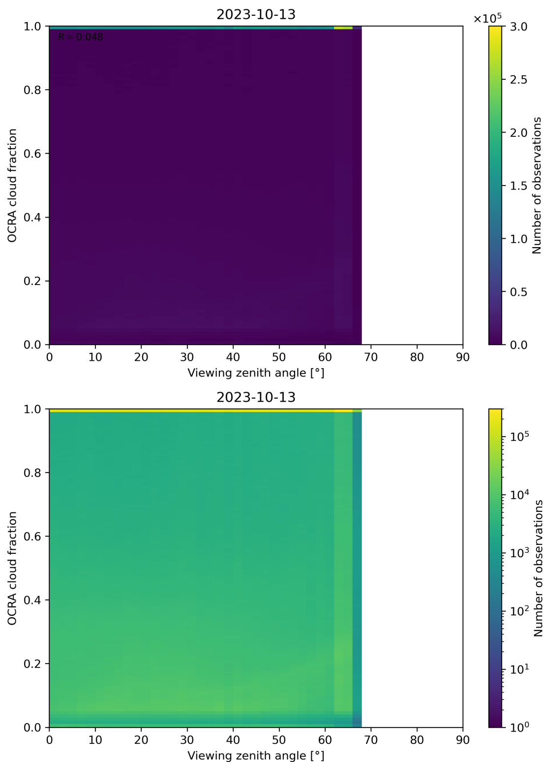
Figure 108: Scatter density plot of “Viewing zenith angle” against “OCRA cloud fraction” for 2023-10-12 to 2023-10-14.
