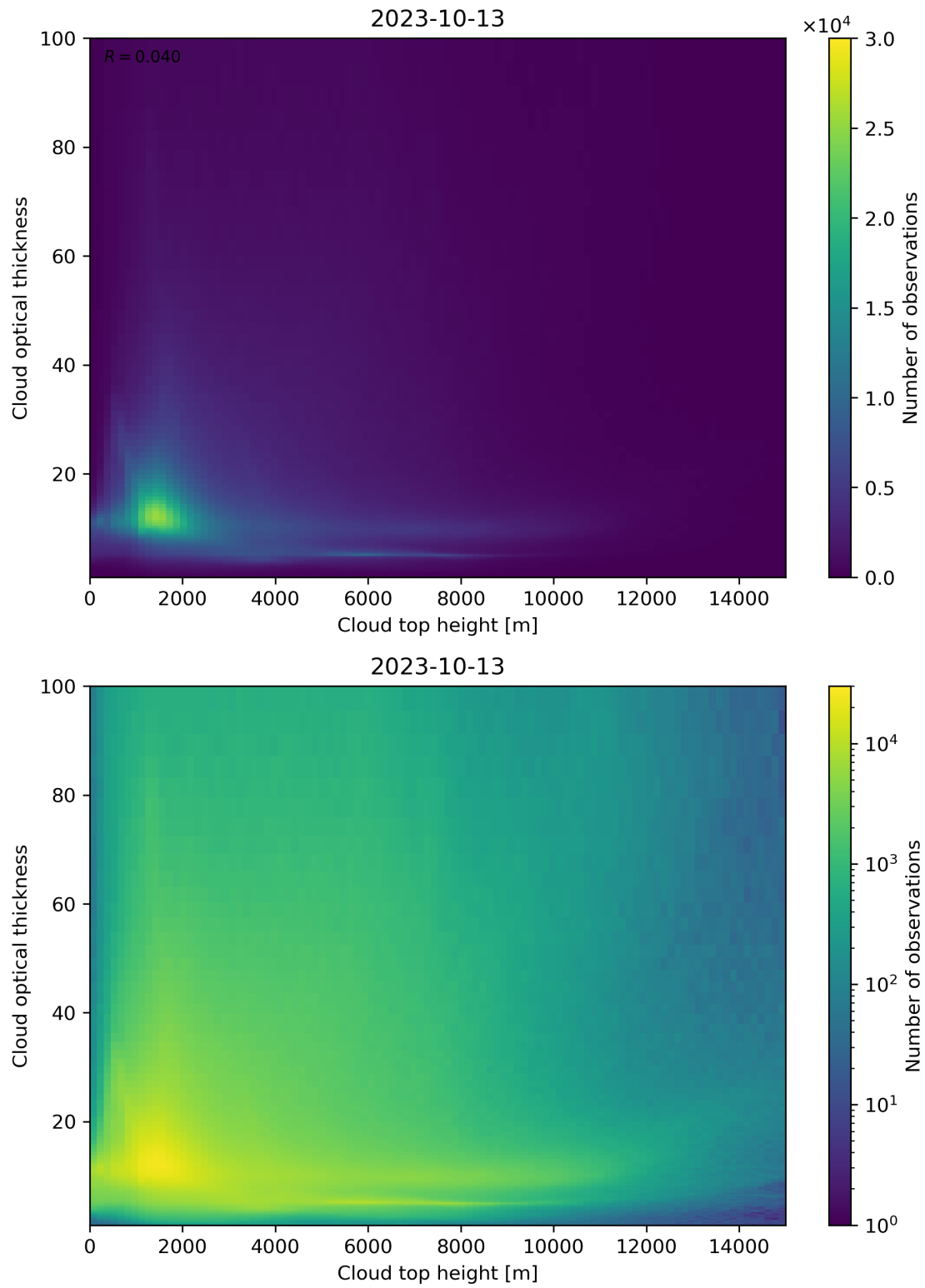
Figure 90: Scatter density plot of “Cloud top height” against “Cloud optical thickness” for 2023-10-12 to 2023-10-14.
