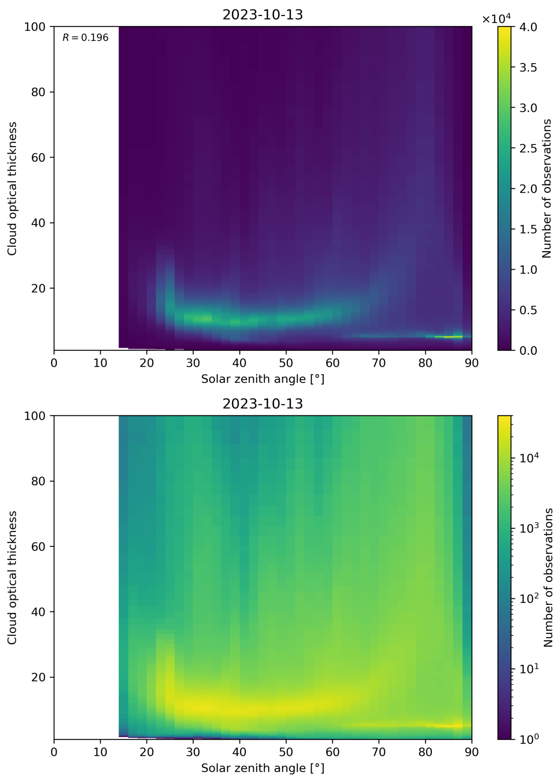
Figure 103: Scatter density plot of “Solar zenith angle” against “Cloud optical thickness” for 2023-10-12 to 2023-10-14.
