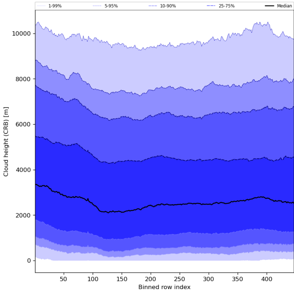
Figure 59: Along track statistics of “Cloud height (CRB)” for 2023-10-12 to 2023-10-14
