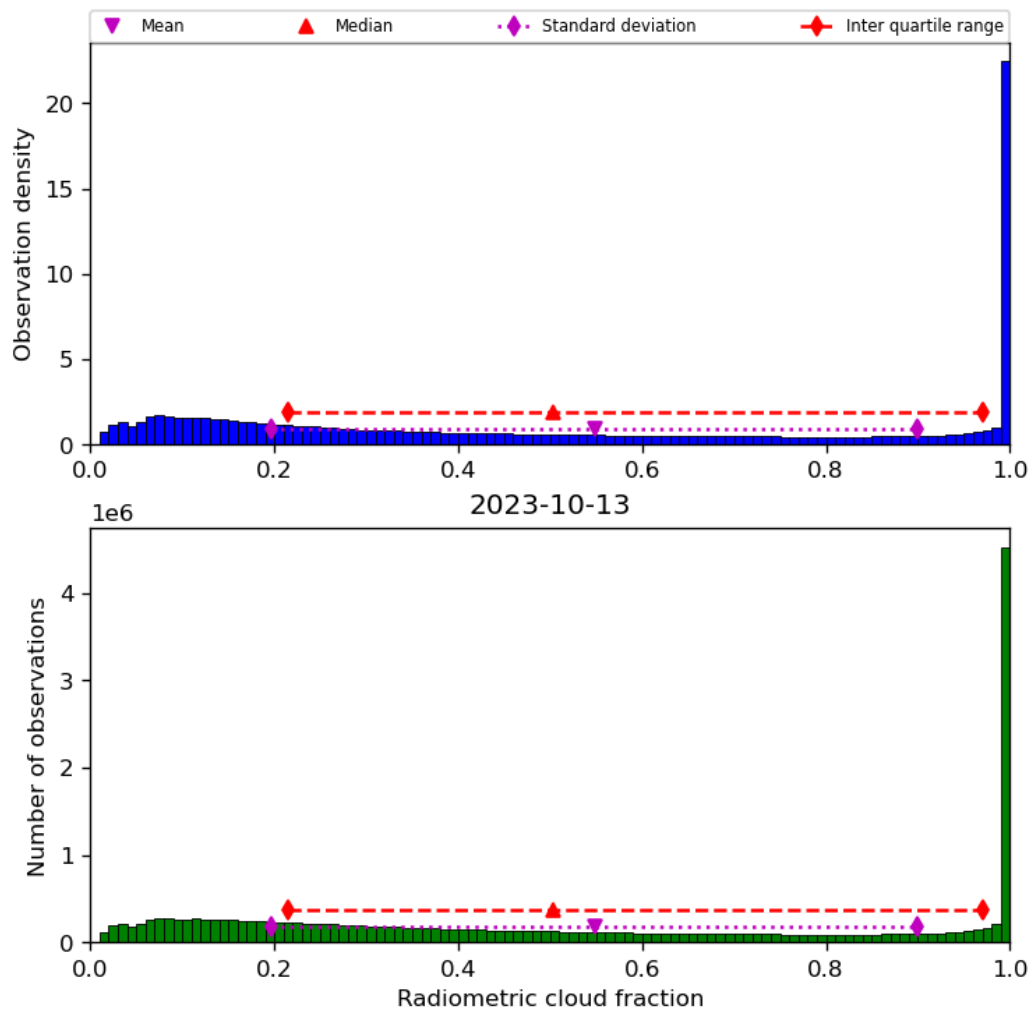
Figure 39: Histogram of “Radiometric cloud fraction” for 2023-10-12 to 2023-10-14
