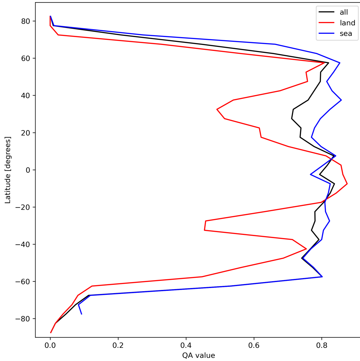
Figure 22: Zonal average of “QA value” for 2023-10-12 to 2023-10-14.
