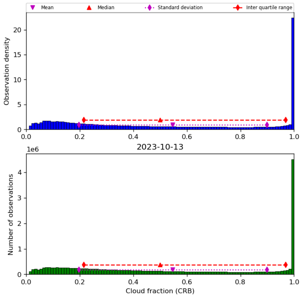
Figure 42: Histogram of “Cloud fraction (CRB)” for 2023-10-12 to 2023-10-14
