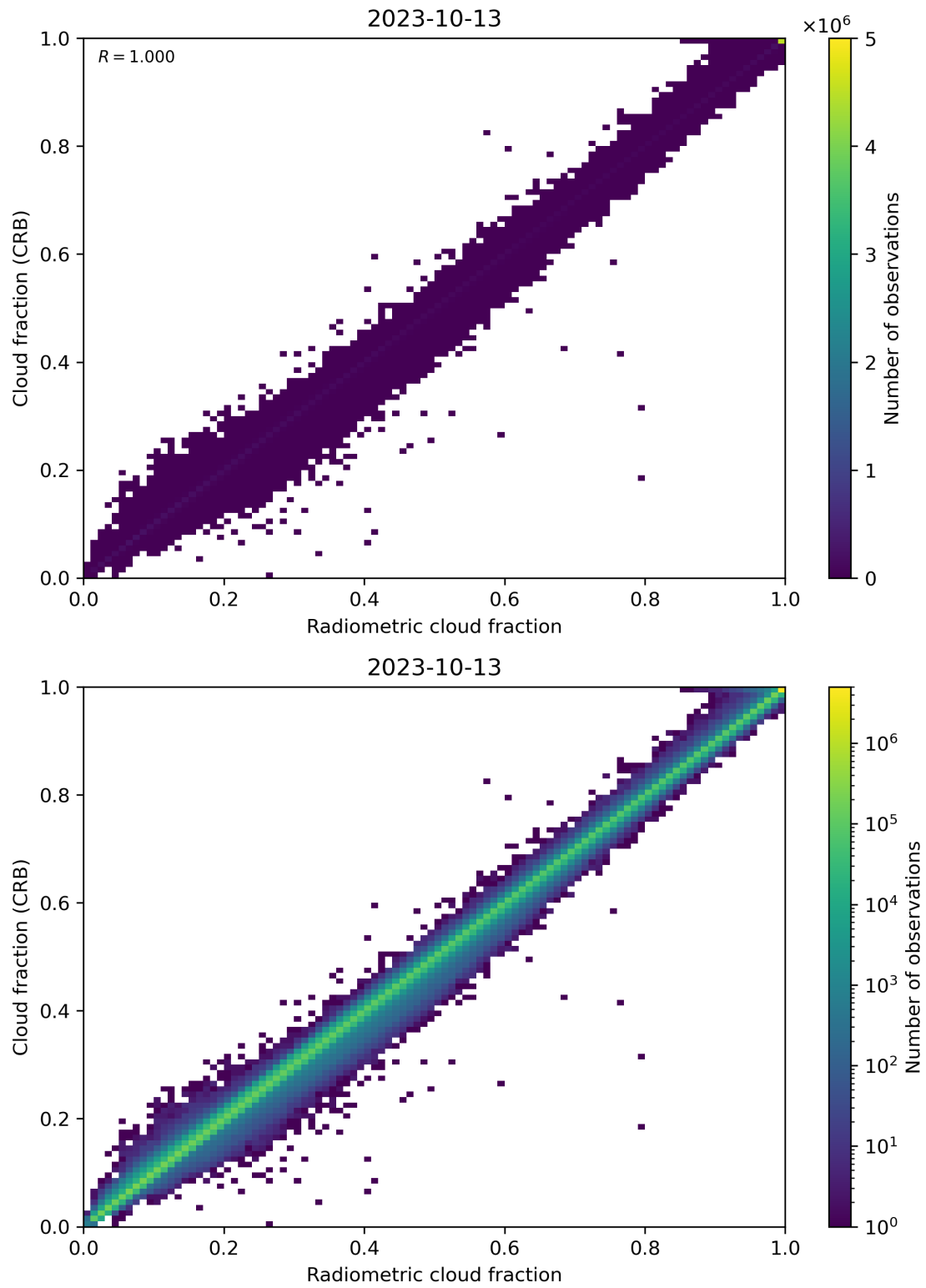
Figure 73: Scatter density plot of “Radiometric cloud fraction” against “Cloud fraction (CRB)” for 2023-10-12 to 2023-10-14.
