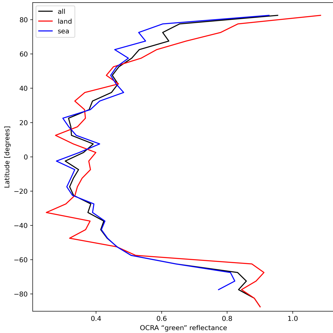
Figure 36: Zonal average of “OCRA “green” reflectance” for 2023-10-12 to 2023-10-14.
