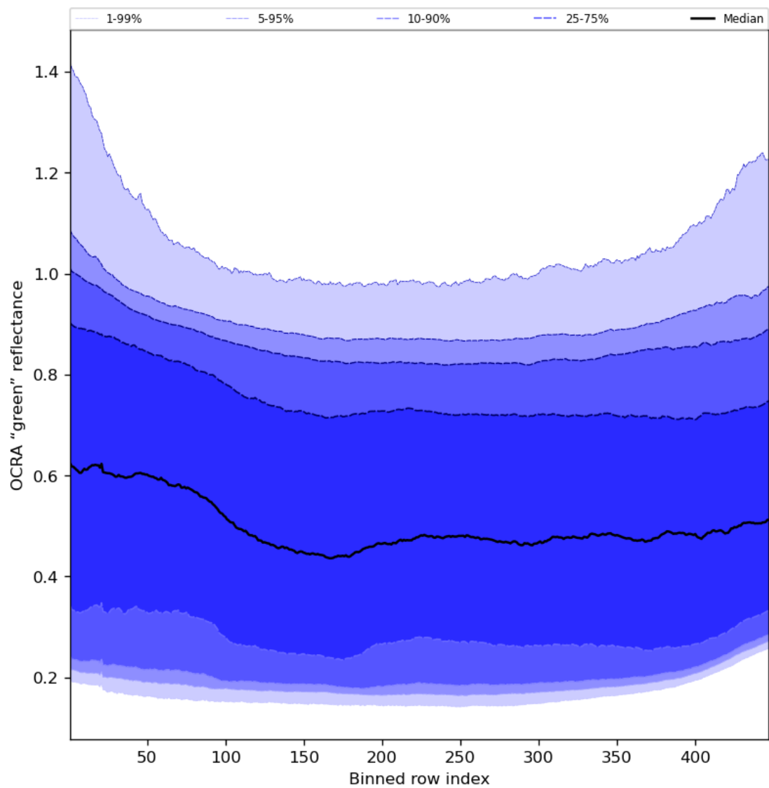
Figure 68: Along track statistics of “OCRA “green” reflectance” for 2023-10-12 to 2023-10-14
