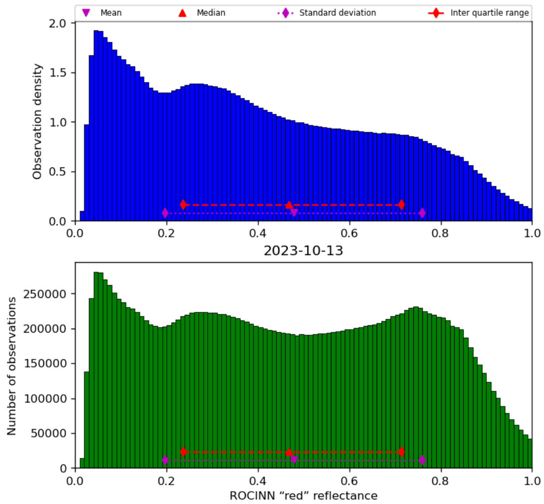
Figure 53: Histogram of “ROCINN “red” reflectance” for 2023-10-12 to 2023-10-14
