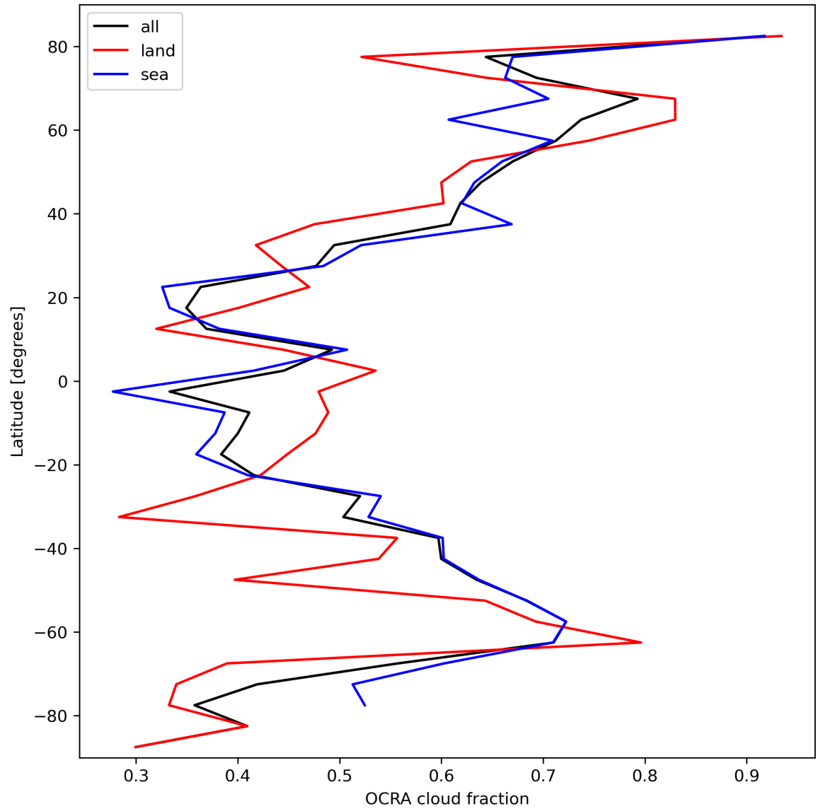
Figure 34: Zonal average of “OCRA cloud fraction” for 2023-10-12 to 2023-10-14.
