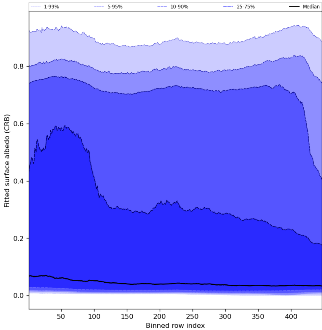
Figure 62: Along track statistics of “Fitted surface albedo (CRB)” for 2023-10-12 to 2023-10-14
