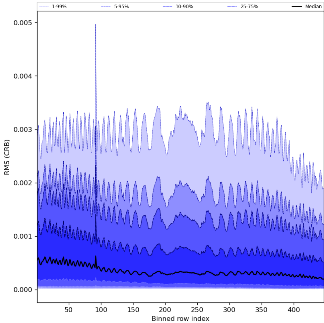
Figure 64: Along track statistics of “RMS (CRB)” for 2023-10-12 to 2023-10-14
