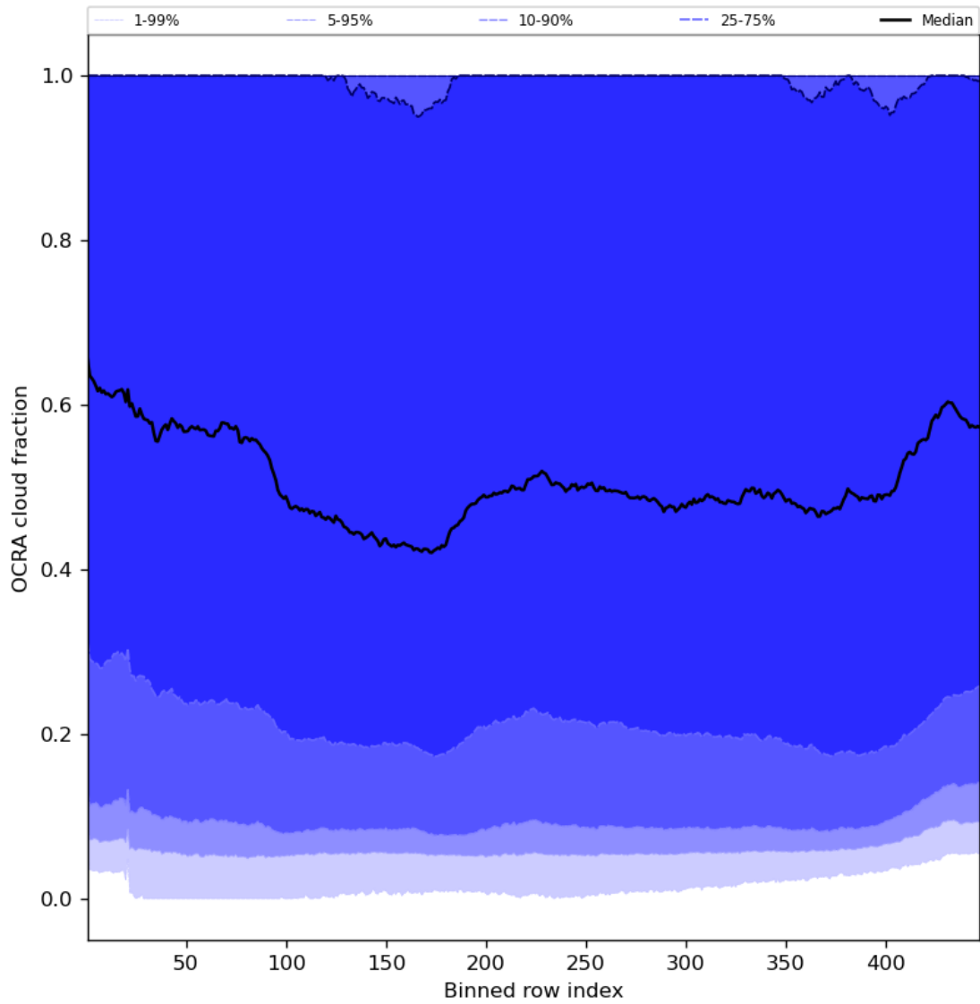
Figure 66: Along track statistics of “OCRA cloud fraction” for 2023-10-12 to 2023-10-14
