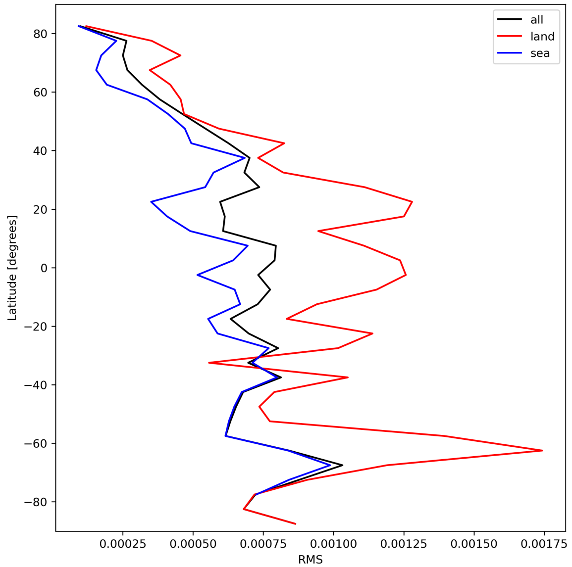
Figure 31: Zonal average of “RMS” for 2023-10-12 to 2023-10-14.
