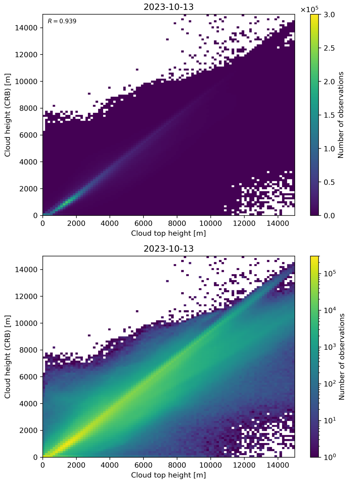
Figure 89: Scatter density plot of “Cloud top height” against “Cloud height (CRB)” for 2023-10-12 to 2023-10-14.
