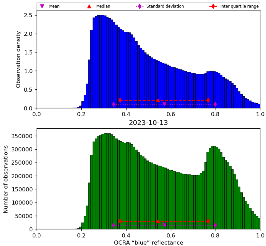
Figure 51: Histogram of “OCRA “blue” reflectance” for 2023-10-12 to 2023-10-14
