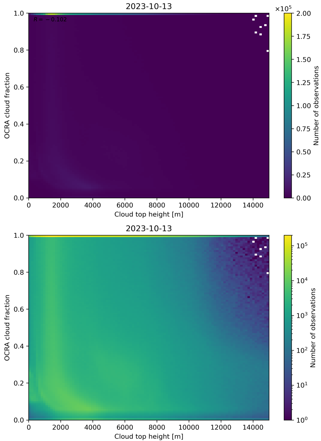
Figure 87: Scatter density plot of “Cloud top height” against “OCRA cloud fraction” for 2023-10-12 to 2023-10-14.
