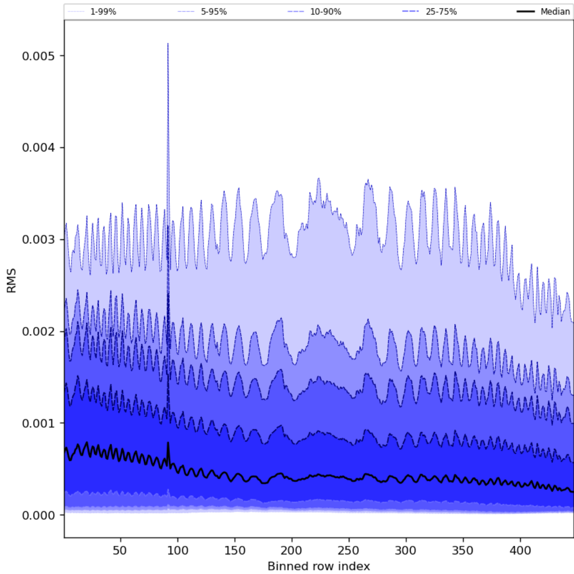
Figure 63: Along track statistics of “RMS” for 2023-10-12 to 2023-10-14
