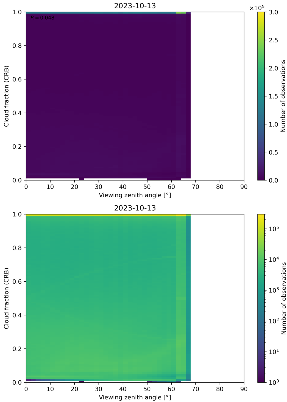
Figure 109: Scatter density plot of “Viewing zenith angle” against “Cloud fraction (CRB)” for 2023-10-12 to 2023-10-14.
