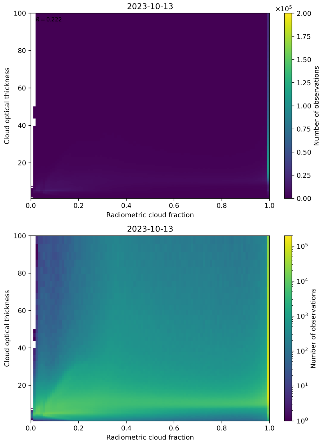
Figure 75: Scatter density plot of “Radiometric cloud fraction” against “Cloud optical thickness” for 2023-10-12 to 2023-10-14.
