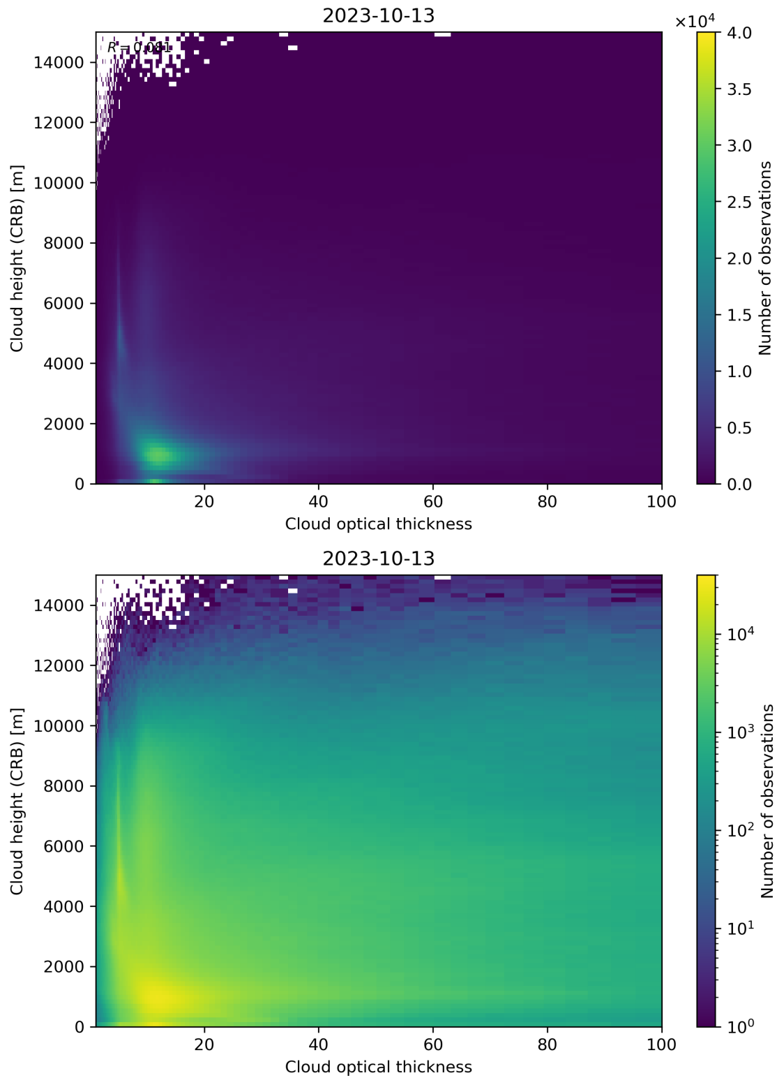
Figure 85: Scatter density plot of “Cloud optical thickness” against “Cloud height (CRB)” for 2023-10-12 to 2023-10-14.
