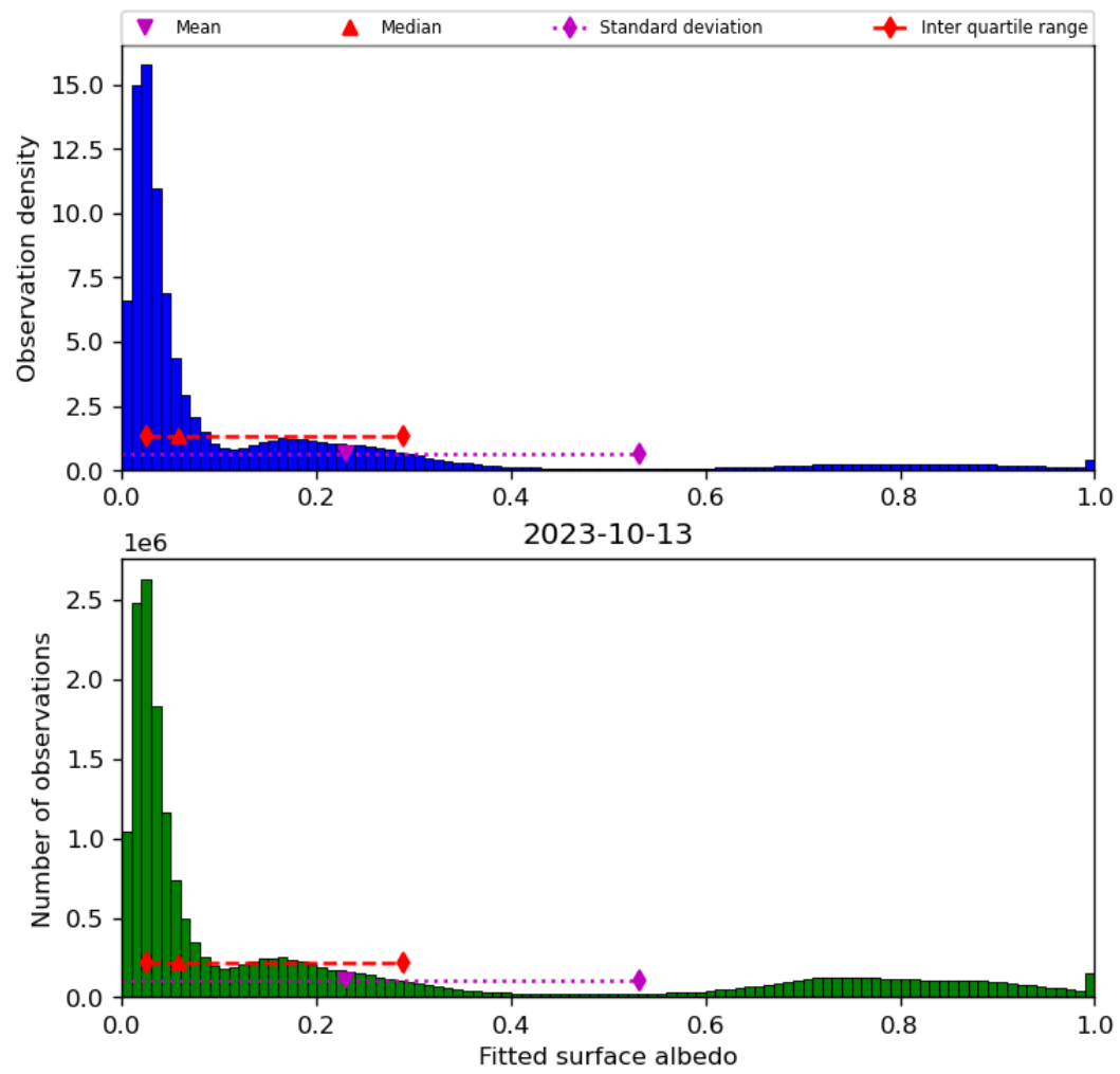
Figure 45: Histogram of “Fitted surface albedo” for 2023-10-12 to 2023-10-14
