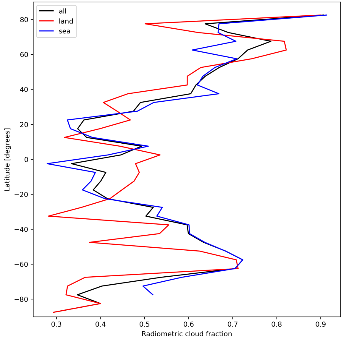
Figure 23: Zonal average of “Radiometric cloud fraction” for 2023-10-12 to 2023-10-14.
