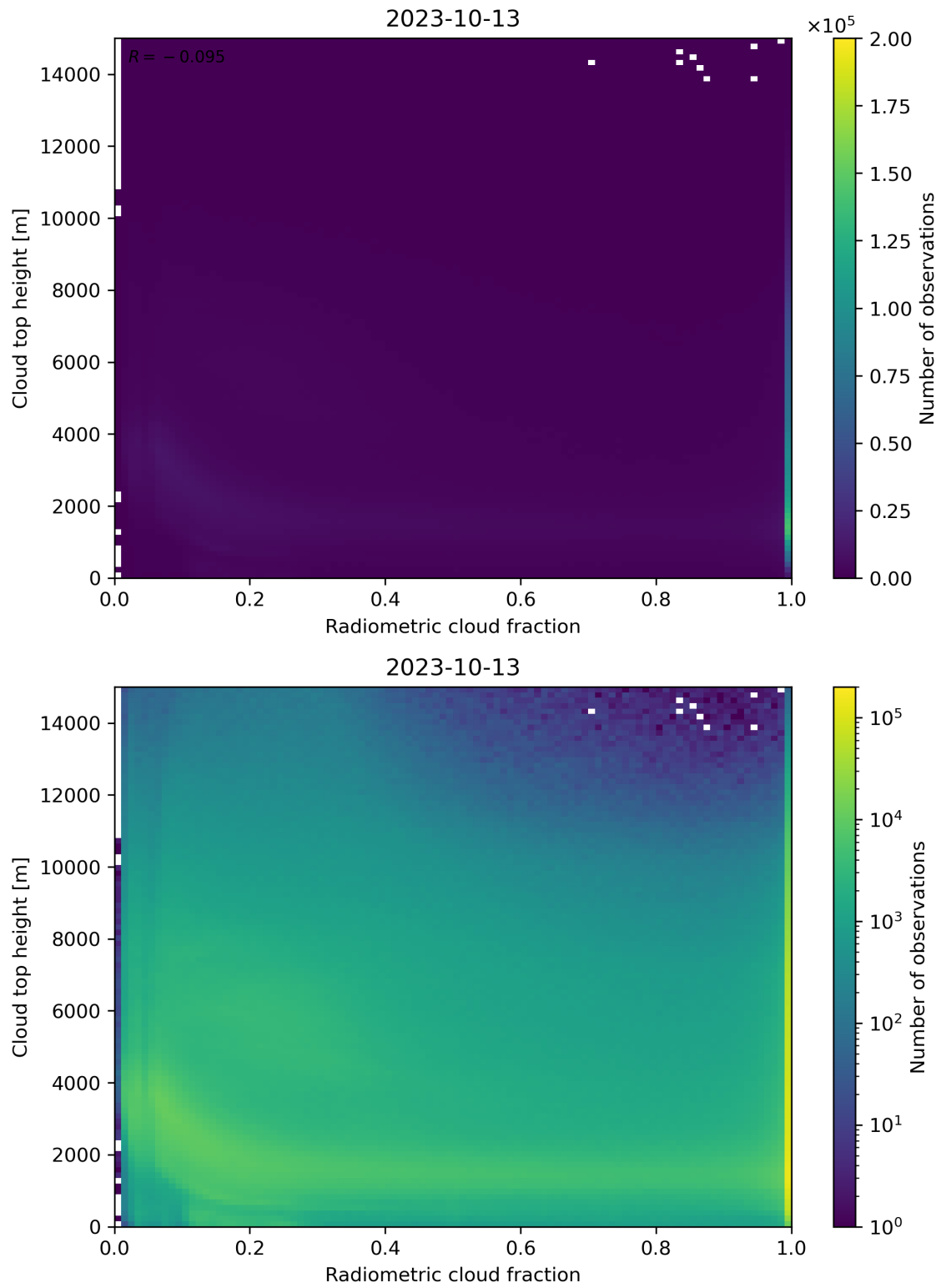
Figure 76: Scatter density plot of “Radiometric cloud fraction” against “Cloud top height” for 2023-10-12 to 2023-10-14.
