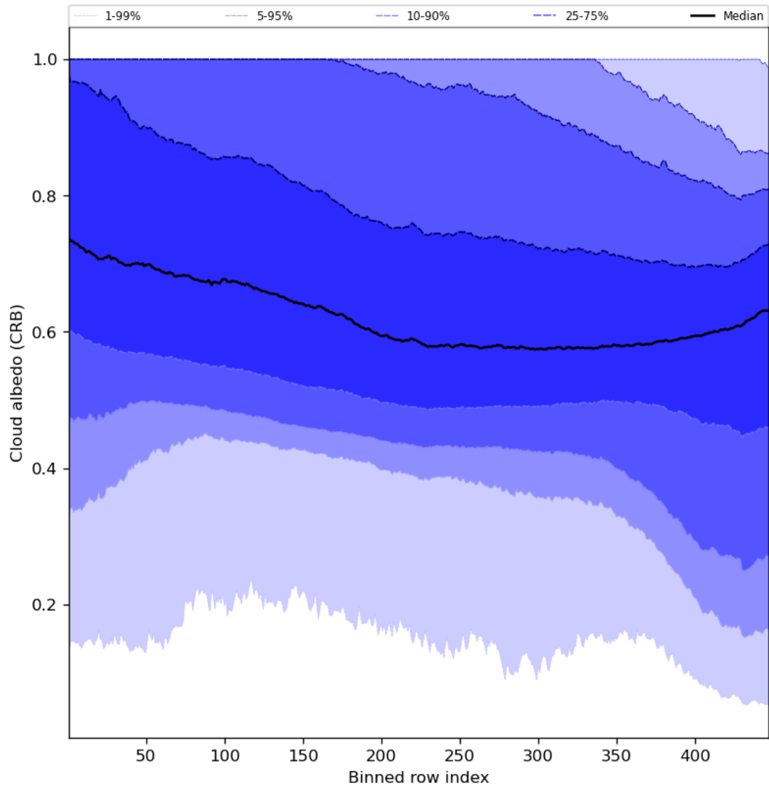
Figure 60: Along track statistics of “Cloud albedo (CRB)” for 2023-10-13 to 2023-10-15
