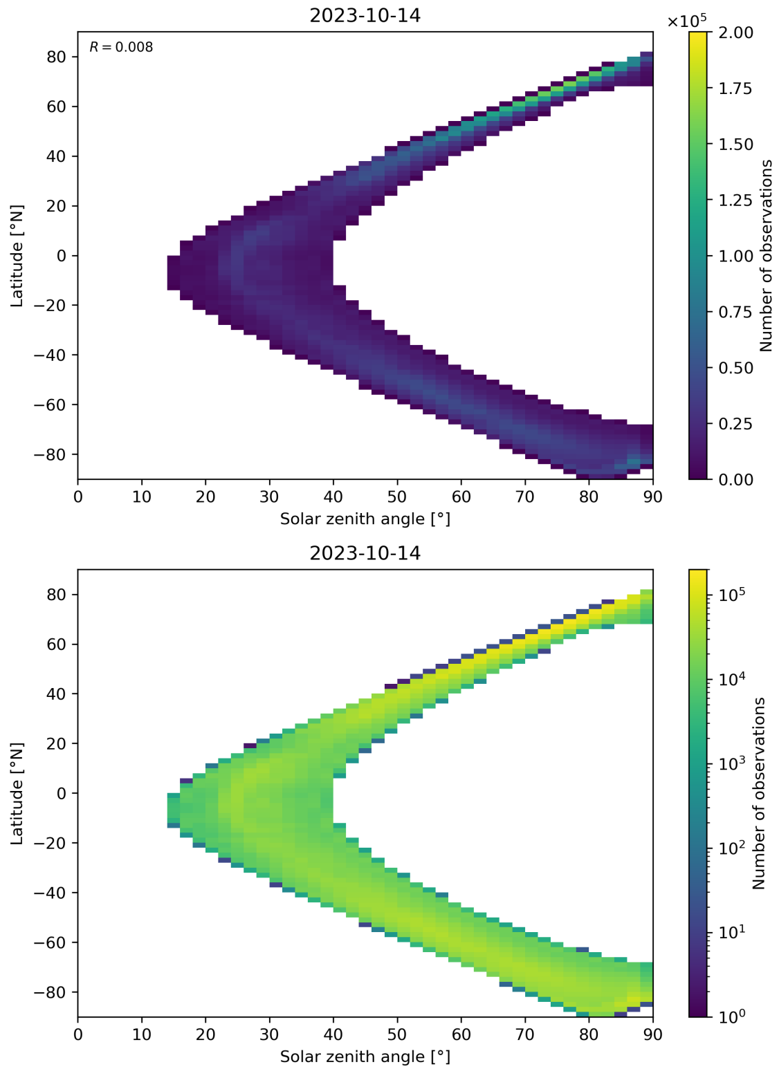
Figure 105: Scatter density plot of “Solar zenith angle” against “Latitude” for 2023-10-13 to 2023-10-15.
