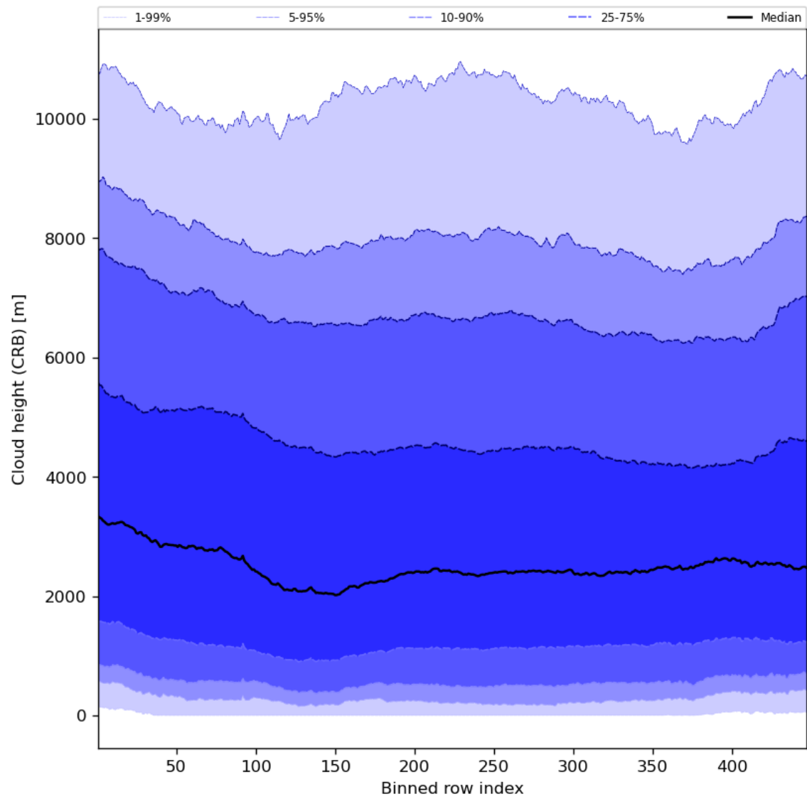
Figure 59: Along track statistics of “Cloud height (CRB)” for 2023-10-13 to 2023-10-15
