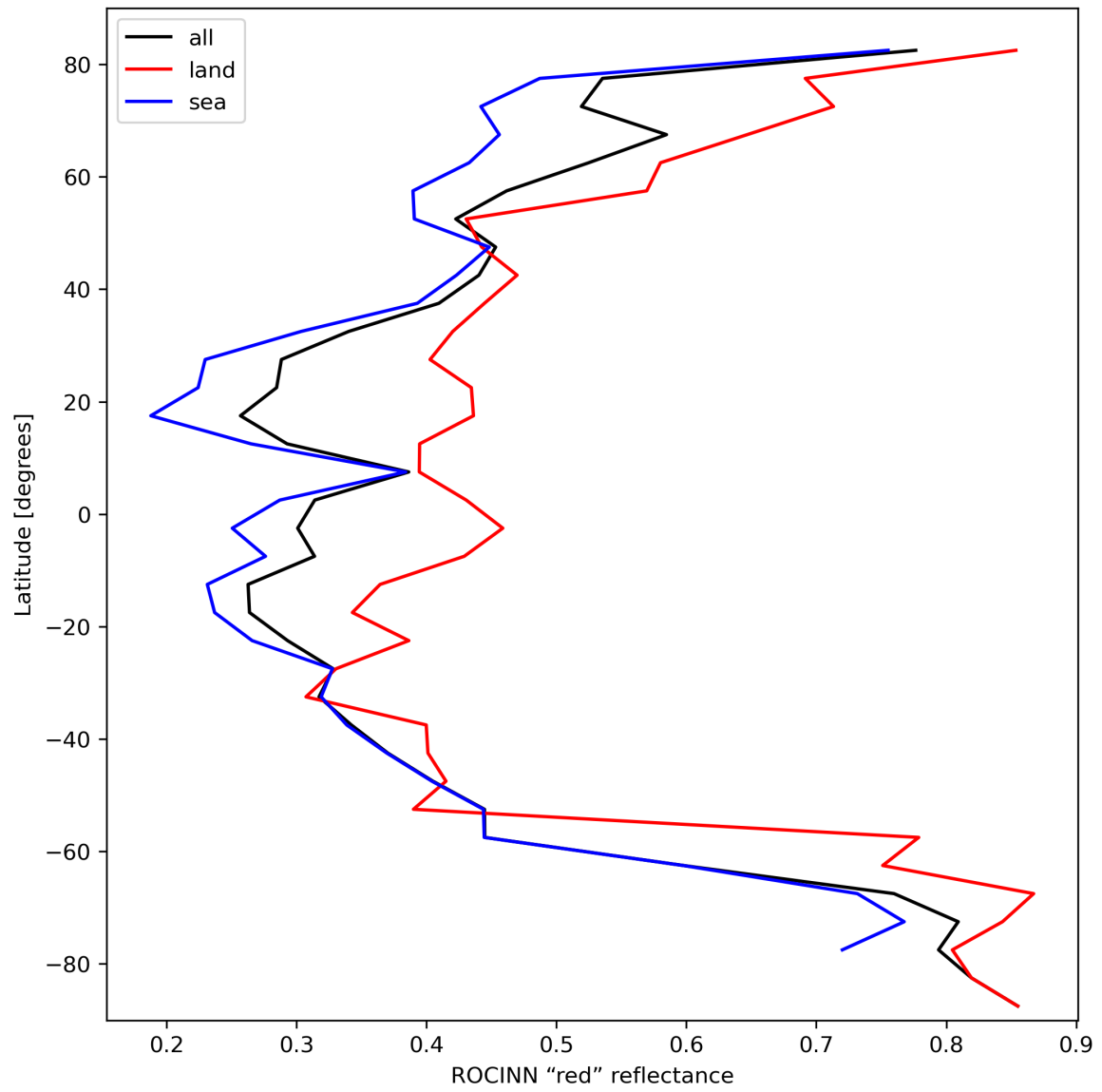
Figure 37: Zonal average of “ROCINN “red” reflectance” for 2023-10-13 to 2023-10-15.
