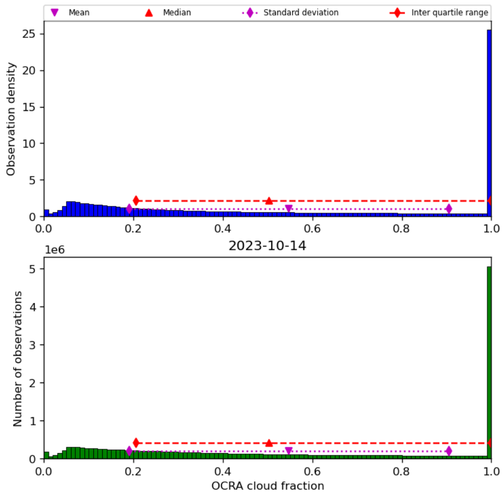
Figure 50: Histogram of “OCRA cloud fraction” for 2023-10-13 to 2023-10-15
