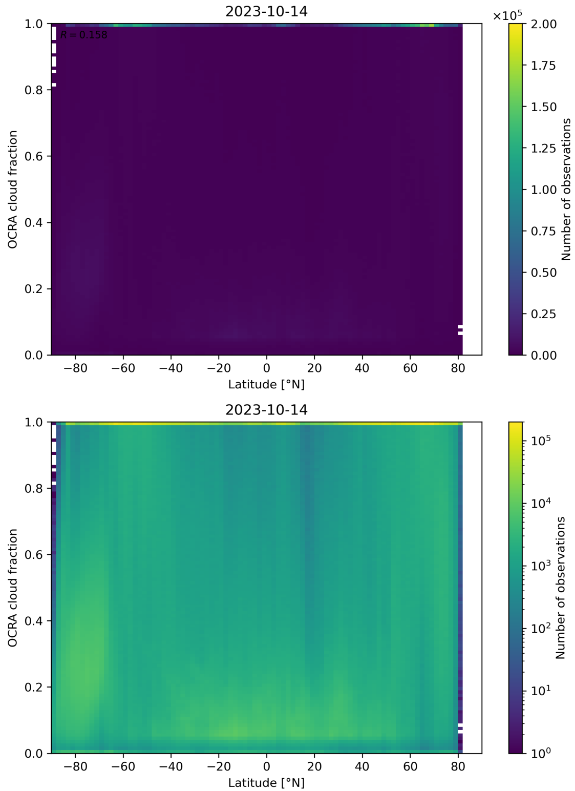
Figure 93: Scatter density plot of “Latitude” against “OCRA cloud fraction” for 2023-10-13 to 2023-10-15.
