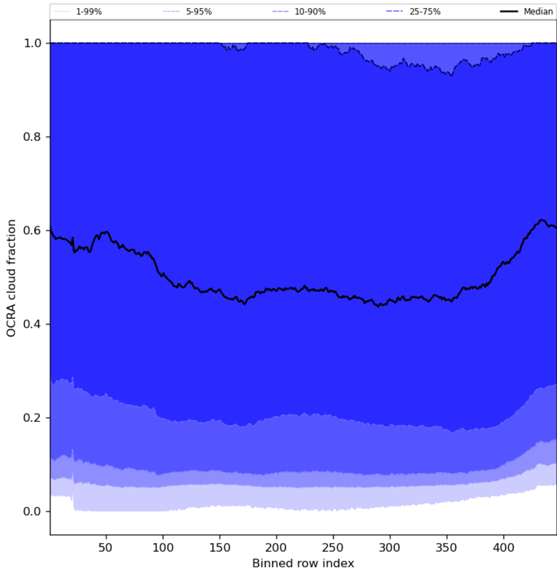
Figure 66: Along track statistics of “OCRA cloud fraction” for 2023-10-13 to 2023-10-15
