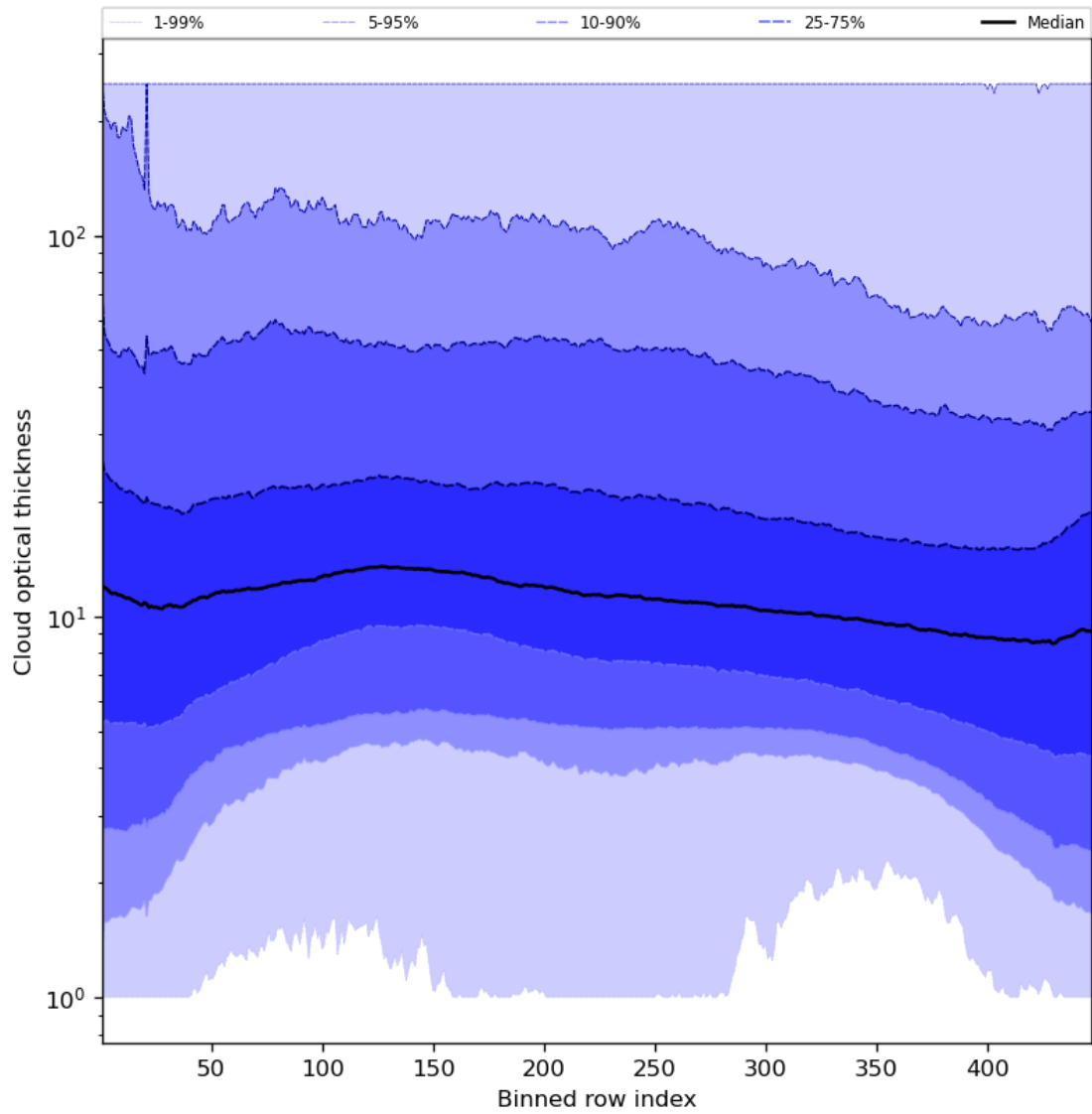
Figure 57: Along track statistics of “Cloud optical thickness” for 2023-10-13 to 2023-10-15
