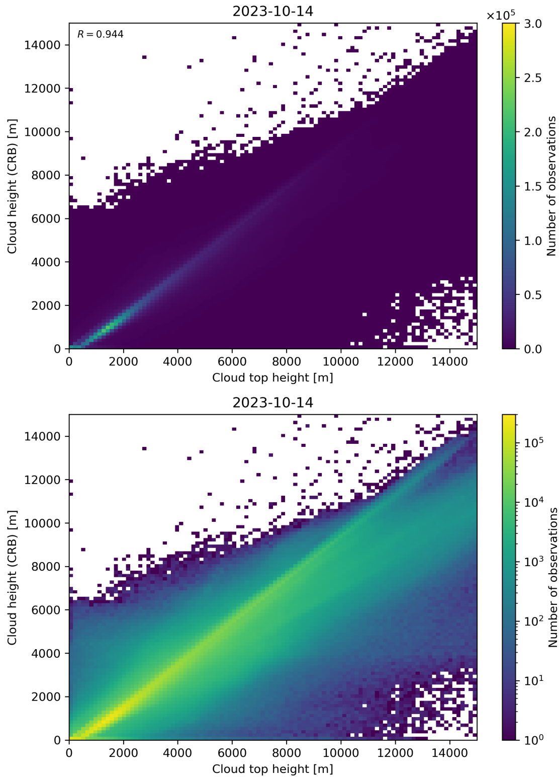
Figure 89: Scatter density plot of “Cloud top height” against “Cloud height (CRB)” for 2023-10-13 to 2023-10-15.
