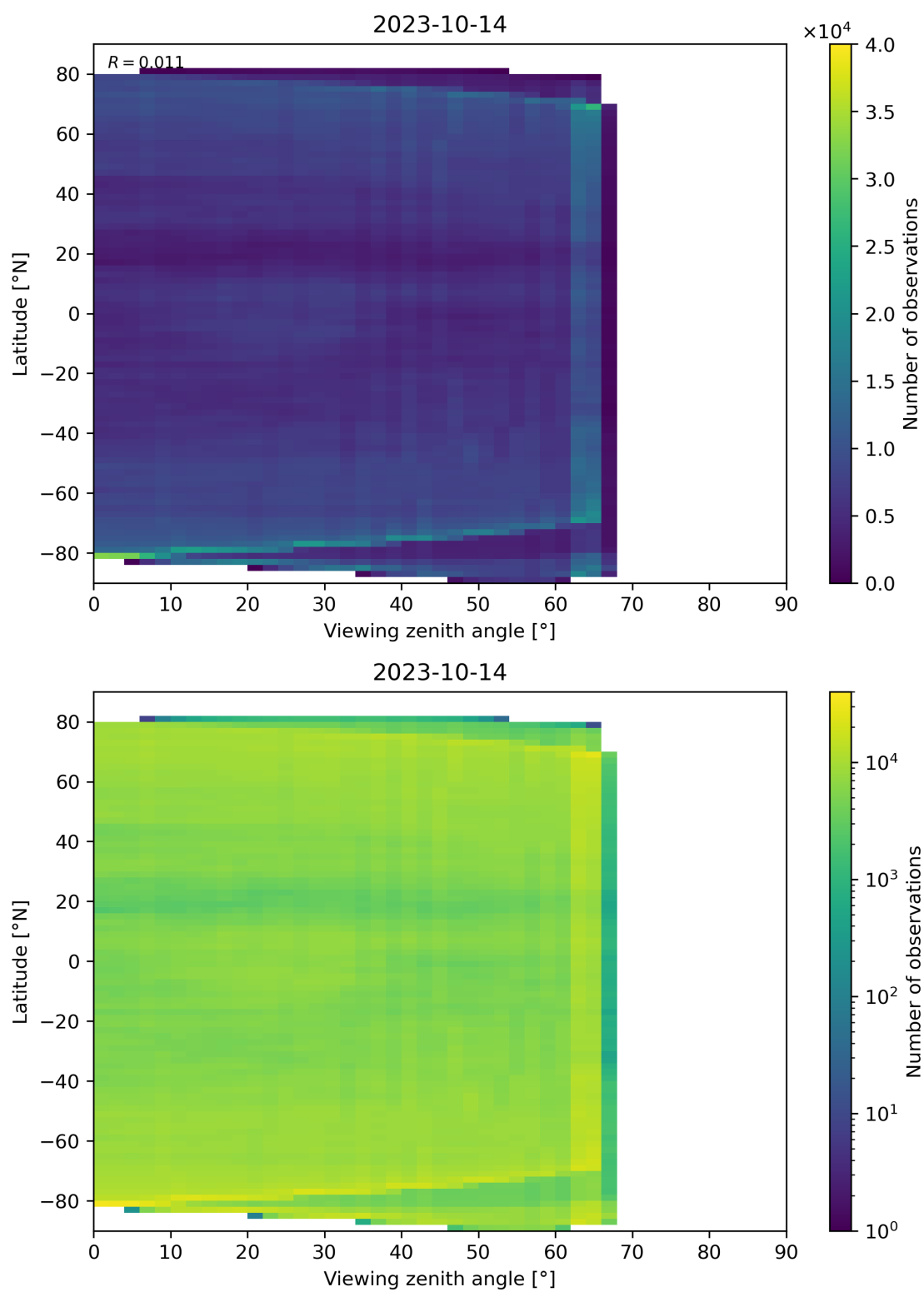
Figure 113: Scatter density plot of “Viewing zenith angle” against “Latitude” for 2023-10-13 to 2023-10-15.
