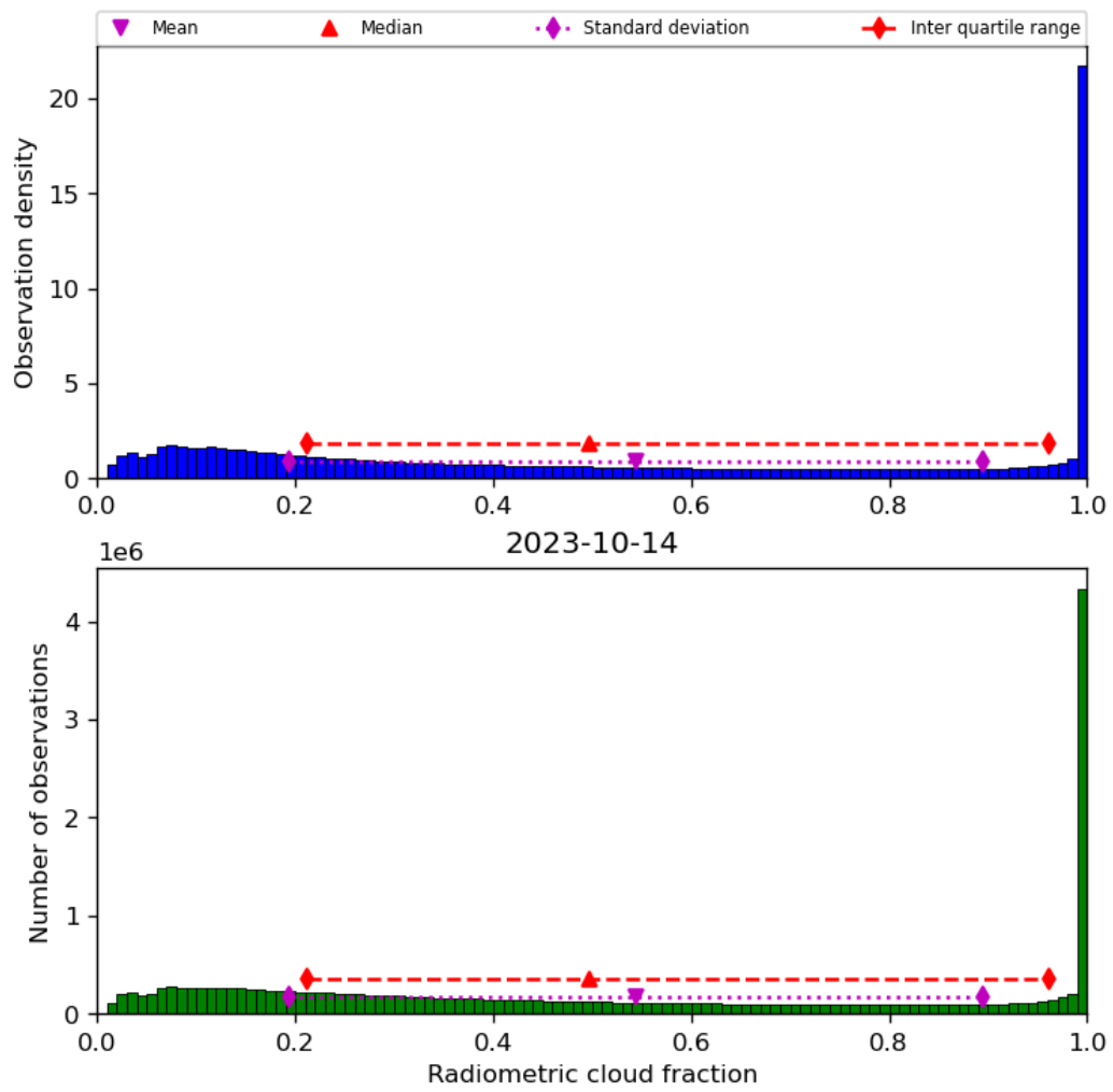
Figure 39: Histogram of “Radiometric cloud fraction” for 2023-10-13 to 2023-10-15
