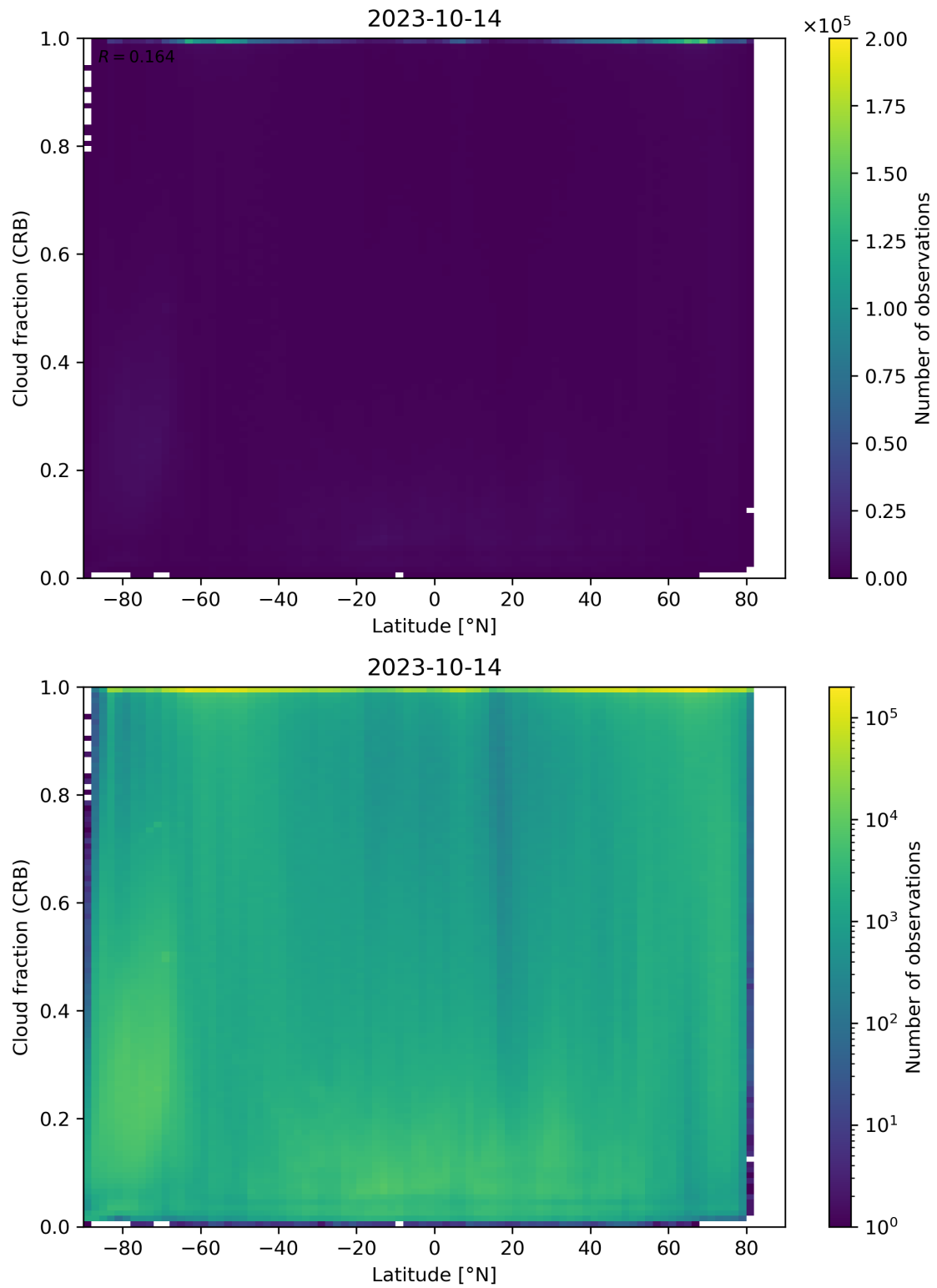
Figure 94: Scatter density plot of “Latitude” against “Cloud fraction (CRB)” for 2023-10-13 to 2023-10-15.
