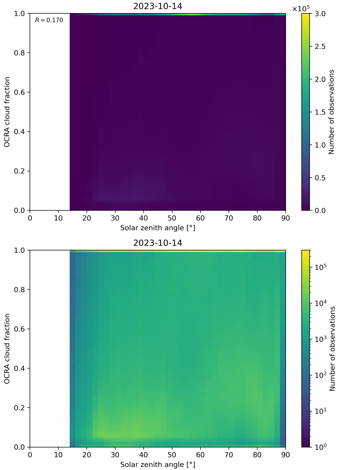
Figure 100: Scatter density plot of “Solar zenith angle” against “OCRA cloud fraction” for 2023-10-13 to 2023-10-15.
