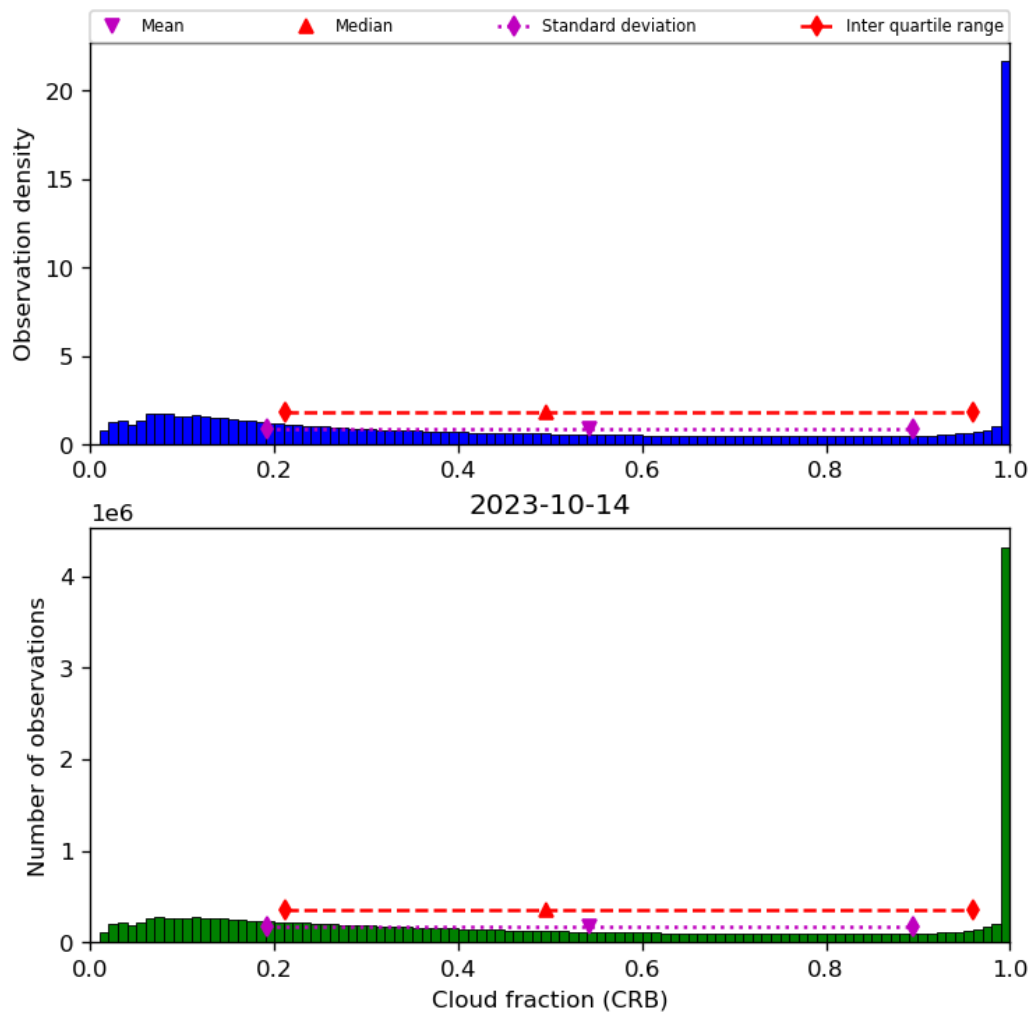
Figure 42: Histogram of “Cloud fraction (CRB)” for 2023-10-13 to 2023-10-15
