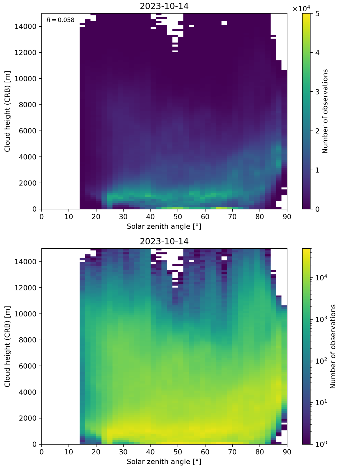
Figure 102: Scatter density plot of “Solar zenith angle” against “Cloud height (CRB)” for 2023-10-13 to 2023-10-15.
