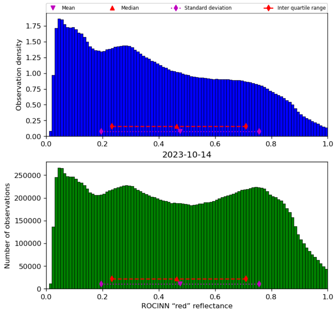
Figure 53: Histogram of “ROCINN “red” reflectance” for 2023-10-13 to 2023-10-15
