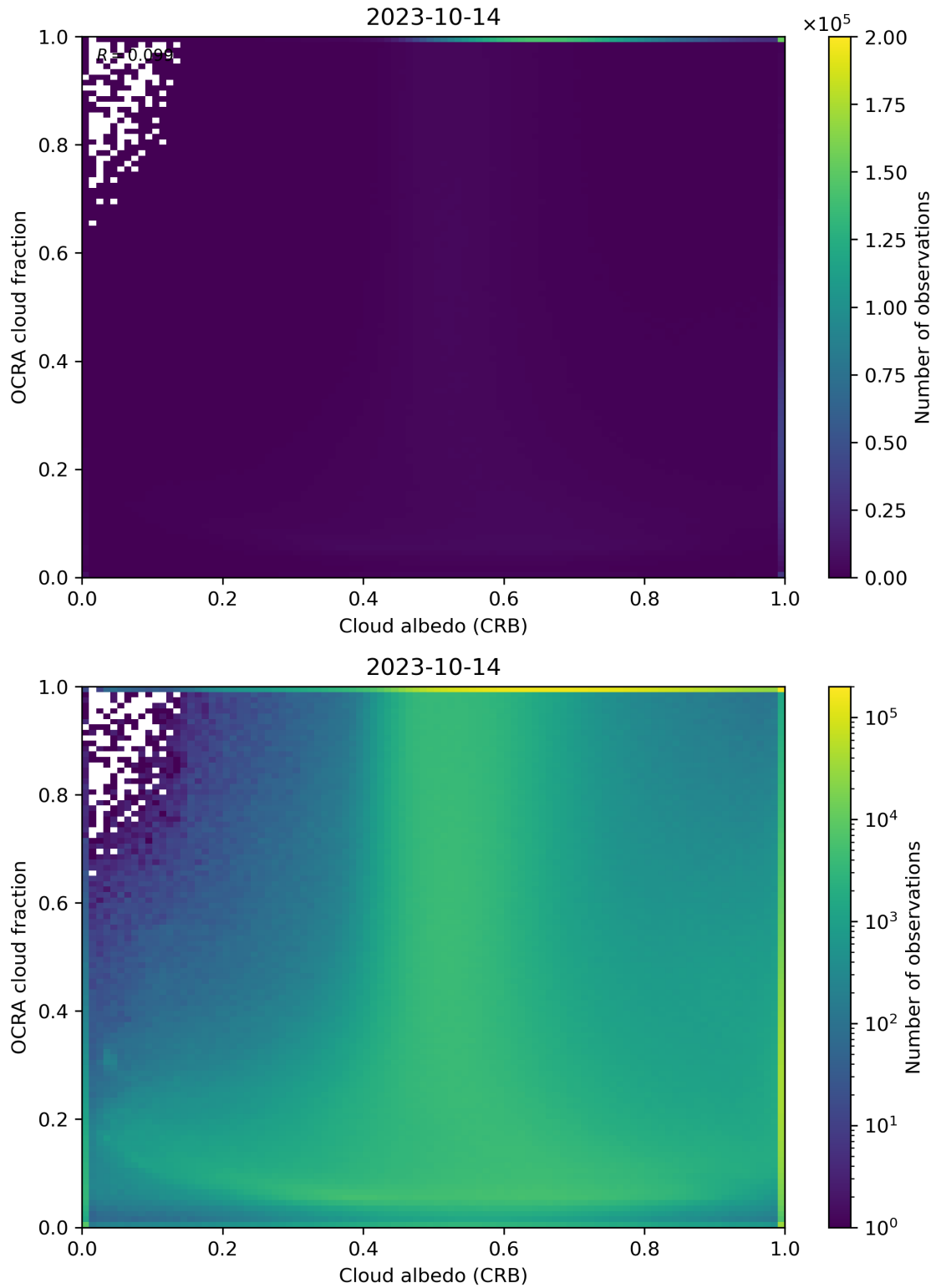
Figure 70: Scatter density plot of “Cloud albedo (CRB)” against “OCRA cloud fraction” for 2023-10-13 to 2023-10-15.
