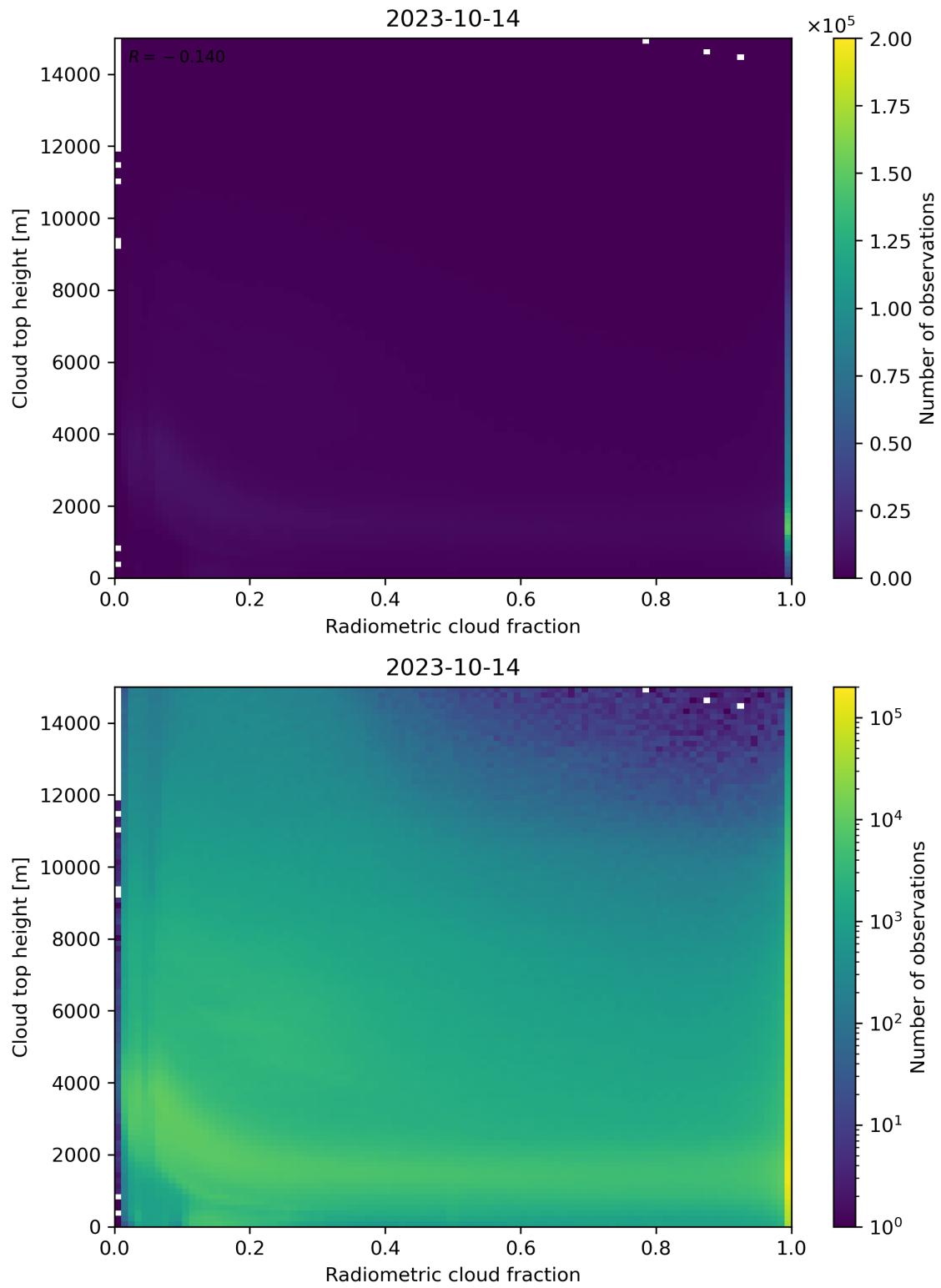
Figure 76: Scatter density plot of “Radiometric cloud fraction” against “Cloud top height” for 2023-10-13 to 2023-10-15.
