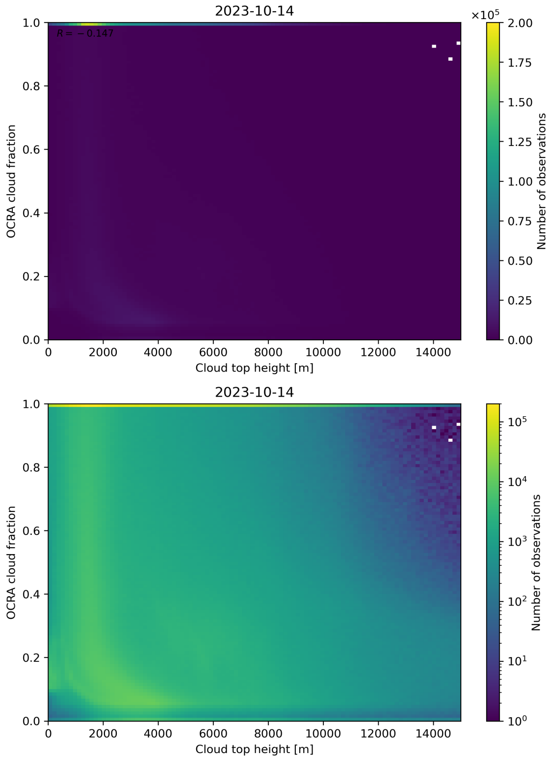
Figure 87: Scatter density plot of “Cloud top height” against “OCRA cloud fraction” for 2023-10-13 to 2023-10-15.
