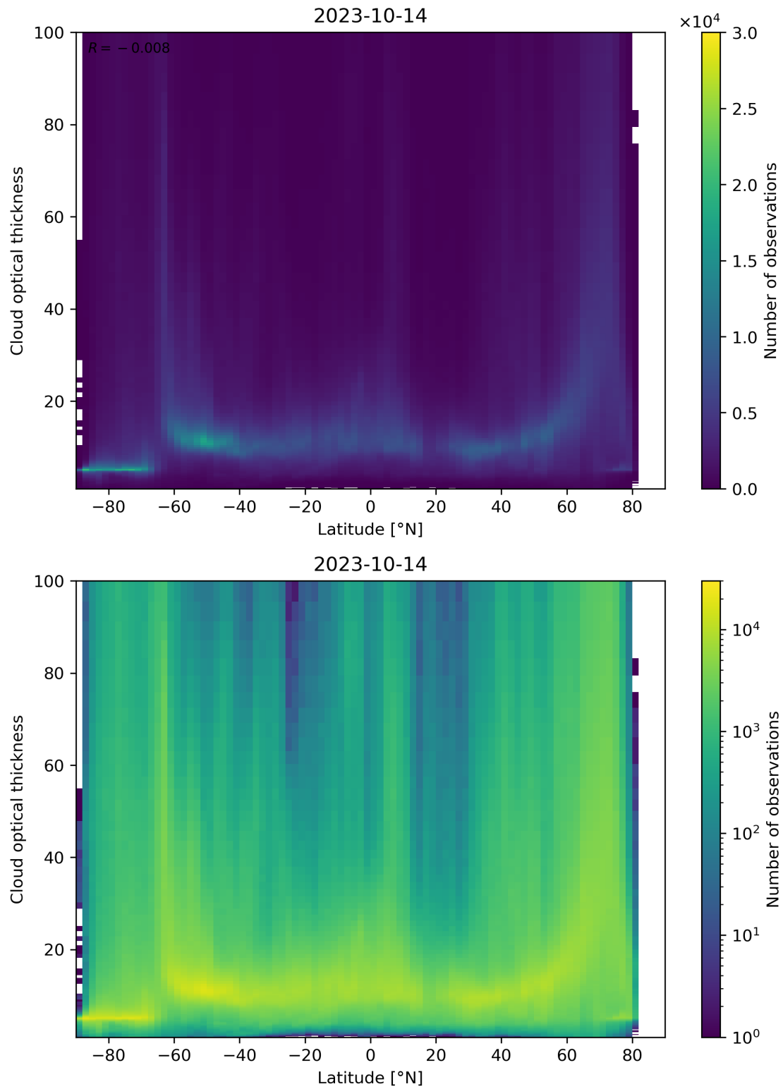
Figure 96: Scatter density plot of “Latitude” against “Cloud optical thickness” for 2023-10-13 to 2023-10-15.
