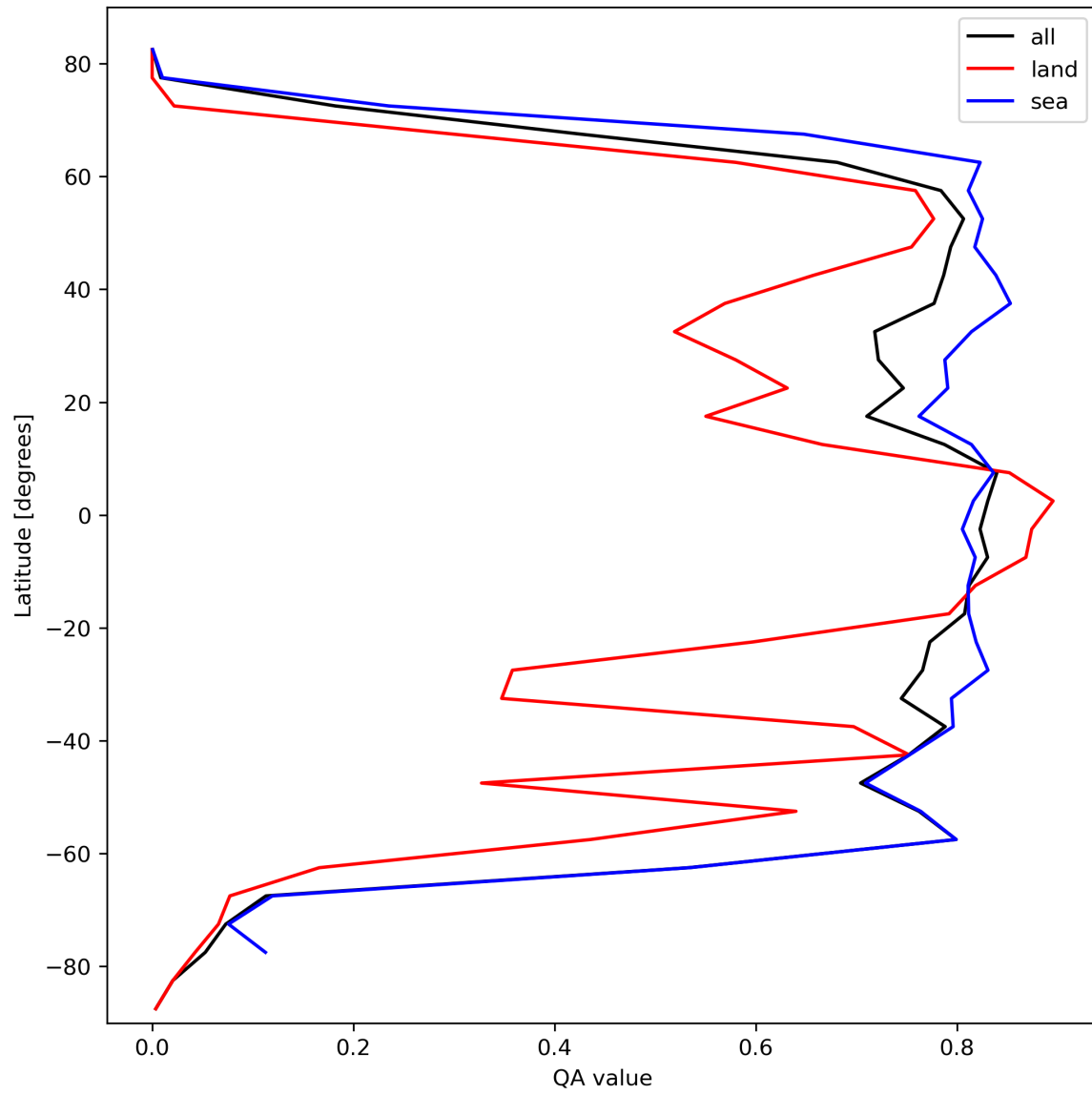
Figure 22: Zonal average of “QA value” for 2023-10-13 to 2023-10-15.
