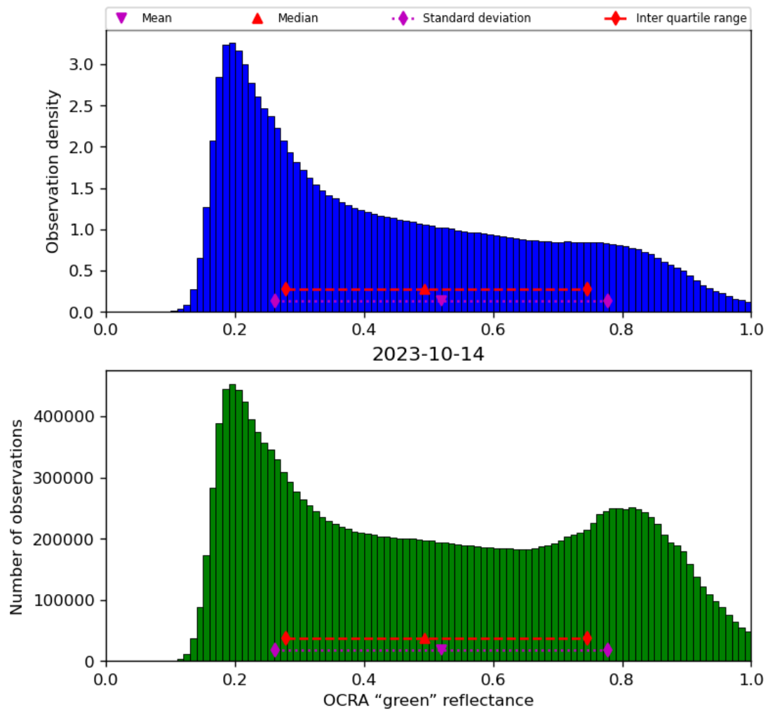
Figure 52: Histogram of “OCRA “green” reflectance” for 2023-10-13 to 2023-10-15
