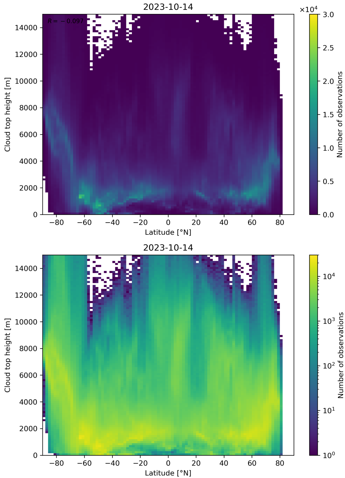
Figure 97: Scatter density plot of “Latitude” against “Cloud top height” for 2023-10-13 to 2023-10-15.
