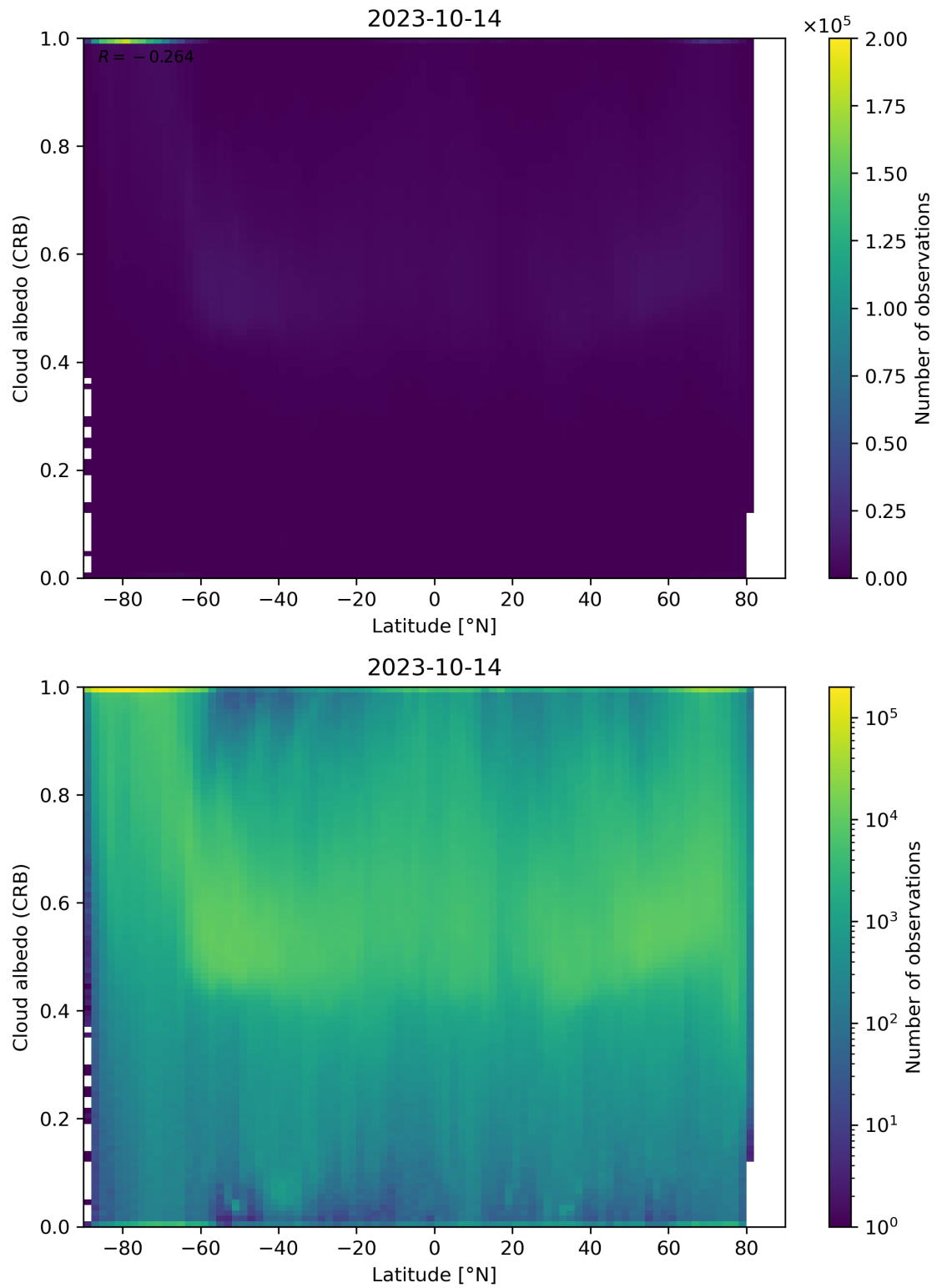
Figure 91: Scatter density plot of “Latitude” against “Cloud albedo (CRB)” for 2023-10-13 to 2023-10-15.
