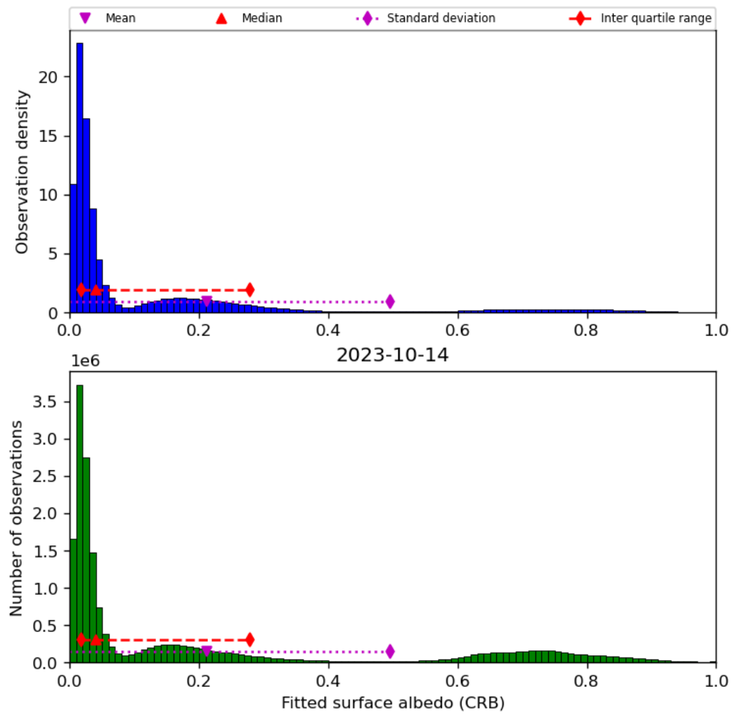
Figure 46: Histogram of “Fitted surface albedo (CRB)” for 2023-10-13 to 2023-10-15
