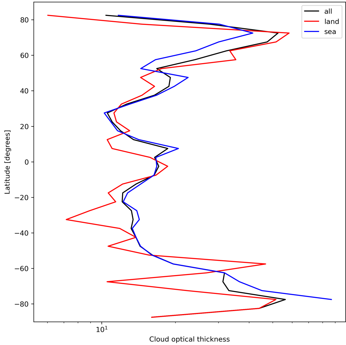
Figure 25: Zonal average of “Cloud optical thickness” for 2023-10-13 to 2023-10-15.
