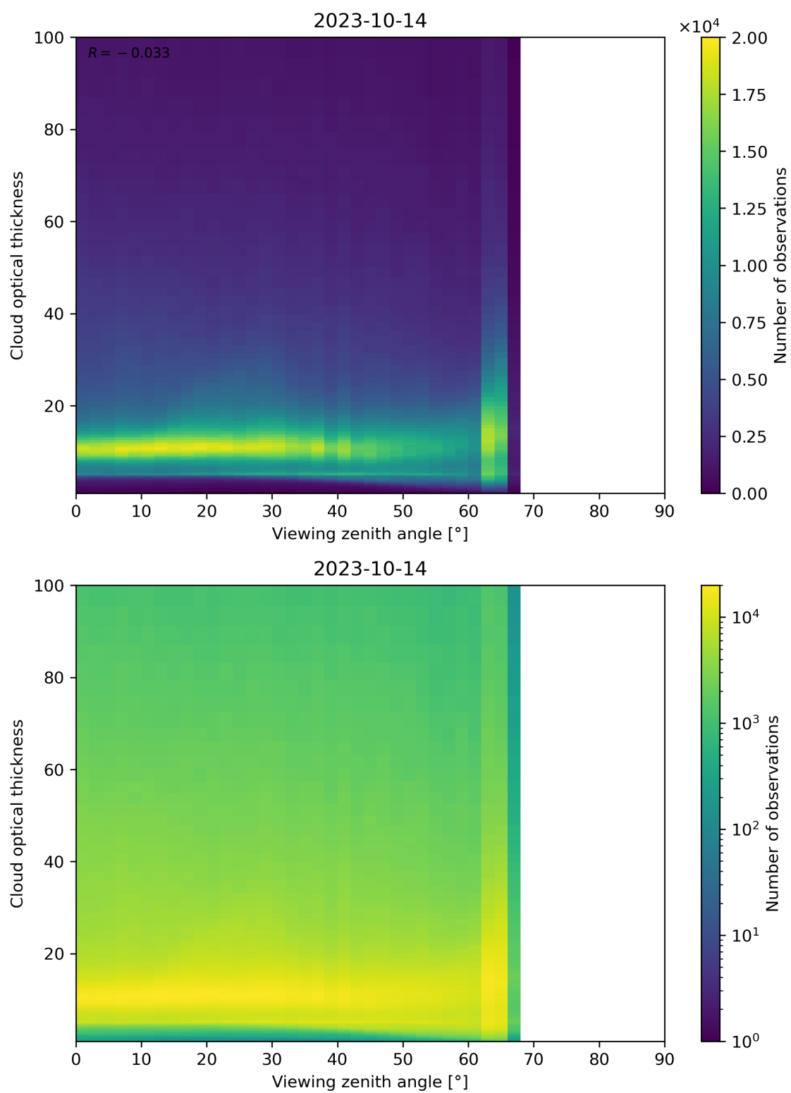
Figure 111: Scatter density plot of “Viewing zenith angle” against “Cloud optical thickness” for 2023-10-13 to 2023-10-15.
