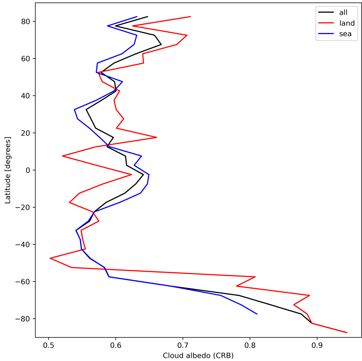
Figure 28: Zonal average of “Cloud albedo (CRB)” for 2023-10-13 to 2023-10-15.
