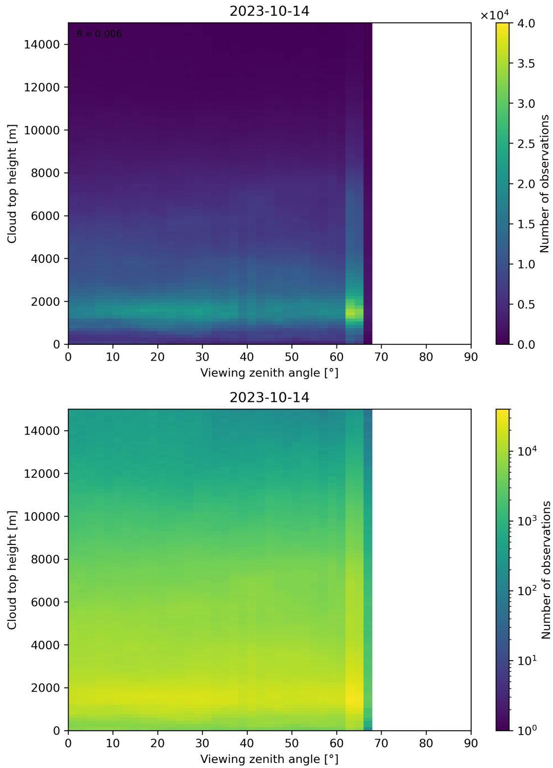
Figure 112: Scatter density plot of “Viewing zenith angle” against “Cloud top height” for 2023-10-13 to 2023-10-15.
