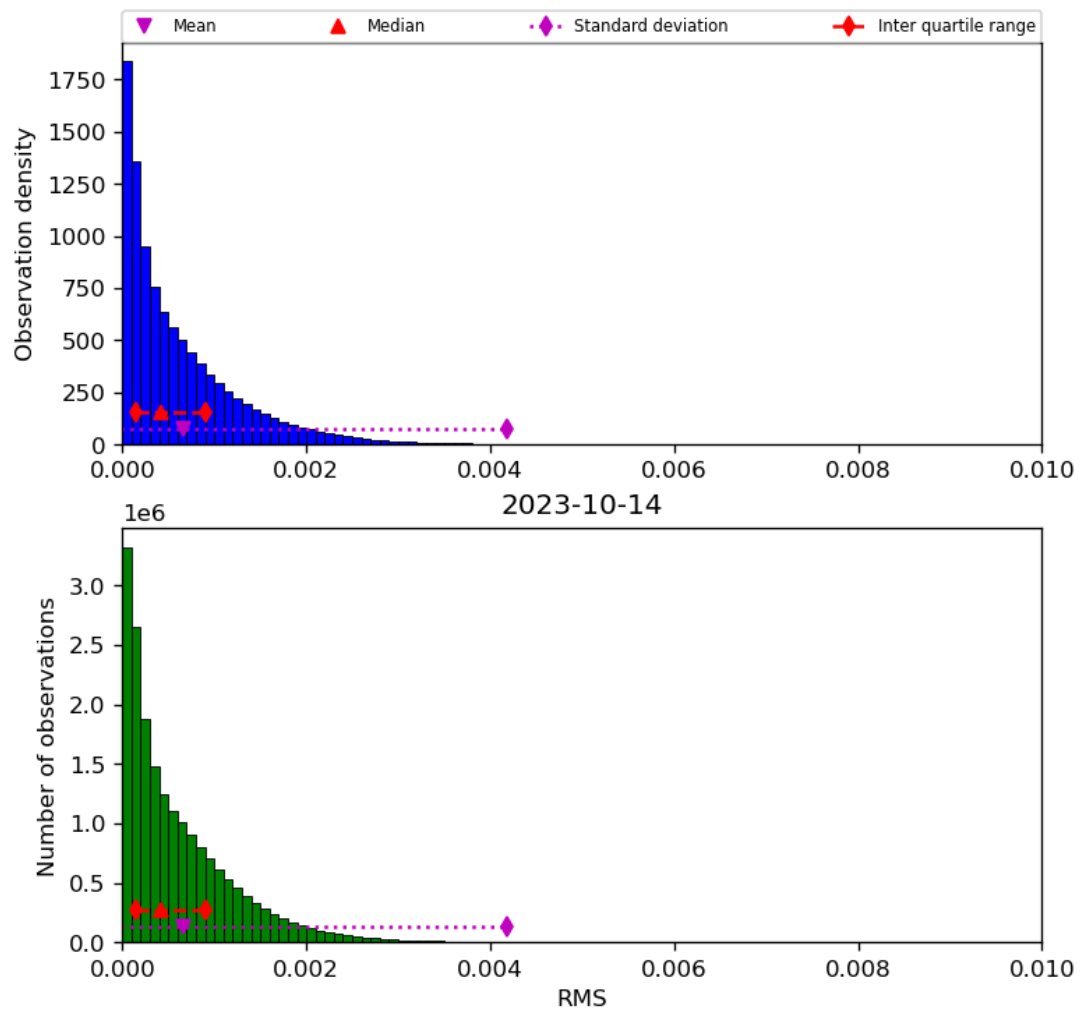
Figure 47: Histogram of “RMS” for 2023-10-13 to 2023-10-15
