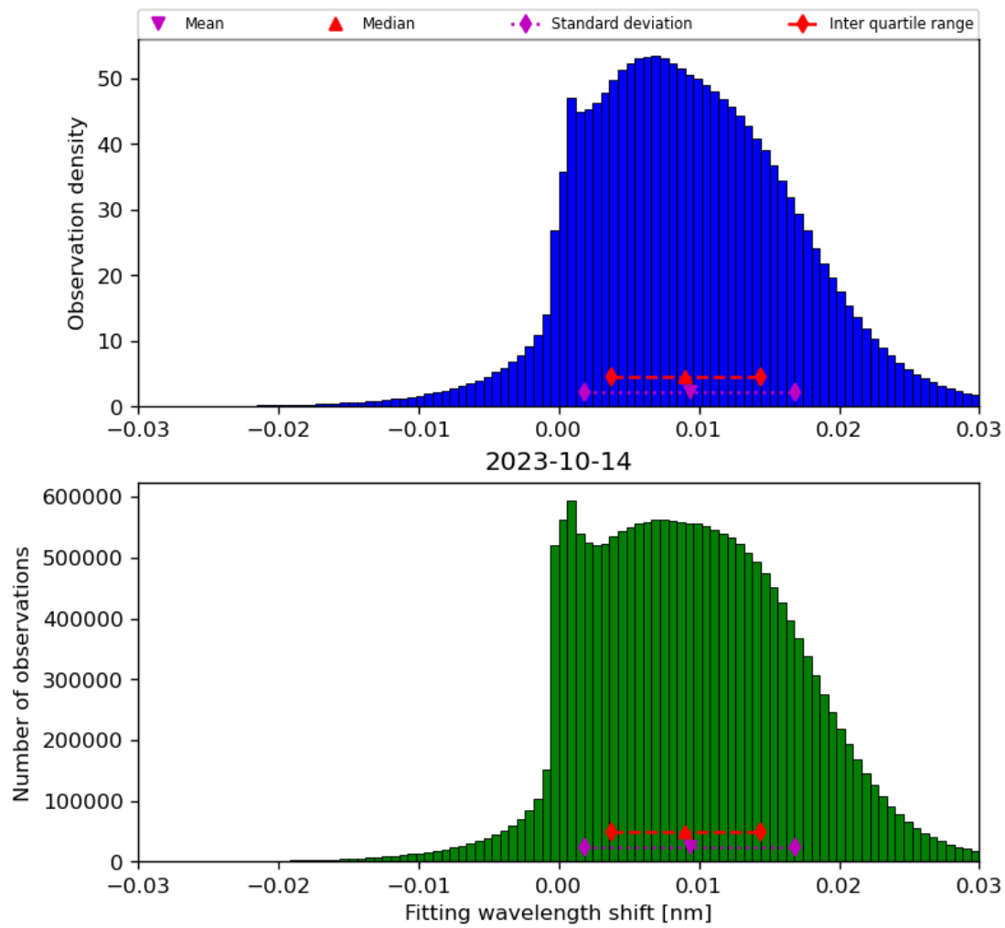
Figure 49: Histogram of “Fitting wavelength shift” for 2023-10-13 to 2023-10-15
