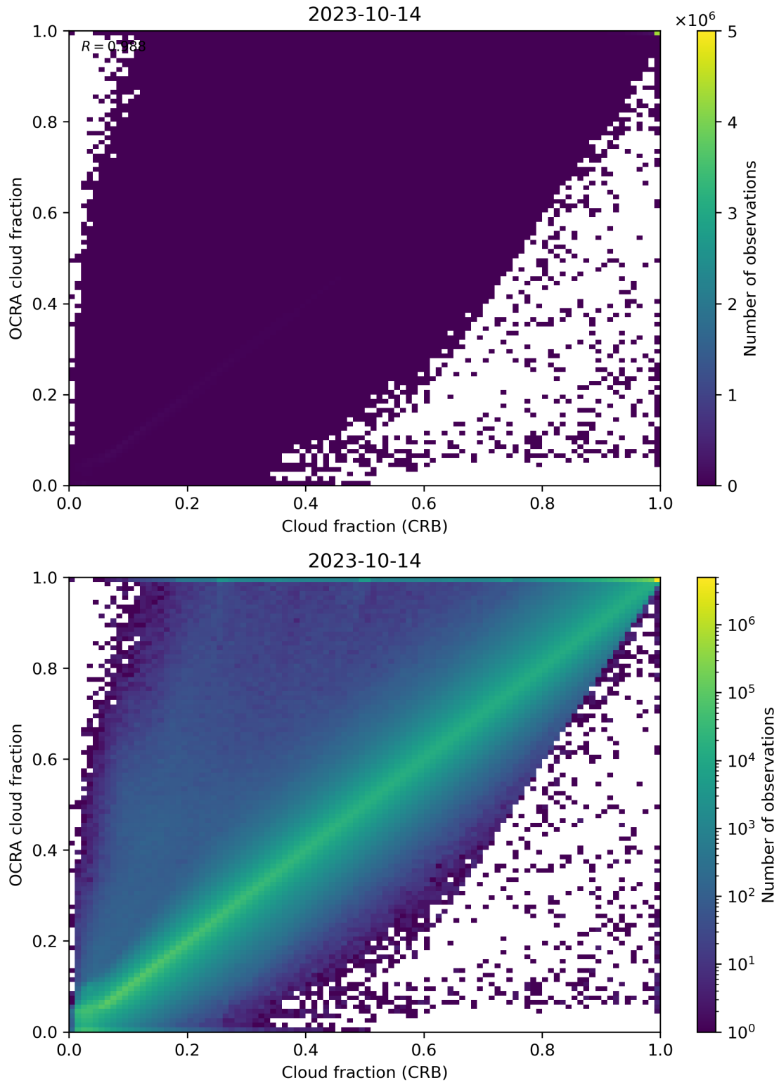
Figure 78: Scatter density plot of “Cloud fraction (CRB)” against “OCRA cloud fraction” for 2023-10-13 to 2023-10-15.
