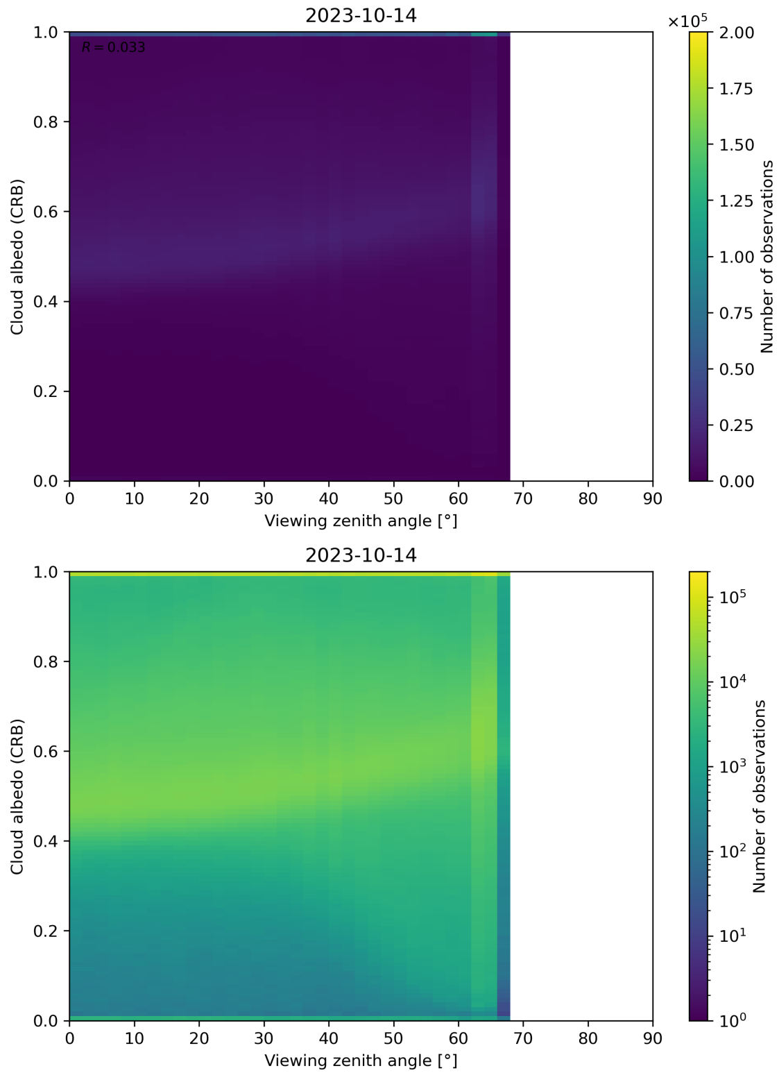
Figure 106: Scatter density plot of “Viewing zenith angle” against “Cloud albedo (CRB)” for 2023-10-13 to 2023-10-15.
