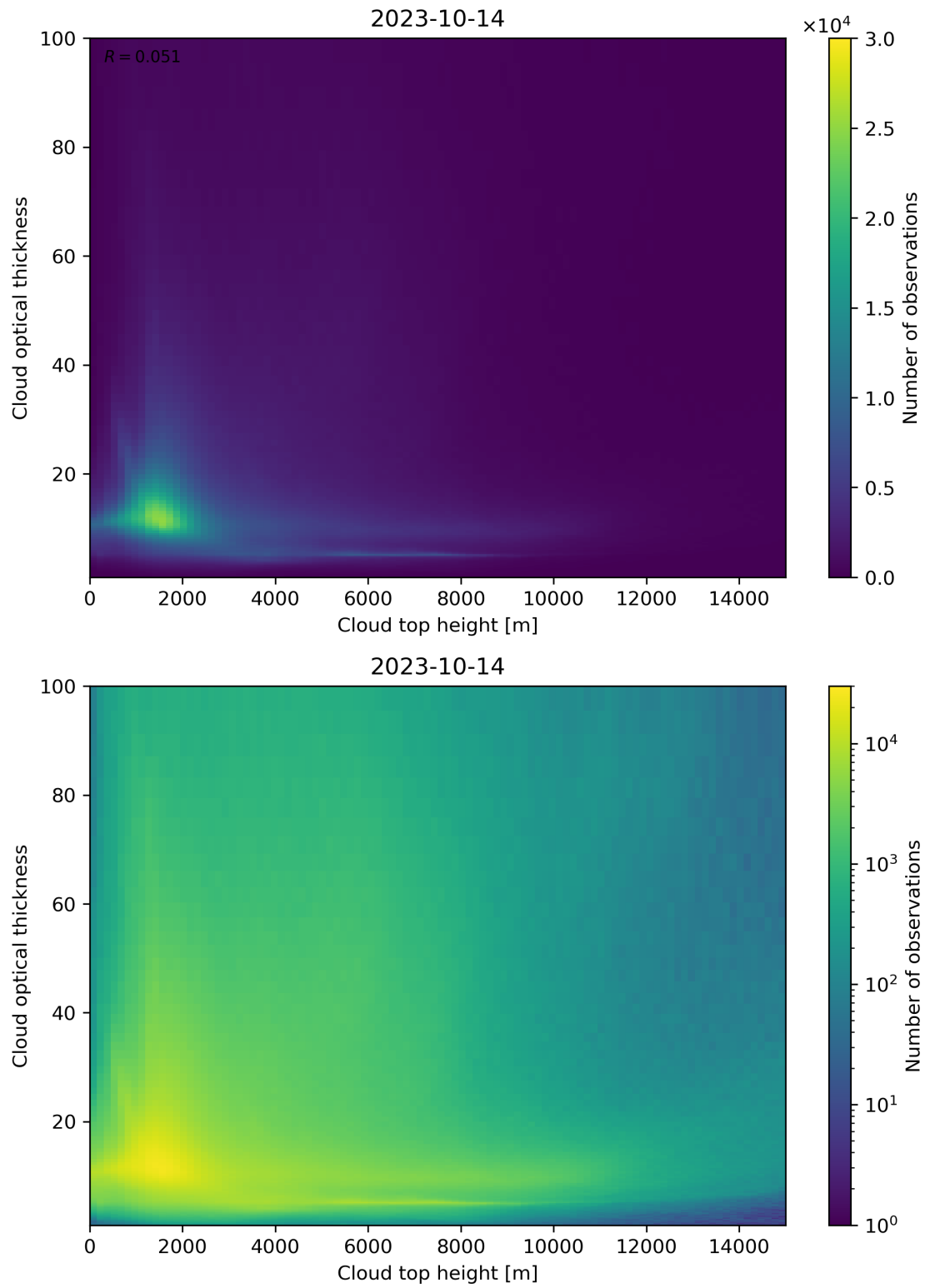
Figure 90: Scatter density plot of “Cloud top height” against “Cloud optical thickness” for 2023-10-13 to 2023-10-15.
