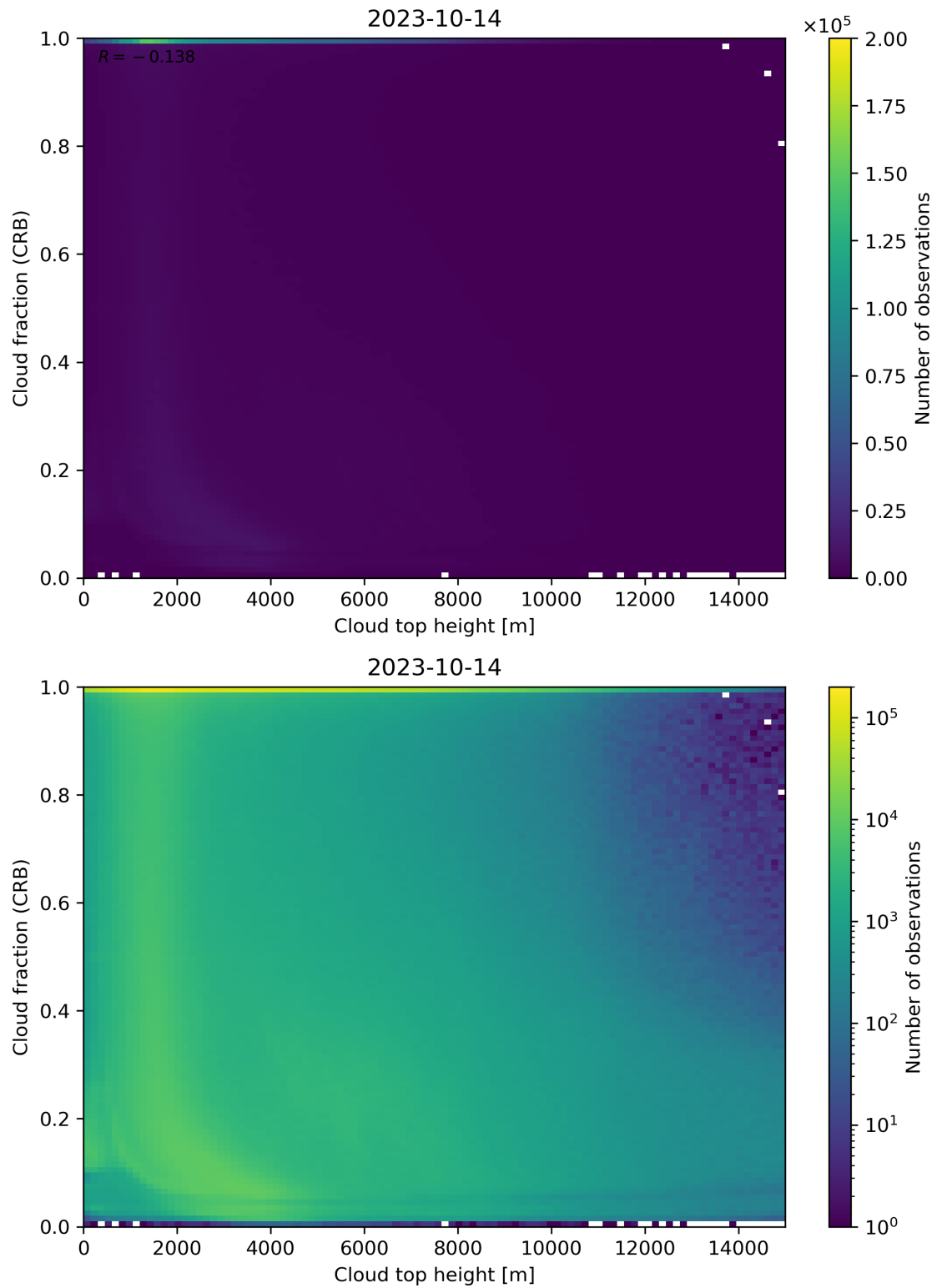
Figure 88: Scatter density plot of “Cloud top height” against “Cloud fraction (CRB)” for 2023-10-13 to 2023-10-15.
