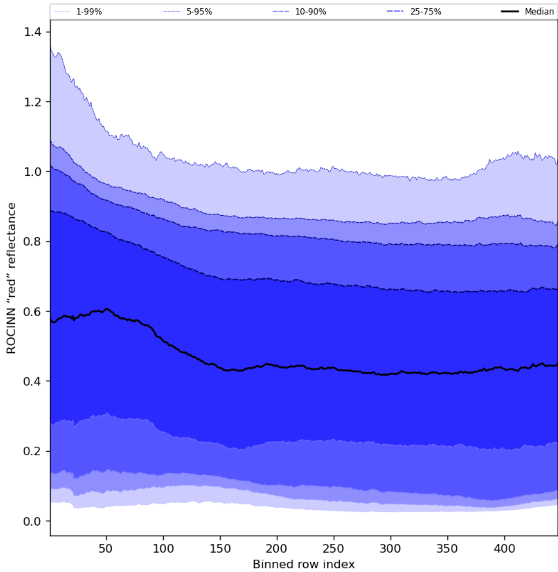
Figure 69: Along track statistics of “ROCINN “red” reflectance” for 2023-10-13 to 2023-10-15
