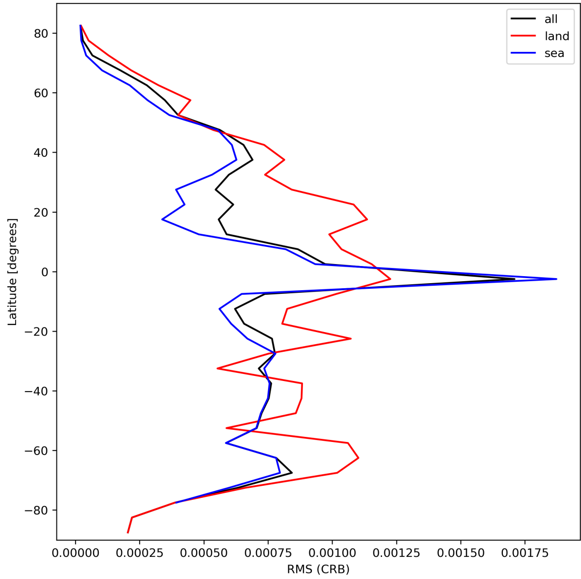
Figure 32: Zonal average of “RMS (CRB)” for 2023-10-13 to 2023-10-15.
