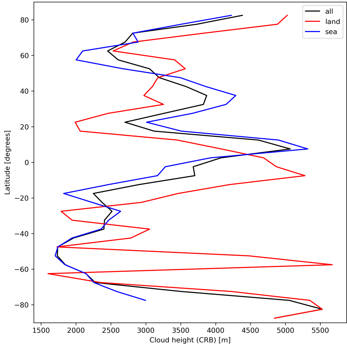
Figure 27: Zonal average of “Cloud height (CRB)” for 2023-10-13 to 2023-10-15.
