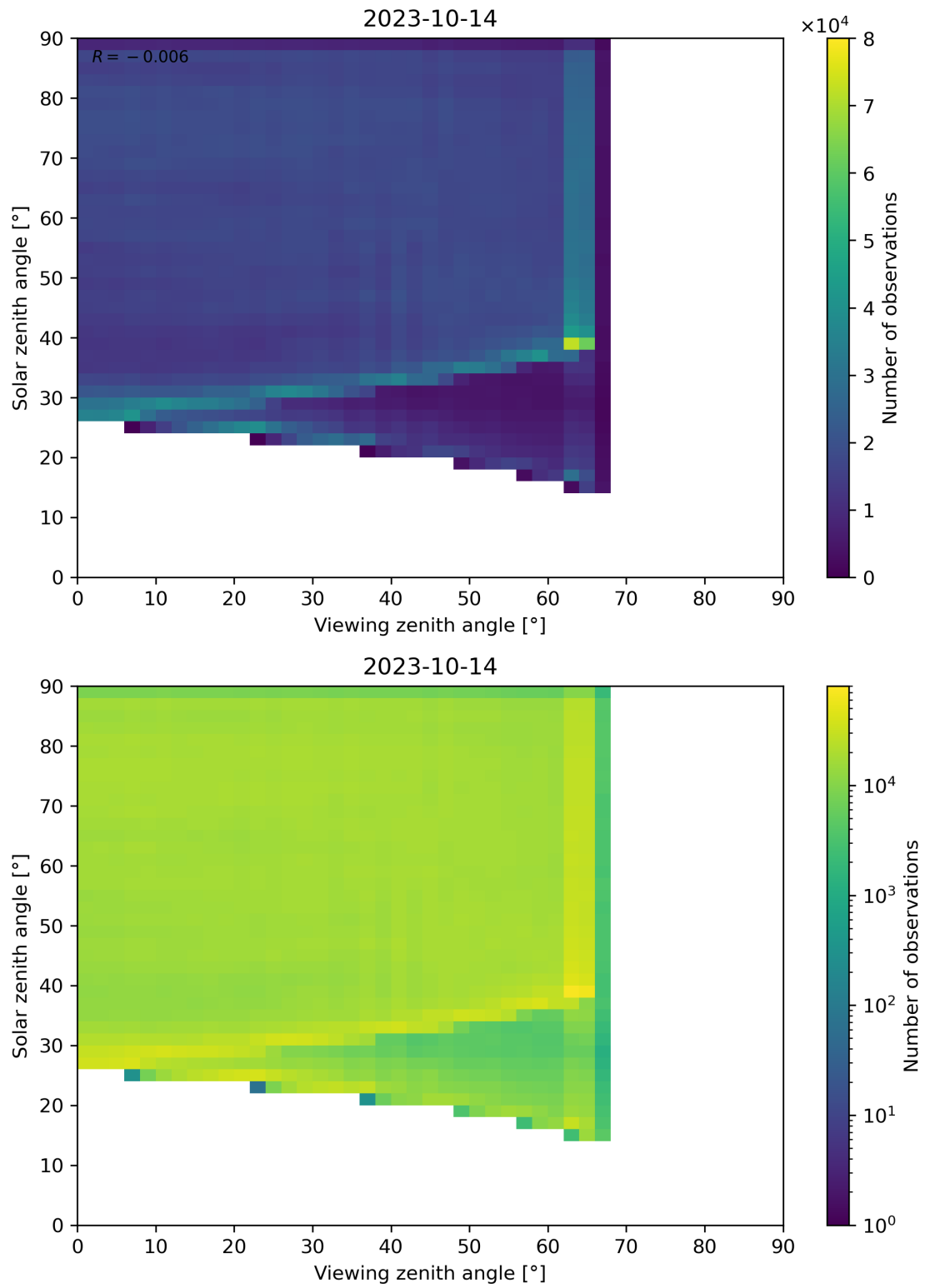
Figure 114: Scatter density plot of “Viewing zenith angle” against “Solar zenith angle” for 2023-10-13 to 2023-10-15.
