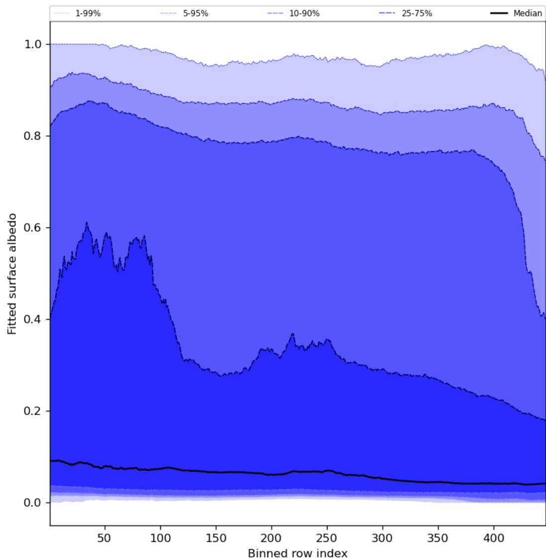
Figure 61: Along track statistics of “Fitted surface albedo” for 2023-10-13 to 2023-10-15
