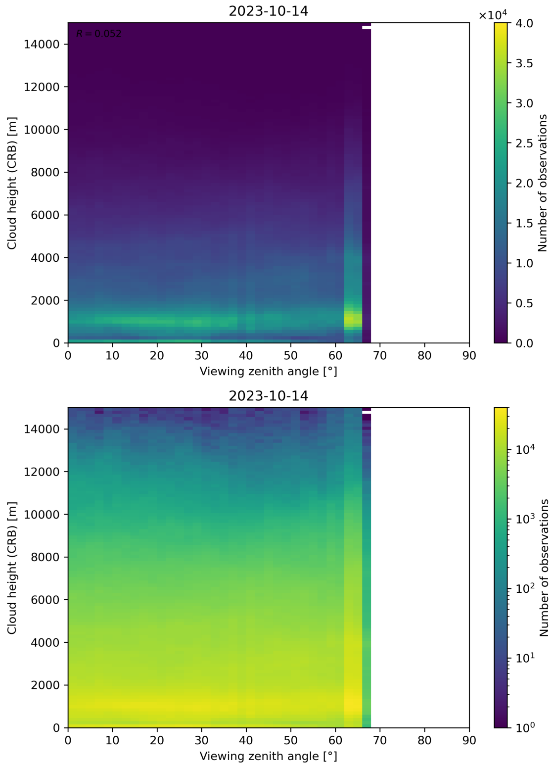
Figure 110: Scatter density plot of “Viewing zenith angle” against “Cloud height (CRB)” for 2023-10-13 to 2023-10-15.
