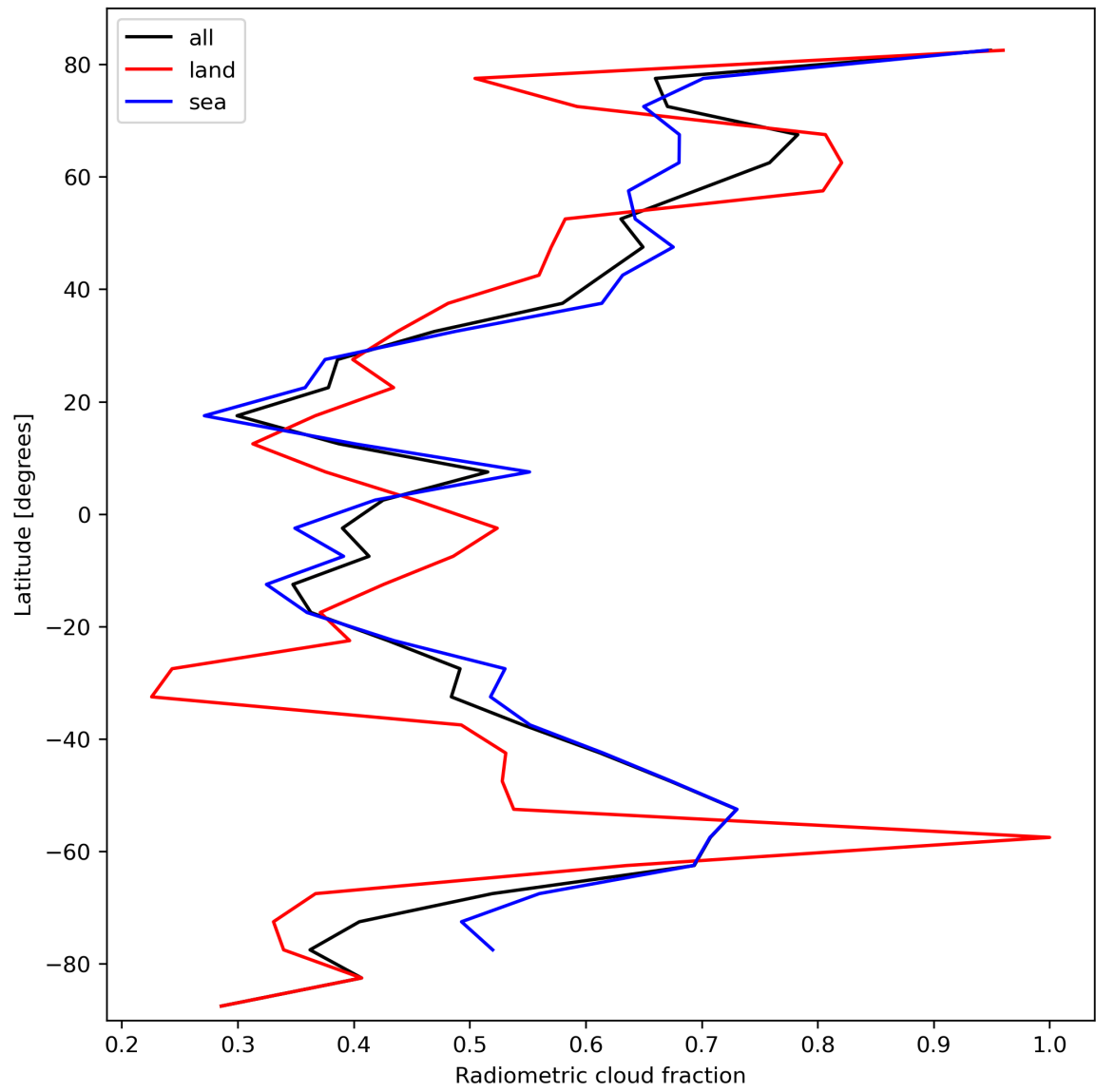
Figure 23: Zonal average of “Radiometric cloud fraction” for 2023-10-13 to 2023-10-15.
