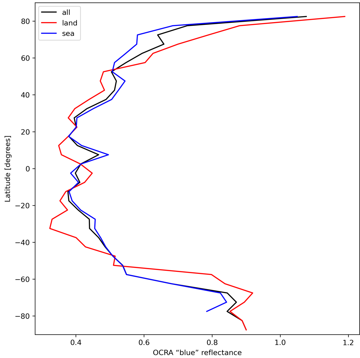
Figure 35: Zonal average of “OCRA “blue” reflectance” for 2023-10-13 to 2023-10-15.
