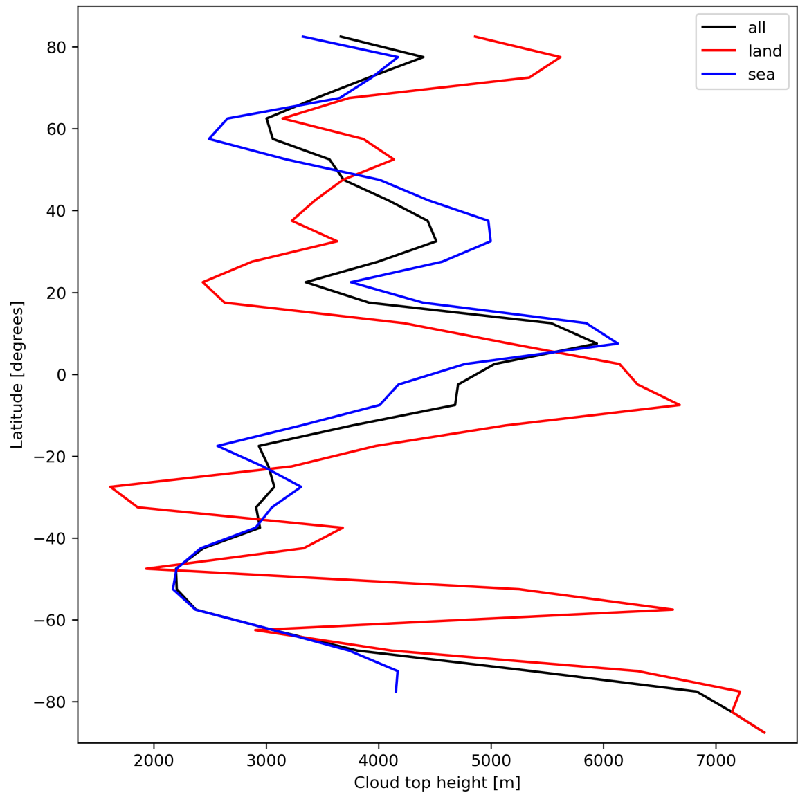
Figure 24: Zonal average of “Cloud top height” for 2023-10-13 to 2023-10-15.
