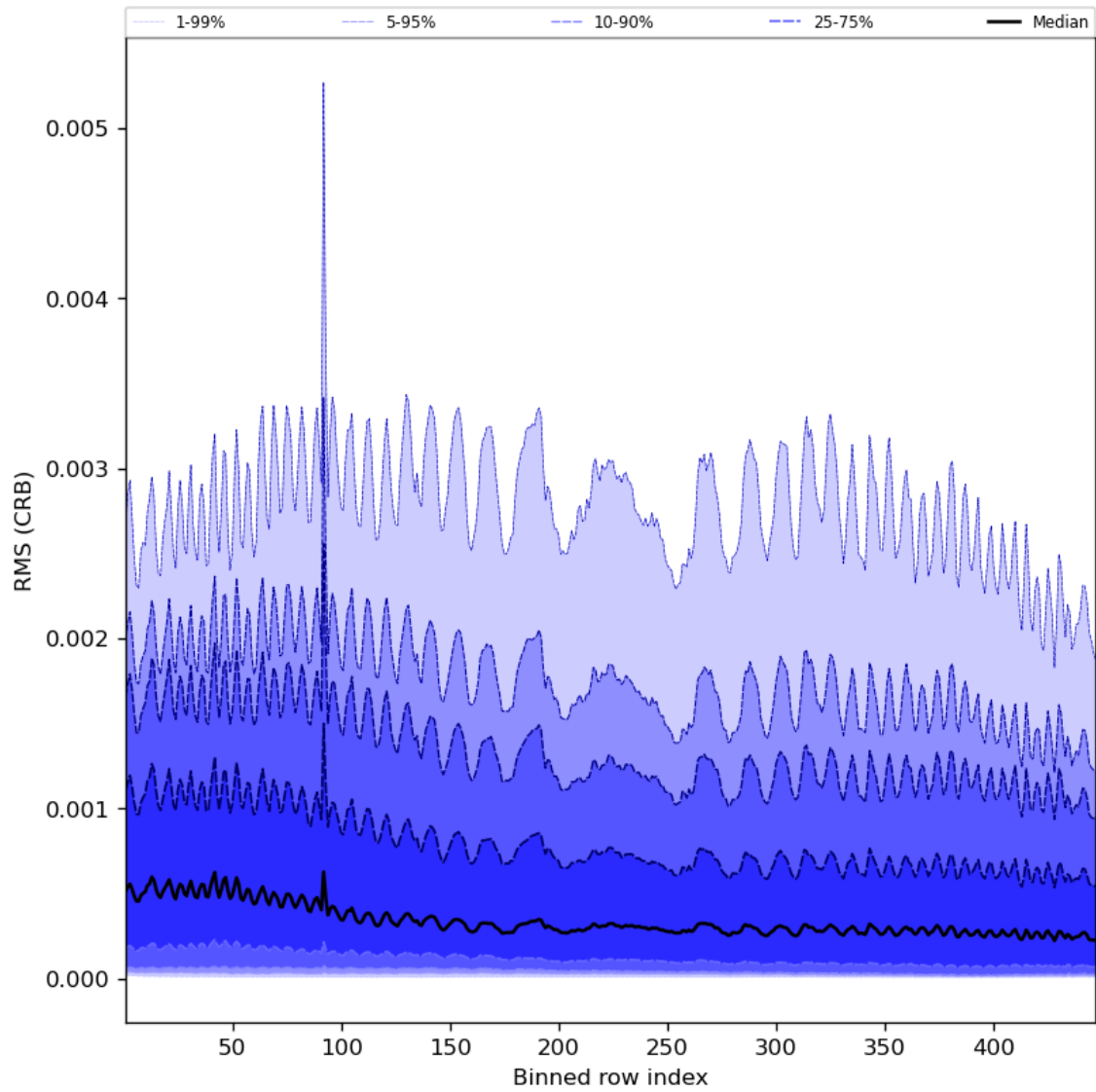
Figure 64: Along track statistics of “RMS (CRB)” for 2023-10-13 to 2023-10-15
