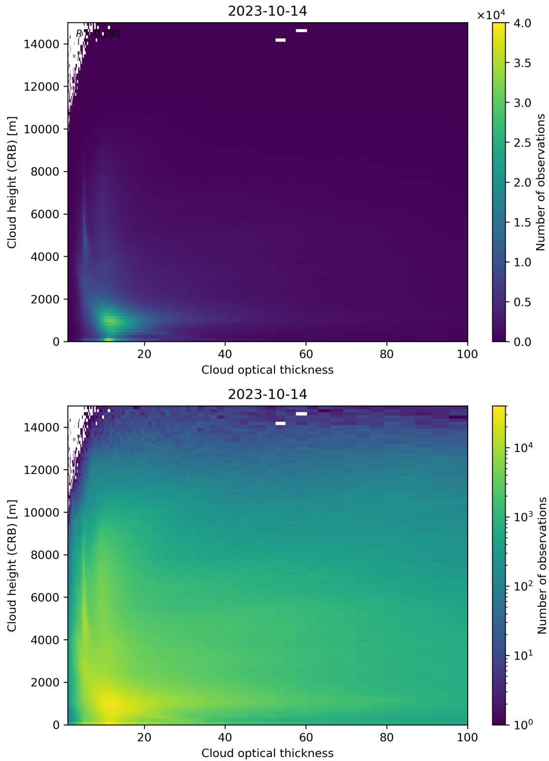
Figure 85: Scatter density plot of “Cloud optical thickness” against “Cloud height (CRB)” for 2023-10-13 to 2023-10-15.
