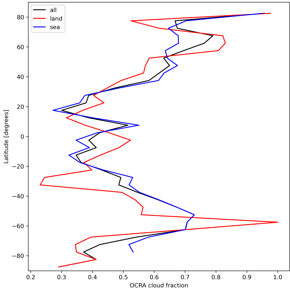
Figure 34: Zonal average of “OCRA cloud fraction” for 2023-10-13 to 2023-10-15.
