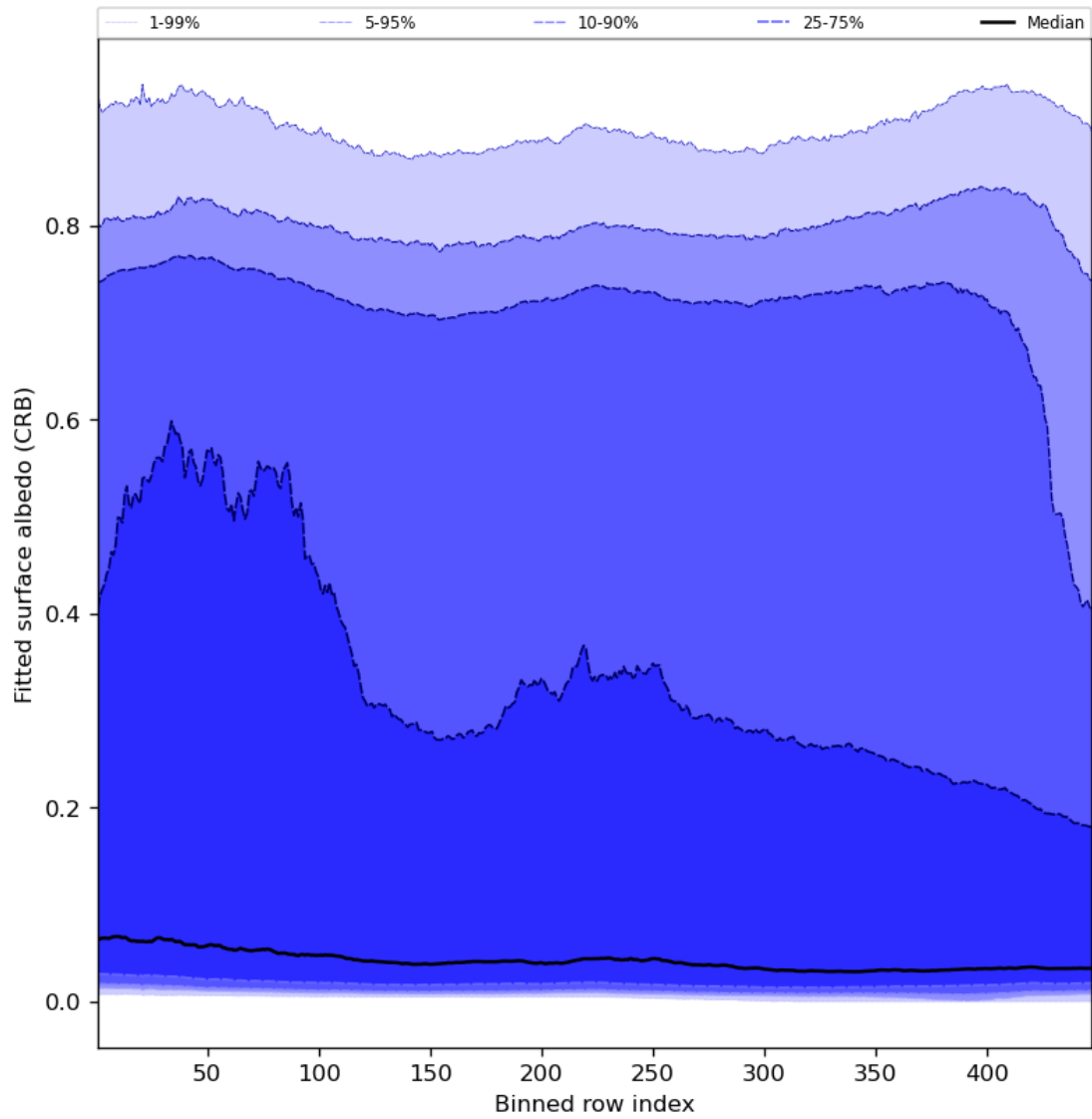
Figure 62: Along track statistics of “Fitted surface albedo (CRB)” for 2023-10-13 to 2023-10-15
