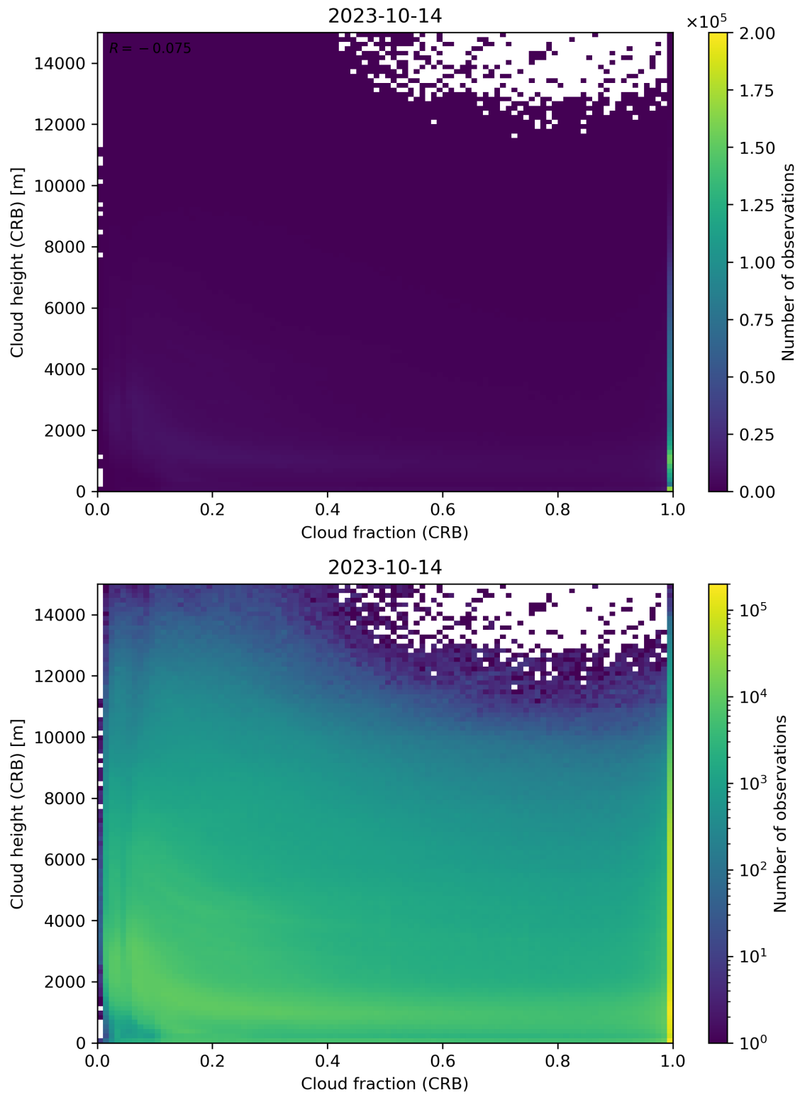
Figure 79: Scatter density plot of “Cloud fraction (CRB)” against “Cloud height (CRB)” for 2023-10-13 to 2023-10-15.
