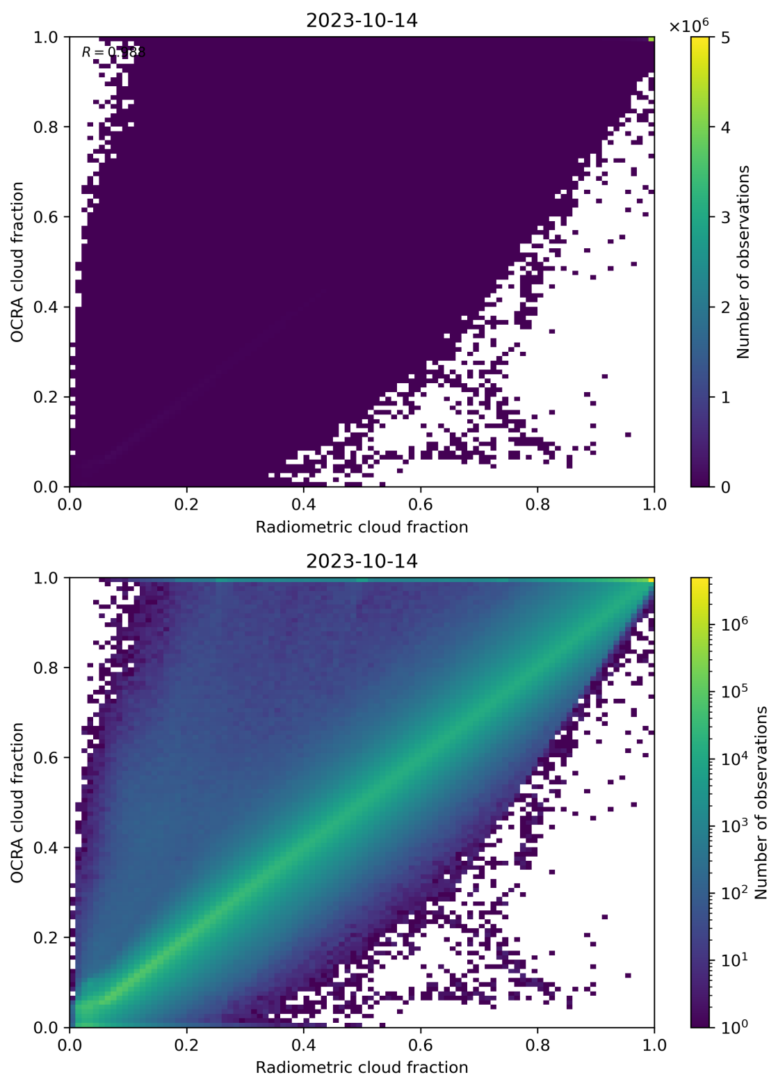
Figure 72: Scatter density plot of “Radiometric cloud fraction” against “OCRA cloud fraction” for 2023-10-13 to 2023-10-15.
