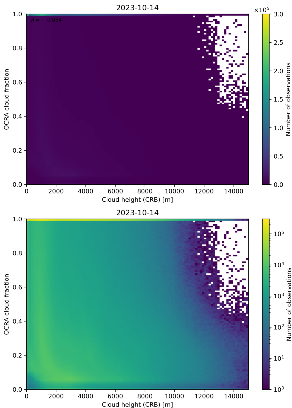
Figure 81: Scatter density plot of “Cloud height (CRB)” against “OCRA cloud fraction” for 2023-10-13 to 2023-10-15.
