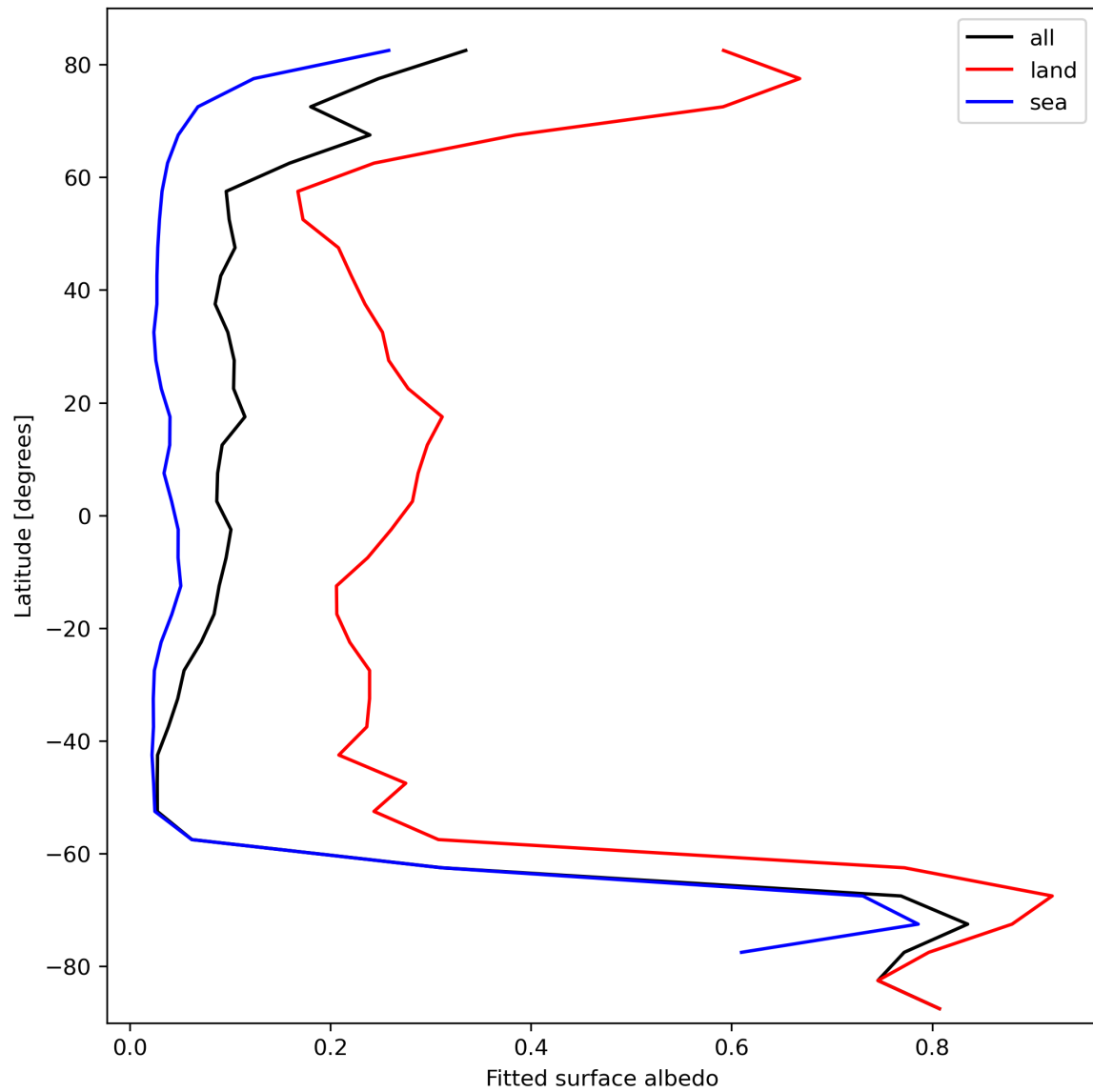
Figure 29: Zonal average of “Fitted surface albedo” for 2023-10-13 to 2023-10-15.
