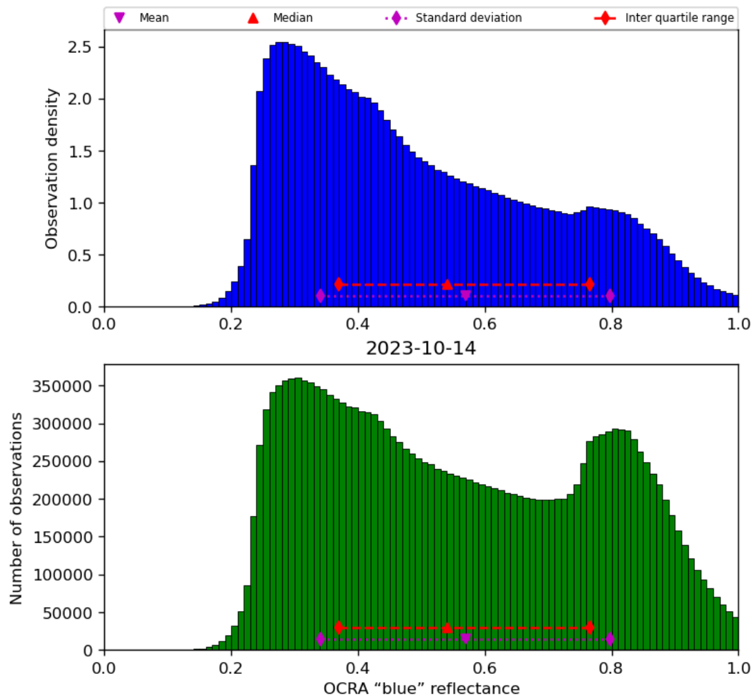
Figure 51: Histogram of “OCRA “blue” reflectance” for 2023-10-13 to 2023-10-15
