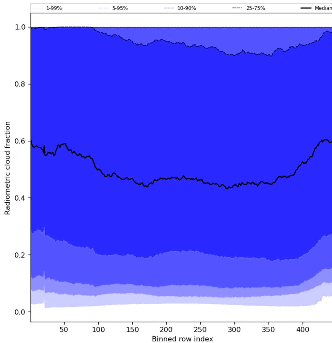
Figure 55: Along track statistics of “Radiometric cloud fraction” for 2023-10-13 to 2023-10-15
