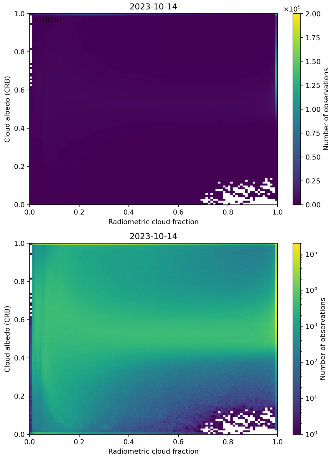
Figure 71: Scatter density plot of “Radiometric cloud fraction” against “Cloud albedo (CRB)” for 2023-10-13 to 2023-10-15.
