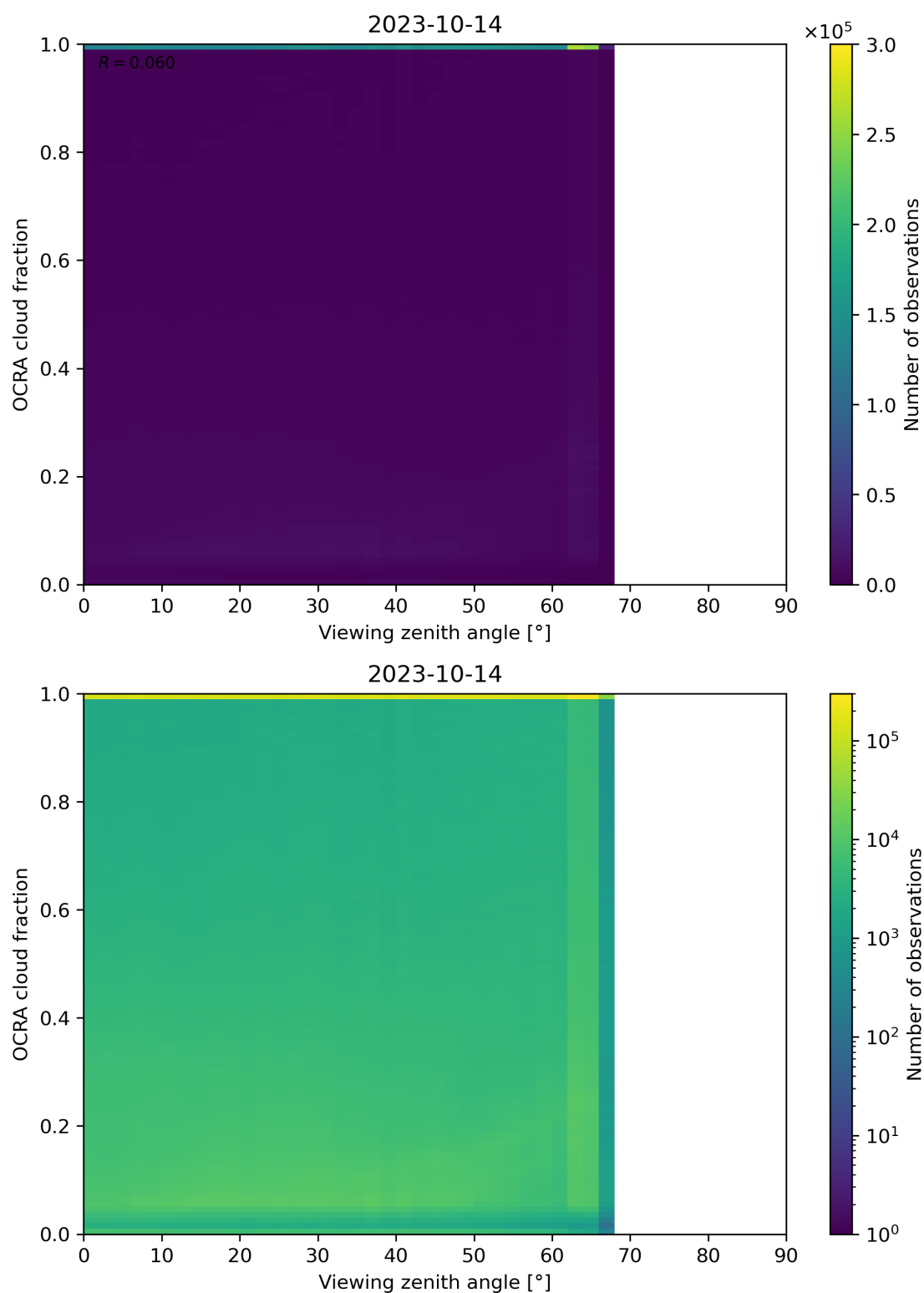
Figure 108: Scatter density plot of “Viewing zenith angle” against “OCRA cloud fraction” for 2023-10-13 to 2023-10-15.
