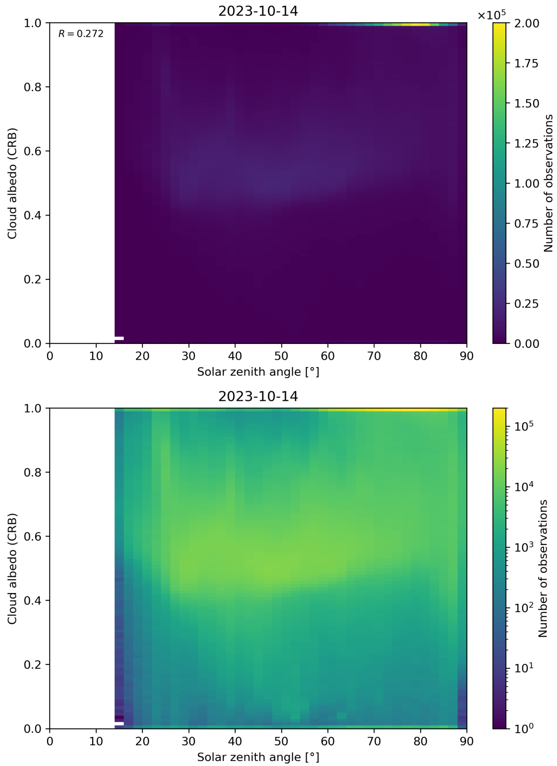
Figure 98: Scatter density plot of “Solar zenith angle” against “Cloud albedo (CRB)” for 2023-10-13 to 2023-10-15.
