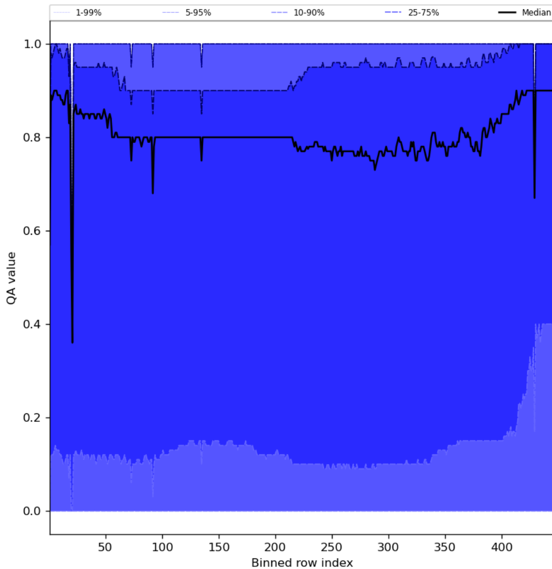
Figure 54: Along track statistics of “QA value” for 2023-10-13 to 2023-10-15
