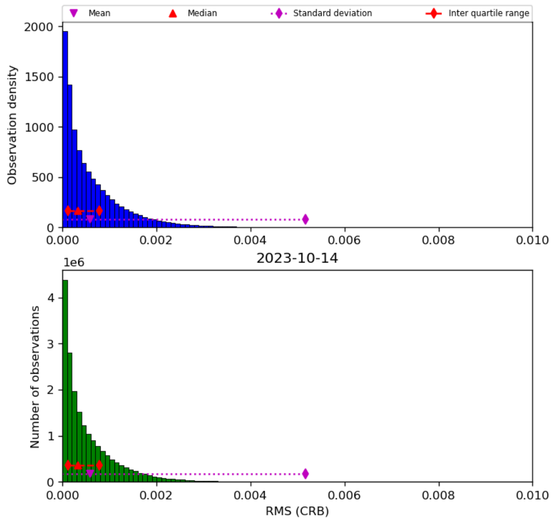
Figure 48: Histogram of “RMS (CRB)” for 2023-10-13 to 2023-10-15
