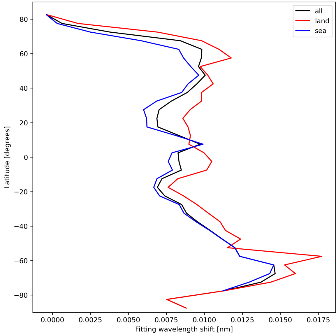
Figure 33: Zonal average of “Fitting wavelength shift” for 2023-10-13 to 2023-10-15.
