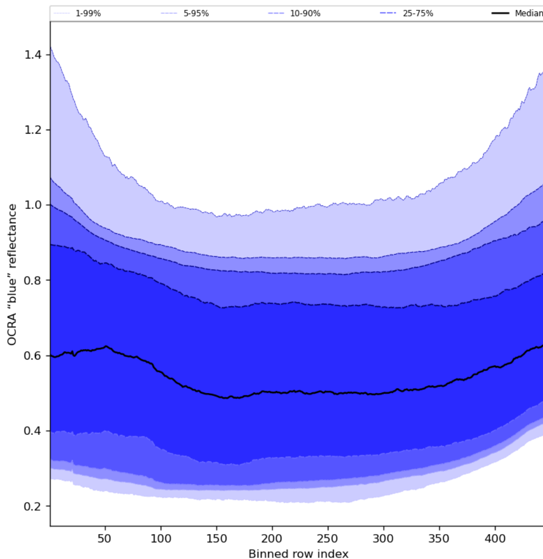
Figure 67: Along track statistics of “OCRA “blue” reflectance” for 2023-10-13 to 2023-10-15
