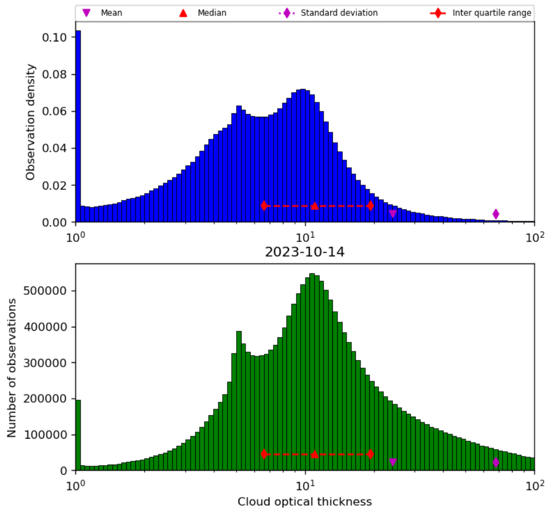
Figure 41: Histogram of “Cloud optical thickness” for 2023-10-13 to 2023-10-15
