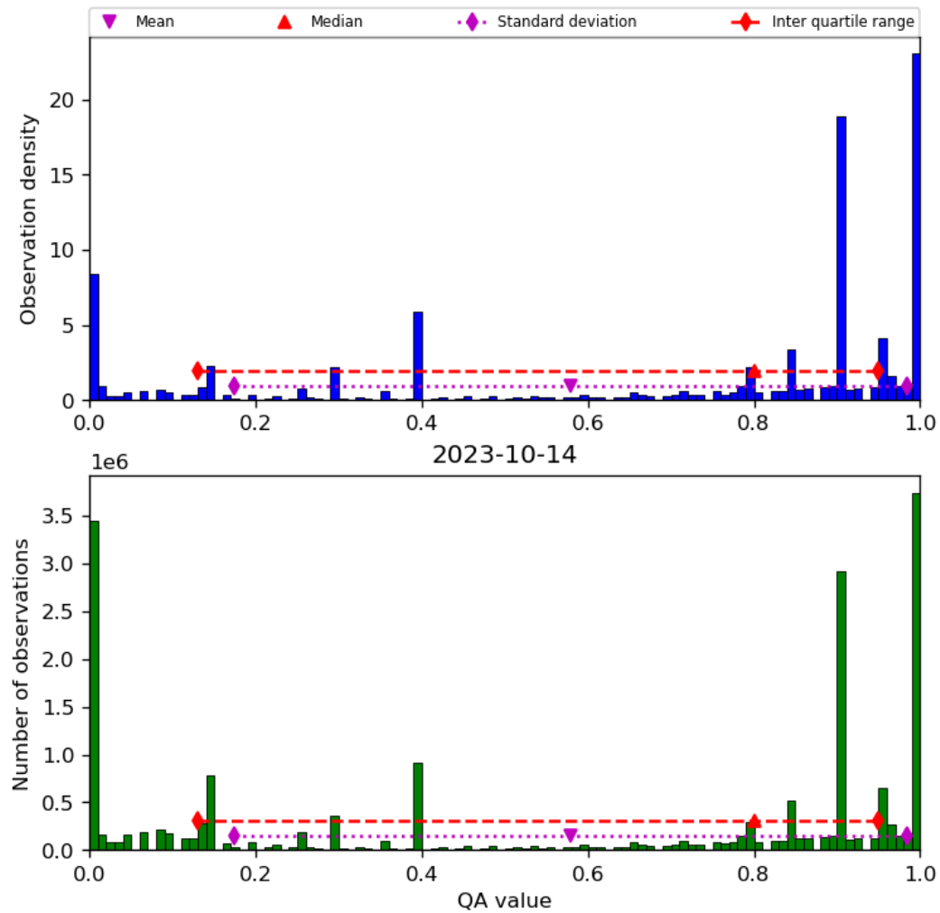
Figure 38: Histogram of “QA value” for 2023-10-13 to 2023-10-15
