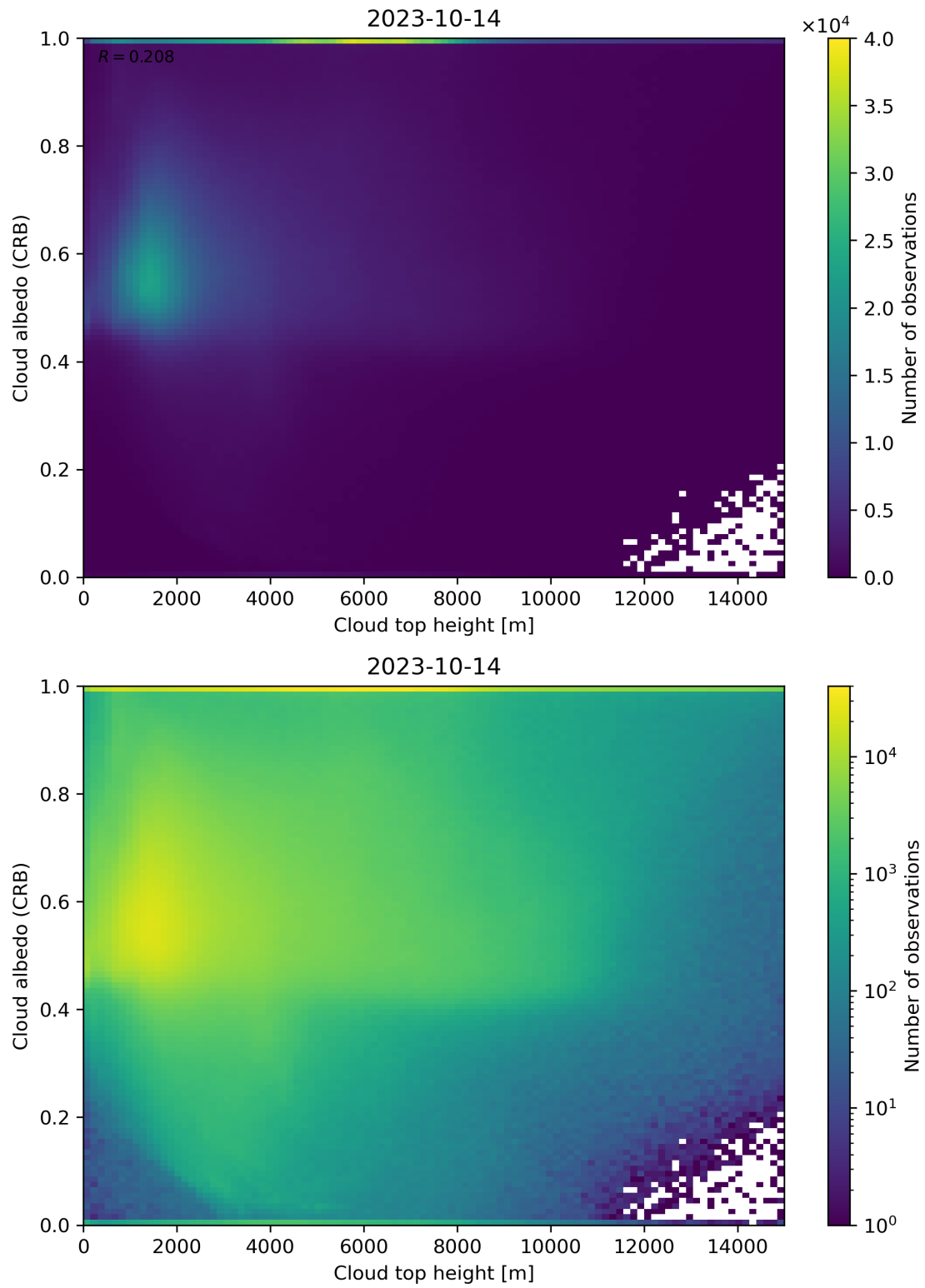
Figure 86: Scatter density plot of “Cloud top height” against “Cloud albedo (CRB)” for 2023-10-13 to 2023-10-15.
