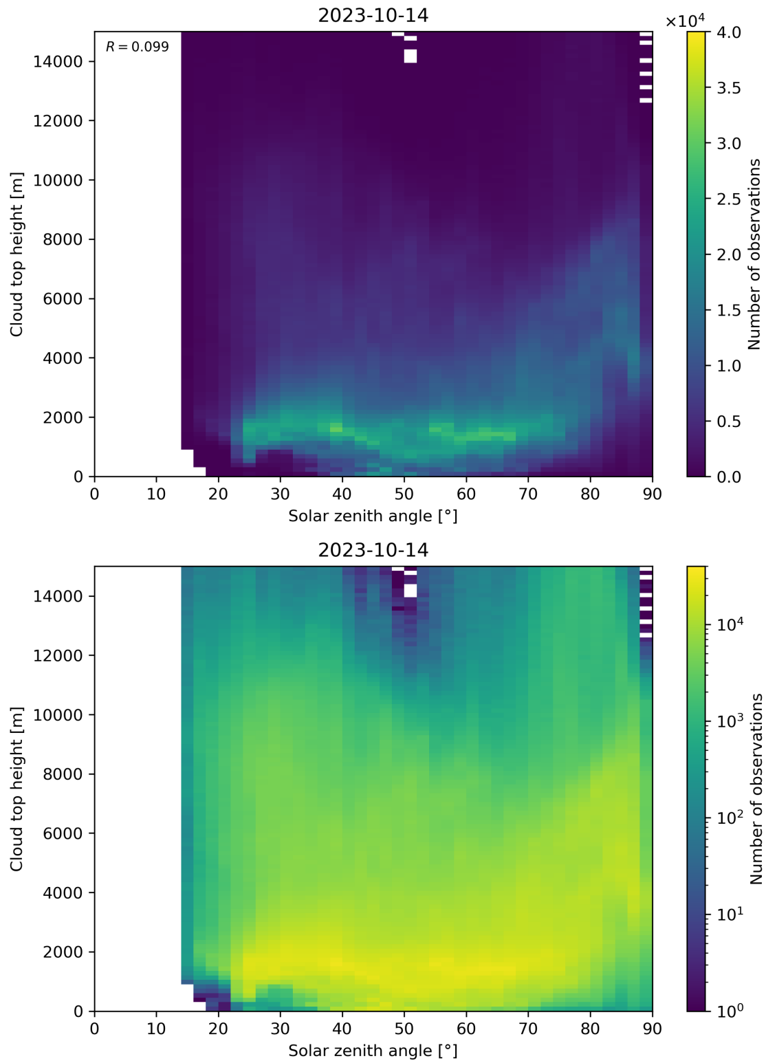
Figure 104: Scatter density plot of “Solar zenith angle” against “Cloud top height” for 2023-10-13 to 2023-10-15.
