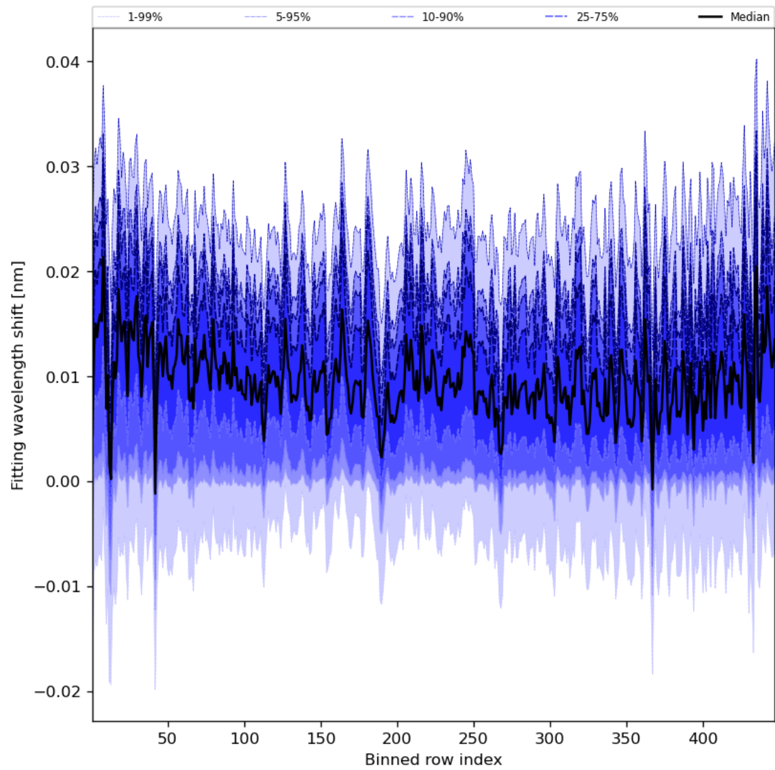
Figure 65: Along track statistics of “Fitting wavelength shift” for 2023-10-13 to 2023-10-15
