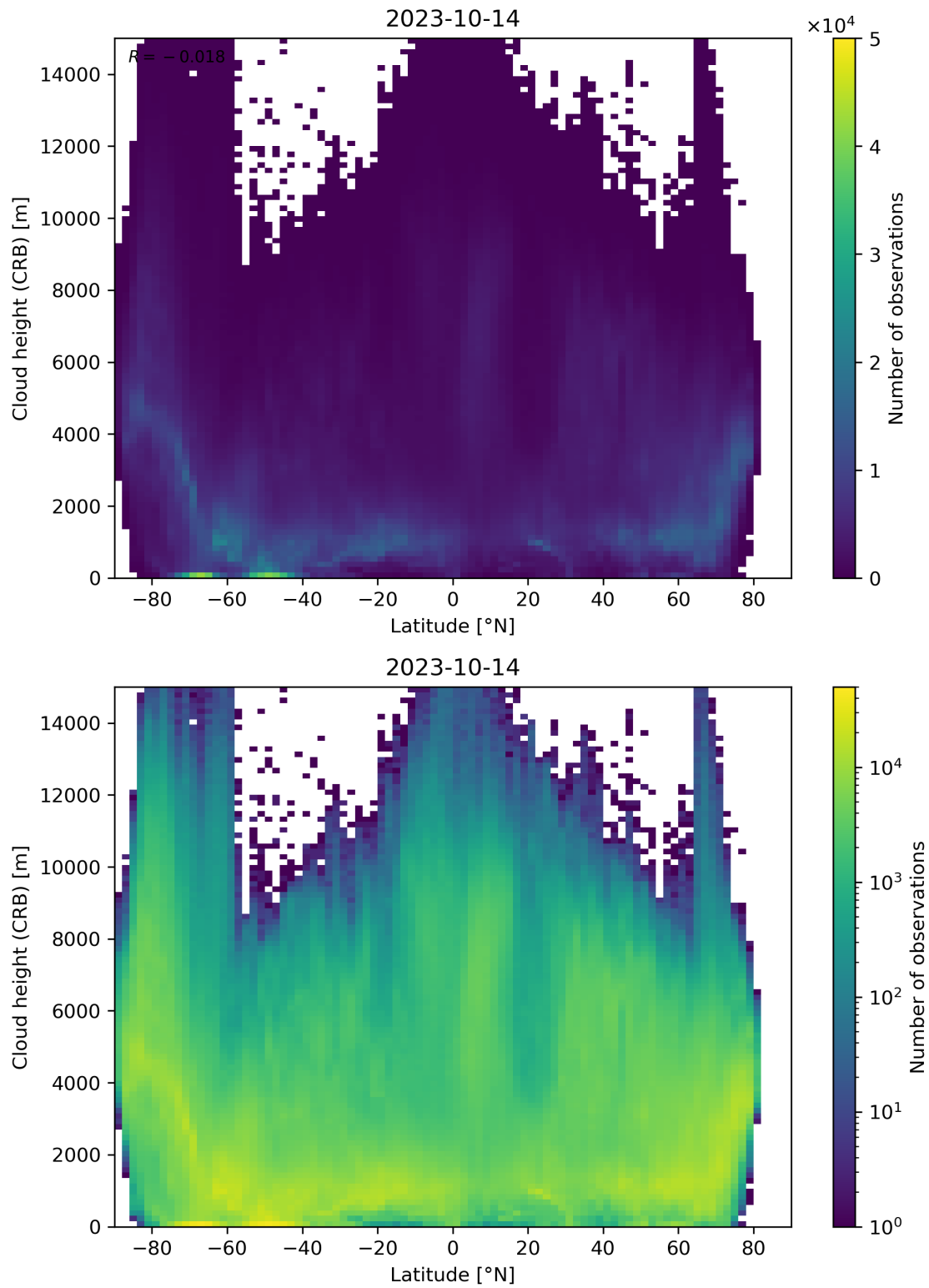
Figure 95: Scatter density plot of “Latitude” against “Cloud height (CRB)” for 2023-10-13 to 2023-10-15.
