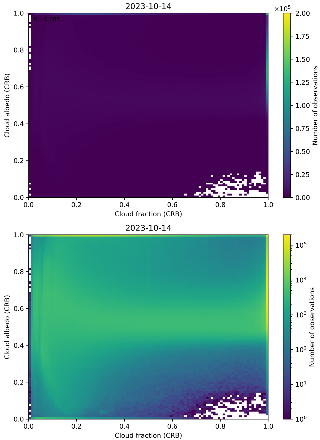
Figure 77: Scatter density plot of “Cloud fraction (CRB)” against “Cloud albedo (CRB)” for 2023-10-13 to 2023-10-15.
