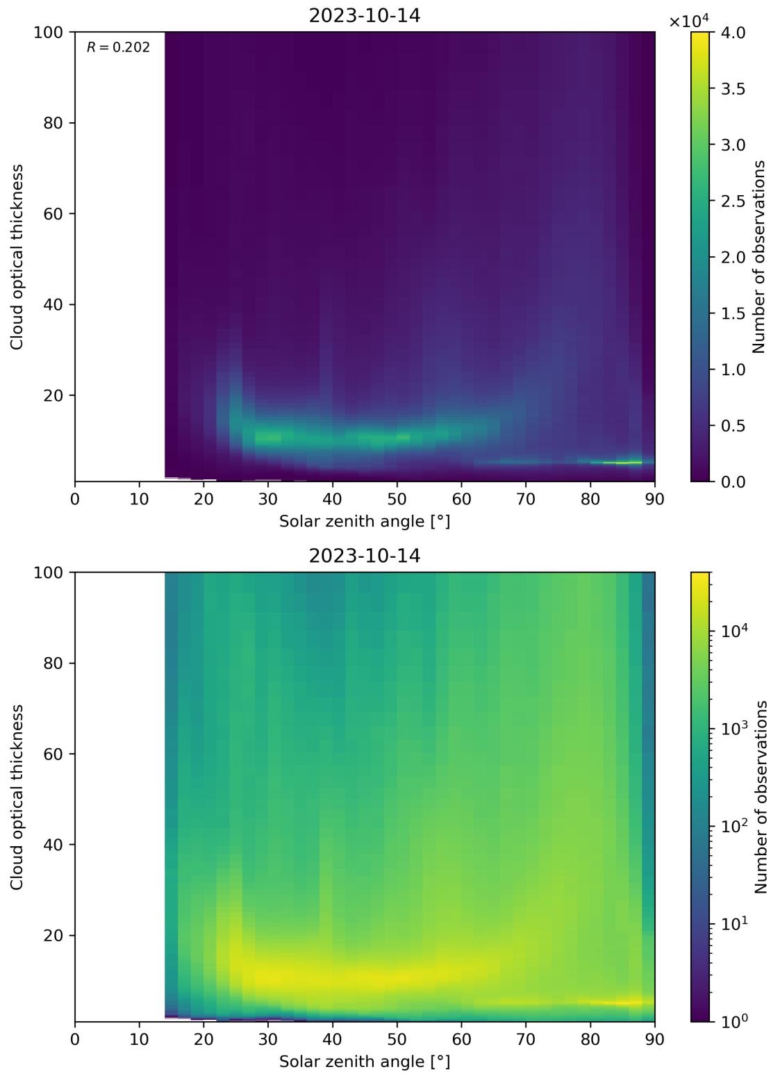
Figure 103: Scatter density plot of “Solar zenith angle” against “Cloud optical thickness” for 2023-10-13 to 2023-10-15.
