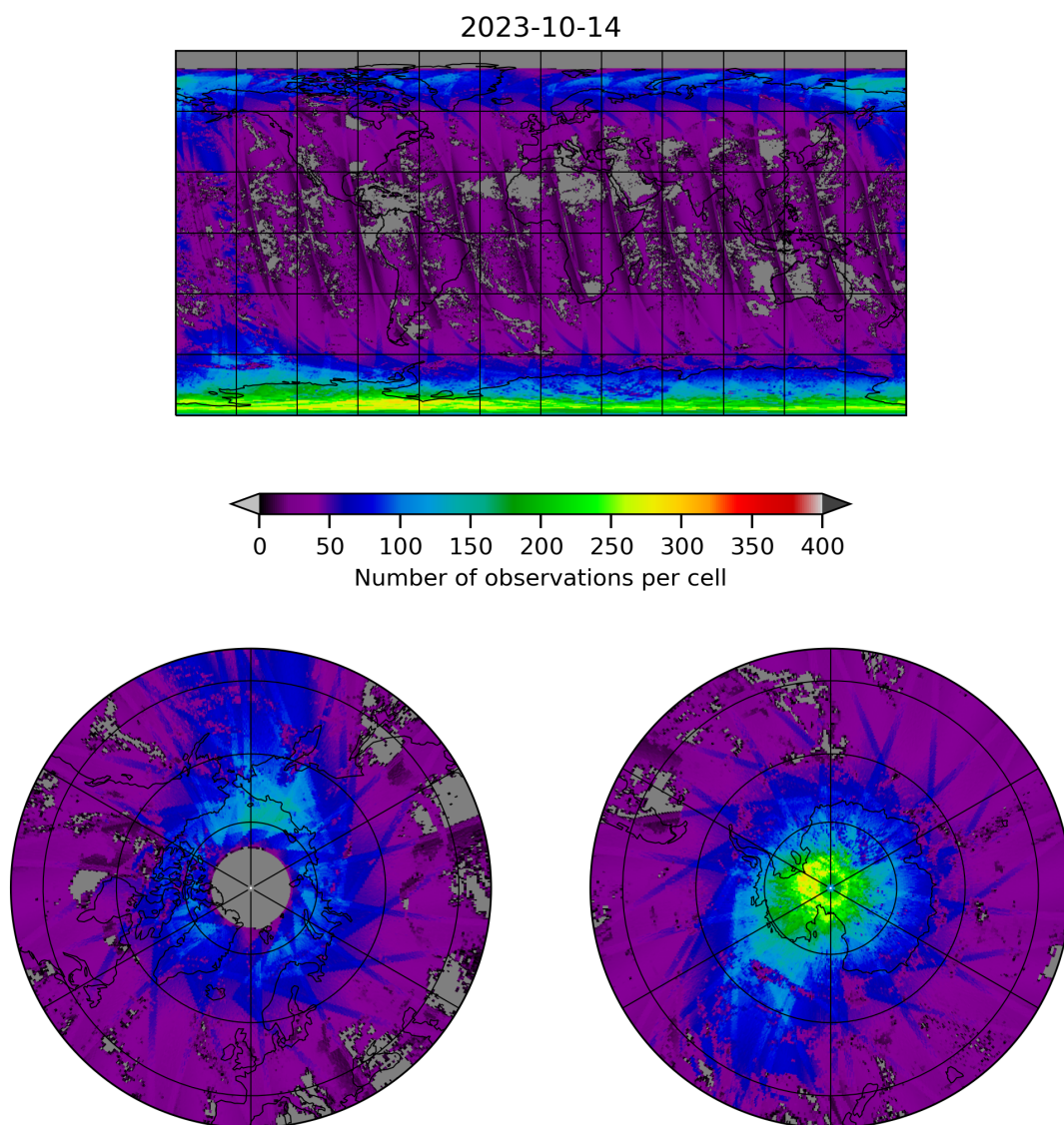
Figure 21: Map of the number of observations for 2023-10-13 to 2023-10-15
