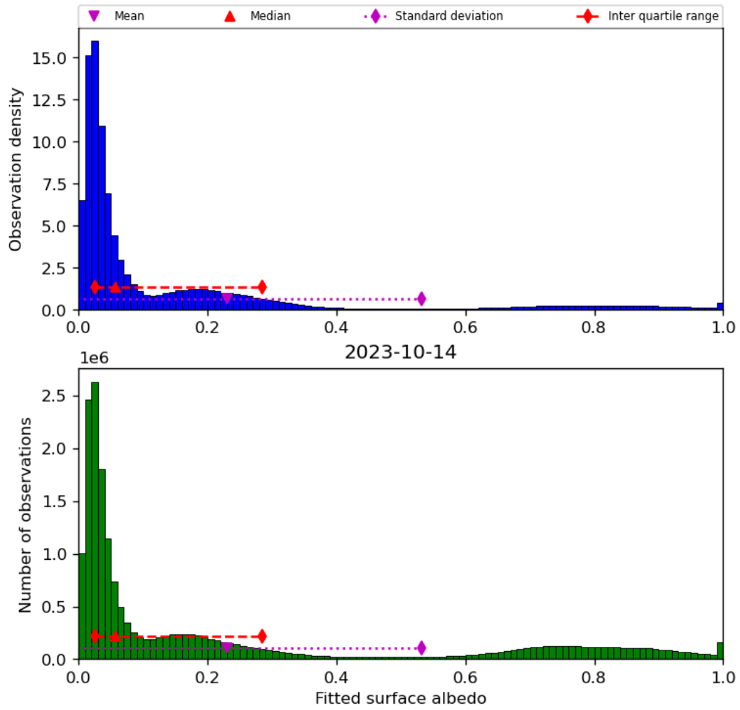
Figure 45: Histogram of “Fitted surface albedo” for 2023-10-13 to 2023-10-15
