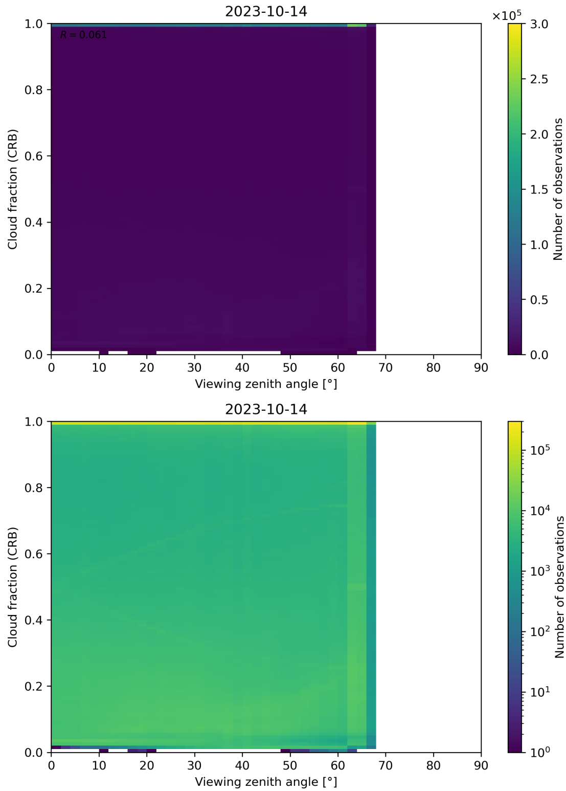
Figure 109: Scatter density plot of “Viewing zenith angle” against “Cloud fraction (CRB)” for 2023-10-13 to 2023-10-15.
