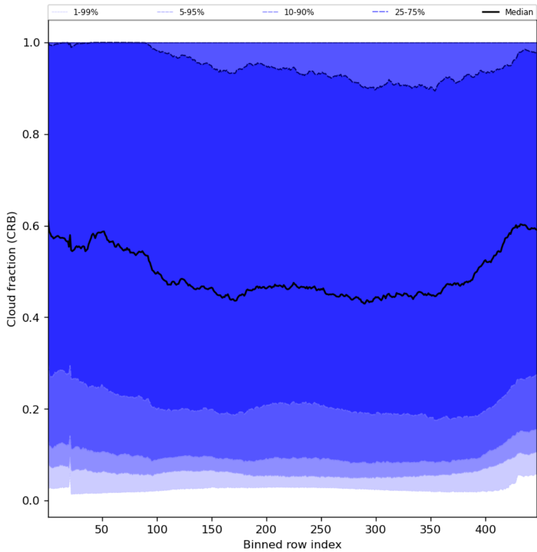
Figure 58: Along track statistics of “Cloud fraction (CRB)” for 2023-10-13 to 2023-10-15
