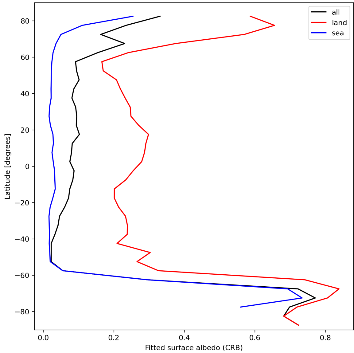
Figure 30: Zonal average of “Fitted surface albedo (CRB)” for 2023-10-13 to 2023-10-15.
