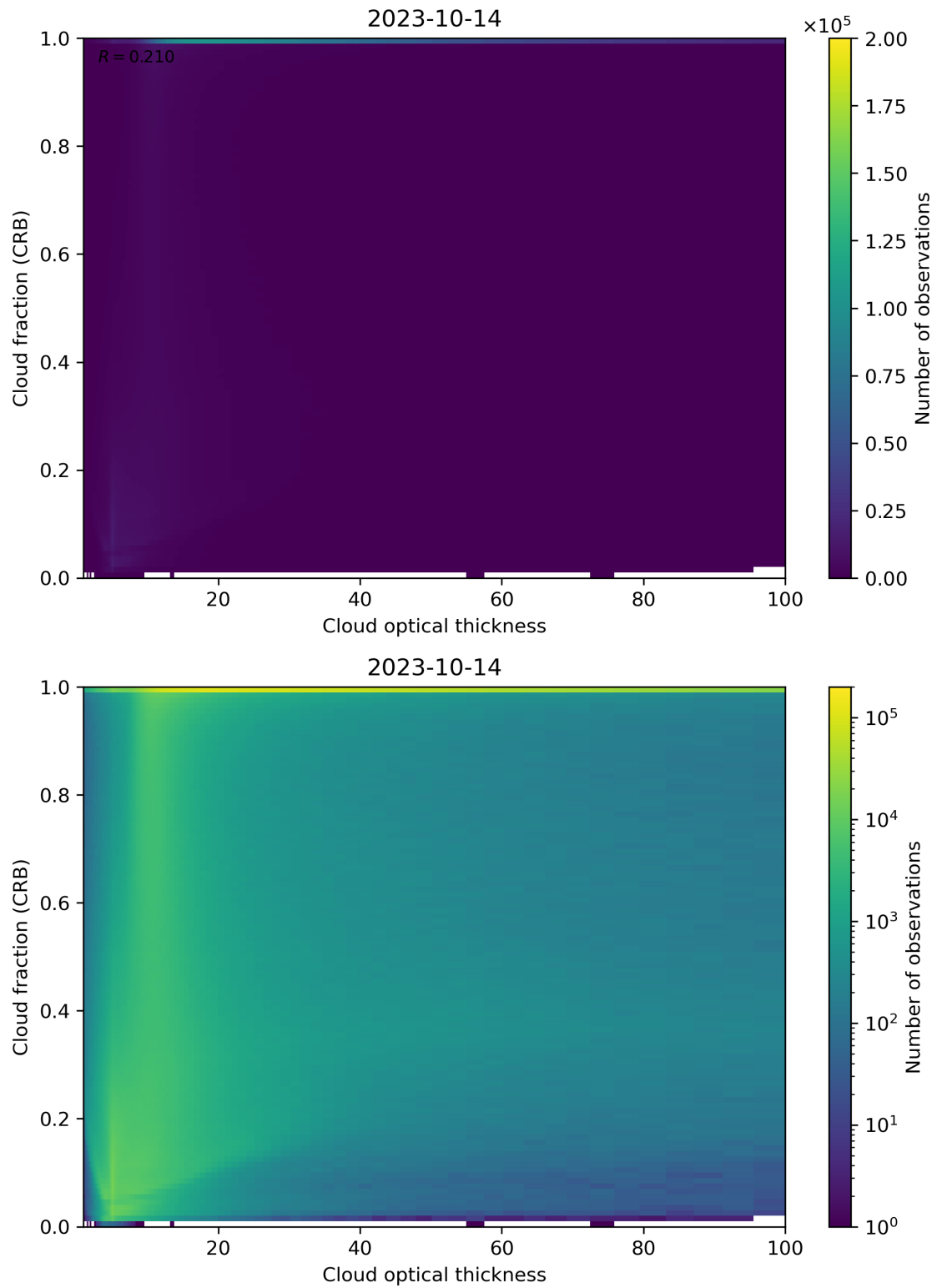
Figure 84: Scatter density plot of “Cloud optical thickness” against “Cloud fraction (CRB)” for 2023-10-13 to 2023-10-15.
