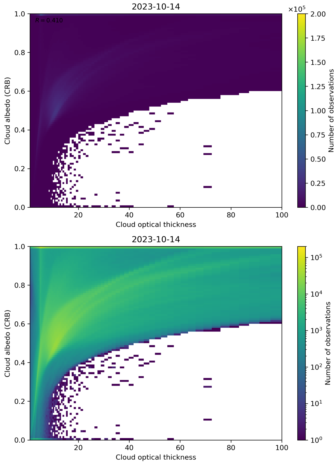
Figure 82: Scatter density plot of “Cloud optical thickness” against “Cloud albedo (CRB)” for 2023-10-13 to 2023-10-15.
