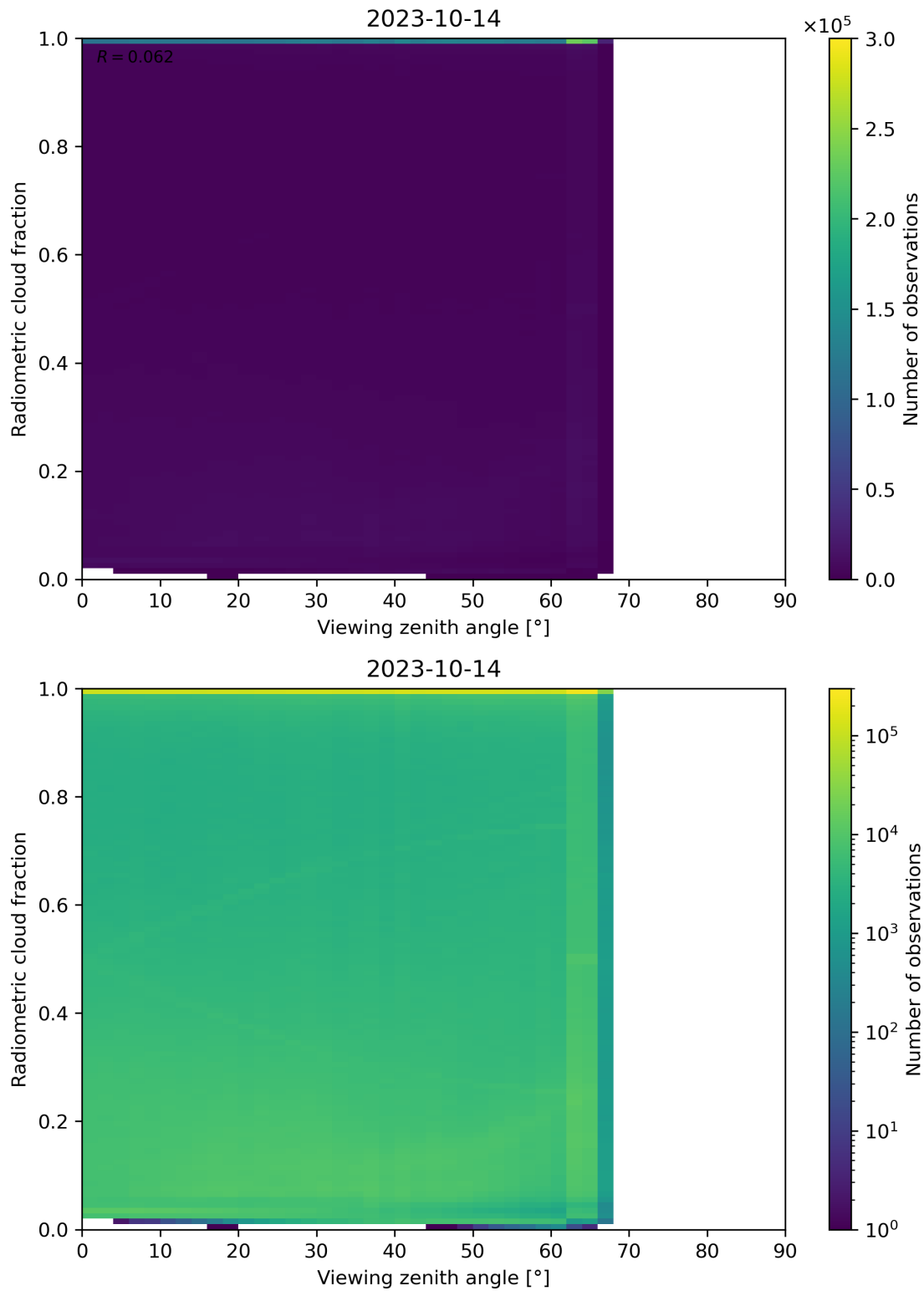
Figure 107: Scatter density plot of “Viewing zenith angle” against “Radiometric cloud fraction” for 2023-10-13 to 2023-10-15.
