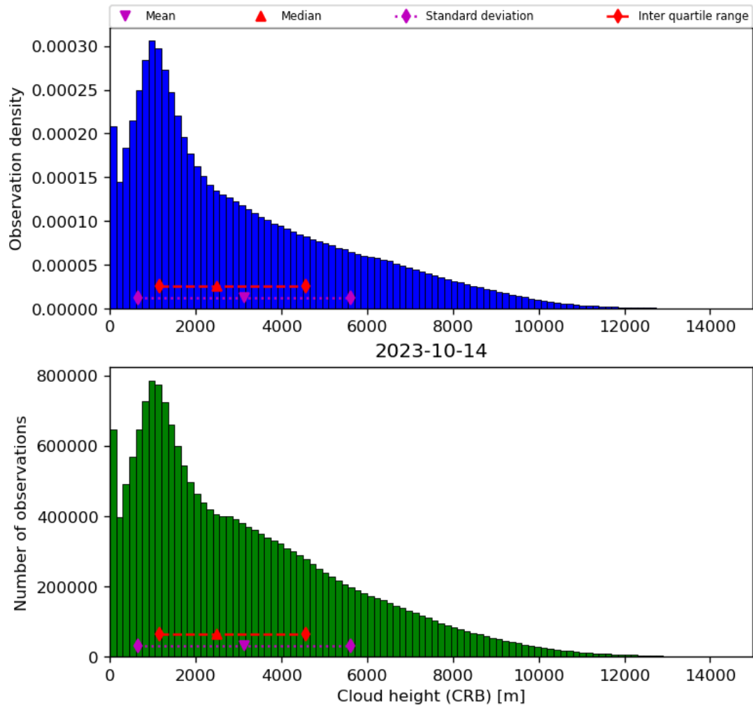
Figure 43: Histogram of “Cloud height (CRB)” for 2023-10-13 to 2023-10-15
