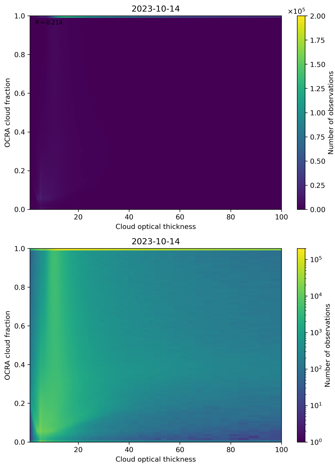
Figure 83: Scatter density plot of “Cloud optical thickness” against “OCRA cloud fraction” for 2023-10-13 to 2023-10-15.
