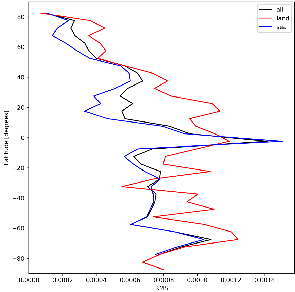
Figure 31: Zonal average of “RMS” for 2023-10-13 to 2023-10-15.
