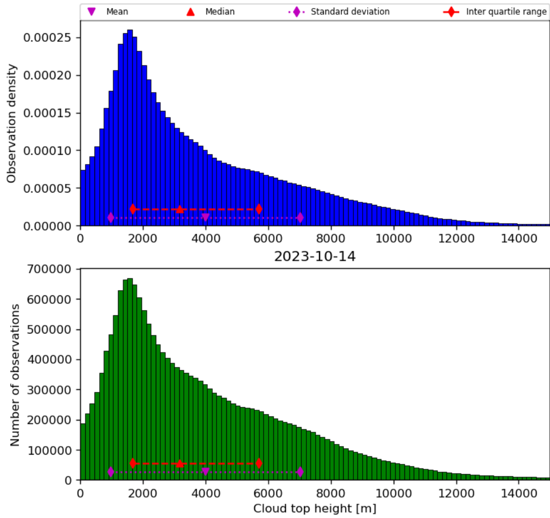
Figure 40: Histogram of “Cloud top height” for 2023-10-13 to 2023-10-15
