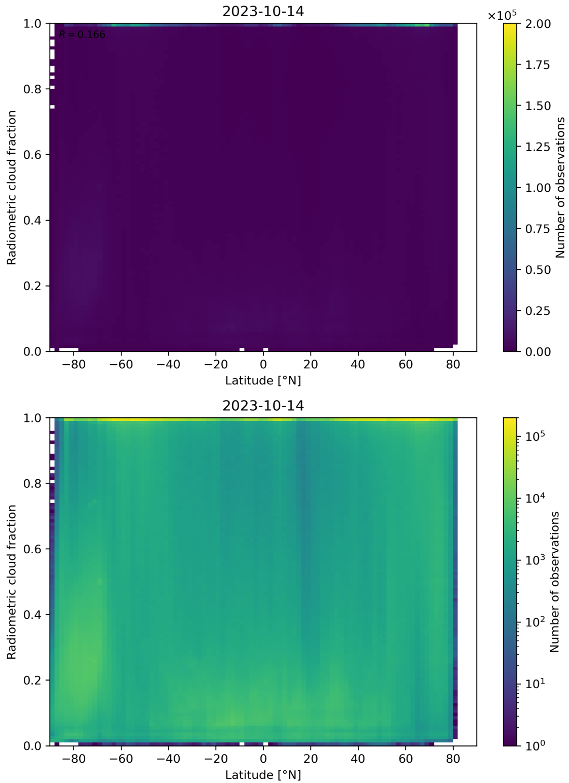
Figure 92: Scatter density plot of “Latitude” against “Radiometric cloud fraction” for 2023-10-13 to 2023-10-15.
