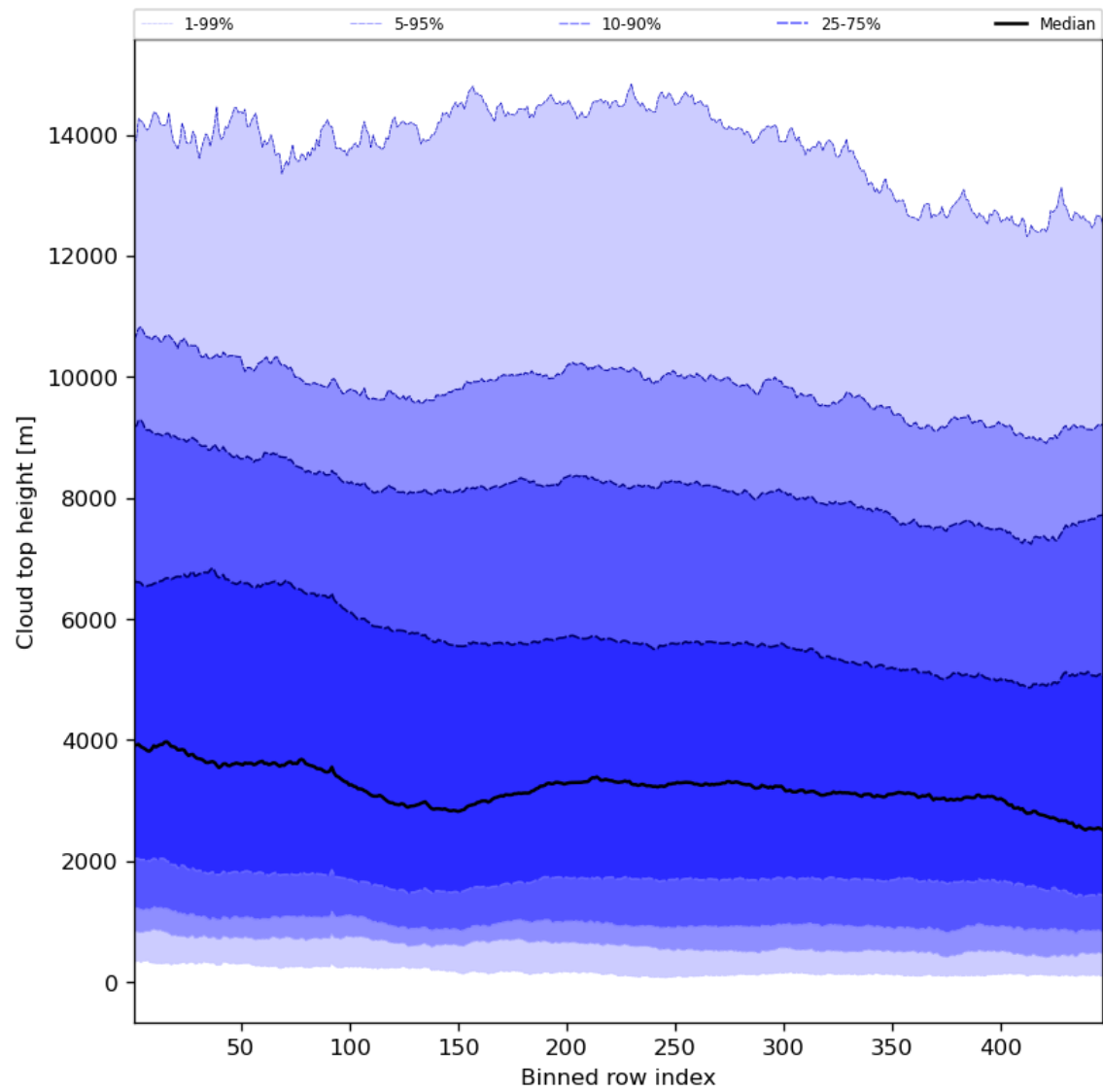
Figure 56: Along track statistics of “Cloud top height” for 2023-10-13 to 2023-10-15
