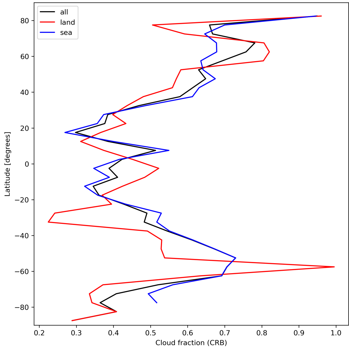
Figure 26: Zonal average of “Cloud fraction (CRB)” for 2023-10-13 to 2023-10-15.
