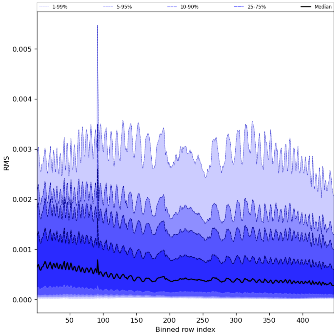
Figure 63: Along track statistics of “RMS” for 2023-10-13 to 2023-10-15
