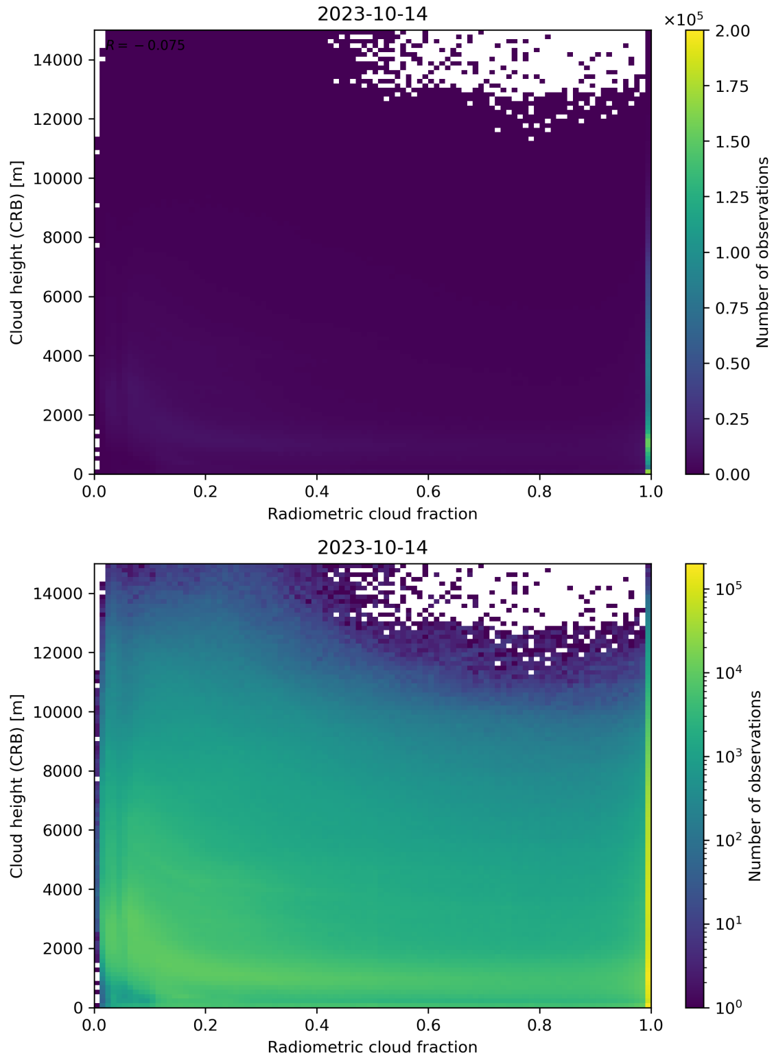
Figure 74: Scatter density plot of “Radiometric cloud fraction” against “Cloud height (CRB)” for 2023-10-13 to 2023-10-15.
