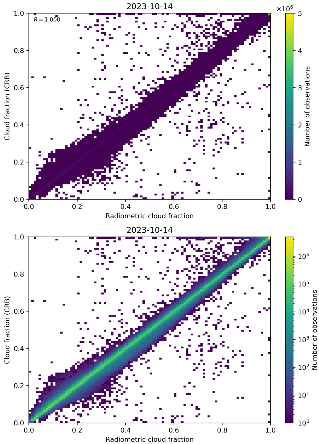
Figure 73: Scatter density plot of “Radiometric cloud fraction” against “Cloud fraction (CRB)” for 2023-10-13 to 2023-10-15.
