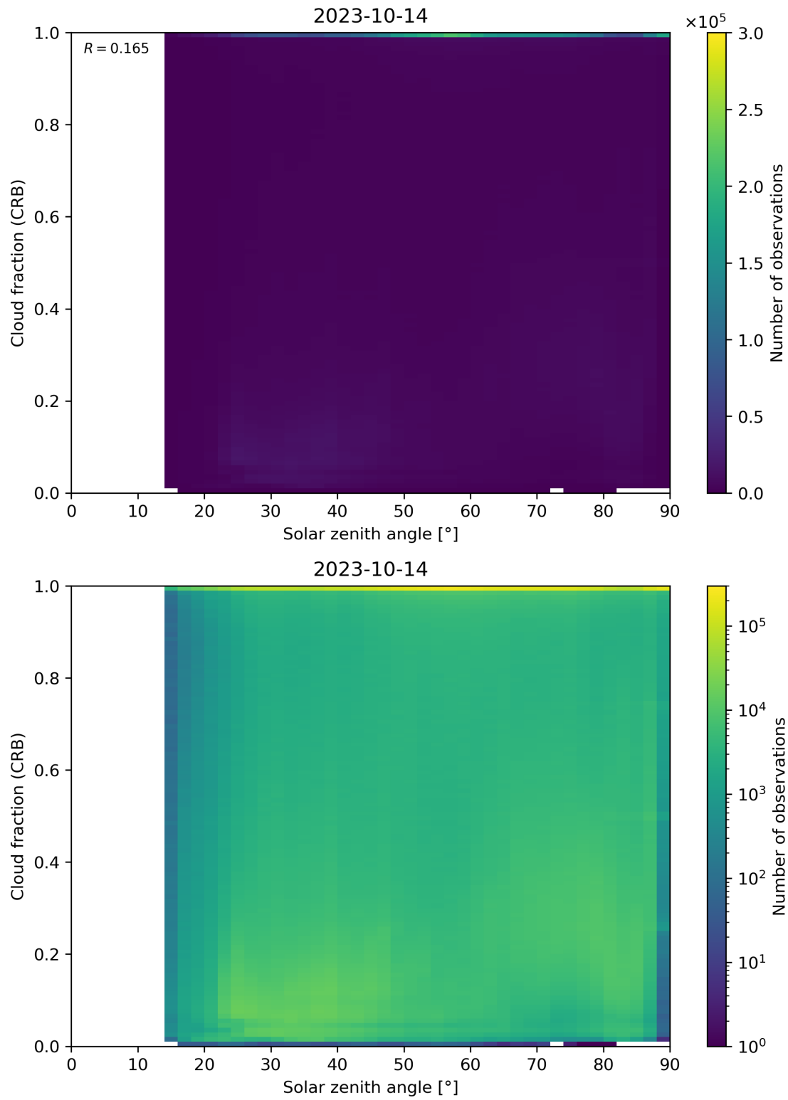
Figure 101: Scatter density plot of “Solar zenith angle” against “Cloud fraction (CRB)” for 2023-10-13 to 2023-10-15.
