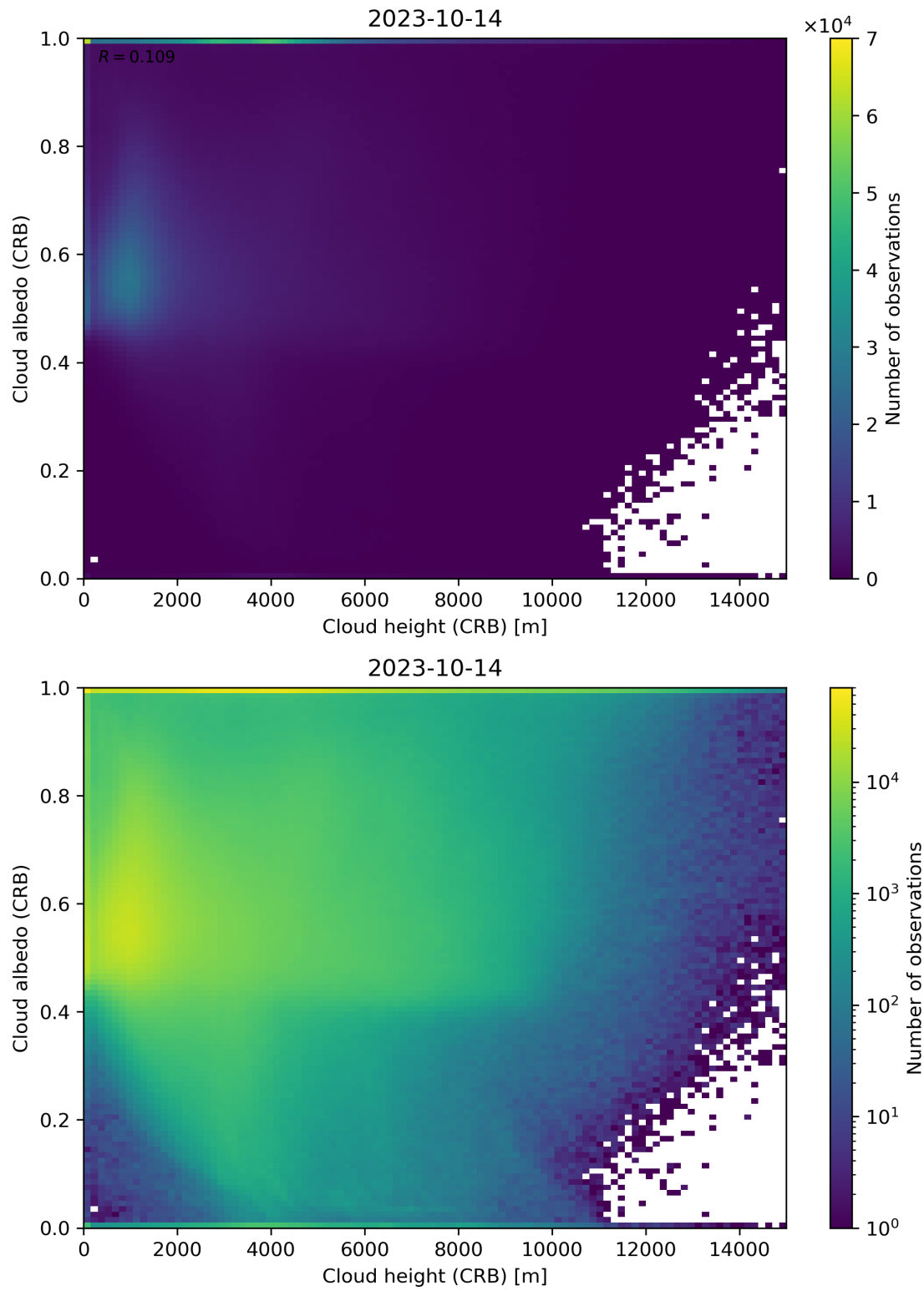
Figure 80: Scatter density plot of “Cloud height (CRB)” against “Cloud albedo (CRB)” for 2023-10-13 to 2023-10-15.
