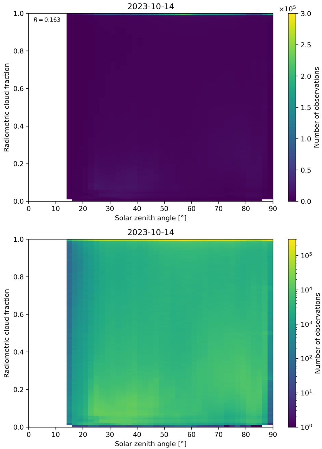
Figure 99: Scatter density plot of “Solar zenith angle” against “Radiometric cloud fraction” for 2023-10-13 to 2023-10-15.
