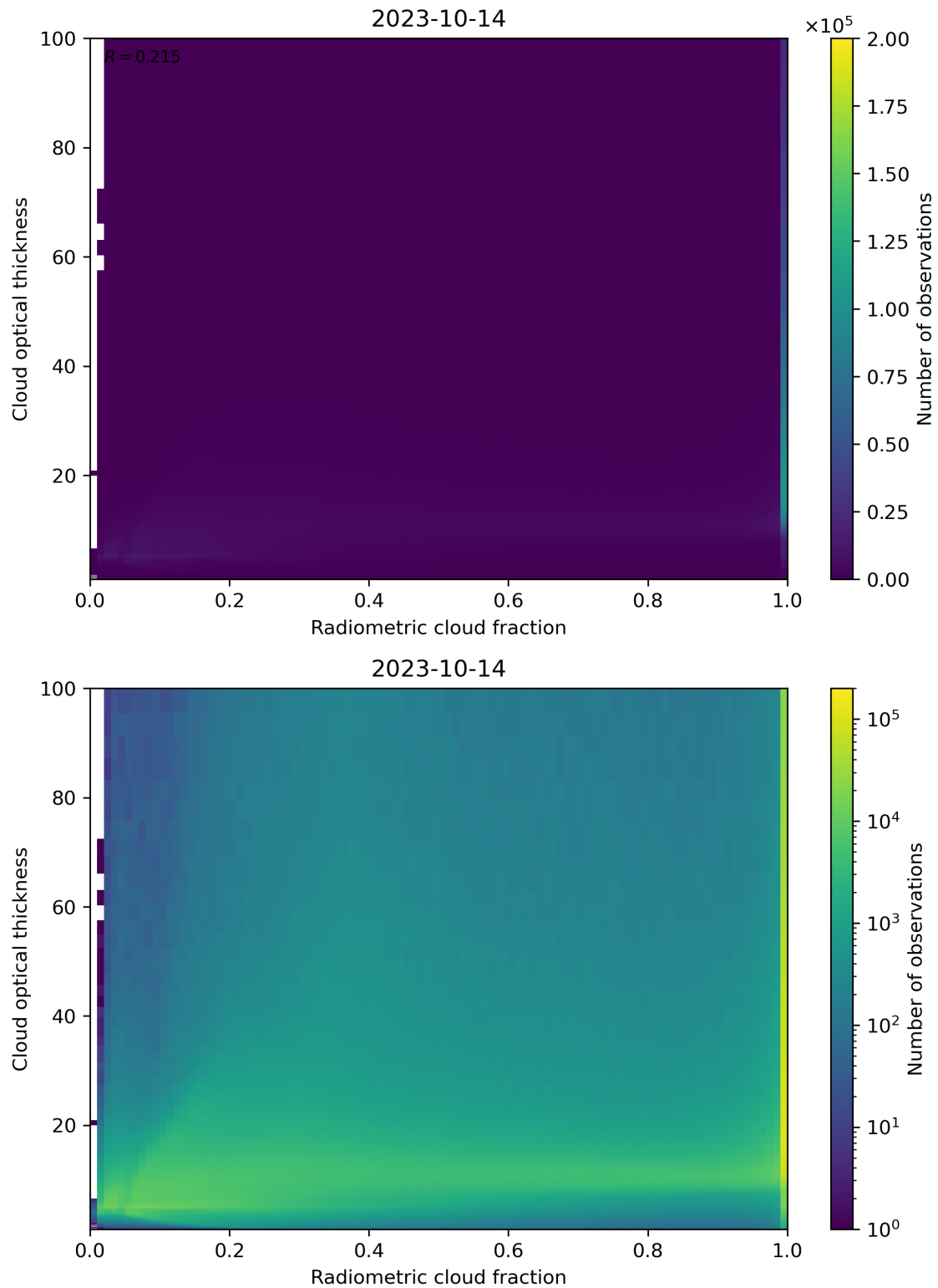
Figure 75: Scatter density plot of “Radiometric cloud fraction” against “Cloud optical thickness” for 2023-10-13 to 2023-10-15.
