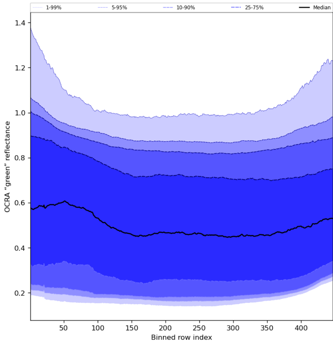
Figure 68: Along track statistics of "OCRA "green" reflectance" for 2023-10-13 to 2023-10-15
