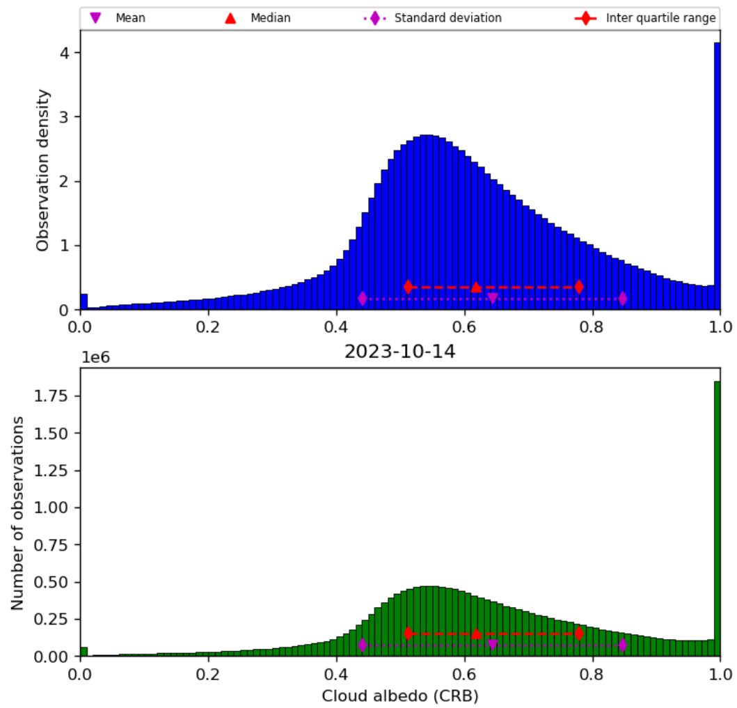
Figure 44: Histogram of “Cloud albedo (CRB)” for 2023-10-13 to 2023-10-15
