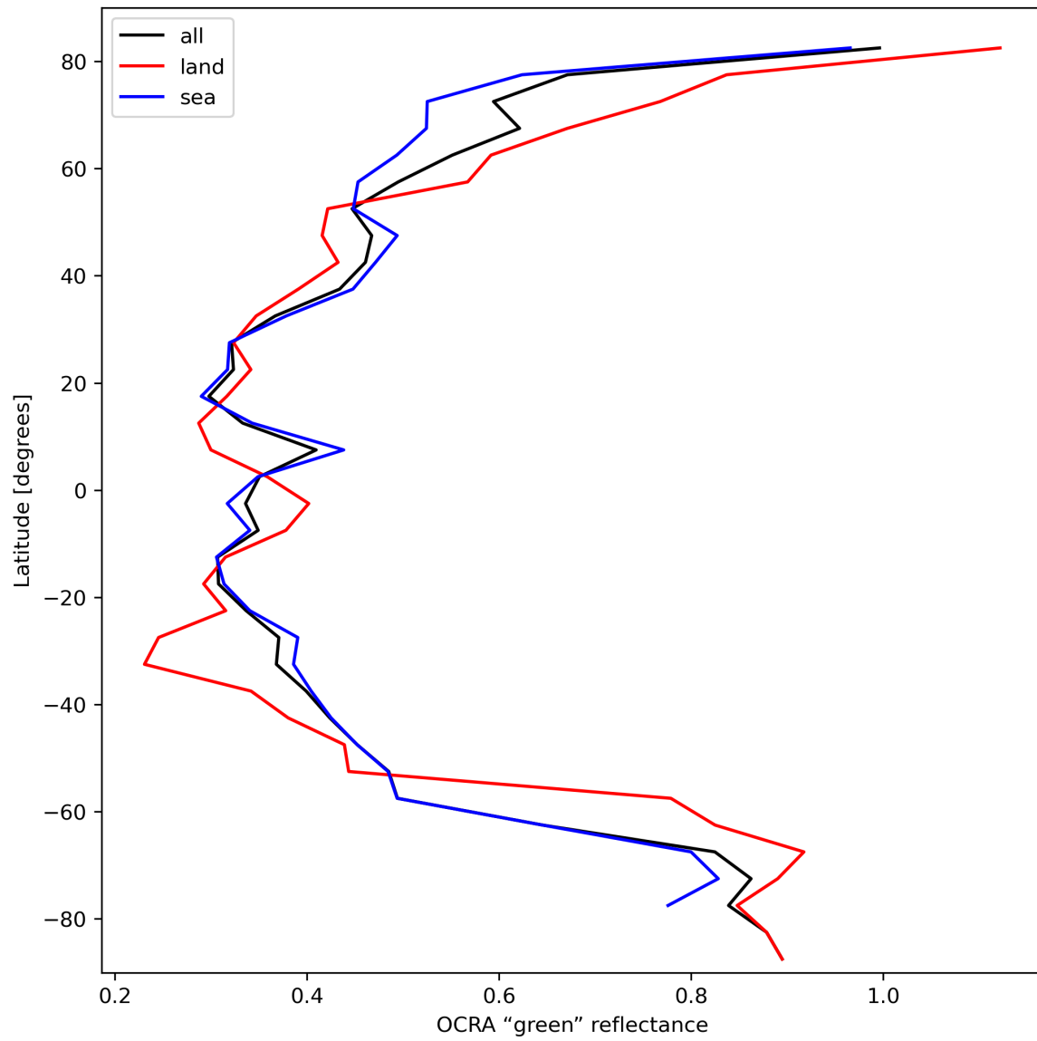
Figure 36: Zonal average of “OCRA “green” reflectance” for 2023-10-13 to 2023-10-15.
