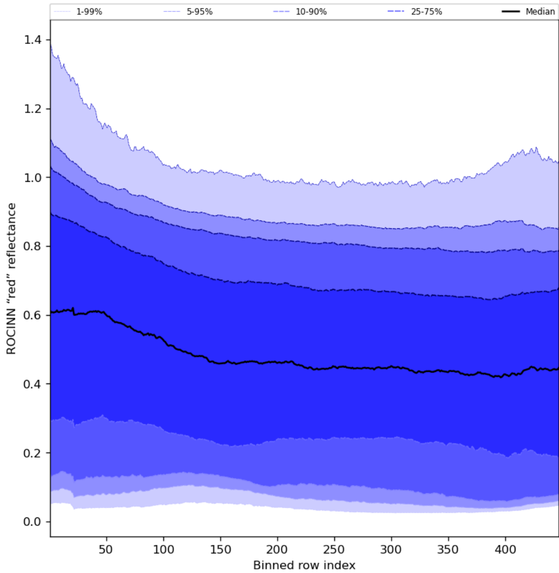
Figure 69: Along track statistics of “ROCINN “red” reflectance” for 2023-10-14 to 2023-10-16
