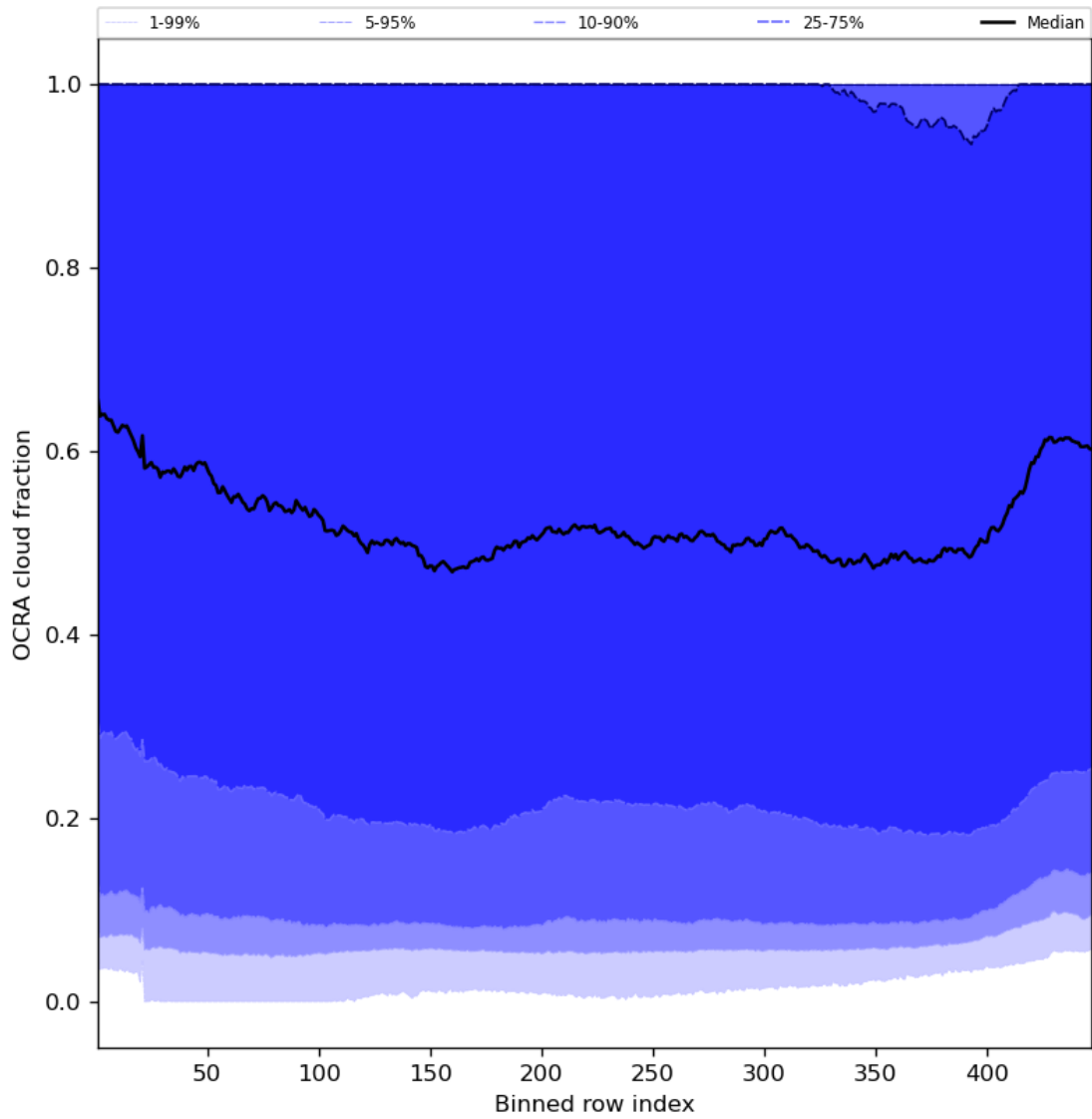
Figure 66: Along track statistics of “OCRA cloud fraction” for 2023-10-14 to 2023-10-16
