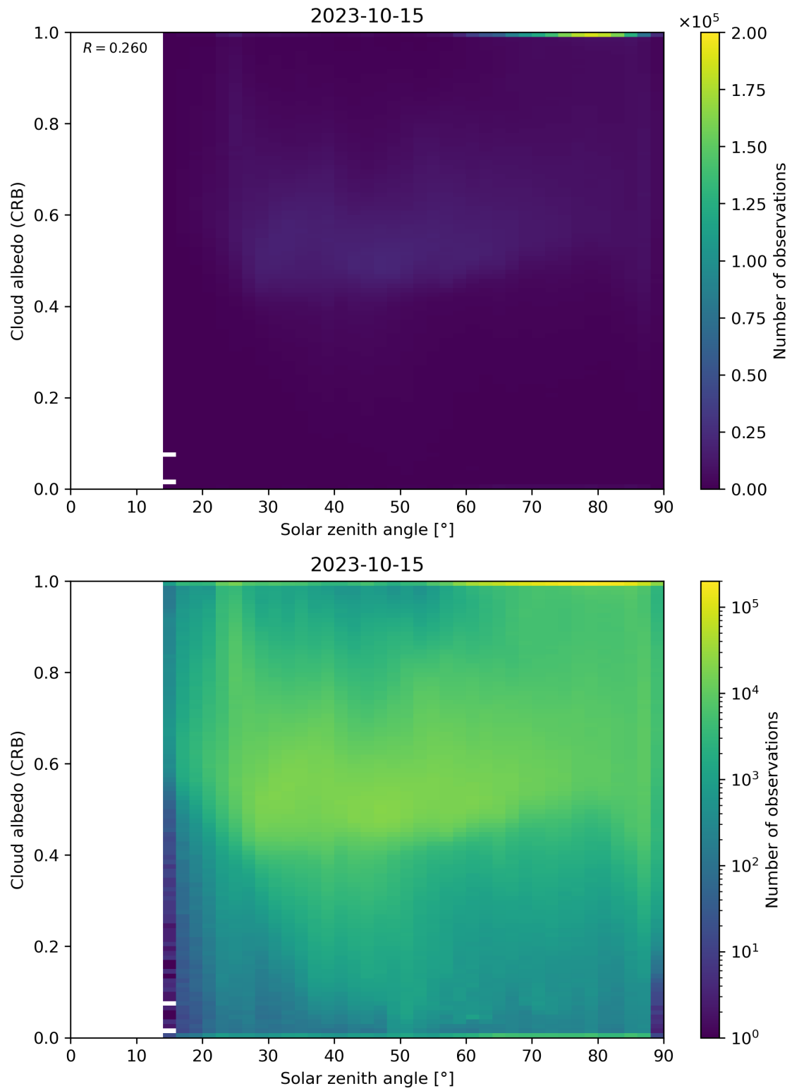
Figure 98: Scatter density plot of “Solar zenith angle” against “Cloud albedo (CRB)” for 2023-10-14 to 2023-10-16.
