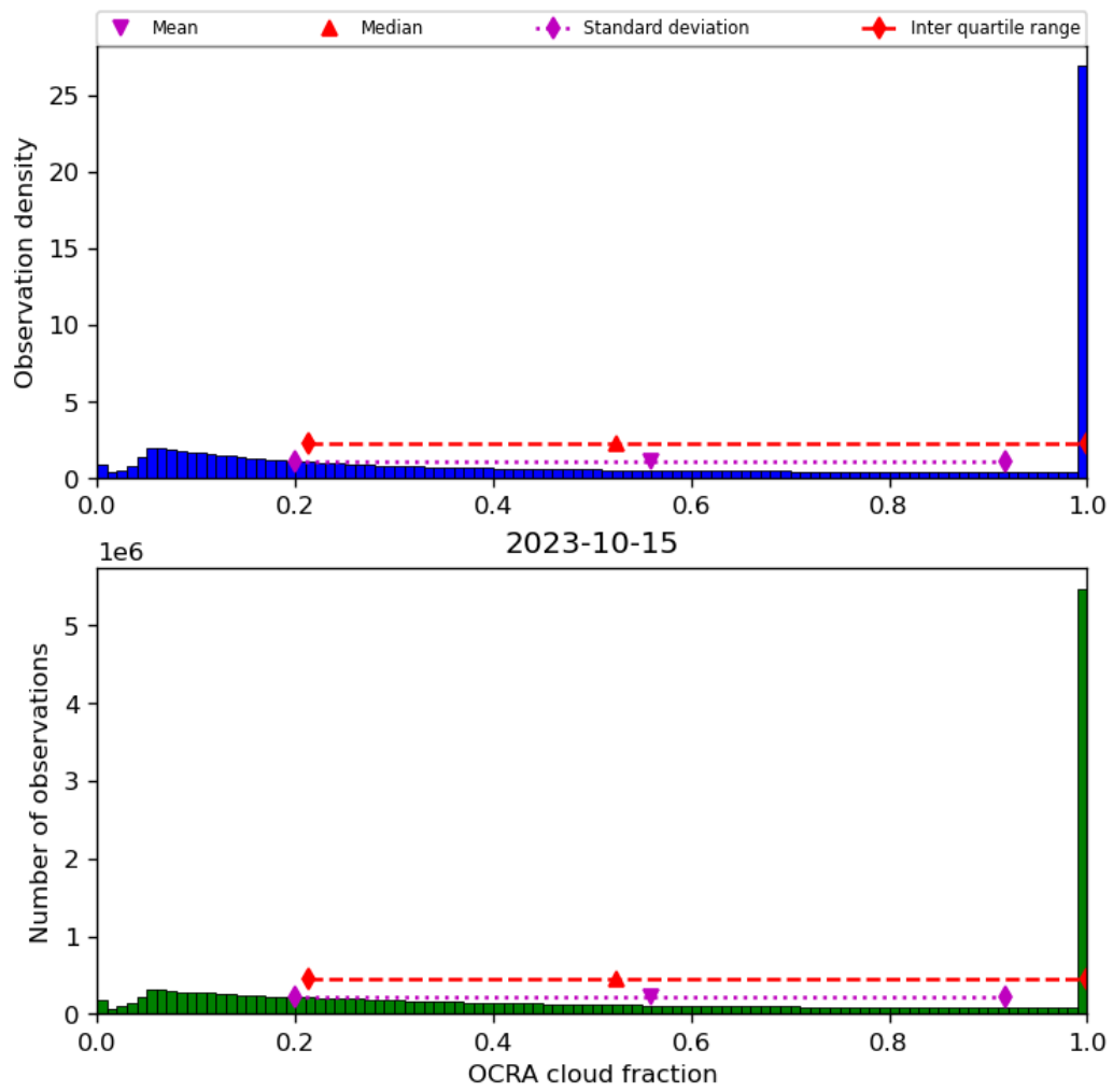
Figure 50: Histogram of “OCRA cloud fraction” for 2023-10-14 to 2023-10-16
