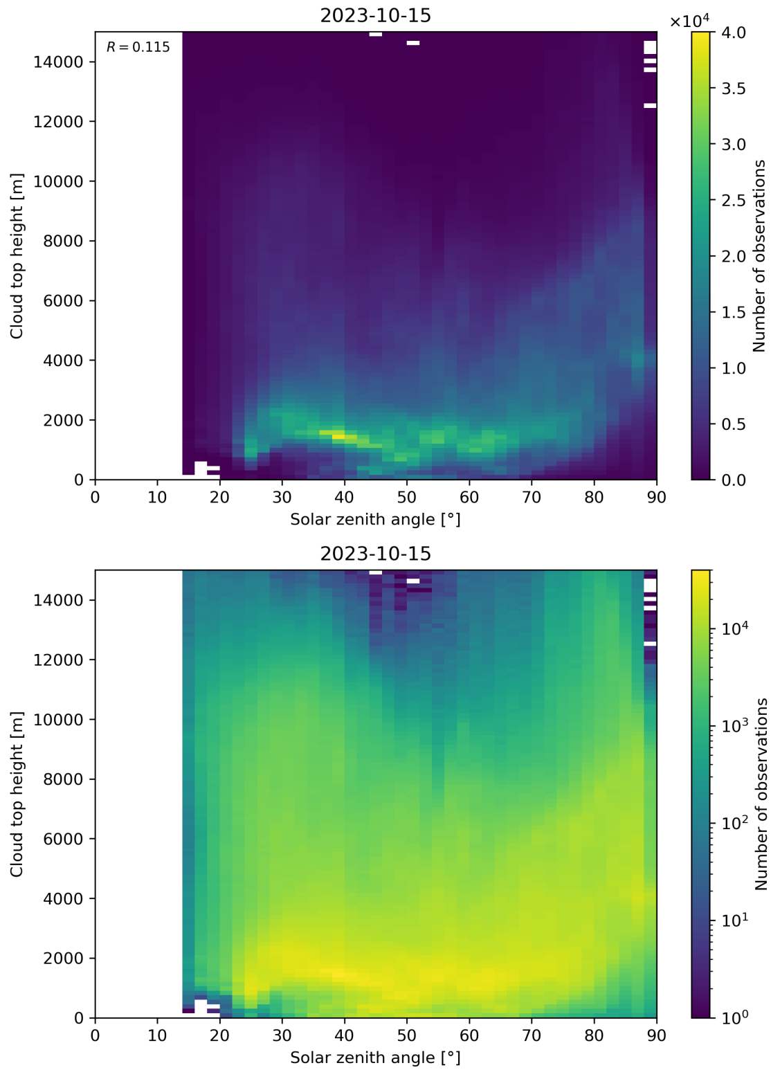
Figure 104: Scatter density plot of “Solar zenith angle” against “Cloud top height” for 2023-10-14 to 2023-10-16.
