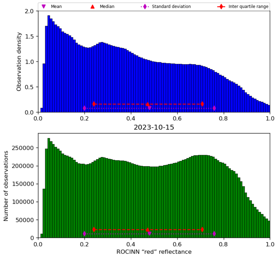
Figure 53: Histogram of “ROCINN “red” reflectance” for 2023-10-14 to 2023-10-16
