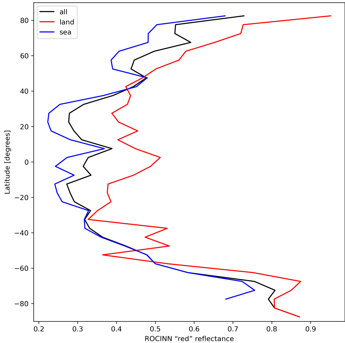
Figure 37: Zonal average of “ROCINN “red” reflectance” for 2023-10-14 to 2023-10-16.
