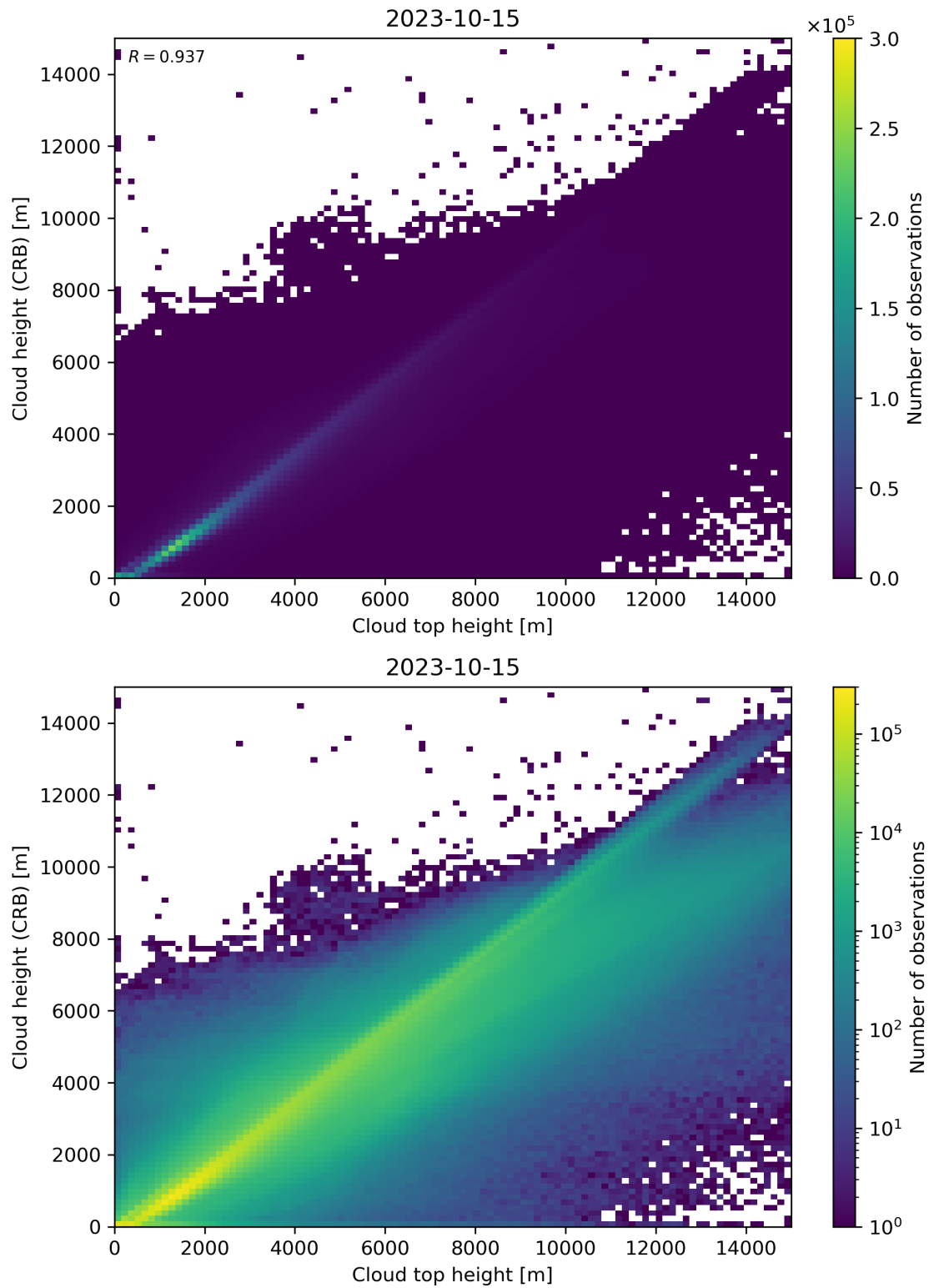
Figure 89: Scatter density plot of “Cloud top height” against “Cloud height (CRB)” for 2023-10-14 to 2023-10-16.
