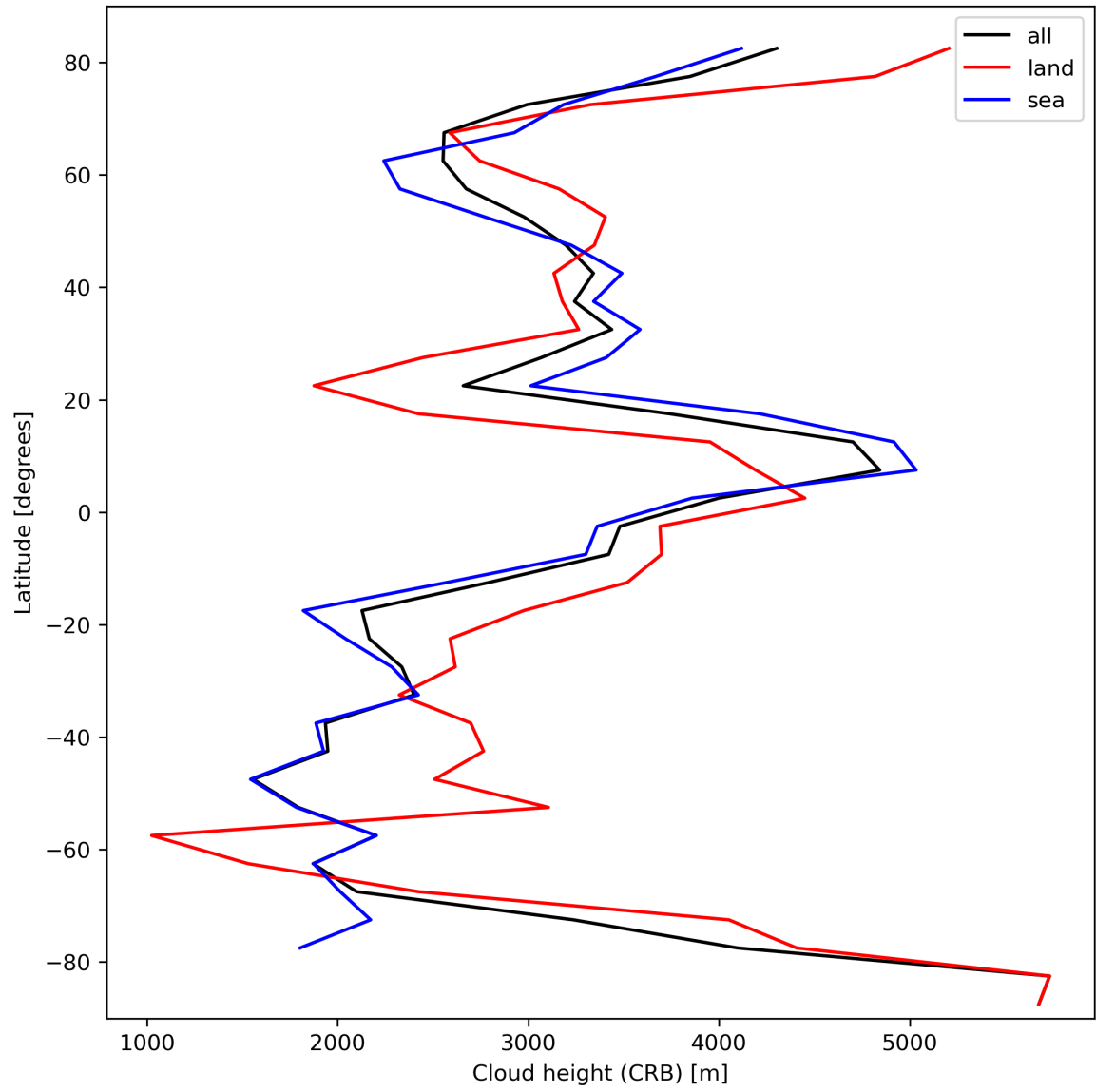
Figure 27: Zonal average of “Cloud height (CRB)” for 2023-10-14 to 2023-10-16.
