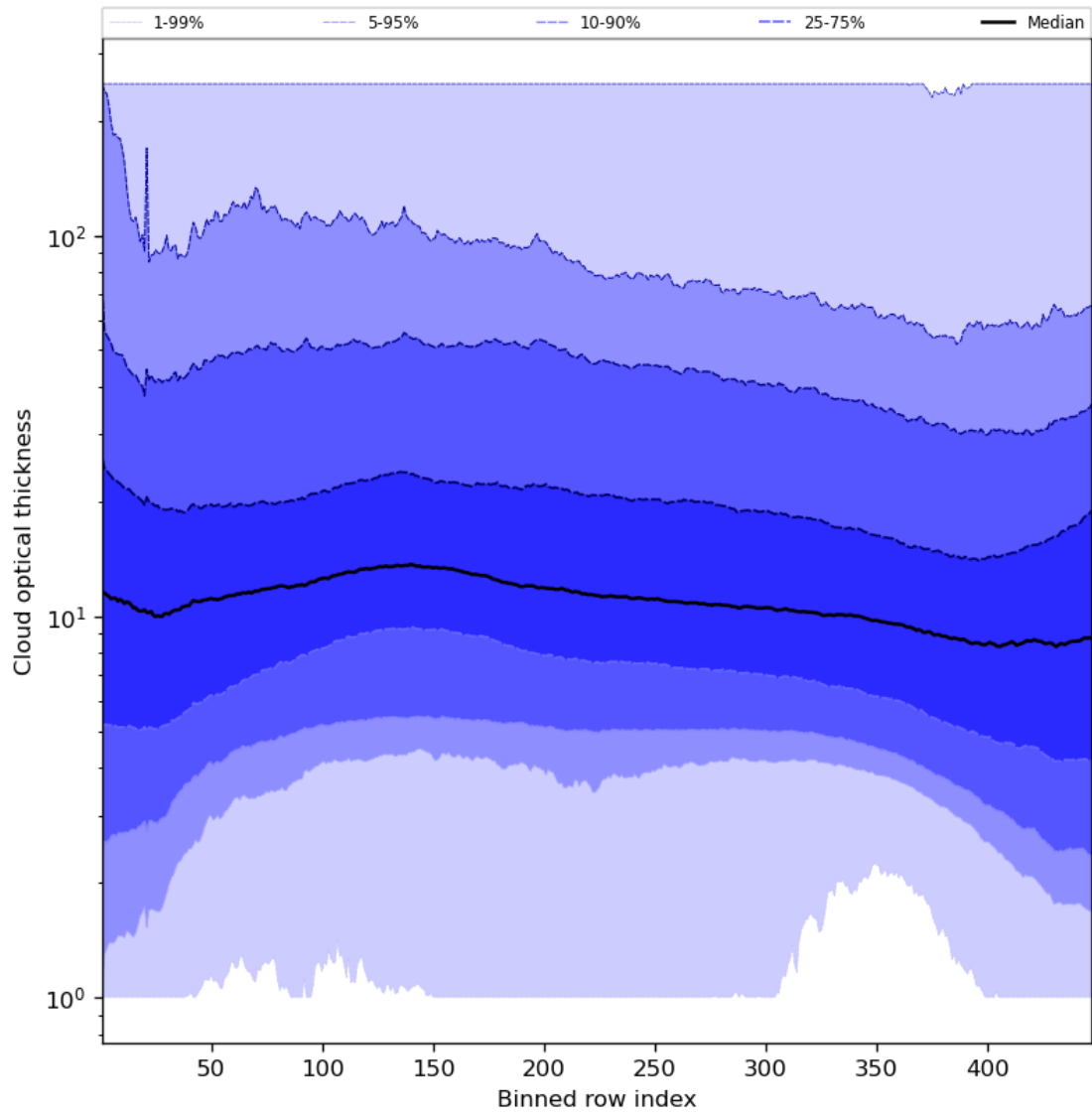
Figure 57: Along track statistics of “Cloud optical thickness” for 2023-10-14 to 2023-10-16
