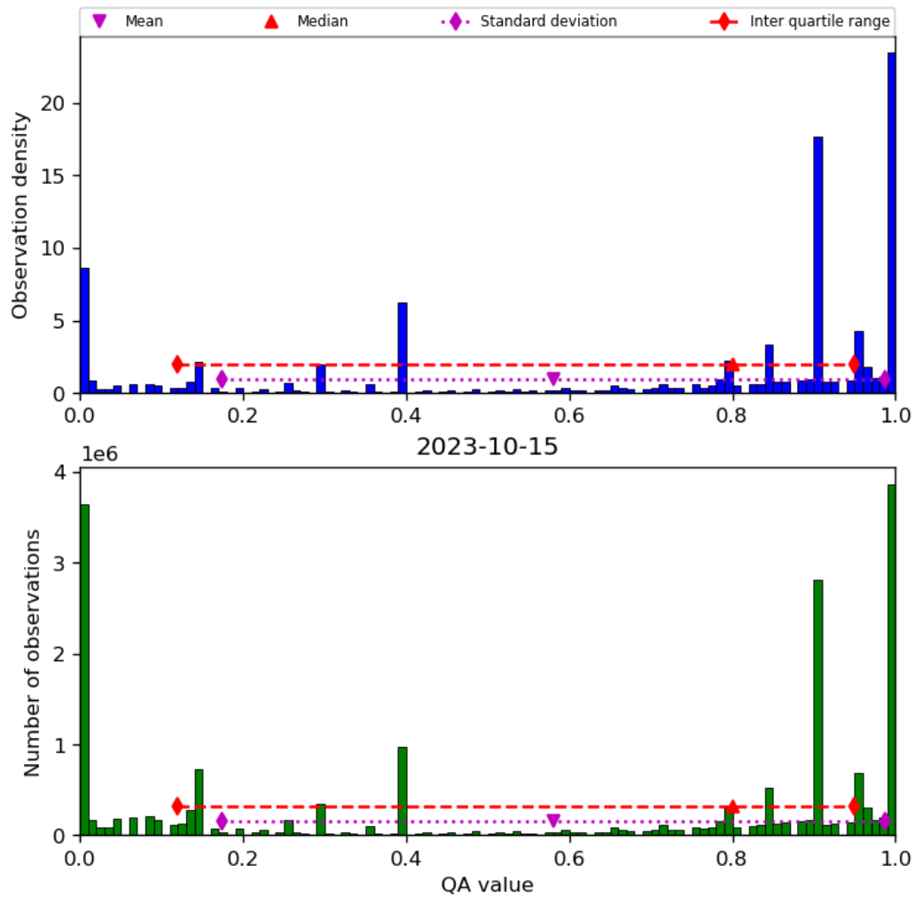
Figure 38: Histogram of “QA value” for 2023-10-14 to 2023-10-16
