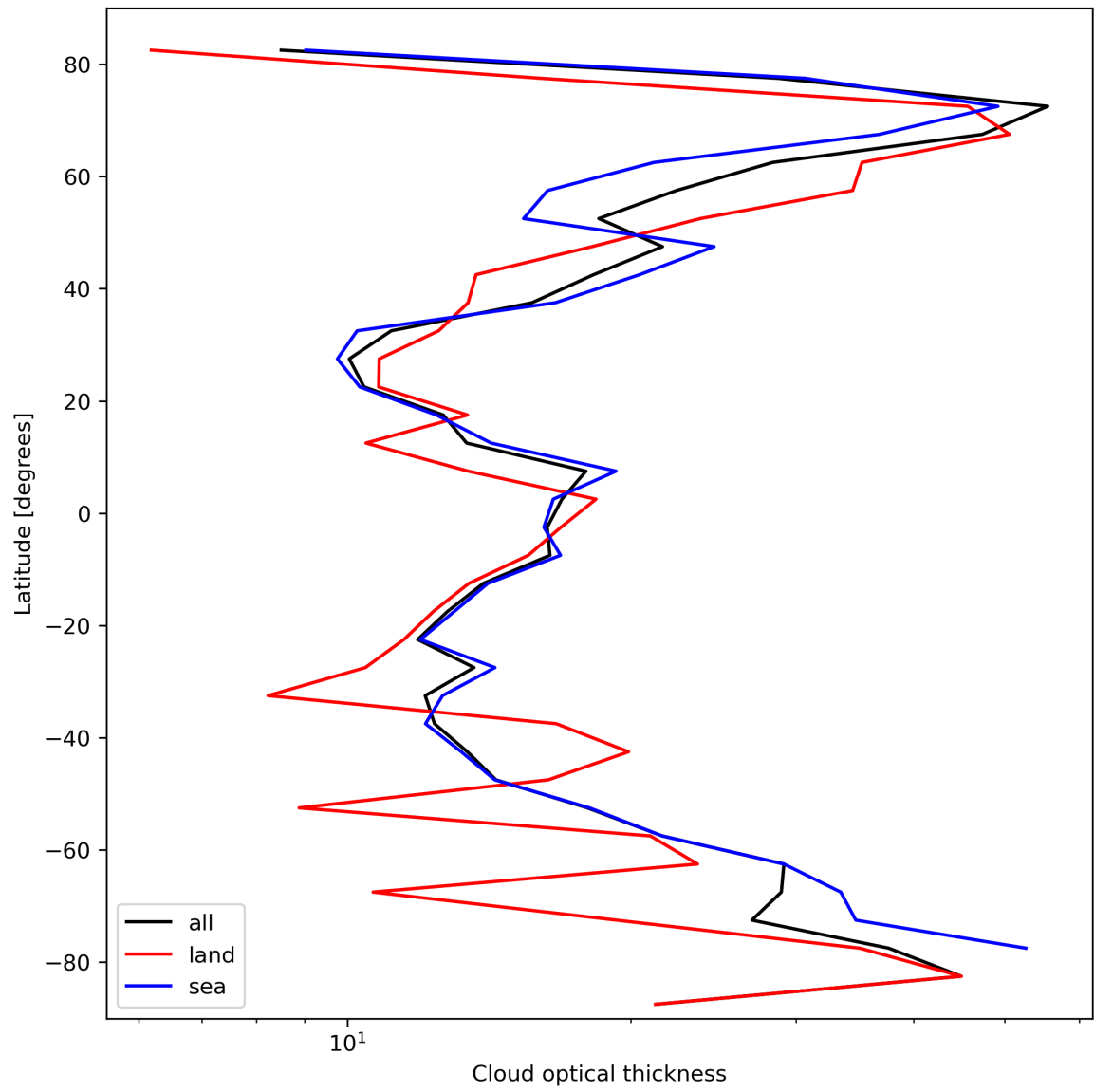
Figure 25: Zonal average of “Cloud optical thickness” for 2023-10-14 to 2023-10-16.
