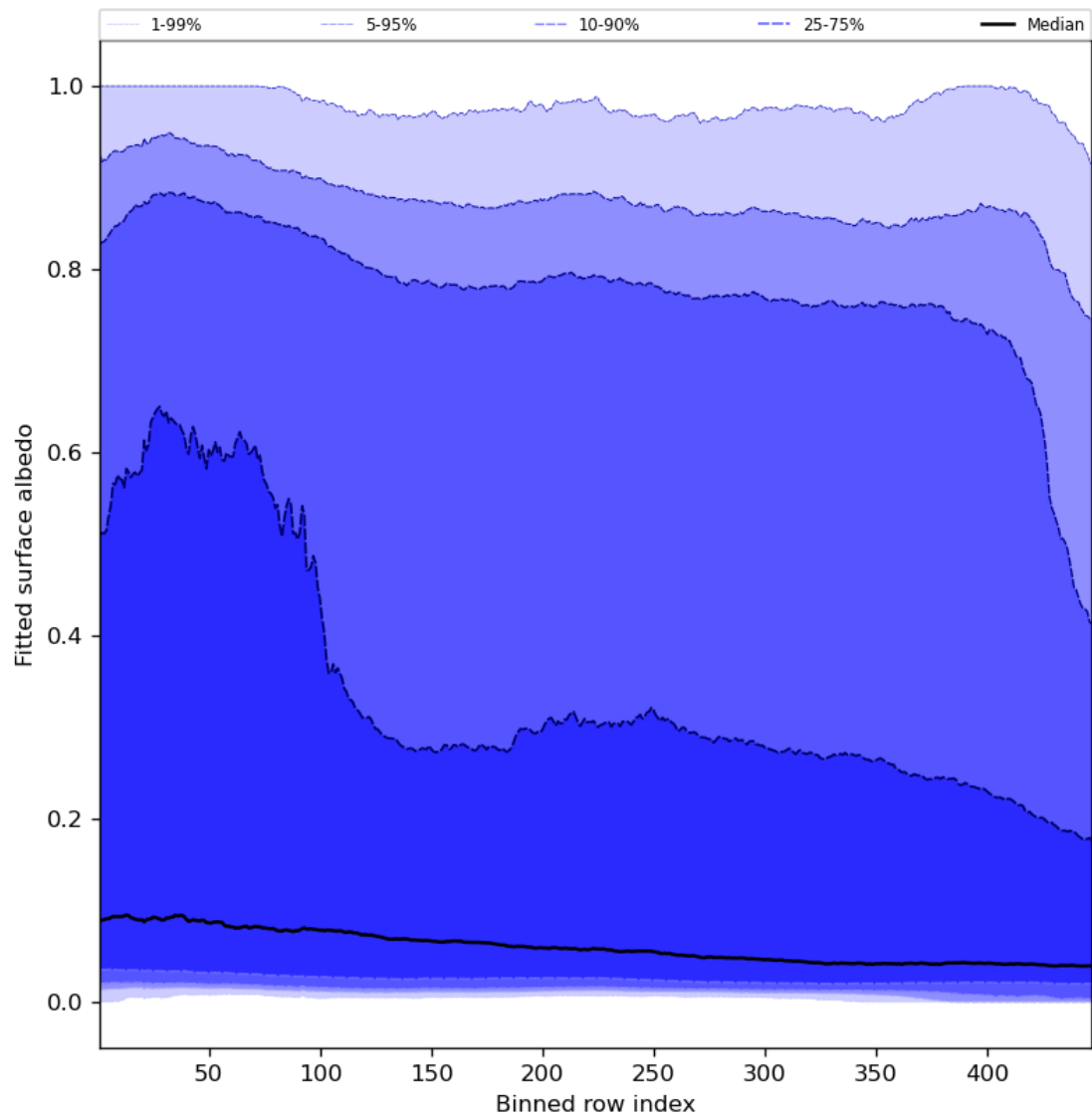
Figure 61: Along track statistics of “Fitted surface albedo” for 2023-10-14 to 2023-10-16
