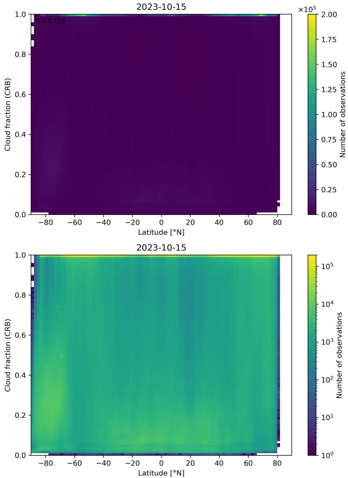
Figure 94: Scatter density plot of “Latitude” against “Cloud fraction (CRB)” for 2023-10-14 to 2023-10-16.
