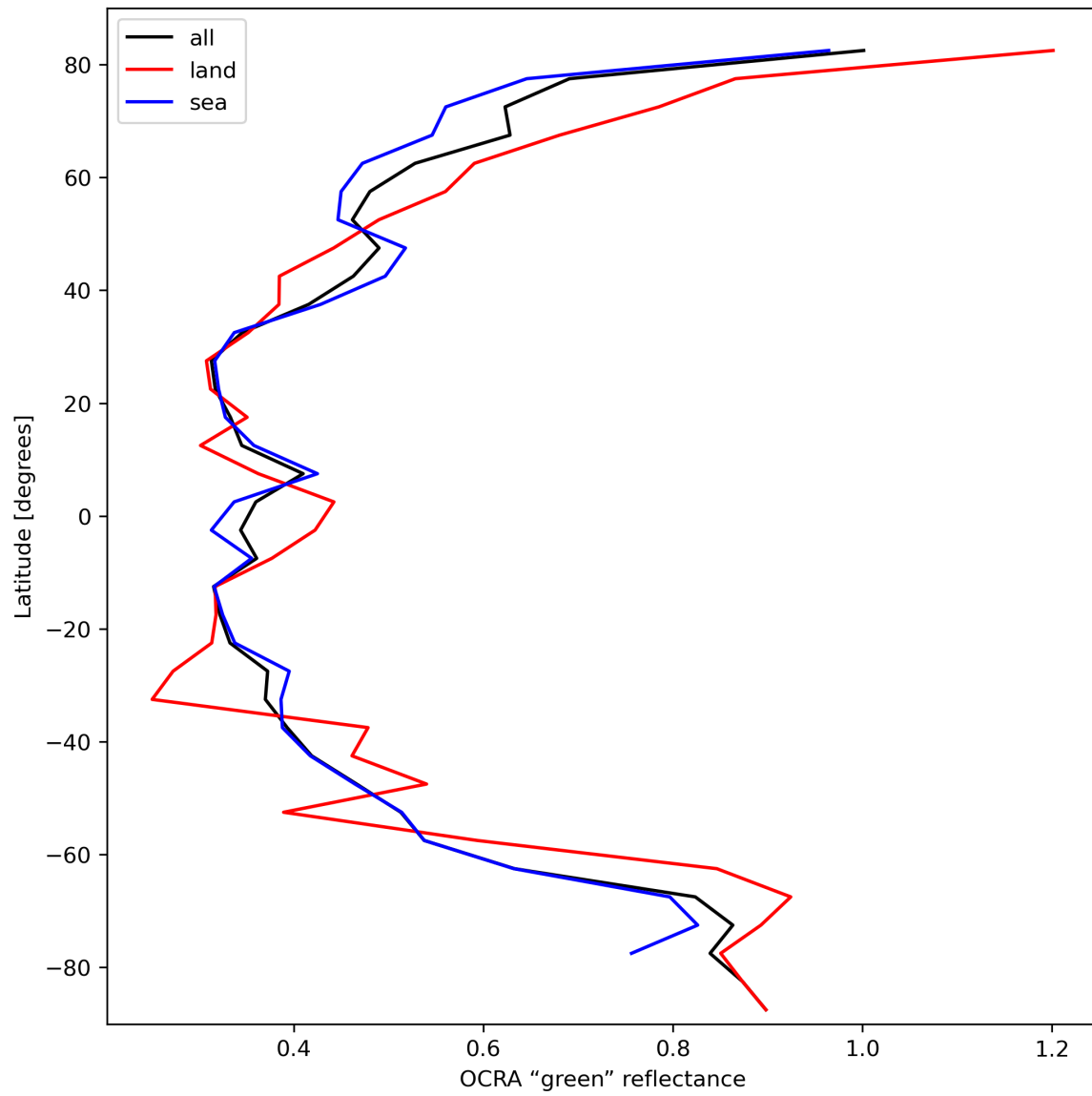
Figure 36: Zonal average of “OCRA “green” reflectance” for 2023-10-14 to 2023-10-16.
