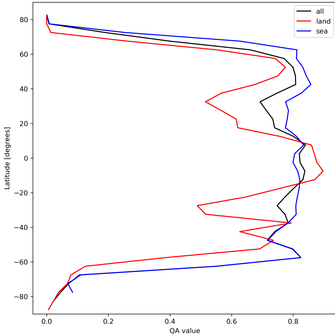
Figure 22: Zonal average of “QA value” for 2023-10-14 to 2023-10-16.
