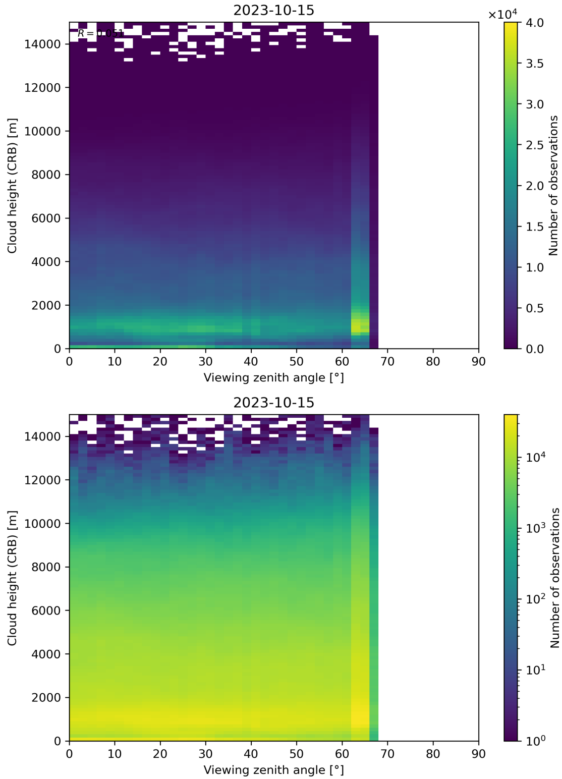
Figure 110: Scatter density plot of “Viewing zenith angle” against “Cloud height (CRB)” for 2023-10-14 to 2023-10-16.
