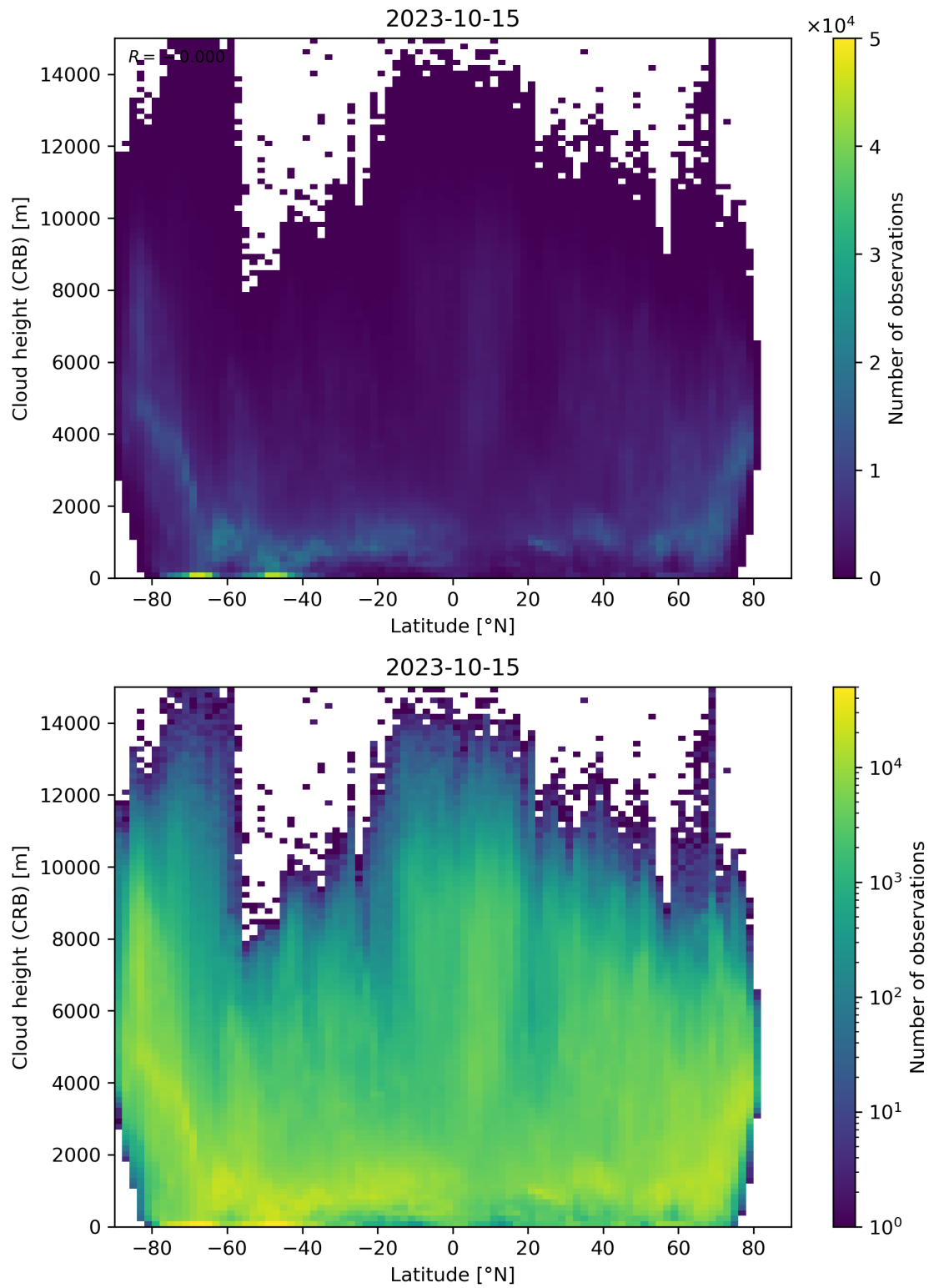
Figure 95: Scatter density plot of “Latitude” against “Cloud height (CRB)” for 2023-10-14 to 2023-10-16.
