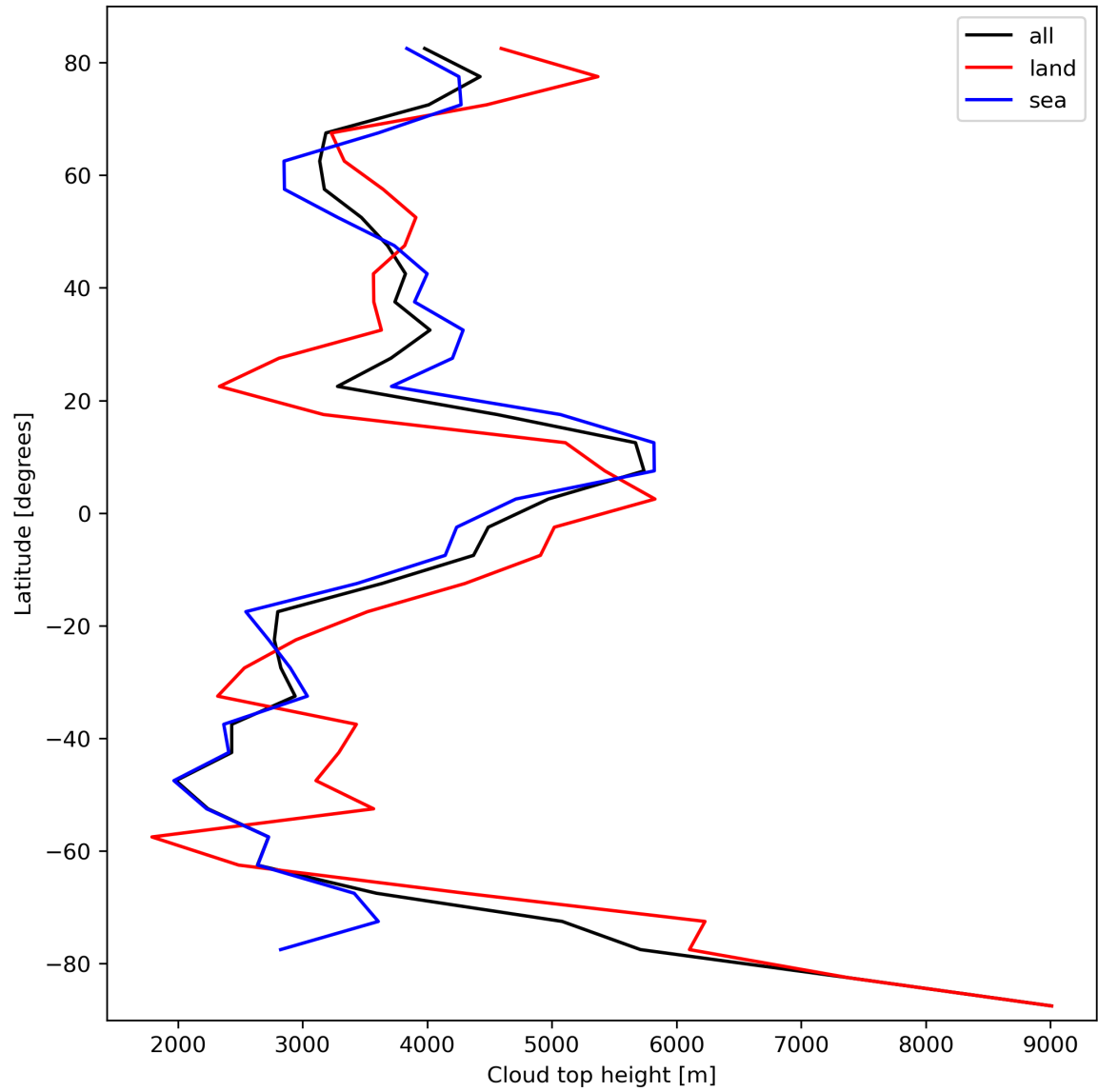
Figure 24: Zonal average of “Cloud top height” for 2023-10-14 to 2023-10-16.
