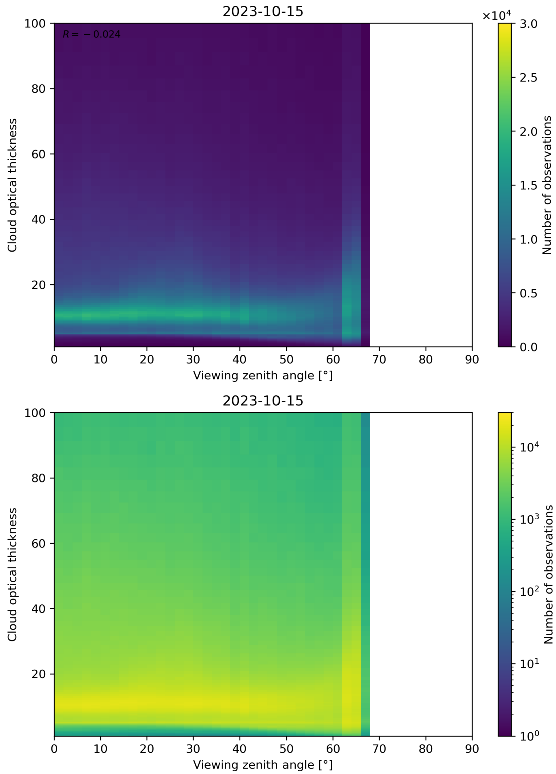
Figure 111: Scatter density plot of “Viewing zenith angle” against “Cloud optical thickness” for 2023-10-14 to 2023-10-16.
