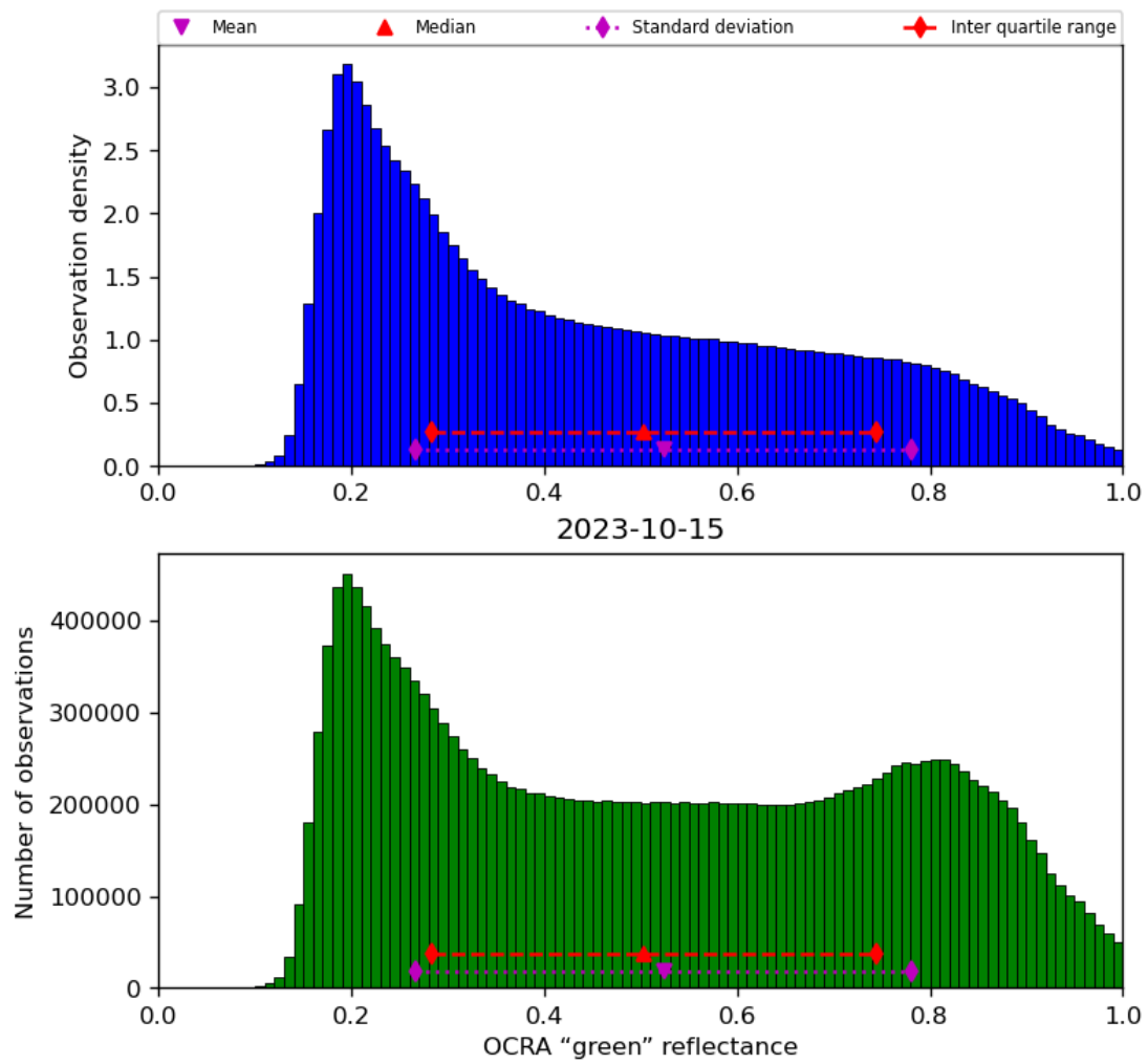
Figure 52: Histogram of “OCRA “green” reflectance” for 2023-10-14 to 2023-10-16
