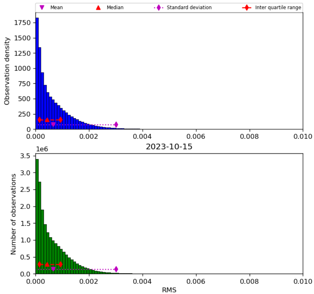
Figure 47: Histogram of “RMS” for 2023-10-14 to 2023-10-16
