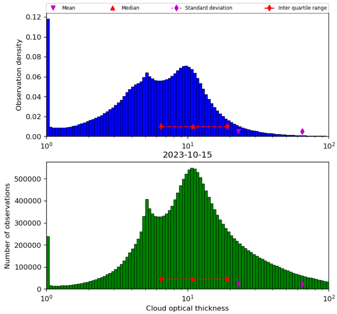
Figure 41: Histogram of “Cloud optical thickness” for 2023-10-14 to 2023-10-16
