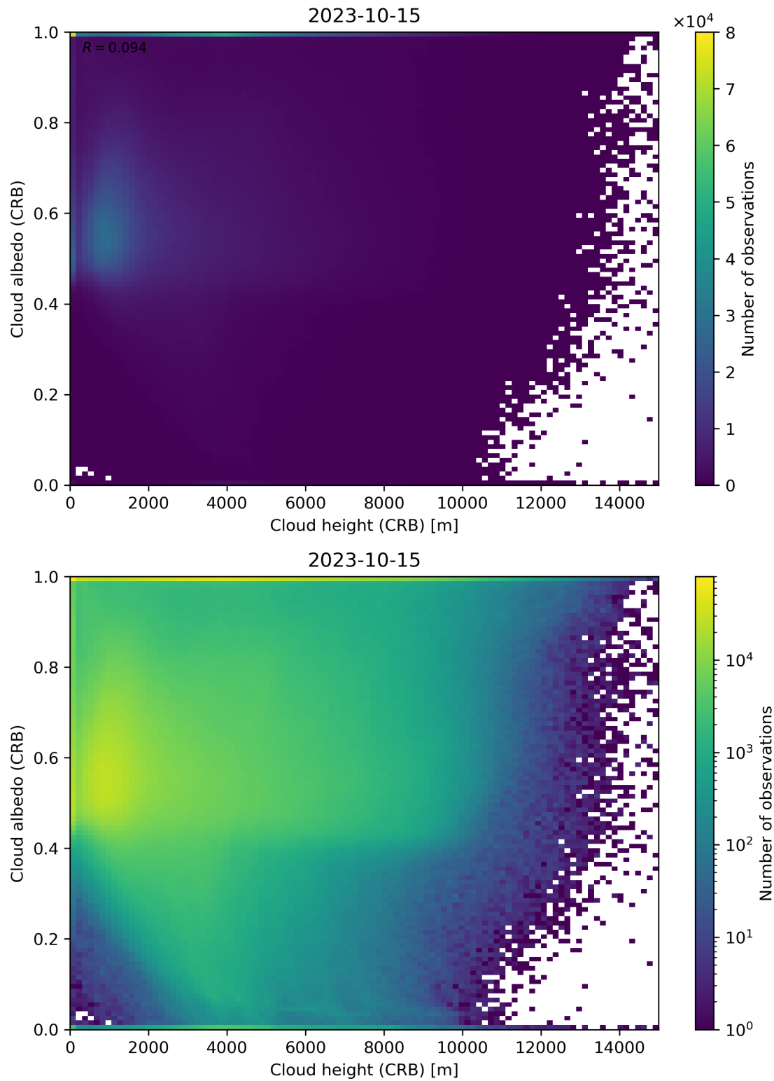
Figure 80: Scatter density plot of “Cloud height (CRB)” against “Cloud albedo (CRB)” for 2023-10-14 to 2023-10-16.
