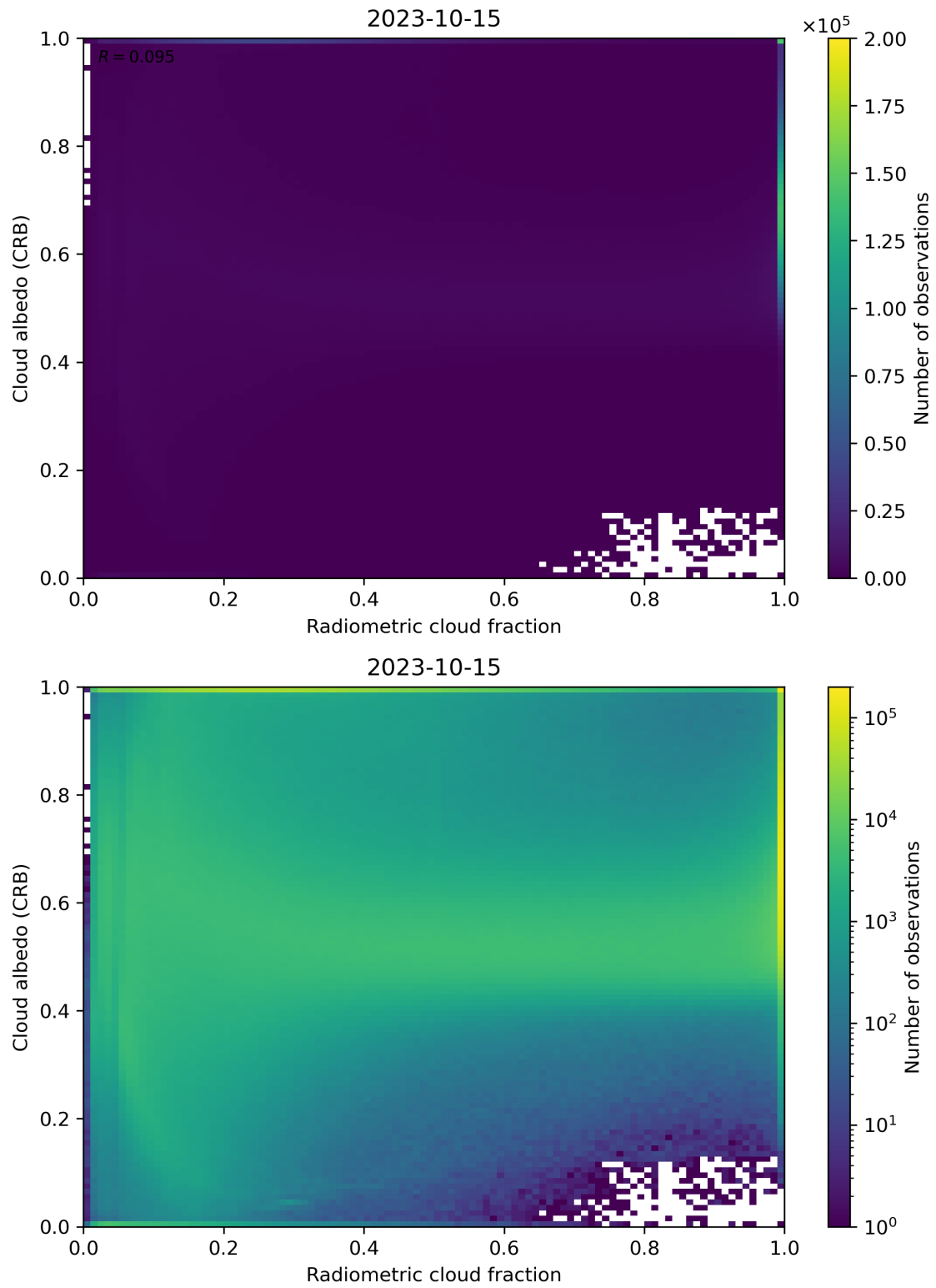
Figure 71: Scatter density plot of “Radiometric cloud fraction” against “Cloud albedo (CRB)” for 2023-10-14 to 2023-10-16.
