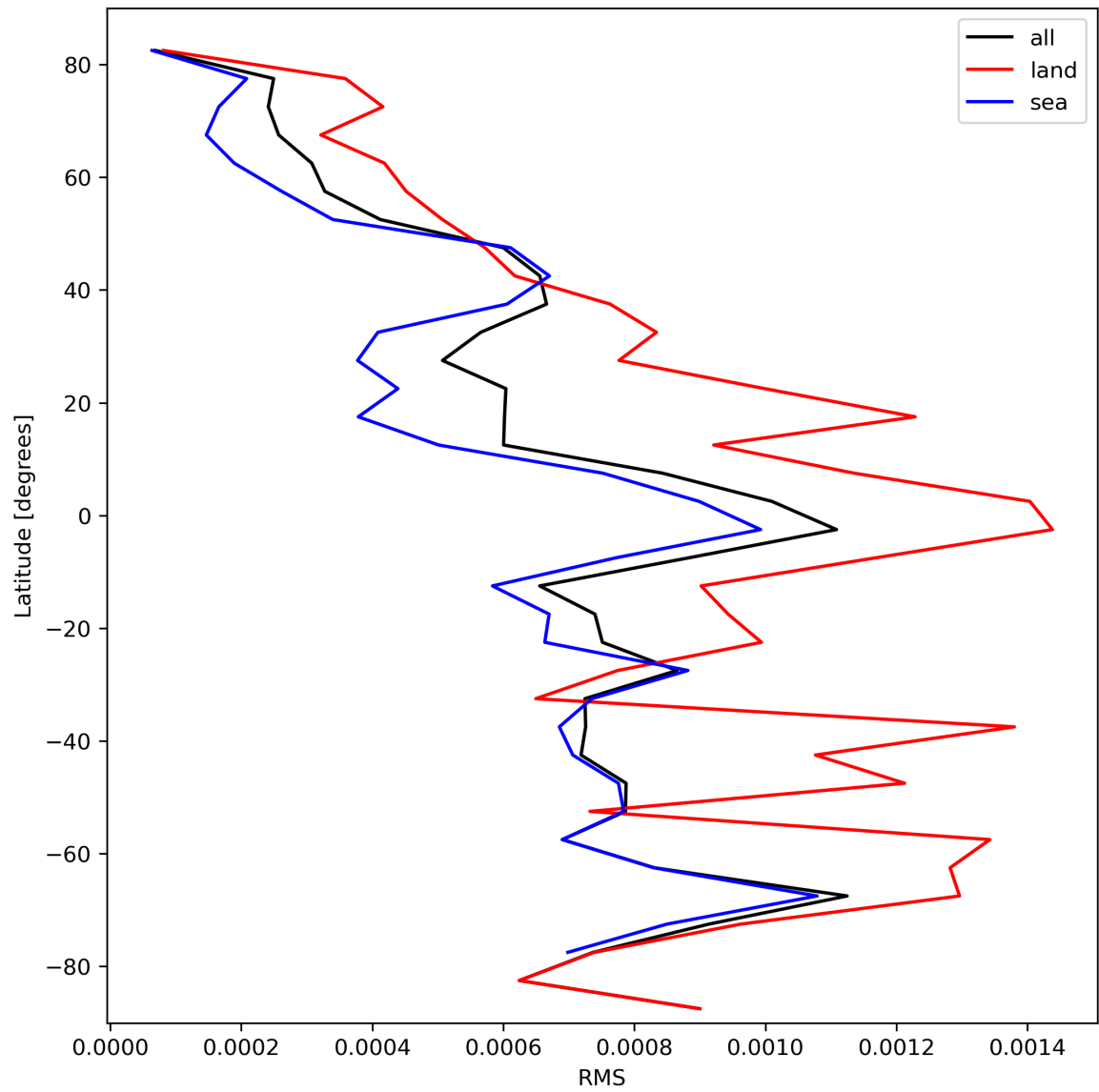
Figure 31: Zonal average of “RMS” for 2023-10-14 to 2023-10-16.
