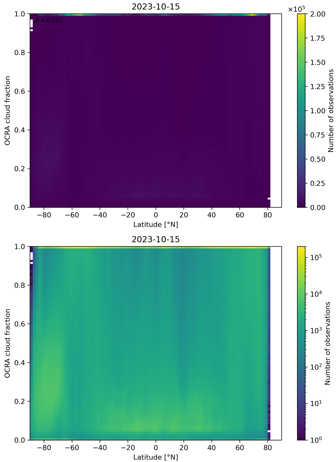
Figure 93: Scatter density plot of “Latitude” against “OCRA cloud fraction” for 2023-10-14 to 2023-10-16.
