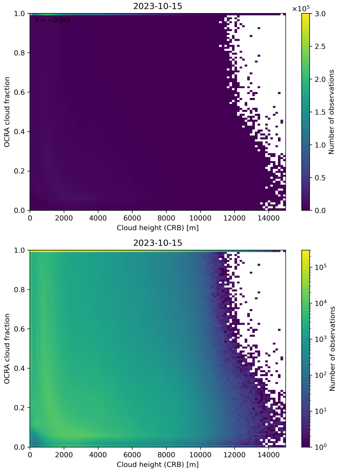
Figure 81: Scatter density plot of “Cloud height (CRB)” against “OCRA cloud fraction” for 2023-10-14 to 2023-10-16.
