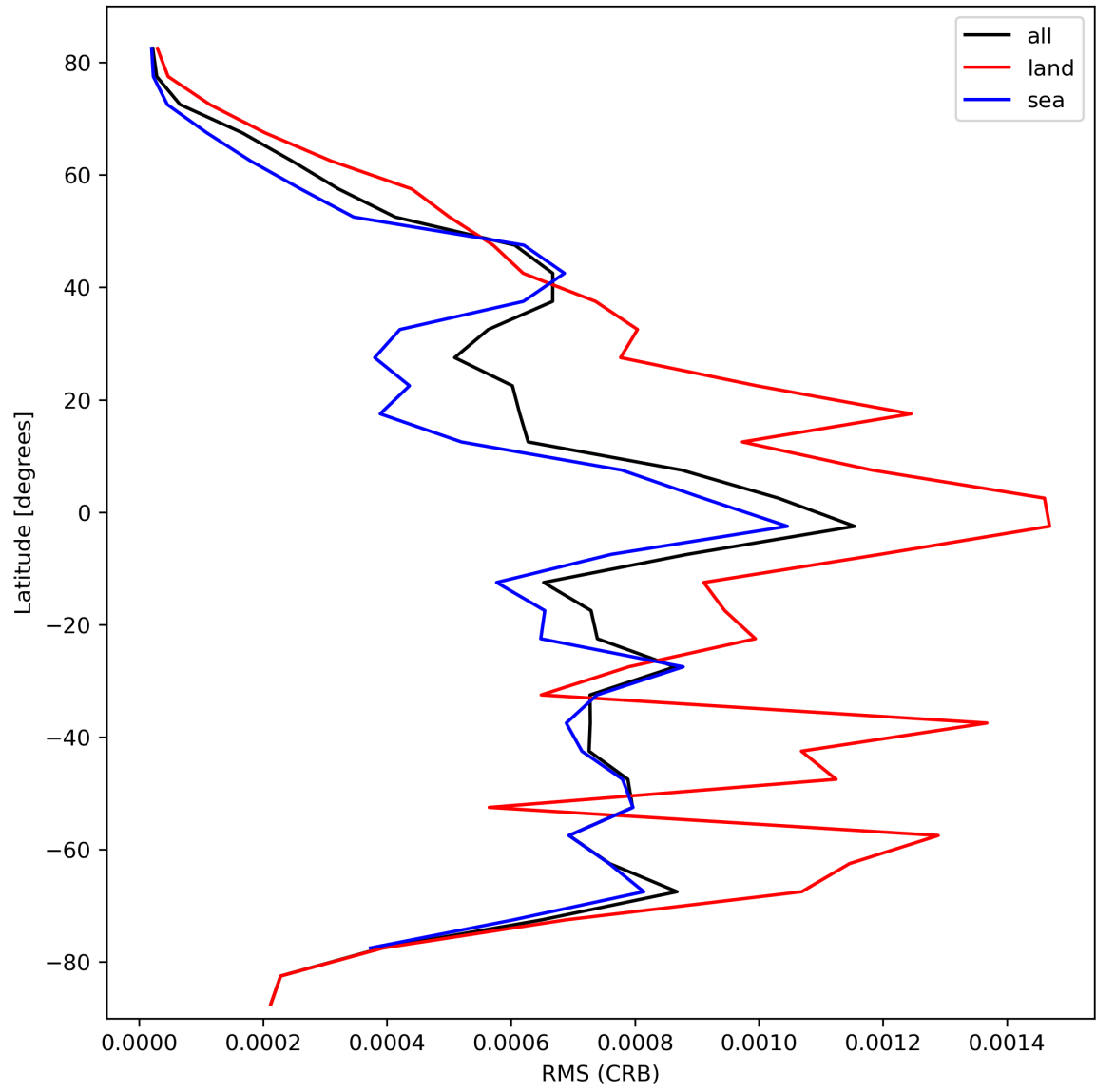
Figure 32: Zonal average of “RMS (CRB)” for 2023-10-14 to 2023-10-16.
