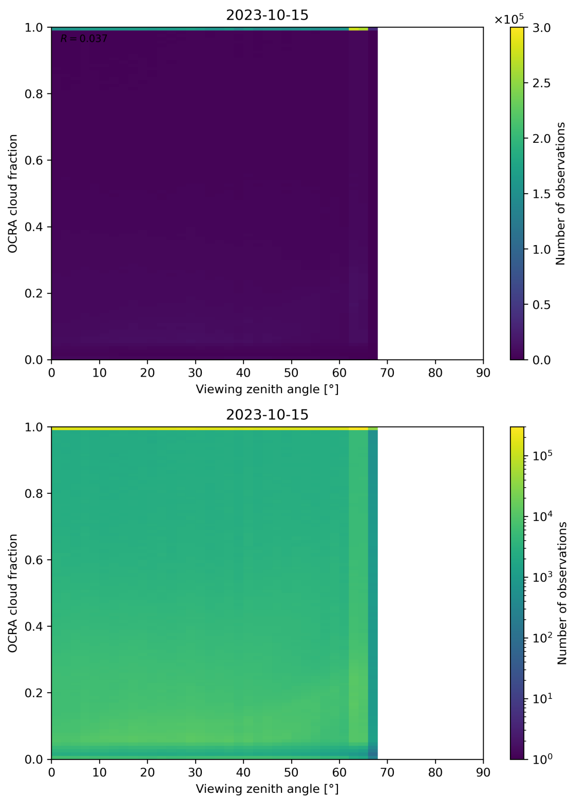
Figure 108: Scatter density plot of “Viewing zenith angle” against “OCRA cloud fraction” for 2023-10-14 to 2023-10-16.
