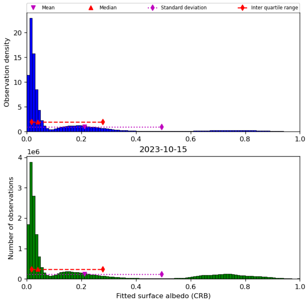
Figure 46: Histogram of “Fitted surface albedo (CRB)” for 2023-10-14 to 2023-10-16
