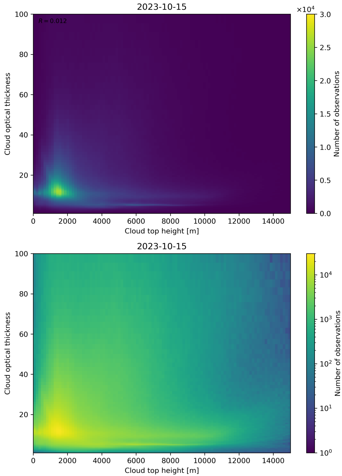
Figure 90: Scatter density plot of “Cloud top height” against “Cloud optical thickness” for 2023-10-14 to 2023-10-16.
