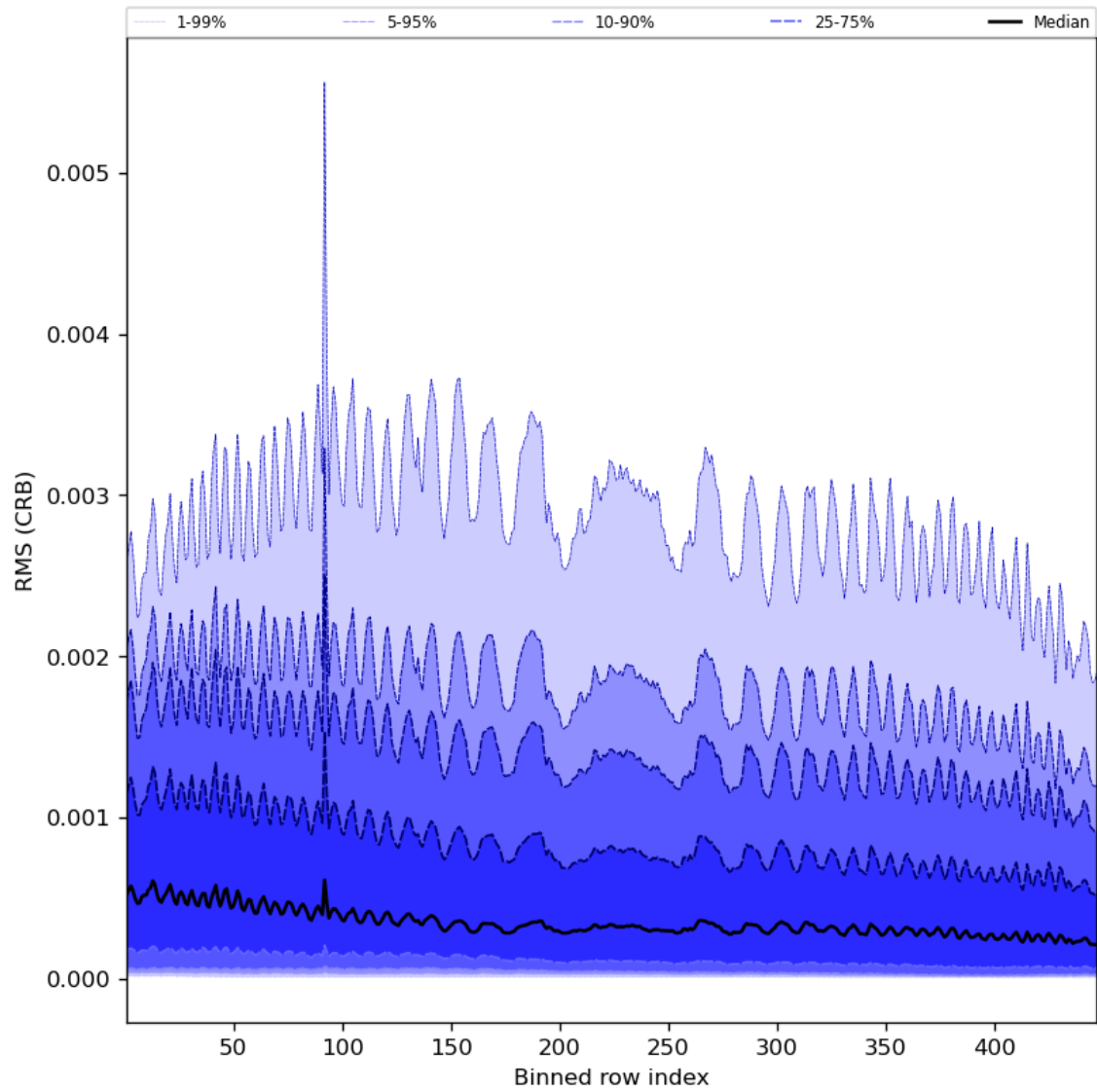
Figure 64: Along track statistics of “RMS (CRB)” for 2023-10-14 to 2023-10-16
