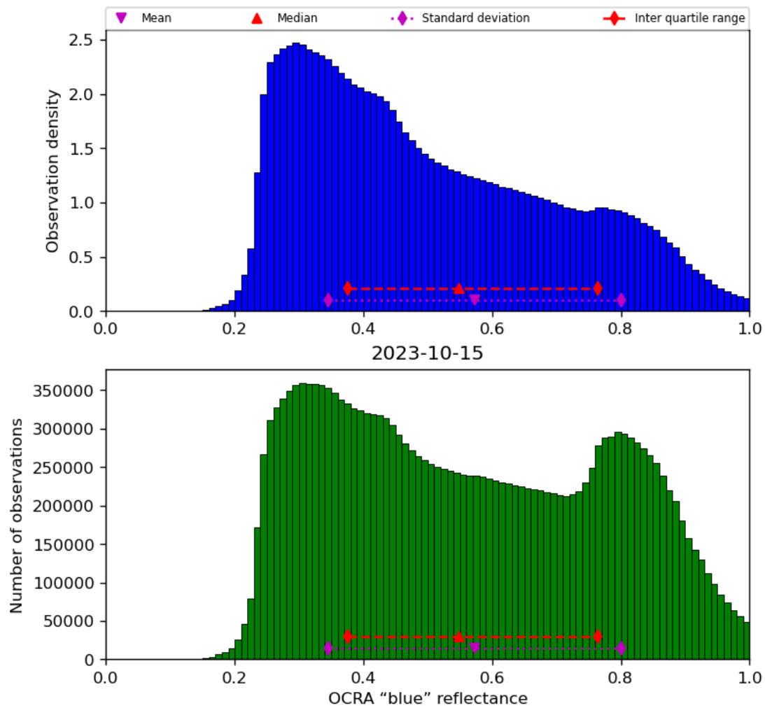
Figure 51: Histogram of “OCRA “blue” reflectance” for 2023-10-14 to 2023-10-16
