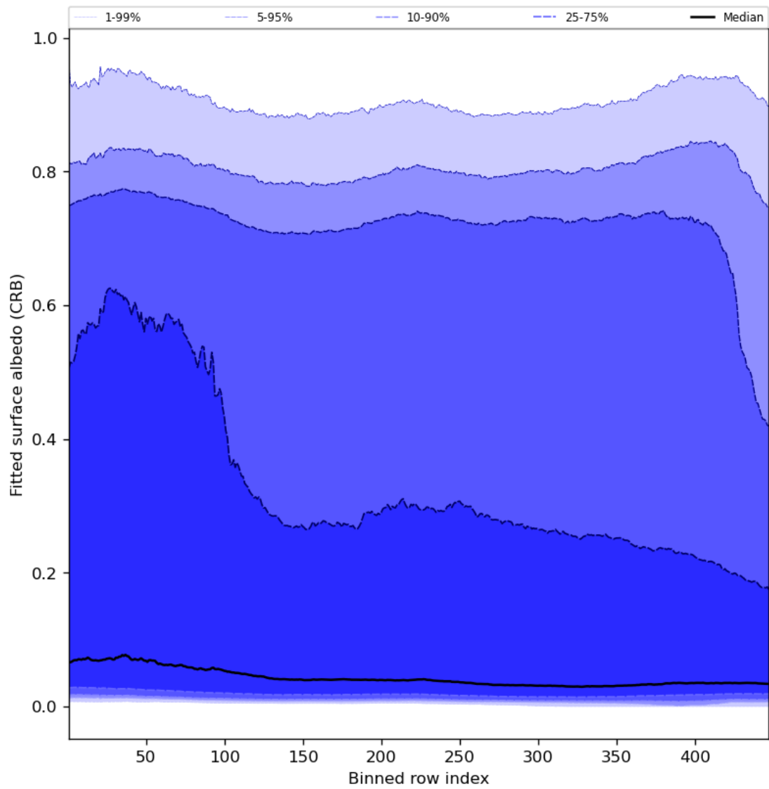
Figure 62: Along track statistics of “Fitted surface albedo (CRB)” for 2023-10-14 to 2023-10-16
