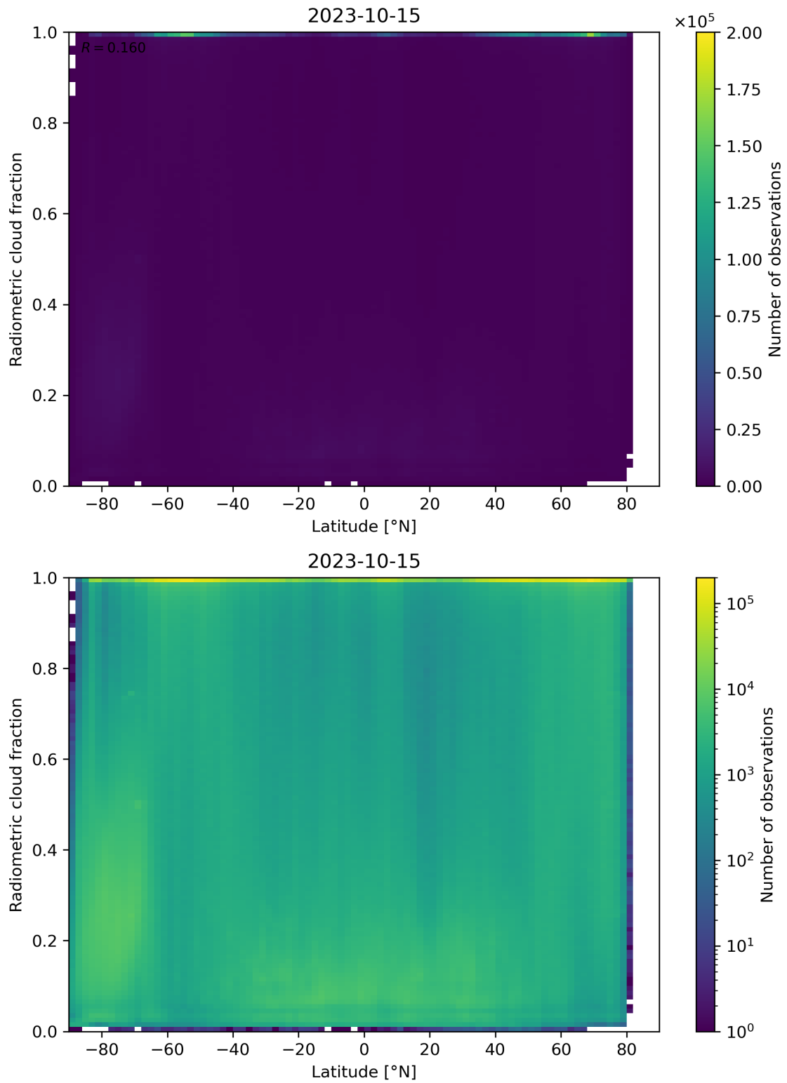
Figure 92: Scatter density plot of “Latitude” against “Radiometric cloud fraction” for 2023-10-14 to 2023-10-16.
