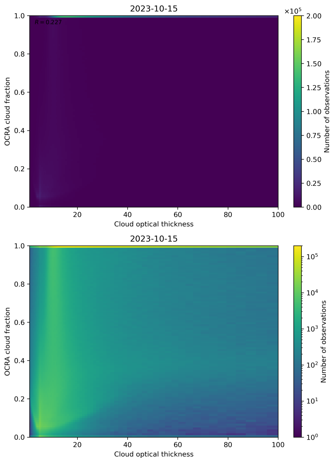
Figure 83: Scatter density plot of “Cloud optical thickness” against “OCRA cloud fraction” for 2023-10-14 to 2023-10-16.
