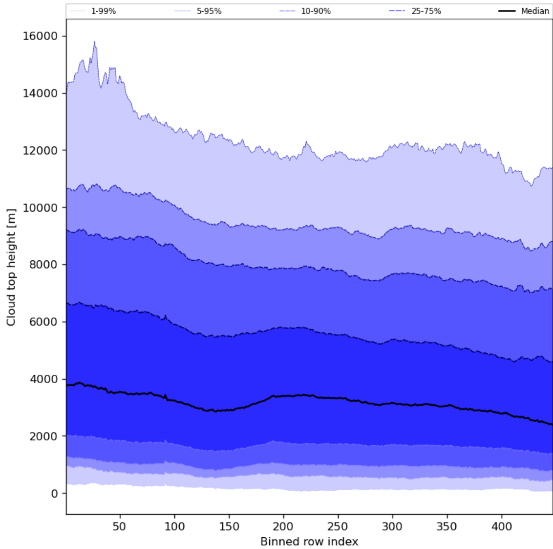
Figure 56: Along track statistics of “Cloud top height” for 2023-10-14 to 2023-10-16
