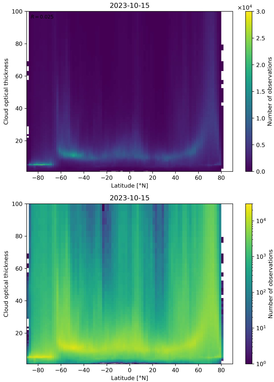
Figure 96: Scatter density plot of “Latitude” against “Cloud optical thickness” for 2023-10-14 to 2023-10-16.
