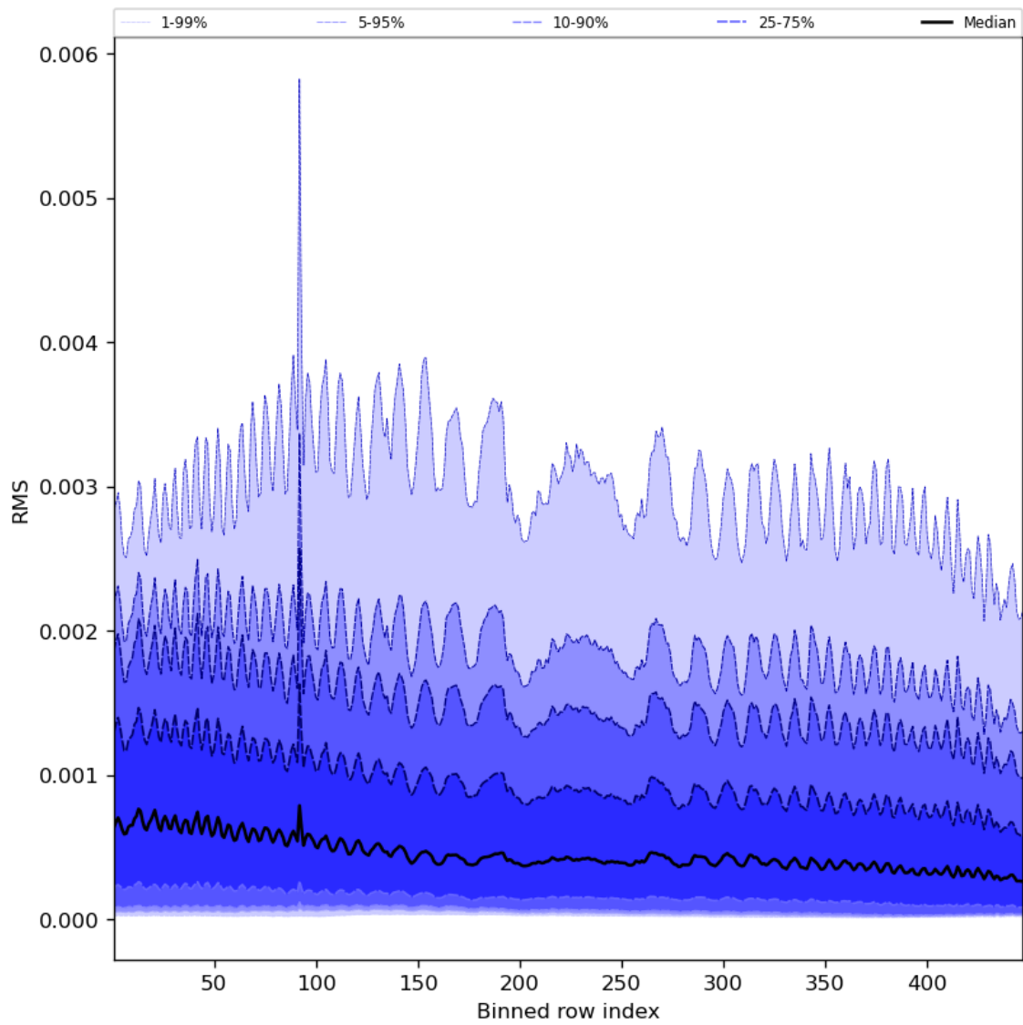
Figure 63: Along track statistics of “RMS” for 2023-10-14 to 2023-10-16
