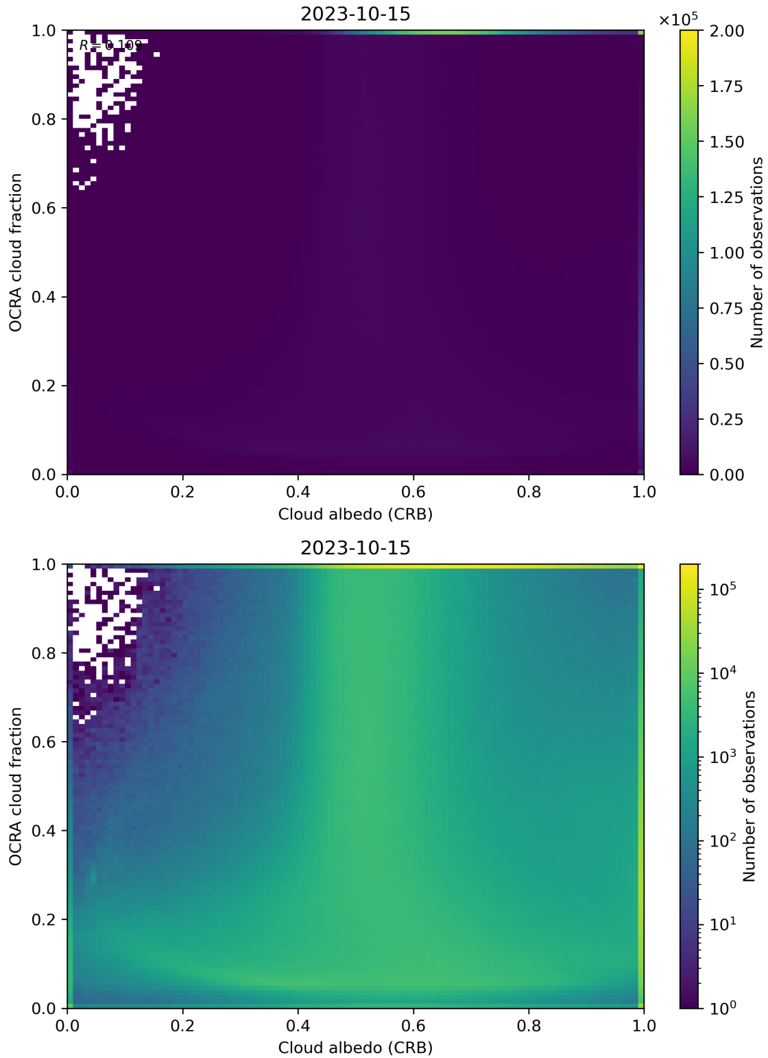
Figure 70: Scatter density plot of “Cloud albedo (CRB)” against “OCRA cloud fraction” for 2023-10-14 to 2023-10-16.
