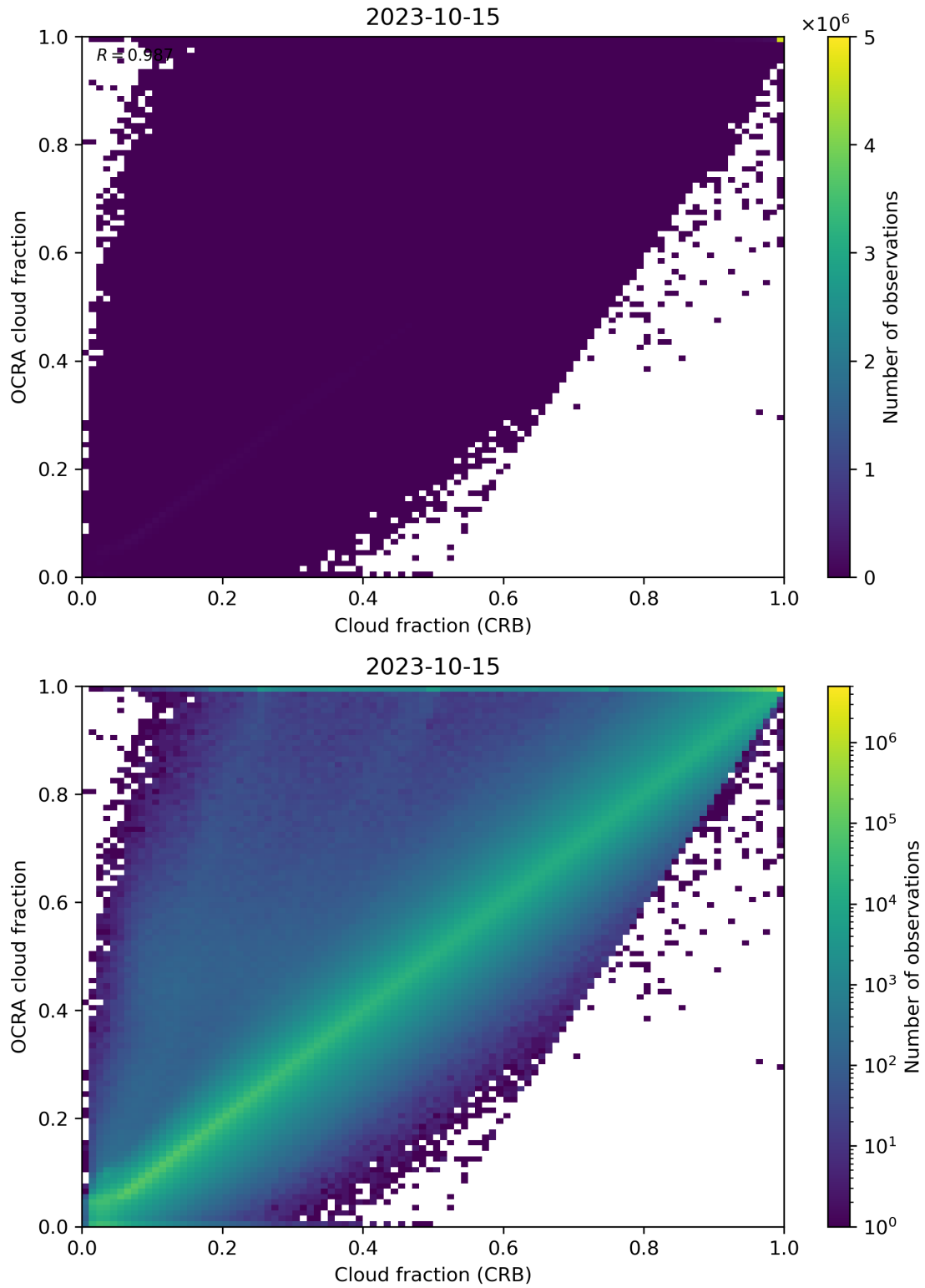
Figure 78: Scatter density plot of “Cloud fraction (CRB)” against “OCRA cloud fraction” for 2023-10-14 to 2023-10-16.
