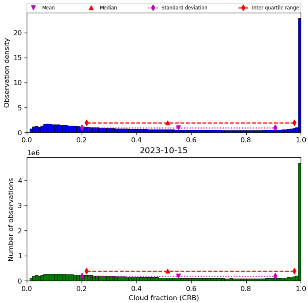
Figure 42: Histogram of “Cloud fraction (CRB)” for 2023-10-14 to 2023-10-16
