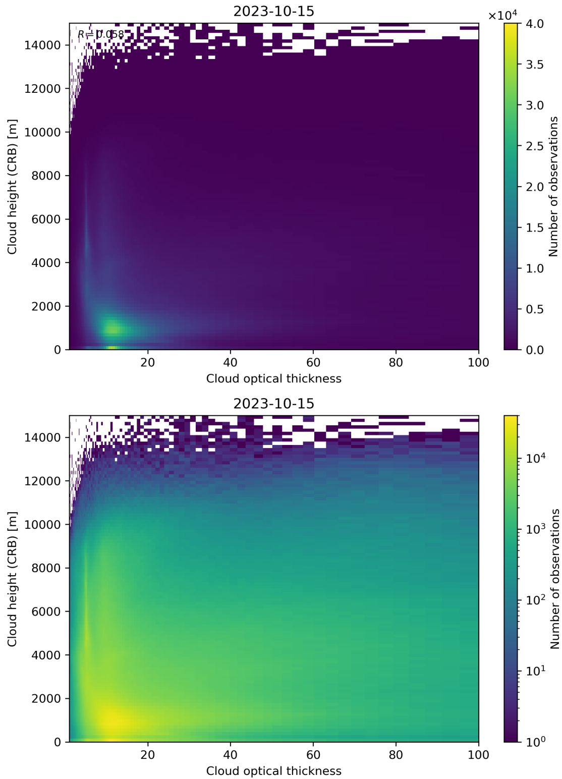
Figure 85: Scatter density plot of “Cloud optical thickness” against “Cloud height (CRB)” for 2023-10-14 to 2023-10-16.
