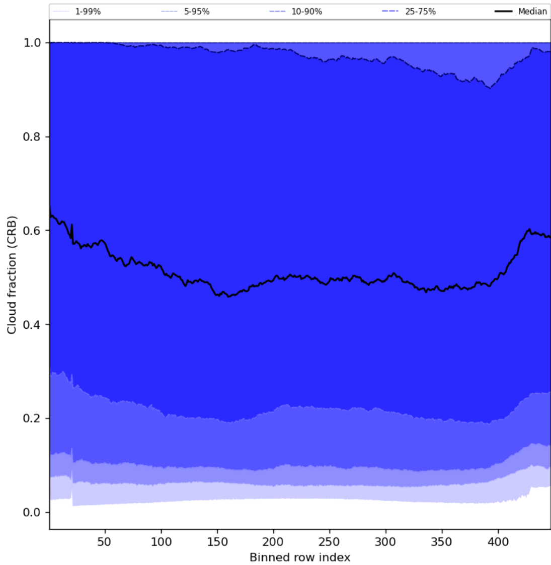
Figure 58: Along track statistics of “Cloud fraction (CRB)” for 2023-10-14 to 2023-10-16
