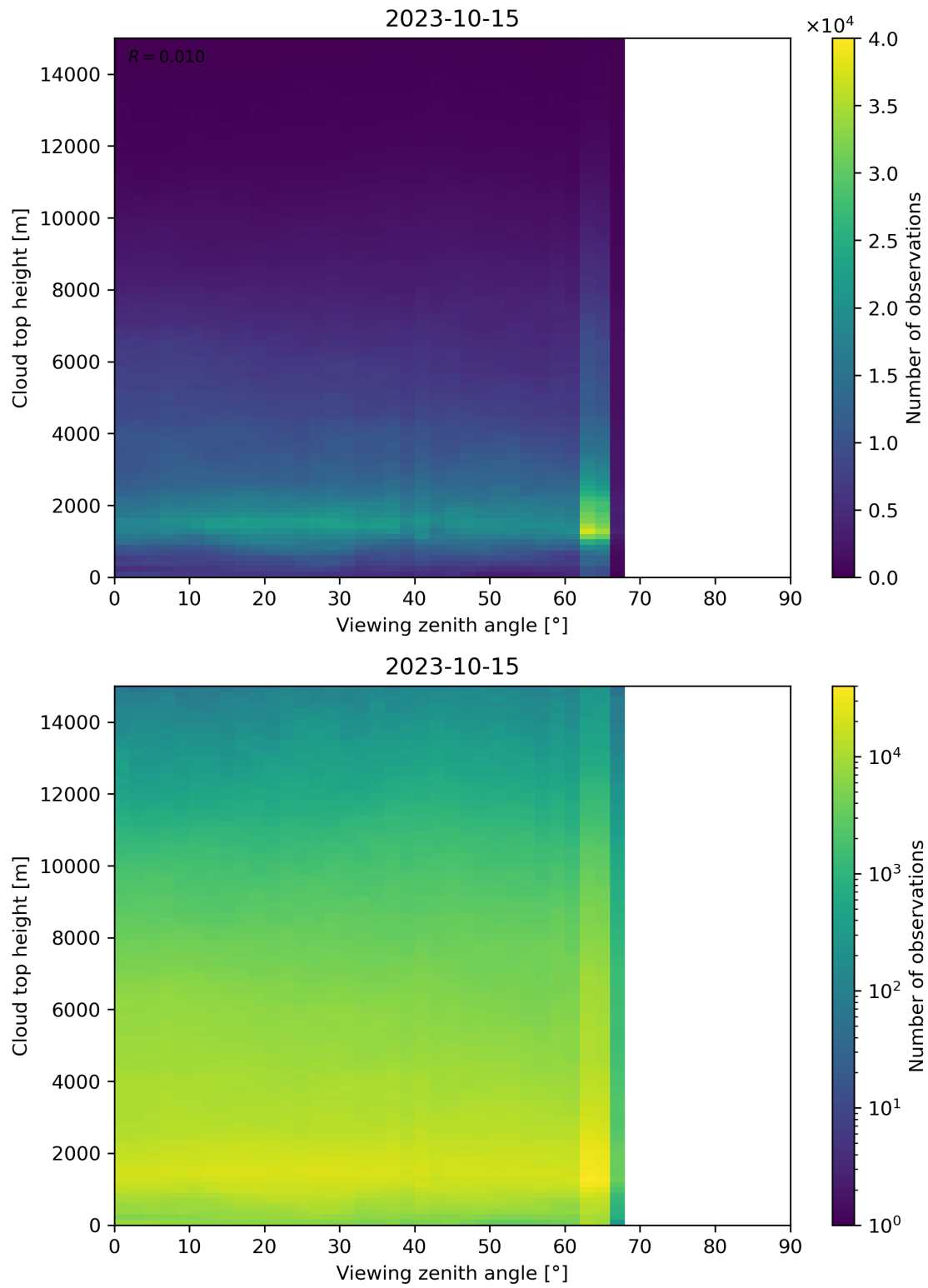
Figure 112: Scatter density plot of “Viewing zenith angle” against “Cloud top height” for 2023-10-14 to 2023-10-16.
