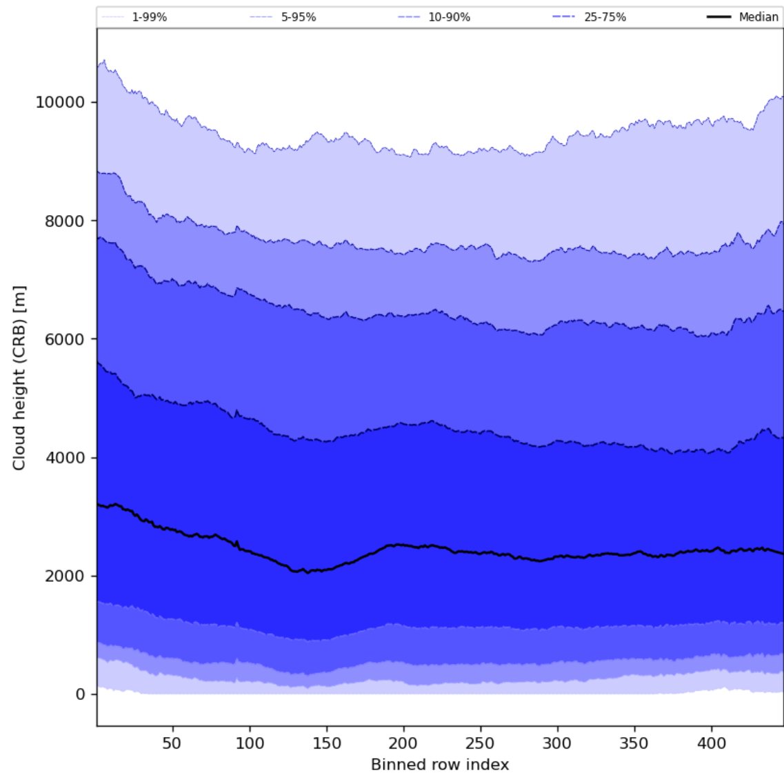
Figure 59: Along track statistics of “Cloud height (CRB)” for 2023-10-14 to 2023-10-16
