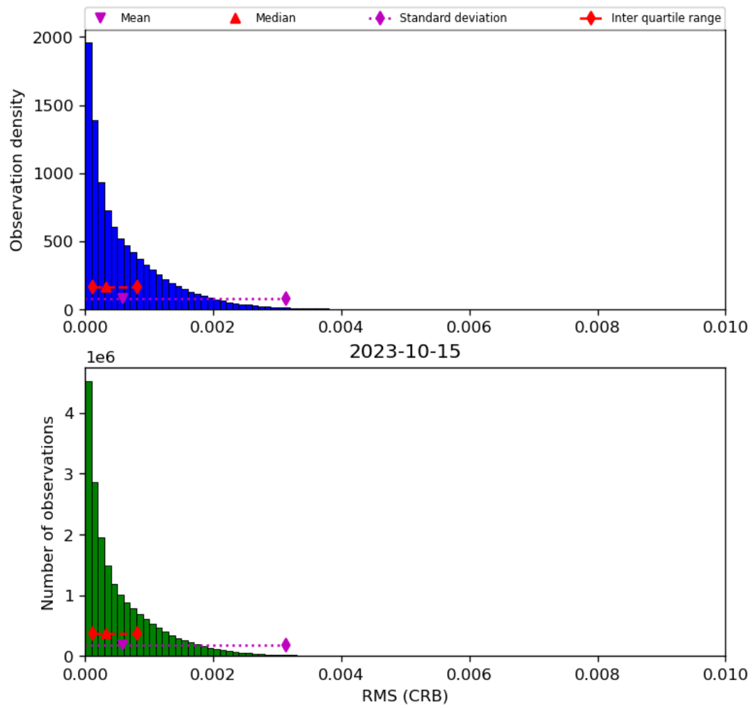
Figure 48: Histogram of “RMS (CRB)” for 2023-10-14 to 2023-10-16
