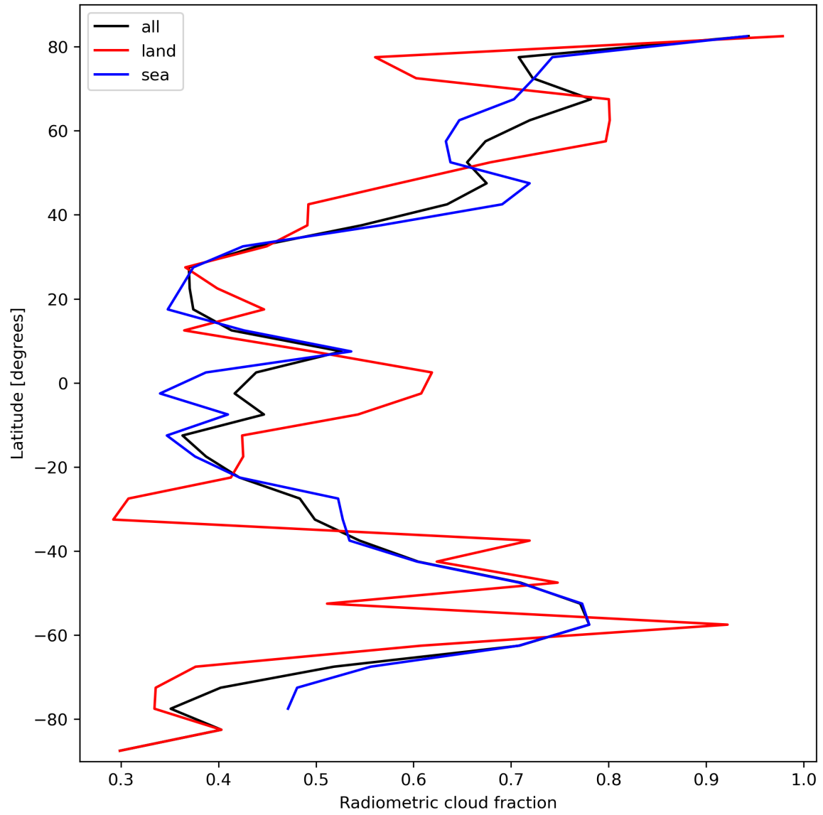
Figure 23: Zonal average of “Radiometric cloud fraction” for 2023-10-14 to 2023-10-16.
