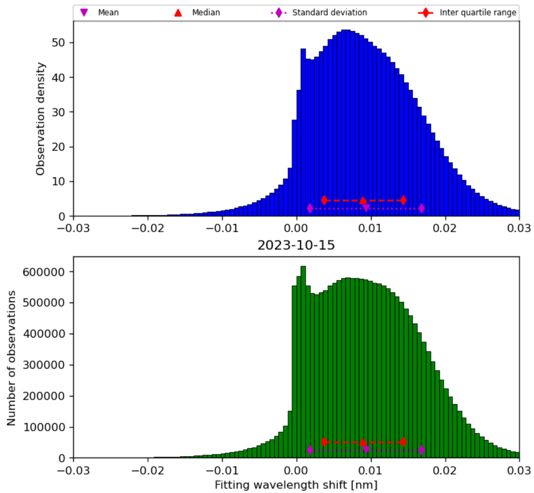
Figure 49: Histogram of “Fitting wavelength shift” for 2023-10-14 to 2023-10-16
