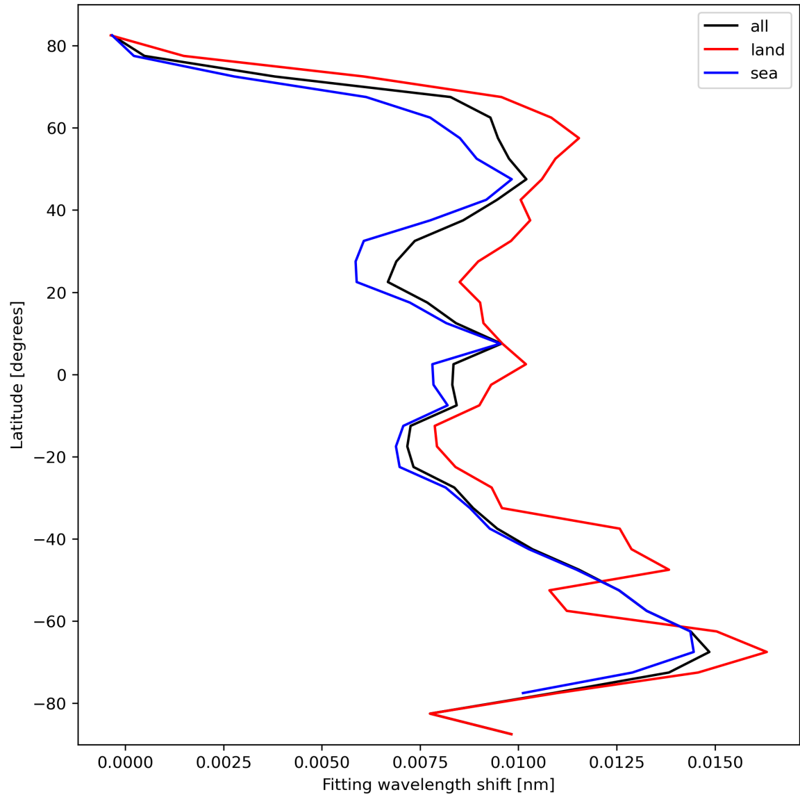
Figure 33: Zonal average of “Fitting wavelength shift” for 2023-10-14 to 2023-10-16.
