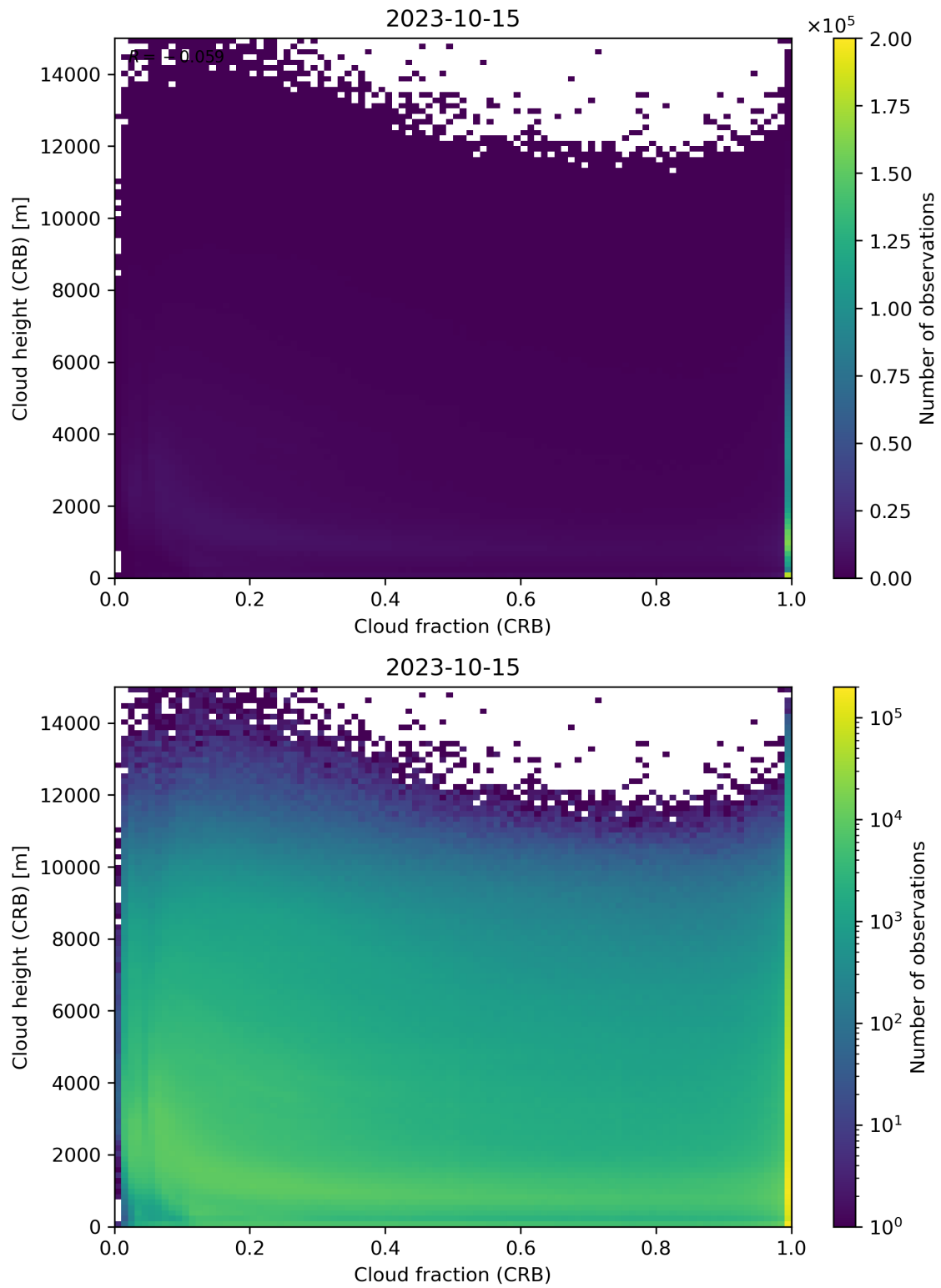
Figure 79: Scatter density plot of “Cloud fraction (CRB)” against “Cloud height (CRB)” for 2023-10-14 to 2023-10-16.
