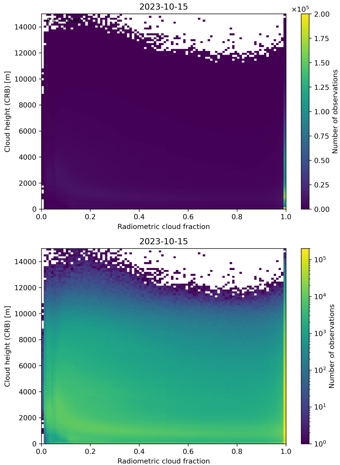
Figure 74: Scatter density plot of “Radiometric cloud fraction” against “Cloud height (CRB)” for 2023-10-14 to 2023-10-16.
