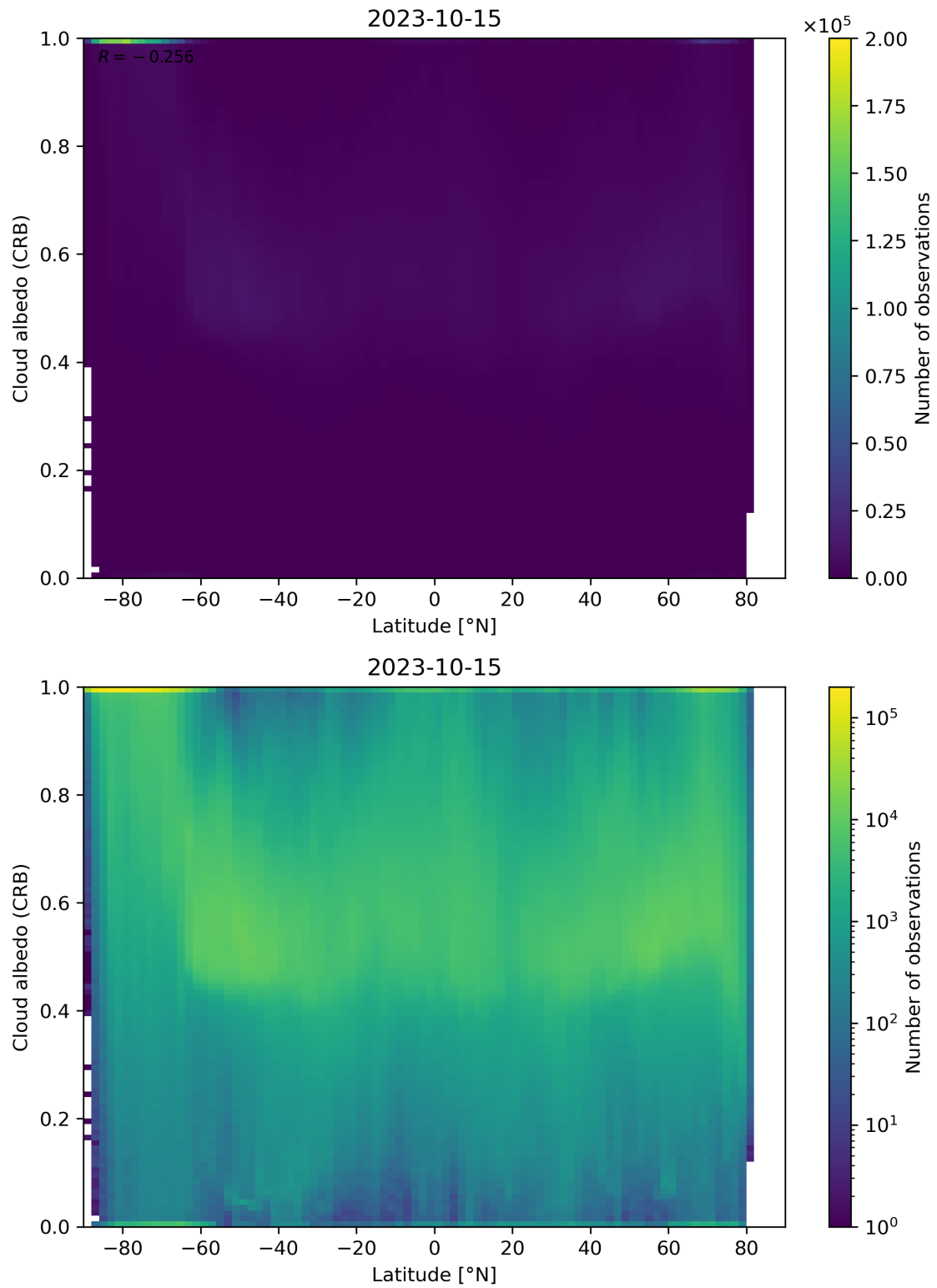
Figure 91: Scatter density plot of “Latitude” against “Cloud albedo (CRB)” for 2023-10-14 to 2023-10-16.
