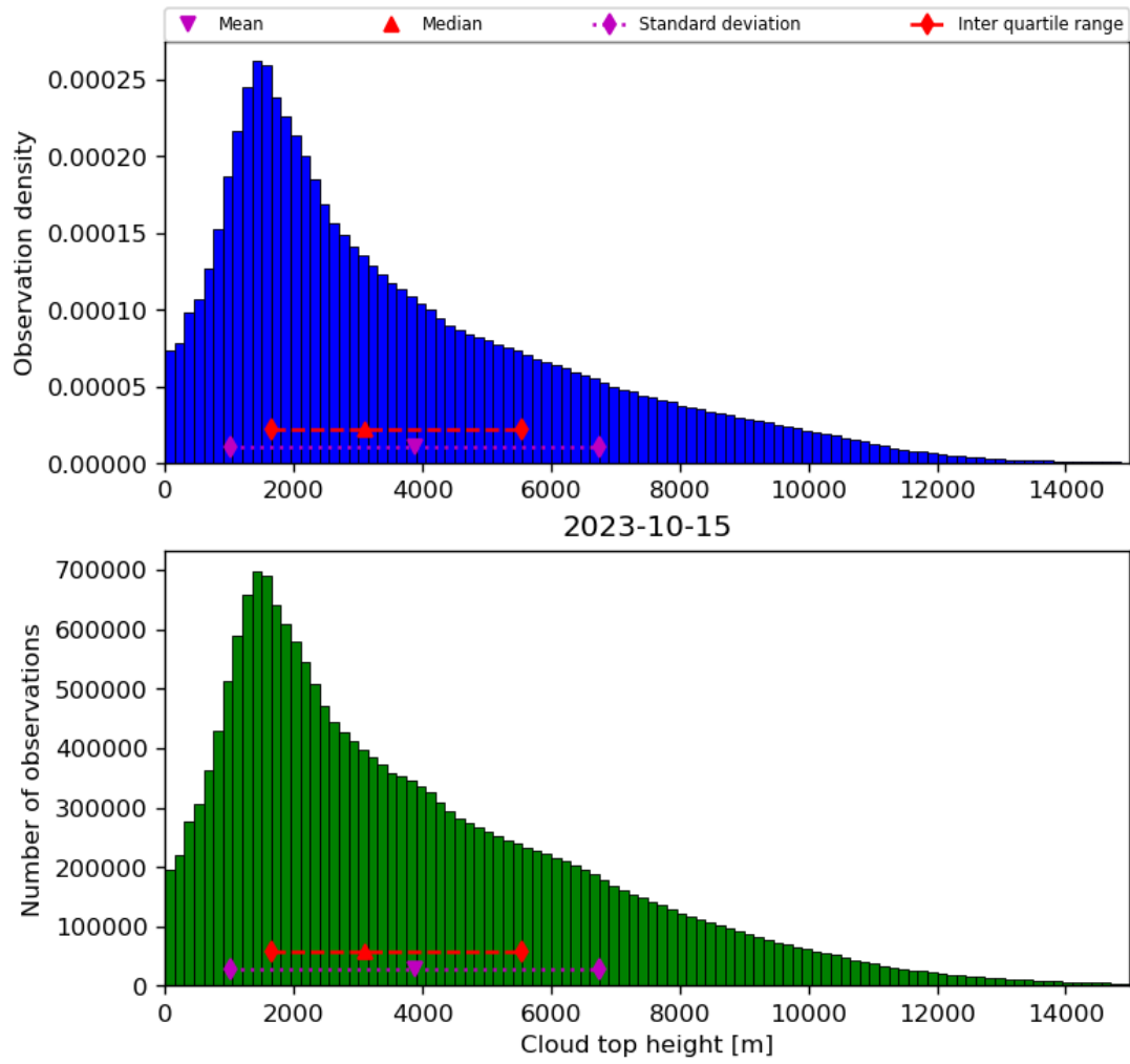
Figure 40: Histogram of “Cloud top height” for 2023-10-14 to 2023-10-16
