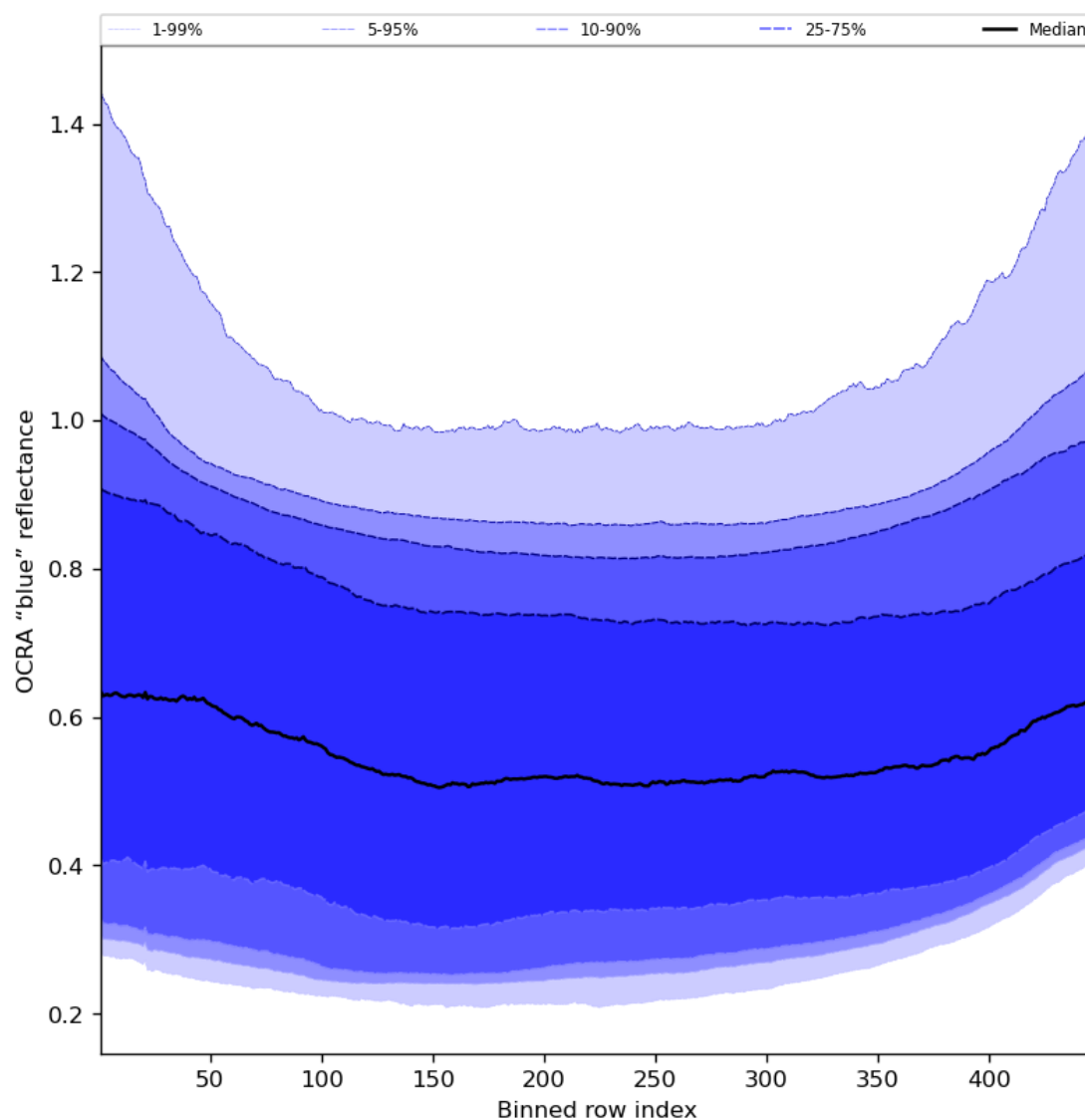
Figure 67: Along track statistics of “OCRA “blue” reflectance” for 2023-10-14 to 2023-10-16
