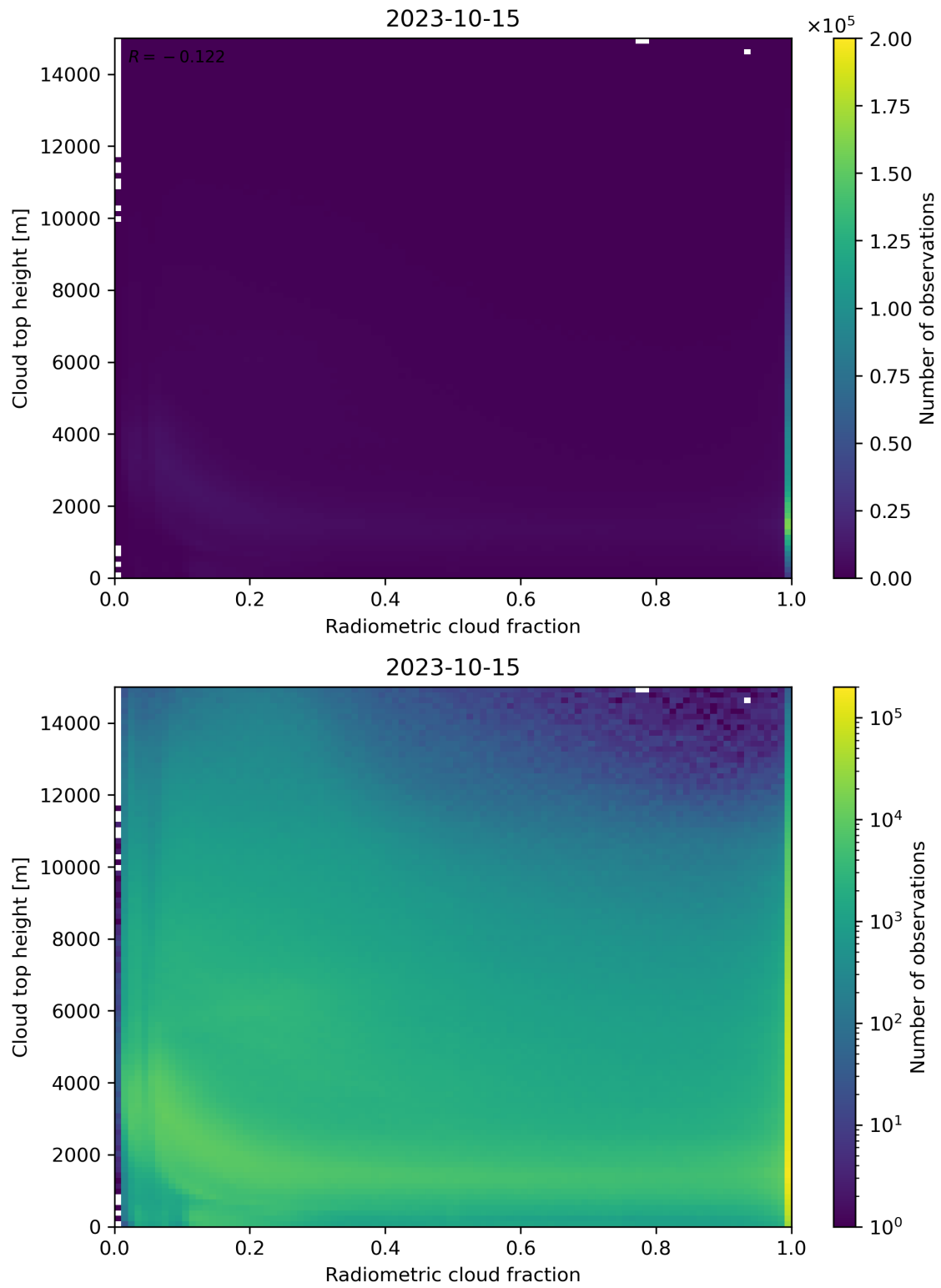
Figure 76: Scatter density plot of “Radiometric cloud fraction” against “Cloud top height” for 2023-10-14 to 2023-10-16.
