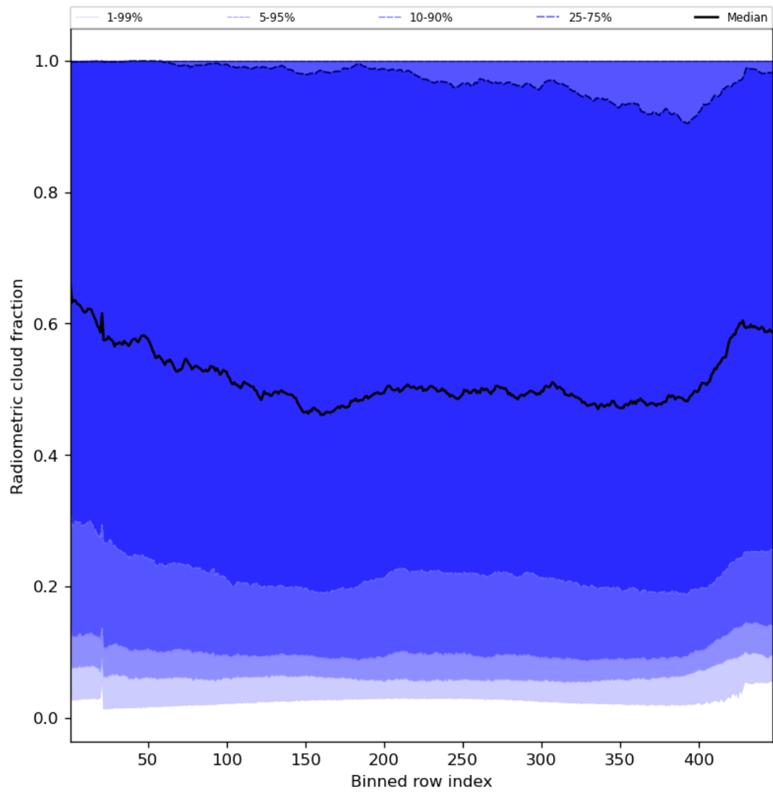
Figure 55: Along track statistics of “Radiometric cloud fraction” for 2023-10-14 to 2023-10-16
