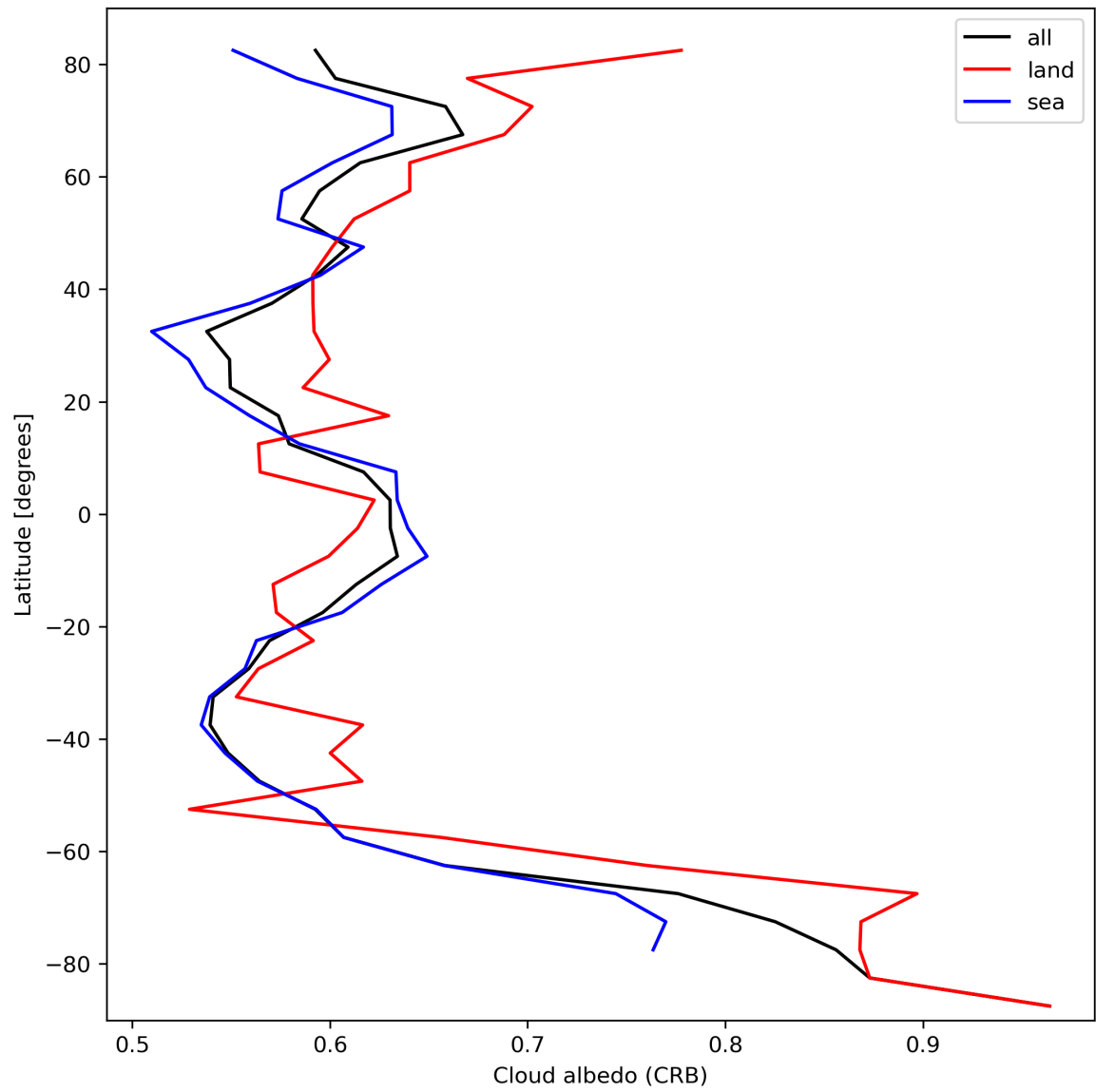
Figure 28: Zonal average of “Cloud albedo (CRB)” for 2023-10-14 to 2023-10-16.
