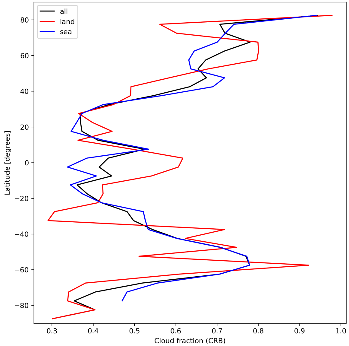
Figure 26: Zonal average of “Cloud fraction (CRB)” for 2023-10-14 to 2023-10-16.
