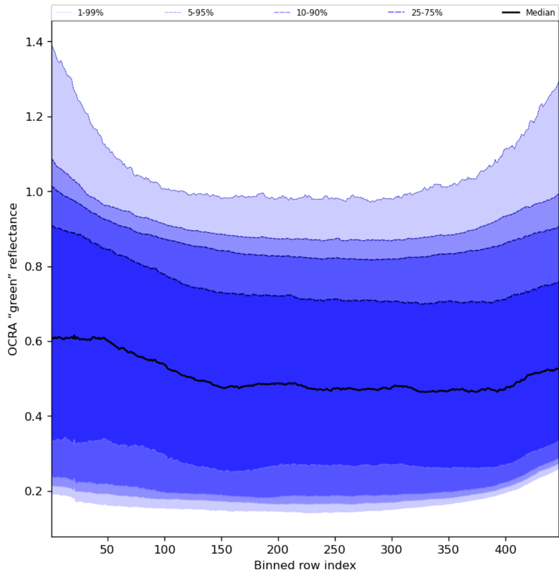
Figure 68: Along track statistics of “OCRA “green” reflectance” for 2023-10-14 to 2023-10-16
