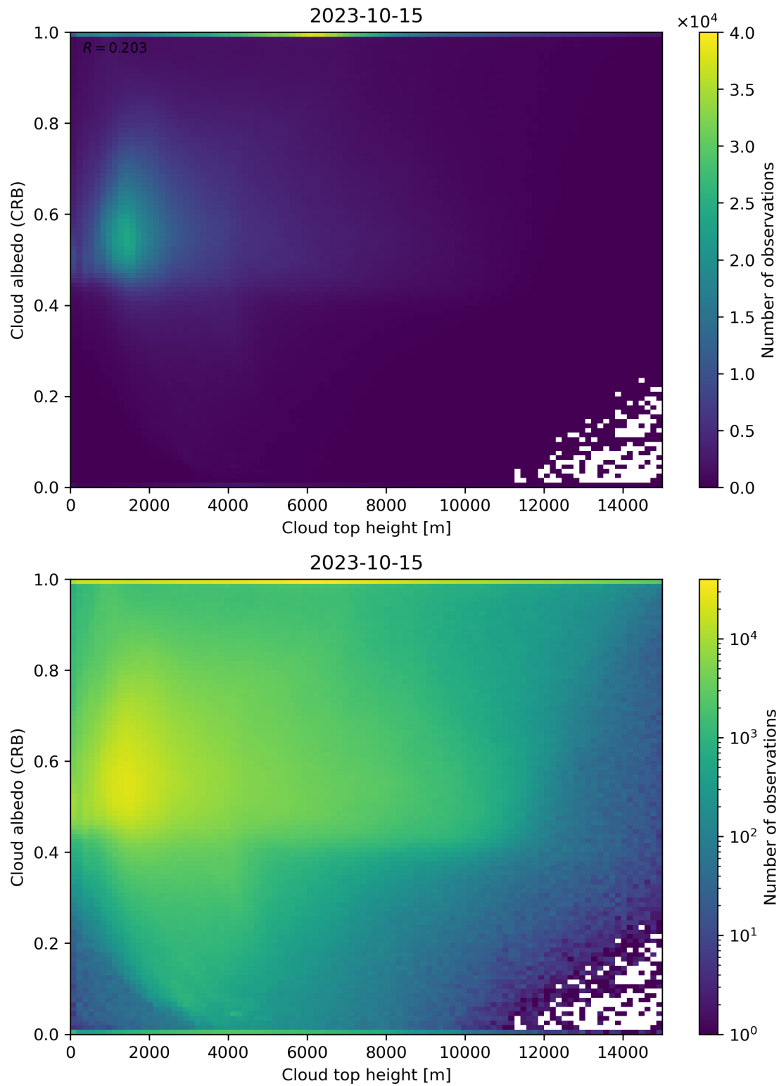
Figure 86: Scatter density plot of “Cloud top height” against “Cloud albedo (CRB)” for 2023-10-14 to 2023-10-16.
