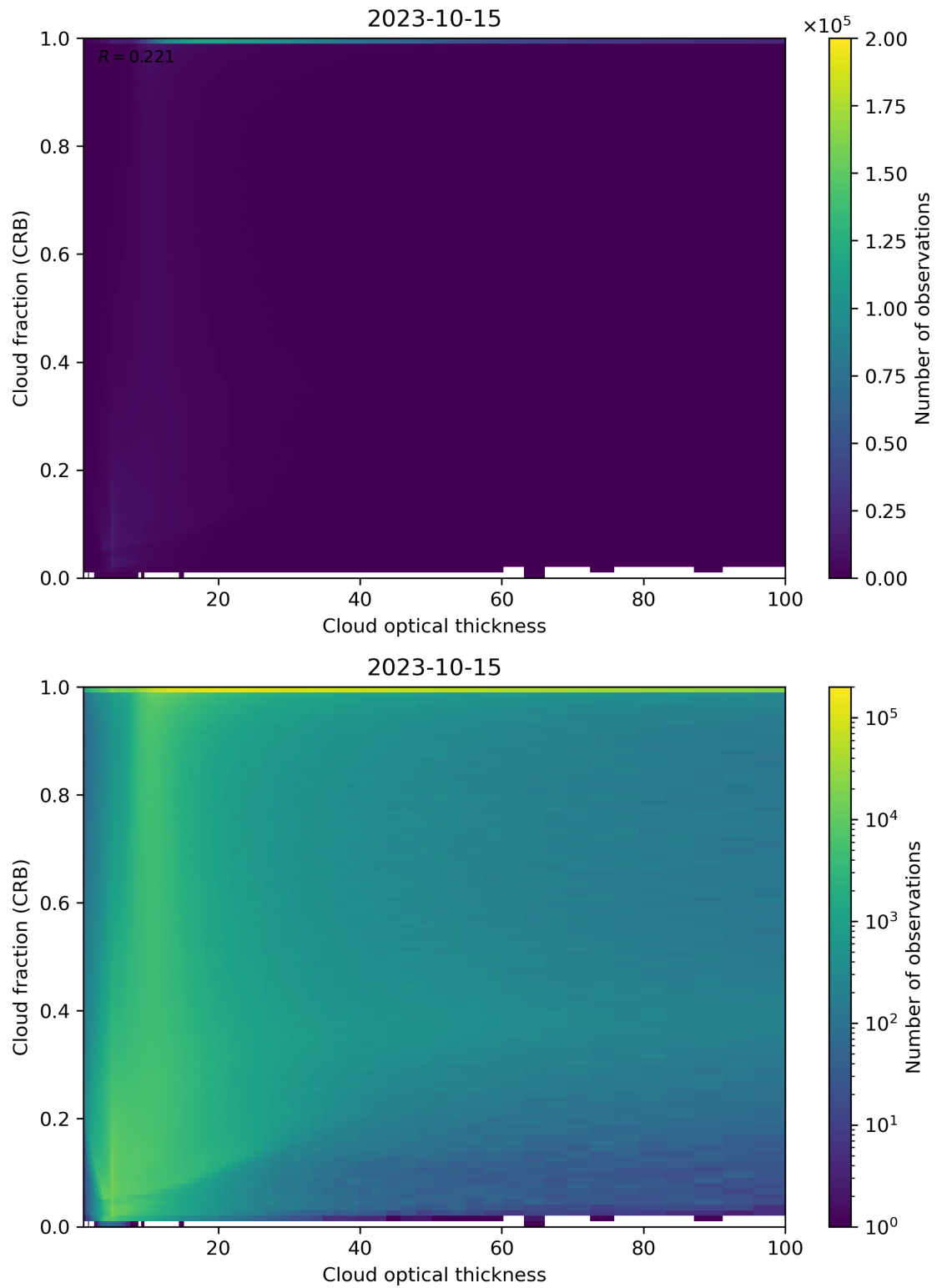
Figure 84: Scatter density plot of “Cloud optical thickness” against “Cloud fraction (CRB)” for 2023-10-14 to 2023-10-16.
