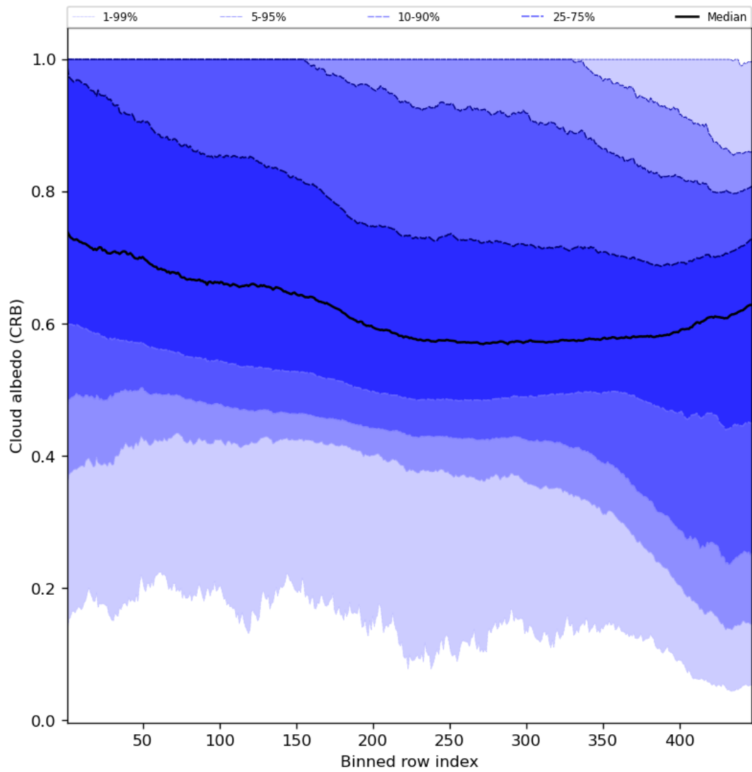
Figure 60: Along track statistics of “Cloud albedo (CRB)” for 2023-10-14 to 2023-10-16
