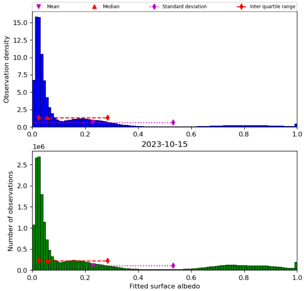
Figure 45: Histogram of “Fitted surface albedo” for 2023-10-14 to 2023-10-16
