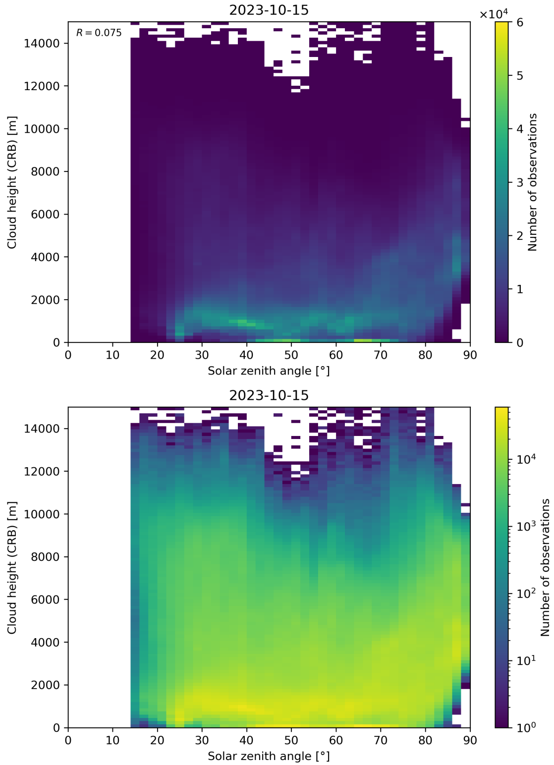
Figure 102: Scatter density plot of “Solar zenith angle” against “Cloud height (CRB)” for 2023-10-14 to 2023-10-16.
