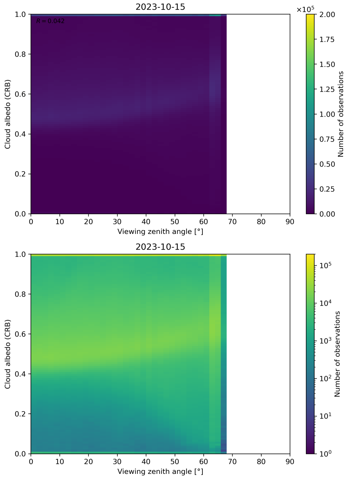
Figure 106: Scatter density plot of “Viewing zenith angle” against “Cloud albedo (CRB)” for 2023-10-14 to 2023-10-16.
