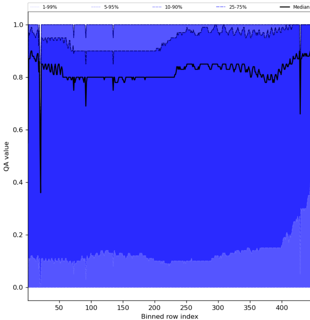
Figure 54: Along track statistics of “QA value” for 2023-10-14 to 2023-10-16
