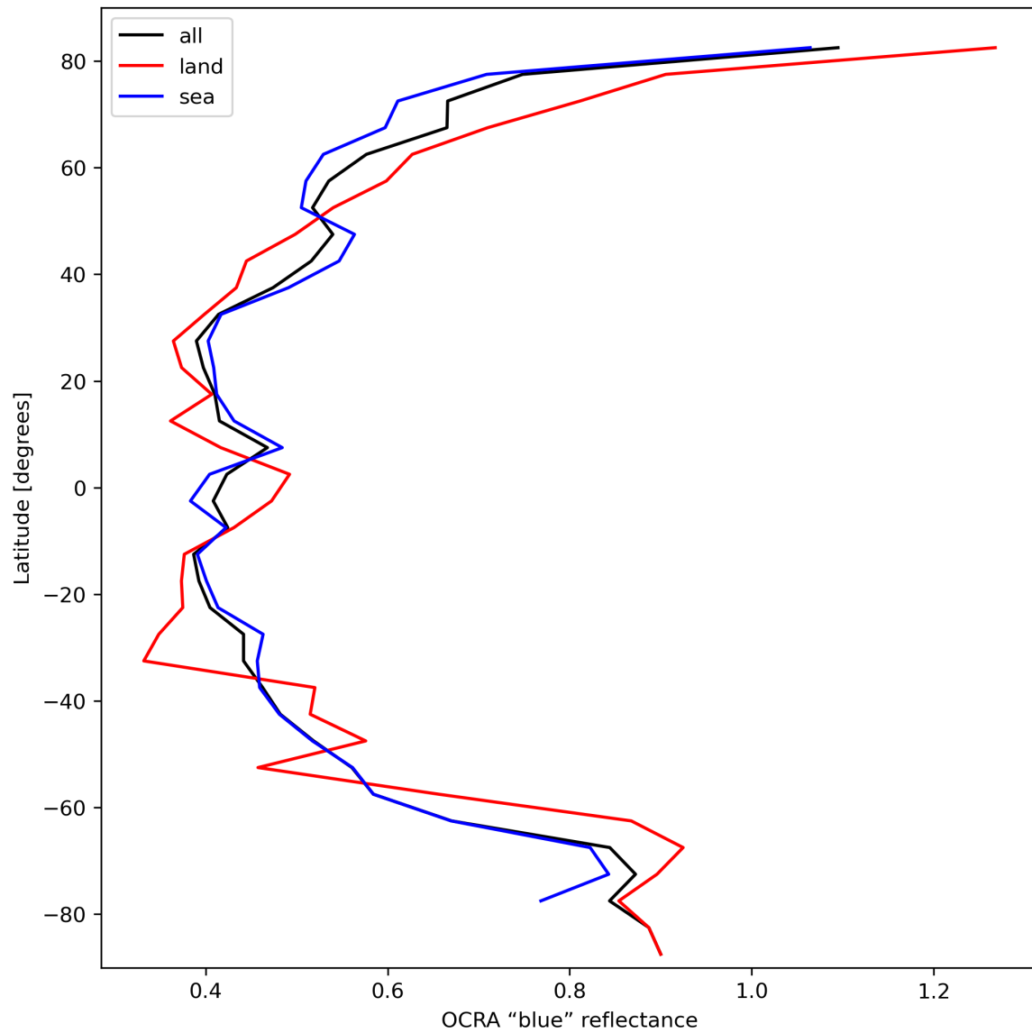
Figure 35: Zonal average of “OCRA “blue” reflectance” for 2023-10-14 to 2023-10-16.
