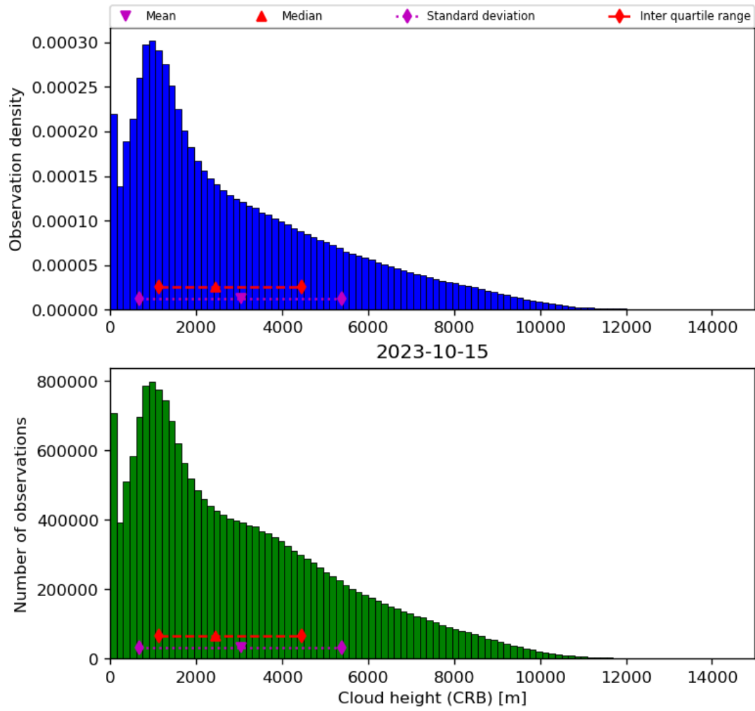
Figure 43: Histogram of “Cloud height (CRB)” for 2023-10-14 to 2023-10-16
