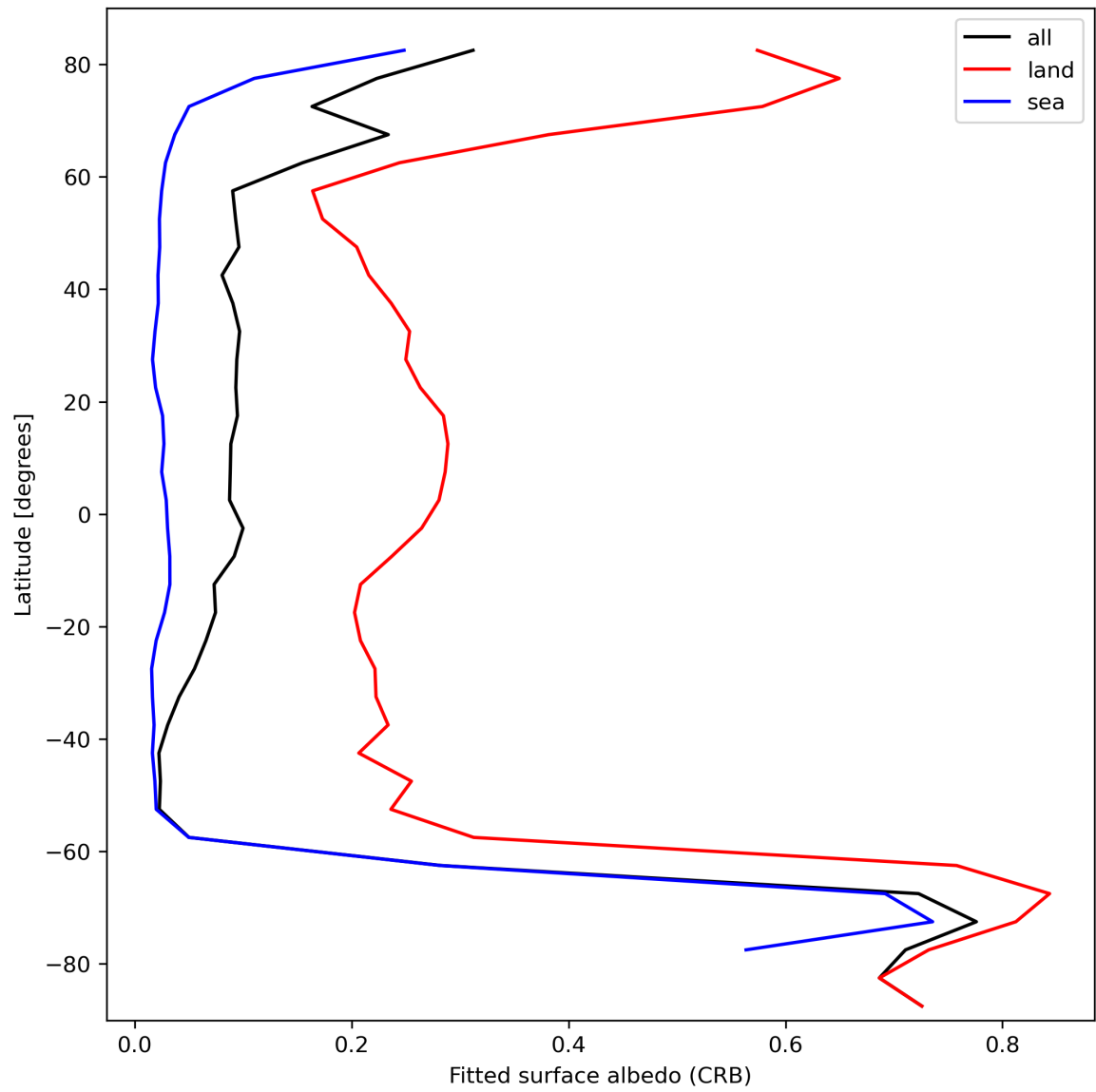
Figure 30: Zonal average of “Fitted surface albedo (CRB)” for 2023-10-14 to 2023-10-16.
