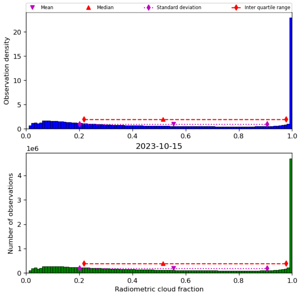
Figure 39: Histogram of “Radiometric cloud fraction” for 2023-10-14 to 2023-10-16
