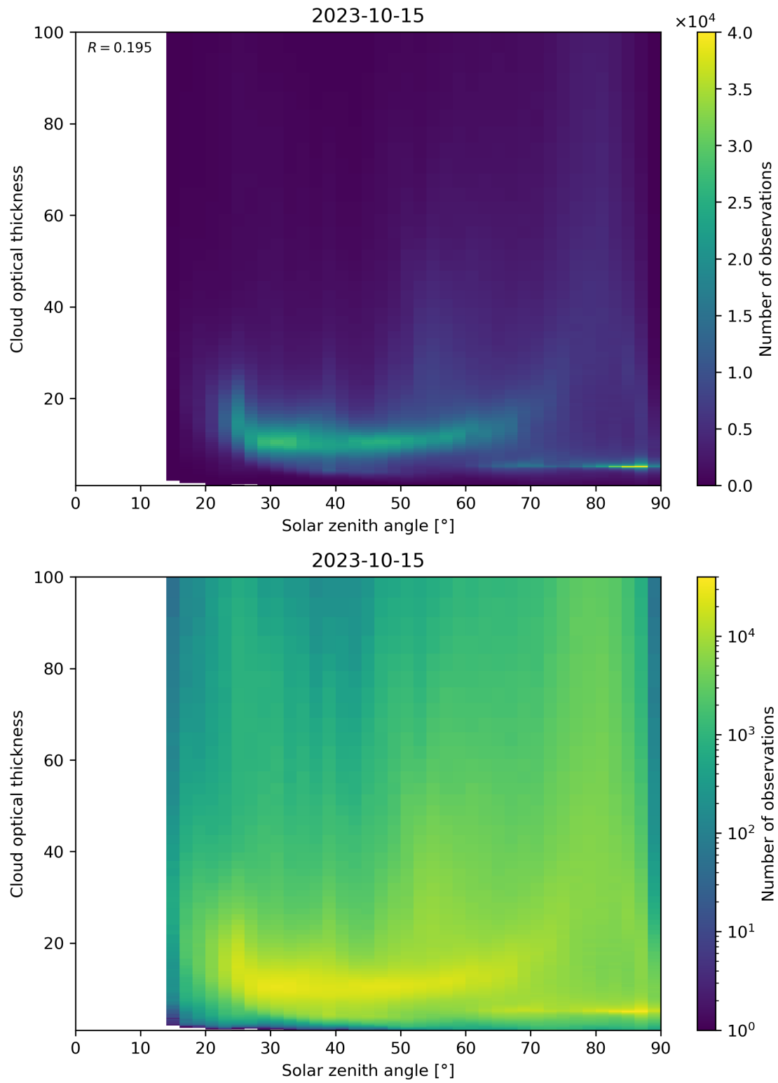
Figure 103: Scatter density plot of “Solar zenith angle” against “Cloud optical thickness” for 2023-10-14 to 2023-10-16.
