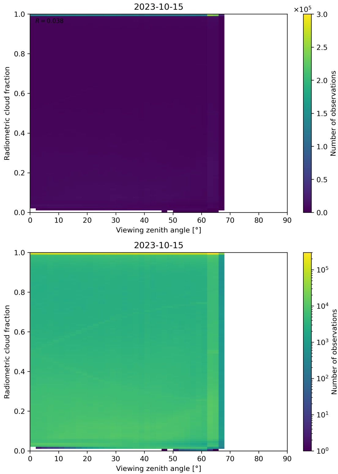
Figure 107: Scatter density plot of “Viewing zenith angle” against “Radiometric cloud fraction” for 2023-10-14 to 2023-10-16.
