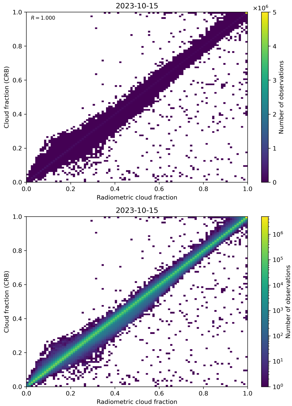
Figure 73: Scatter density plot of “Radiometric cloud fraction” against “Cloud fraction (CRB)” for 2023-10-14 to 2023-10-16.
