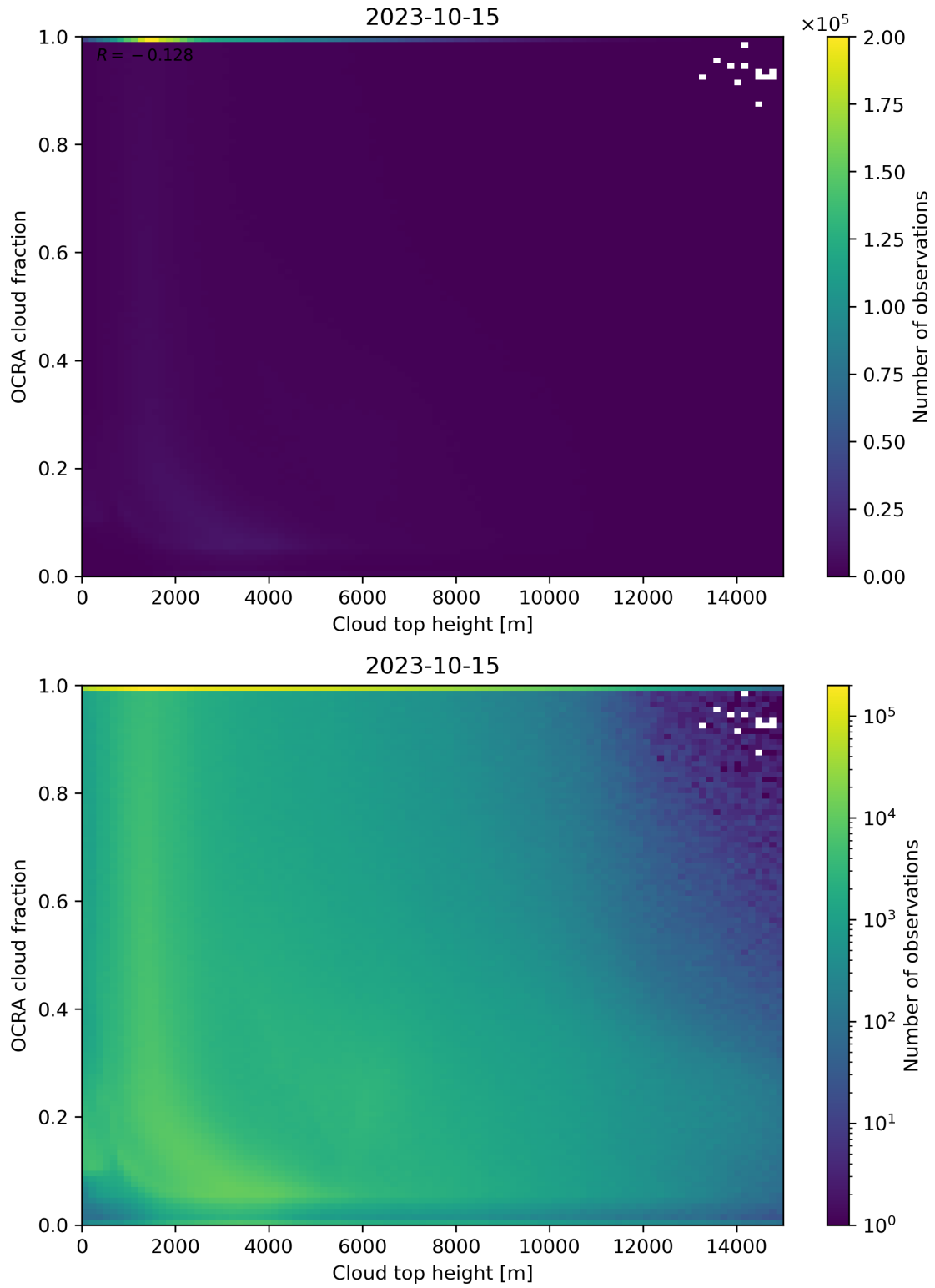
Figure 87: Scatter density plot of “Cloud top height” against “OCRA cloud fraction” for 2023-10-14 to 2023-10-16.
