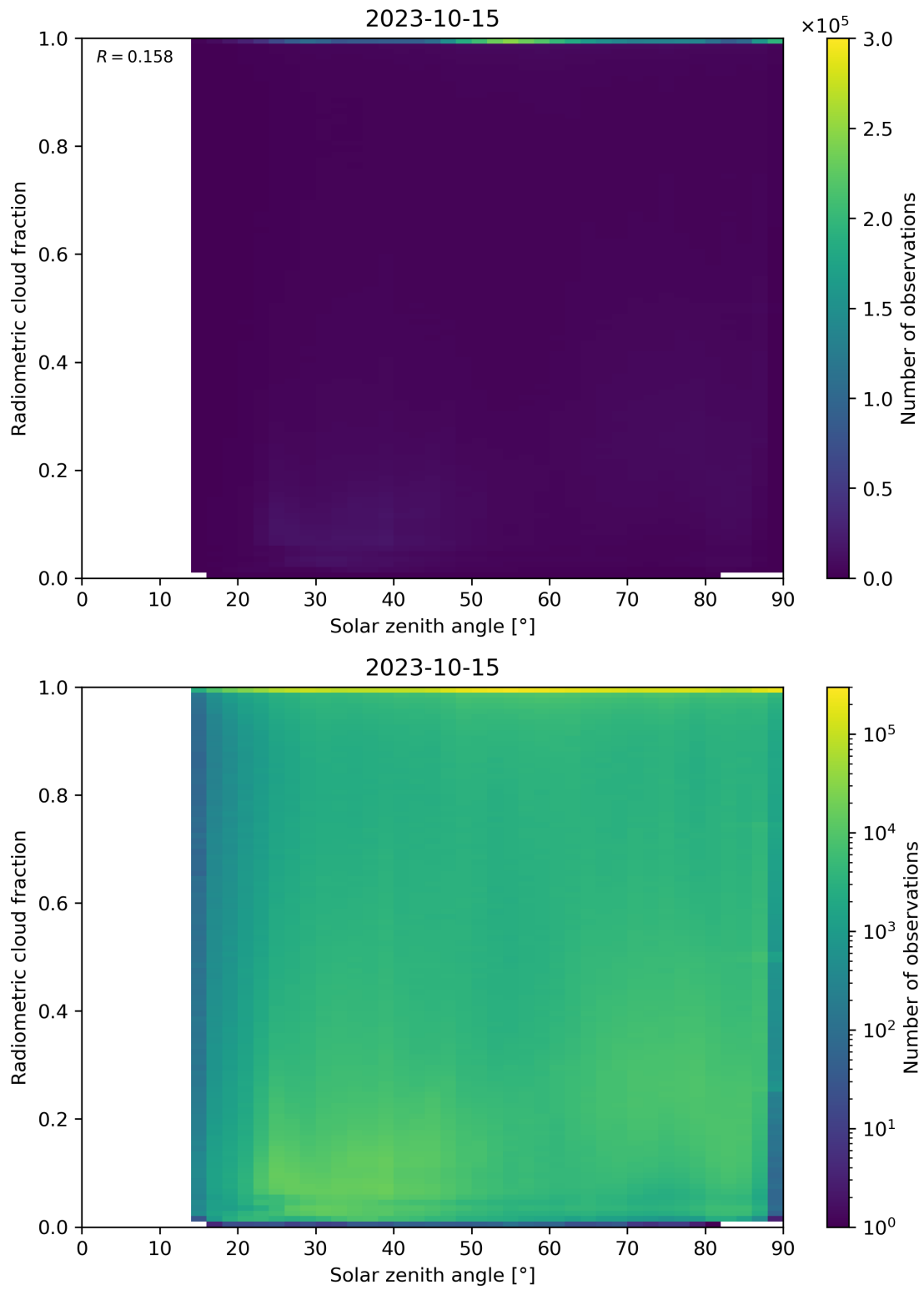
Figure 99: Scatter density plot of “Solar zenith angle” against “Radiometric cloud fraction” for 2023-10-14 to 2023-10-16.
