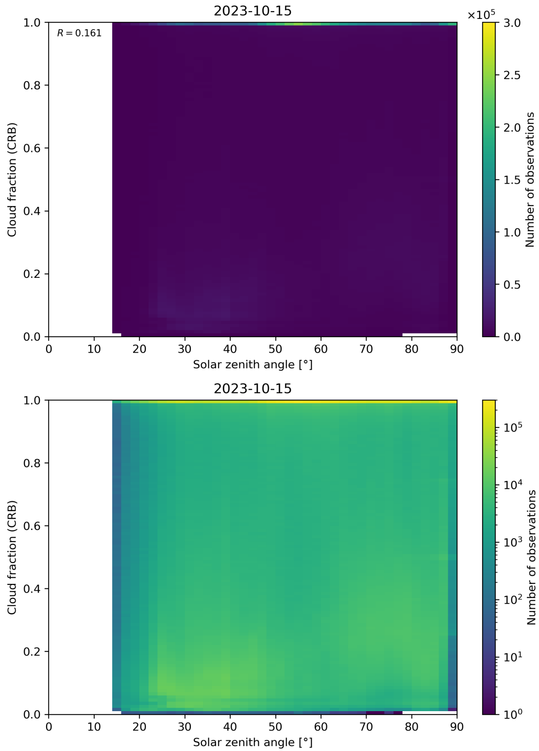
Figure 101: Scatter density plot of “Solar zenith angle” against “Cloud fraction (CRB)” for 2023-10-14 to 2023-10-16.
