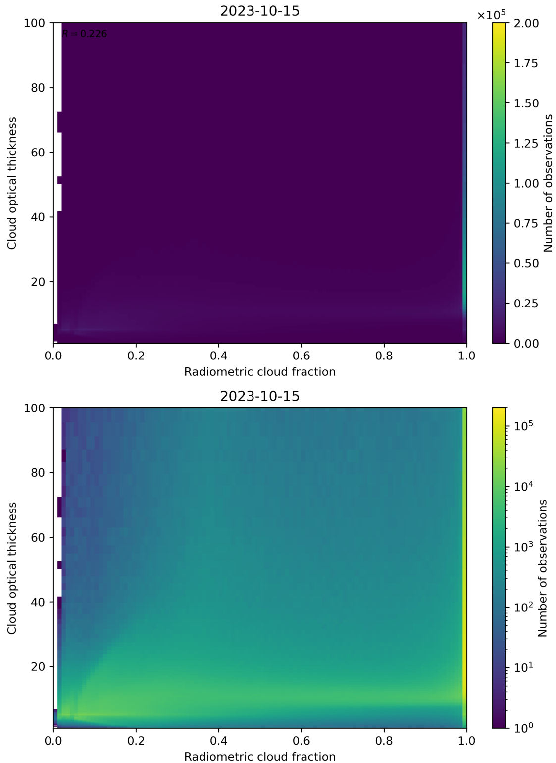
Figure 75: Scatter density plot of “Radiometric cloud fraction” against “Cloud optical thickness” for 2023-10-14 to 2023-10-16.
