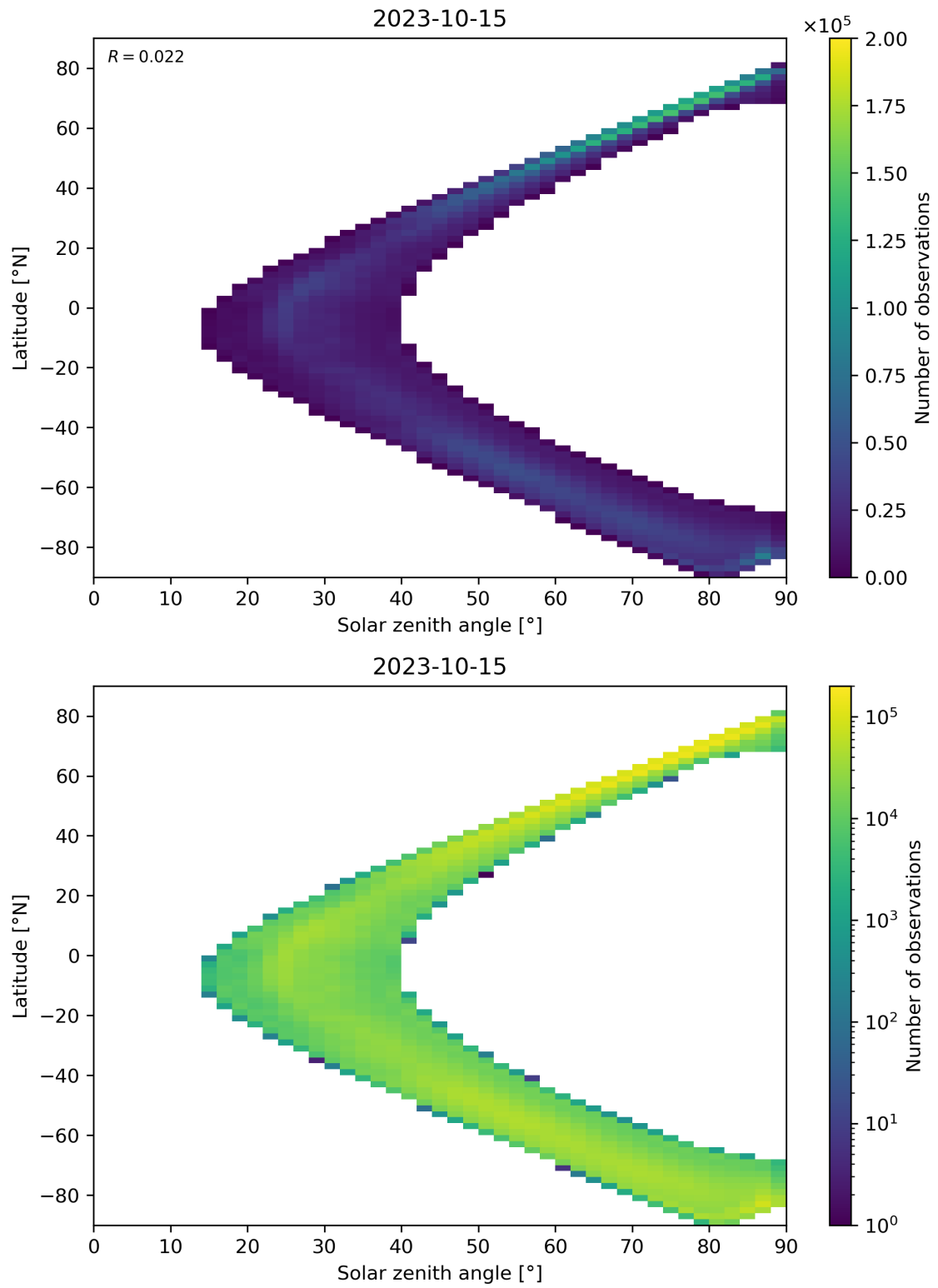
Figure 105: Scatter density plot of “Solar zenith angle” against “Latitude” for 2023-10-14 to 2023-10-16.
