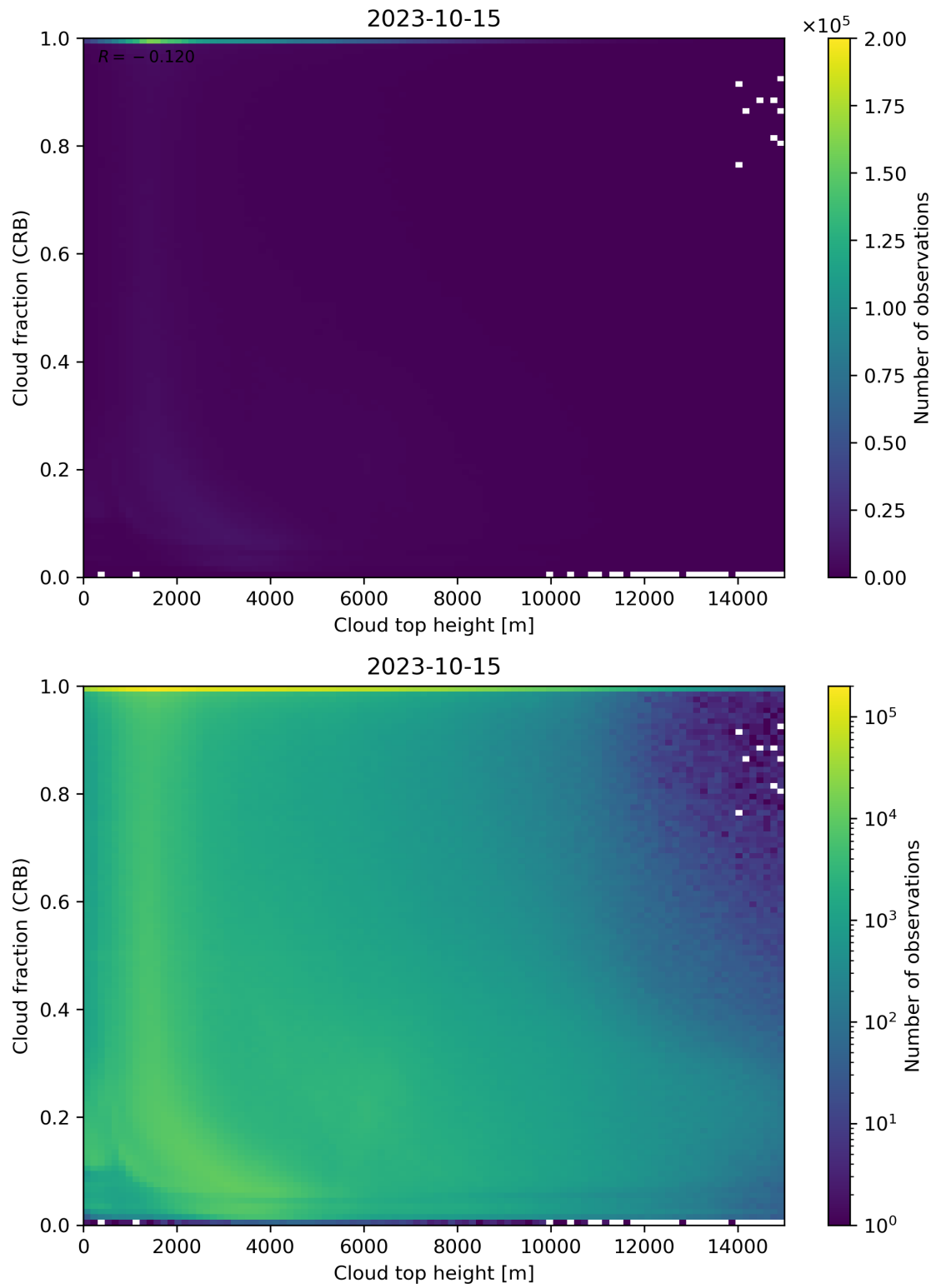
Figure 88: Scatter density plot of “Cloud top height” against “Cloud fraction (CRB)” for 2023-10-14 to 2023-10-16.
