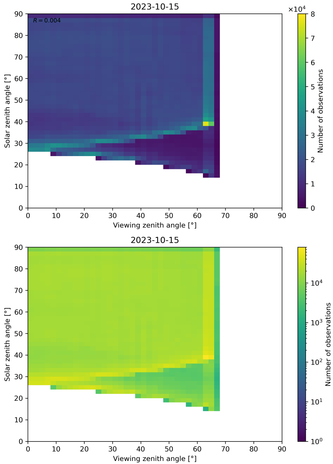
Figure 114: Scatter density plot of “Viewing zenith angle” against “Solar zenith angle” for 2023-10-14 to 2023-10-16.
