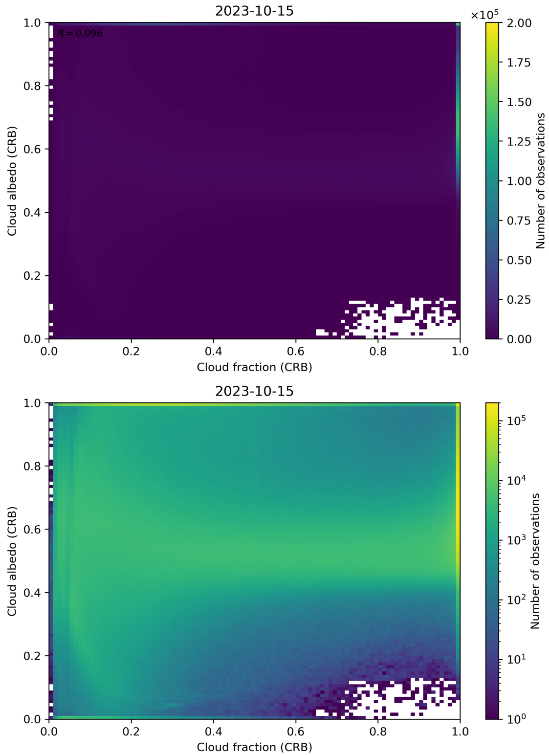
Figure 77: Scatter density plot of “Cloud fraction (CRB)” against “Cloud albedo (CRB)” for 2023-10-14 to 2023-10-16.
