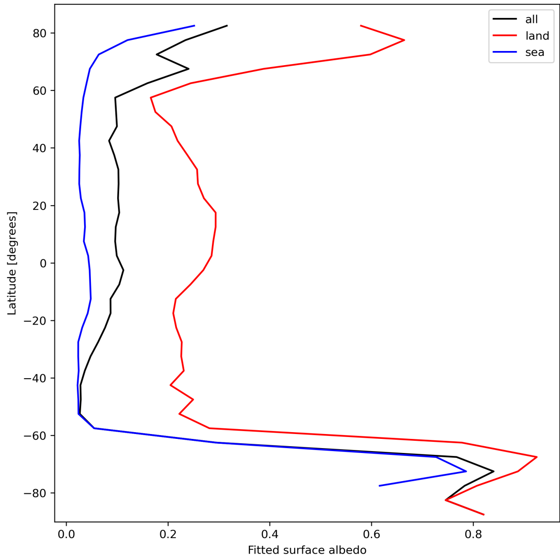
Figure 29: Zonal average of “Fitted surface albedo” for 2023-10-14 to 2023-10-16.
