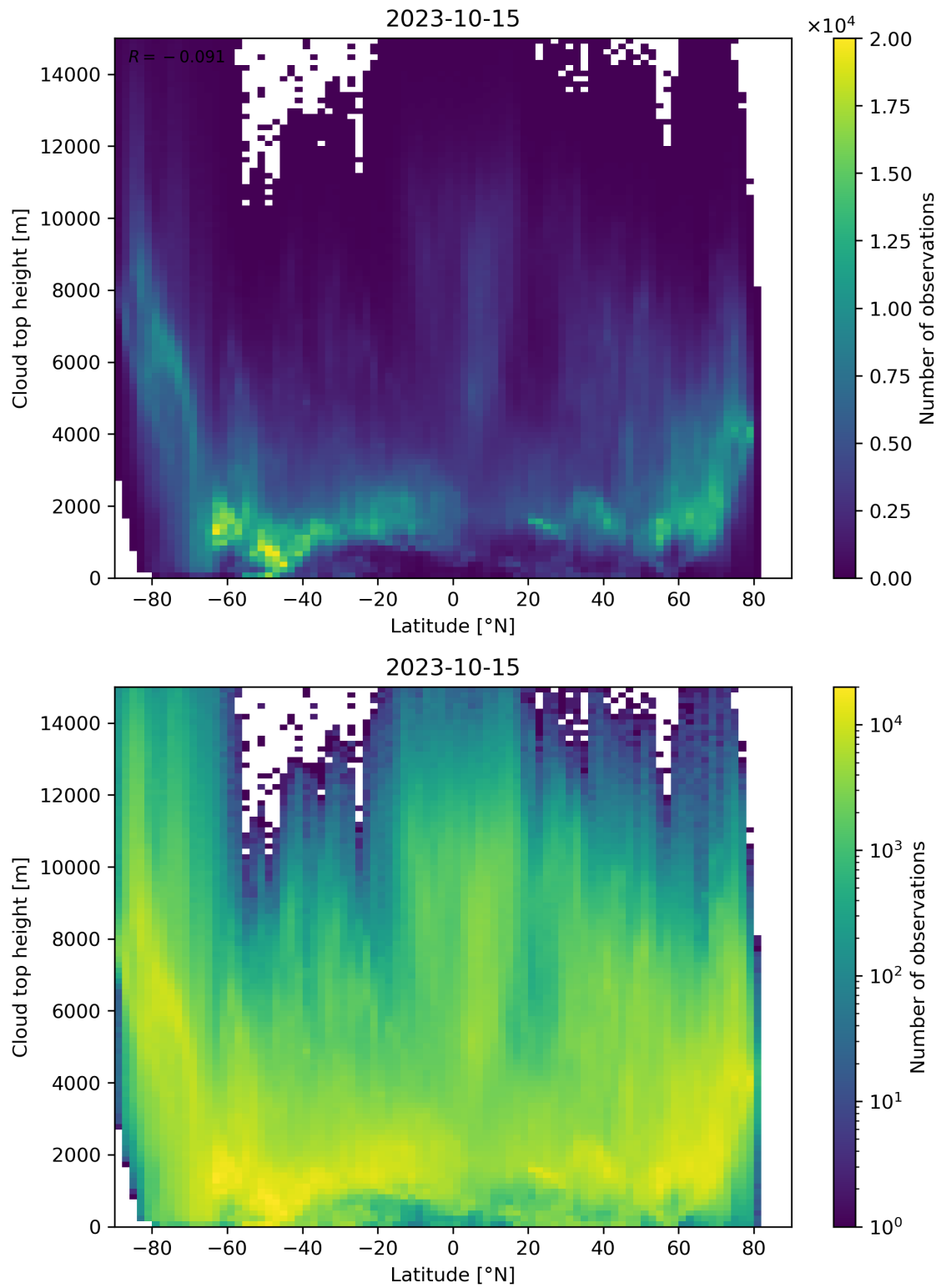
Figure 97: Scatter density plot of “Latitude” against “Cloud top height” for 2023-10-14 to 2023-10-16.
