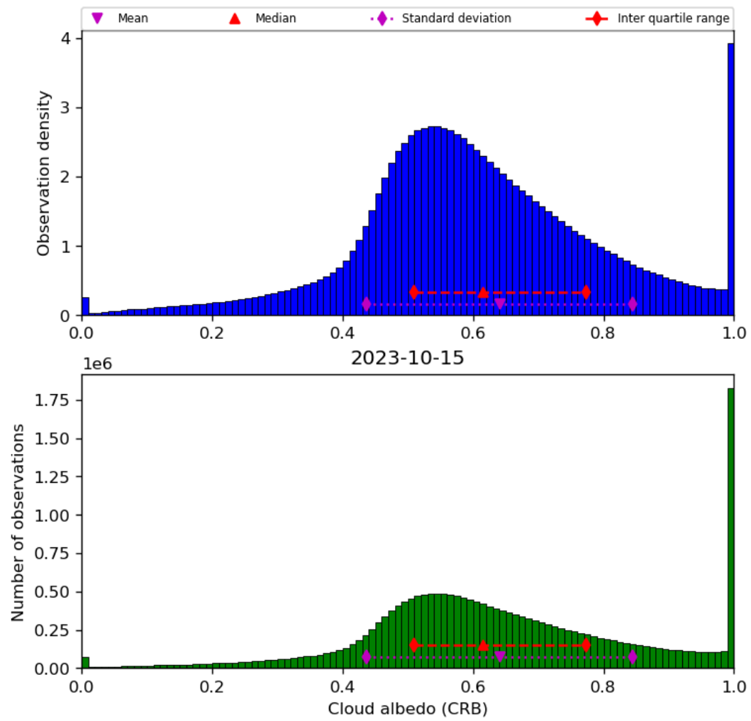
Figure 44: Histogram of “Cloud albedo (CRB)” for 2023-10-14 to 2023-10-16
