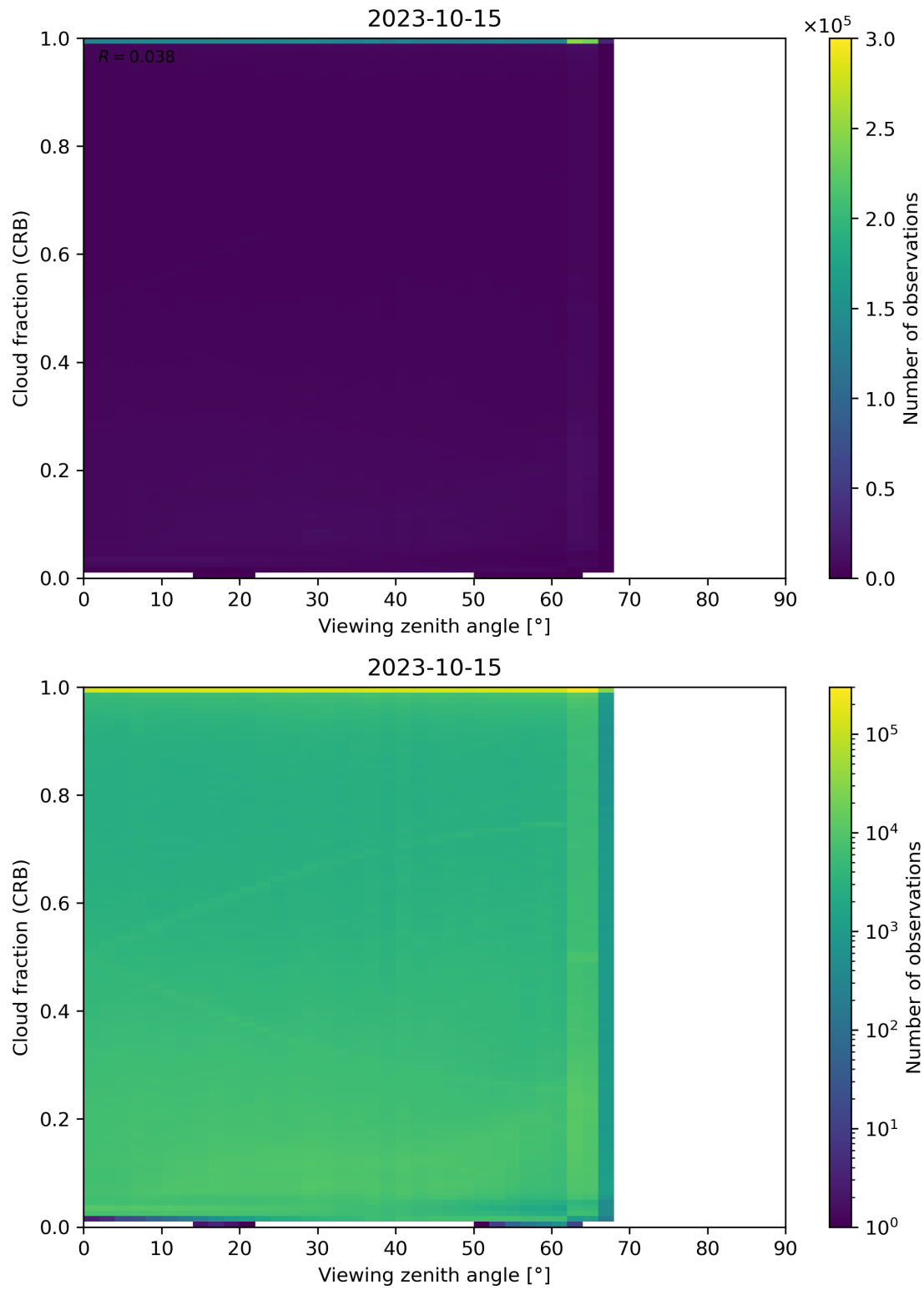
Figure 109: Scatter density plot of “Viewing zenith angle” against “Cloud fraction (CRB)” for 2023-10-14 to 2023-10-16.
