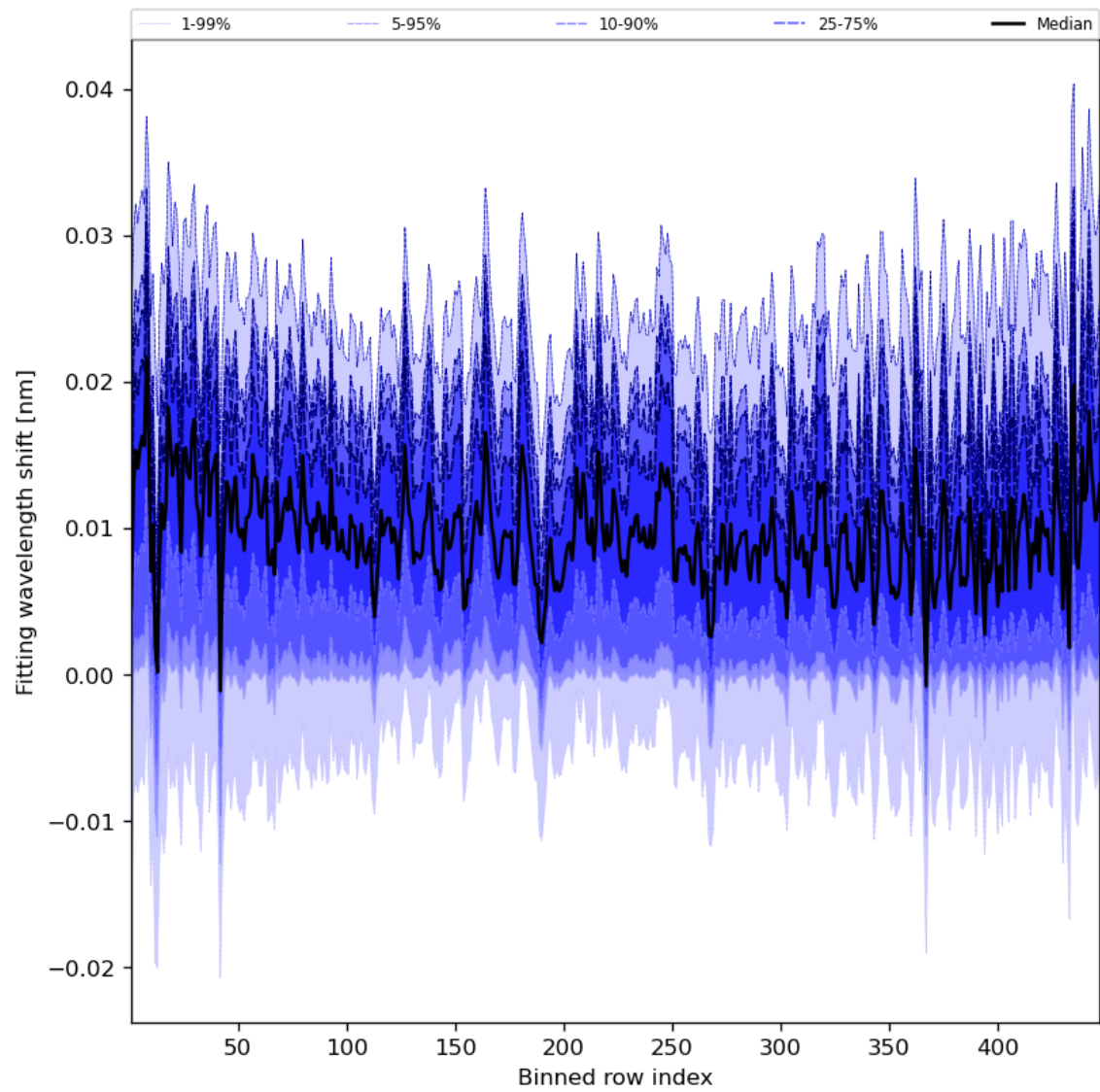
Figure 65: Along track statistics of “Fitting wavelength shift” for 2023-10-14 to 2023-10-16
