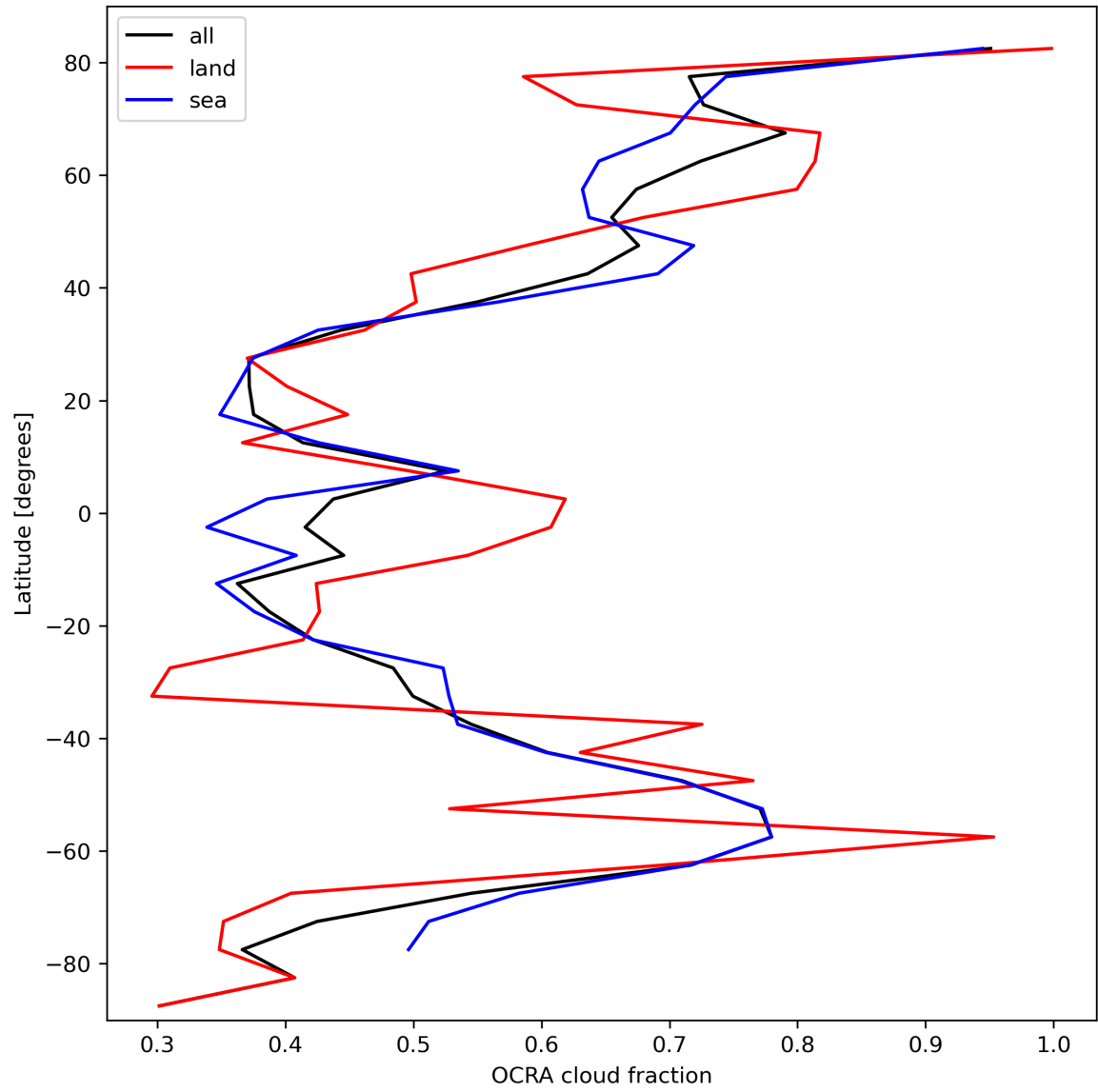
Figure 34: Zonal average of “OCRA cloud fraction” for 2023-10-14 to 2023-10-16.
