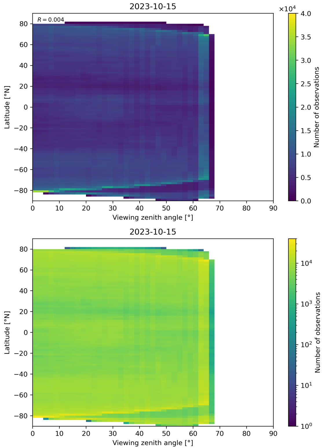
Figure 113: Scatter density plot of “Viewing zenith angle” against “Latitude” for 2023-10-14 to 2023-10-16.
