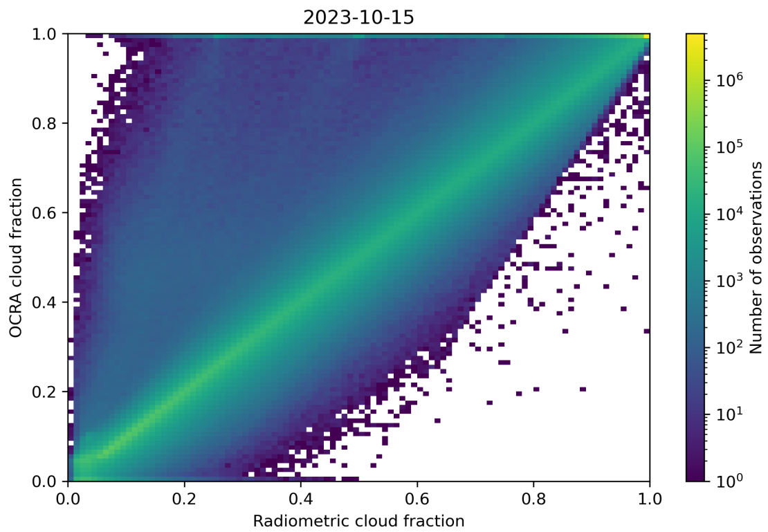
Figure 72: Scatter density plot of “Radiometric cloud fraction” against “OCRA cloud fraction” for 2023-10-14 to 2023-10-16.
