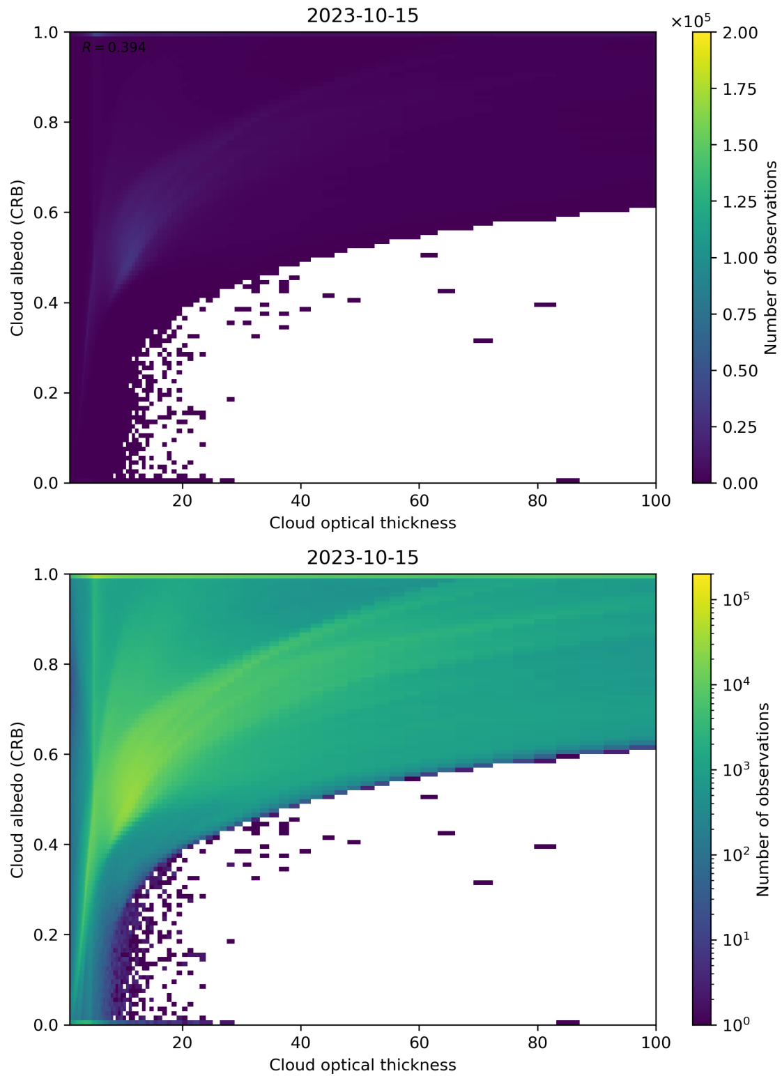
Figure 82: Scatter density plot of “Cloud optical thickness” against “Cloud albedo (CRB)” for 2023-10-14 to 2023-10-16.
