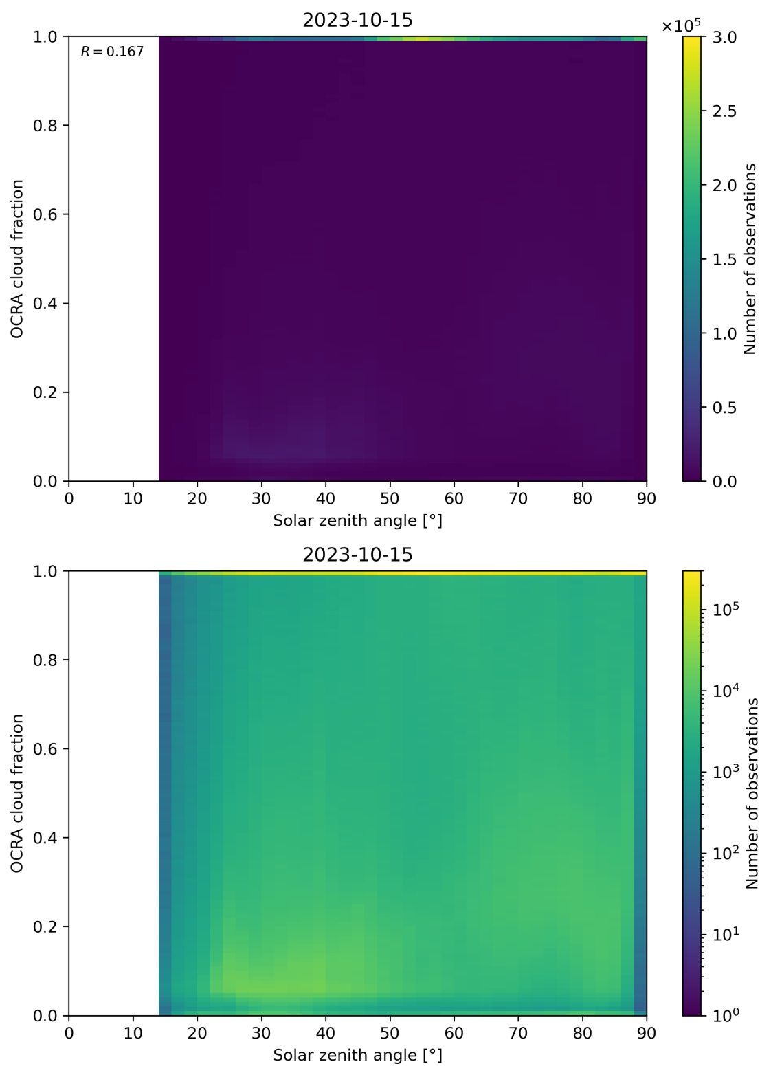
Figure 100: Scatter density plot of “Solar zenith angle” against “OCRA cloud fraction” for 2023-10-14 to 2023-10-16.
