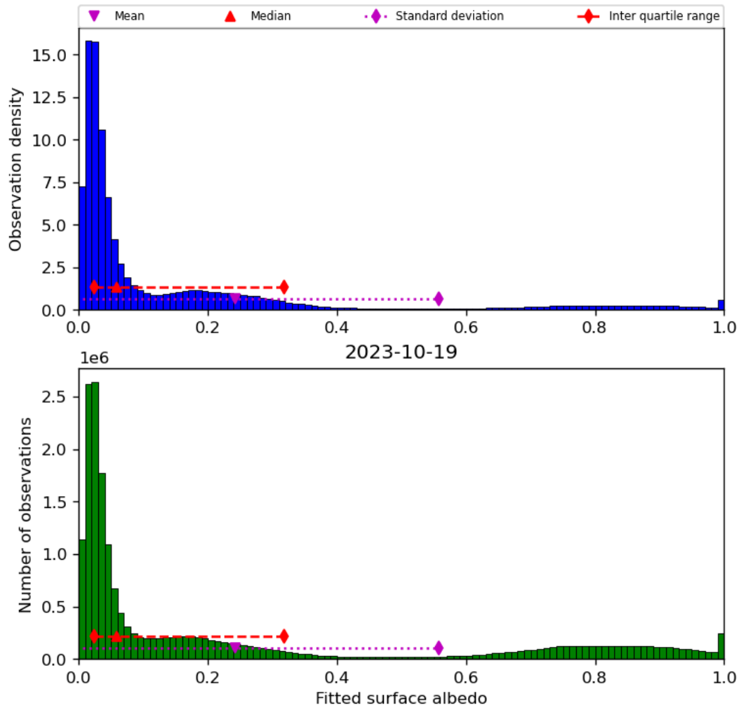
Figure 45: Histogram of “Fitted surface albedo” for 2023-10-18 to 2023-10-20
