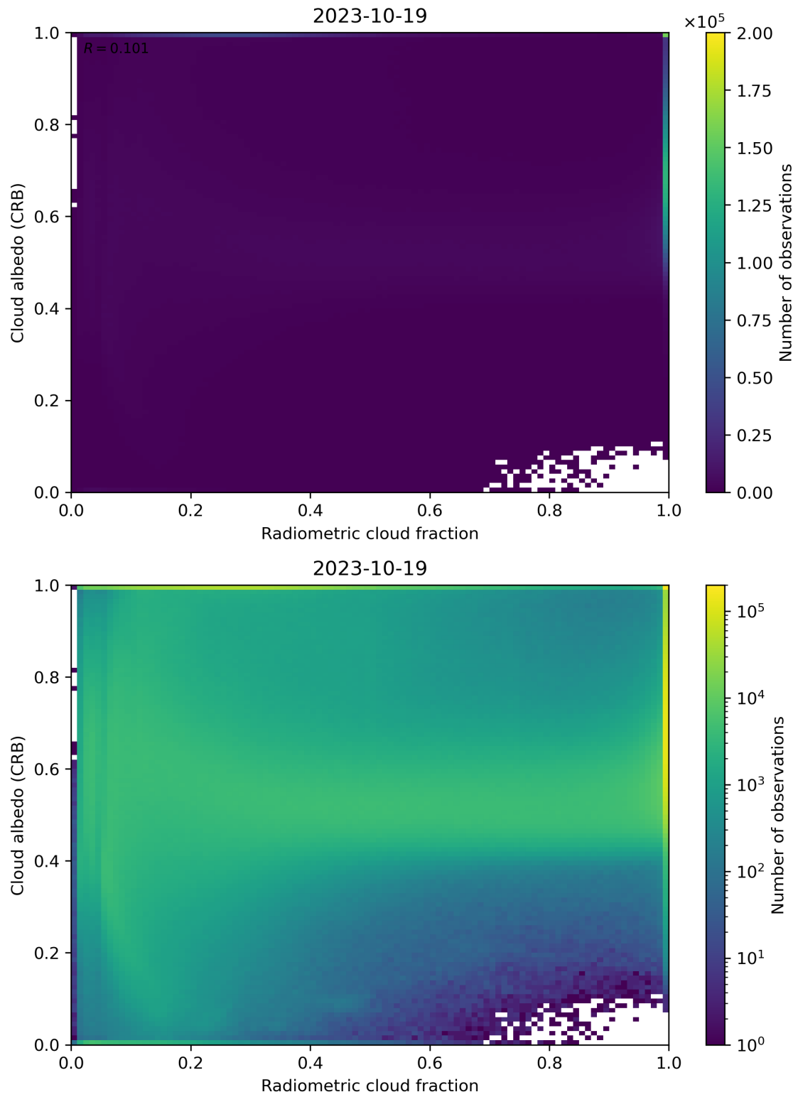
Figure 71: Scatter density plot of “Radiometric cloud fraction” against “Cloud albedo (CRB)” for 2023-10-18 to 2023-10-20.
