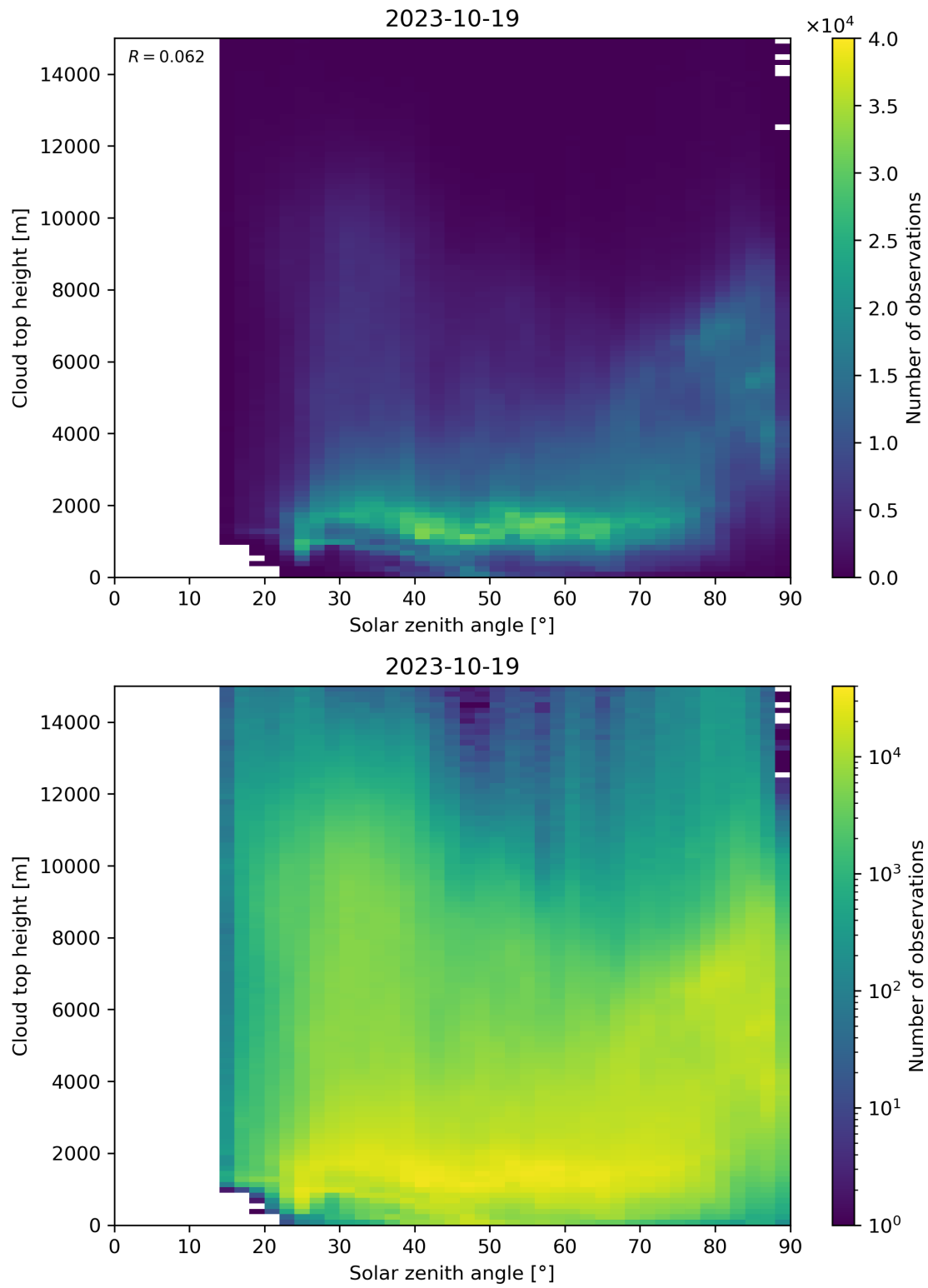
Figure 104: Scatter density plot of “Solar zenith angle” against “Cloud top height” for 2023-10-18 to 2023-10-20.
