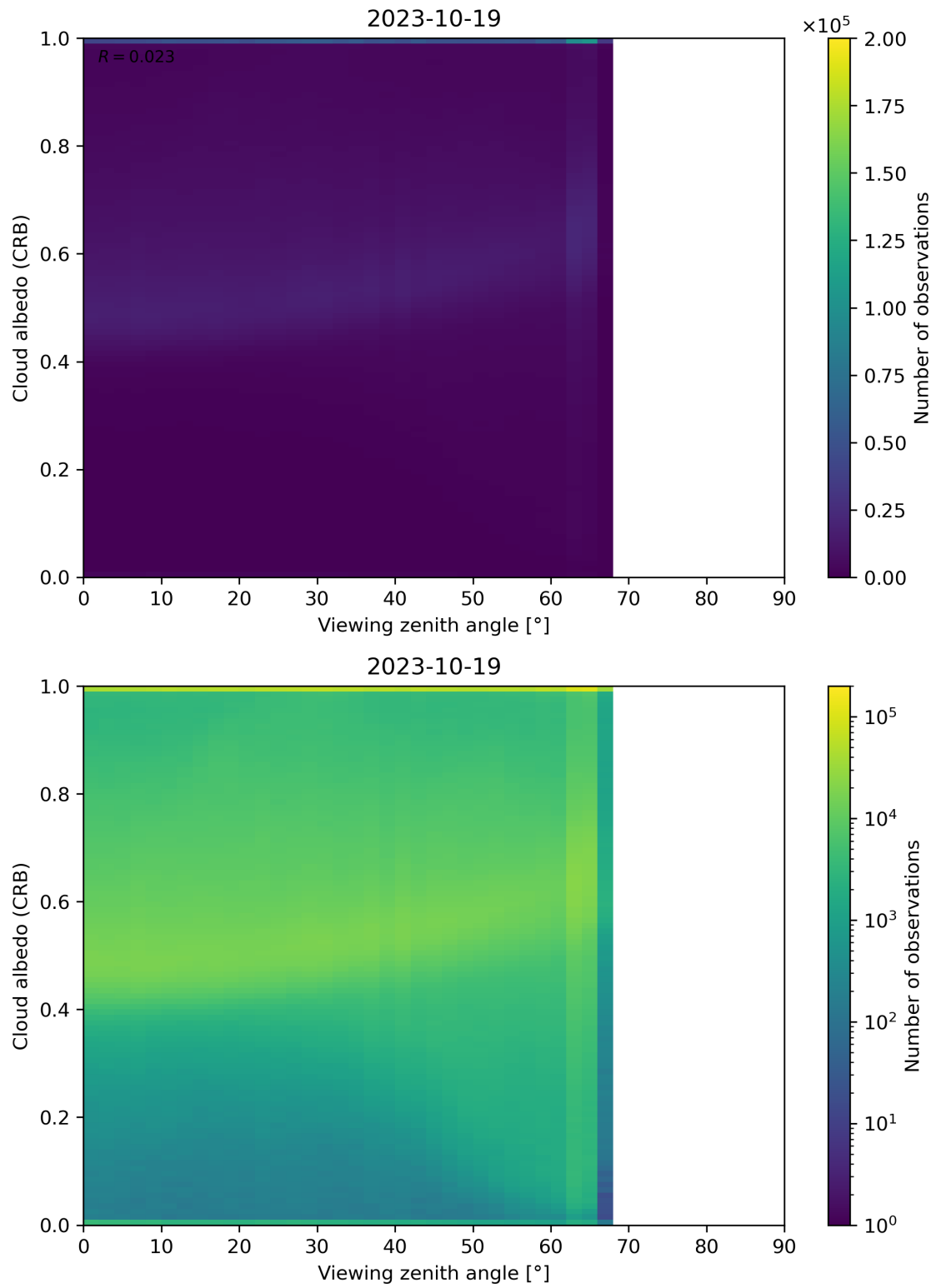
Figure 106: Scatter density plot of “Viewing zenith angle” against “Cloud albedo (CRB)” for 2023-10-18 to 2023-10-20.
