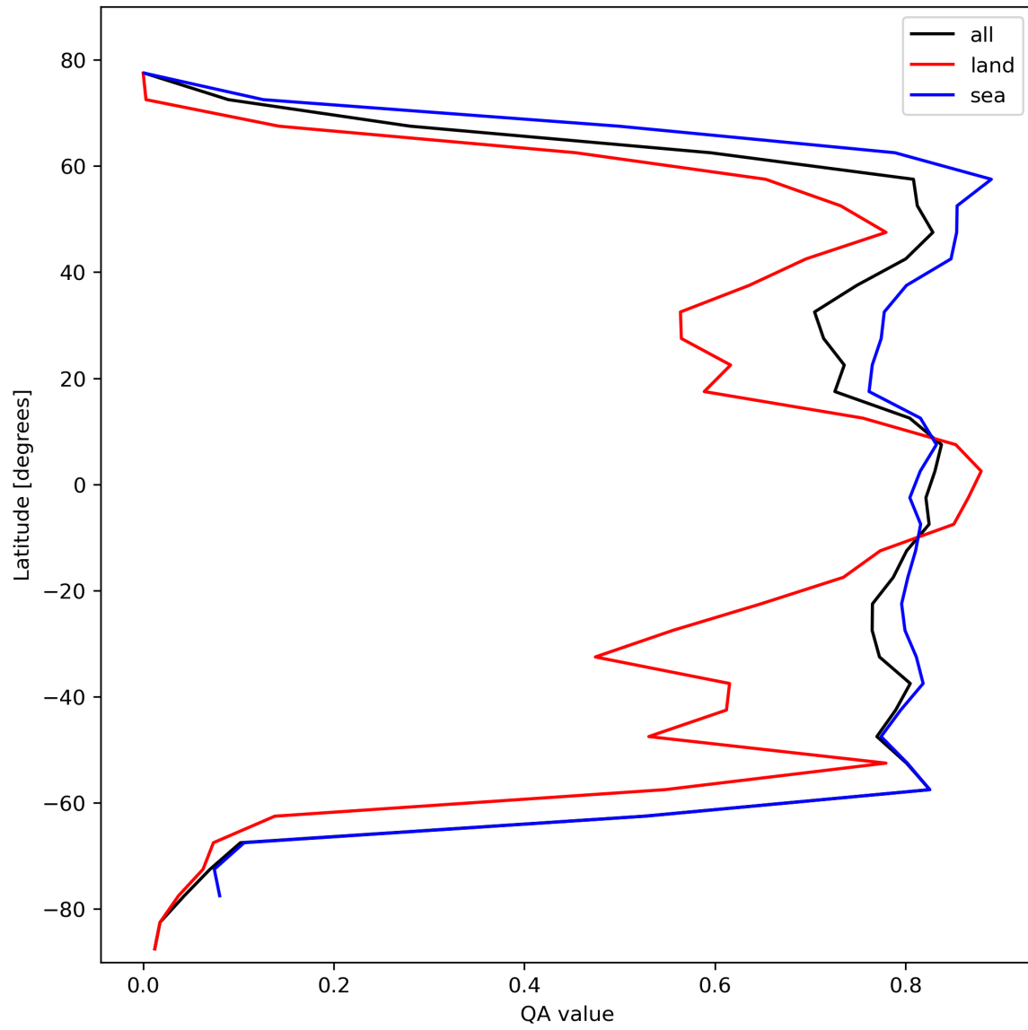
Figure 22: Zonal average of “QA value” for 2023-10-18 to 2023-10-20.
