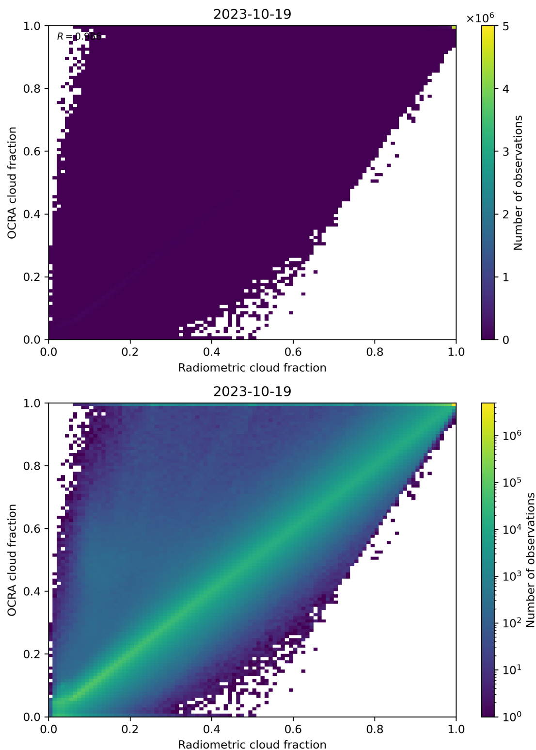
Figure 72: Scatter density plot of “Radiometric cloud fraction” against “OCRA cloud fraction” for 2023-10-18 to 2023-10-20.
