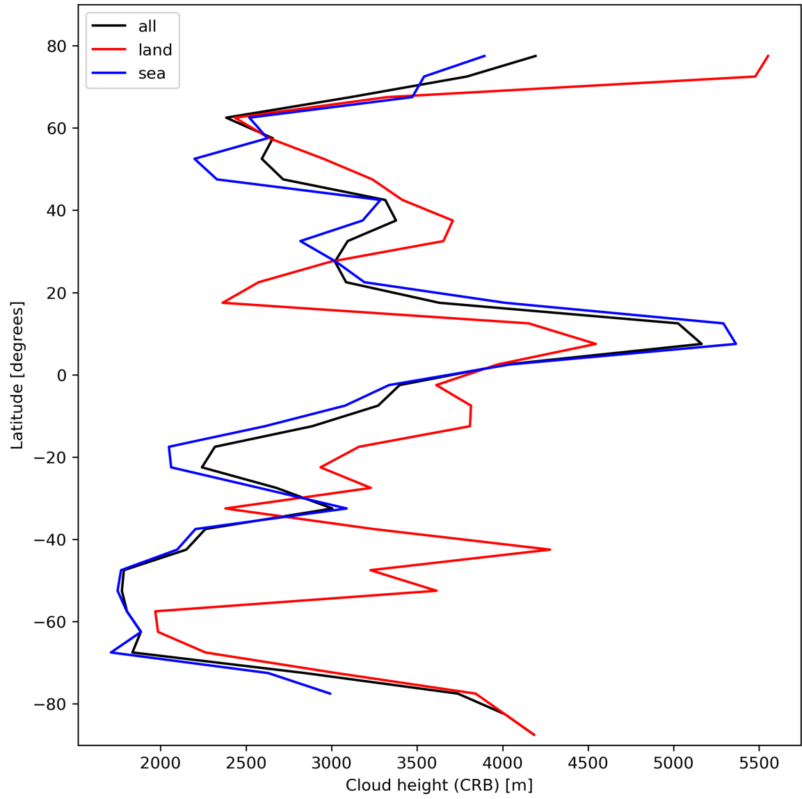
Figure 27: Zonal average of “Cloud height (CRB)” for 2023-10-18 to 2023-10-20.
