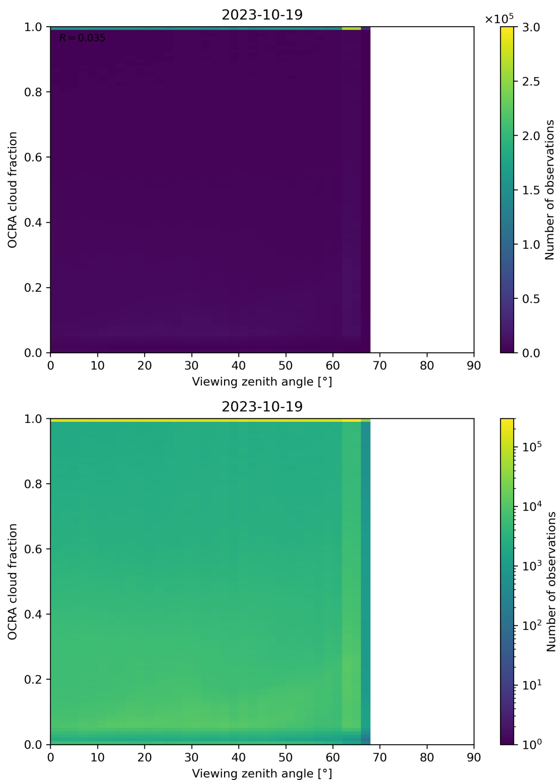
Figure 108: Scatter density plot of “Viewing zenith angle” against “OCRA cloud fraction” for 2023-10-18 to 2023-10-20.
