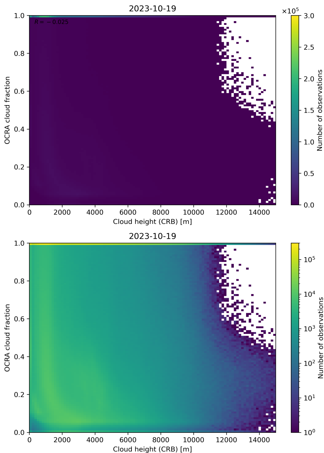
Figure 81: Scatter density plot of “Cloud height (CRB)” against “OCRA cloud fraction” for 2023-10-18 to 2023-10-20.
