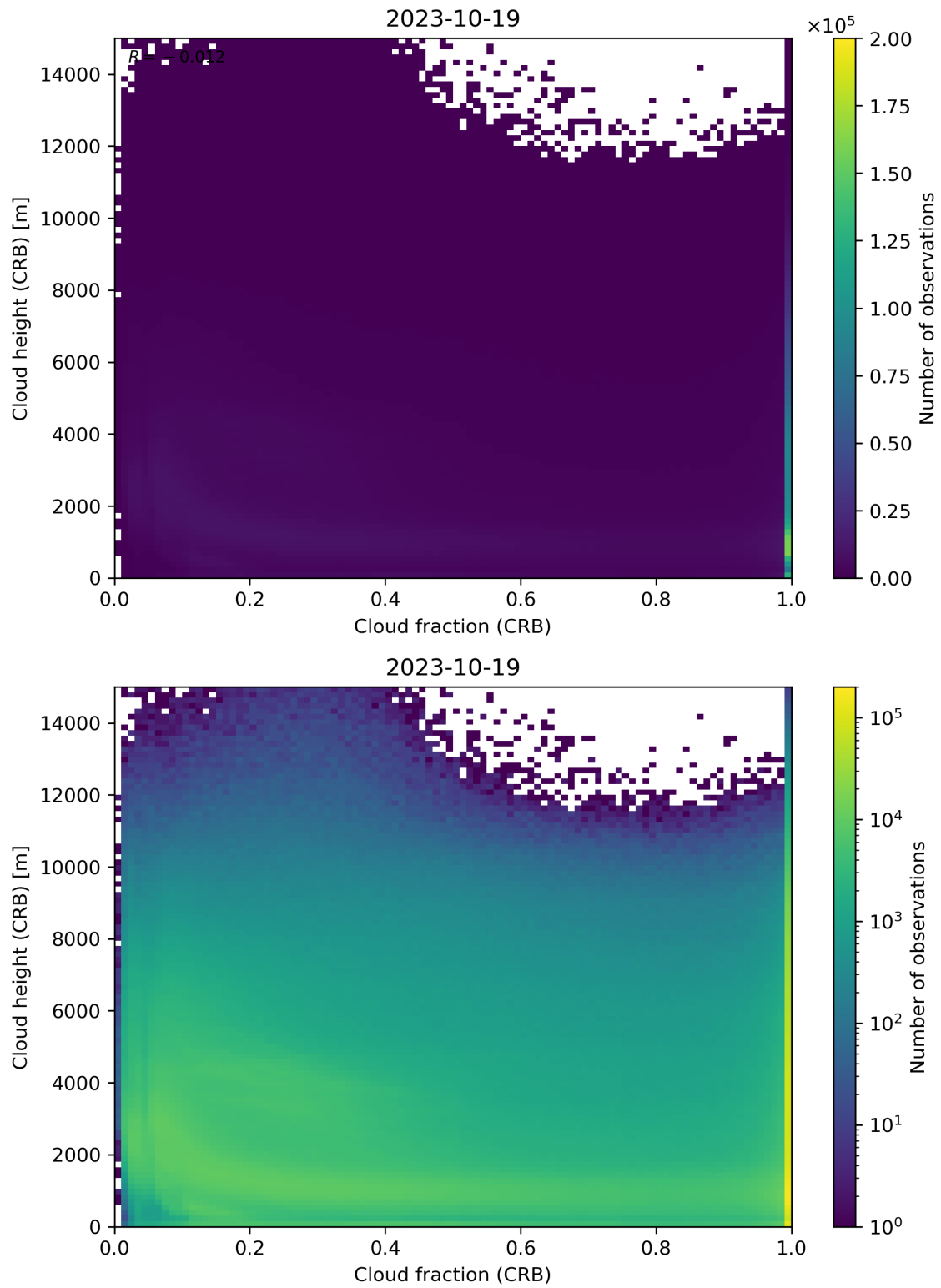
Figure 79: Scatter density plot of “Cloud fraction (CRB)” against “Cloud height (CRB)” for 2023-10-18 to 2023-10-20.
