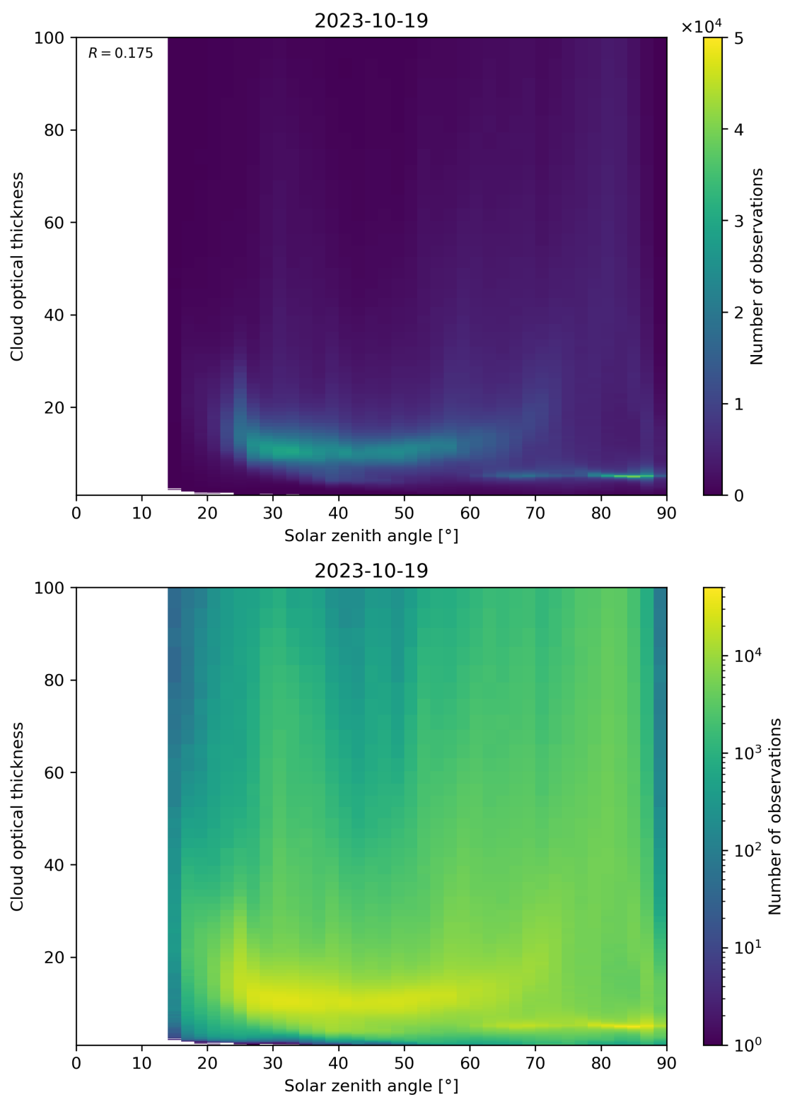
Figure 103: Scatter density plot of “Solar zenith angle” against “Cloud optical thickness” for 2023-10-18 to 2023-10-20.
