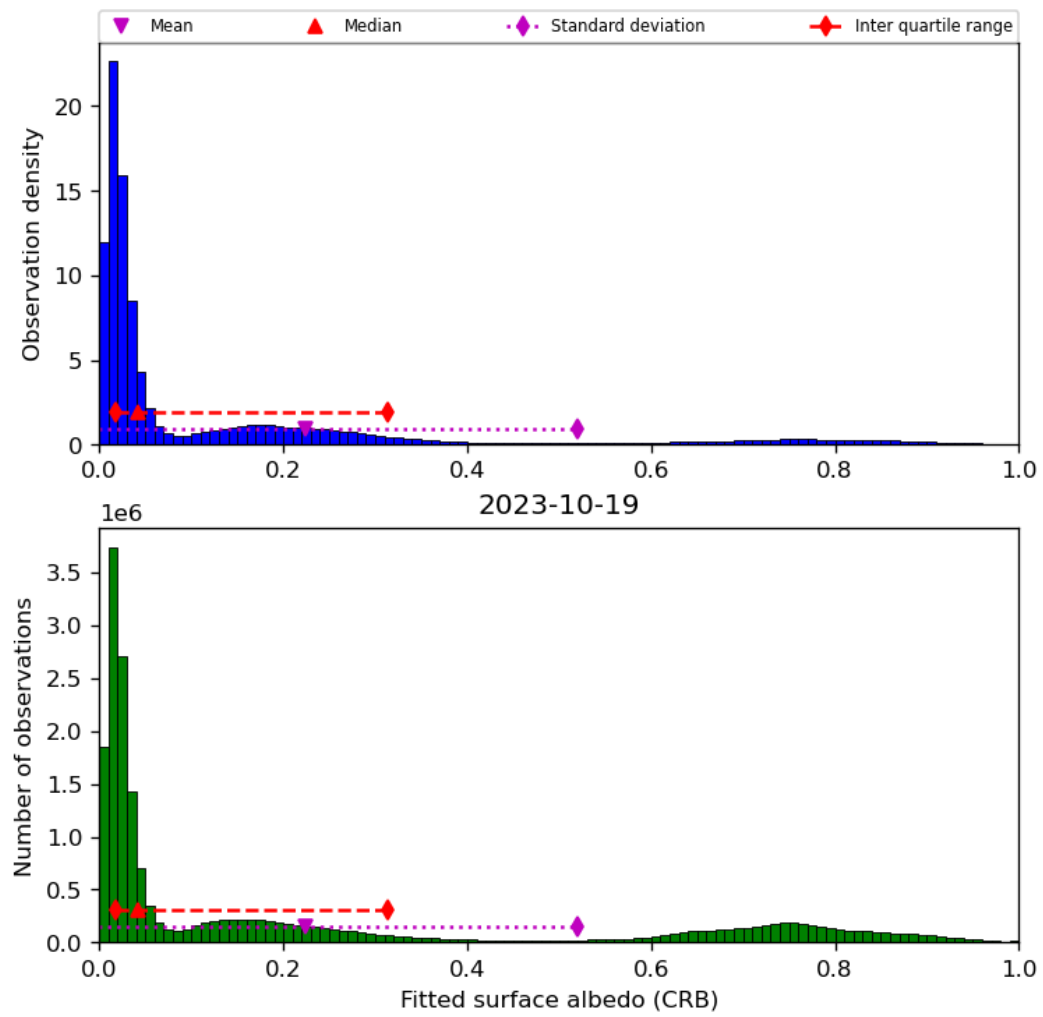
Figure 46: Histogram of “Fitted surface albedo (CRB)” for 2023-10-18 to 2023-10-20
