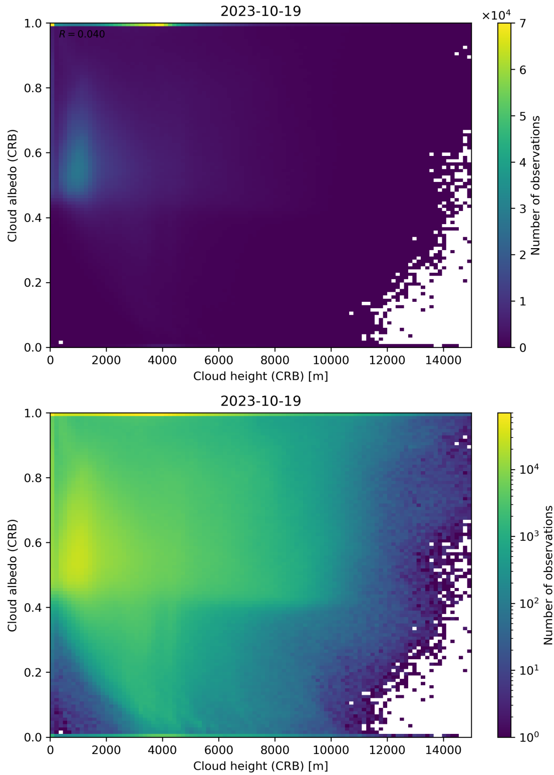
Figure 80: Scatter density plot of “Cloud height (CRB)” against “Cloud albedo (CRB)” for 2023-10-18 to 2023-10-20.
