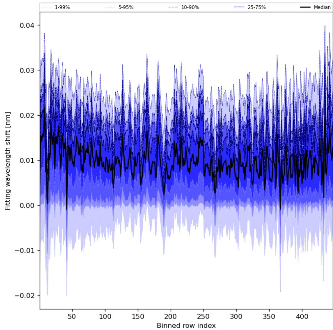
Figure 65: Along track statistics of “Fitting wavelength shift” for 2023-10-18 to 2023-10-20
