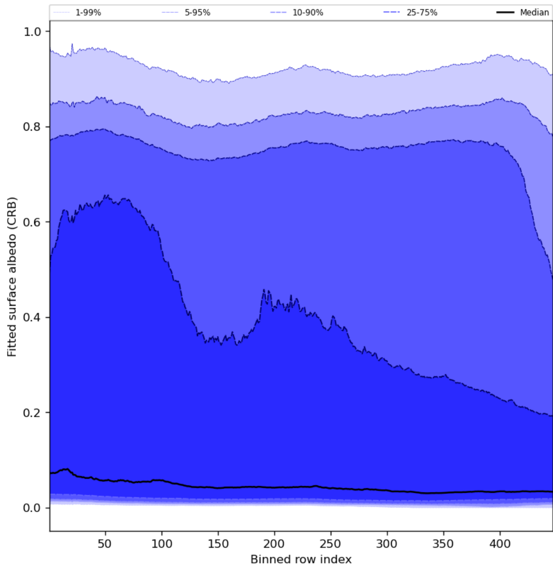
Figure 62: Along track statistics of “Fitted surface albedo (CRB)” for 2023-10-18 to 2023-10-20
