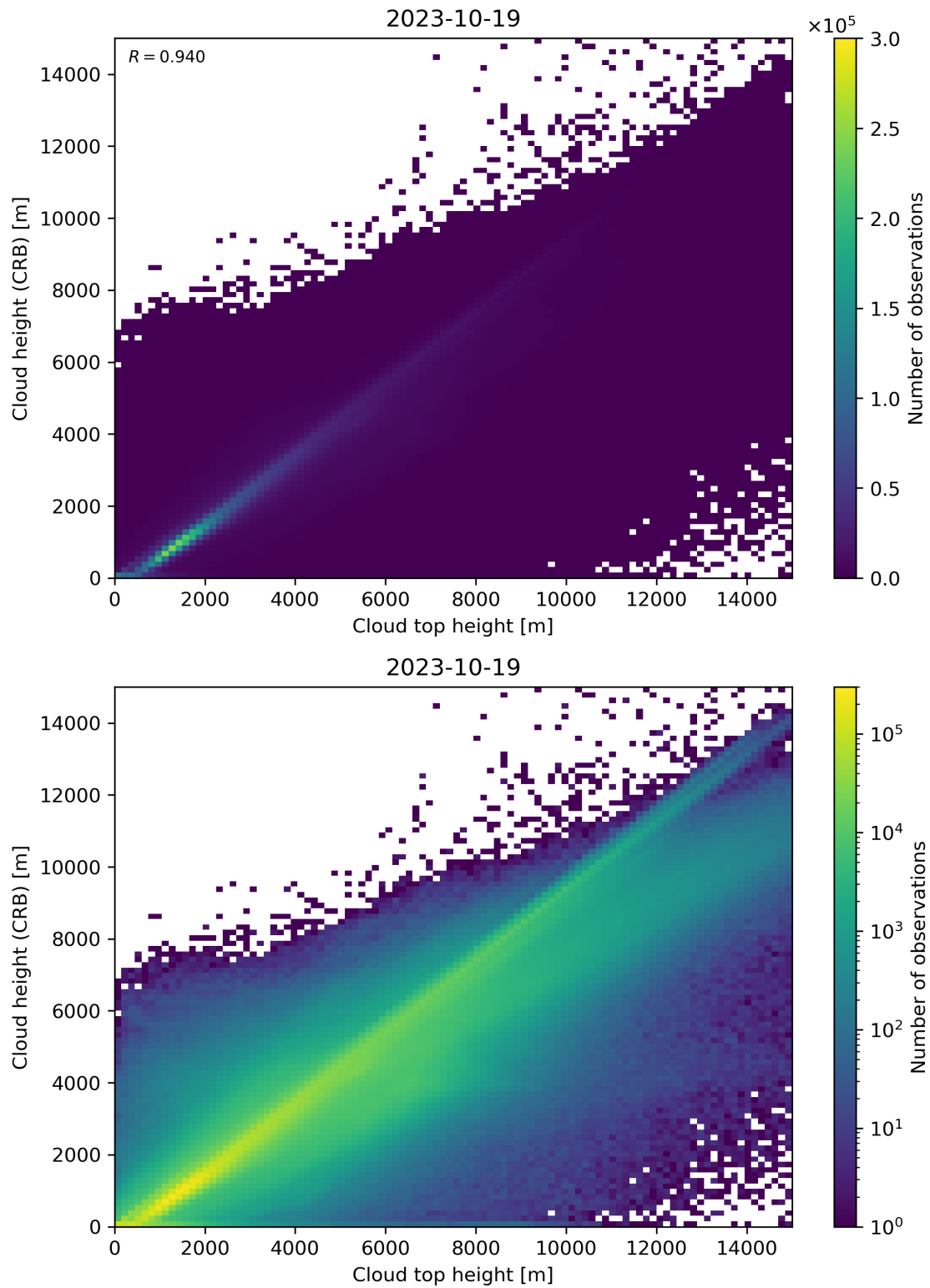
Figure 89: Scatter density plot of “Cloud top height” against “Cloud height (CRB)” for 2023-10-18 to 2023-10-20.
