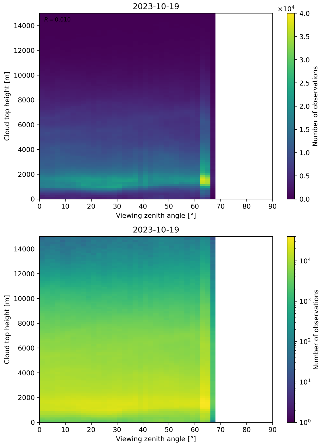
Figure 112: Scatter density plot of “Viewing zenith angle” against “Cloud top height” for 2023-10-18 to 2023-10-20.
