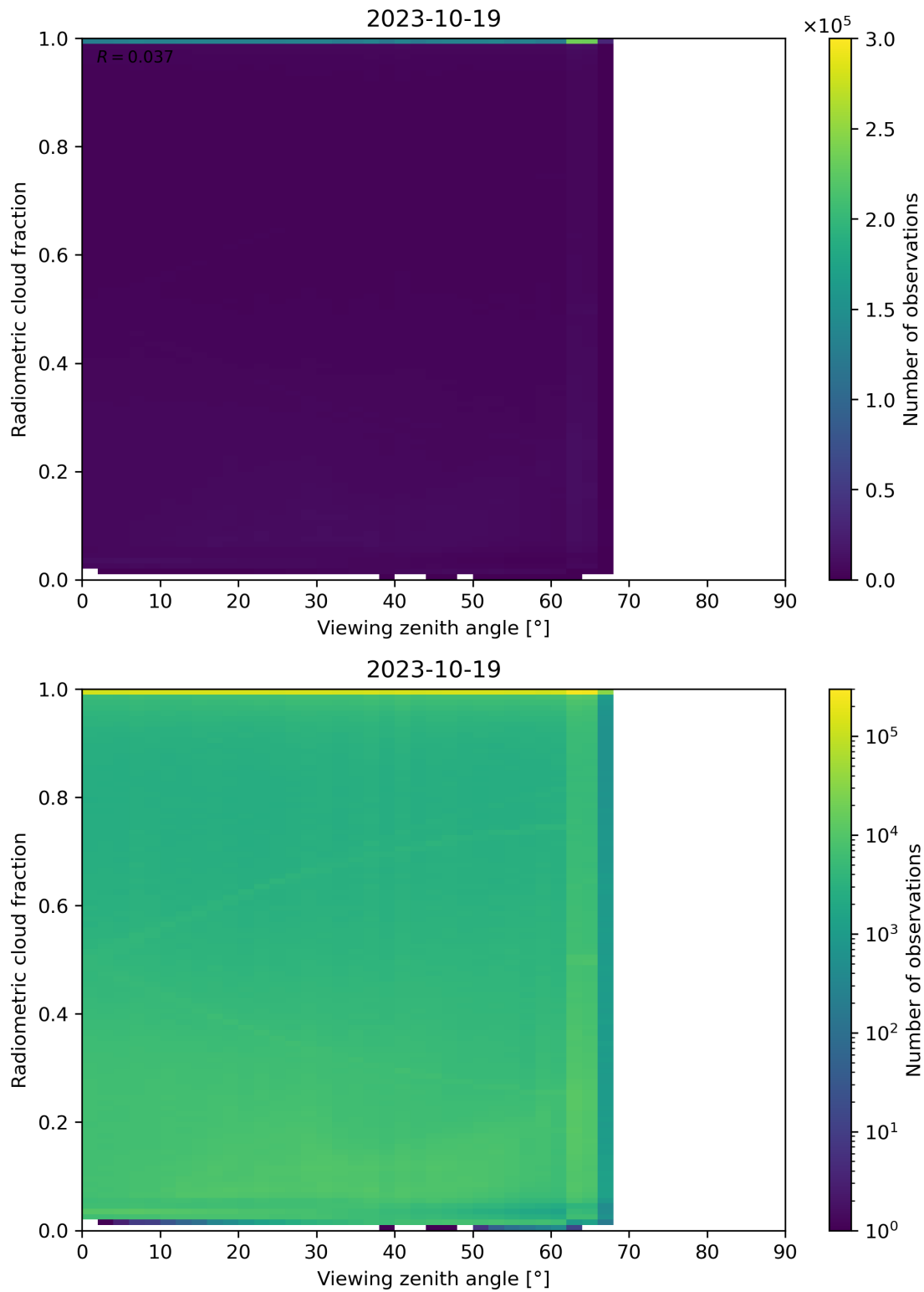
Figure 107: Scatter density plot of “Viewing zenith angle” against “Radiometric cloud fraction” for 2023-10-18 to 2023-10-20.
