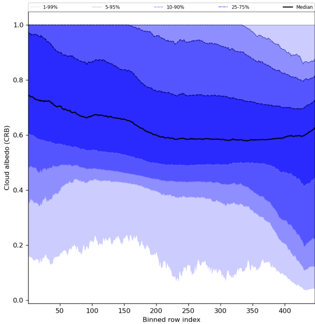
Figure 60: Along track statistics of “Cloud albedo (CRB)” for 2023-10-18 to 2023-10-20
