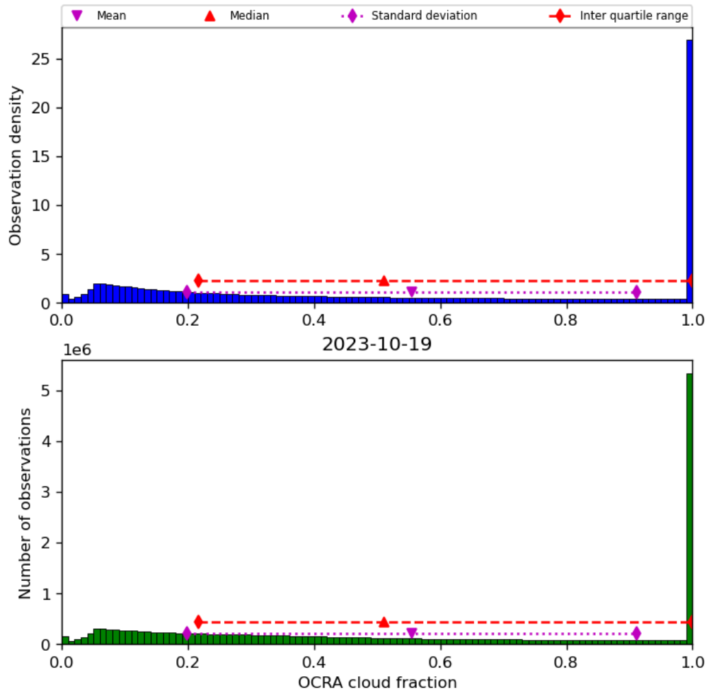
Figure 50: Histogram of “OCRA cloud fraction” for 2023-10-18 to 2023-10-20
