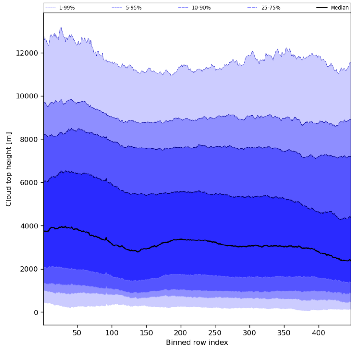
Figure 56: Along track statistics of “Cloud top height” for 2023-10-18 to 2023-10-20
