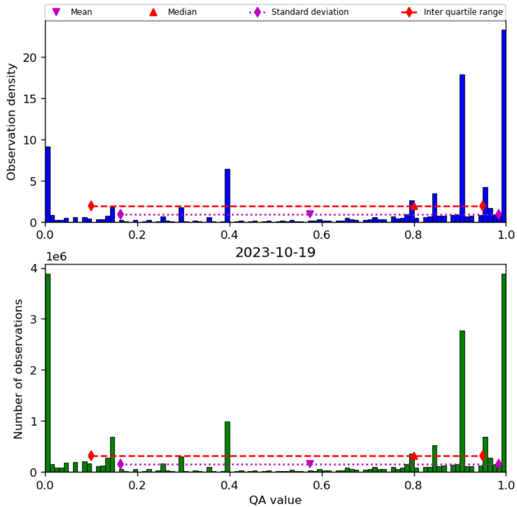
Figure 38: Histogram of “QA value” for 2023-10-18 to 2023-10-20
