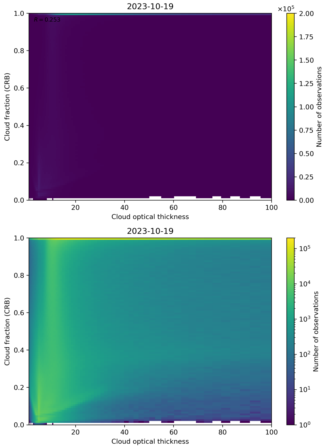
Figure 84: Scatter density plot of “Cloud optical thickness” against “Cloud fraction (CRB)” for 2023-10-18 to 2023-10-20.
