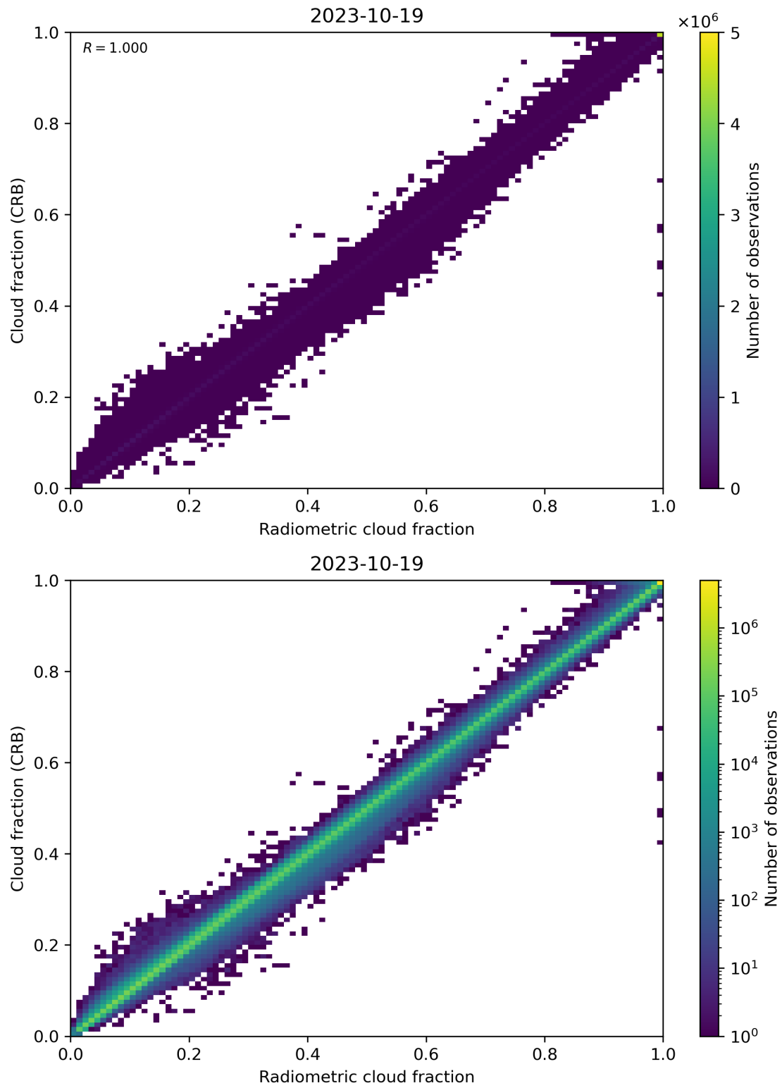
Figure 73: Scatter density plot of “Radiometric cloud fraction” against “Cloud fraction (CRB)” for 2023-10-18 to 2023-10-20.
