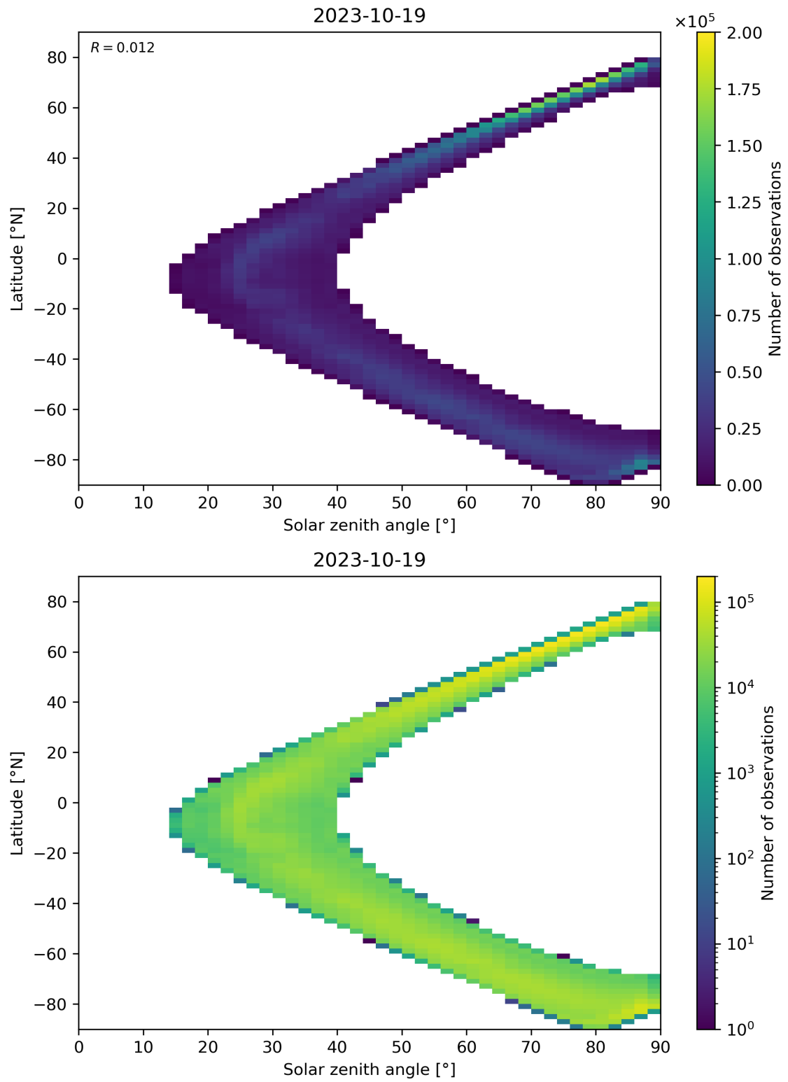
Figure 105: Scatter density plot of “Solar zenith angle” against “Latitude” for 2023-10-18 to 2023-10-20.
