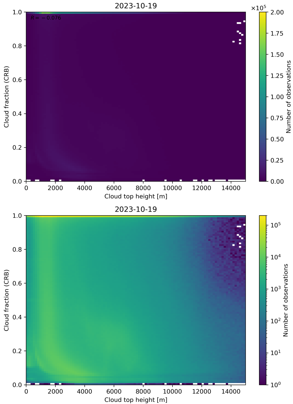
Figure 88: Scatter density plot of “Cloud top height” against “Cloud fraction (CRB)” for 2023-10-18 to 2023-10-20.
