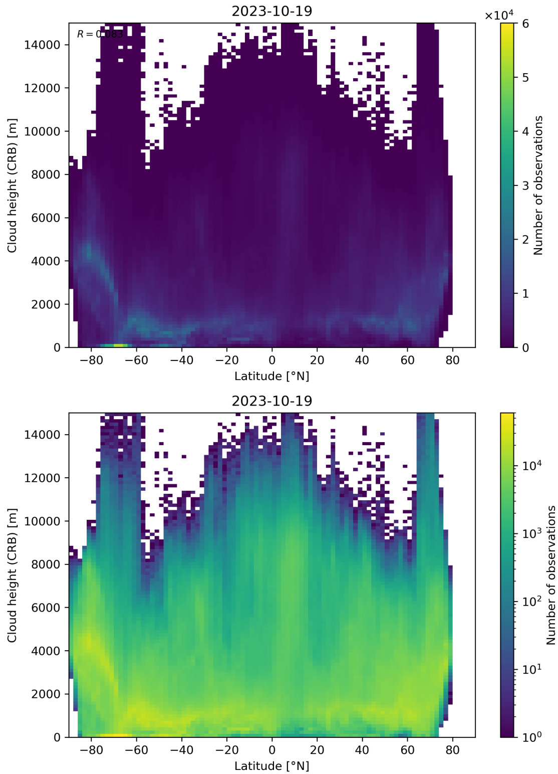
Figure 95: Scatter density plot of “Latitude” against “Cloud height (CRB)” for 2023-10-18 to 2023-10-20.
