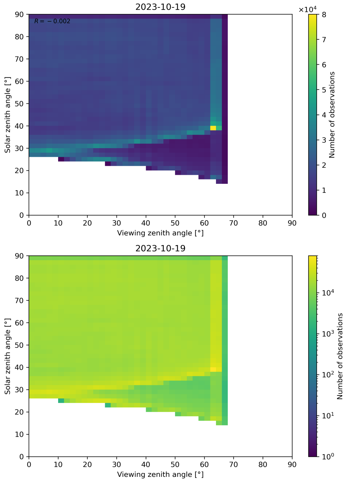
Figure 114: Scatter density plot of “Viewing zenith angle” against “Solar zenith angle” for 2023-10-18 to 2023-10-20.
