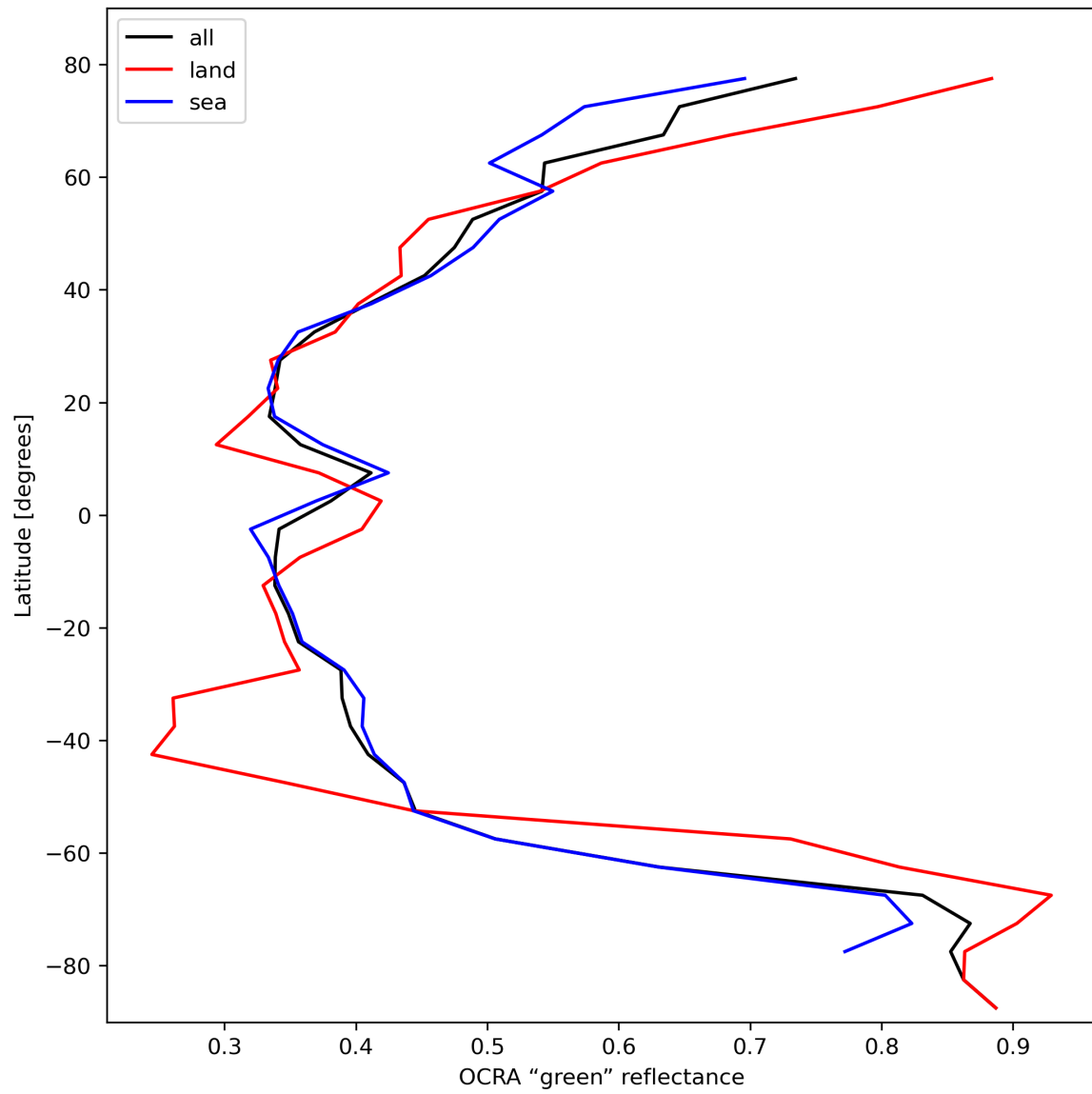
Figure 36: Zonal average of “OCRA “green” reflectance” for 2023-10-18 to 2023-10-20.
