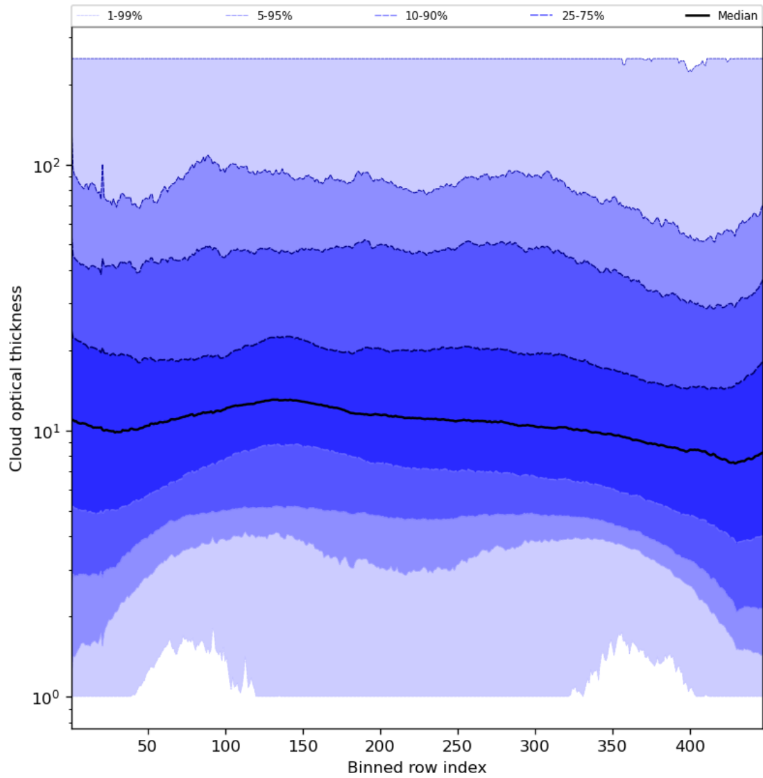
Figure 57: Along track statistics of “Cloud optical thickness” for 2023-10-18 to 2023-10-20
