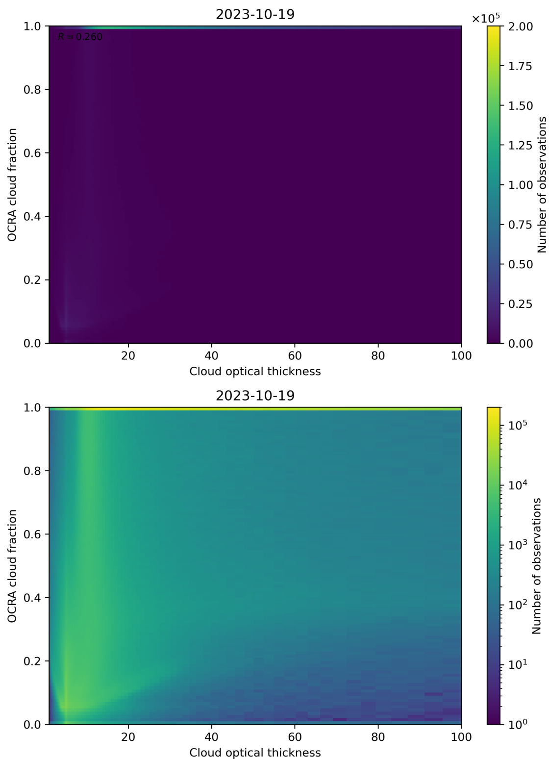
Figure 83: Scatter density plot of “Cloud optical thickness” against “OCRA cloud fraction” for 2023-10-18 to 2023-10-20.
