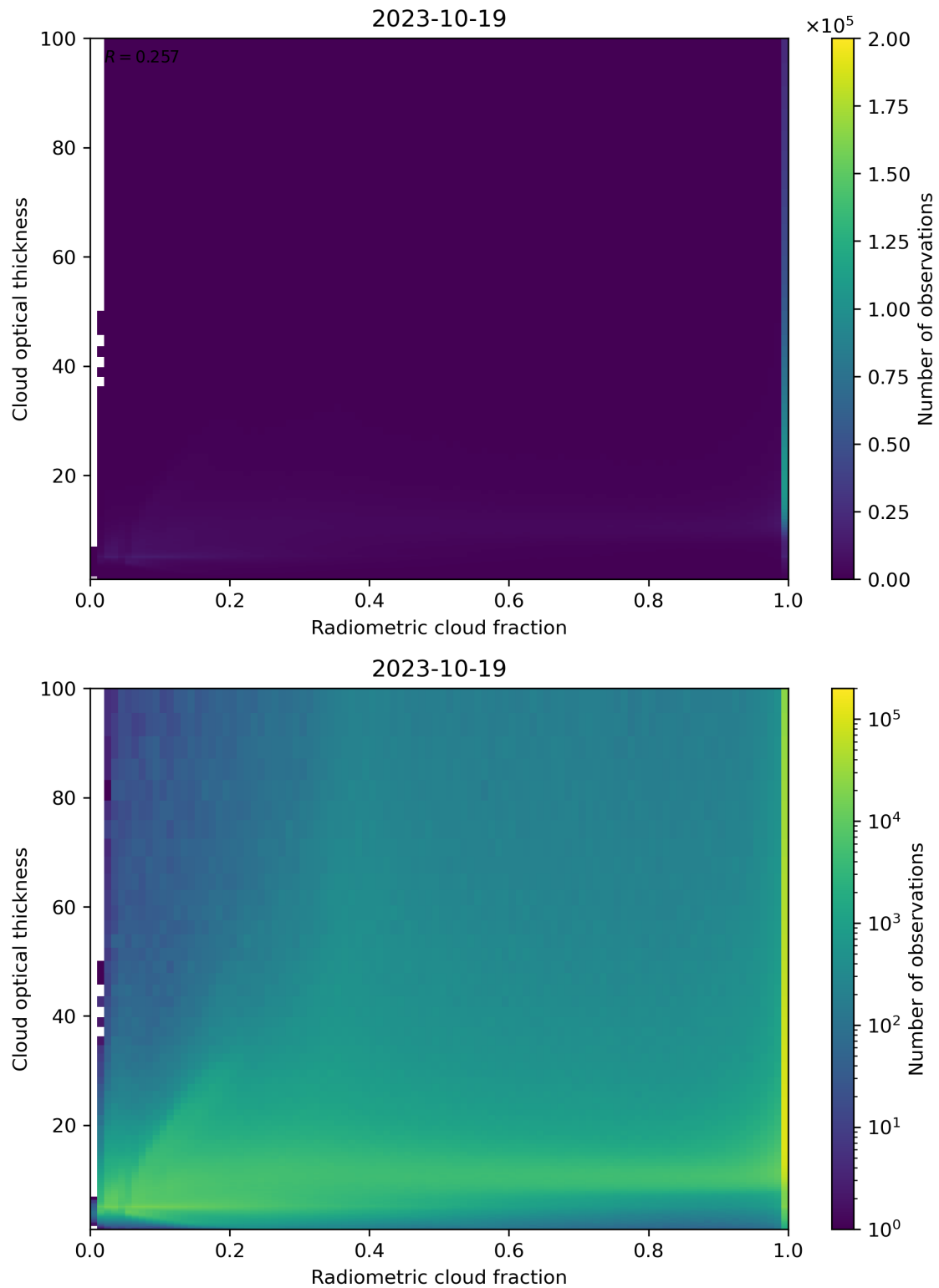
Figure 75: Scatter density plot of “Radiometric cloud fraction” against “Cloud optical thickness” for 2023-10-18 to 2023-10-20.
