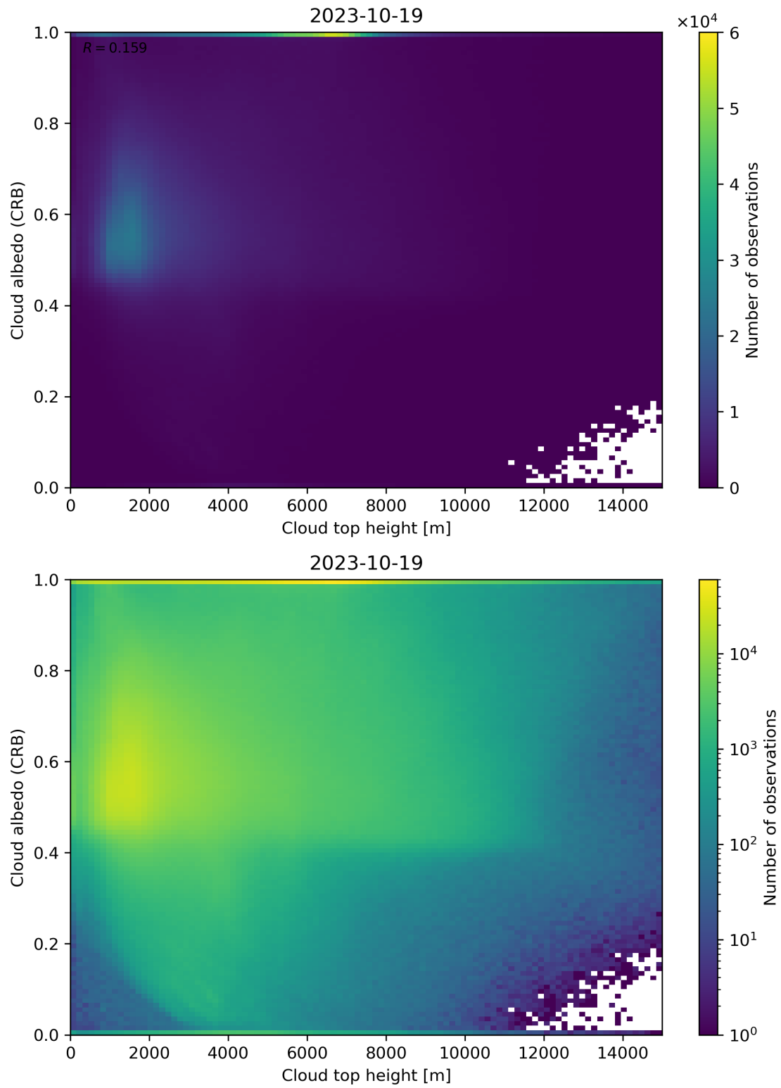
Figure 86: Scatter density plot of “Cloud top height” against “Cloud albedo (CRB)” for 2023-10-18 to 2023-10-20.
