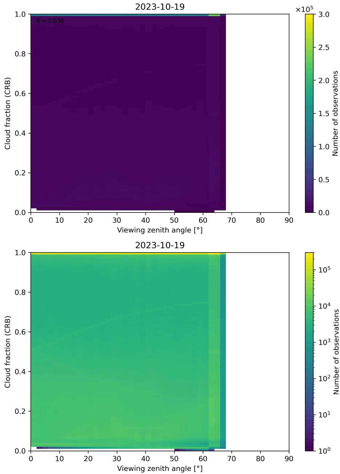
Figure 109: Scatter density plot of “Viewing zenith angle” against “Cloud fraction (CRB)” for 2023-10-18 to 2023-10-20.
