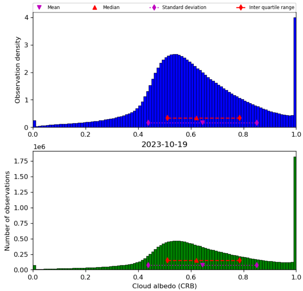
Figure 44: Histogram of “Cloud albedo (CRB)” for 2023-10-18 to 2023-10-20
