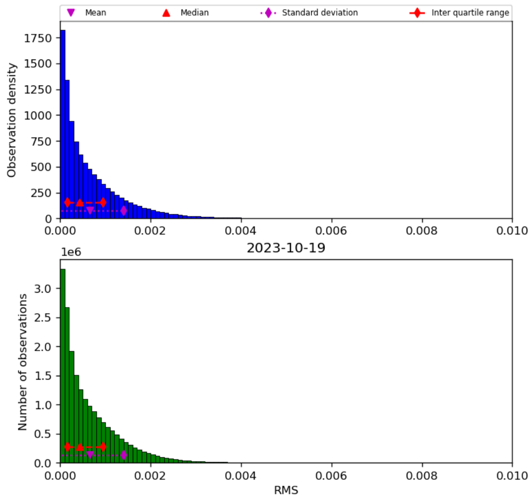
Figure 47: Histogram of “RMS” for 2023-10-18 to 2023-10-20
