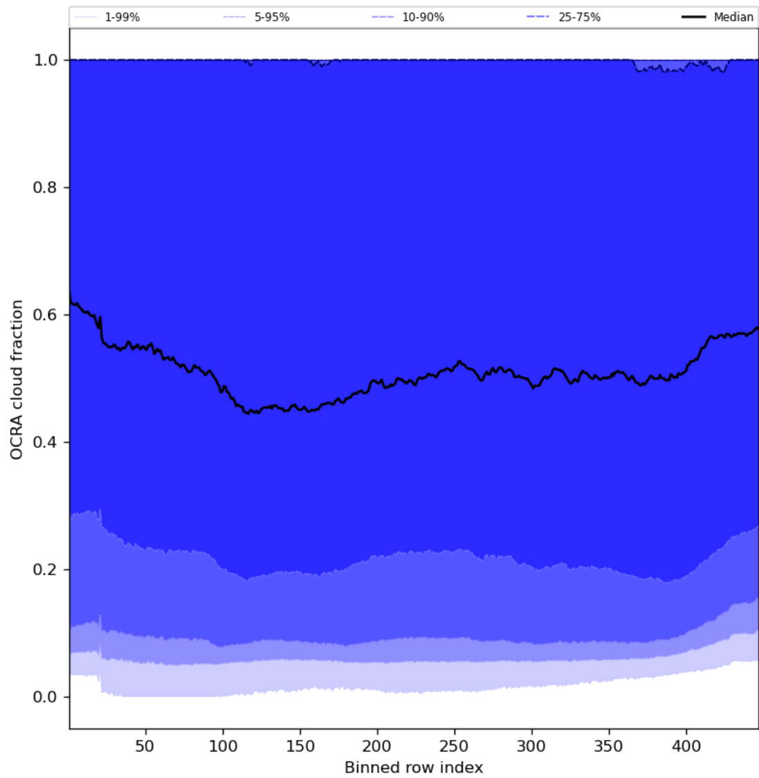
Figure 66: Along track statistics of “OCRA cloud fraction” for 2023-10-18 to 2023-10-20
