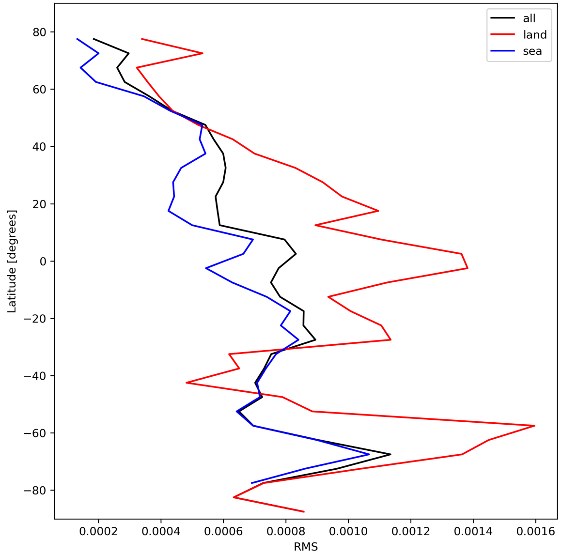
Figure 31: Zonal average of “RMS” for 2023-10-18 to 2023-10-20.
