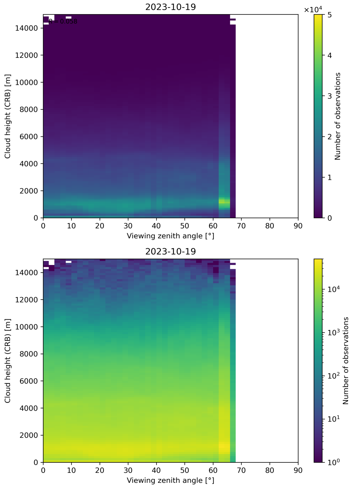
Figure 110: Scatter density plot of “Viewing zenith angle” against “Cloud height (CRB)” for 2023-10-18 to 2023-10-20.
