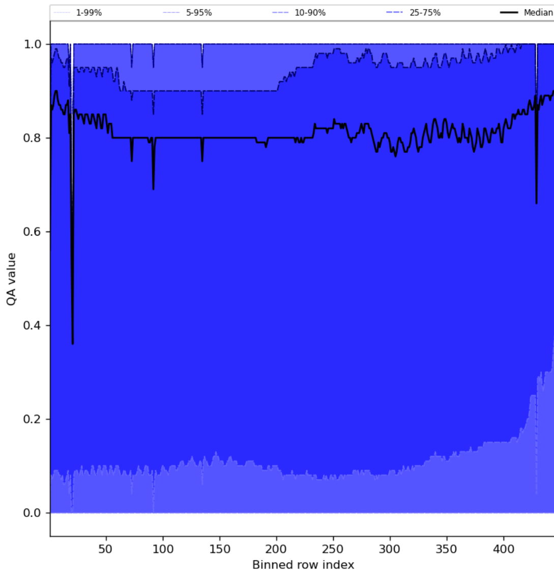
Figure 54: Along track statistics of “QA value” for 2023-10-18 to 2023-10-20
