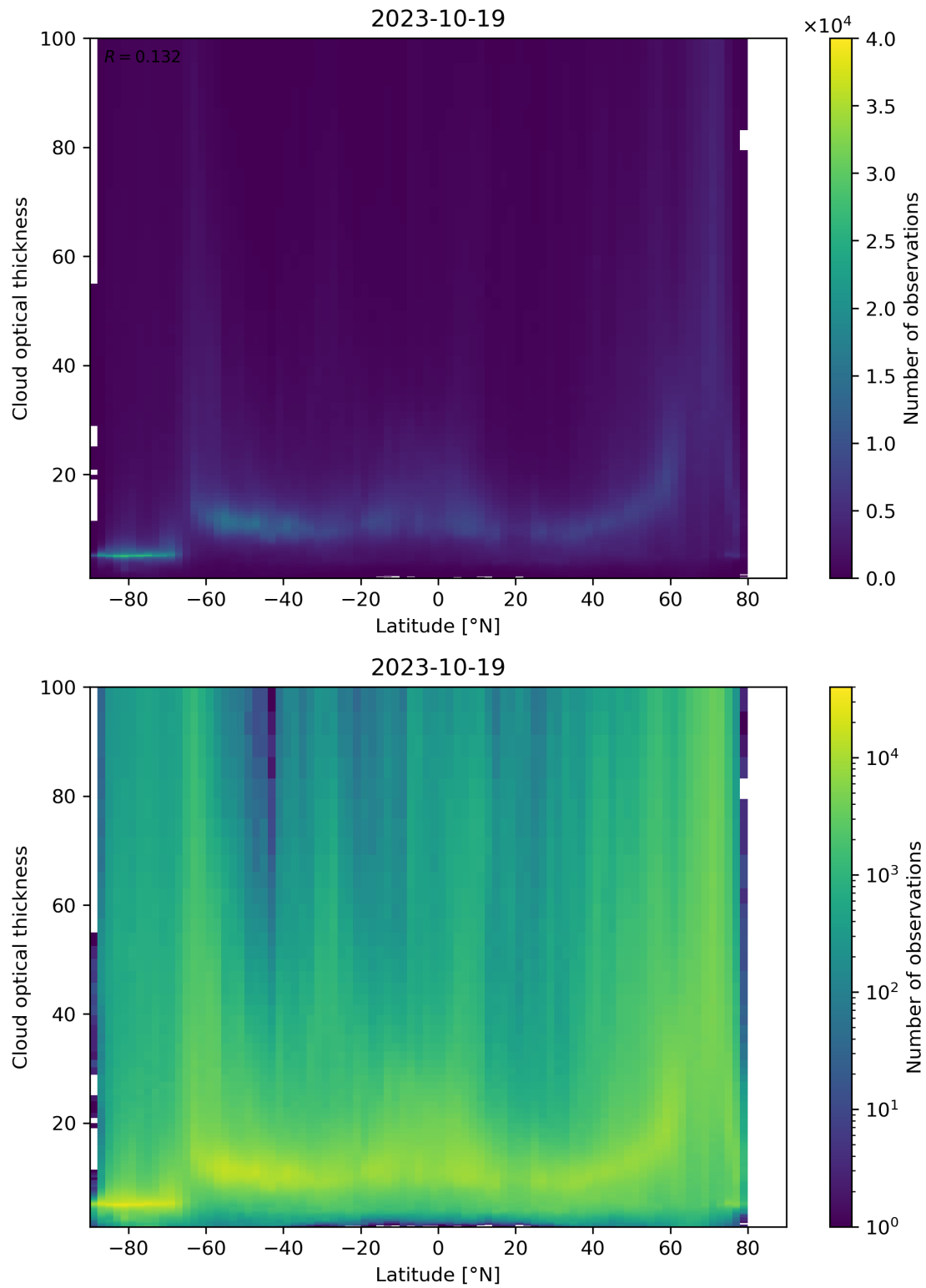
Figure 96: Scatter density plot of “Latitude” against “Cloud optical thickness” for 2023-10-18 to 2023-10-20.
