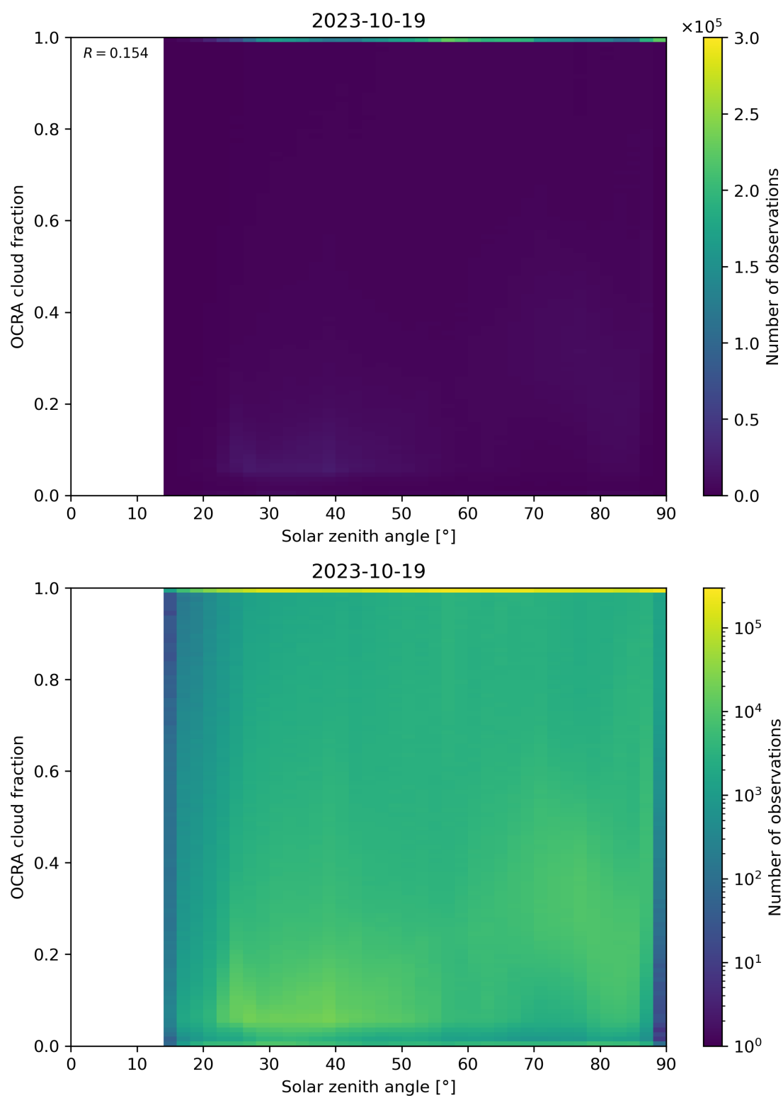
Figure 100: Scatter density plot of “Solar zenith angle” against “OCRA cloud fraction” for 2023-10-18 to 2023-10-20.
