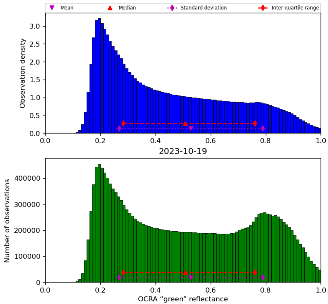
Figure 52: Histogram of “OCRA “green” reflectance” for 2023-10-18 to 2023-10-20
