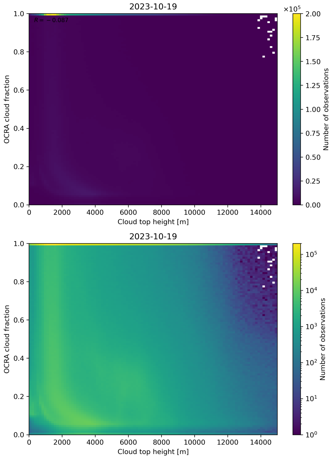
Figure 87: Scatter density plot of “Cloud top height” against “OCRA cloud fraction” for 2023-10-18 to 2023-10-20.
