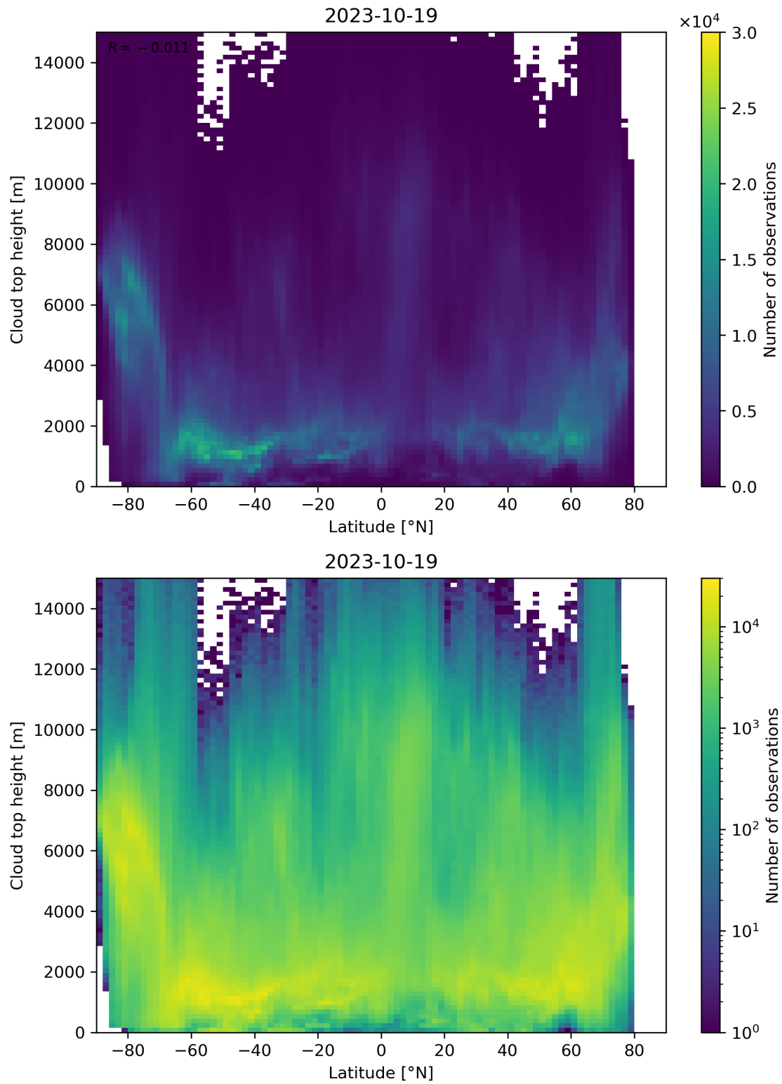
Figure 97: Scatter density plot of “Latitude” against “Cloud top height” for 2023-10-18 to 2023-10-20.
