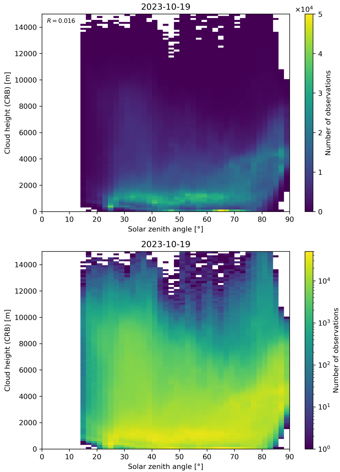
Figure 102: Scatter density plot of “Solar zenith angle” against “Cloud height (CRB)” for 2023-10-18 to 2023-10-20.
