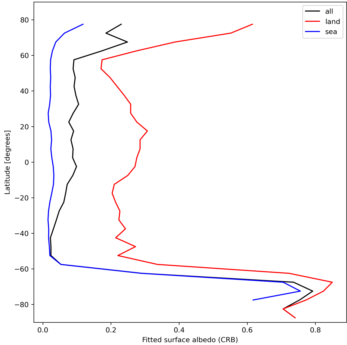
Figure 30: Zonal average of “Fitted surface albedo (CRB)” for 2023-10-18 to 2023-10-20.
