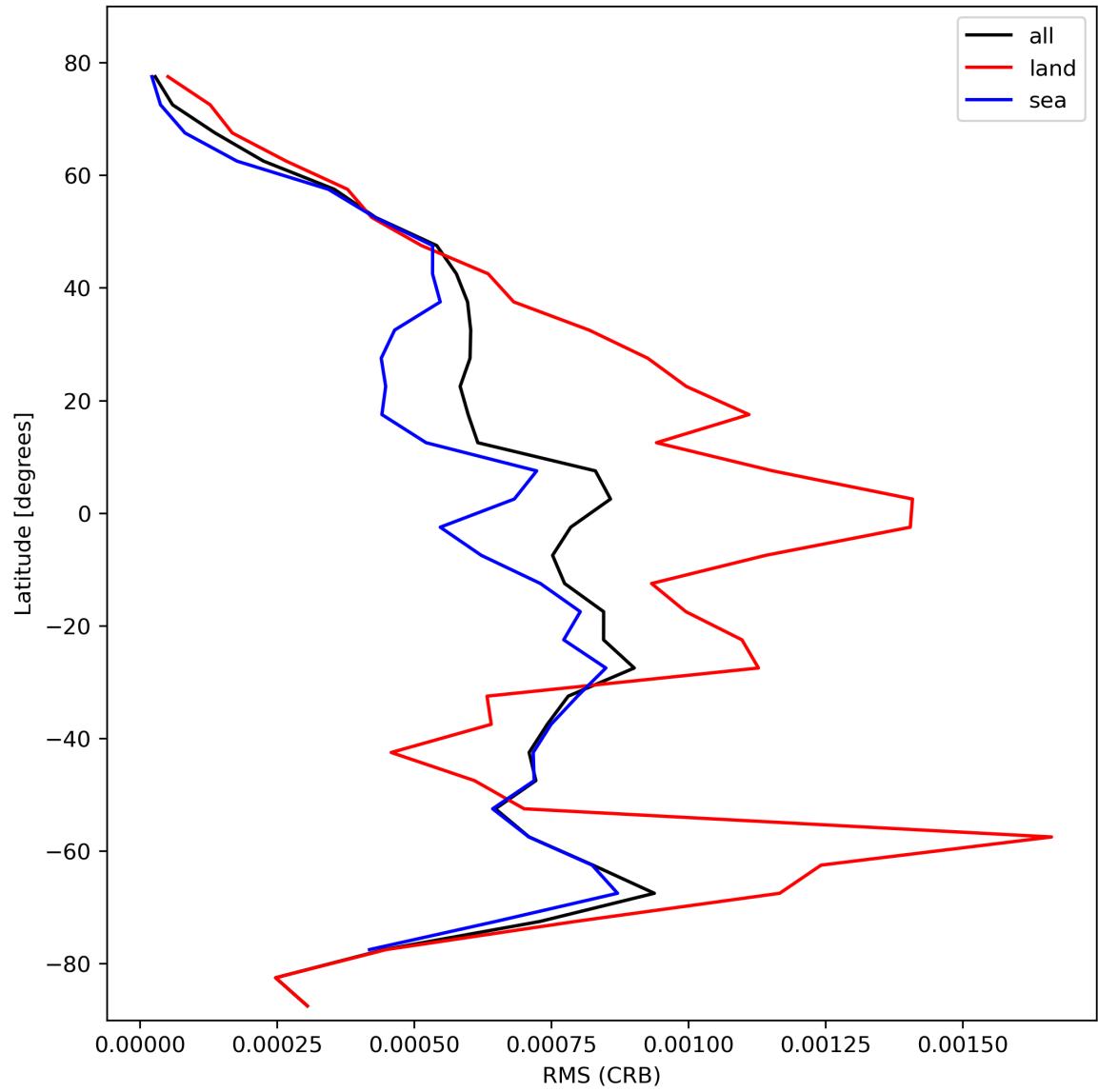
Figure 32: Zonal average of “RMS (CRB)” for 2023-10-18 to 2023-10-20.
