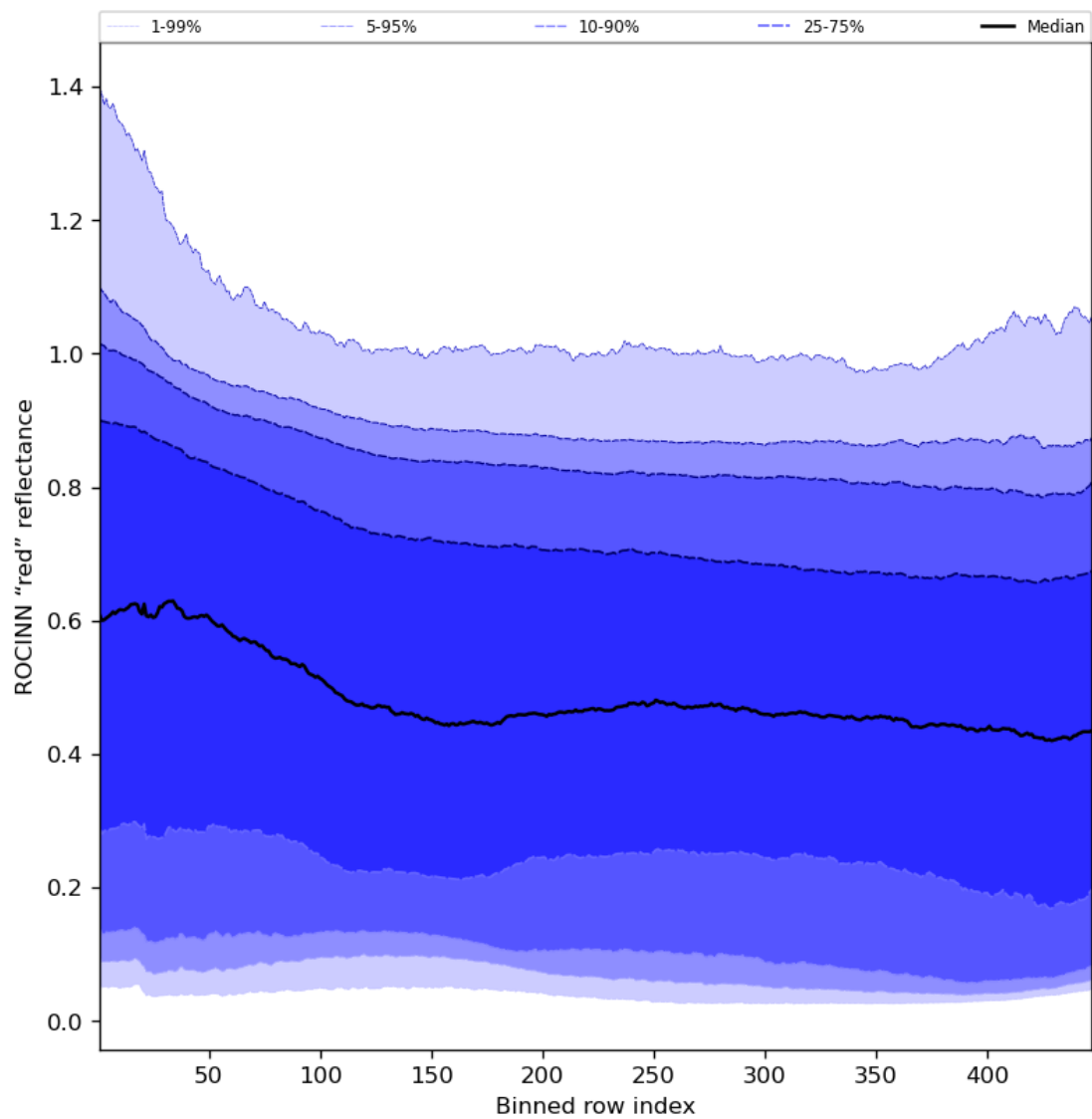
Figure 69: Along track statistics of “ROCINN “red” reflectance” for 2023-10-18 to 2023-10-20
