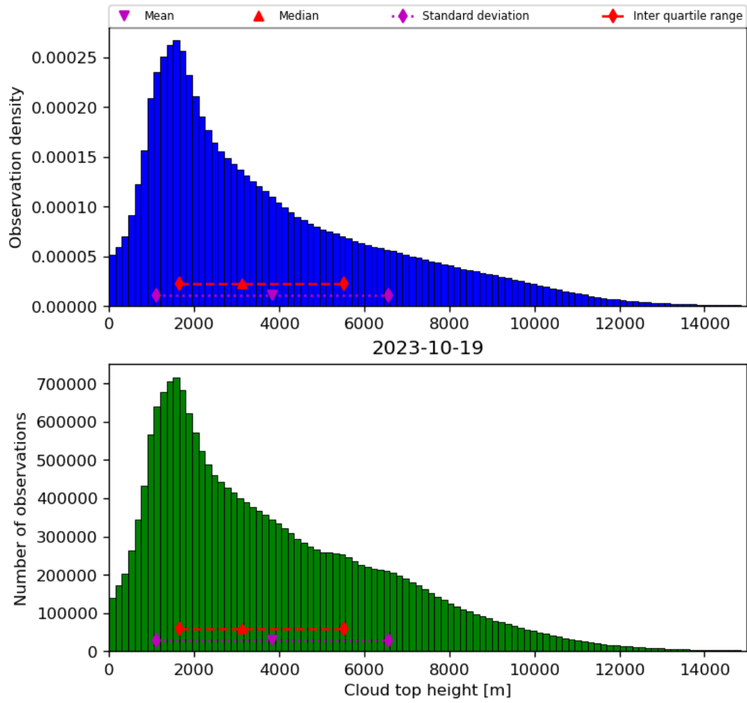
Figure 40: Histogram of “Cloud top height” for 2023-10-18 to 2023-10-20
