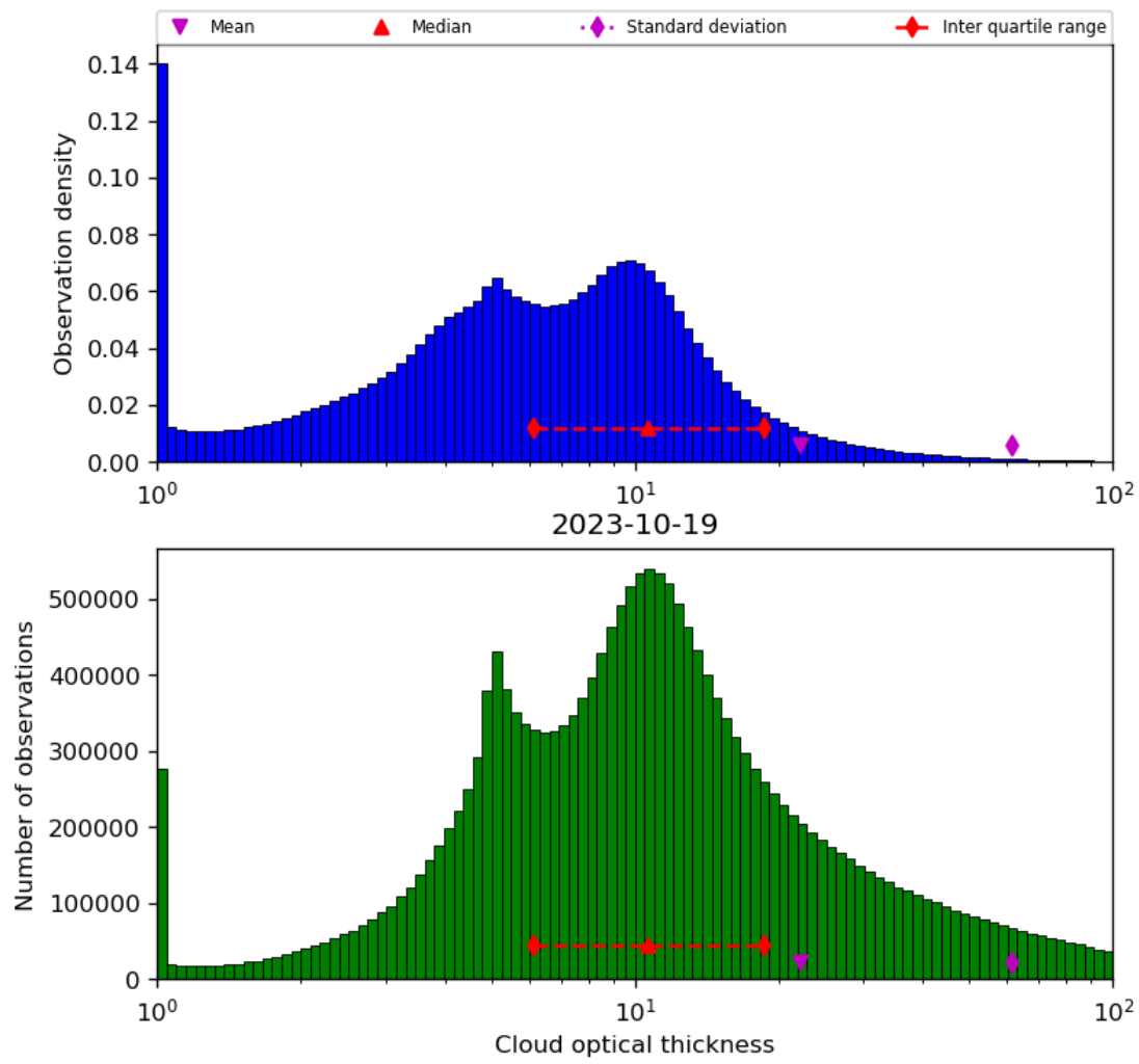
Figure 41: Histogram of “Cloud optical thickness” for 2023-10-18 to 2023-10-20
