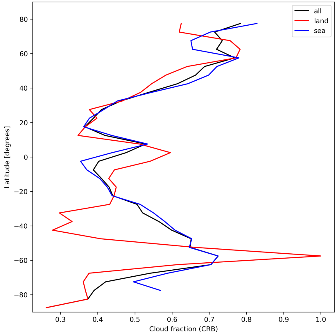
Figure 26: Zonal average of “Cloud fraction (CRB)” for 2023-10-18 to 2023-10-20.
