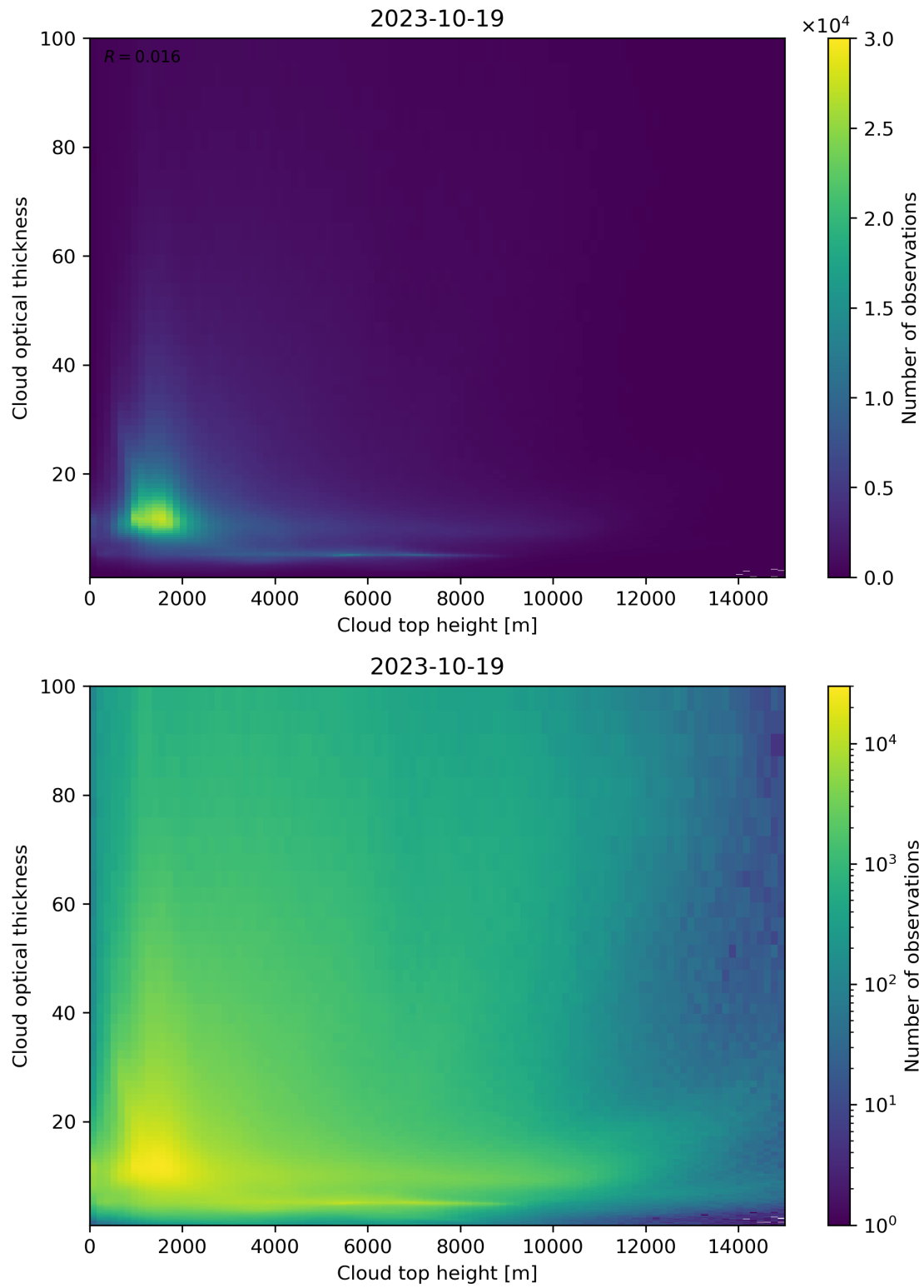
Figure 90: Scatter density plot of “Cloud top height” against “Cloud optical thickness” for 2023-10-18 to 2023-10-20.
