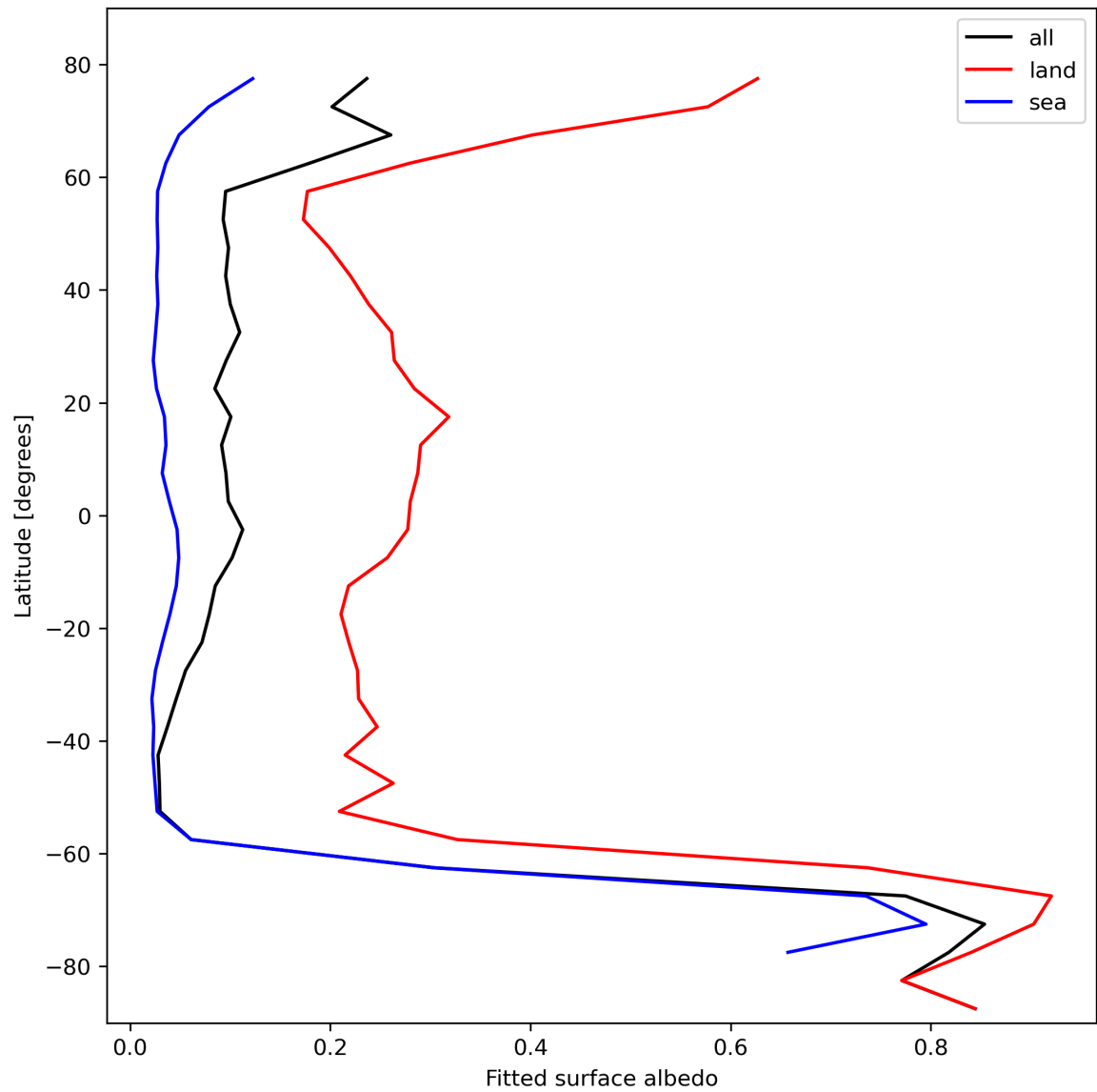
Figure 29: Zonal average of “Fitted surface albedo” for 2023-10-18 to 2023-10-20.
