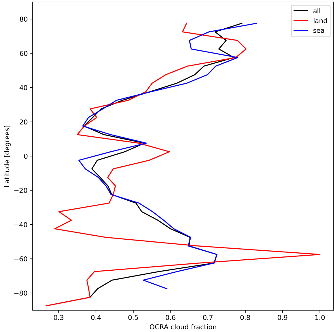
Figure 34: Zonal average of “OCRA cloud fraction” for 2023-10-18 to 2023-10-20.
