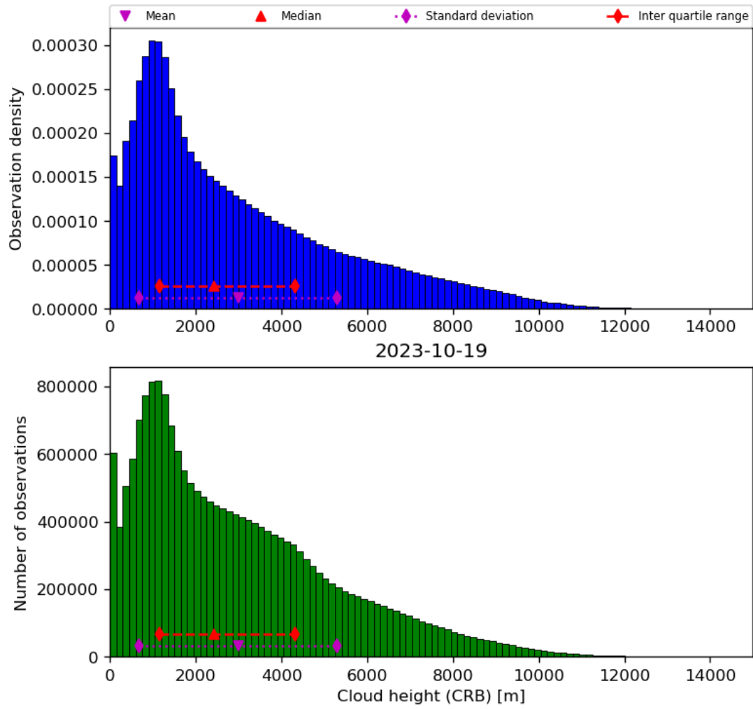
Figure 43: Histogram of “Cloud height (CRB)” for 2023-10-18 to 2023-10-20
