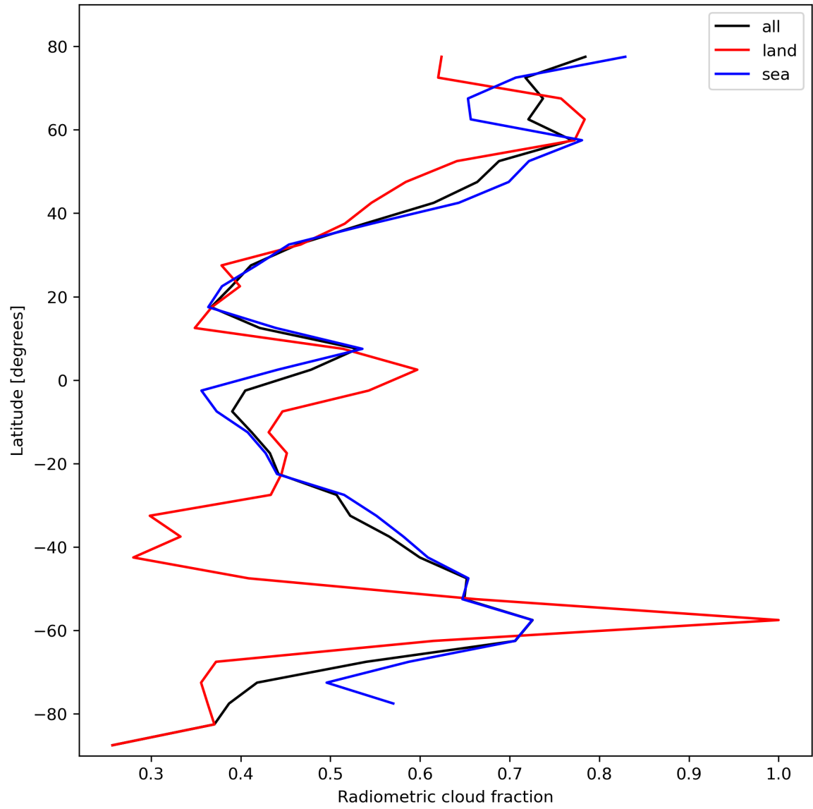
Figure 23: Zonal average of “Radiometric cloud fraction” for 2023-10-18 to 2023-10-20.
