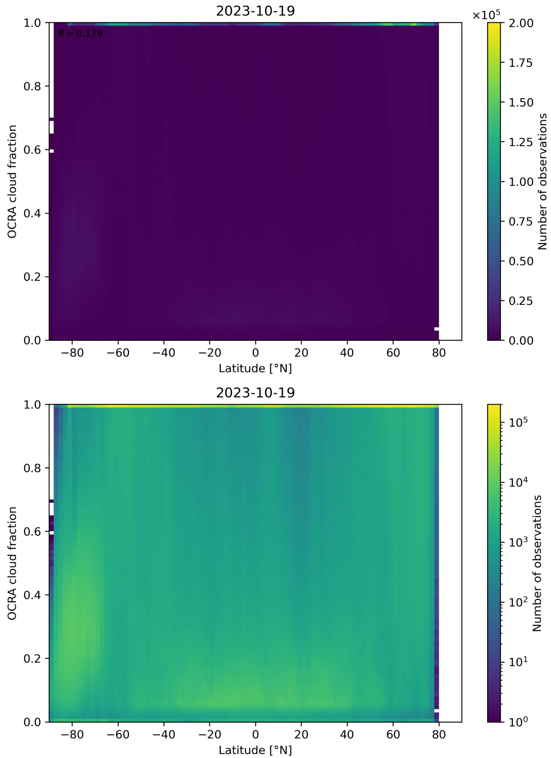
Figure 93: Scatter density plot of “Latitude” against “OCRA cloud fraction” for 2023-10-18 to 2023-10-20.
