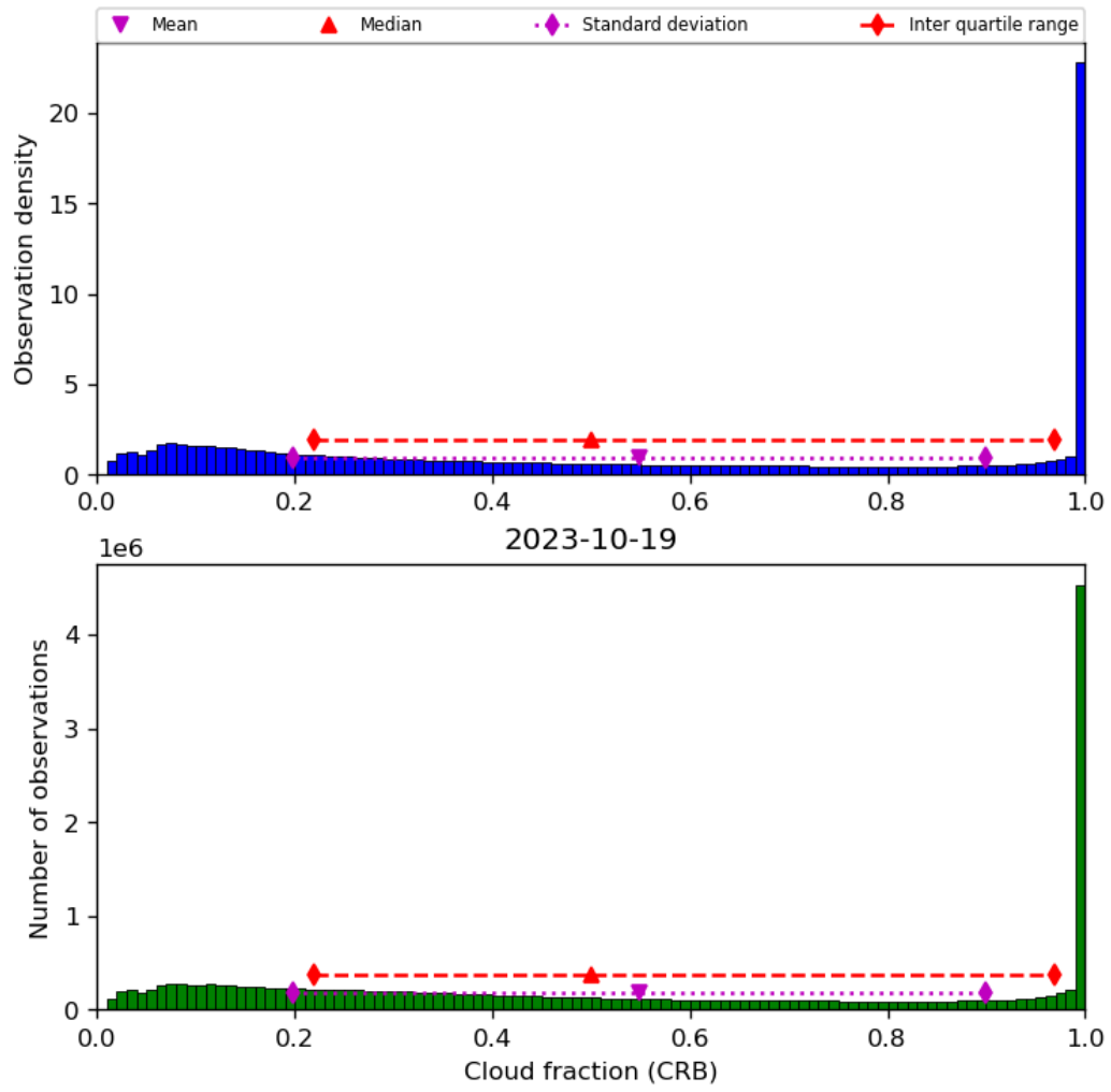
Figure 42: Histogram of “Cloud fraction (CRB)” for 2023-10-18 to 2023-10-20
