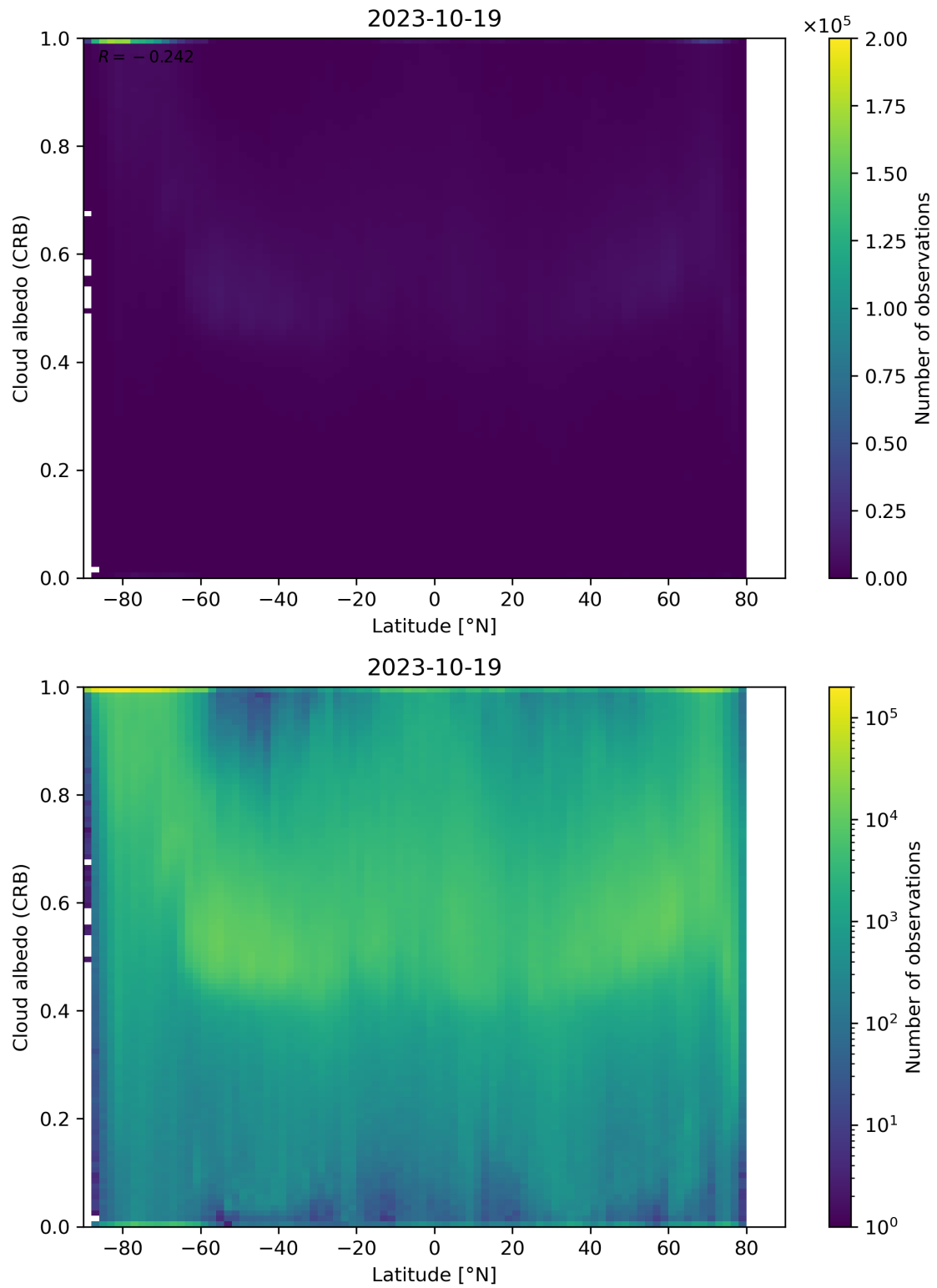
Figure 91: Scatter density plot of “Latitude” against “Cloud albedo (CRB)” for 2023-10-18 to 2023-10-20.
