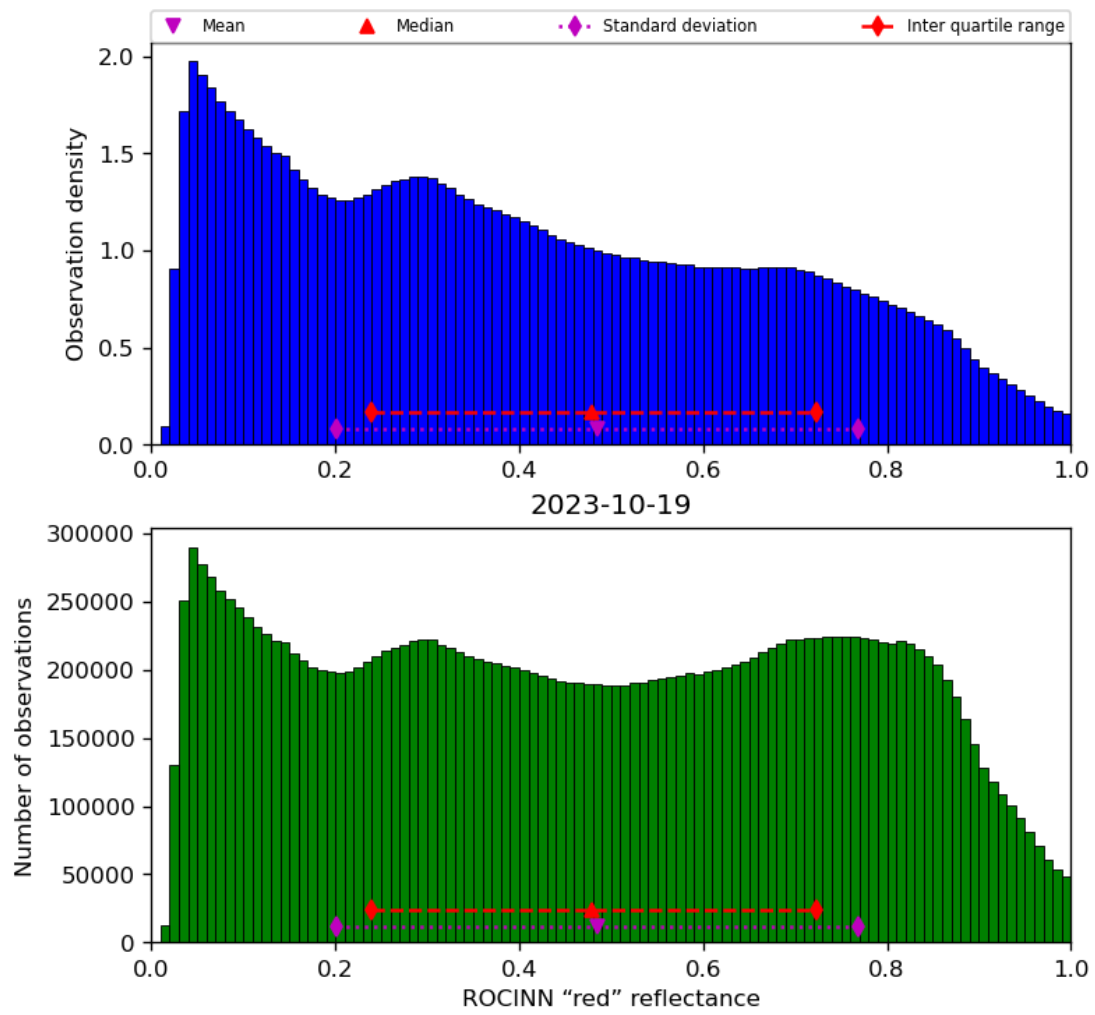
Figure 53: Histogram of “ROCINN “red” reflectance” for 2023-10-18 to 2023-10-20
