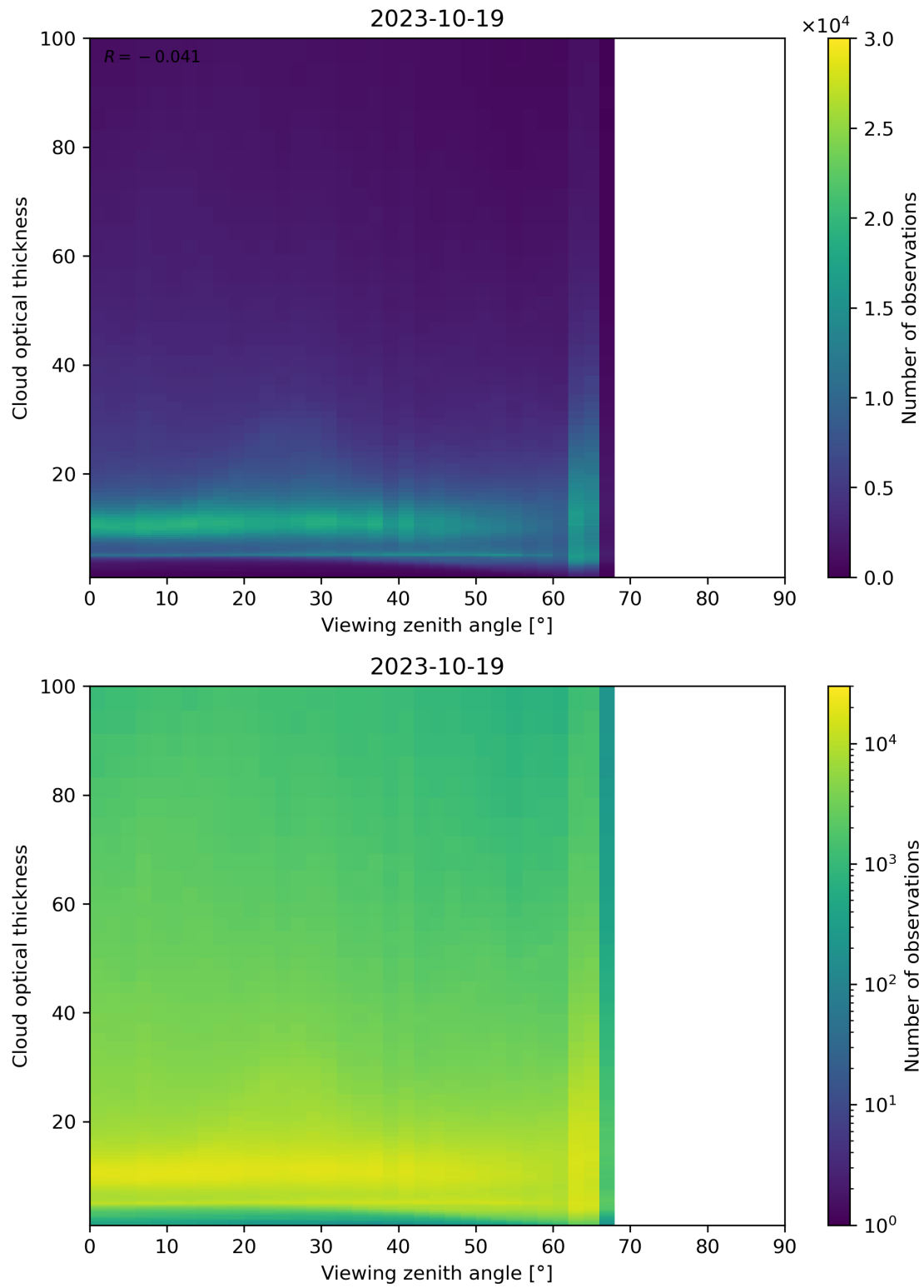
Figure 111: Scatter density plot of “Viewing zenith angle” against “Cloud optical thickness” for 2023-10-18 to 2023-10-20.
