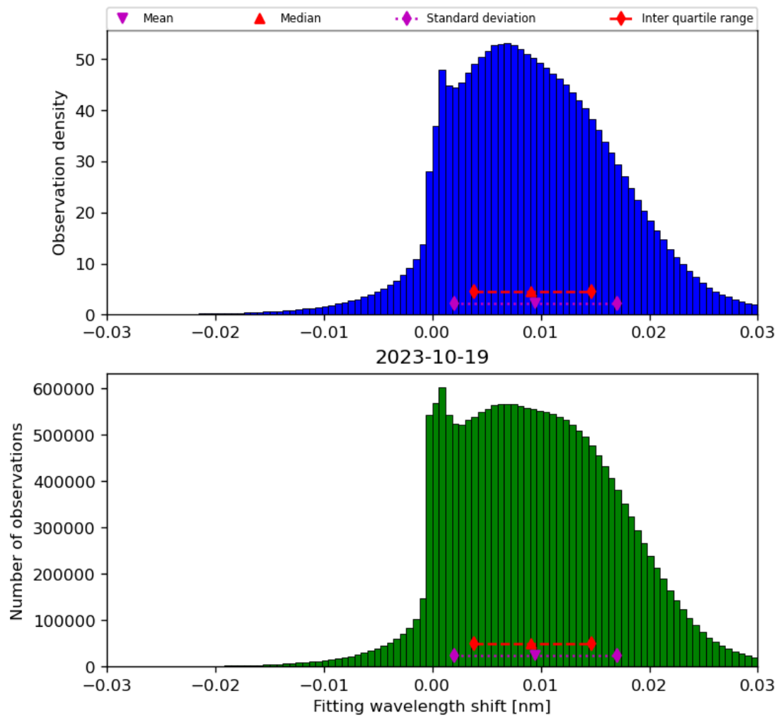
Figure 49: Histogram of “Fitting wavelength shift” for 2023-10-18 to 2023-10-20
