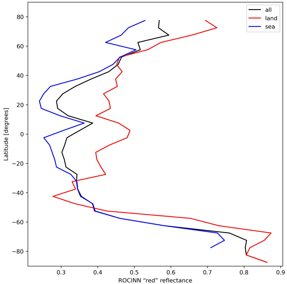
Figure 37: Zonal average of “ROCINN “red” reflectance” for 2023-10-18 to 2023-10-20.
