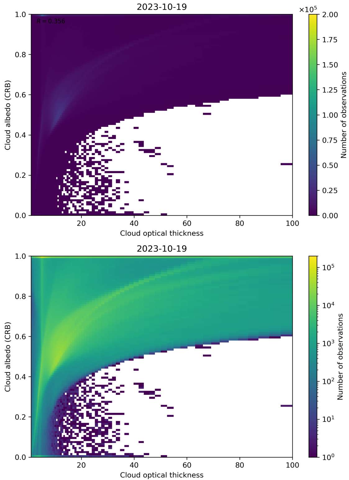
Figure 82: Scatter density plot of “Cloud optical thickness” against “Cloud albedo (CRB)” for 2023-10-18 to 2023-10-20.
