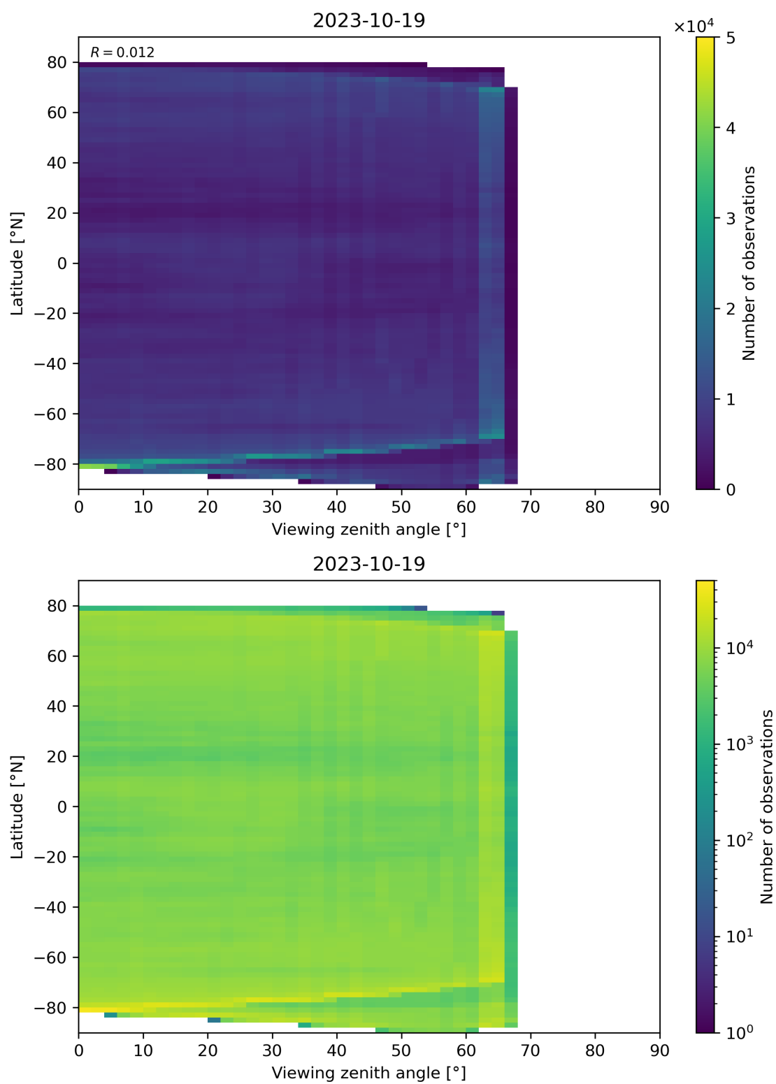
Figure 113: Scatter density plot of “Viewing zenith angle” against “Latitude” for 2023-10-18 to 2023-10-20.
