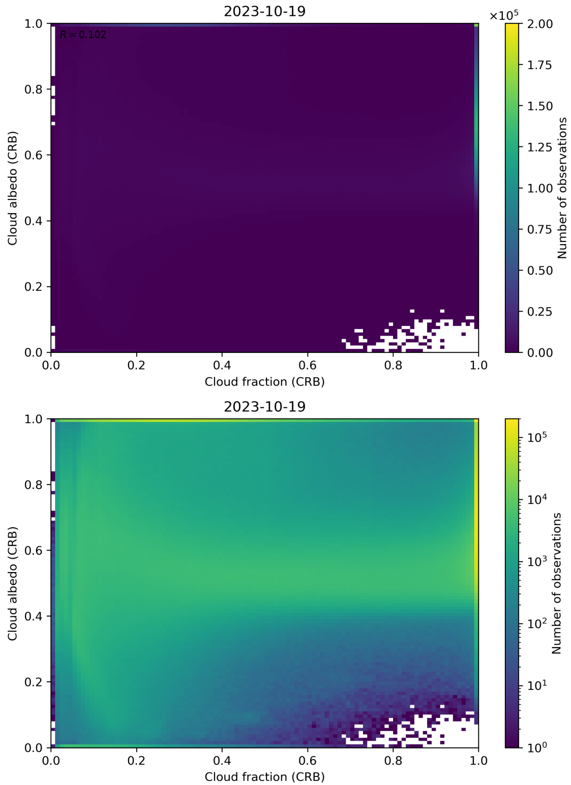
Figure 77: Scatter density plot of “Cloud fraction (CRB)” against “Cloud albedo (CRB)” for 2023-10-18 to 2023-10-20.
