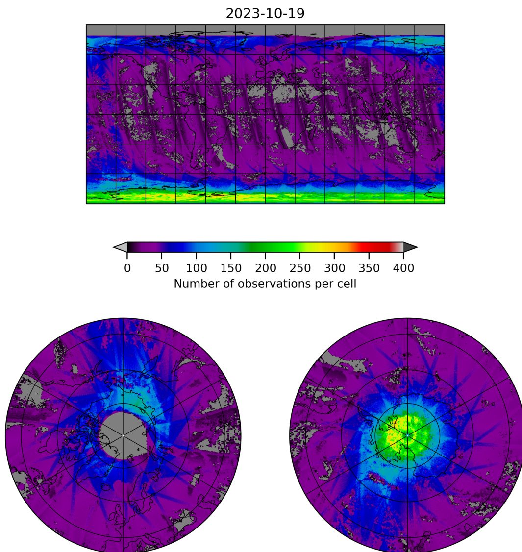
Figure 21: Map of the number of observations for 2023-10-18 to 2023-10-20
