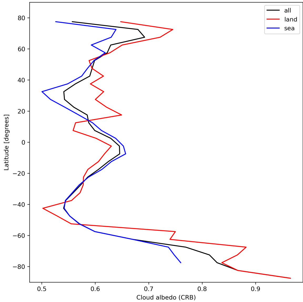
Figure 28: Zonal average of “Cloud albedo (CRB)” for 2023-10-18 to 2023-10-20.
