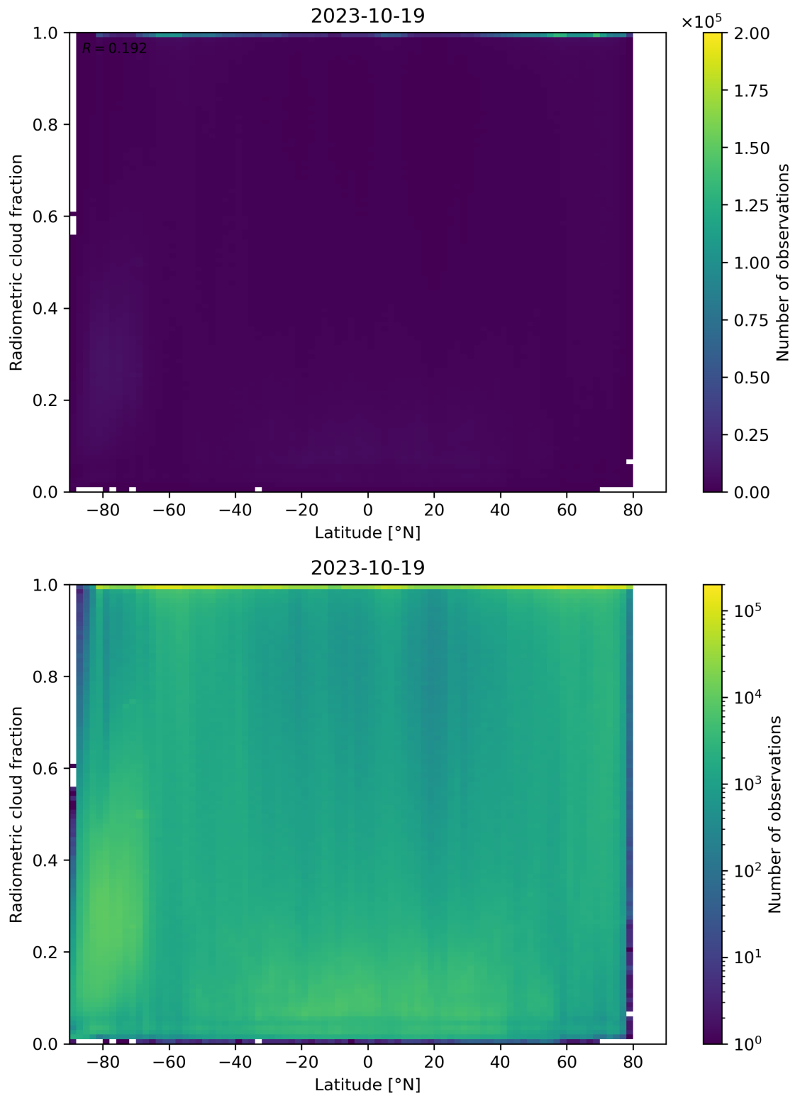
Figure 92: Scatter density plot of “Latitude” against “Radiometric cloud fraction” for 2023-10-18 to 2023-10-20.
