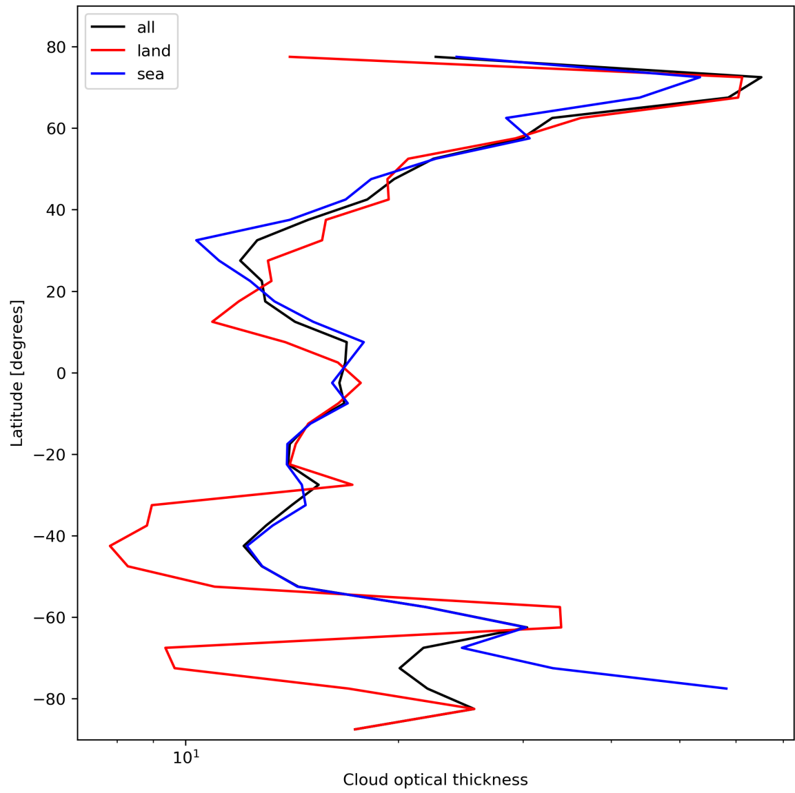
Figure 25: Zonal average of “Cloud optical thickness” for 2023-10-18 to 2023-10-20.
