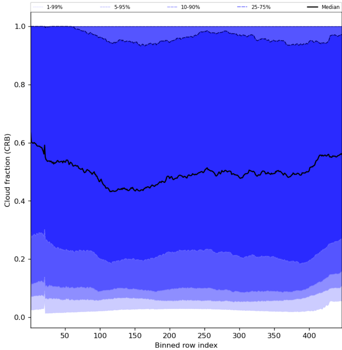
Figure 58: Along track statistics of “Cloud fraction (CRB)” for 2023-10-18 to 2023-10-20
