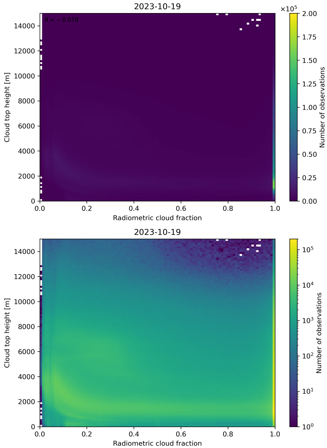
Figure 76: Scatter density plot of “Radiometric cloud fraction” against “Cloud top height” for 2023-10-18 to 2023-10-20.
