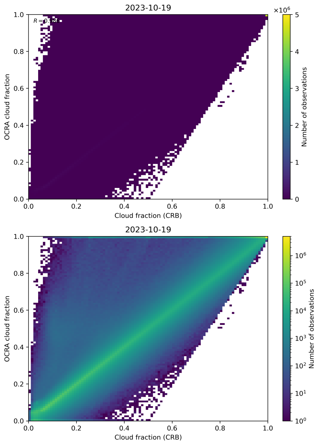
Figure 78: Scatter density plot of “Cloud fraction (CRB)” against “OCRA cloud fraction” for 2023-10-18 to 2023-10-20.
