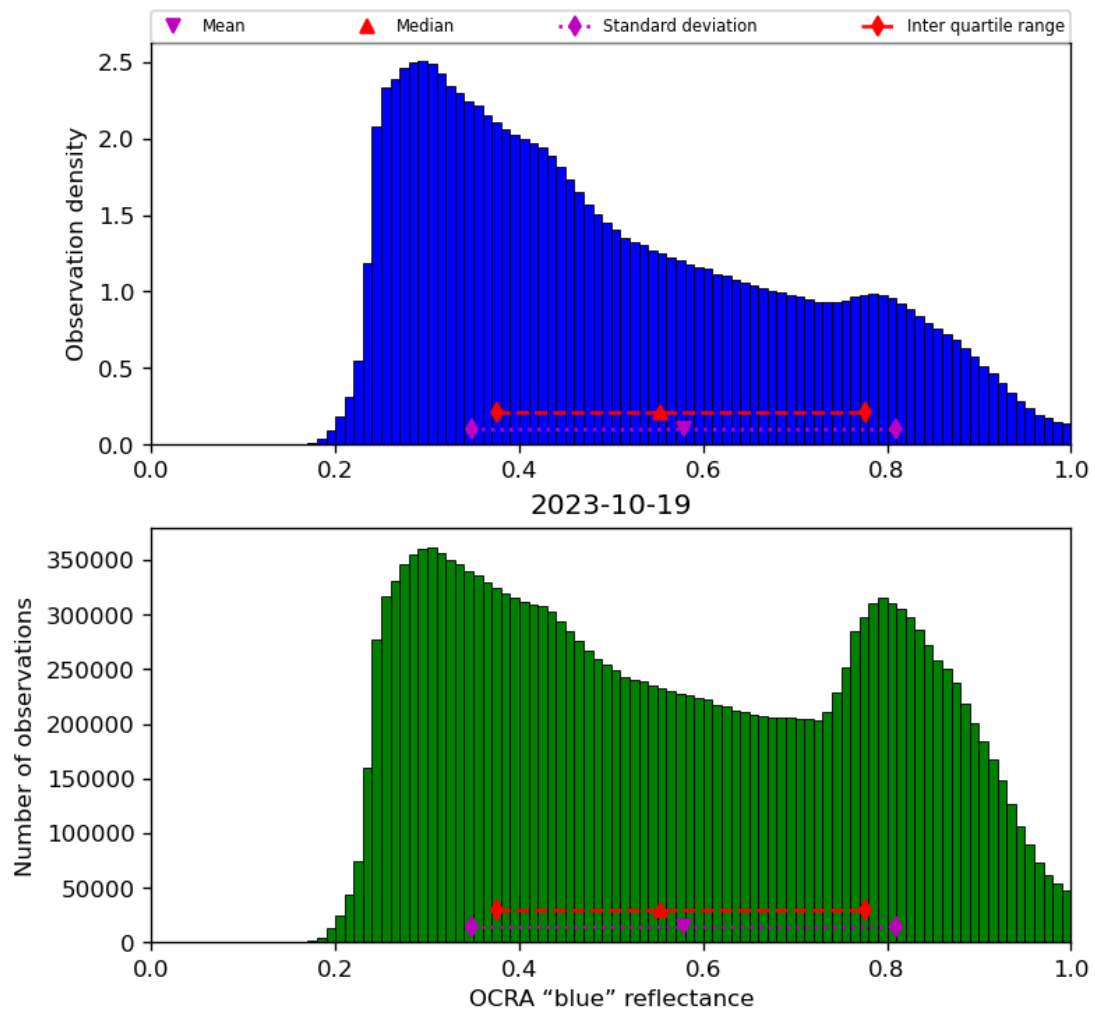
Figure 51: Histogram of “OCRA “blue” reflectance” for 2023-10-18 to 2023-10-20
