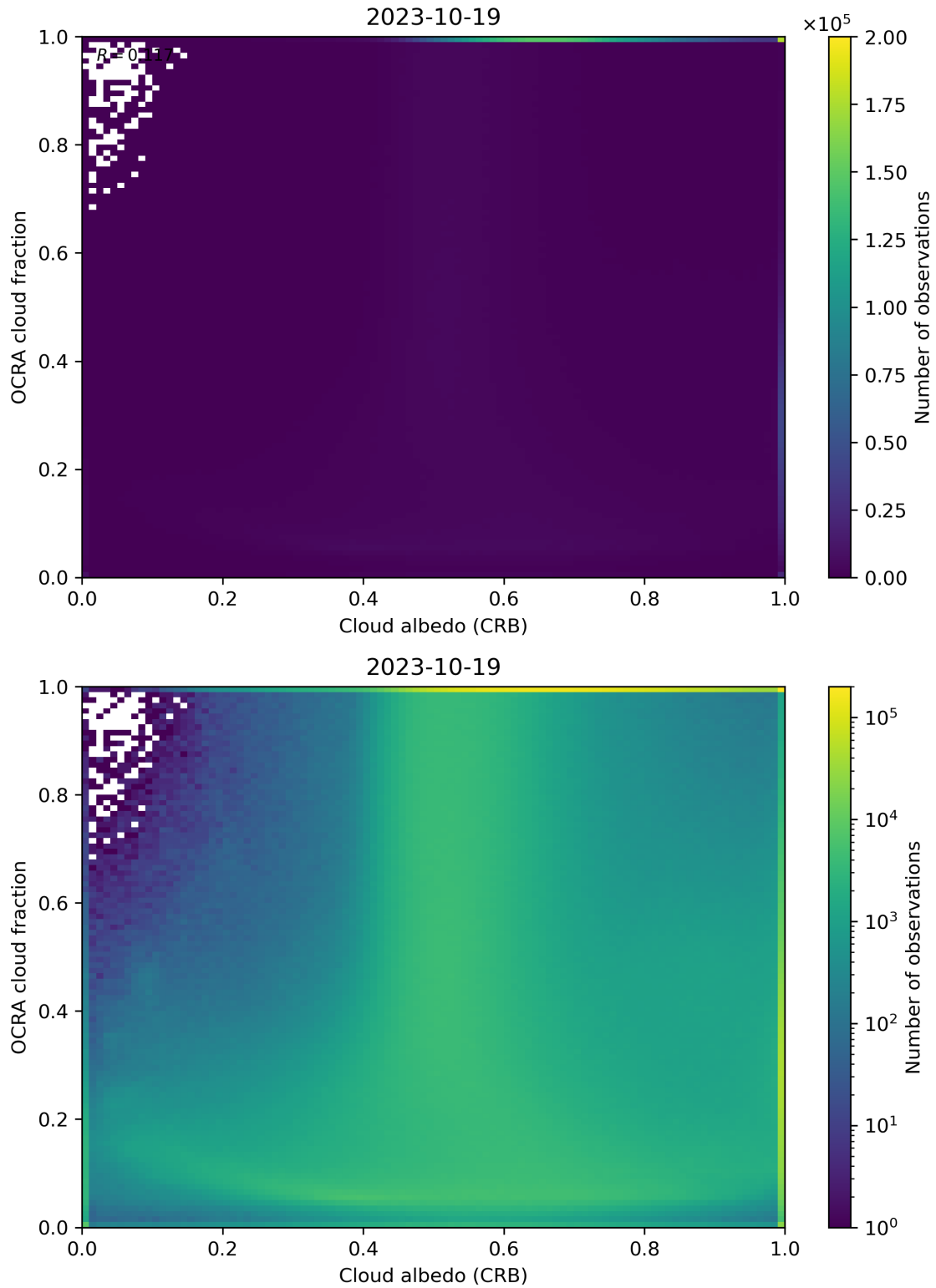
Figure 70: Scatter density plot of “Cloud albedo (CRB)” against “OCRA cloud fraction” for 2023-10-18 to 2023-10-20.
