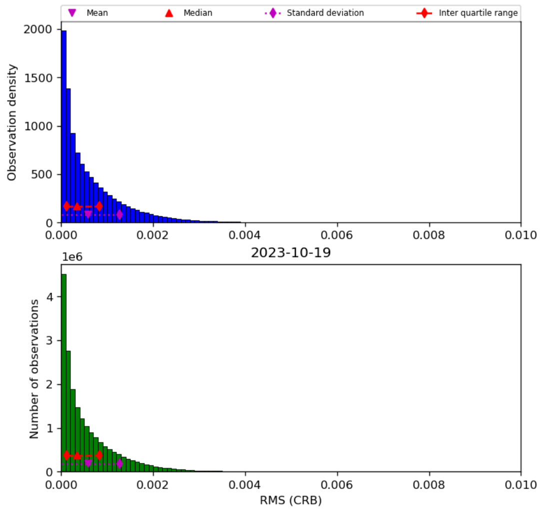
Figure 48: Histogram of “RMS (CRB)” for 2023-10-18 to 2023-10-20
