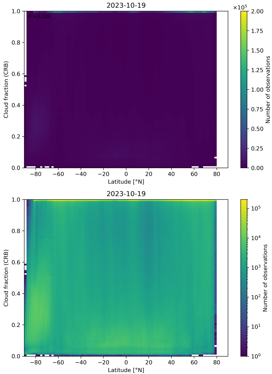
Figure 94: Scatter density plot of “Latitude” against “Cloud fraction (CRB)” for 2023-10-18 to 2023-10-20.
