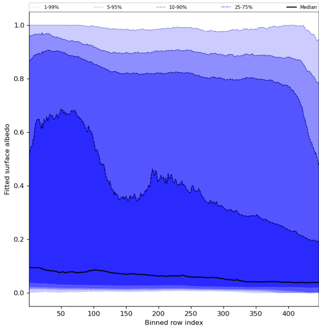
Figure 61: Along track statistics of “Fitted surface albedo” for 2023-10-18 to 2023-10-20
