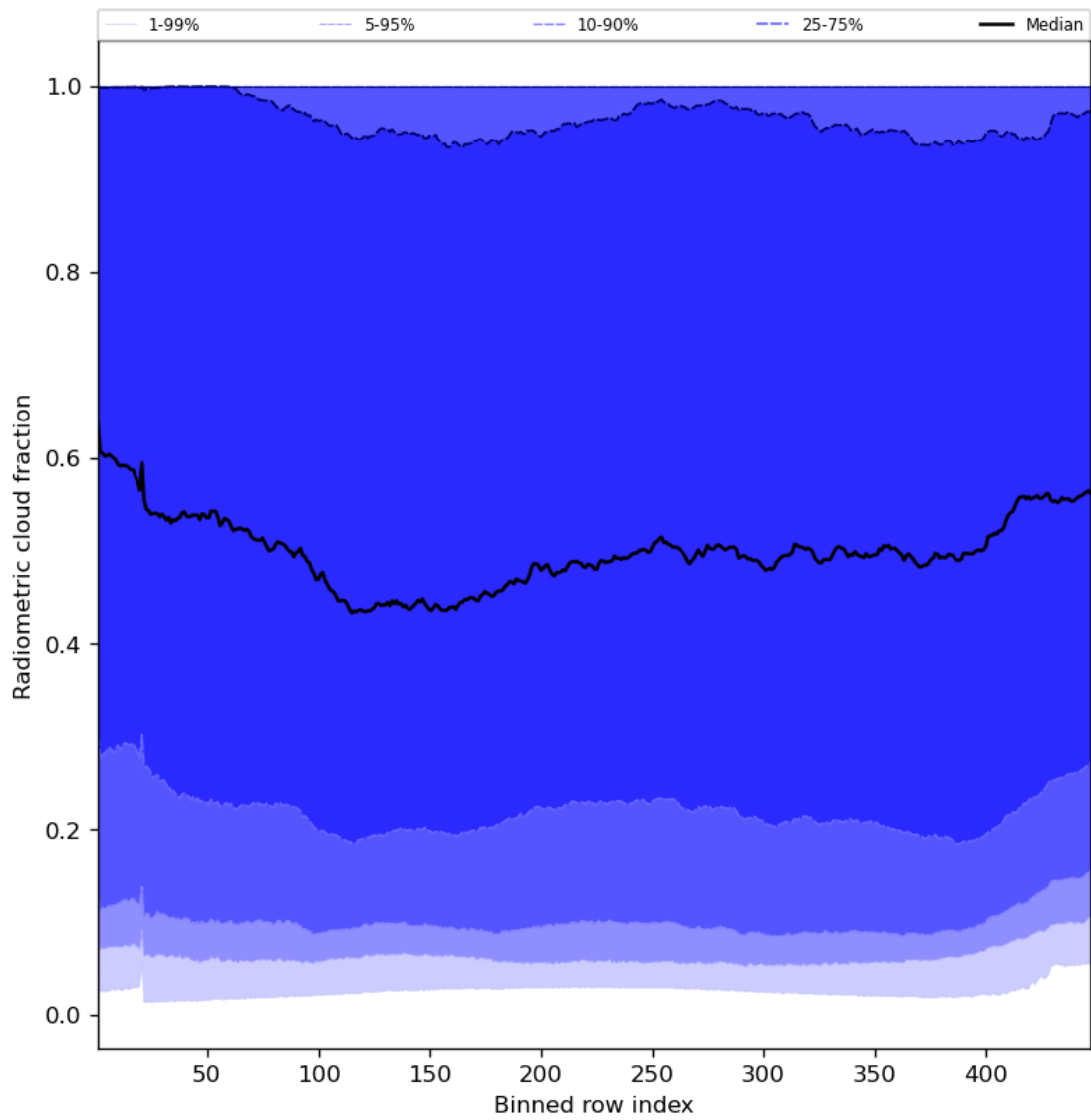
Figure 55: Along track statistics of “Radiometric cloud fraction” for 2023-10-18 to 2023-10-20
