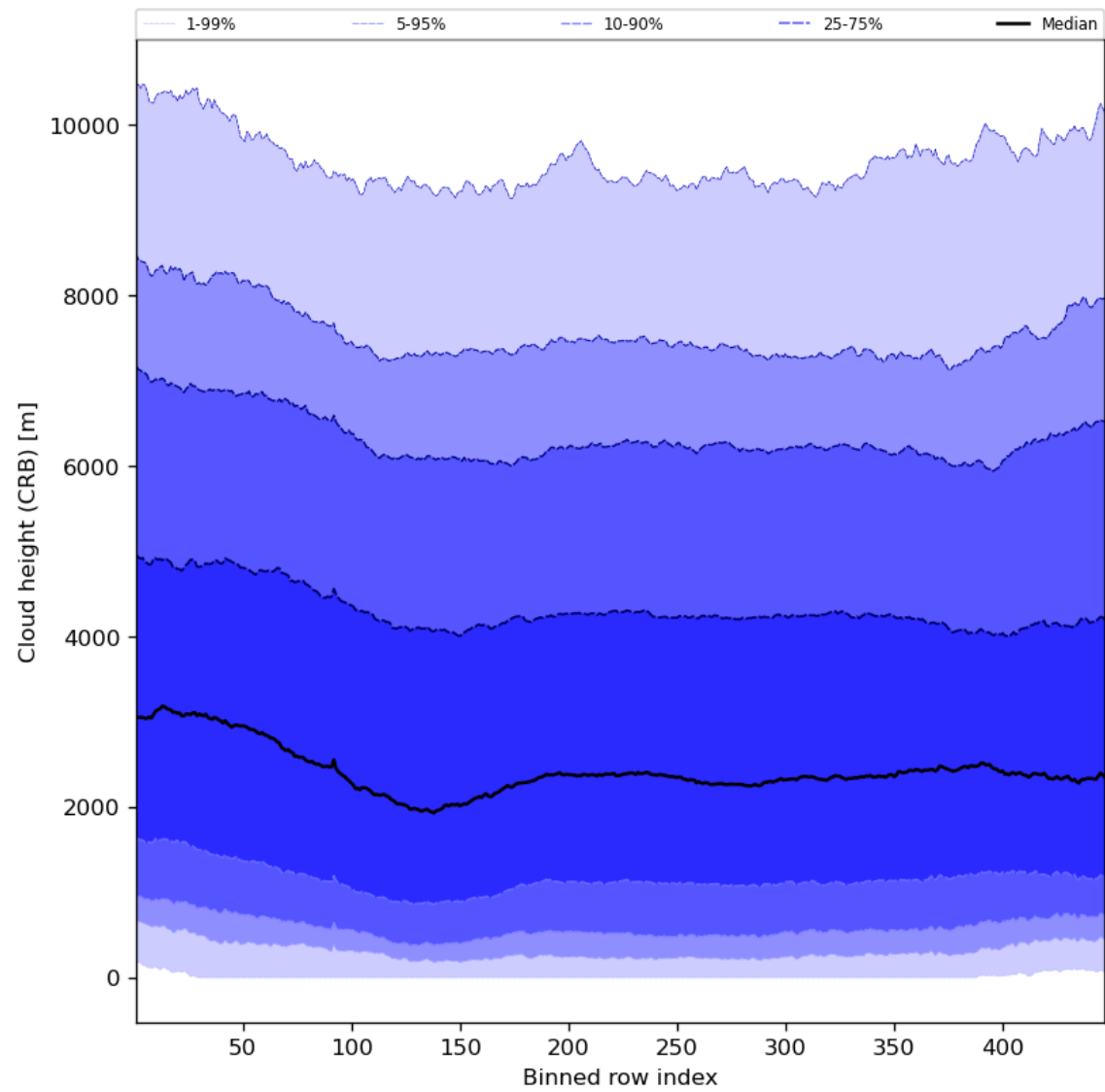
Figure 59: Along track statistics of “Cloud height (CRB)” for 2023-10-18 to 2023-10-20
