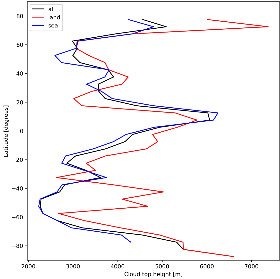
Figure 24: Zonal average of “Cloud top height” for 2023-10-18 to 2023-10-20.
