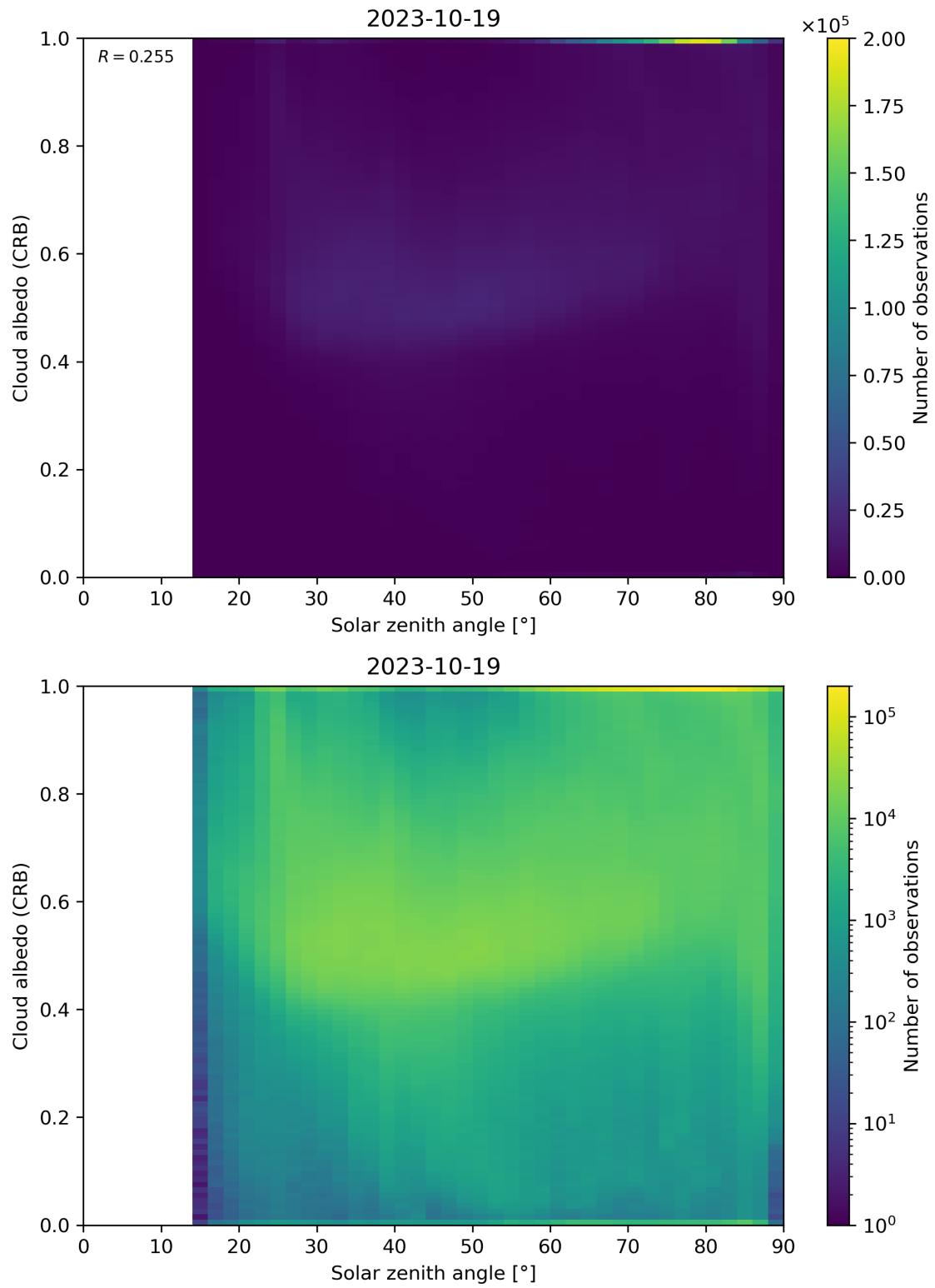
Figure 98: Scatter density plot of “Solar zenith angle” against “Cloud albedo (CRB)” for 2023-10-18 to 2023-10-20.
