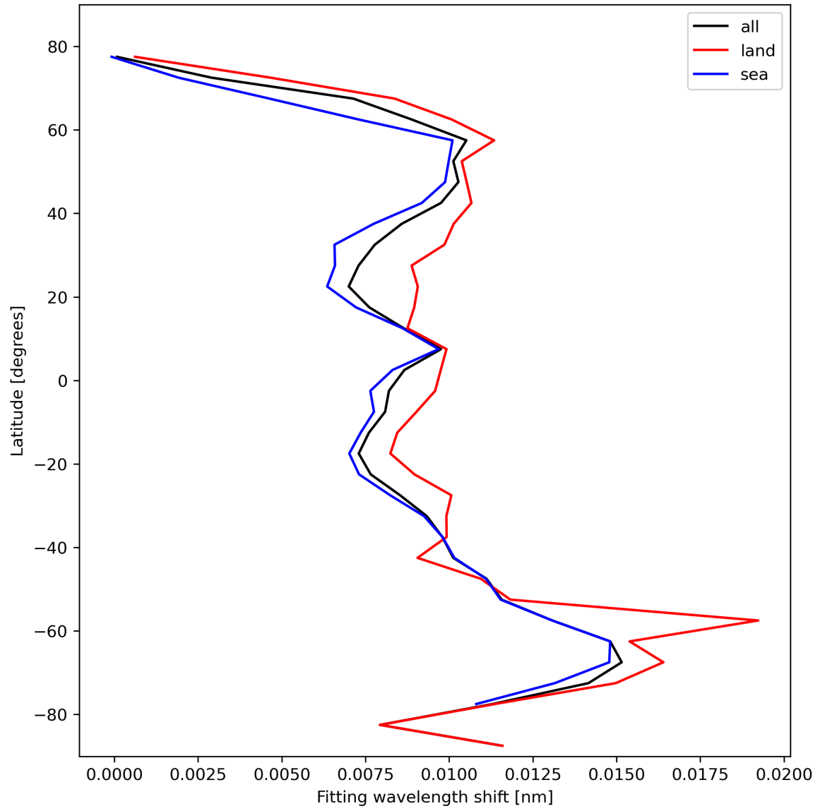
Figure 33: Zonal average of “Fitting wavelength shift” for 2023-10-18 to 2023-10-20.
