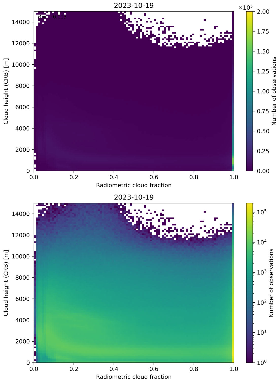
Figure 74: Scatter density plot of “Radiometric cloud fraction” against “Cloud height (CRB)” for 2023-10-18 to 2023-10-20.
