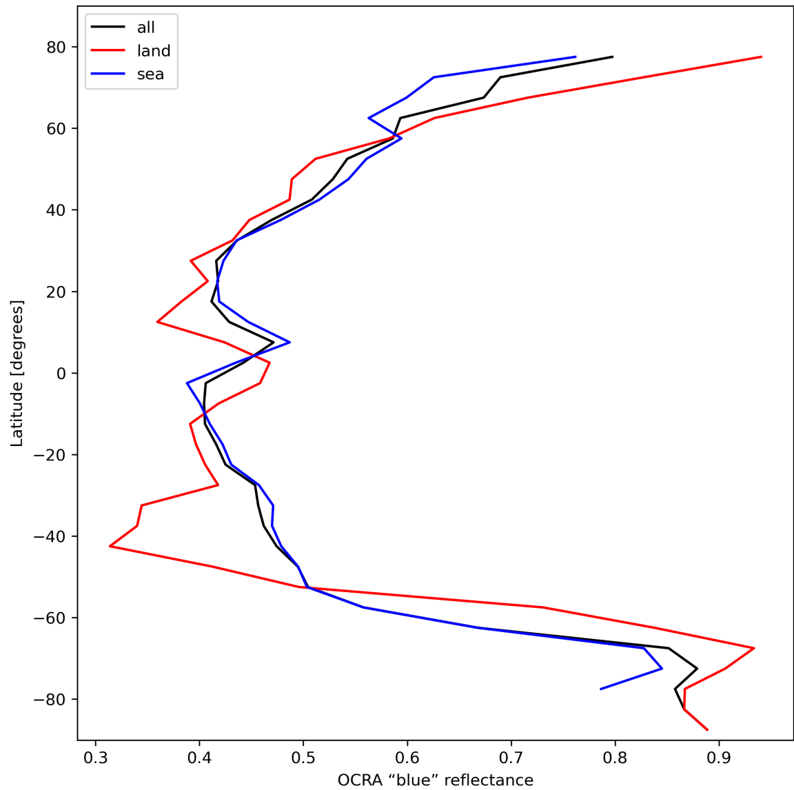
Figure 35: Zonal average of “OCRA “blue” reflectance” for 2023-10-18 to 2023-10-20.
