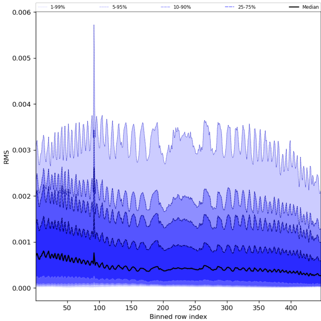
Figure 63: Along track statistics of “RMS” for 2023-10-18 to 2023-10-20
