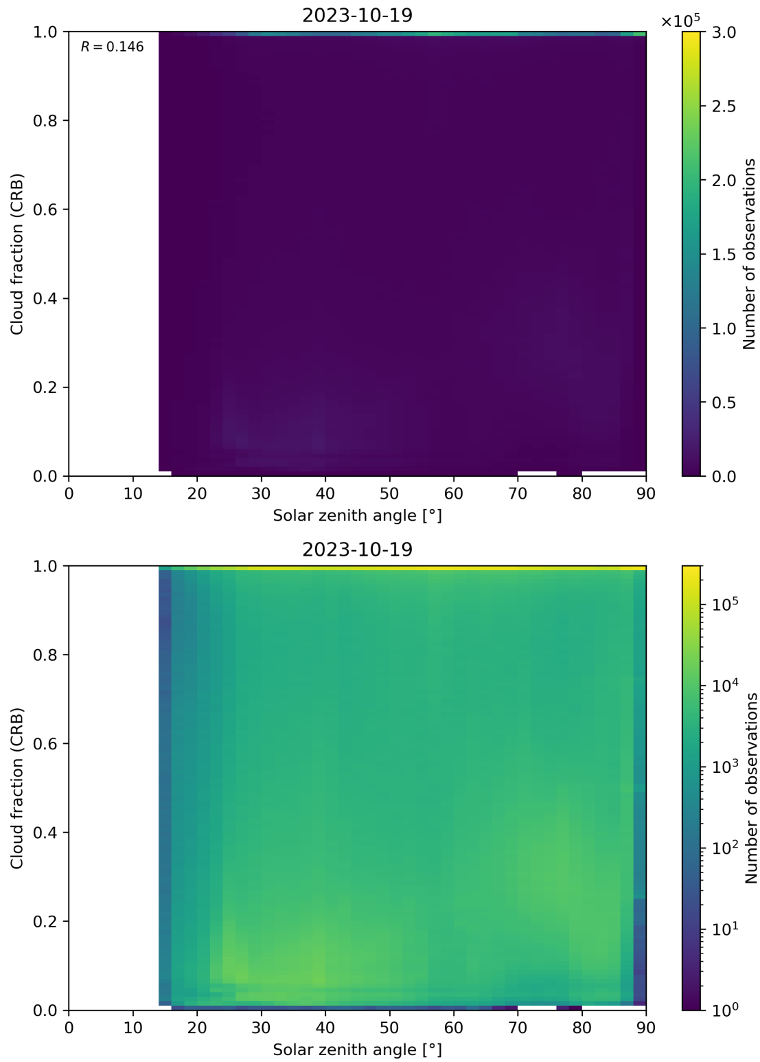
Figure 101: Scatter density plot of “Solar zenith angle” against “Cloud fraction (CRB)” for 2023-10-18 to 2023-10-20.
