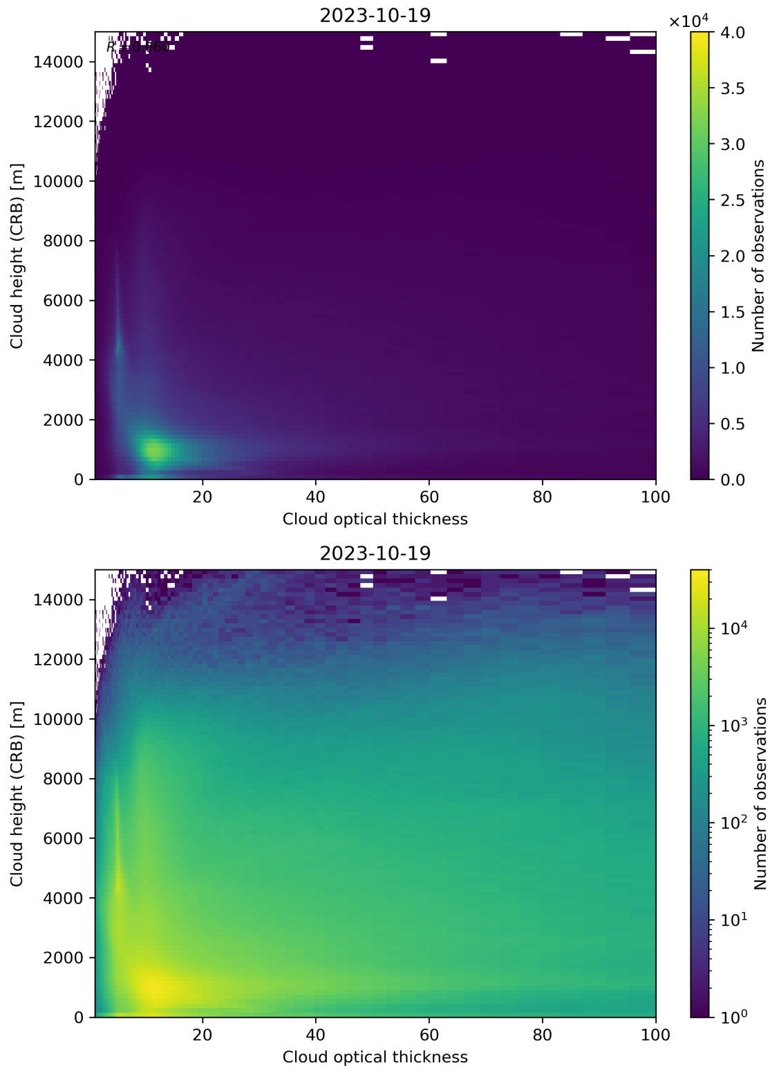
Figure 85: Scatter density plot of “Cloud optical thickness” against “Cloud height (CRB)” for 2023-10-18 to 2023-10-20.
