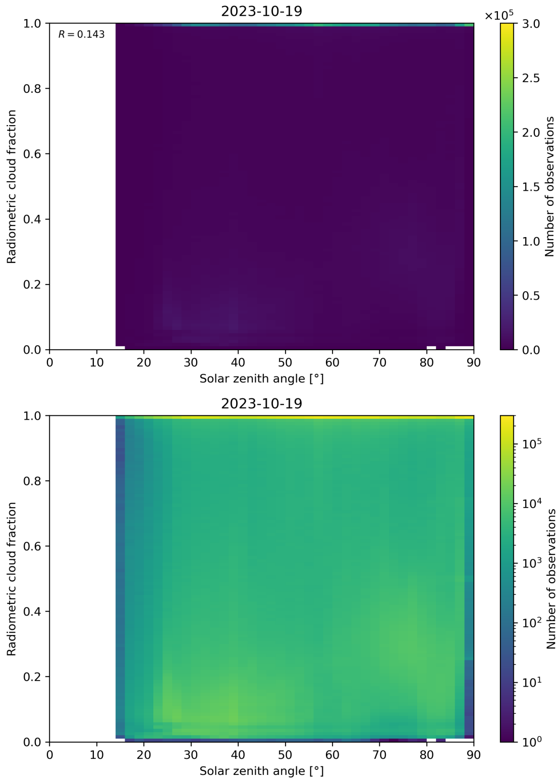
Figure 99: Scatter density plot of “Solar zenith angle” against “Radiometric cloud fraction” for 2023-10-18 to 2023-10-20.
