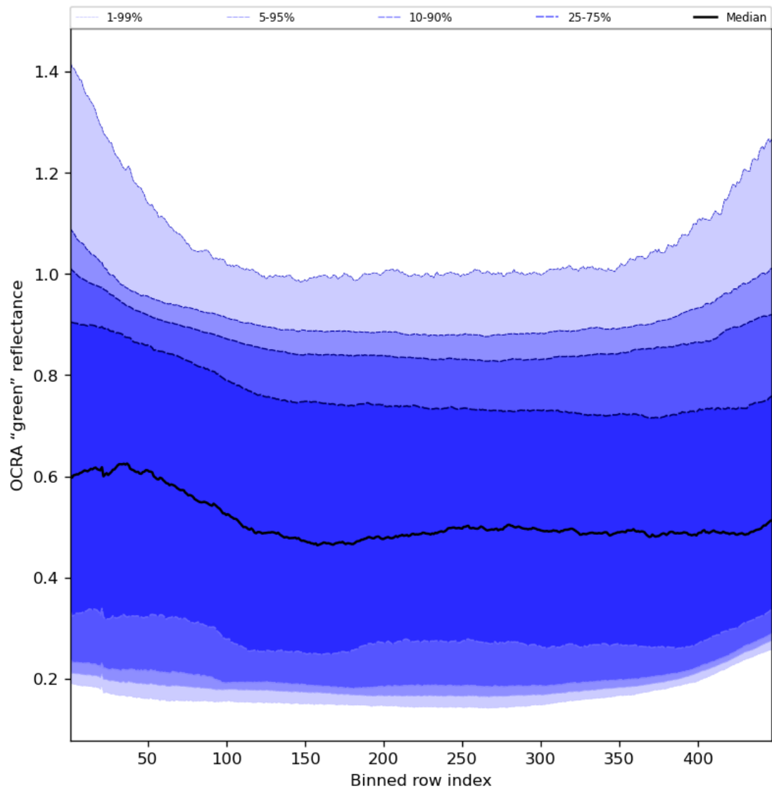
Figure 68: Along track statistics of “OCRA “green” reflectance” for 2023-10-18 to 2023-10-20
