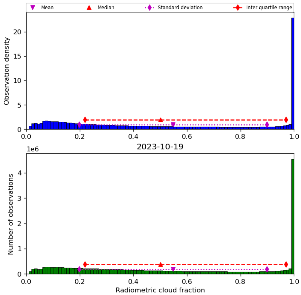
Figure 39: Histogram of “Radiometric cloud fraction” for 2023-10-18 to 2023-10-20
