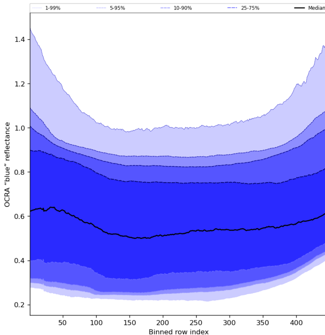
Figure 67: Along track statistics of “OCRA “blue” reflectance” for 2023-10-18 to 2023-10-20
