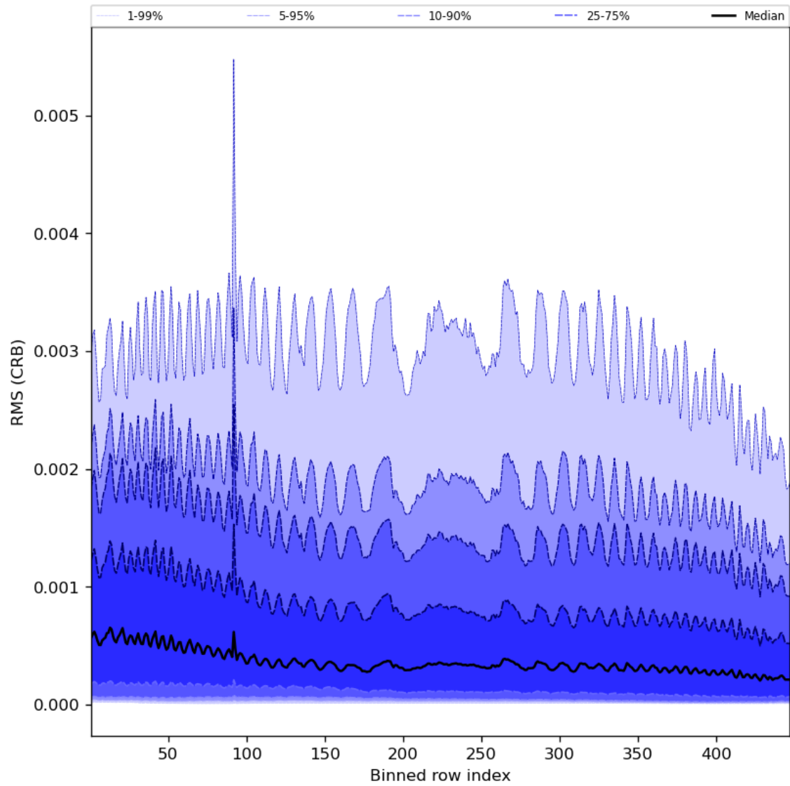
Figure 64: Along track statistics of “RMS (CRB)” for 2023-10-18 to 2023-10-20
