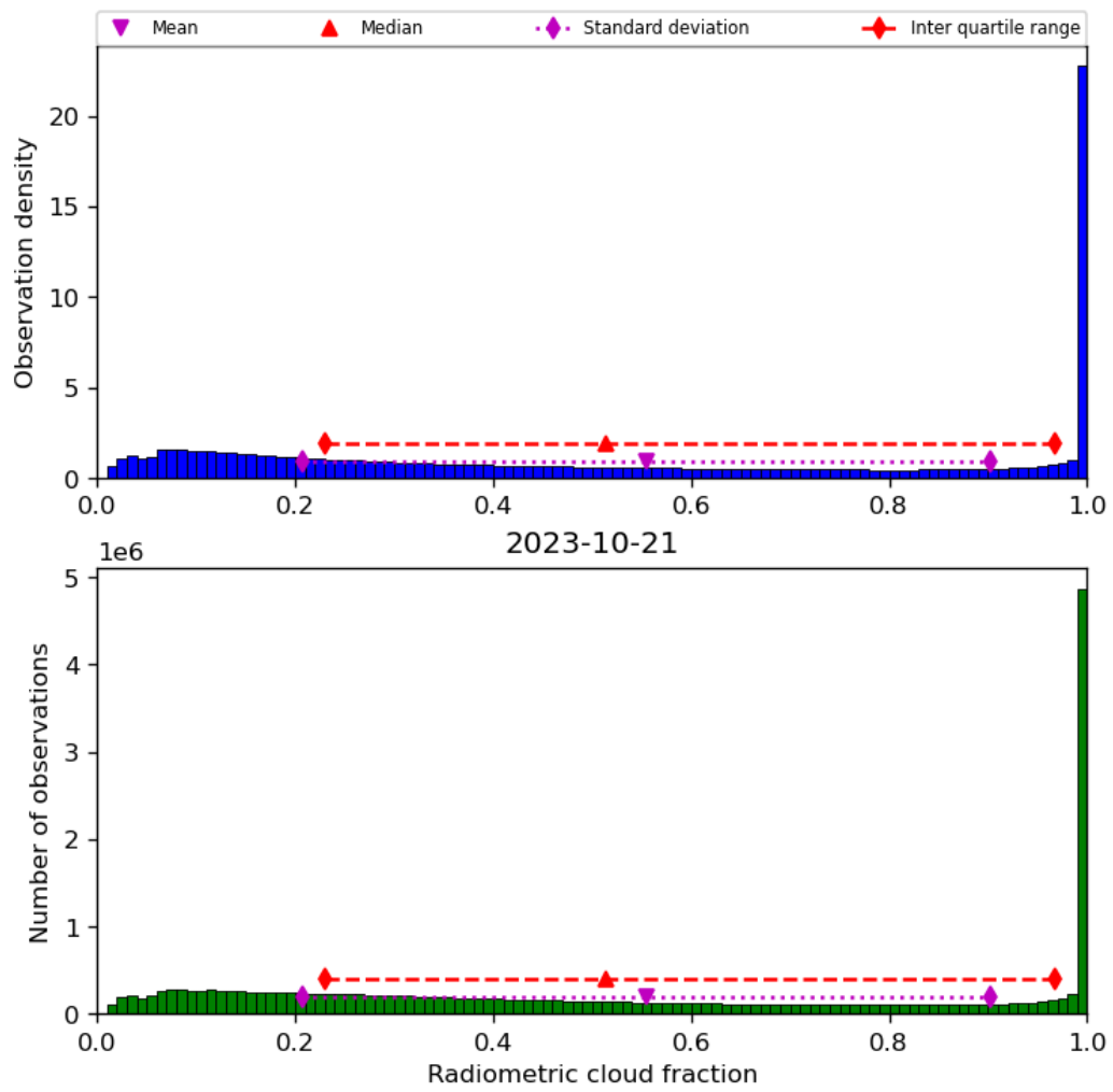
Figure 39: Histogram of “Radiometric cloud fraction” for 2023-10-20 to 2023-10-22
