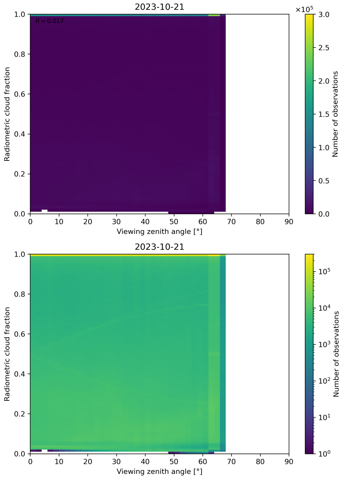
Figure 107: Scatter density plot of “Viewing zenith angle” against “Radiometric cloud fraction” for 2023-10-20 to 2023-10-22.
