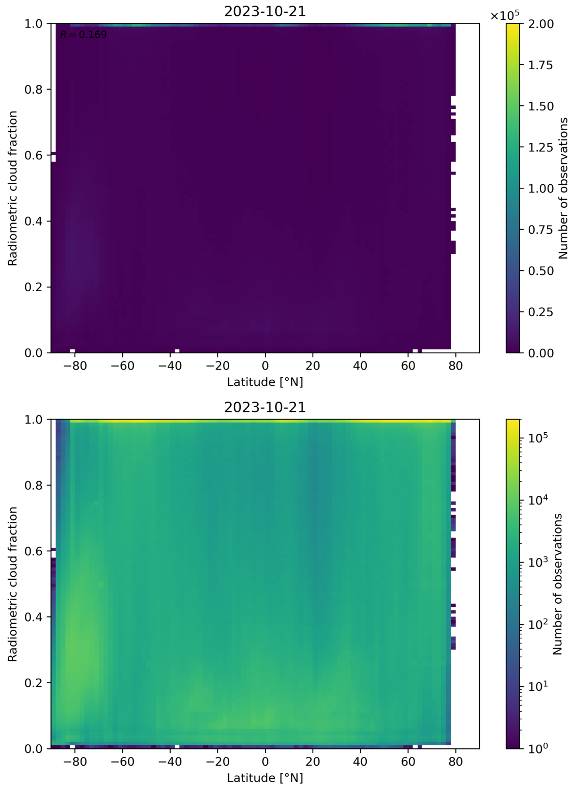
Figure 92: Scatter density plot of “Latitude” against “Radiometric cloud fraction” for 2023-10-20 to 2023-10-22.
