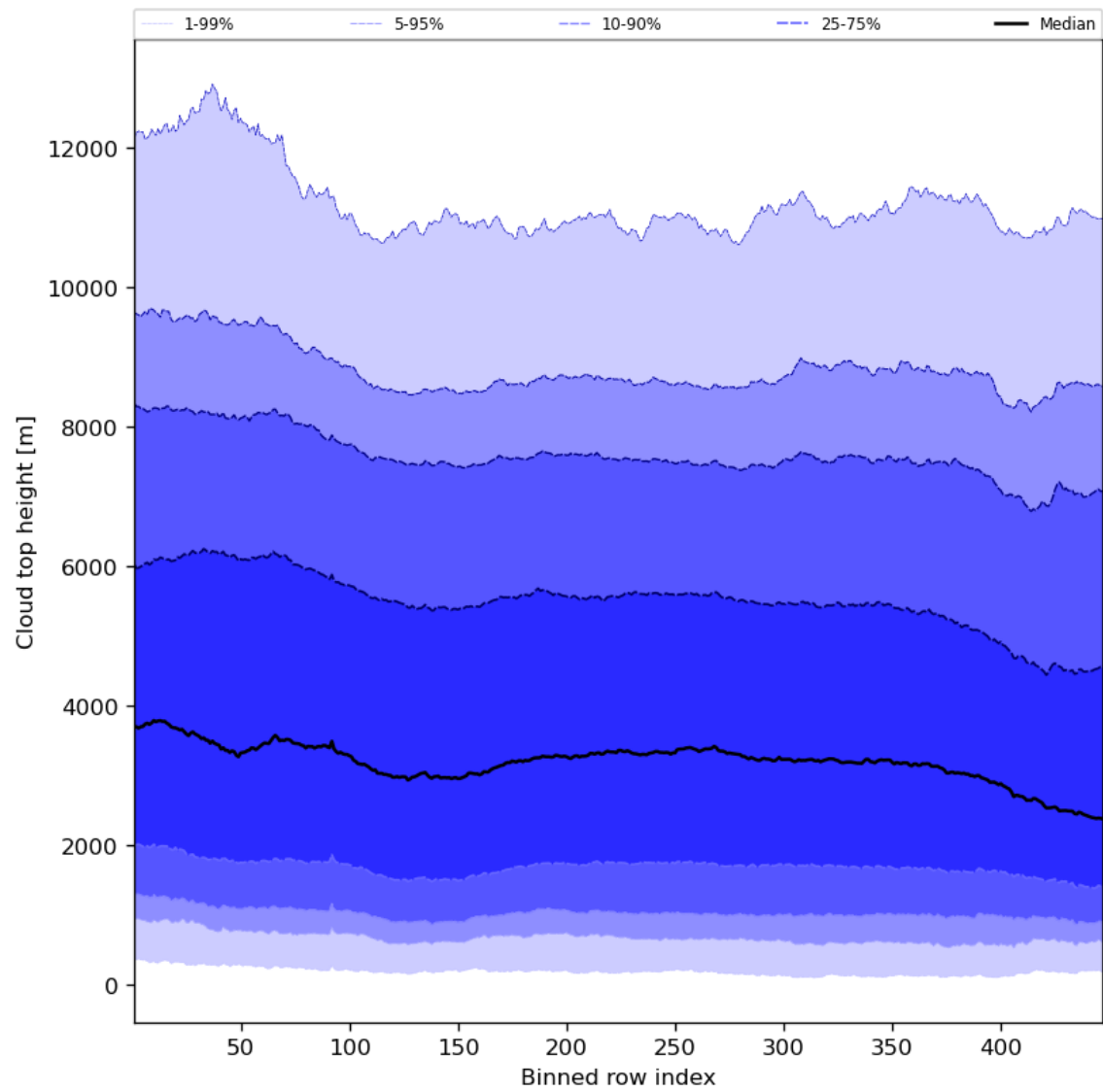
Figure 56: Along track statistics of “Cloud top height” for 2023-10-20 to 2023-10-22
