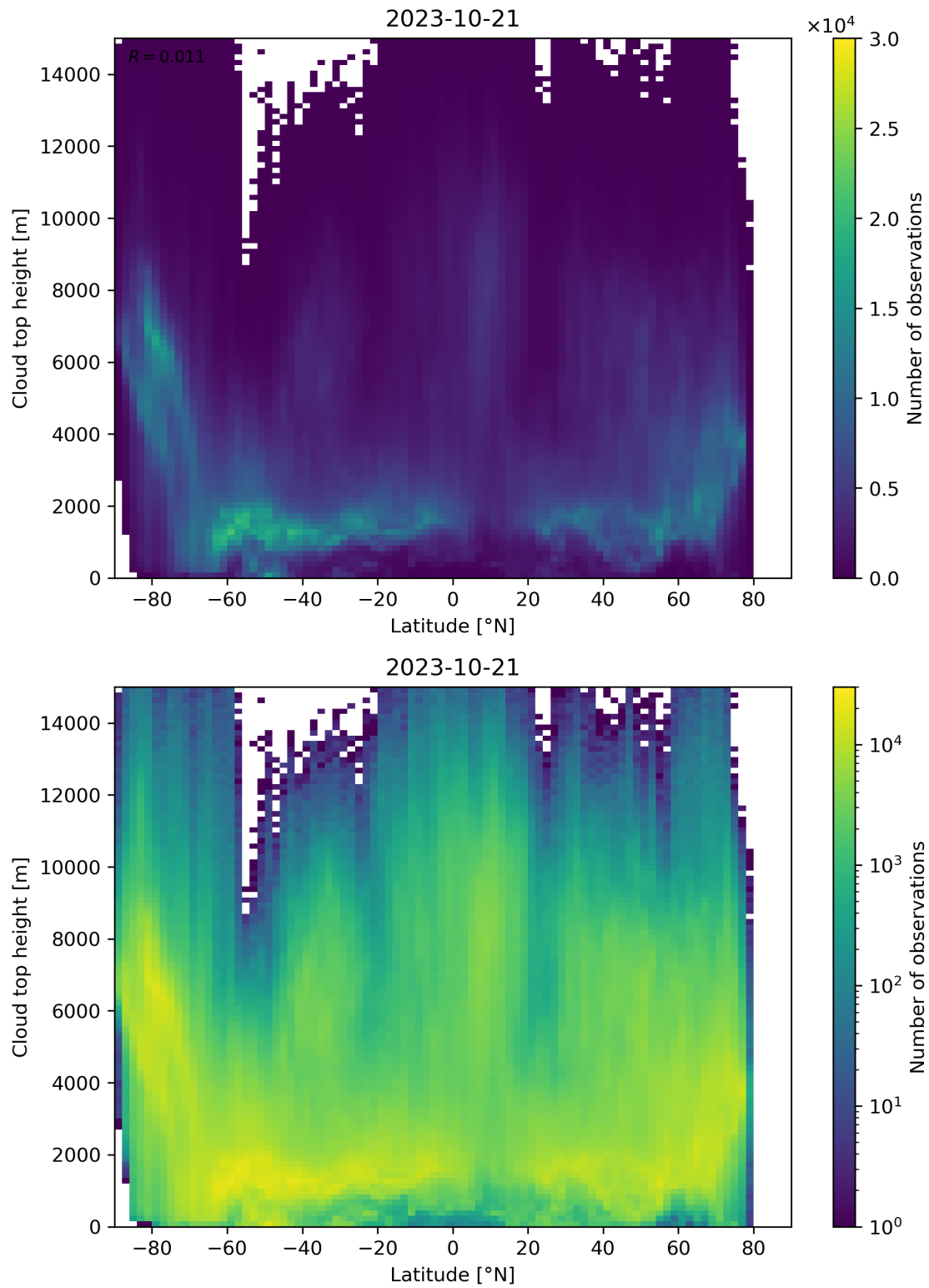
Figure 97: Scatter density plot of “Latitude” against “Cloud top height” for 2023-10-20 to 2023-10-22.
