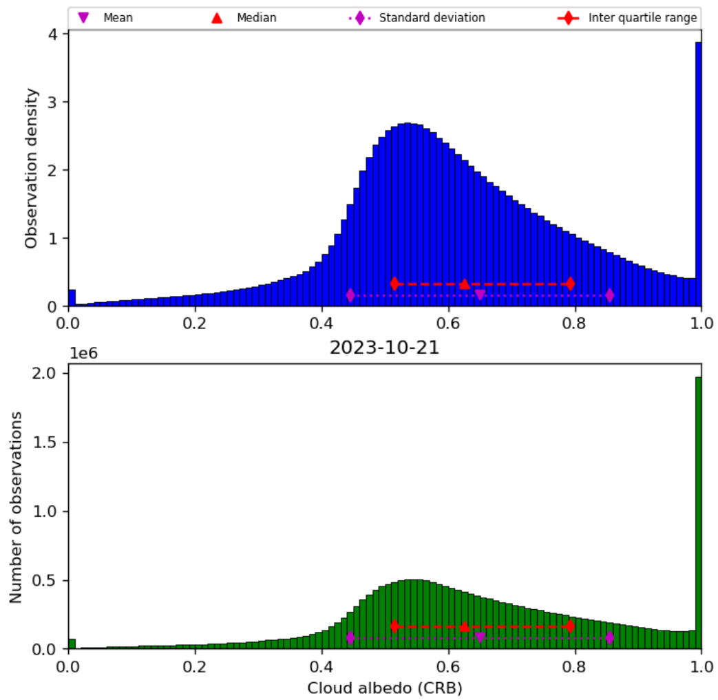
Figure 44: Histogram of “Cloud albedo (CRB)” for 2023-10-20 to 2023-10-22
