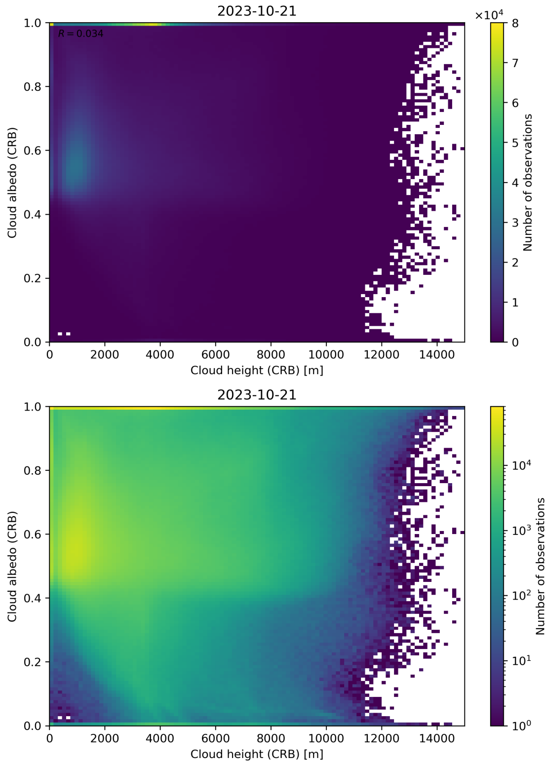
Figure 80: Scatter density plot of “Cloud height (CRB)” against “Cloud albedo (CRB)” for 2023-10-20 to 2023-10-22.
