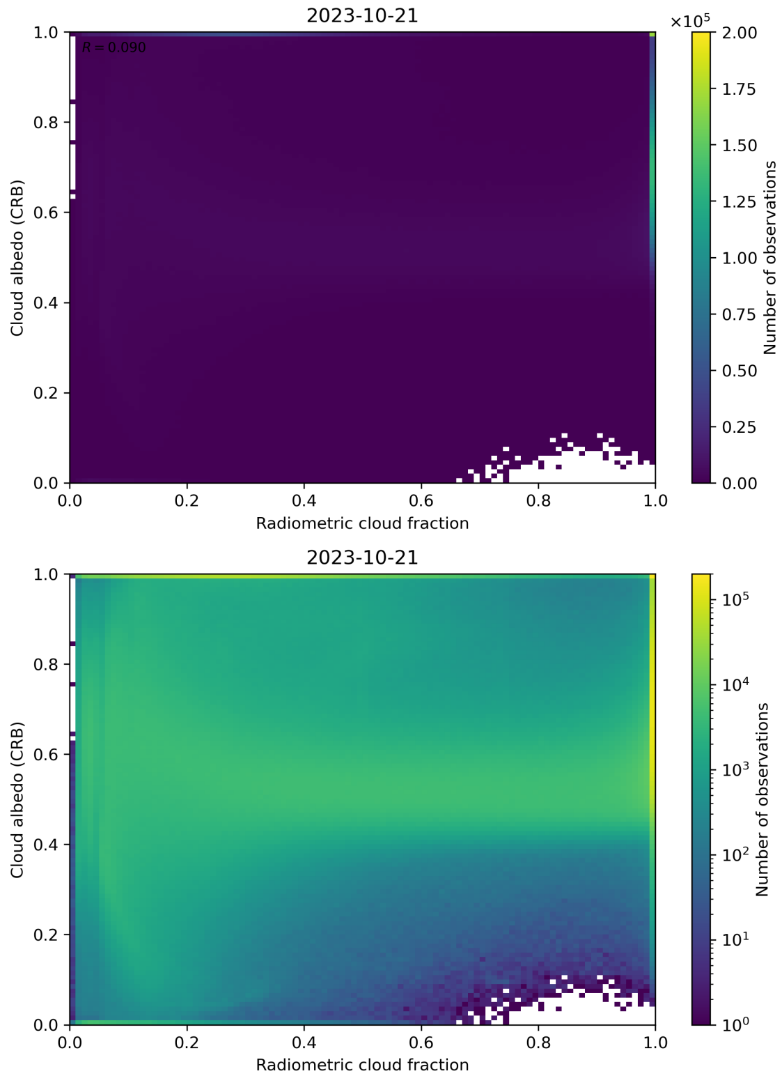
Figure 71: Scatter density plot of “Radiometric cloud fraction” against “Cloud albedo (CRB)” for 2023-10-20 to 2023-10-22.
