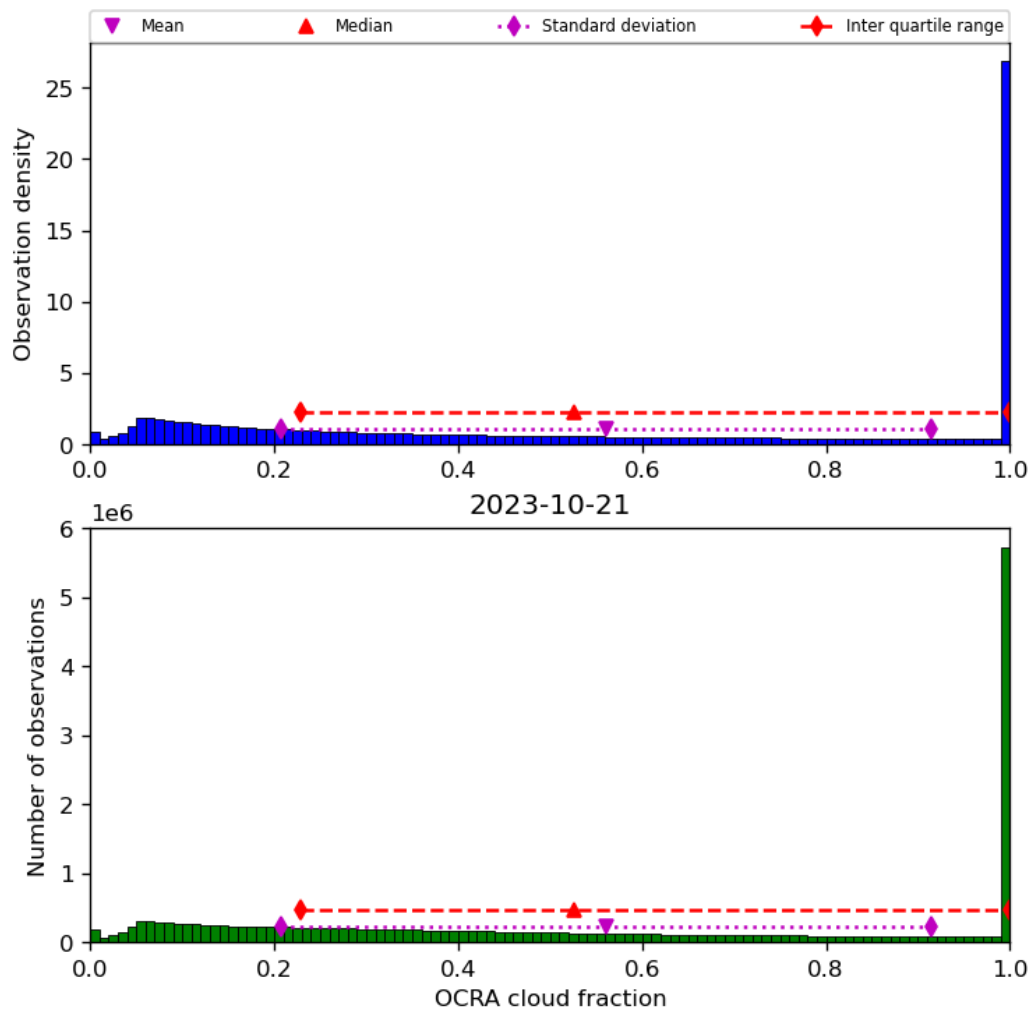
Figure 50: Histogram of “OCRA cloud fraction” for 2023-10-20 to 2023-10-22
