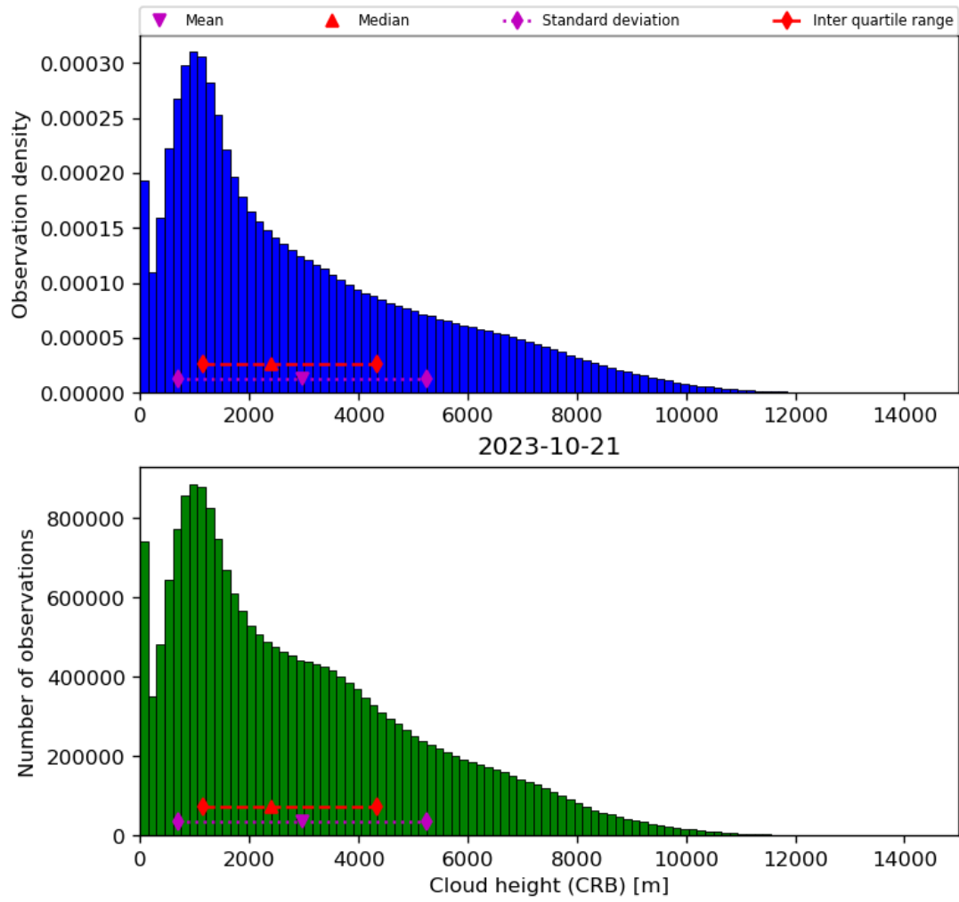
Figure 43: Histogram of “Cloud height (CRB)” for 2023-10-20 to 2023-10-22
