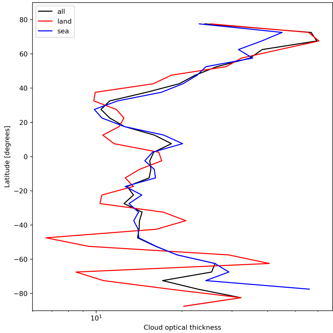
Figure 25: Zonal average of “Cloud optical thickness” for 2023-10-20 to 2023-10-22.
