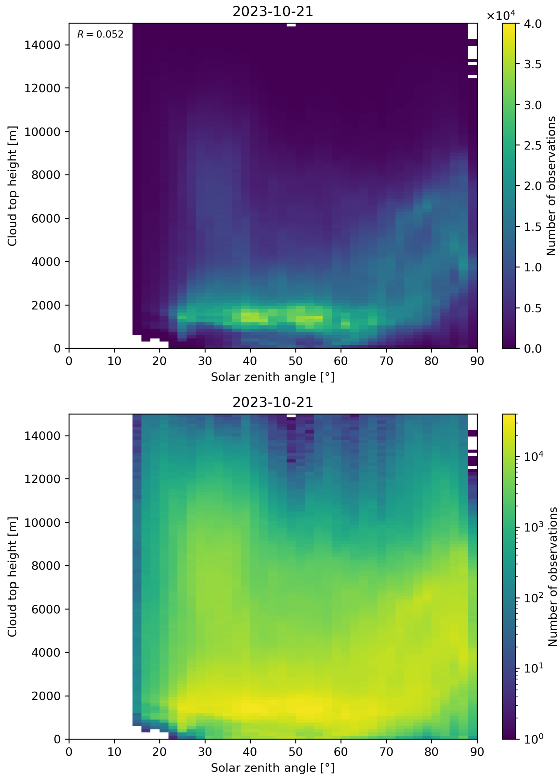
Figure 104: Scatter density plot of “Solar zenith angle” against “Cloud top height” for 2023-10-20 to 2023-10-22.
