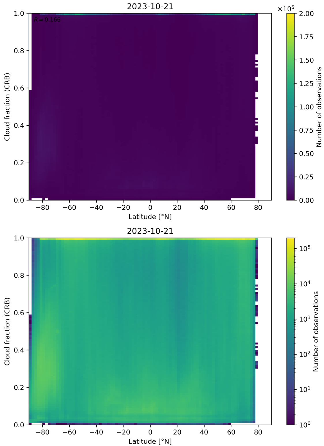
Figure 94: Scatter density plot of “Latitude” against “Cloud fraction (CRB)” for 2023-10-20 to 2023-10-22.
