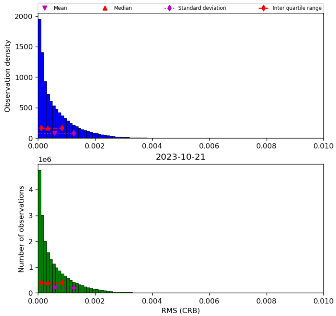
Figure 48: Histogram of “RMS (CRB)” for 2023-10-20 to 2023-10-22
