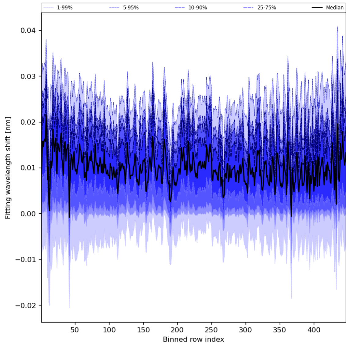
Figure 65: Along track statistics of “Fitting wavelength shift” for 2023-10-20 to 2023-10-22
