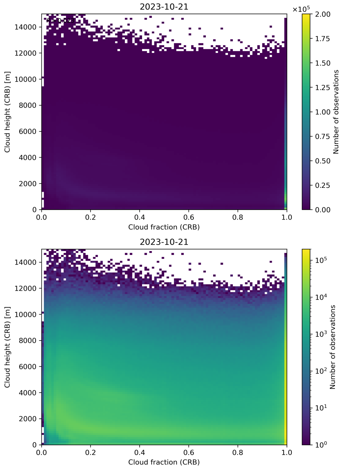
Figure 79: Scatter density plot of “Cloud fraction (CRB)” against “Cloud height (CRB)” for 2023-10-20 to 2023-10-22.
