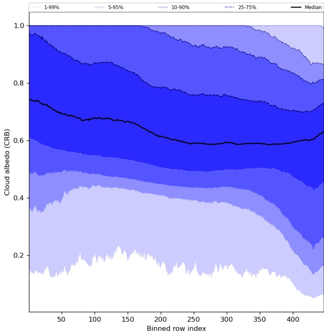
Figure 60: Along track statistics of “Cloud albedo (CRB)” for 2023-10-20 to 2023-10-22
