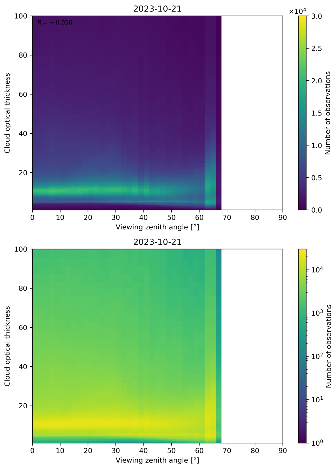
Figure 111: Scatter density plot of “Viewing zenith angle” against “Cloud optical thickness” for 2023-10-20 to 2023-10-22.
