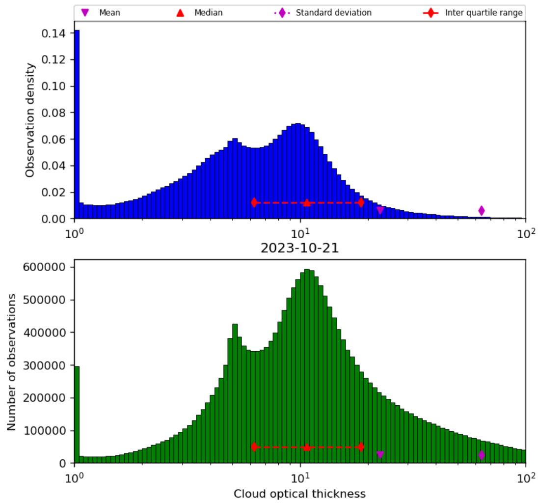
Figure 41: Histogram of “Cloud optical thickness” for 2023-10-20 to 2023-10-22
