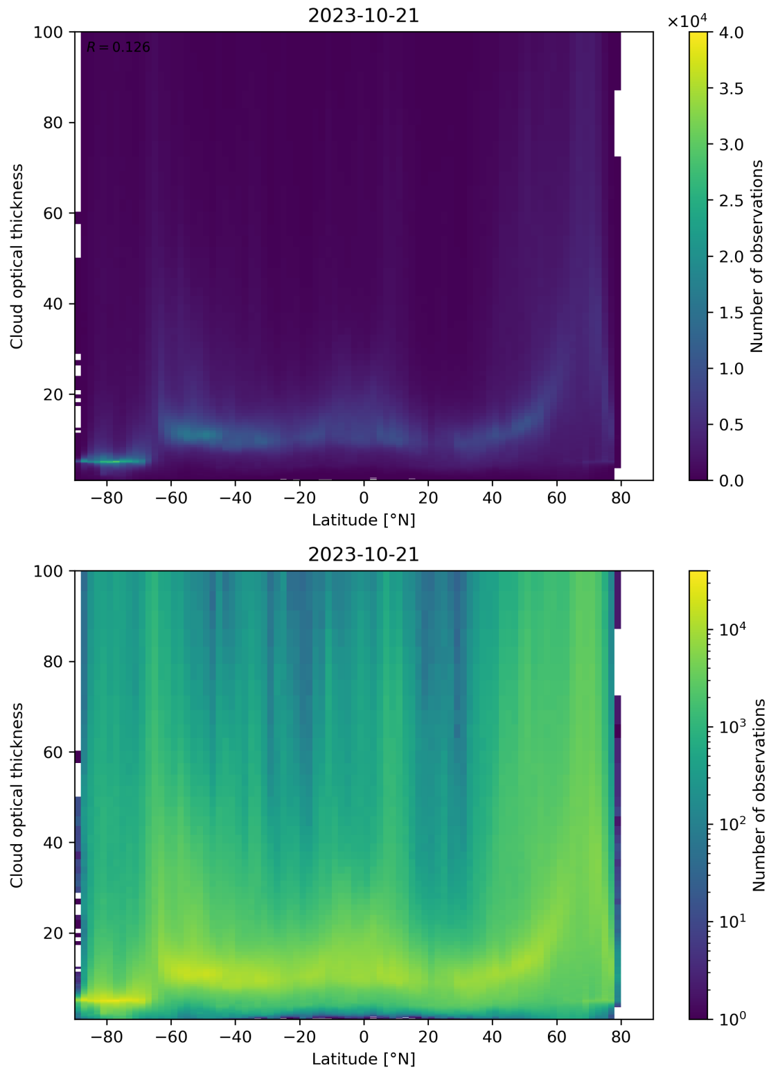
Figure 96: Scatter density plot of “Latitude” against “Cloud optical thickness” for 2023-10-20 to 2023-10-22.
