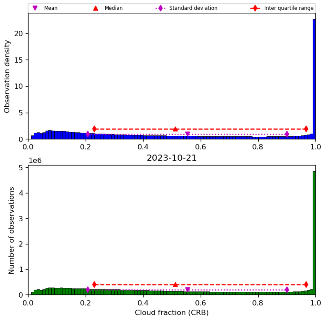
Figure 42: Histogram of “Cloud fraction (CRB)” for 2023-10-20 to 2023-10-22
