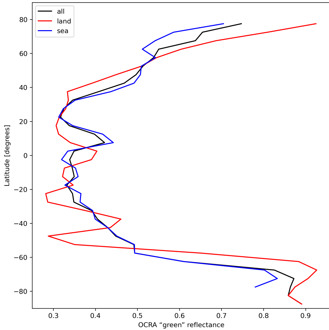
Figure 36: Zonal average of “OCRA “green” reflectance” for 2023-10-20 to 2023-10-22.
