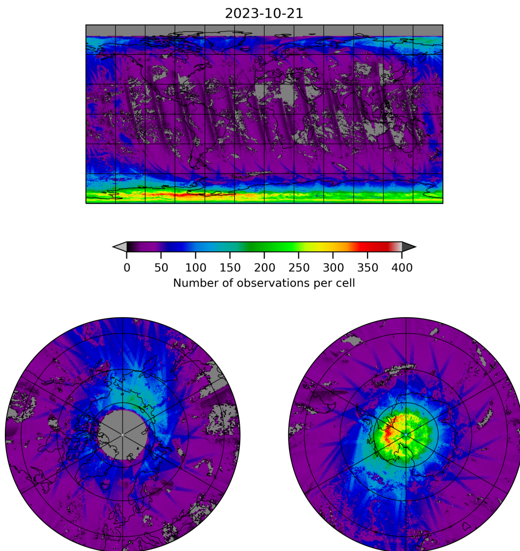
Figure 21: Map of the number of observations for 2023-10-20 to 2023-10-22
