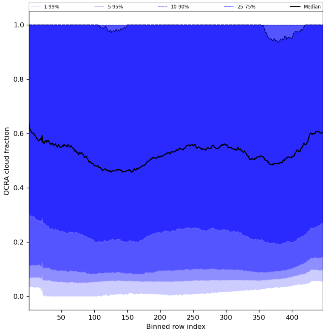
Figure 66: Along track statistics of “OCRA cloud fraction” for 2023-10-20 to 2023-10-22
