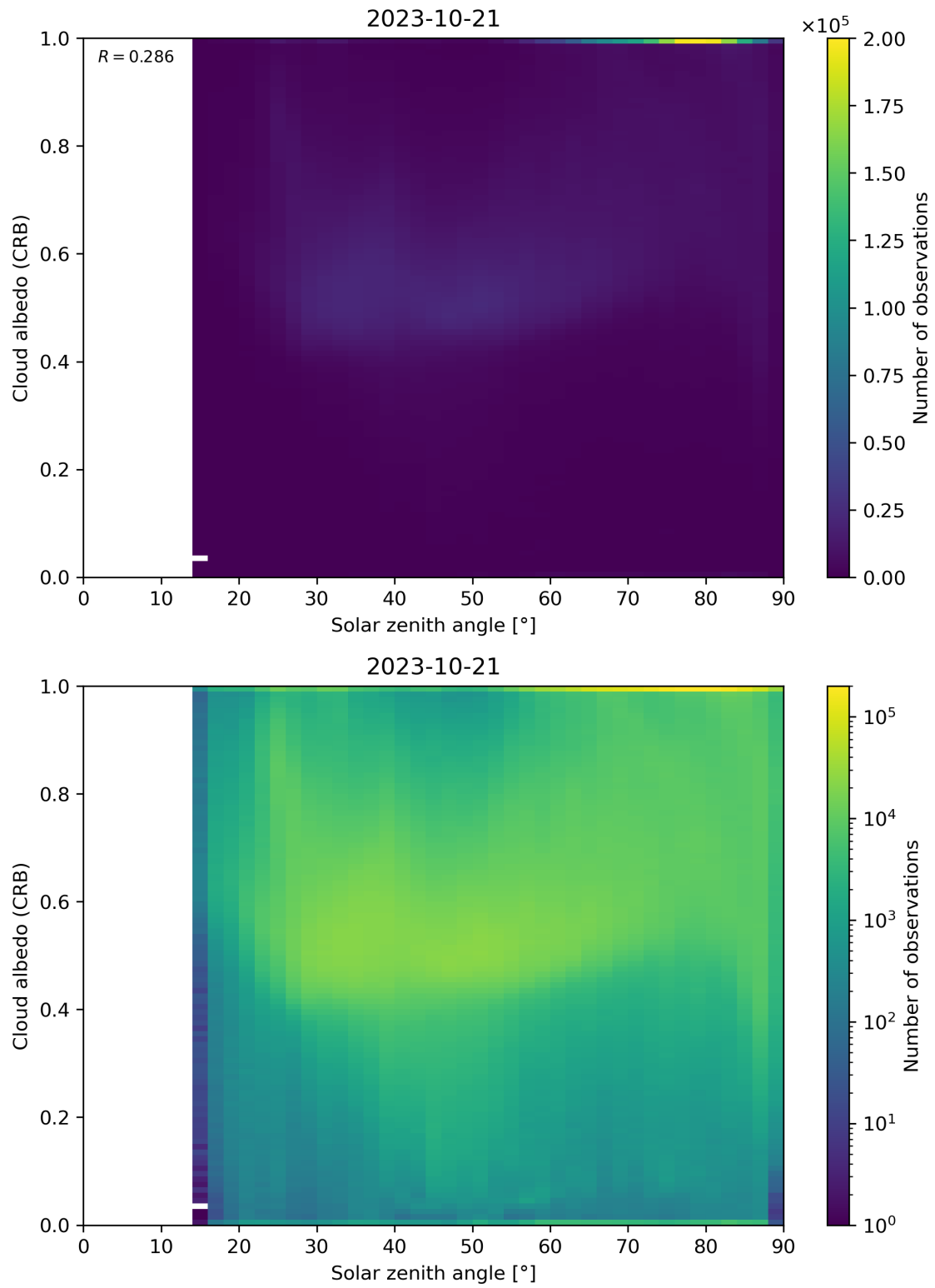
Figure 98: Scatter density plot of “Solar zenith angle” against “Cloud albedo (CRB)” for 2023-10-20 to 2023-10-22.
