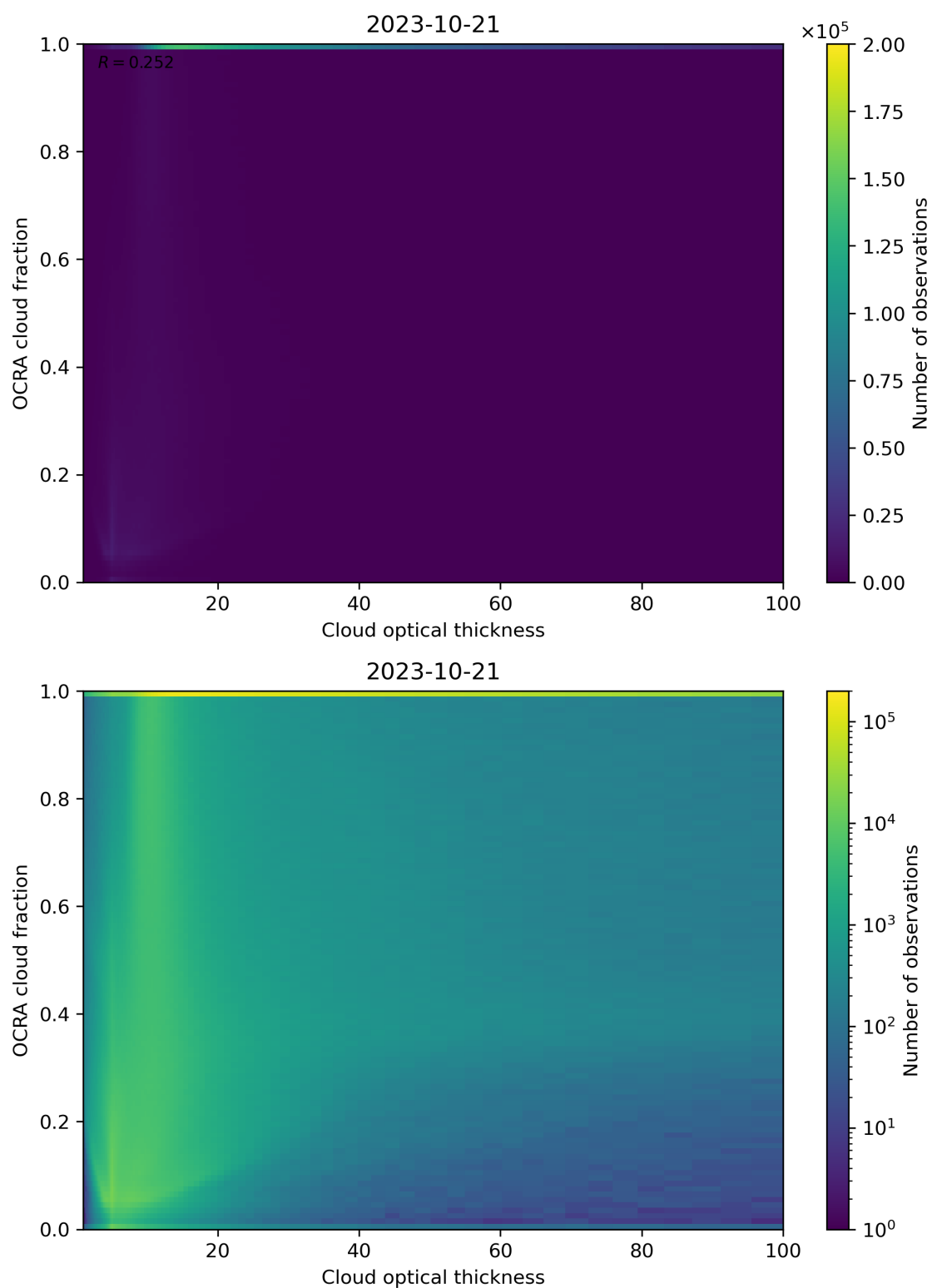
Figure 83: Scatter density plot of “Cloud optical thickness” against “OCRA cloud fraction” for 2023-10-20 to 2023-10-22.
