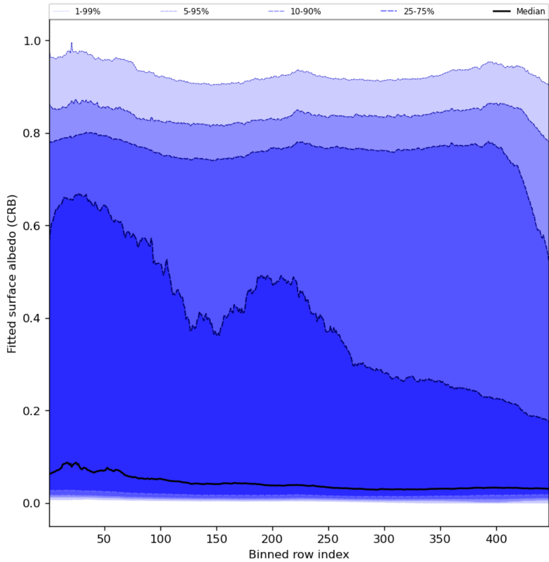
Figure 62: Along track statistics of “Fitted surface albedo (CRB)” for 2023-10-20 to 2023-10-22
