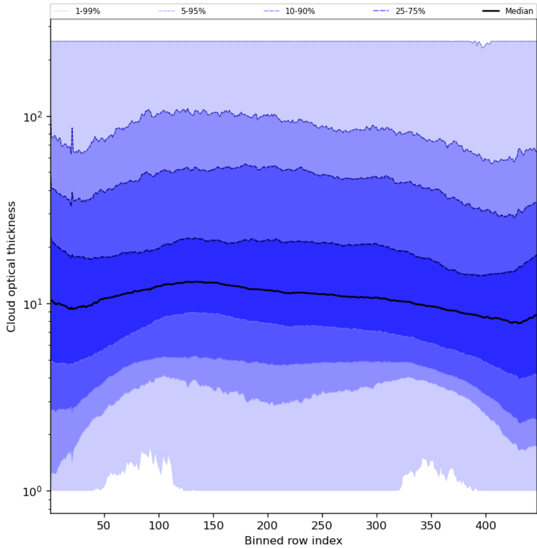
Figure 57: Along track statistics of “Cloud optical thickness” for 2023-10-20 to 2023-10-22
