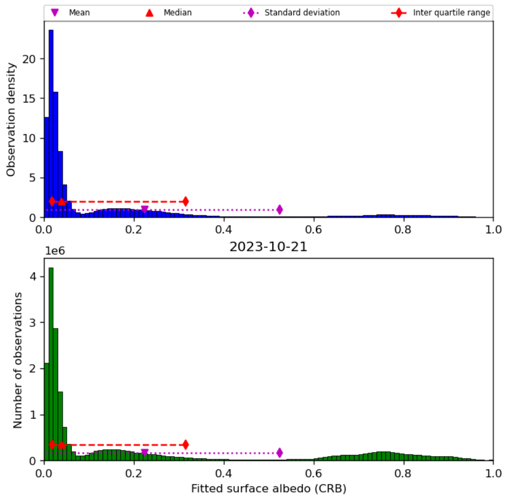
Figure 46: Histogram of “Fitted surface albedo (CRB)” for 2023-10-20 to 2023-10-22
