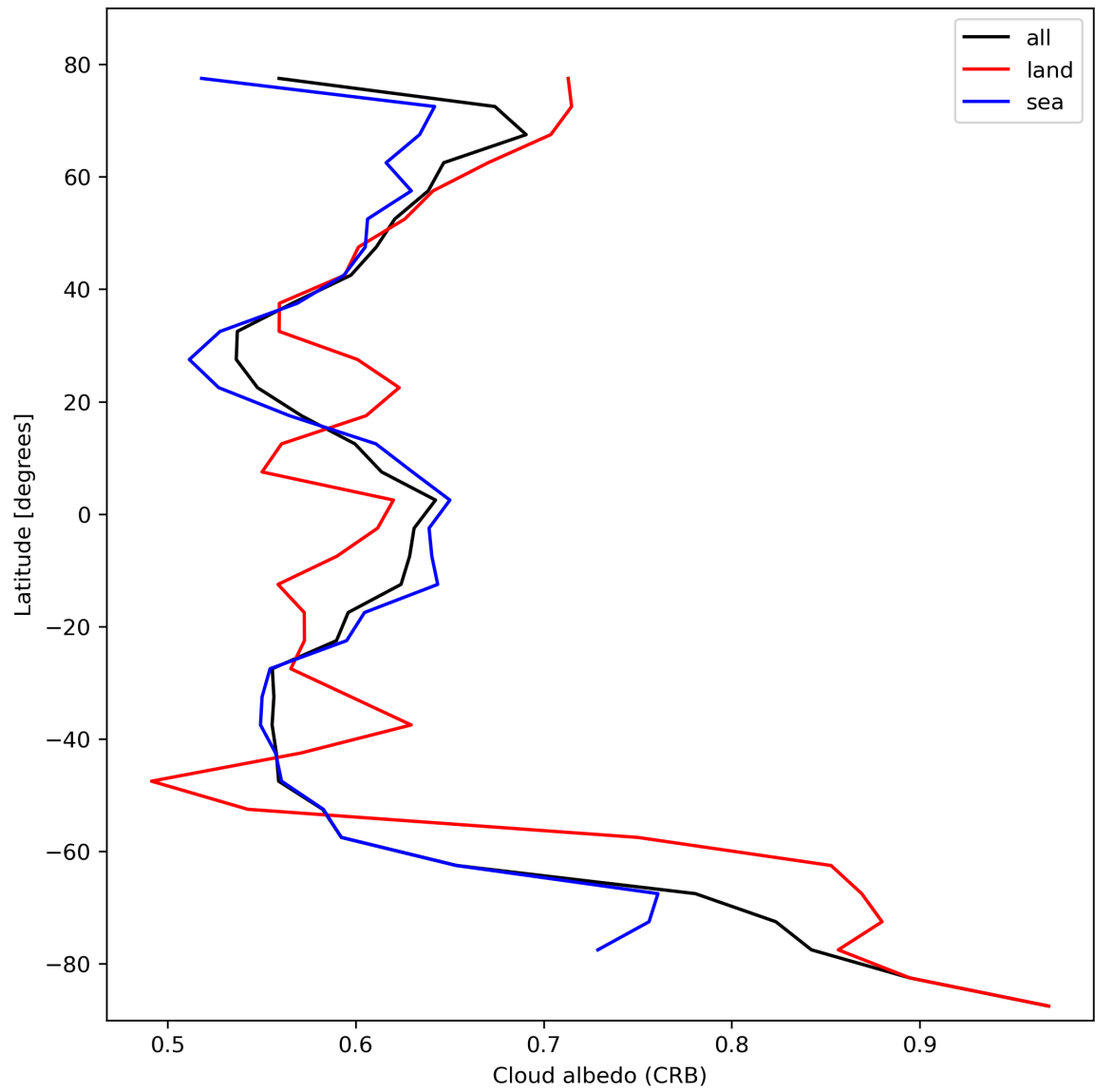
Figure 28: Zonal average of “Cloud albedo (CRB)” for 2023-10-20 to 2023-10-22.
