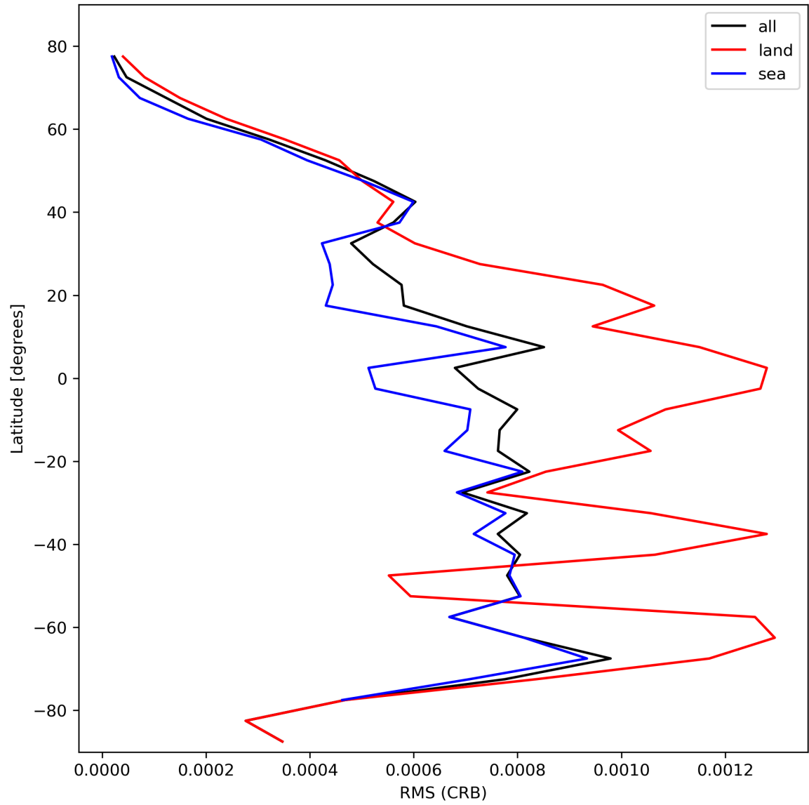
Figure 32: Zonal average of “RMS (CRB)” for 2023-10-20 to 2023-10-22.
