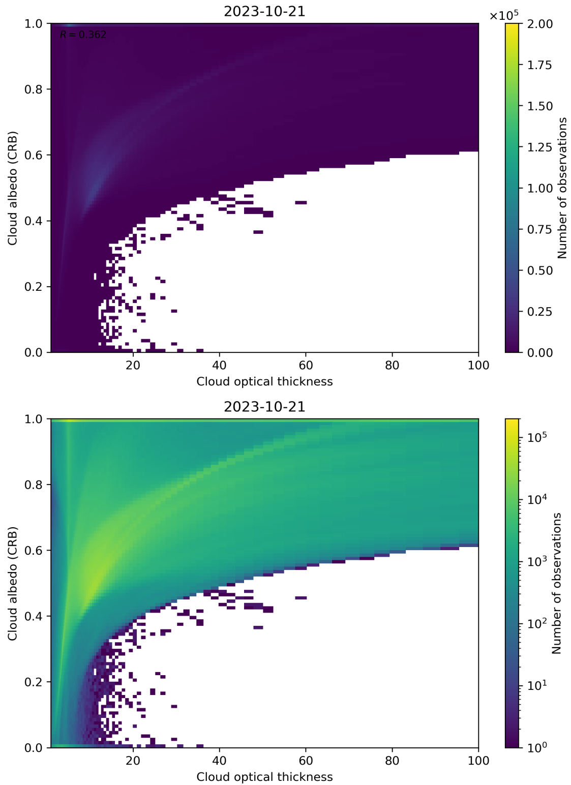
Figure 82: Scatter density plot of “Cloud optical thickness” against “Cloud albedo (CRB)” for 2023-10-20 to 2023-10-22.
