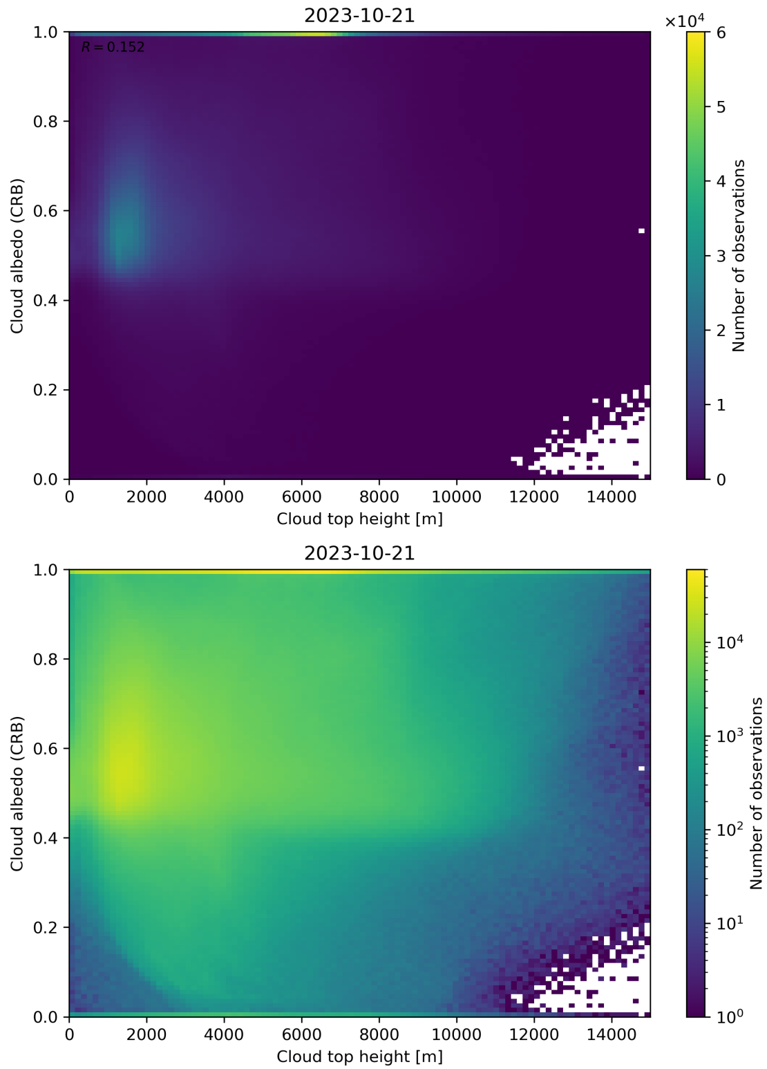
Figure 86: Scatter density plot of “Cloud top height” against “Cloud albedo (CRB)” for 2023-10-20 to 2023-10-22.
