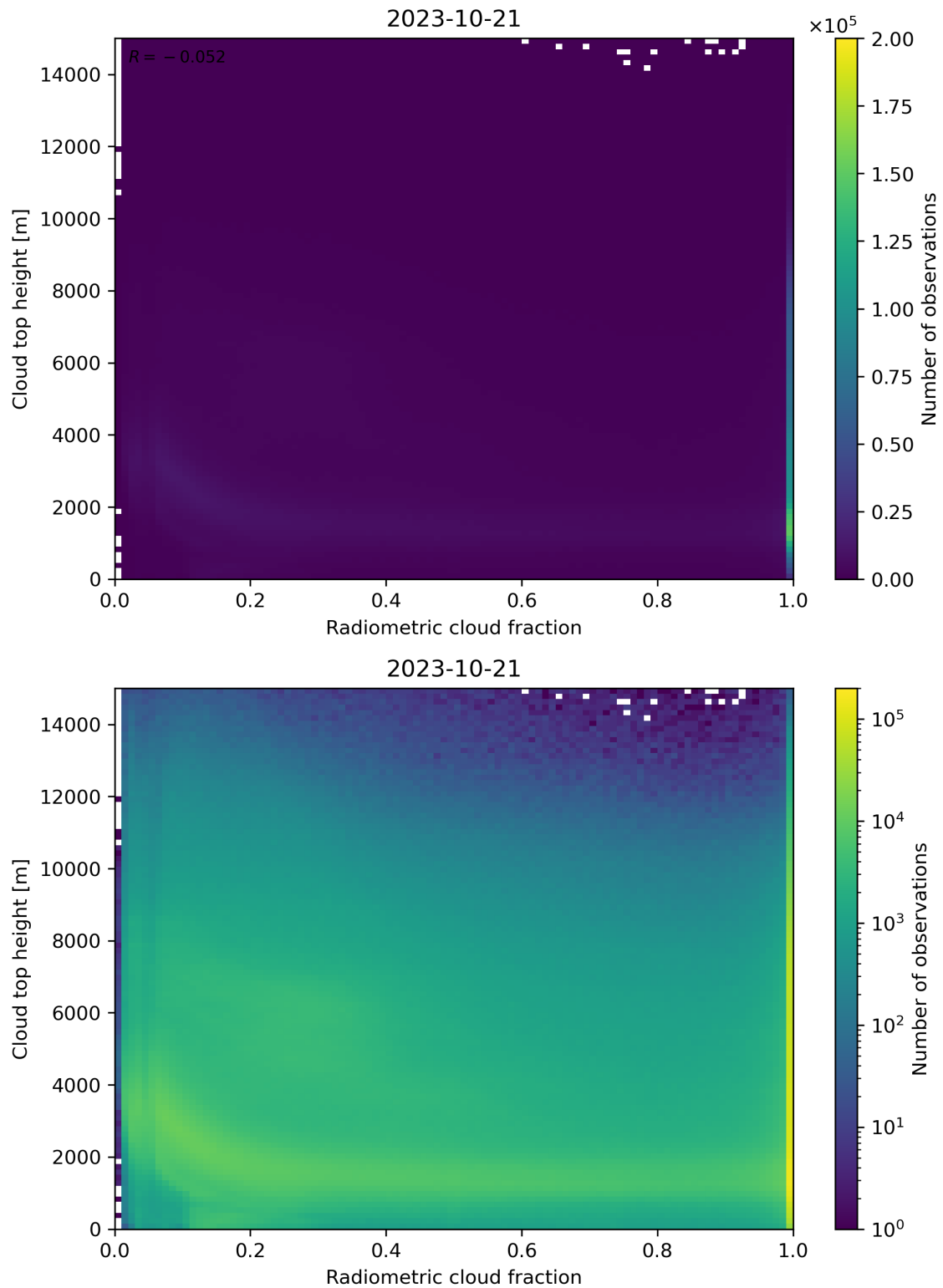
Figure 76: Scatter density plot of “Radiometric cloud fraction” against “Cloud top height” for 2023-10-20 to 2023-10-22.
