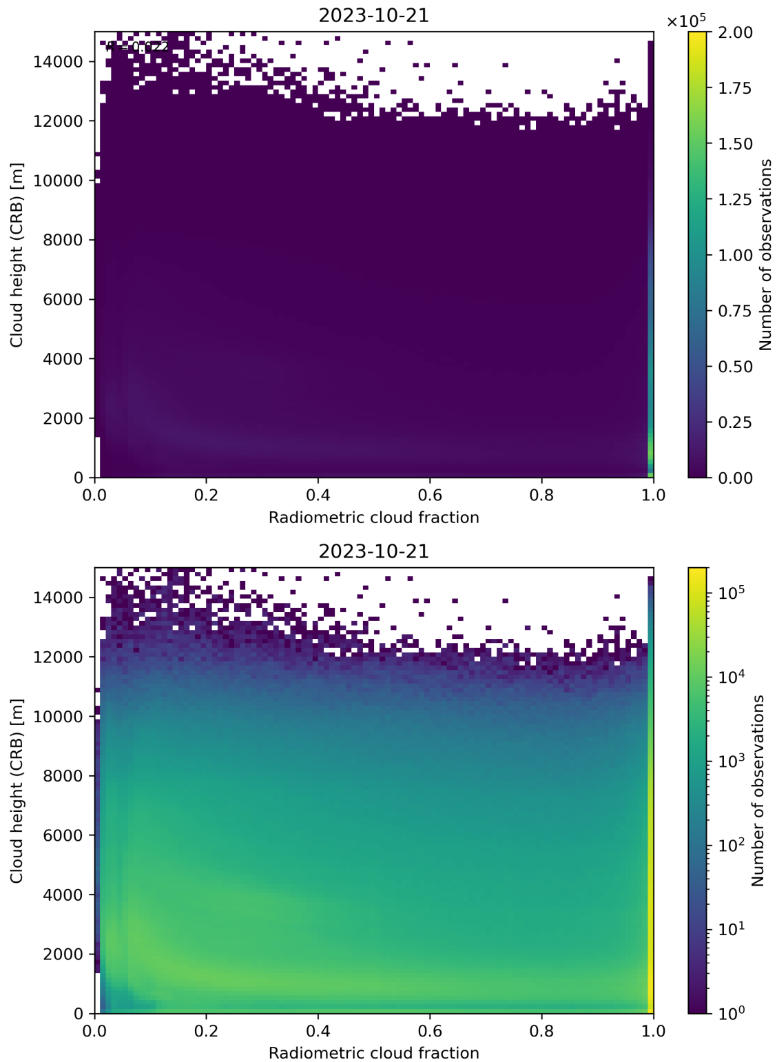
Figure 74: Scatter density plot of “Radiometric cloud fraction” against “Cloud height (CRB)” for 2023-10-20 to 2023-10-22.
