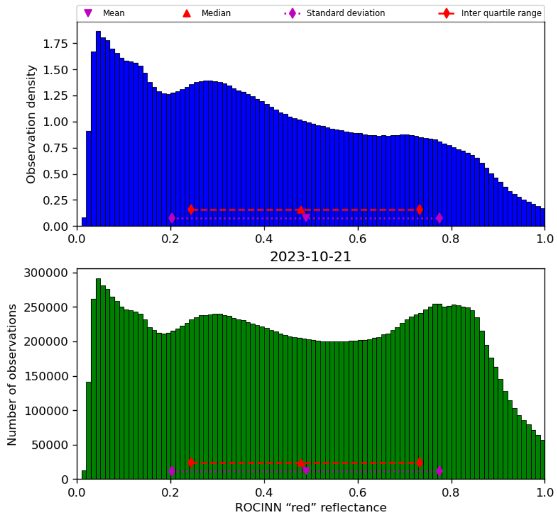
Figure 53: Histogram of “ROCINN “red” reflectance” for 2023-10-20 to 2023-10-22
