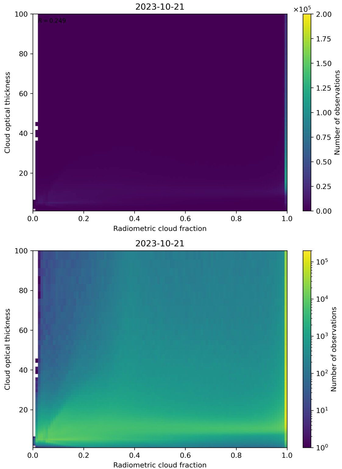
Figure 75: Scatter density plot of “Radiometric cloud fraction” against “Cloud optical thickness” for 2023-10-20 to 2023-10-22.
