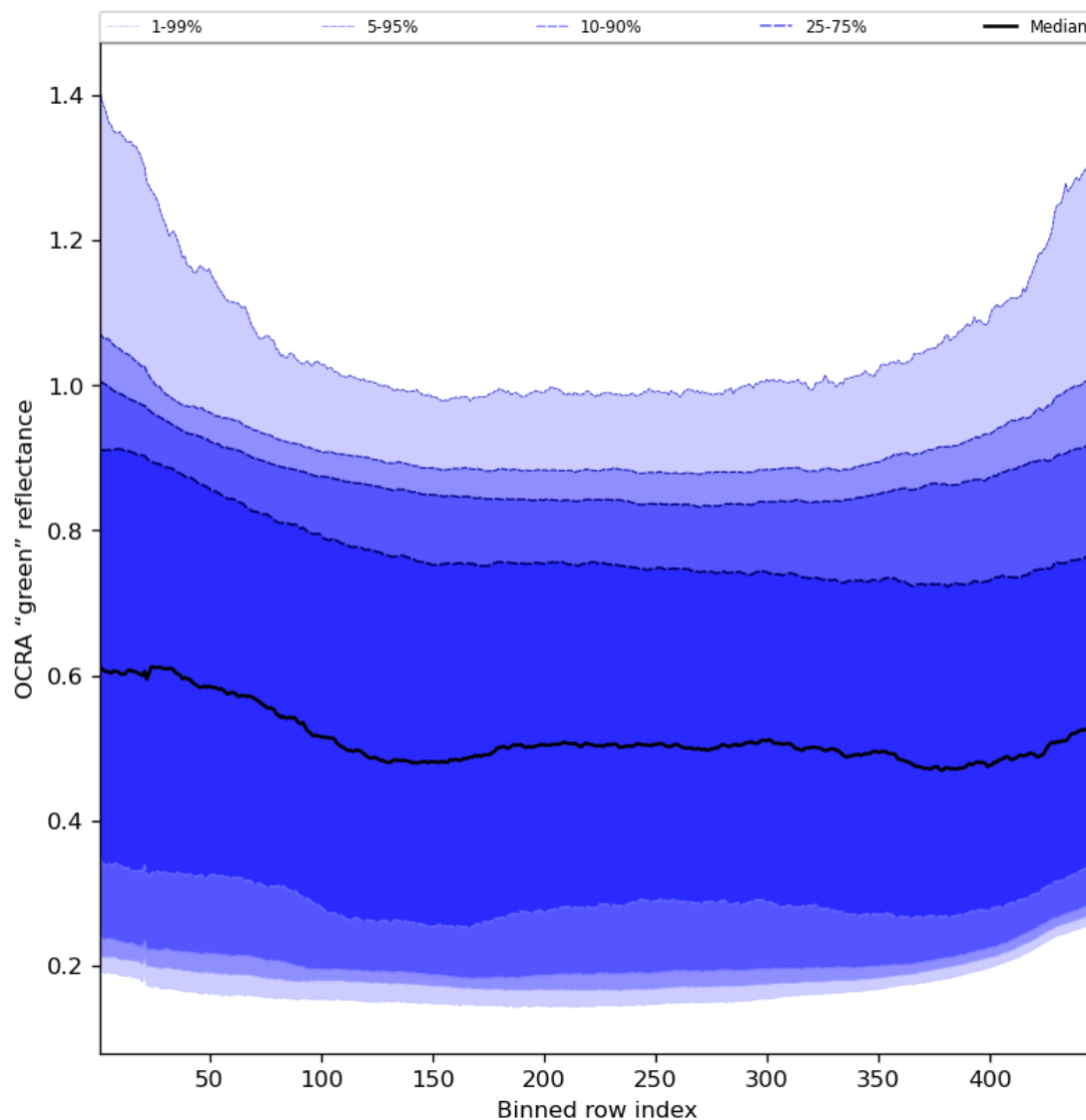
Figure 68: Along track statistics of “OCRA “green” reflectance” for 2023-10-20 to 2023-10-22
