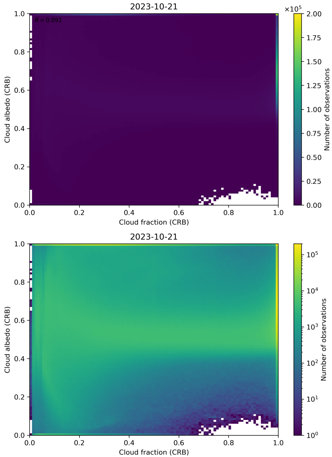
Figure 77: Scatter density plot of “Cloud fraction (CRB)” against “Cloud albedo (CRB)” for 2023-10-20 to 2023-10-22.
