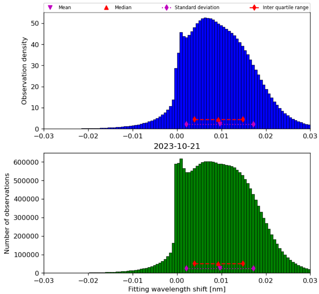
Figure 49: Histogram of “Fitting wavelength shift” for 2023-10-20 to 2023-10-22
