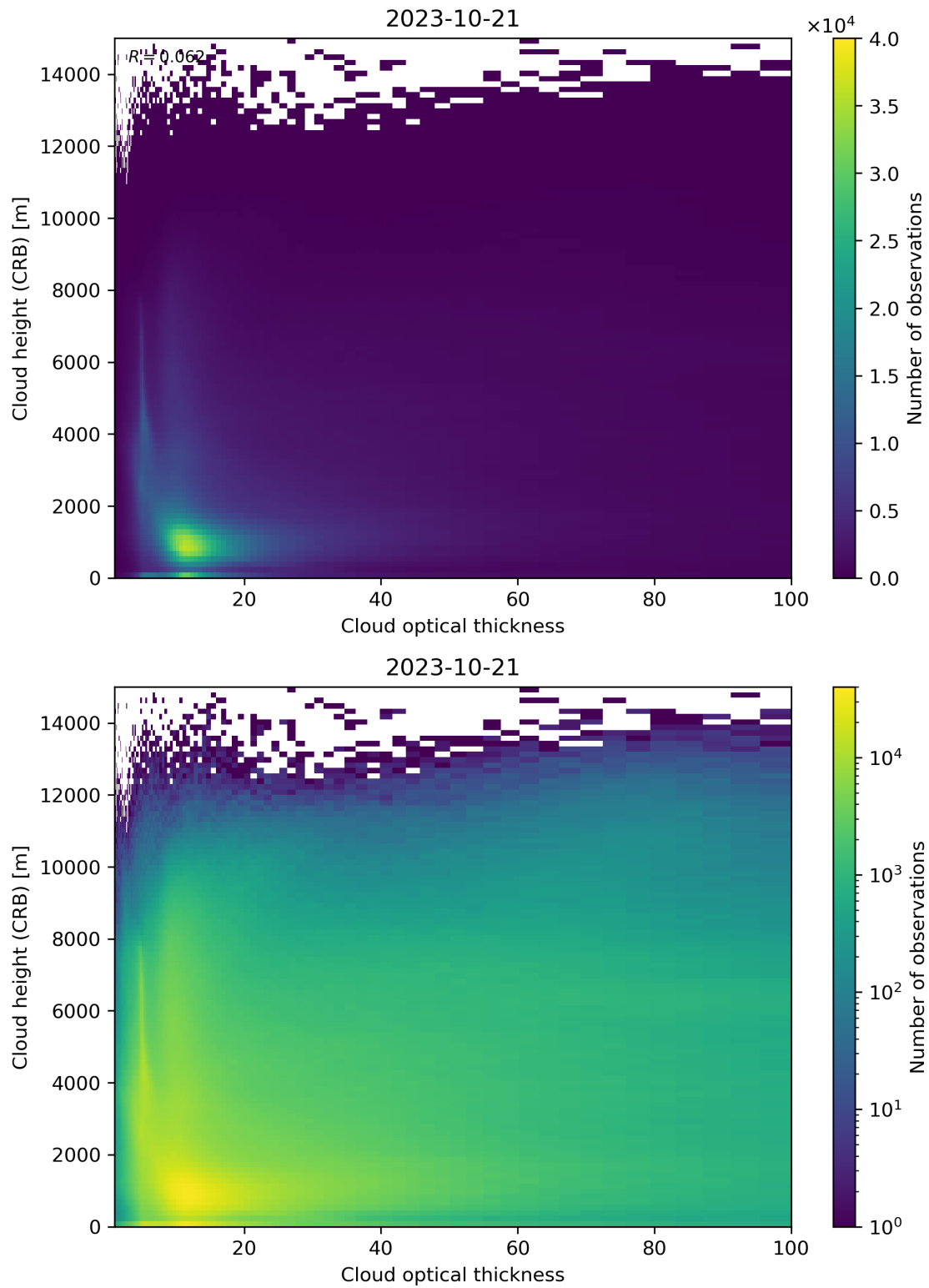
Figure 85: Scatter density plot of “Cloud optical thickness” against “Cloud height (CRB)” for 2023-10-20 to 2023-10-22.
