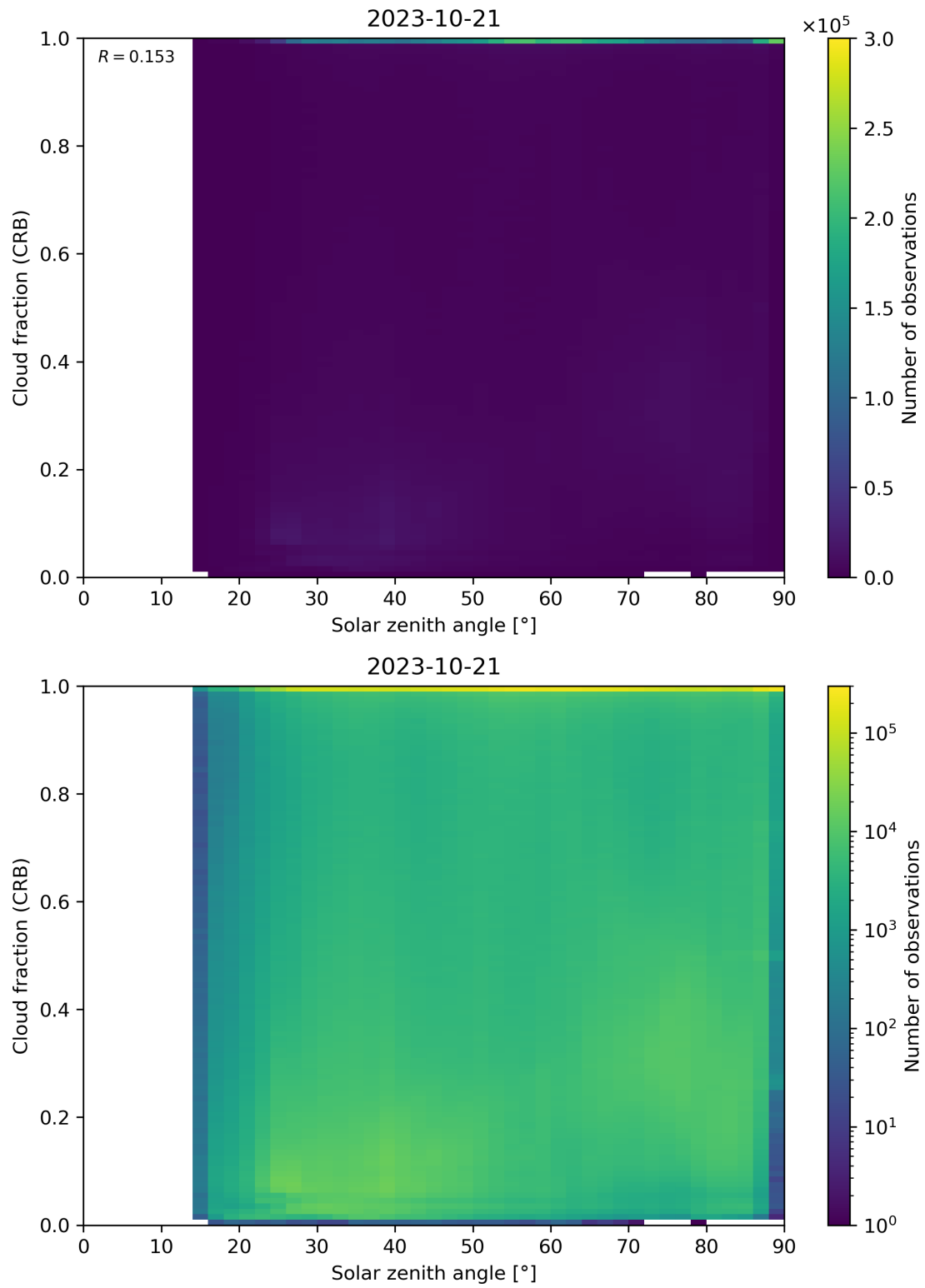
Figure 101: Scatter density plot of “Solar zenith angle” against “Cloud fraction (CRB)” for 2023-10-20 to 2023-10-22.
