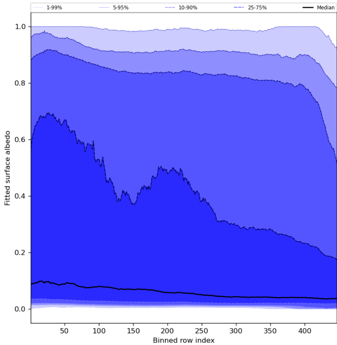
Figure 61: Along track statistics of “Fitted surface albedo” for 2023-10-20 to 2023-10-22
