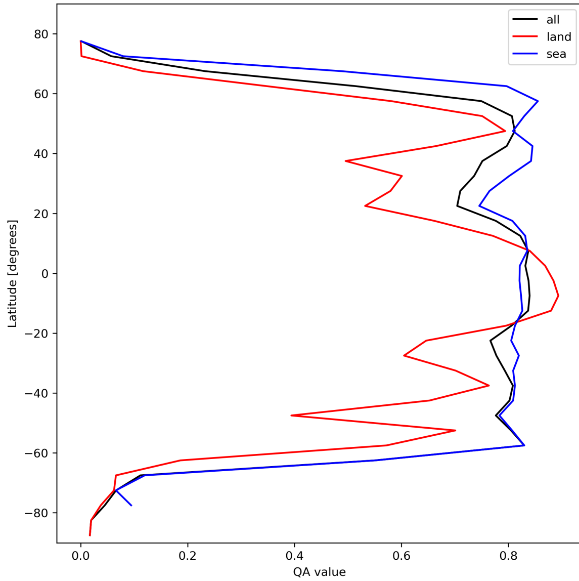
Figure 22: Zonal average of “QA value” for 2023-10-20 to 2023-10-22.
