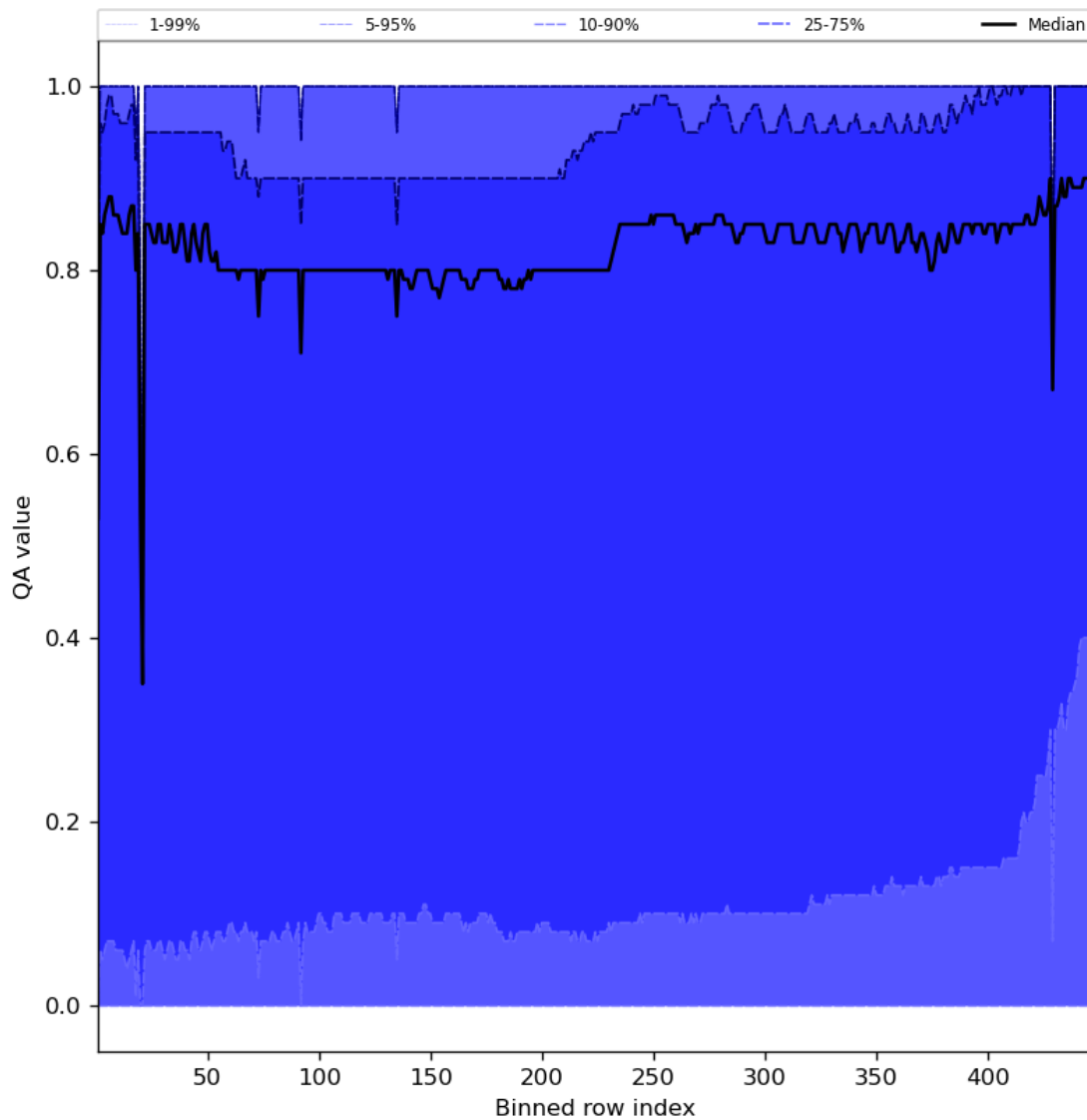
Figure 54: Along track statistics of “QA value” for 2023-10-20 to 2023-10-22
