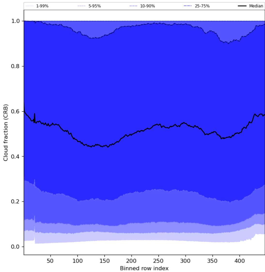
Figure 58: Along track statistics of “Cloud fraction (CRB)” for 2023-10-20 to 2023-10-22
