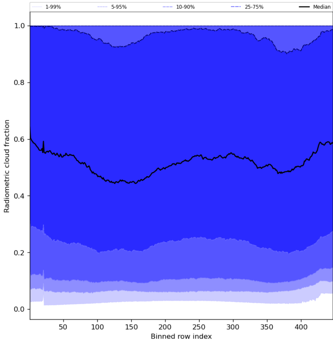
Figure 55: Along track statistics of “Radiometric cloud fraction” for 2023-10-20 to 2023-10-22
