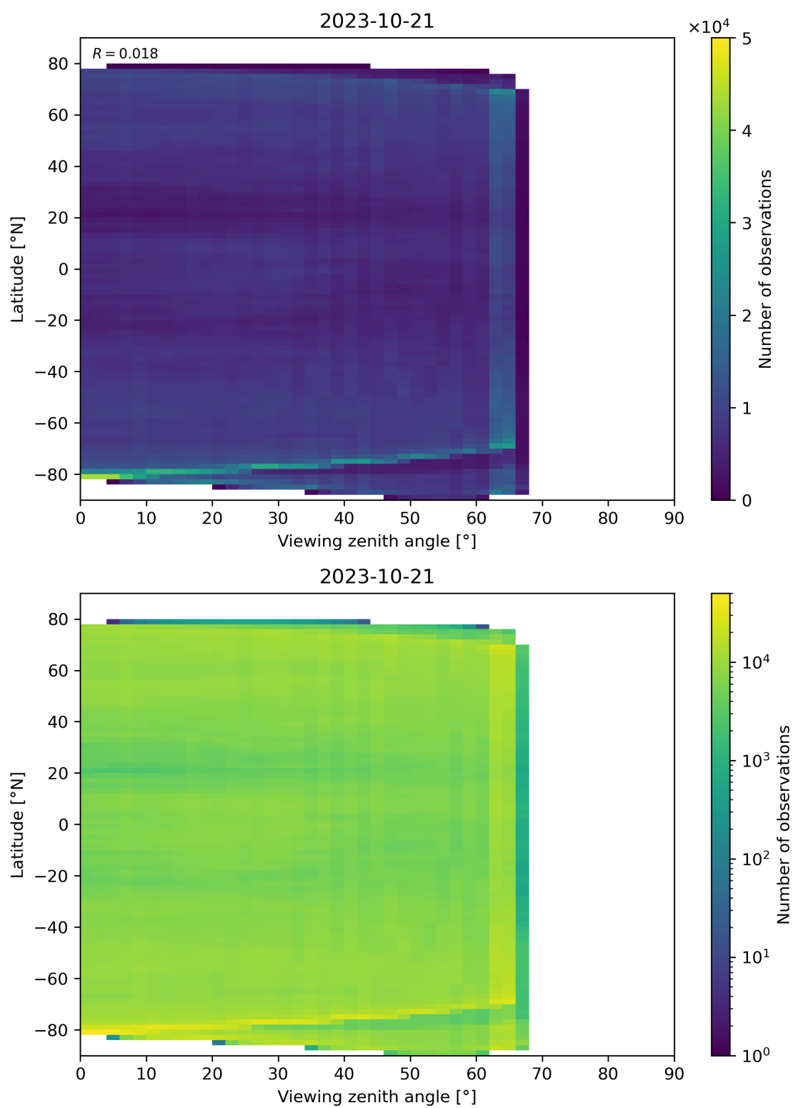
Figure 113: Scatter density plot of “Viewing zenith angle” against “Latitude” for 2023-10-20 to 2023-10-22.
