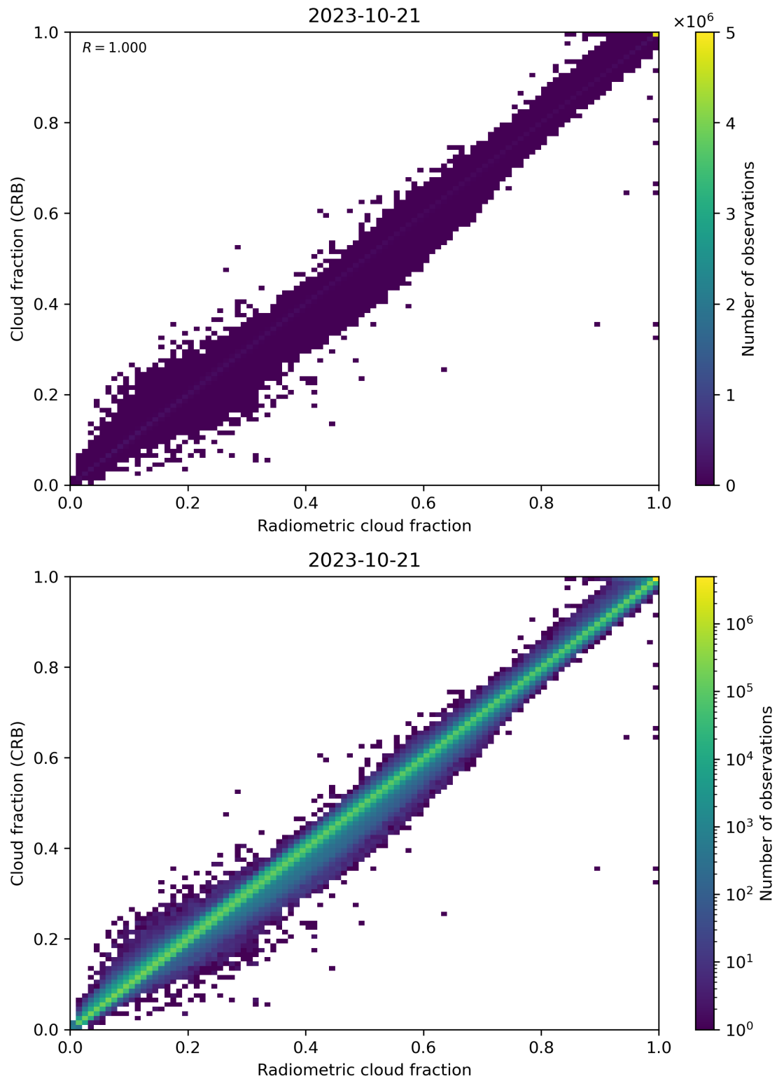
Figure 73: Scatter density plot of “Radiometric cloud fraction” against “Cloud fraction (CRB)” for 2023-10-20 to 2023-10-22.
