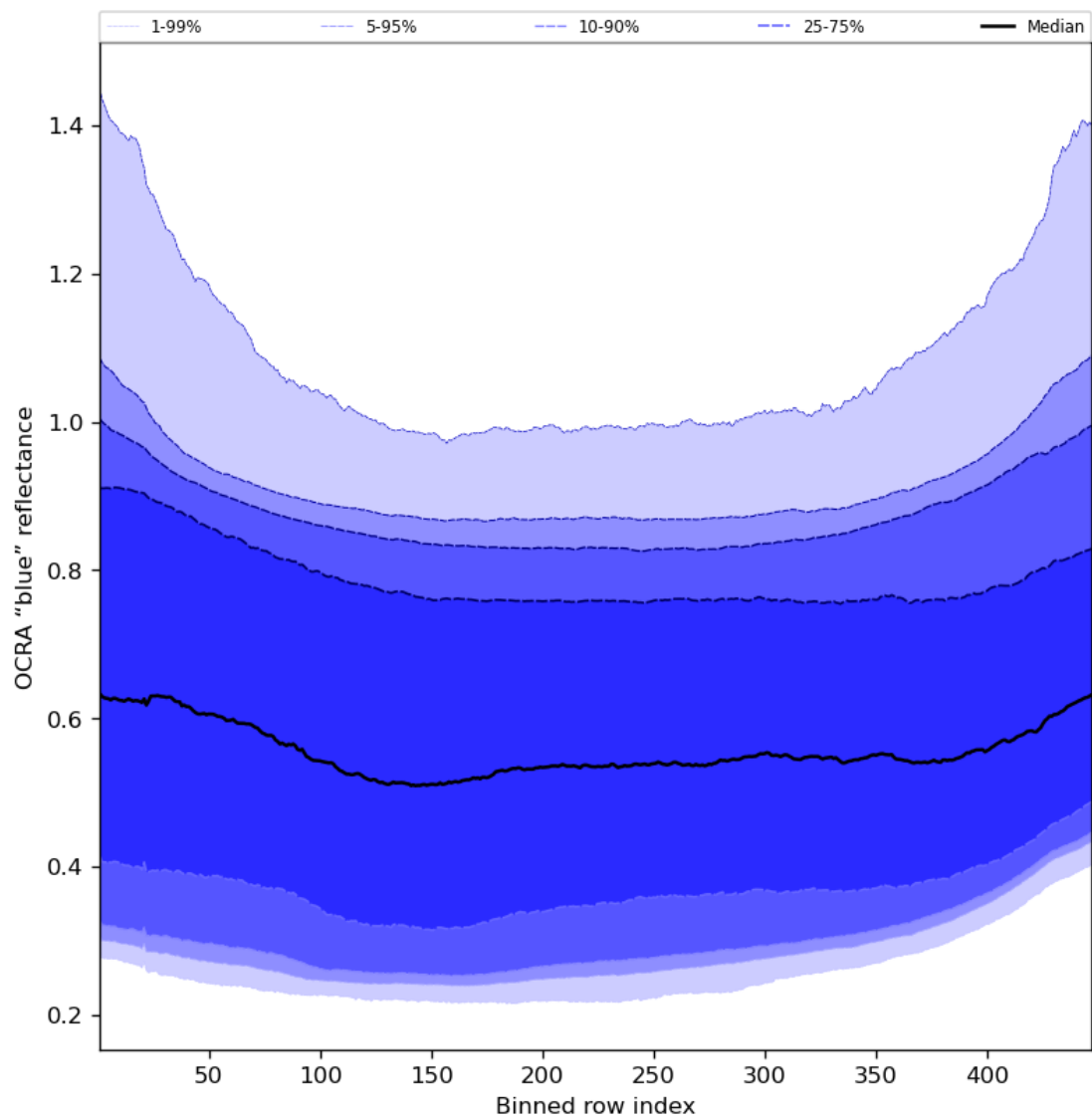
Figure 67: Along track statistics of “OCRA “blue” reflectance” for 2023-10-20 to 2023-10-22
