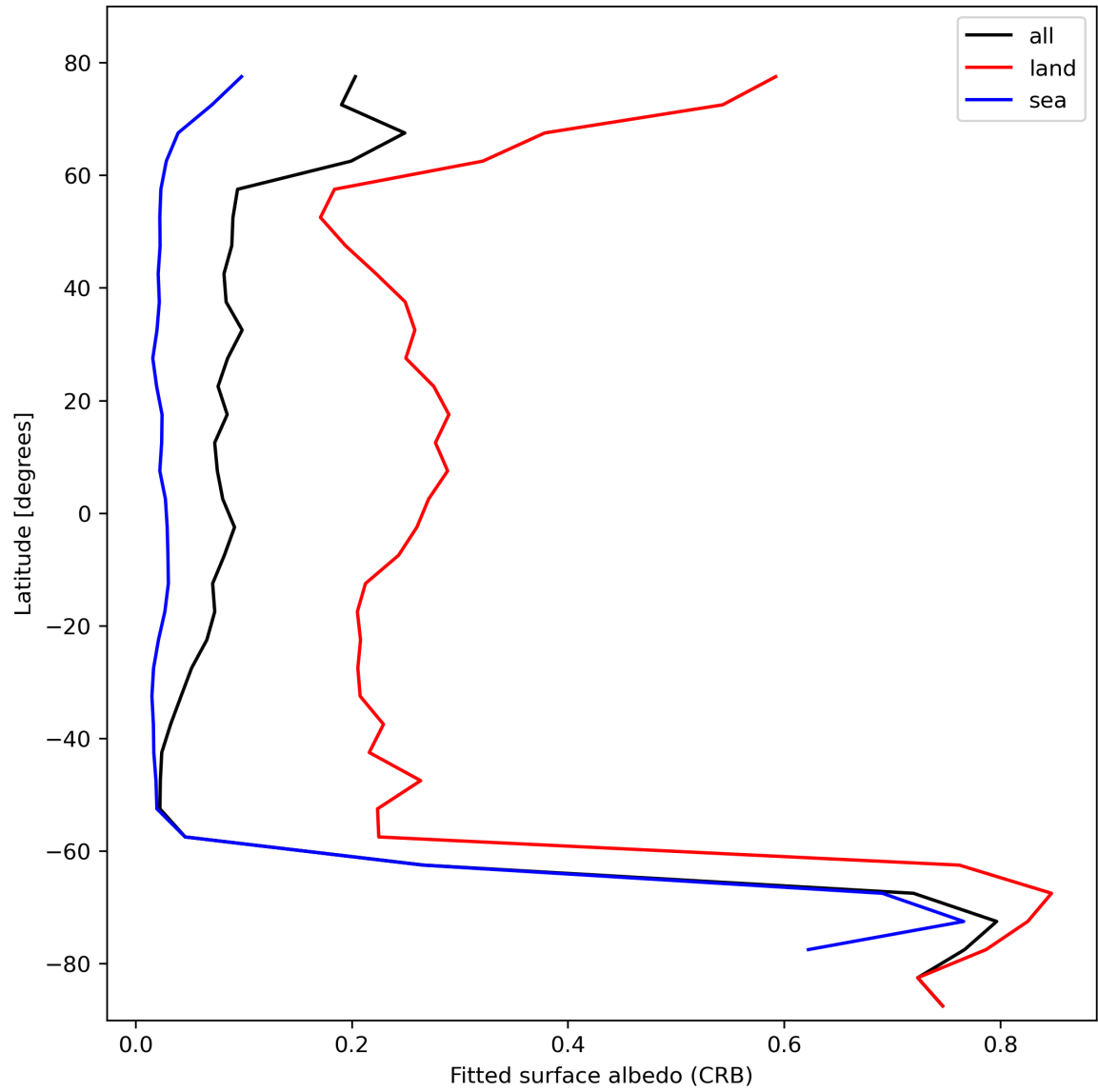
Figure 30: Zonal average of “Fitted surface albedo (CRB)” for 2023-10-20 to 2023-10-22.
