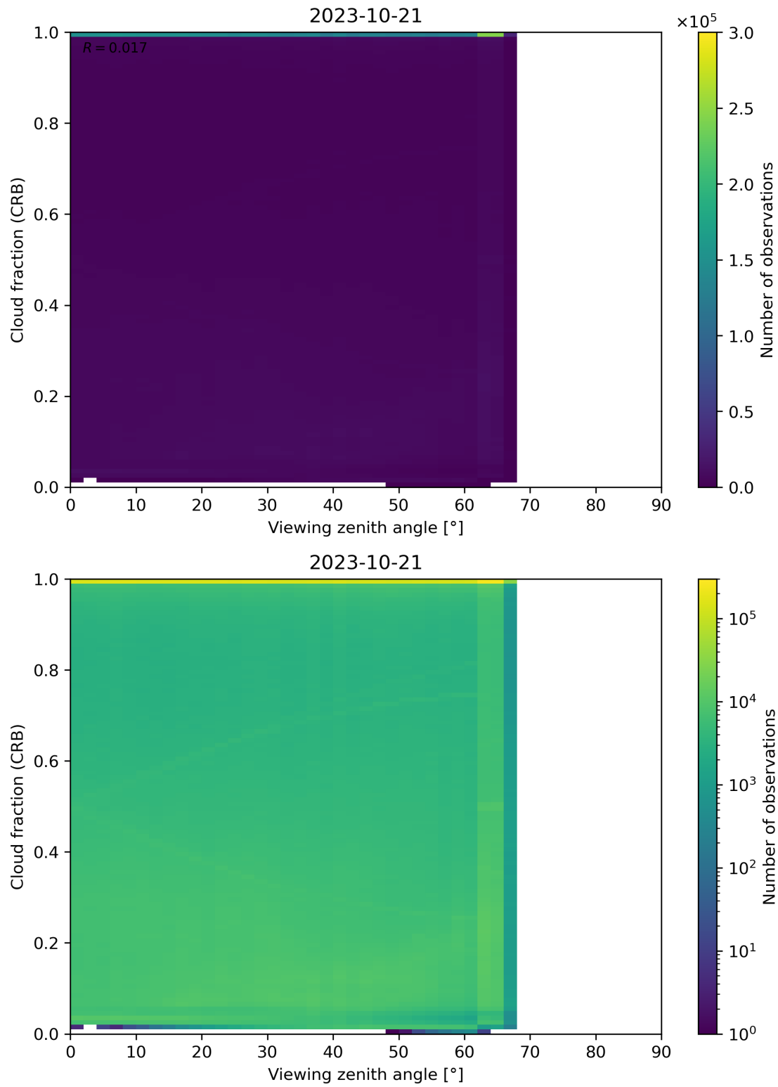
Figure 109: Scatter density plot of “Viewing zenith angle” against “Cloud fraction (CRB)” for 2023-10-20 to 2023-10-22.
