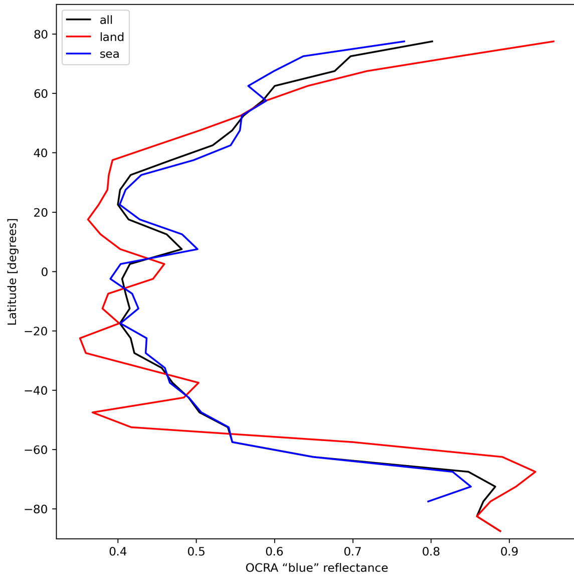
Figure 35: Zonal average of “OCRA “blue” reflectance” for 2023-10-20 to 2023-10-22.
