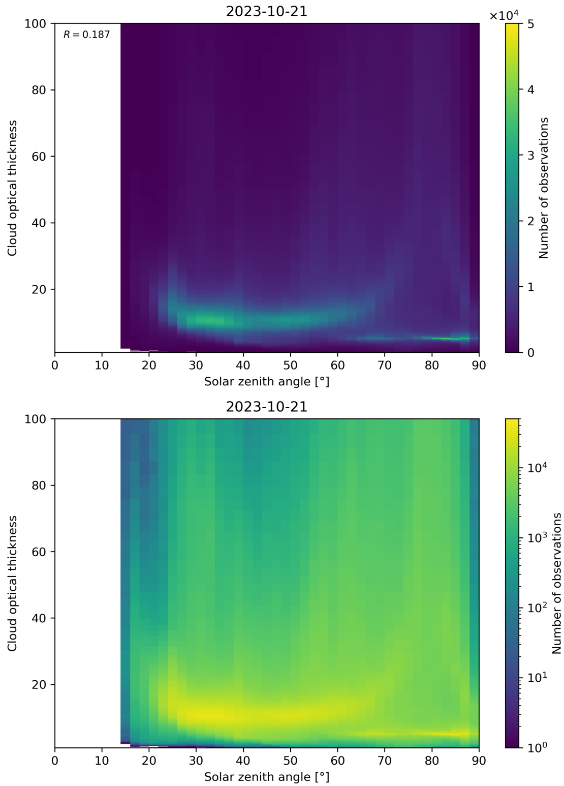
Figure 103: Scatter density plot of “Solar zenith angle” against “Cloud optical thickness” for 2023-10-20 to 2023-10-22.
