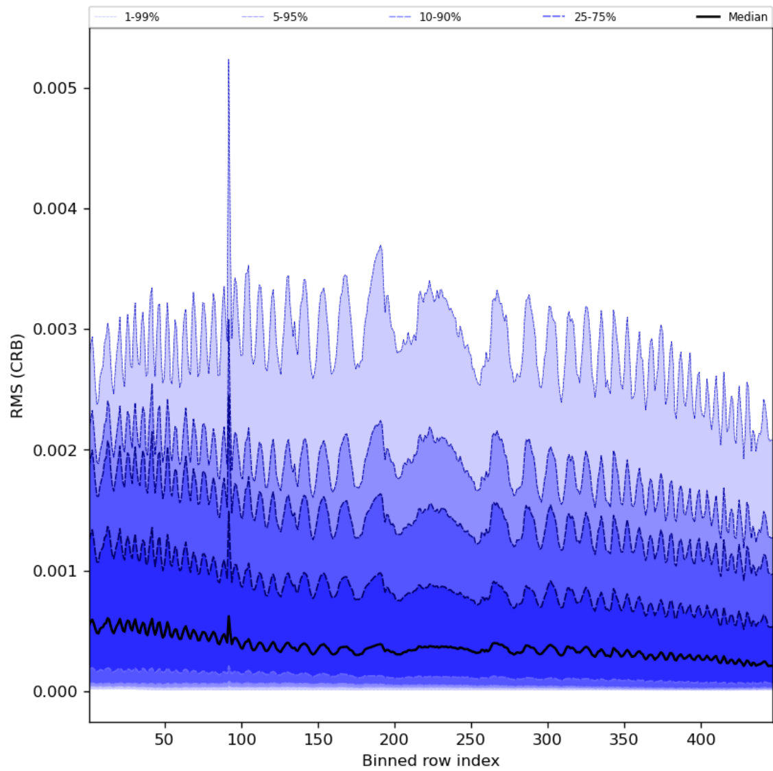
Figure 64: Along track statistics of “RMS (CRB)” for 2023-10-20 to 2023-10-22
