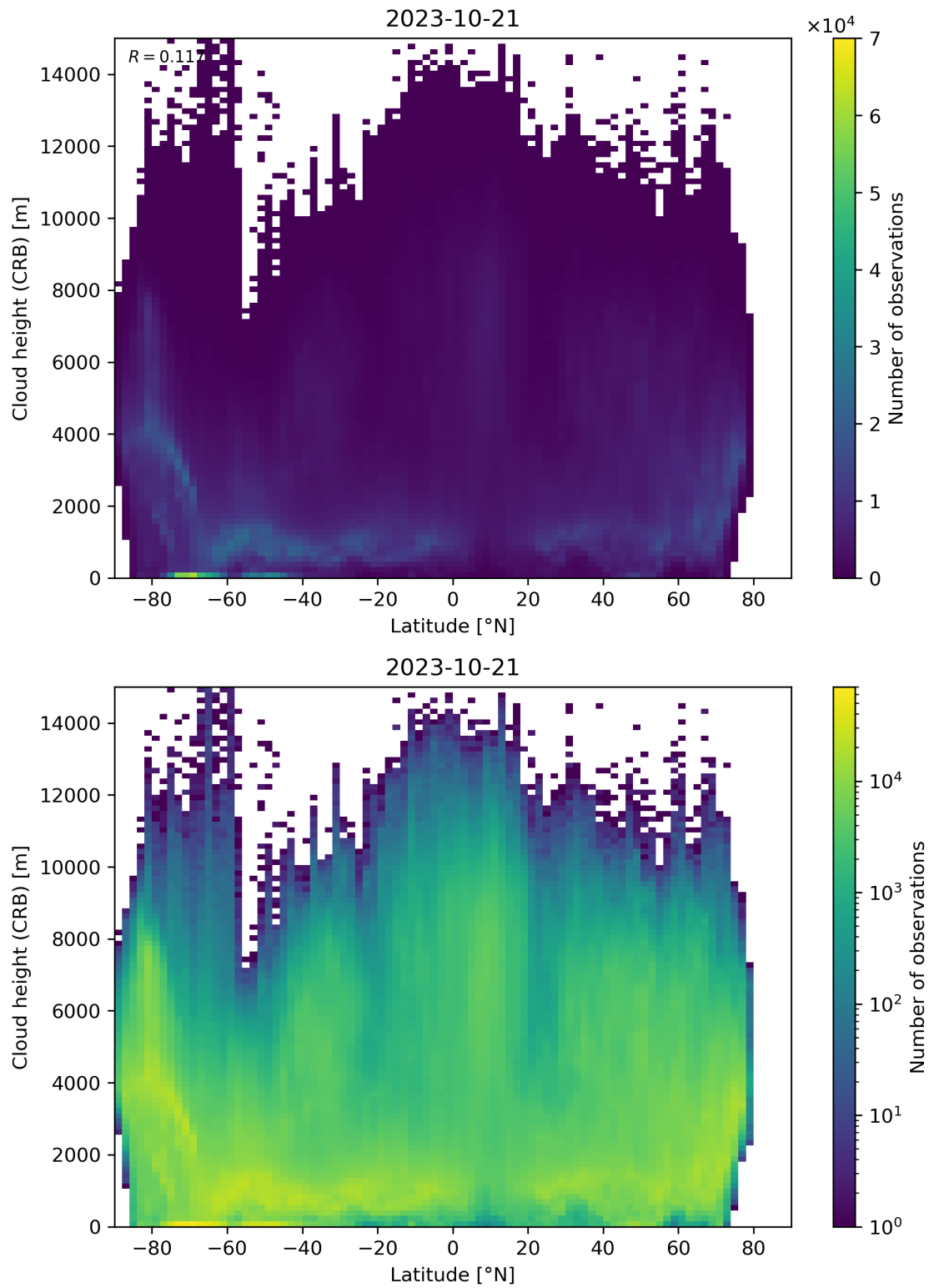
Figure 95: Scatter density plot of “Latitude” against “Cloud height (CRB)” for 2023-10-20 to 2023-10-22.
