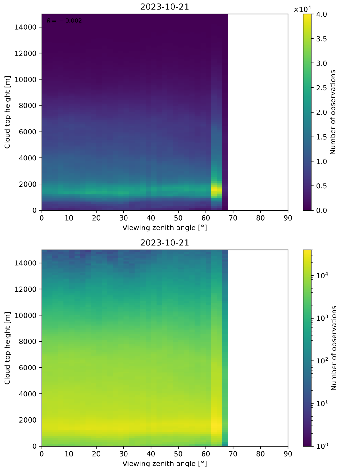
Figure 112: Scatter density plot of “Viewing zenith angle” against “Cloud top height” for 2023-10-20 to 2023-10-22.
