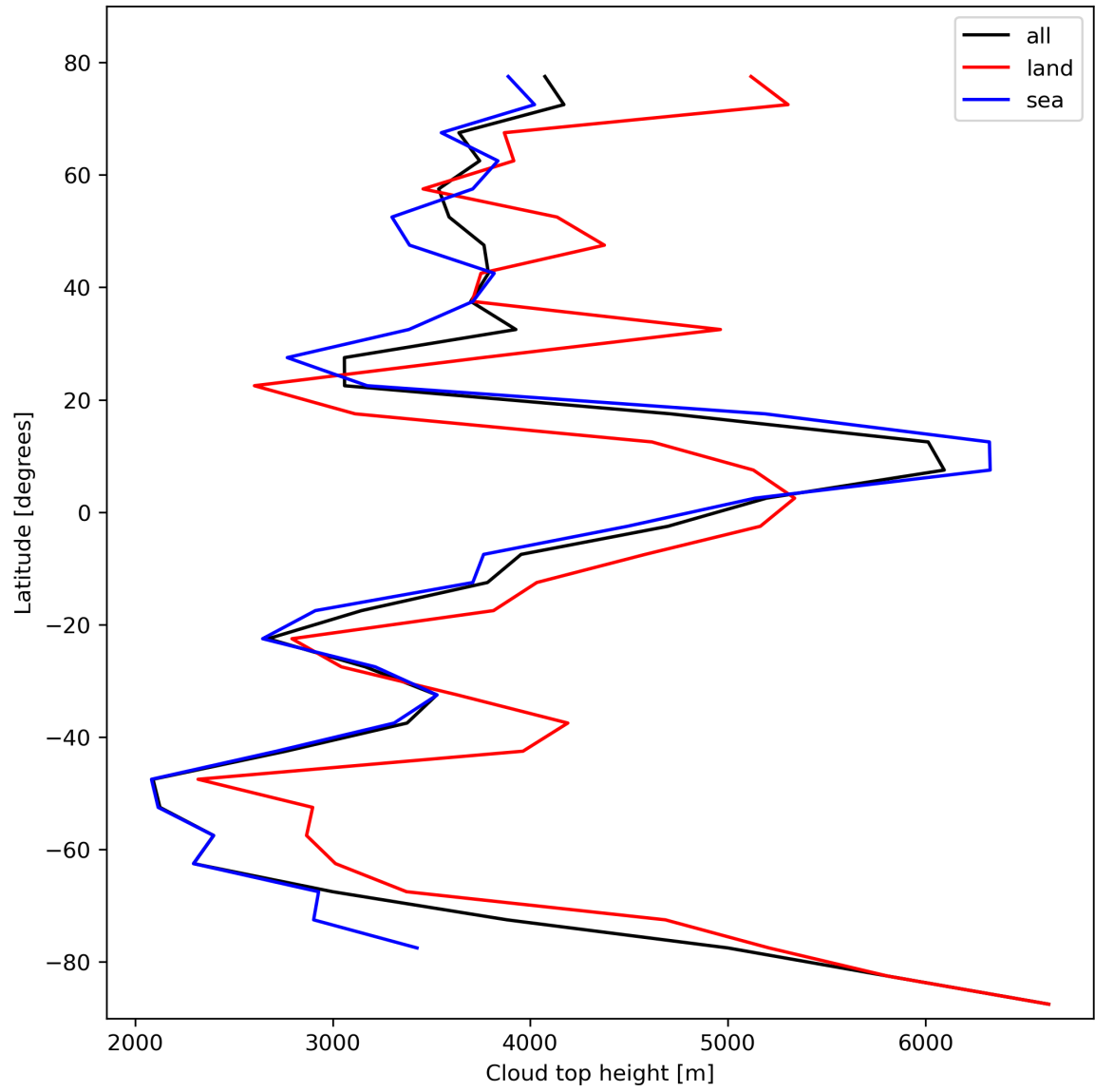
Figure 24: Zonal average of “Cloud top height” for 2023-10-20 to 2023-10-22.
