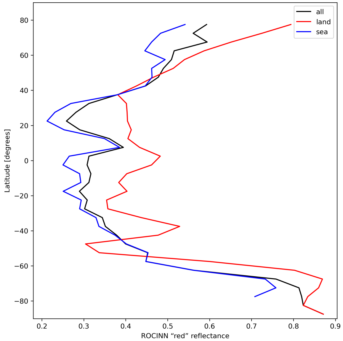
Figure 37: Zonal average of “ROCINN “red” reflectance” for 2023-10-20 to 2023-10-22.
