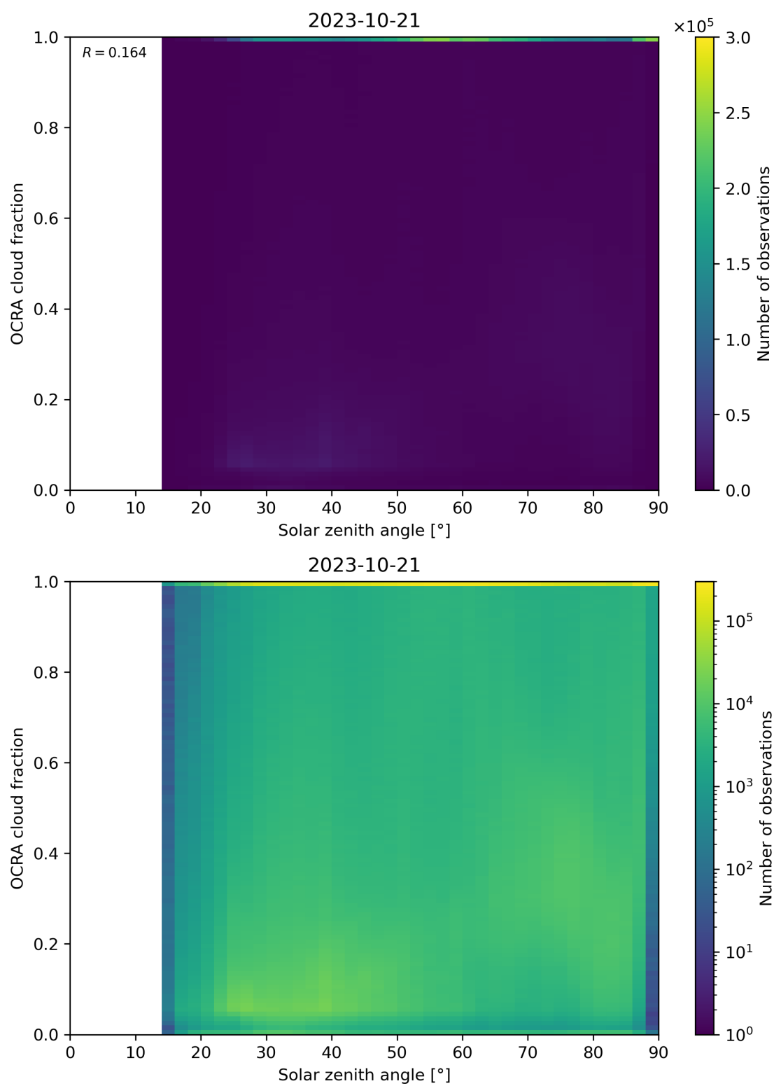
Figure 100: Scatter density plot of “Solar zenith angle” against “OCRA cloud fraction” for 2023-10-20 to 2023-10-22.
