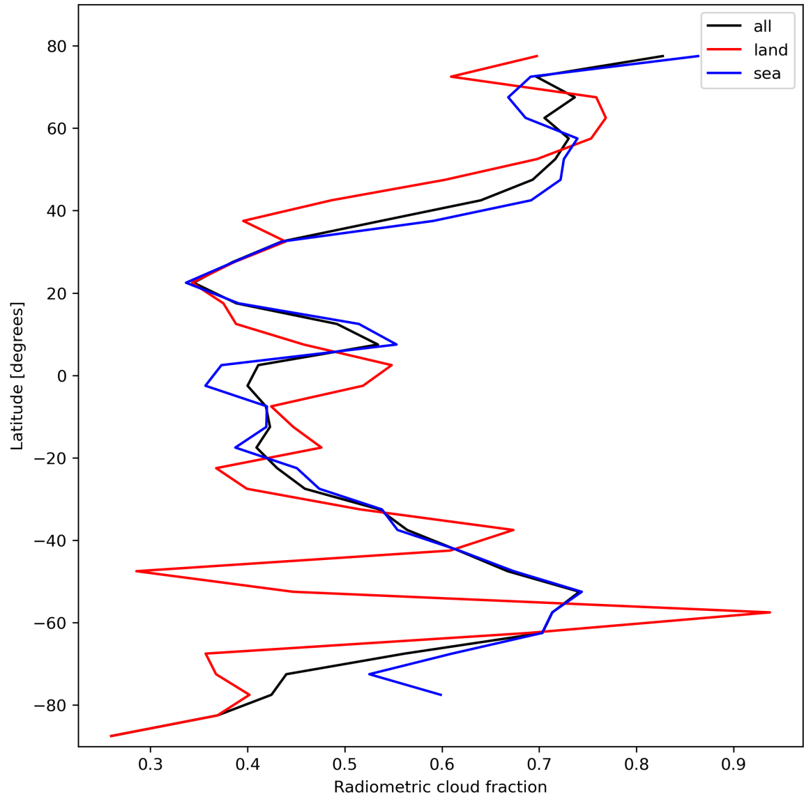
Figure 23: Zonal average of “Radiometric cloud fraction” for 2023-10-20 to 2023-10-22.
