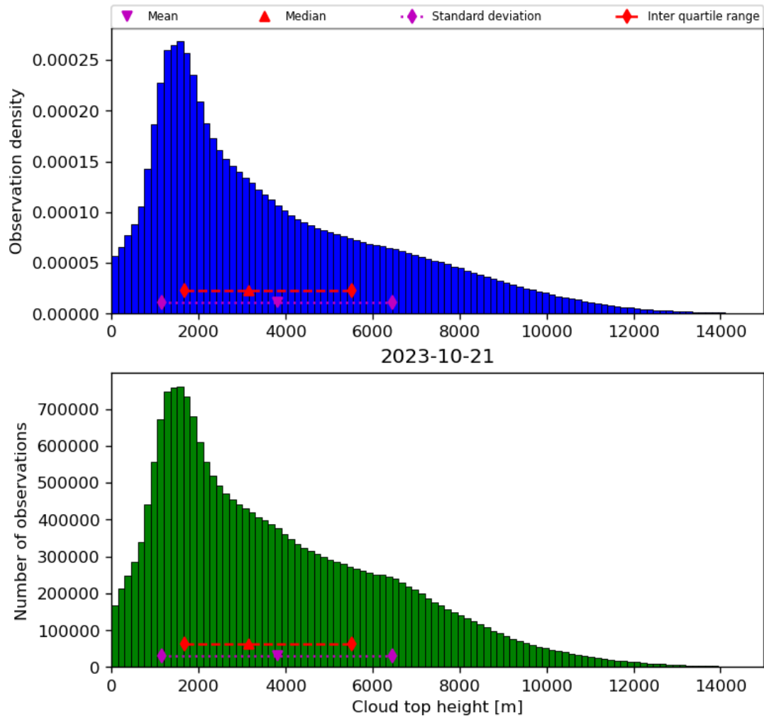
Figure 40: Histogram of “Cloud top height” for 2023-10-20 to 2023-10-22
