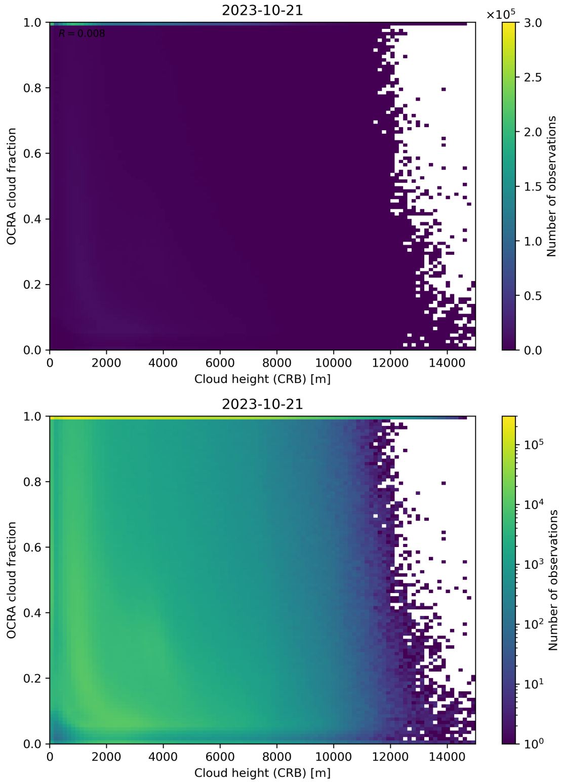
Figure 81: Scatter density plot of “Cloud height (CRB)” against “OCRA cloud fraction” for 2023-10-20 to 2023-10-22.
