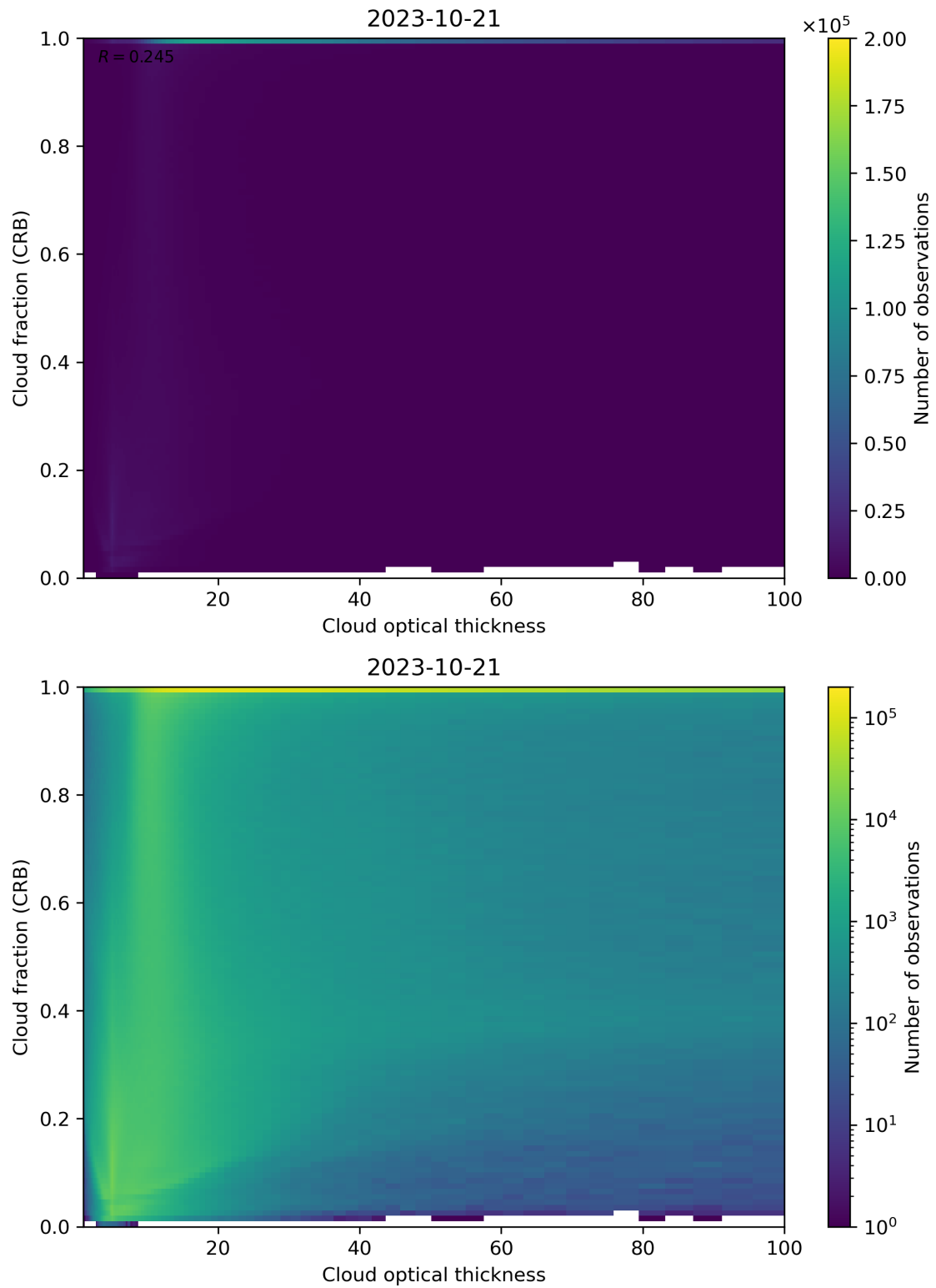
Figure 84: Scatter density plot of “Cloud optical thickness” against “Cloud fraction (CRB)” for 2023-10-20 to 2023-10-22.
