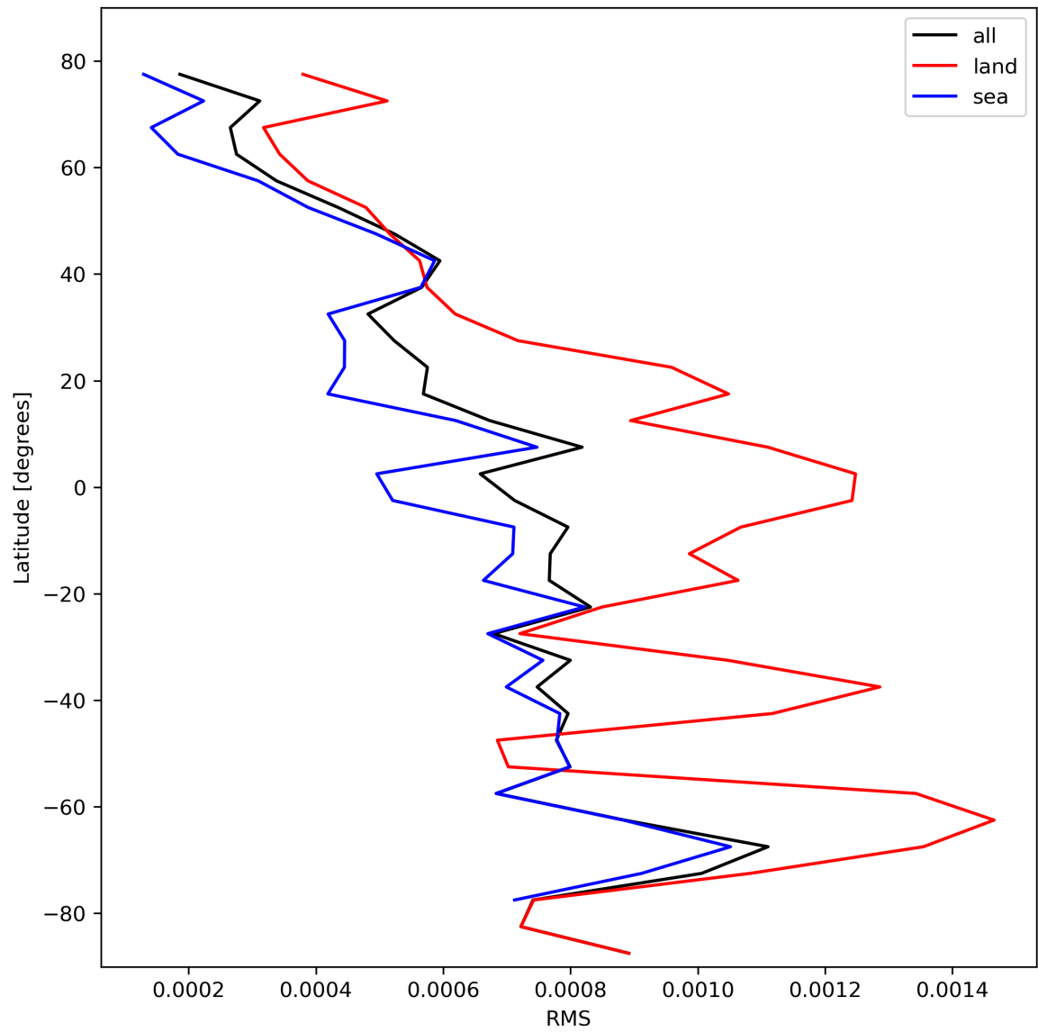
Figure 31: Zonal average of “RMS” for 2023-10-20 to 2023-10-22.
