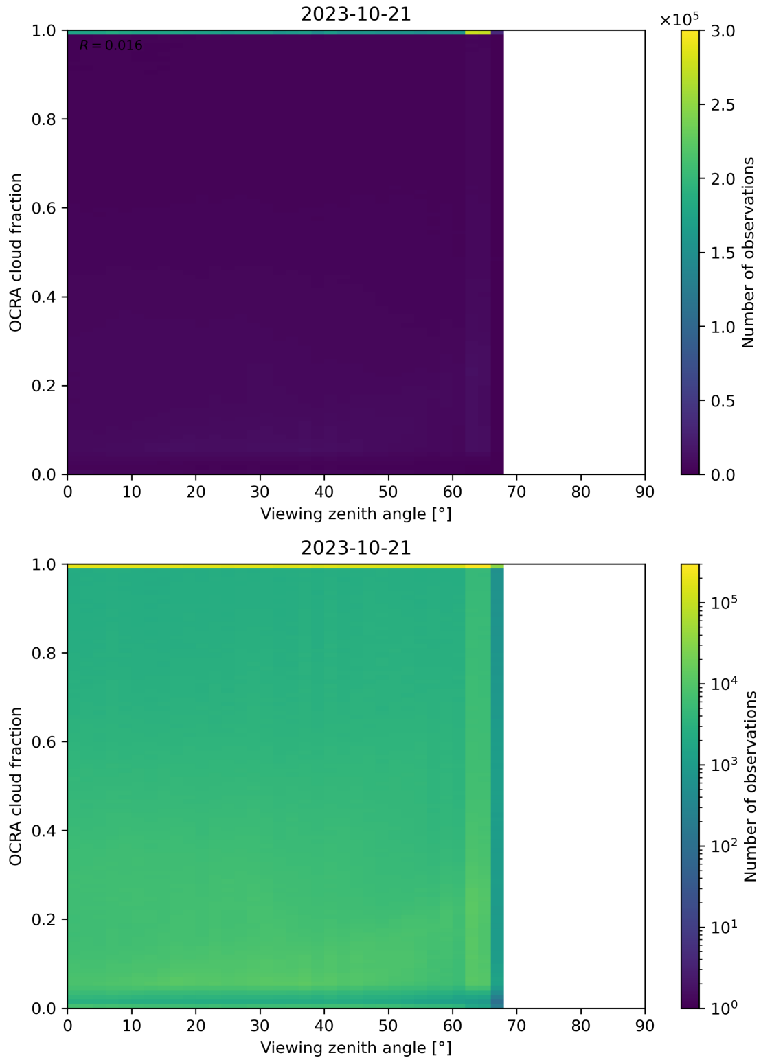
Figure 108: Scatter density plot of “Viewing zenith angle” against “OCRA cloud fraction” for 2023-10-20 to 2023-10-22.
