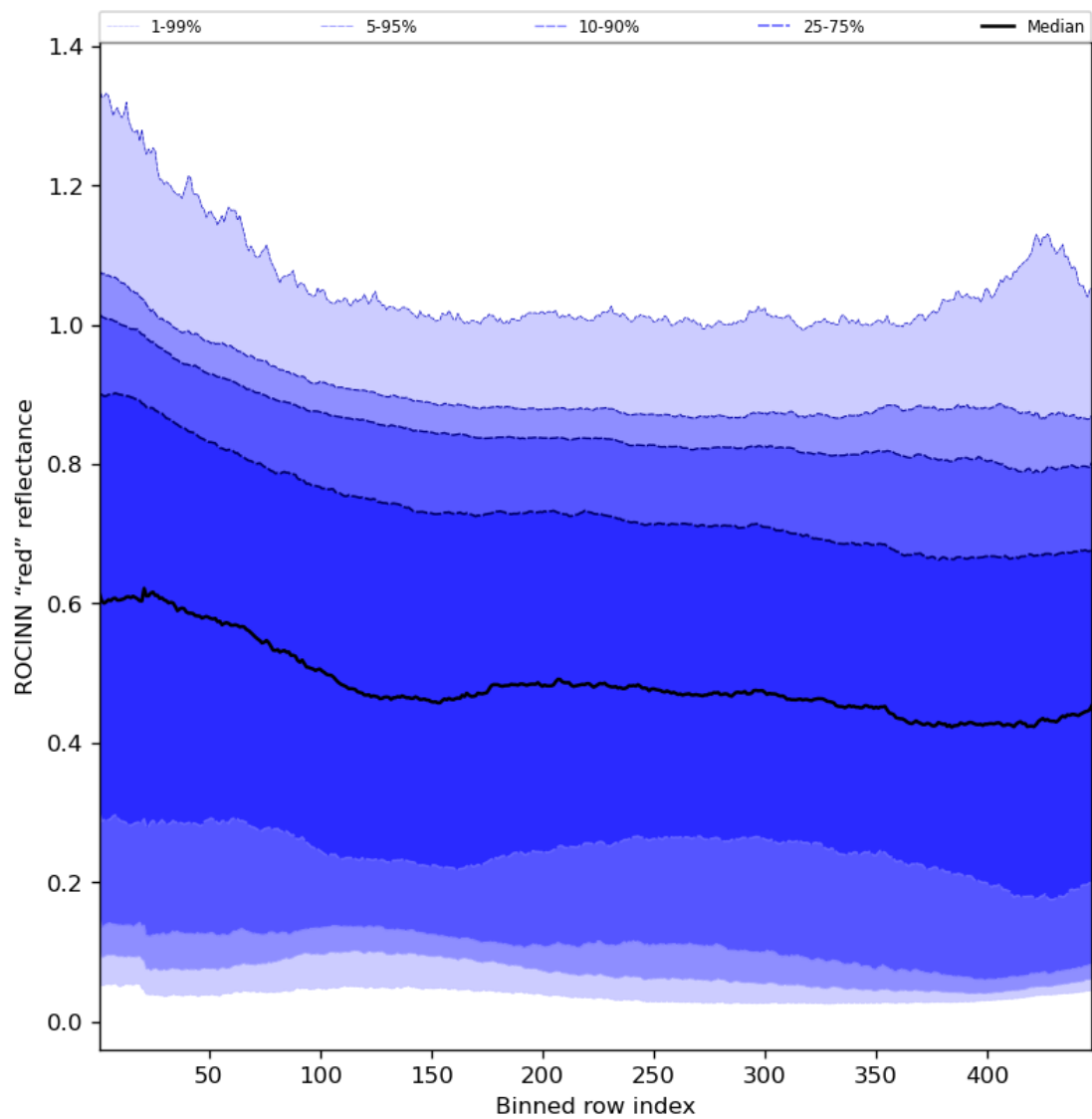
Figure 69: Along track statistics of “ROCINN “red” reflectance” for 2023-10-20 to 2023-10-22
