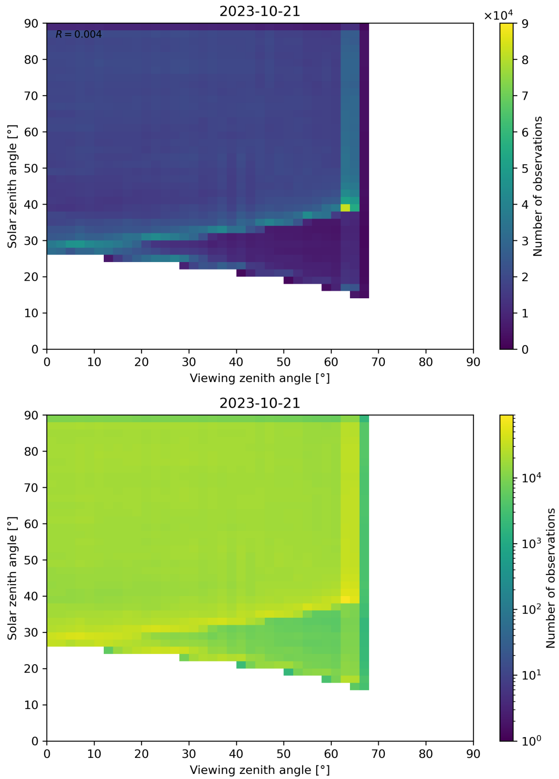
Figure 114: Scatter density plot of “Viewing zenith angle” against “Solar zenith angle” for 2023-10-20 to 2023-10-22.
