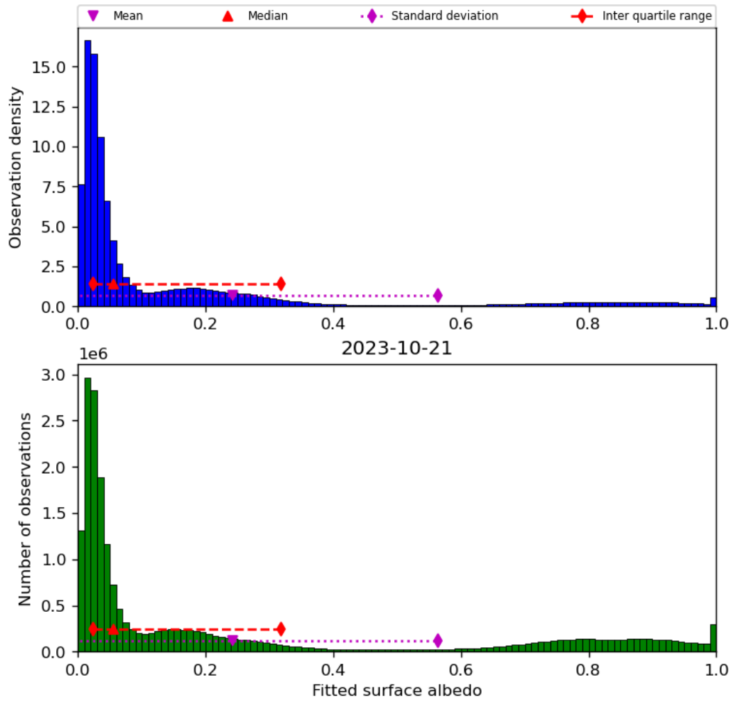
Figure 45: Histogram of “Fitted surface albedo” for 2023-10-20 to 2023-10-22
