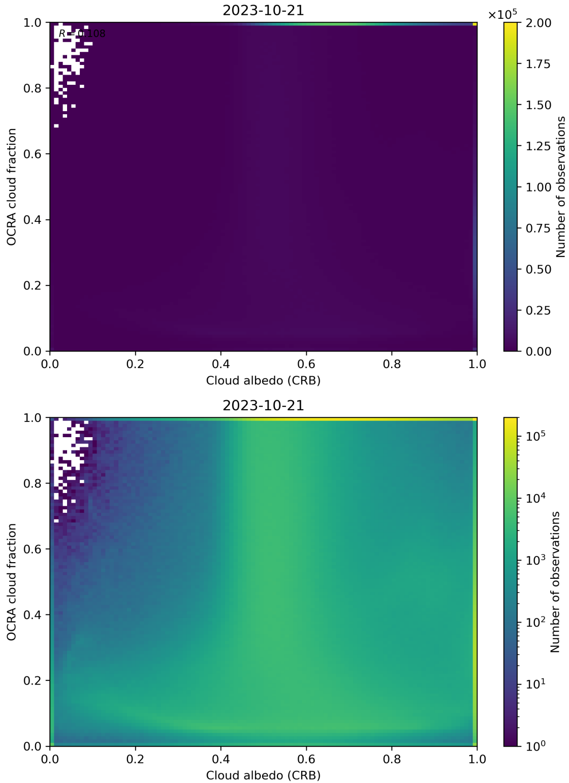
Figure 70: Scatter density plot of “Cloud albedo (CRB)” against “OCRA cloud fraction” for 2023-10-20 to 2023-10-22.
