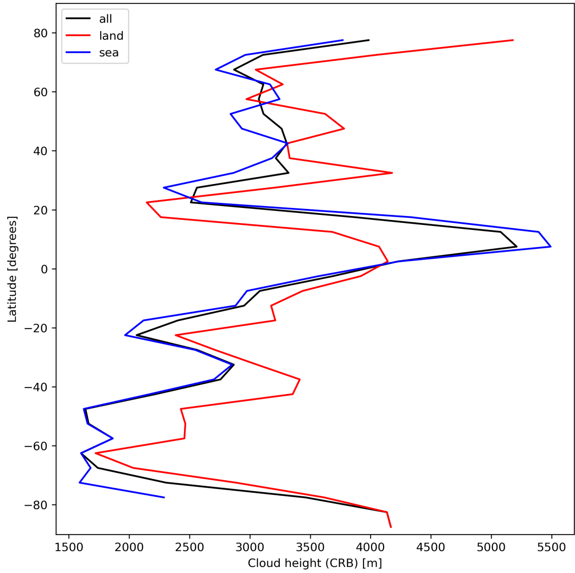
Figure 27: Zonal average of “Cloud height (CRB)” for 2023-10-20 to 2023-10-22.
