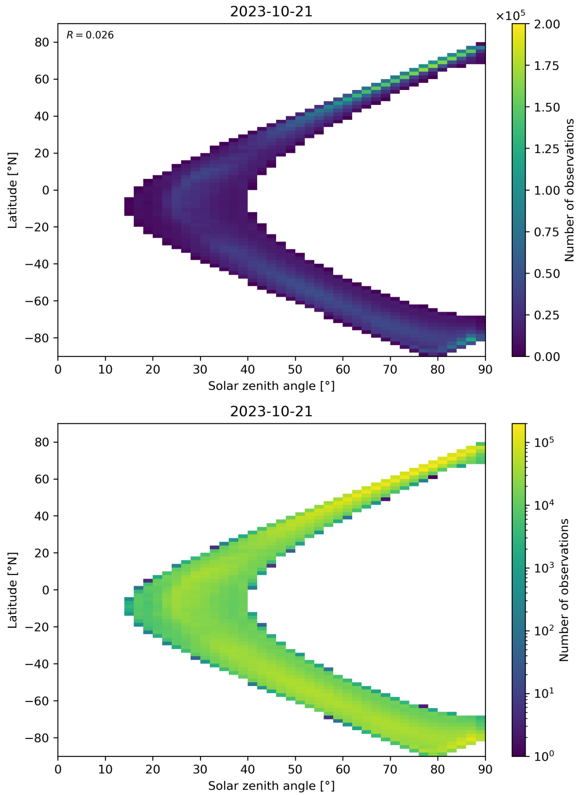
Figure 105: Scatter density plot of “Solar zenith angle” against “Latitude” for 2023-10-20 to 2023-10-22.
