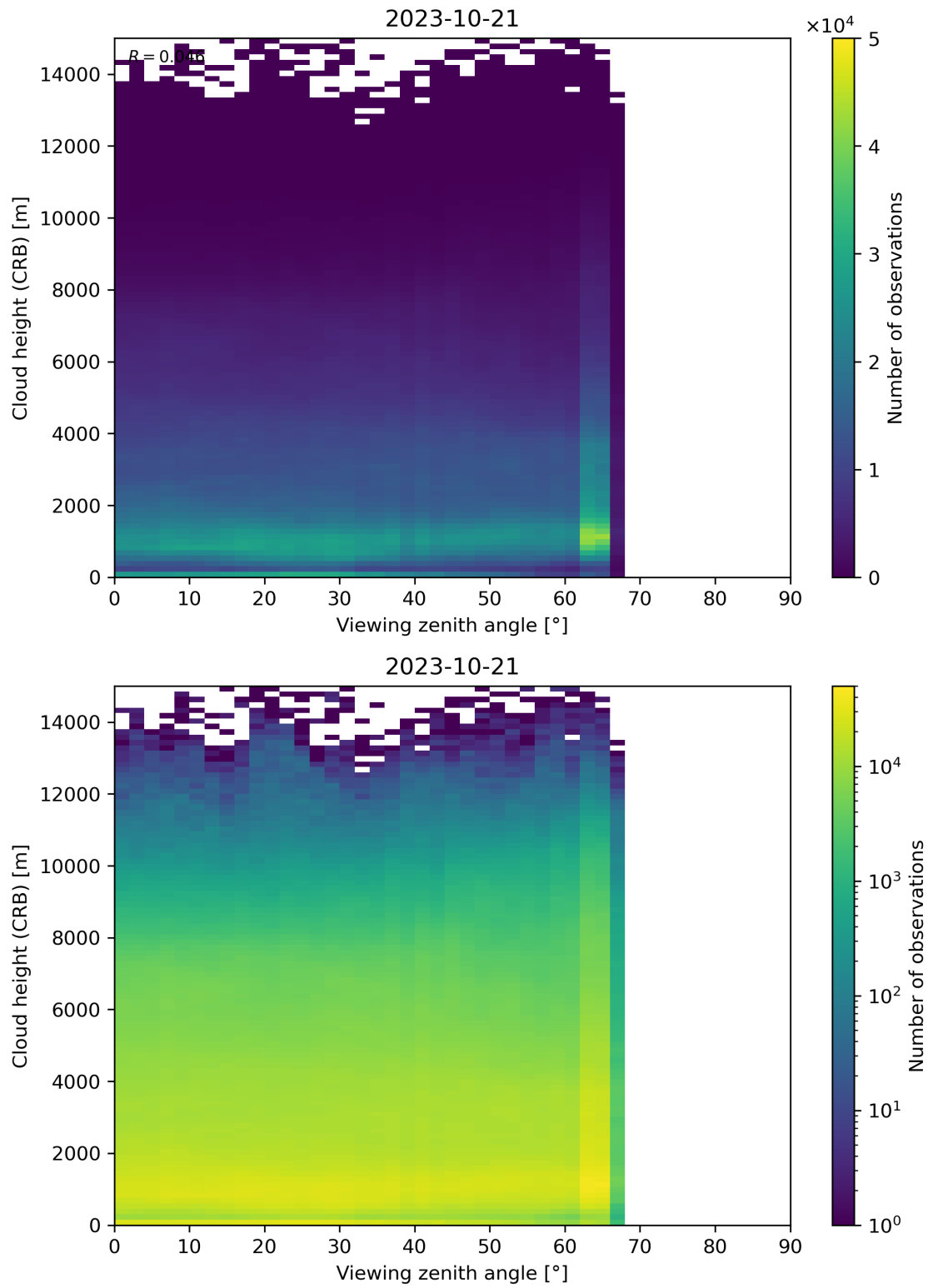
Figure 110: Scatter density plot of “Viewing zenith angle” against “Cloud height (CRB)” for 2023-10-20 to 2023-10-22.
