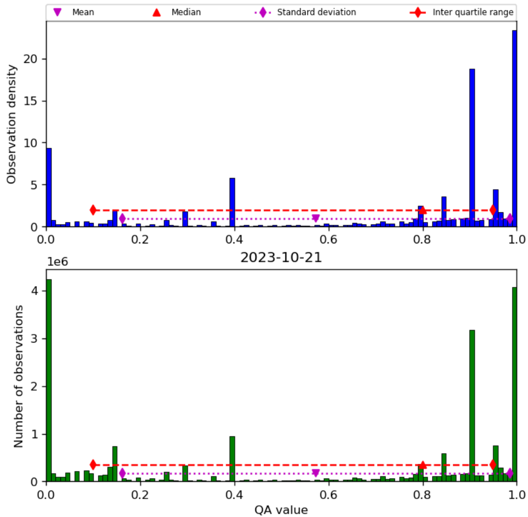
Figure 38: Histogram of “QA value” for 2023-10-20 to 2023-10-22
