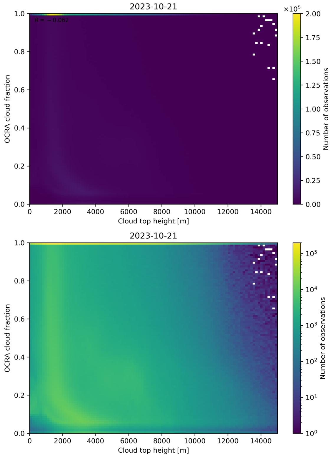
Figure 87: Scatter density plot of “Cloud top height” against “OCRA cloud fraction” for 2023-10-20 to 2023-10-22.
