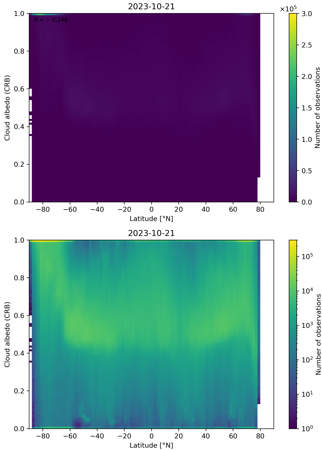
Figure 91: Scatter density plot of “Latitude” against “Cloud albedo (CRB)” for 2023-10-20 to 2023-10-22.
