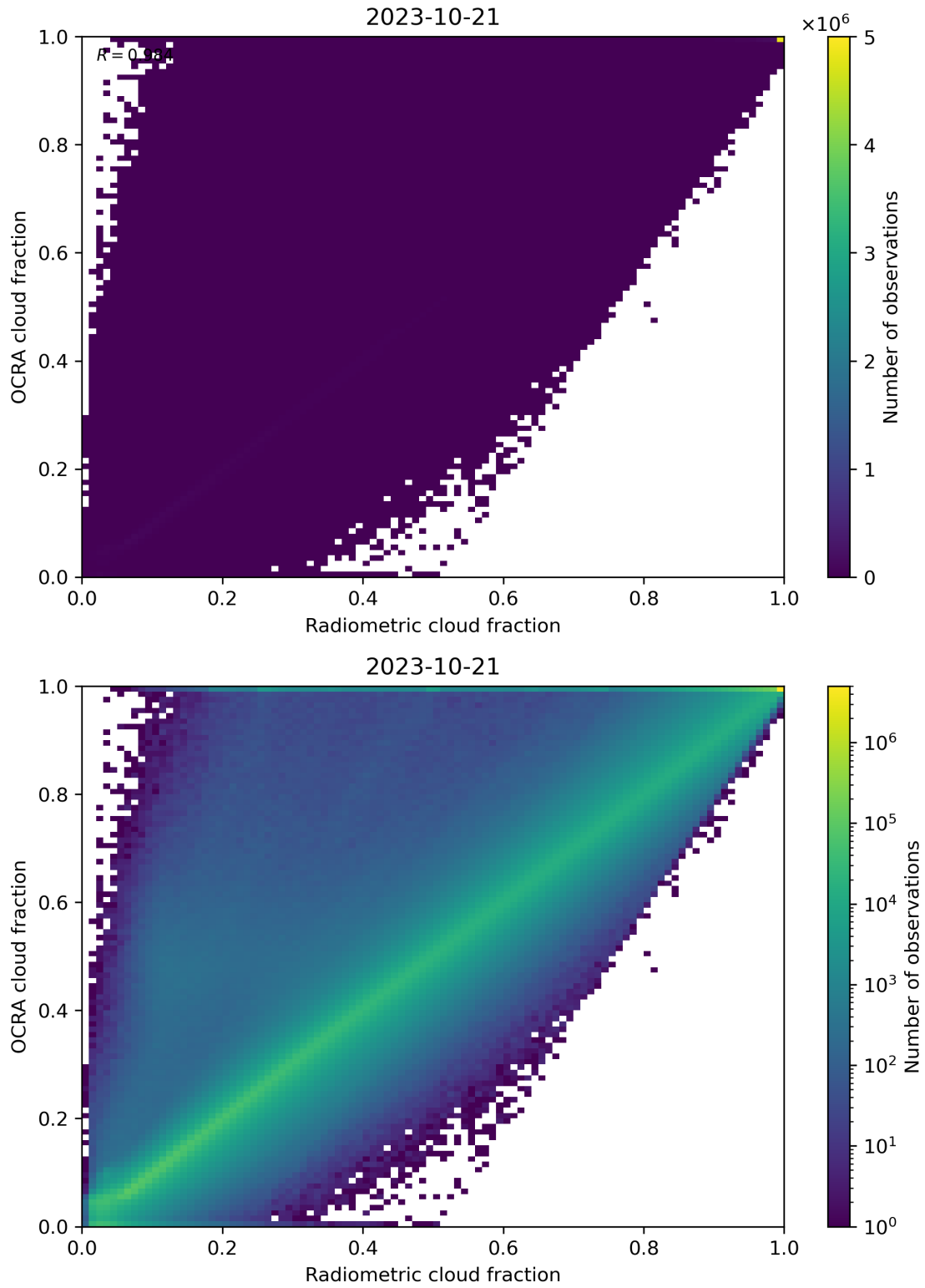
Figure 72: Scatter density plot of “Radiometric cloud fraction” against “OCRA cloud fraction” for 2023-10-20 to 2023-10-22.
