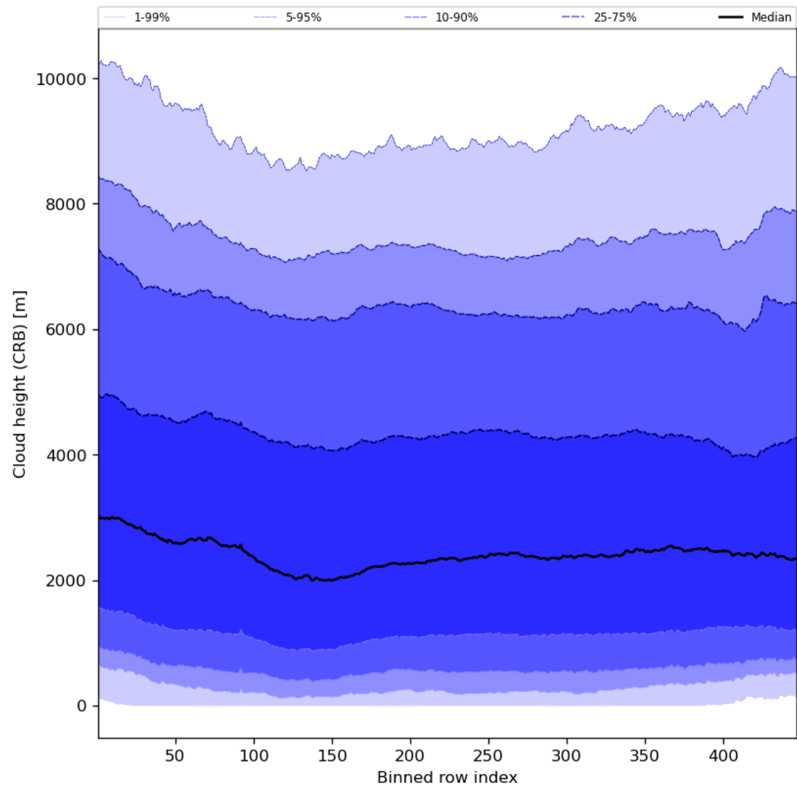
Figure 59: Along track statistics of “Cloud height (CRB)” for 2023-10-20 to 2023-10-22
