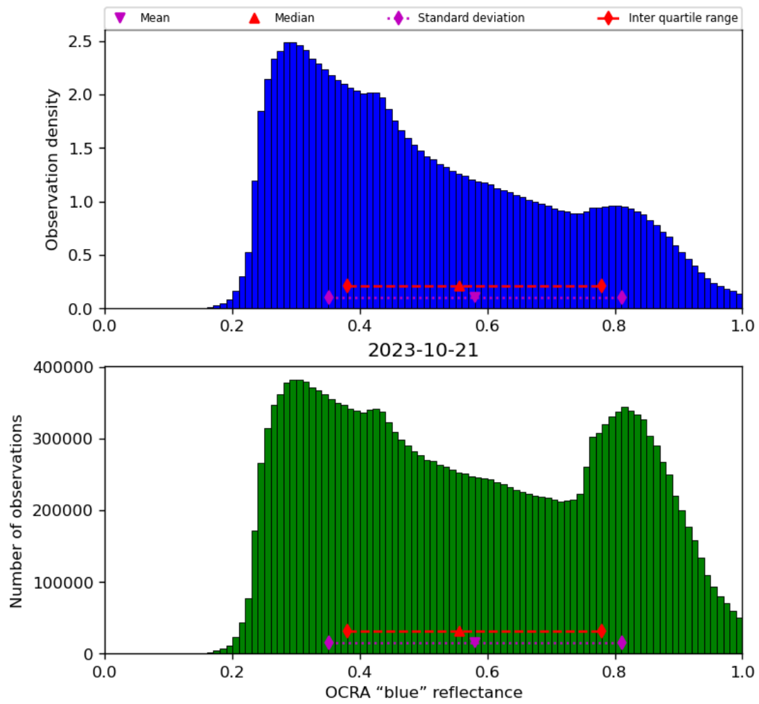
Figure 51: Histogram of “OCRA “blue” reflectance” for 2023-10-20 to 2023-10-22
