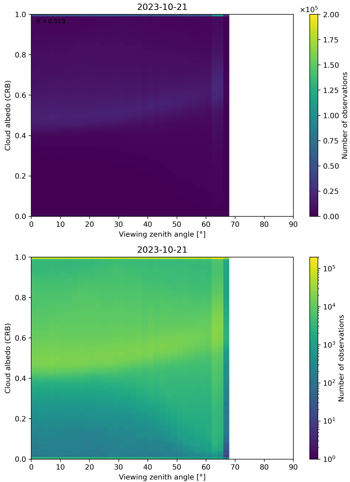
Figure 106: Scatter density plot of “Viewing zenith angle” against “Cloud albedo (CRB)” for 2023-10-20 to 2023-10-22.
