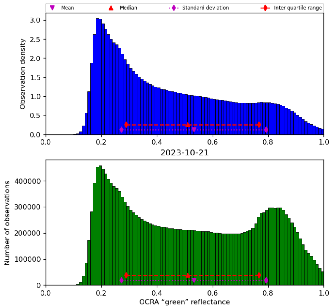
Figure 52: Histogram of “OCRA “green” reflectance” for 2023-10-20 to 2023-10-22
