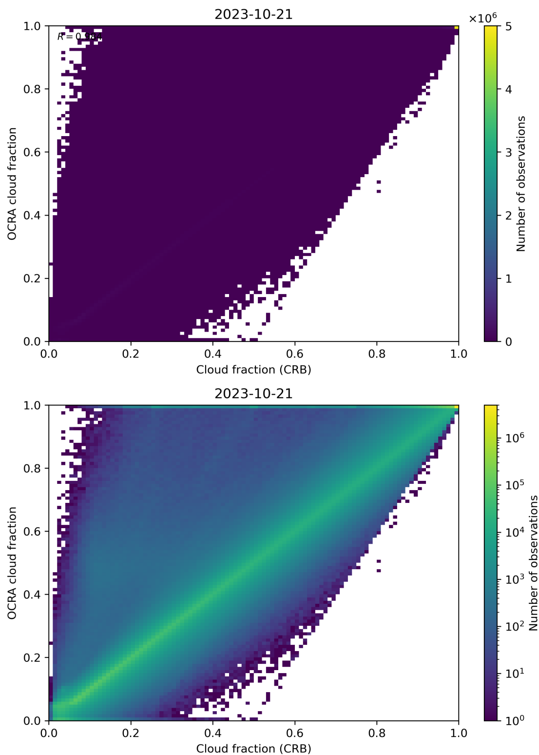
Figure 78: Scatter density plot of “Cloud fraction (CRB)” against “OCRA cloud fraction” for 2023-10-20 to 2023-10-22.
