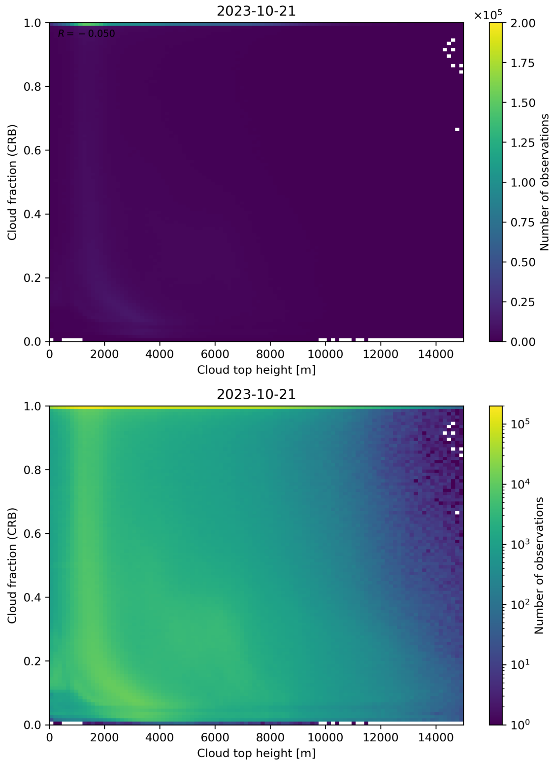
Figure 88: Scatter density plot of “Cloud top height” against “Cloud fraction (CRB)” for 2023-10-20 to 2023-10-22.
