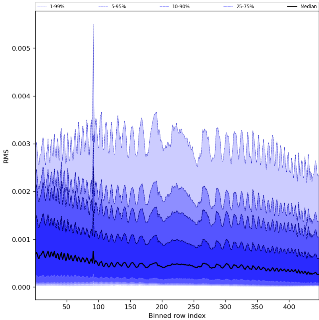
Figure 63: Along track statistics of “RMS” for 2023-10-20 to 2023-10-22
