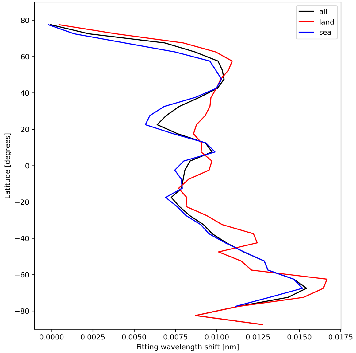
Figure 33: Zonal average of “Fitting wavelength shift” for 2023-10-20 to 2023-10-22.
