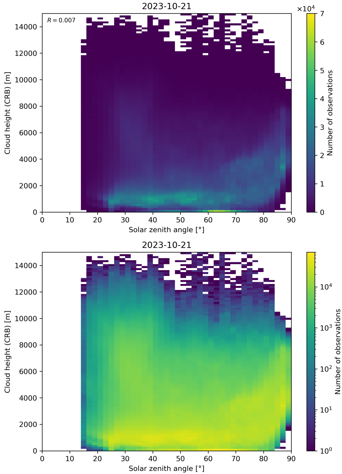
Figure 102: Scatter density plot of “Solar zenith angle” against “Cloud height (CRB)” for 2023-10-20 to 2023-10-22.
