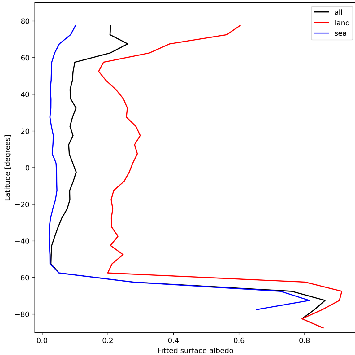
Figure 29: Zonal average of “Fitted surface albedo” for 2023-10-20 to 2023-10-22.
