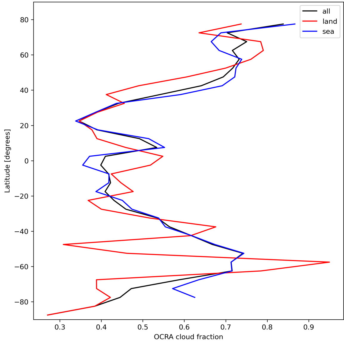
Figure 34: Zonal average of “OCRA cloud fraction” for 2023-10-20 to 2023-10-22.
