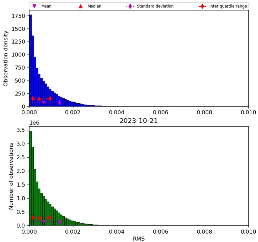
Figure 47: Histogram of “RMS” for 2023-10-20 to 2023-10-22
