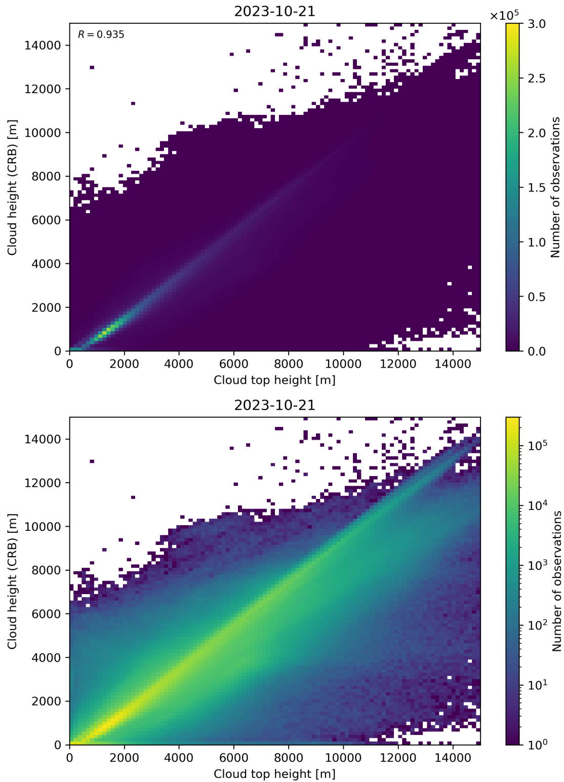
Figure 89: Scatter density plot of “Cloud top height” against “Cloud height (CRB)” for 2023-10-20 to 2023-10-22.
