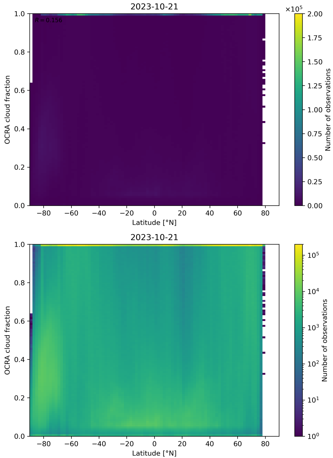
Figure 93: Scatter density plot of “Latitude” against “OCRA cloud fraction” for 2023-10-20 to 2023-10-22.
