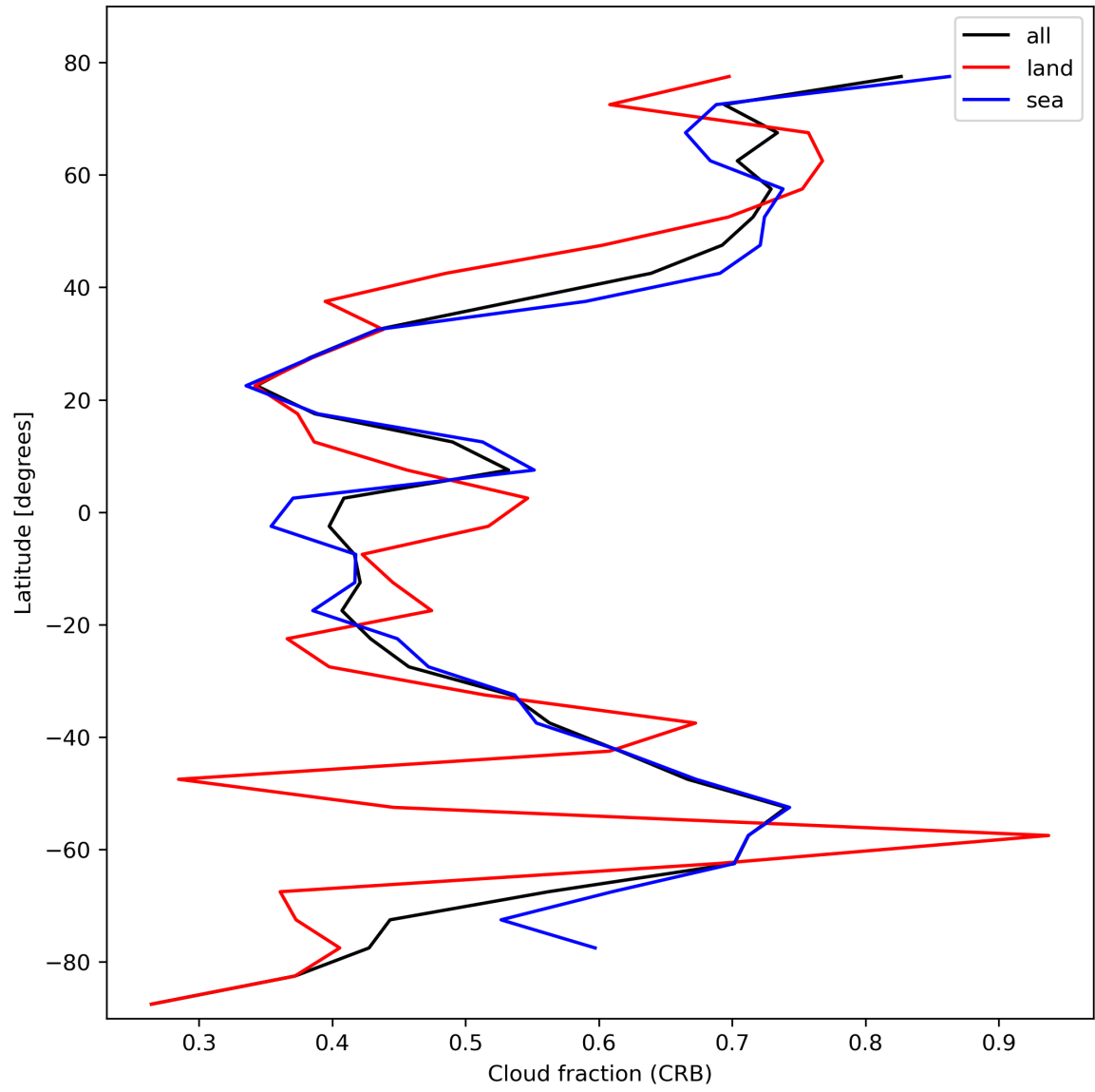
Figure 26: Zonal average of “Cloud fraction (CRB)” for 2023-10-20 to 2023-10-22.
