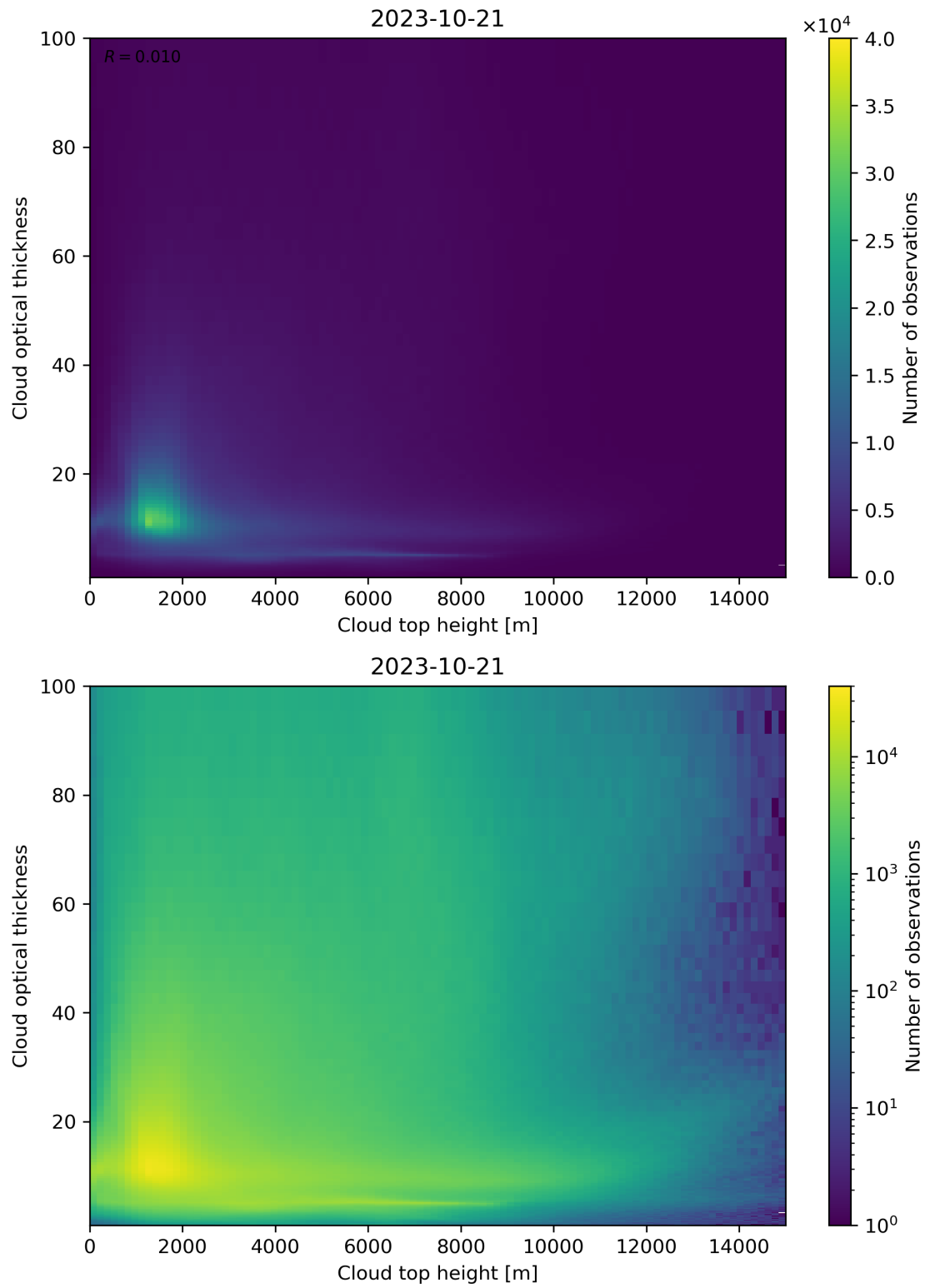
Figure 90: Scatter density plot of “Cloud top height” against “Cloud optical thickness” for 2023-10-20 to 2023-10-22.
