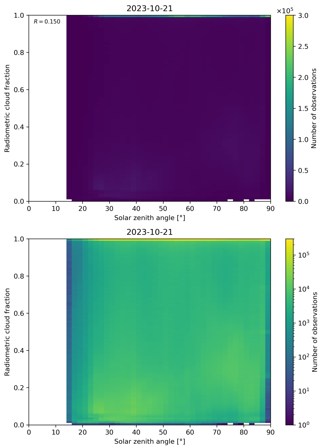
Figure 99: Scatter density plot of “Solar zenith angle” against “Radiometric cloud fraction” for 2023-10-20 to 2023-10-22.
