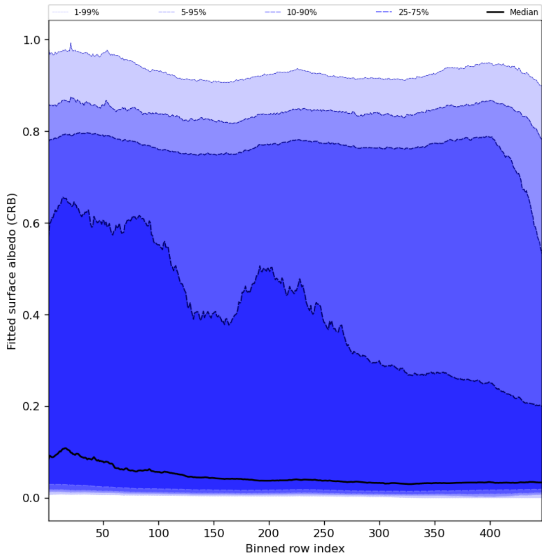
Figure 62: Along track statistics of “Fitted surface albedo (CRB)” for 2023-10-22 to 2023-10-23
