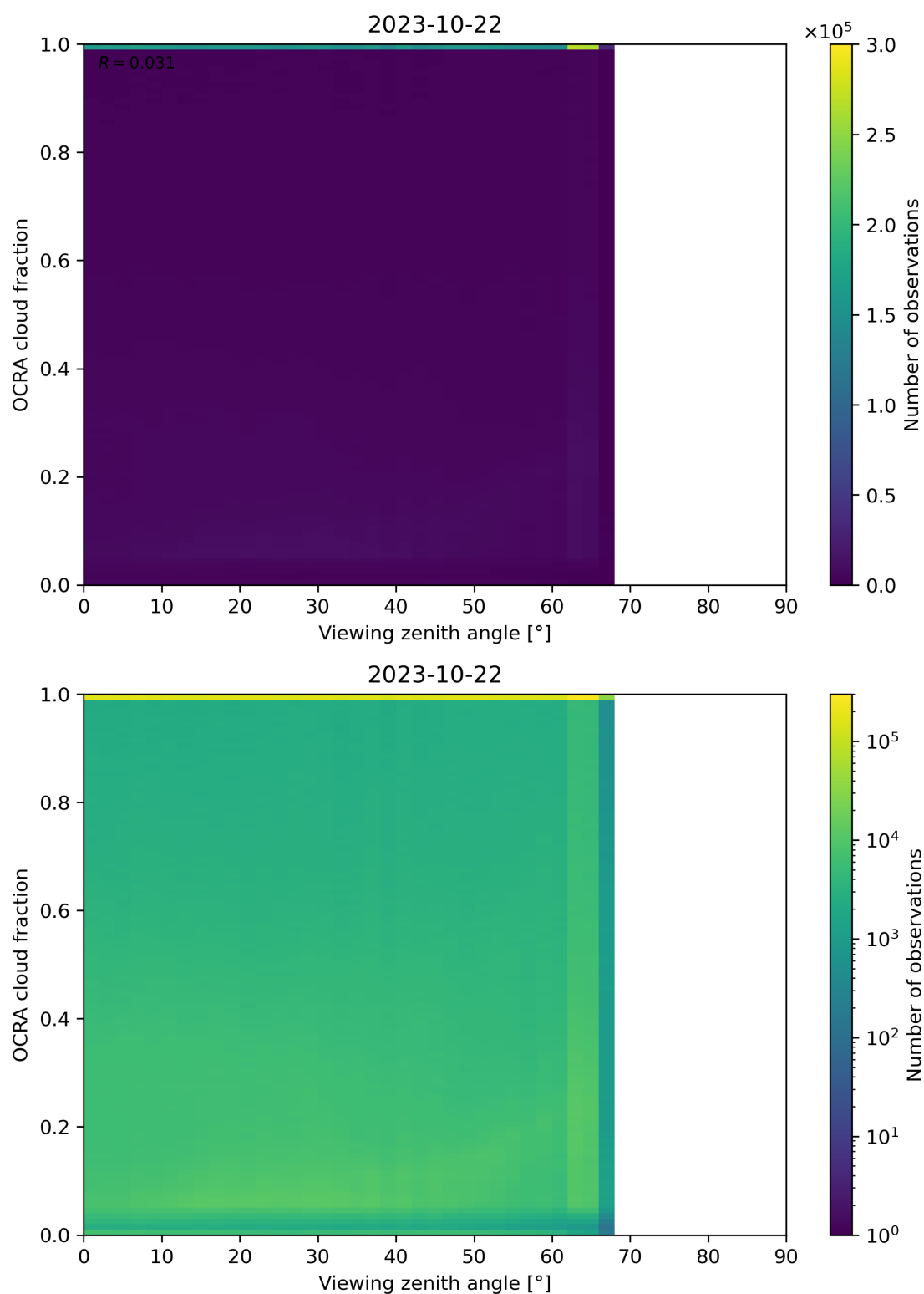
Figure 108: Scatter density plot of “Viewing zenith angle” against “OCRA cloud fraction” for 2023-10-22 to 2023-10-23.
