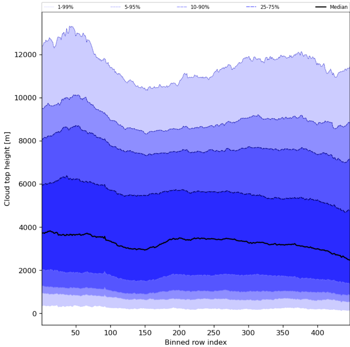
Figure 56: Along track statistics of “Cloud top height” for 2023-10-22 to 2023-10-23
