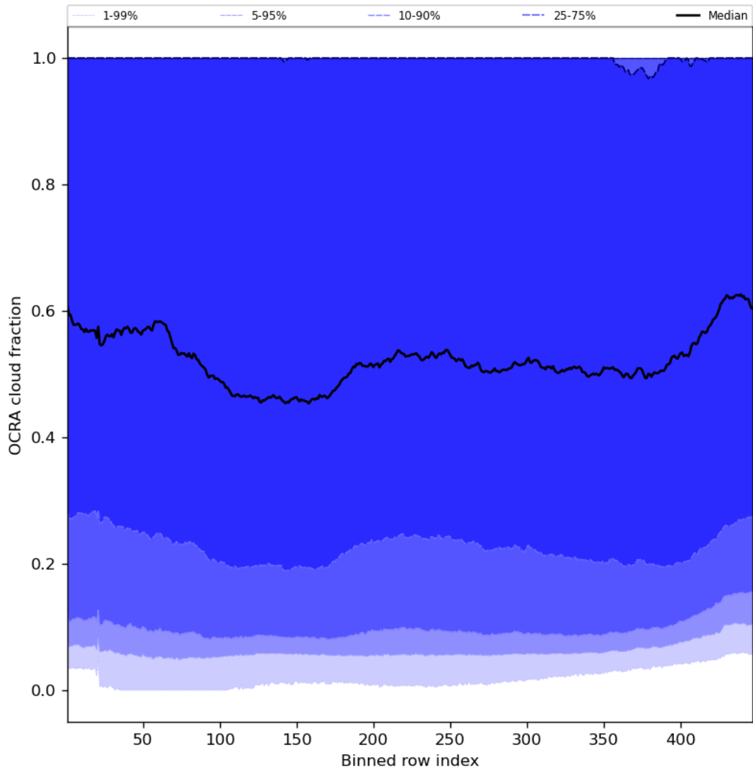
Figure 66: Along track statistics of “OCRA cloud fraction” for 2023-10-22 to 2023-10-23
