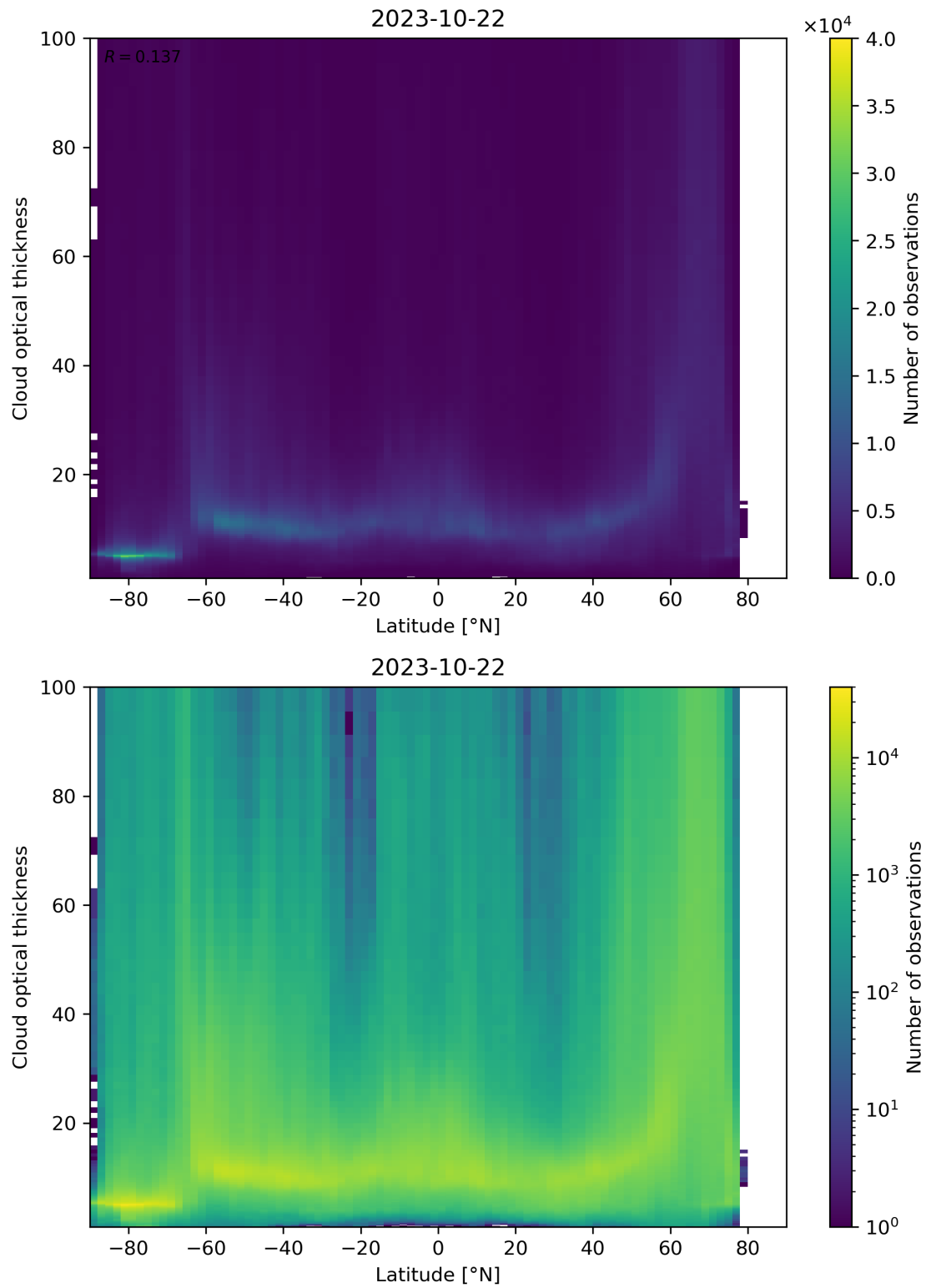
Figure 96: Scatter density plot of “Latitude” against “Cloud optical thickness” for 2023-10-22 to 2023-10-23.
