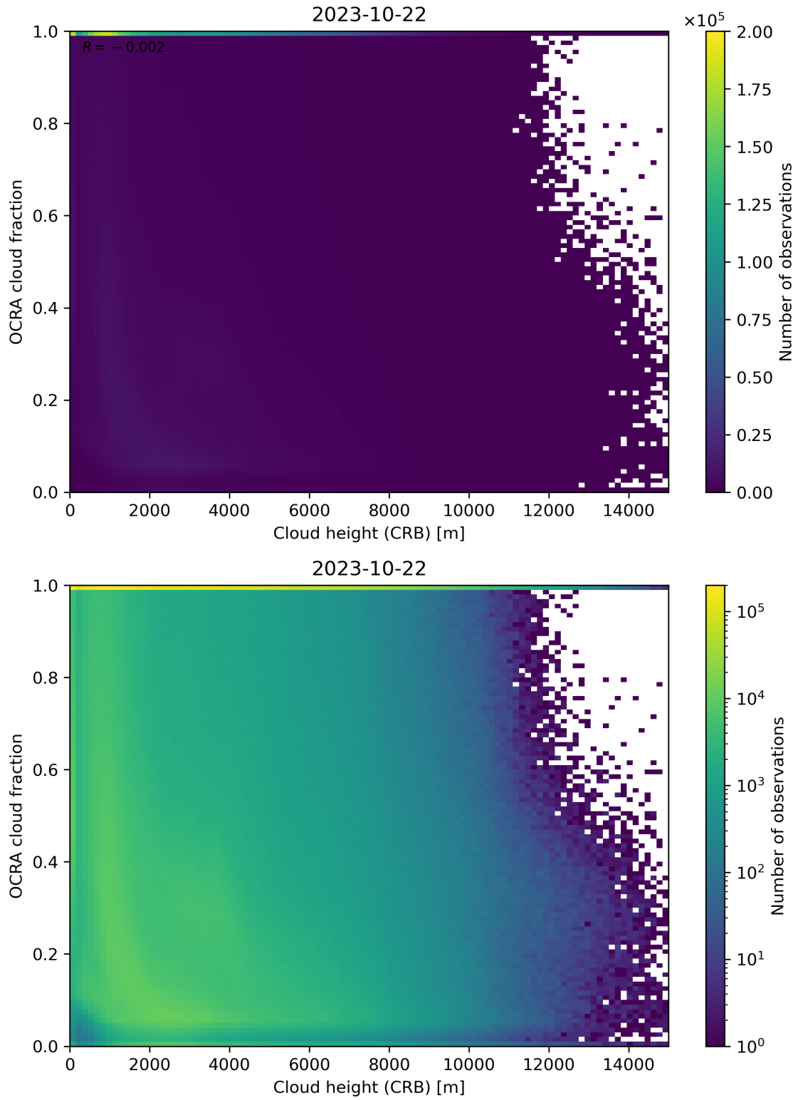
Figure 81: Scatter density plot of “Cloud height (CRB)” against “OCRA cloud fraction” for 2023-10-22 to 2023-10-23.
