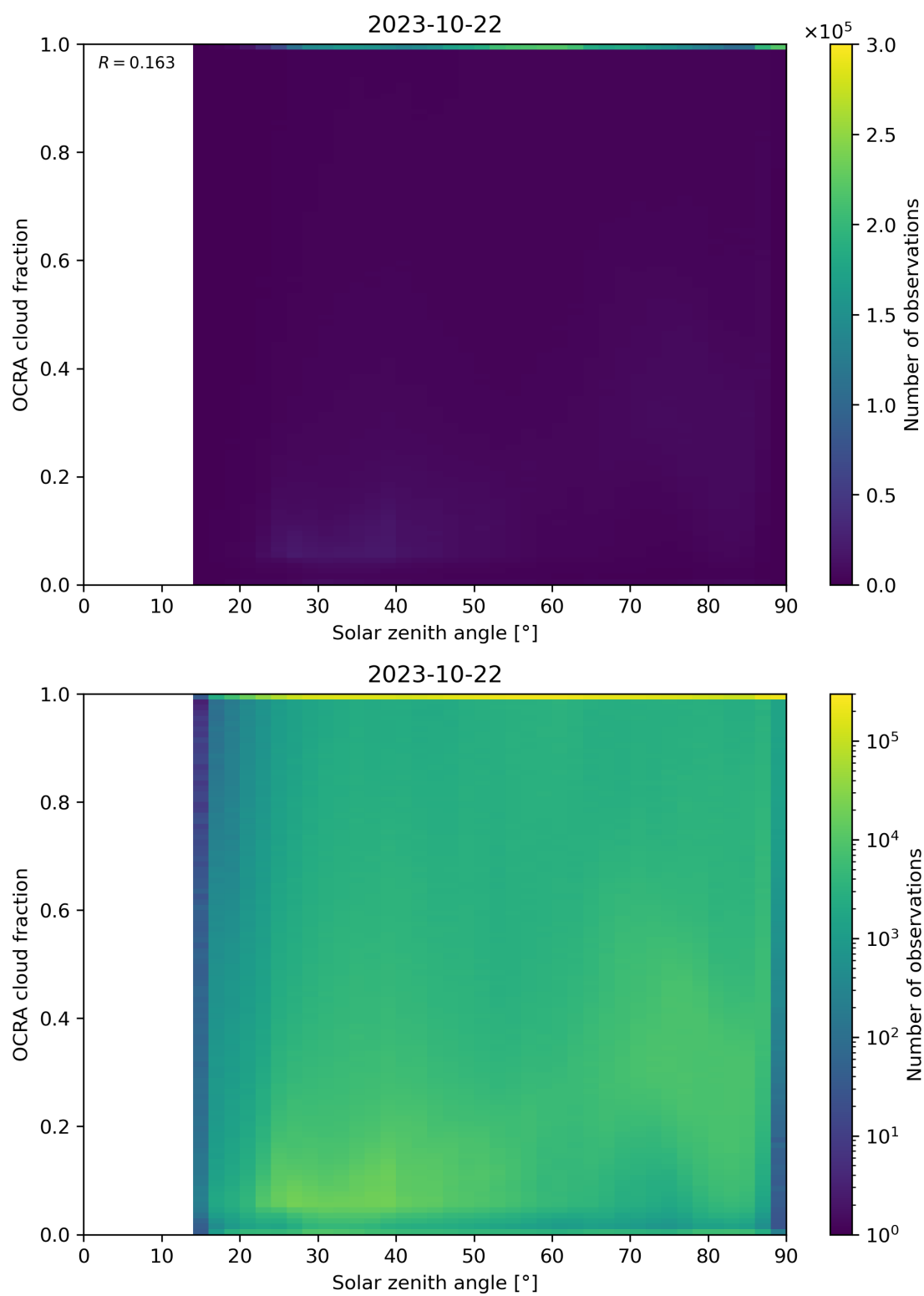
Figure 100: Scatter density plot of “Solar zenith angle” against “OCRA cloud fraction” for 2023-10-22 to 2023-10-23.
