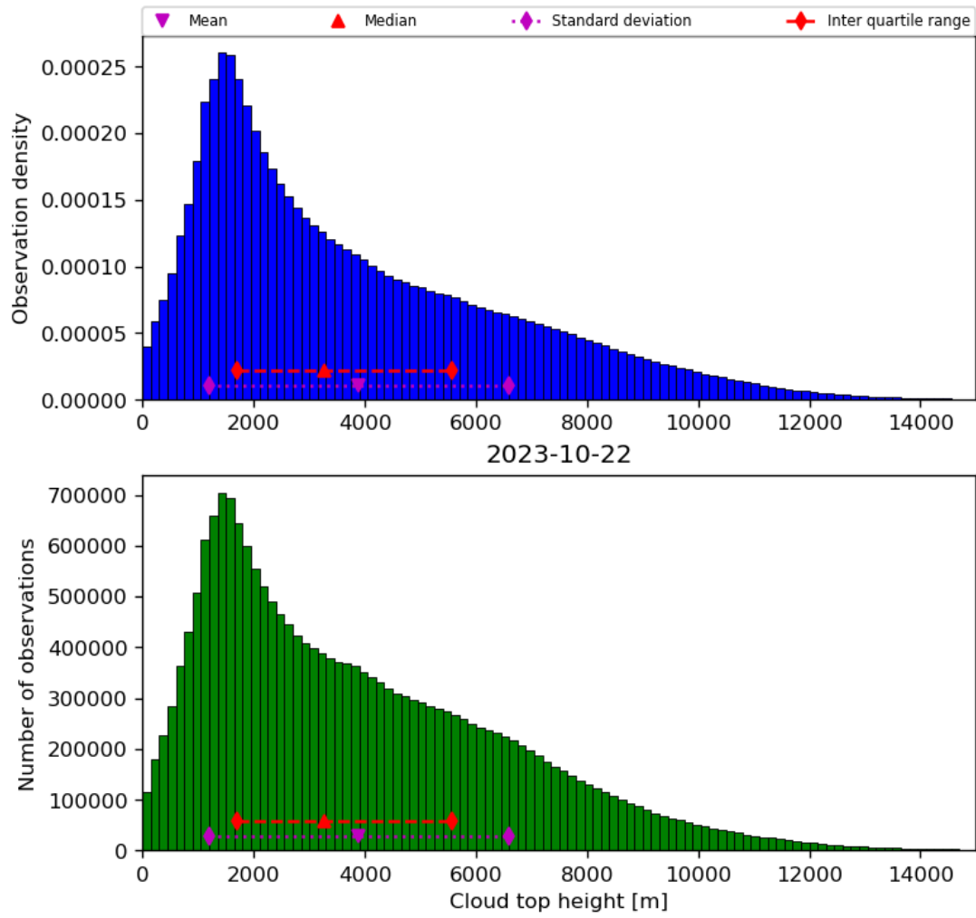
Figure 40: Histogram of “Cloud top height” for 2023-10-22 to 2023-10-23
