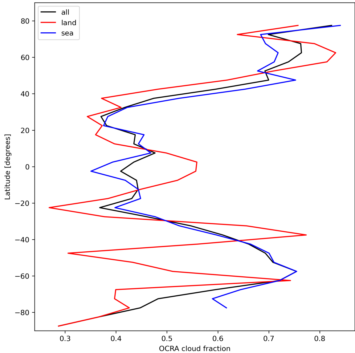
Figure 34: Zonal average of “OCRA cloud fraction” for 2023-10-22 to 2023-10-23.
