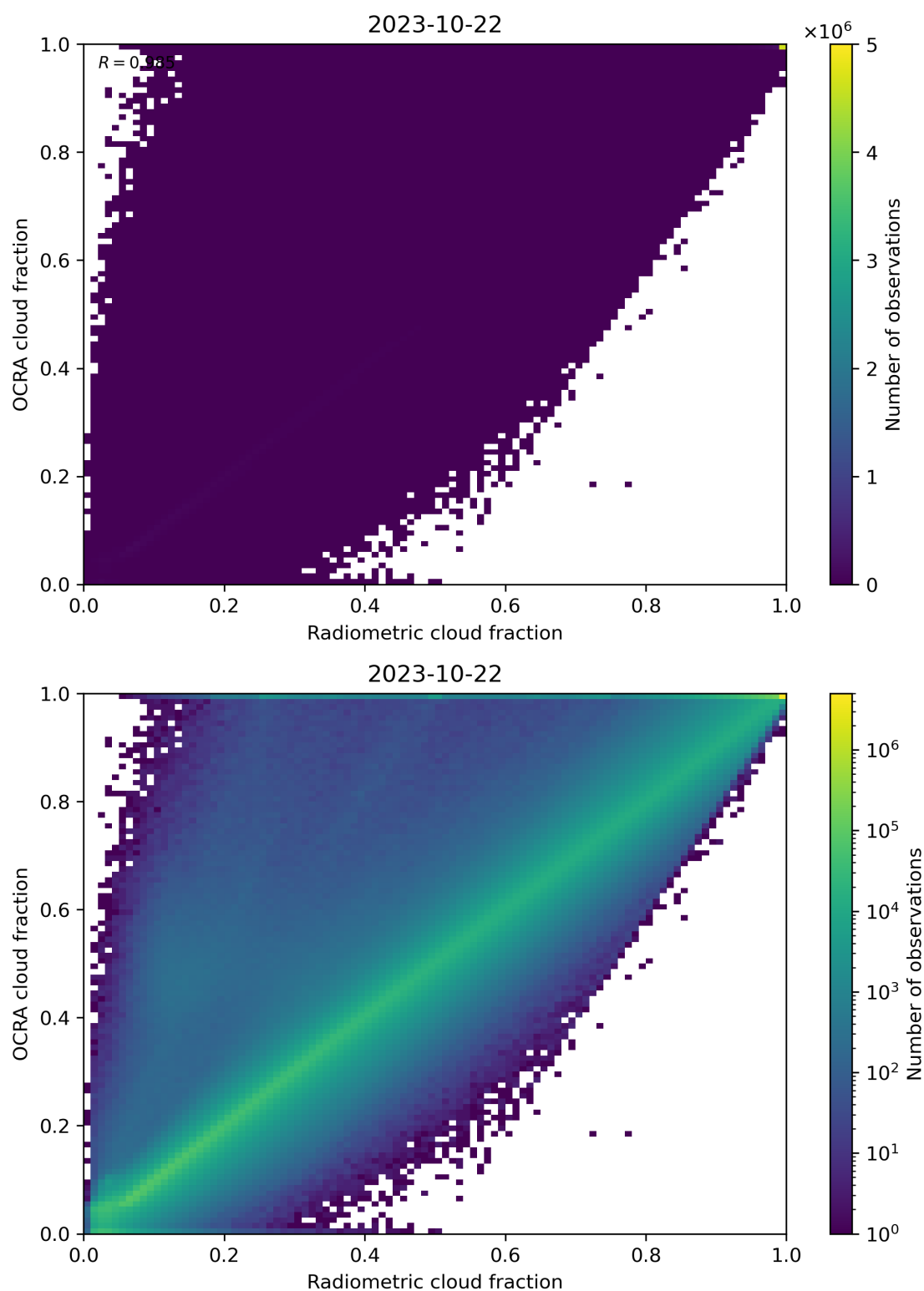
Figure 72: Scatter density plot of “Radiometric cloud fraction” against “OCRA cloud fraction” for 2023-10-22 to 2023-10-23.
