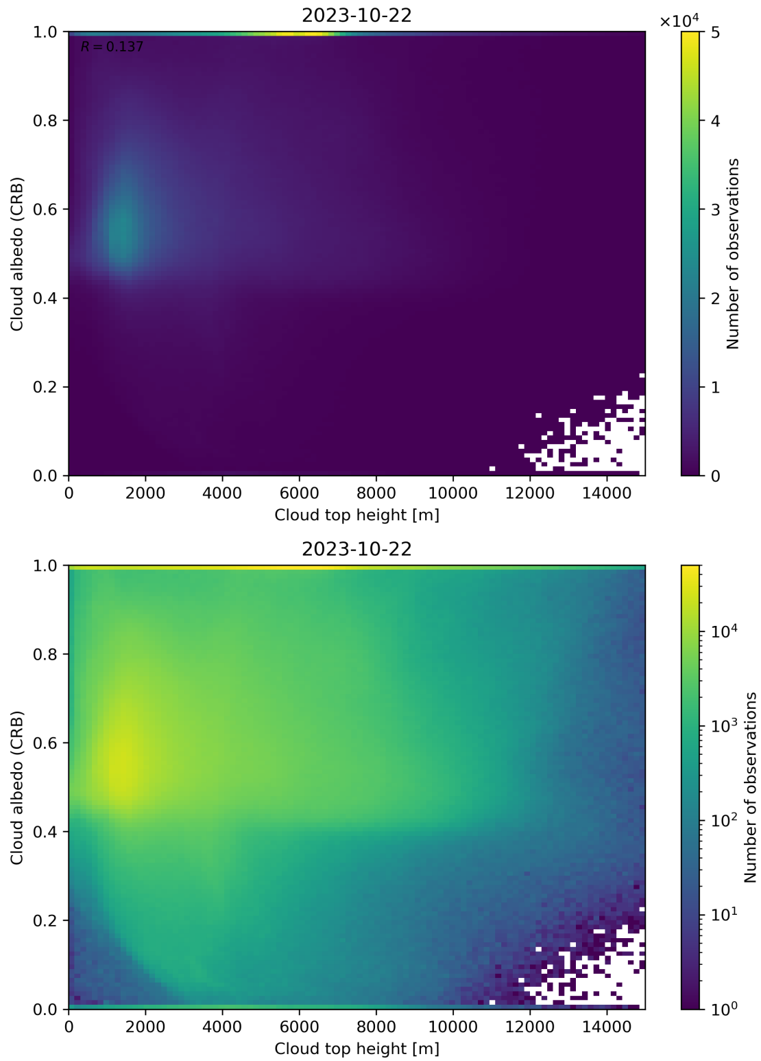
Figure 86: Scatter density plot of “Cloud top height” against “Cloud albedo (CRB)” for 2023-10-22 to 2023-10-23.
