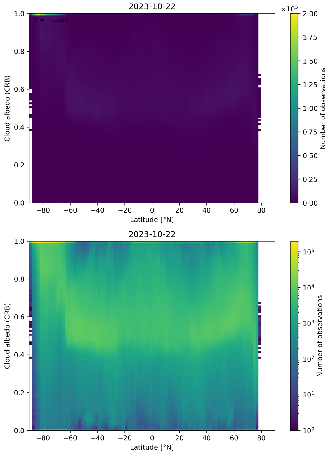
Figure 91: Scatter density plot of “Latitude” against “Cloud albedo (CRB)” for 2023-10-22 to 2023-10-23.
