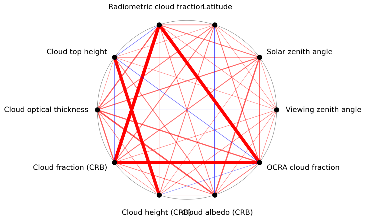
Figure 1: Map of correlation graph for 2023-10-22 to 2023-10-23.
