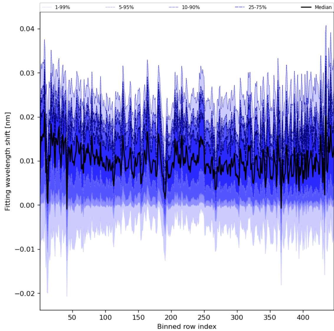
Figure 65: Along track statistics of “Fitting wavelength shift” for 2023-10-22 to 2023-10-23
