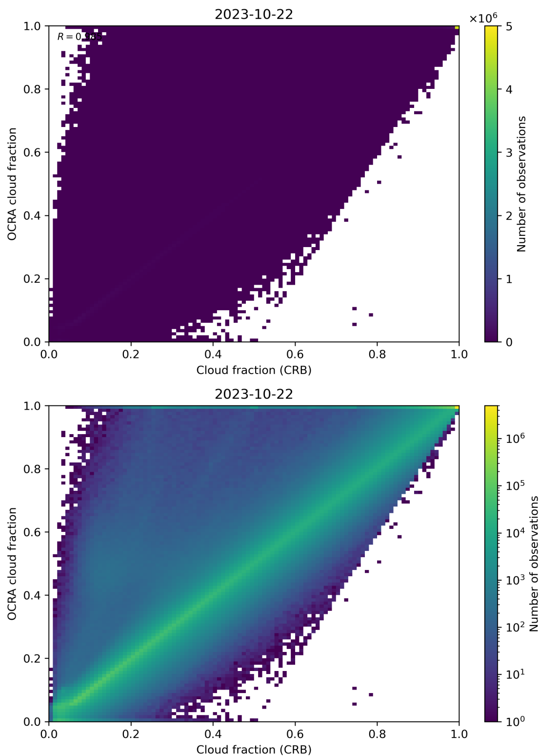
Figure 78: Scatter density plot of “Cloud fraction (CRB)” against “OCRA cloud fraction” for 2023-10-22 to 2023-10-23.
