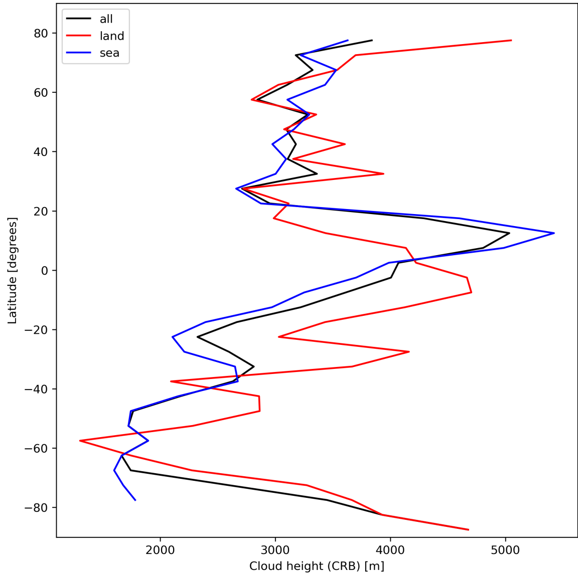
Figure 27: Zonal average of “Cloud height (CRB)” for 2023-10-22 to 2023-10-23.
