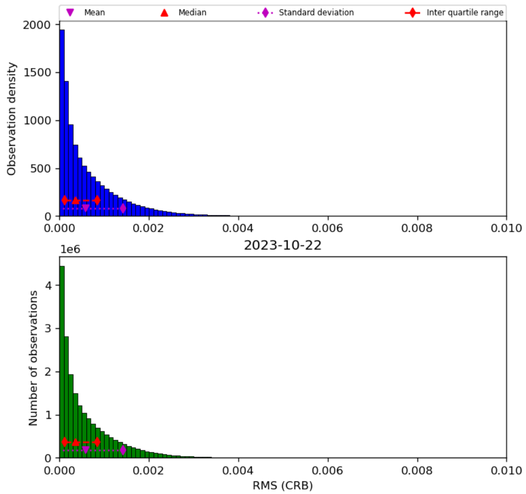
Figure 48: Histogram of “RMS (CRB)” for 2023-10-22 to 2023-10-23
