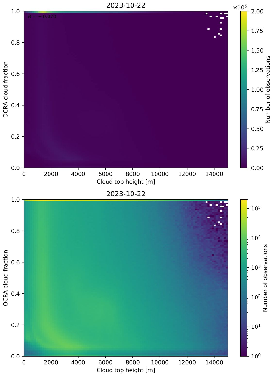
Figure 87: Scatter density plot of “Cloud top height” against “OCRA cloud fraction” for 2023-10-22 to 2023-10-23.
