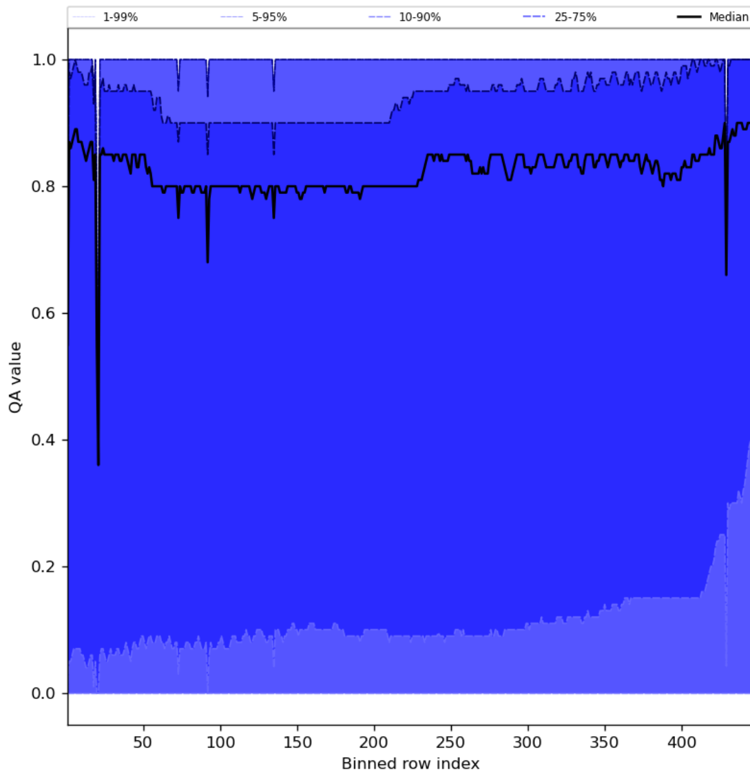
Figure 54: Along track statistics of “QA value” for 2023-10-22 to 2023-10-23
