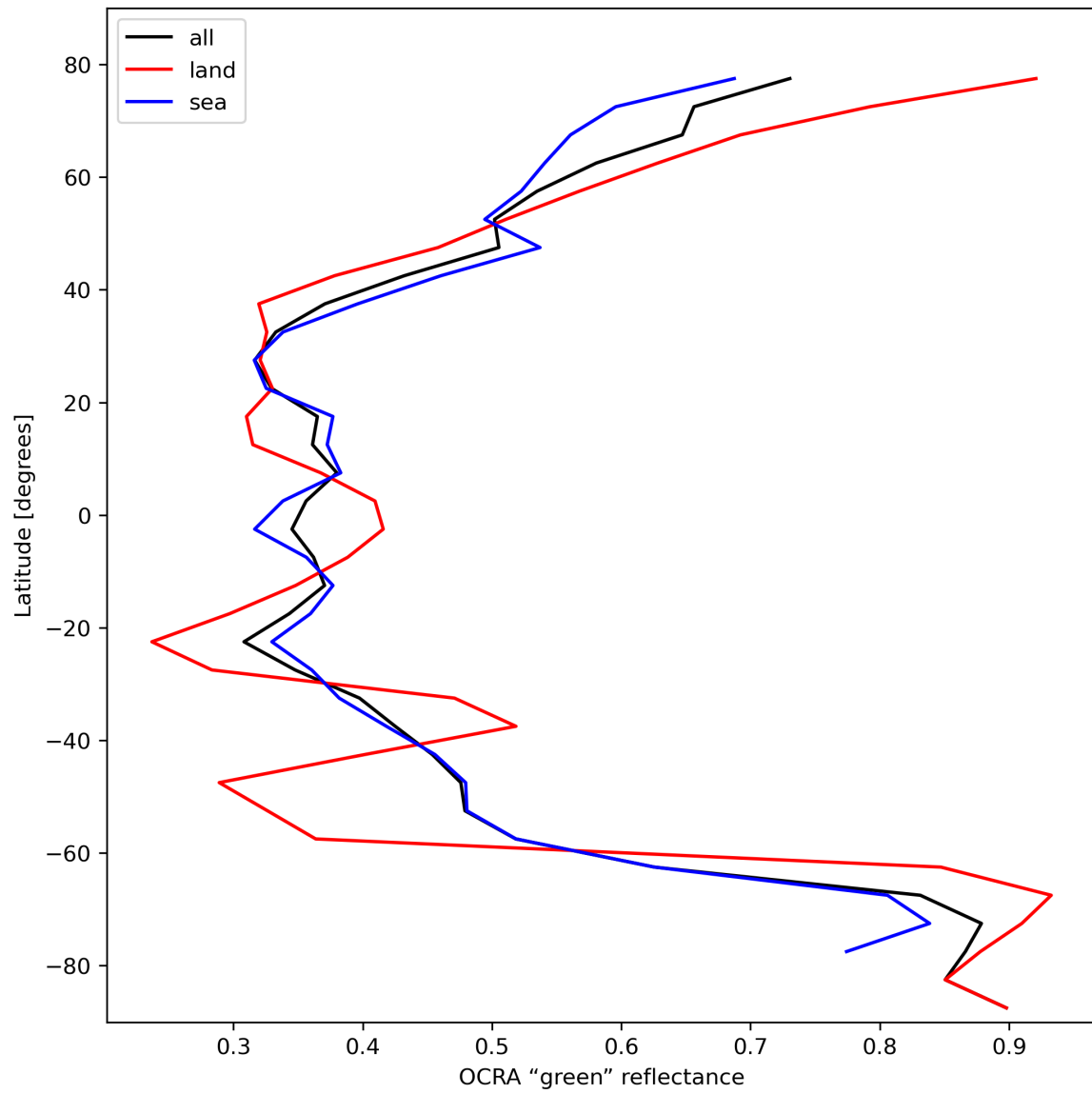
Figure 36: Zonal average of “OCRA “green” reflectance” for 2023-10-22 to 2023-10-23.
