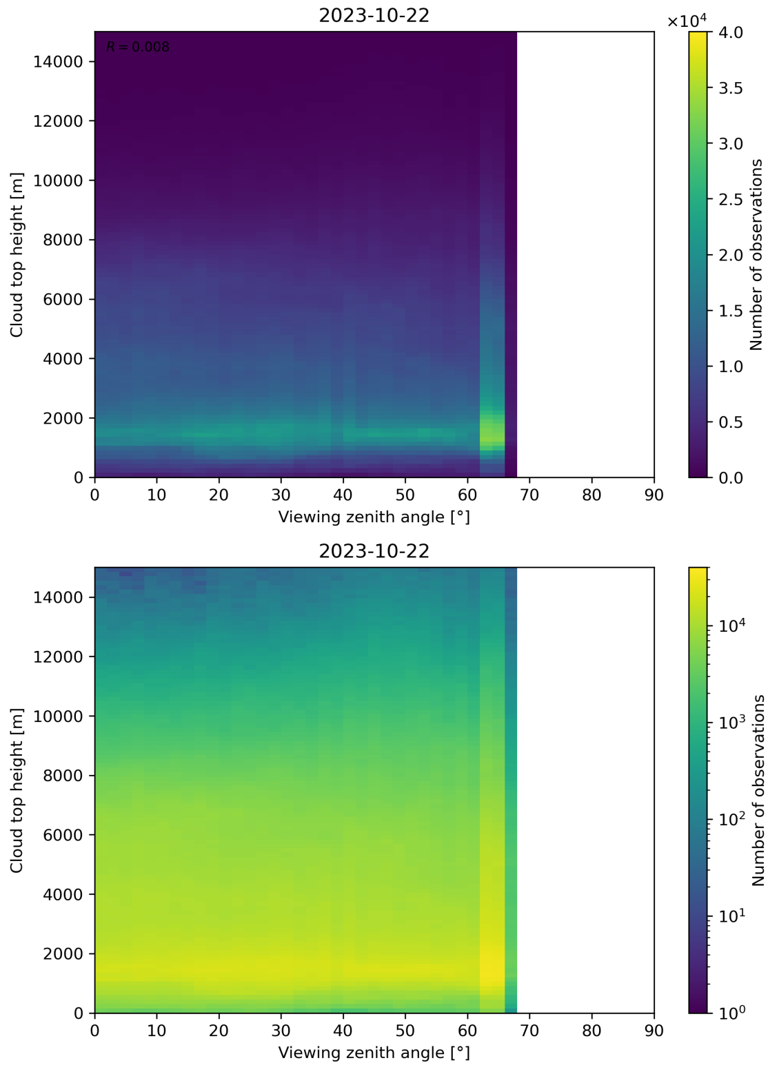
Figure 112: Scatter density plot of “Viewing zenith angle” against “Cloud top height” for 2023-10-22 to 2023-10-23.
