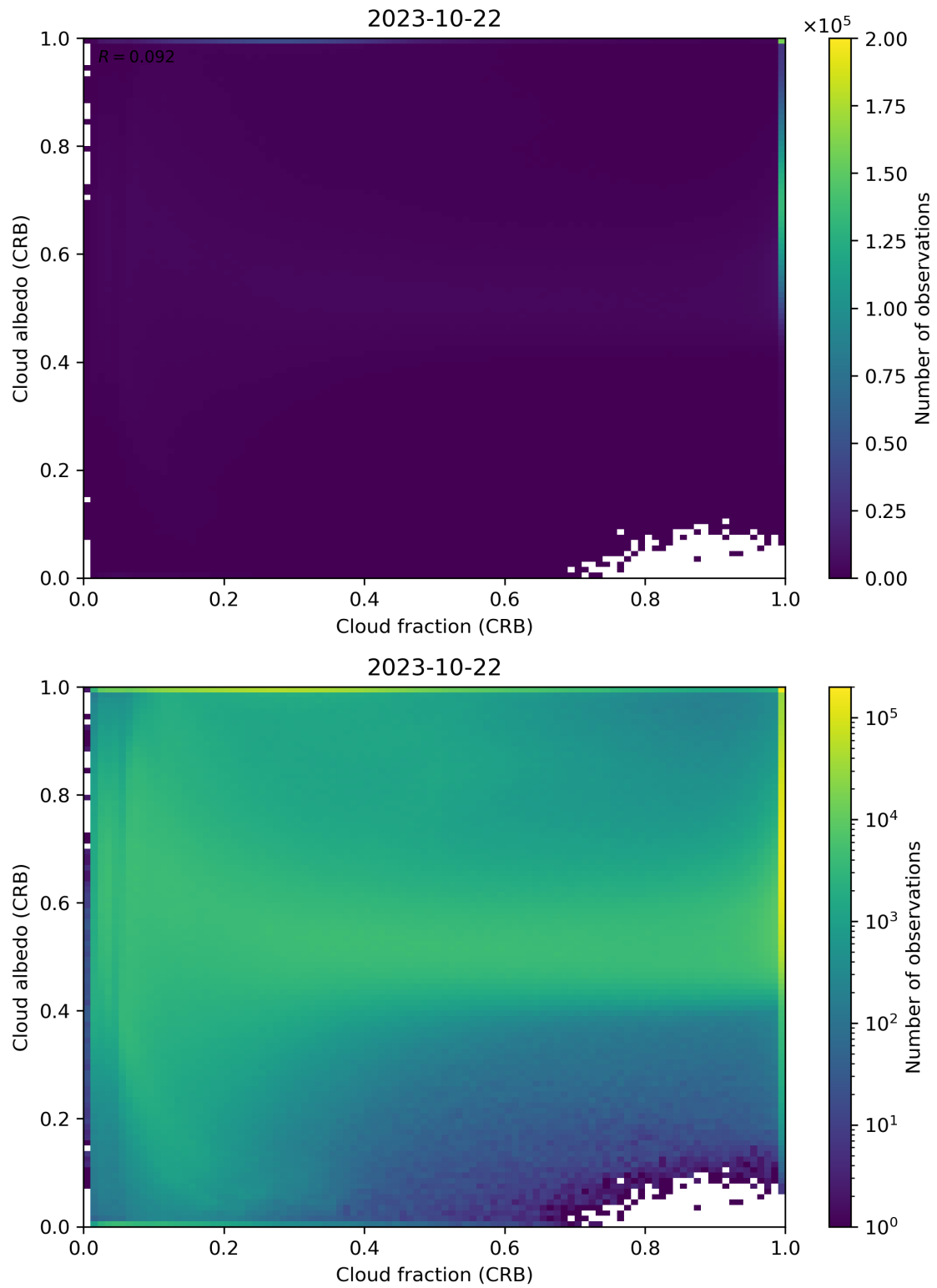
Figure 77: Scatter density plot of “Cloud fraction (CRB)” against “Cloud albedo (CRB)” for 2023-10-22 to 2023-10-23.
