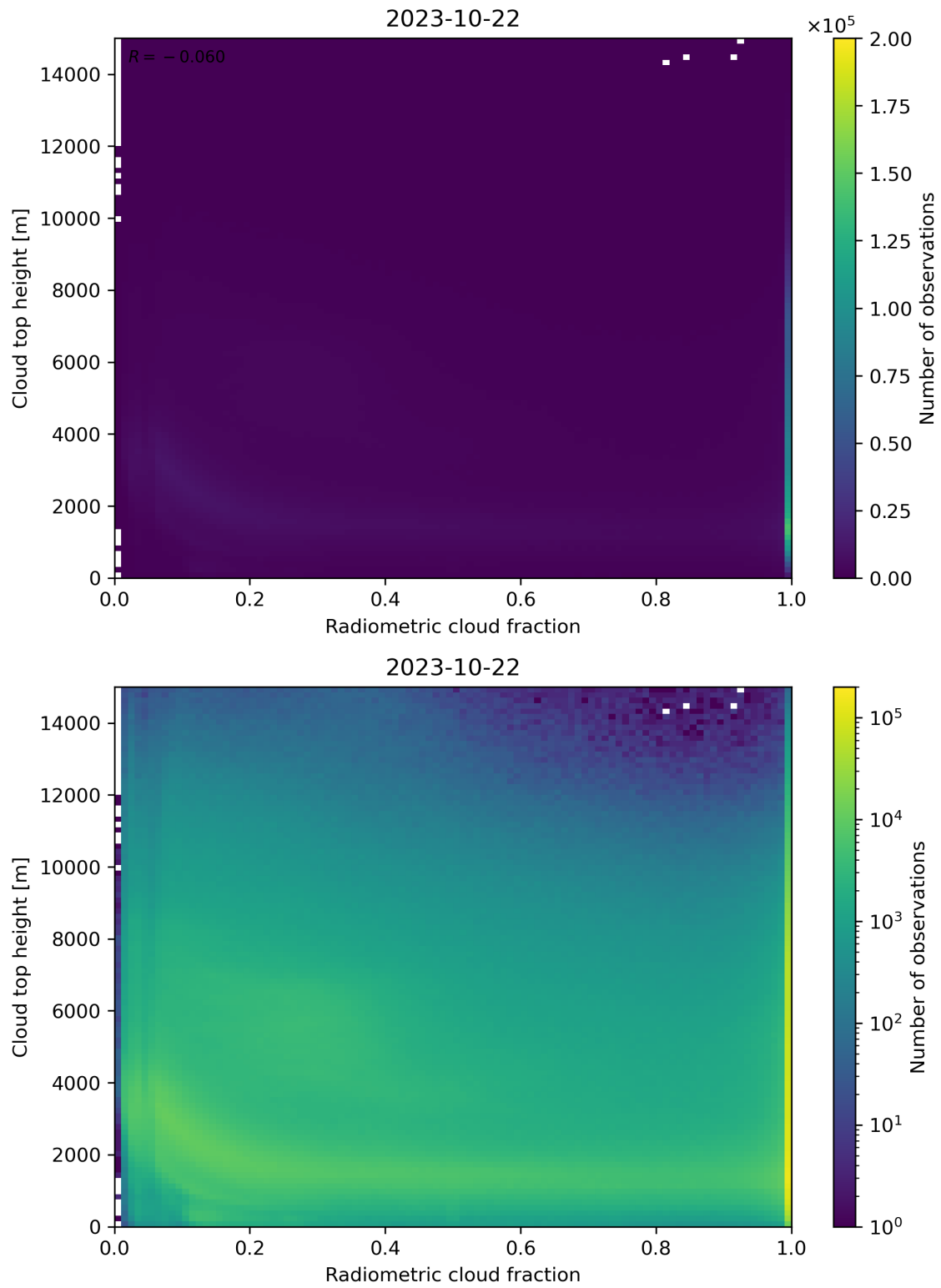
Figure 76: Scatter density plot of “Radiometric cloud fraction” against “Cloud top height” for 2023-10-22 to 2023-10-23.
