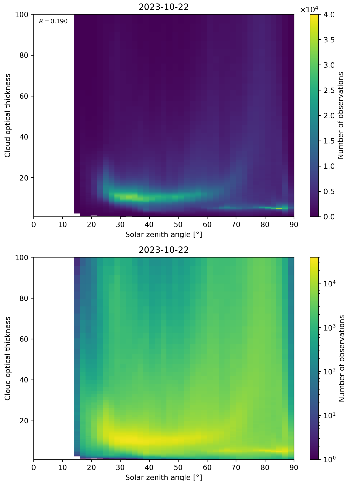
Figure 103: Scatter density plot of “Solar zenith angle” against “Cloud optical thickness” for 2023-10-22 to 2023-10-23.
