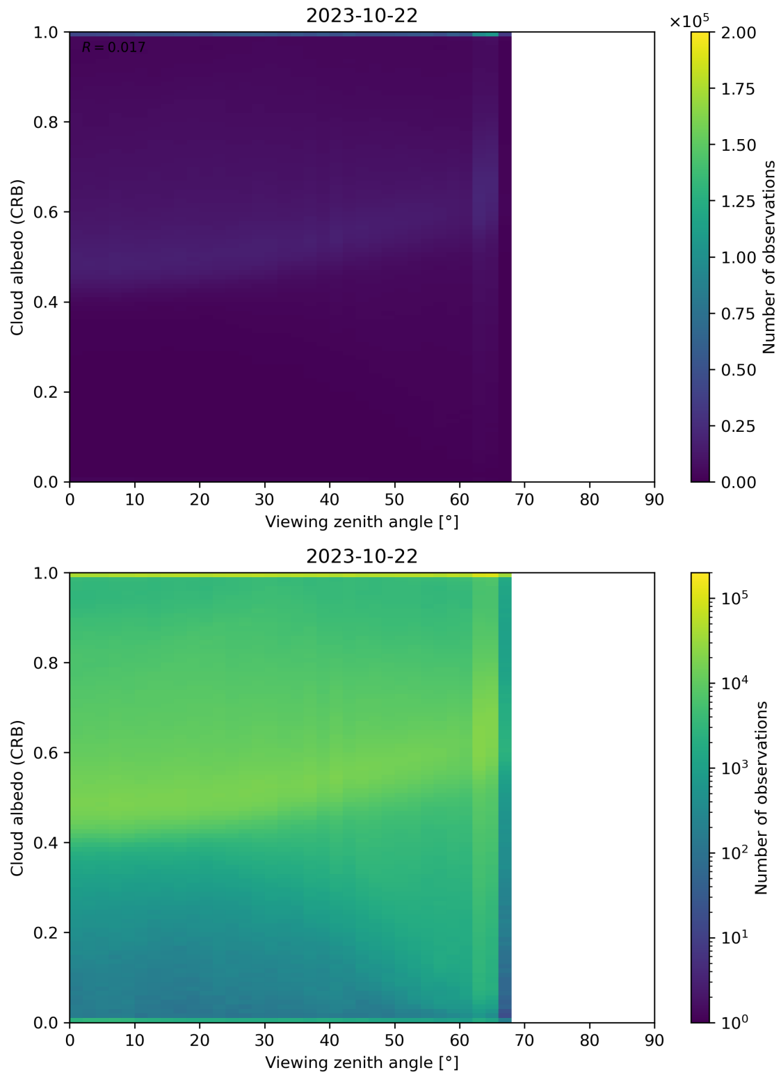
Figure 106: Scatter density plot of “Viewing zenith angle” against “Cloud albedo (CRB)” for 2023-10-22 to 2023-10-23.
