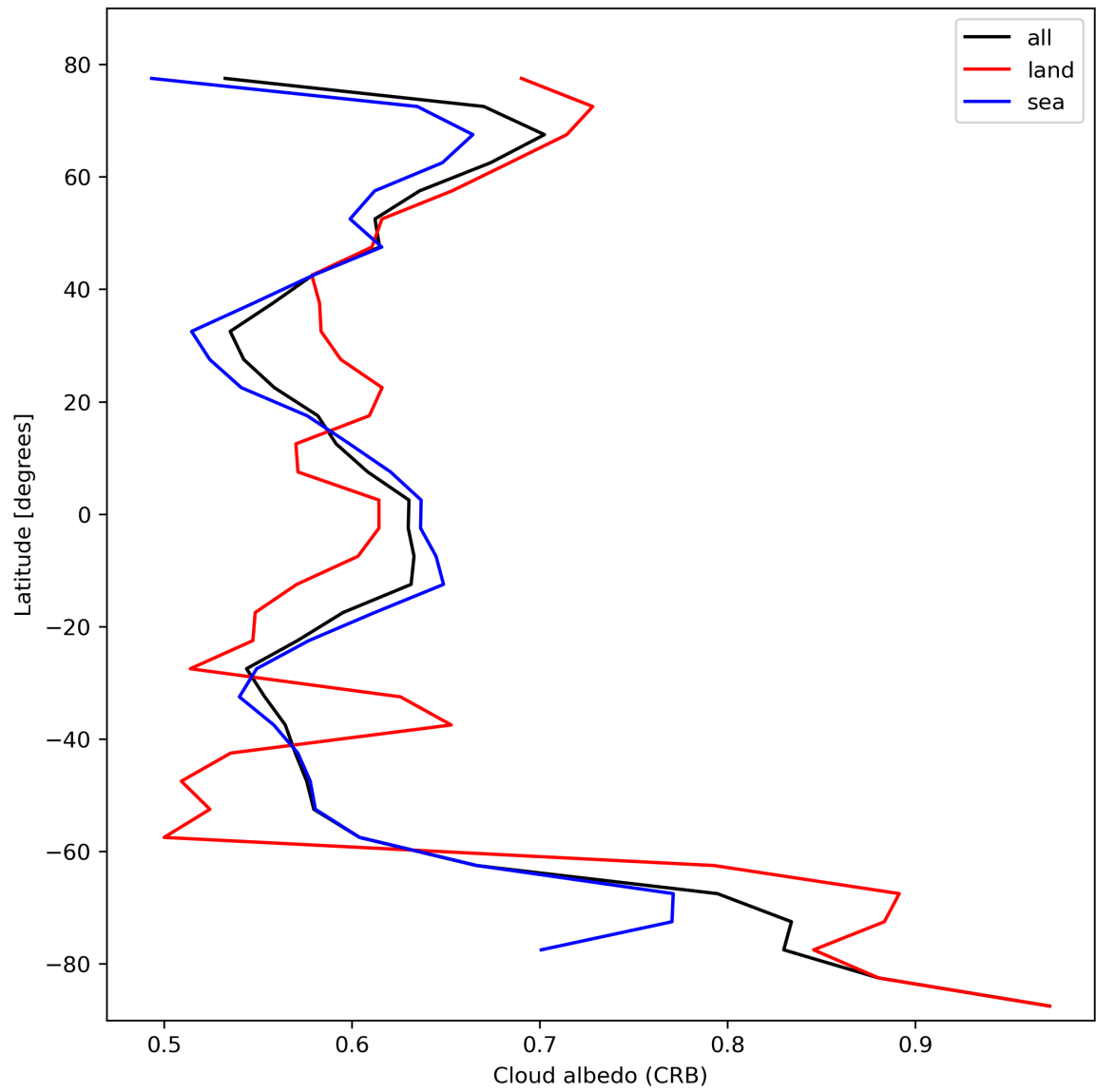
Figure 28: Zonal average of “Cloud albedo (CRB)” for 2023-10-22 to 2023-10-23.
