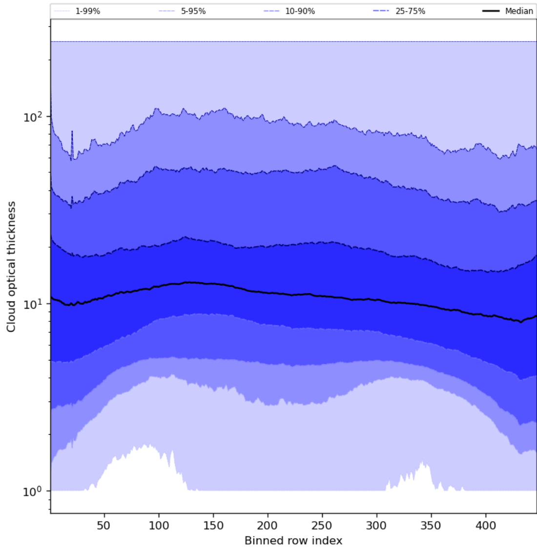
Figure 57: Along track statistics of “Cloud optical thickness” for 2023-10-22 to 2023-10-23
