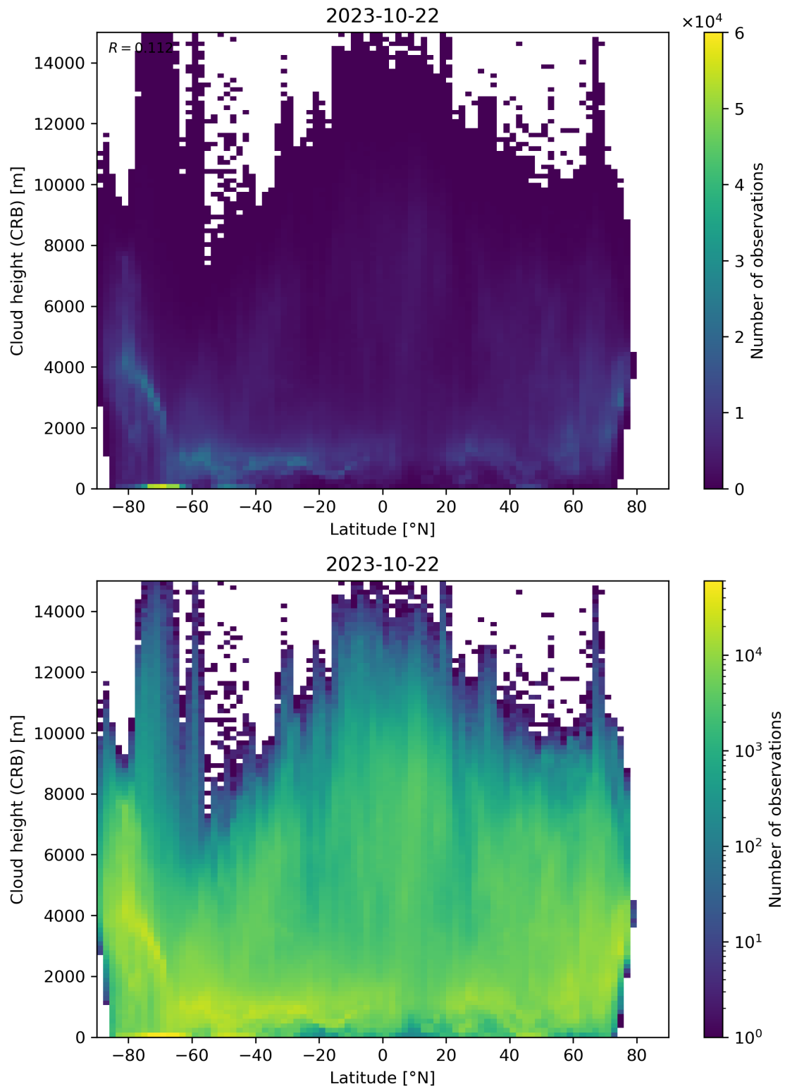
Figure 95: Scatter density plot of “Latitude” against “Cloud height (CRB)” for 2023-10-22 to 2023-10-23.
