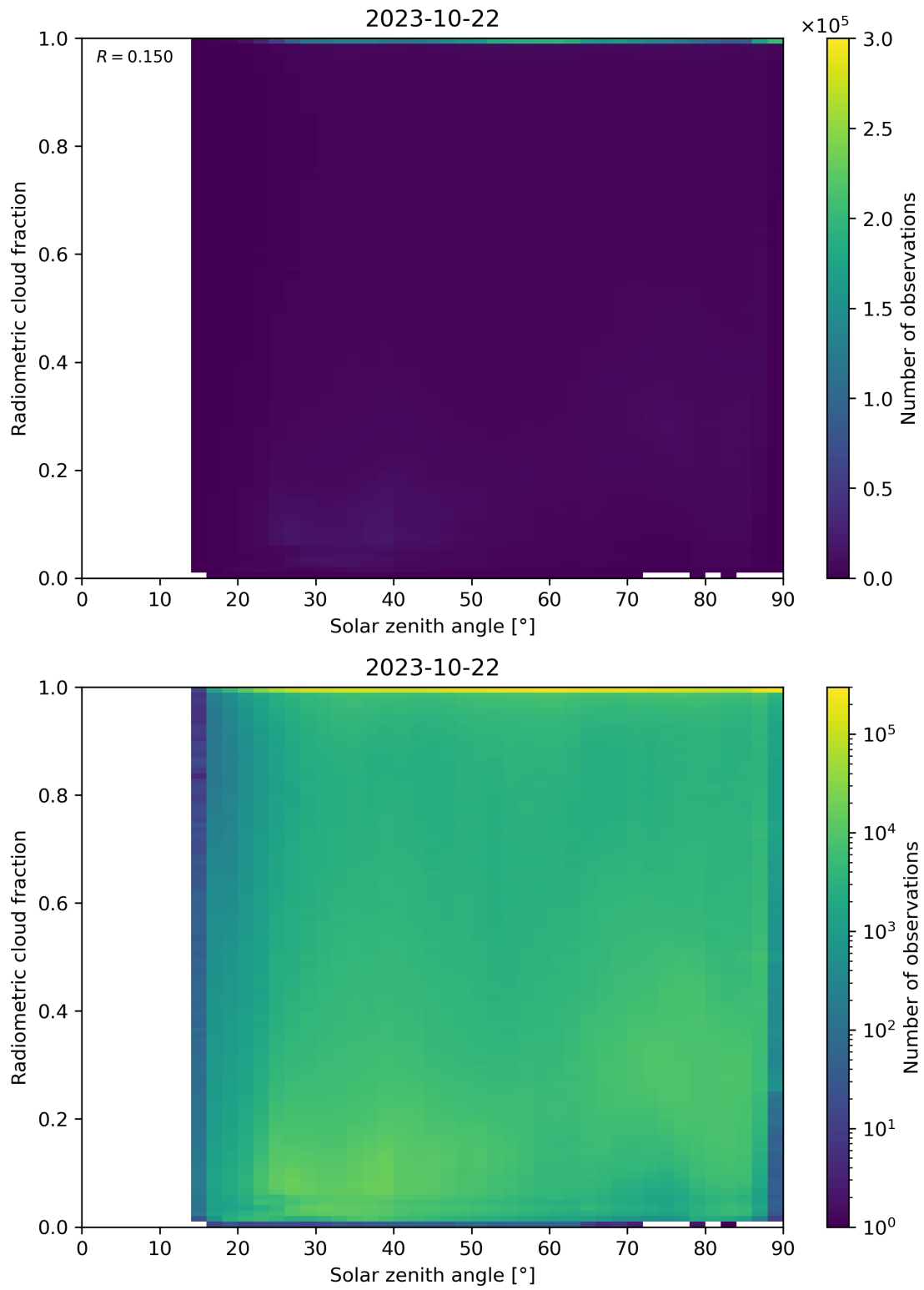
Figure 99: Scatter density plot of “Solar zenith angle” against “Radiometric cloud fraction” for 2023-10-22 to 2023-10-23.
