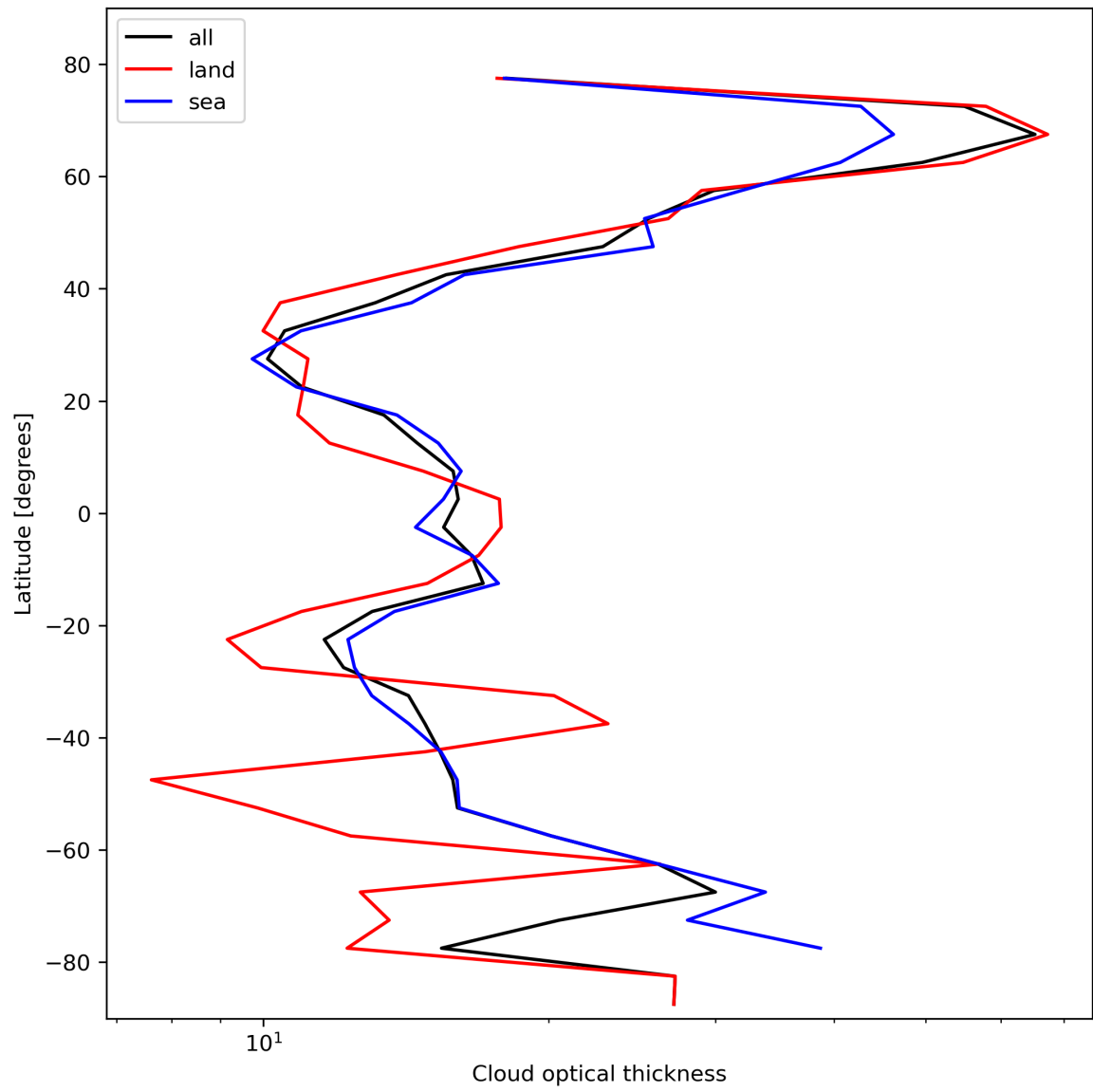
Figure 25: Zonal average of “Cloud optical thickness” for 2023-10-22 to 2023-10-23.
