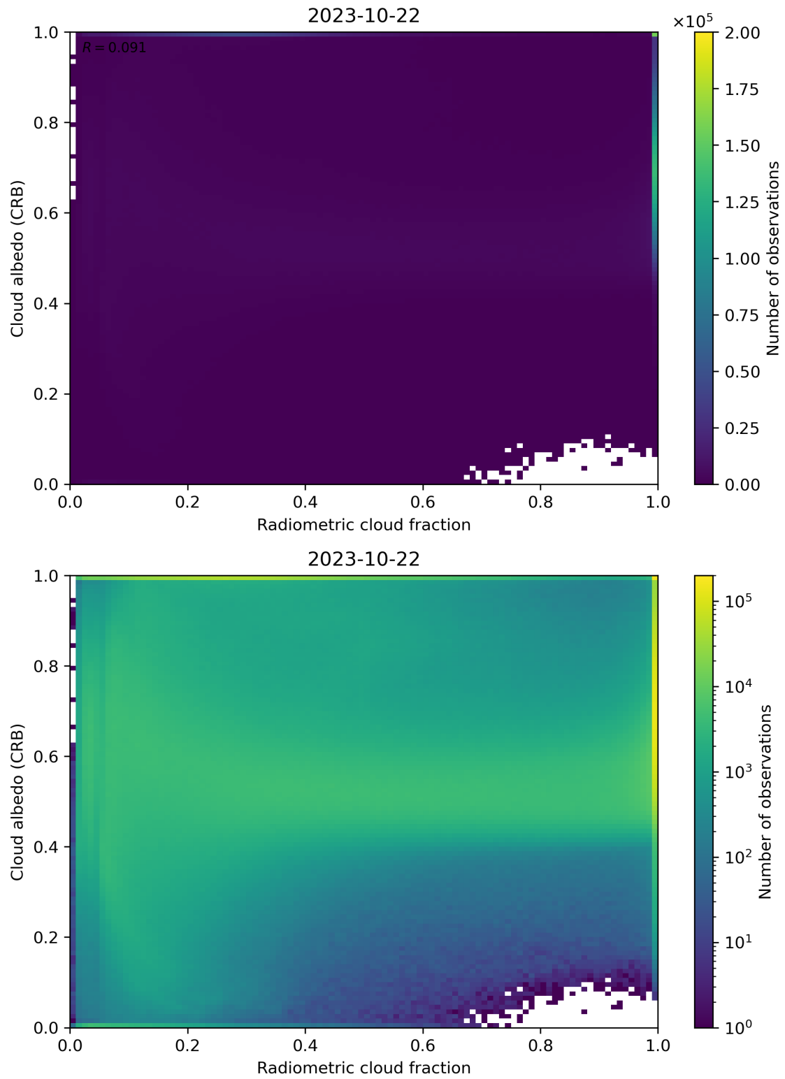
Figure 71: Scatter density plot of “Radiometric cloud fraction” against “Cloud albedo (CRB)” for 2023-10-22 to 2023-10-23.
