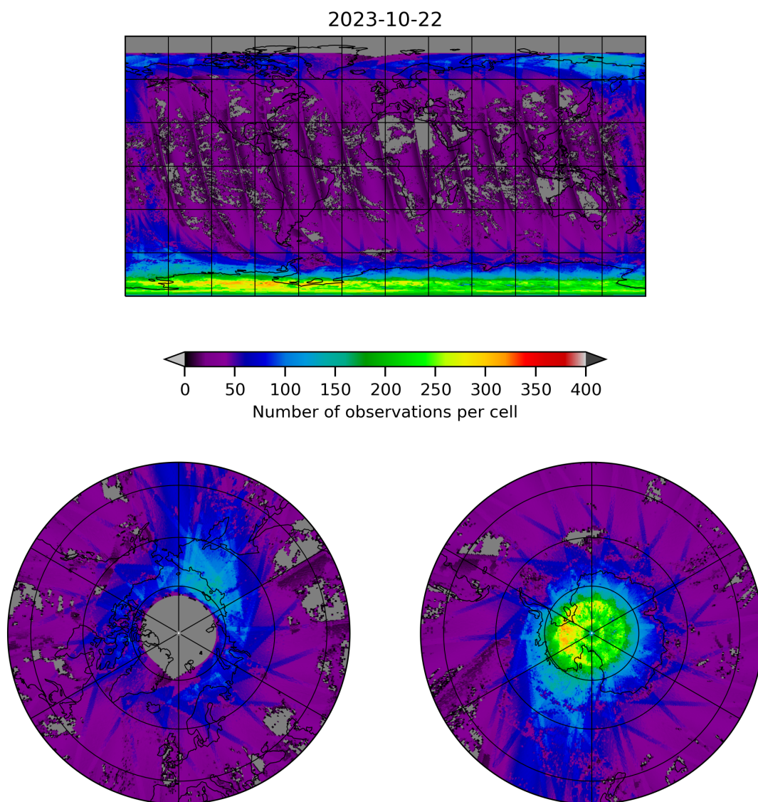
Figure 21: Map of the number of observations for 2023-10-22 to 2023-10-23
