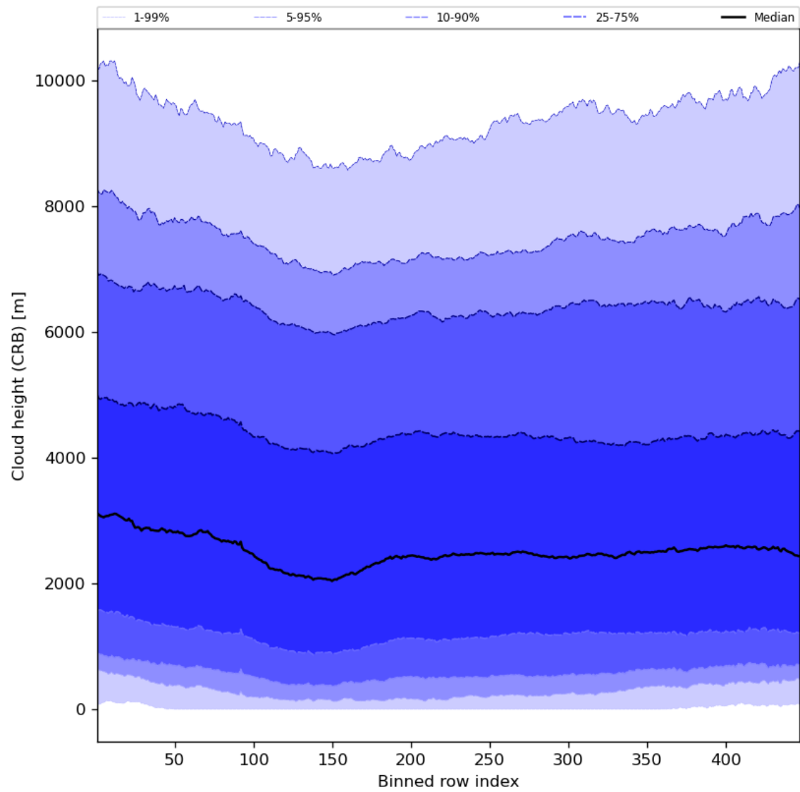
Figure 59: Along track statistics of “Cloud height (CRB)” for 2023-10-22 to 2023-10-23
