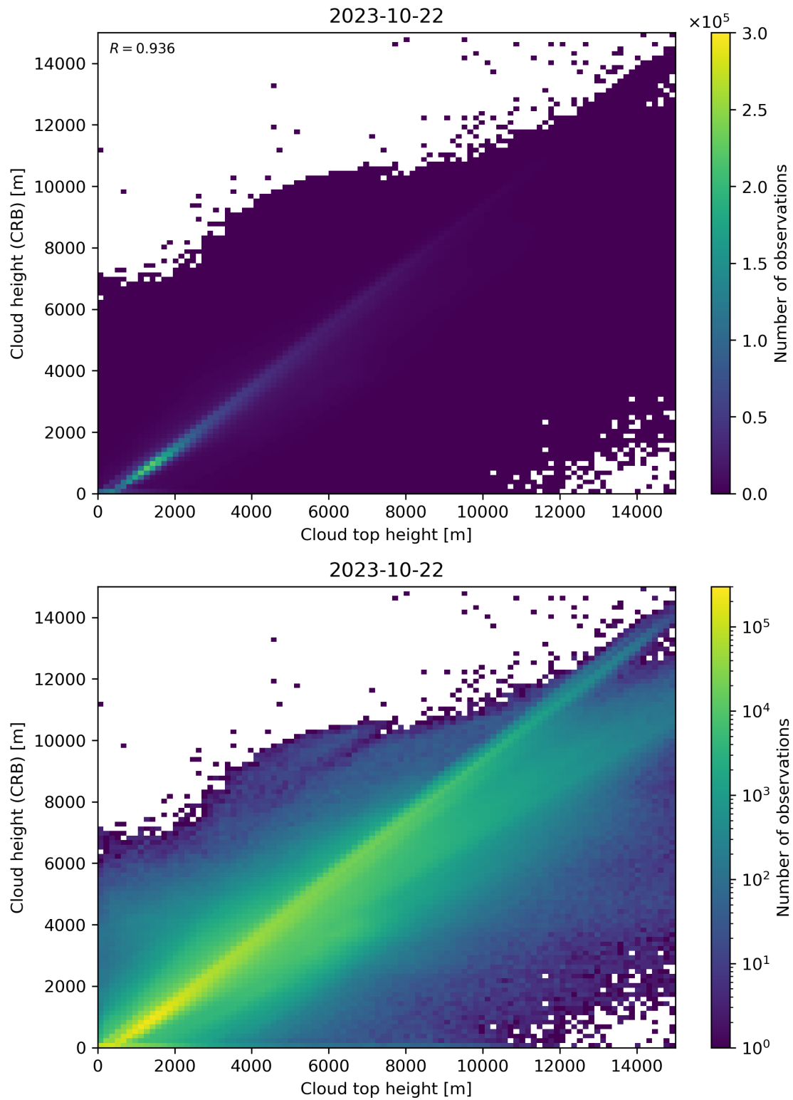
Figure 89: Scatter density plot of “Cloud top height” against “Cloud height (CRB)” for 2023-10-22 to 2023-10-23.
