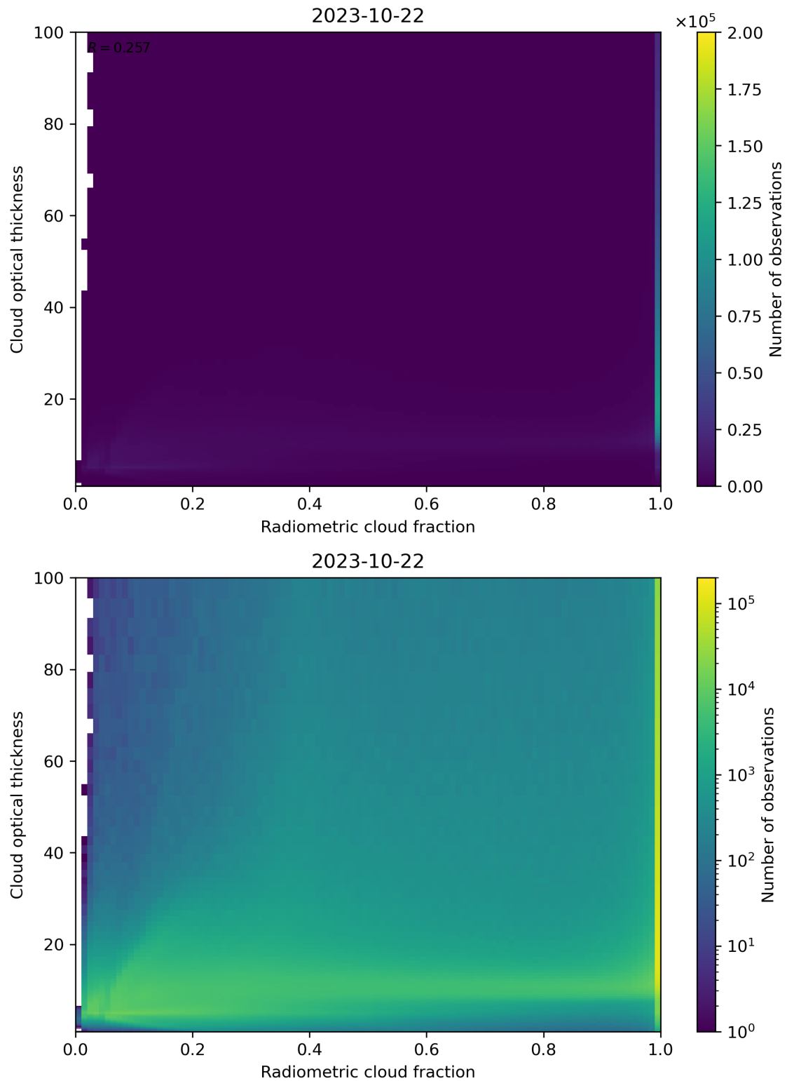
Figure 75: Scatter density plot of “Radiometric cloud fraction” against “Cloud optical thickness” for 2023-10-22 to 2023-10-23.
