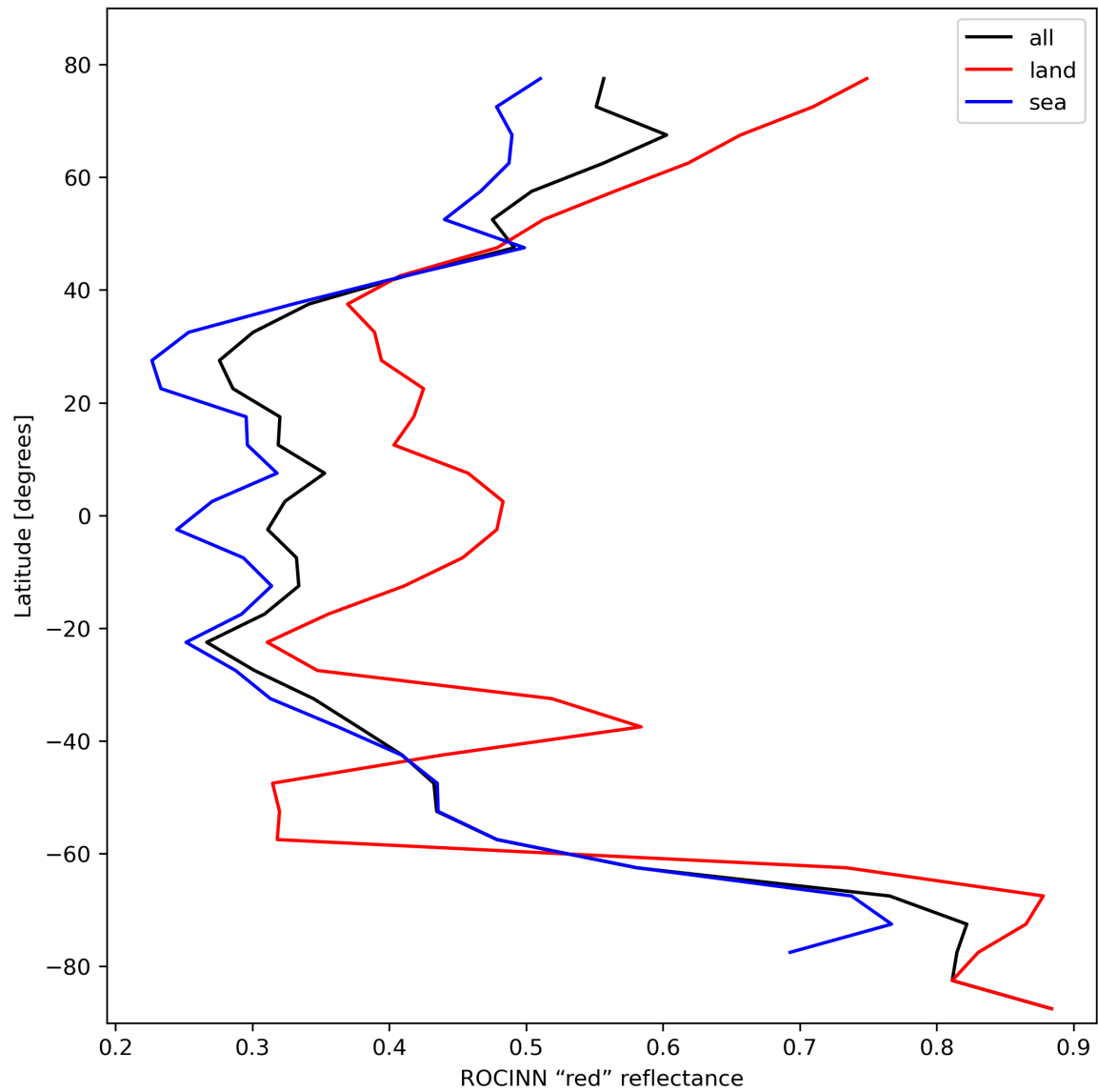
Figure 37: Zonal average of “ROCINN “red” reflectance” for 2023-10-22 to 2023-10-23.
