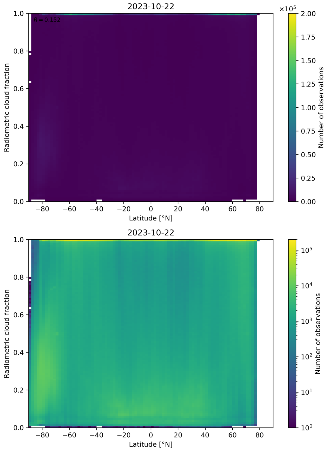
Figure 92: Scatter density plot of “Latitude” against “Radiometric cloud fraction” for 2023-10-22 to 2023-10-23.
