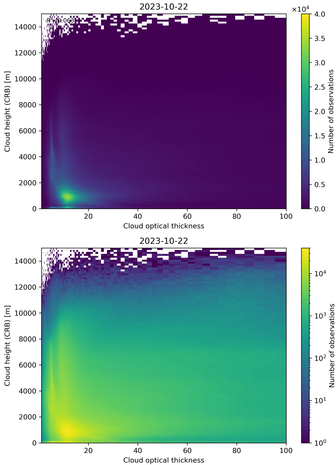
Figure 85: Scatter density plot of “Cloud optical thickness” against “Cloud height (CRB)” for 2023-10-22 to 2023-10-23.
