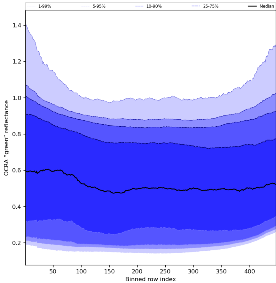
Figure 68: Along track statistics of “OCRA “green” reflectance” for 2023-10-22 to 2023-10-23
