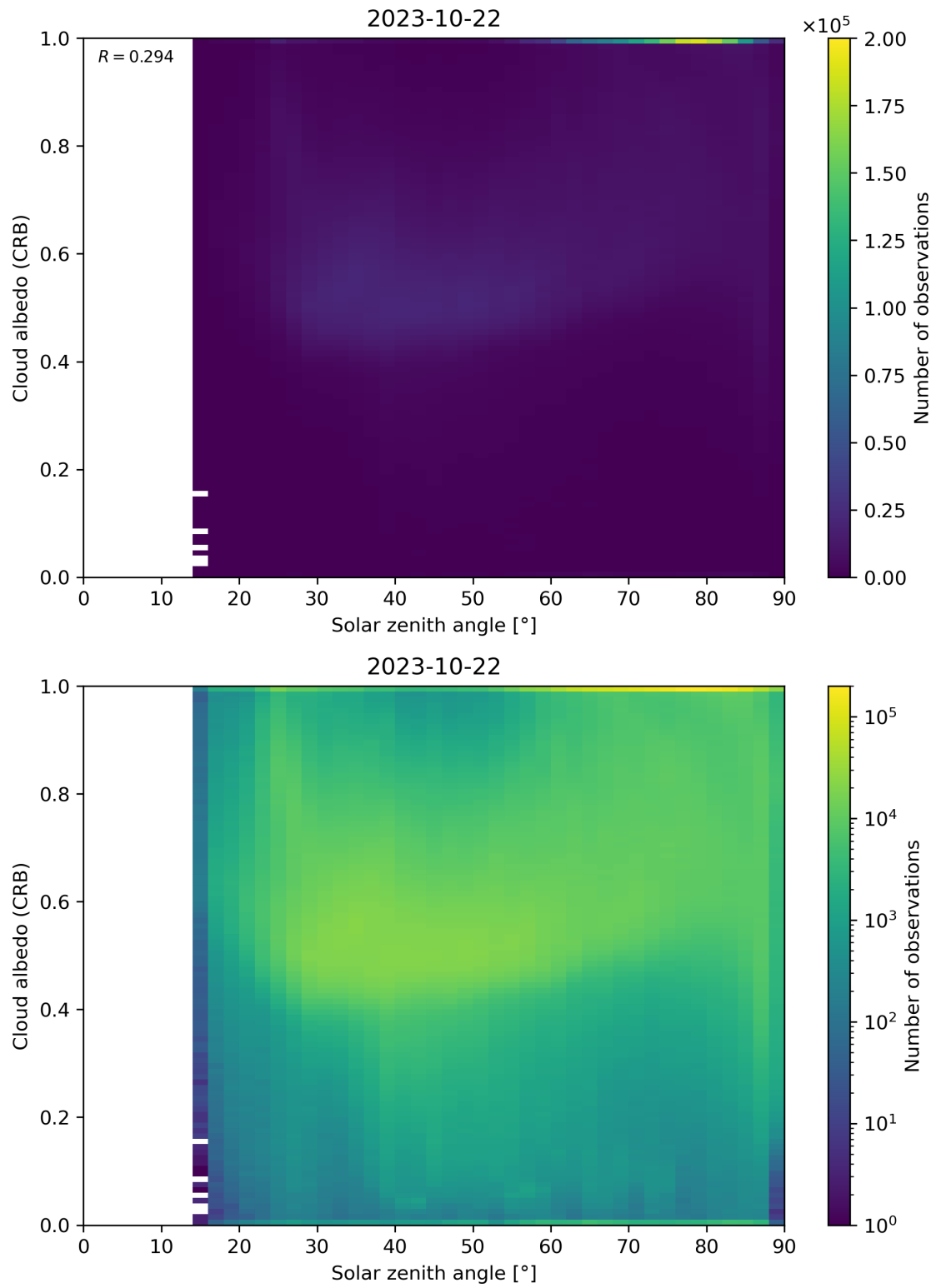
Figure 98: Scatter density plot of “Solar zenith angle” against “Cloud albedo (CRB)” for 2023-10-22 to 2023-10-23.
