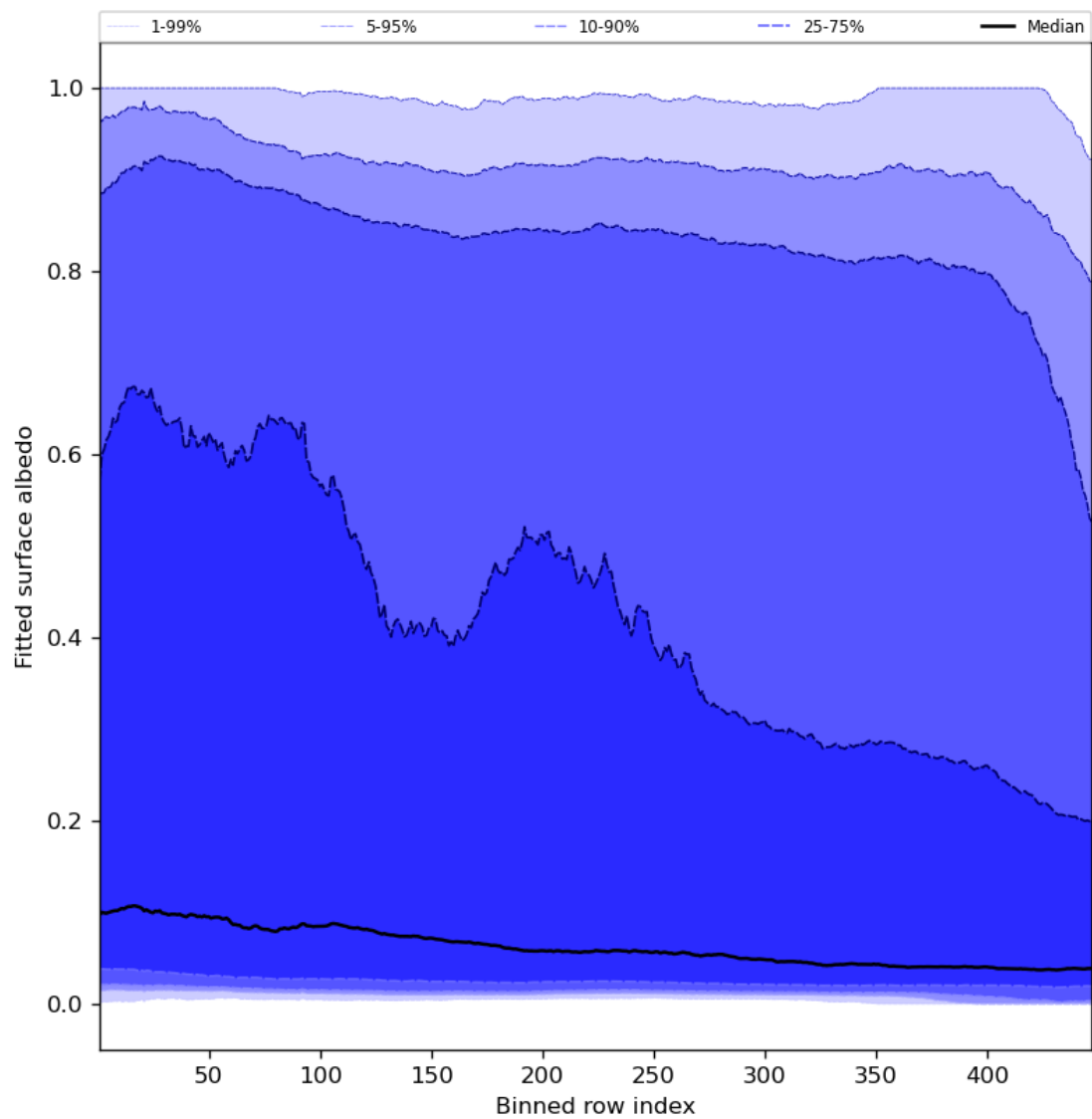
Figure 61: Along track statistics of “Fitted surface albedo” for 2023-10-22 to 2023-10-23
