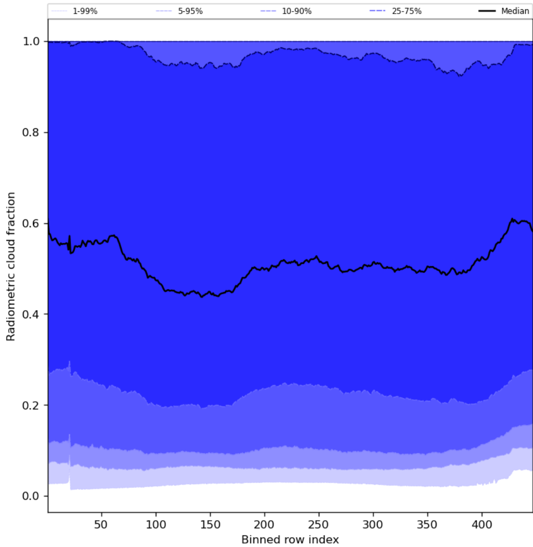
Figure 55: Along track statistics of “Radiometric cloud fraction” for 2023-10-22 to 2023-10-23
