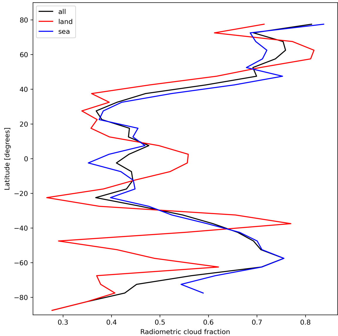
Figure 23: Zonal average of “Radiometric cloud fraction” for 2023-10-22 to 2023-10-23.
