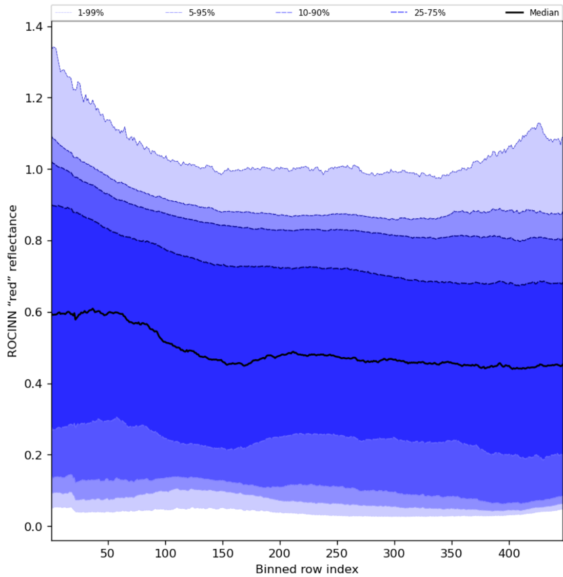
Figure 69: Along track statistics of “ROCINN “red” reflectance” for 2023-10-22 to 2023-10-23
