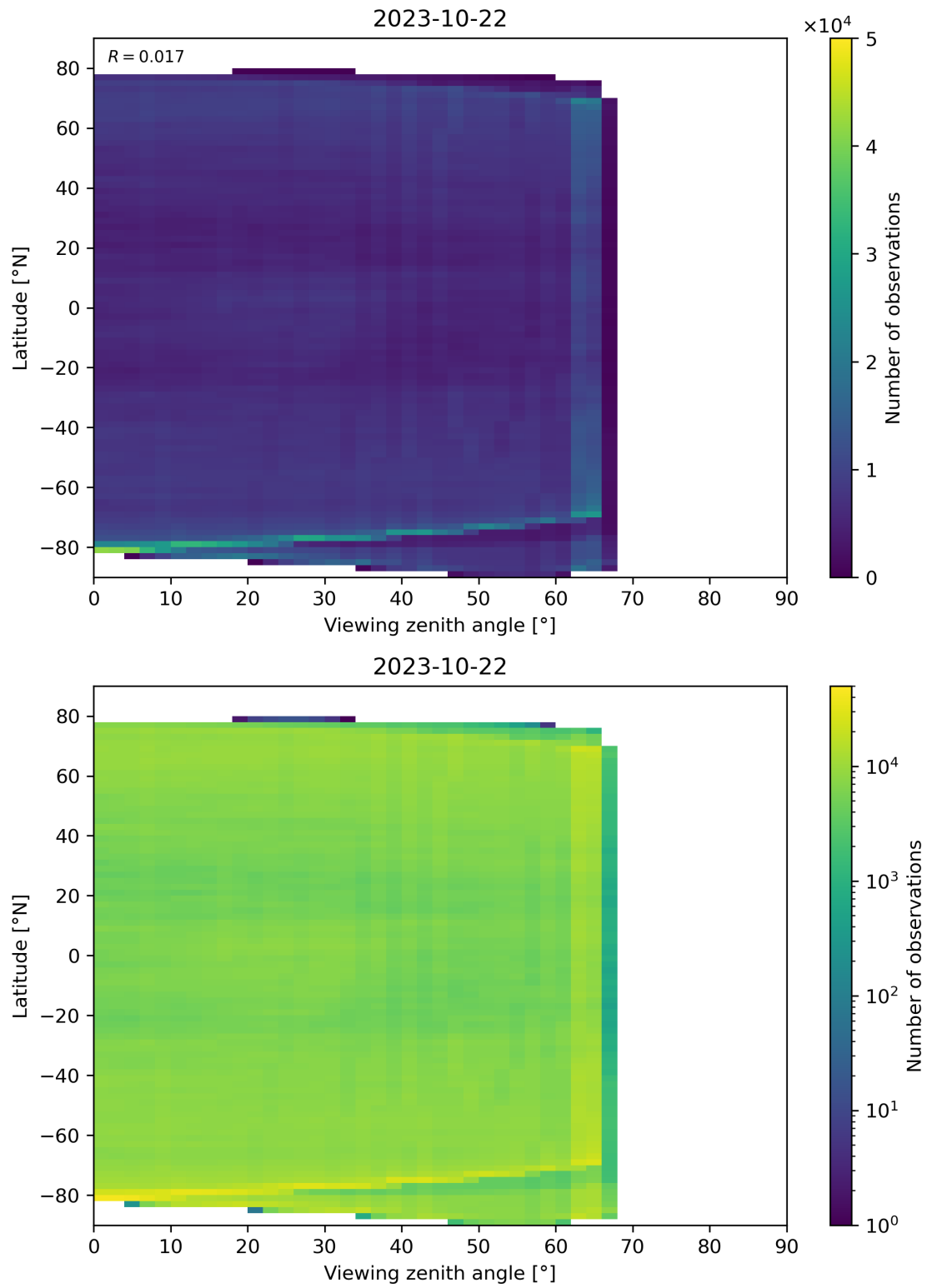
Figure 113: Scatter density plot of “Viewing zenith angle” against “Latitude” for 2023-10-22 to 2023-10-23.
