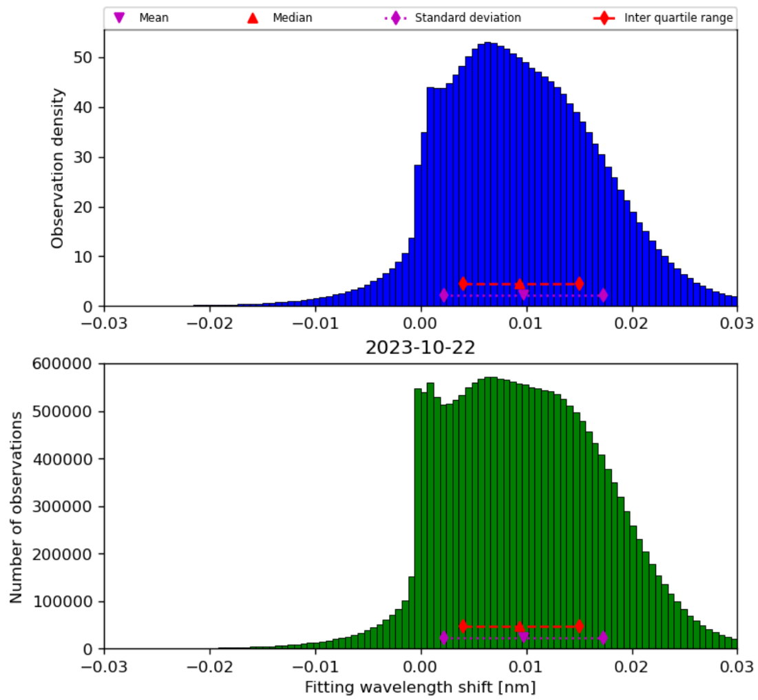
Figure 49: Histogram of “Fitting wavelength shift” for 2023-10-22 to 2023-10-23
