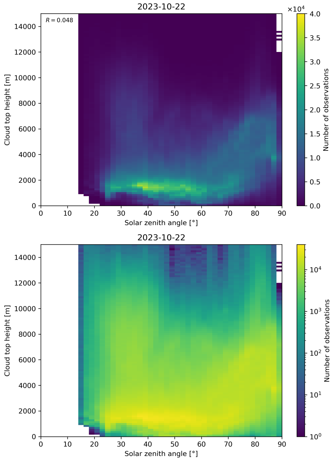
Figure 104: Scatter density plot of “Solar zenith angle” against “Cloud top height” for 2023-10-22 to 2023-10-23.
