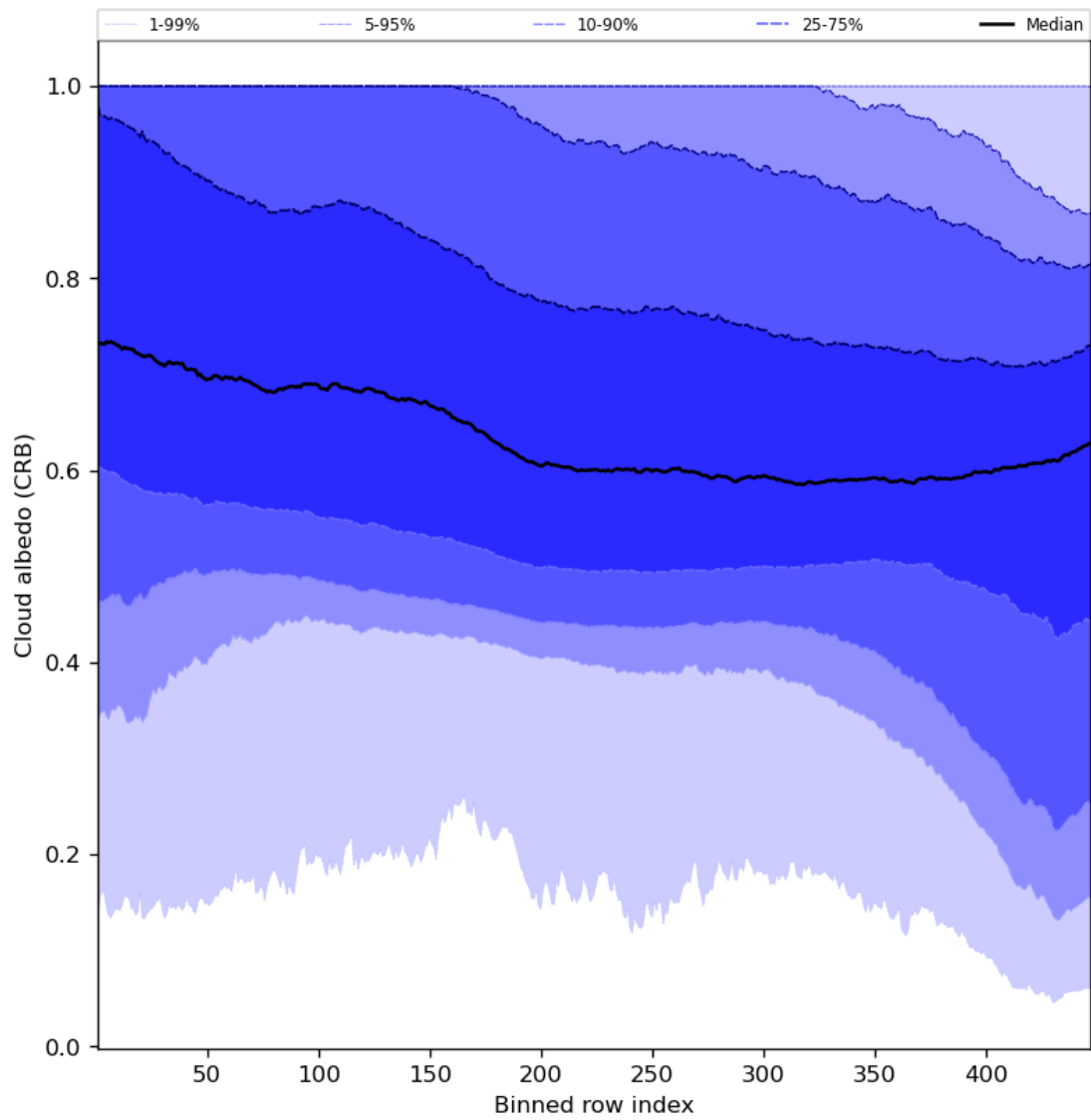
Figure 60: Along track statistics of “Cloud albedo (CRB)” for 2023-10-22 to 2023-10-23
