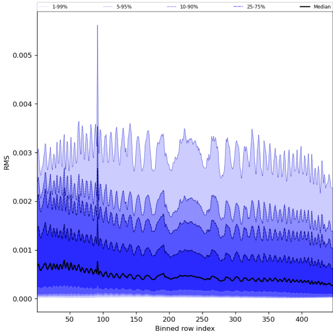
Figure 63: Along track statistics of “RMS” for 2023-10-22 to 2023-10-23
