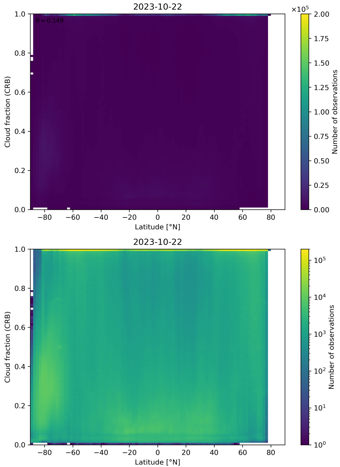
Figure 94: Scatter density plot of “Latitude” against “Cloud fraction (CRB)” for 2023-10-22 to 2023-10-23.
