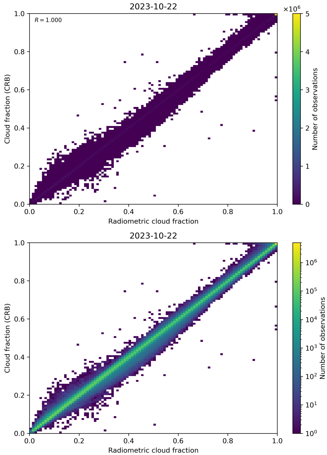
Figure 73: Scatter density plot of “Radiometric cloud fraction” against “Cloud fraction (CRB)” for 2023-10-22 to 2023-10-23.
