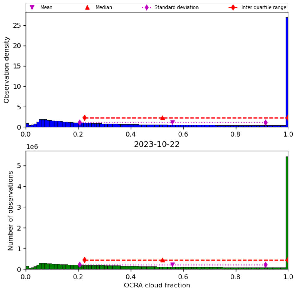
Figure 50: Histogram of “OCRA cloud fraction” for 2023-10-22 to 2023-10-23
