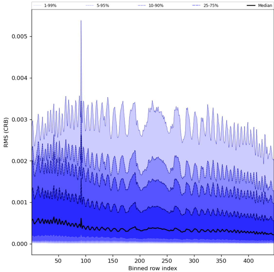
Figure 64: Along track statistics of “RMS (CRB)” for 2023-10-22 to 2023-10-23
