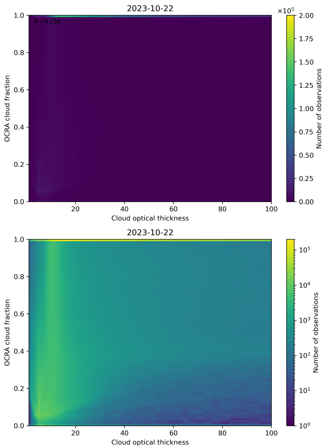
Figure 83: Scatter density plot of “Cloud optical thickness” against “OCRA cloud fraction” for 2023-10-22 to 2023-10-23.
