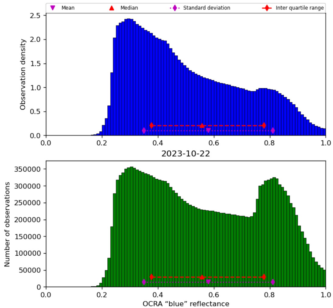
Figure 51: Histogram of “OCRA “blue” reflectance” for 2023-10-22 to 2023-10-23
