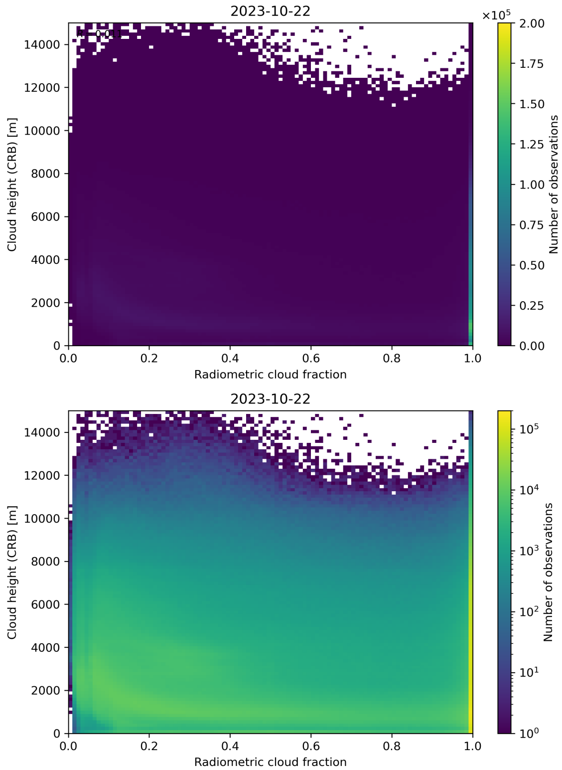
Figure 74: Scatter density plot of “Radiometric cloud fraction” against “Cloud height (CRB)” for 2023-10-22 to 2023-10-23.
