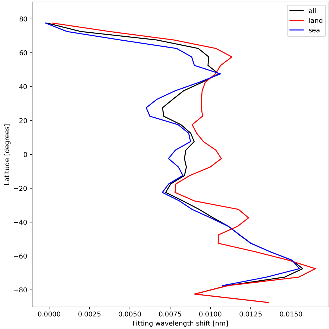
Figure 33: Zonal average of “Fitting wavelength shift” for 2023-10-22 to 2023-10-23.
