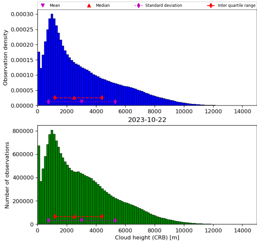
Figure 43: Histogram of “Cloud height (CRB)” for 2023-10-22 to 2023-10-23
