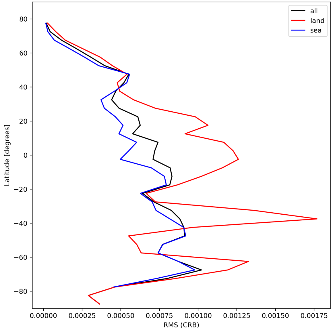
Figure 32: Zonal average of “RMS (CRB)” for 2023-10-22 to 2023-10-23.
