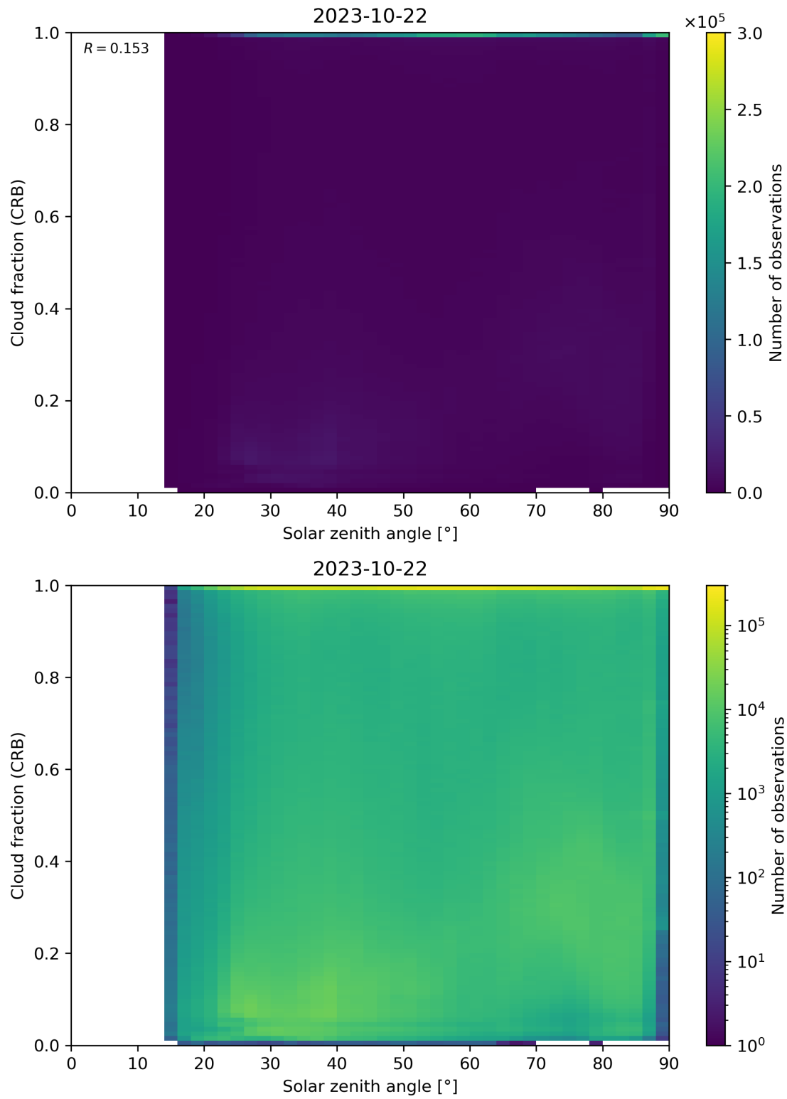
Figure 101: Scatter density plot of “Solar zenith angle” against “Cloud fraction (CRB)” for 2023-10-22 to 2023-10-23.
