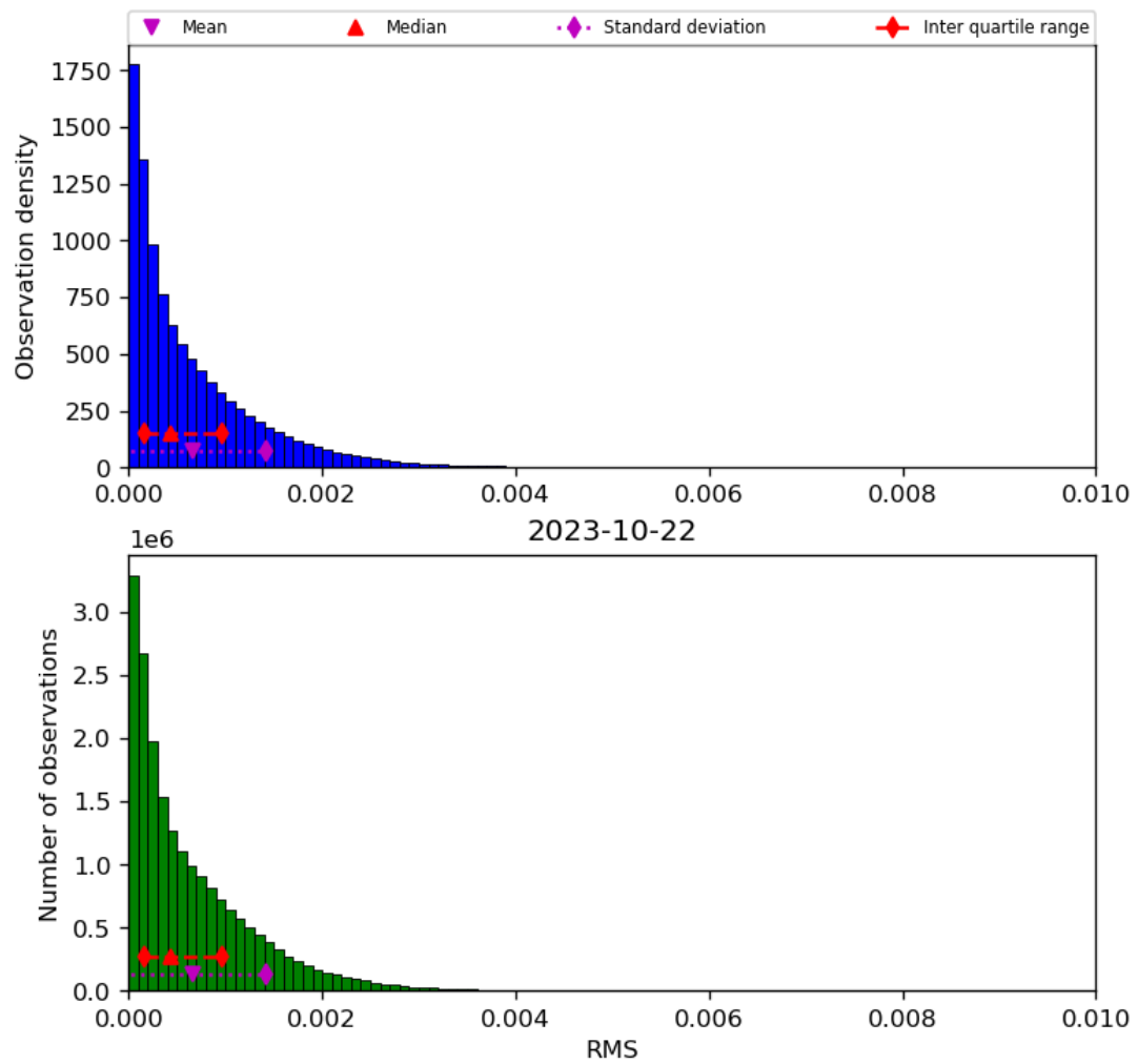
Figure 47: Histogram of “RMS” for 2023-10-22 to 2023-10-23
