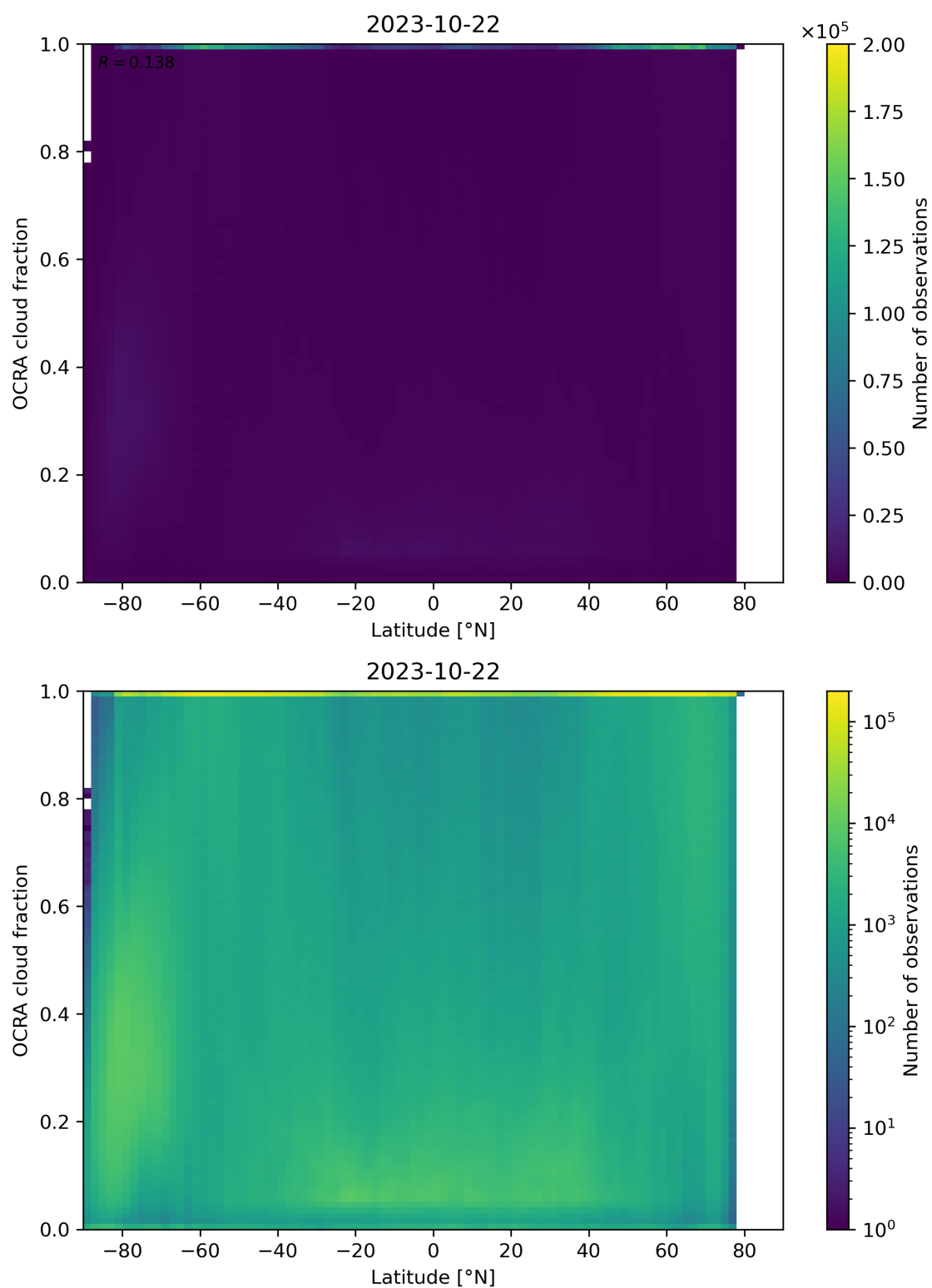
Figure 93: Scatter density plot of “Latitude” against “OCRA cloud fraction” for 2023-10-22 to 2023-10-23.
