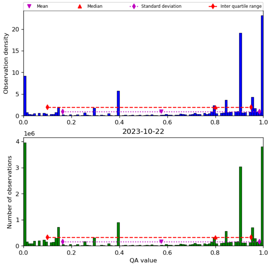
Figure 38: Histogram of “QA value” for 2023-10-22 to 2023-10-23
