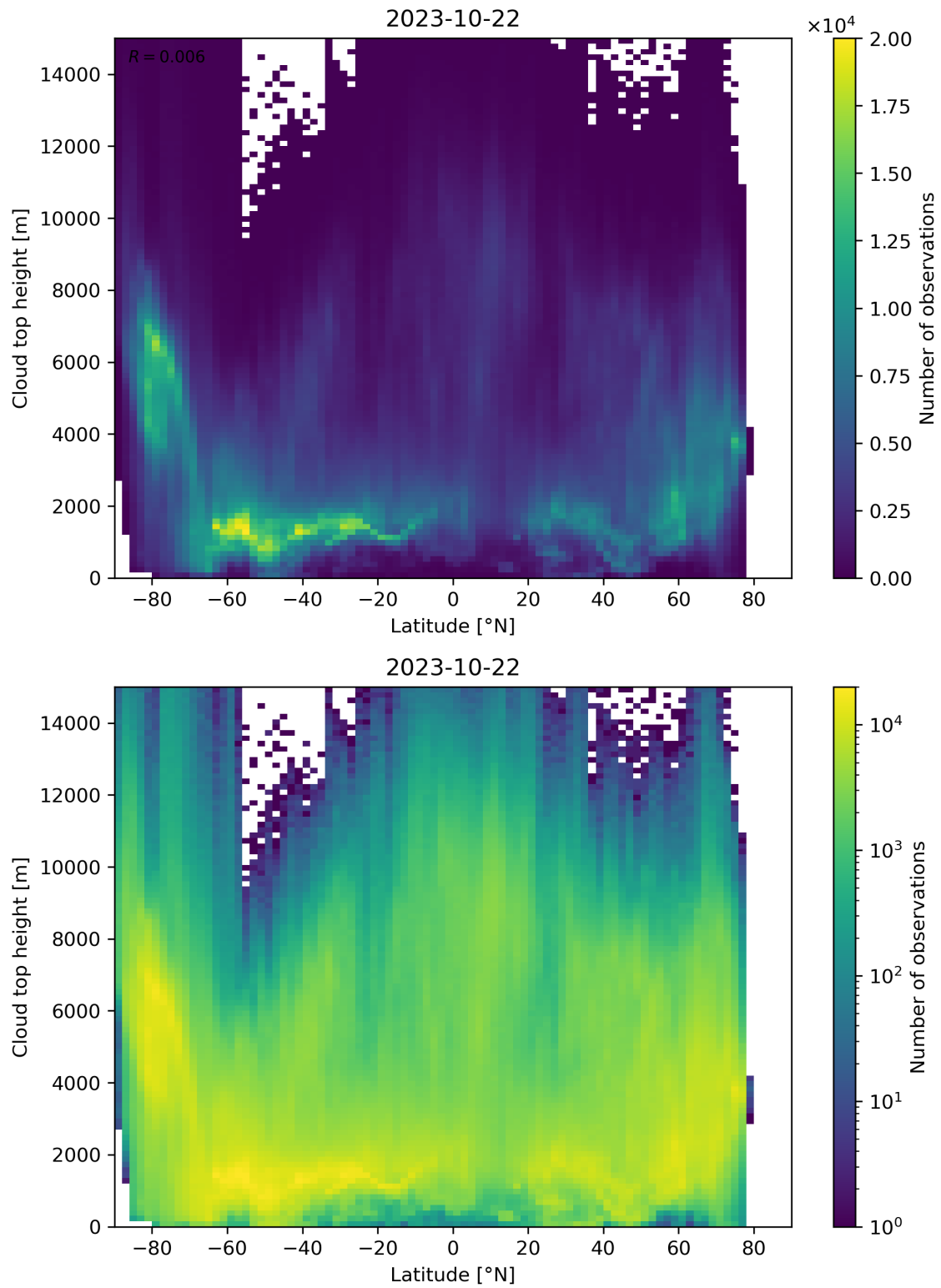
Figure 97: Scatter density plot of “Latitude” against “Cloud top height” for 2023-10-22 to 2023-10-23.
