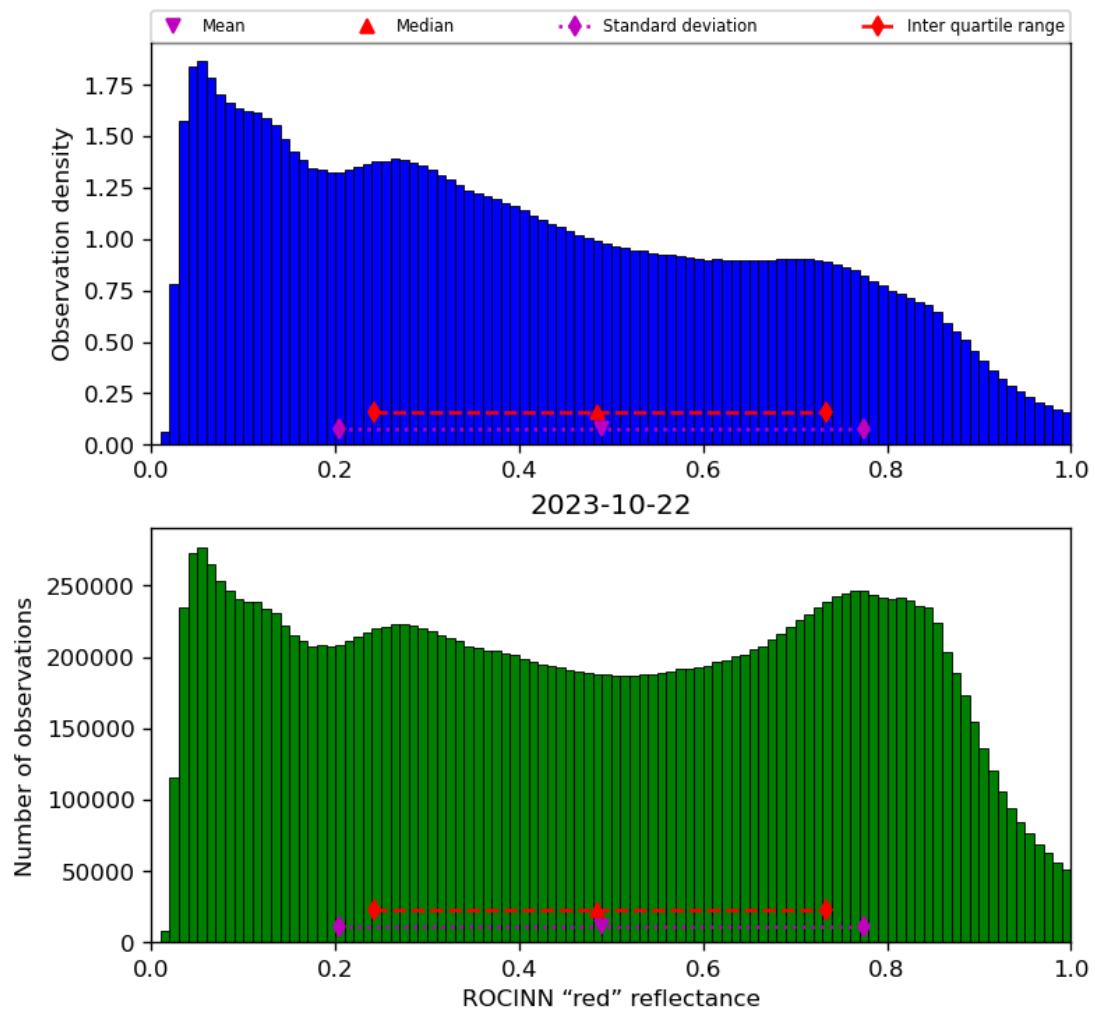
Figure 53: Histogram of “ROCINN “red” reflectance” for 2023-10-22 to 2023-10-23
