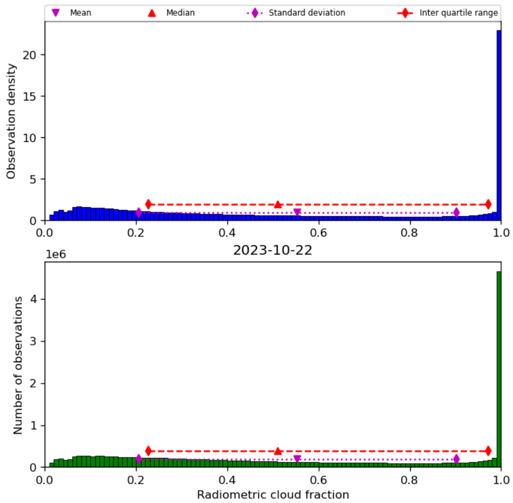
Figure 39: Histogram of “Radiometric cloud fraction” for 2023-10-22 to 2023-10-23
