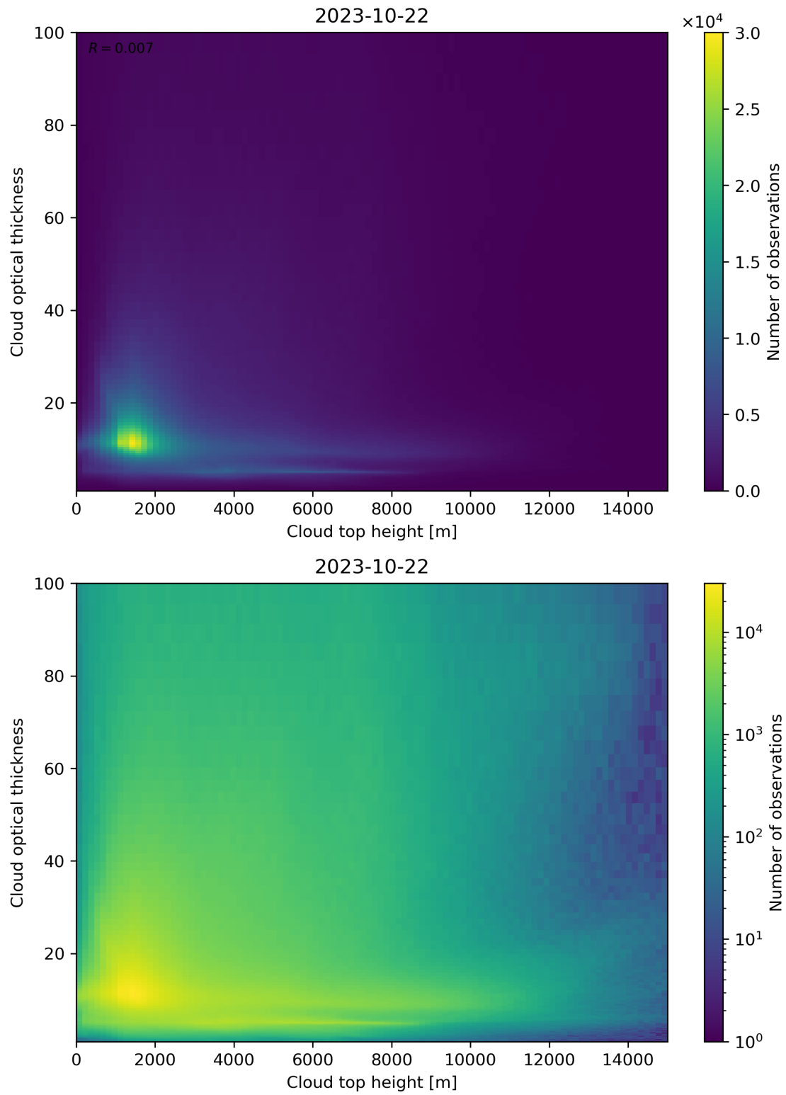
Figure 90: Scatter density plot of “Cloud top height” against “Cloud optical thickness” for 2023-10-22 to 2023-10-23.
