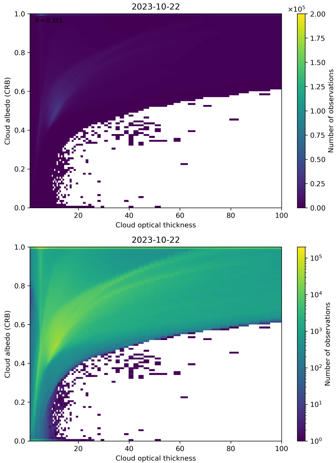
Figure 82: Scatter density plot of “Cloud optical thickness” against “Cloud albedo (CRB)” for 2023-10-22 to 2023-10-23.
