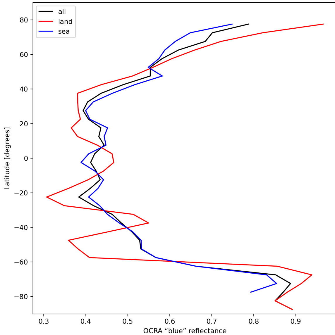
Figure 35: Zonal average of “OCRA “blue” reflectance” for 2023-10-22 to 2023-10-23.
