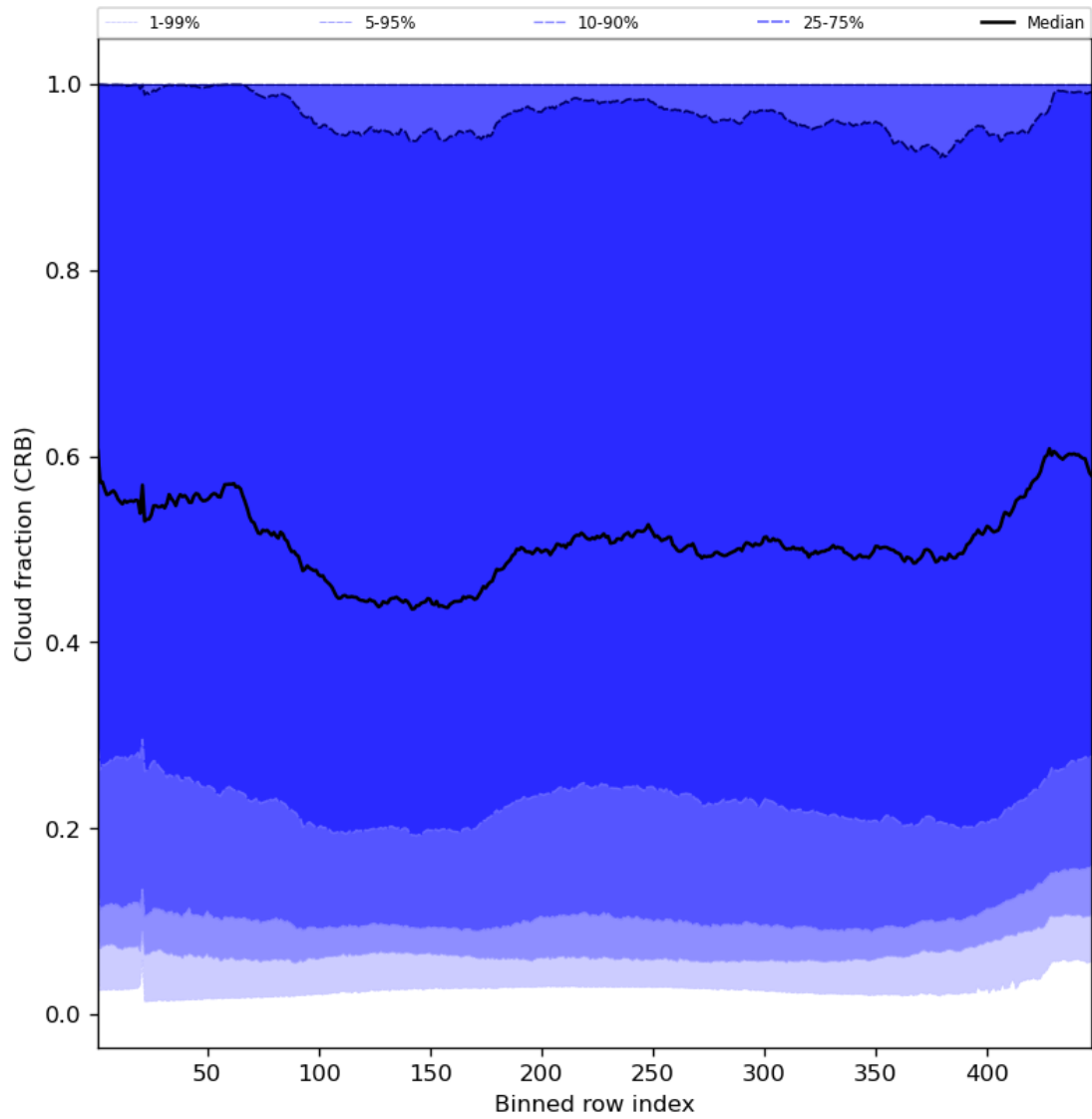
Figure 58: Along track statistics of “Cloud fraction (CRB)” for 2023-10-22 to 2023-10-23
