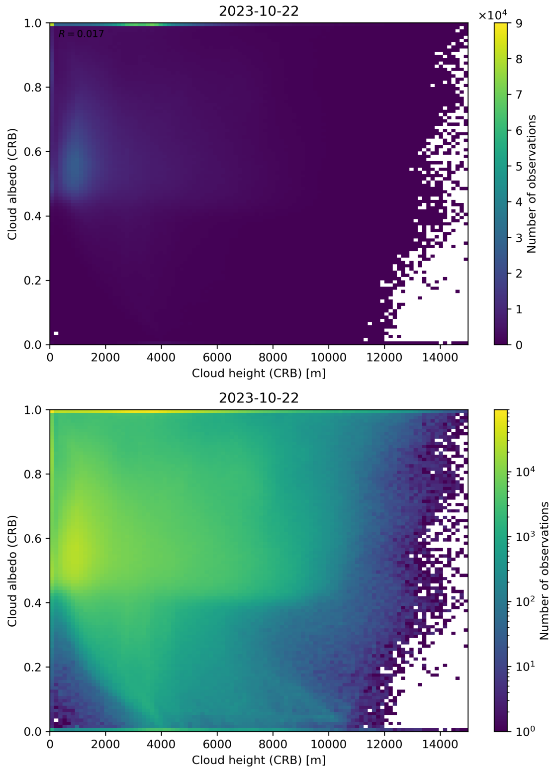
Figure 80: Scatter density plot of “Cloud height (CRB)” against “Cloud albedo (CRB)” for 2023-10-22 to 2023-10-23.
