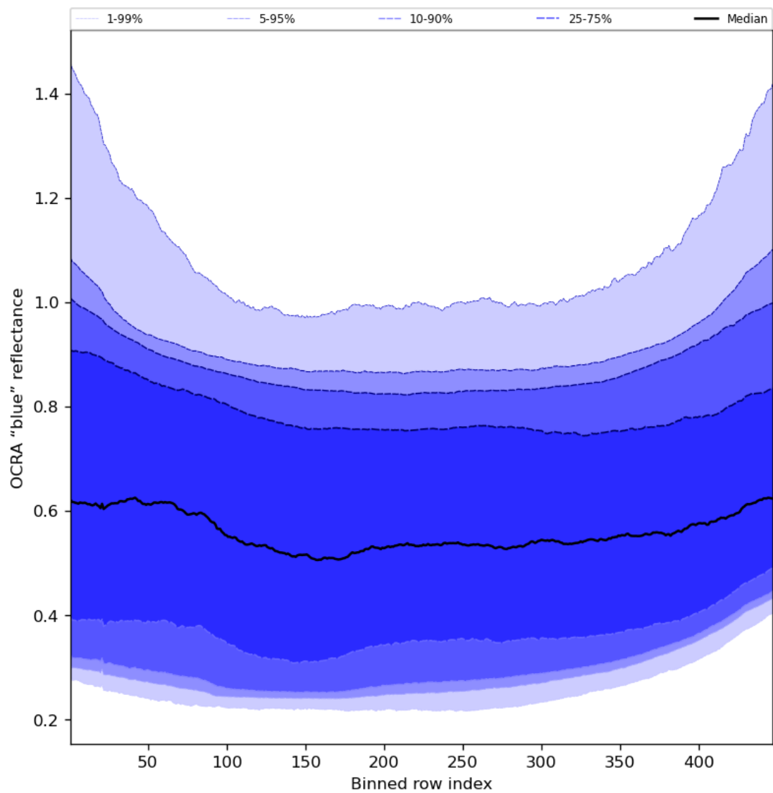
Figure 67: Along track statistics of “OCRA “blue” reflectance” for 2023-10-22 to 2023-10-23
