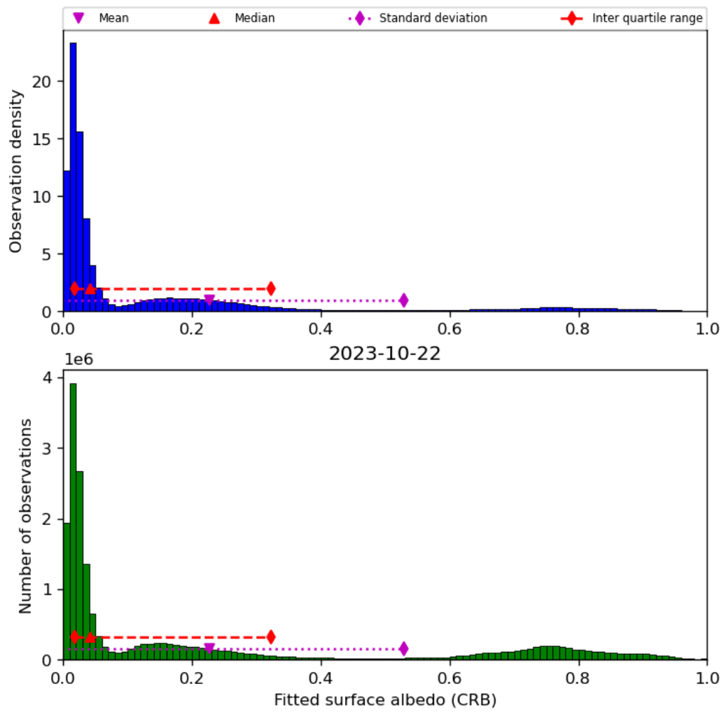
Figure 46: Histogram of “Fitted surface albedo (CRB)” for 2023-10-22 to 2023-10-23
