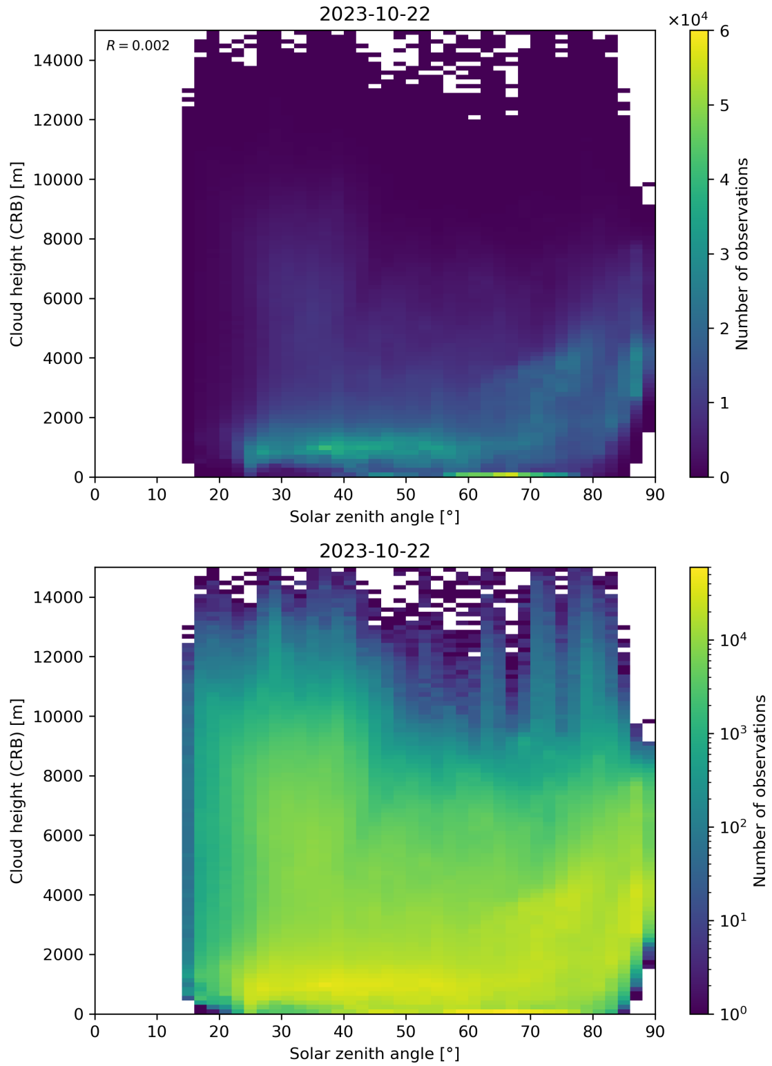
Figure 102: Scatter density plot of “Solar zenith angle” against “Cloud height (CRB)” for 2023-10-22 to 2023-10-23.
