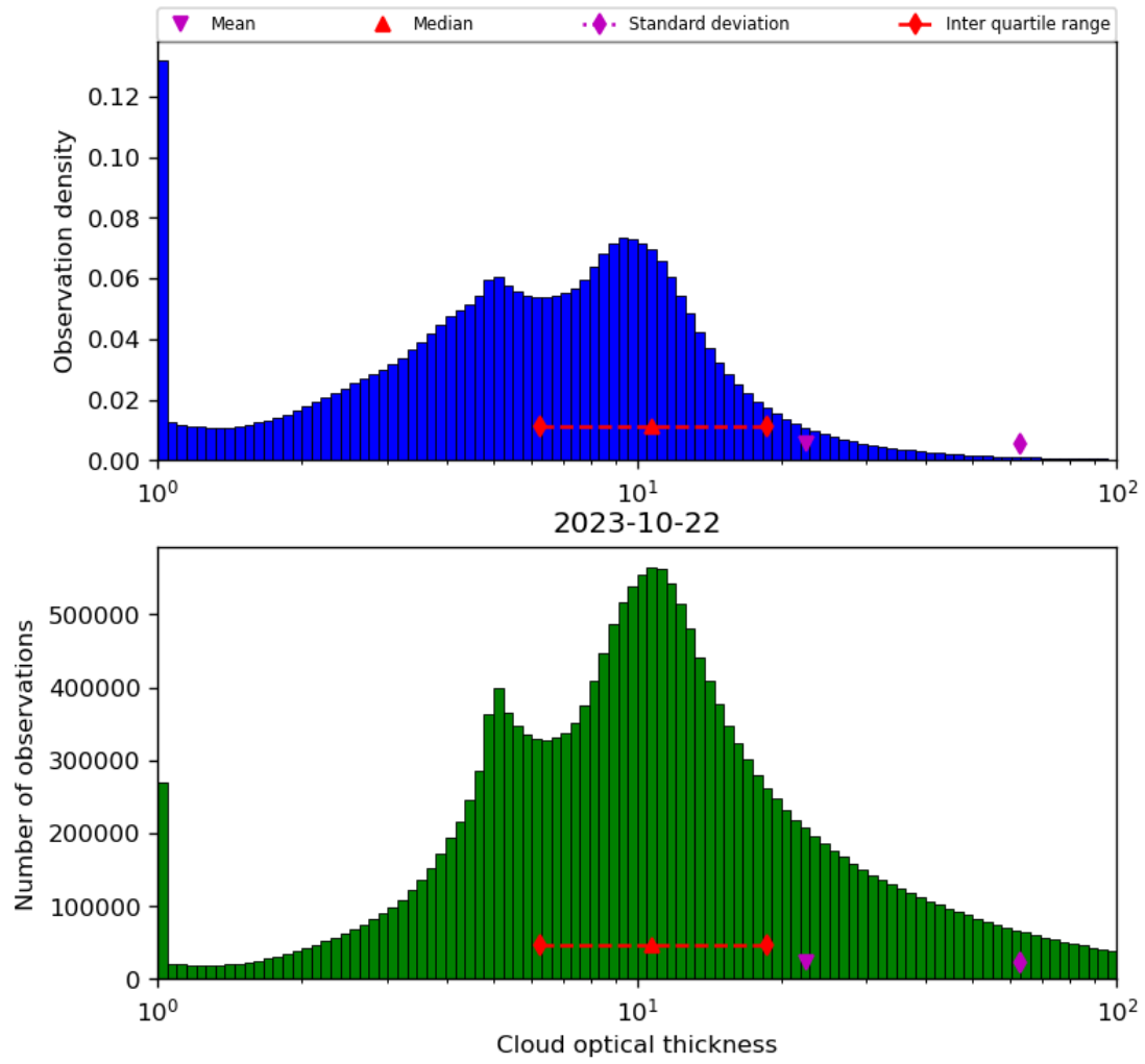
Figure 41: Histogram of “Cloud optical thickness” for 2023-10-22 to 2023-10-23
