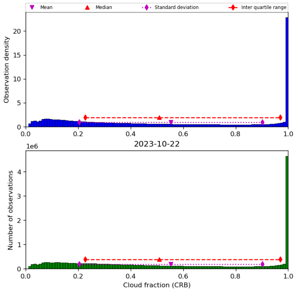
Figure 42: Histogram of “Cloud fraction (CRB)” for 2023-10-22 to 2023-10-23
