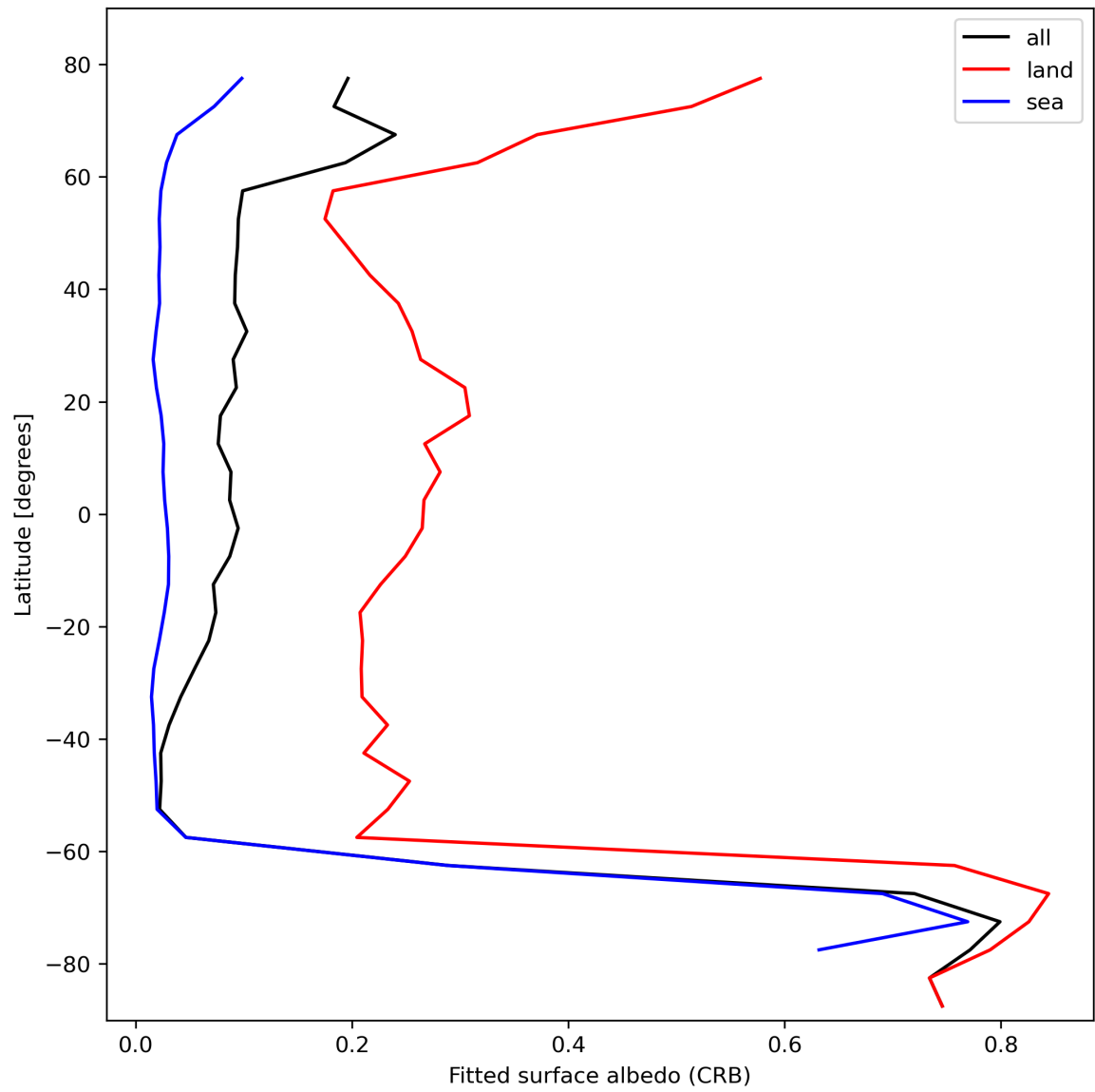
Figure 30: Zonal average of “Fitted surface albedo (CRB)” for 2023-10-22 to 2023-10-23.
