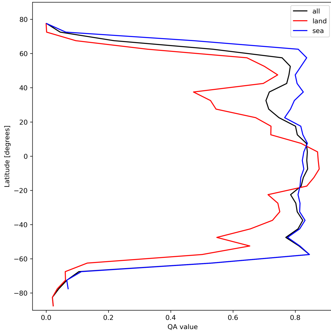
Figure 22: Zonal average of “QA value” for 2023-10-22 to 2023-10-23.
