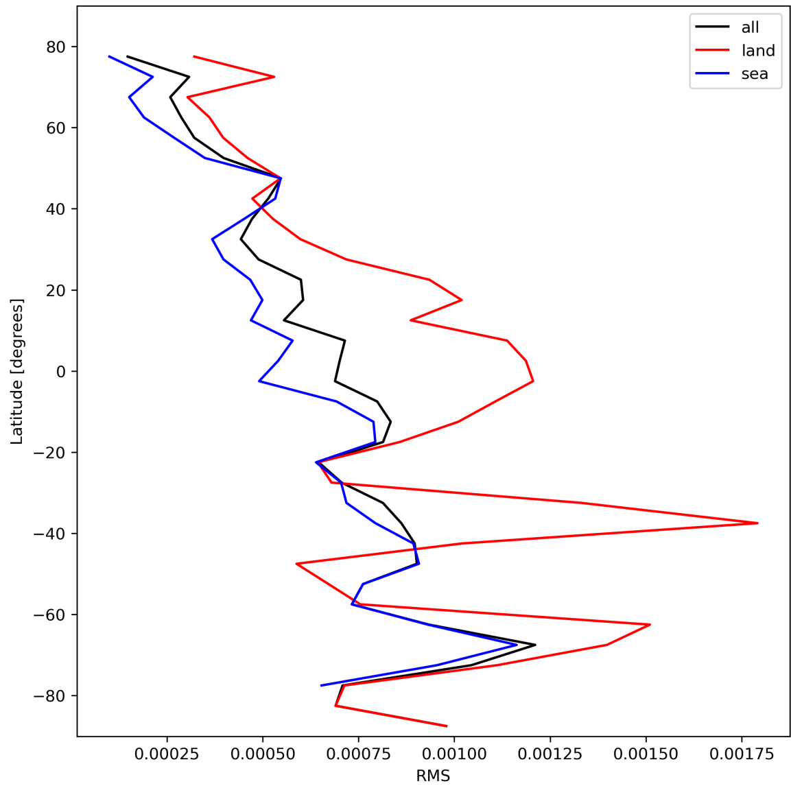
Figure 31: Zonal average of “RMS” for 2023-10-22 to 2023-10-23.
