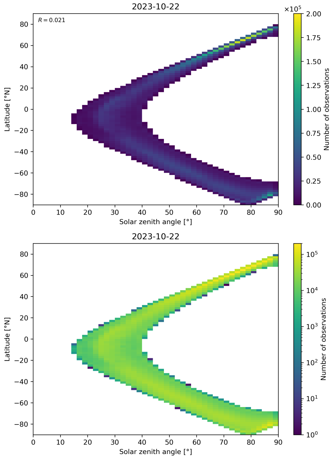
Figure 105: Scatter density plot of “Solar zenith angle” against “Latitude” for 2023-10-22 to 2023-10-23.
