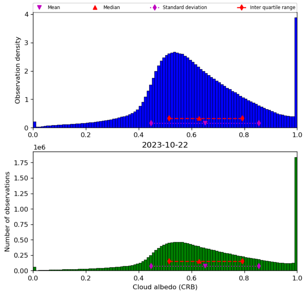
Figure 44: Histogram of “Cloud albedo (CRB)” for 2023-10-22 to 2023-10-23
