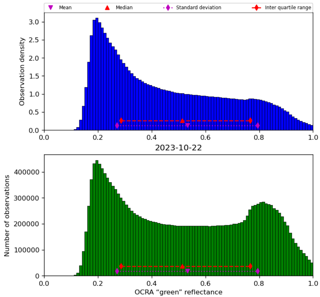
Figure 52: Histogram of “OCRA “green” reflectance” for 2023-10-22 to 2023-10-23
