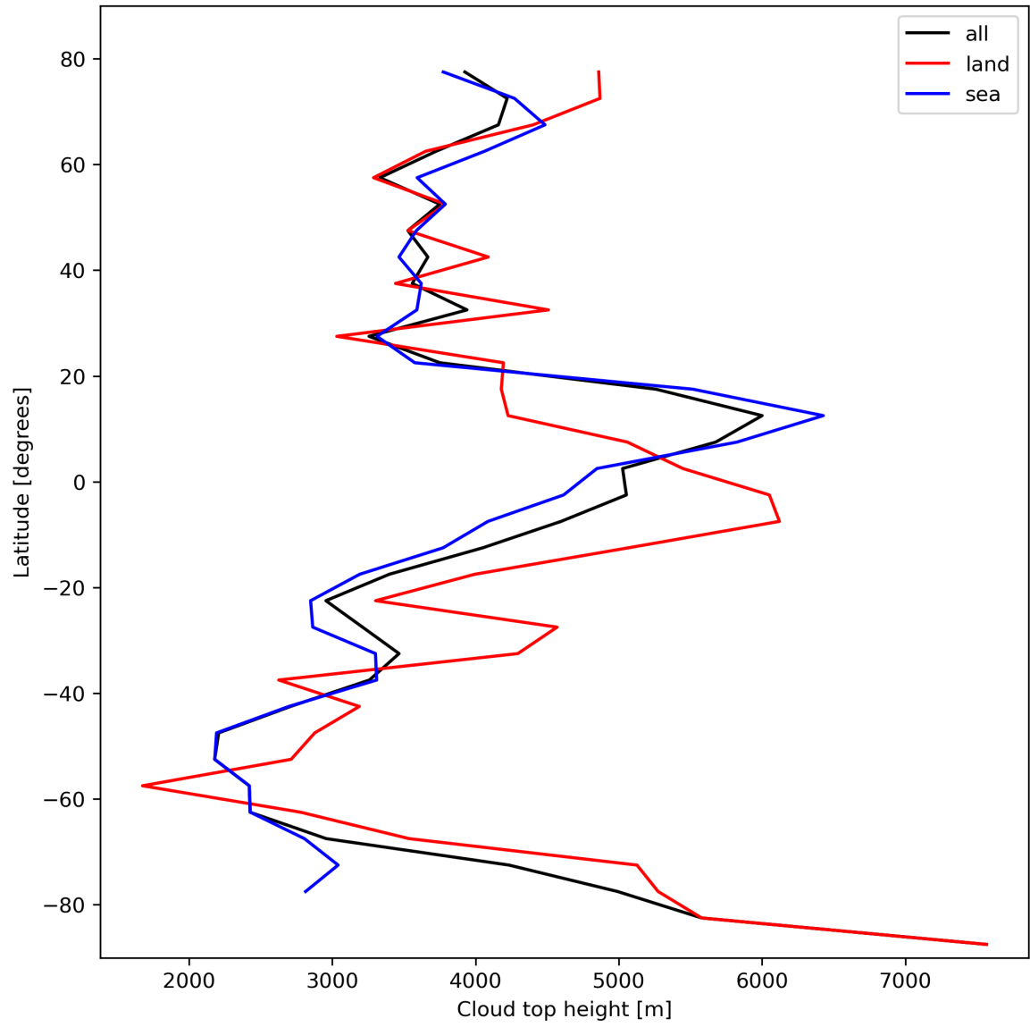
Figure 24: Zonal average of “Cloud top height” for 2023-10-22 to 2023-10-23.
