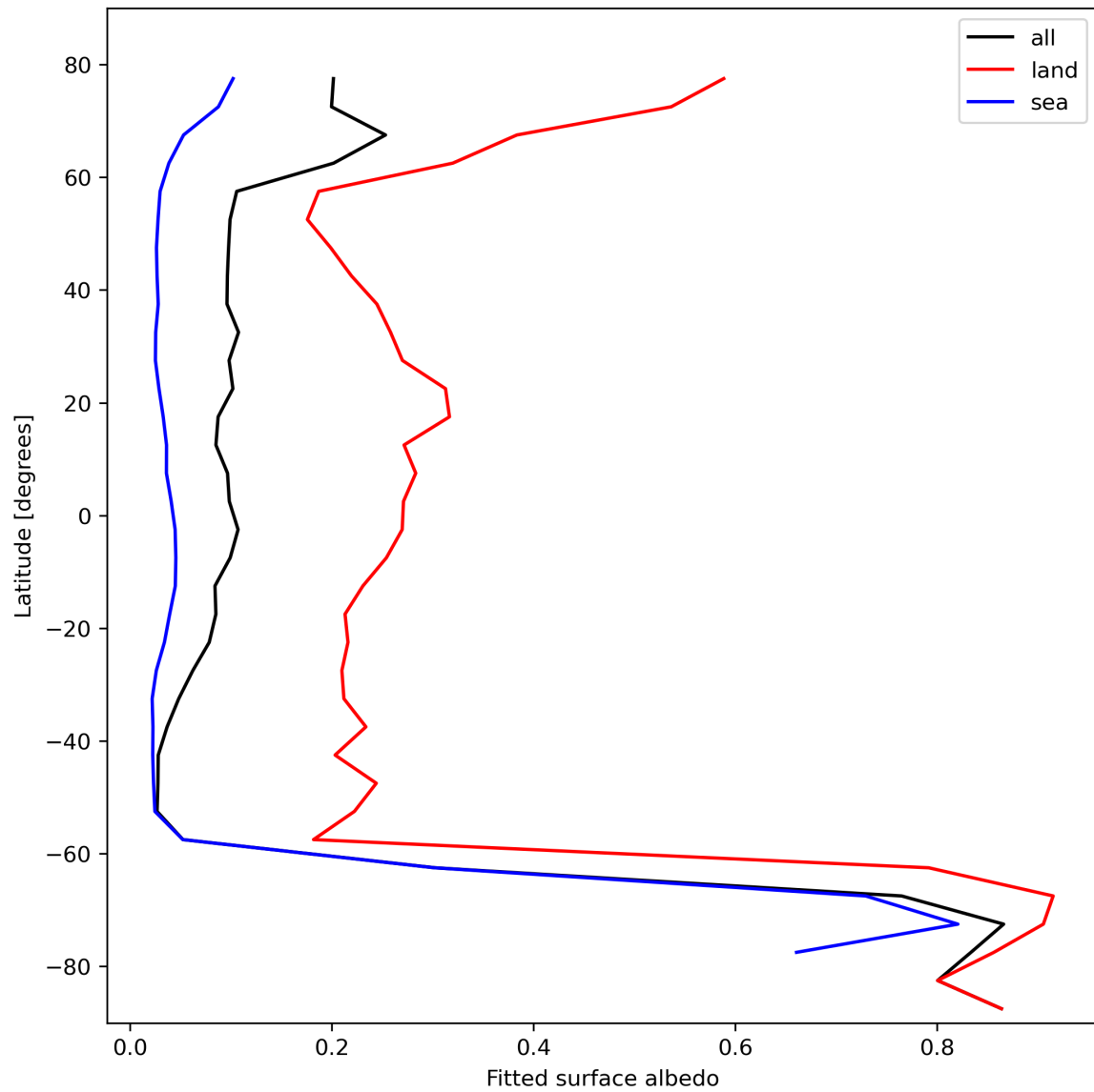
Figure 29: Zonal average of “Fitted surface albedo” for 2023-10-22 to 2023-10-23.
