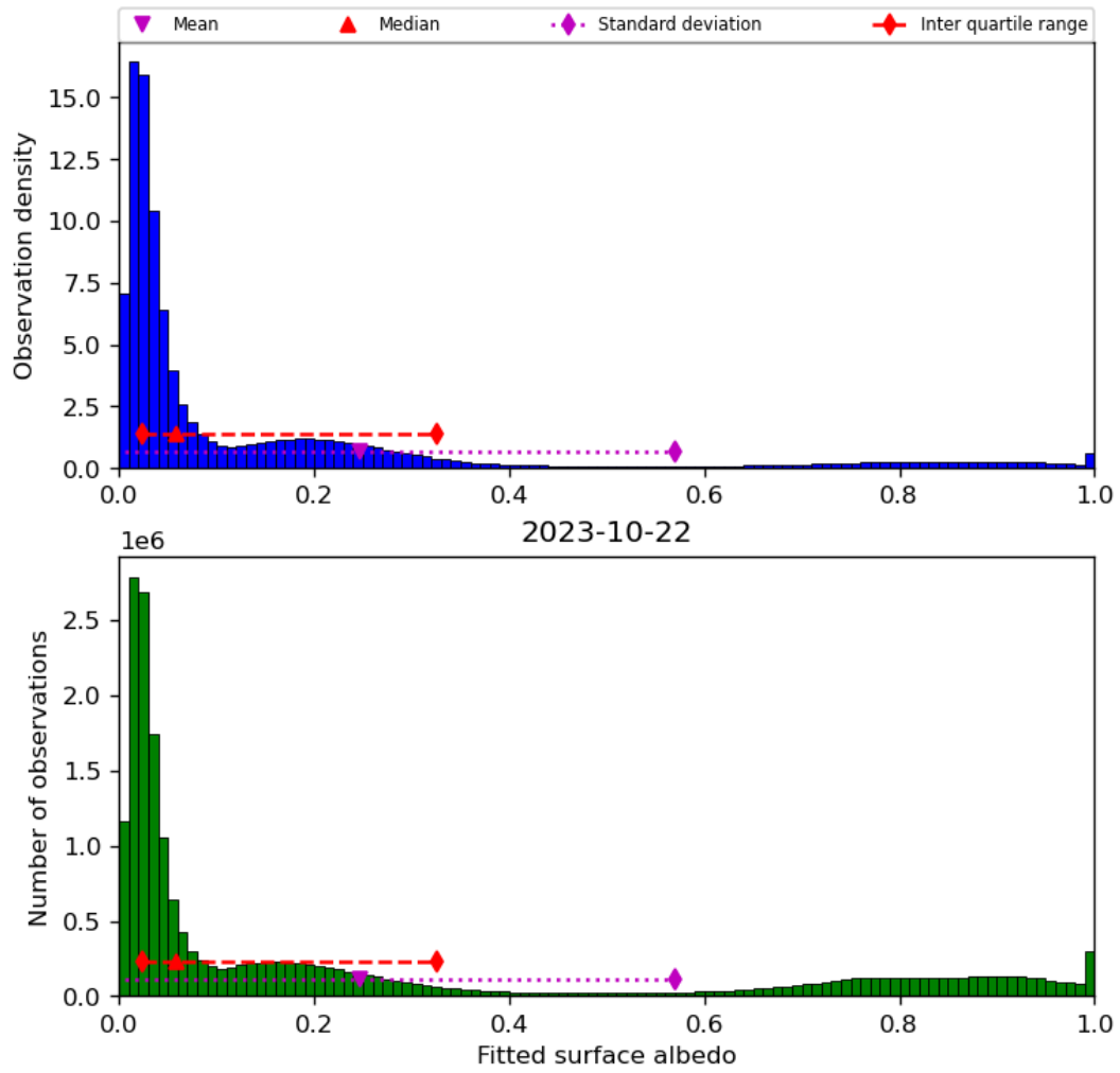
Figure 45: Histogram of “Fitted surface albedo” for 2023-10-22 to 2023-10-23
