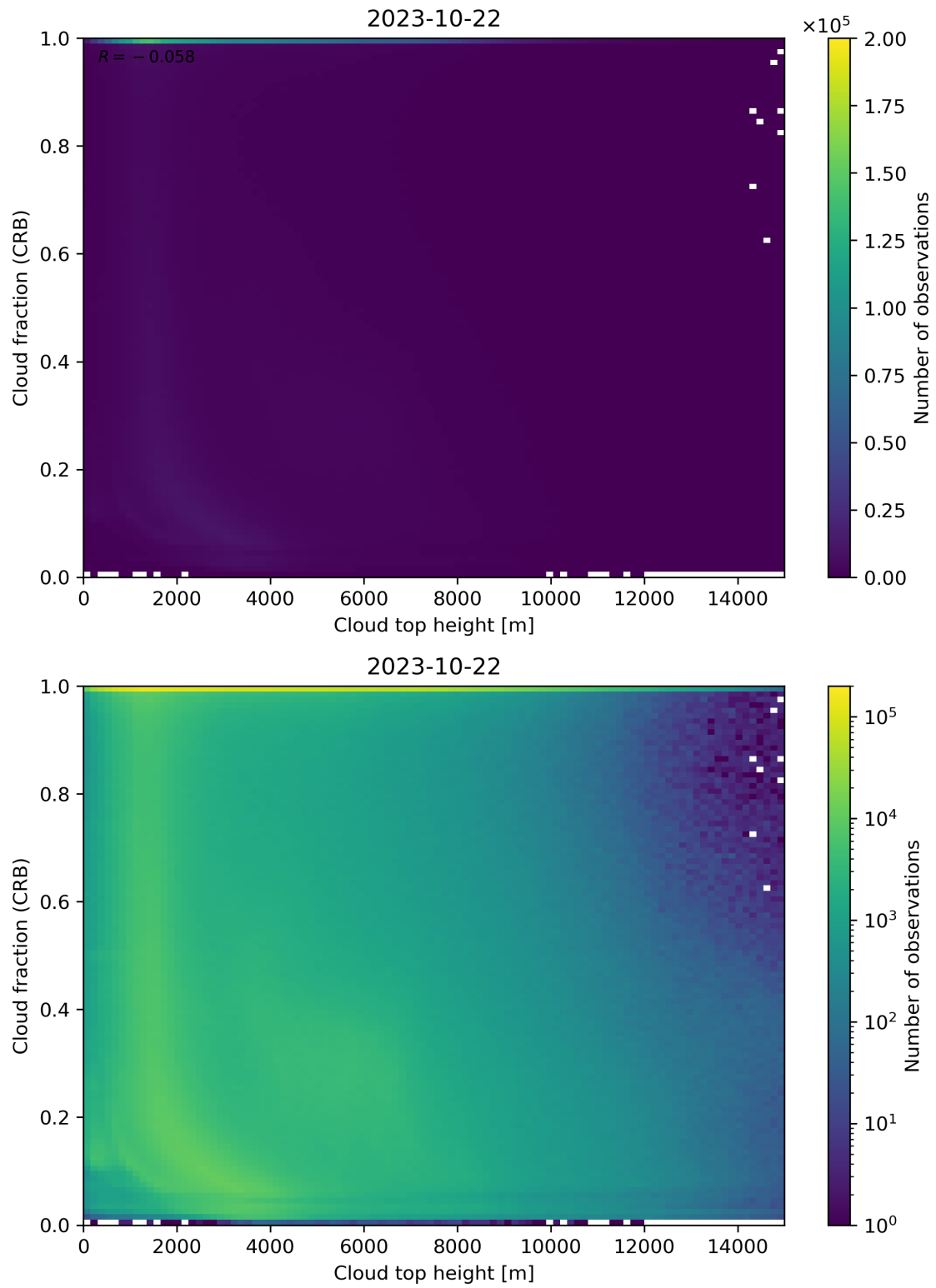
Figure 88: Scatter density plot of “Cloud top height” against “Cloud fraction (CRB)” for 2023-10-22 to 2023-10-23.
