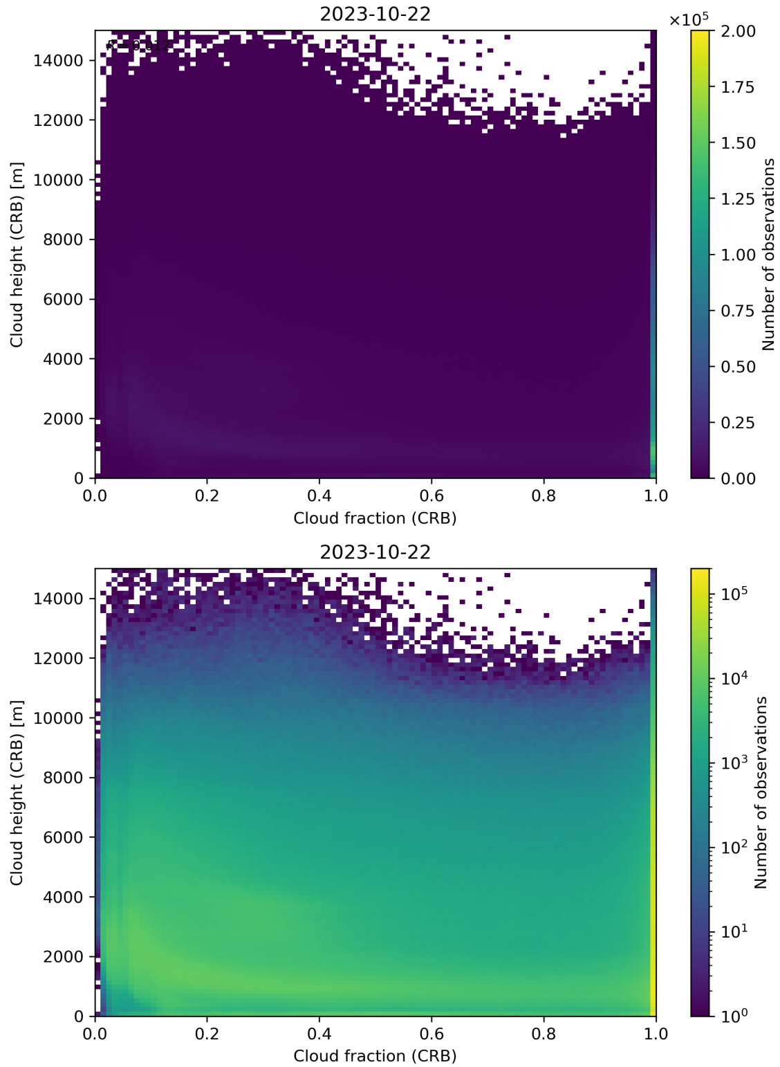
Figure 79: Scatter density plot of “Cloud fraction (CRB)” against “Cloud height (CRB)” for 2023-10-22 to 2023-10-23.
