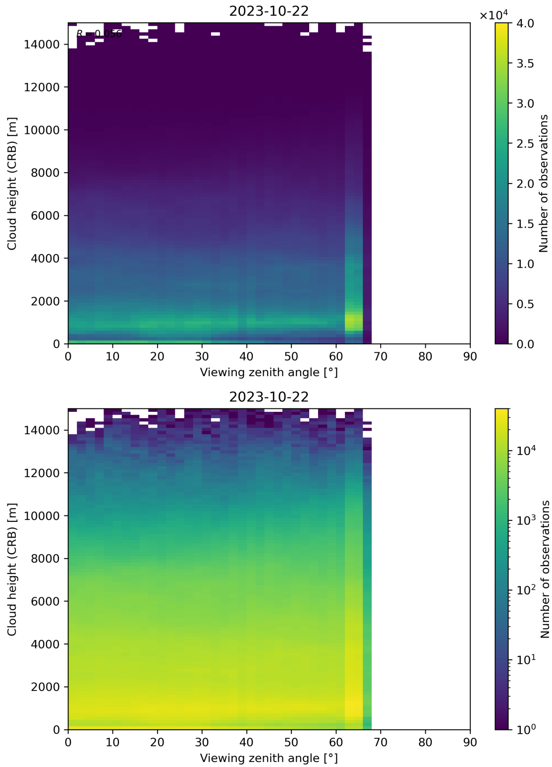
Figure 110: Scatter density plot of “Viewing zenith angle” against “Cloud height (CRB)” for 2023-10-22 to 2023-10-23.
