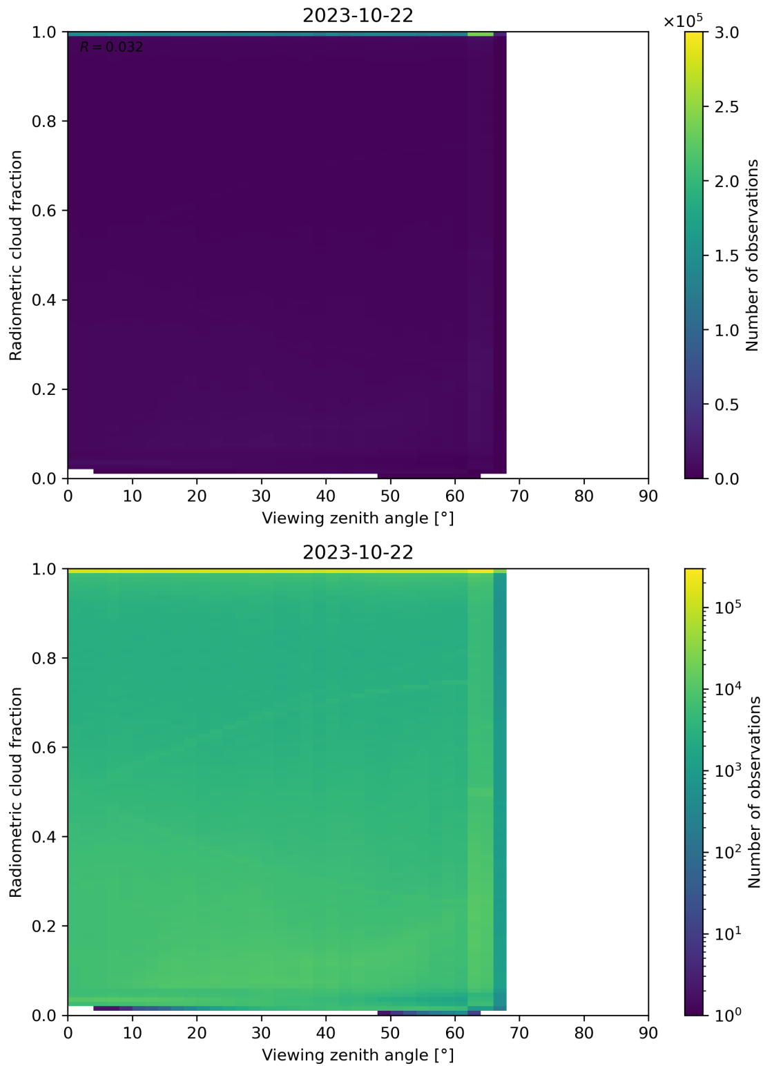
Figure 107: Scatter density plot of “Viewing zenith angle” against “Radiometric cloud fraction” for 2023-10-22 to 2023-10-23.
