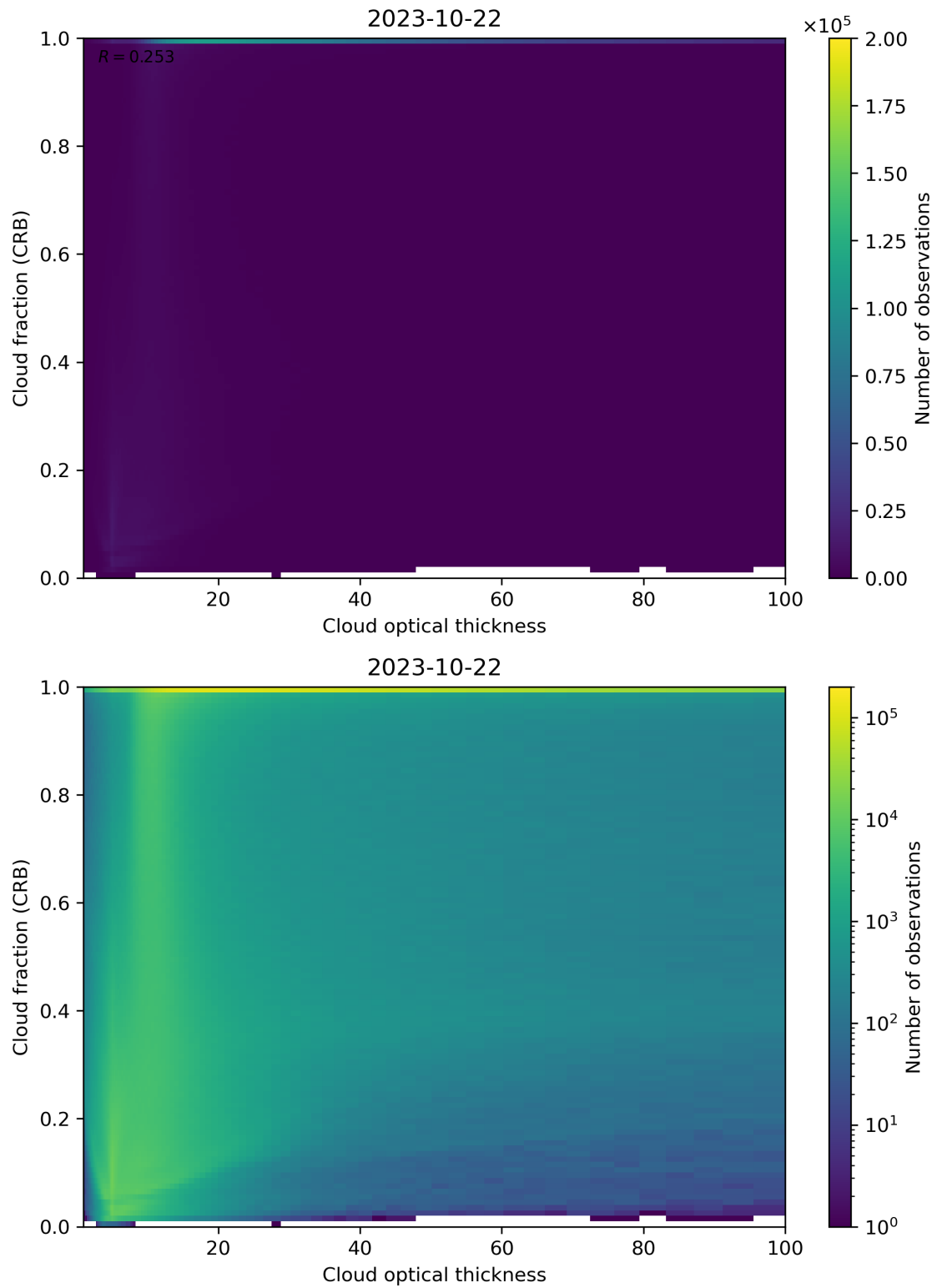
Figure 84: Scatter density plot of “Cloud optical thickness” against “Cloud fraction (CRB)” for 2023-10-22 to 2023-10-23.
