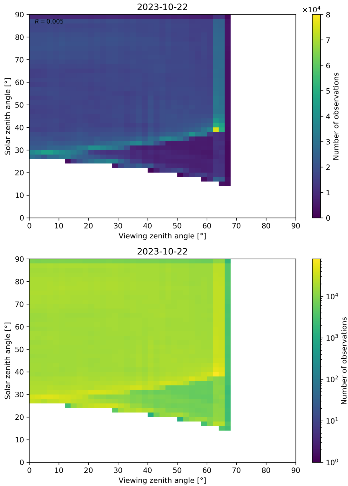
Figure 114: Scatter density plot of “Viewing zenith angle” against “Solar zenith angle” for 2023-10-22 to 2023-10-23.
