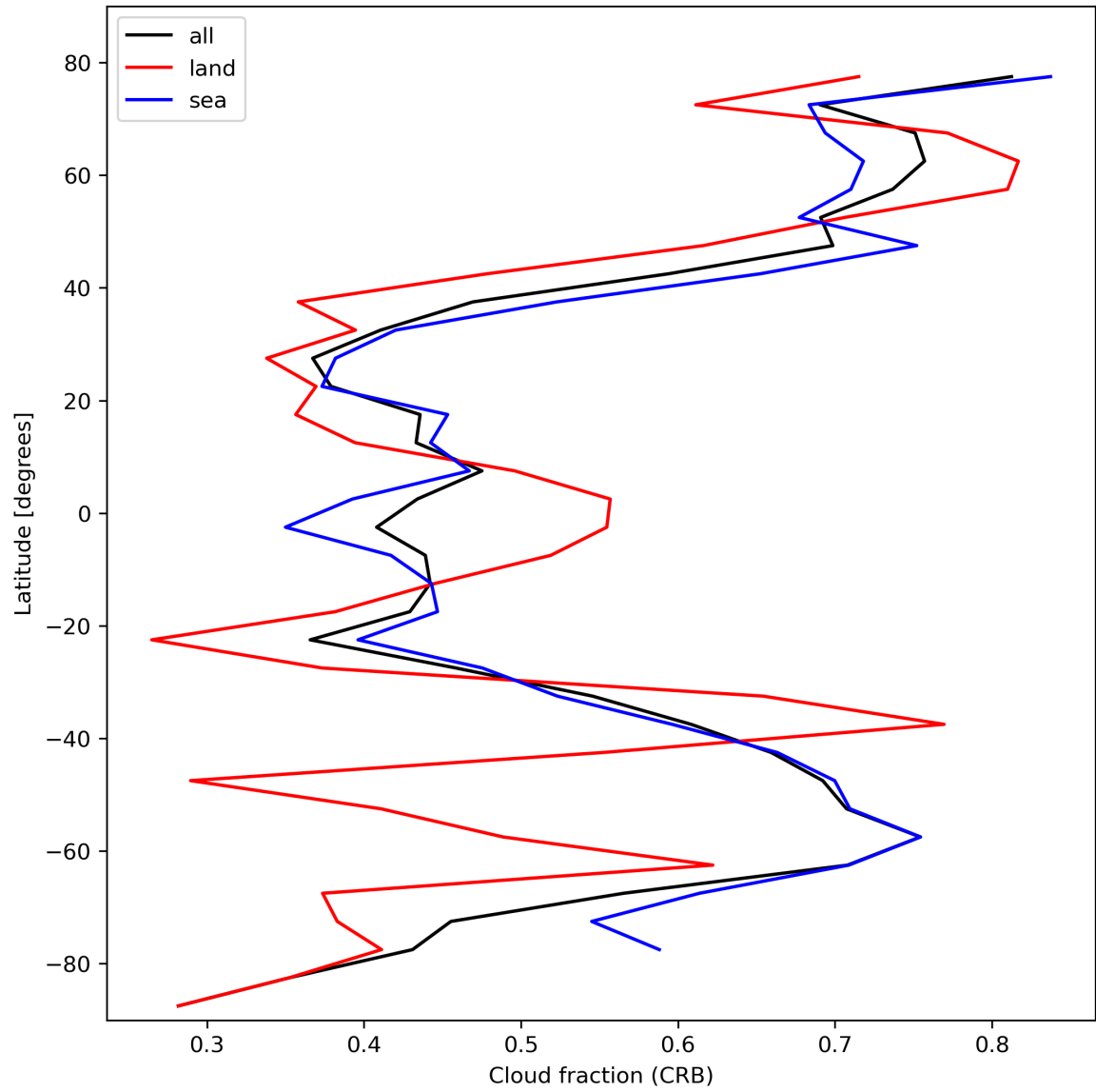
Figure 26: Zonal average of “Cloud fraction (CRB)” for 2023-10-22 to 2023-10-23.
