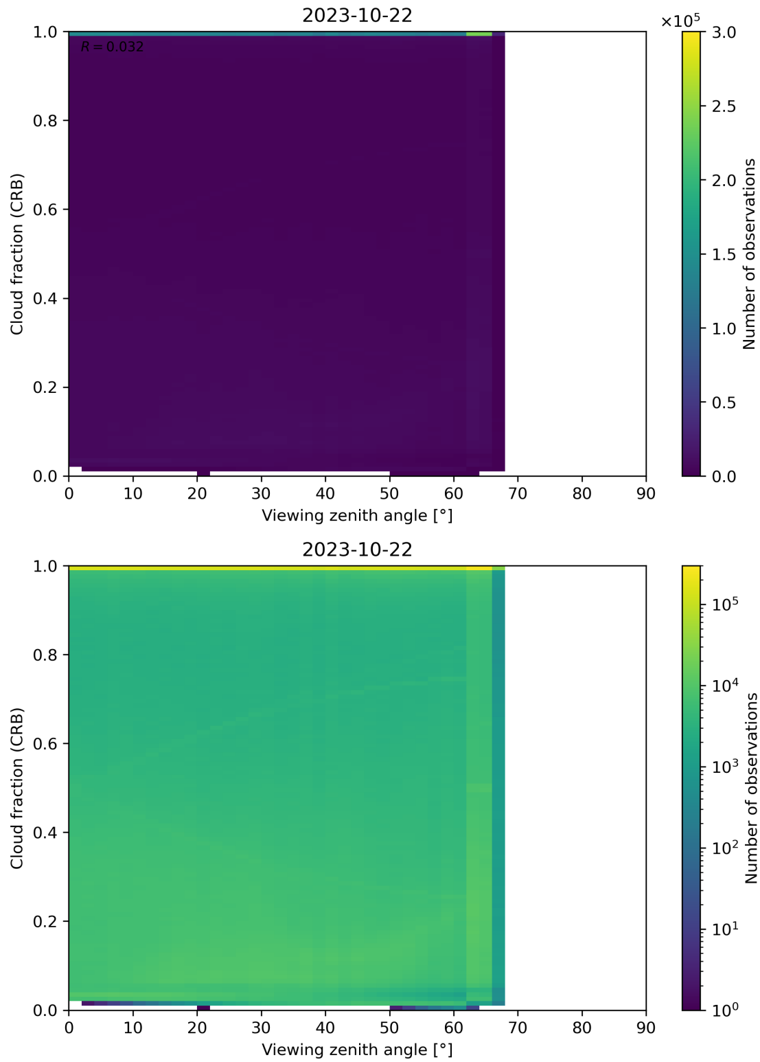
Figure 109: Scatter density plot of “Viewing zenith angle” against “Cloud fraction (CRB)” for 2023-10-22 to 2023-10-23.
