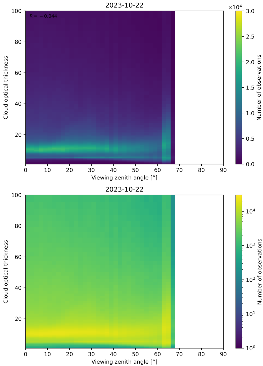
Figure 111: Scatter density plot of “Viewing zenith angle” against “Cloud optical thickness” for 2023-10-22 to 2023-10-23.
