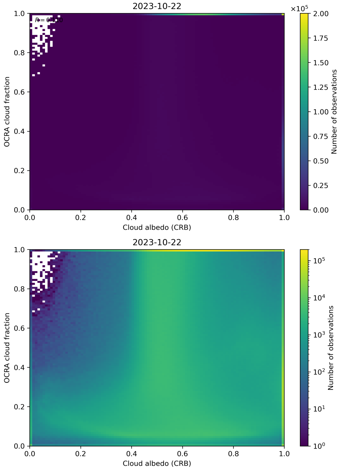
Figure 70: Scatter density plot of “Cloud albedo (CRB)” against “OCRA cloud fraction” for 2023-10-22 to 2023-10-23.
