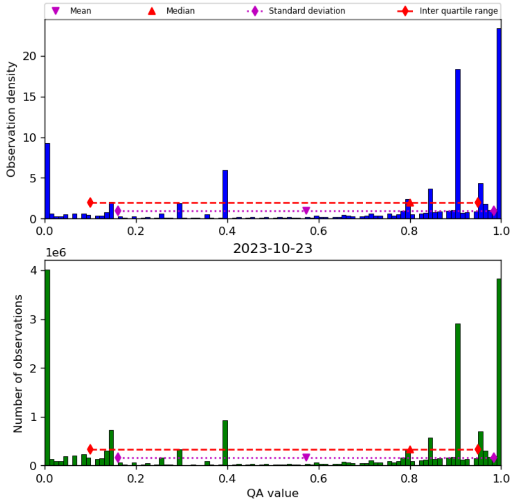
Figure 38: Histogram of “QA value” for 2023-10-22 to 2023-10-24
