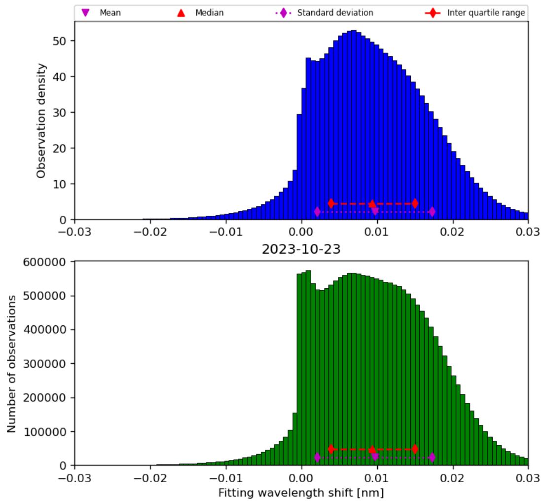
Figure 49: Histogram of “Fitting wavelength shift” for 2023-10-22 to 2023-10-24
