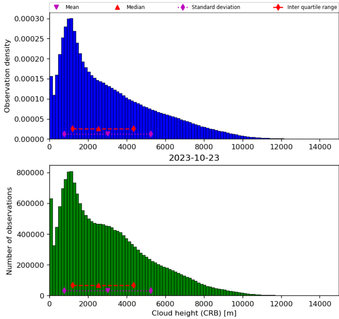
Figure 43: Histogram of “Cloud height (CRB)” for 2023-10-22 to 2023-10-24
