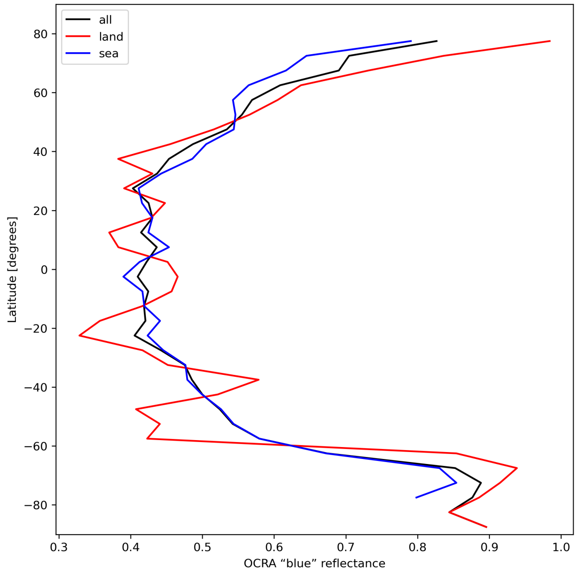
Figure 35: Zonal average of “OCRA “blue” reflectance” for 2023-10-22 to 2023-10-24.
