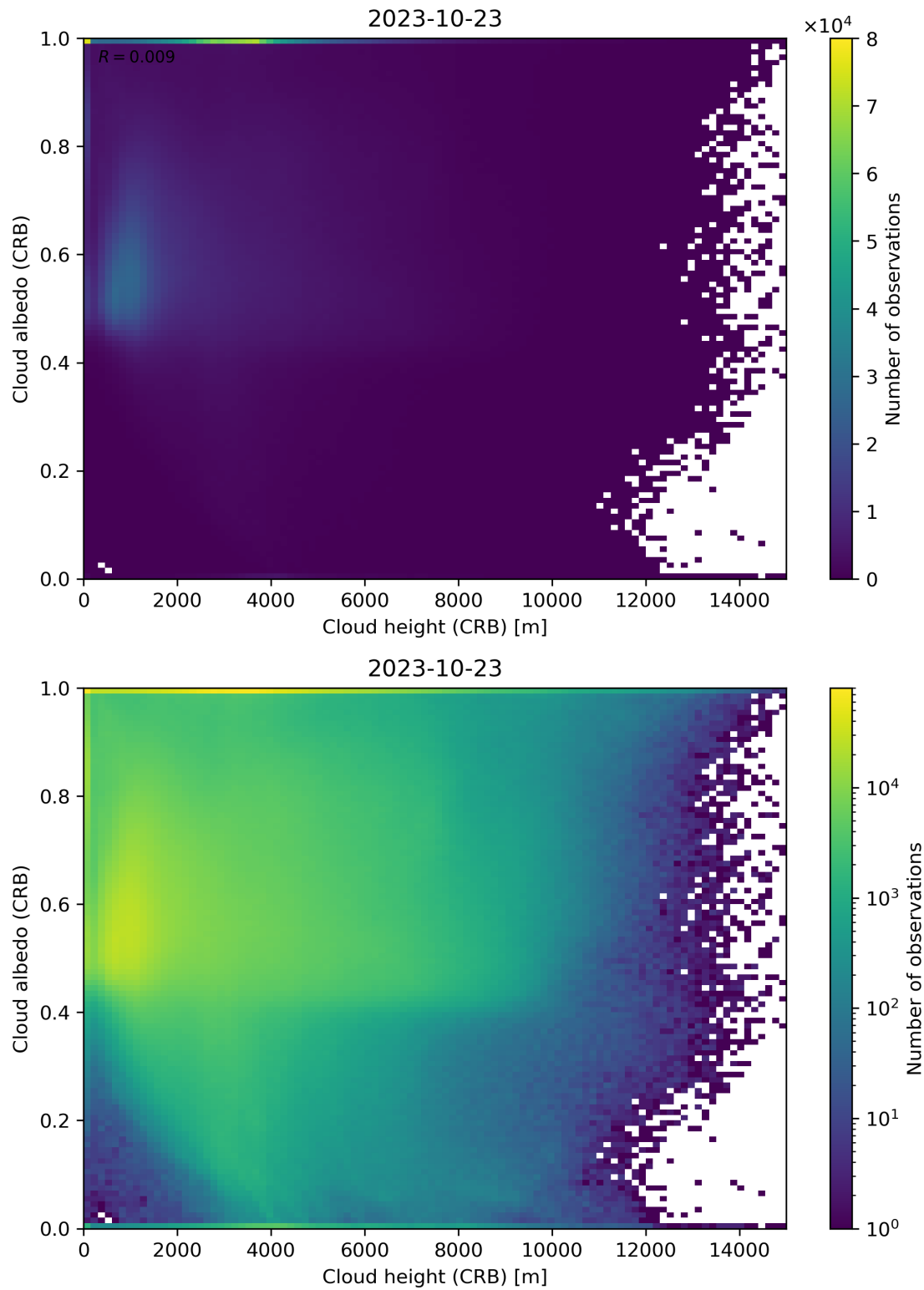
Figure 80: Scatter density plot of “Cloud height (CRB)” against “Cloud albedo (CRB)” for 2023-10-22 to 2023-10-24.
