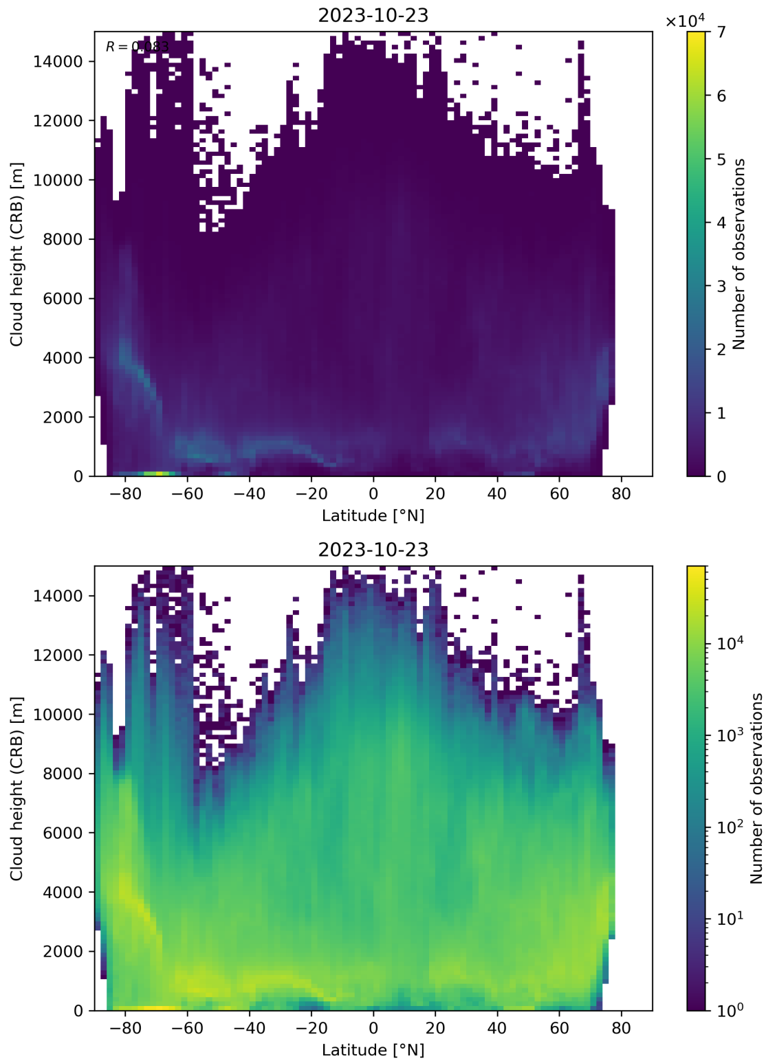
Figure 95: Scatter density plot of “Latitude” against “Cloud height (CRB)” for 2023-10-22 to 2023-10-24.
