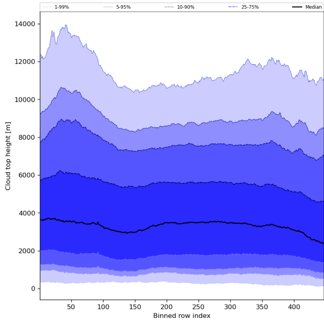
Figure 56: Along track statistics of “Cloud top height” for 2023-10-22 to 2023-10-24
