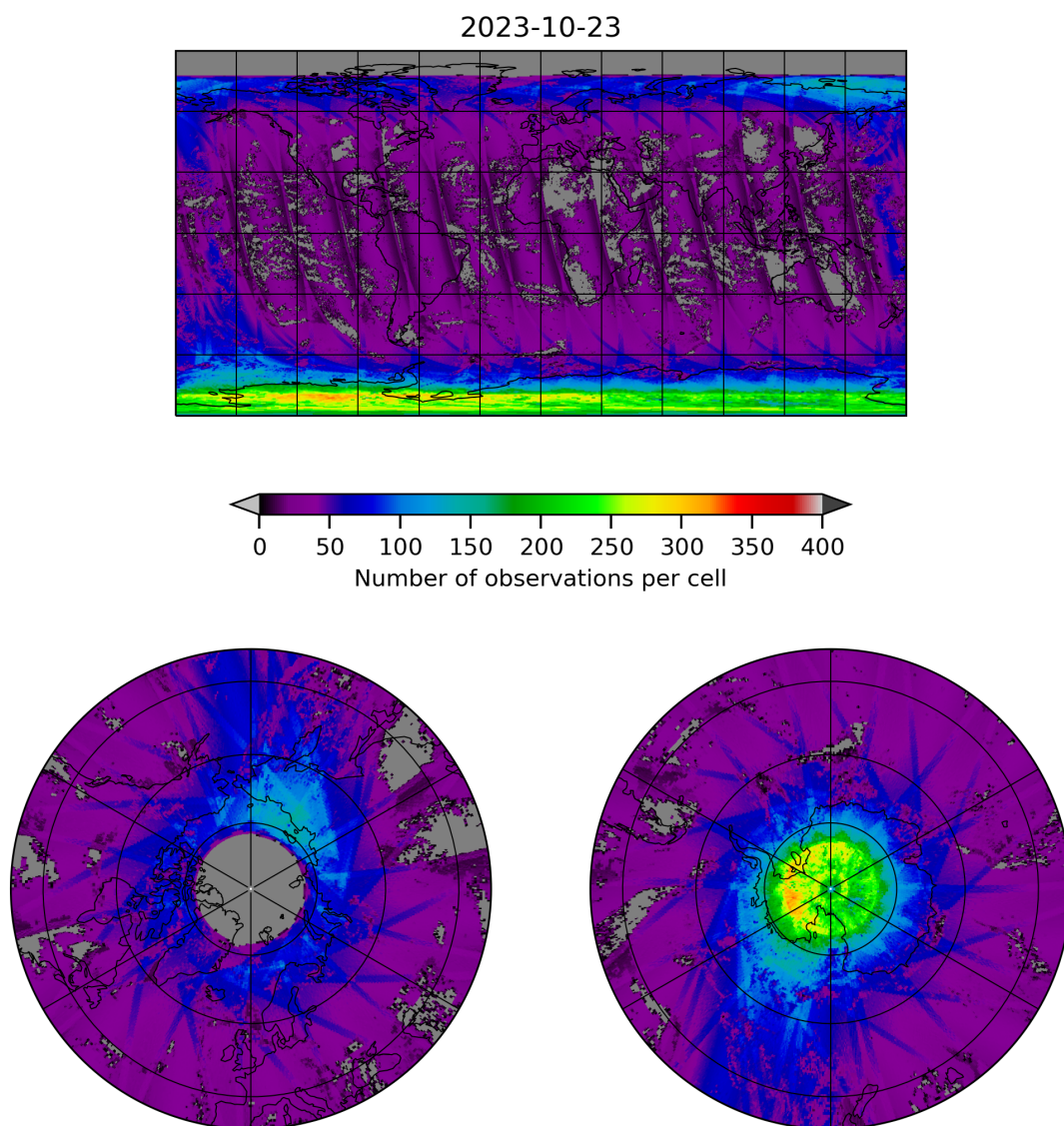
Figure 21: Map of the number of observations for 2023-10-22 to 2023-10-24
