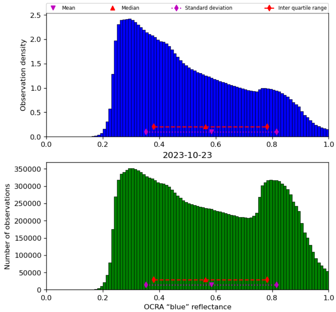
Figure 51: Histogram of “OCRA “blue” reflectance” for 2023-10-22 to 2023-10-24
