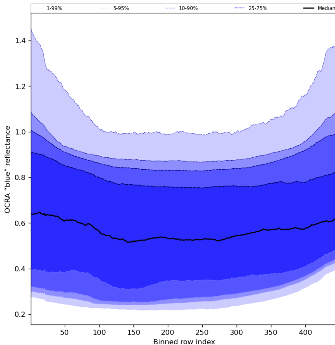
Figure 67: Along track statistics of “OCRA “blue” reflectance” for 2023-10-22 to 2023-10-24
