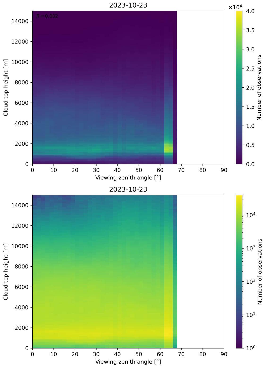
Figure 112: Scatter density plot of “Viewing zenith angle” against “Cloud top height” for 2023-10-22 to 2023-10-24.
