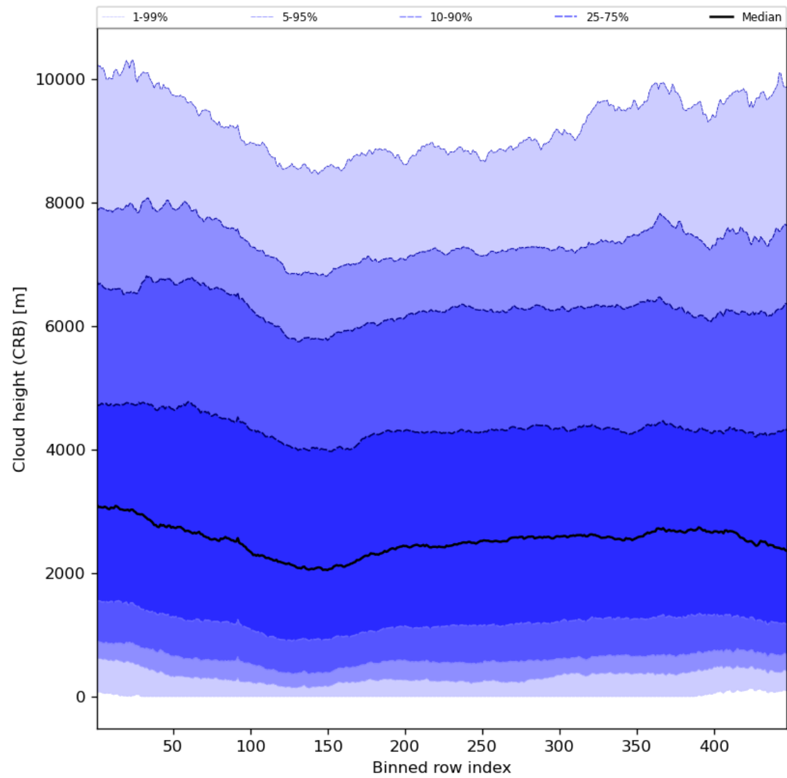
Figure 59: Along track statistics of “Cloud height (CRB)” for 2023-10-22 to 2023-10-24
