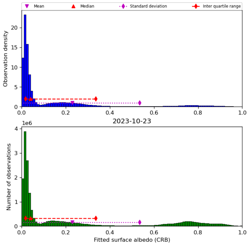
Figure 46: Histogram of “Fitted surface albedo (CRB)” for 2023-10-22 to 2023-10-24
