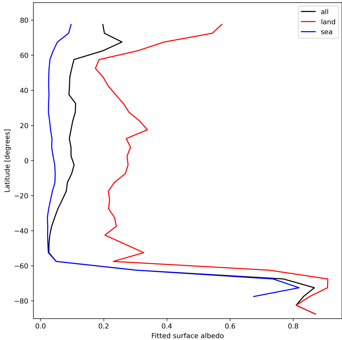
Figure 29: Zonal average of “Fitted surface albedo” for 2023-10-22 to 2023-10-24.
