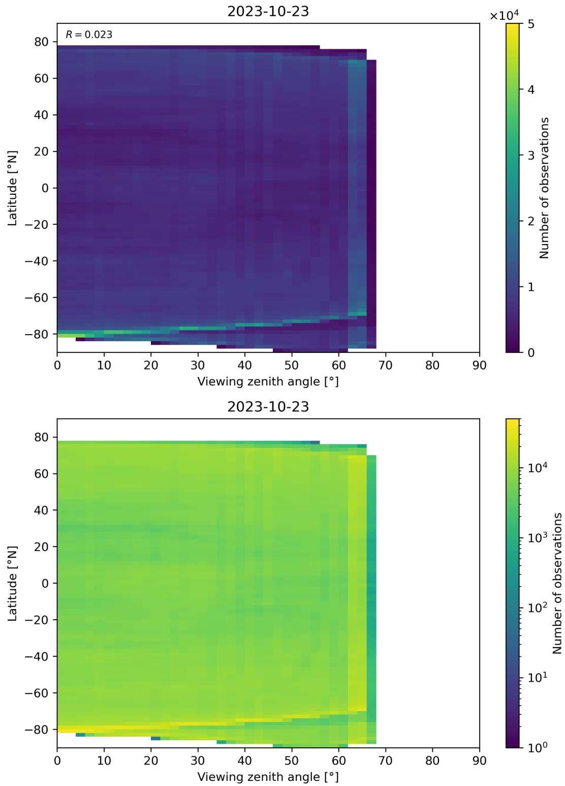
Figure 113: Scatter density plot of “Viewing zenith angle” against “Latitude” for 2023-10-22 to 2023-10-24.
