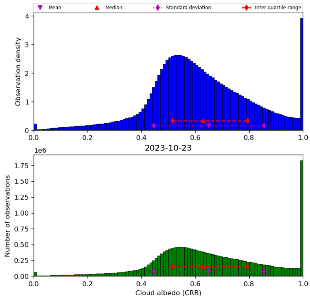
Figure 44: Histogram of “Cloud albedo (CRB)” for 2023-10-22 to 2023-10-24
