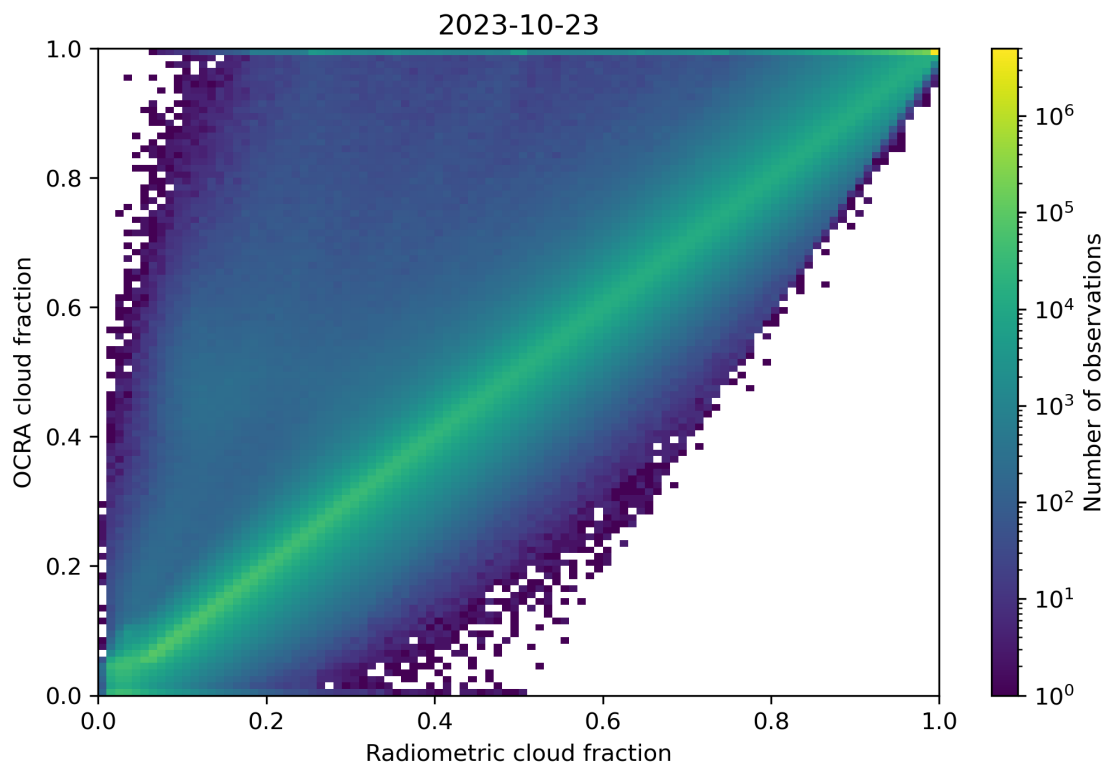
Figure 72: Scatter density plot of “Radiometric cloud fraction” against “OCRA cloud fraction” for 2023-10-22 to 2023-10-24.
