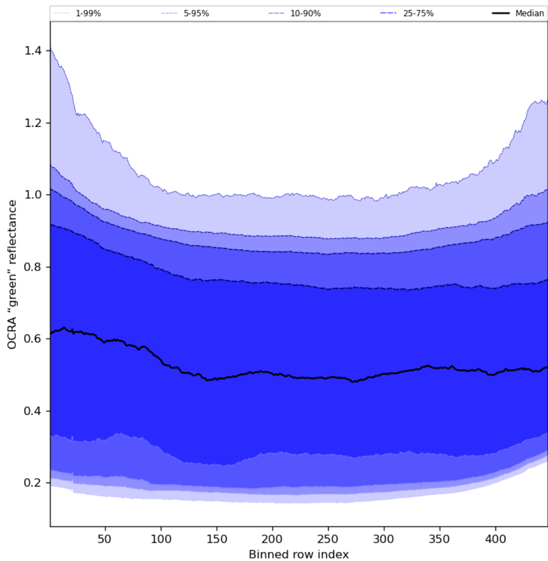
Figure 68: Along track statistics of "OCRA "green" reflectance" for 2023-10-22 to 2023-10-24
