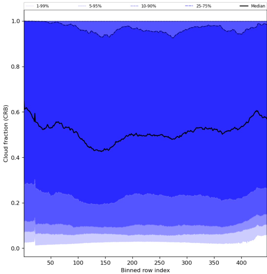
Figure 58: Along track statistics of “Cloud fraction (CRB)” for 2023-10-22 to 2023-10-24
