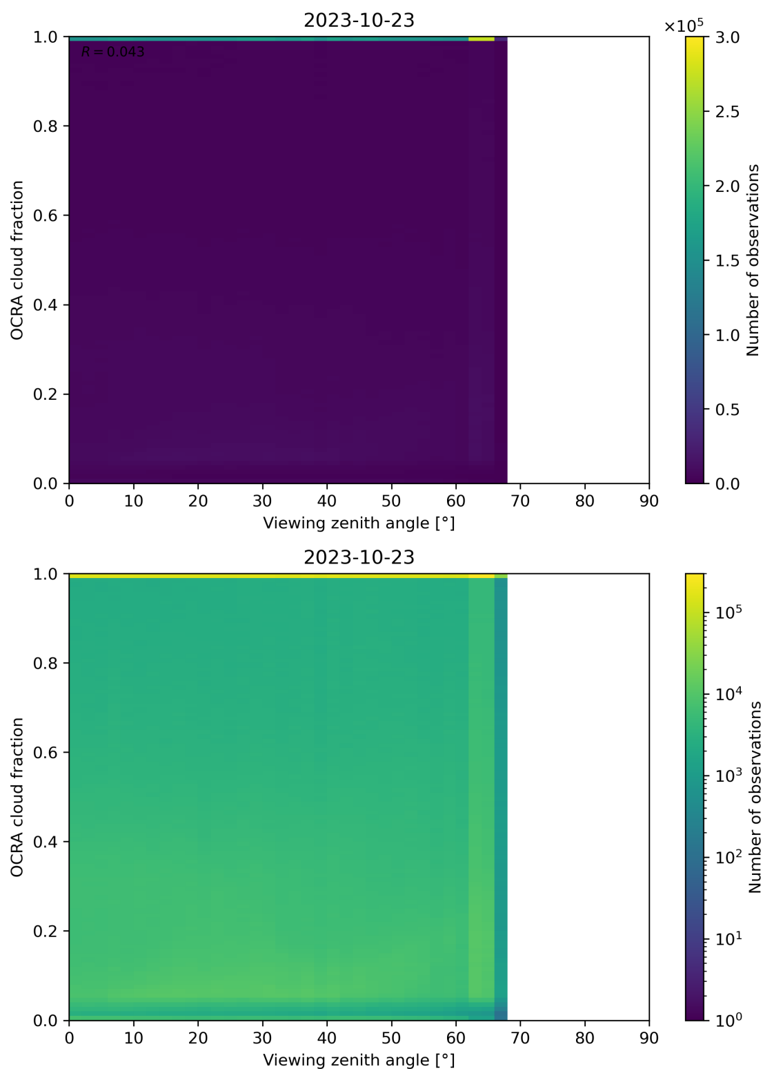
Figure 108: Scatter density plot of “Viewing zenith angle” against “OCRA cloud fraction” for 2023-10-22 to 2023-10-24.
