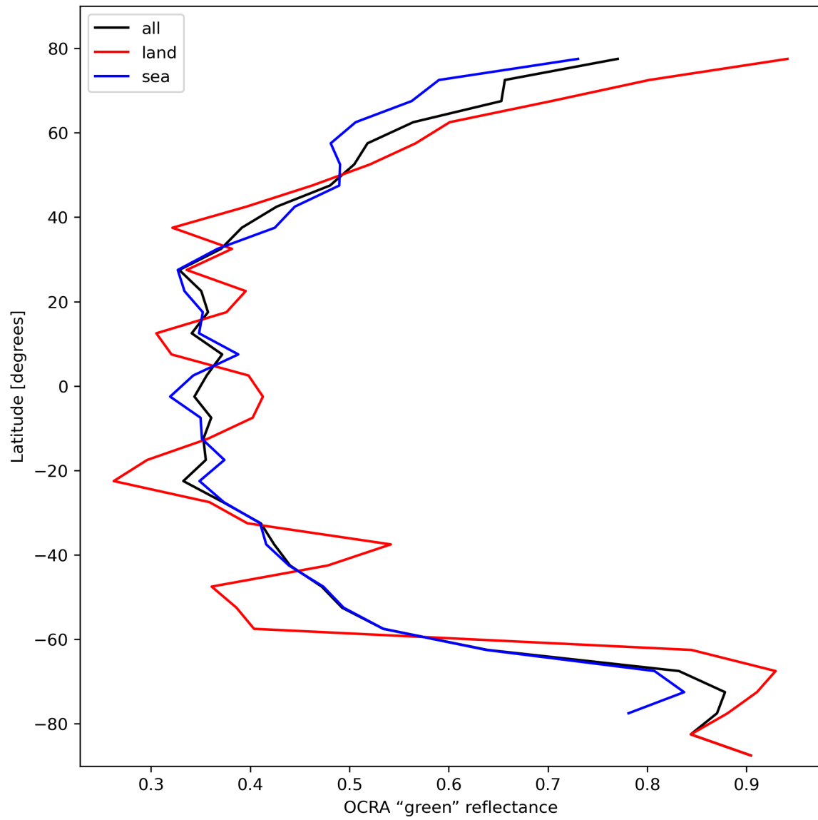
Figure 36: Zonal average of “OCRA “green” reflectance” for 2023-10-22 to 2023-10-24.
