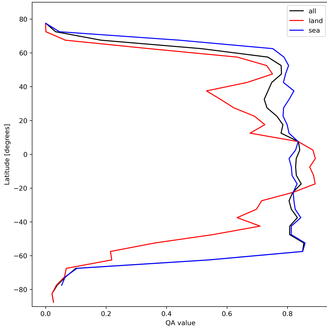
Figure 22: Zonal average of “QA value” for 2023-10-22 to 2023-10-24.
