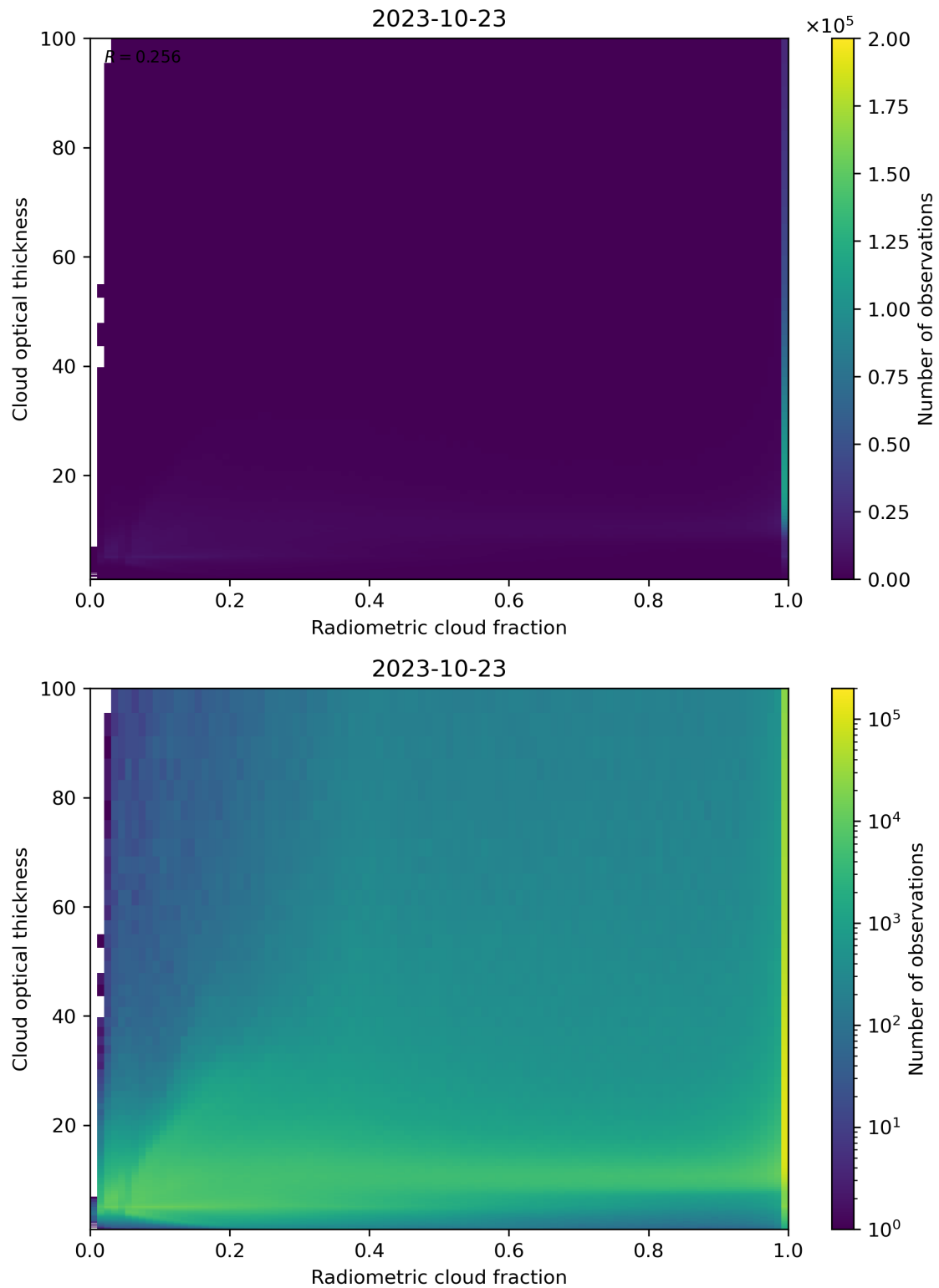
Figure 75: Scatter density plot of “Radiometric cloud fraction” against “Cloud optical thickness” for 2023-10-22 to 2023-10-24.
