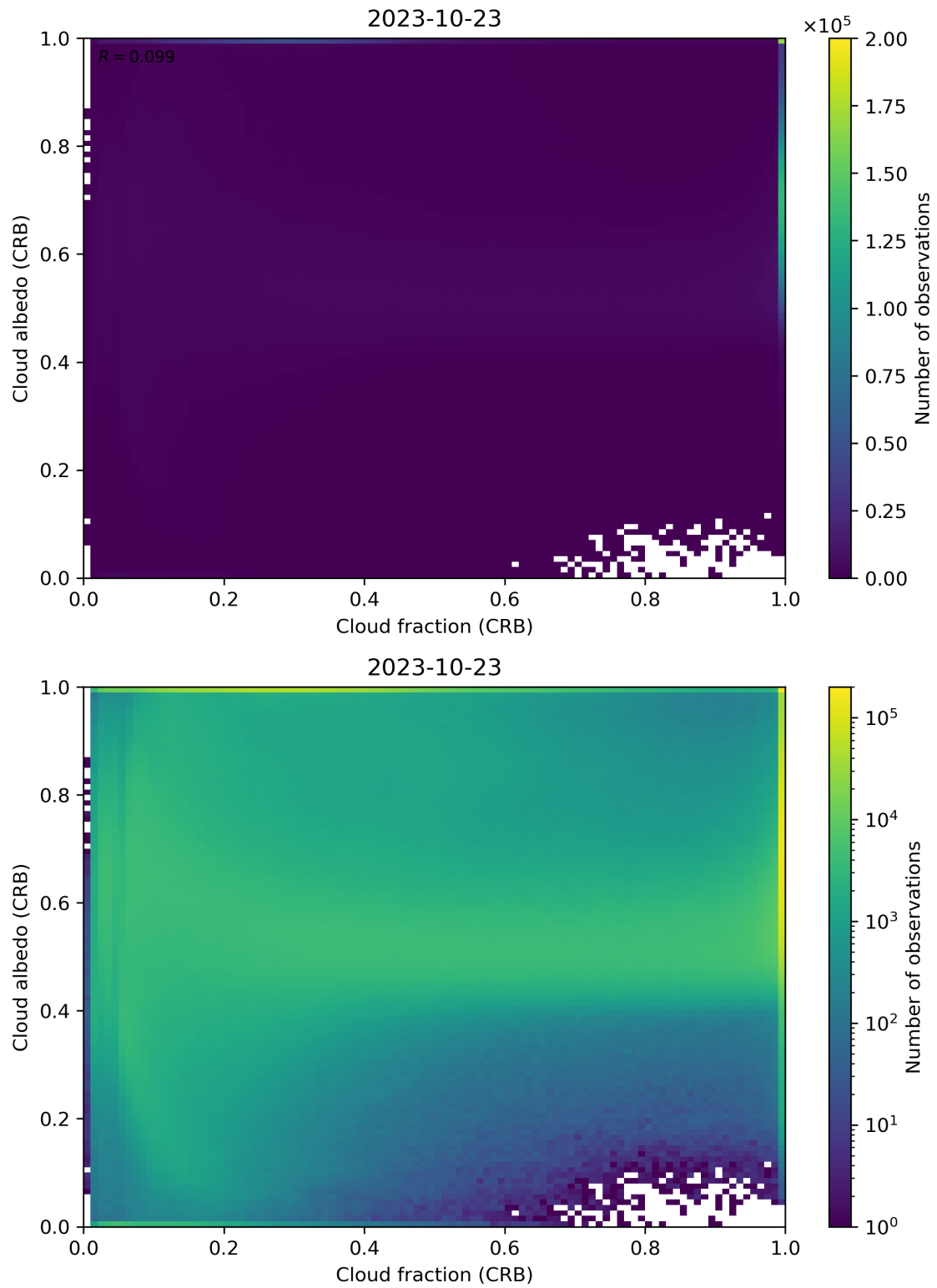
Figure 77: Scatter density plot of “Cloud fraction (CRB)” against “Cloud albedo (CRB)” for 2023-10-22 to 2023-10-24.
