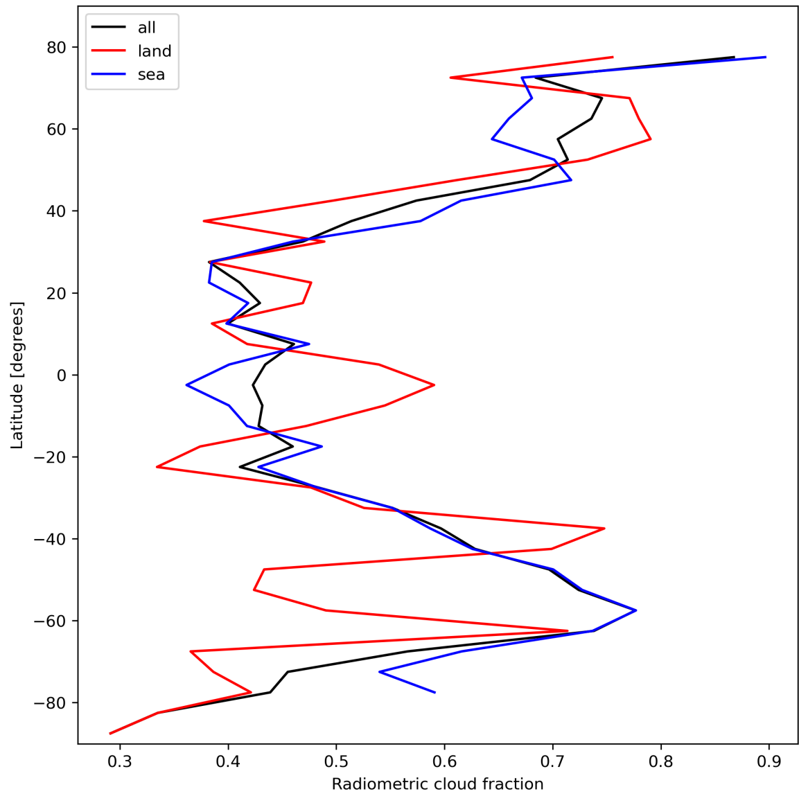
Figure 23: Zonal average of “Radiometric cloud fraction” for 2023-10-22 to 2023-10-24.
