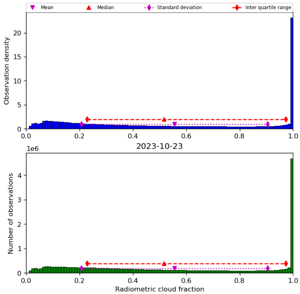
Figure 39: Histogram of “Radiometric cloud fraction” for 2023-10-22 to 2023-10-24
