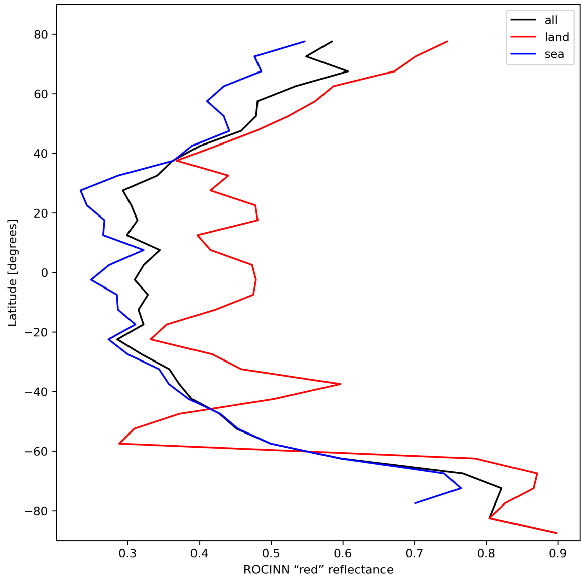
Figure 37: Zonal average of “ROCINN “red” reflectance” for 2023-10-22 to 2023-10-24.
