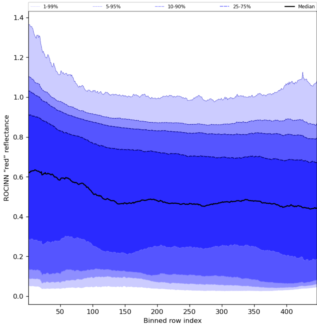
Figure 69: Along track statistics of “ROCINN “red” reflectance” for 2023-10-22 to 2023-10-24
