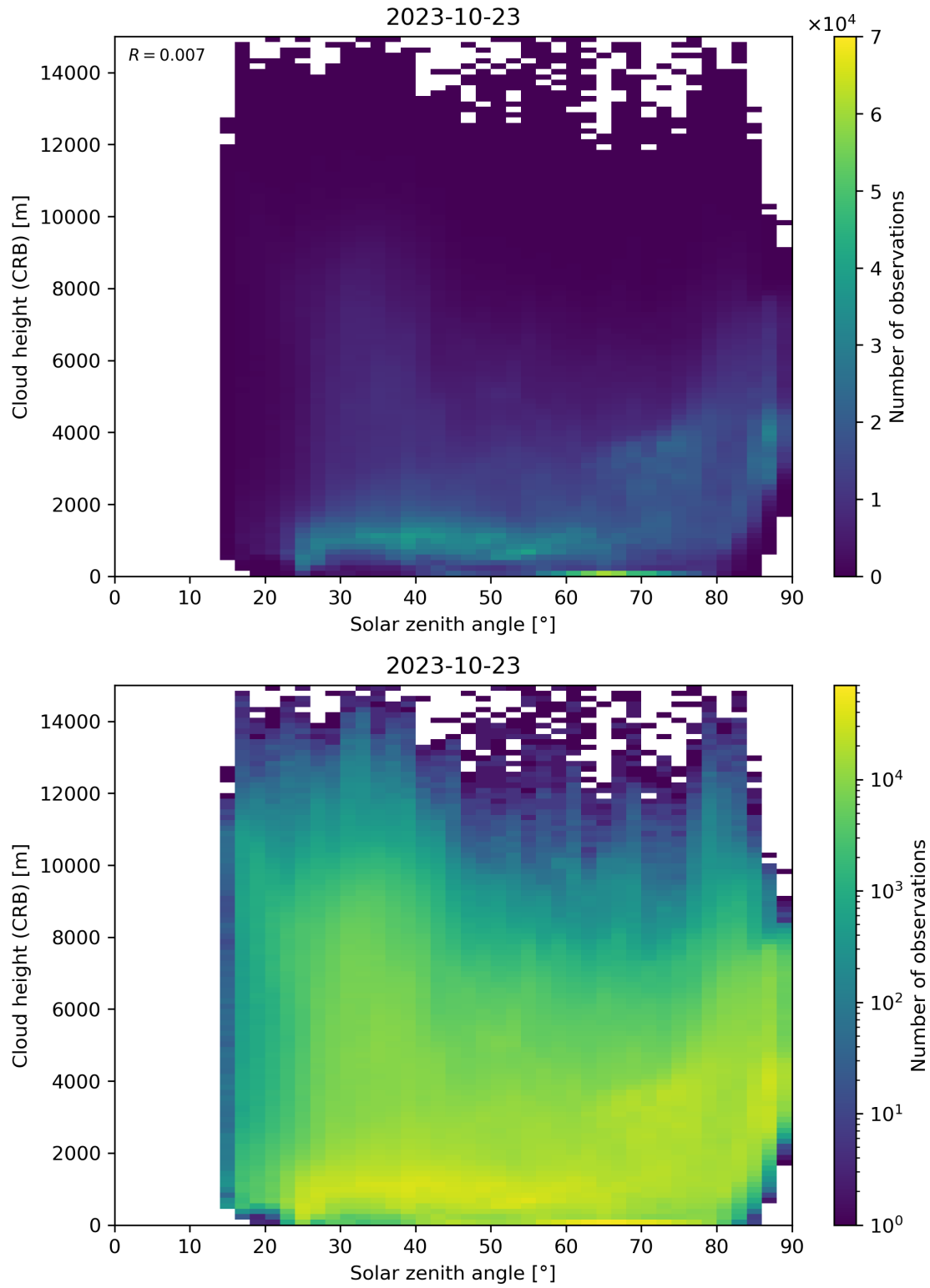
Figure 102: Scatter density plot of “Solar zenith angle” against “Cloud height (CRB)” for 2023-10-22 to 2023-10-24.
