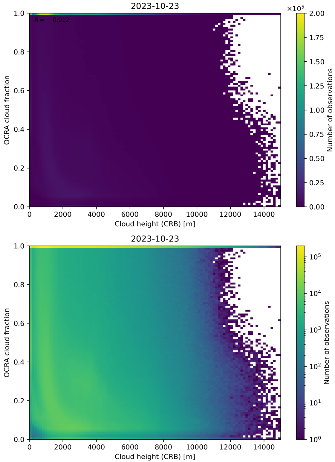
Figure 81: Scatter density plot of “Cloud height (CRB)” against “OCRA cloud fraction” for 2023-10-22 to 2023-10-24.
