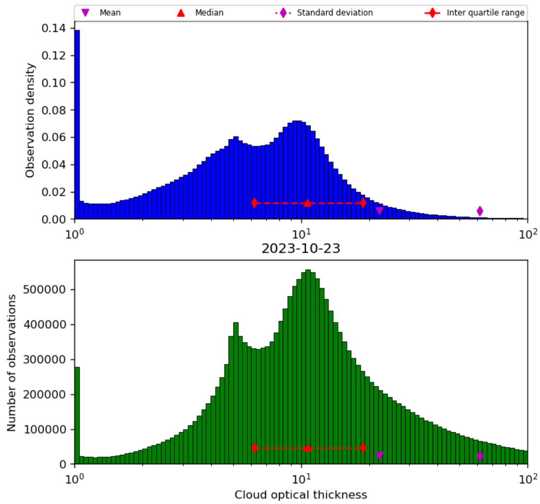
Figure 41: Histogram of “Cloud optical thickness” for 2023-10-22 to 2023-10-24
