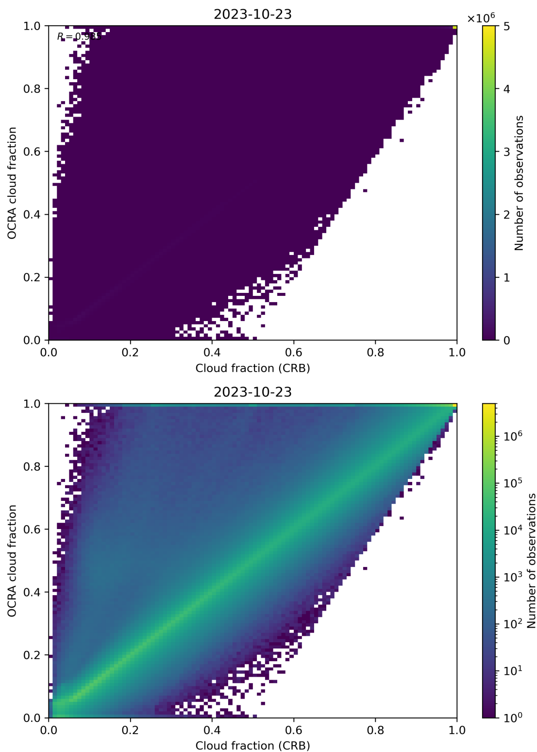
Figure 78: Scatter density plot of “Cloud fraction (CRB)” against “OCRA cloud fraction” for 2023-10-22 to 2023-10-24.
