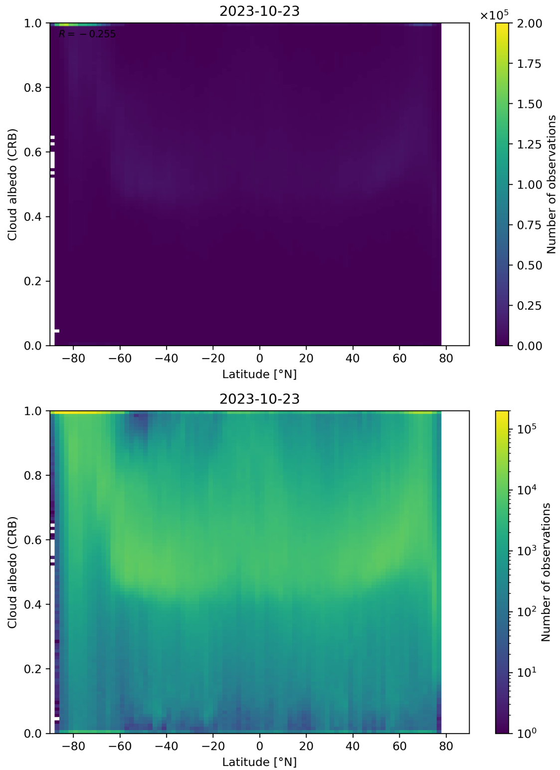
Figure 91: Scatter density plot of “Latitude” against “Cloud albedo (CRB)” for 2023-10-22 to 2023-10-24.
