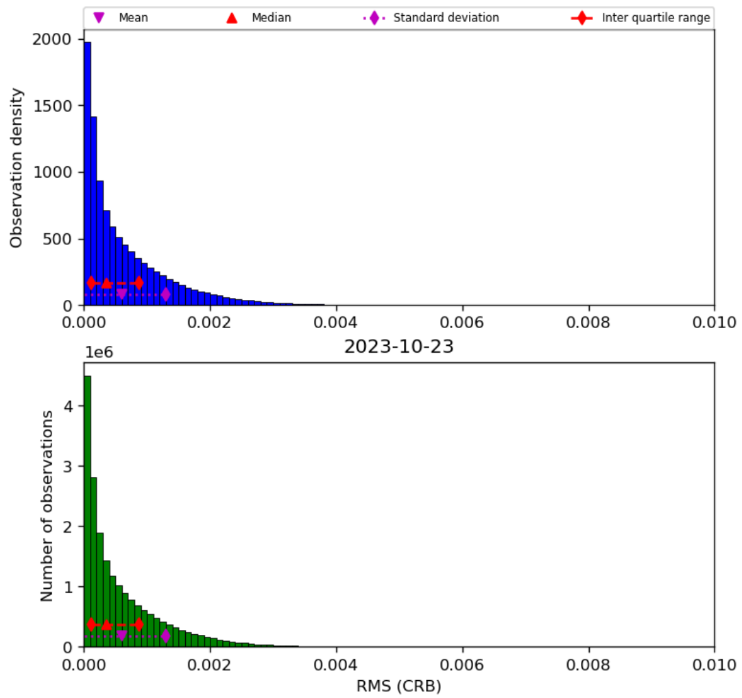
Figure 48: Histogram of “RMS (CRB)” for 2023-10-22 to 2023-10-24
