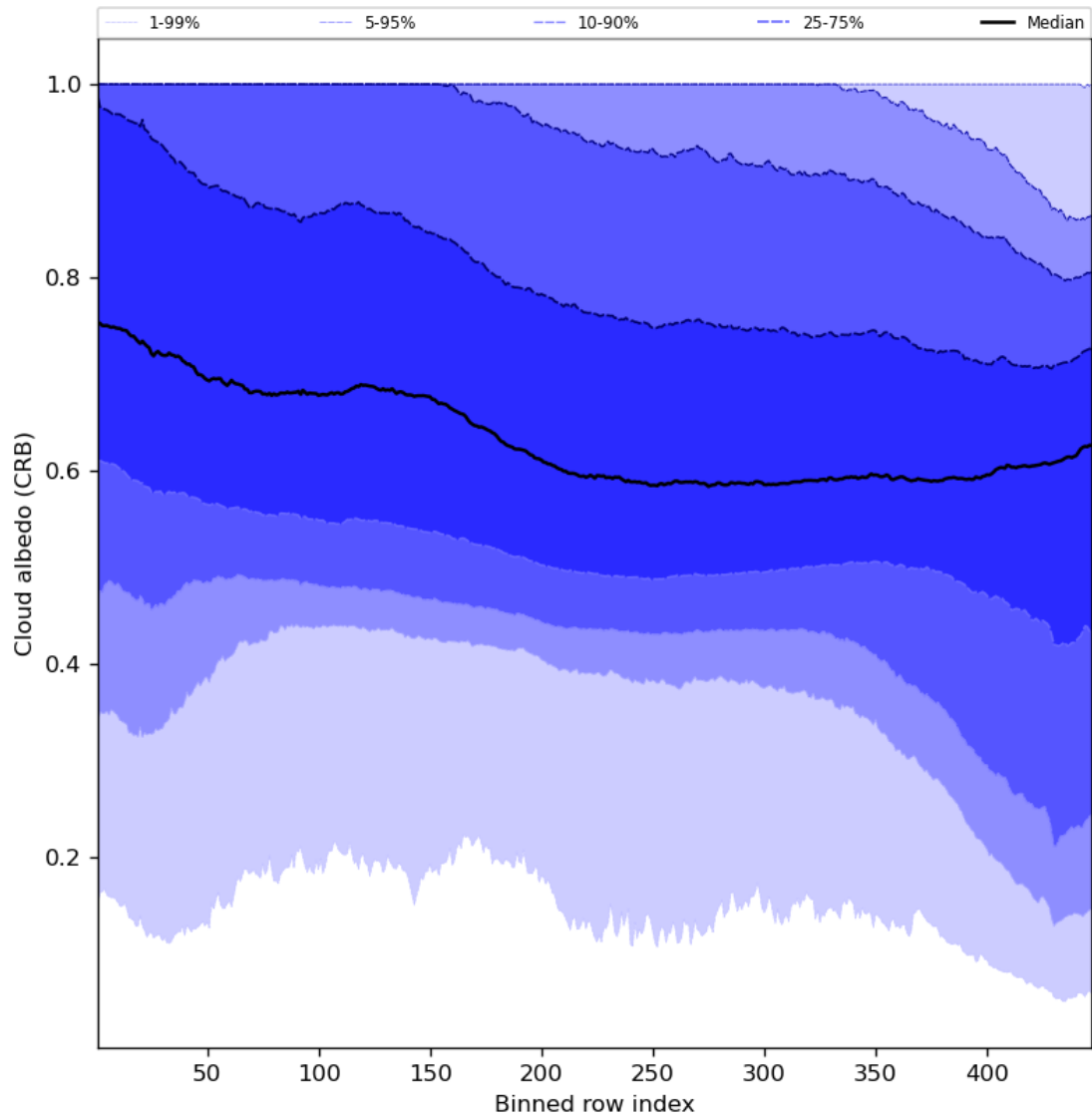
Figure 60: Along track statistics of “Cloud albedo (CRB)” for 2023-10-22 to 2023-10-24
