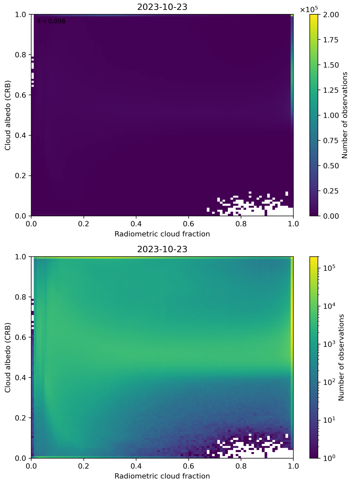
Figure 71: Scatter density plot of “Radiometric cloud fraction” against “Cloud albedo (CRB)” for 2023-10-22 to 2023-10-24.
