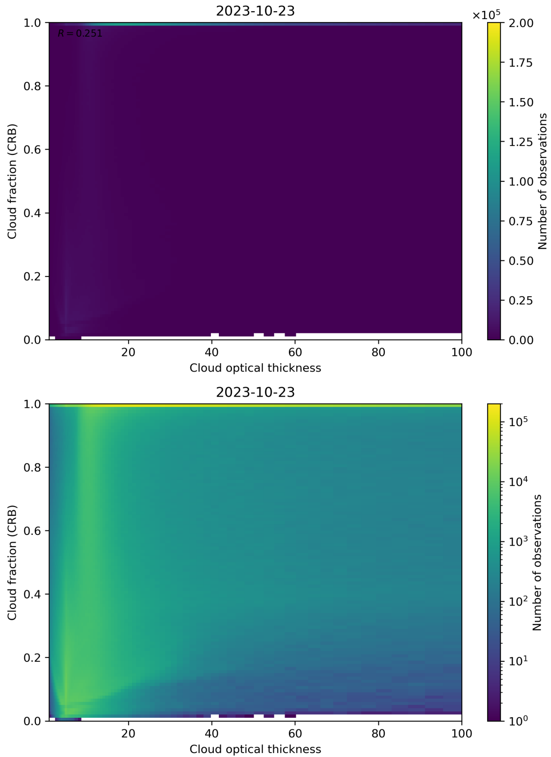
Figure 84: Scatter density plot of “Cloud optical thickness” against “Cloud fraction (CRB)” for 2023-10-22 to 2023-10-24.
