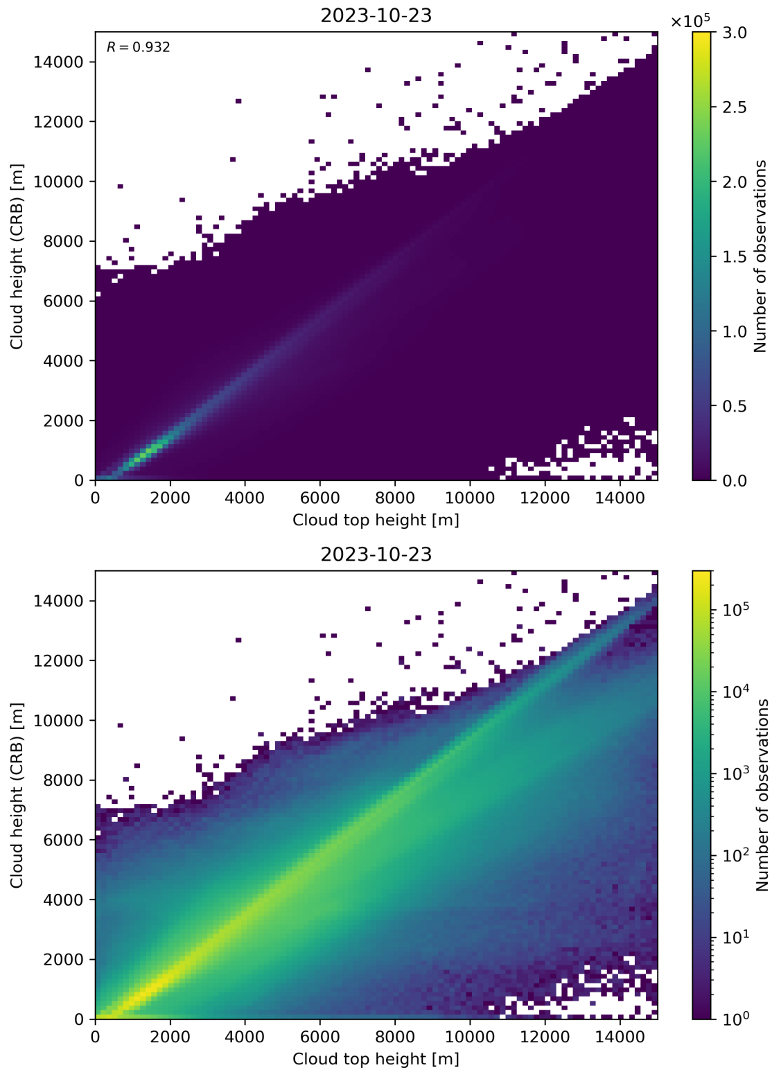
Figure 89: Scatter density plot of “Cloud top height” against “Cloud height (CRB)” for 2023-10-22 to 2023-10-24.
