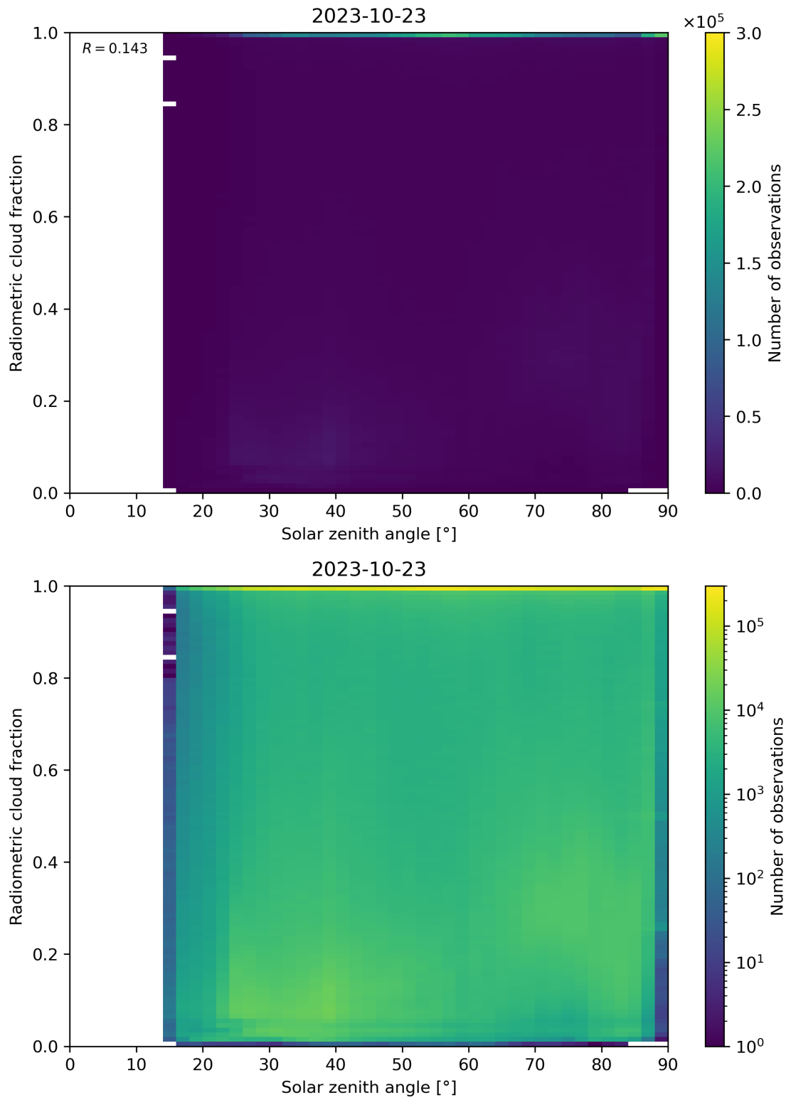
Figure 99: Scatter density plot of “Solar zenith angle” against “Radiometric cloud fraction” for 2023-10-22 to 2023-10-24.
