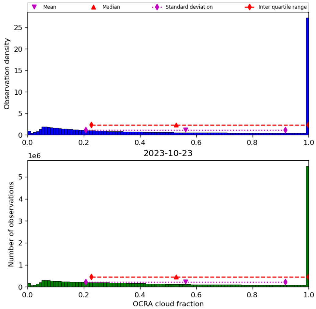
Figure 50: Histogram of “OCRA cloud fraction” for 2023-10-22 to 2023-10-24
