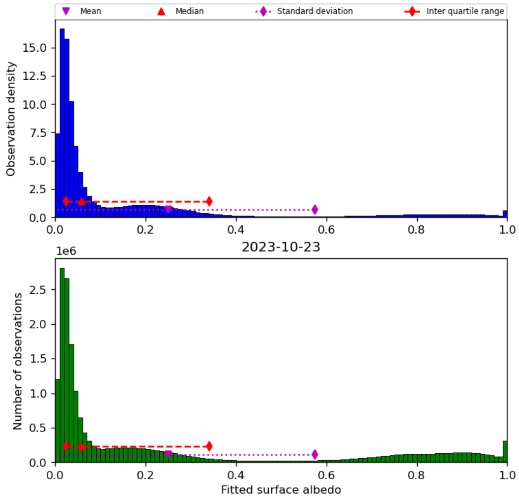
Figure 45: Histogram of “Fitted surface albedo” for 2023-10-22 to 2023-10-24
