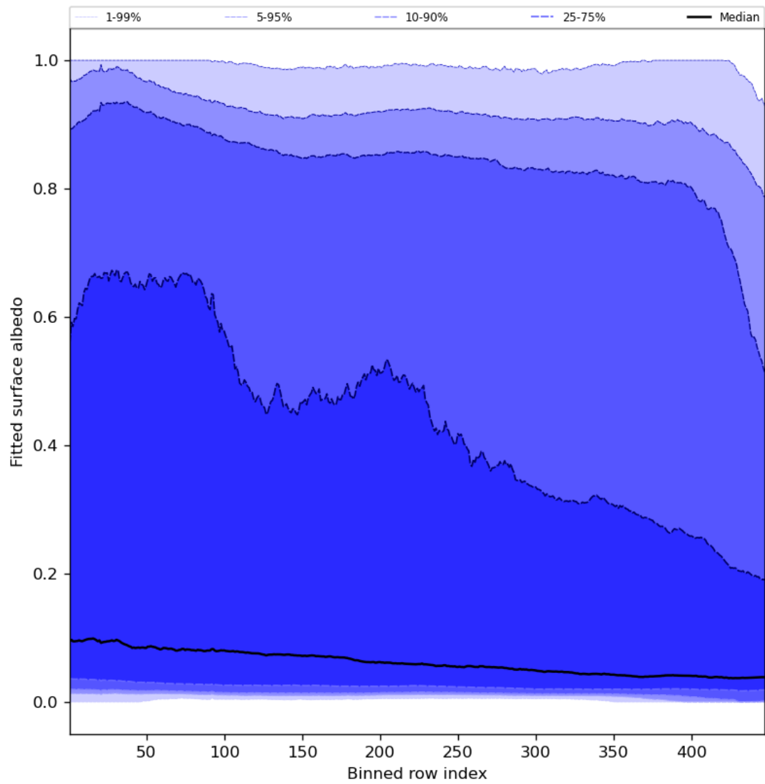
Figure 61: Along track statistics of “Fitted surface albedo” for 2023-10-22 to 2023-10-24
