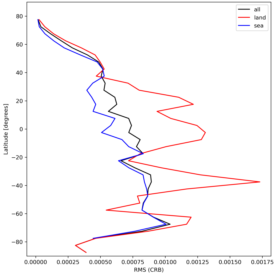
Figure 32: Zonal average of “RMS (CRB)” for 2023-10-22 to 2023-10-24.
