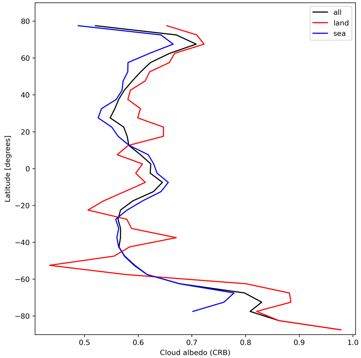
Figure 28: Zonal average of “Cloud albedo (CRB)” for 2023-10-22 to 2023-10-24.
