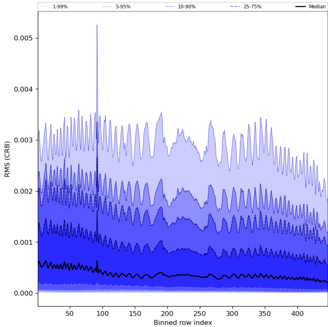
Figure 64: Along track statistics of “RMS (CRB)” for 2023-10-22 to 2023-10-24
