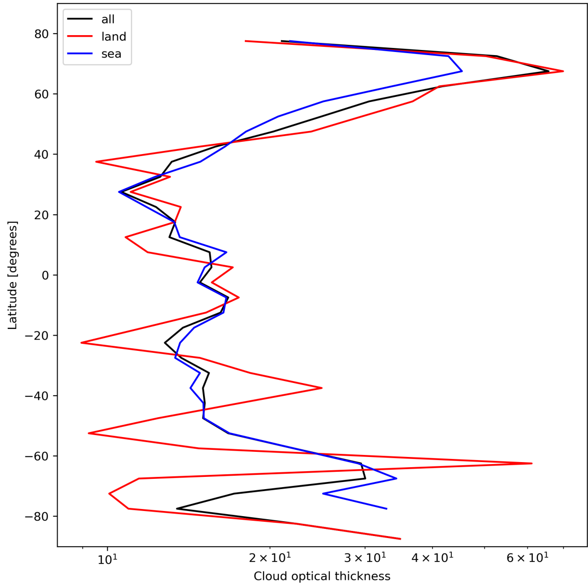
Figure 25: Zonal average of “Cloud optical thickness” for 2023-10-22 to 2023-10-24.
