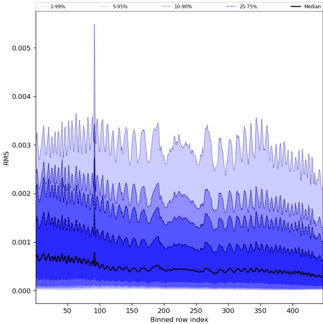
Figure 63: Along track statistics of “RMS” for 2023-10-22 to 2023-10-24
