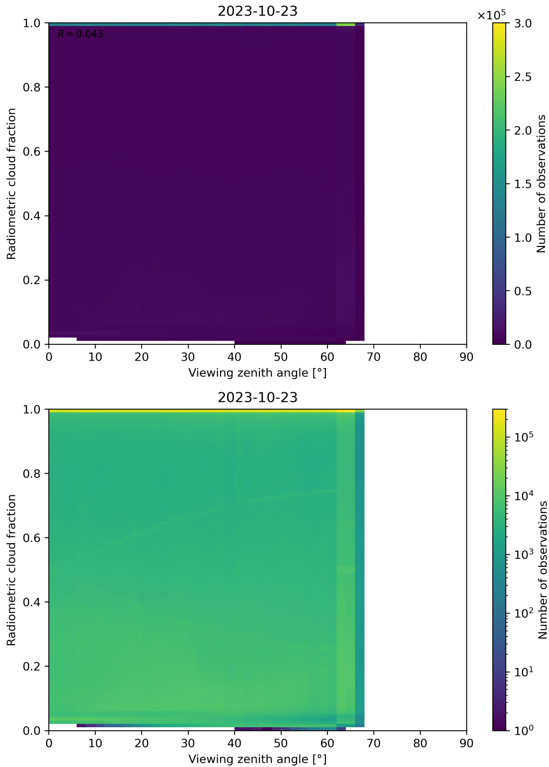
Figure 107: Scatter density plot of “Viewing zenith angle” against “Radiometric cloud fraction” for 2023-10-22 to 2023-10-24.
