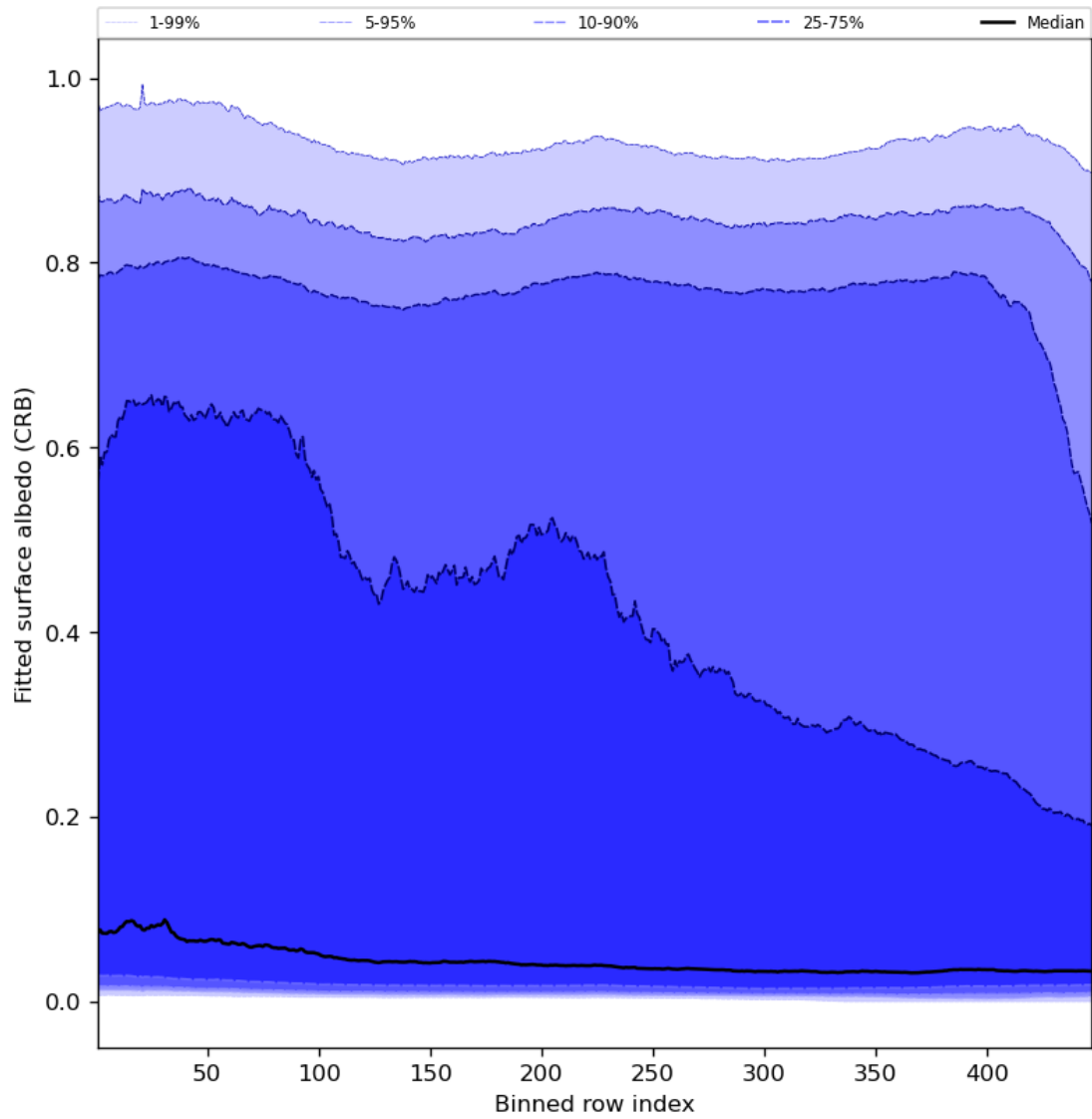
Figure 62: Along track statistics of “Fitted surface albedo (CRB)” for 2023-10-22 to 2023-10-24
