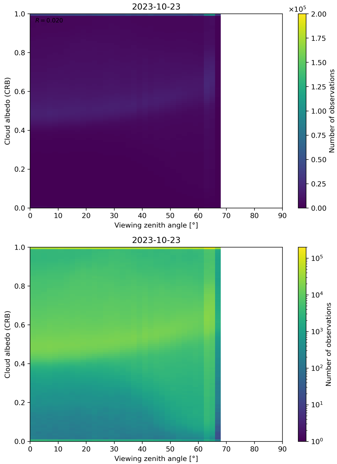
Figure 106: Scatter density plot of “Viewing zenith angle” against “Cloud albedo (CRB)” for 2023-10-22 to 2023-10-24.
