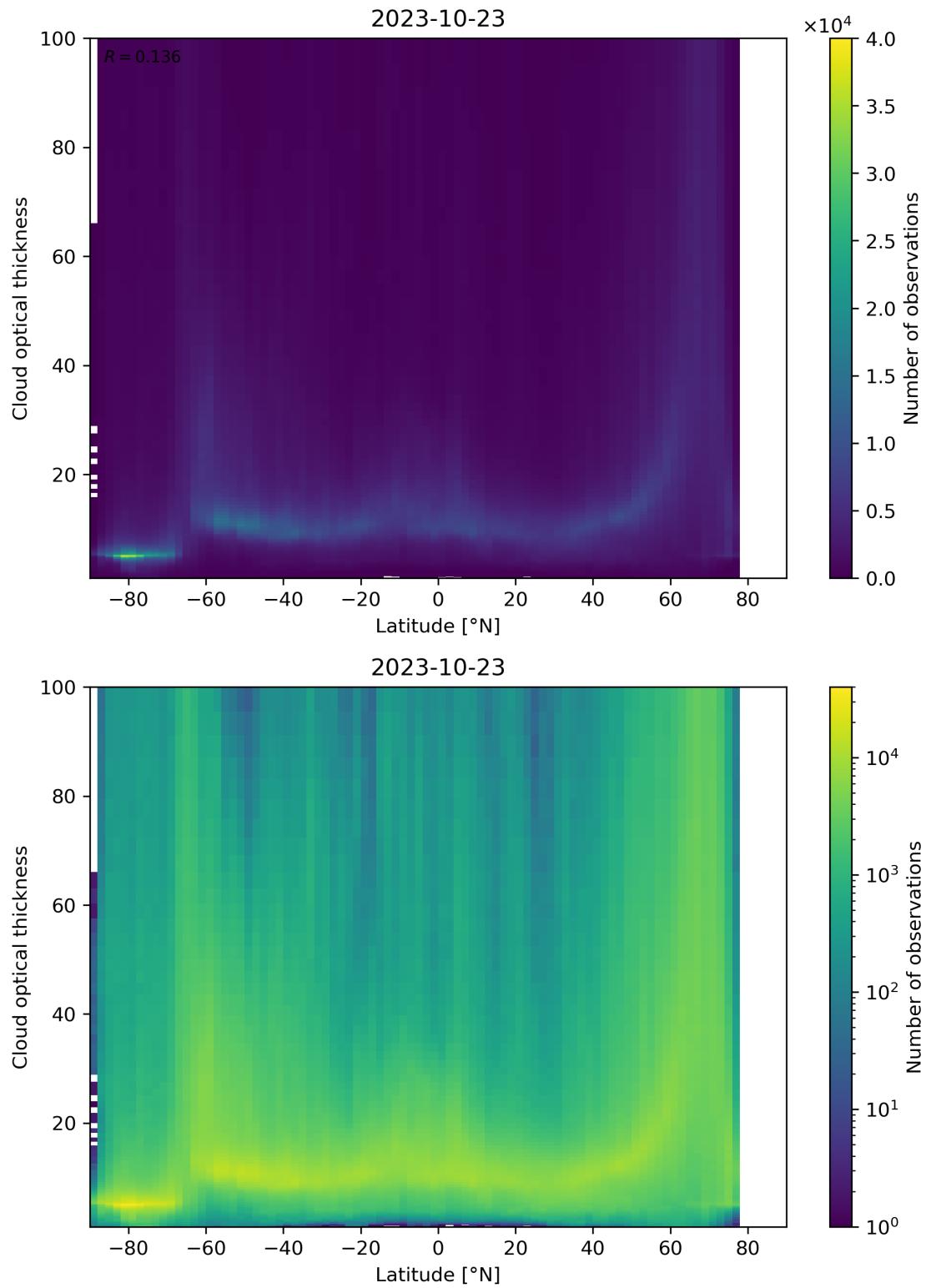
Figure 96: Scatter density plot of “Latitude” against “Cloud optical thickness” for 2023-10-22 to 2023-10-24.
