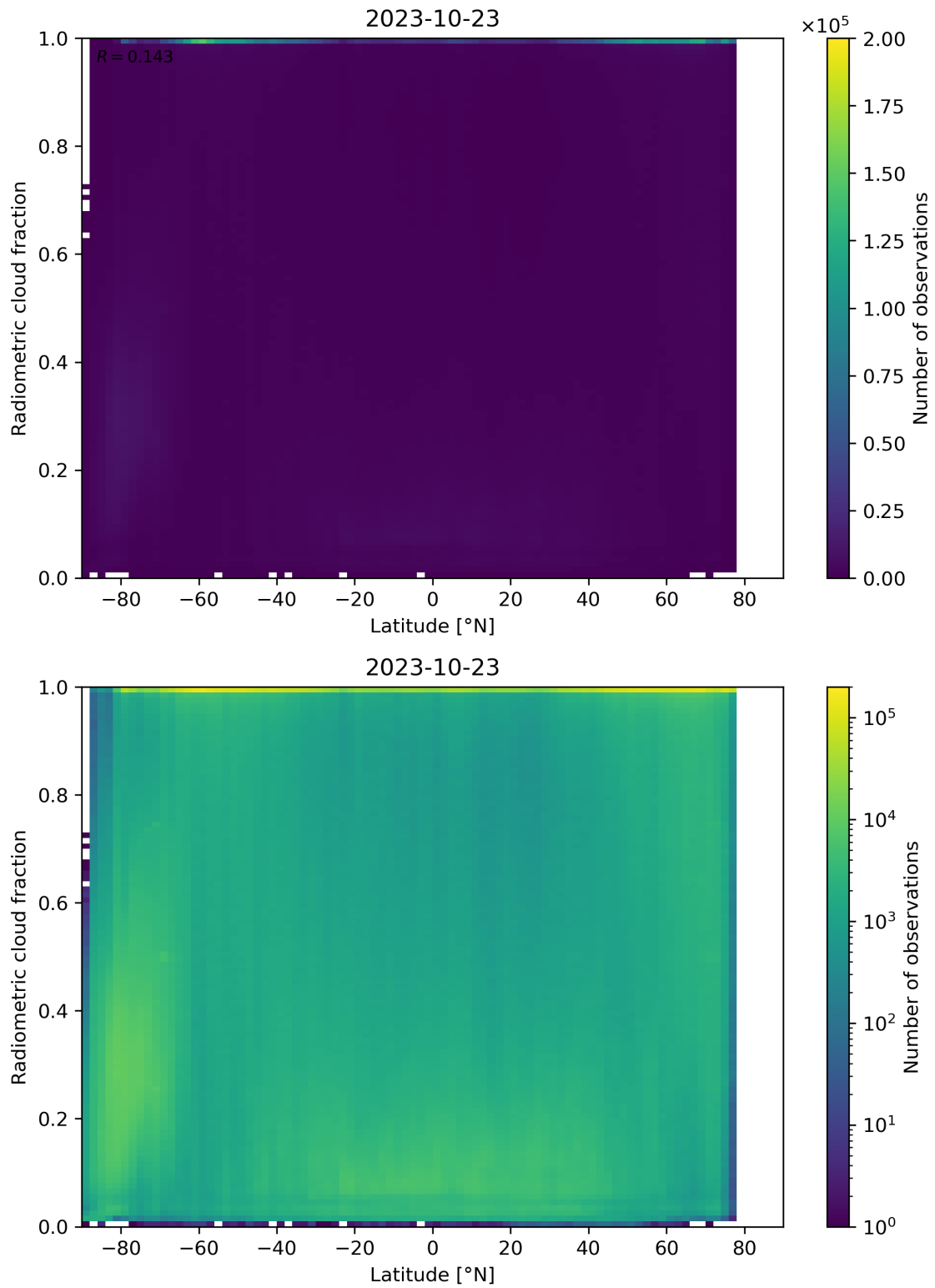
Figure 92: Scatter density plot of “Latitude” against “Radiometric cloud fraction” for 2023-10-22 to 2023-10-24.
