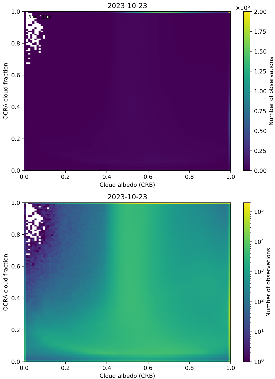
Figure 70: Scatter density plot of “Cloud albedo (CRB)” against “OCRA cloud fraction” for 2023-10-22 to 2023-10-24.
