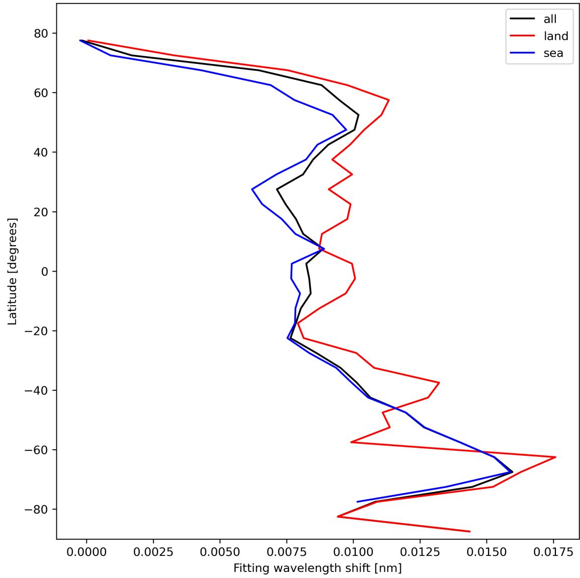
Figure 33: Zonal average of “Fitting wavelength shift” for 2023-10-22 to 2023-10-24.
