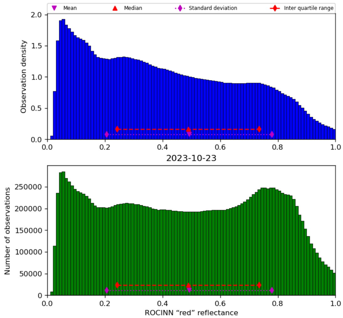
Figure 53: Histogram of “ROCINN “red” reflectance” for 2023-10-22 to 2023-10-24
