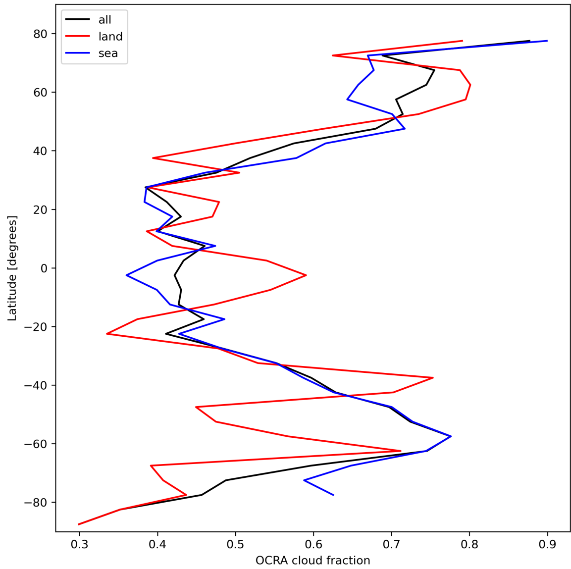
Figure 34: Zonal average of “OCRA cloud fraction” for 2023-10-22 to 2023-10-24.
