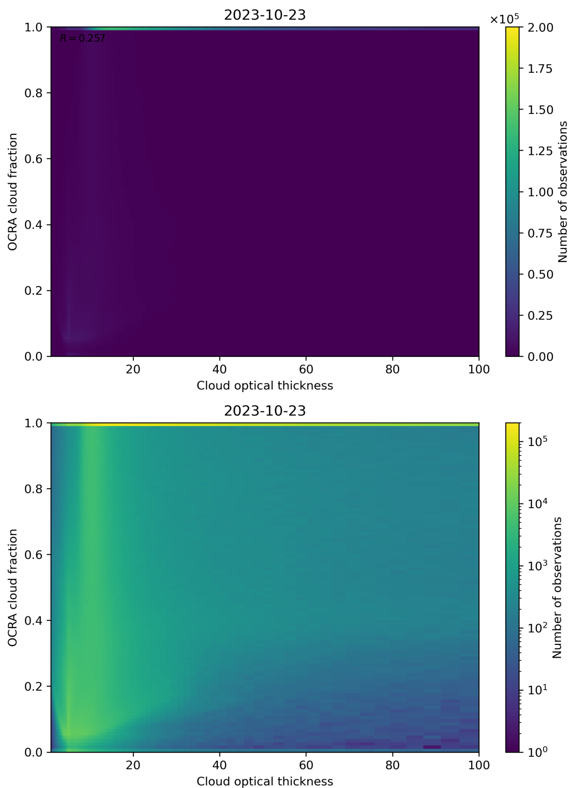
Figure 83: Scatter density plot of “Cloud optical thickness” against “OCRA cloud fraction” for 2023-10-22 to 2023-10-24.
