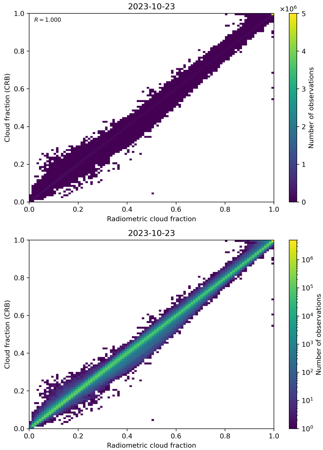
Figure 73: Scatter density plot of “Radiometric cloud fraction” against “Cloud fraction (CRB)” for 2023-10-22 to 2023-10-24.
