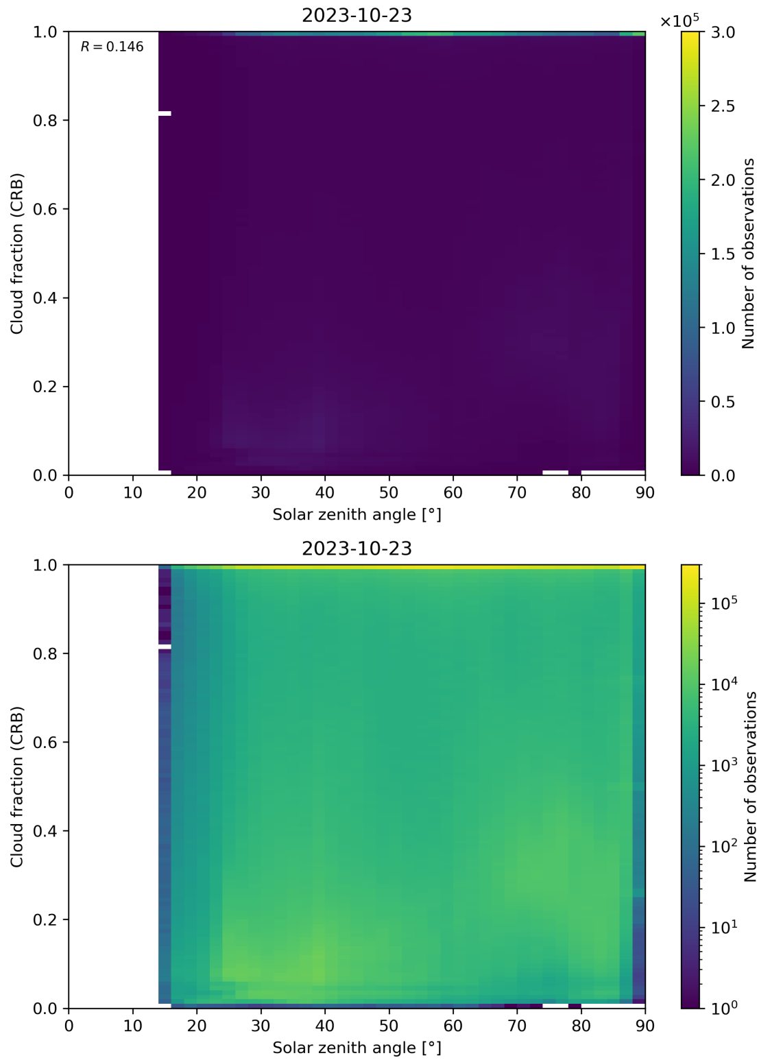
Figure 101: Scatter density plot of “Solar zenith angle” against “Cloud fraction (CRB)” for 2023-10-22 to 2023-10-24.
