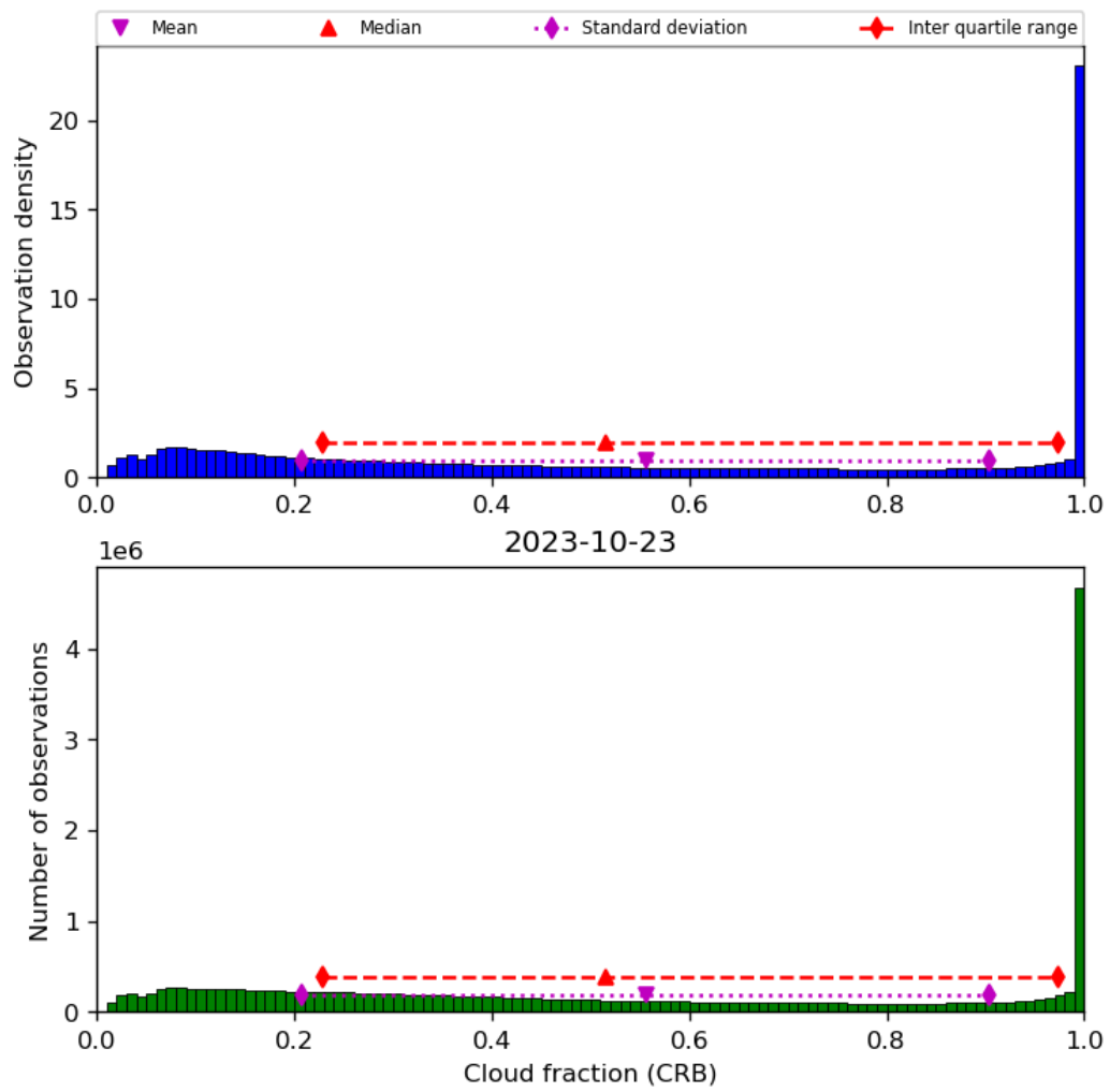
Figure 42: Histogram of “Cloud fraction (CRB)” for 2023-10-22 to 2023-10-24
