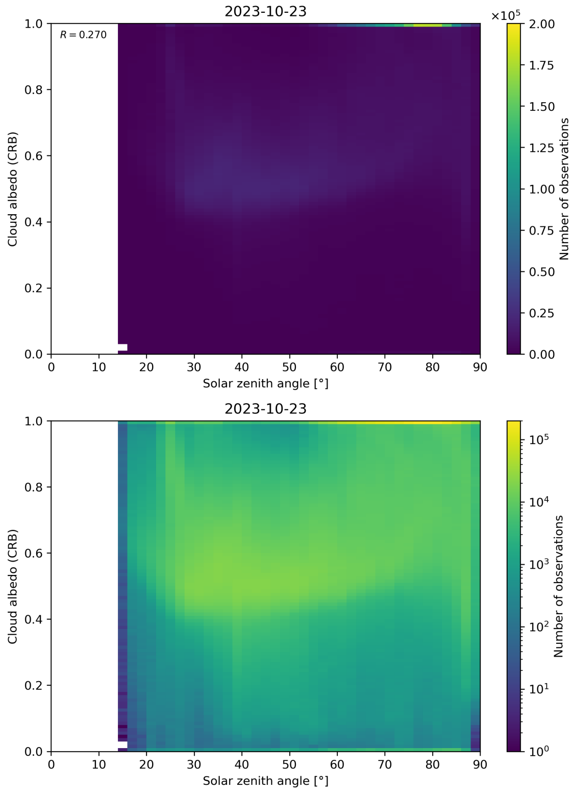
Figure 98: Scatter density plot of “Solar zenith angle” against “Cloud albedo (CRB)” for 2023-10-22 to 2023-10-24.
