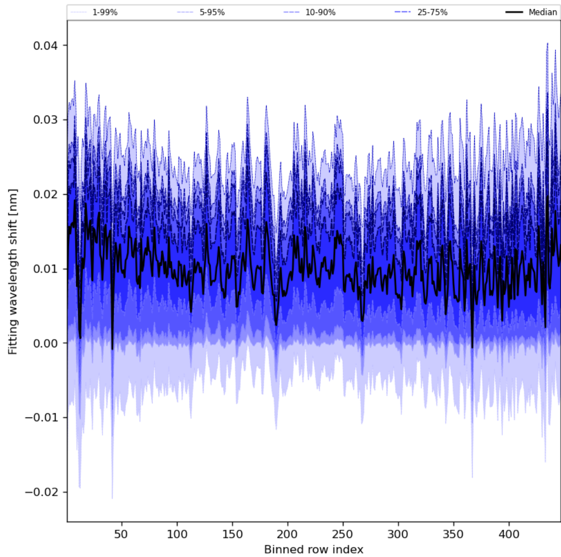
Figure 65: Along track statistics of “Fitting wavelength shift” for 2023-10-22 to 2023-10-24
