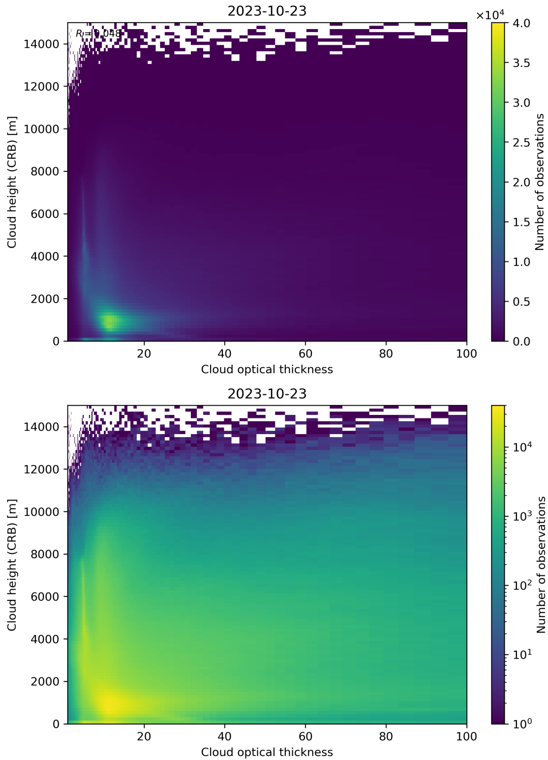
Figure 85: Scatter density plot of “Cloud optical thickness” against “Cloud height (CRB)” for 2023-10-22 to 2023-10-24.
