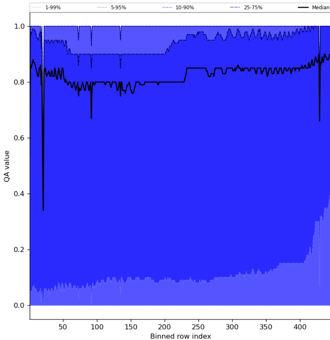
Figure 54: Along track statistics of “QA value” for 2023-10-22 to 2023-10-24
