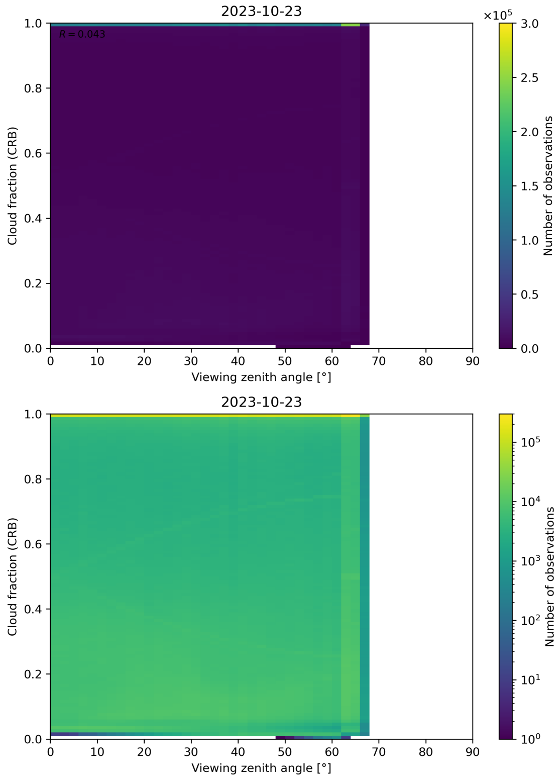
Figure 109: Scatter density plot of “Viewing zenith angle” against “Cloud fraction (CRB)” for 2023-10-22 to 2023-10-24.
