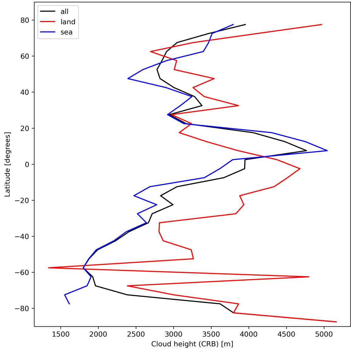
Figure 27: Zonal average of “Cloud height (CRB)” for 2023-10-22 to 2023-10-24.
