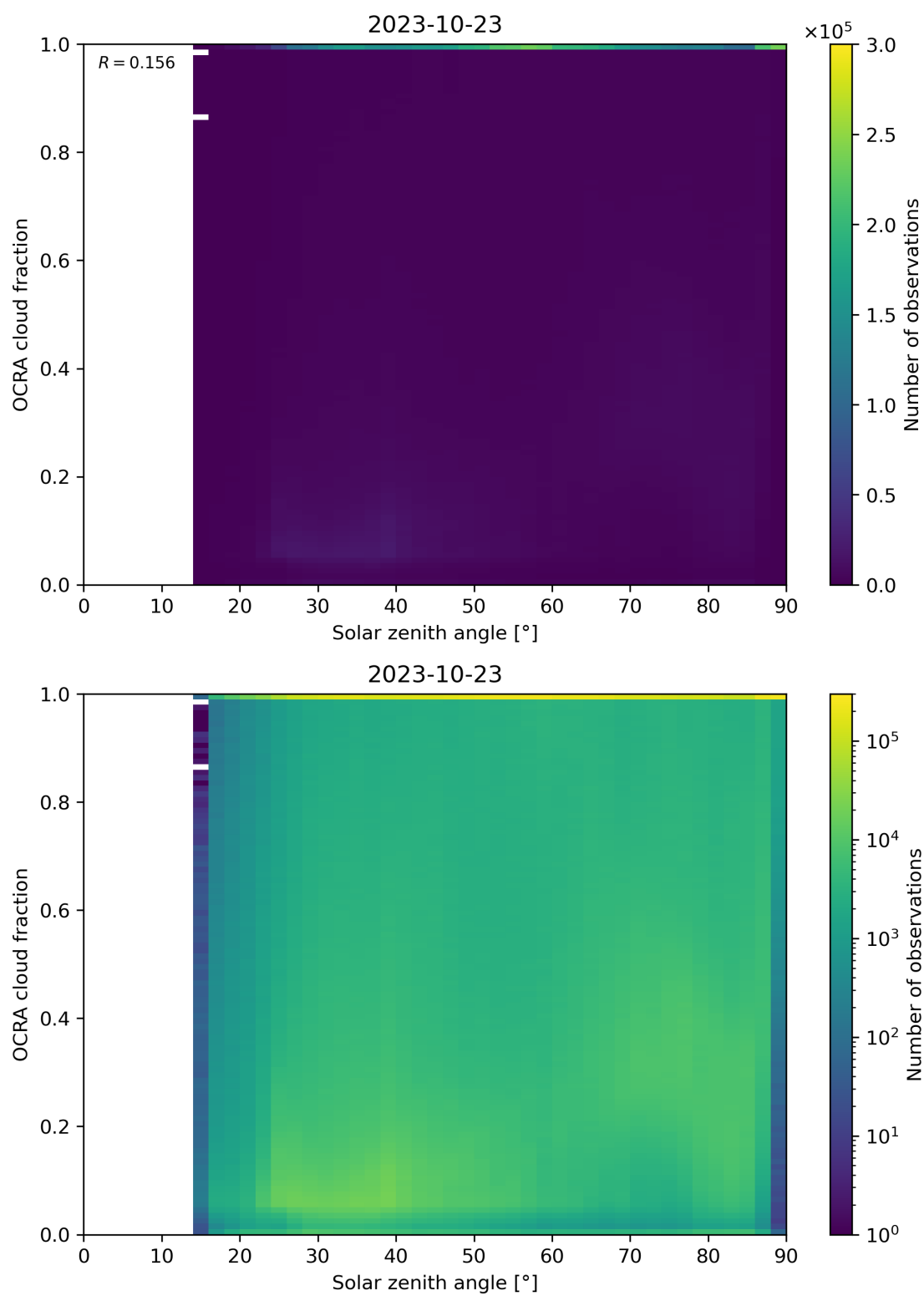
Figure 100: Scatter density plot of “Solar zenith angle” against “OCRA cloud fraction” for 2023-10-22 to 2023-10-24.
