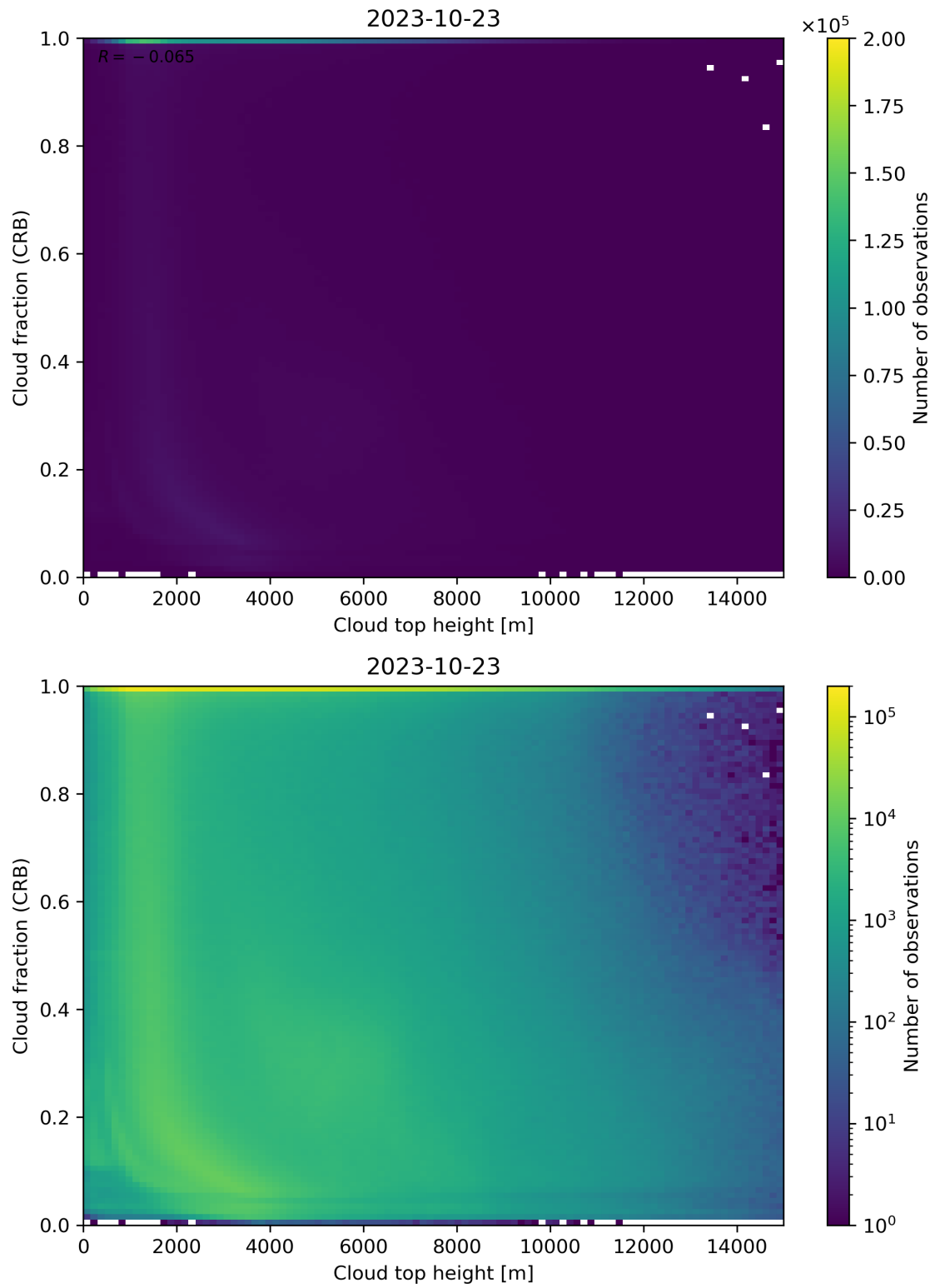
Figure 88: Scatter density plot of “Cloud top height” against “Cloud fraction (CRB)” for 2023-10-22 to 2023-10-24.
