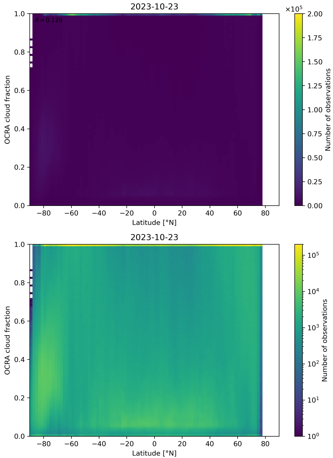
Figure 93: Scatter density plot of “Latitude” against “OCRA cloud fraction” for 2023-10-22 to 2023-10-24.
