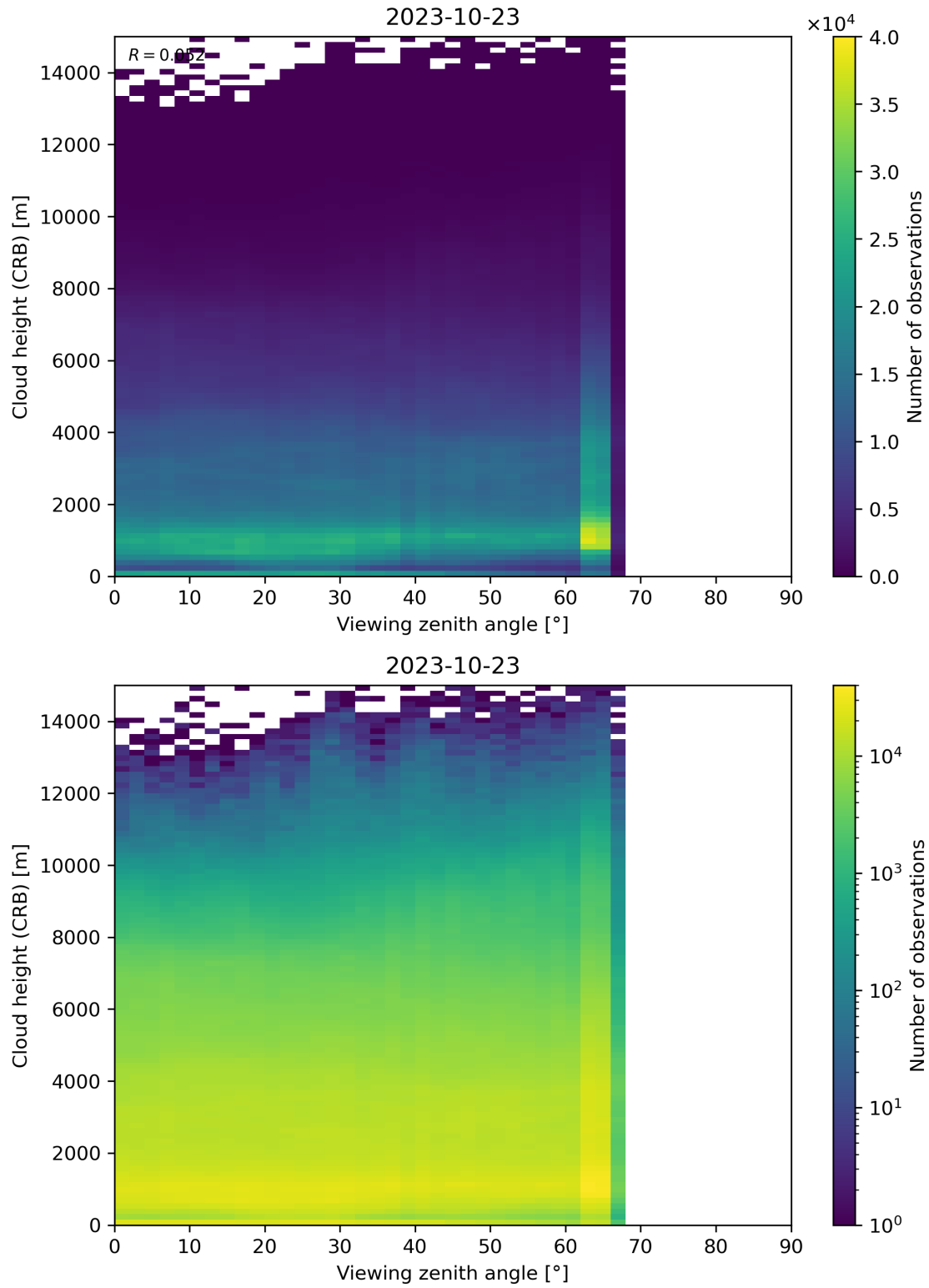
Figure 110: Scatter density plot of “Viewing zenith angle” against “Cloud height (CRB)” for 2023-10-22 to 2023-10-24.
