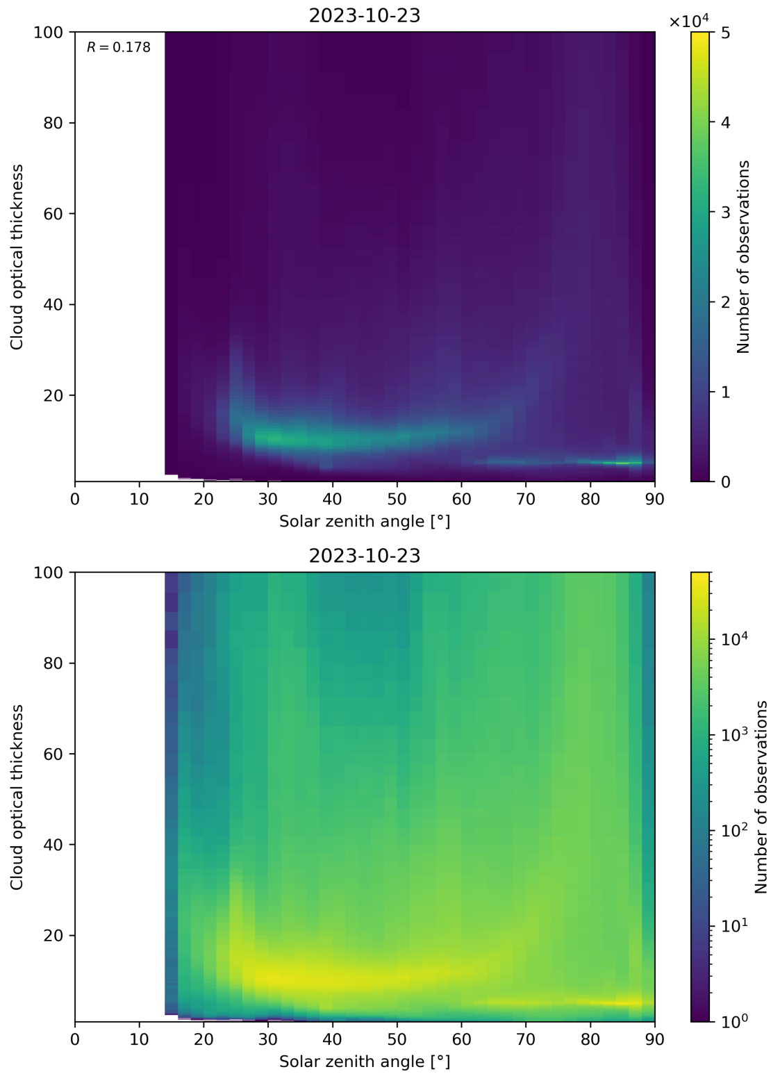
Figure 103: Scatter density plot of “Solar zenith angle” against “Cloud optical thickness” for 2023-10-22 to 2023-10-24.
