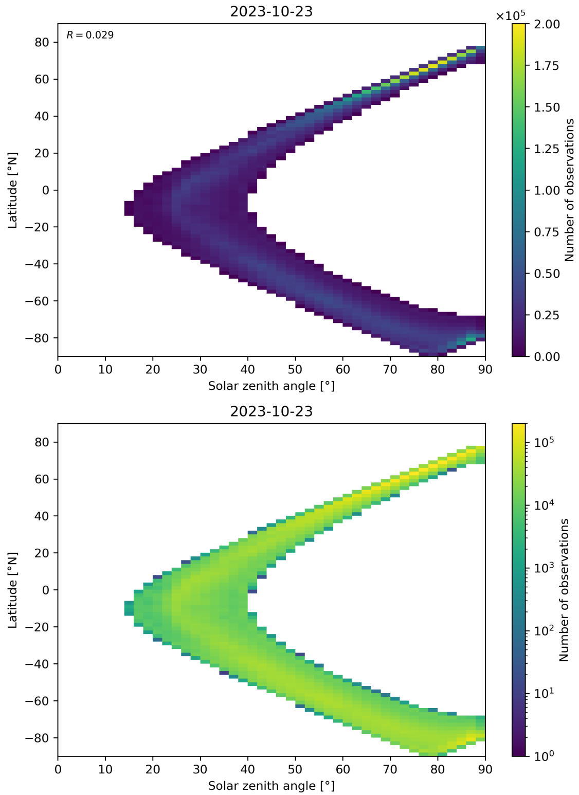
Figure 105: Scatter density plot of “Solar zenith angle” against “Latitude” for 2023-10-22 to 2023-10-24.
