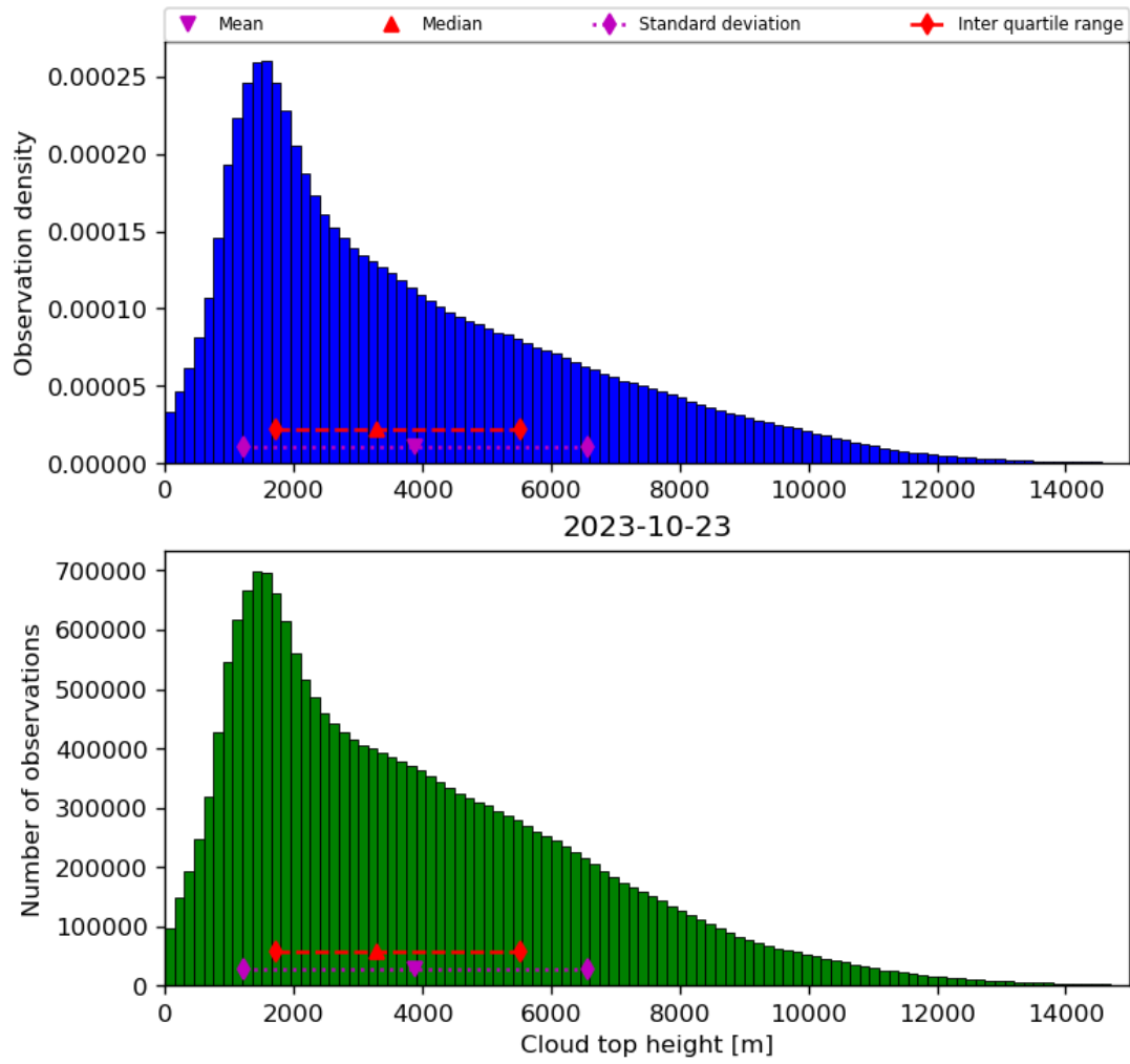
Figure 40: Histogram of “Cloud top height” for 2023-10-22 to 2023-10-24
