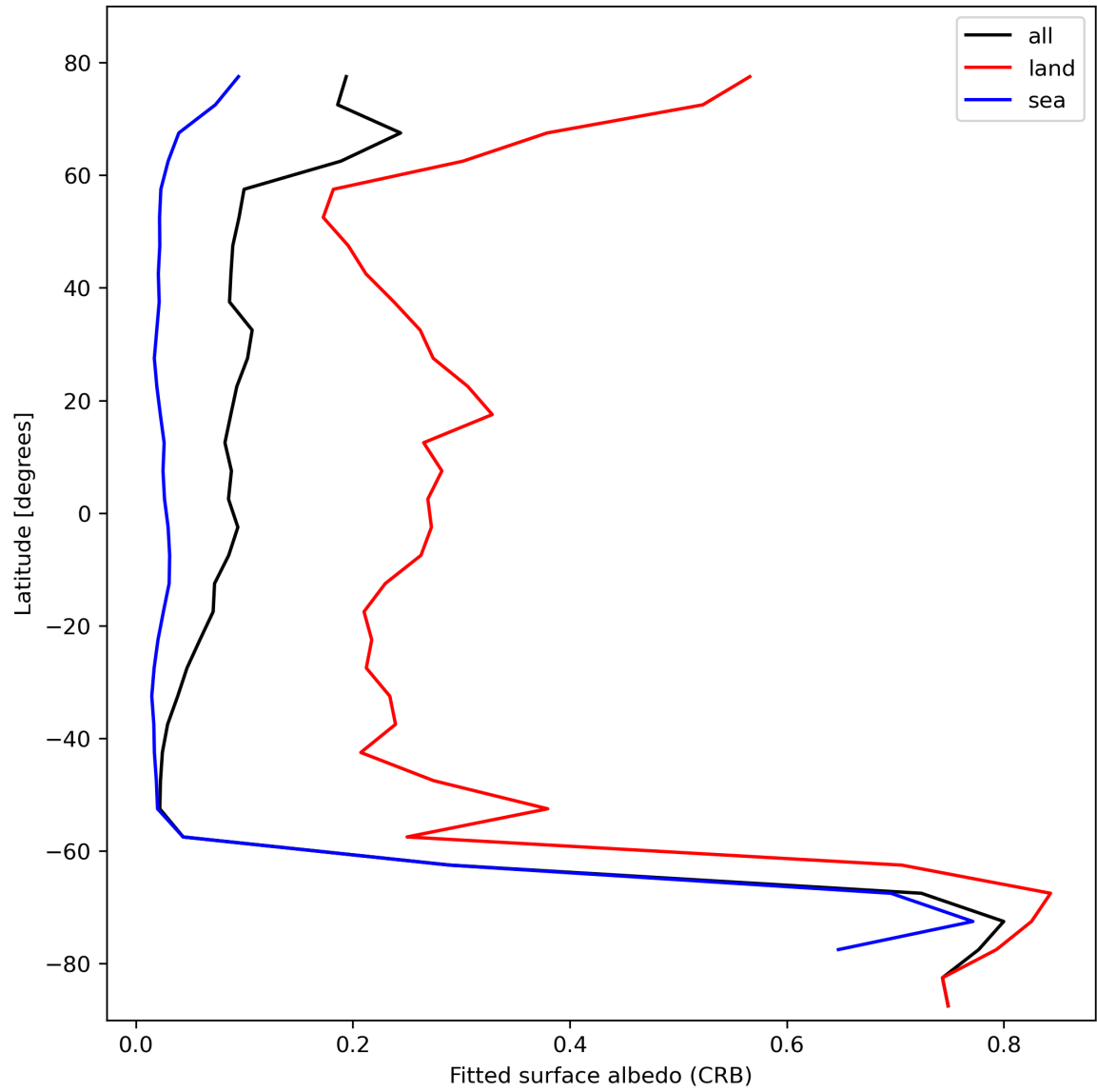
Figure 30: Zonal average of “Fitted surface albedo (CRB)” for 2023-10-22 to 2023-10-24.
