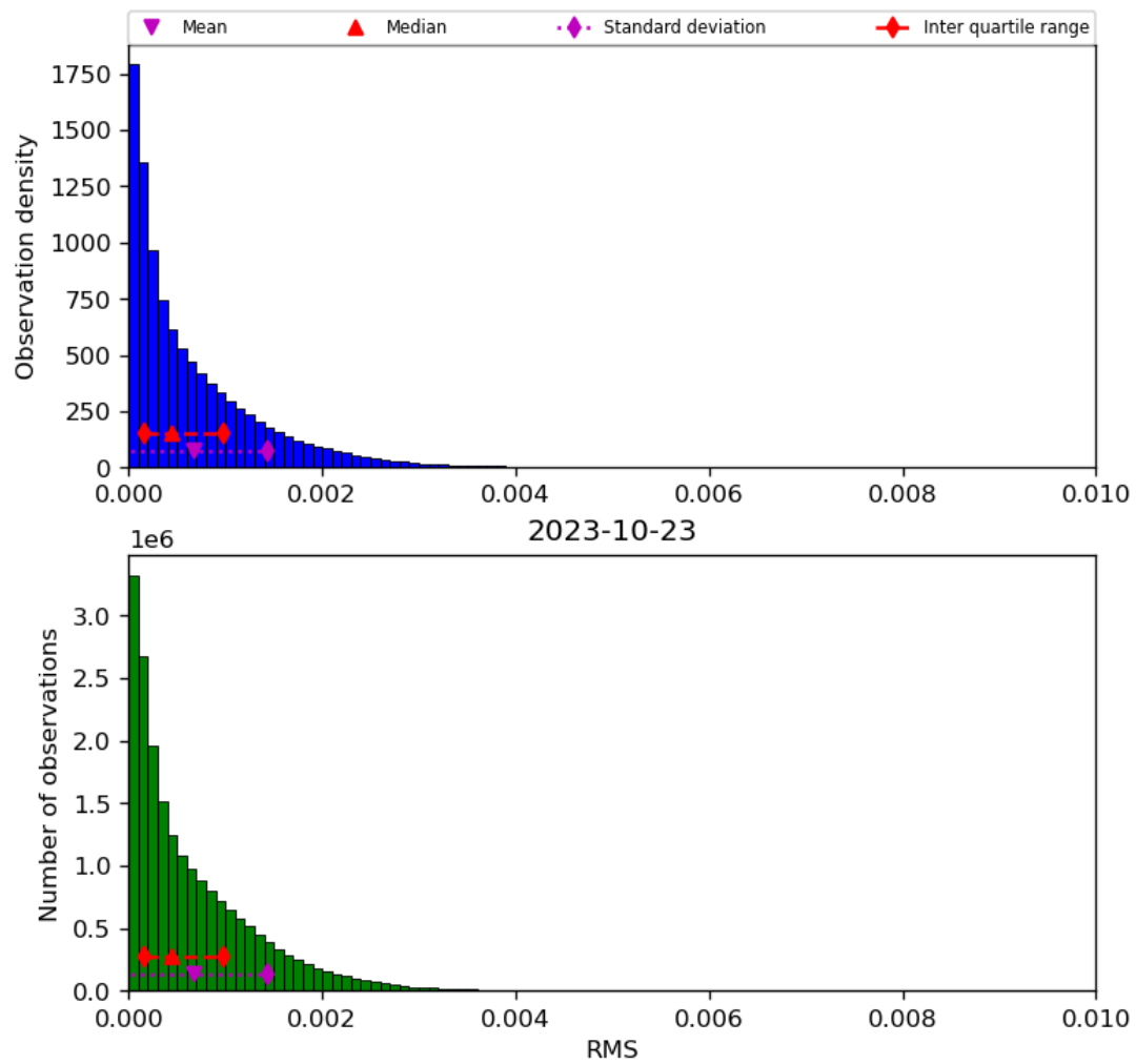
Figure 47: Histogram of “RMS” for 2023-10-22 to 2023-10-24
