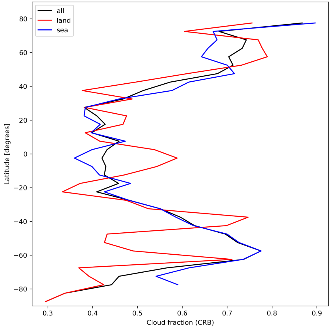
Figure 26: Zonal average of “Cloud fraction (CRB)” for 2023-10-22 to 2023-10-24.
