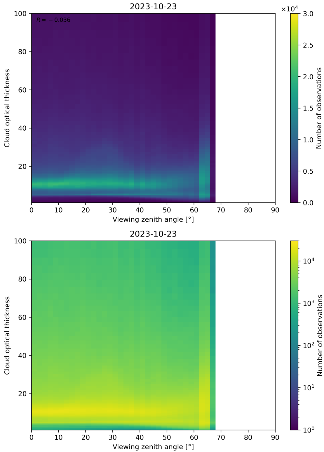
Figure 111: Scatter density plot of “Viewing zenith angle” against “Cloud optical thickness” for 2023-10-22 to 2023-10-24.
