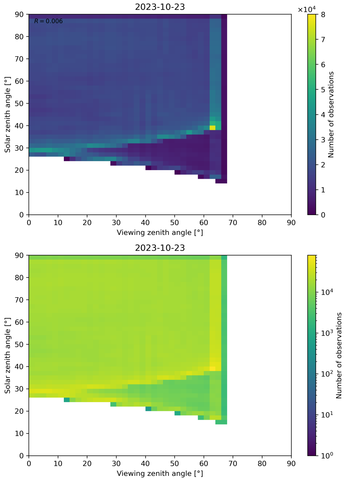
Figure 114: Scatter density plot of “Viewing zenith angle” against “Solar zenith angle” for 2023-10-22 to 2023-10-24.
