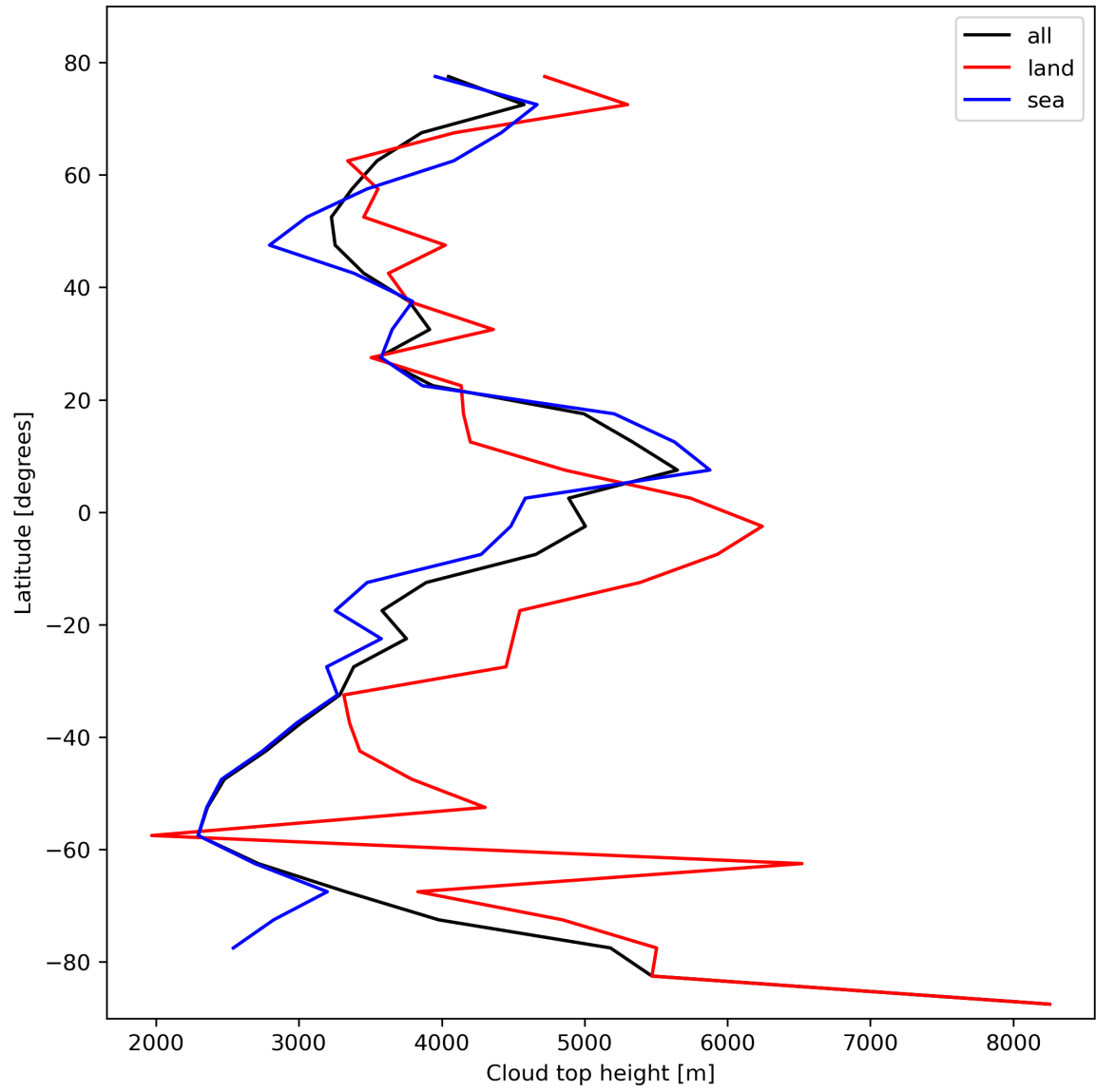
Figure 24: Zonal average of “Cloud top height” for 2023-10-22 to 2023-10-24.
