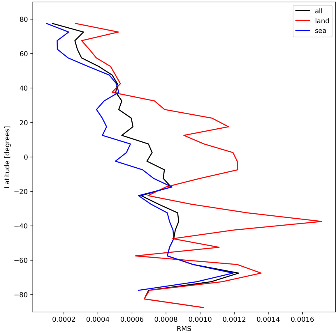
Figure 31: Zonal average of “RMS” for 2023-10-22 to 2023-10-24.
