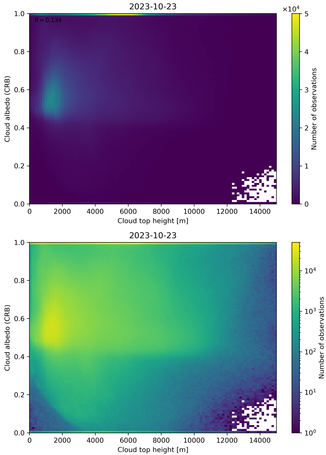
Figure 86: Scatter density plot of “Cloud top height” against “Cloud albedo (CRB)” for 2023-10-22 to 2023-10-24.
