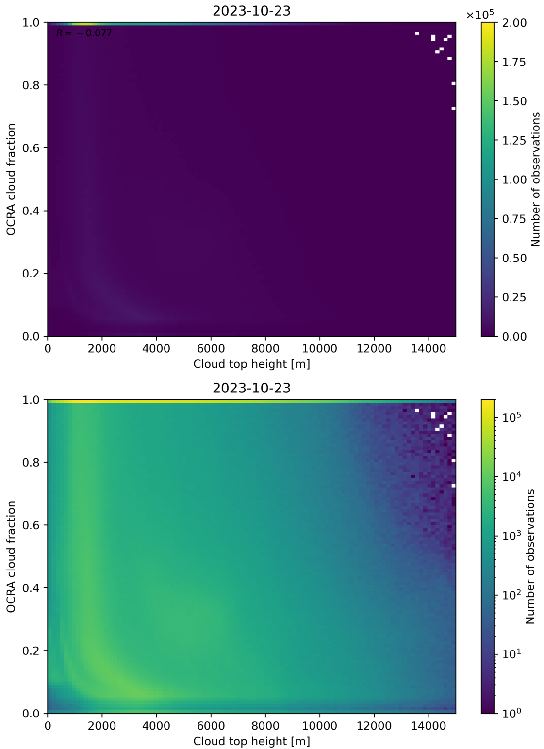
Figure 87: Scatter density plot of “Cloud top height” against “OCRA cloud fraction” for 2023-10-22 to 2023-10-24.
