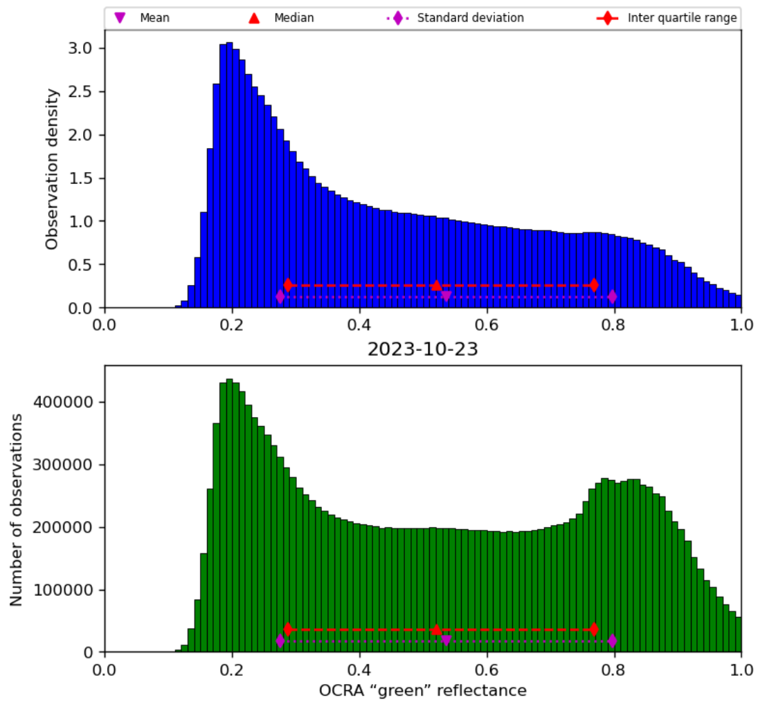
Figure 52: Histogram of “OCRA “green” reflectance” for 2023-10-22 to 2023-10-24
