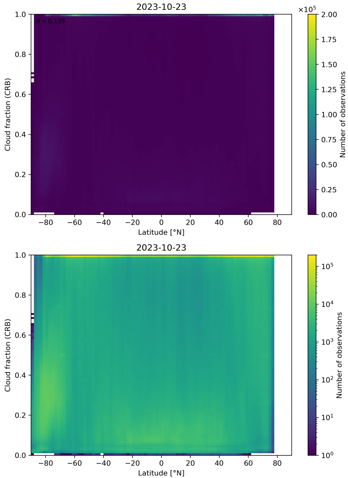
Figure 94: Scatter density plot of “Latitude” against “Cloud fraction (CRB)” for 2023-10-22 to 2023-10-24.
