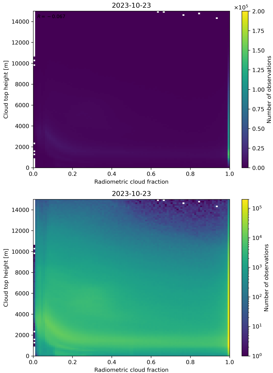
Figure 76: Scatter density plot of “Radiometric cloud fraction” against “Cloud top height” for 2023-10-22 to 2023-10-24.
