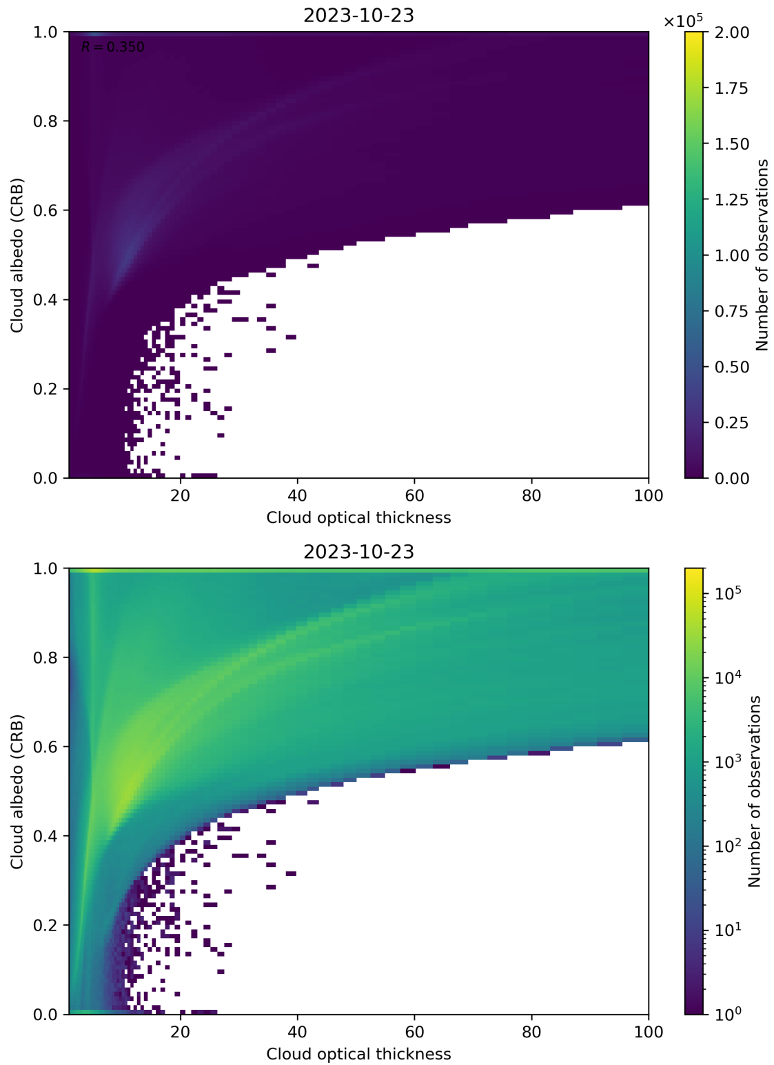
Figure 82: Scatter density plot of “Cloud optical thickness” against “Cloud albedo (CRB)” for 2023-10-22 to 2023-10-24.
