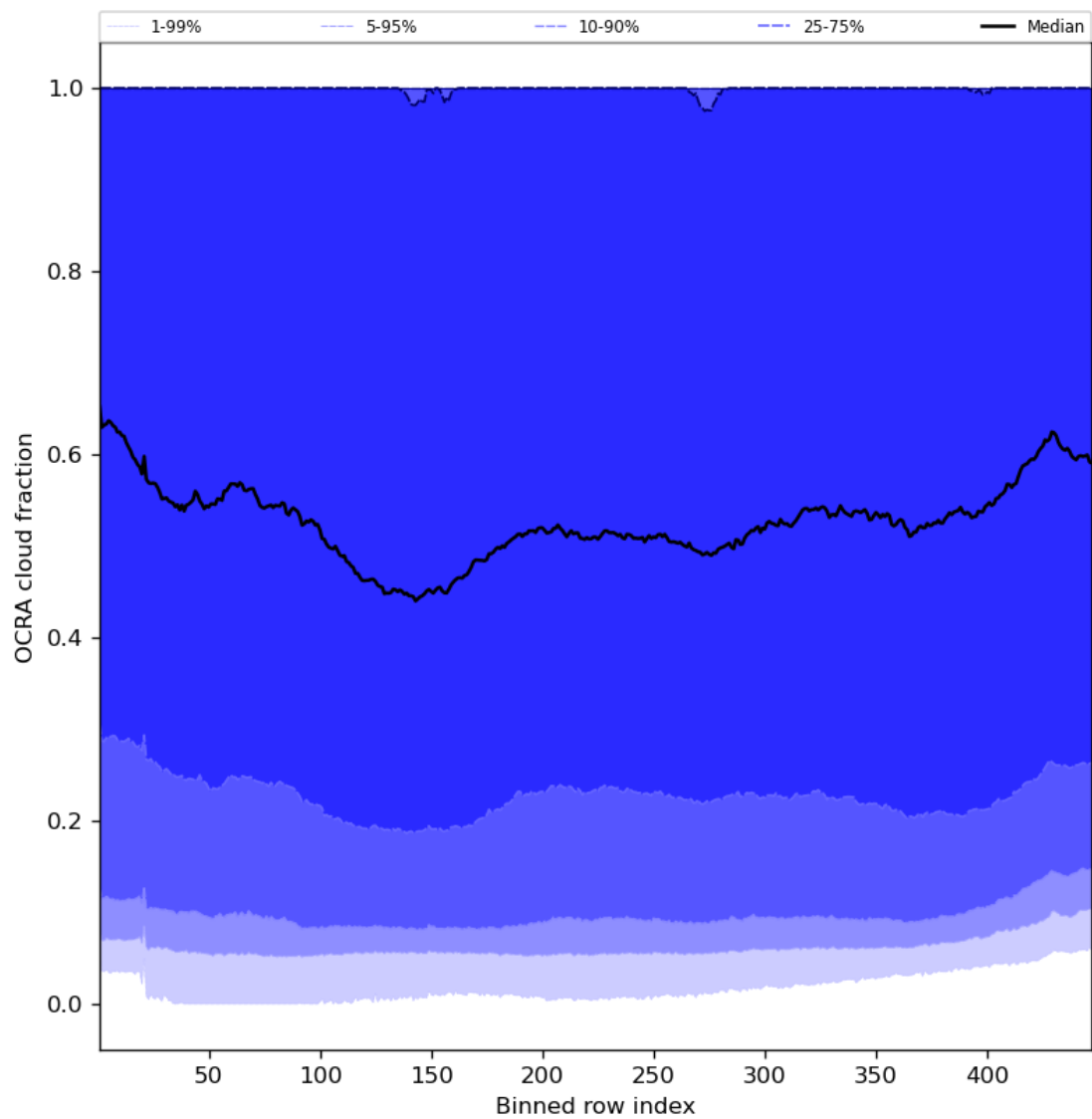
Figure 66: Along track statistics of “OCRA cloud fraction” for 2023-10-22 to 2023-10-24
