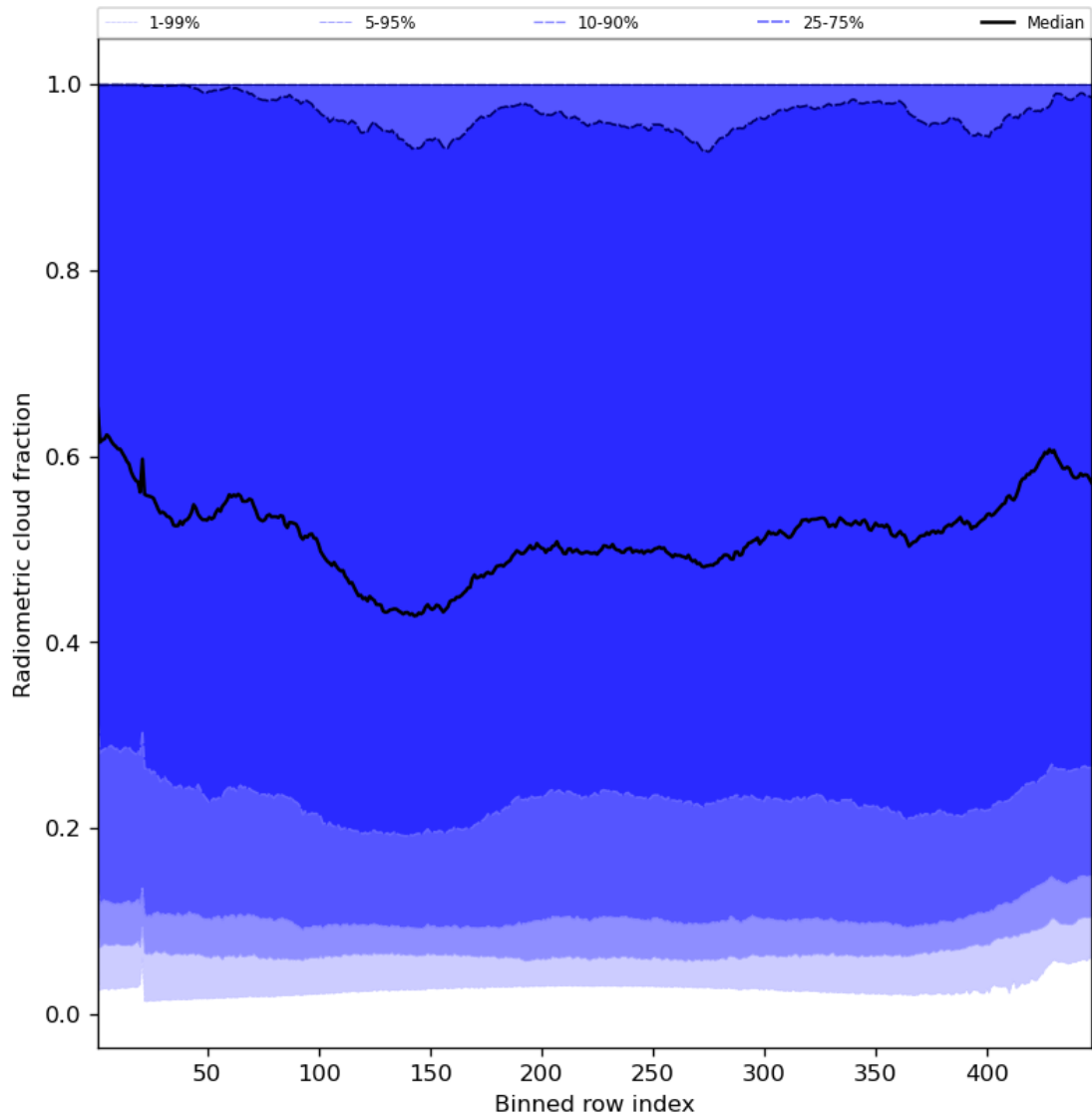
Figure 55: Along track statistics of “Radiometric cloud fraction” for 2023-10-22 to 2023-10-24
