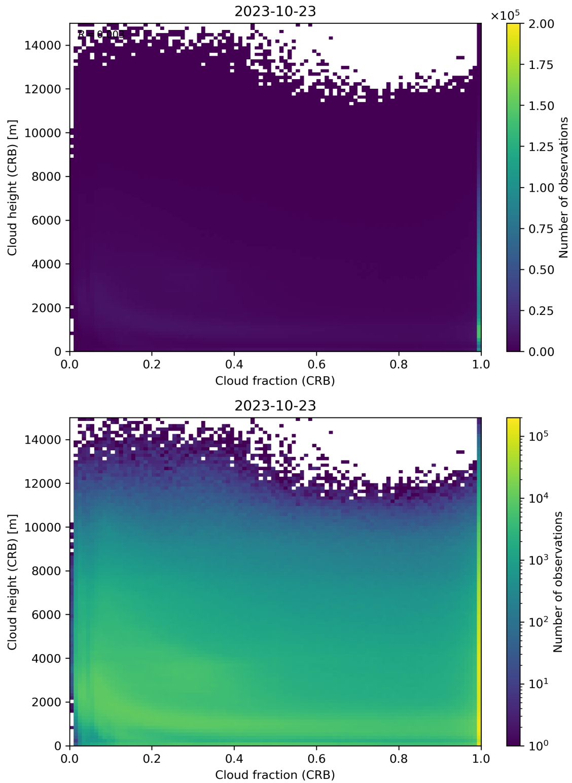
Figure 79: Scatter density plot of “Cloud fraction (CRB)” against “Cloud height (CRB)” for 2023-10-22 to 2023-10-24.
