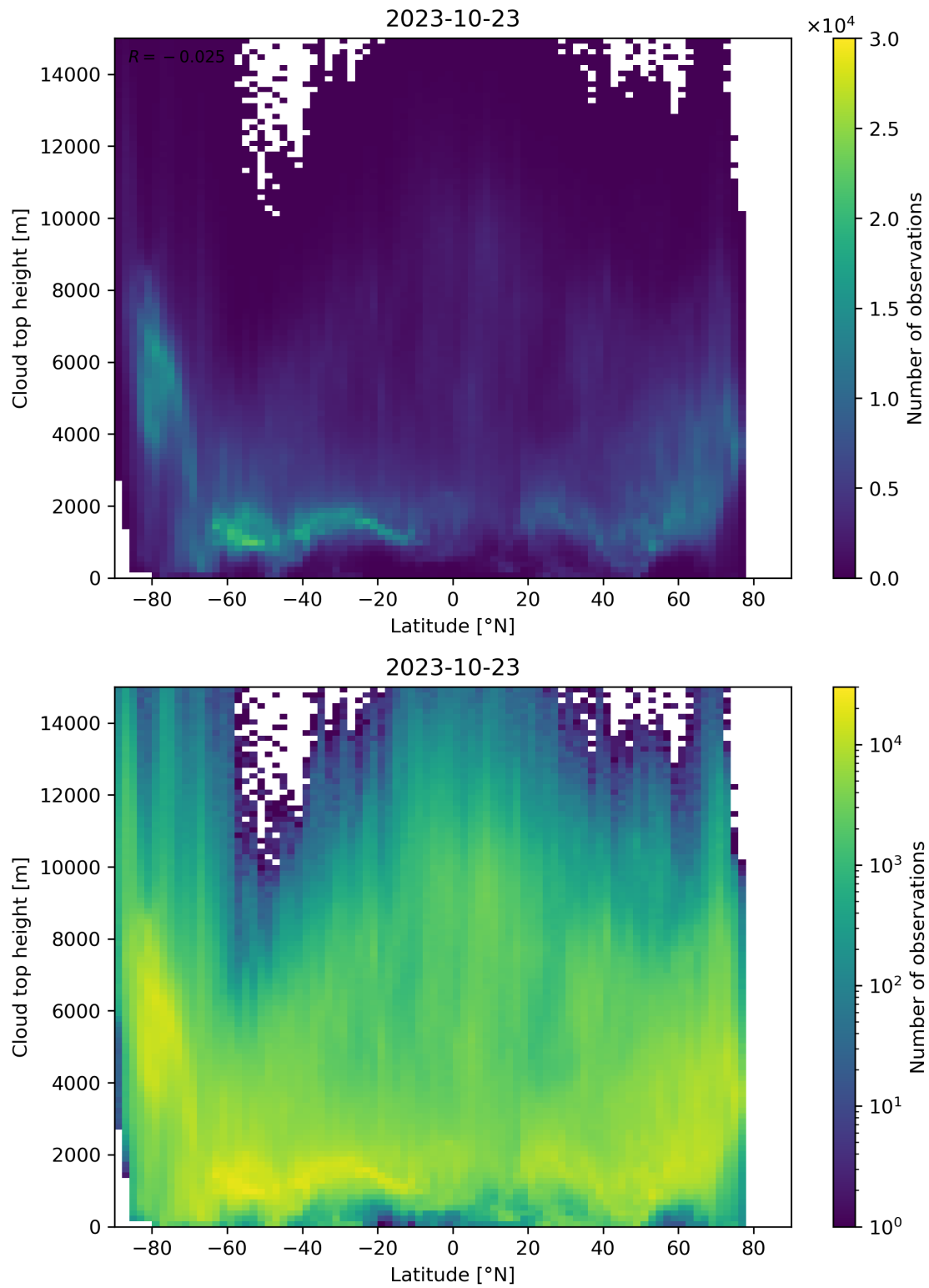
Figure 97: Scatter density plot of “Latitude” against “Cloud top height” for 2023-10-22 to 2023-10-24.
