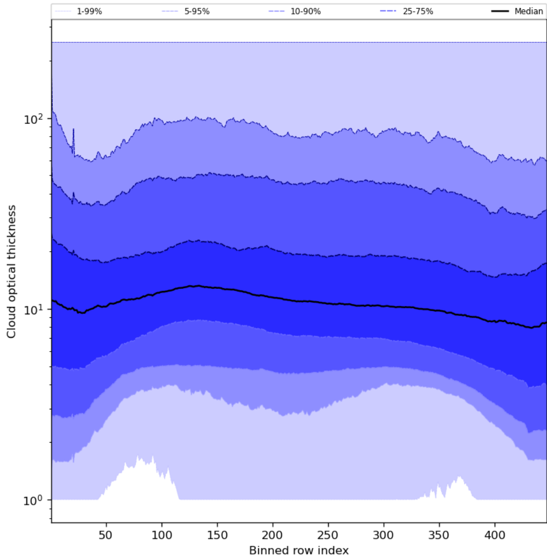
Figure 57: Along track statistics of “Cloud optical thickness” for 2023-10-22 to 2023-10-24
