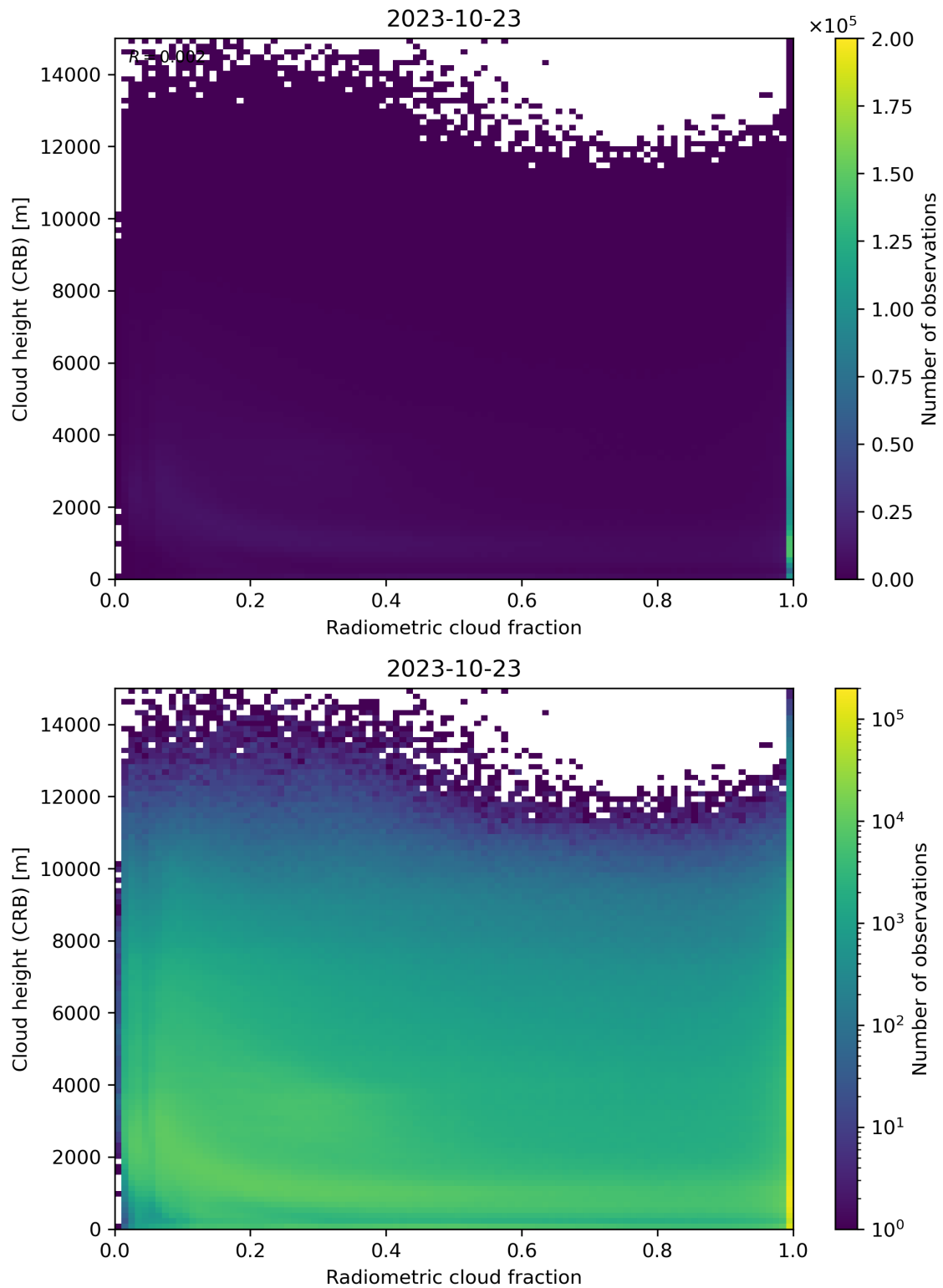
Figure 74: Scatter density plot of “Radiometric cloud fraction” against “Cloud height (CRB)” for 2023-10-22 to 2023-10-24.
