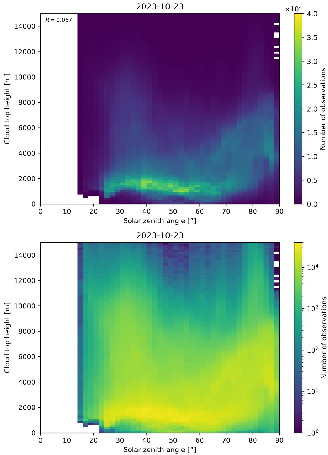
Figure 104: Scatter density plot of “Solar zenith angle” against “Cloud top height” for 2023-10-22 to 2023-10-24.
