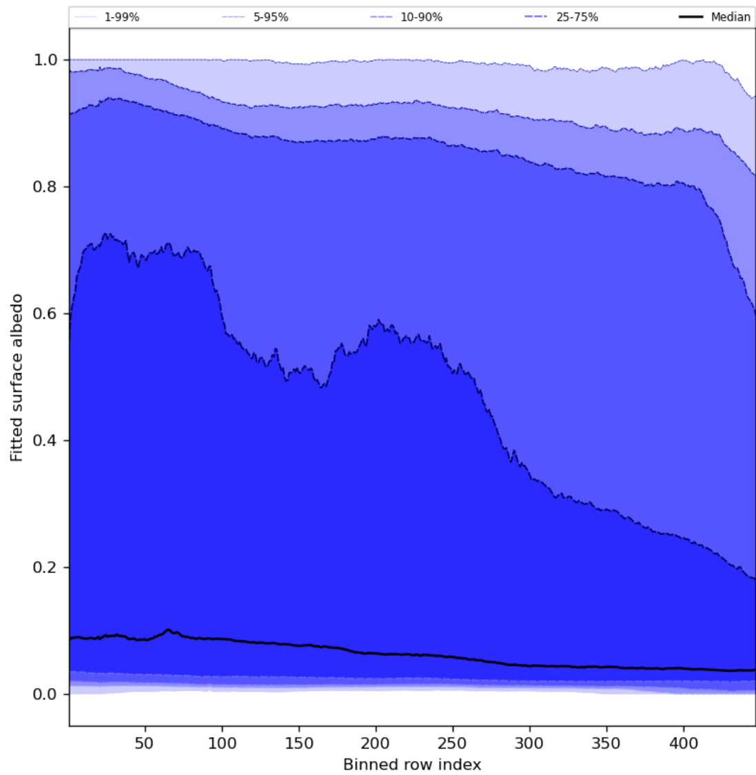
Figure 61: Along track statistics of “Fitted surface albedo” for 2023-10-25 to 2023-10-27
