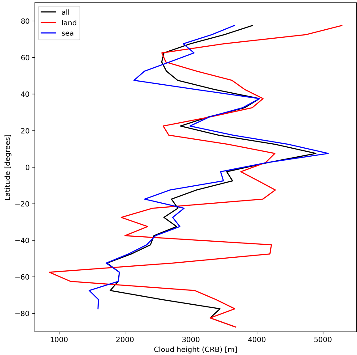
Figure 27: Zonal average of “Cloud height (CRB)” for 2023-10-25 to 2023-10-27.
