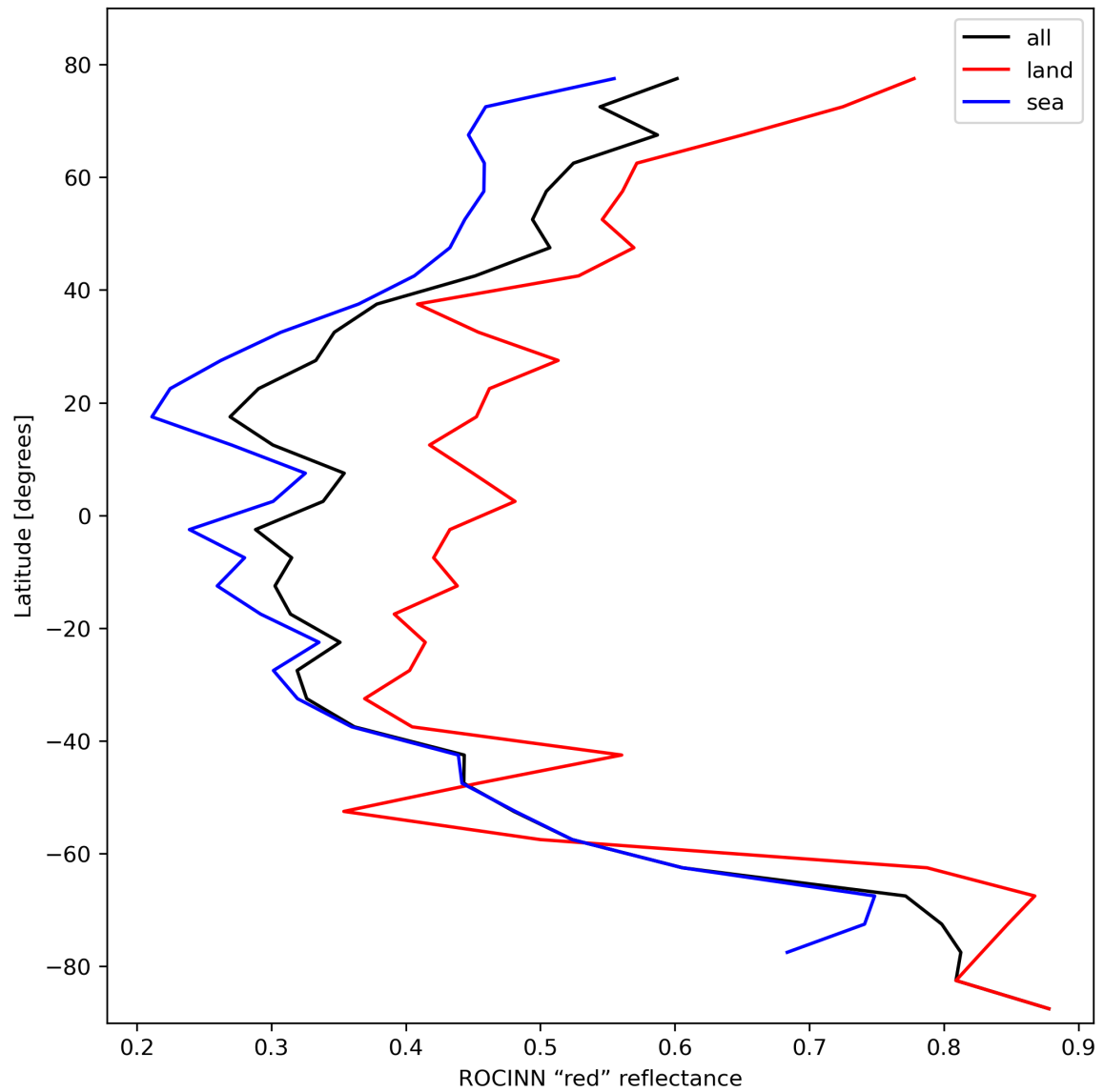
Figure 37: Zonal average of “ROCINN “red” reflectance” for 2023-10-25 to 2023-10-27.
