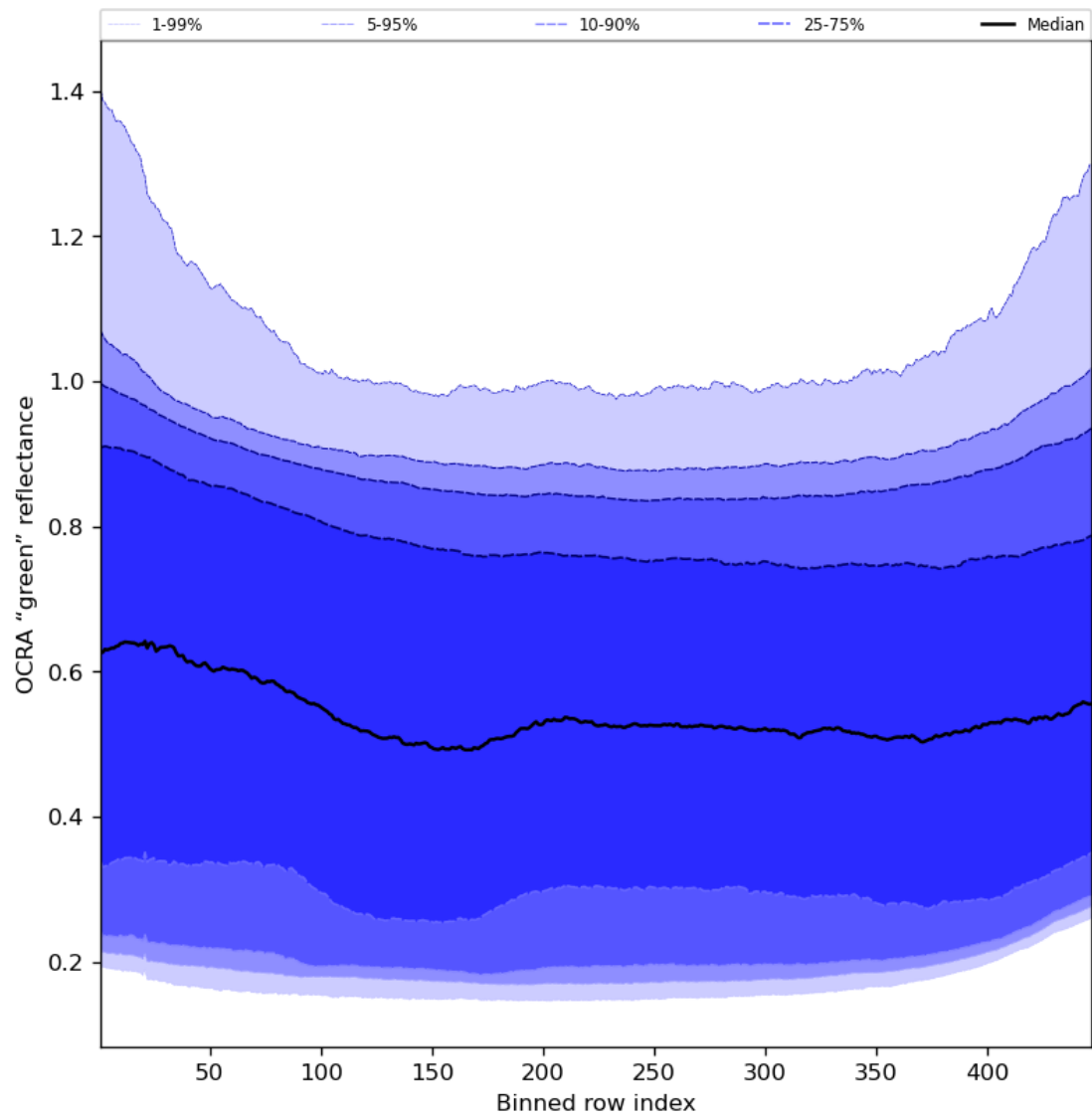
Figure 68: Along track statistics of "OCRA "green" reflectance" for 2023-10-25 to 2023-10-27
