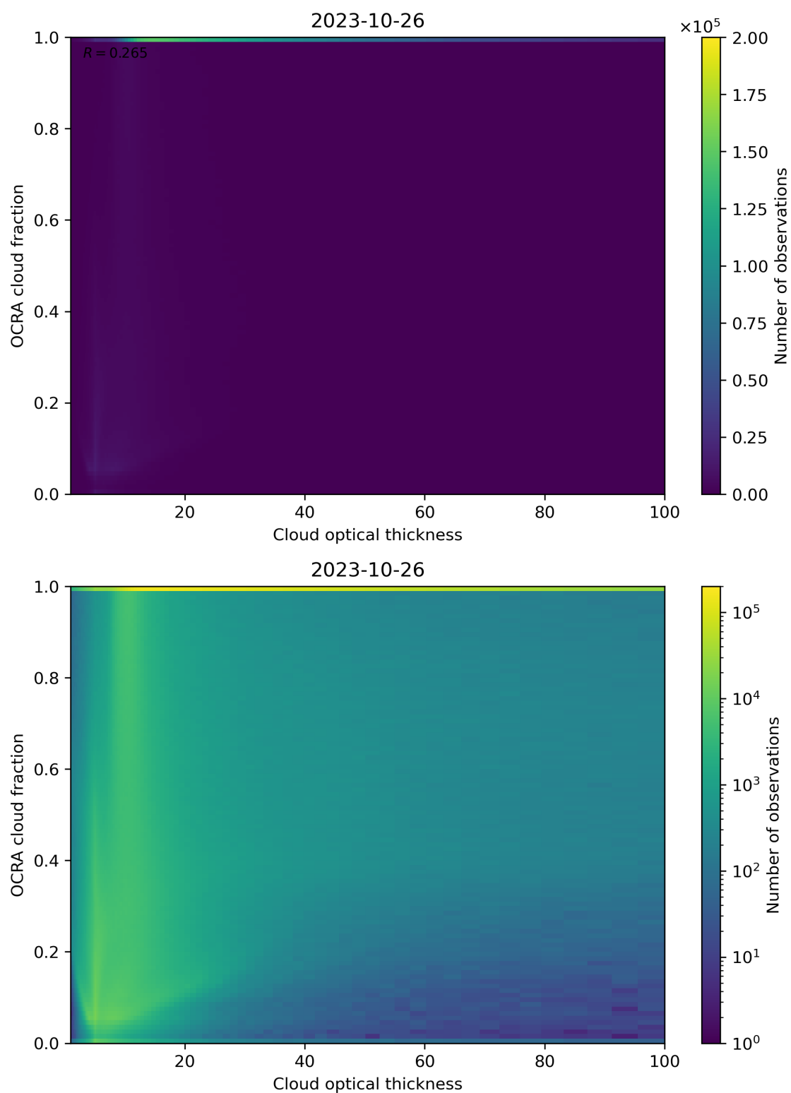
Figure 83: Scatter density plot of “Cloud optical thickness” against “OCRA cloud fraction” for 2023-10-25 to 2023-10-27.
