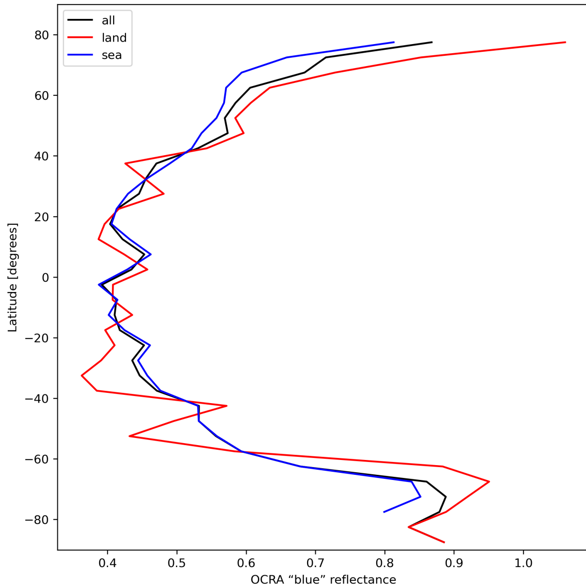
Figure 35: Zonal average of “OCRA “blue” reflectance” for 2023-10-25 to 2023-10-27.
