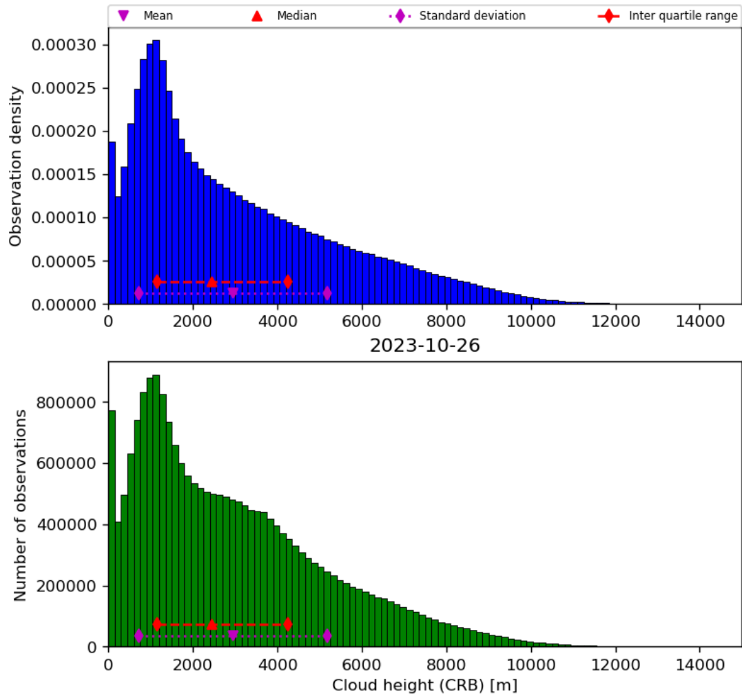
Figure 43: Histogram of “Cloud height (CRB)” for 2023-10-25 to 2023-10-27
