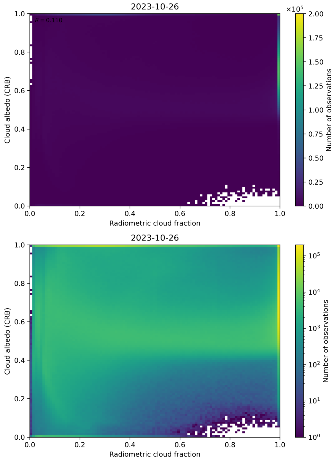
Figure 71: Scatter density plot of “Radiometric cloud fraction” against “Cloud albedo (CRB)” for 2023-10-25 to 2023-10-27.
