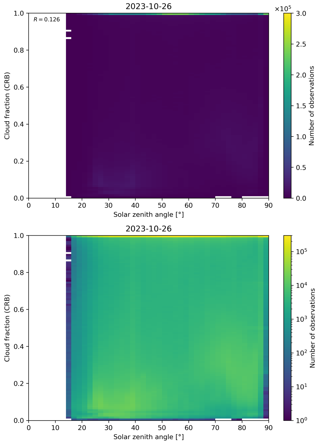
Figure 101: Scatter density plot of “Solar zenith angle” against “Cloud fraction (CRB)” for 2023-10-25 to 2023-10-27.
