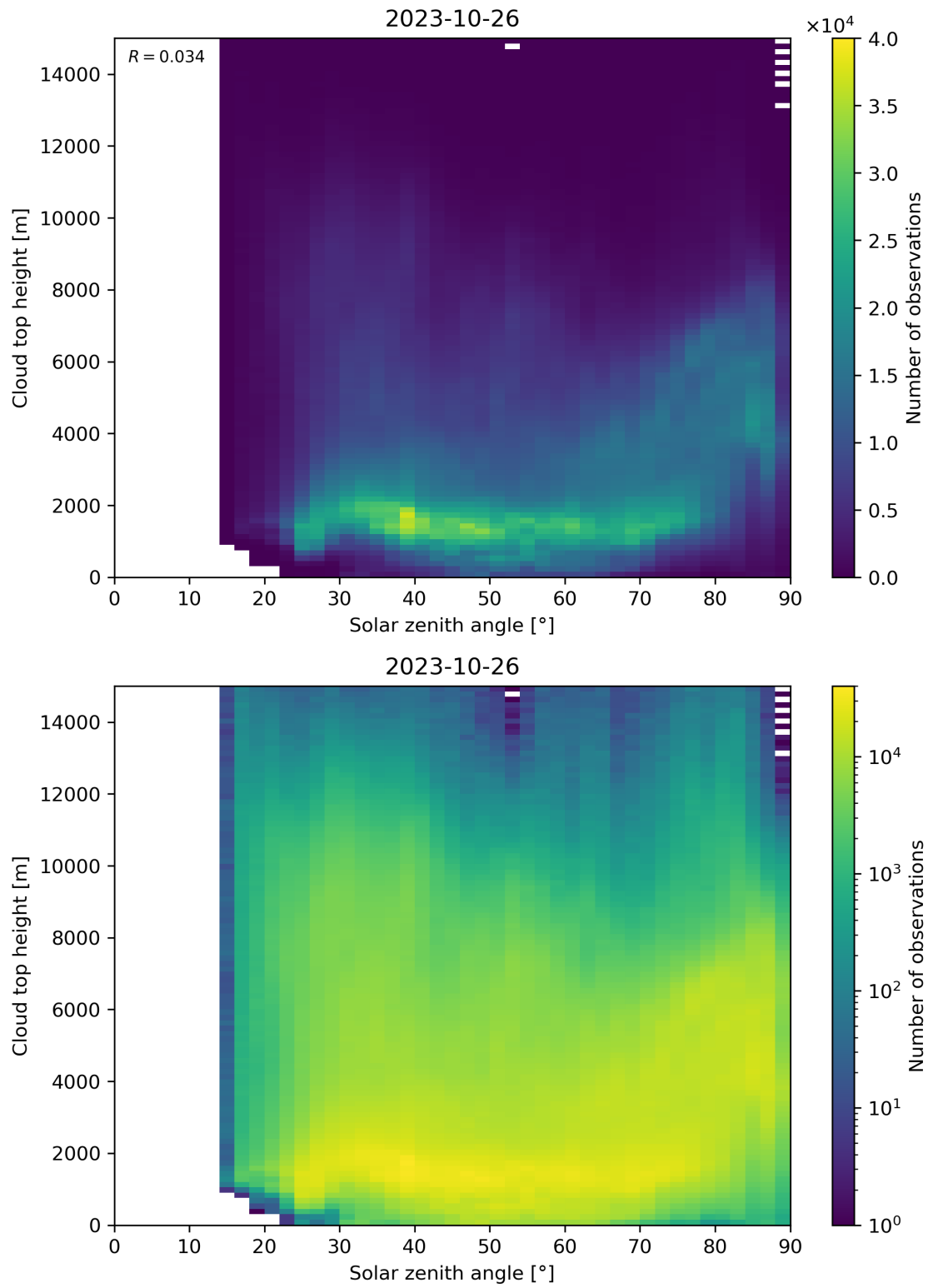
Figure 104: Scatter density plot of “Solar zenith angle” against “Cloud top height” for 2023-10-25 to 2023-10-27.
