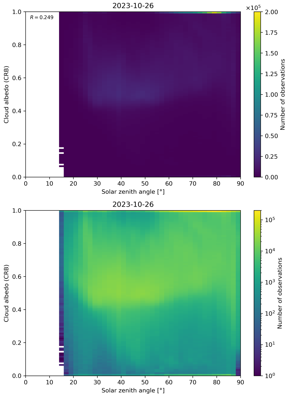
Figure 98: Scatter density plot of “Solar zenith angle” against “Cloud albedo (CRB)” for 2023-10-25 to 2023-10-27.
