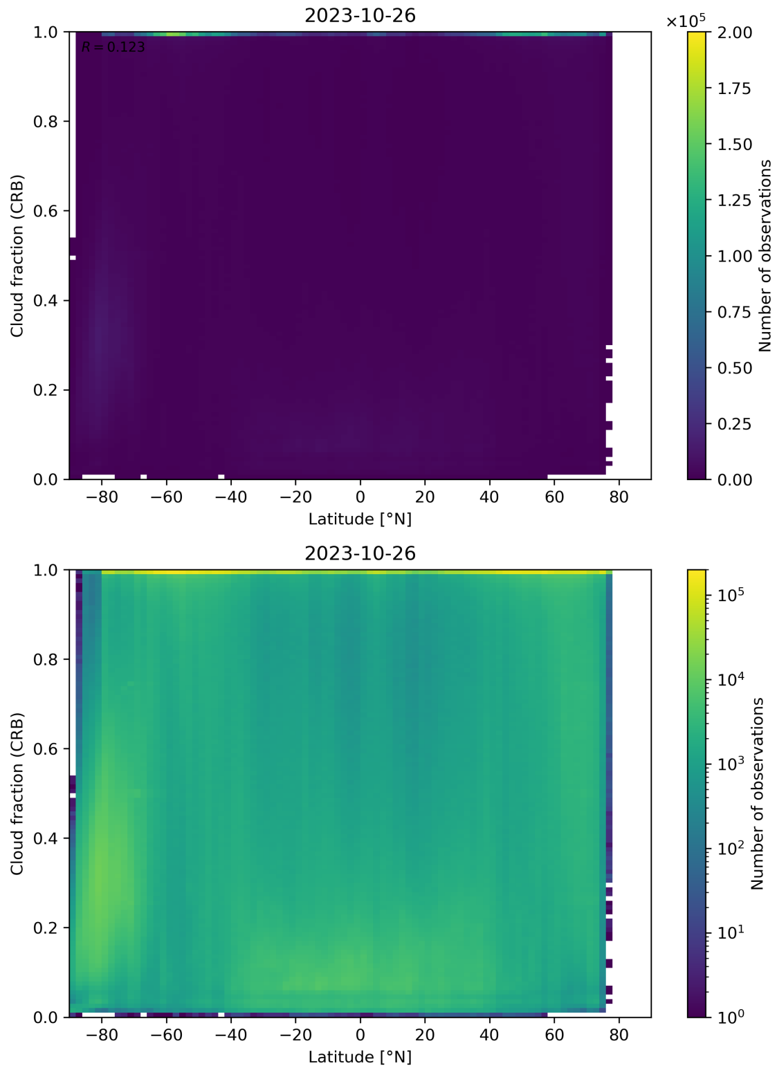
Figure 94: Scatter density plot of “Latitude” against “Cloud fraction (CRB)” for 2023-10-25 to 2023-10-27.
