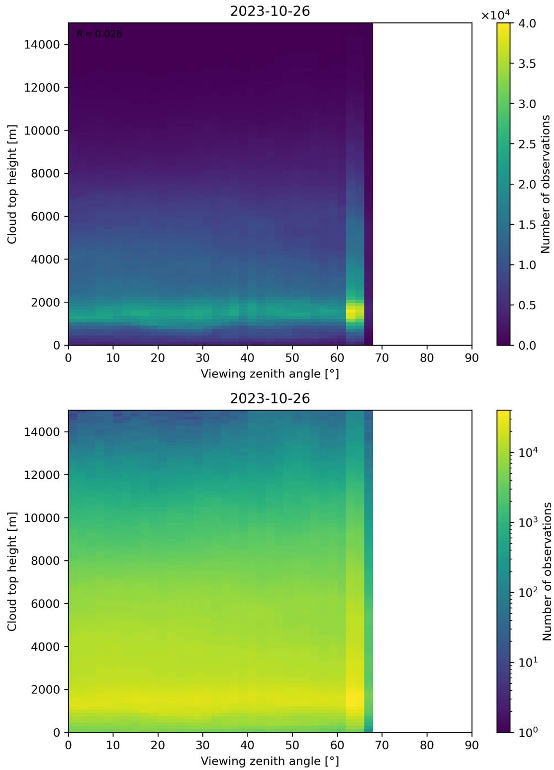
Figure 112: Scatter density plot of “Viewing zenith angle” against “Cloud top height” for 2023-10-25 to 2023-10-27.
