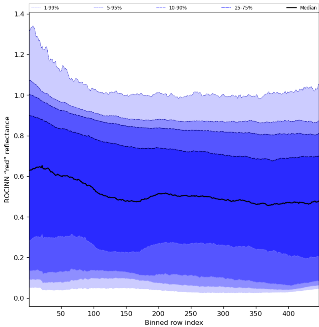
Figure 69: Along track statistics of “ROCINN “red” reflectance” for 2023-10-25 to 2023-10-27
