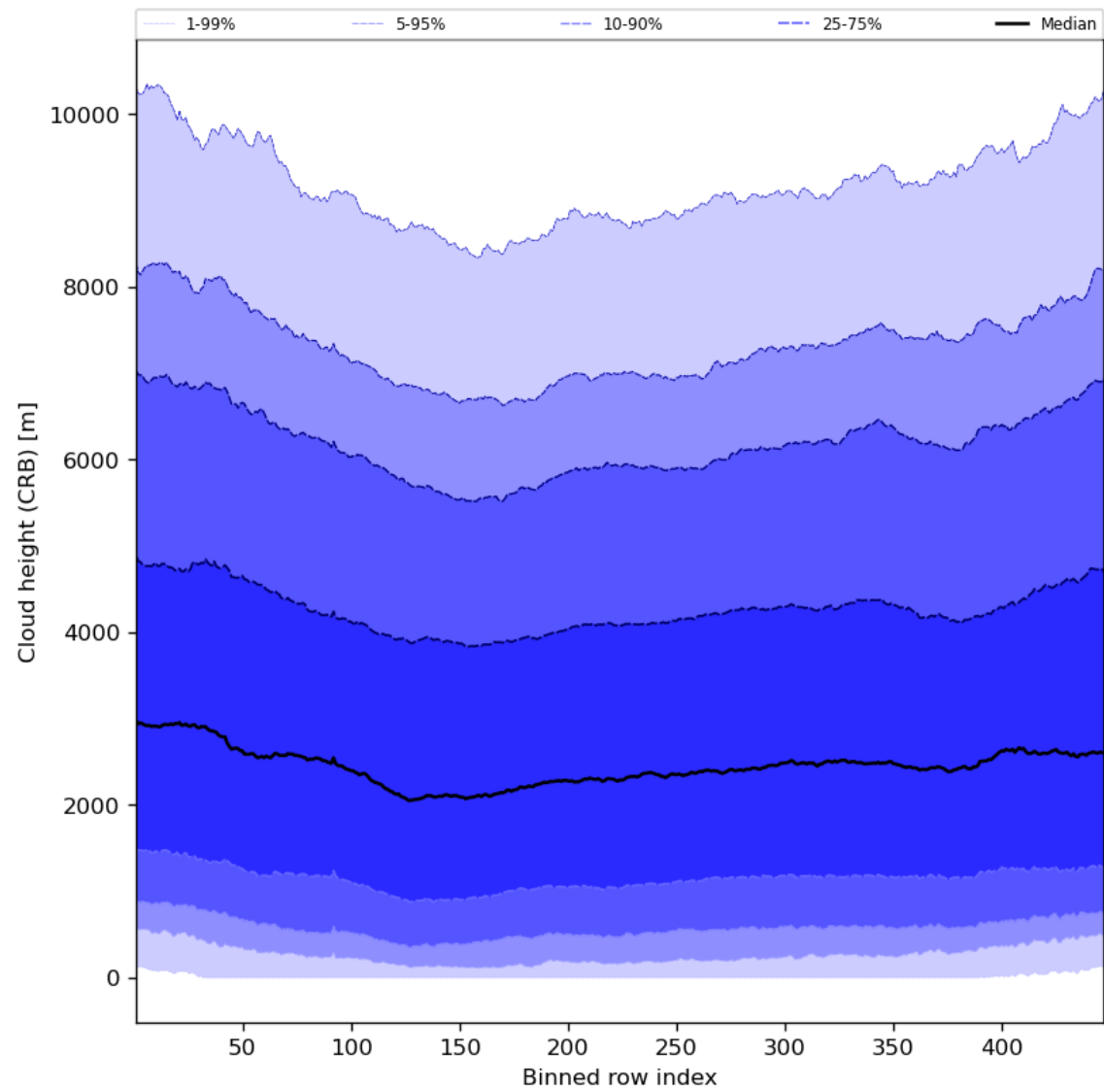
Figure 59: Along track statistics of “Cloud height (CRB)” for 2023-10-25 to 2023-10-27
