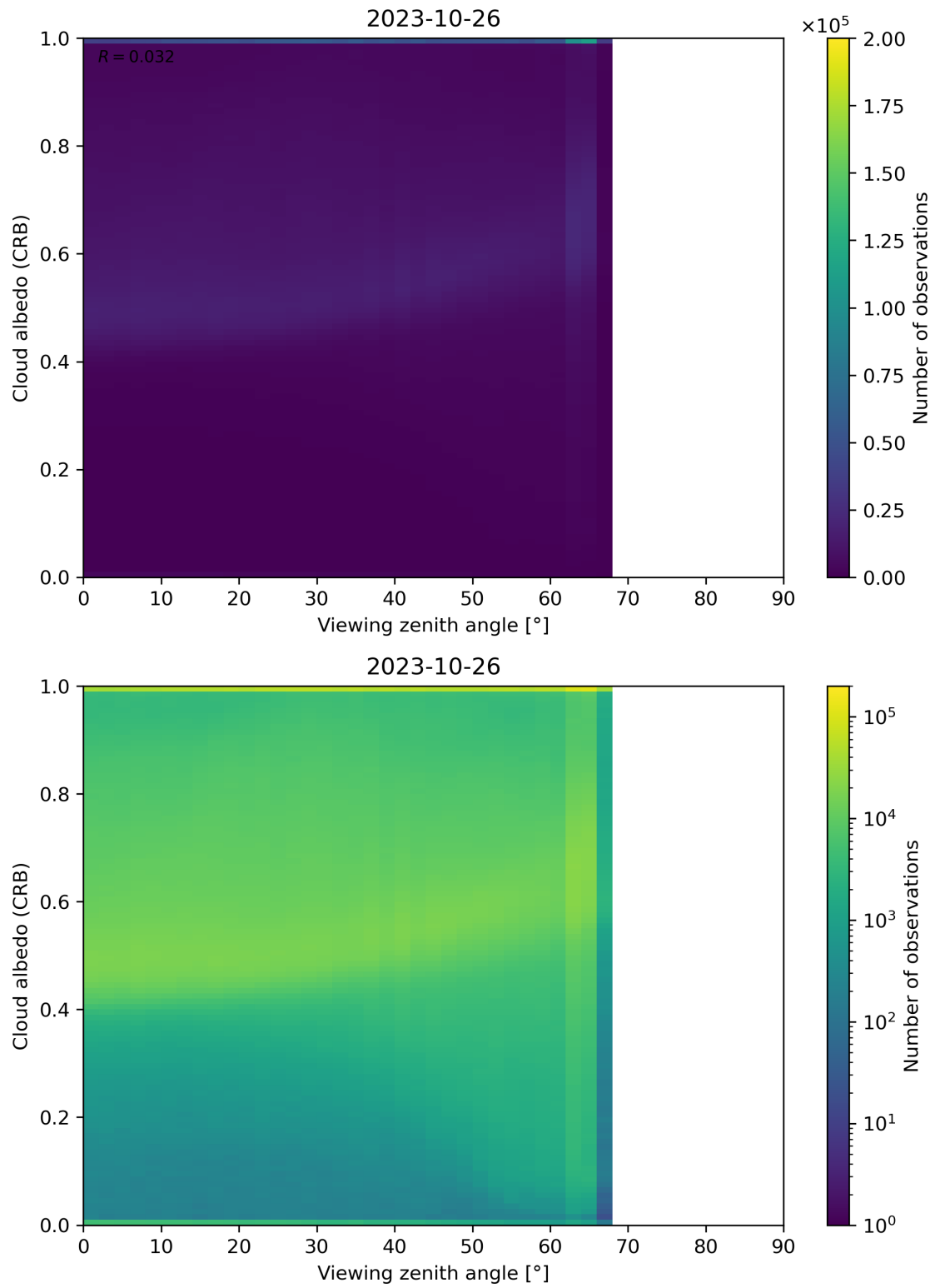
Figure 106: Scatter density plot of “Viewing zenith angle” against “Cloud albedo (CRB)” for 2023-10-25 to 2023-10-27.
