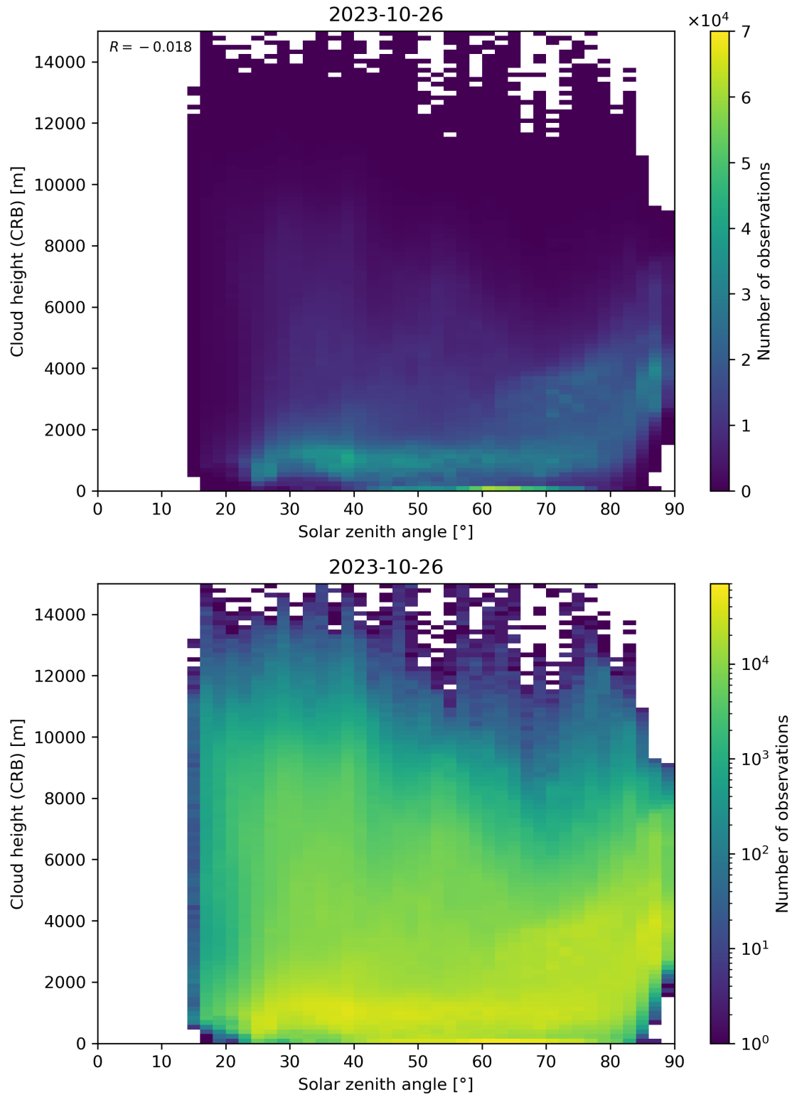
Figure 102: Scatter density plot of “Solar zenith angle” against “Cloud height (CRB)” for 2023-10-25 to 2023-10-27.
