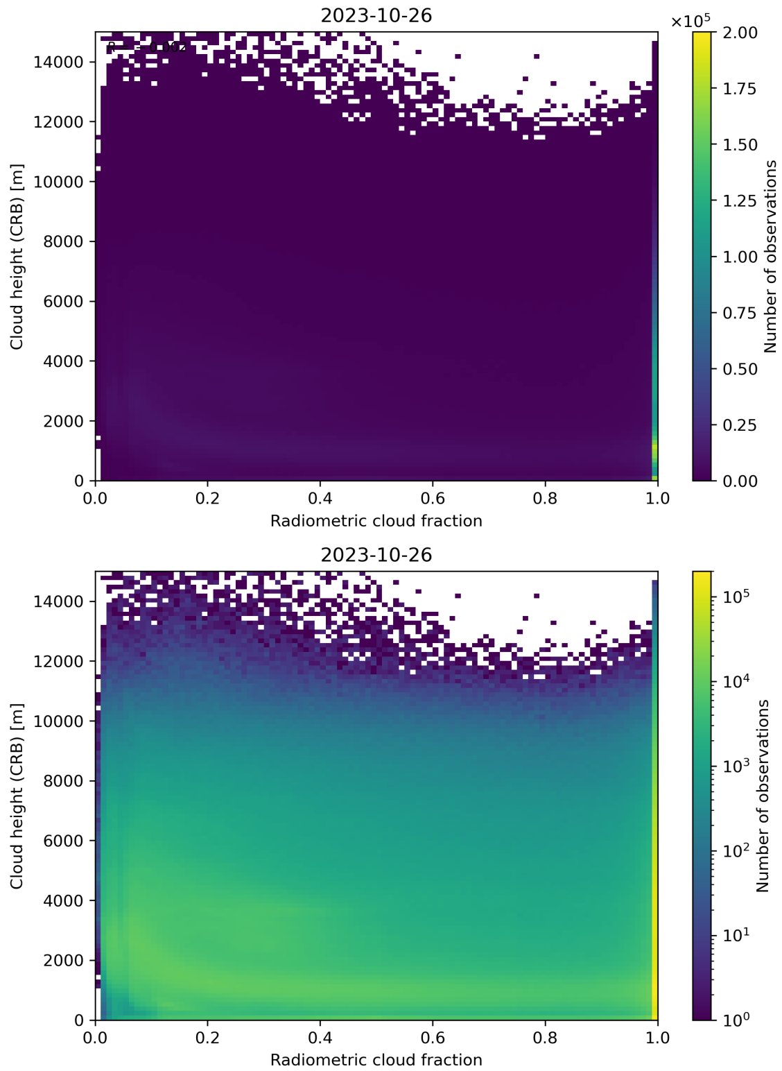
Figure 74: Scatter density plot of “Radiometric cloud fraction” against “Cloud height (CRB)” for 2023-10-25 to 2023-10-27.
