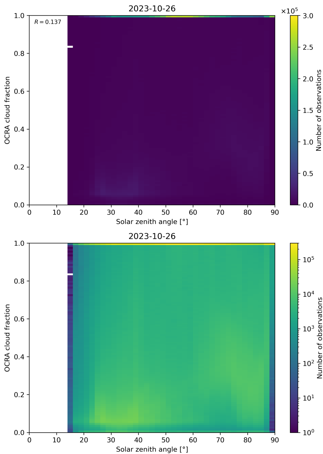
Figure 100: Scatter density plot of “Solar zenith angle” against “OCRA cloud fraction” for 2023-10-25 to 2023-10-27.
