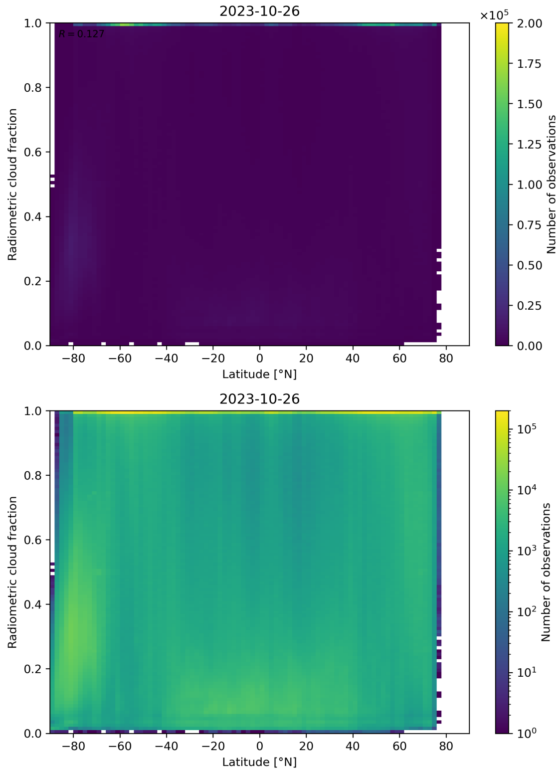
Figure 92: Scatter density plot of “Latitude” against “Radiometric cloud fraction” for 2023-10-25 to 2023-10-27.
