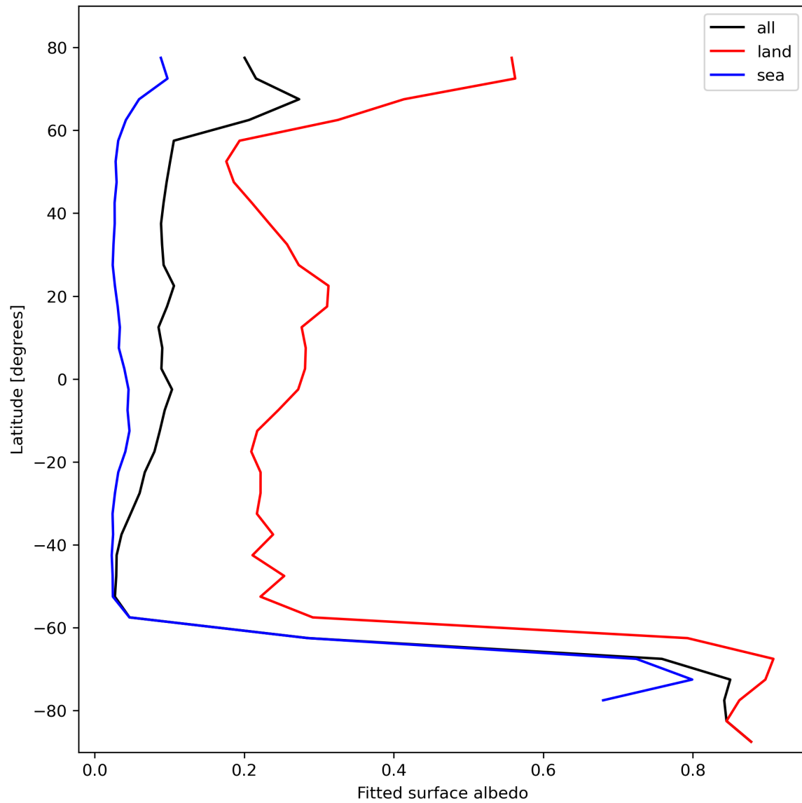
Figure 29: Zonal average of “Fitted surface albedo” for 2023-10-25 to 2023-10-27.
