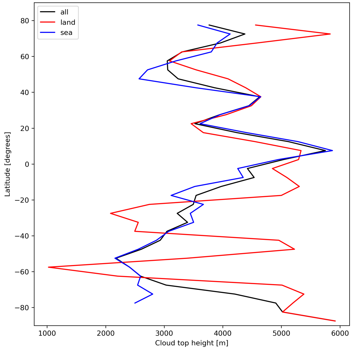
Figure 24: Zonal average of “Cloud top height” for 2023-10-25 to 2023-10-27.
