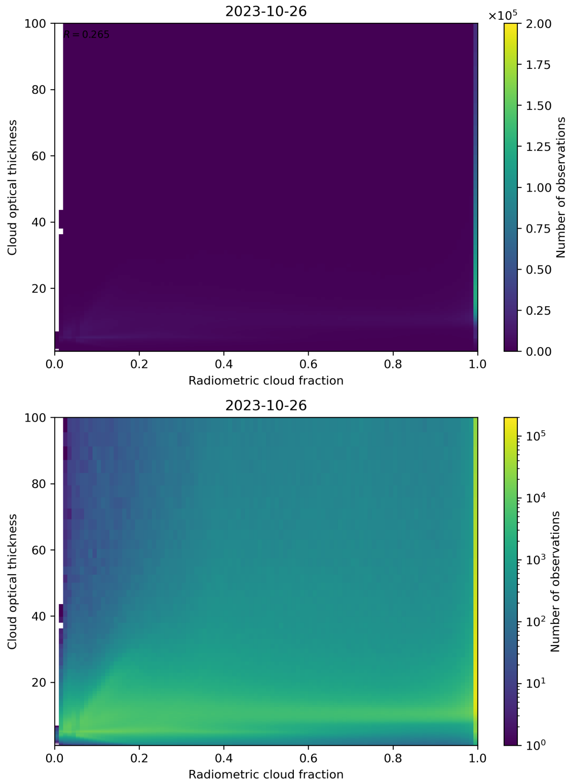
Figure 75: Scatter density plot of “Radiometric cloud fraction” against “Cloud optical thickness” for 2023-10-25 to 2023-10-27.
