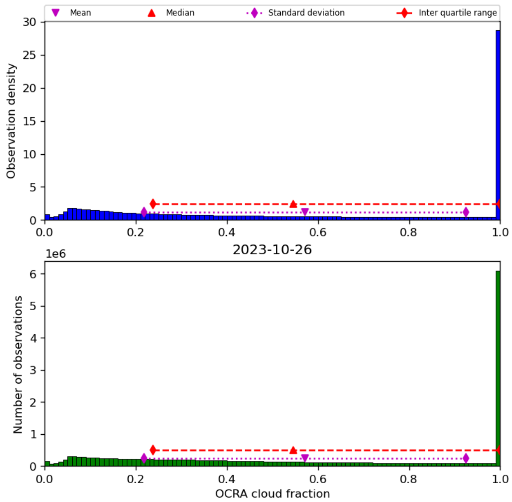
Figure 50: Histogram of “OCRA cloud fraction” for 2023-10-25 to 2023-10-27
