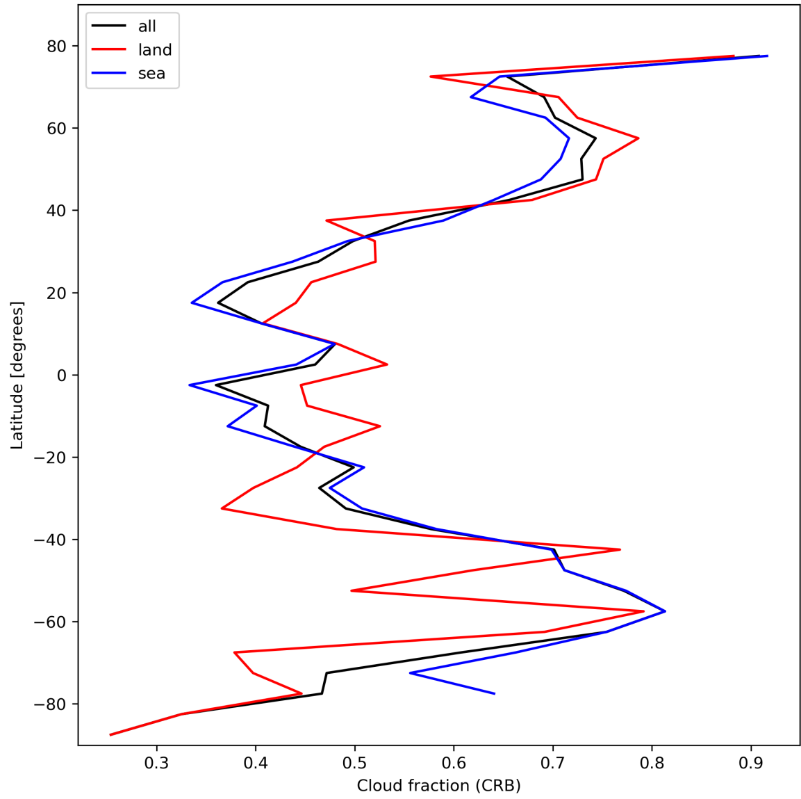
Figure 26: Zonal average of “Cloud fraction (CRB)” for 2023-10-25 to 2023-10-27.
