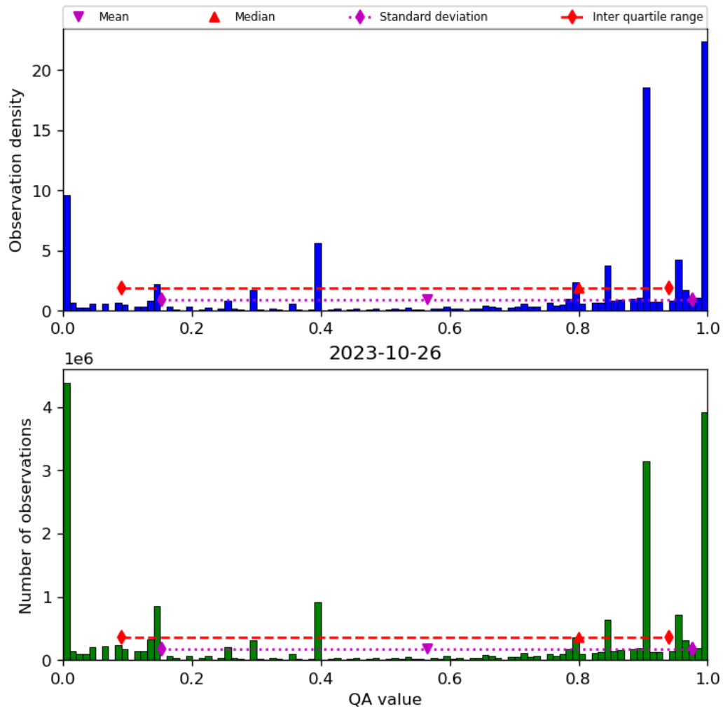
Figure 38: Histogram of “QA value” for 2023-10-25 to 2023-10-27
