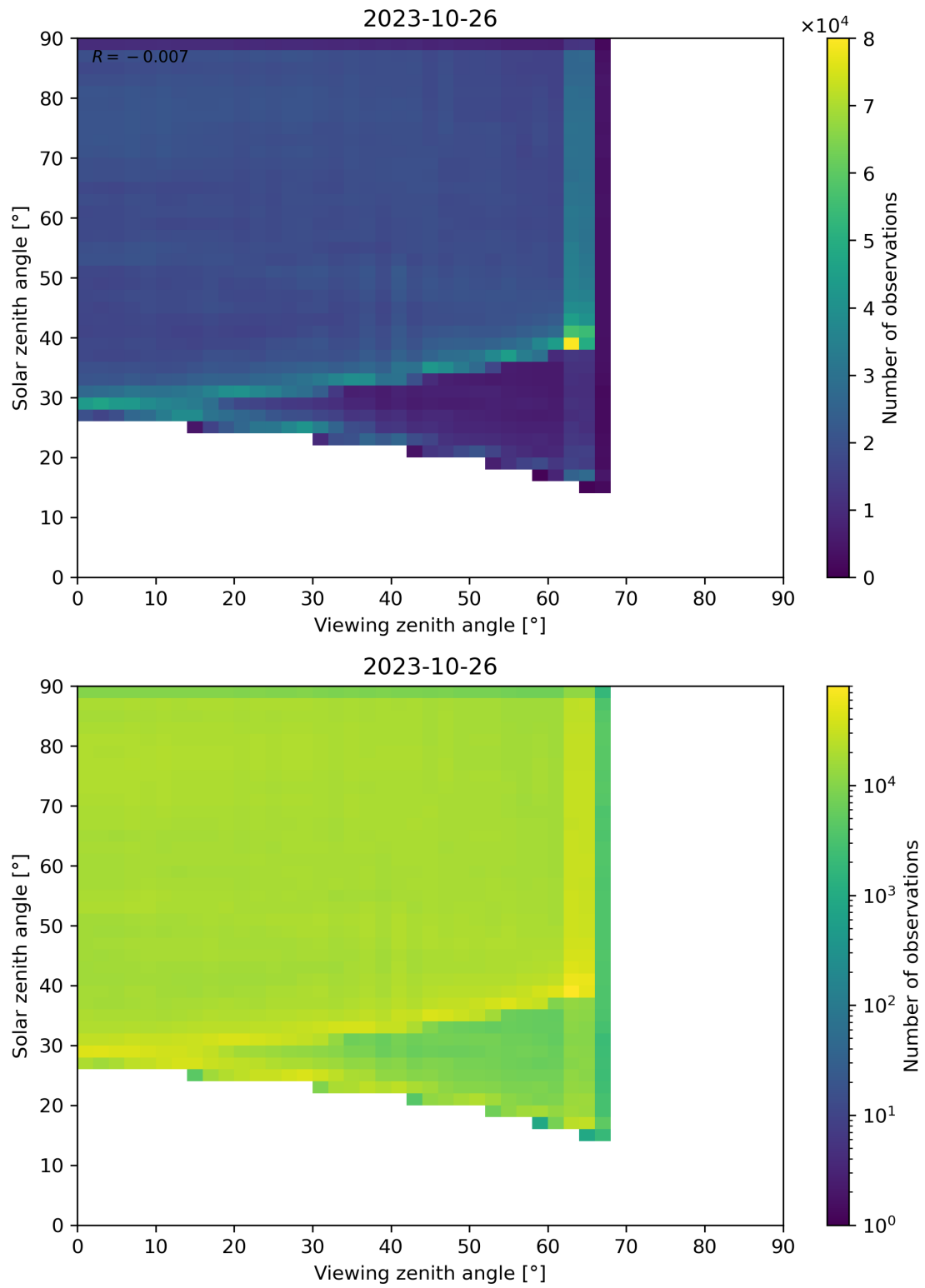
Figure 114: Scatter density plot of “Viewing zenith angle” against “Solar zenith angle” for 2023-10-25 to 2023-10-27.
