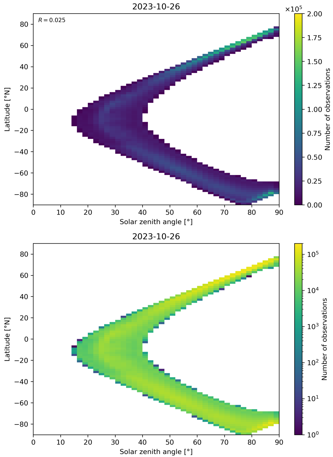
Figure 105: Scatter density plot of “Solar zenith angle” against “Latitude” for 2023-10-25 to 2023-10-27.
