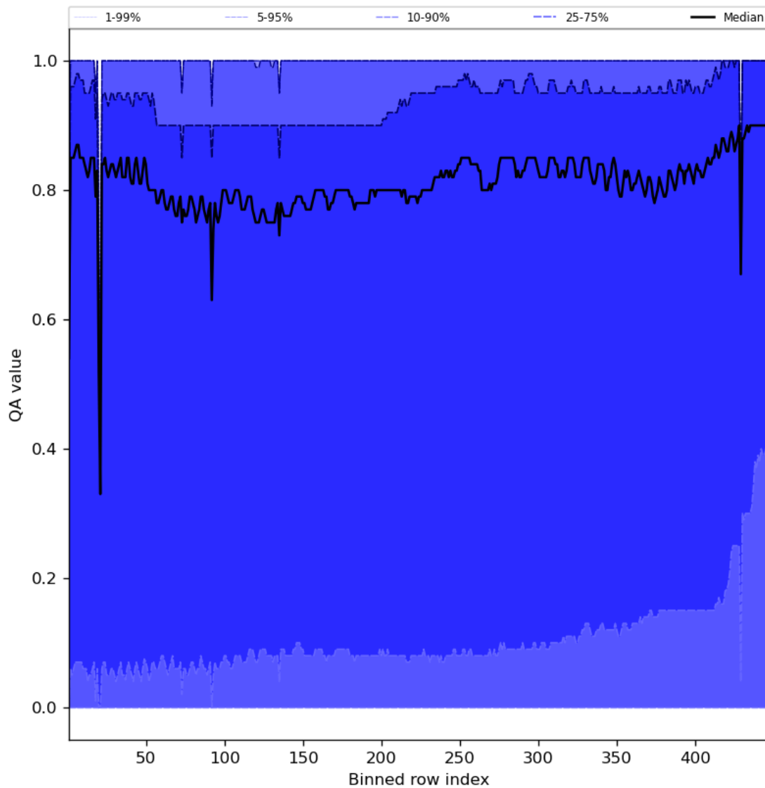
Figure 54: Along track statistics of “QA value” for 2023-10-25 to 2023-10-27
