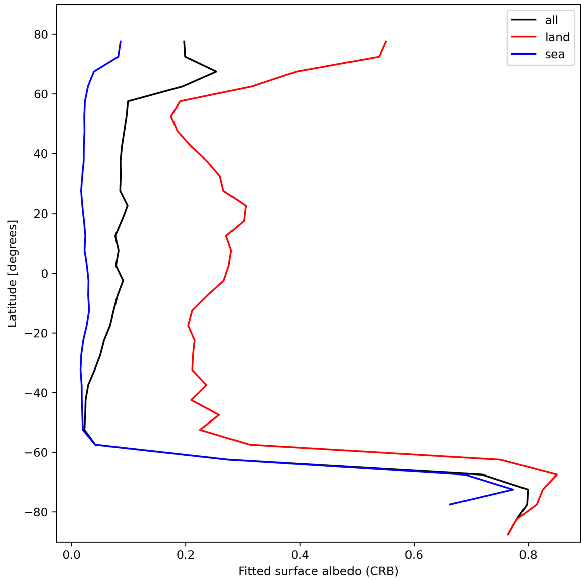
Figure 30: Zonal average of “Fitted surface albedo (CRB)” for 2023-10-25 to 2023-10-27.
