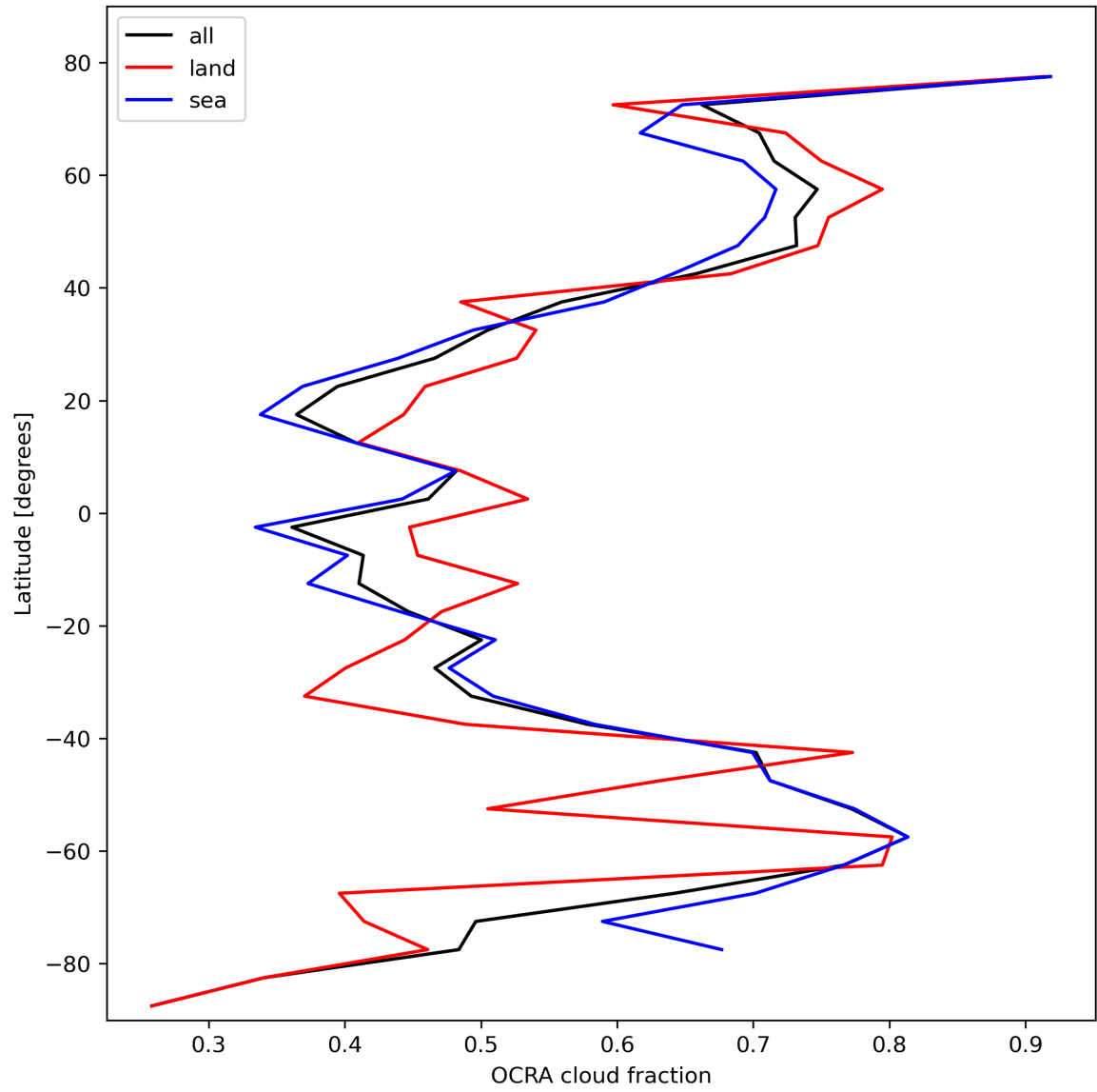
Figure 34: Zonal average of “OCRA cloud fraction” for 2023-10-25 to 2023-10-27.
