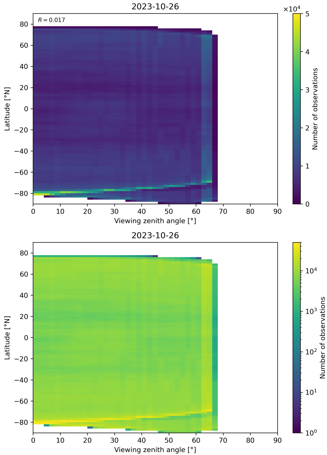
Figure 113: Scatter density plot of “Viewing zenith angle” against “Latitude” for 2023-10-25 to 2023-10-27.
