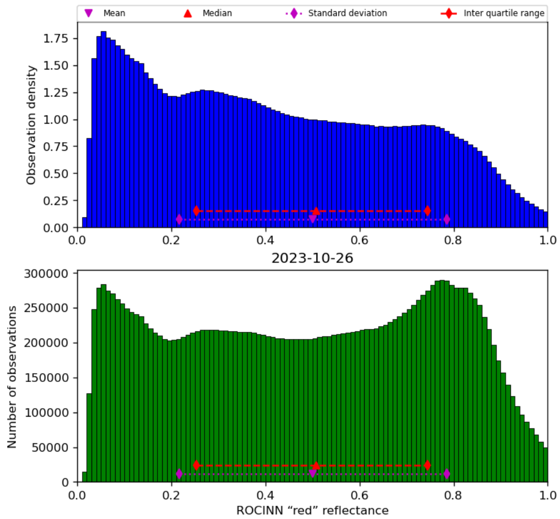
Figure 53: Histogram of “ROCINN “red” reflectance” for 2023-10-25 to 2023-10-27
