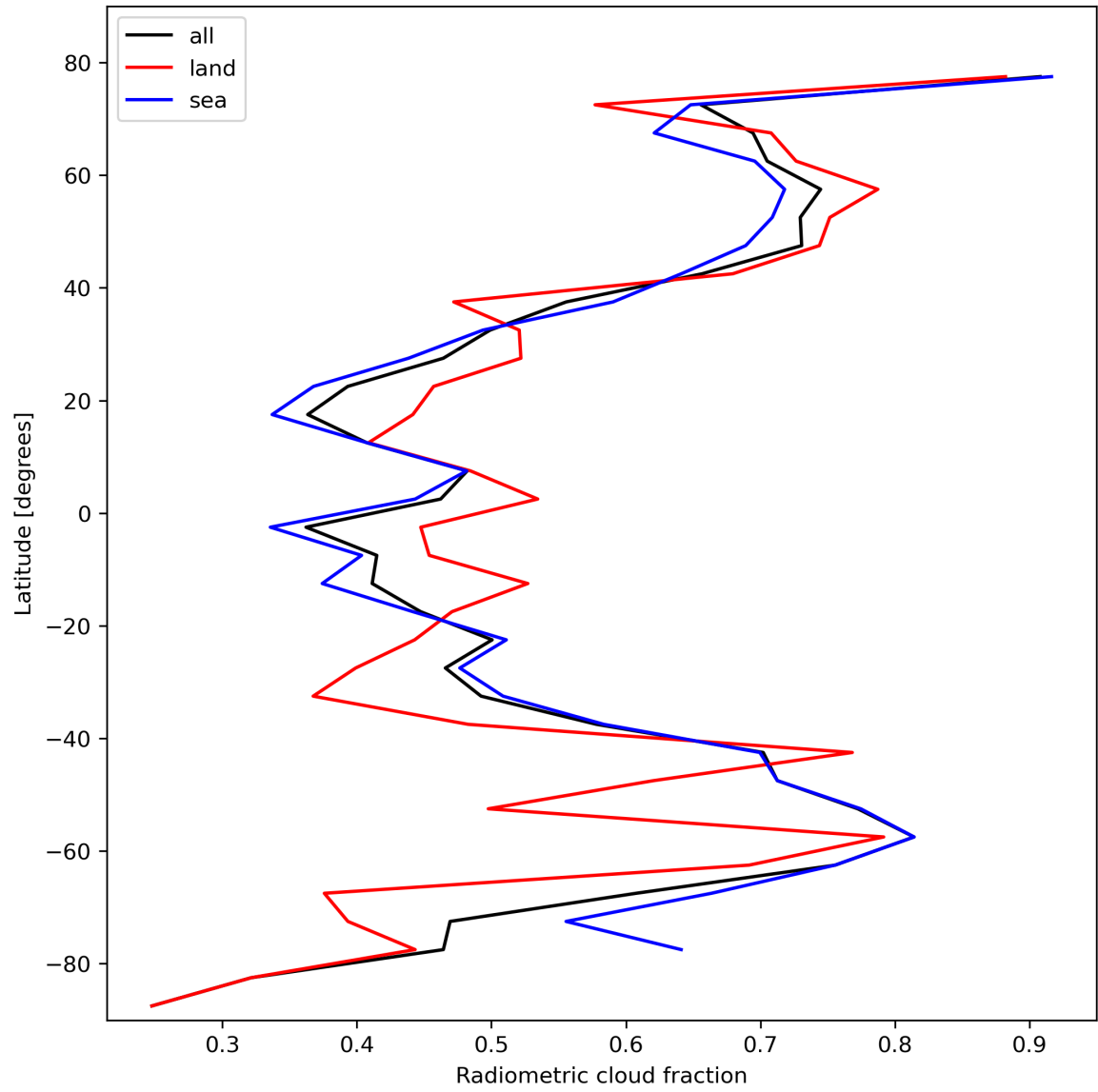
Figure 23: Zonal average of “Radiometric cloud fraction” for 2023-10-25 to 2023-10-27.
