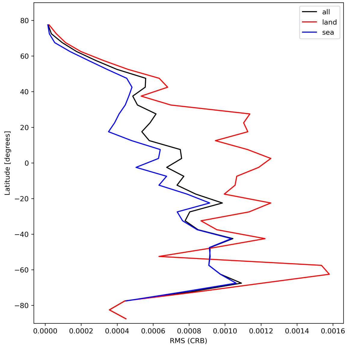
Figure 32: Zonal average of “RMS (CRB)” for 2023-10-25 to 2023-10-27.
