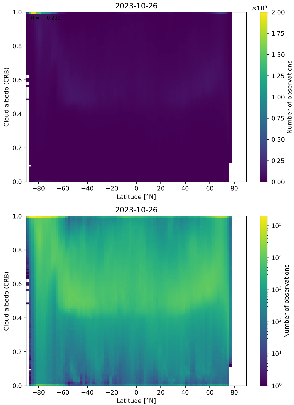
Figure 91: Scatter density plot of “Latitude” against “Cloud albedo (CRB)” for 2023-10-25 to 2023-10-27.
