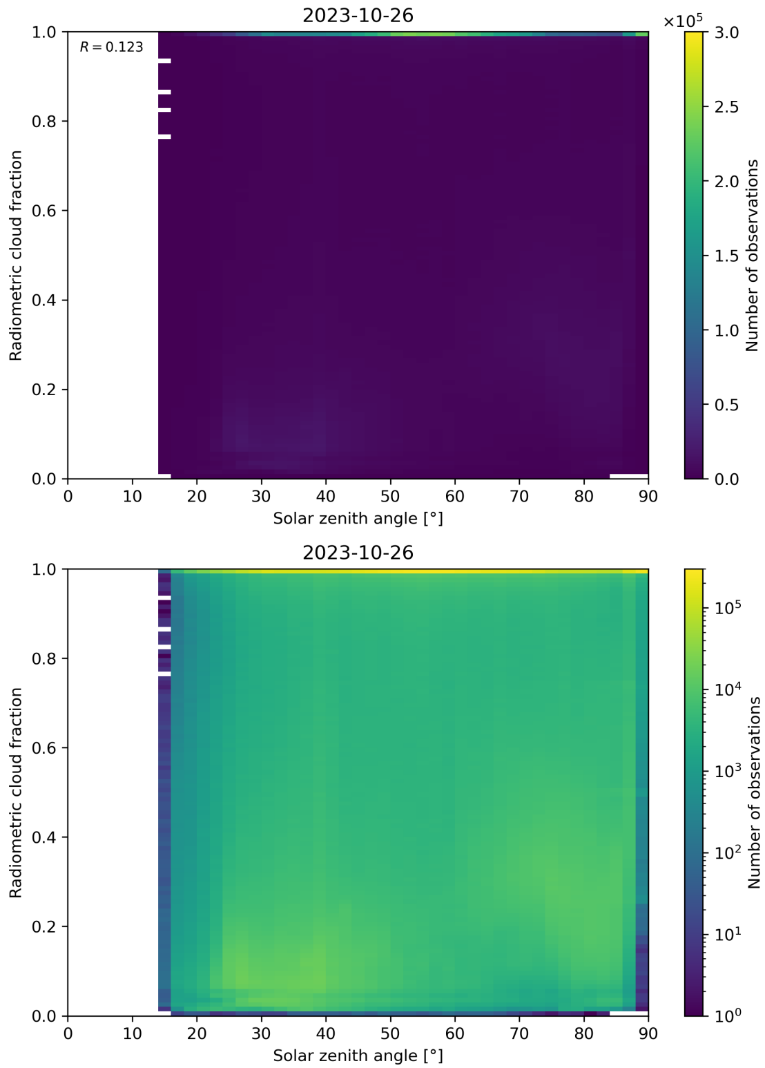
Figure 99: Scatter density plot of “Solar zenith angle” against “Radiometric cloud fraction” for 2023-10-25 to 2023-10-27.
