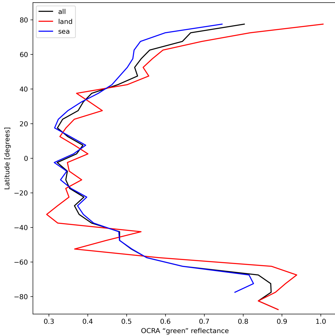
Figure 36: Zonal average of “OCRA “green” reflectance” for 2023-10-25 to 2023-10-27.
