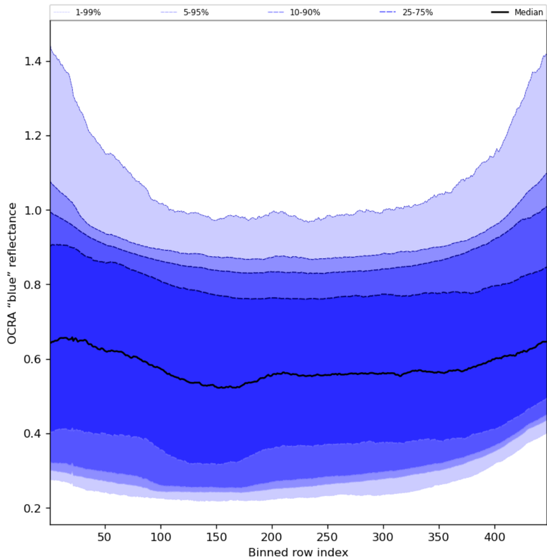
Figure 67: Along track statistics of "OCRA "blue" reflectance" for 2023-10-25 to 2023-10-27
