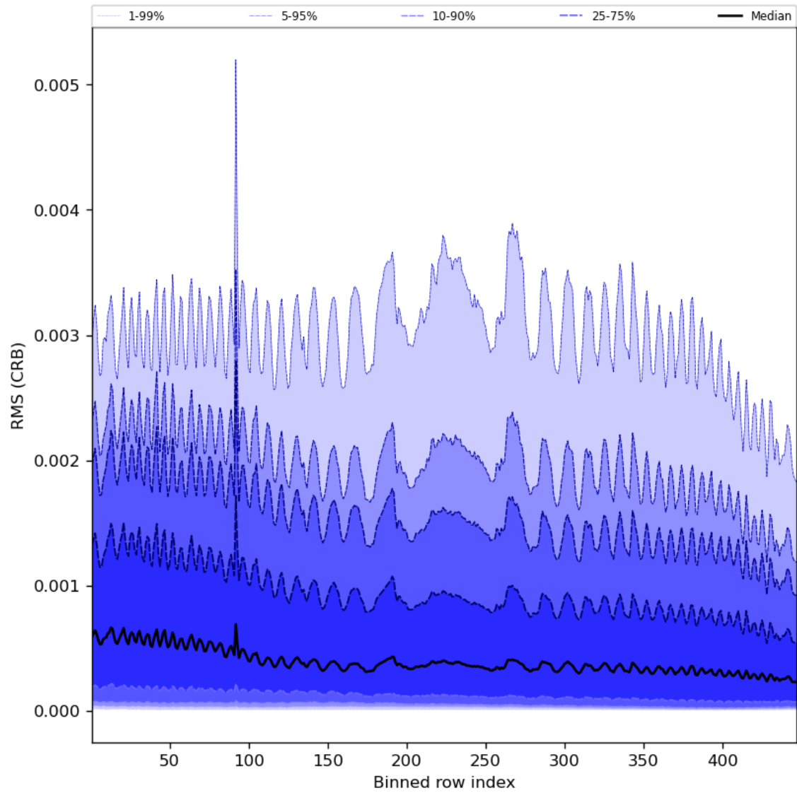
Figure 64: Along track statistics of “RMS (CRB)” for 2023-10-25 to 2023-10-27
