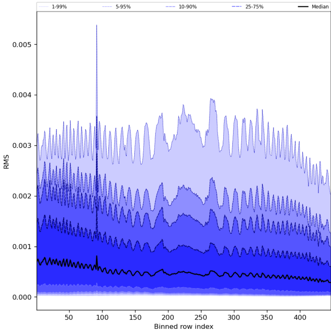
Figure 63: Along track statistics of “RMS” for 2023-10-25 to 2023-10-27
