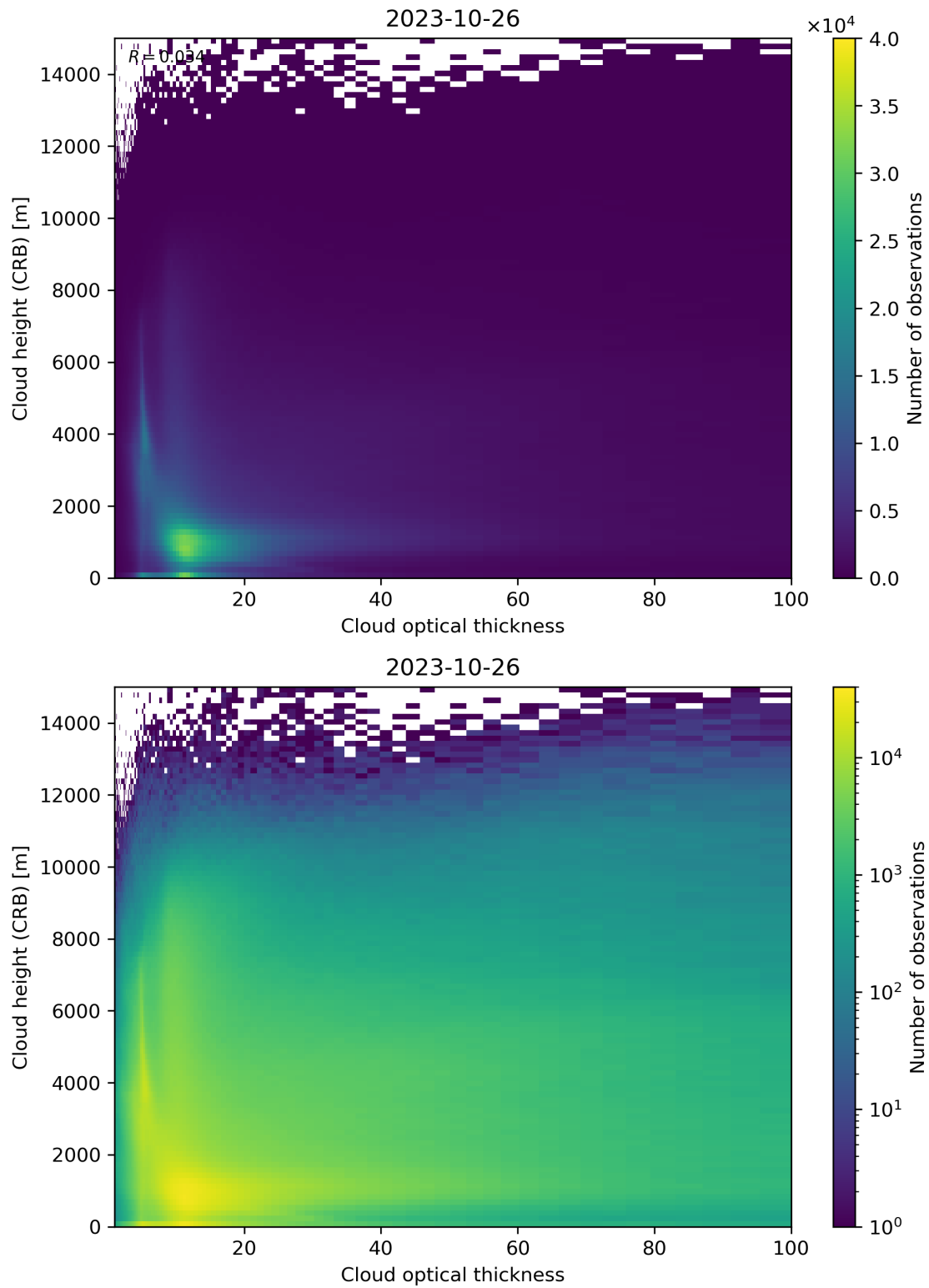
Figure 85: Scatter density plot of “Cloud optical thickness” against “Cloud height (CRB)” for 2023-10-25 to 2023-10-27.
