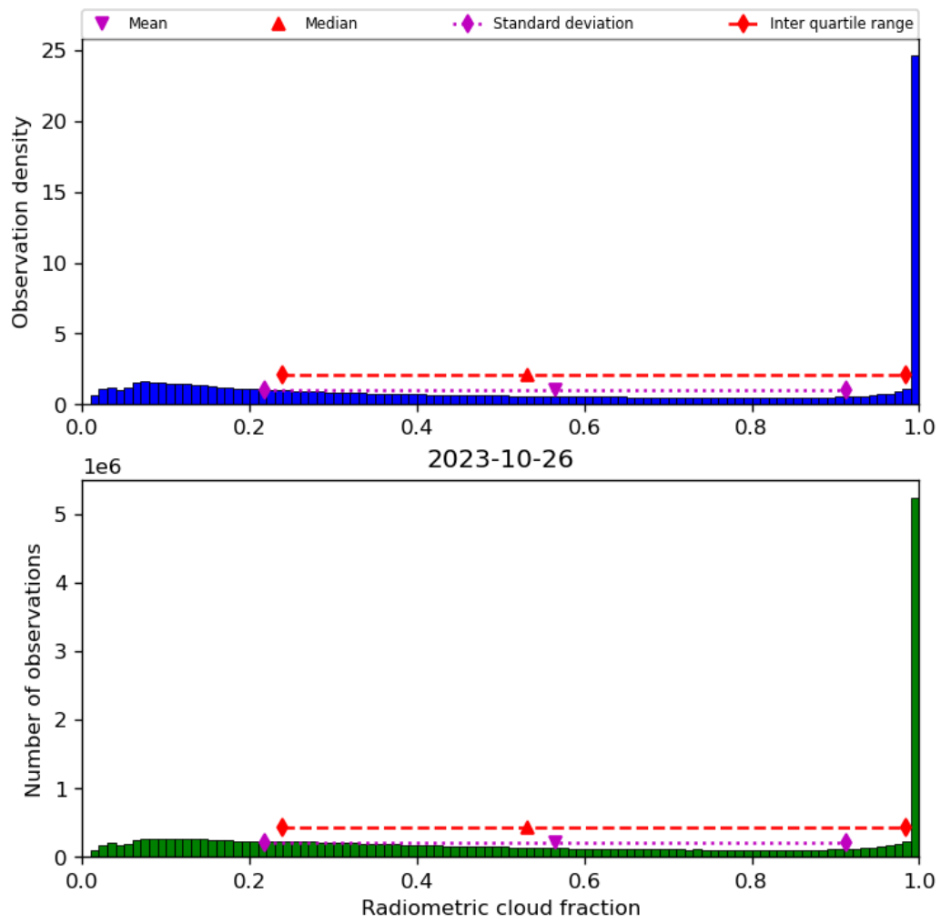
Figure 39: Histogram of “Radiometric cloud fraction” for 2023-10-25 to 2023-10-27
