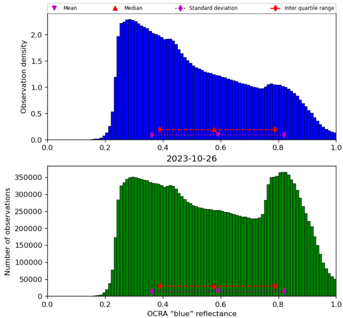
Figure 51: Histogram of “OCRA “blue” reflectance” for 2023-10-25 to 2023-10-27
