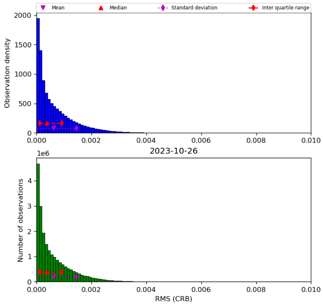
Figure 48: Histogram of “RMS (CRB)” for 2023-10-25 to 2023-10-27
