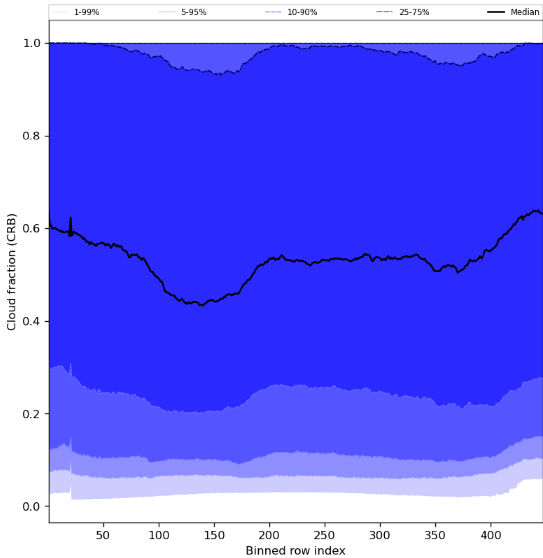
Figure 58: Along track statistics of “Cloud fraction (CRB)” for 2023-10-25 to 2023-10-27
