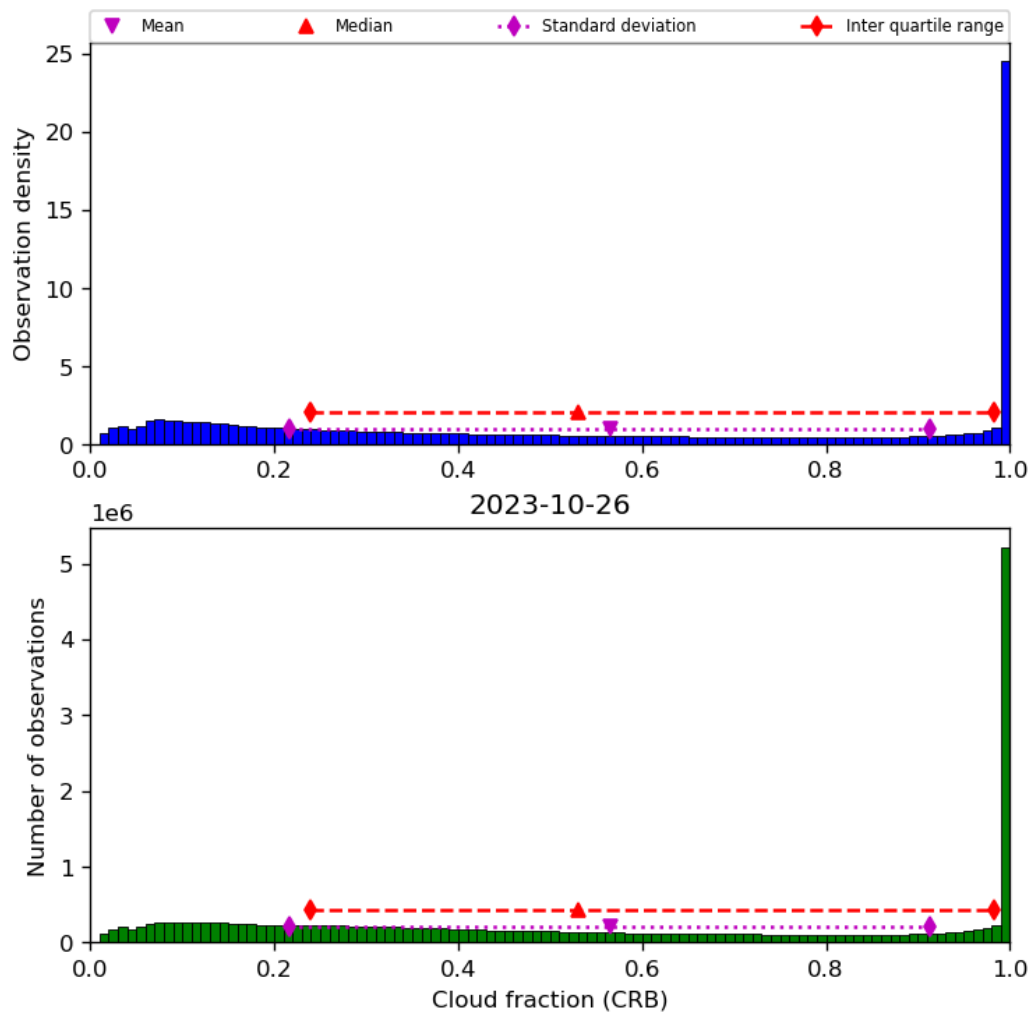
Figure 42: Histogram of “Cloud fraction (CRB)” for 2023-10-25 to 2023-10-27
