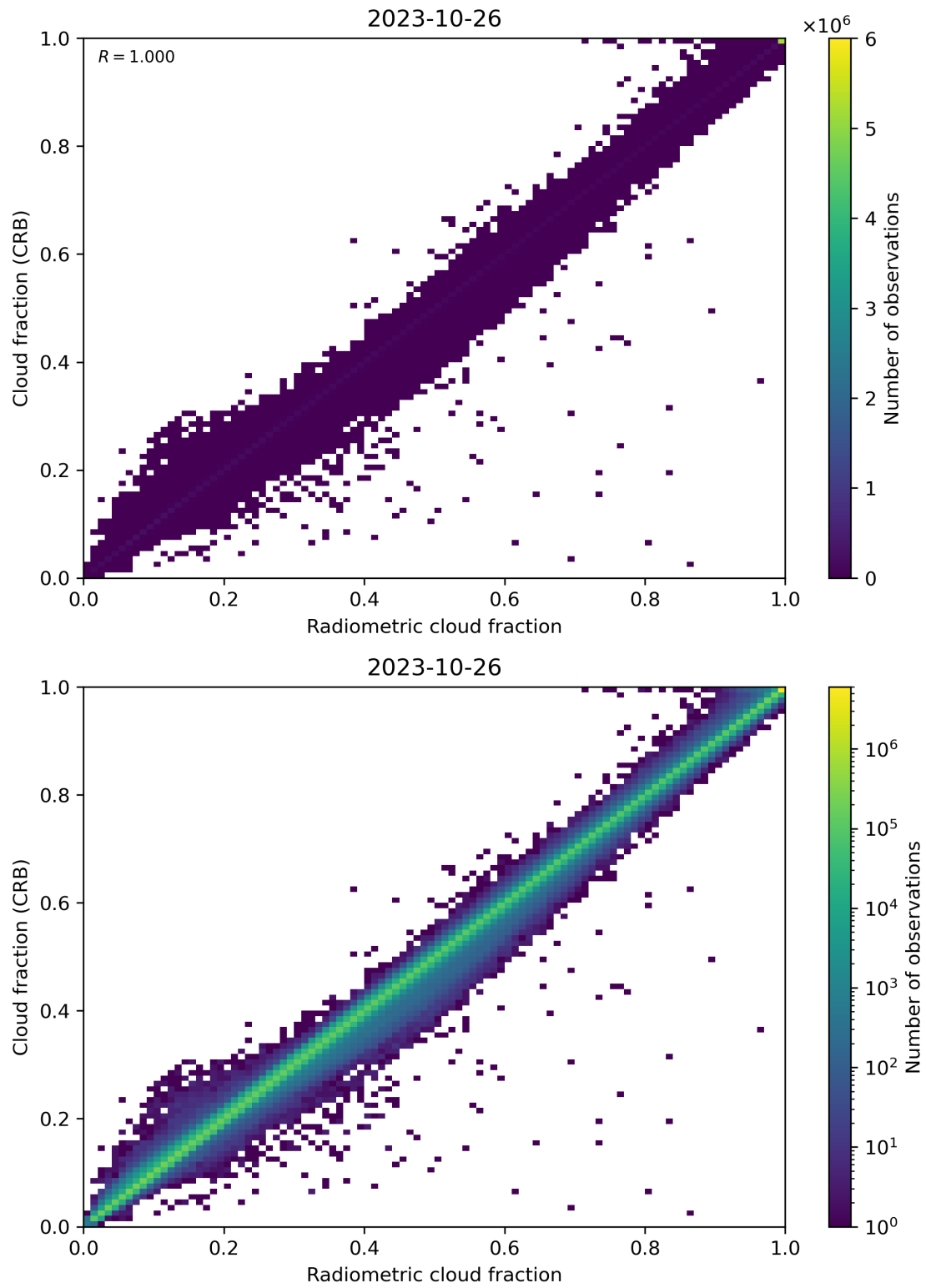
Figure 73: Scatter density plot of “Radiometric cloud fraction” against “Cloud fraction (CRB)” for 2023-10-25 to 2023-10-27.
