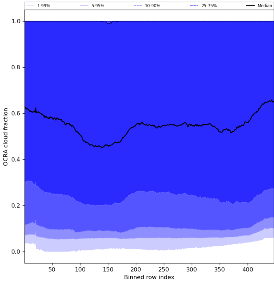
Figure 66: Along track statistics of “OCRA cloud fraction” for 2023-10-25 to 2023-10-27
