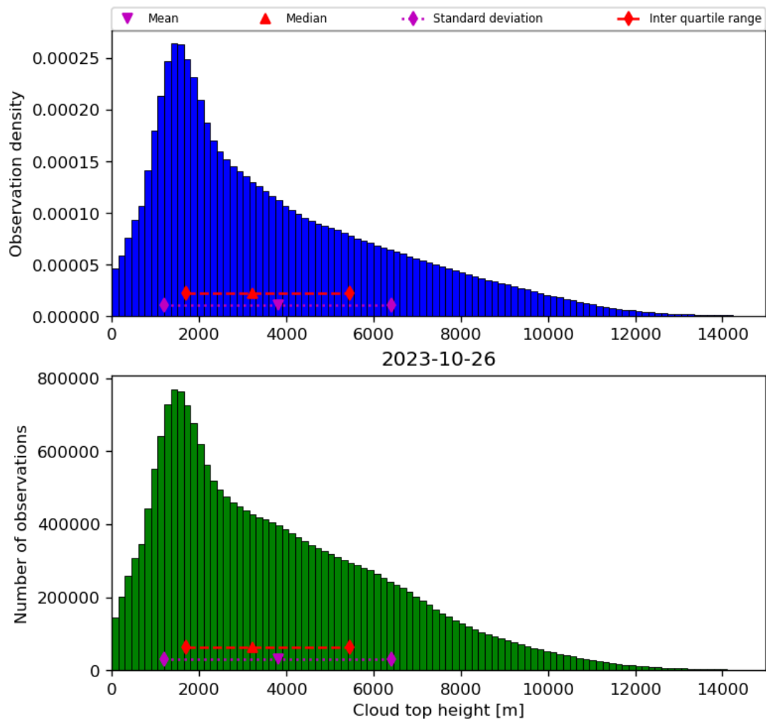
Figure 40: Histogram of “Cloud top height” for 2023-10-25 to 2023-10-27
