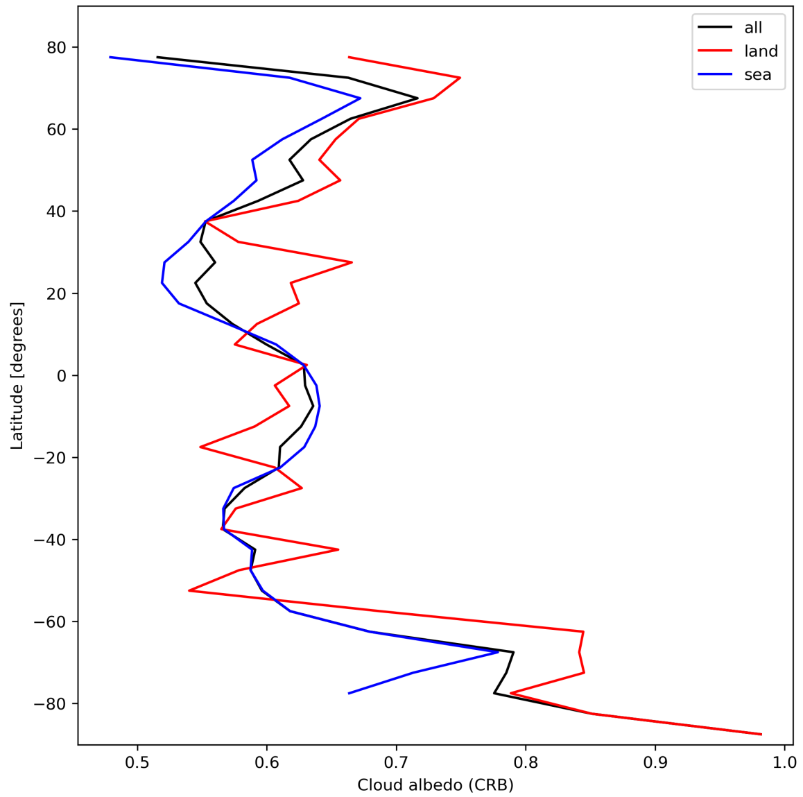
Figure 28: Zonal average of “Cloud albedo (CRB)” for 2023-10-25 to 2023-10-27.
