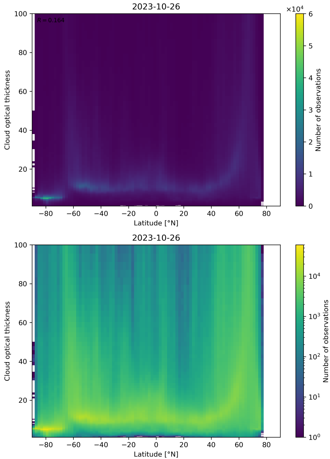
Figure 96: Scatter density plot of “Latitude” against “Cloud optical thickness” for 2023-10-25 to 2023-10-27.
