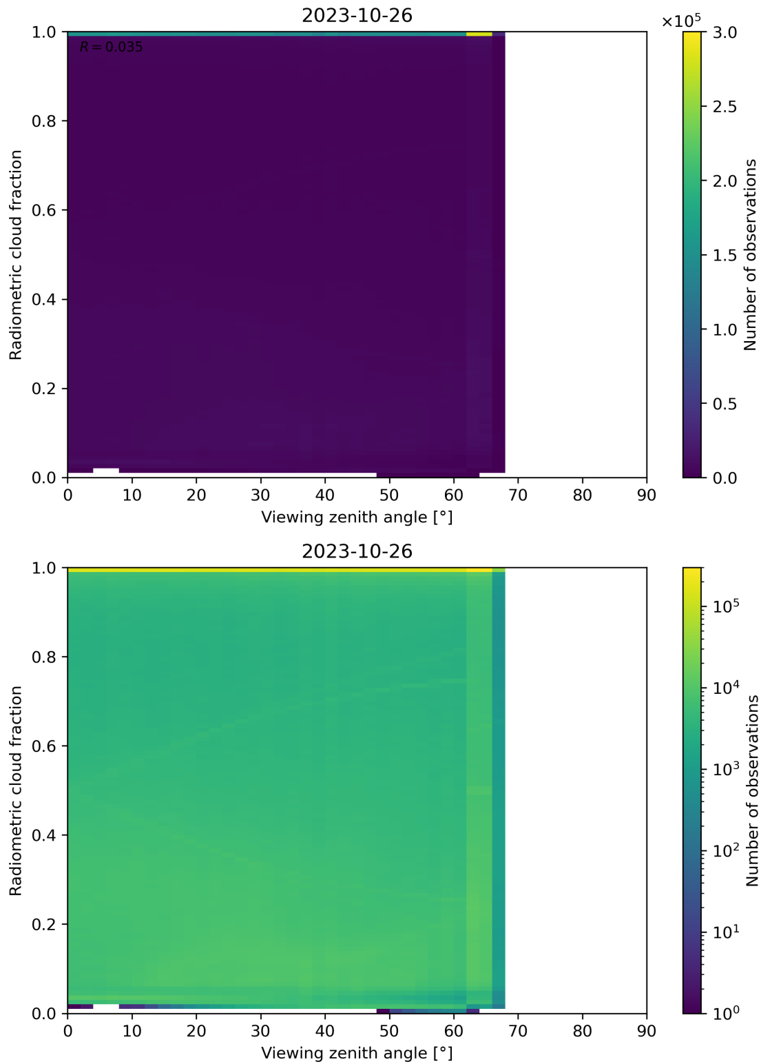
Figure 107: Scatter density plot of “Viewing zenith angle” against “Radiometric cloud fraction” for 2023-10-25 to 2023-10-27.
