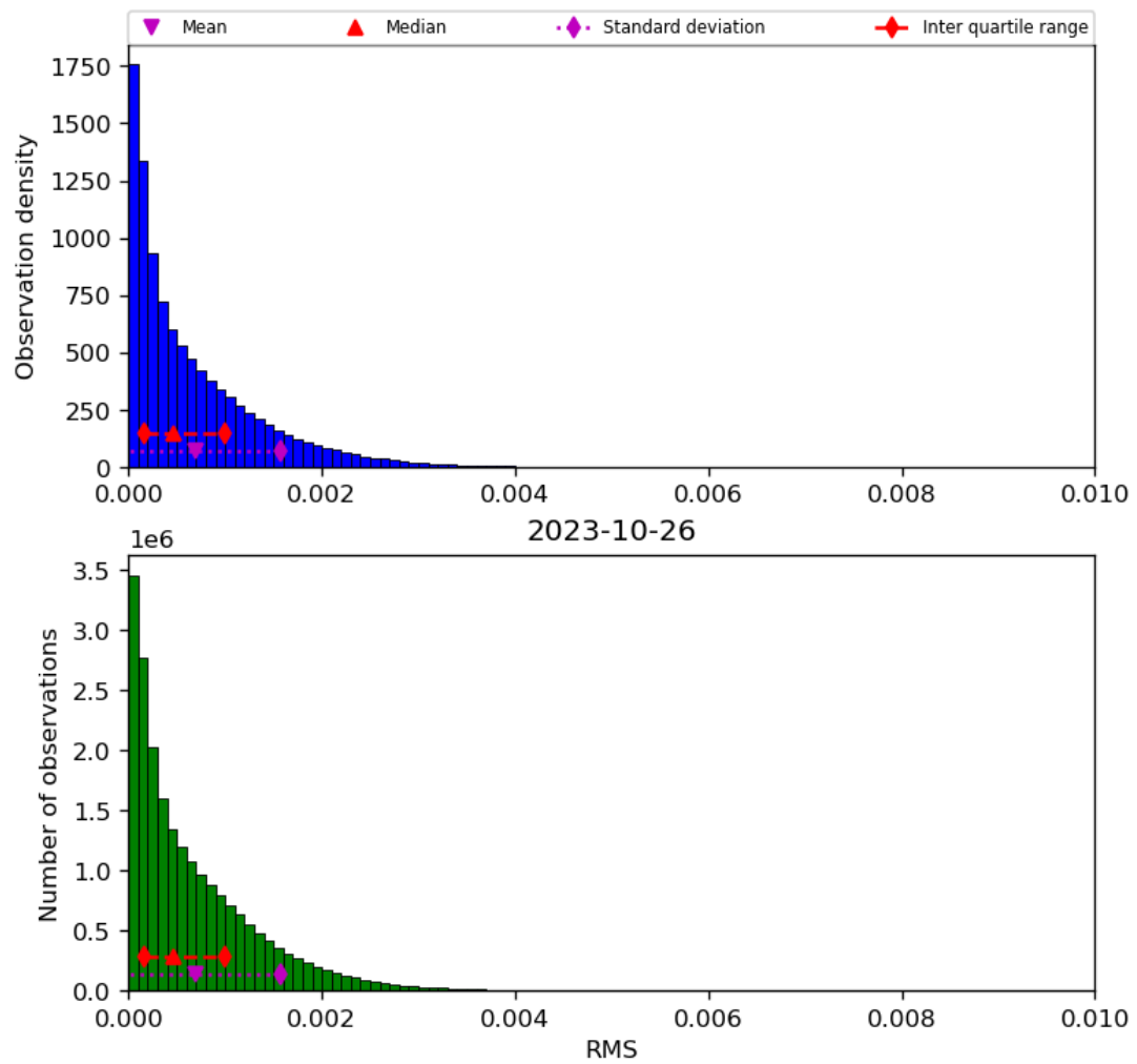
Figure 47: Histogram of “RMS” for 2023-10-25 to 2023-10-27
