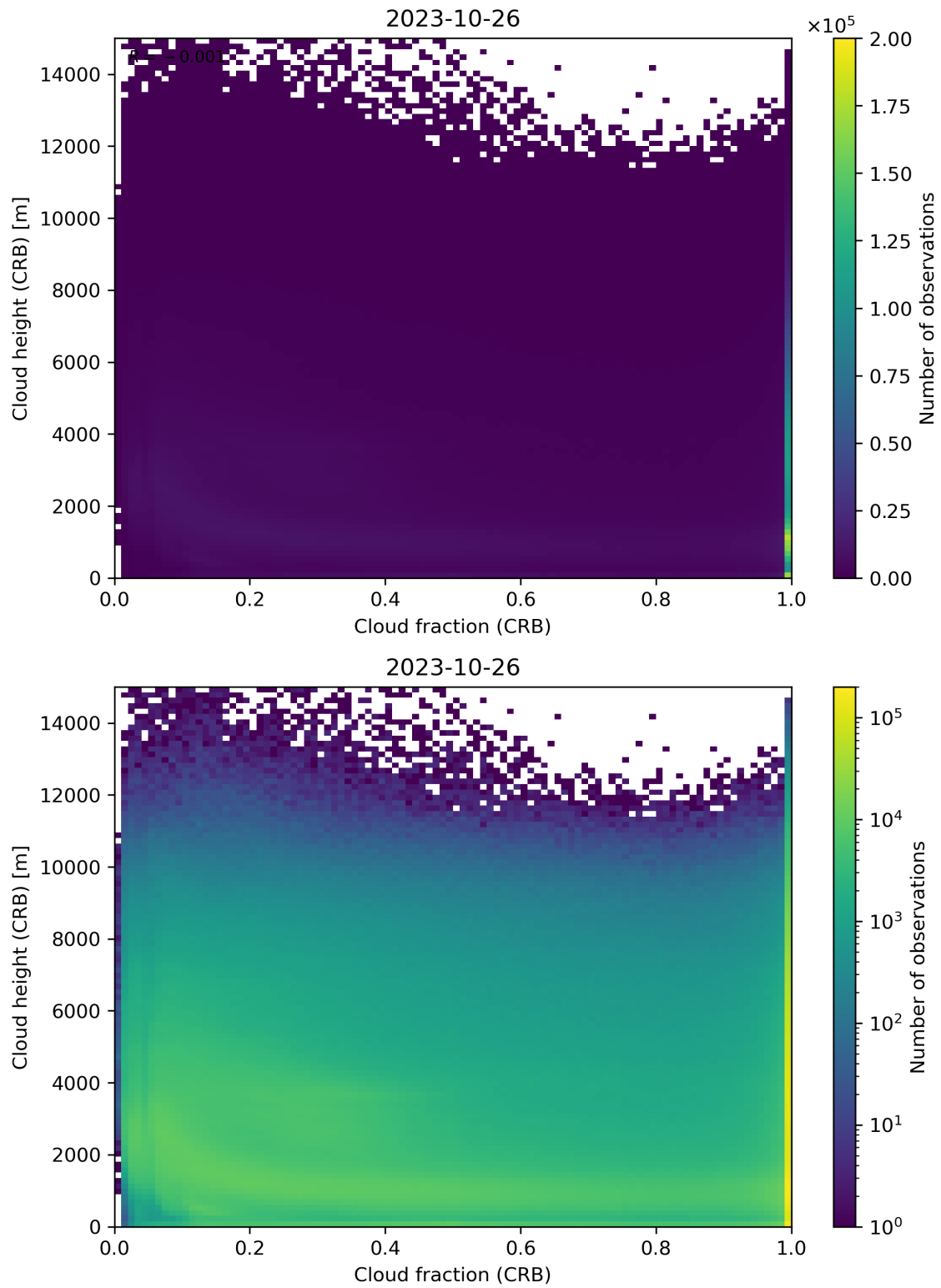
Figure 79: Scatter density plot of “Cloud fraction (CRB)” against “Cloud height (CRB)” for 2023-10-25 to 2023-10-27.
