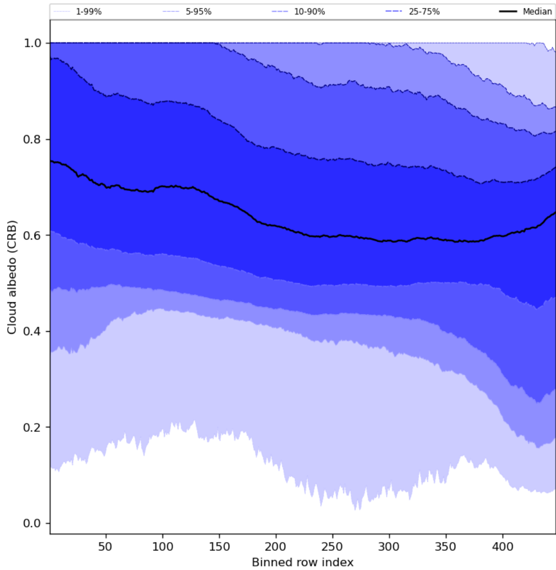
Figure 60: Along track statistics of “Cloud albedo (CRB)” for 2023-10-25 to 2023-10-27
