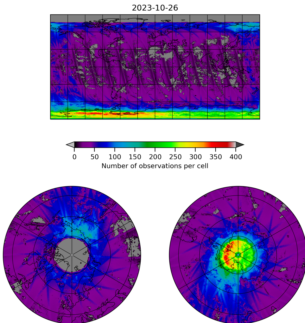
Figure 21: Map of the number of observations for 2023-10-25 to 2023-10-27
