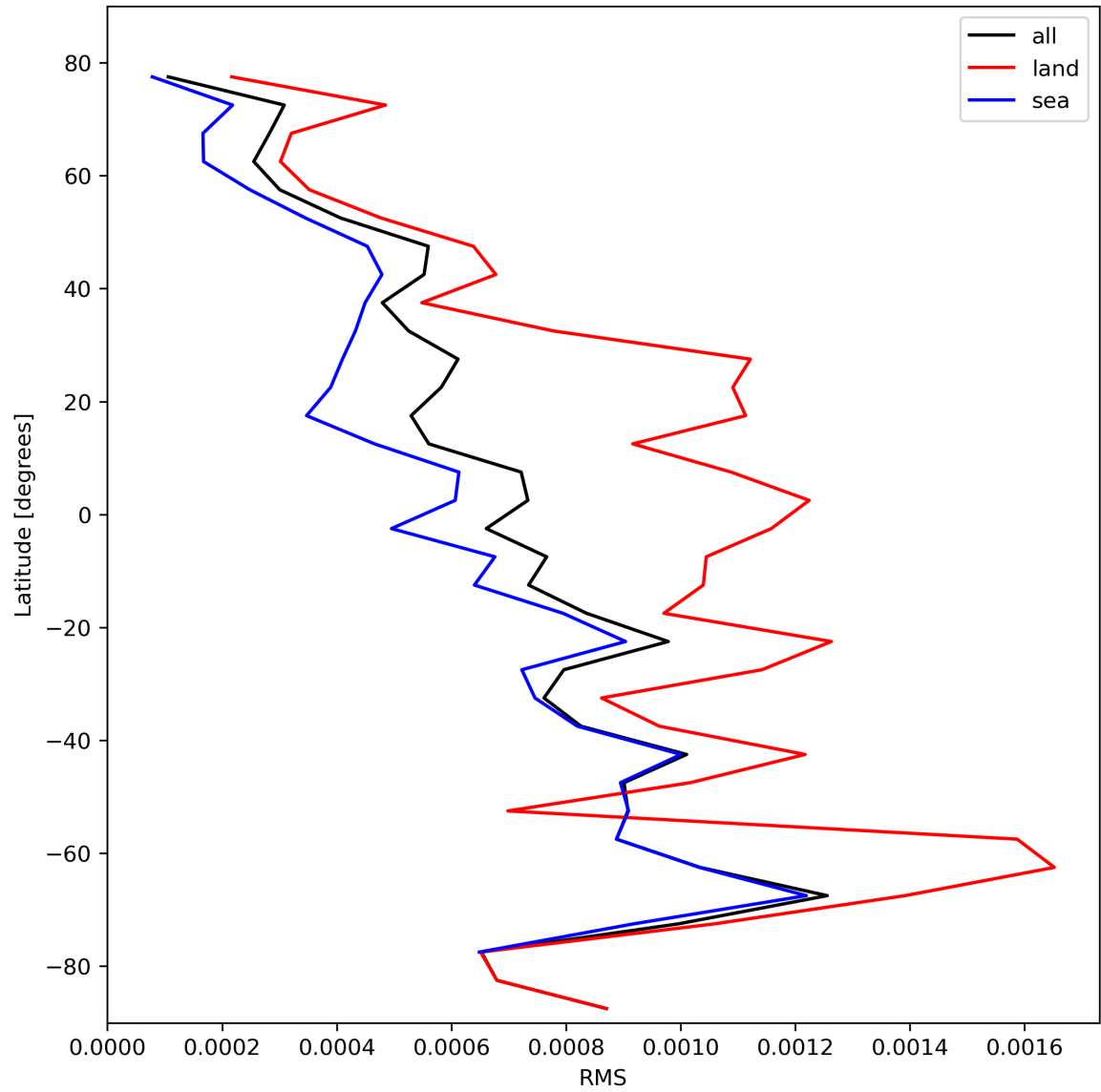
Figure 31: Zonal average of “RMS” for 2023-10-25 to 2023-10-27.
