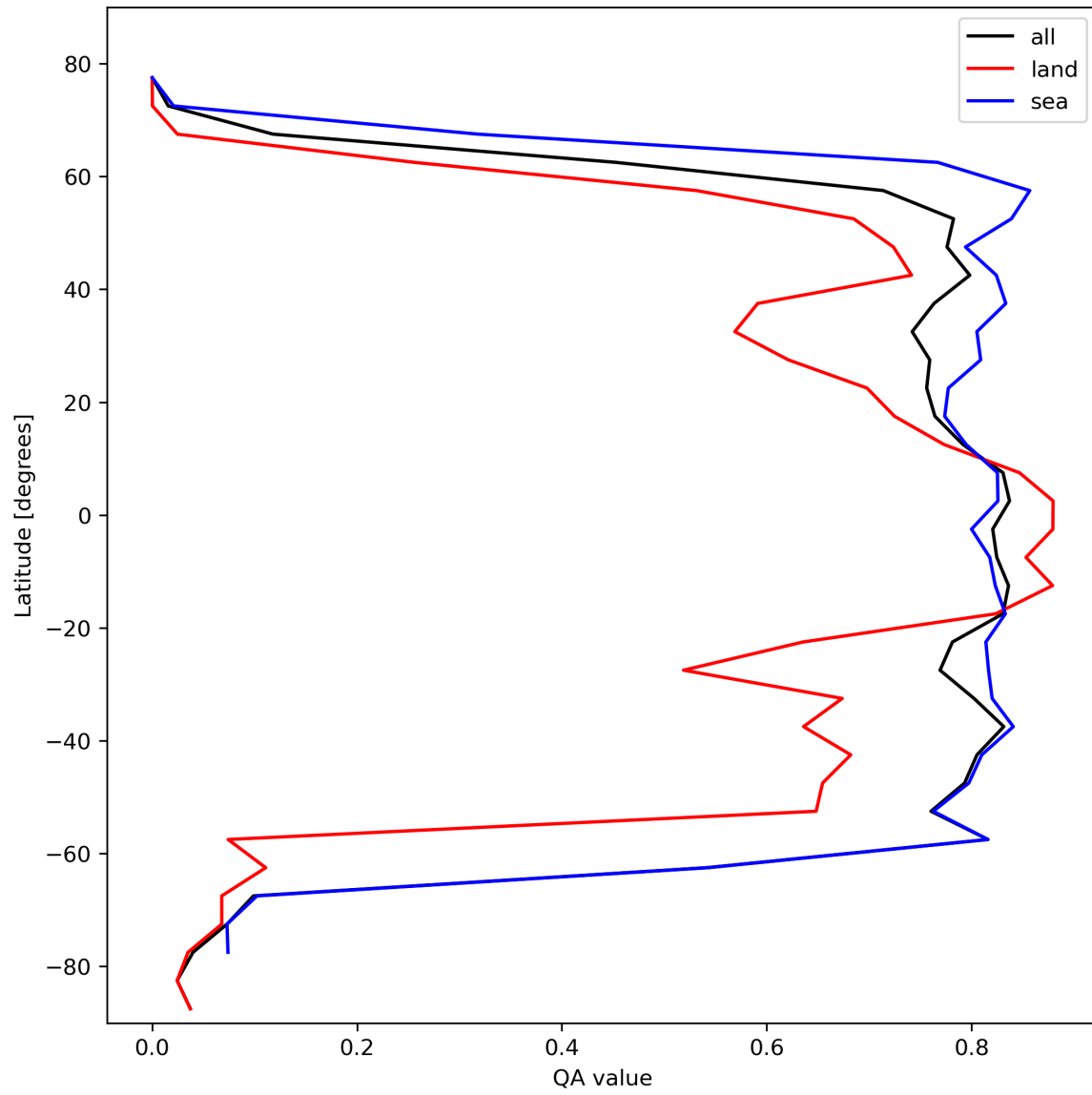
Figure 22: Zonal average of “QA value” for 2023-10-25 to 2023-10-27.
