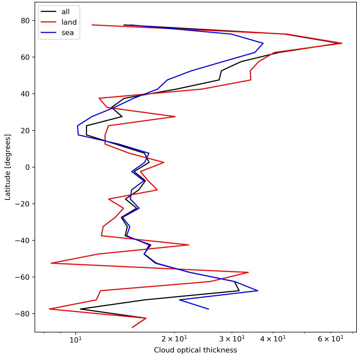
Figure 25: Zonal average of “Cloud optical thickness” for 2023-10-25 to 2023-10-27.
