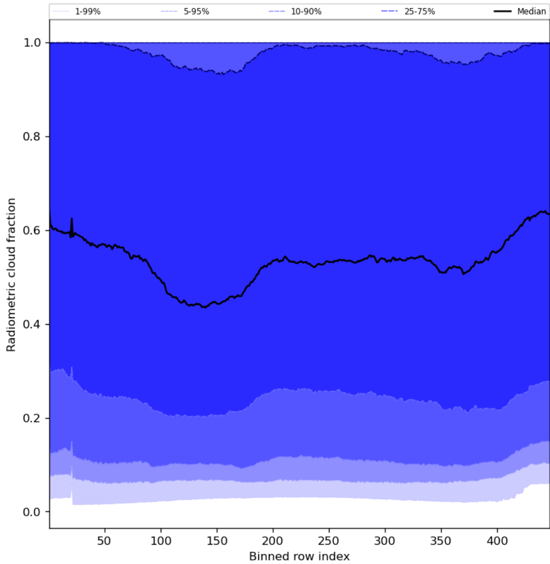
Figure 55: Along track statistics of “Radiometric cloud fraction” for 2023-10-25 to 2023-10-27
