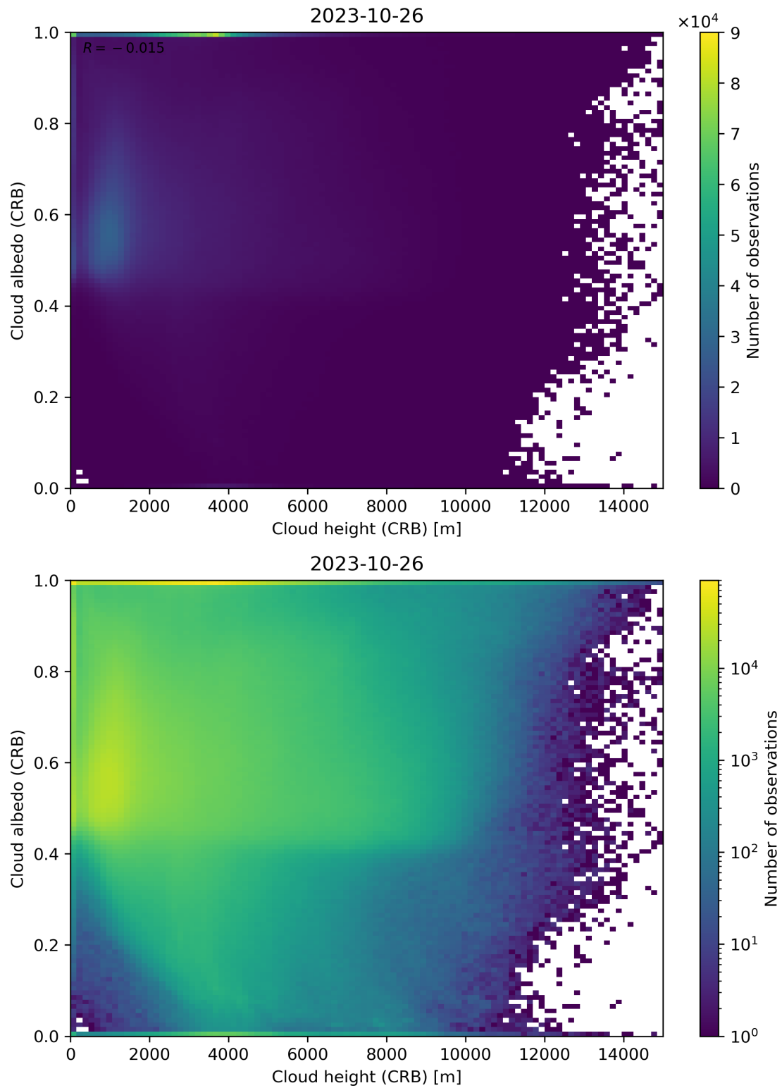
Figure 80: Scatter density plot of “Cloud height (CRB)” against “Cloud albedo (CRB)” for 2023-10-25 to 2023-10-27.
