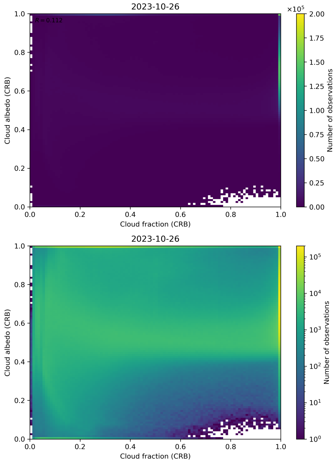
Figure 77: Scatter density plot of “Cloud fraction (CRB)” against “Cloud albedo (CRB)” for 2023-10-25 to 2023-10-27.
