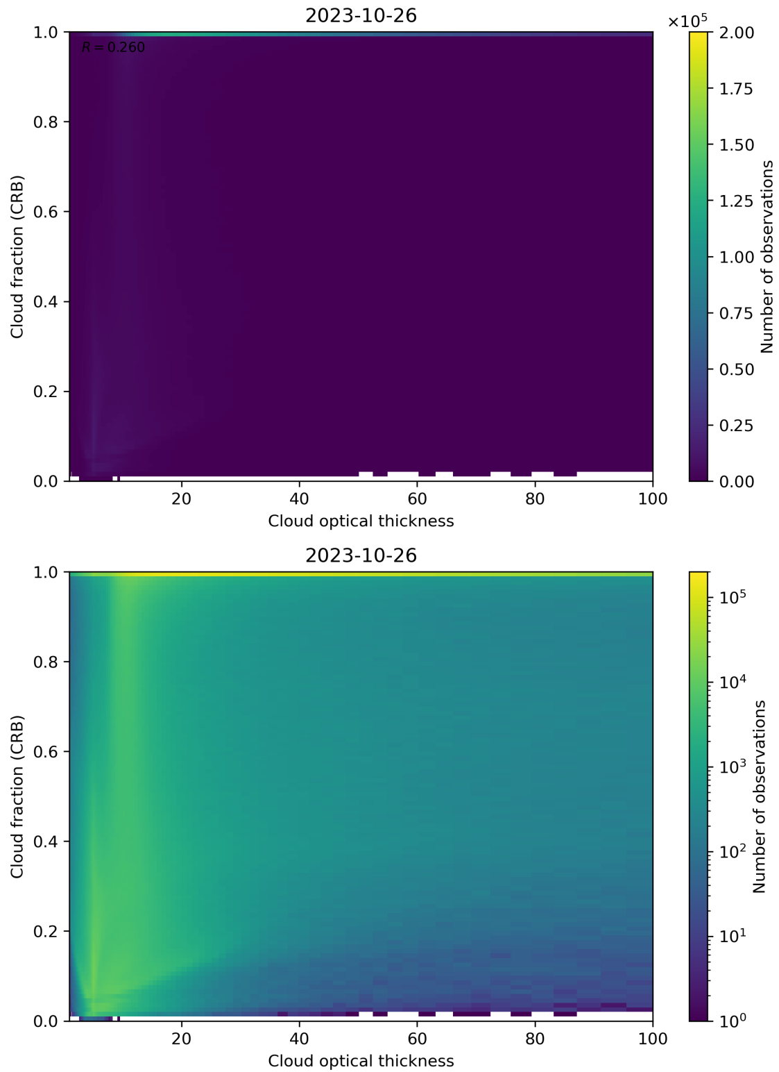
Figure 84: Scatter density plot of “Cloud optical thickness” against “Cloud fraction (CRB)” for 2023-10-25 to 2023-10-27.
