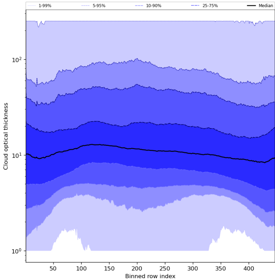
Figure 57: Along track statistics of “Cloud optical thickness” for 2023-10-25 to 2023-10-27
