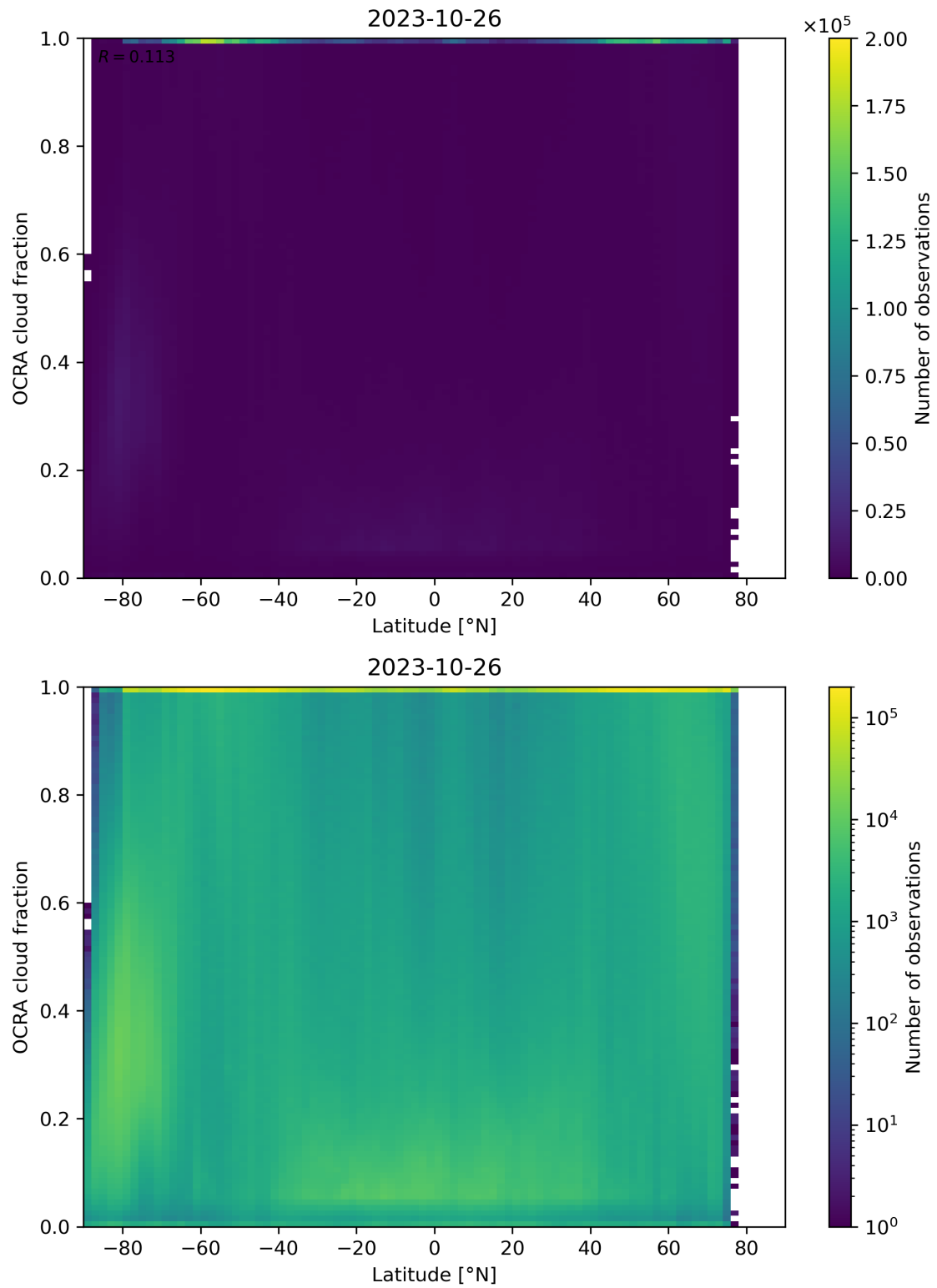
Figure 93: Scatter density plot of “Latitude” against “OCRA cloud fraction” for 2023-10-25 to 2023-10-27.
