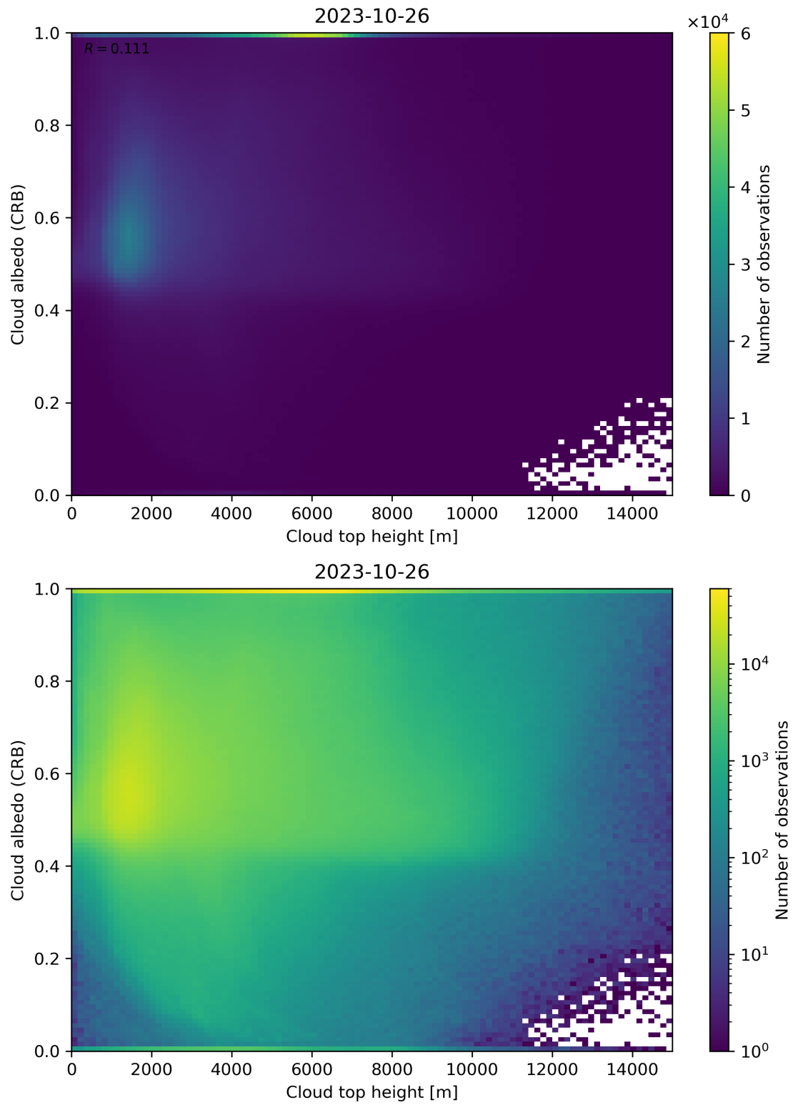
Figure 86: Scatter density plot of “Cloud top height” against “Cloud albedo (CRB)” for 2023-10-25 to 2023-10-27.
