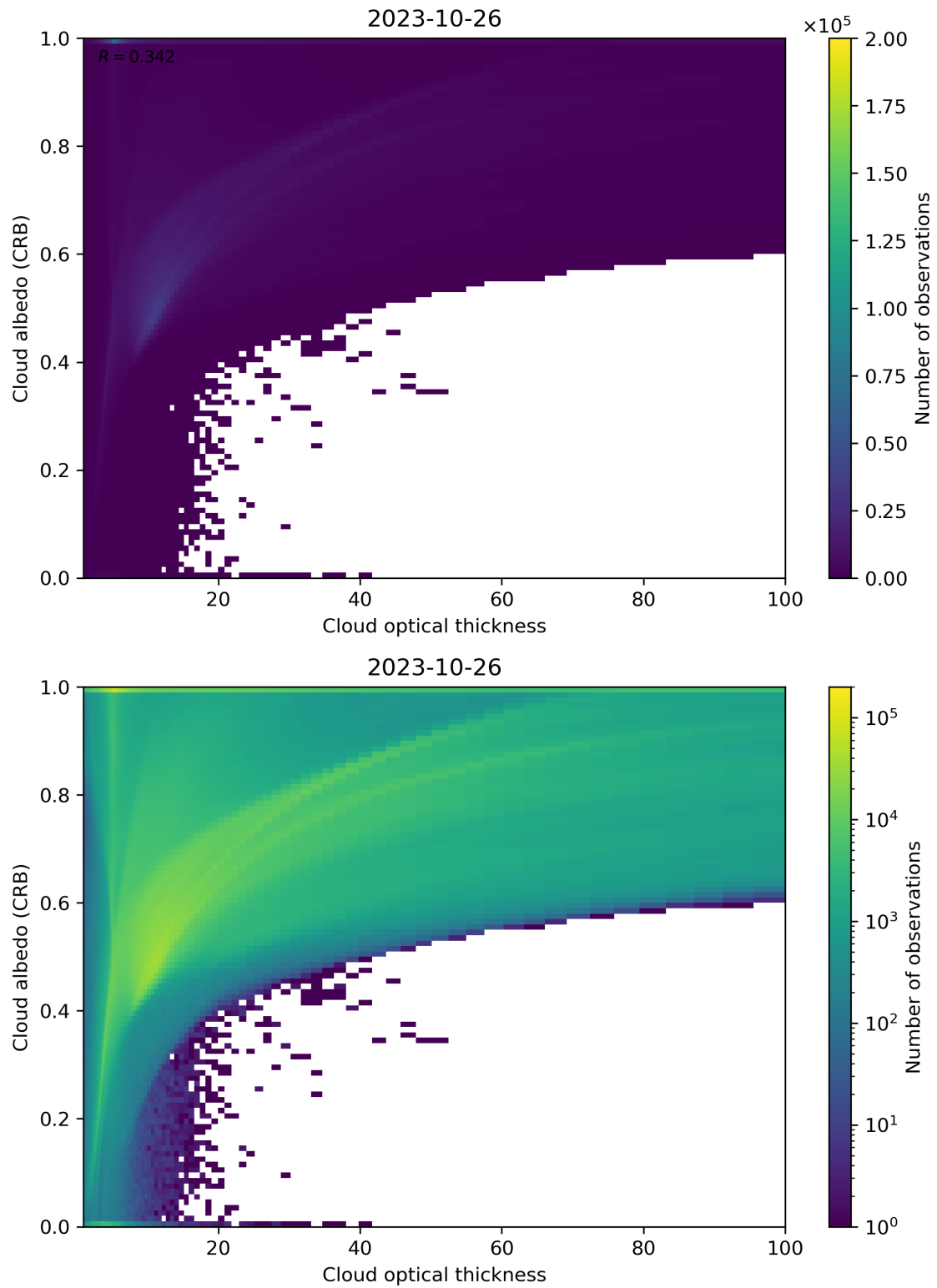
Figure 82: Scatter density plot of “Cloud optical thickness” against “Cloud albedo (CRB)” for 2023-10-25 to 2023-10-27.
