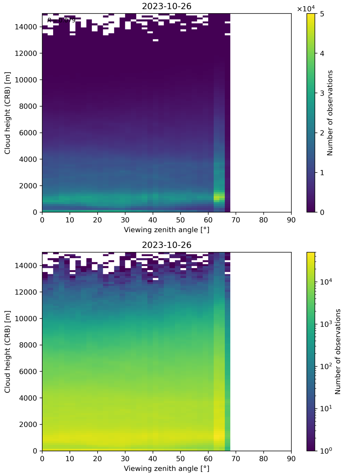
Figure 110: Scatter density plot of “Viewing zenith angle” against “Cloud height (CRB)” for 2023-10-25 to 2023-10-27.
