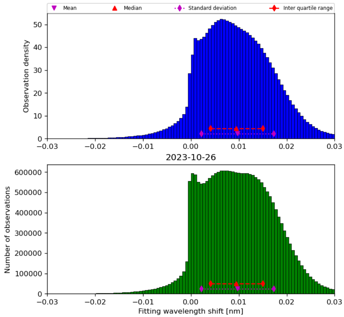
Figure 49: Histogram of “Fitting wavelength shift” for 2023-10-25 to 2023-10-27
