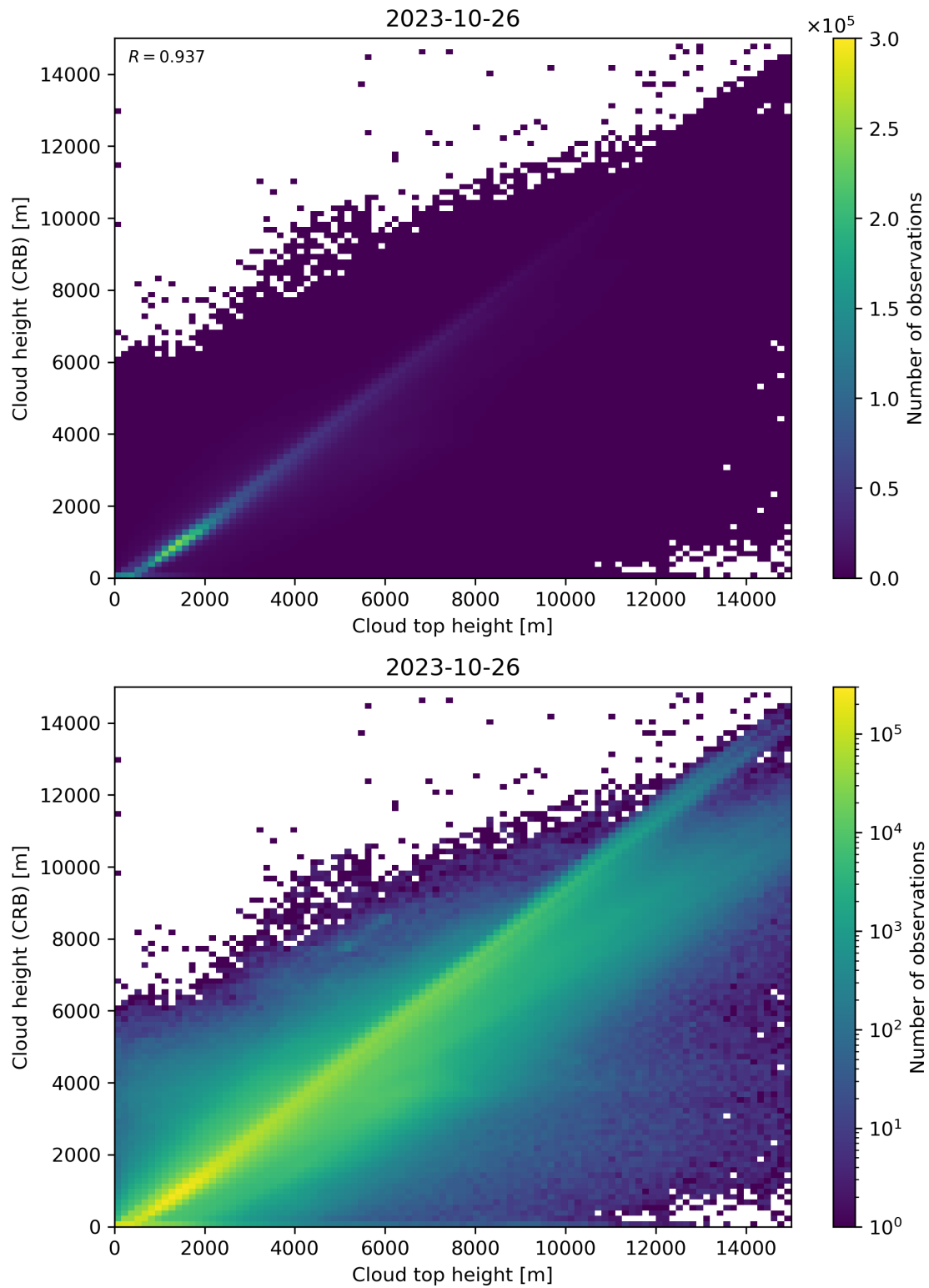
Figure 89: Scatter density plot of “Cloud top height” against “Cloud height (CRB)” for 2023-10-25 to 2023-10-27.
