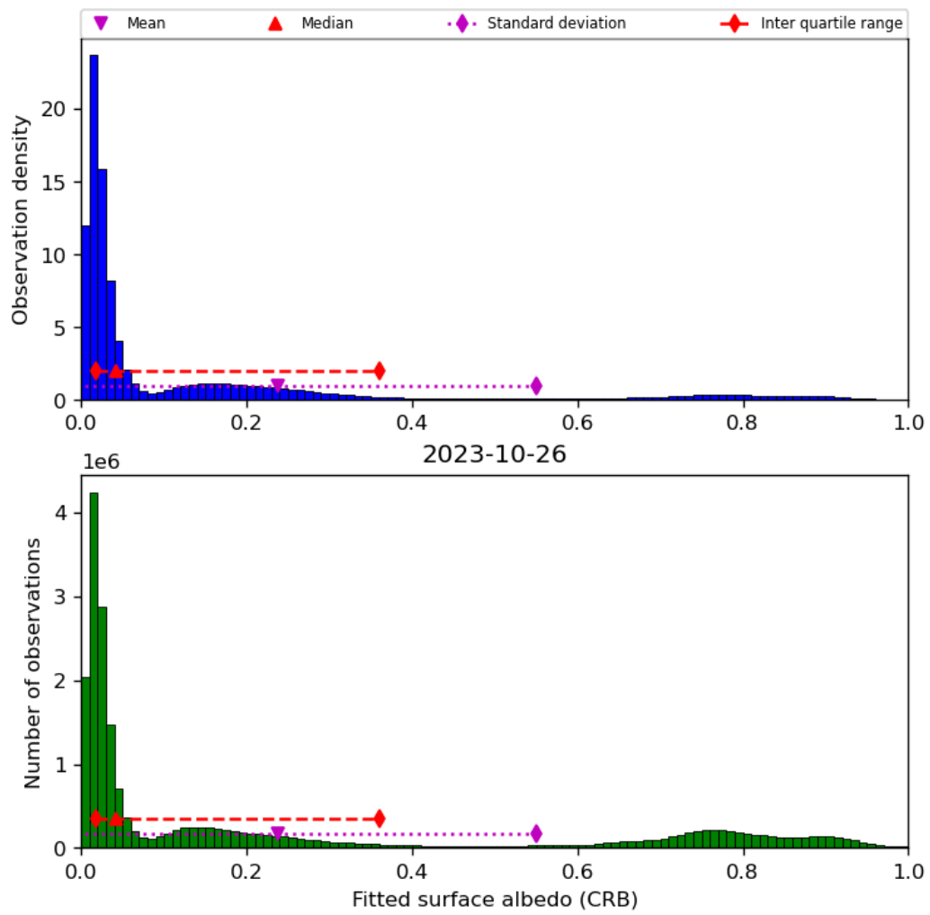
Figure 46: Histogram of “Fitted surface albedo (CRB)” for 2023-10-25 to 2023-10-27
