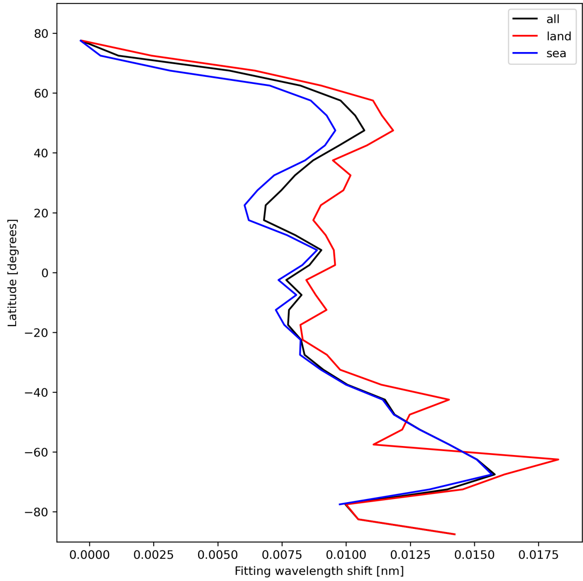
Figure 33: Zonal average of “Fitting wavelength shift” for 2023-10-25 to 2023-10-27.
