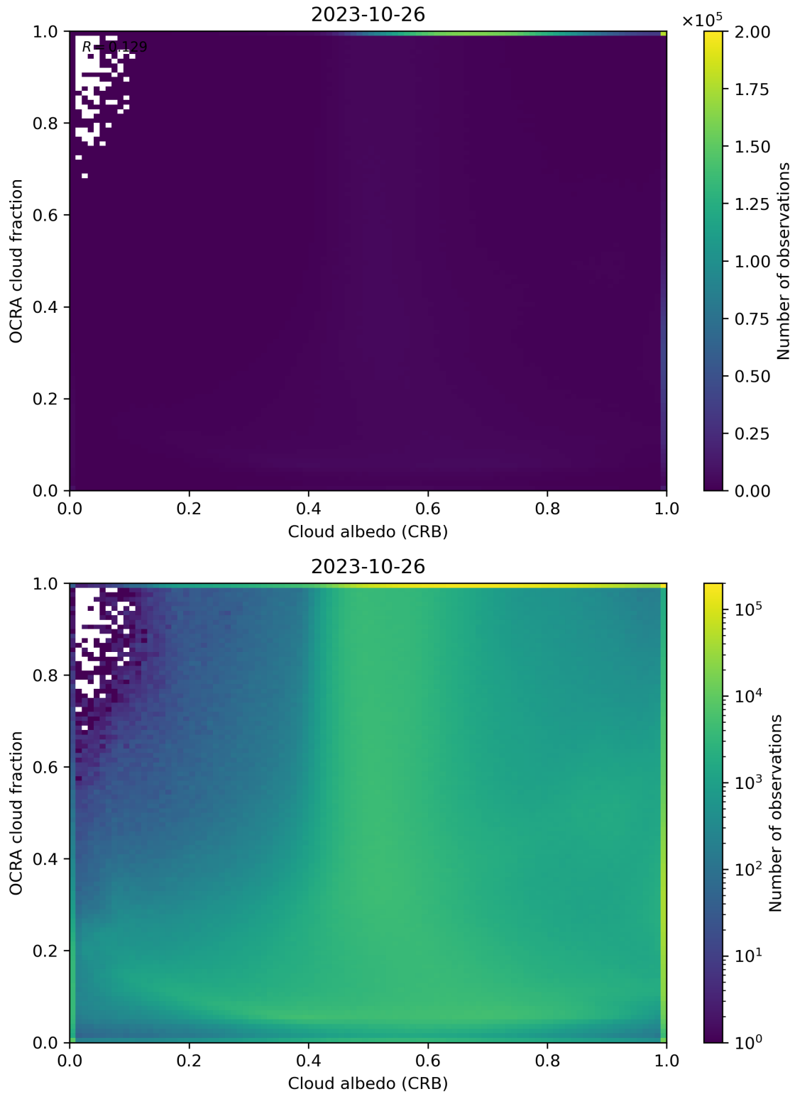
Figure 70: Scatter density plot of “Cloud albedo (CRB)” against “OCRA cloud fraction” for 2023-10-25 to 2023-10-27.
