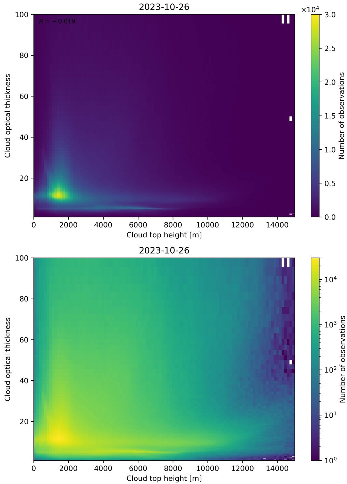
Figure 90: Scatter density plot of “Cloud top height” against “Cloud optical thickness” for 2023-10-25 to 2023-10-27.
