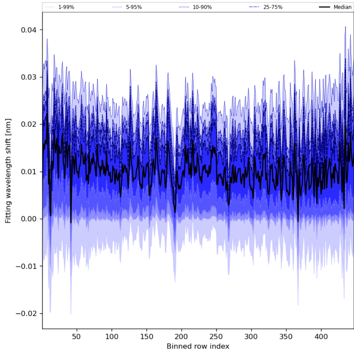
Figure 65: Along track statistics of “Fitting wavelength shift” for 2023-10-25 to 2023-10-27
