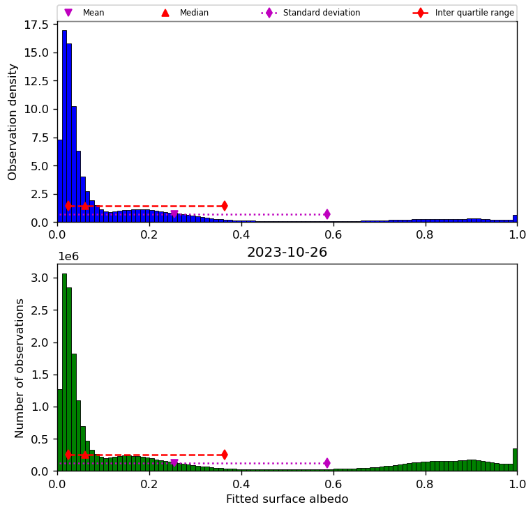
Figure 45: Histogram of “Fitted surface albedo” for 2023-10-25 to 2023-10-27
