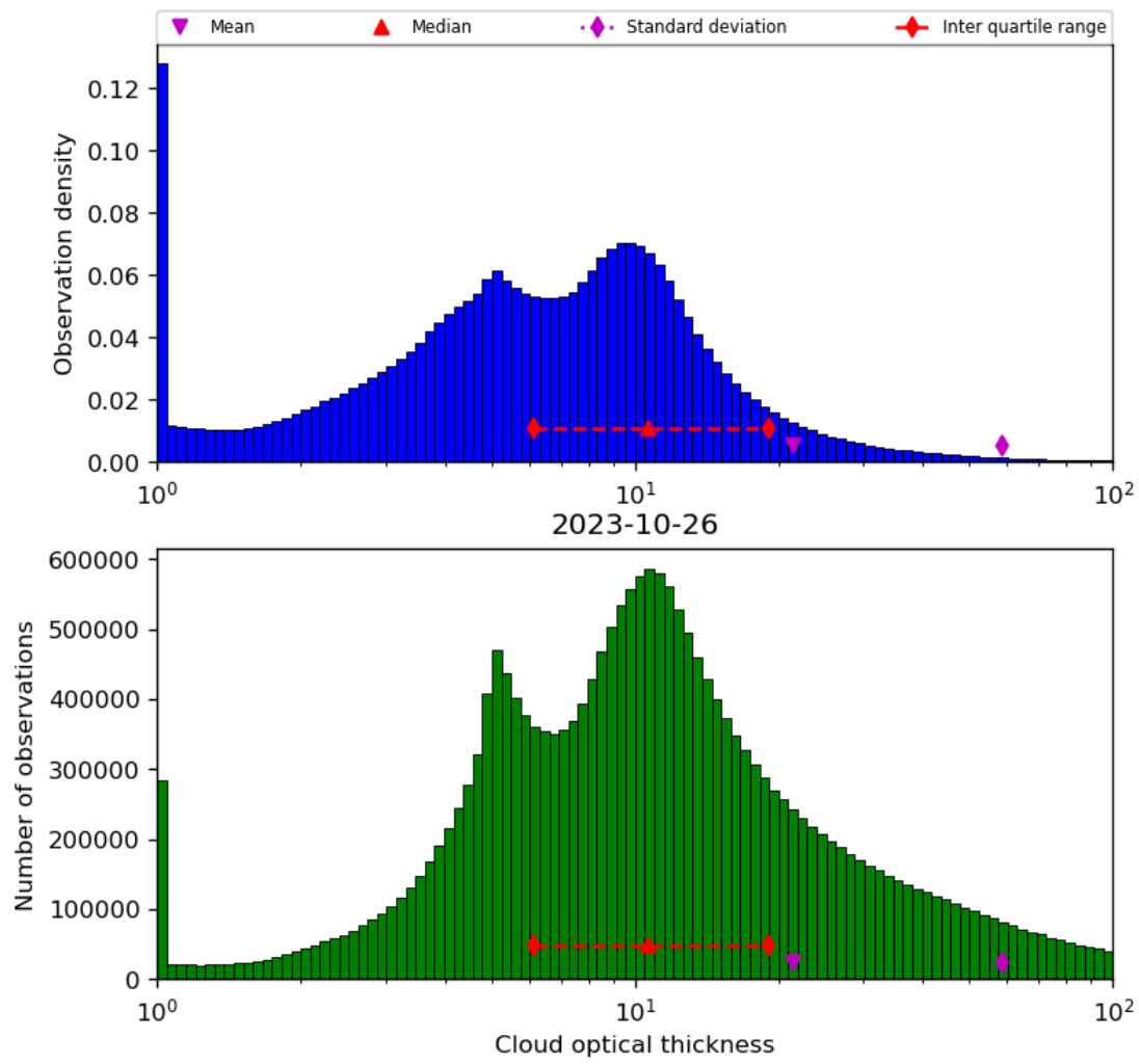
Figure 41: Histogram of “Cloud optical thickness” for 2023-10-25 to 2023-10-27
