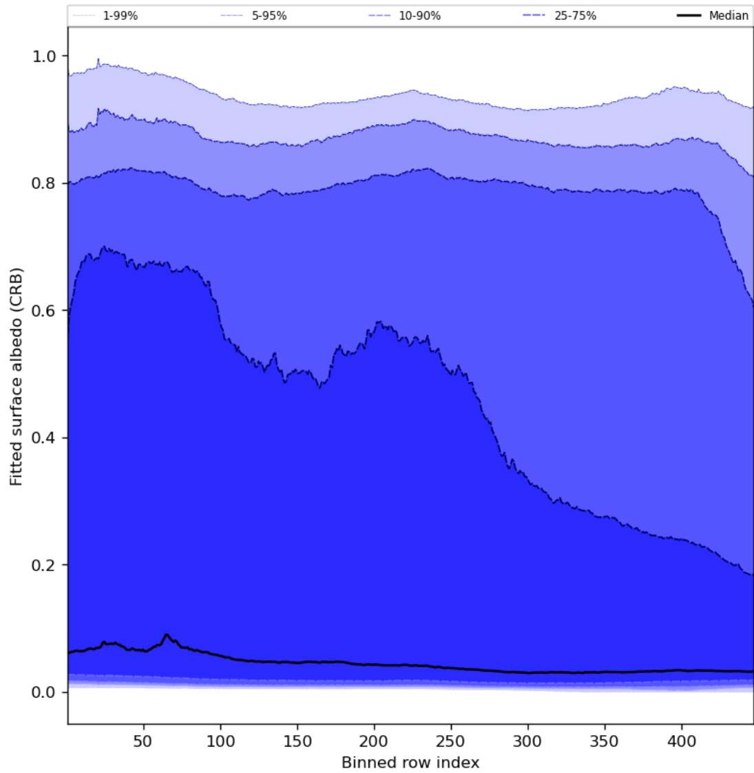
Figure 62: Along track statistics of “Fitted surface albedo (CRB)” for 2023-10-25 to 2023-10-27
