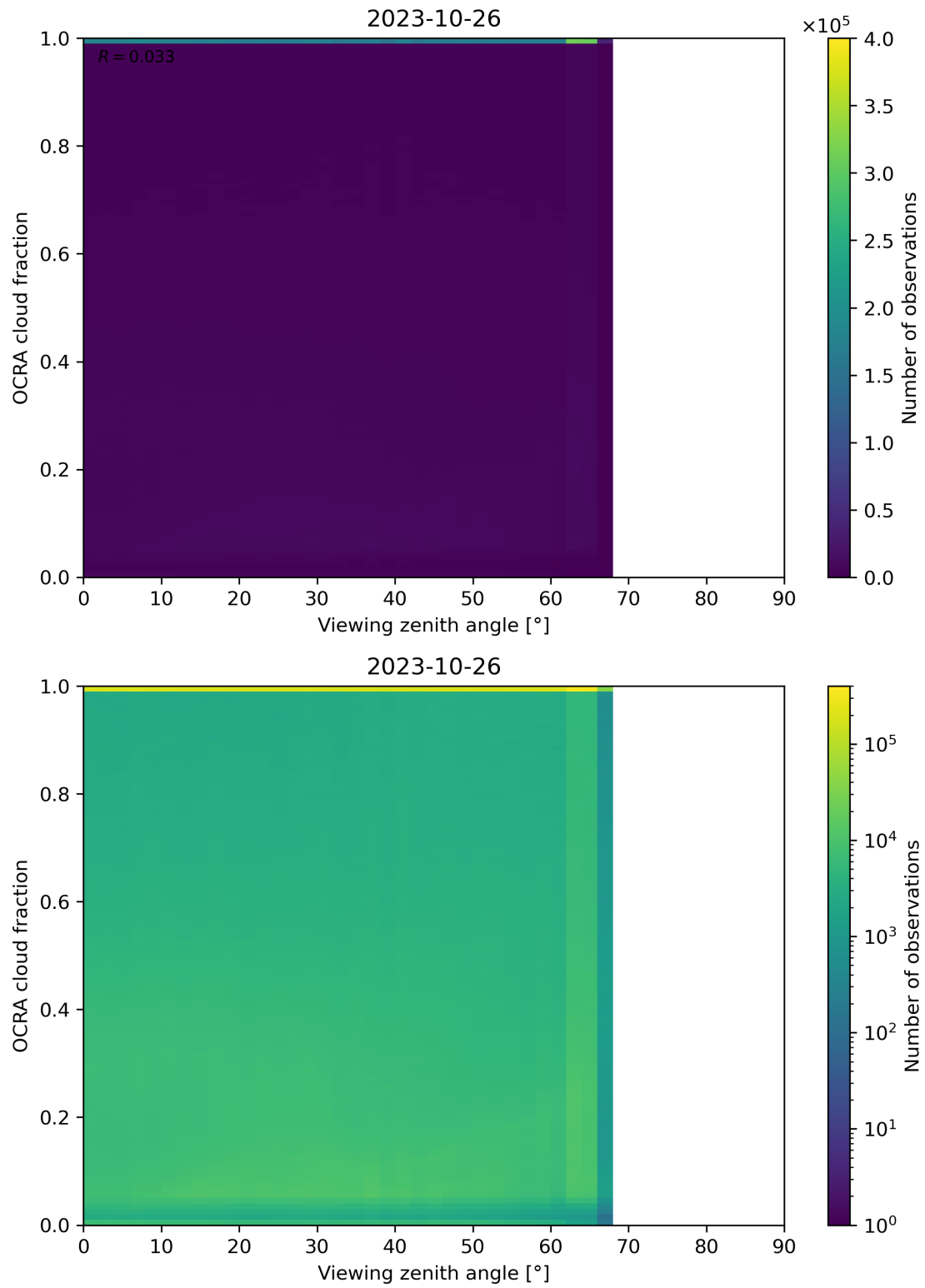
Figure 108: Scatter density plot of “Viewing zenith angle” against “OCRA cloud fraction” for 2023-10-25 to 2023-10-27.
