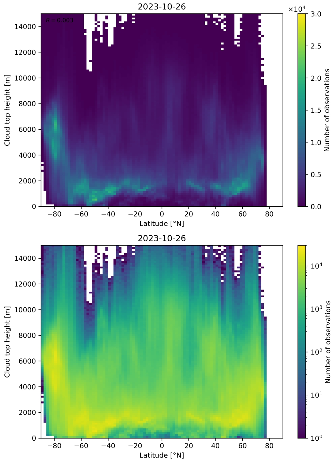
Figure 97: Scatter density plot of “Latitude” against “Cloud top height” for 2023-10-25 to 2023-10-27.
