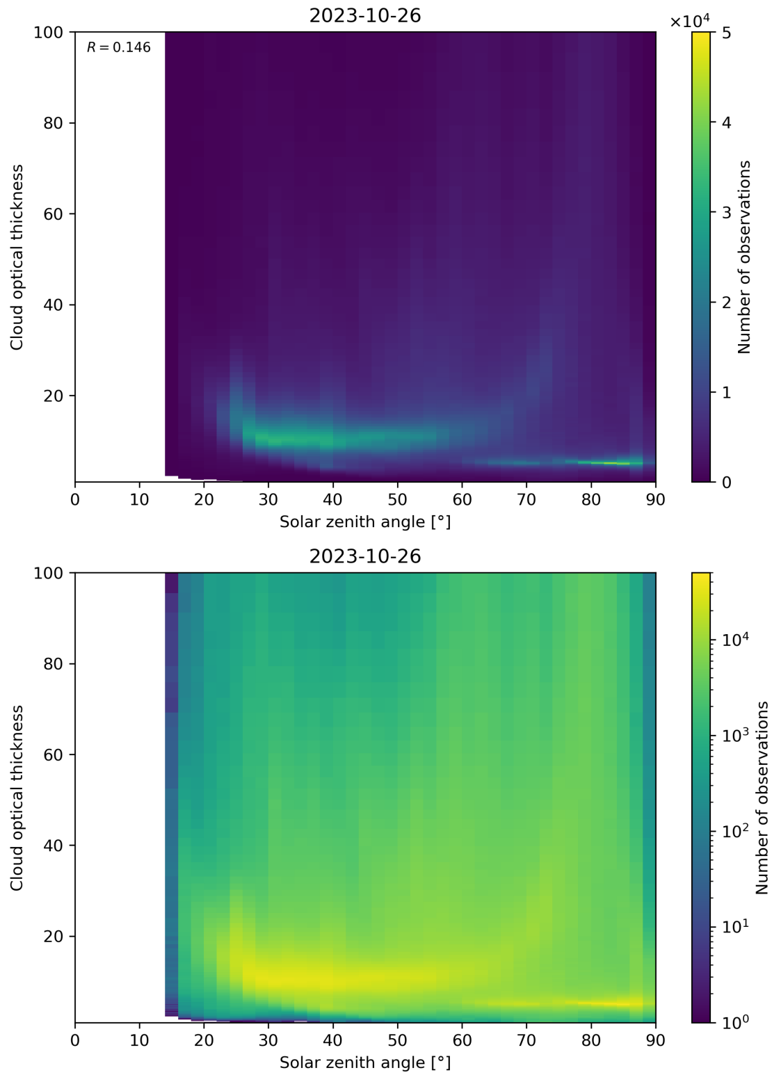
Figure 103: Scatter density plot of “Solar zenith angle” against “Cloud optical thickness” for 2023-10-25 to 2023-10-27.
