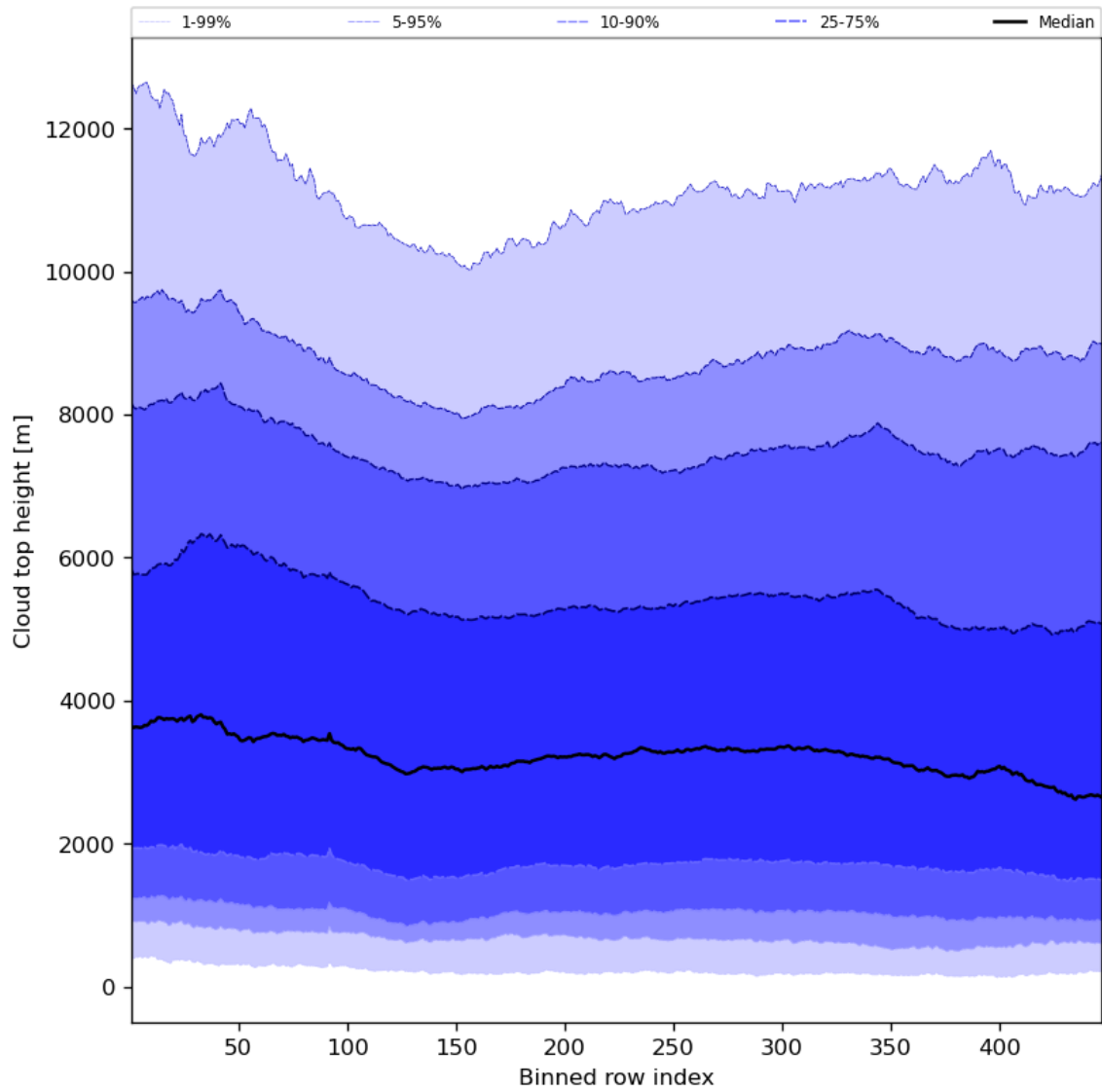
Figure 56: Along track statistics of “Cloud top height” for 2023-10-25 to 2023-10-27
