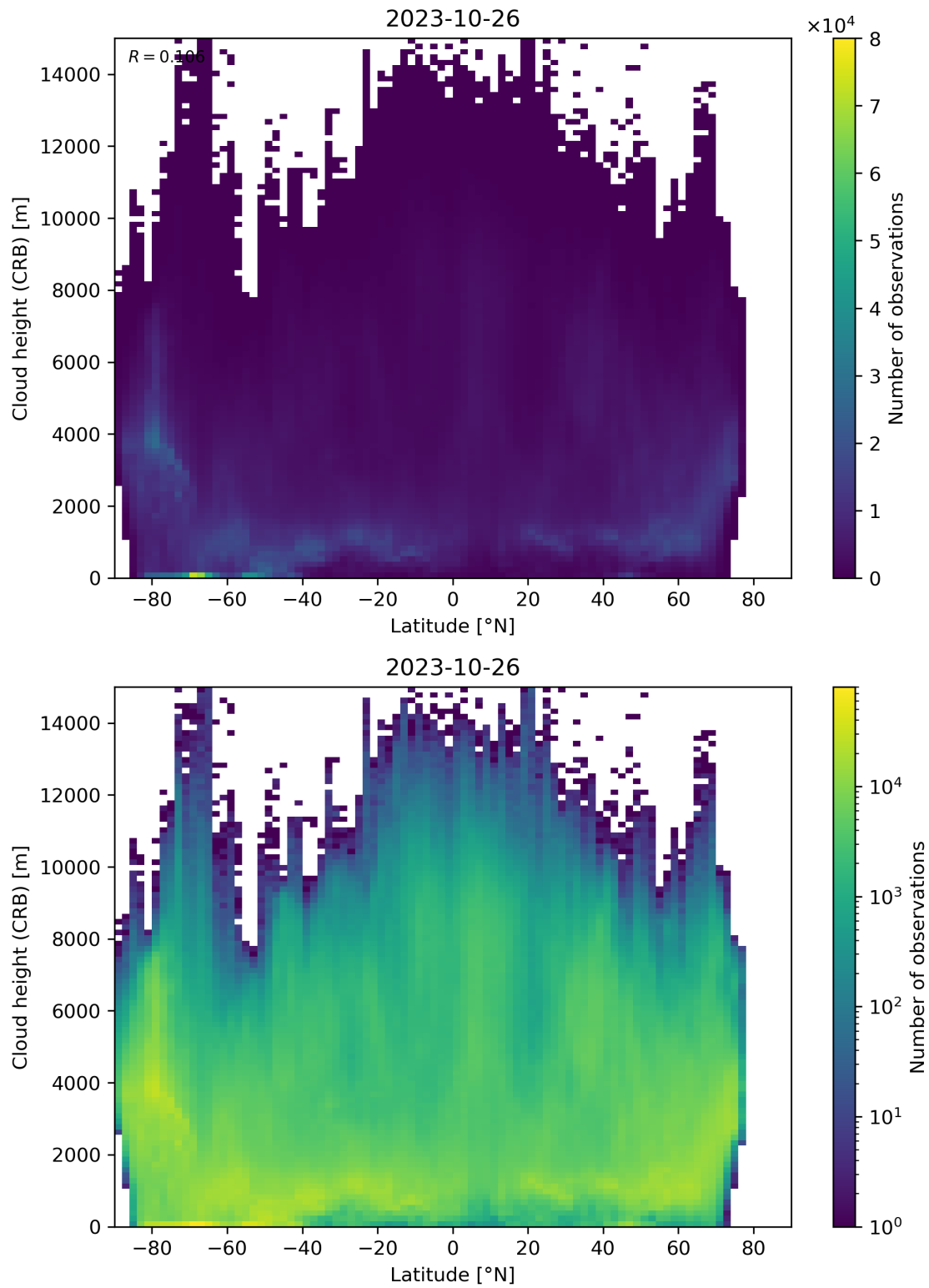
Figure 95: Scatter density plot of “Latitude” against “Cloud height (CRB)” for 2023-10-25 to 2023-10-27.
