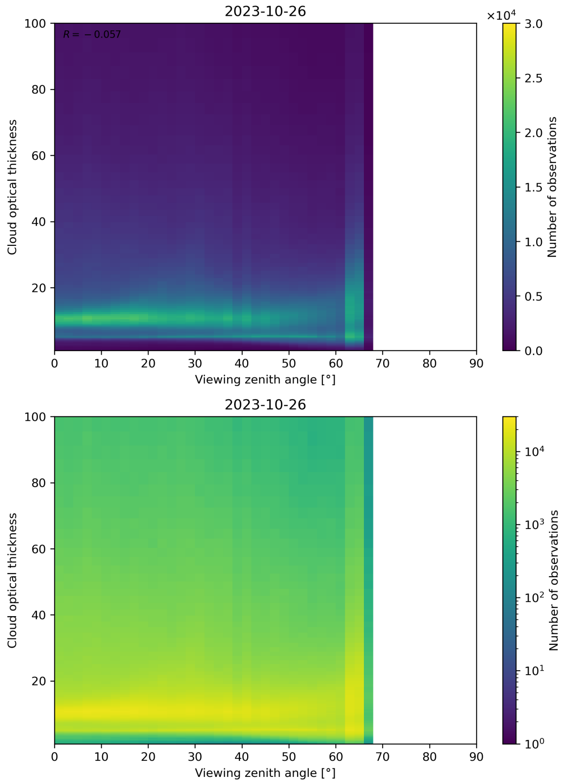
Figure 111: Scatter density plot of “Viewing zenith angle” against “Cloud optical thickness” for 2023-10-25 to 2023-10-27.
