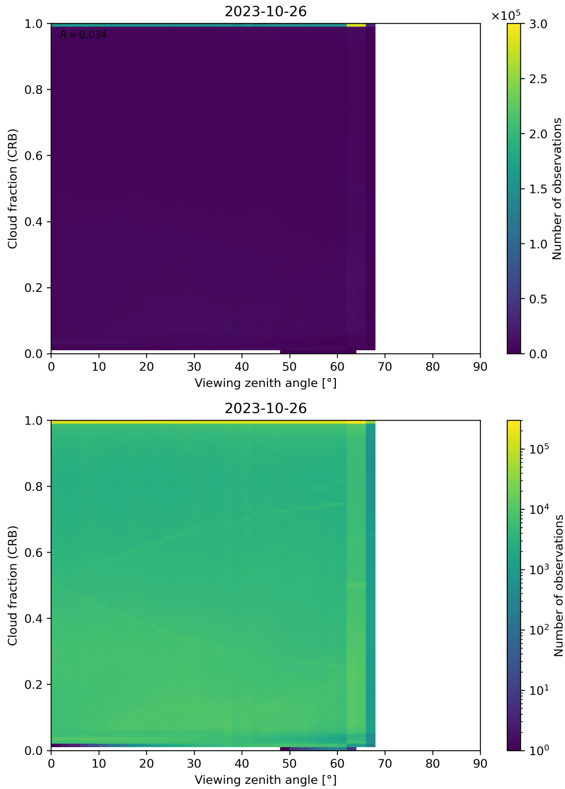
Figure 109: Scatter density plot of “Viewing zenith angle” against “Cloud fraction (CRB)” for 2023-10-25 to 2023-10-27.
