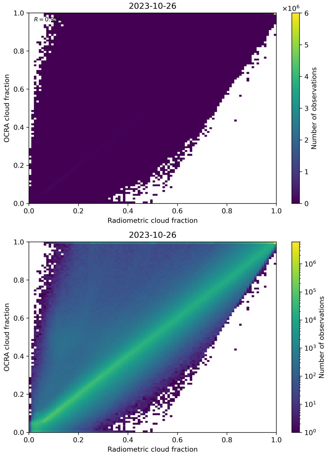
Figure 72: Scatter density plot of “Radiometric cloud fraction” against “OCRA cloud fraction” for 2023-10-25 to 2023-10-27.
