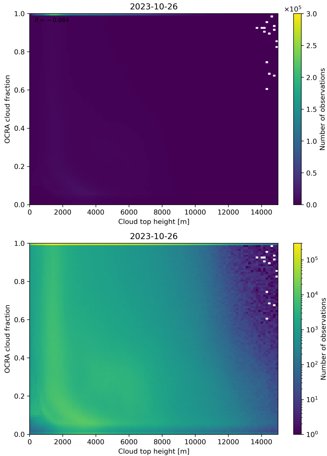
Figure 87: Scatter density plot of “Cloud top height” against “OCRA cloud fraction” for 2023-10-25 to 2023-10-27.
