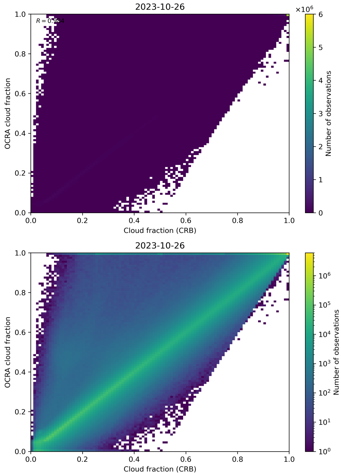
Figure 78: Scatter density plot of “Cloud fraction (CRB)” against “OCRA cloud fraction” for 2023-10-25 to 2023-10-27.
