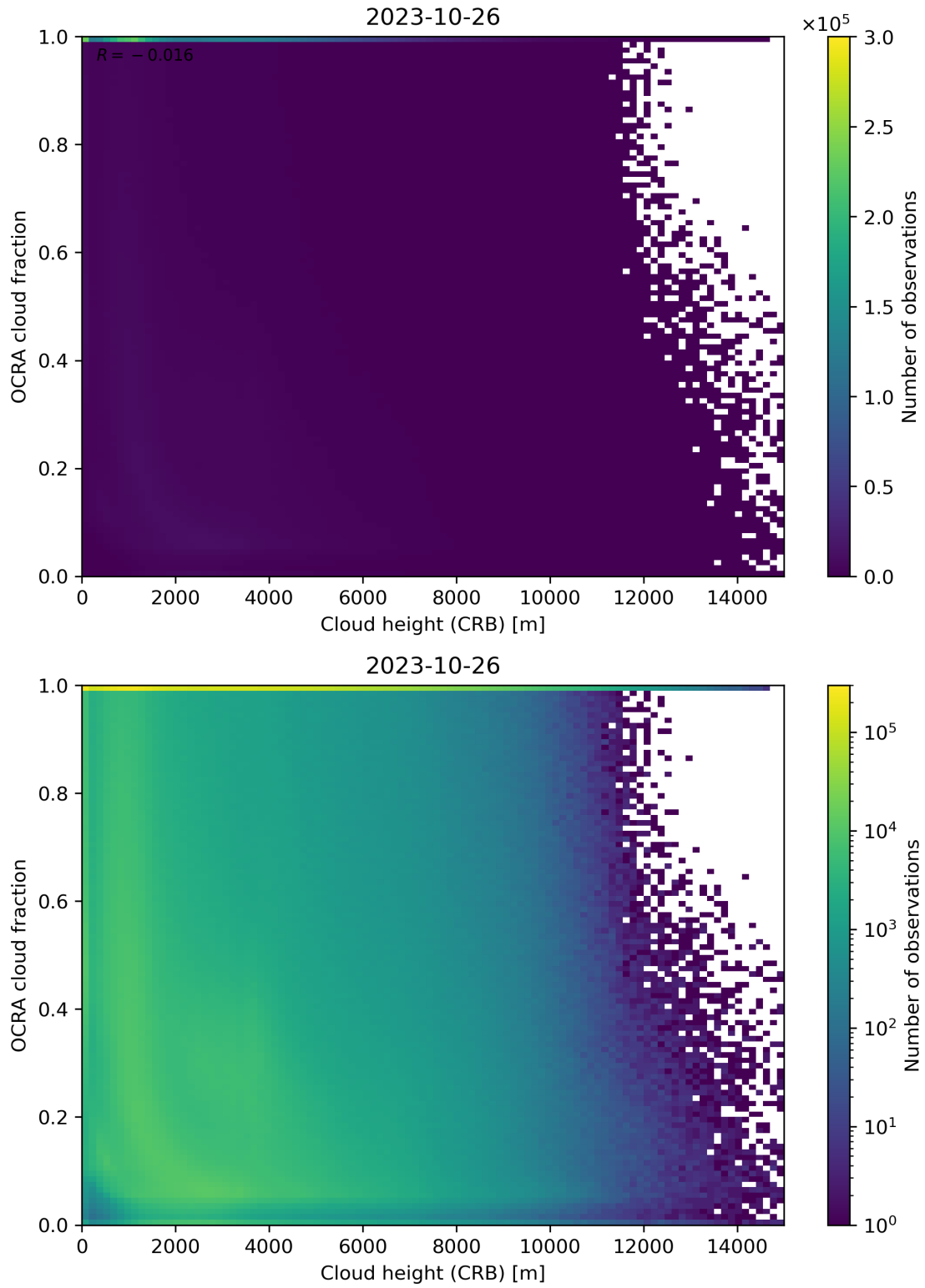
Figure 81: Scatter density plot of “Cloud height (CRB)” against “OCRA cloud fraction” for 2023-10-25 to 2023-10-27.
