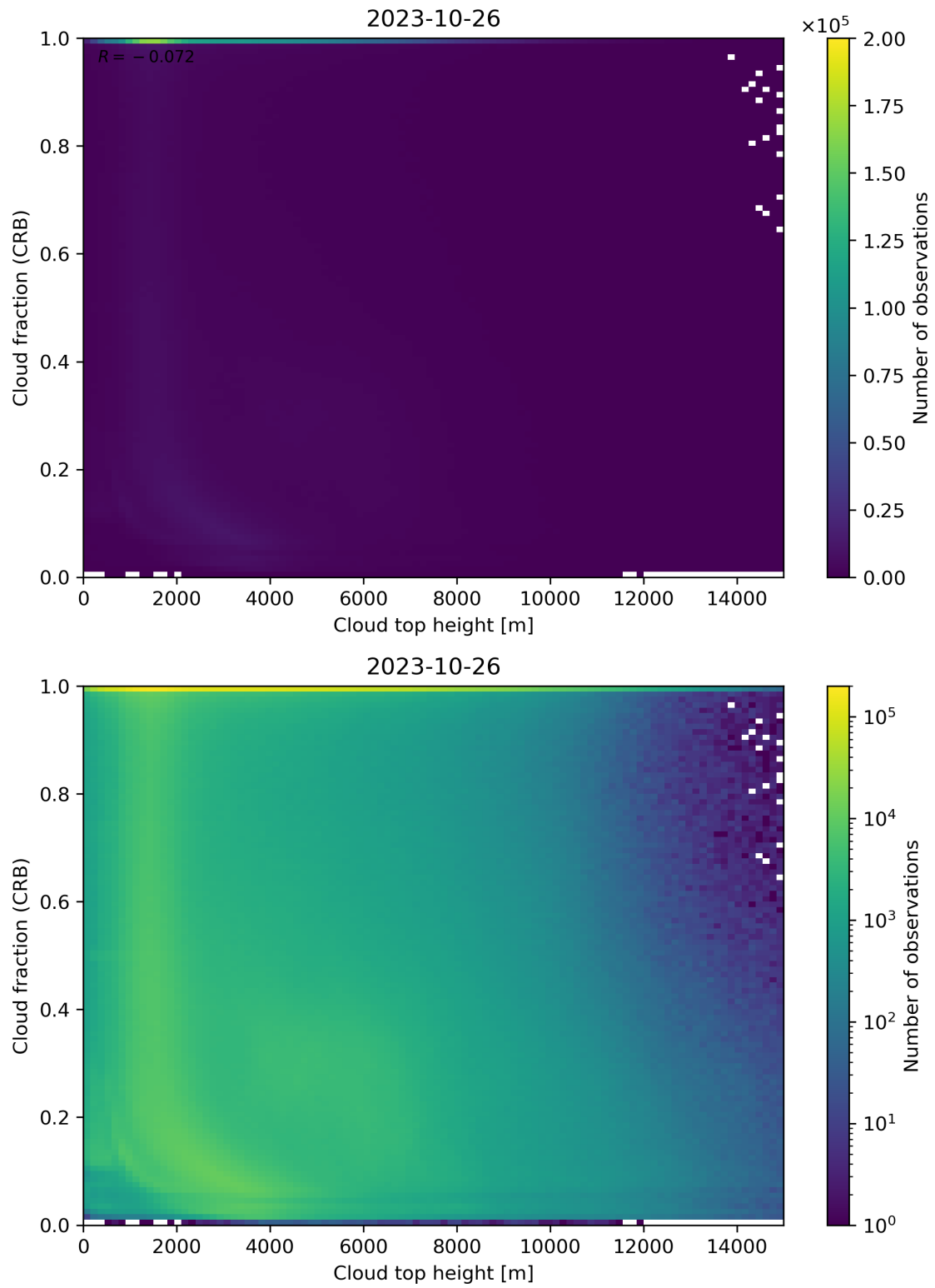
Figure 88: Scatter density plot of “Cloud top height” against “Cloud fraction (CRB)” for 2023-10-25 to 2023-10-27.
