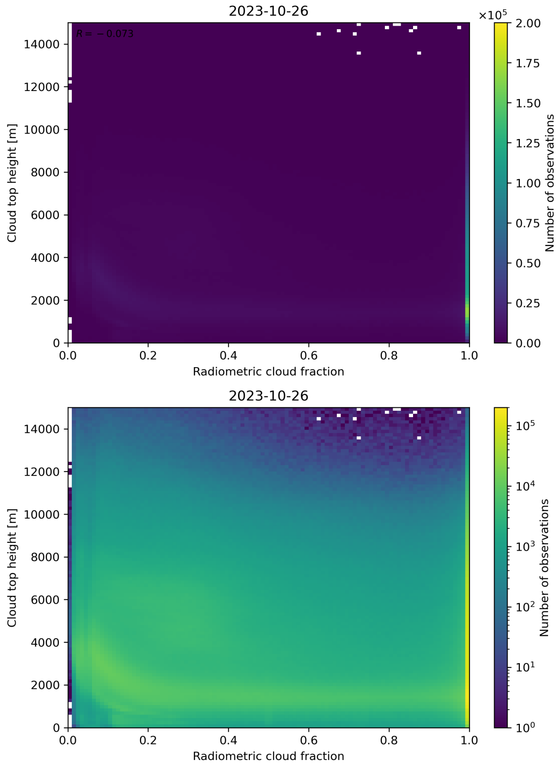
Figure 76: Scatter density plot of “Radiometric cloud fraction” against “Cloud top height” for 2023-10-25 to 2023-10-27.
