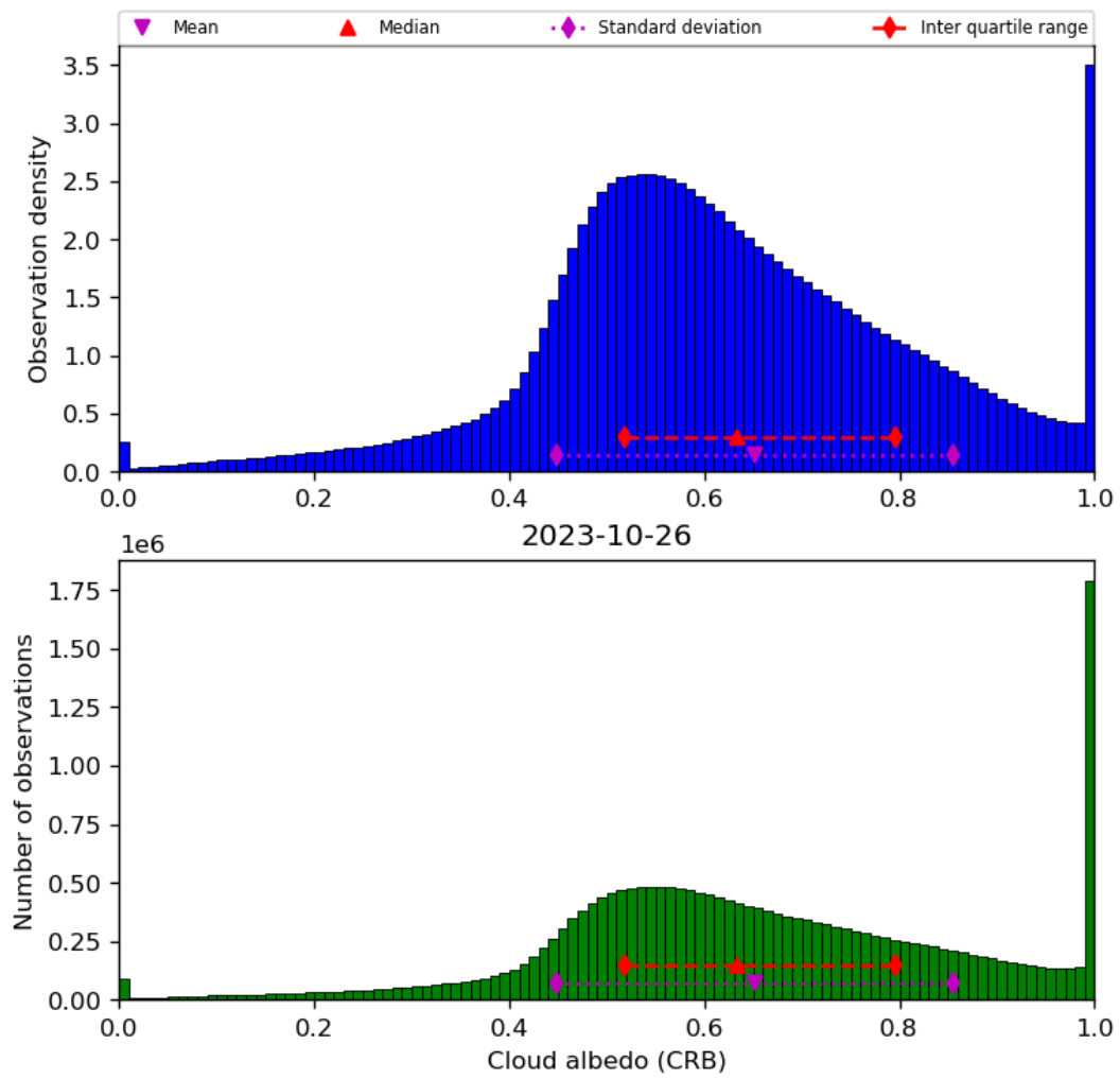
Figure 44: Histogram of “Cloud albedo (CRB)” for 2023-10-25 to 2023-10-27
