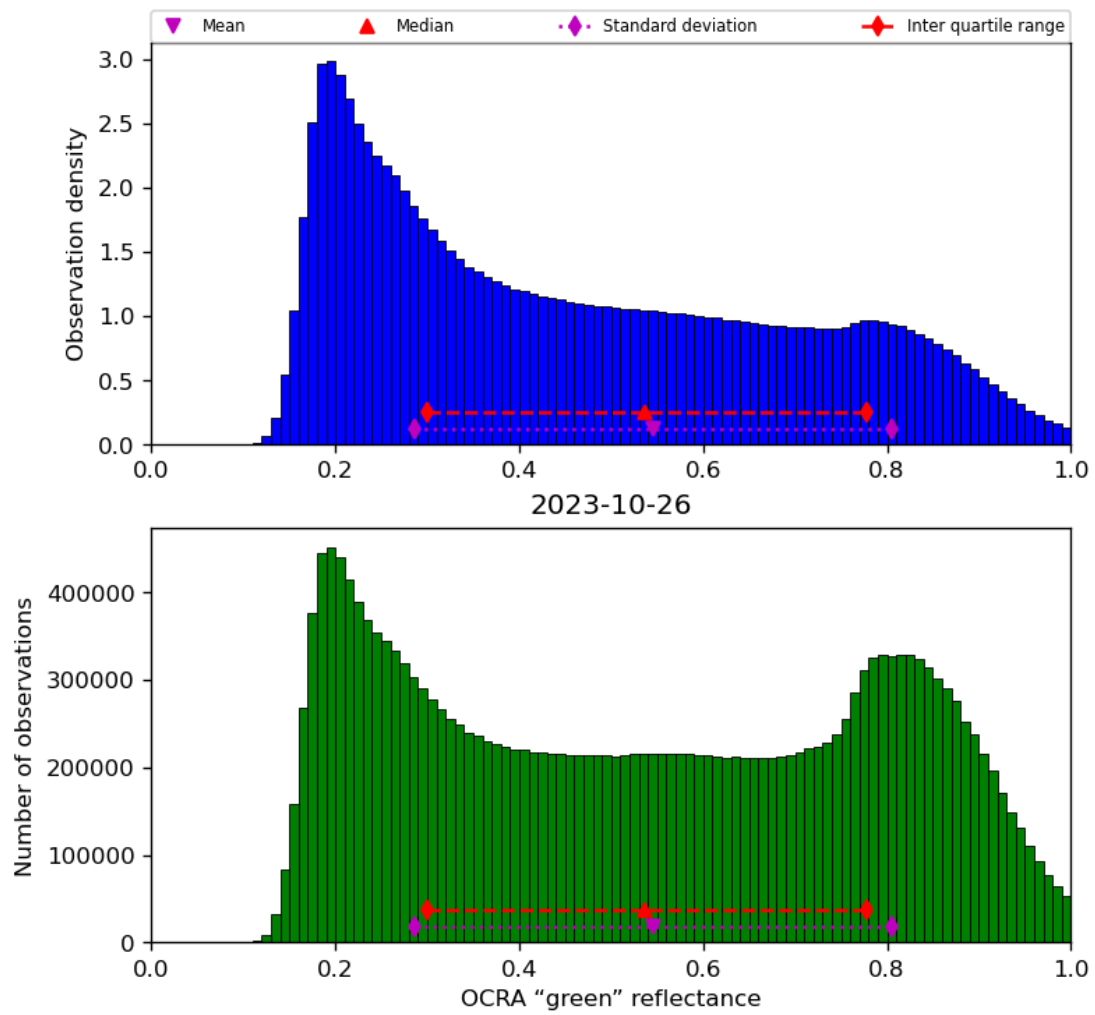
Figure 52: Histogram of “OCRA “green” reflectance” for 2023-10-25 to 2023-10-27
