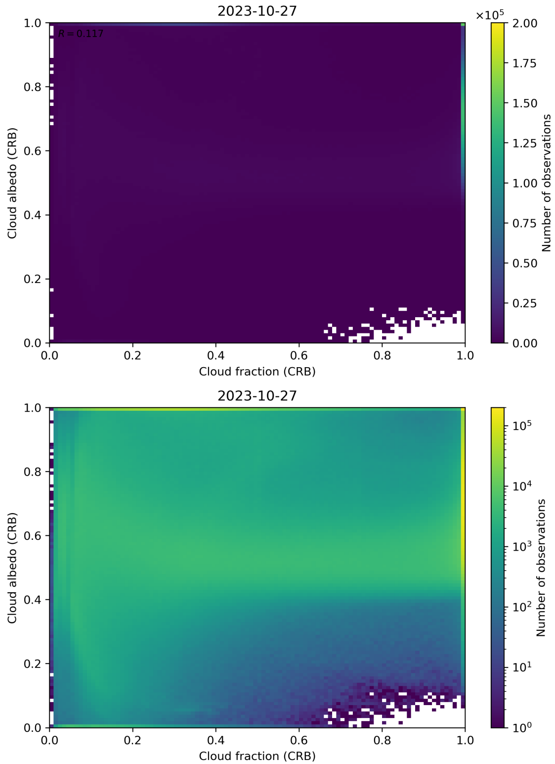
Figure 77: Scatter density plot of “Cloud fraction (CRB)” against “Cloud albedo (CRB)” for 2023-10-27 to 2023-10-28.
