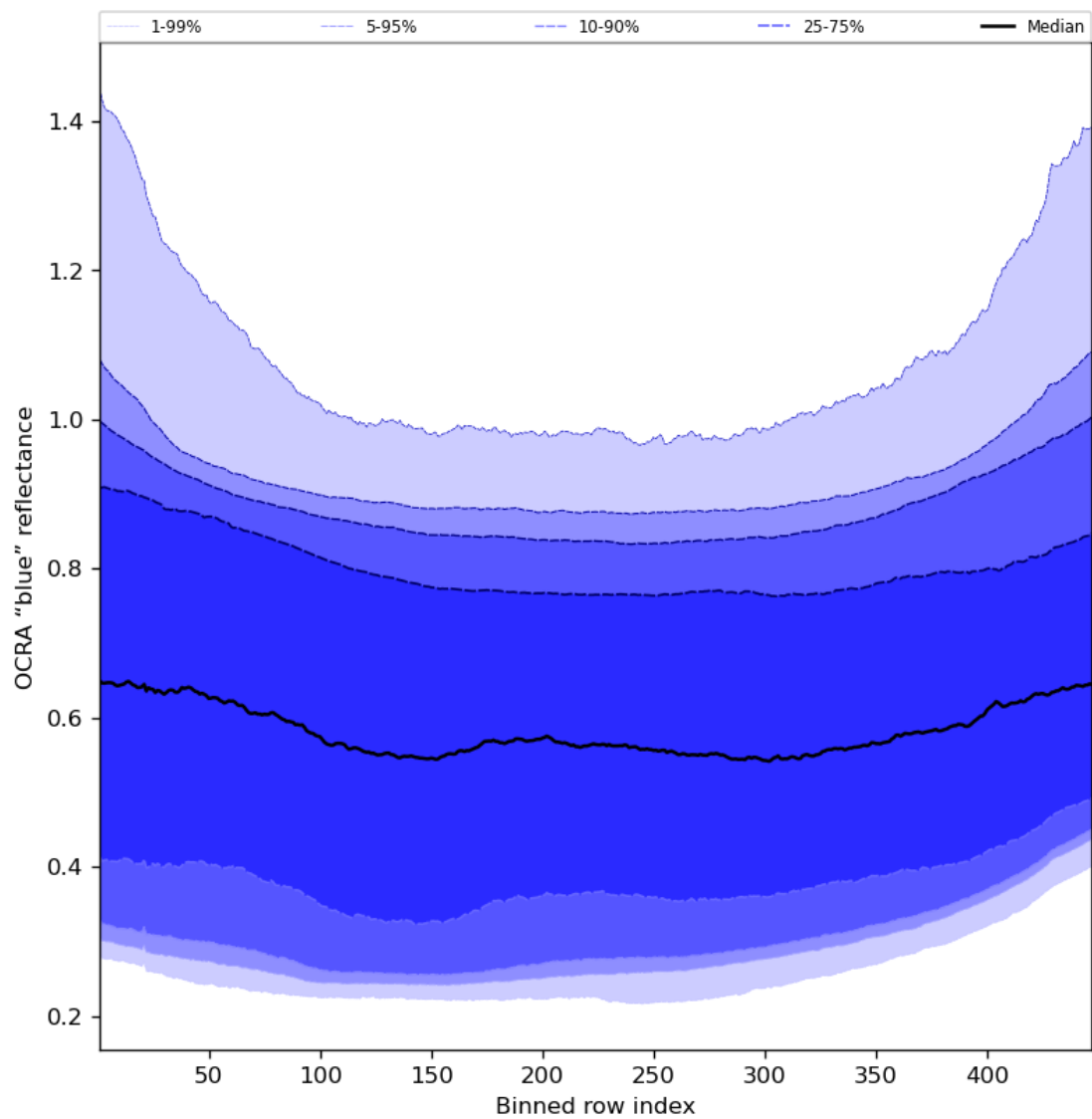
Figure 67: Along track statistics of “OCRA “blue” reflectance” for 2023-10-27 to 2023-10-28
