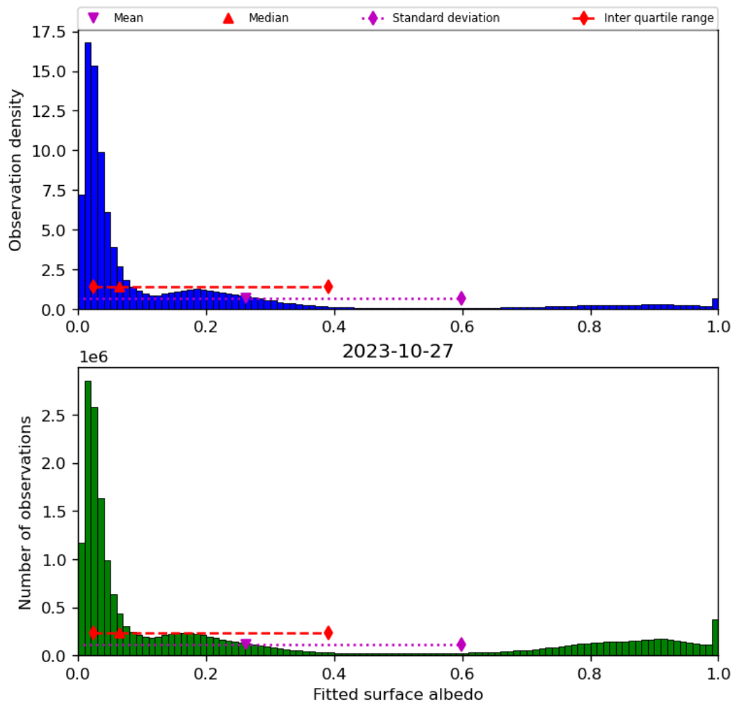
Figure 45: Histogram of “Fitted surface albedo” for 2023-10-27 to 2023-10-28
