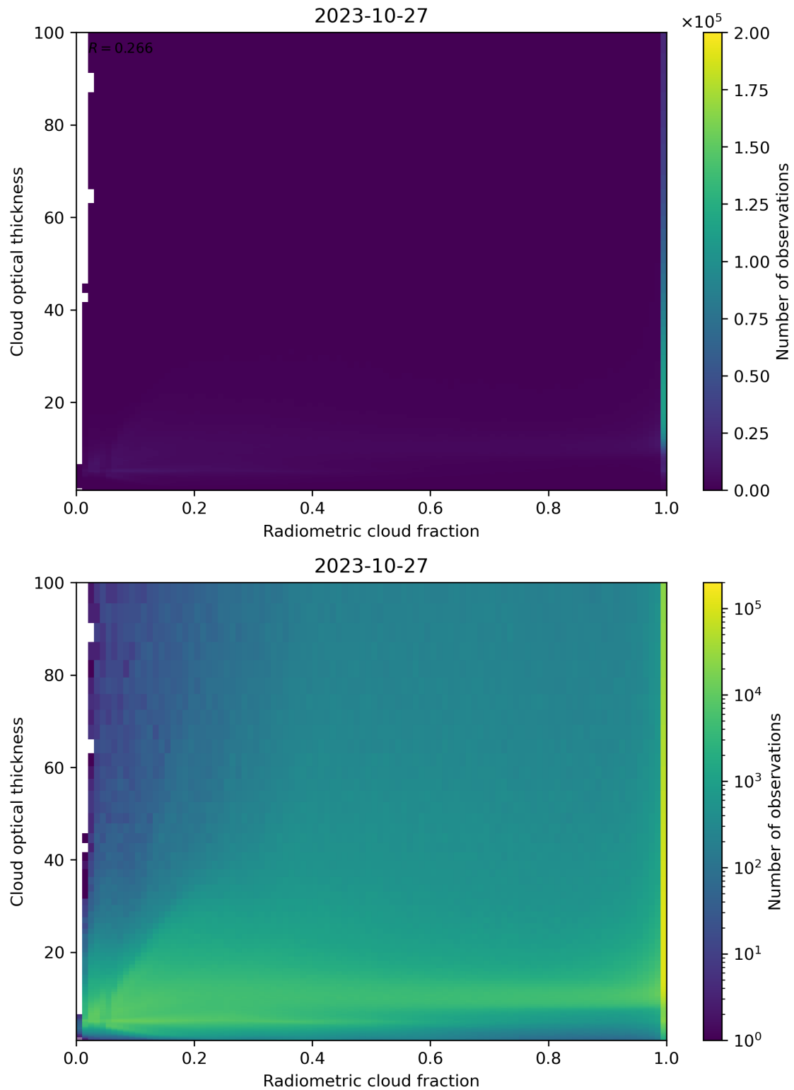
Figure 75: Scatter density plot of “Radiometric cloud fraction” against “Cloud optical thickness” for 2023-10-27 to 2023-10-28.
