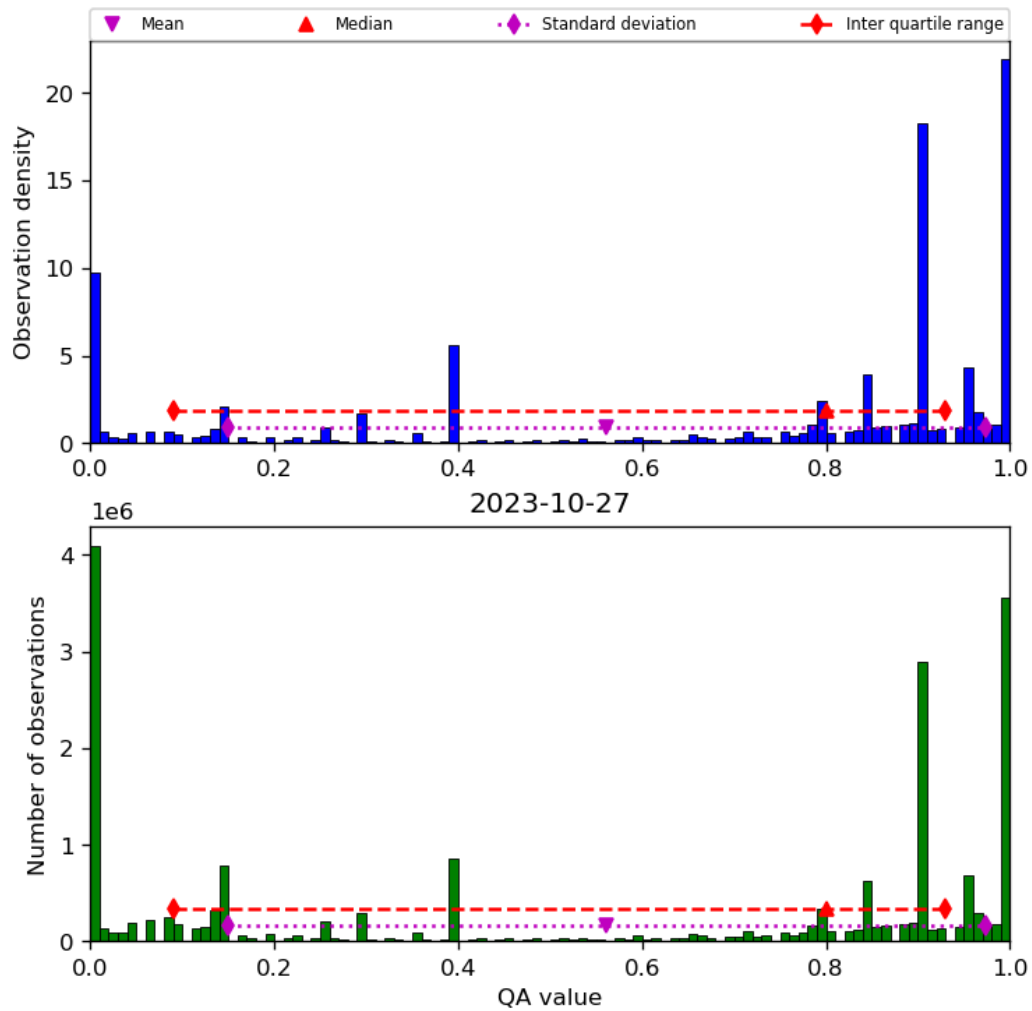
Figure 38: Histogram of “QA value” for 2023-10-27 to 2023-10-28
