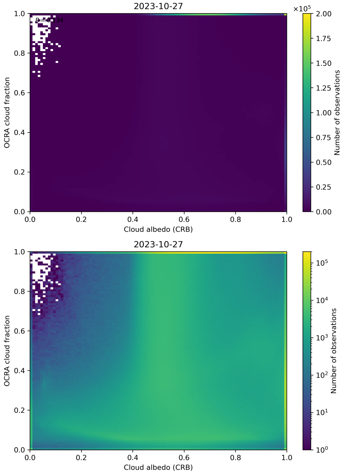
Figure 70: Scatter density plot of “Cloud albedo (CRB)” against “OCRA cloud fraction” for 2023-10-27 to 2023-10-28.
