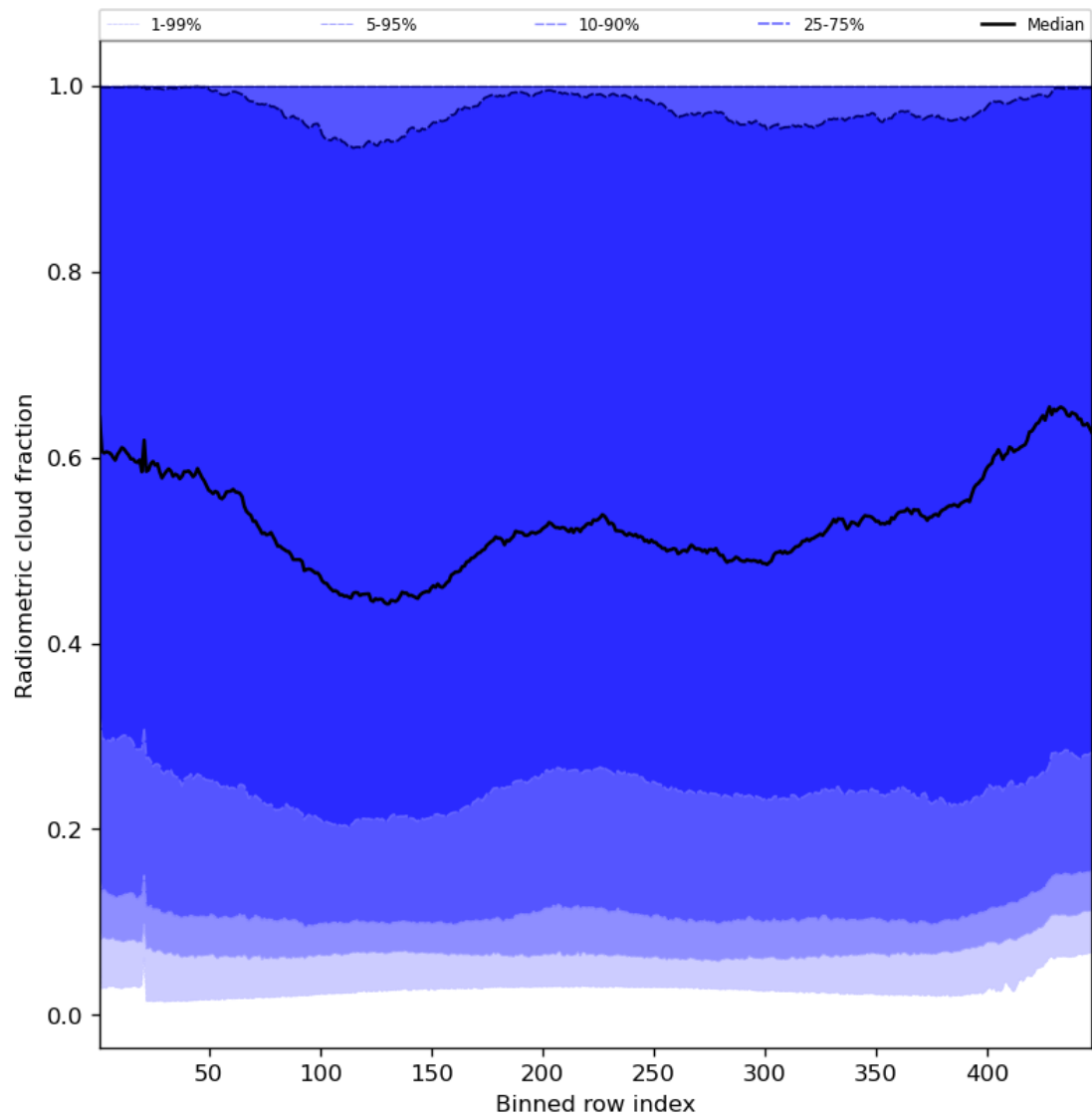
Figure 55: Along track statistics of “Radiometric cloud fraction” for 2023-10-27 to 2023-10-28
