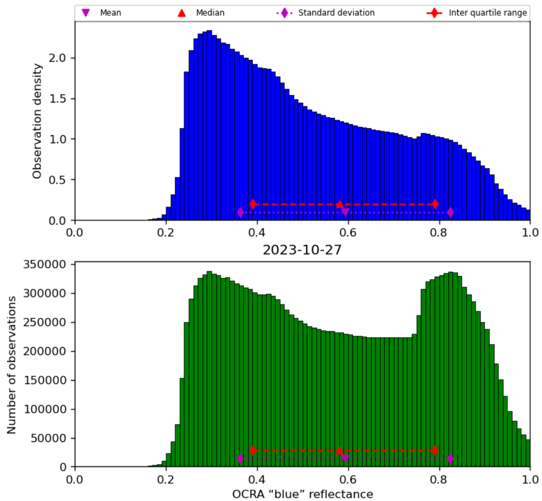
Figure 51: Histogram of “OCRA “blue” reflectance” for 2023-10-27 to 2023-10-28
