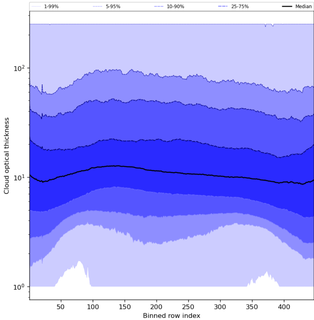
Figure 57: Along track statistics of “Cloud optical thickness” for 2023-10-27 to 2023-10-28
