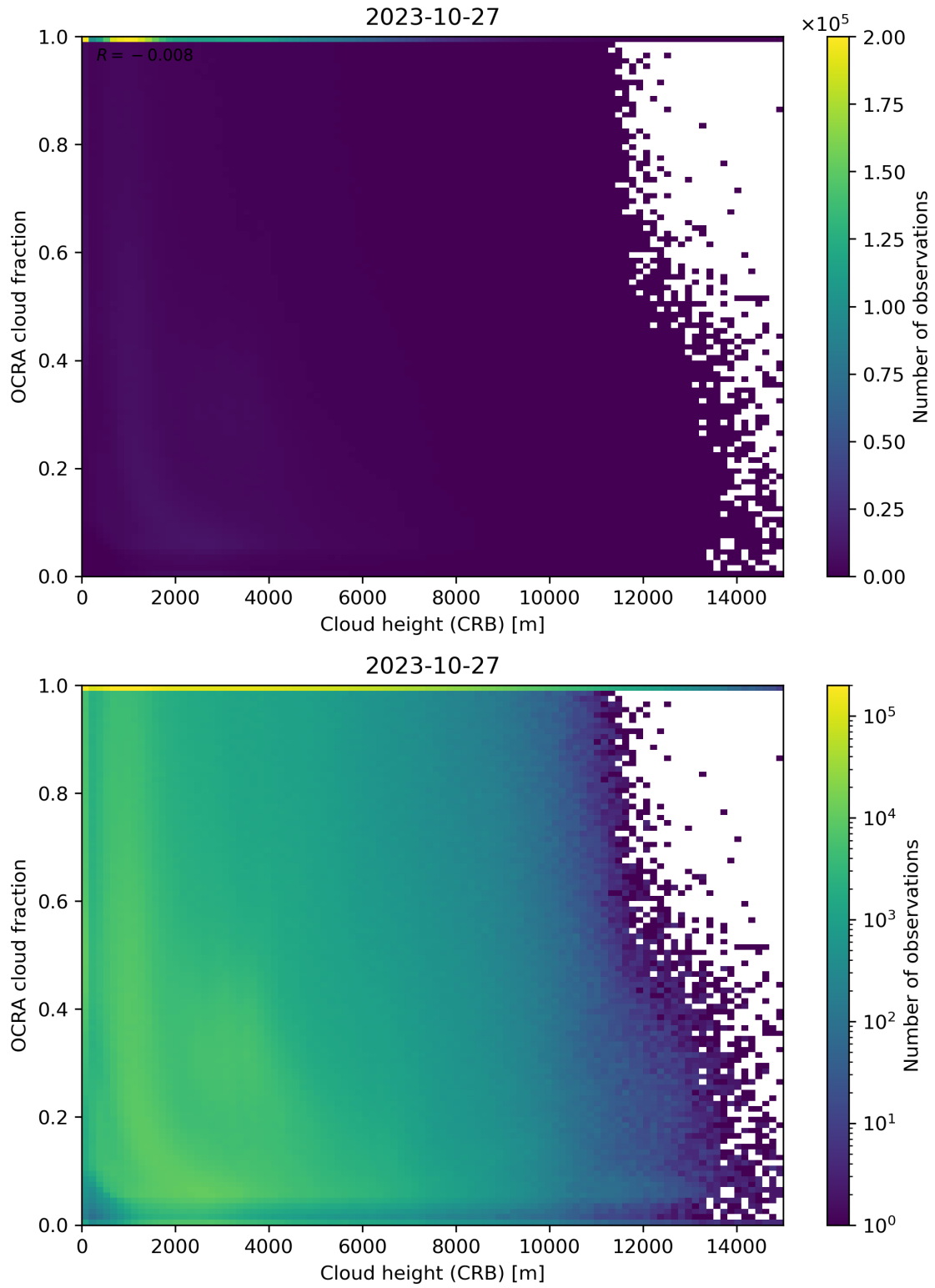
Figure 81: Scatter density plot of “Cloud height (CRB)” against “OCRA cloud fraction” for 2023-10-27 to 2023-10-28.
