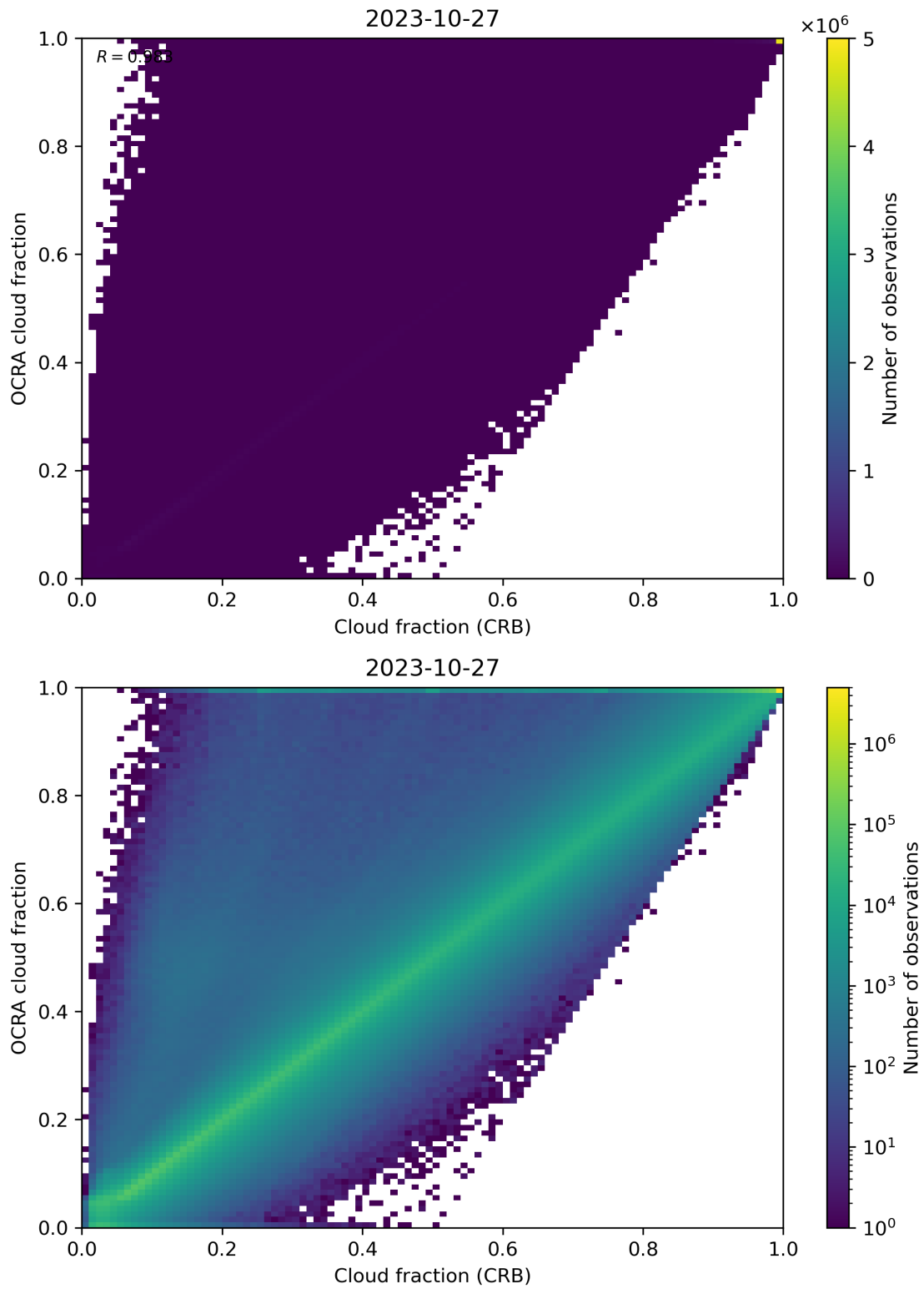
Figure 78: Scatter density plot of “Cloud fraction (CRB)” against “OCRA cloud fraction” for 2023-10-27 to 2023-10-28.
