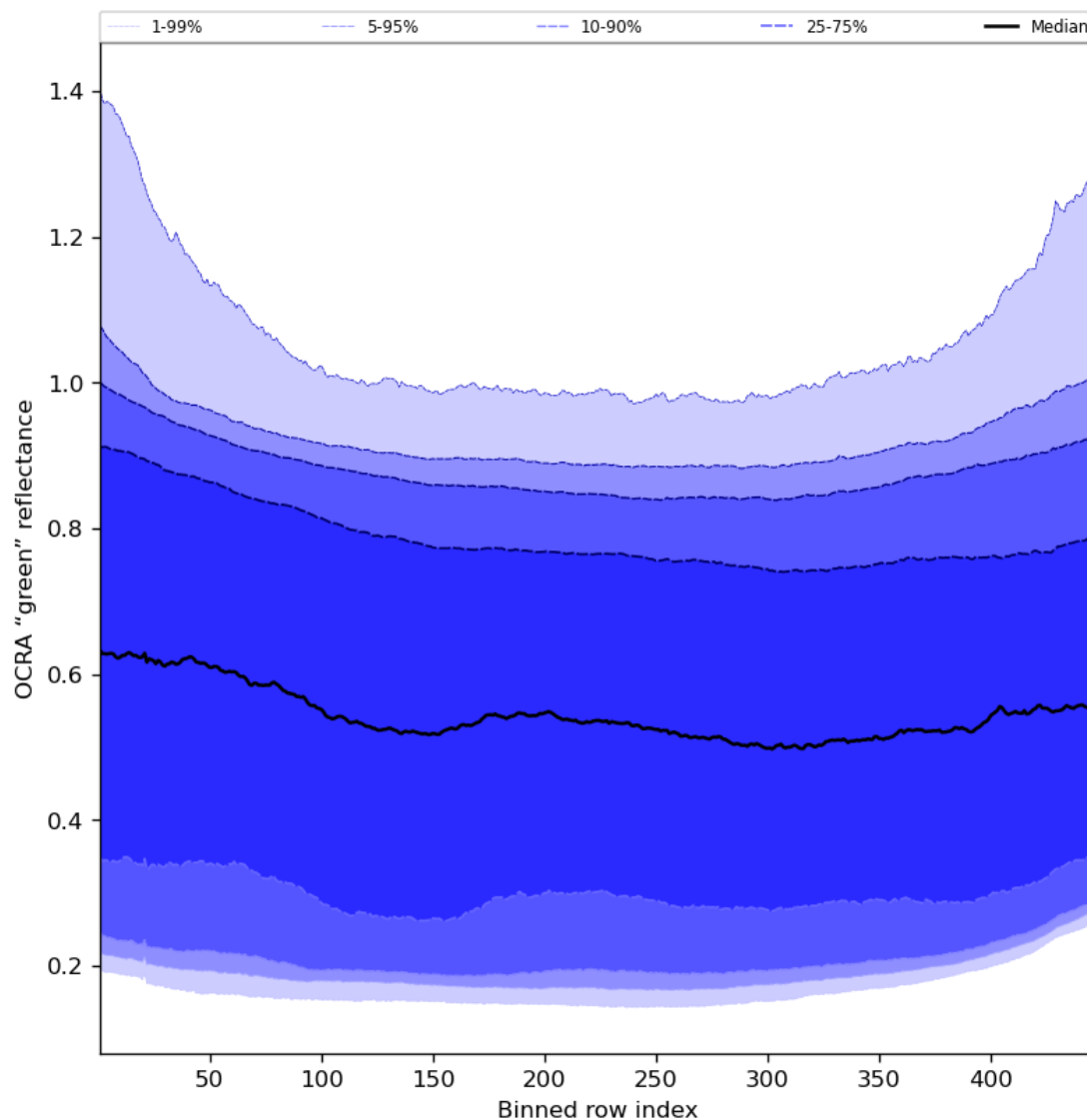
Figure 68: Along track statistics of "OCRA "green" reflectance" for 2023-10-27 to 2023-10-28
