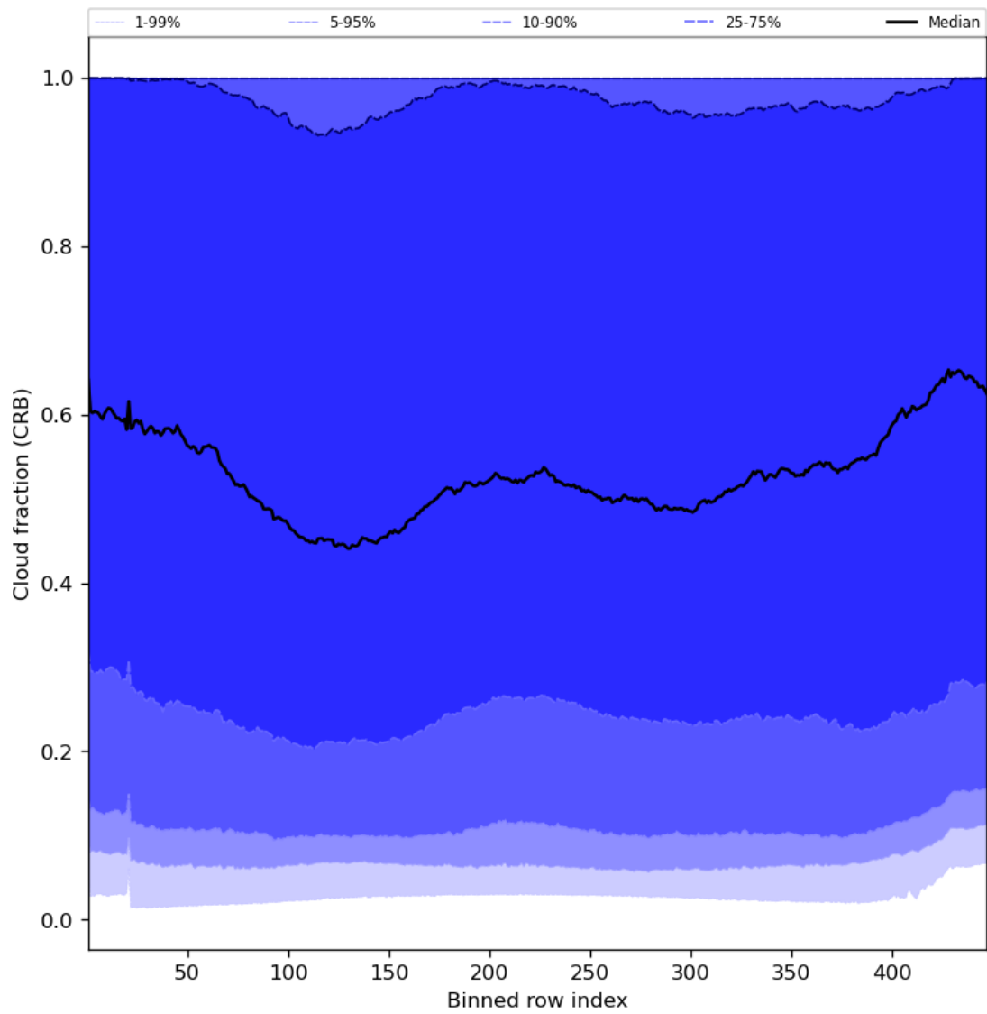
Figure 58: Along track statistics of “Cloud fraction (CRB)” for 2023-10-27 to 2023-10-28
