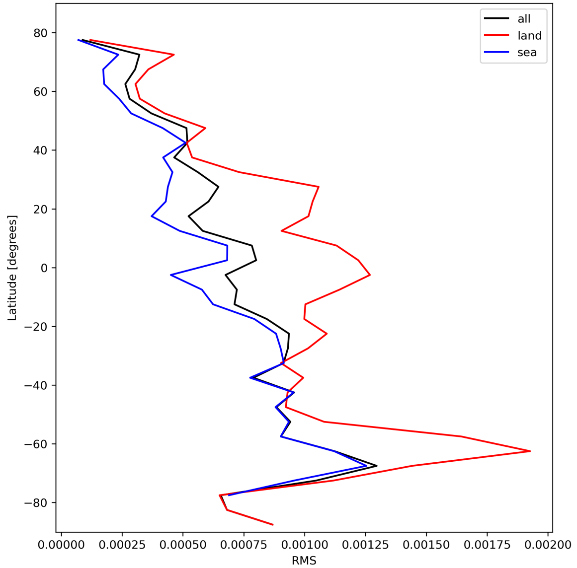
Figure 31: Zonal average of “RMS” for 2023-10-27 to 2023-10-28.
