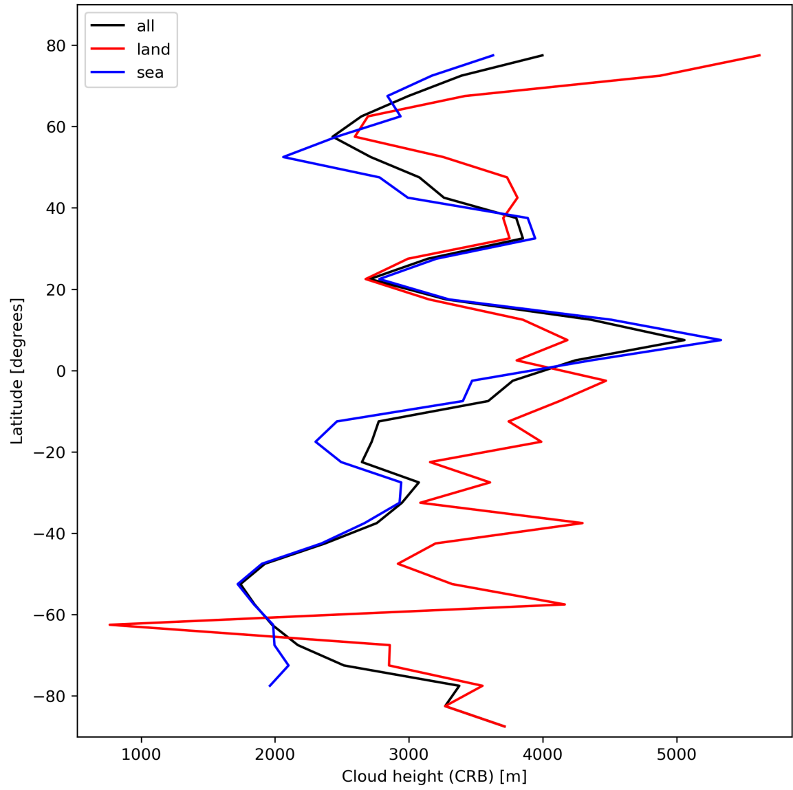
Figure 27: Zonal average of “Cloud height (CRB)” for 2023-10-27 to 2023-10-28.
