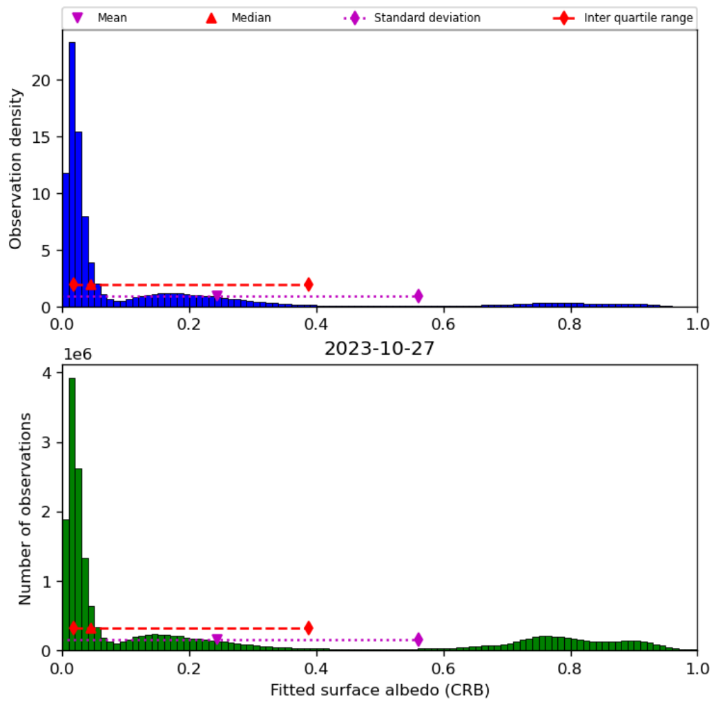
Figure 46: Histogram of “Fitted surface albedo (CRB)” for 2023-10-27 to 2023-10-28
