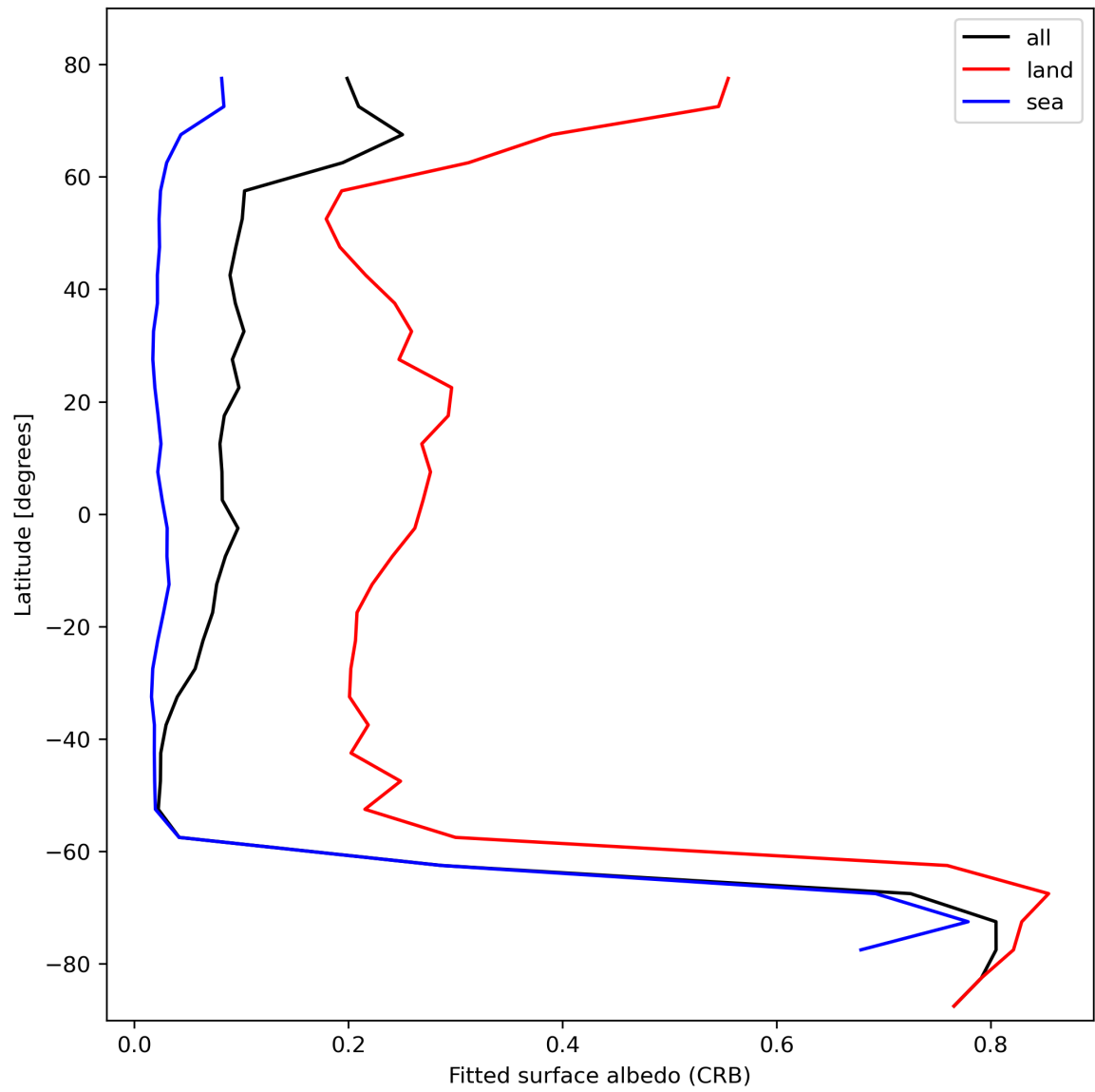
Figure 30: Zonal average of “Fitted surface albedo (CRB)” for 2023-10-27 to 2023-10-28.
