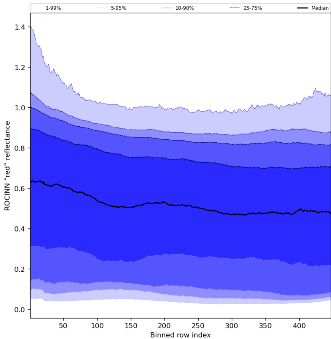
Figure 69: Along track statistics of “ROCINN “red” reflectance” for 2023-10-27 to 2023-10-28
