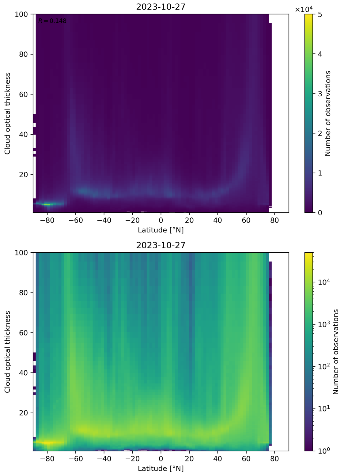
Figure 96: Scatter density plot of “Latitude” against “Cloud optical thickness” for 2023-10-27 to 2023-10-28.
