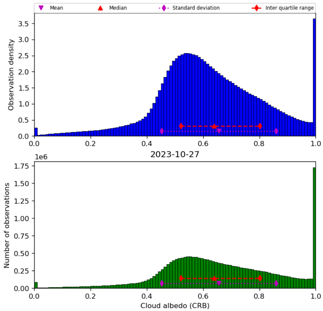
Figure 44: Histogram of “Cloud albedo (CRB)” for 2023-10-27 to 2023-10-28
