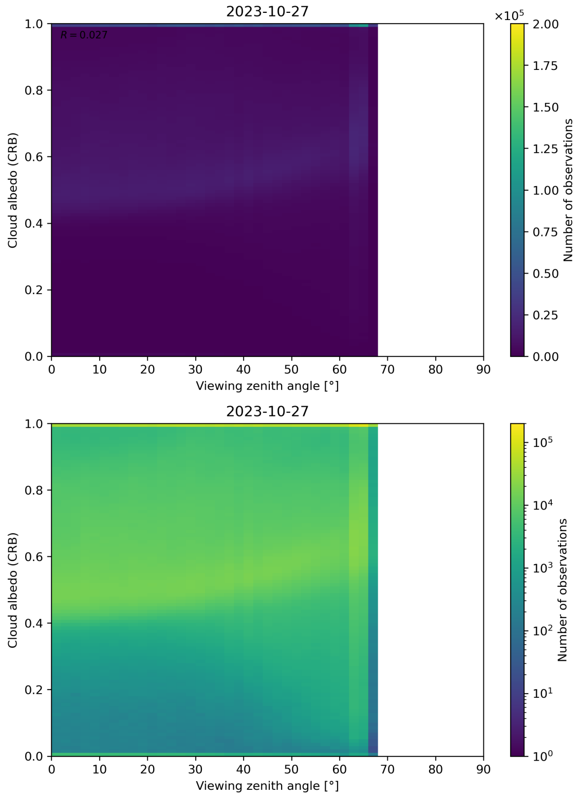
Figure 106: Scatter density plot of “Viewing zenith angle” against “Cloud albedo (CRB)” for 2023-10-27 to 2023-10-28.
