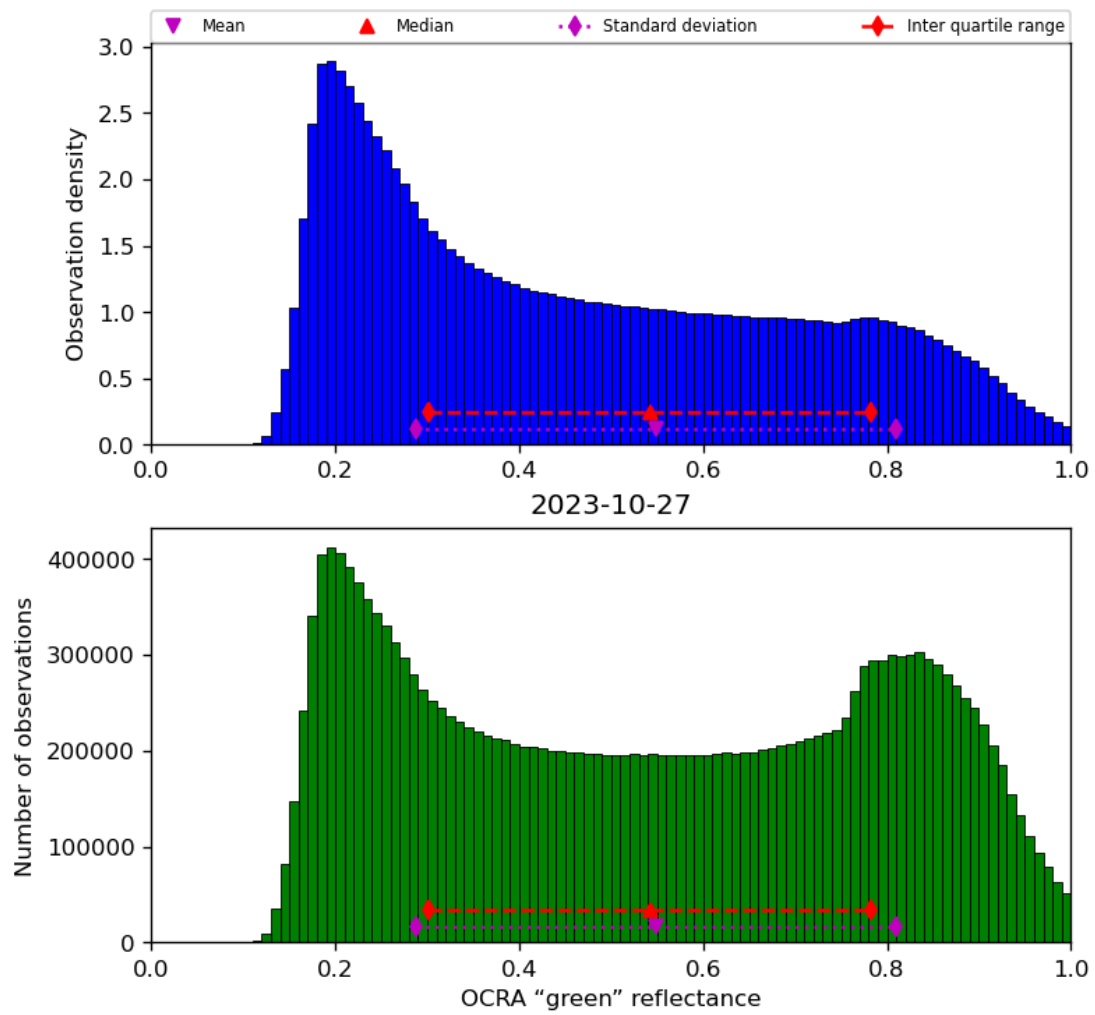
Figure 52: Histogram of “OCRA “green” reflectance” for 2023-10-27 to 2023-10-28
