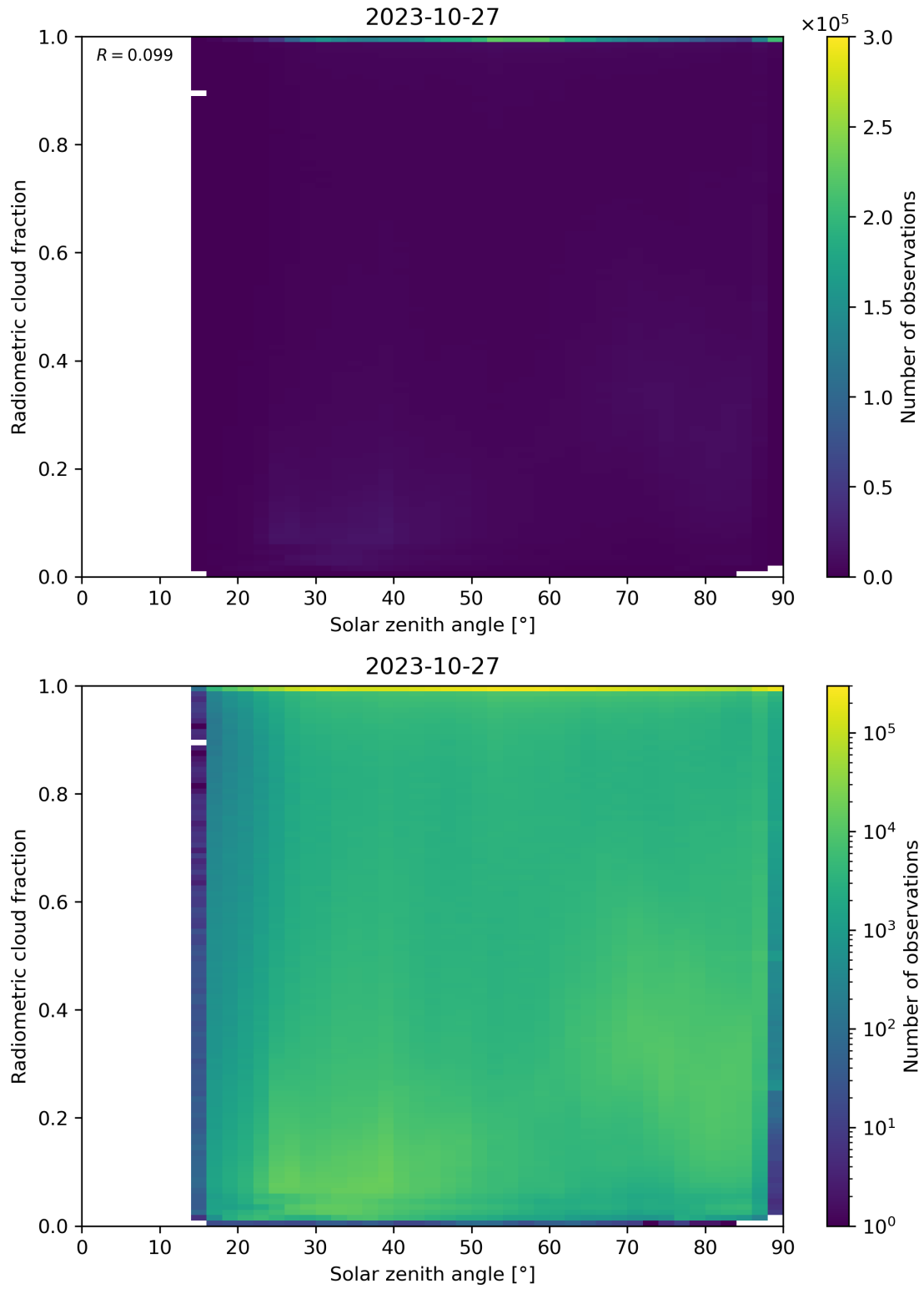
Figure 99: Scatter density plot of “Solar zenith angle” against “Radiometric cloud fraction” for 2023-10-27 to 2023-10-28.
