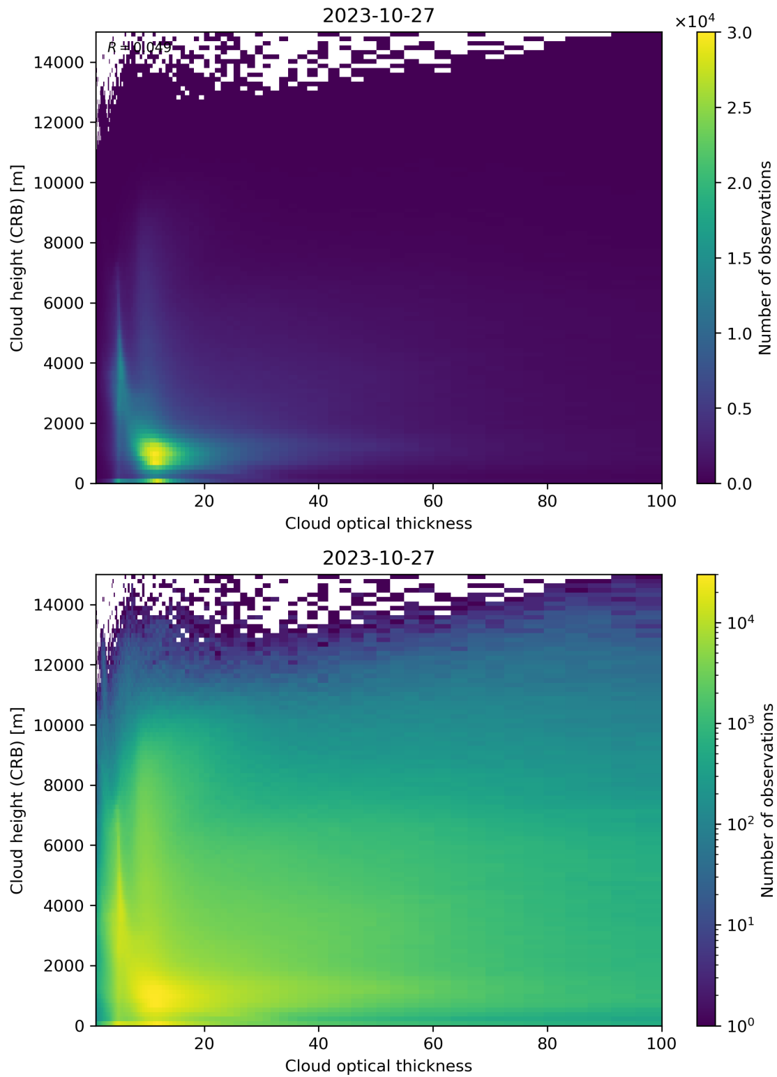
Figure 85: Scatter density plot of “Cloud optical thickness” against “Cloud height (CRB)” for 2023-10-27 to 2023-10-28.
