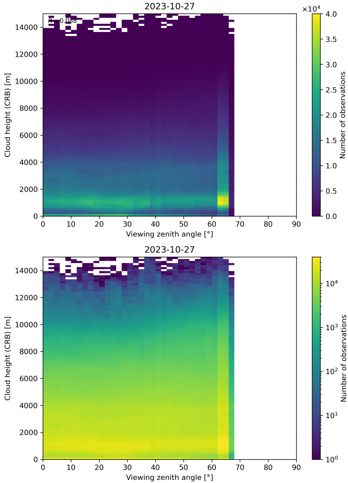
Figure 110: Scatter density plot of “Viewing zenith angle” against “Cloud height (CRB)” for 2023-10-27 to 2023-10-28.
