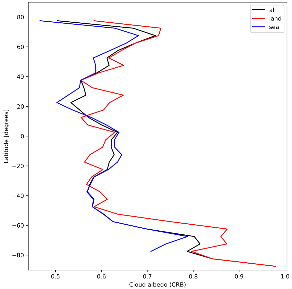
Figure 28: Zonal average of “Cloud albedo (CRB)” for 2023-10-27 to 2023-10-28.
