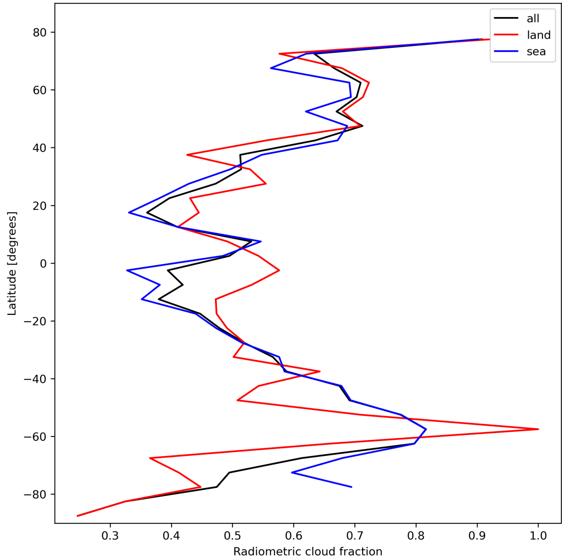
Figure 23: Zonal average of “Radiometric cloud fraction” for 2023-10-27 to 2023-10-28.
