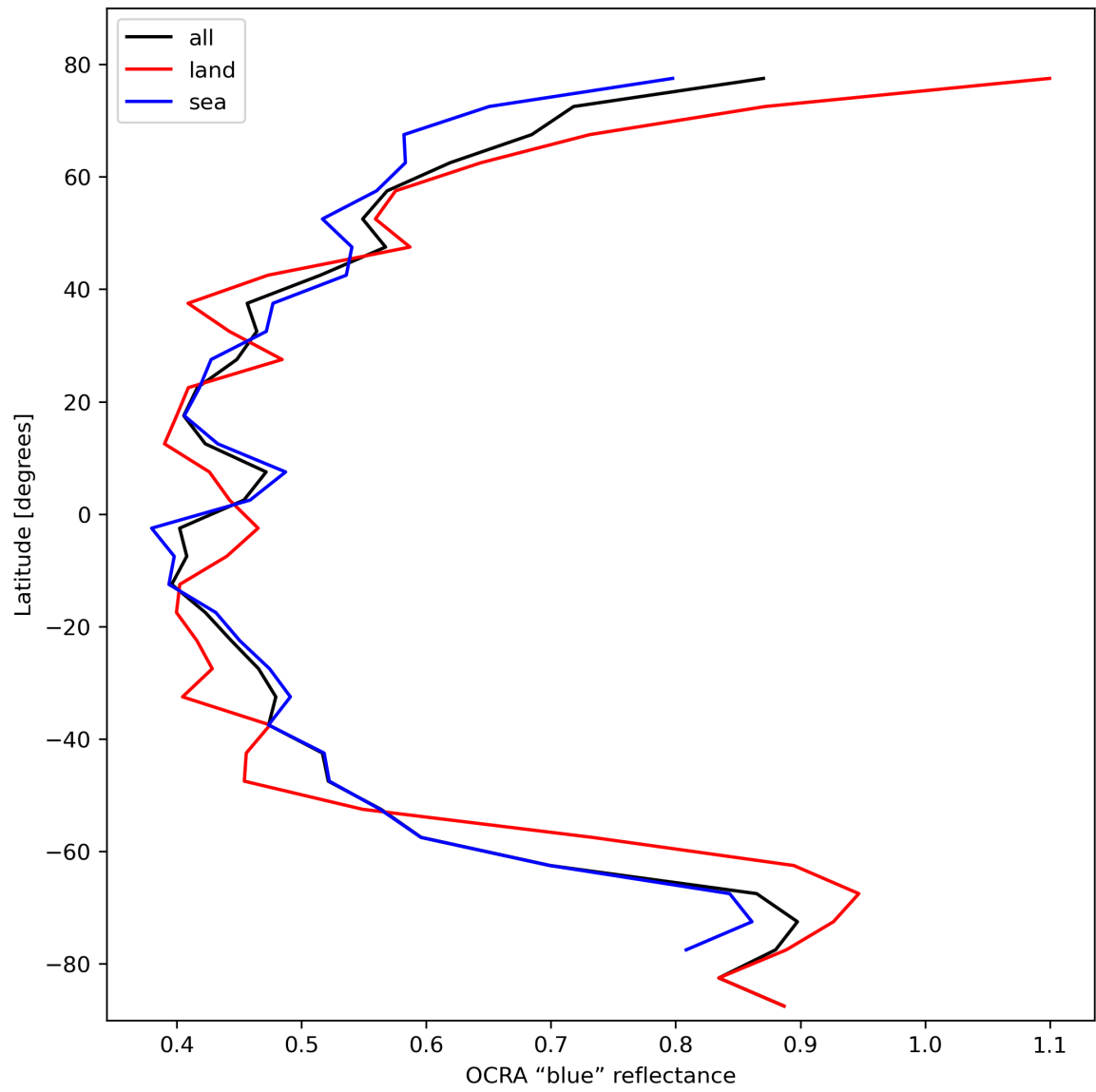
Figure 35: Zonal average of “OCRA “blue” reflectance” for 2023-10-27 to 2023-10-28.
