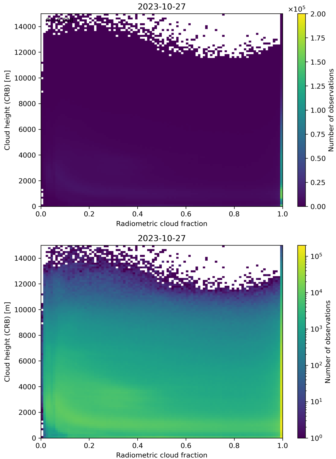
Figure 74: Scatter density plot of “Radiometric cloud fraction” against “Cloud height (CRB)” for 2023-10-27 to 2023-10-28.
