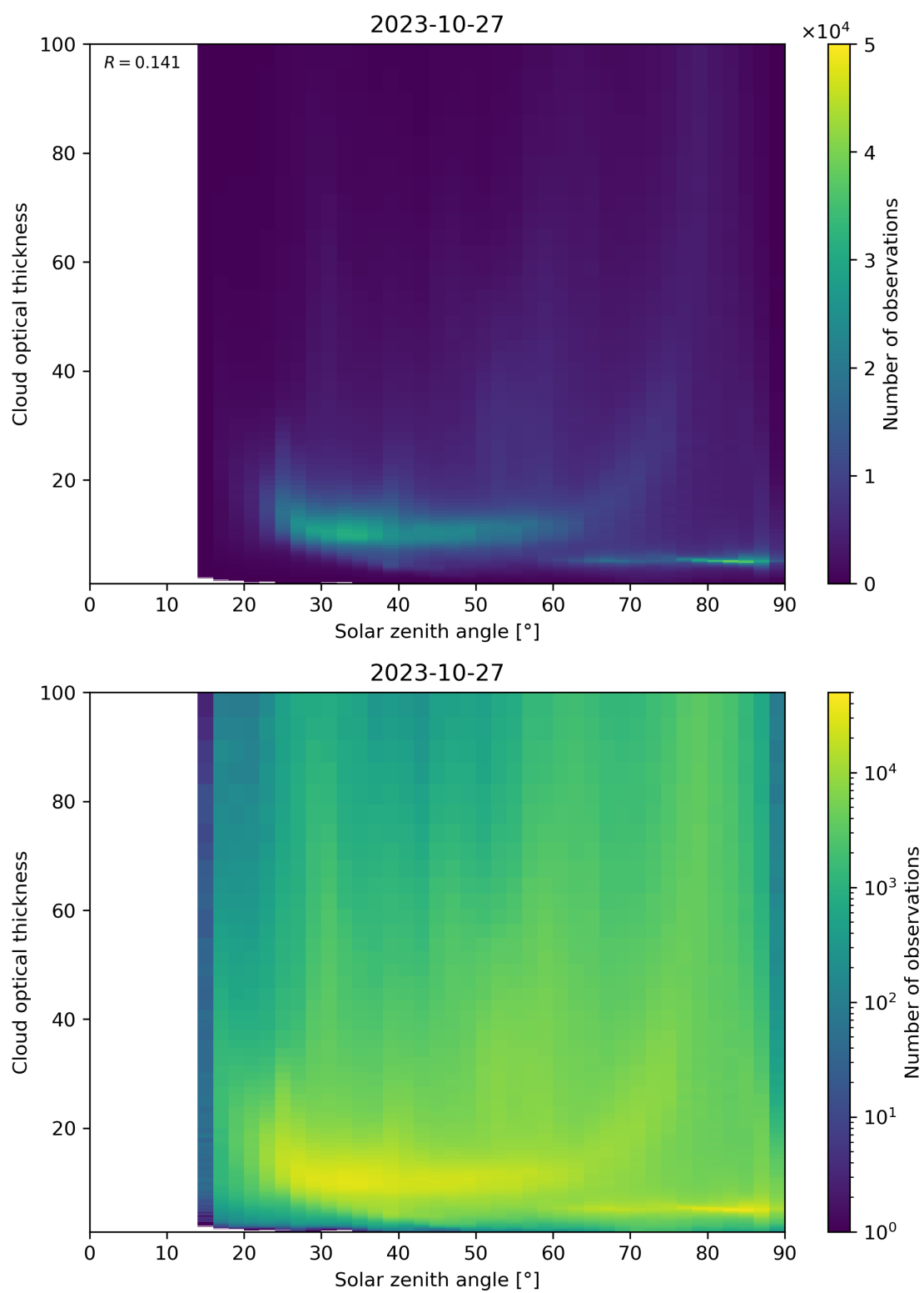
Figure 103: Scatter density plot of “Solar zenith angle” against “Cloud optical thickness” for 2023-10-27 to 2023-10-28.
