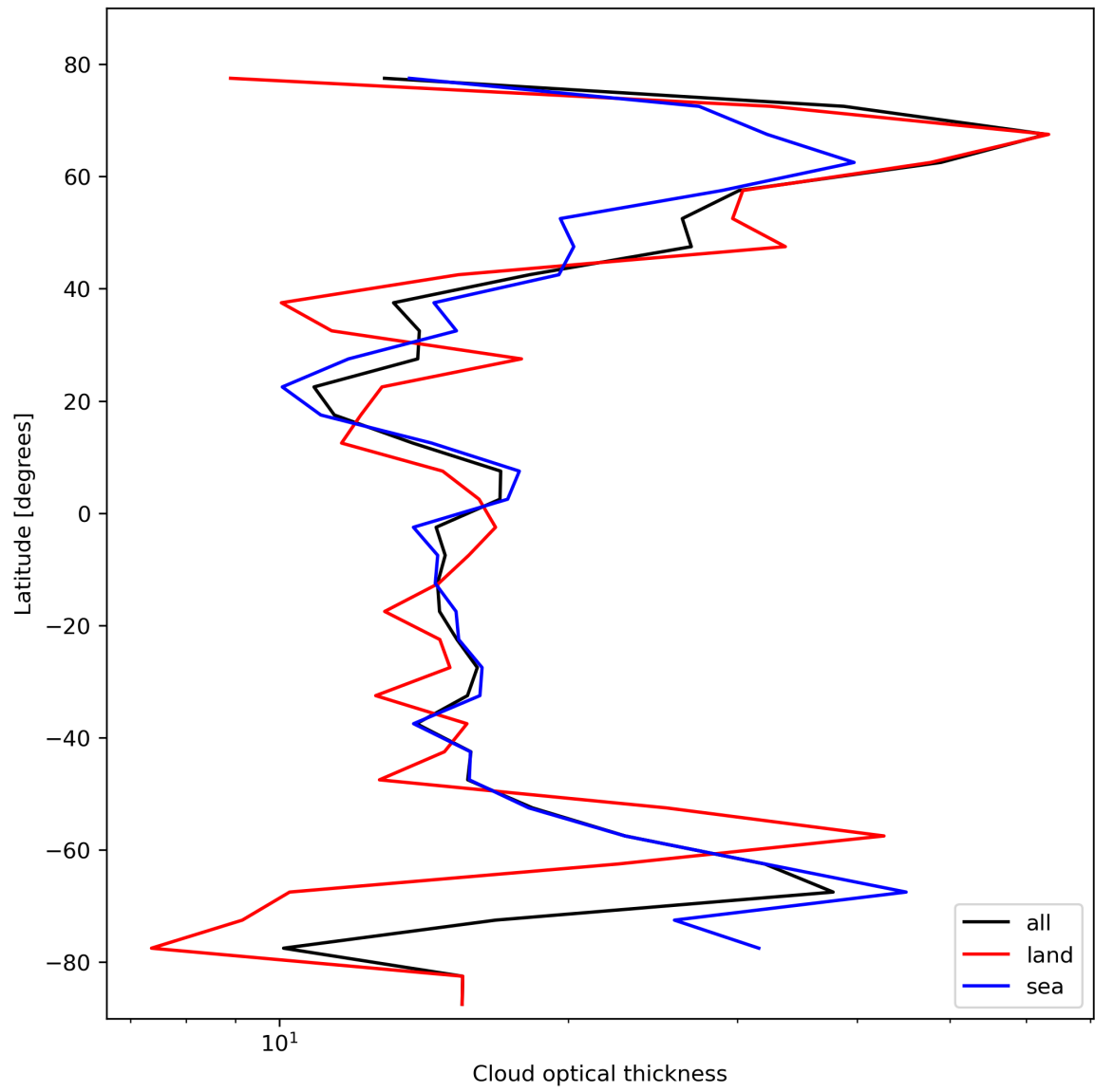
Figure 25: Zonal average of “Cloud optical thickness” for 2023-10-27 to 2023-10-28.
