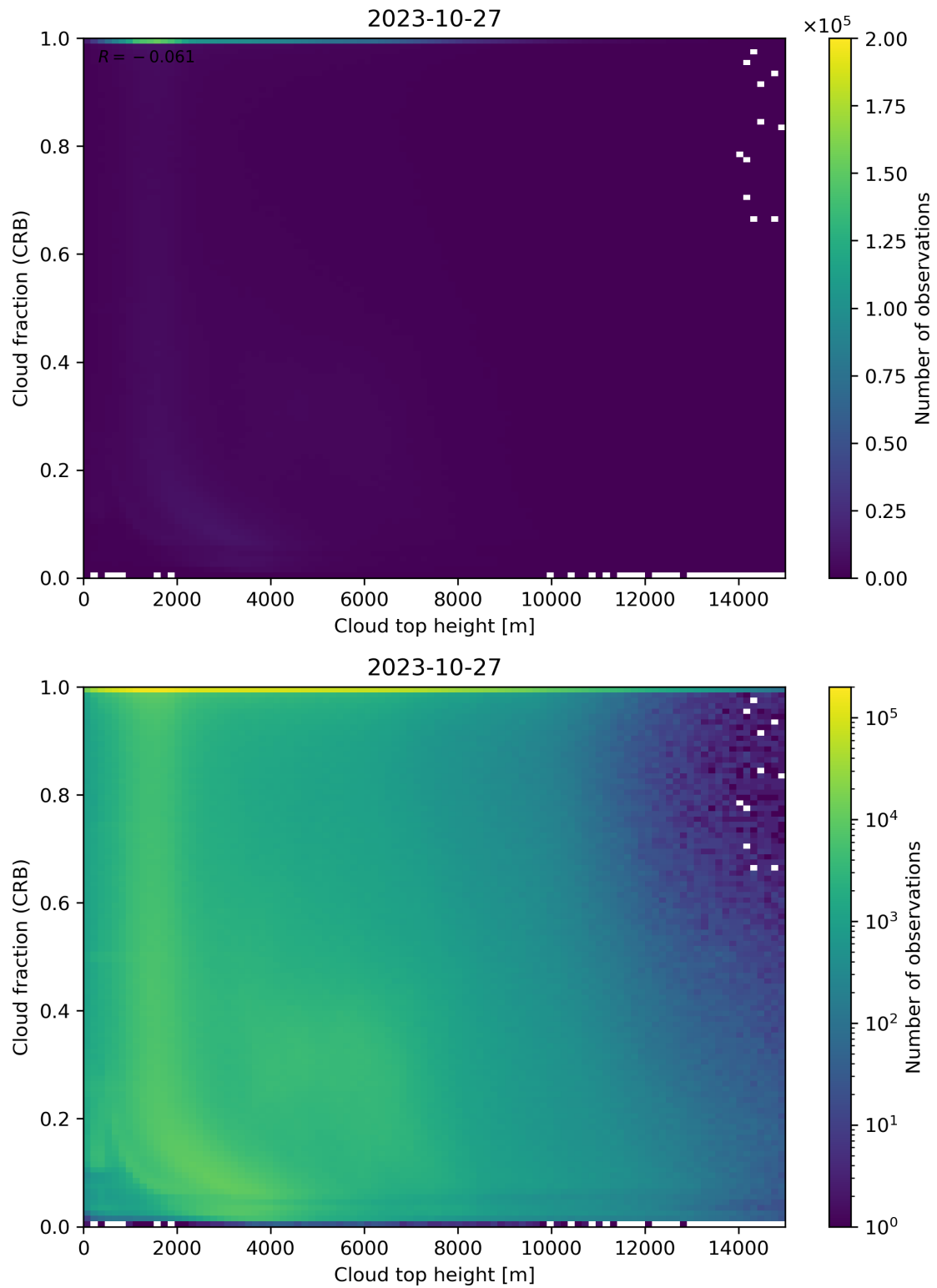
Figure 88: Scatter density plot of “Cloud top height” against “Cloud fraction (CRB)” for 2023-10-27 to 2023-10-28.
