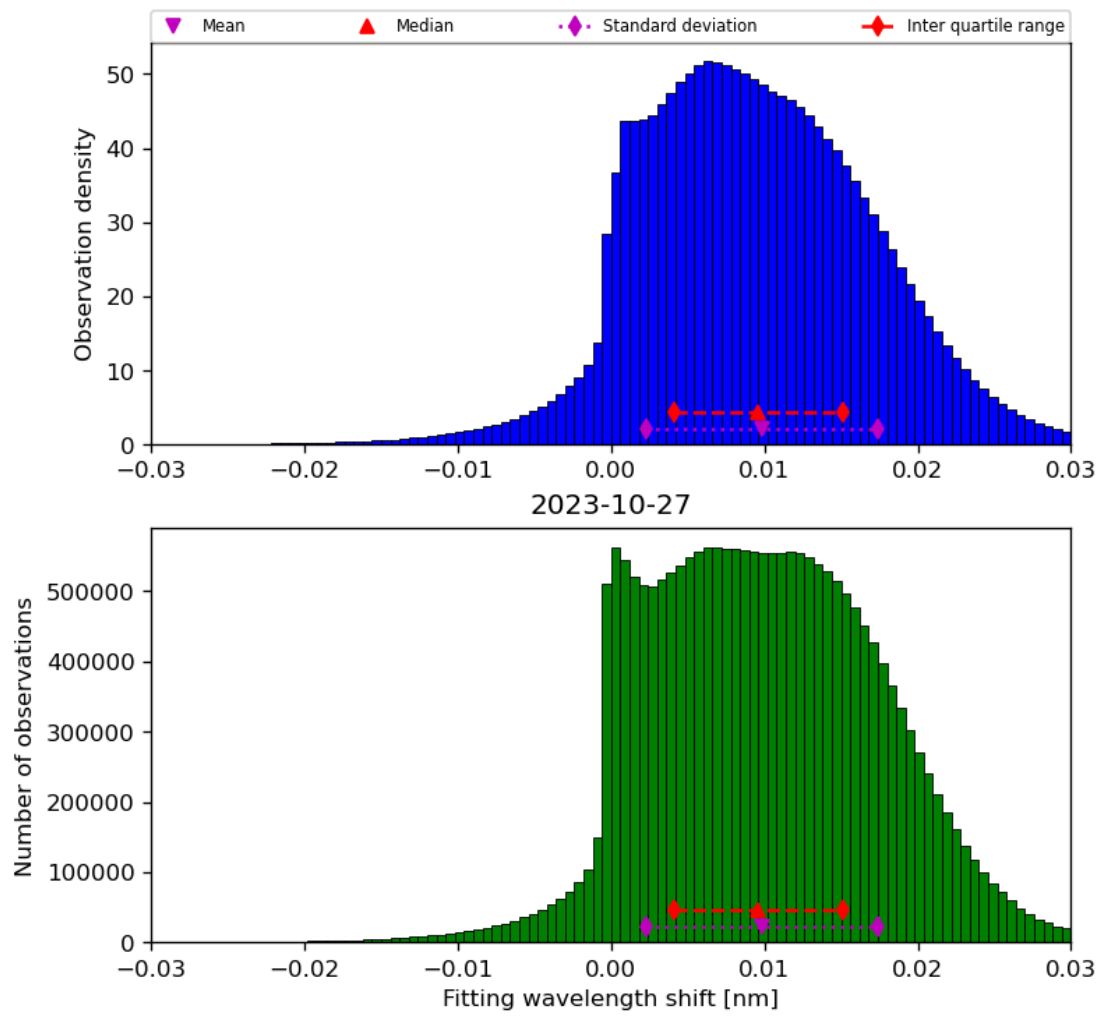
Figure 49: Histogram of “Fitting wavelength shift” for 2023-10-27 to 2023-10-28
