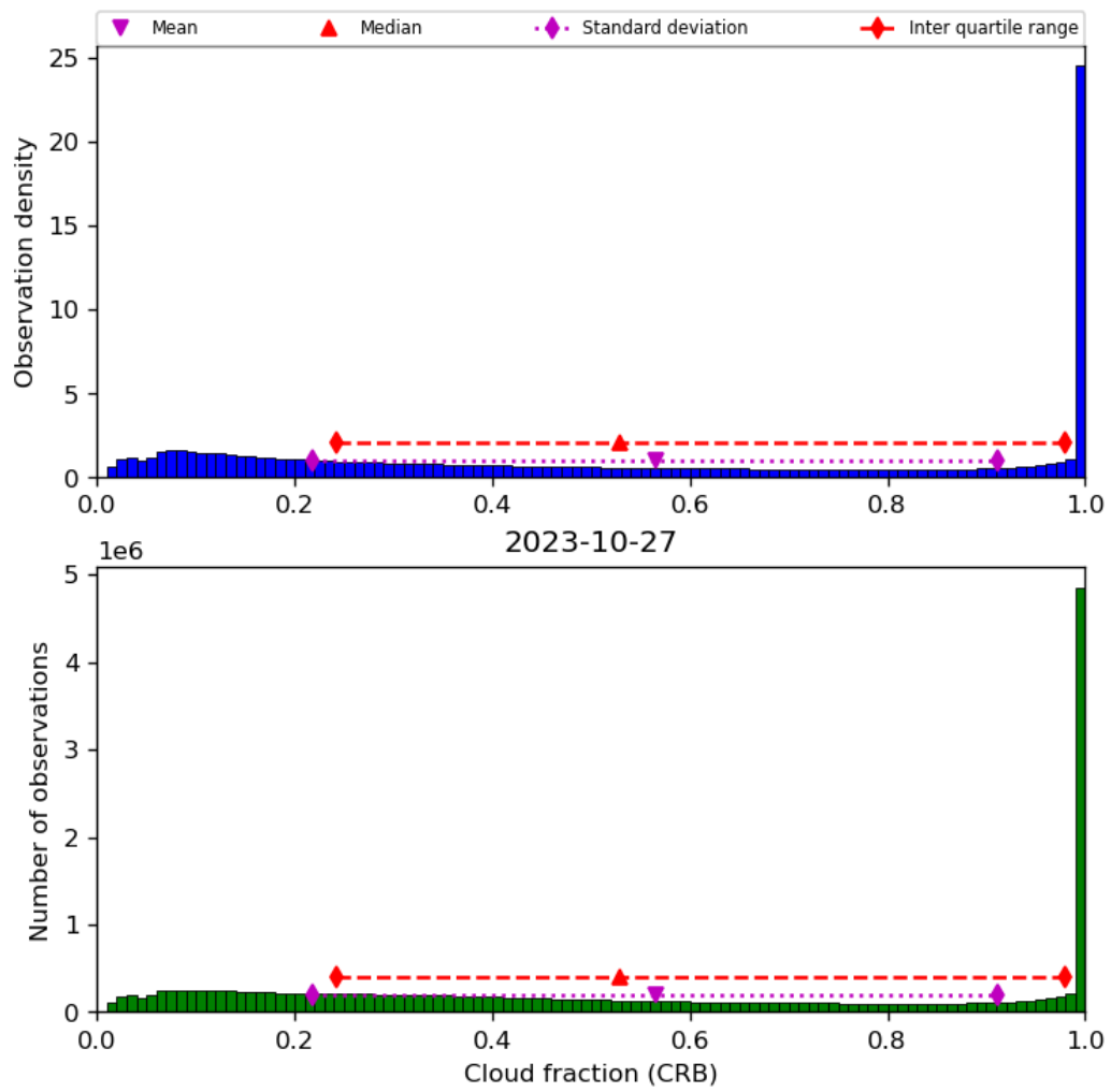
Figure 42: Histogram of “Cloud fraction (CRB)” for 2023-10-27 to 2023-10-28
