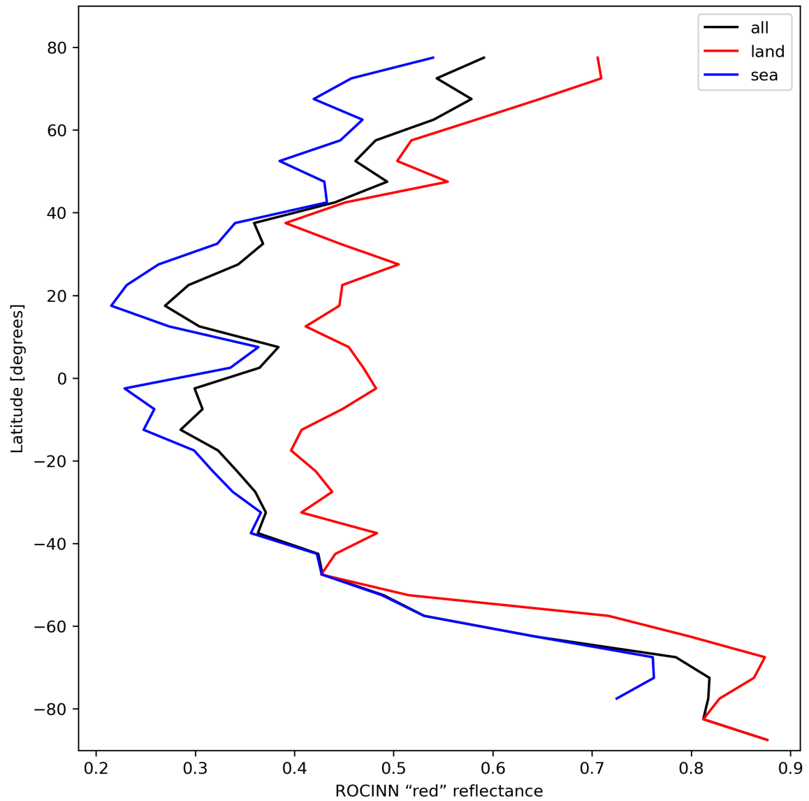
Figure 37: Zonal average of “ROCINN “red” reflectance” for 2023-10-27 to 2023-10-28.
