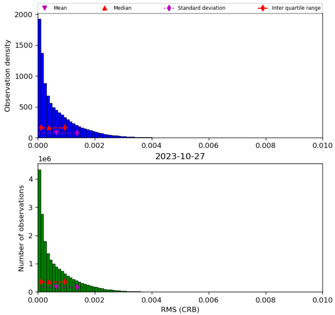
Figure 48: Histogram of “RMS (CRB)” for 2023-10-27 to 2023-10-28
