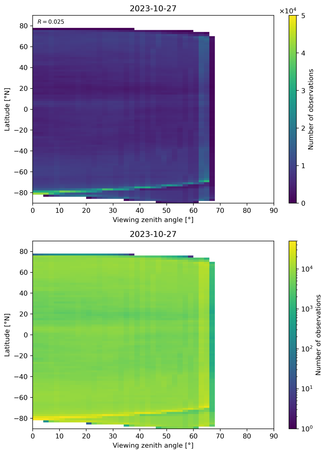
Figure 113: Scatter density plot of “Viewing zenith angle” against “Latitude” for 2023-10-27 to 2023-10-28.
