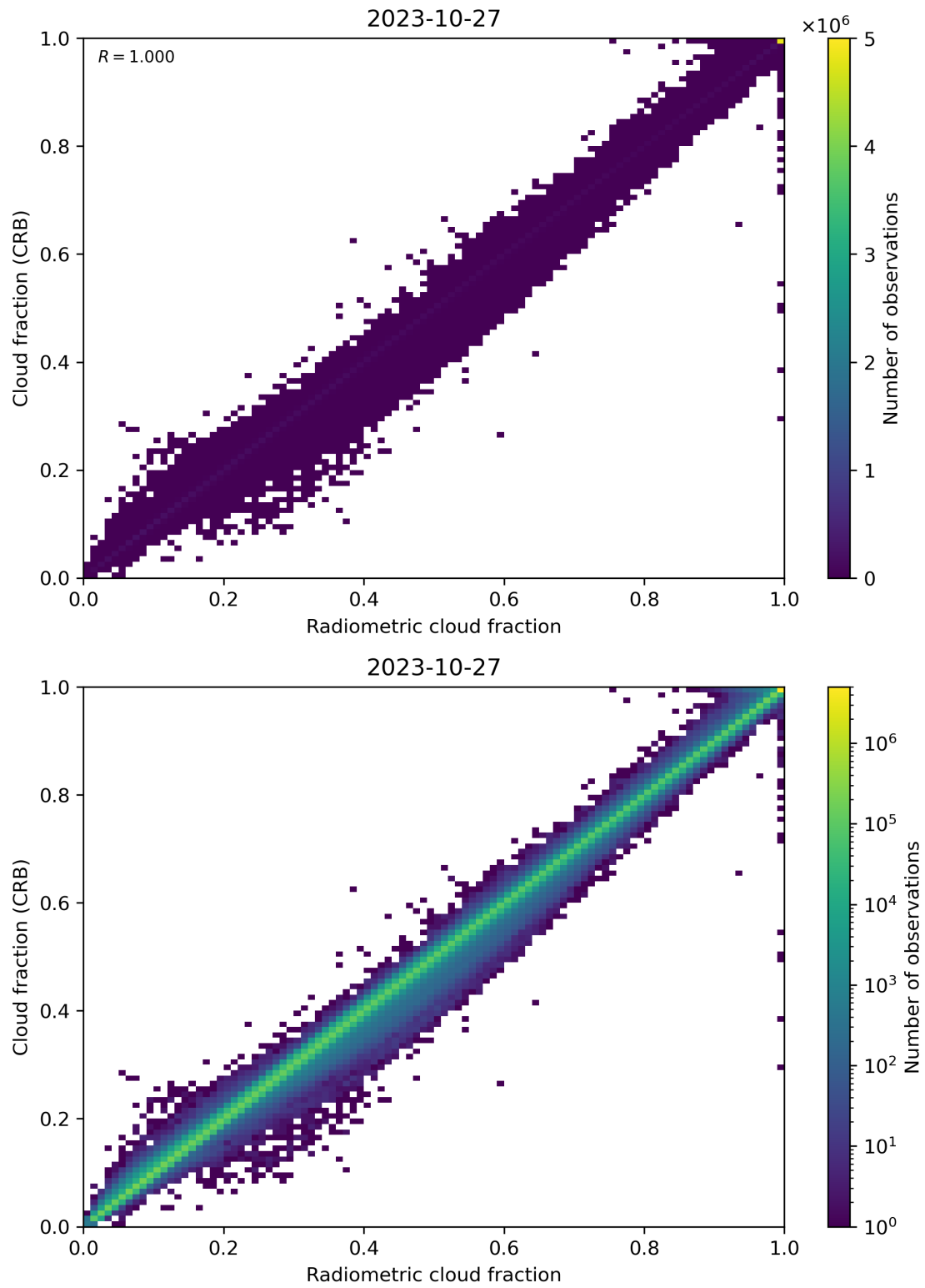
Figure 73: Scatter density plot of “Radiometric cloud fraction” against “Cloud fraction (CRB)” for 2023-10-27 to 2023-10-28.
