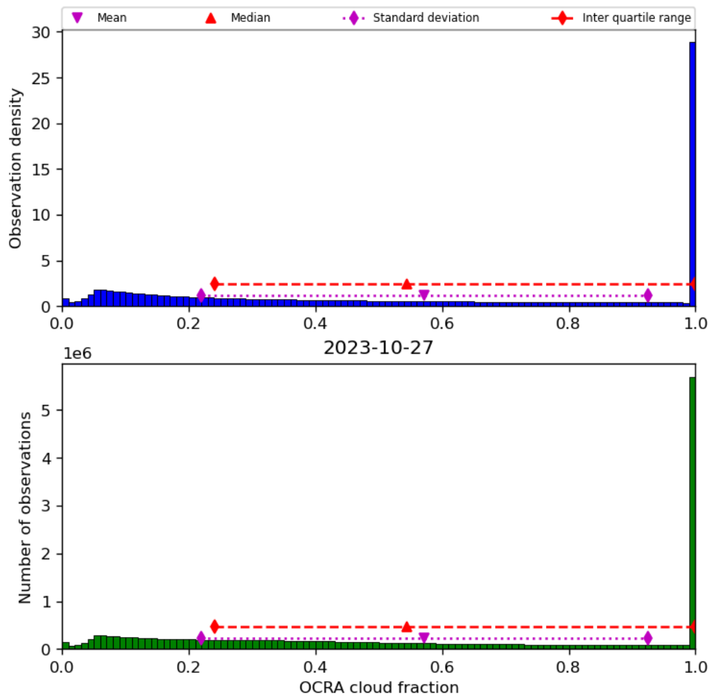
Figure 50: Histogram of “OCRA cloud fraction” for 2023-10-27 to 2023-10-28
