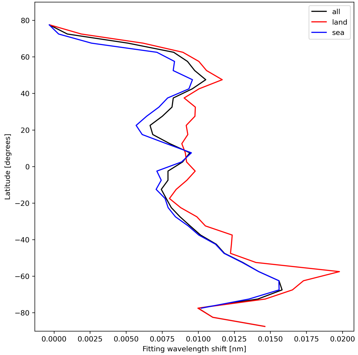
Figure 33: Zonal average of “Fitting wavelength shift” for 2023-10-27 to 2023-10-28.
