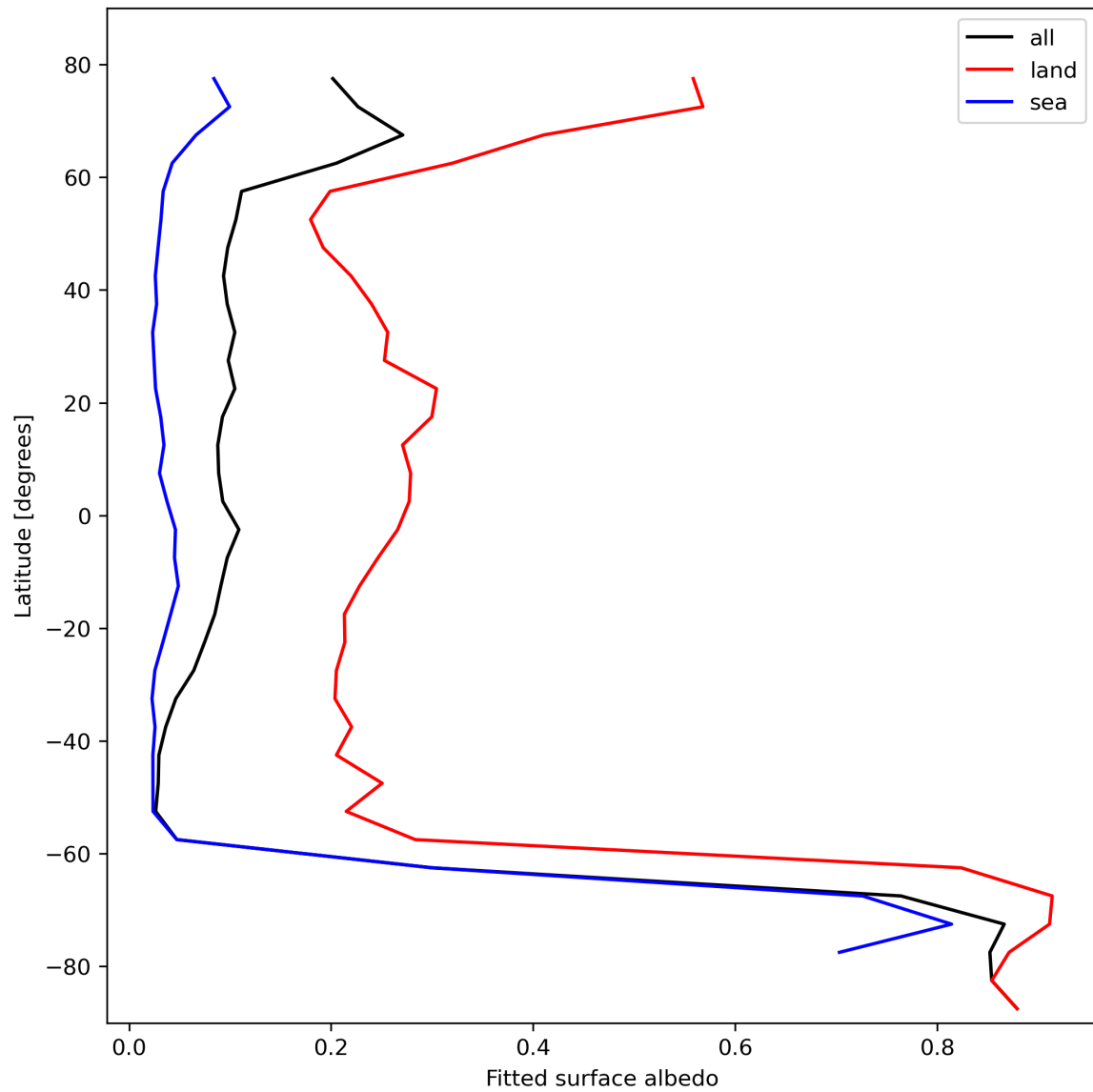
Figure 29: Zonal average of “Fitted surface albedo” for 2023-10-27 to 2023-10-28.
