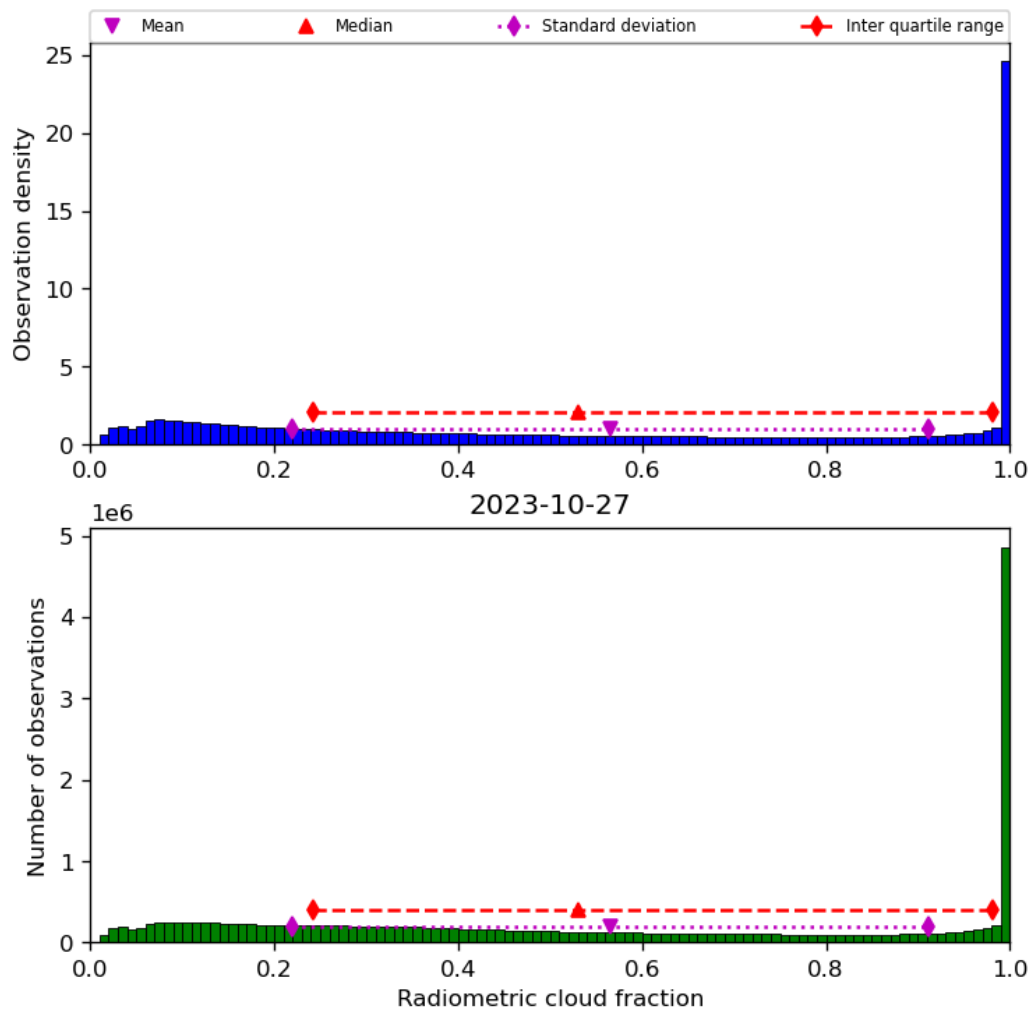
Figure 39: Histogram of “Radiometric cloud fraction” for 2023-10-27 to 2023-10-28
