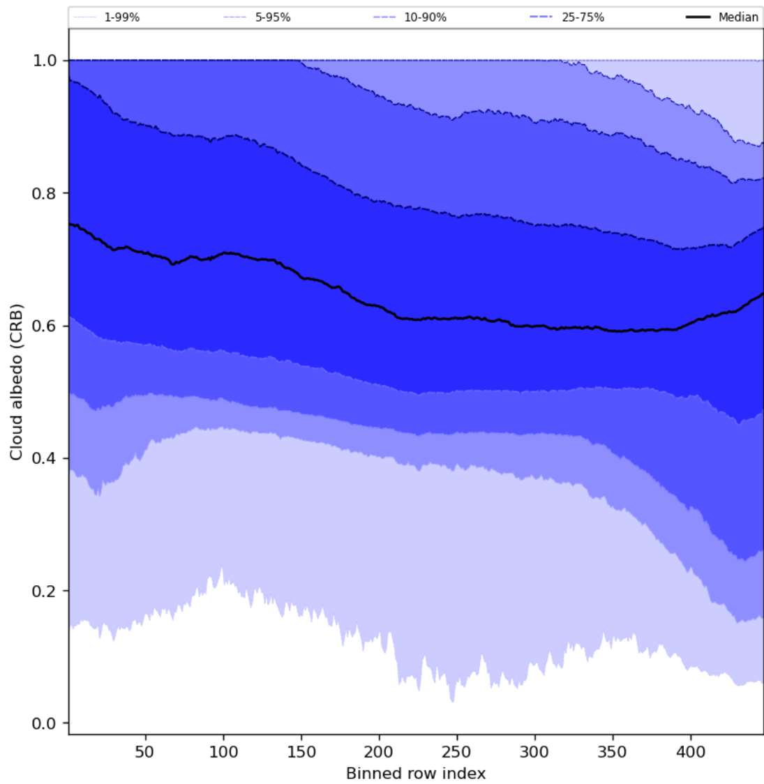
Figure 60: Along track statistics of “Cloud albedo (CRB)” for 2023-10-27 to 2023-10-28
