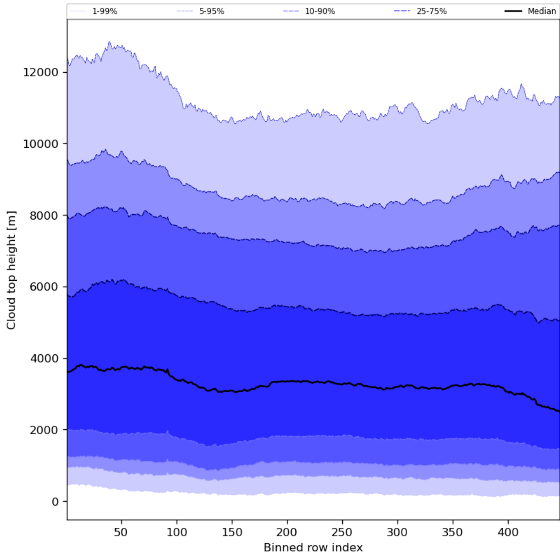
Figure 56: Along track statistics of “Cloud top height” for 2023-10-27 to 2023-10-28
