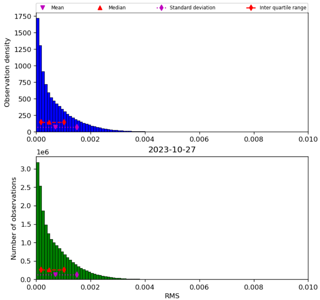
Figure 47: Histogram of “RMS” for 2023-10-27 to 2023-10-28
