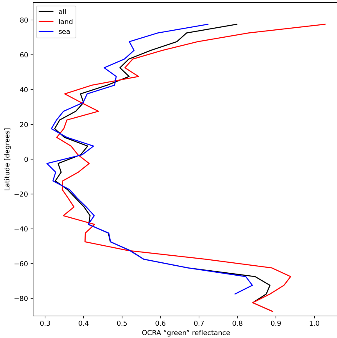
Figure 36: Zonal average of “OCRA “green” reflectance” for 2023-10-27 to 2023-10-28.
