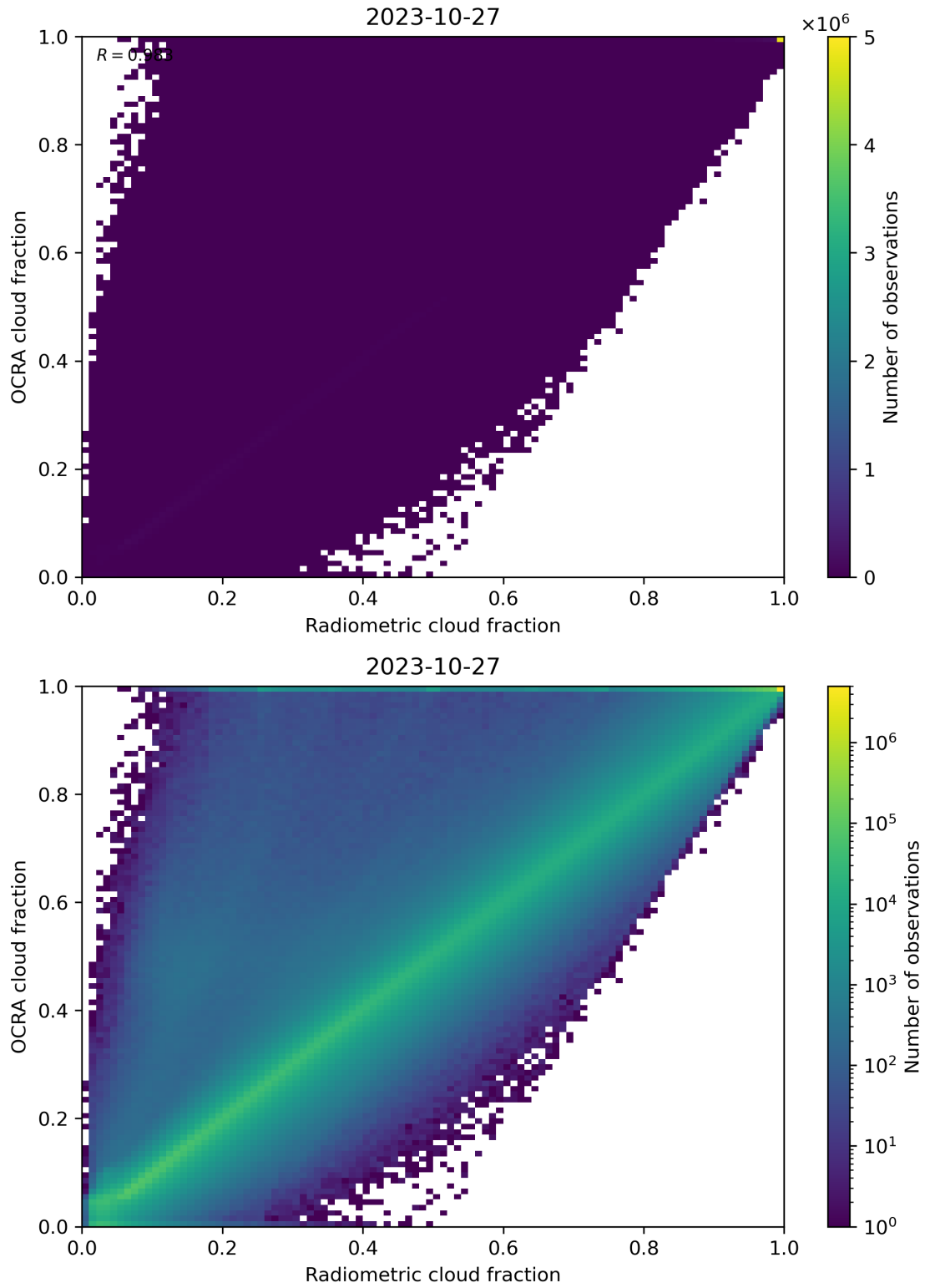
Figure 72: Scatter density plot of “Radiometric cloud fraction” against “OCRA cloud fraction” for 2023-10-27 to 2023-10-28.
