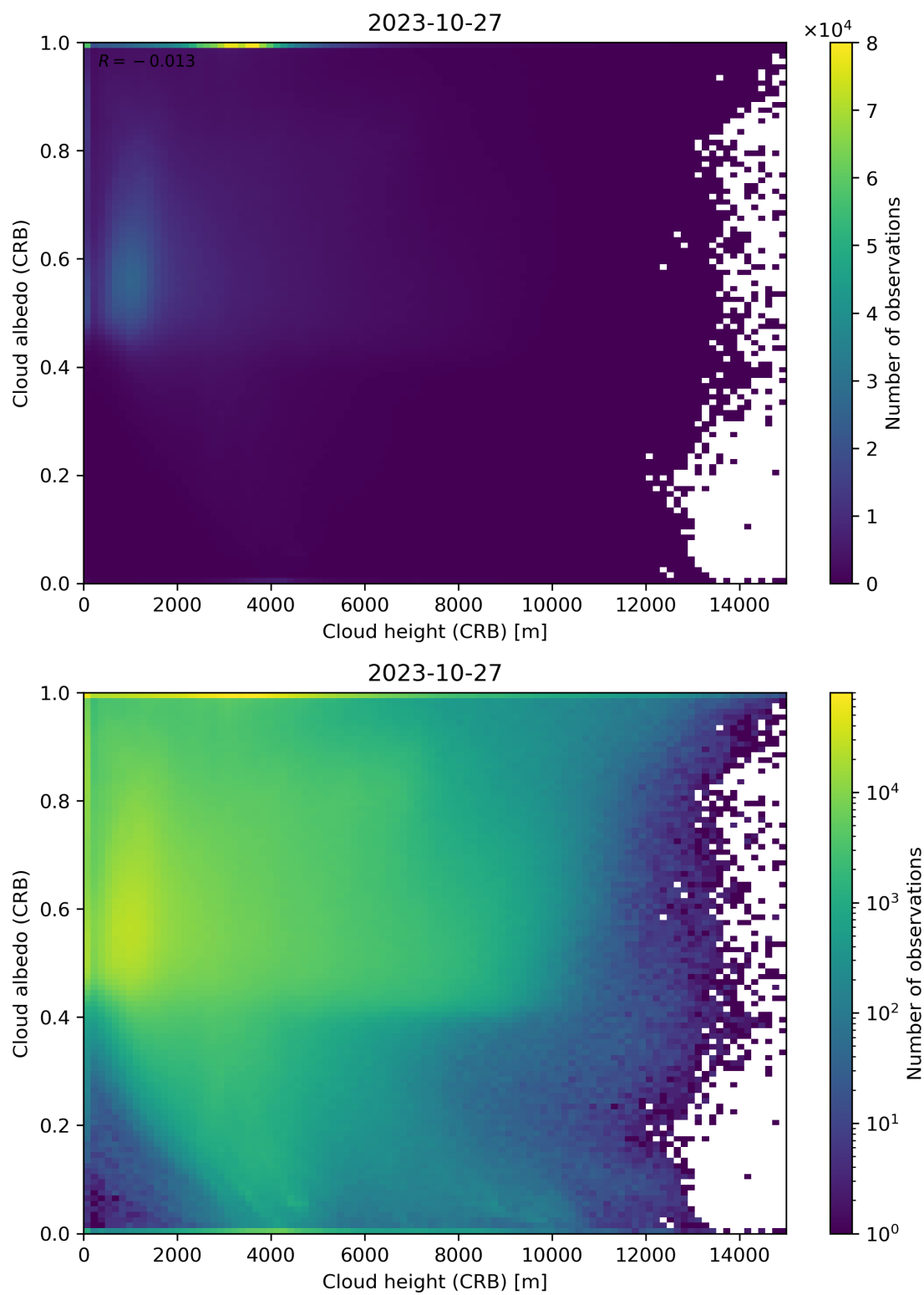
Figure 80: Scatter density plot of “Cloud height (CRB)” against “Cloud albedo (CRB)” for 2023-10-27 to 2023-10-28.
