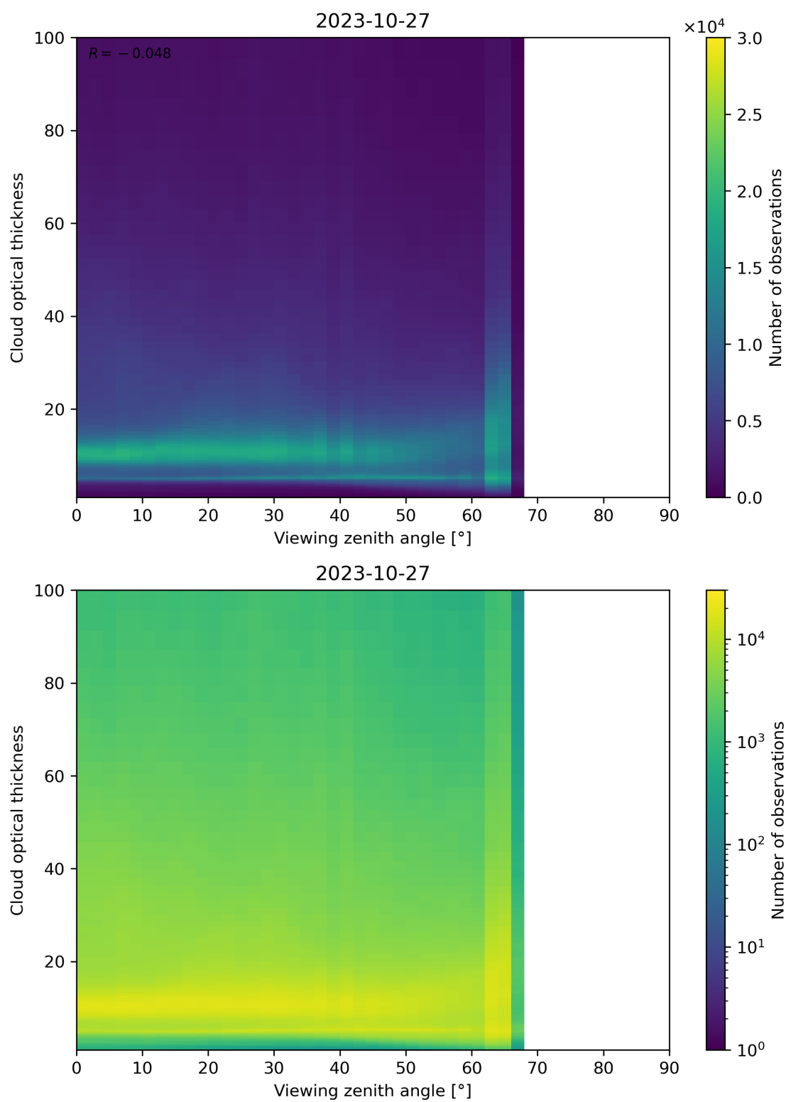
Figure 111: Scatter density plot of “Viewing zenith angle” against “Cloud optical thickness” for 2023-10-27 to 2023-10-28.
