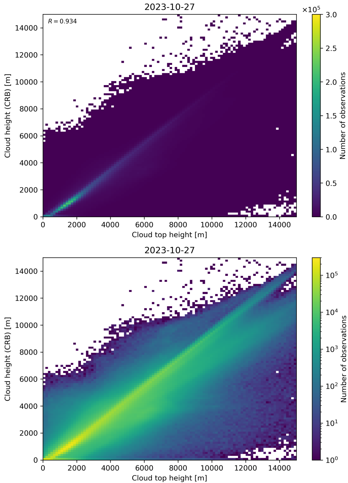
Figure 89: Scatter density plot of “Cloud top height” against “Cloud height (CRB)” for 2023-10-27 to 2023-10-28.
