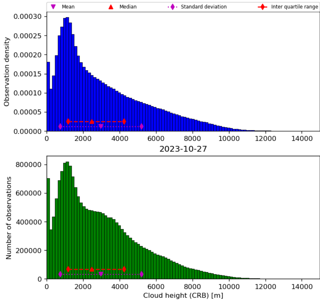
Figure 43: Histogram of “Cloud height (CRB)” for 2023-10-27 to 2023-10-28
