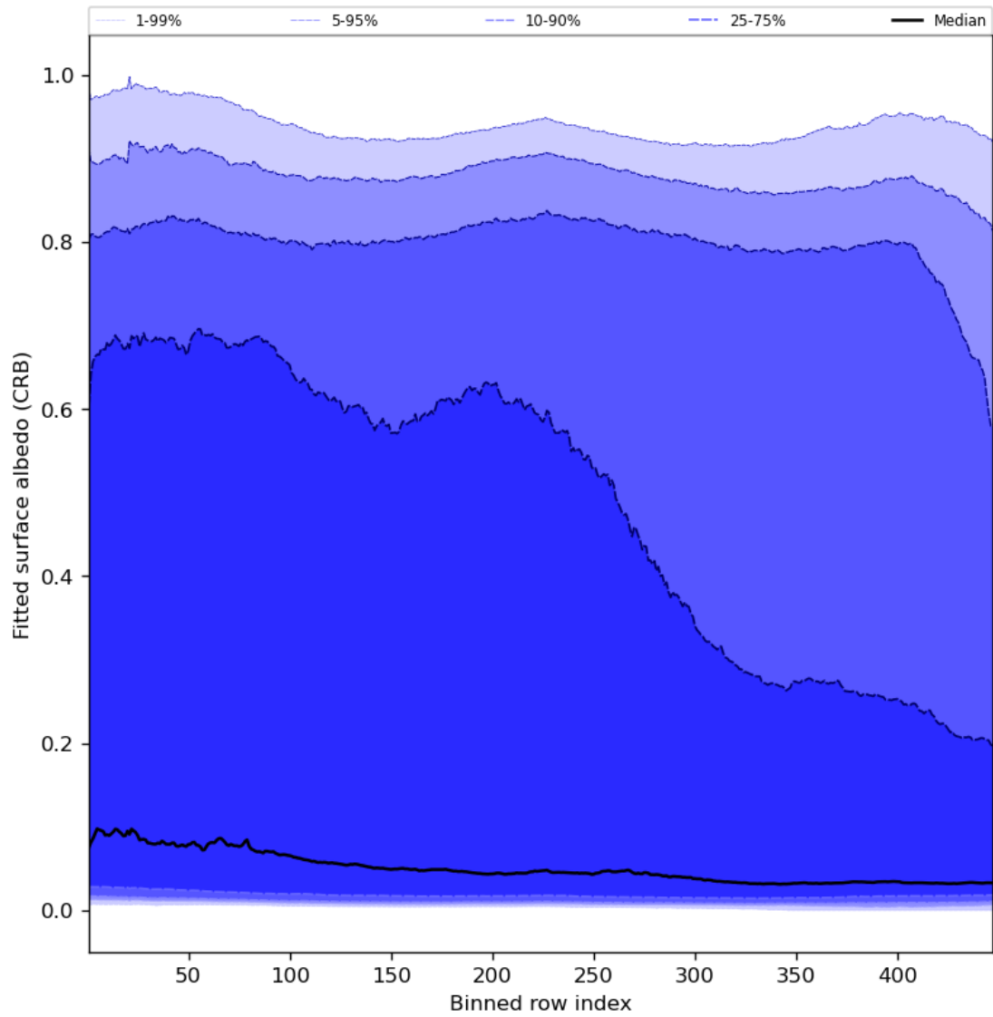
Figure 62: Along track statistics of “Fitted surface albedo (CRB)” for 2023-10-27 to 2023-10-28
