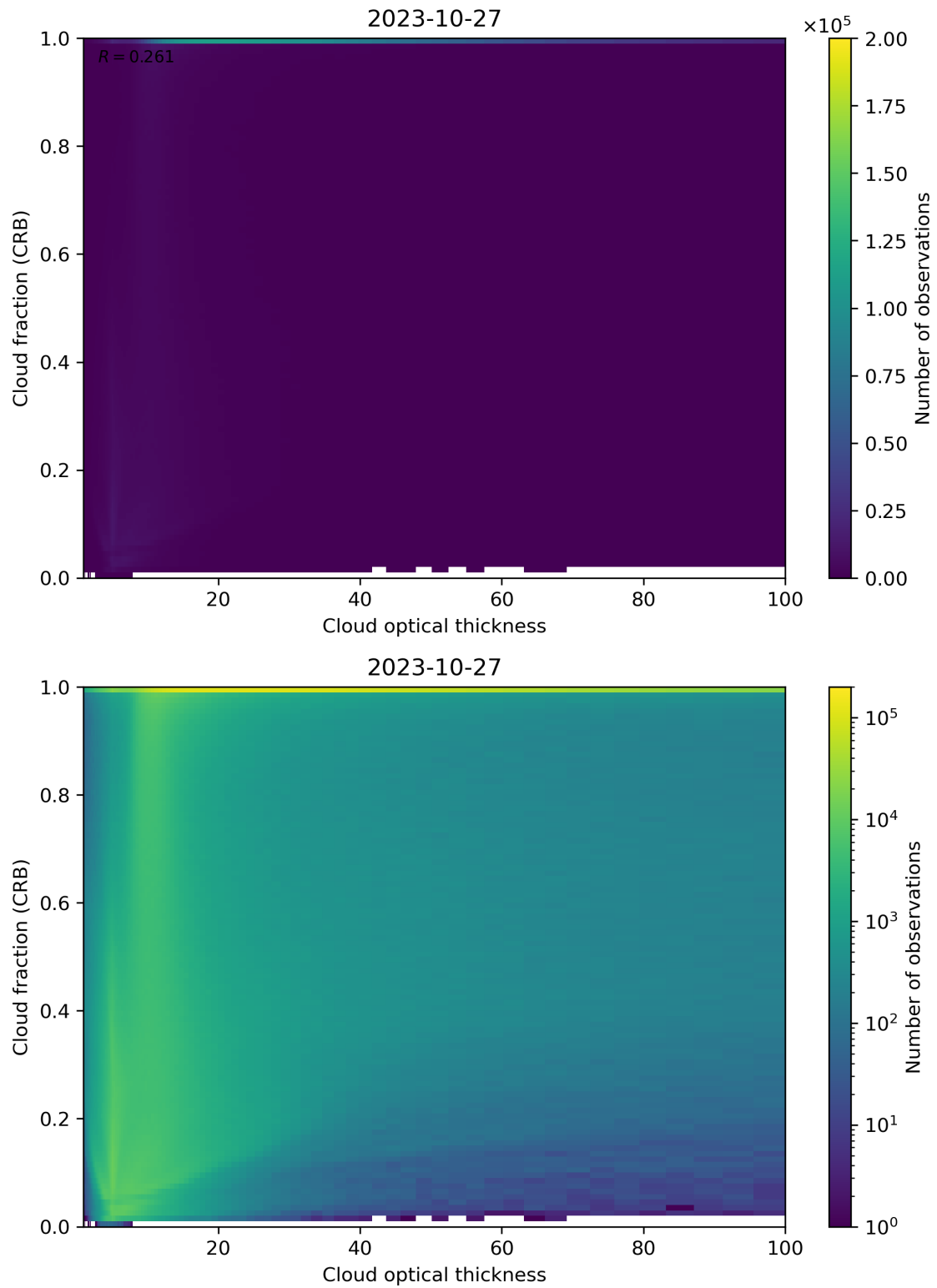
Figure 84: Scatter density plot of “Cloud optical thickness” against “Cloud fraction (CRB)” for 2023-10-27 to 2023-10-28.
