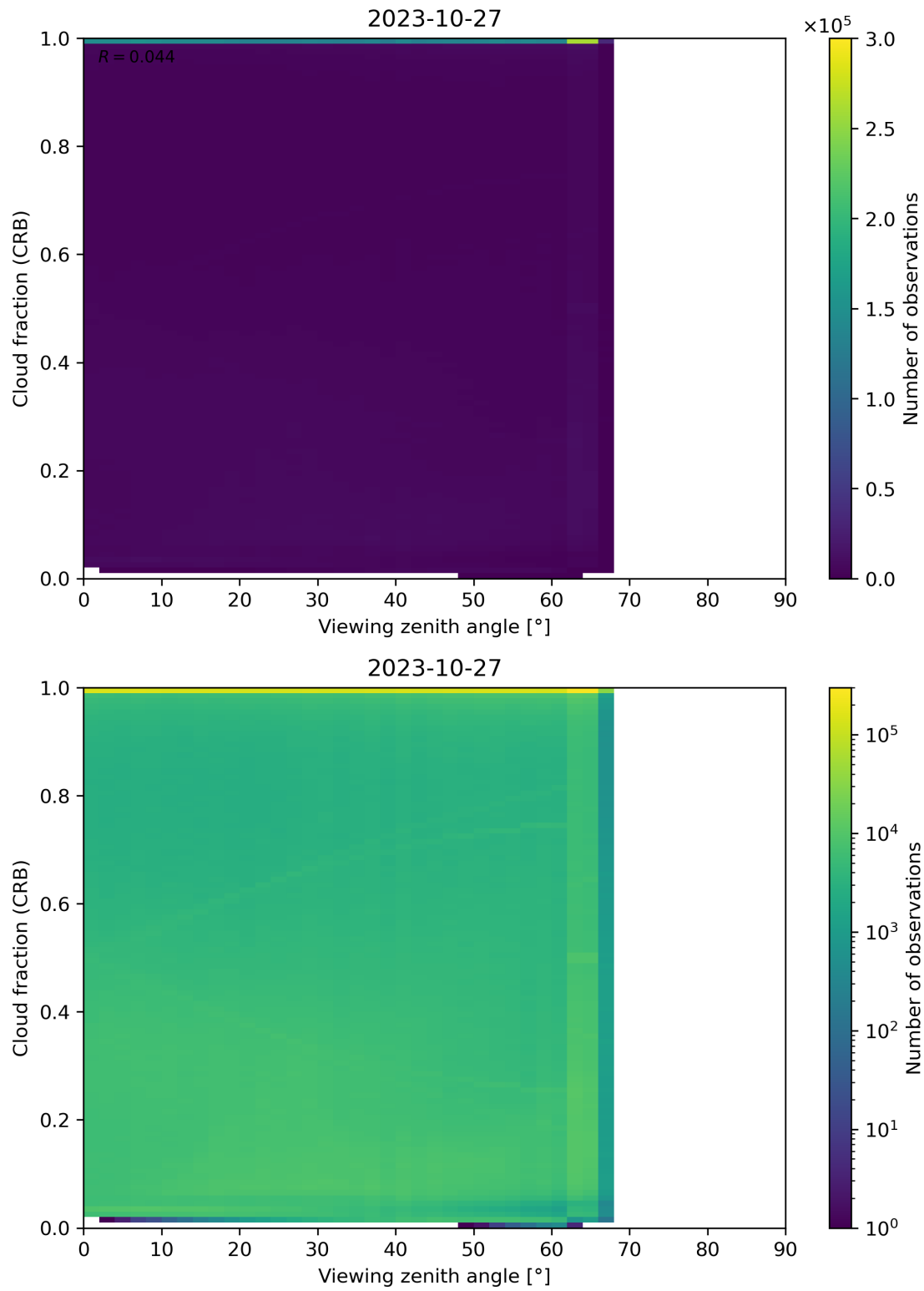
Figure 109: Scatter density plot of “Viewing zenith angle” against “Cloud fraction (CRB)” for 2023-10-27 to 2023-10-28.
