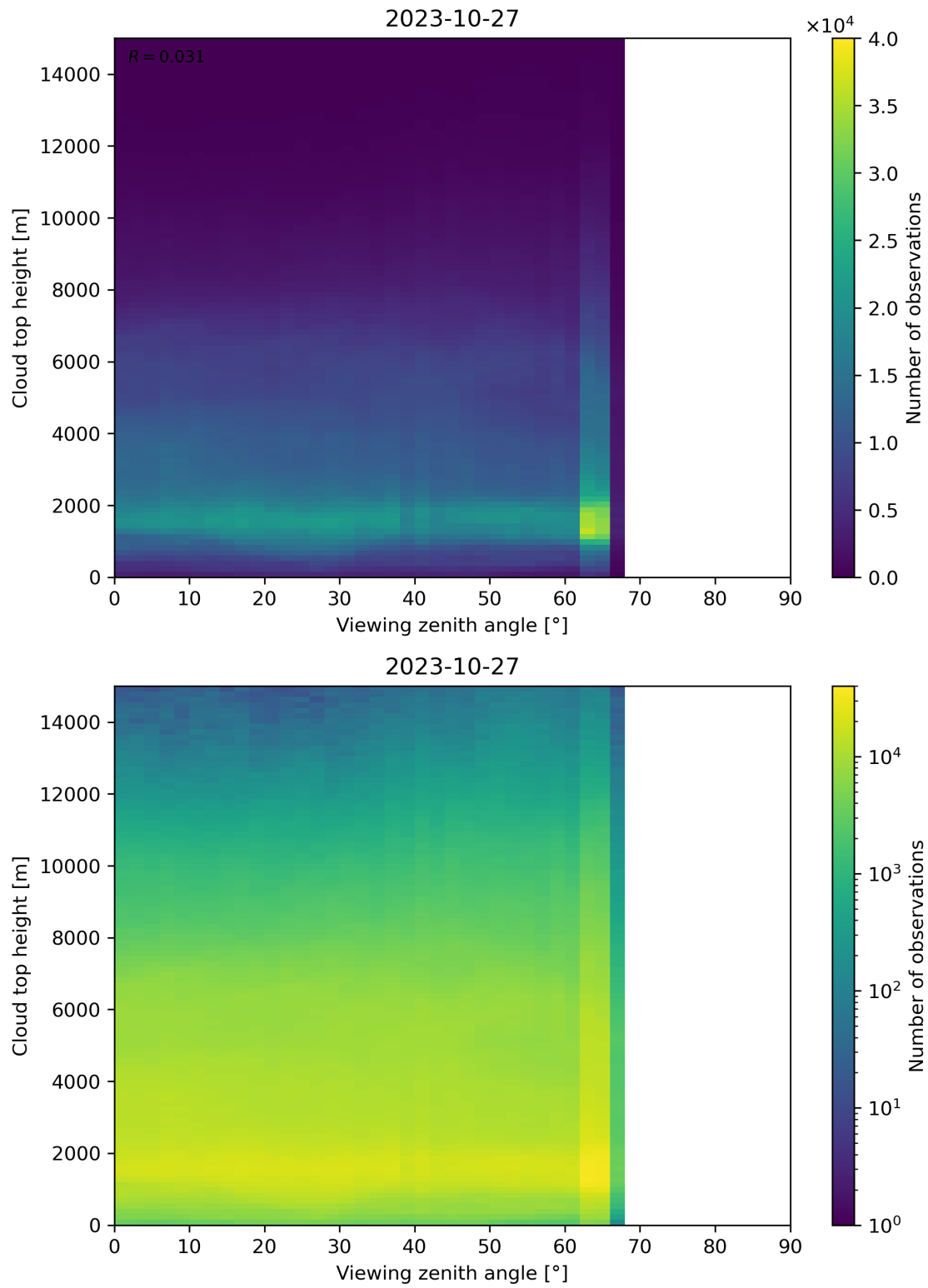
Figure 112: Scatter density plot of “Viewing zenith angle” against “Cloud top height” for 2023-10-27 to 2023-10-28.
