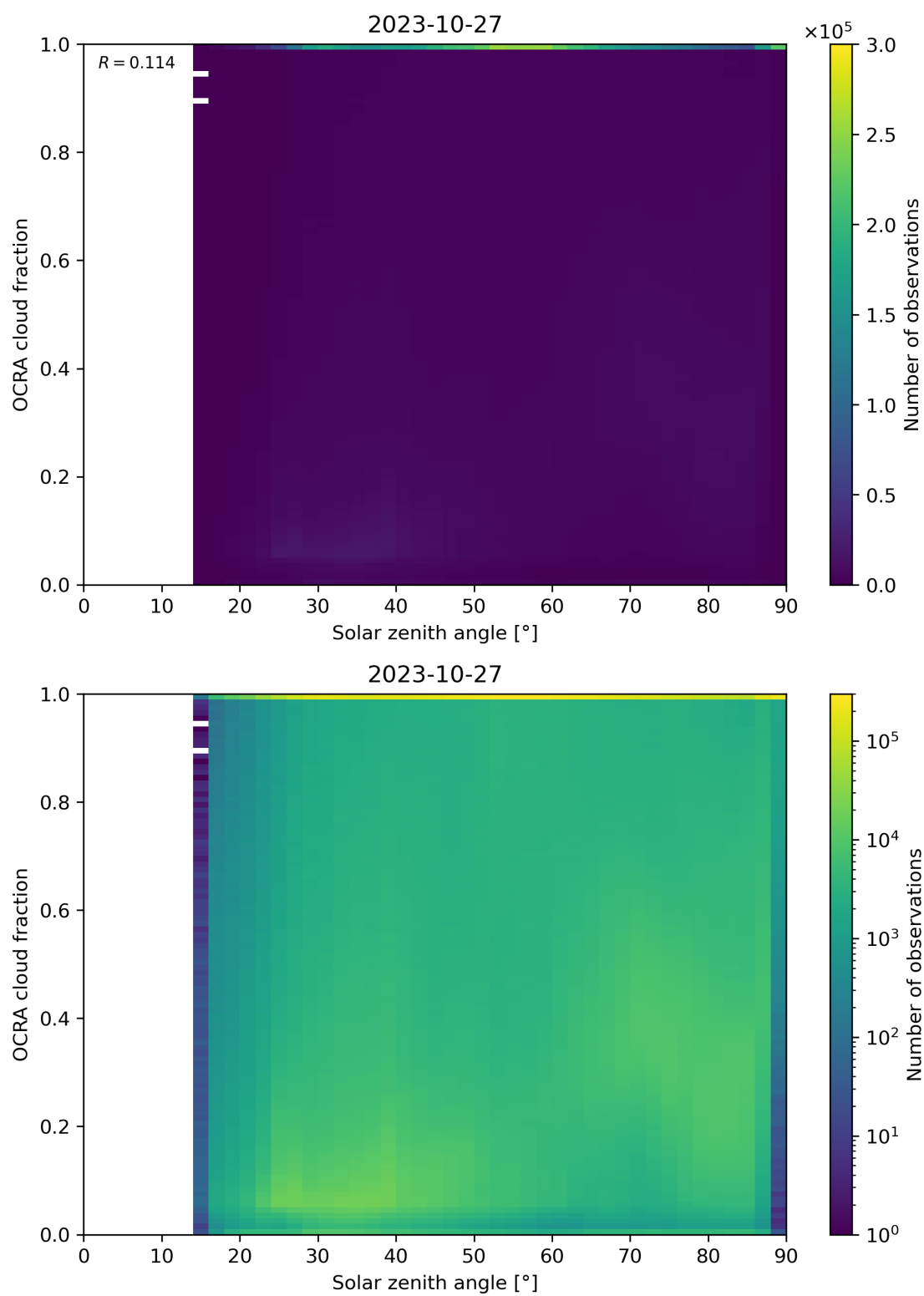
Figure 100: Scatter density plot of “Solar zenith angle” against “OCRA cloud fraction” for 2023-10-27 to 2023-10-28.
