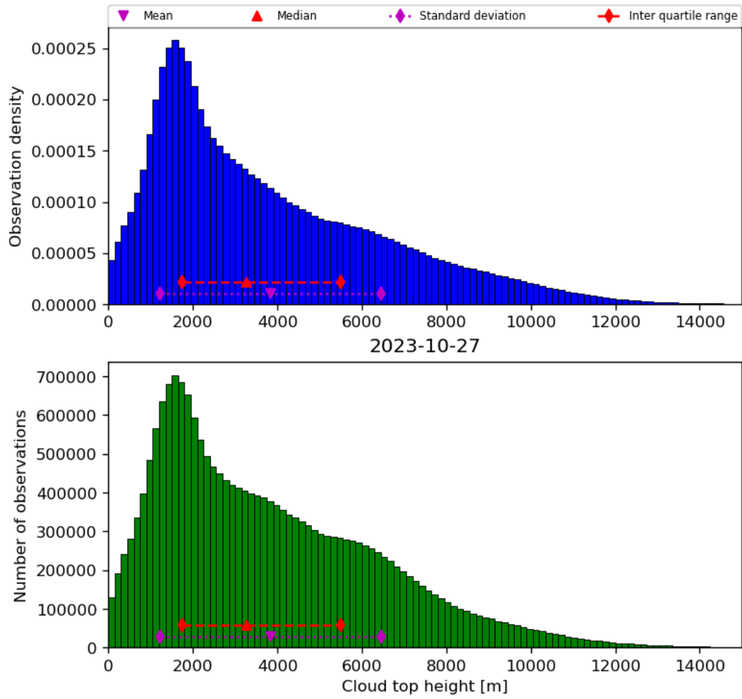
Figure 40: Histogram of “Cloud top height” for 2023-10-27 to 2023-10-28
