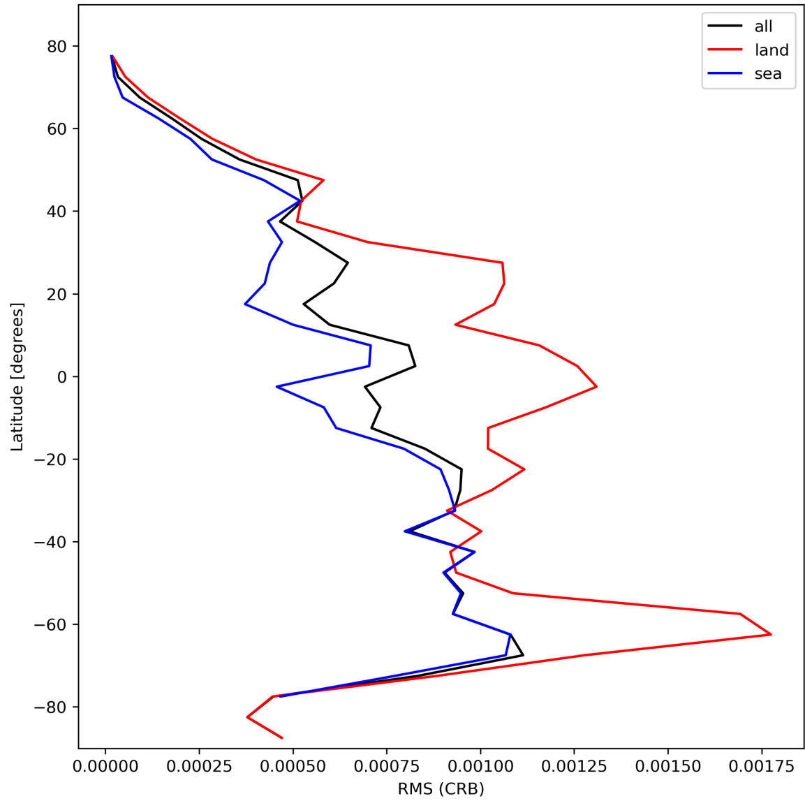
Figure 32: Zonal average of “RMS (CRB)” for 2023-10-27 to 2023-10-28.
