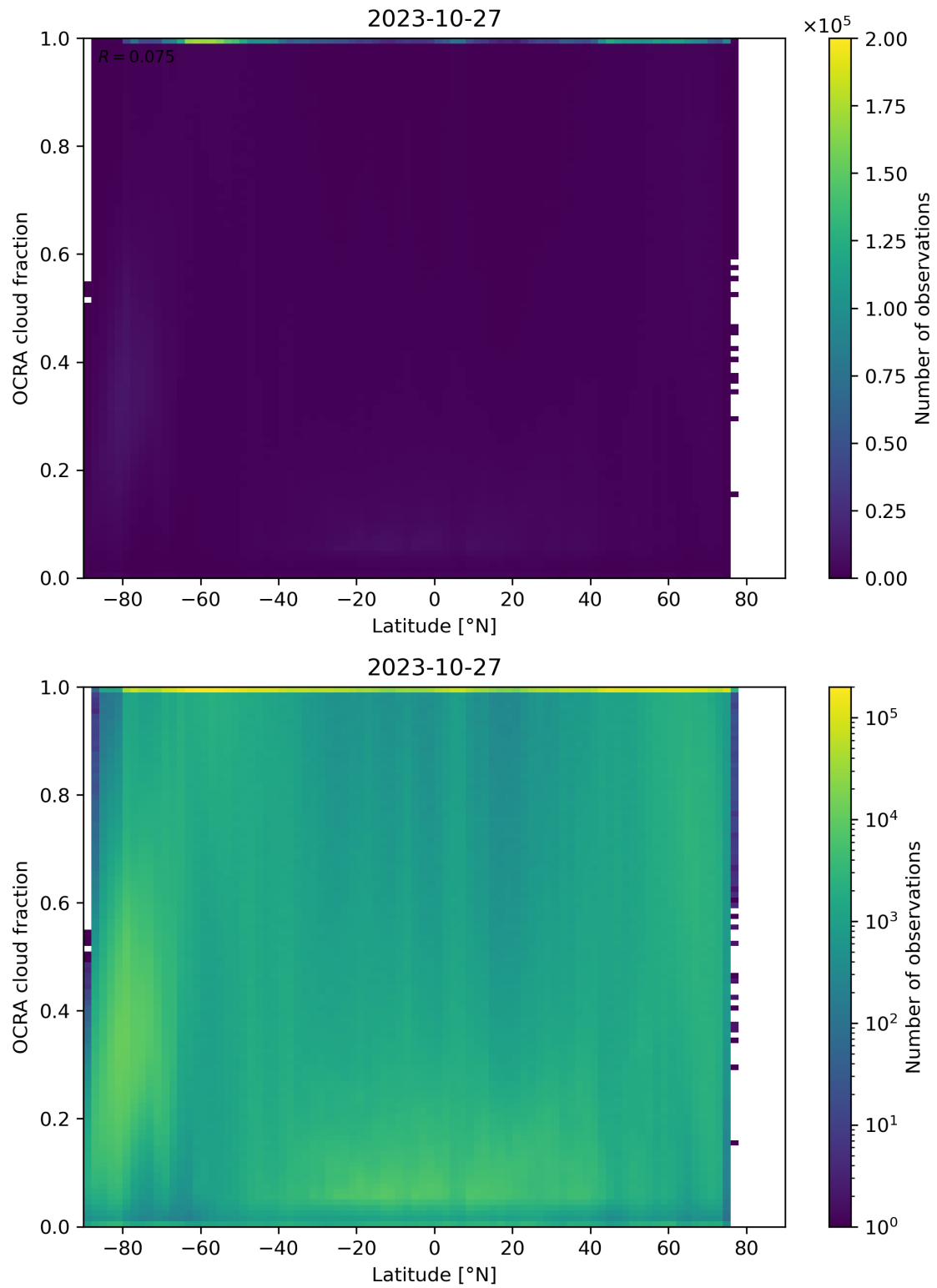
Figure 93: Scatter density plot of “Latitude” against “OCRA cloud fraction” for 2023-10-27 to 2023-10-28.
