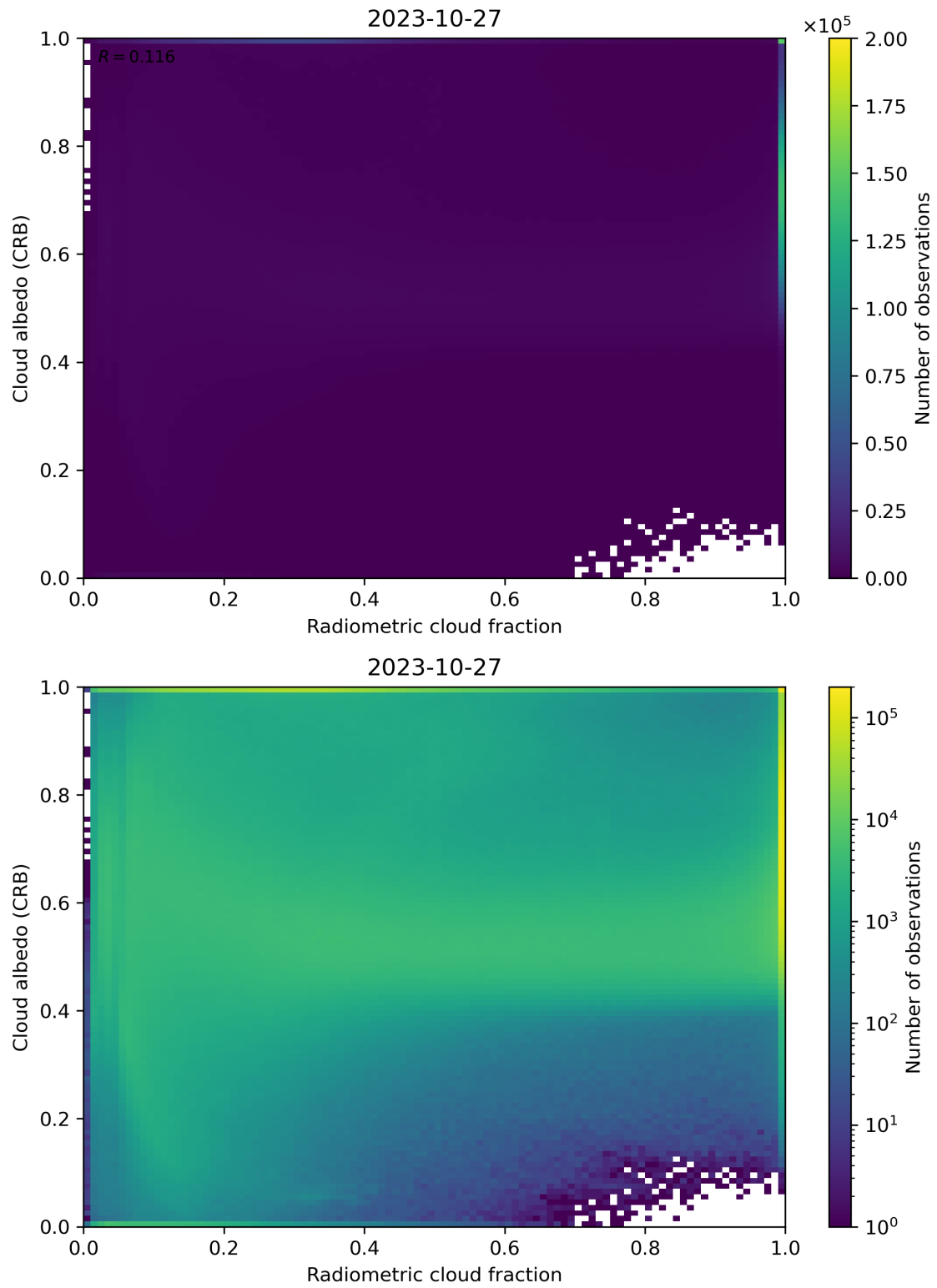
Figure 71: Scatter density plot of “Radiometric cloud fraction” against “Cloud albedo (CRB)” for 2023-10-27 to 2023-10-28.
