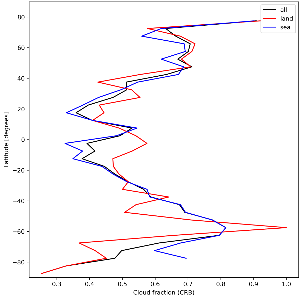
Figure 26: Zonal average of “Cloud fraction (CRB)” for 2023-10-27 to 2023-10-28.
