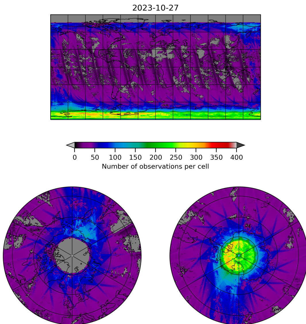
Figure 21: Map of the number of observations for 2023-10-27 to 2023-10-28
