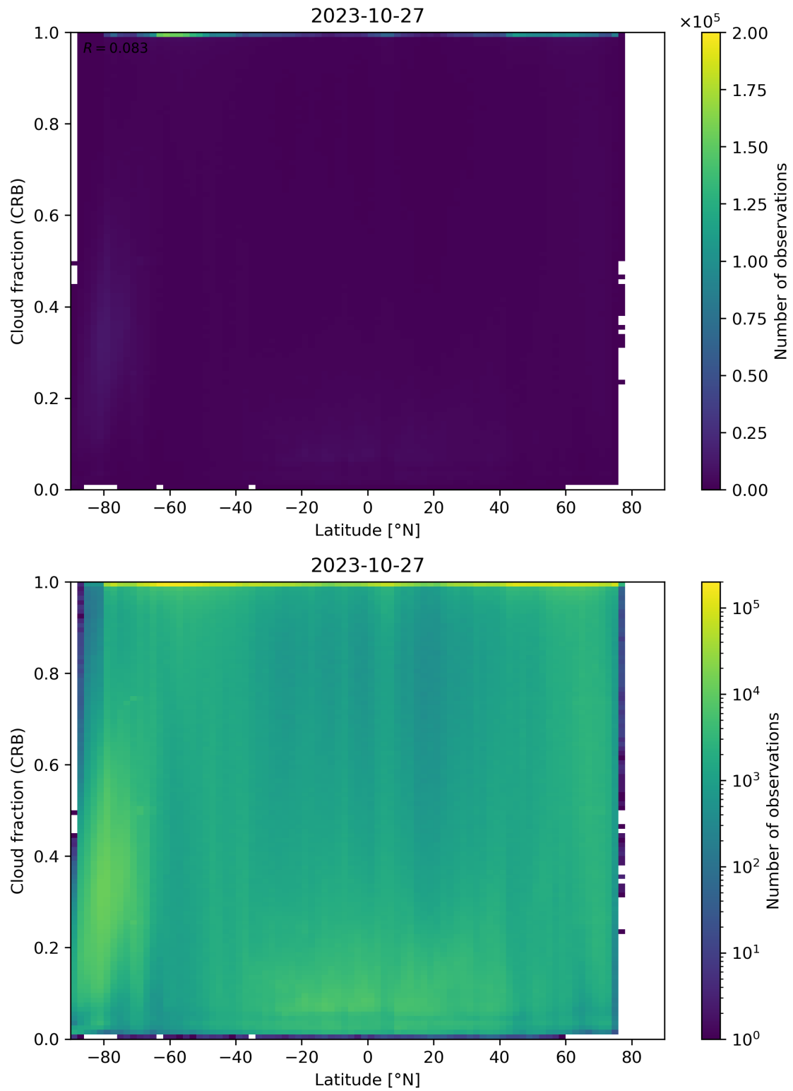
Figure 94: Scatter density plot of “Latitude” against “Cloud fraction (CRB)” for 2023-10-27 to 2023-10-28.
