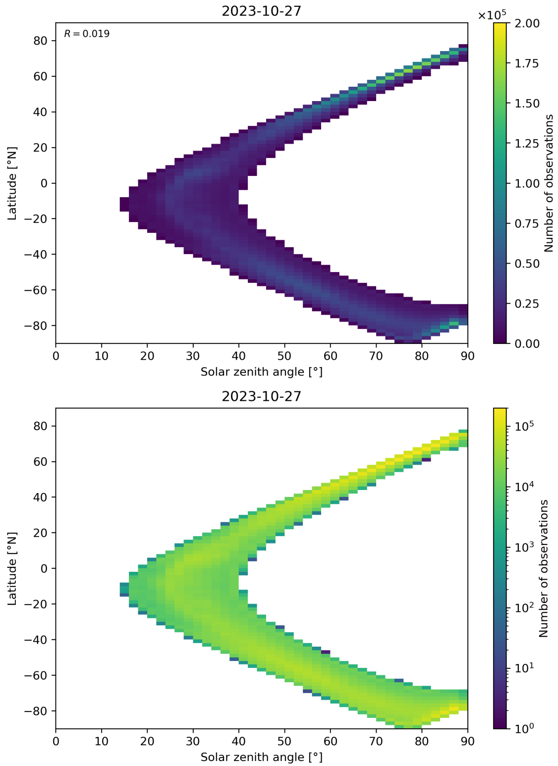
Figure 105: Scatter density plot of “Solar zenith angle” against “Latitude” for 2023-10-27 to 2023-10-28.
