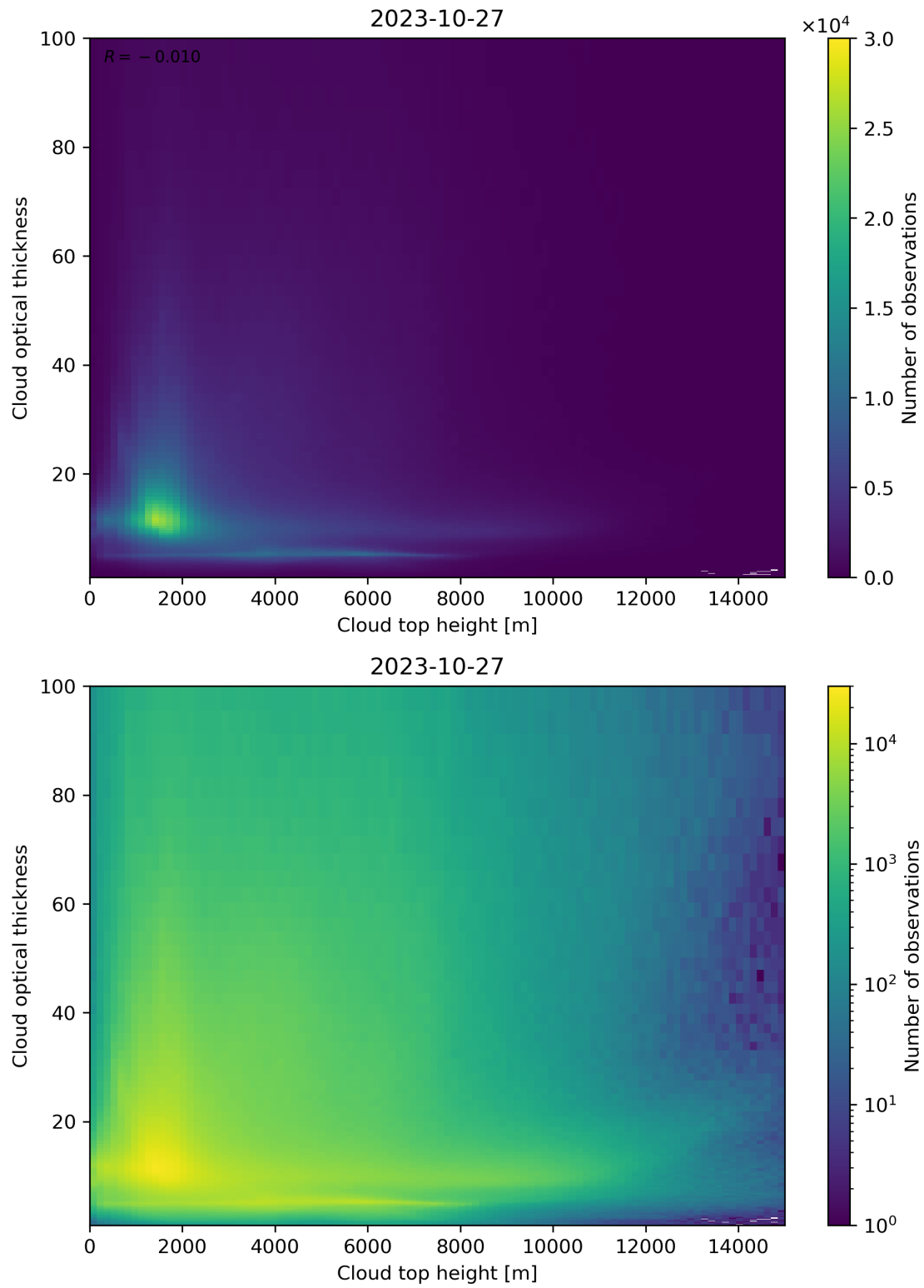
Figure 90: Scatter density plot of “Cloud top height” against “Cloud optical thickness” for 2023-10-27 to 2023-10-28.
