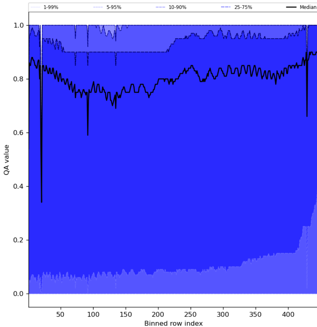
Figure 54: Along track statistics of “QA value” for 2023-10-27 to 2023-10-28
