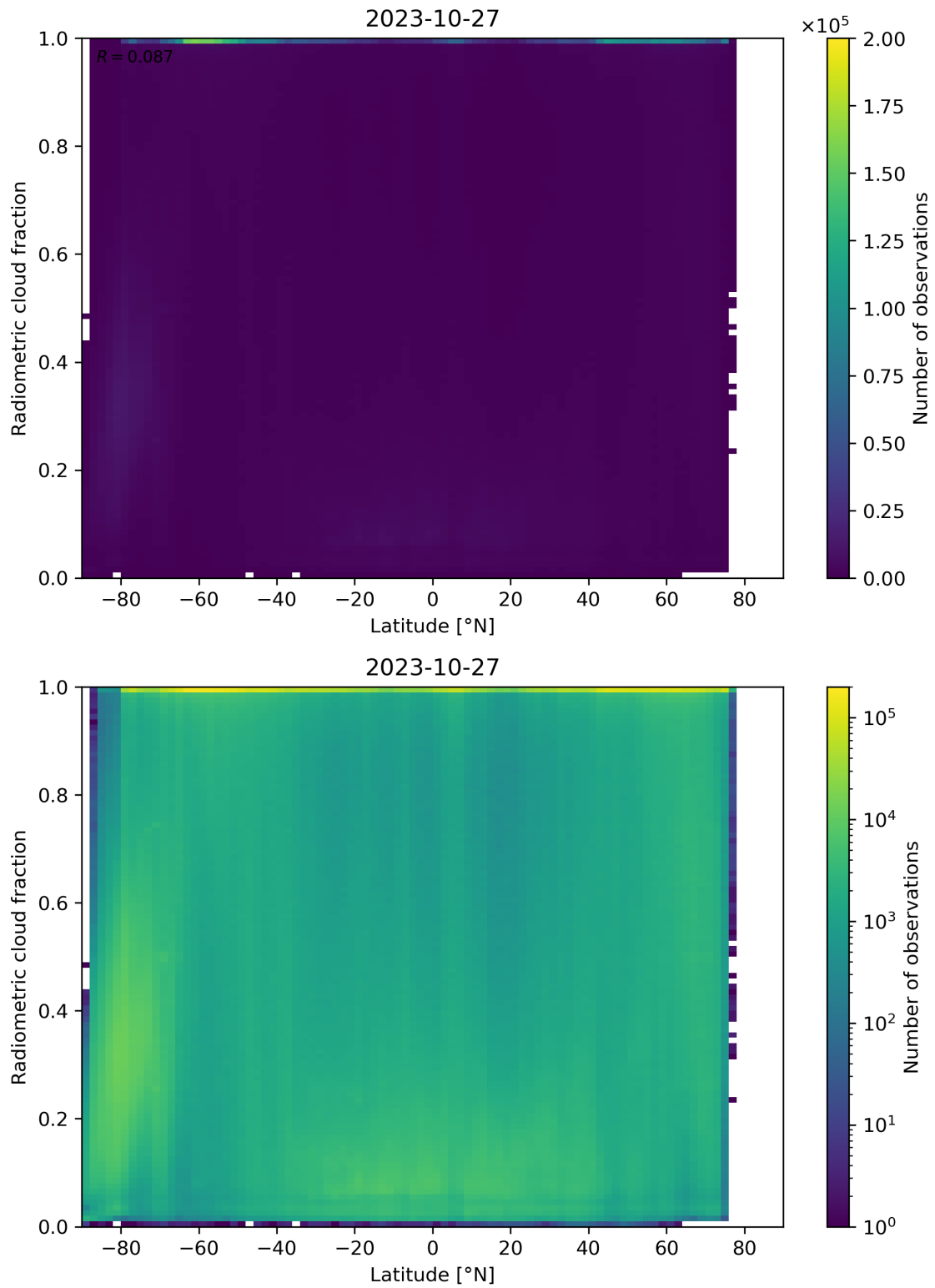
Figure 92: Scatter density plot of “Latitude” against “Radiometric cloud fraction” for 2023-10-27 to 2023-10-28.
