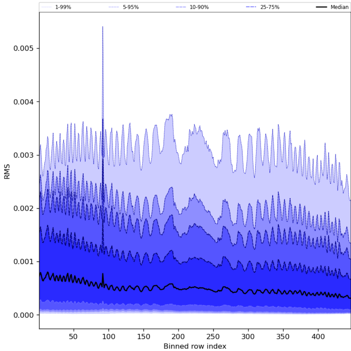
Figure 63: Along track statistics of “RMS” for 2023-10-27 to 2023-10-28
