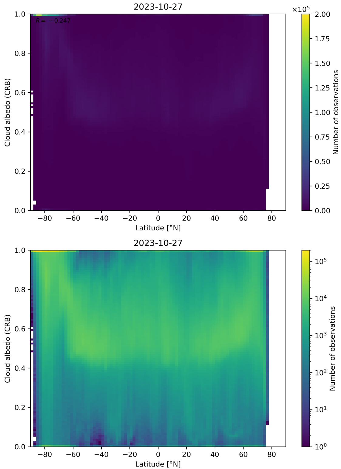
Figure 91: Scatter density plot of “Latitude” against “Cloud albedo (CRB)” for 2023-10-27 to 2023-10-28.
