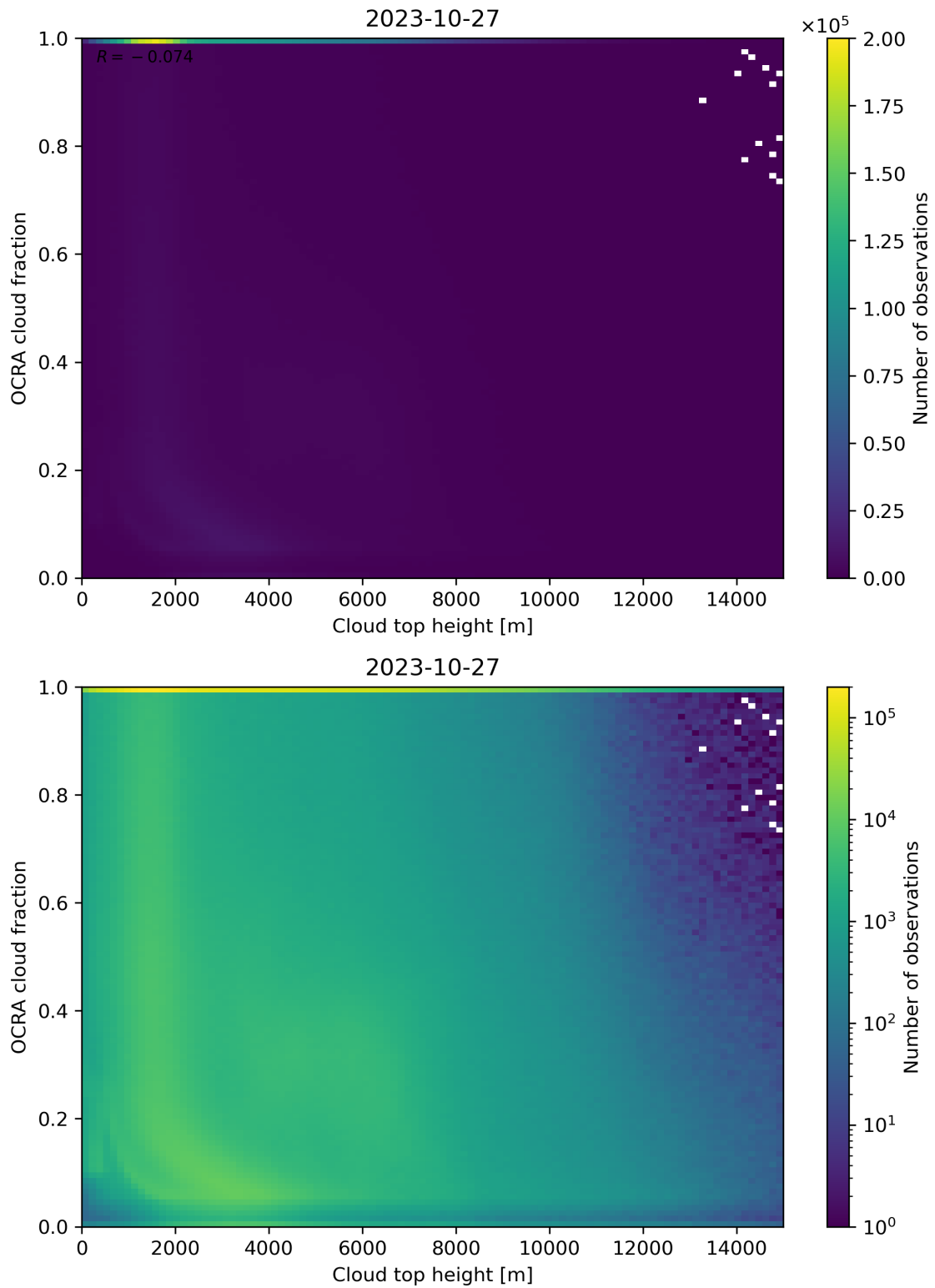
Figure 87: Scatter density plot of “Cloud top height” against “OCRA cloud fraction” for 2023-10-27 to 2023-10-28.
