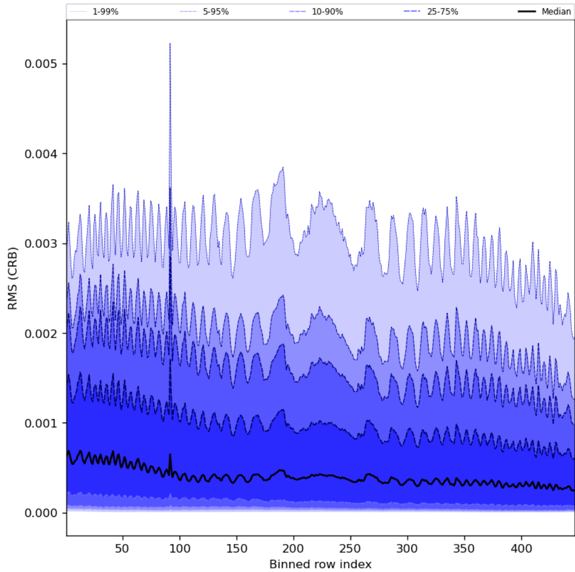
Figure 64: Along track statistics of “RMS (CRB)” for 2023-10-27 to 2023-10-28
