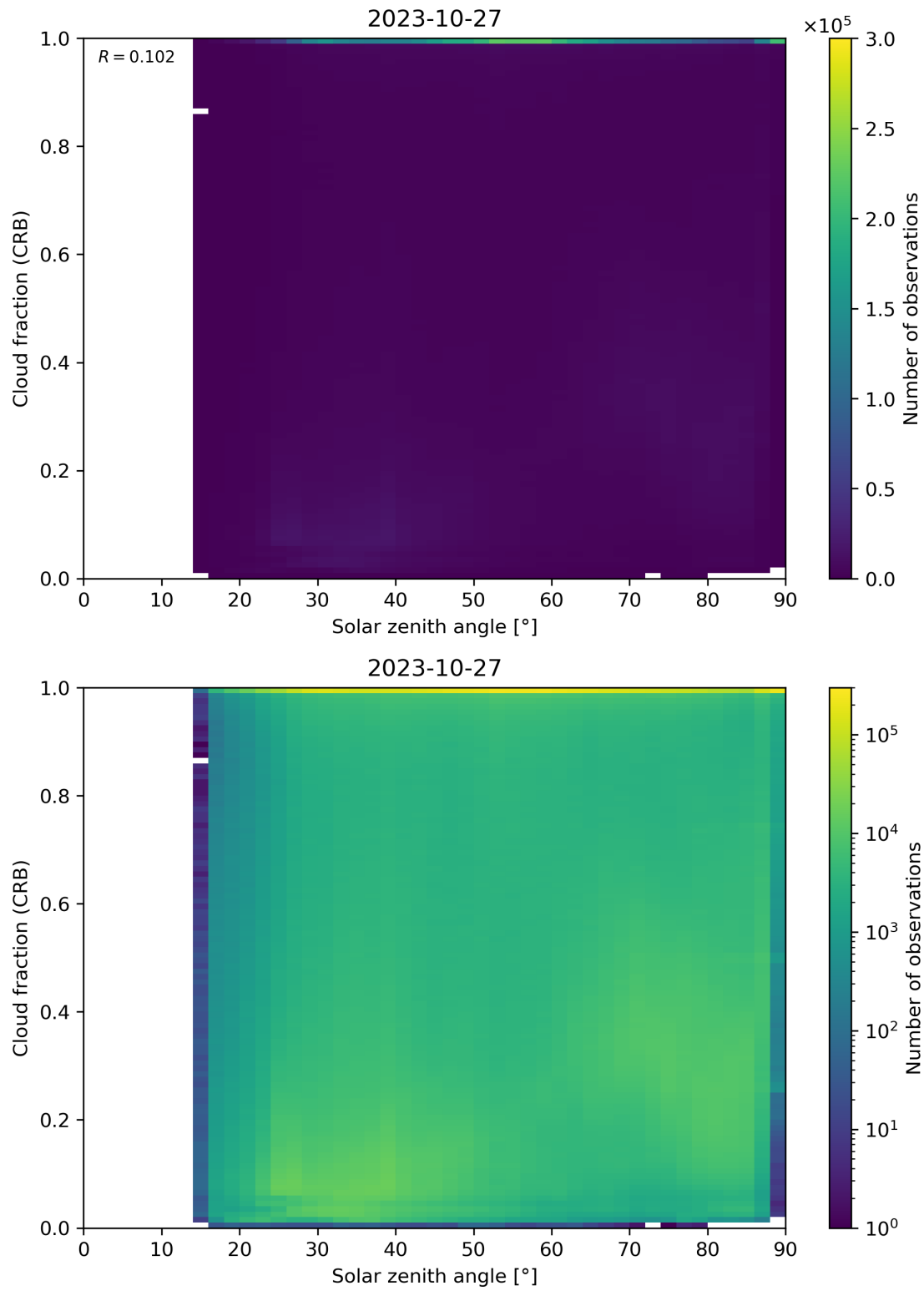
Figure 101: Scatter density plot of “Solar zenith angle” against “Cloud fraction (CRB)” for 2023-10-27 to 2023-10-28.
