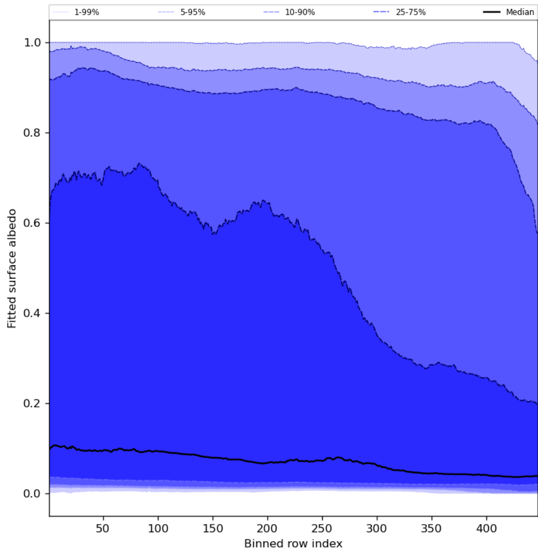
Figure 61: Along track statistics of “Fitted surface albedo” for 2023-10-27 to 2023-10-28
