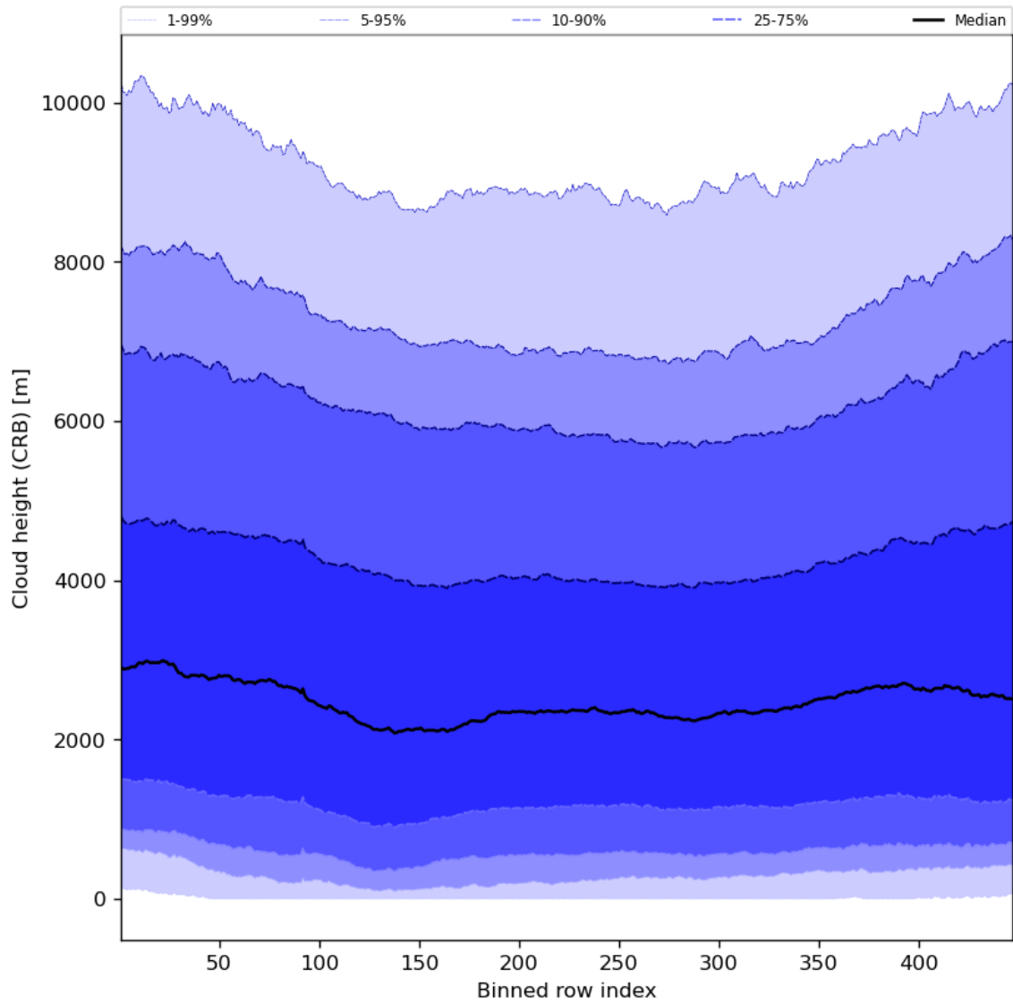
Figure 59: Along track statistics of “Cloud height (CRB)” for 2023-10-27 to 2023-10-28
