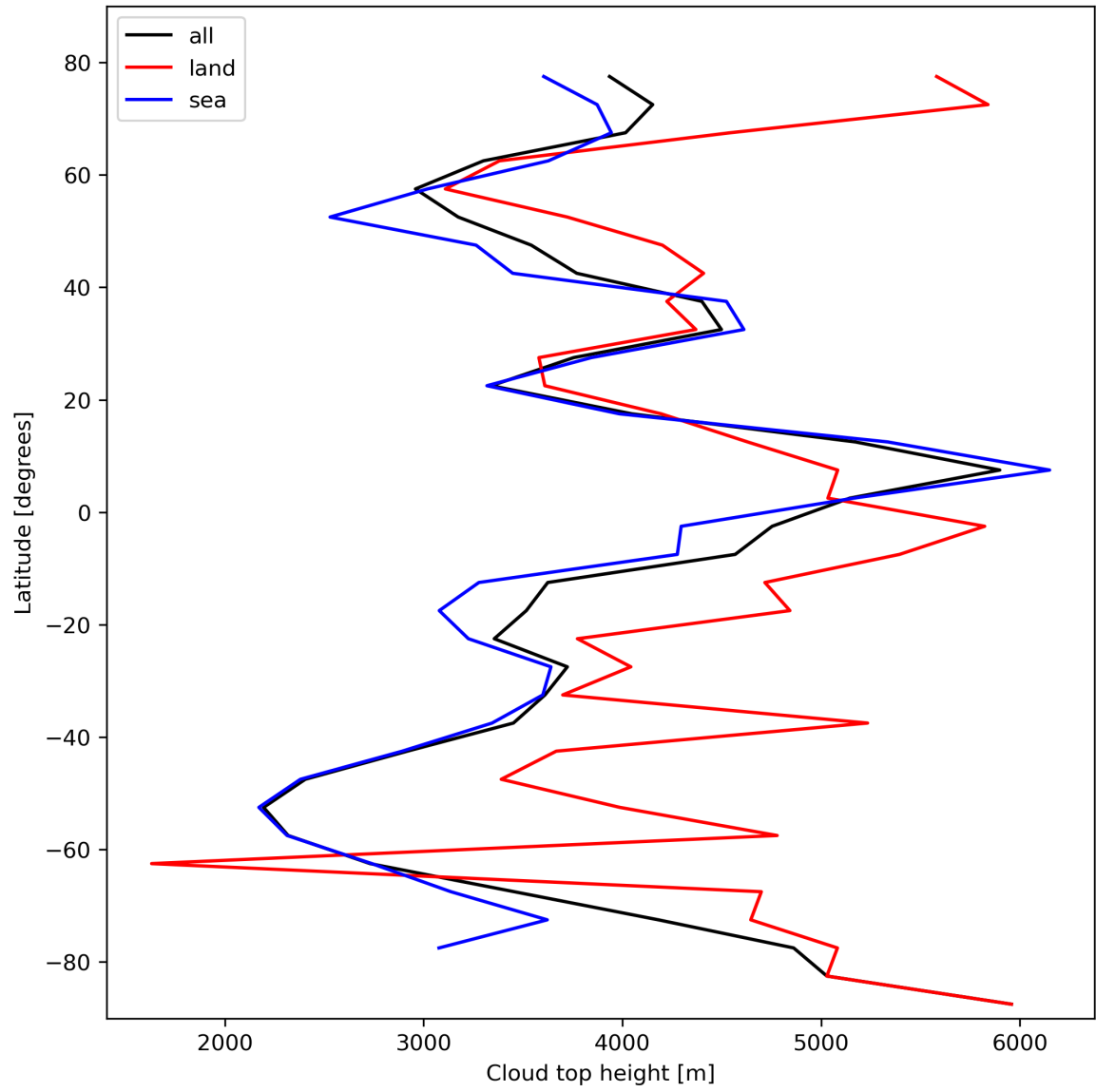
Figure 24: Zonal average of “Cloud top height” for 2023-10-27 to 2023-10-28.
