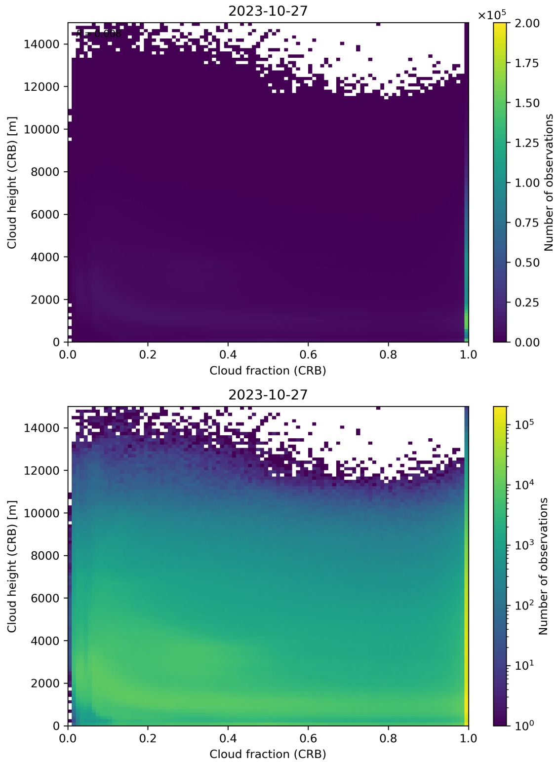
Figure 79: Scatter density plot of “Cloud fraction (CRB)” against “Cloud height (CRB)” for 2023-10-27 to 2023-10-28.
