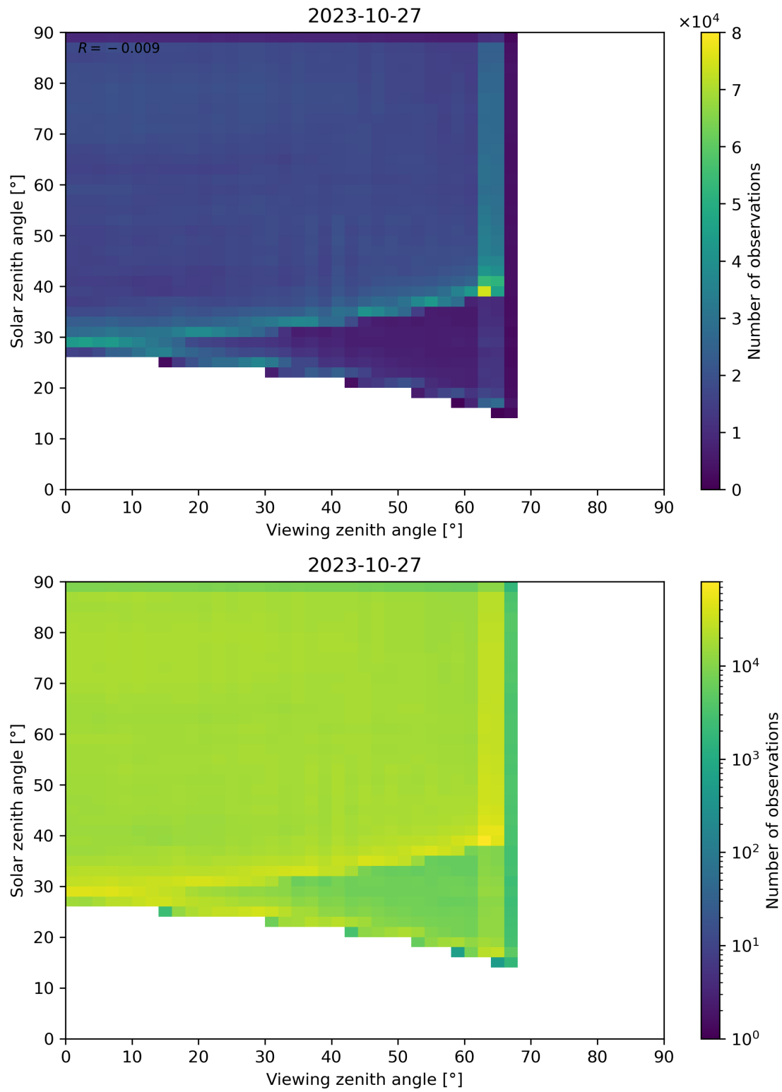
Figure 114: Scatter density plot of “Viewing zenith angle” against “Solar zenith angle” for 2023-10-27 to 2023-10-28.
