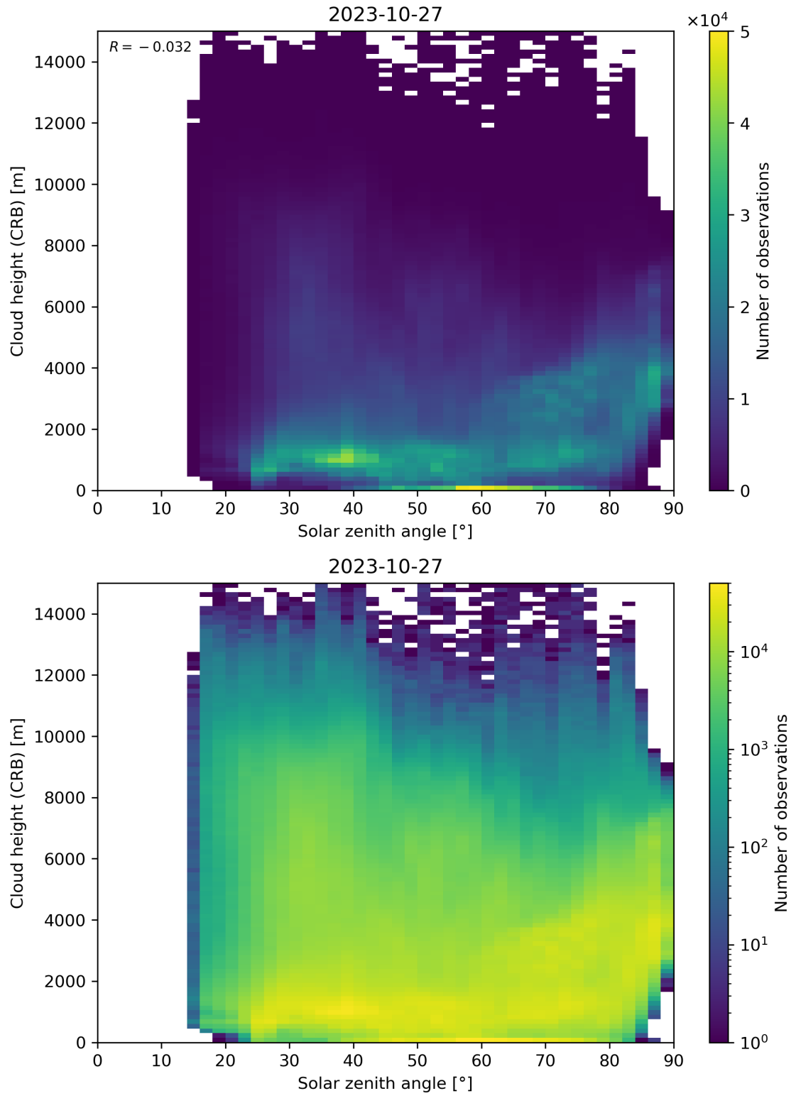
Figure 102: Scatter density plot of “Solar zenith angle” against “Cloud height (CRB)” for 2023-10-27 to 2023-10-28.
