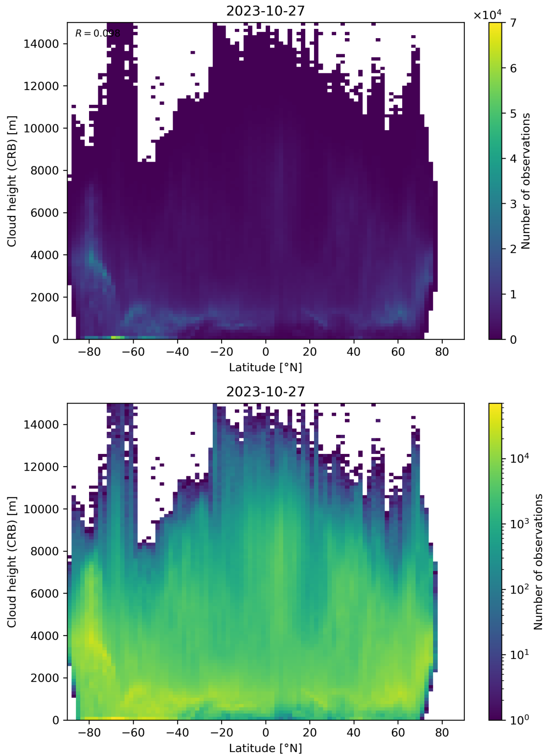
Figure 95: Scatter density plot of “Latitude” against “Cloud height (CRB)” for 2023-10-27 to 2023-10-28.
