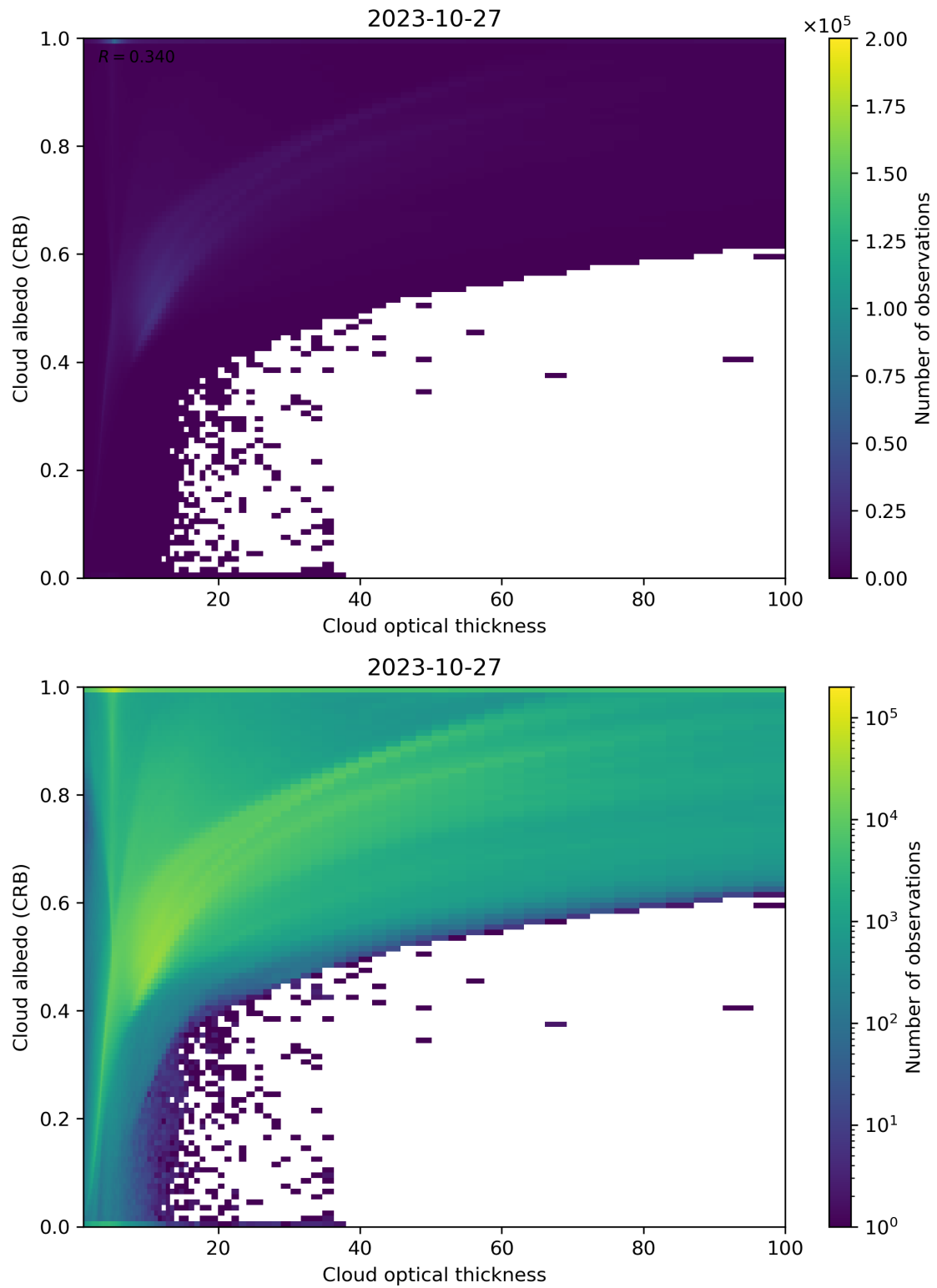
Figure 82: Scatter density plot of “Cloud optical thickness” against “Cloud albedo (CRB)” for 2023-10-27 to 2023-10-28.
