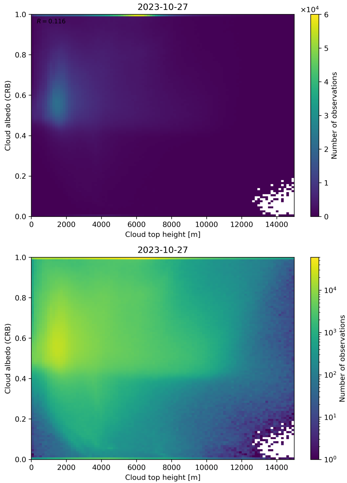
Figure 86: Scatter density plot of “Cloud top height” against “Cloud albedo (CRB)” for 2023-10-27 to 2023-10-28.
