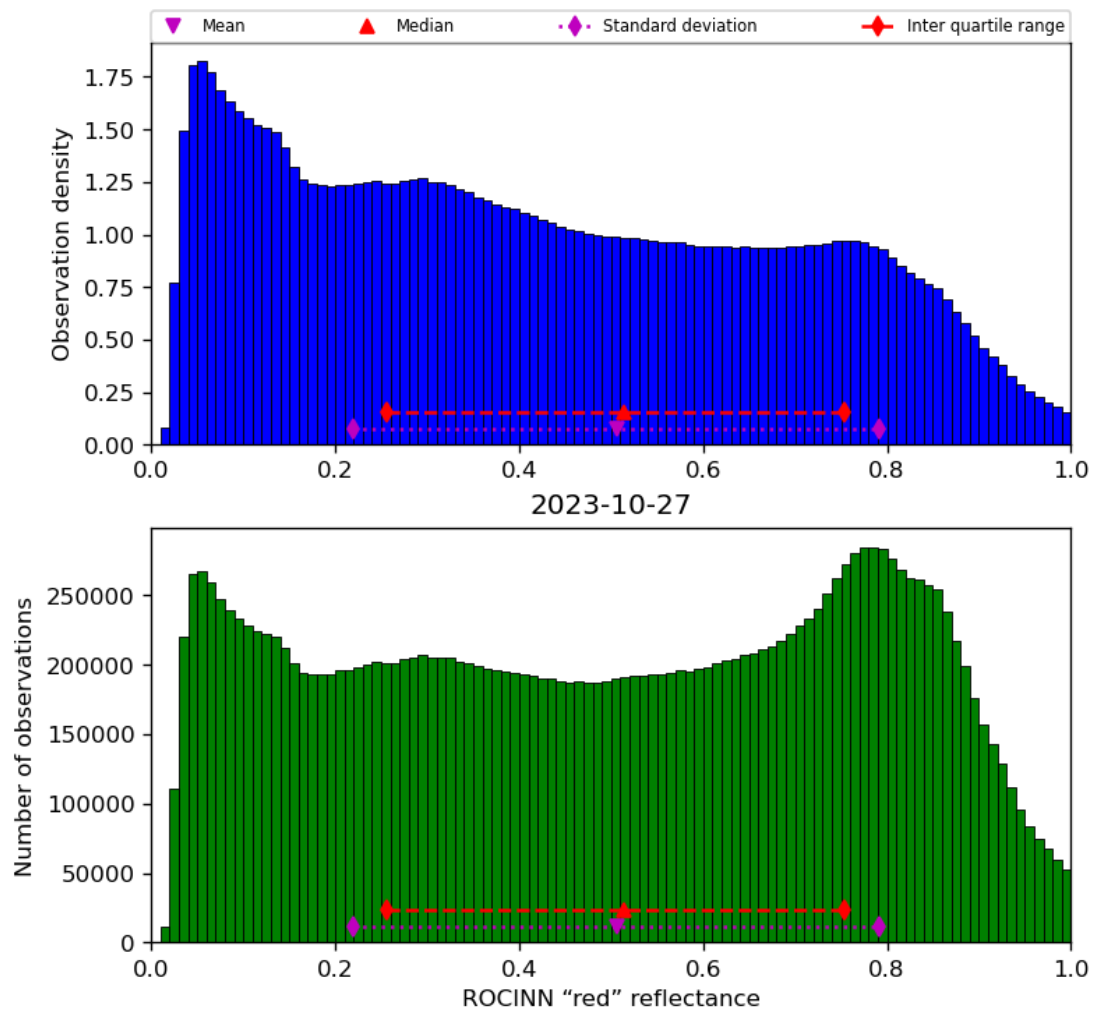
Figure 53: Histogram of “ROCINN “red” reflectance” for 2023-10-27 to 2023-10-28
