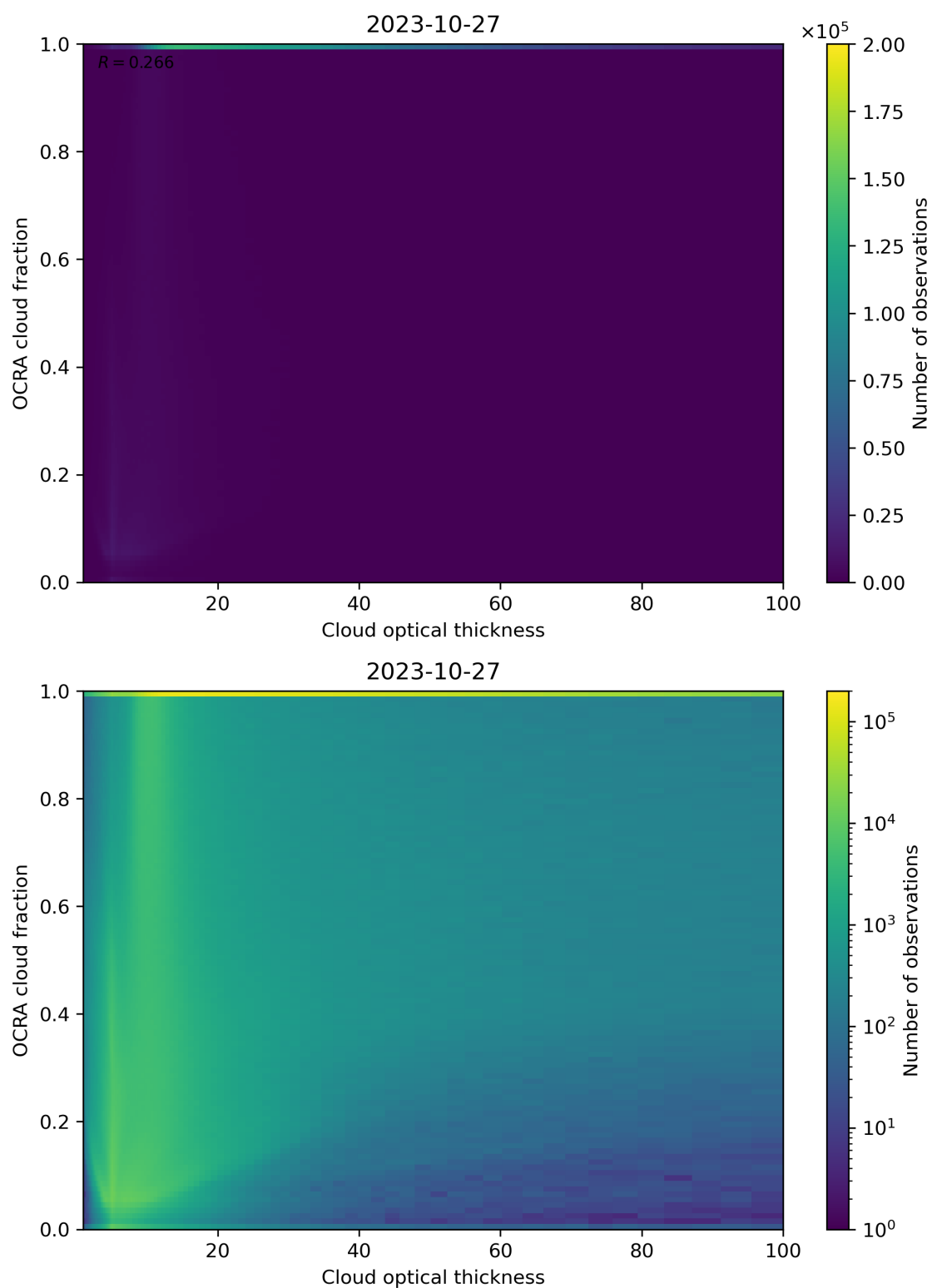
Figure 83: Scatter density plot of “Cloud optical thickness” against “OCRA cloud fraction” for 2023-10-27 to 2023-10-28.
