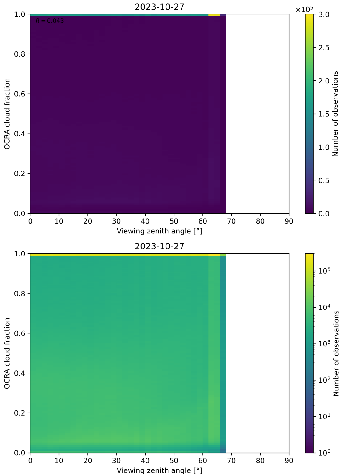
Figure 108: Scatter density plot of “Viewing zenith angle” against “OCRA cloud fraction” for 2023-10-27 to 2023-10-28.
