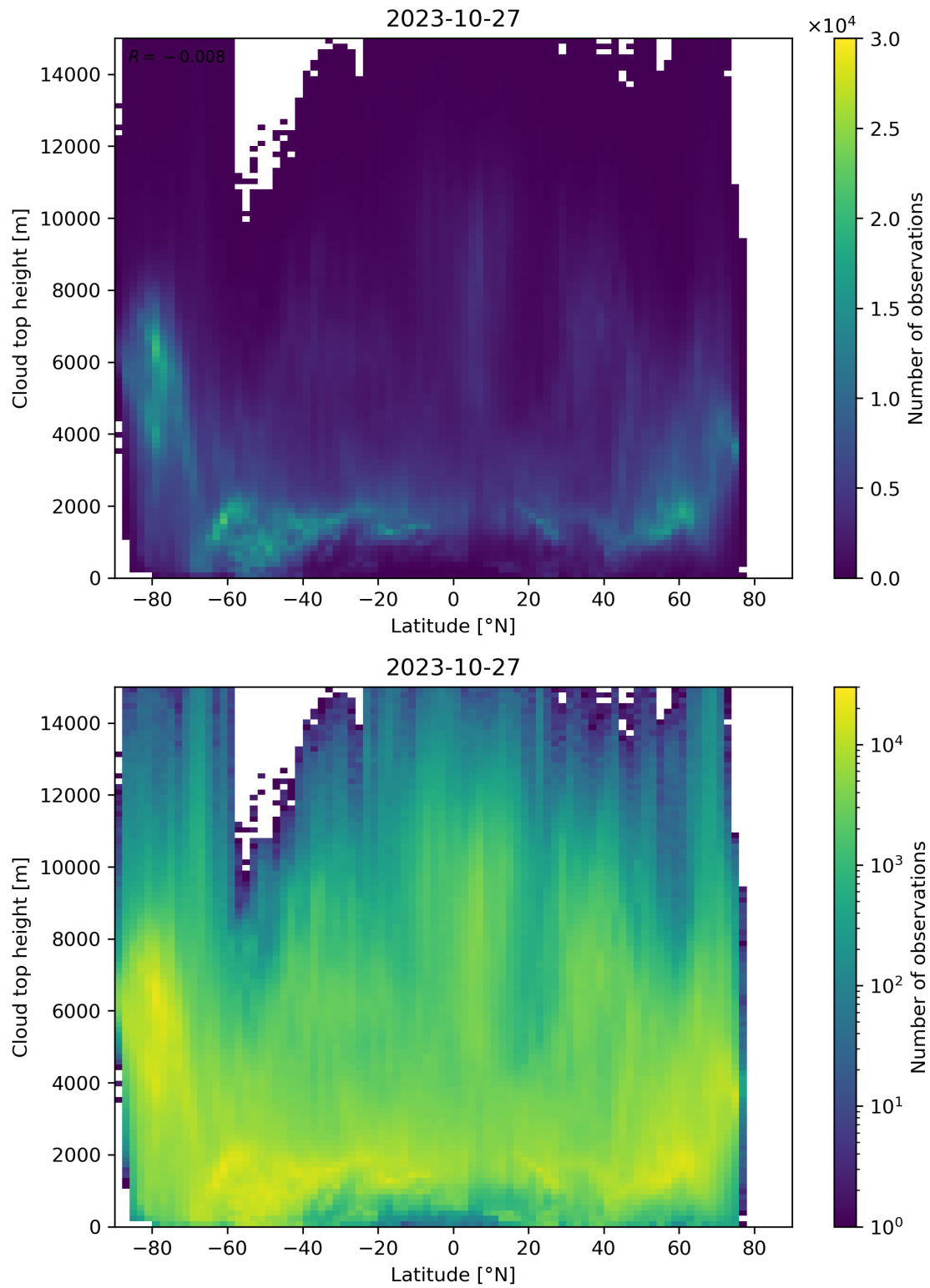
Figure 97: Scatter density plot of “Latitude” against “Cloud top height” for 2023-10-27 to 2023-10-28.
