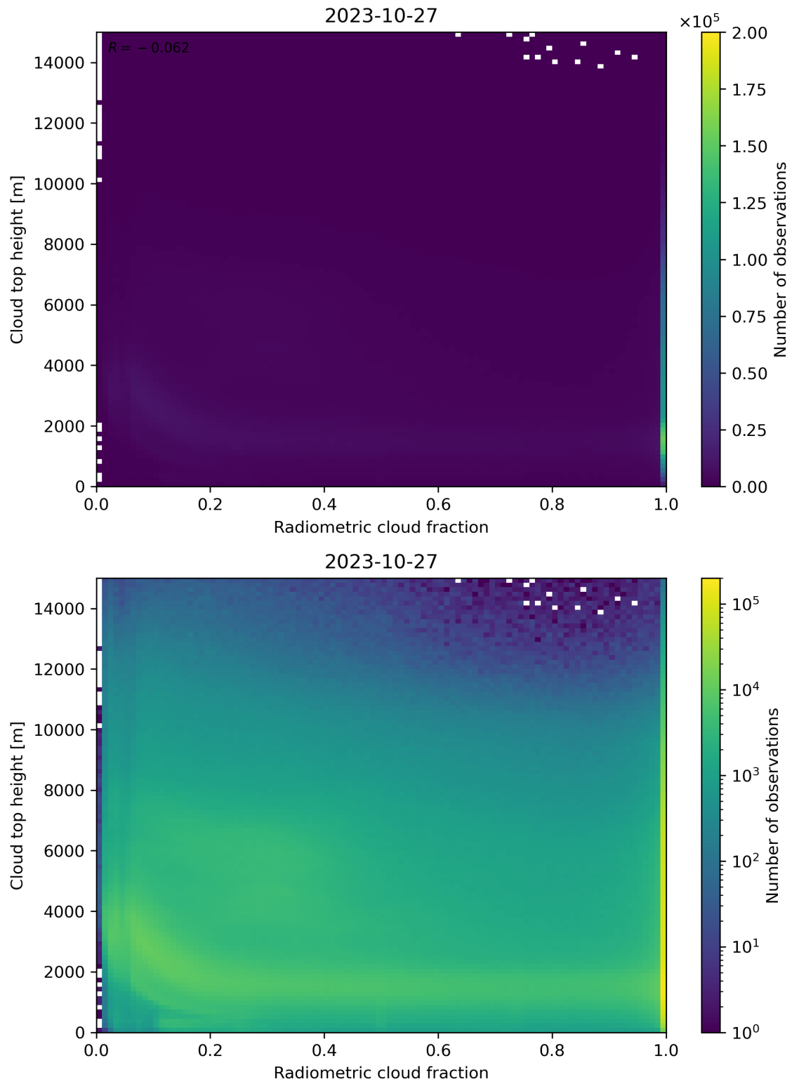
Figure 76: Scatter density plot of “Radiometric cloud fraction” against “Cloud top height” for 2023-10-27 to 2023-10-28.
