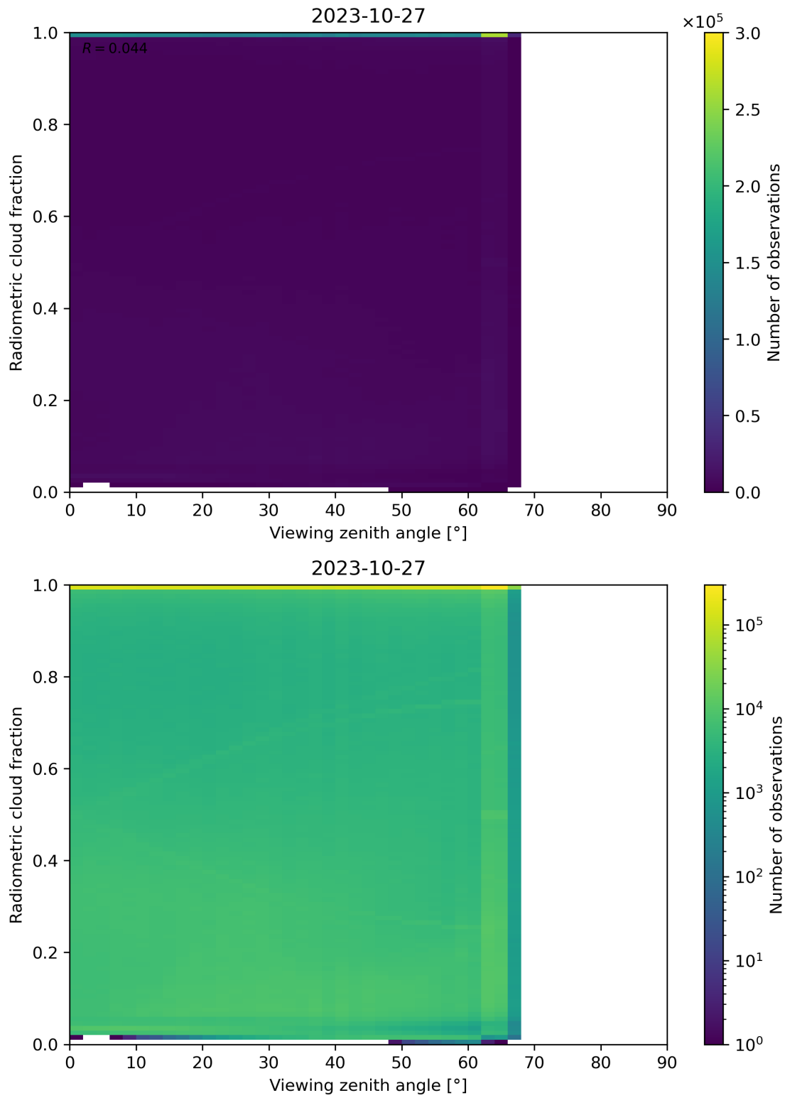
Figure 107: Scatter density plot of “Viewing zenith angle” against “Radiometric cloud fraction” for 2023-10-27 to 2023-10-28.
