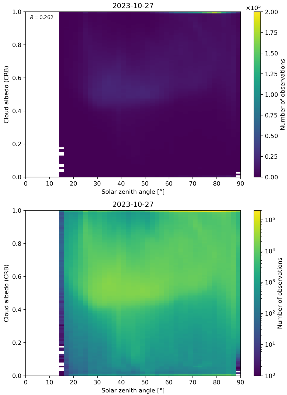
Figure 98: Scatter density plot of “Solar zenith angle” against “Cloud albedo (CRB)” for 2023-10-27 to 2023-10-28.
