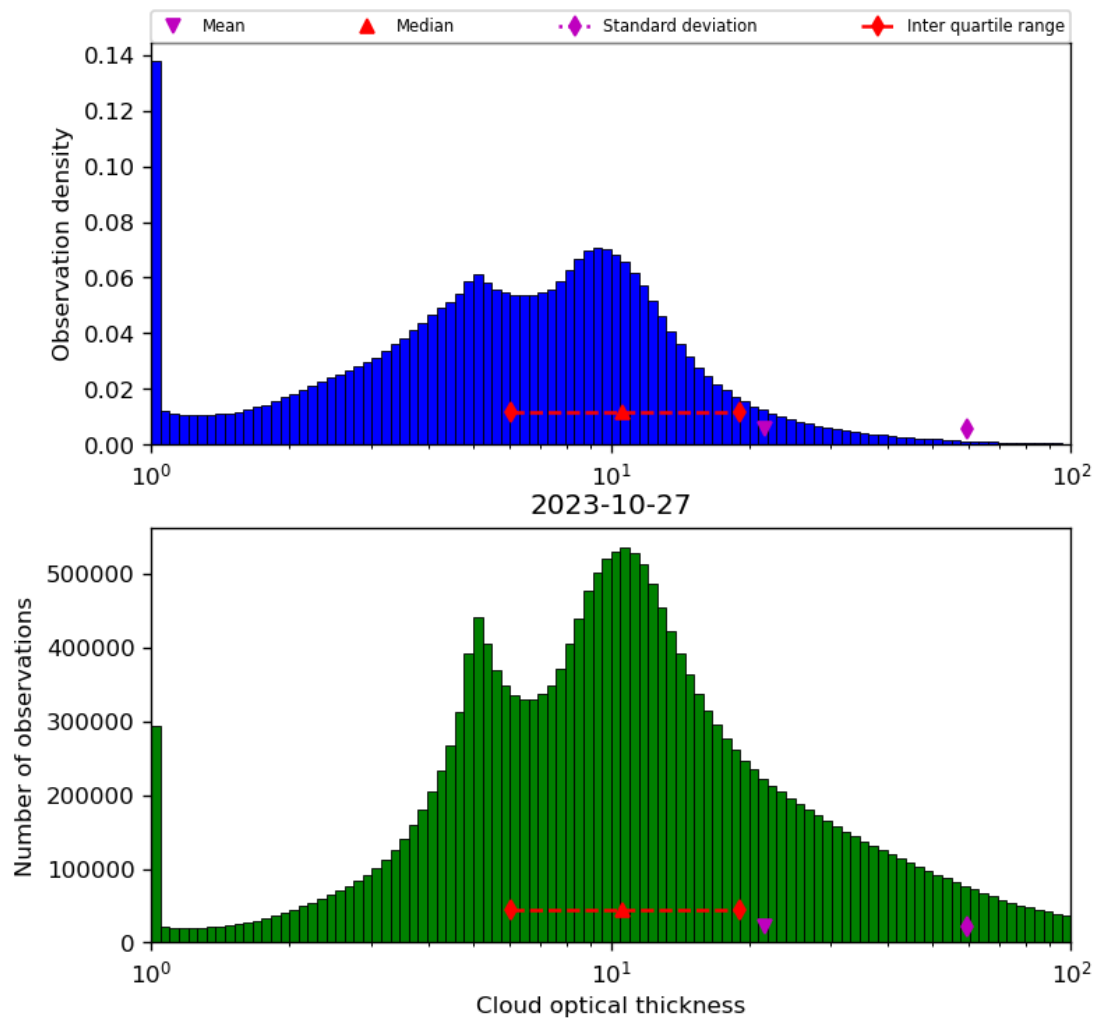
Figure 41: Histogram of “Cloud optical thickness” for 2023-10-27 to 2023-10-28
