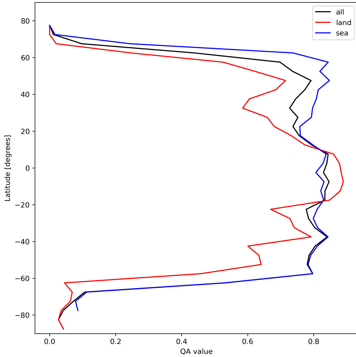
Figure 22: Zonal average of “QA value” for 2023-10-27 to 2023-10-28.
