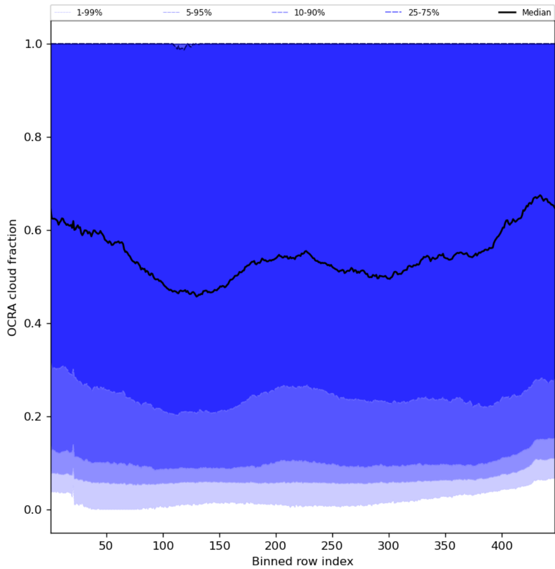
Figure 66: Along track statistics of “OCRA cloud fraction” for 2023-10-27 to 2023-10-28
