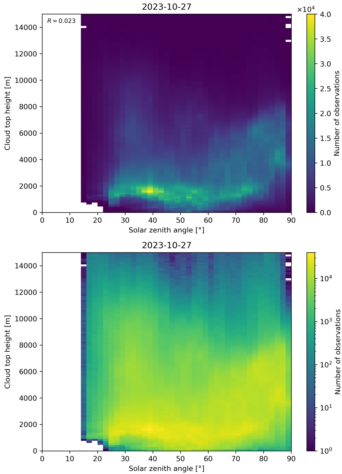
Figure 104: Scatter density plot of “Solar zenith angle” against “Cloud top height” for 2023-10-27 to 2023-10-28.
