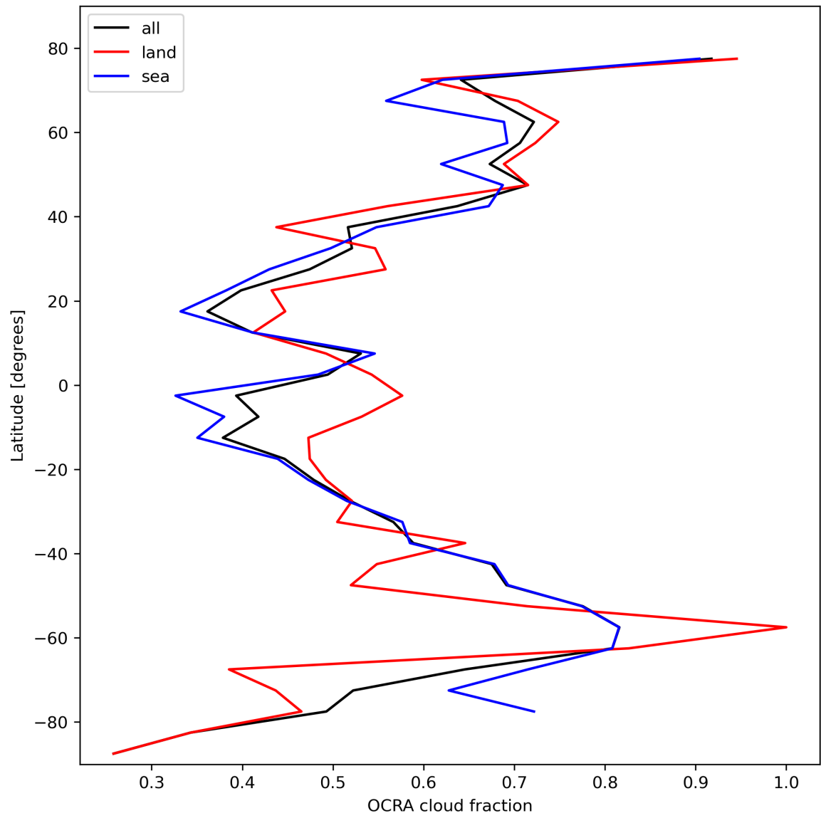
Figure 34: Zonal average of “OCRA cloud fraction” for 2023-10-27 to 2023-10-28.
