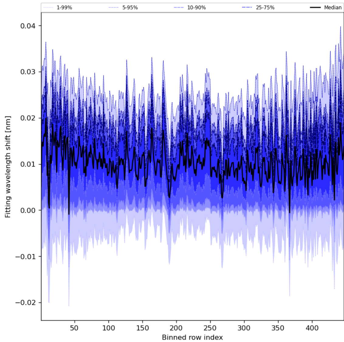
Figure 65: Along track statistics of “Fitting wavelength shift” for 2023-10-27 to 2023-10-28
