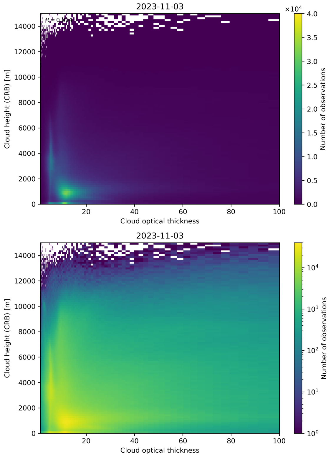
Figure 85: Scatter density plot of “Cloud optical thickness” against “Cloud height (CRB)” for 2023-11-02 to 2023-11-04.
