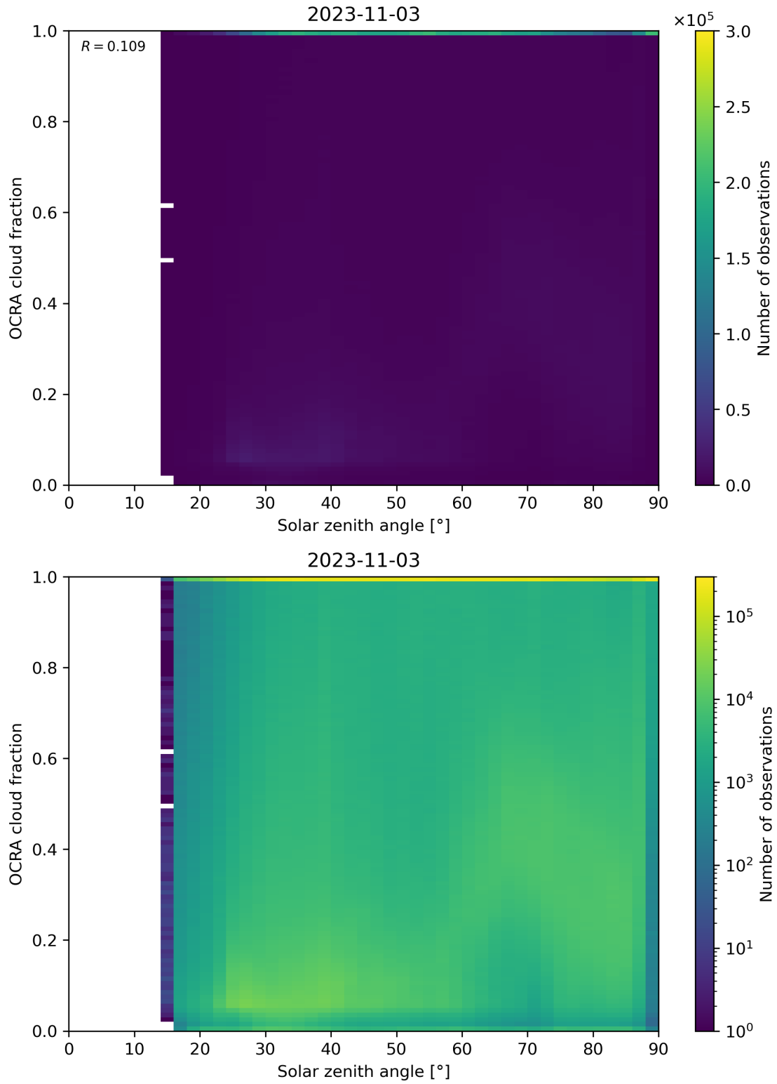
Figure 100: Scatter density plot of “Solar zenith angle” against “OCRA cloud fraction” for 2023-11-02 to 2023-11-04.
