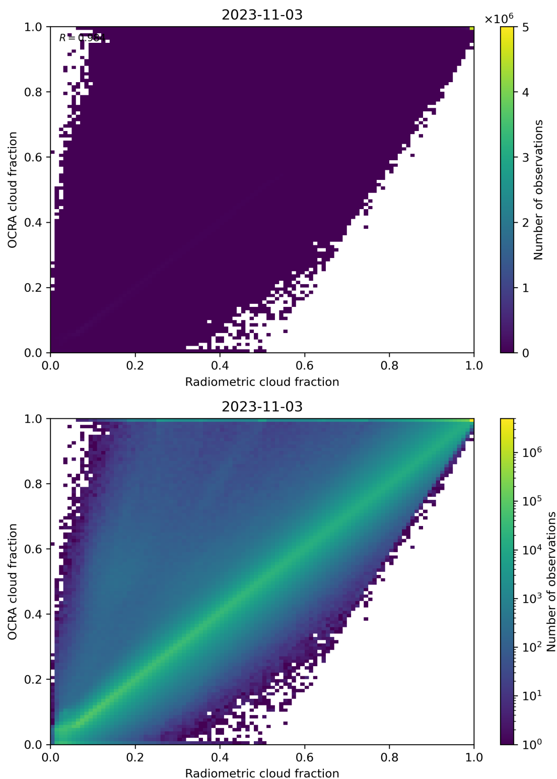
Figure 72: Scatter density plot of “Radiometric cloud fraction” against “OCRA cloud fraction” for 2023-11-02 to 2023-11-04.
