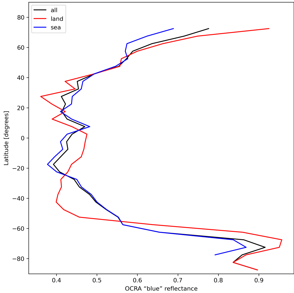
Figure 35: Zonal average of “OCRA “blue” reflectance” for 2023-11-02 to 2023-11-04.
