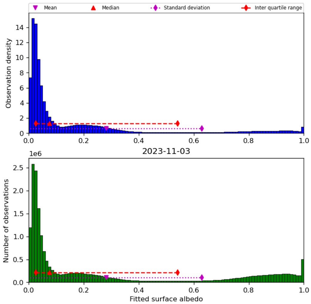
Figure 45: Histogram of “Fitted surface albedo” for 2023-11-02 to 2023-11-04
