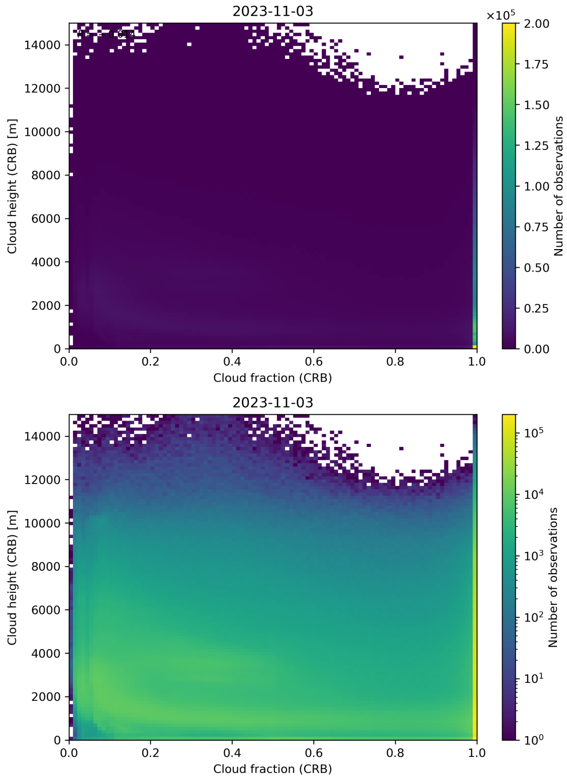
Figure 79: Scatter density plot of “Cloud fraction (CRB)” against “Cloud height (CRB)” for 2023-11-02 to 2023-11-04.
