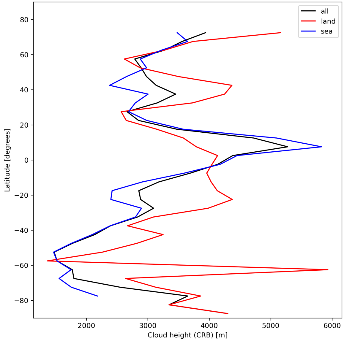
Figure 27: Zonal average of “Cloud height (CRB)” for 2023-11-02 to 2023-11-04.
