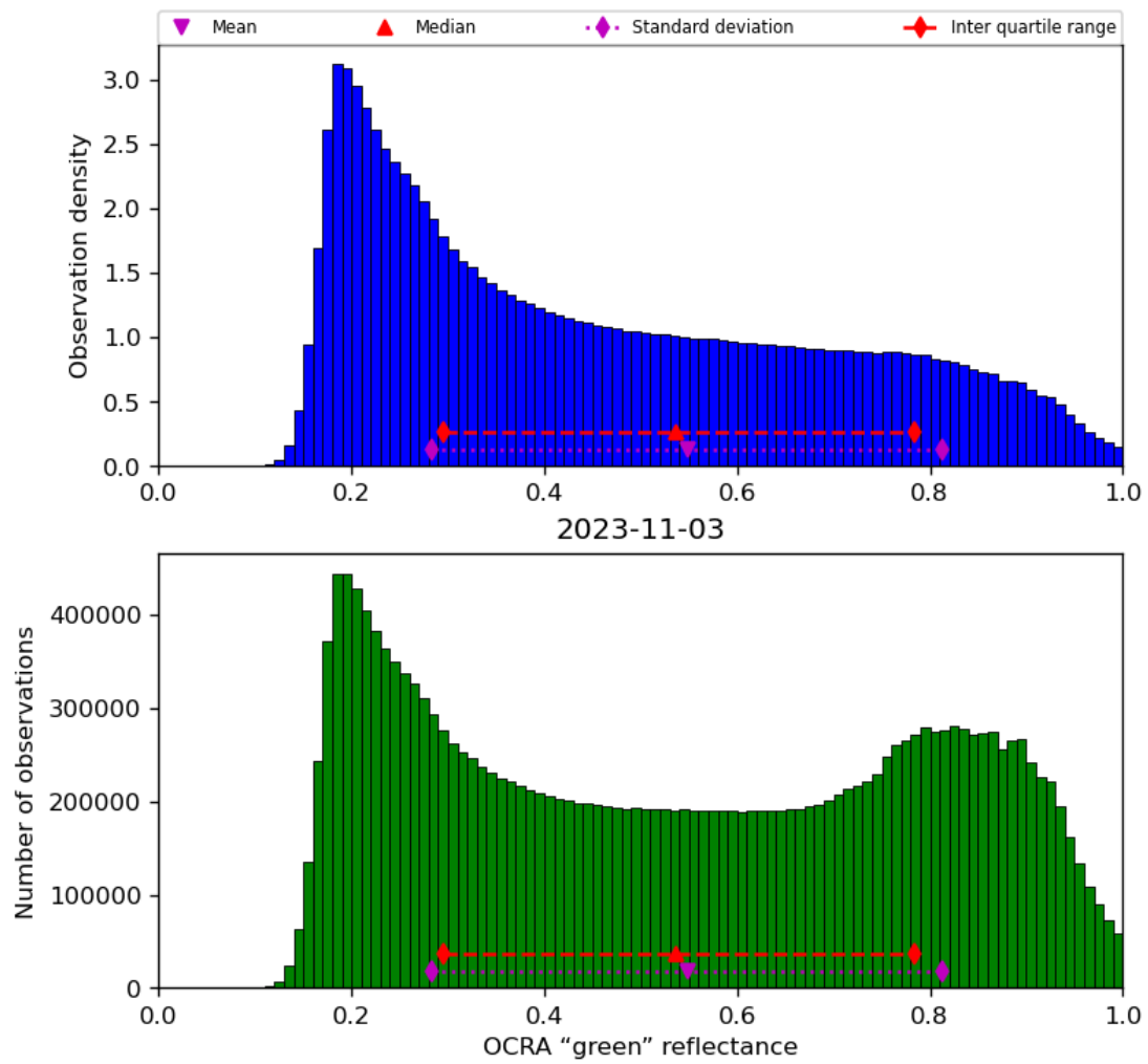
Figure 52: Histogram of “OCRA “green” reflectance” for 2023-11-02 to 2023-11-04
