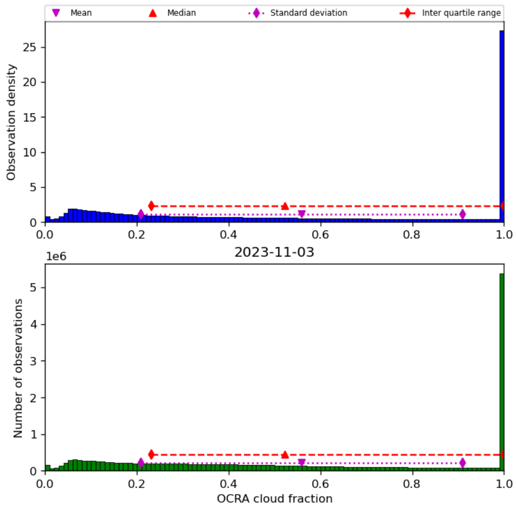
Figure 50: Histogram of “OCRA cloud fraction” for 2023-11-02 to 2023-11-04
