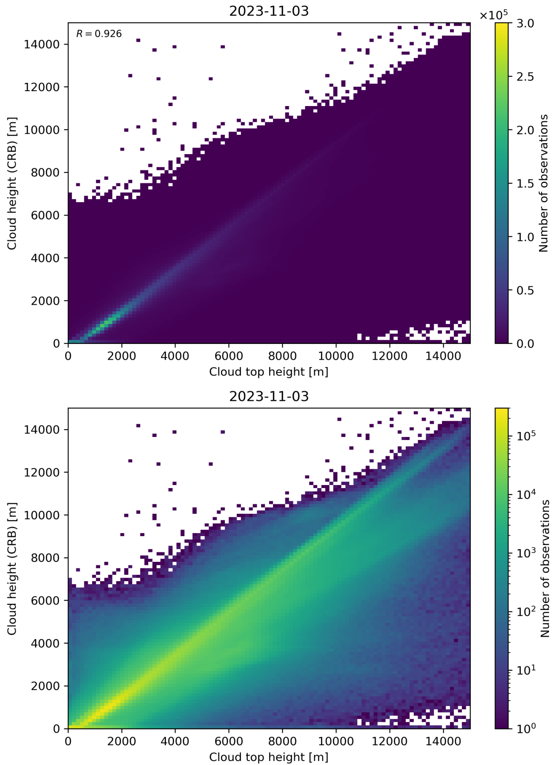
Figure 89: Scatter density plot of “Cloud top height” against “Cloud height (CRB)” for 2023-11-02 to 2023-11-04.
