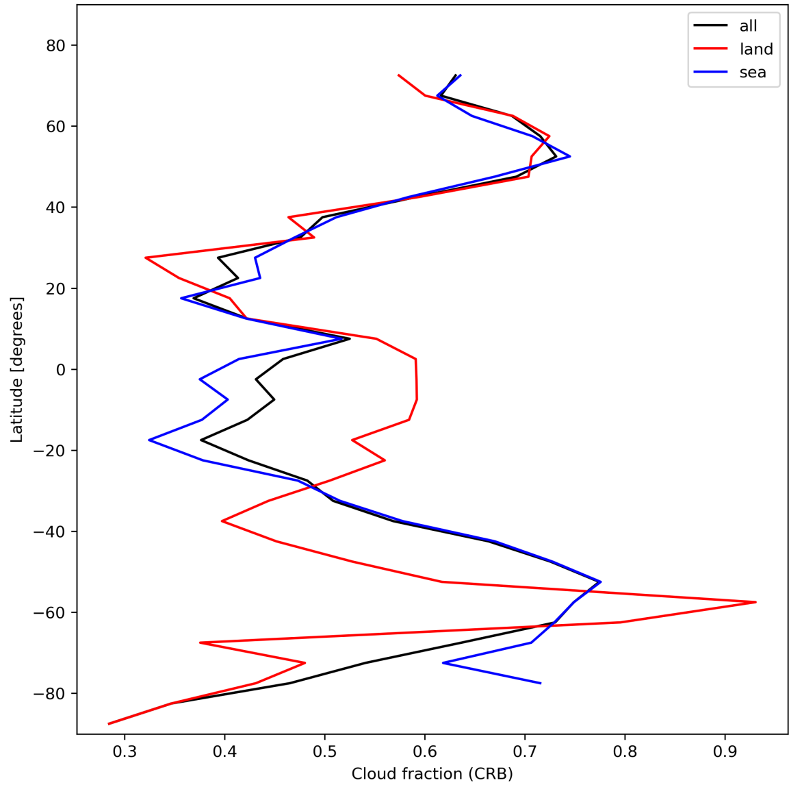
Figure 26: Zonal average of “Cloud fraction (CRB)” for 2023-11-02 to 2023-11-04.
