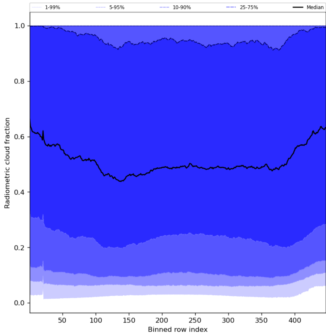
Figure 55: Along track statistics of “Radiometric cloud fraction” for 2023-11-02 to 2023-11-04
