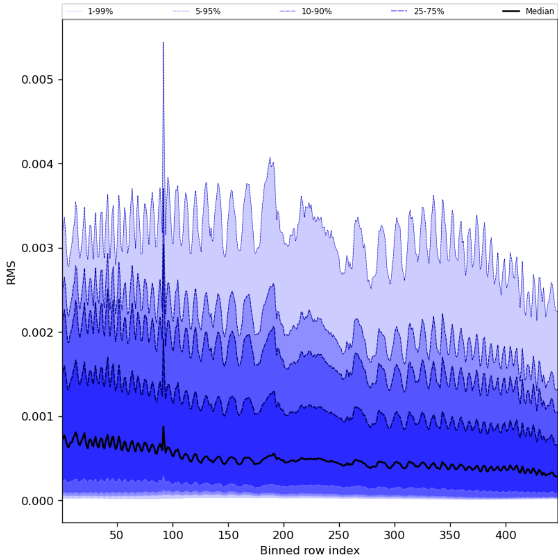
Figure 63: Along track statistics of “RMS” for 2023-11-02 to 2023-11-04
