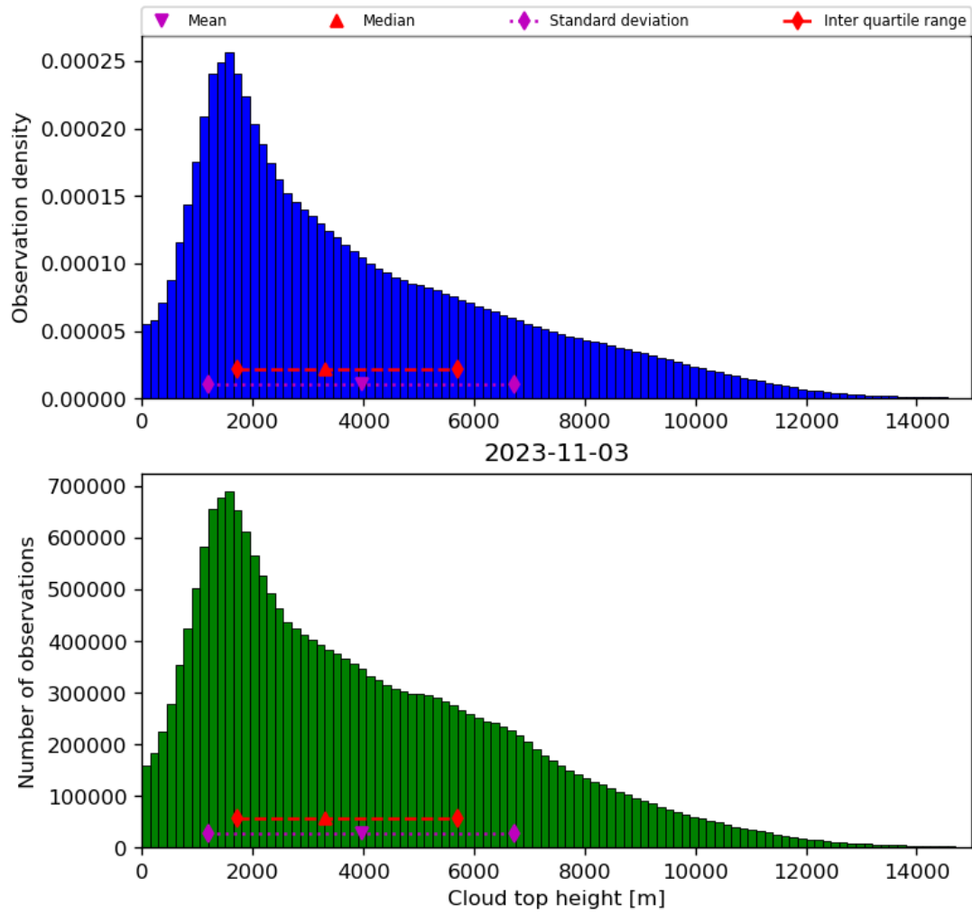
Figure 40: Histogram of “Cloud top height” for 2023-11-02 to 2023-11-04
