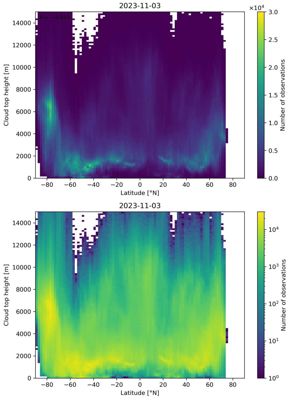
Figure 97: Scatter density plot of “Latitude” against “Cloud top height” for 2023-11-02 to 2023-11-04.
