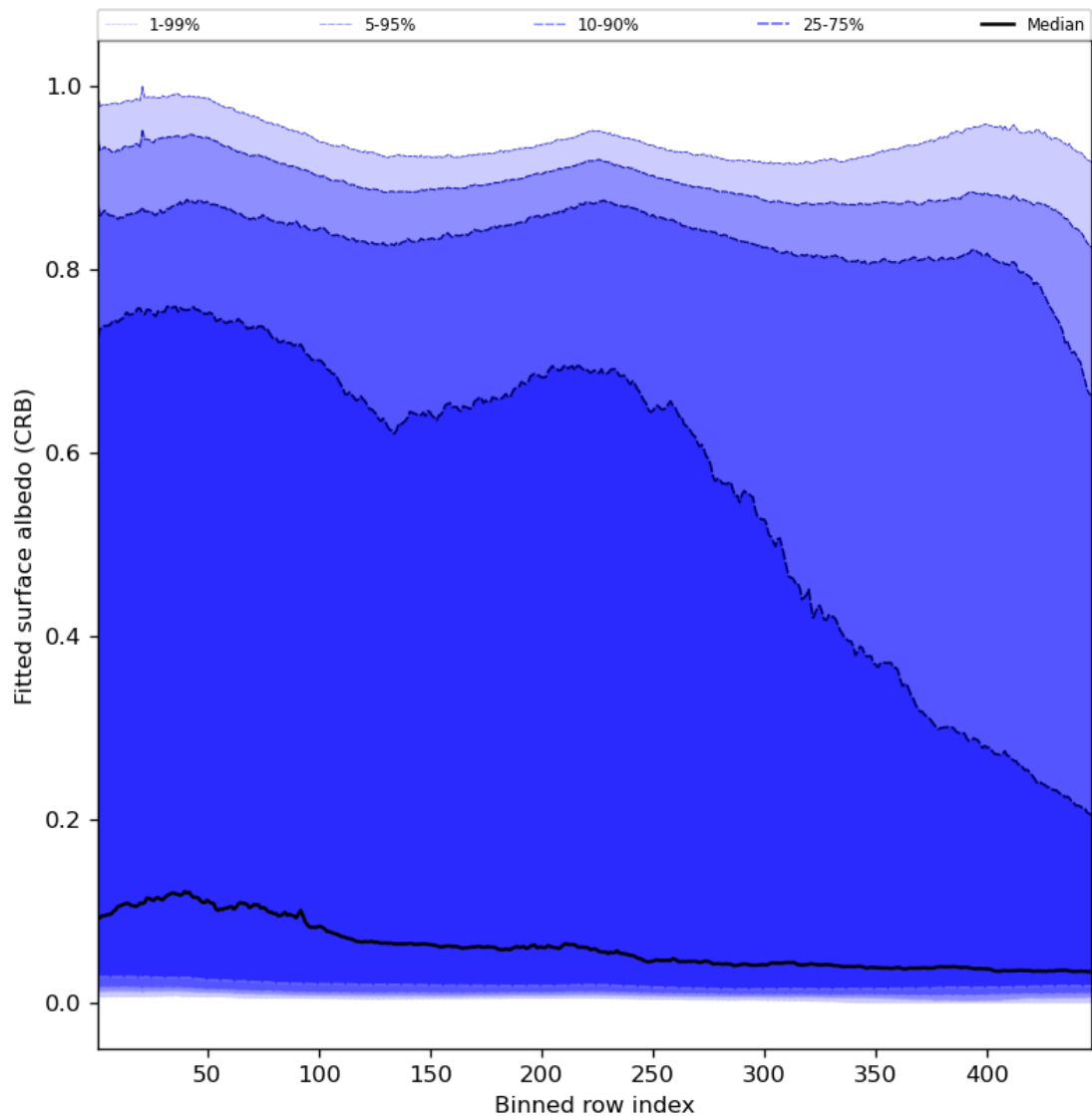
Figure 62: Along track statistics of “Fitted surface albedo (CRB)” for 2023-11-02 to 2023-11-04
