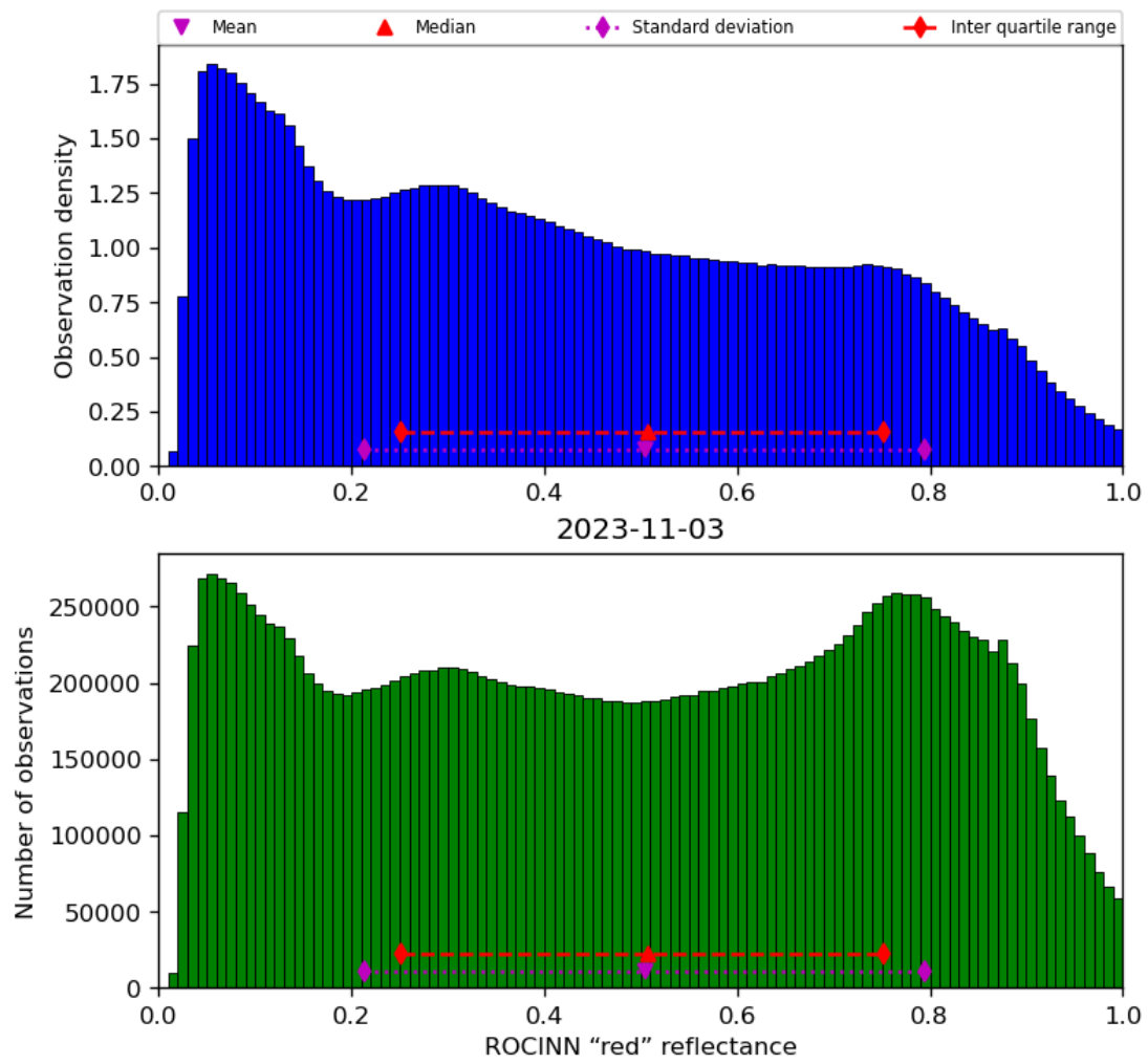
Figure 53: Histogram of “ROCINN “red” reflectance” for 2023-11-02 to 2023-11-04
