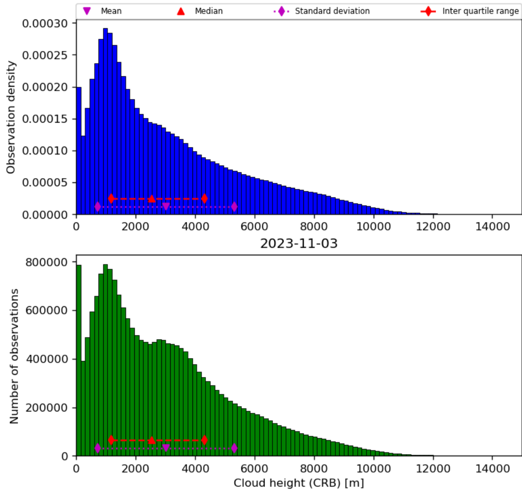
Figure 43: Histogram of “Cloud height (CRB)” for 2023-11-02 to 2023-11-04
