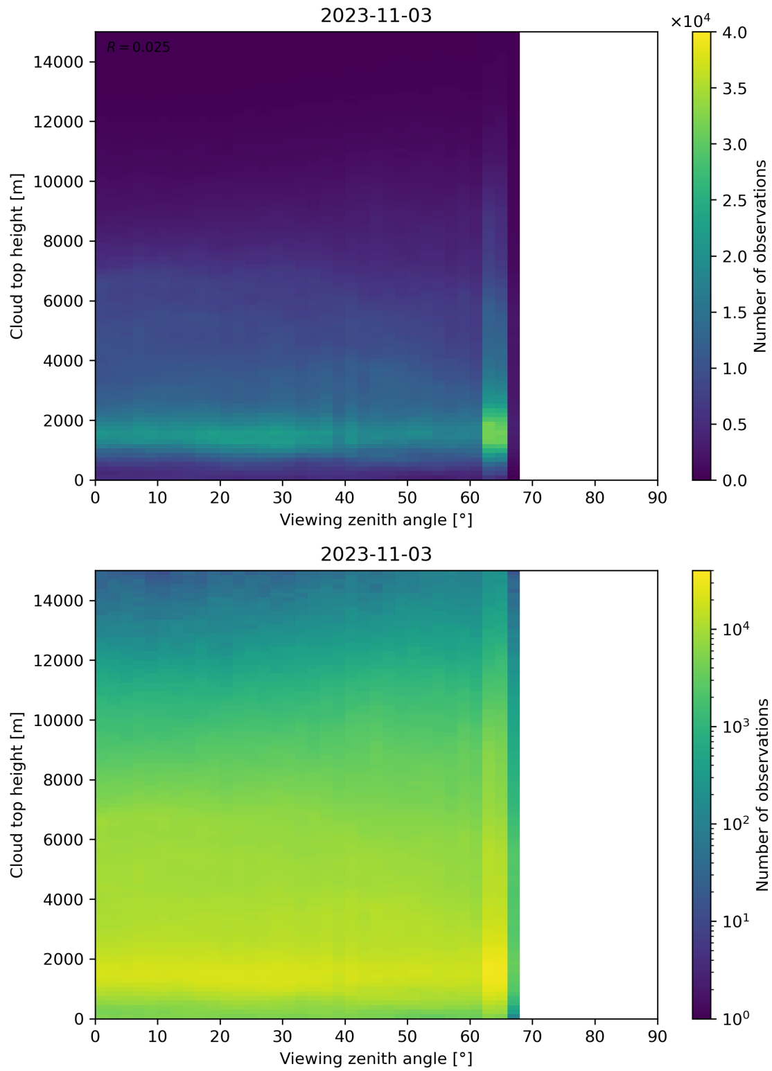
Figure 112: Scatter density plot of “Viewing zenith angle” against “Cloud top height” for 2023-11-02 to 2023-11-04.
