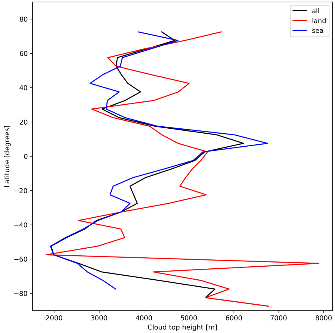
Figure 24: Zonal average of “Cloud top height” for 2023-11-02 to 2023-11-04.
