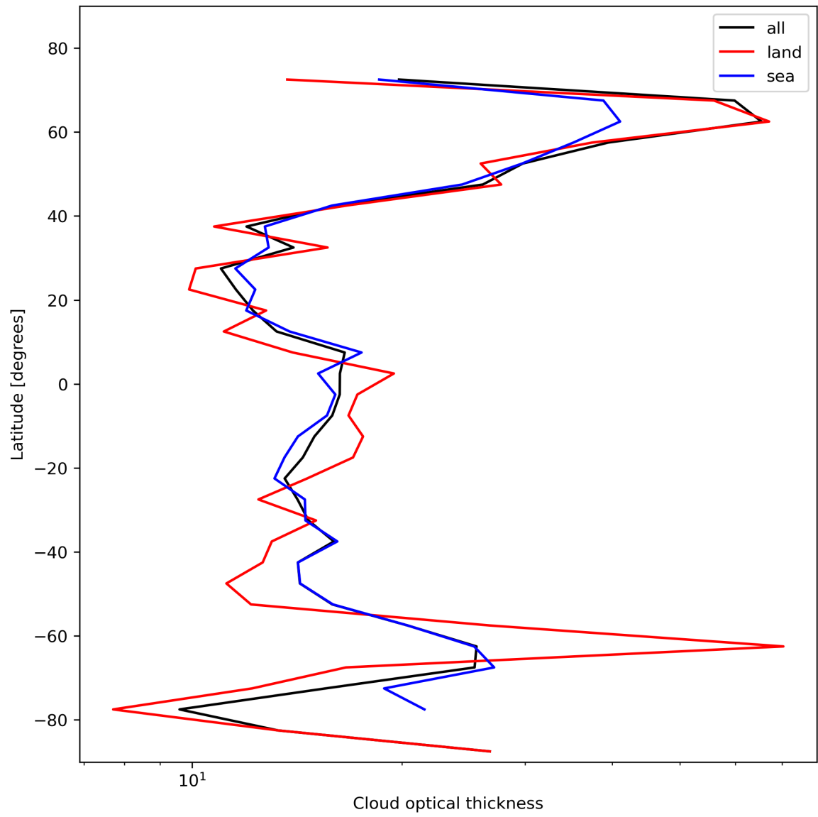
Figure 25: Zonal average of “Cloud optical thickness” for 2023-11-02 to 2023-11-04.
