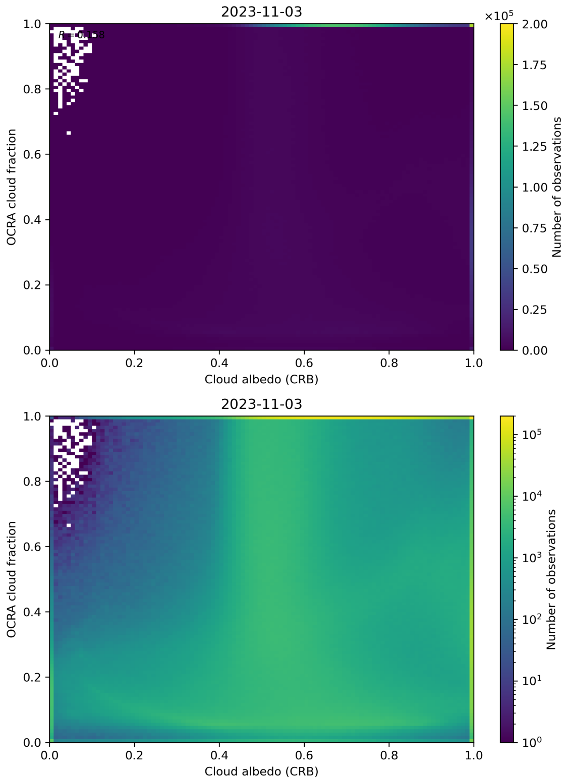
Figure 70: Scatter density plot of “Cloud albedo (CRB)” against “OCRA cloud fraction” for 2023-11-02 to 2023-11-04.
