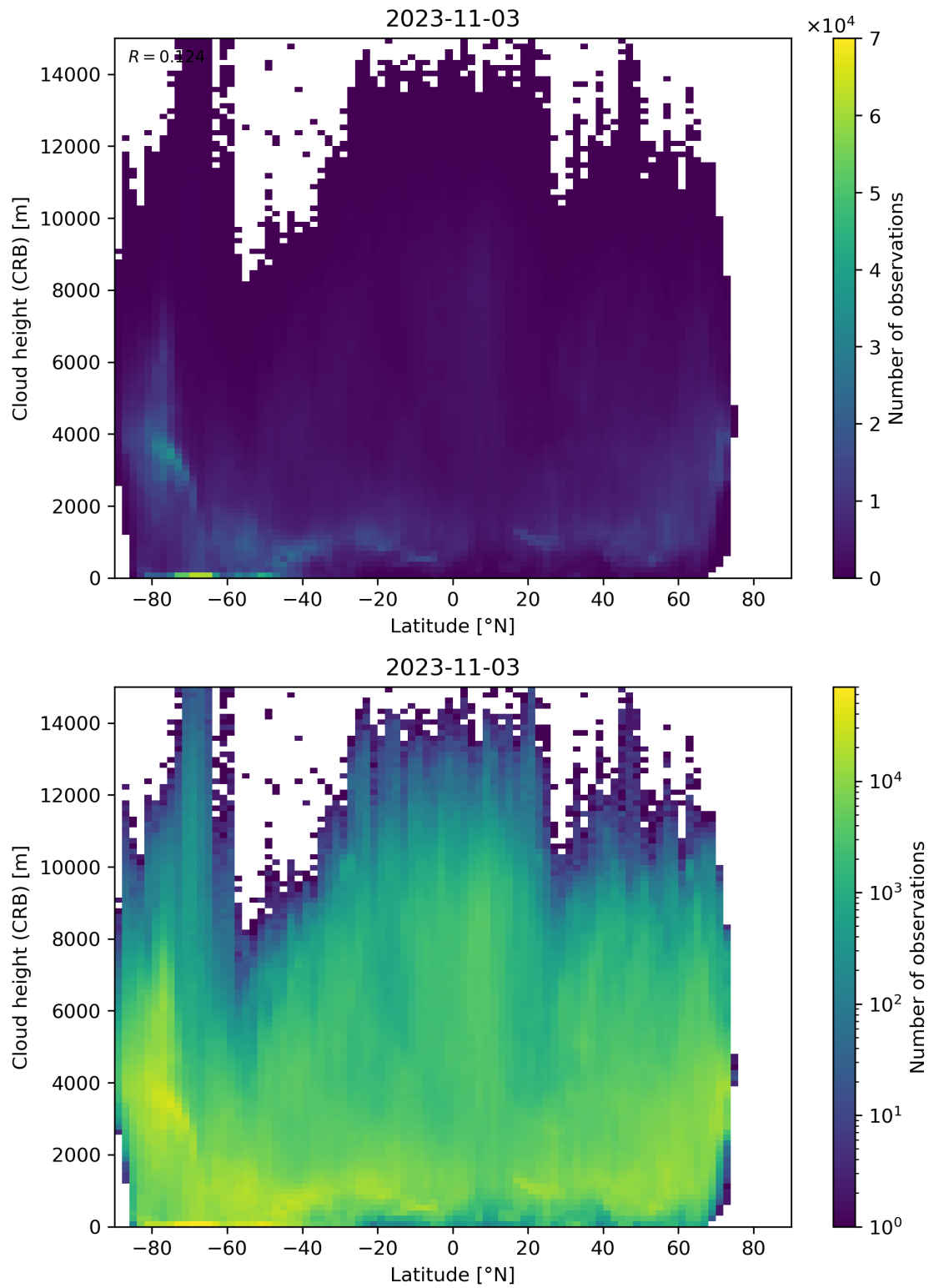
Figure 95: Scatter density plot of “Latitude” against “Cloud height (CRB)” for 2023-11-02 to 2023-11-04.
