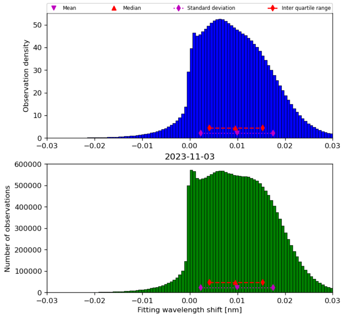
Figure 49: Histogram of “Fitting wavelength shift” for 2023-11-02 to 2023-11-04
