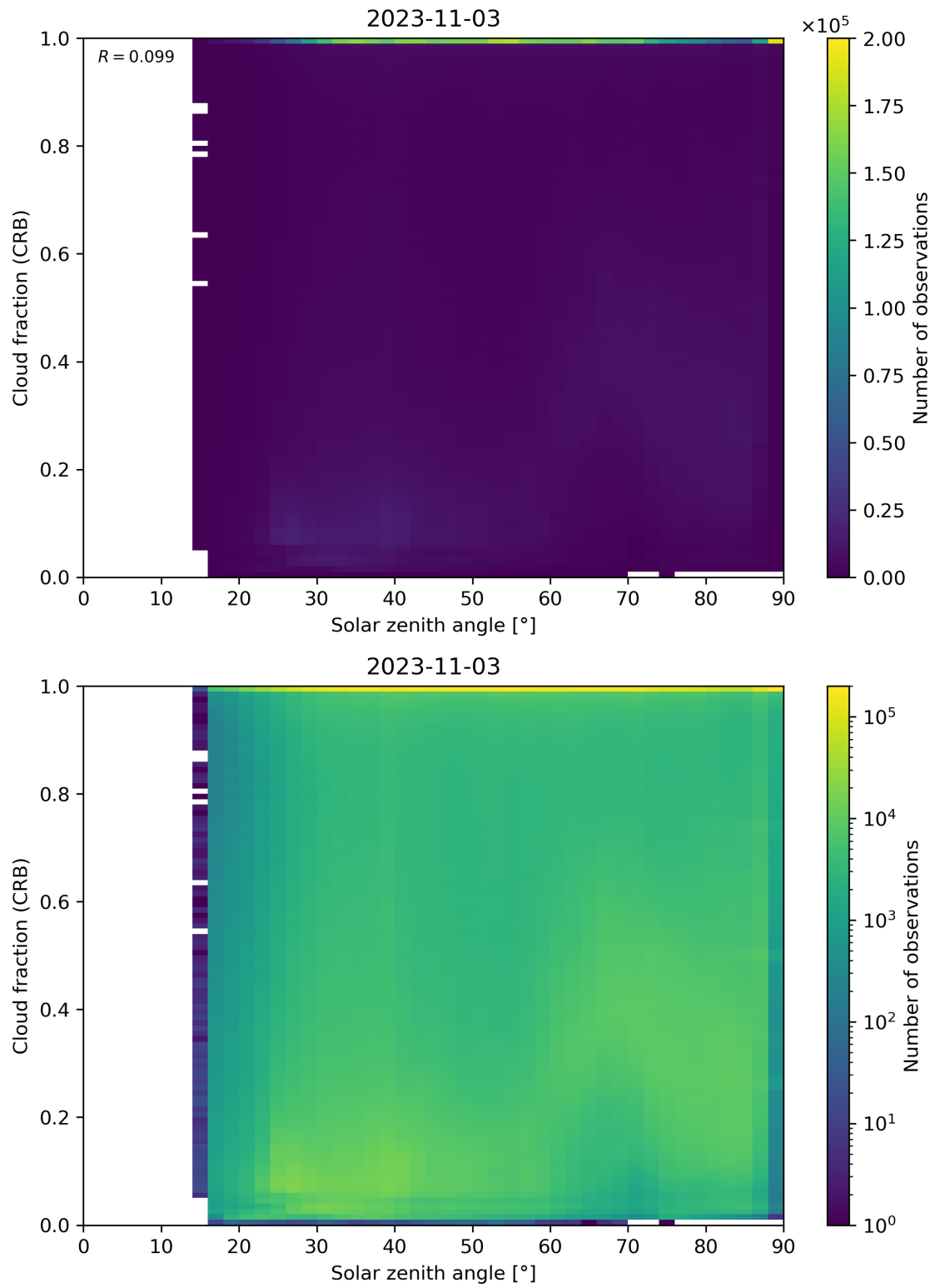
Figure 101: Scatter density plot of “Solar zenith angle” against “Cloud fraction (CRB)” for 2023-11-02 to 2023-11-04.
