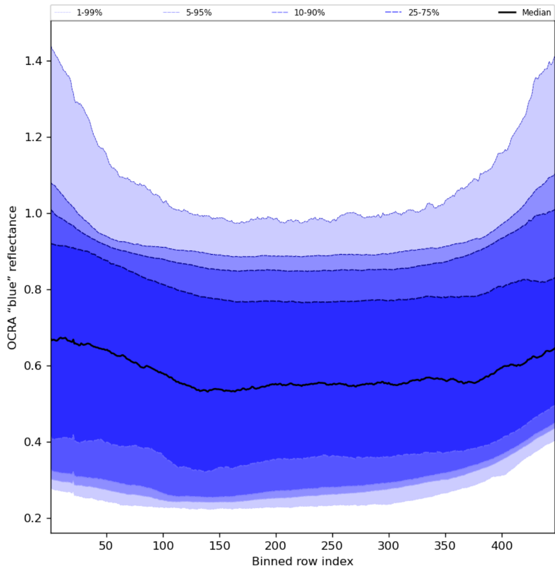
Figure 67: Along track statistics of "OCRA "blue" reflectance" for 2023-11-02 to 2023-11-04
