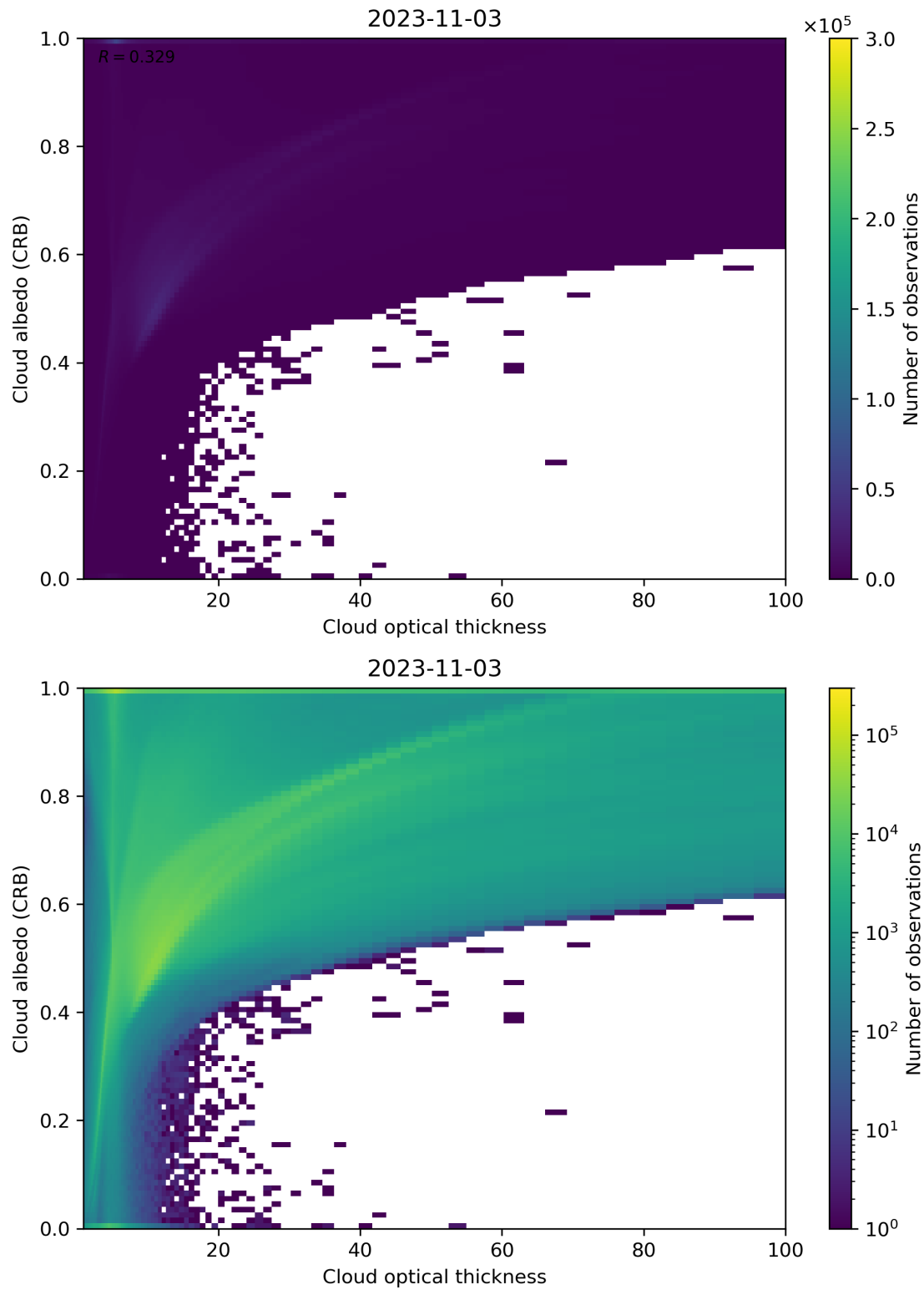
Figure 82: Scatter density plot of “Cloud optical thickness” against “Cloud albedo (CRB)” for 2023-11-02 to 2023-11-04.
