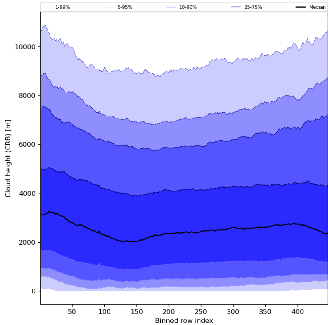
Figure 59: Along track statistics of “Cloud height (CRB)” for 2023-11-02 to 2023-11-04
