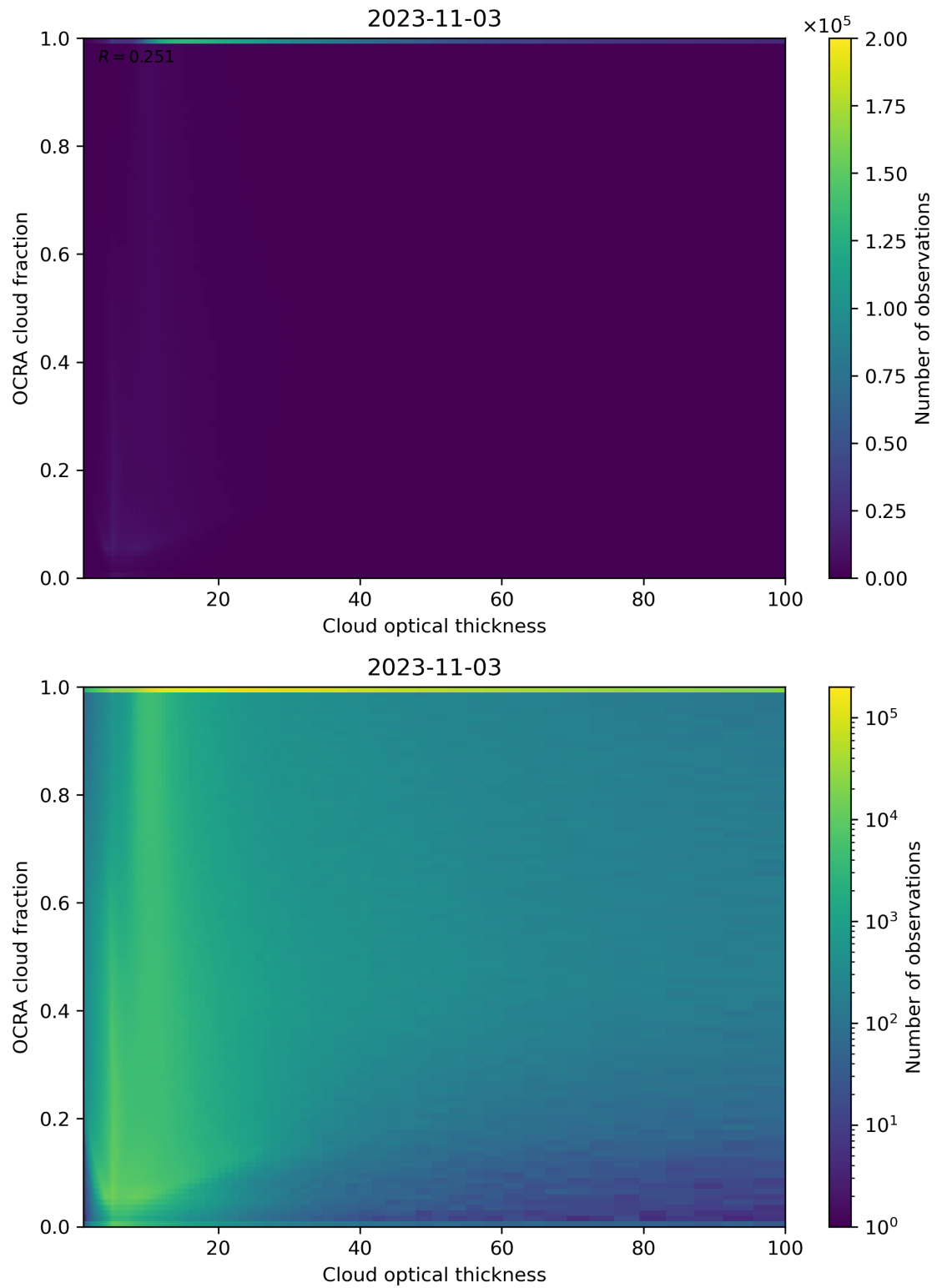
Figure 83: Scatter density plot of “Cloud optical thickness” against “OCRA cloud fraction” for 2023-11-02 to 2023-11-04.
