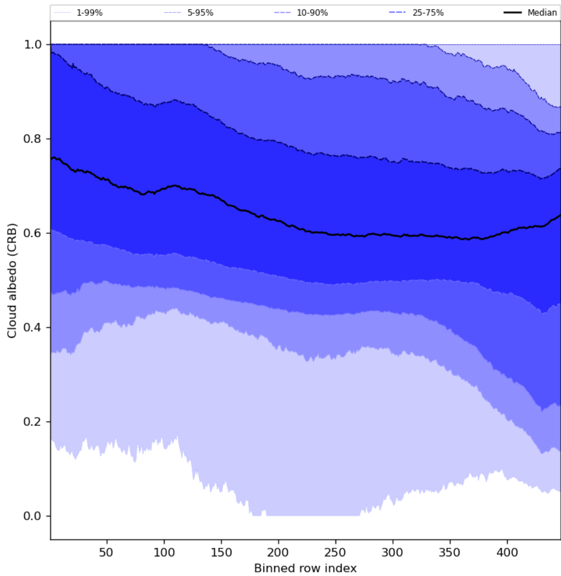
Figure 60: Along track statistics of “Cloud albedo (CRB)” for 2023-11-02 to 2023-11-04
