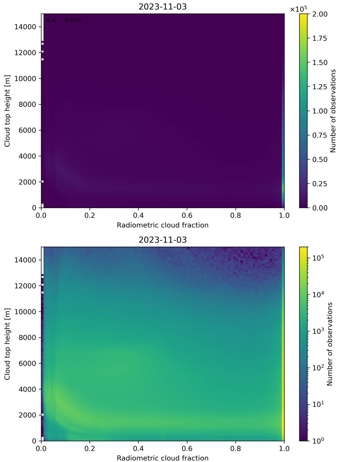
Figure 76: Scatter density plot of “Radiometric cloud fraction” against “Cloud top height” for 2023-11-02 to 2023-11-04.
