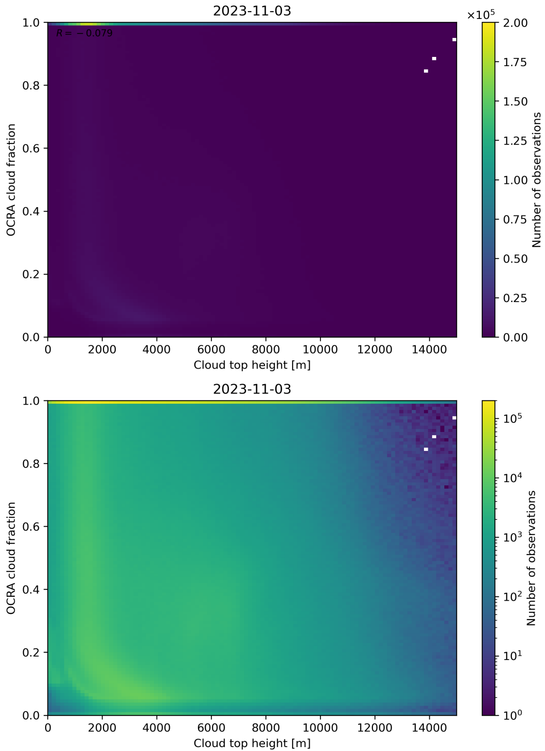
Figure 87: Scatter density plot of “Cloud top height” against “OCRA cloud fraction” for 2023-11-02 to 2023-11-04.
