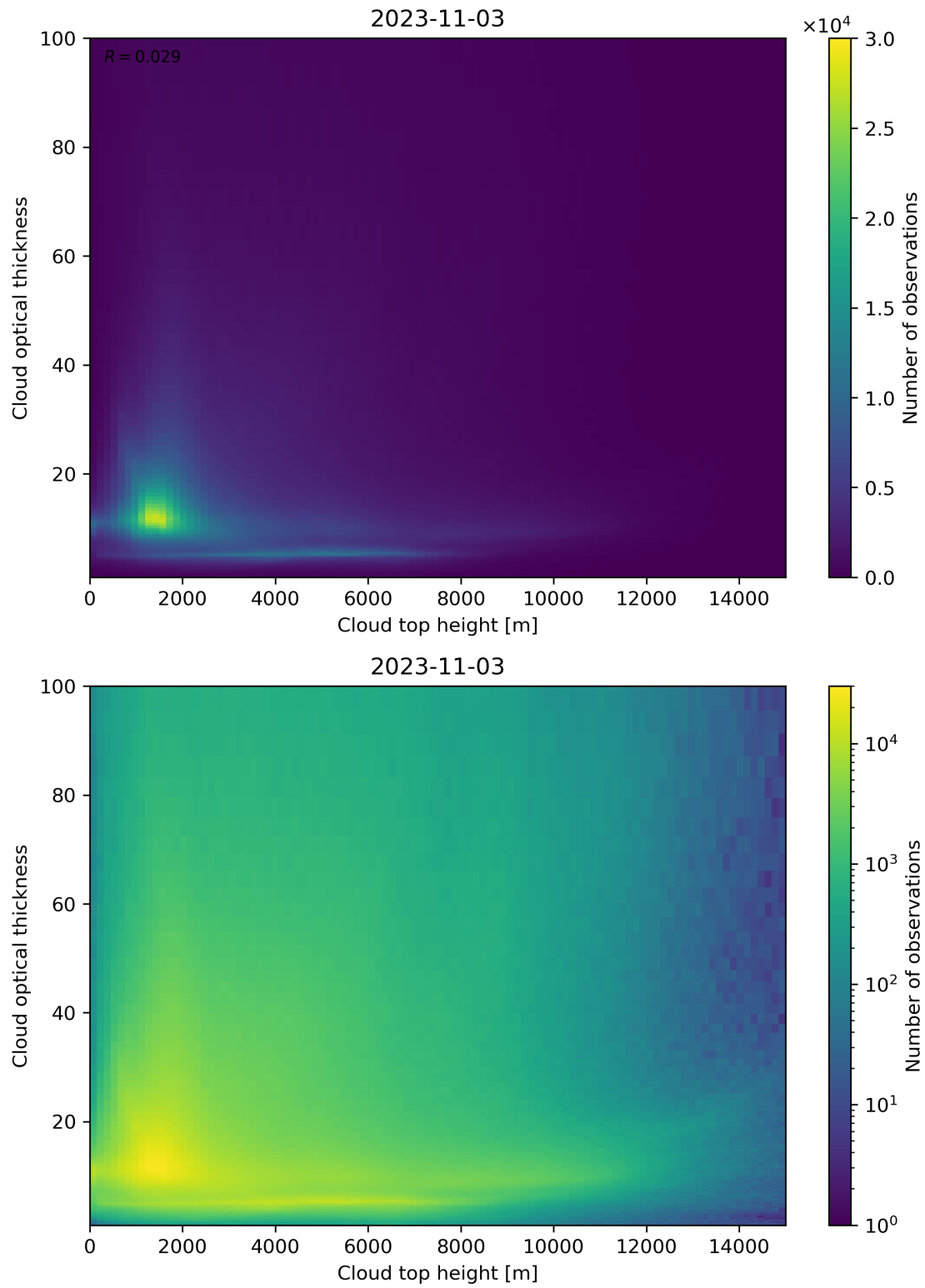
Figure 90: Scatter density plot of “Cloud top height” against “Cloud optical thickness” for 2023-11-02 to 2023-11-04.
