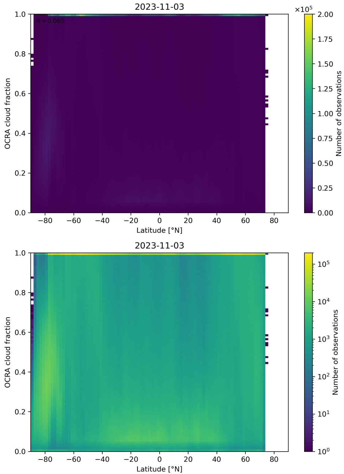
Figure 93: Scatter density plot of “Latitude” against “OCRA cloud fraction” for 2023-11-02 to 2023-11-04.
