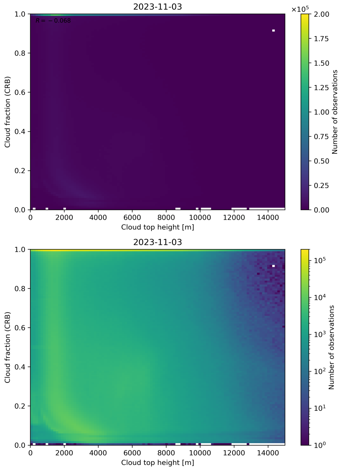
Figure 88: Scatter density plot of “Cloud top height” against “Cloud fraction (CRB)” for 2023-11-02 to 2023-11-04.
