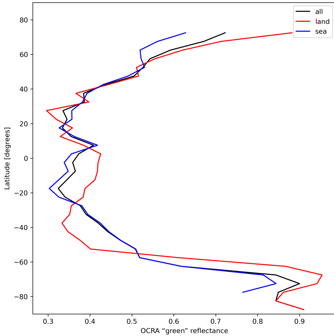
Figure 36: Zonal average of “OCRA “green” reflectance” for 2023-11-02 to 2023-11-04.
