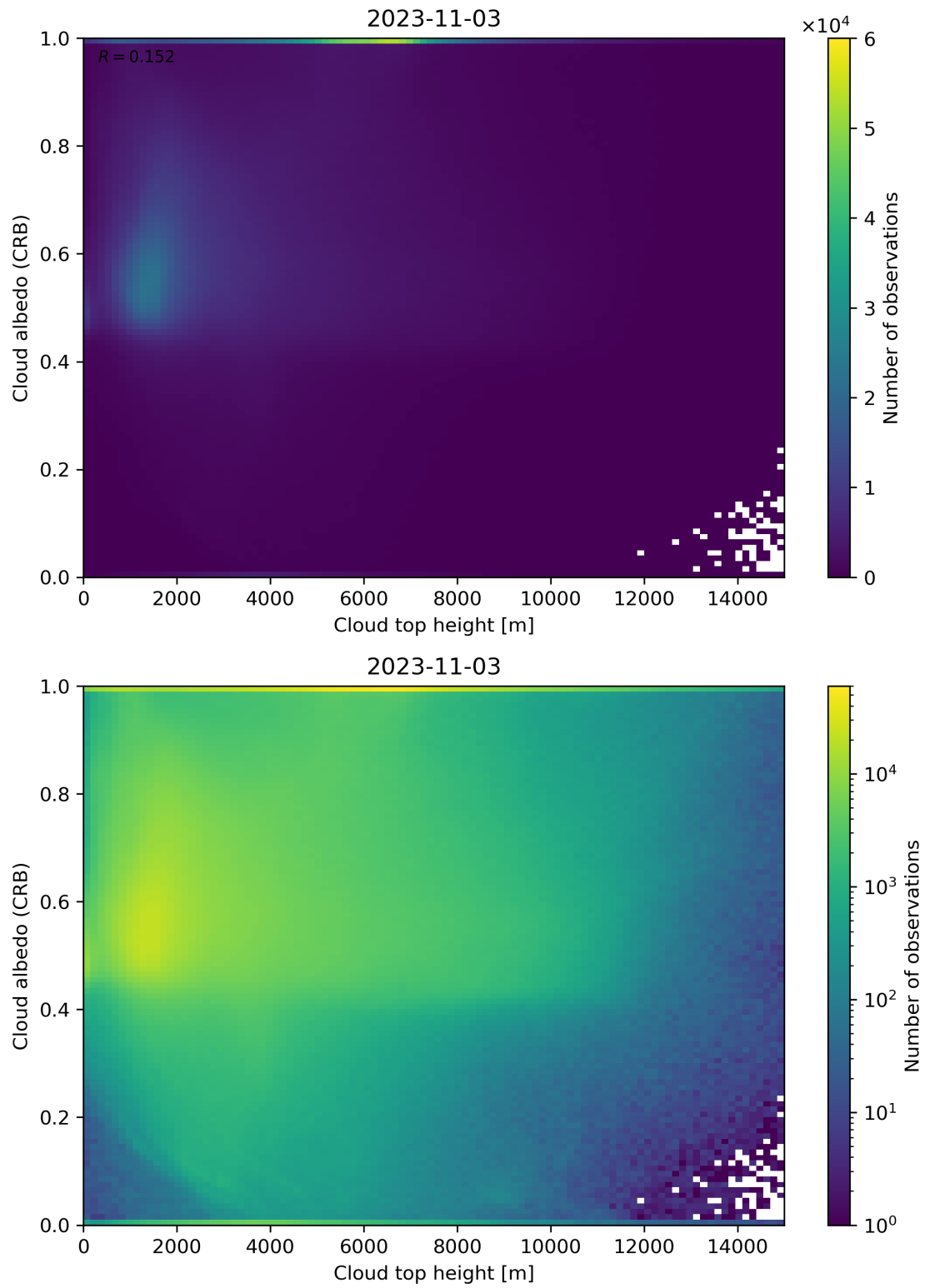
Figure 86: Scatter density plot of “Cloud top height” against “Cloud albedo (CRB)” for 2023-11-02 to 2023-11-04.
