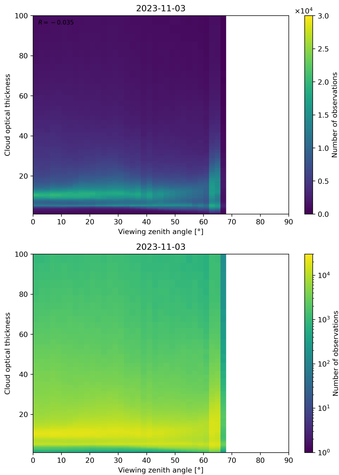
Figure 111: Scatter density plot of “Viewing zenith angle” against “Cloud optical thickness” for 2023-11-02 to 2023-11-04.
