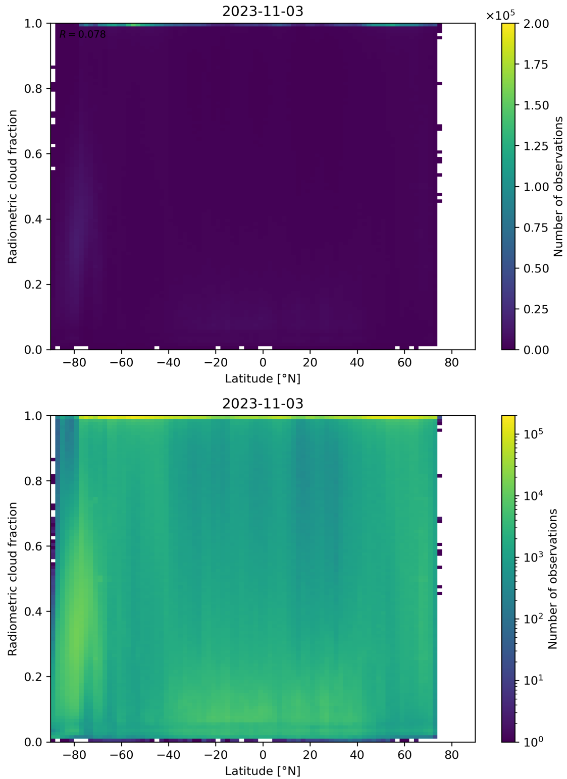
Figure 92: Scatter density plot of “Latitude” against “Radiometric cloud fraction” for 2023-11-02 to 2023-11-04.
