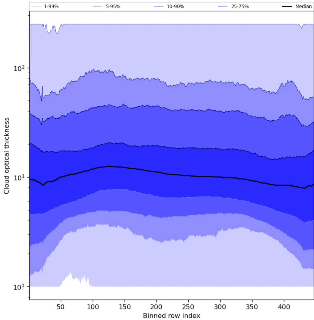
Figure 57: Along track statistics of “Cloud optical thickness” for 2023-11-02 to 2023-11-04
