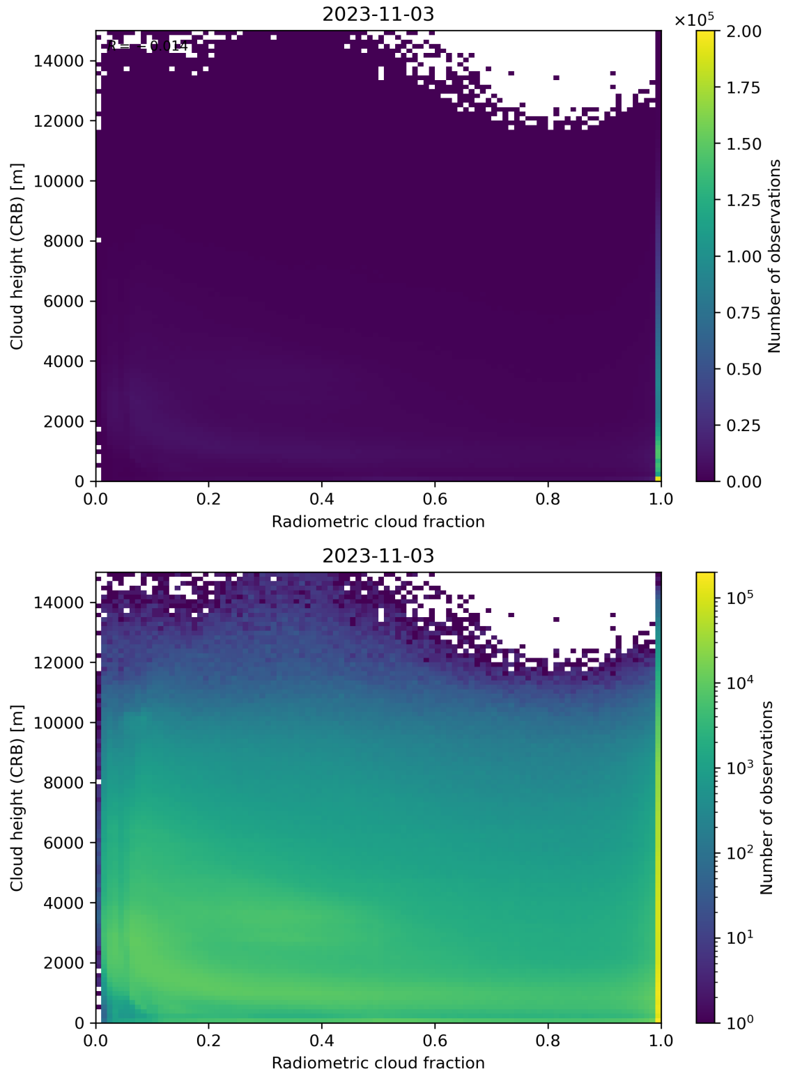
Figure 74: Scatter density plot of “Radiometric cloud fraction” against “Cloud height (CRB)” for 2023-11-02 to 2023-11-04.
