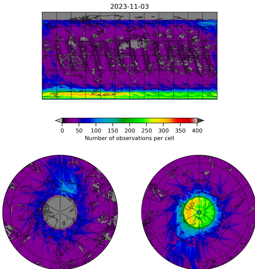
Figure 21: Map of the number of observations for 2023-11-02 to 2023-11-04
