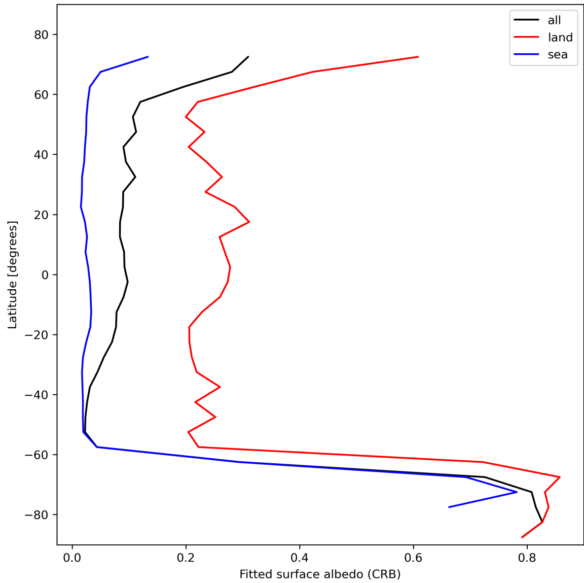
Figure 30: Zonal average of “Fitted surface albedo (CRB)” for 2023-11-02 to 2023-11-04.
