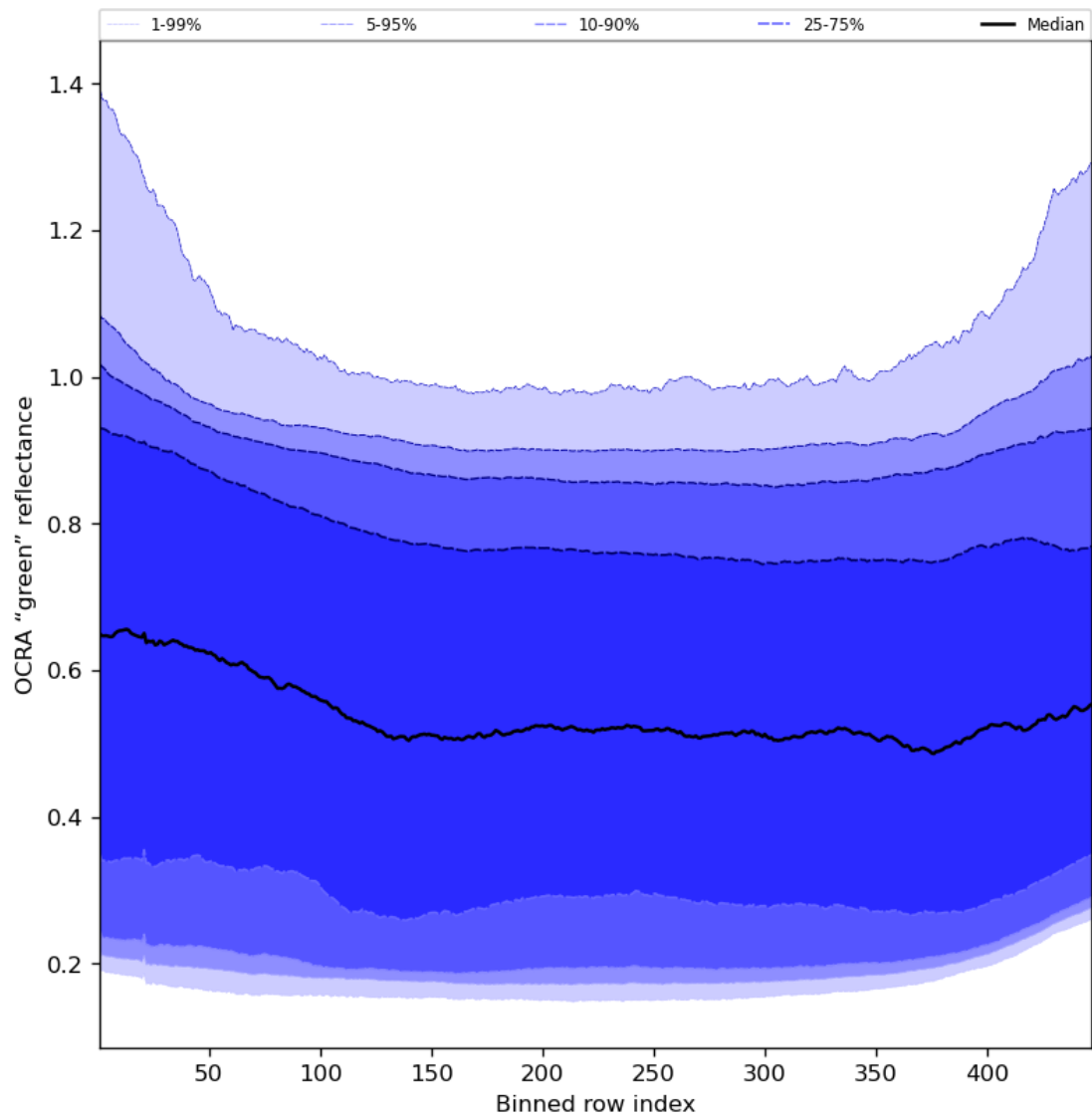
Figure 68: Along track statistics of "OCRA "green" reflectance" for 2023-11-02 to 2023-11-04
