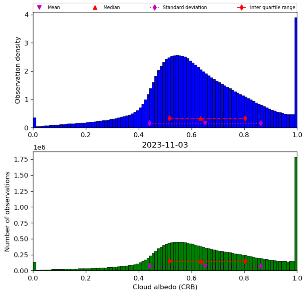
Figure 44: Histogram of “Cloud albedo (CRB)” for 2023-11-02 to 2023-11-04
