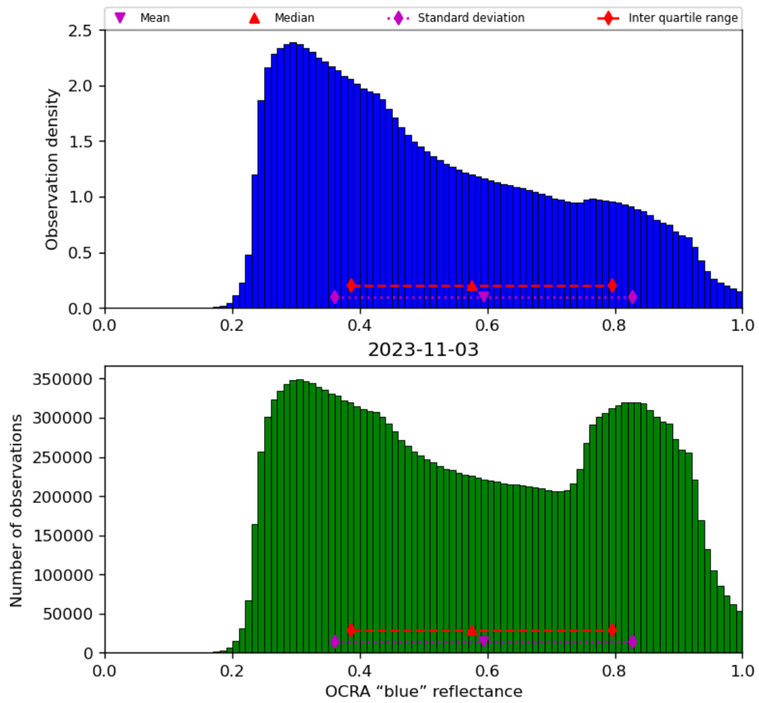
Figure 51: Histogram of “OCRA “blue” reflectance” for 2023-11-02 to 2023-11-04
