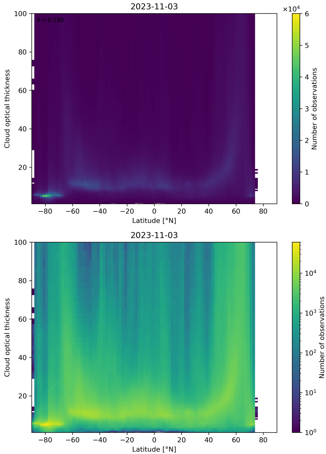
Figure 96: Scatter density plot of “Latitude” against “Cloud optical thickness” for 2023-11-02 to 2023-11-04.
