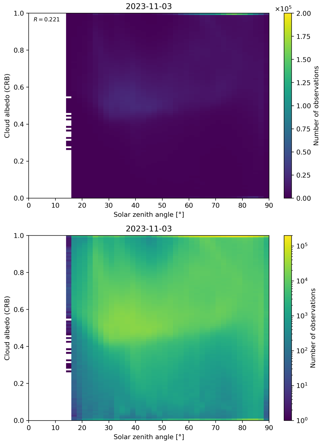
Figure 98: Scatter density plot of “Solar zenith angle” against “Cloud albedo (CRB)” for 2023-11-02 to 2023-11-04.
