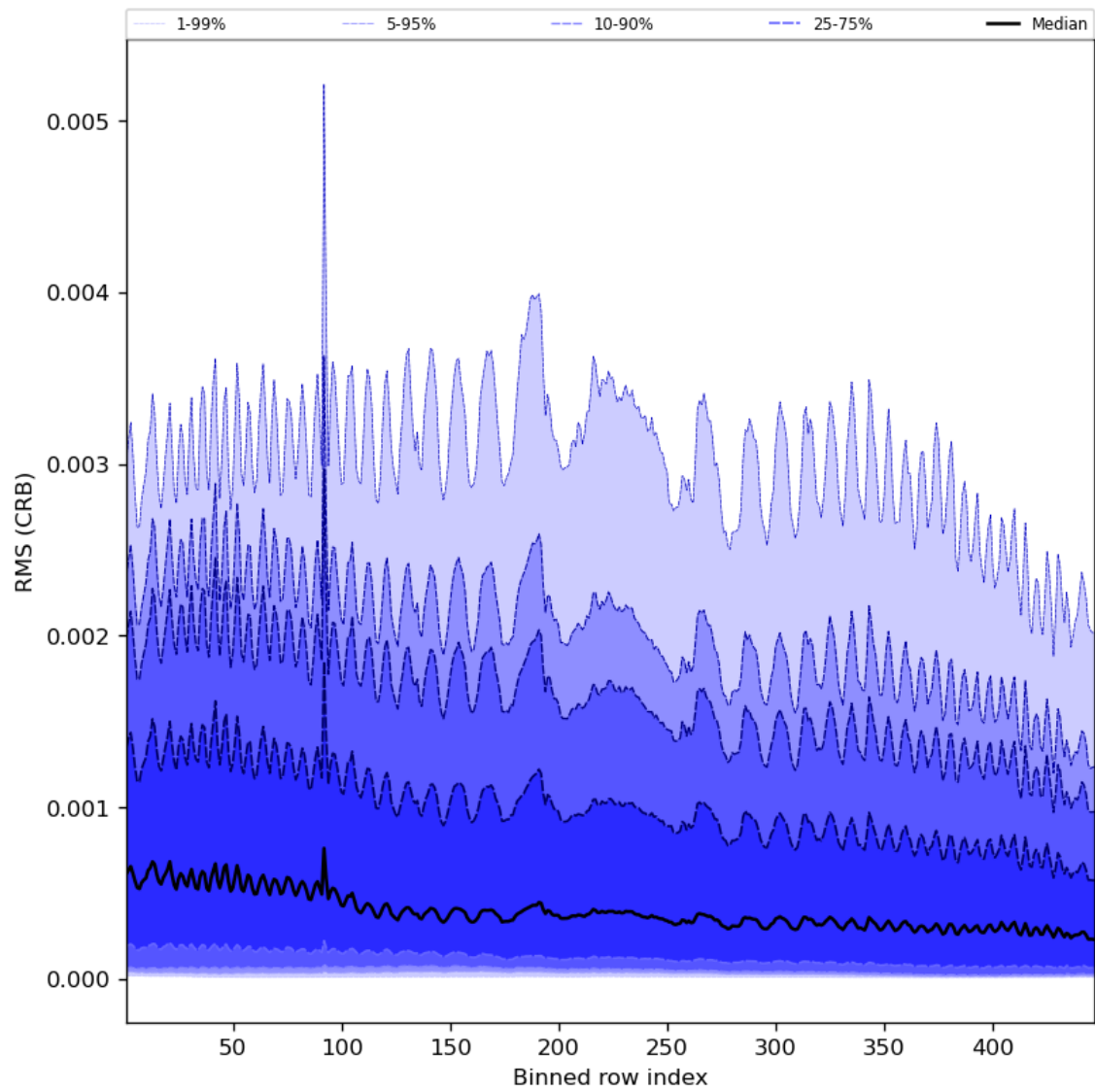
Figure 64: Along track statistics of “RMS (CRB)” for 2023-11-02 to 2023-11-04
