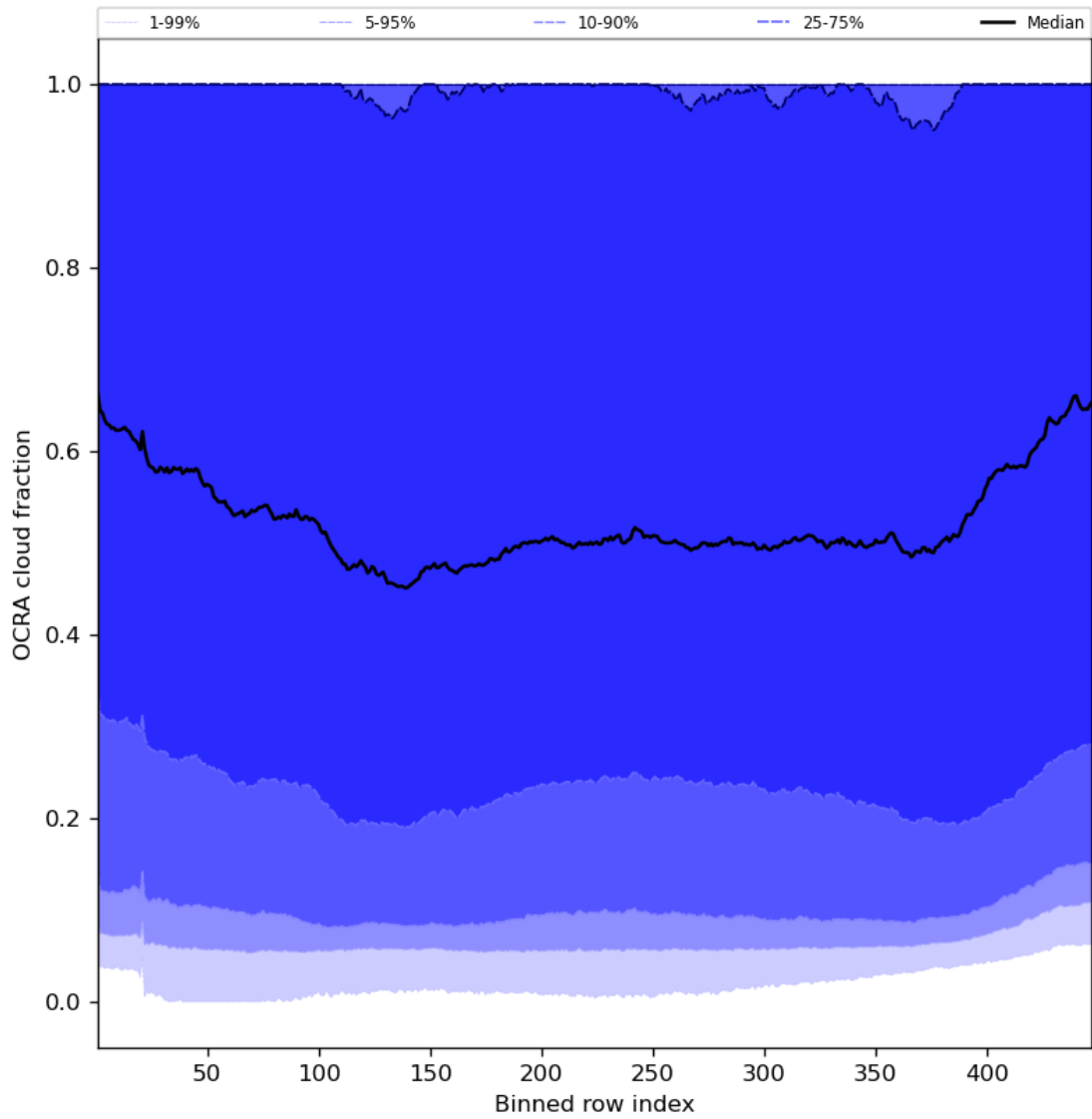
Figure 66: Along track statistics of “OCRA cloud fraction” for 2023-11-02 to 2023-11-04
