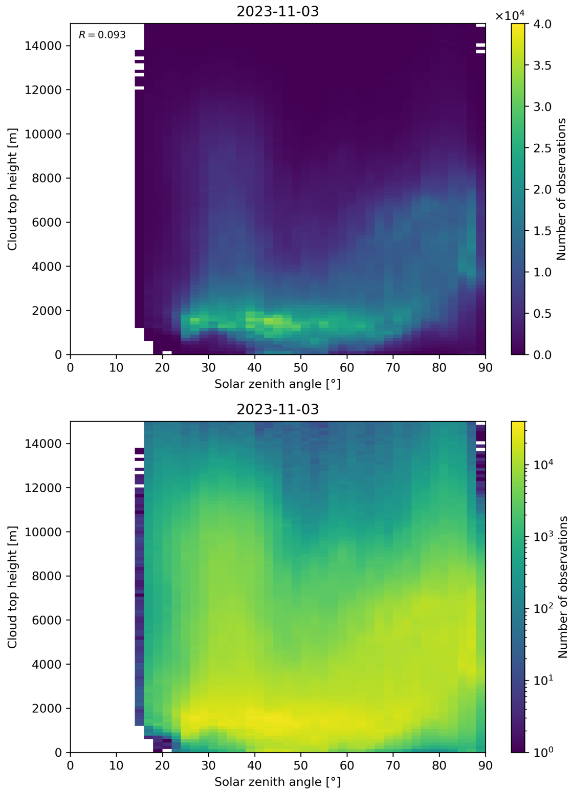
Figure 104: Scatter density plot of “Solar zenith angle” against “Cloud top height” for 2023-11-02 to 2023-11-04.
