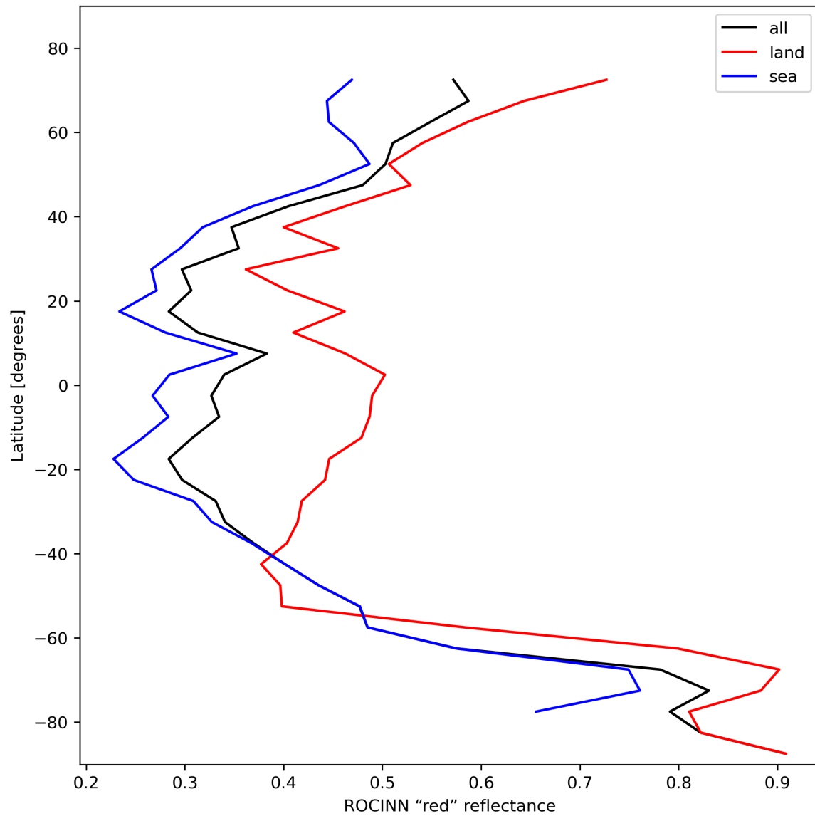
Figure 37: Zonal average of “ROCINN “red” reflectance” for 2023-11-02 to 2023-11-04.
