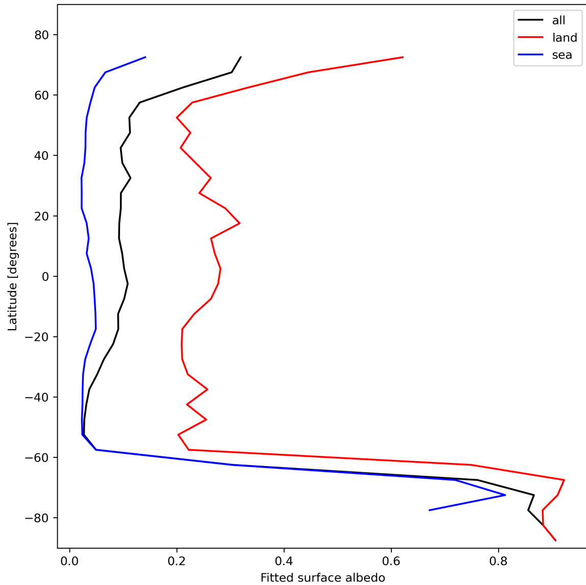
Figure 29: Zonal average of “Fitted surface albedo” for 2023-11-02 to 2023-11-04.
