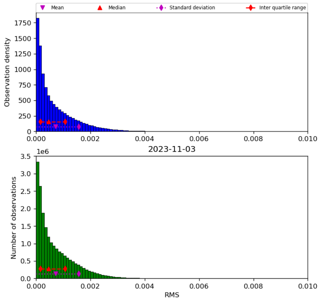
Figure 47: Histogram of “RMS” for 2023-11-02 to 2023-11-04
