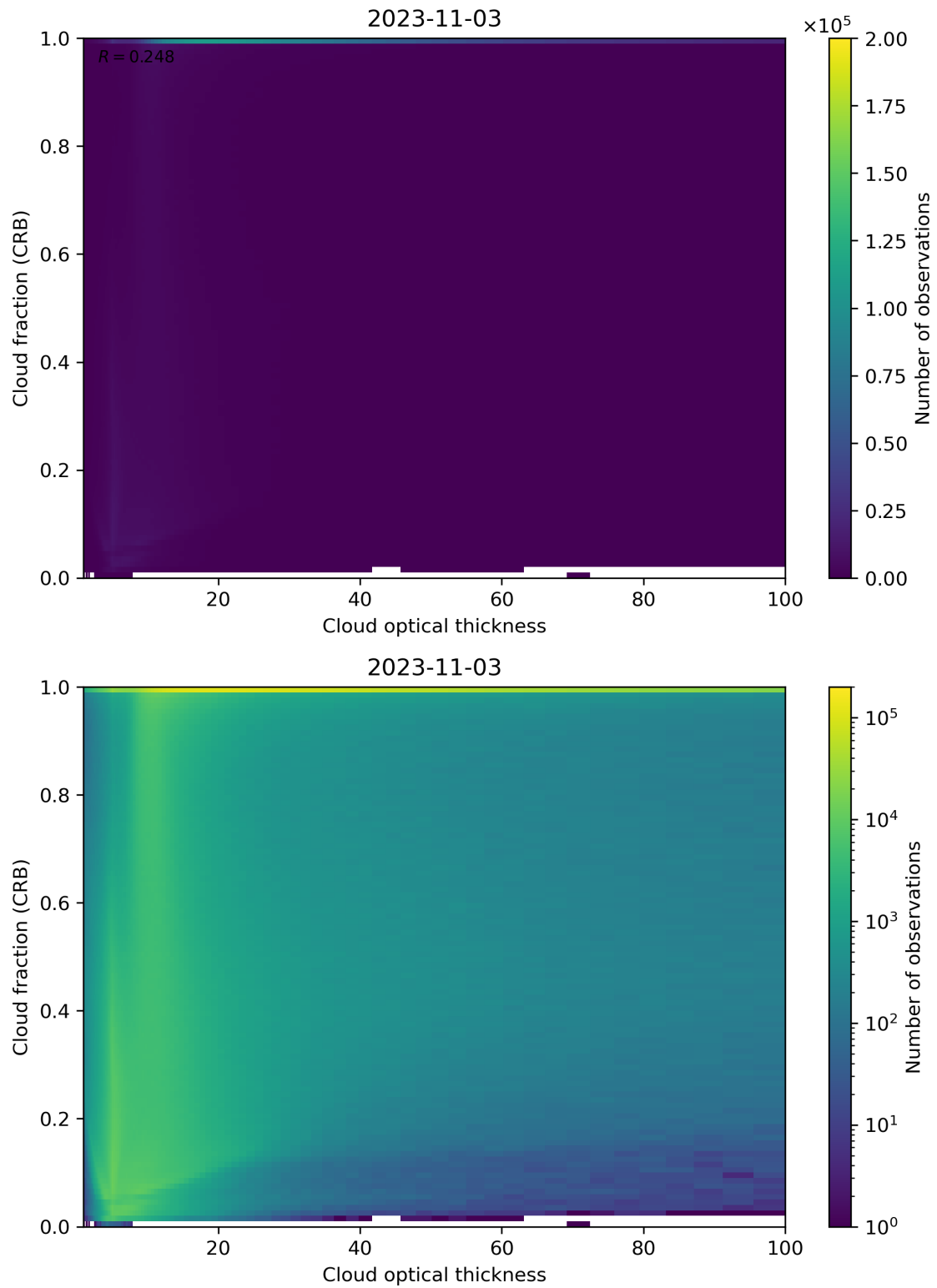
Figure 84: Scatter density plot of “Cloud optical thickness” against “Cloud fraction (CRB)” for 2023-11-02 to 2023-11-04.
