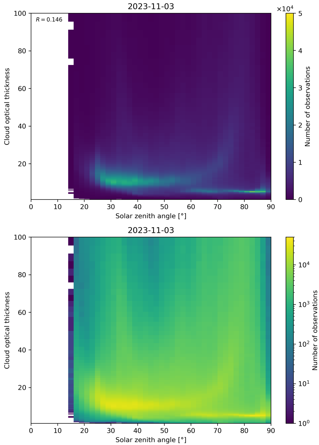
Figure 103: Scatter density plot of “Solar zenith angle” against “Cloud optical thickness” for 2023-11-02 to 2023-11-04.
