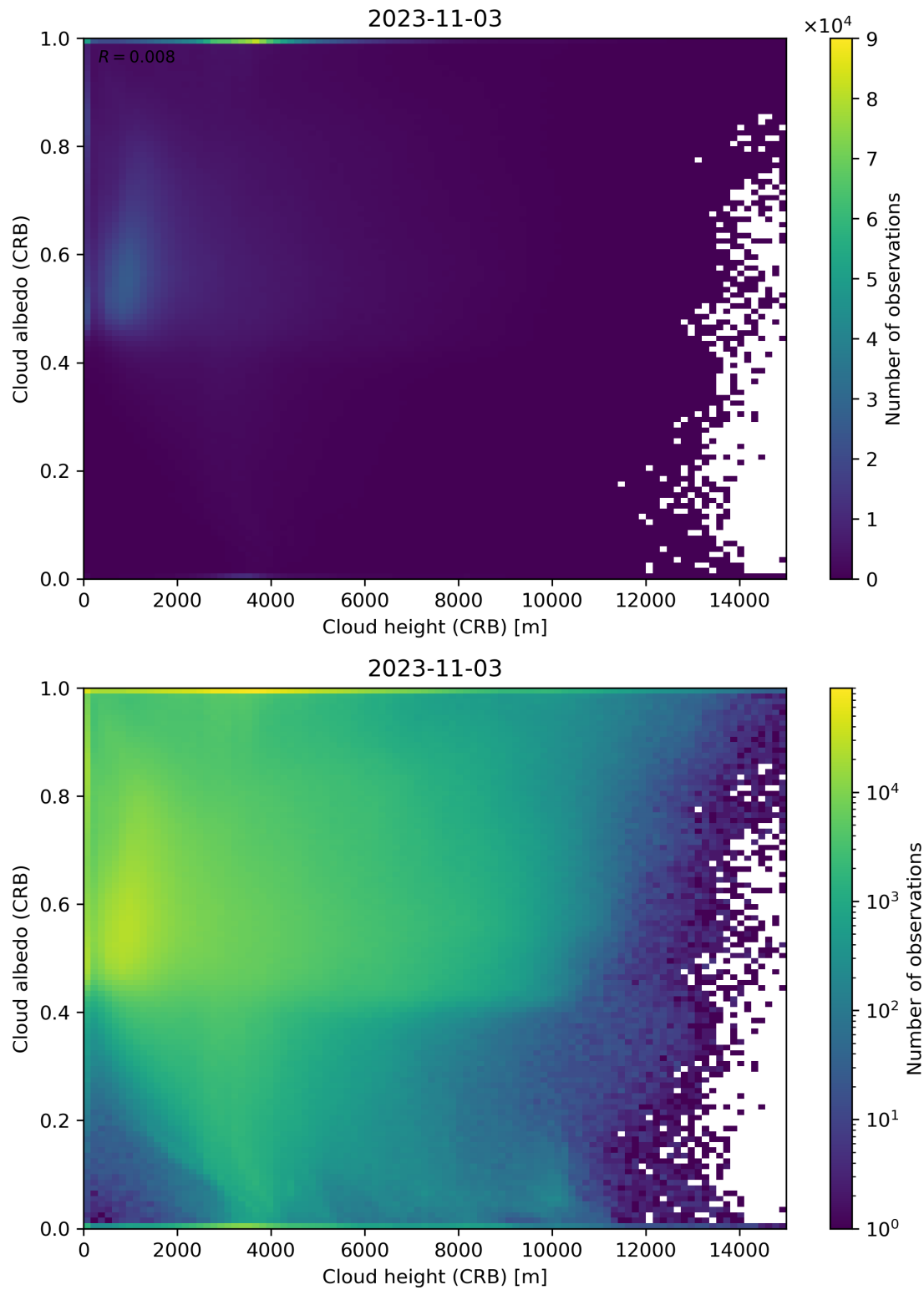
Figure 80: Scatter density plot of “Cloud height (CRB)” against “Cloud albedo (CRB)” for 2023-11-02 to 2023-11-04.
