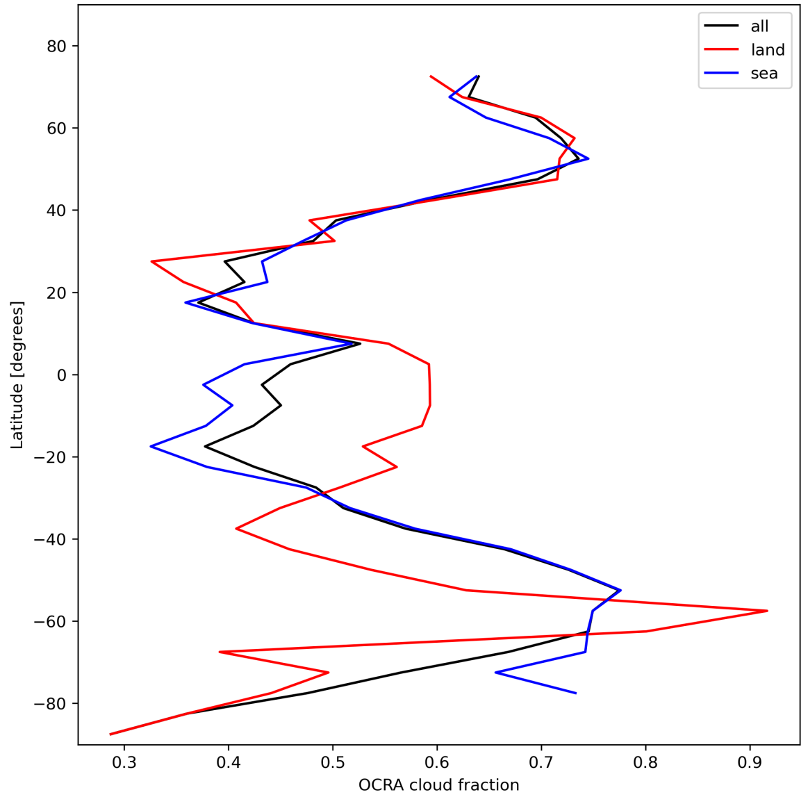
Figure 34: Zonal average of “OCRA cloud fraction” for 2023-11-02 to 2023-11-04.
