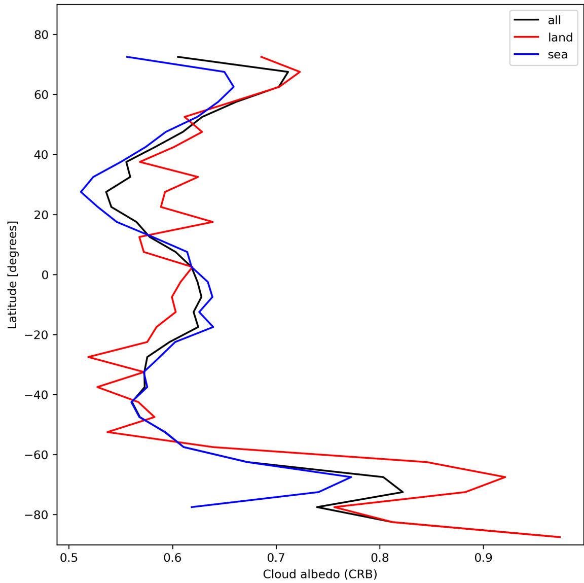
Figure 28: Zonal average of “Cloud albedo (CRB)” for 2023-11-02 to 2023-11-04.
