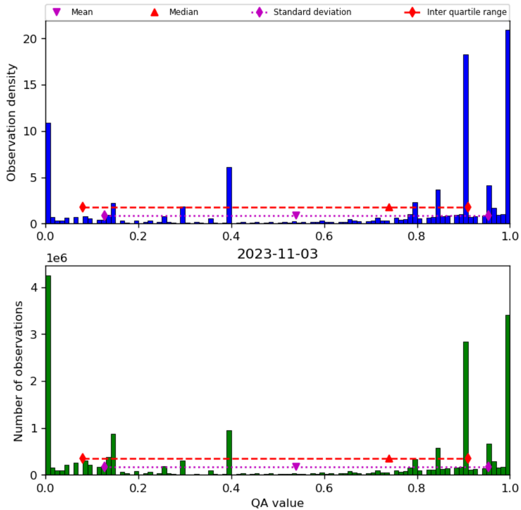
Figure 38: Histogram of “QA value” for 2023-11-02 to 2023-11-04
