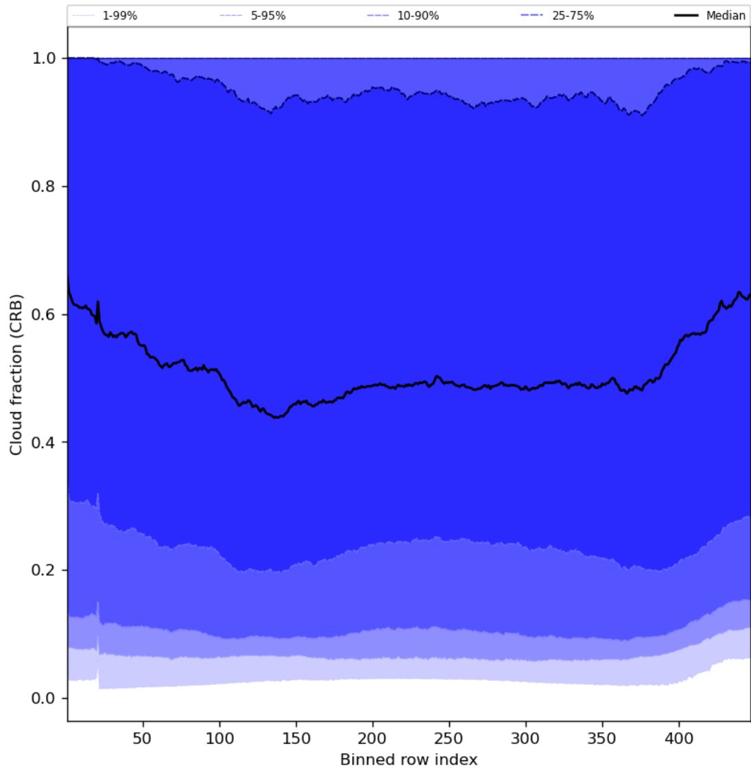
Figure 58: Along track statistics of “Cloud fraction (CRB)” for 2023-11-02 to 2023-11-04
