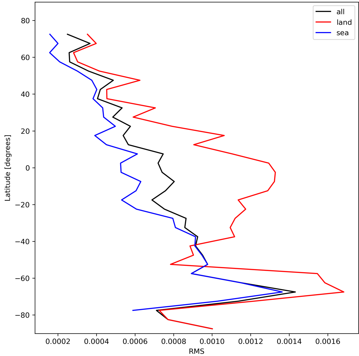
Figure 31: Zonal average of “RMS” for 2023-11-02 to 2023-11-04.
