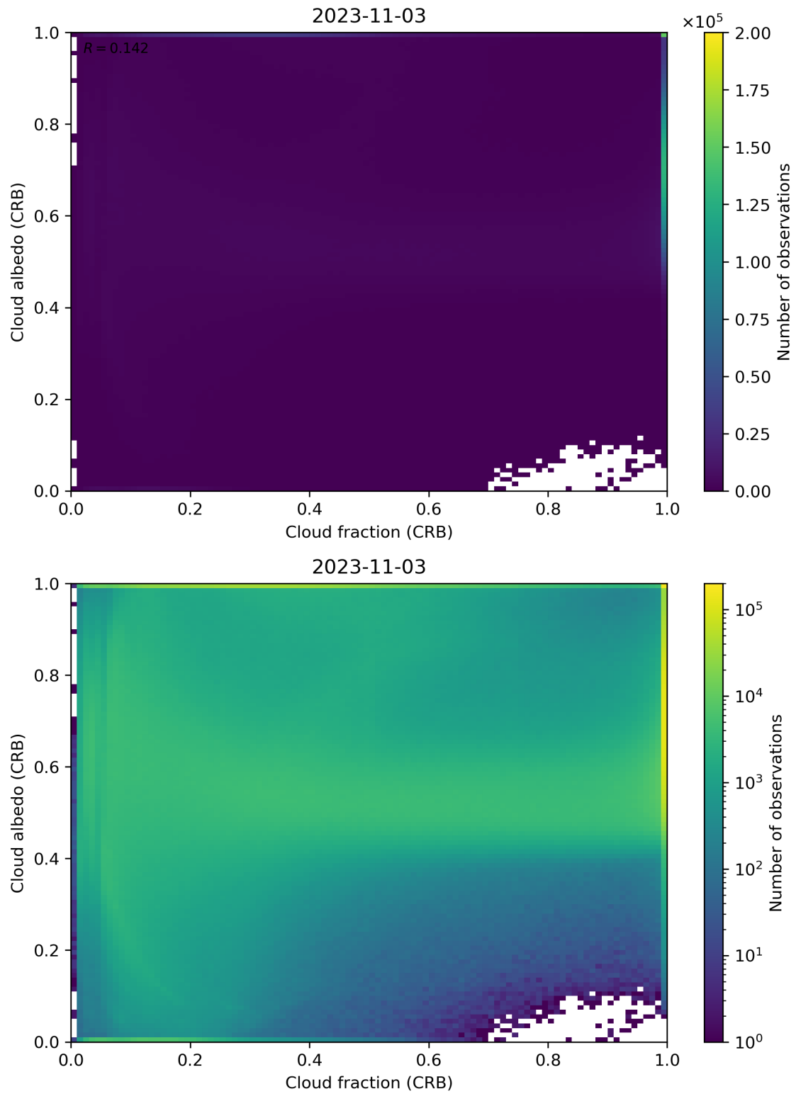
Figure 77: Scatter density plot of “Cloud fraction (CRB)” against “Cloud albedo (CRB)” for 2023-11-02 to 2023-11-04.
