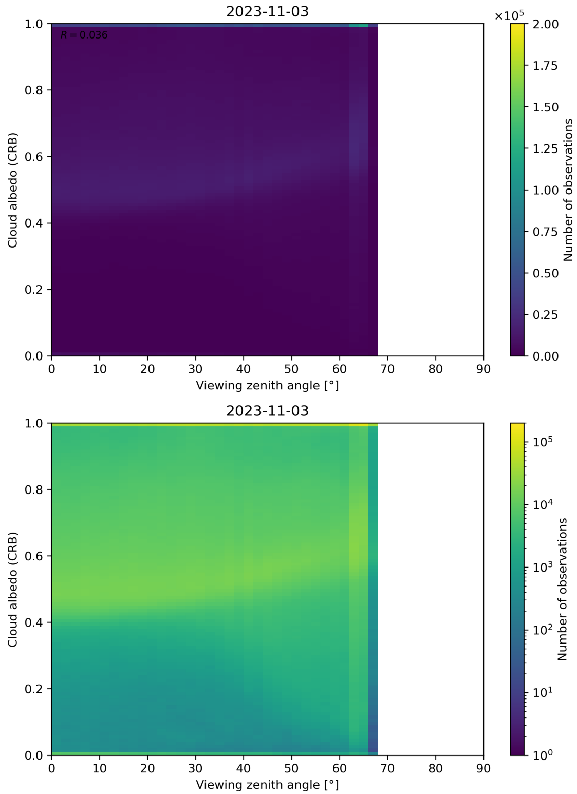
Figure 106: Scatter density plot of “Viewing zenith angle” against “Cloud albedo (CRB)” for 2023-11-02 to 2023-11-04.
