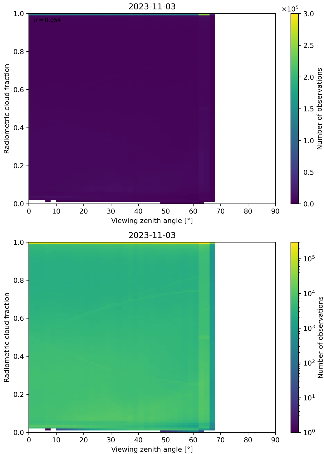
Figure 107: Scatter density plot of “Viewing zenith angle” against “Radiometric cloud fraction” for 2023-11-02 to 2023-11-04.
