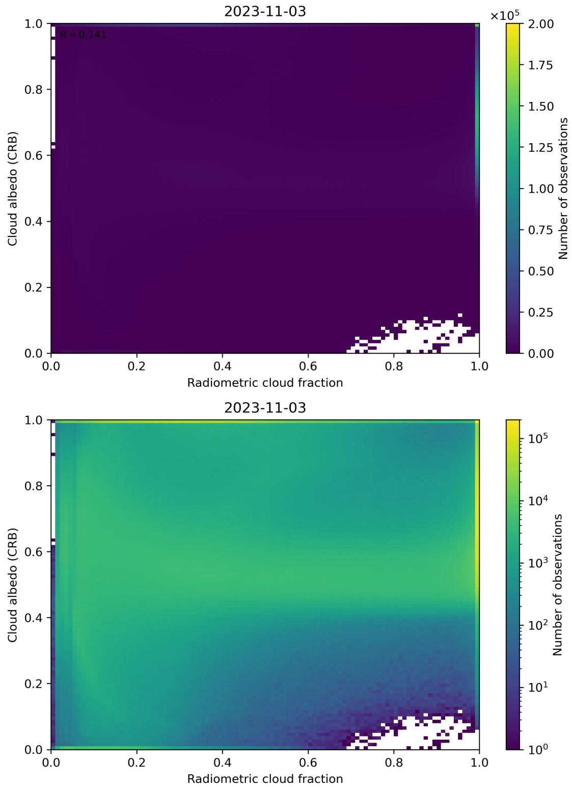
Figure 71: Scatter density plot of “Radiometric cloud fraction” against “Cloud albedo (CRB)” for 2023-11-02 to 2023-11-04.
