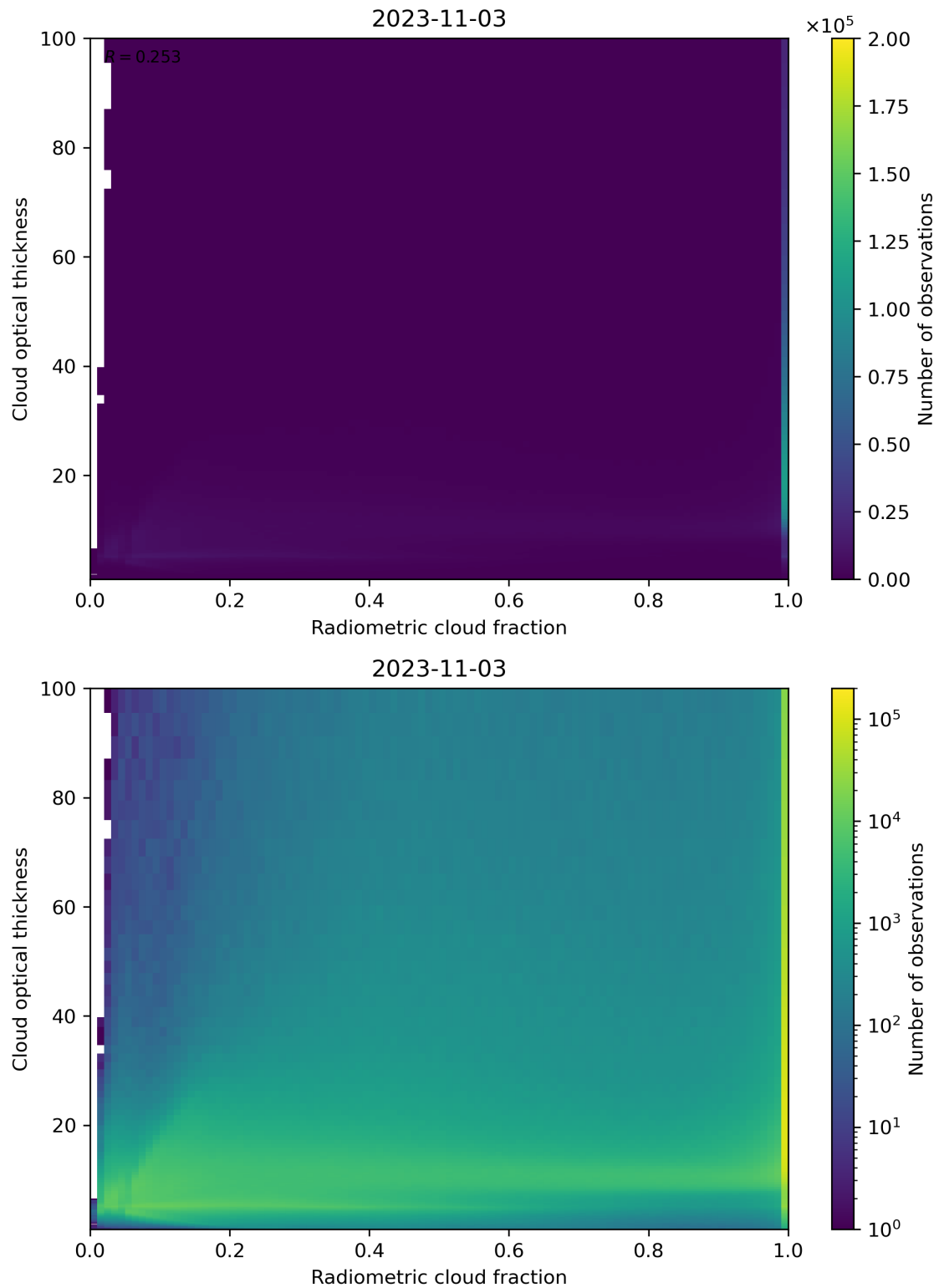
Figure 75: Scatter density plot of “Radiometric cloud fraction” against “Cloud optical thickness” for 2023-11-02 to 2023-11-04.
