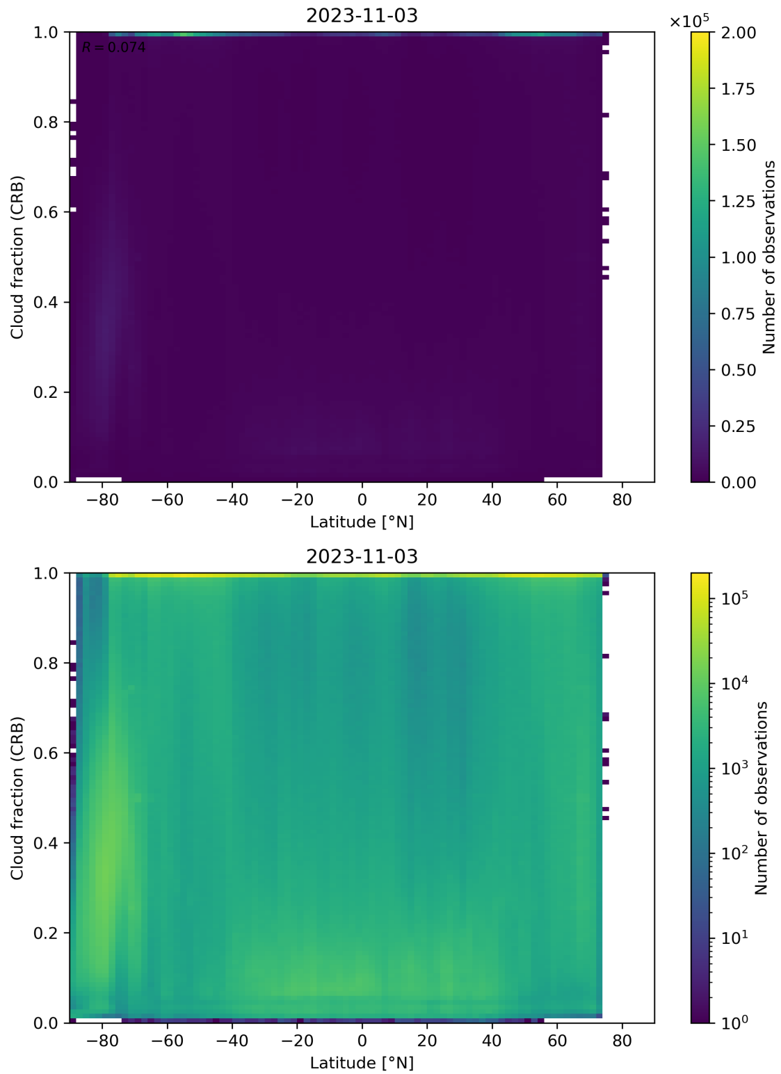
Figure 94: Scatter density plot of “Latitude” against “Cloud fraction (CRB)” for 2023-11-02 to 2023-11-04.
