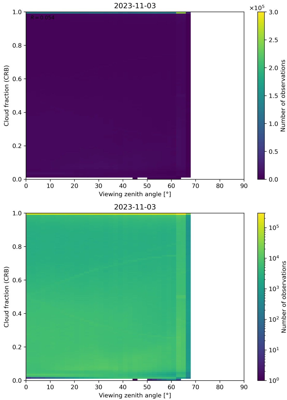
Figure 109: Scatter density plot of “Viewing zenith angle” against “Cloud fraction (CRB)” for 2023-11-02 to 2023-11-04.
