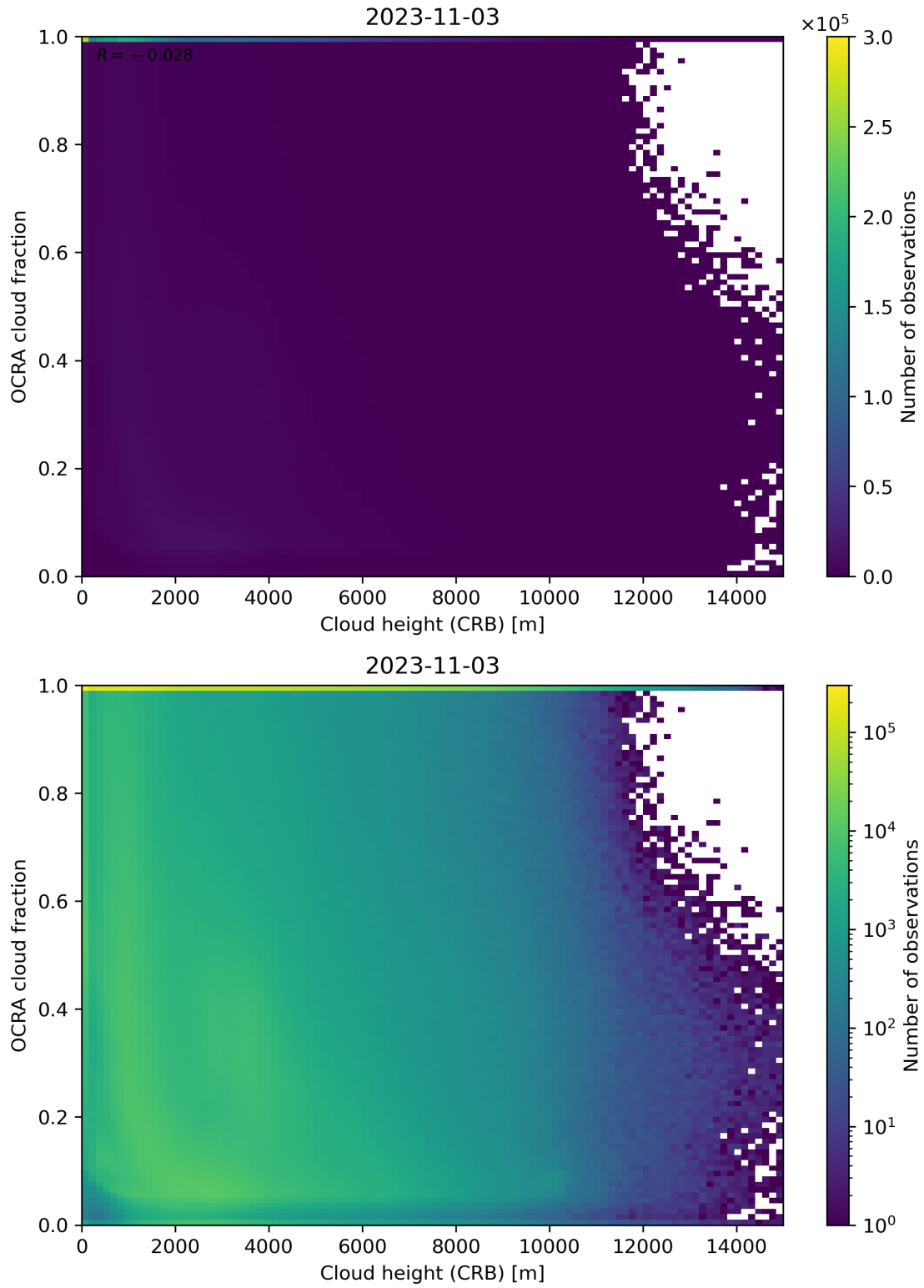
Figure 81: Scatter density plot of “Cloud height (CRB)” against “OCRA cloud fraction” for 2023-11-02 to 2023-11-04.
