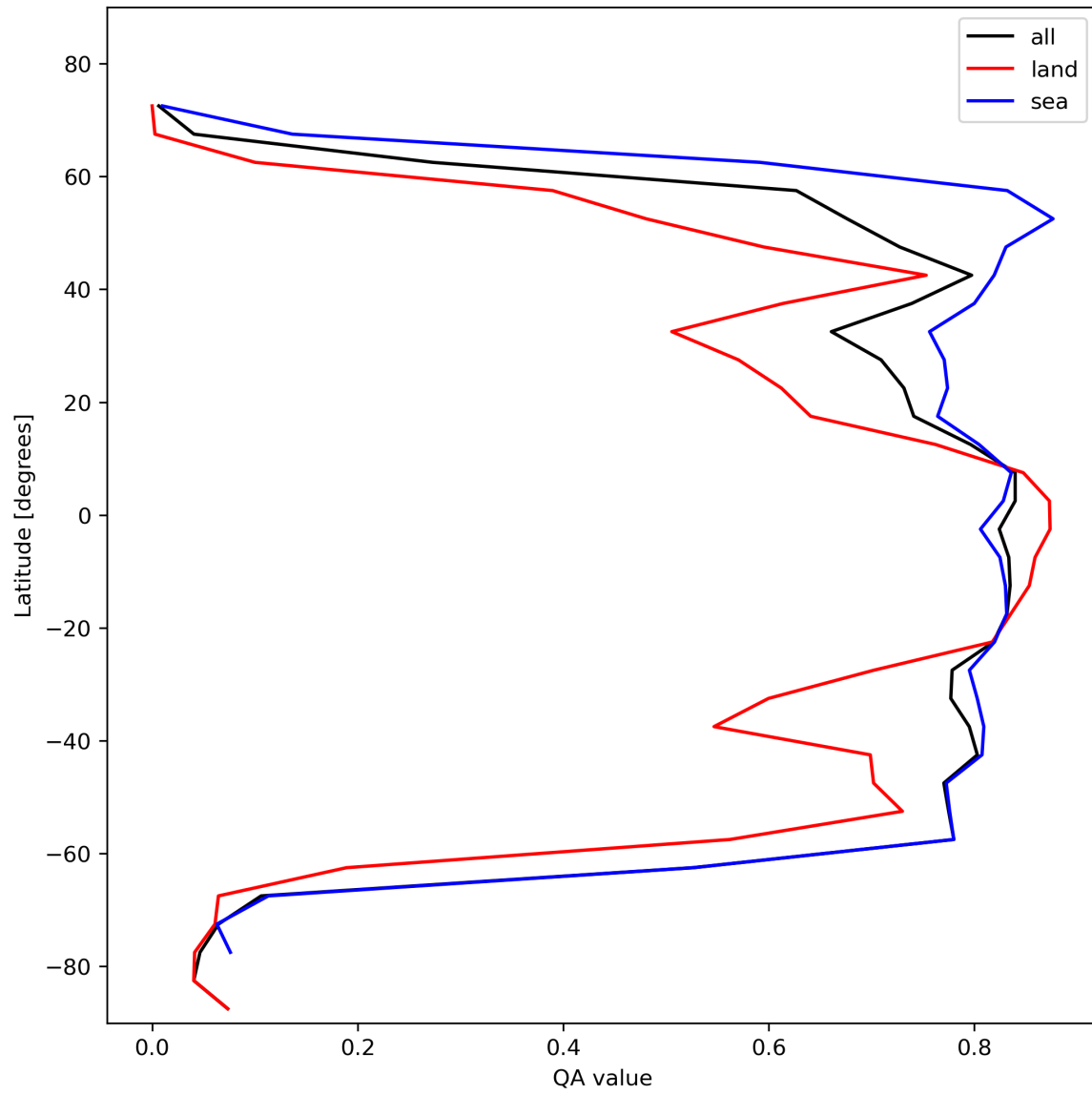
Figure 22: Zonal average of “QA value” for 2023-11-02 to 2023-11-04.
