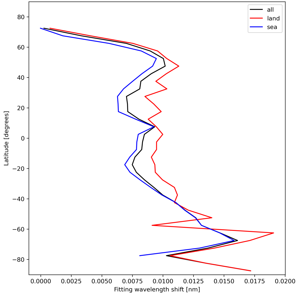
Figure 33: Zonal average of “Fitting wavelength shift” for 2023-11-02 to 2023-11-04.
