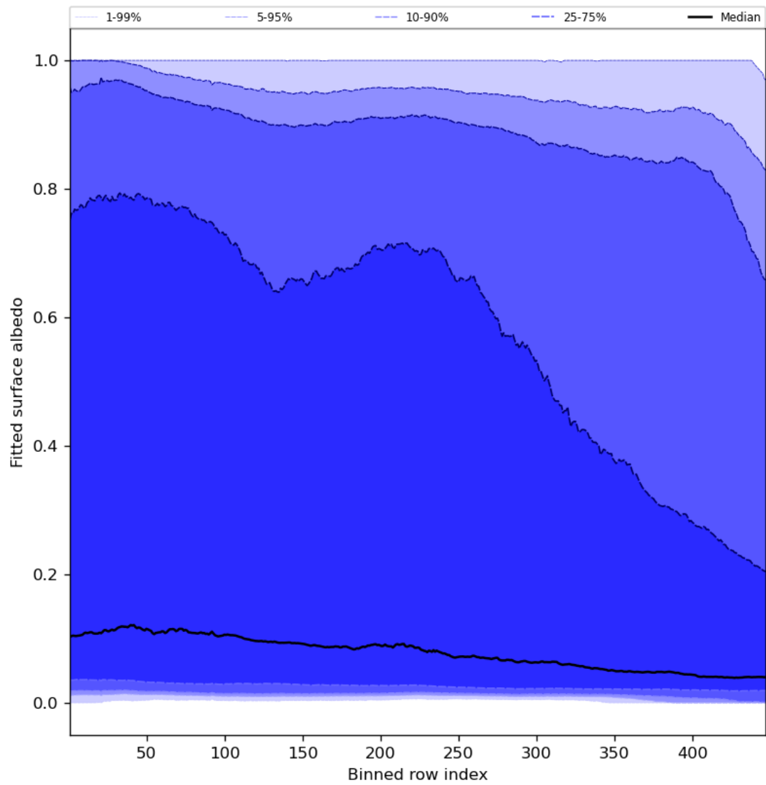
Figure 61: Along track statistics of “Fitted surface albedo” for 2023-11-02 to 2023-11-04
