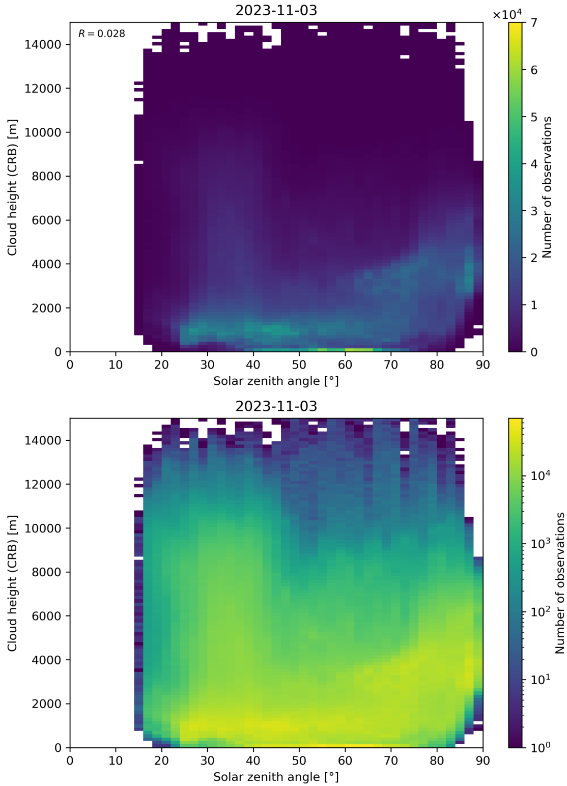
Figure 102: Scatter density plot of “Solar zenith angle” against “Cloud height (CRB)” for 2023-11-02 to 2023-11-04.
