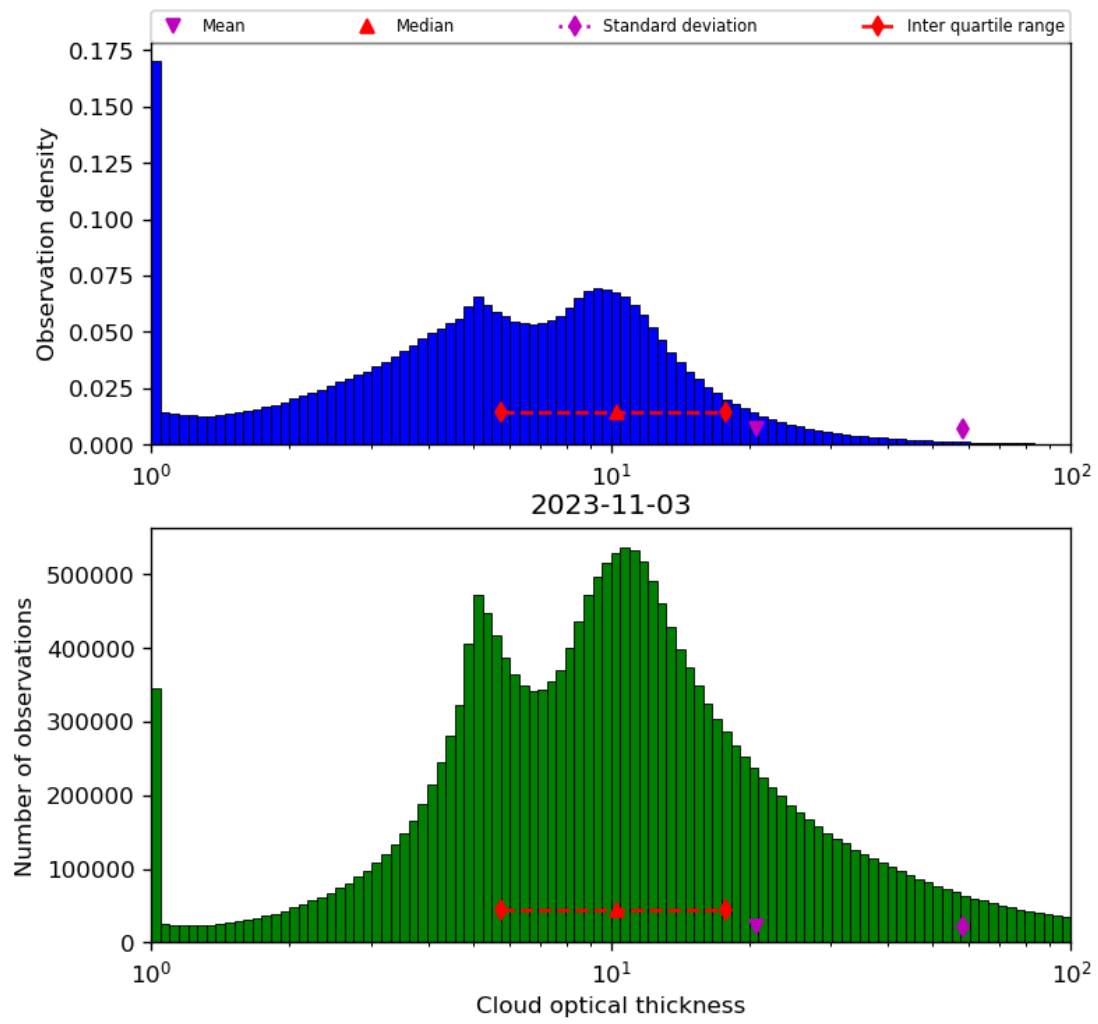
Figure 41: Histogram of “Cloud optical thickness” for 2023-11-02 to 2023-11-04
