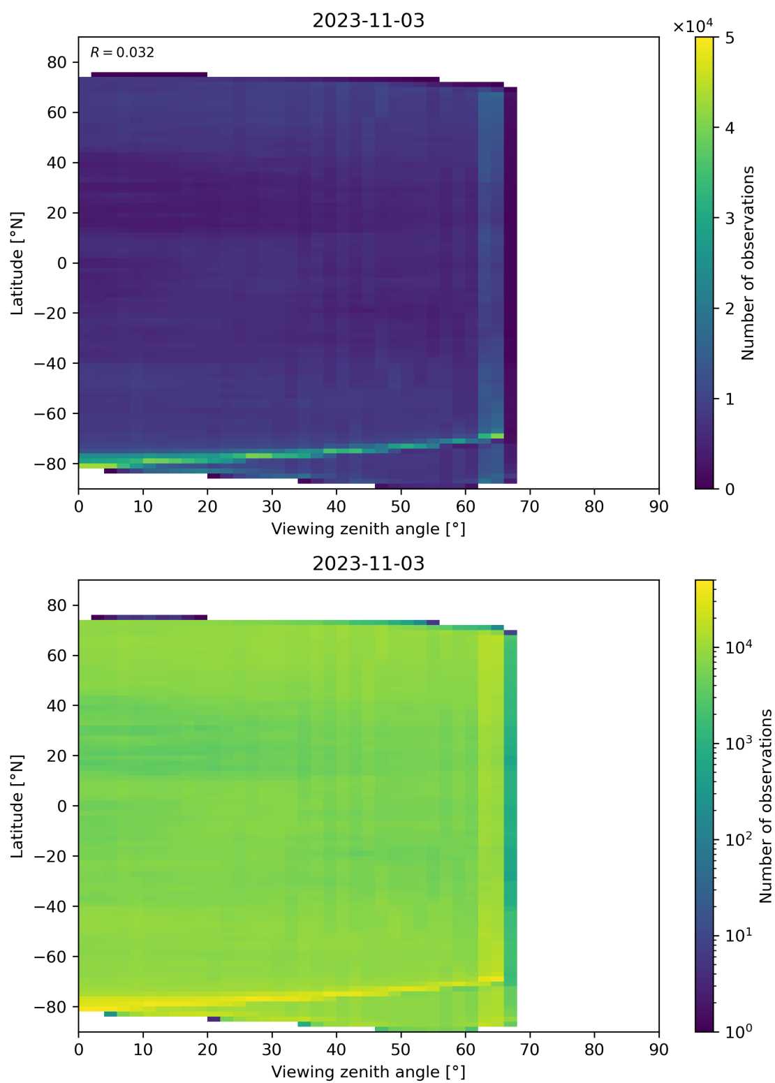
Figure 113: Scatter density plot of “Viewing zenith angle” against “Latitude” for 2023-11-02 to 2023-11-04.
