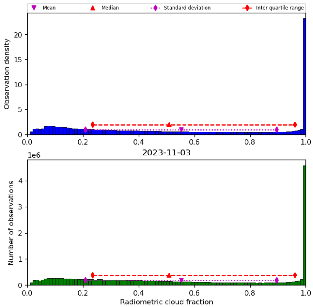
Figure 39: Histogram of “Radiometric cloud fraction” for 2023-11-02 to 2023-11-04
