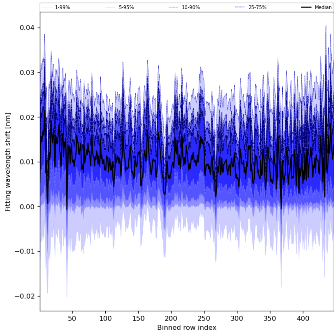
Figure 65: Along track statistics of “Fitting wavelength shift” for 2023-11-02 to 2023-11-04
