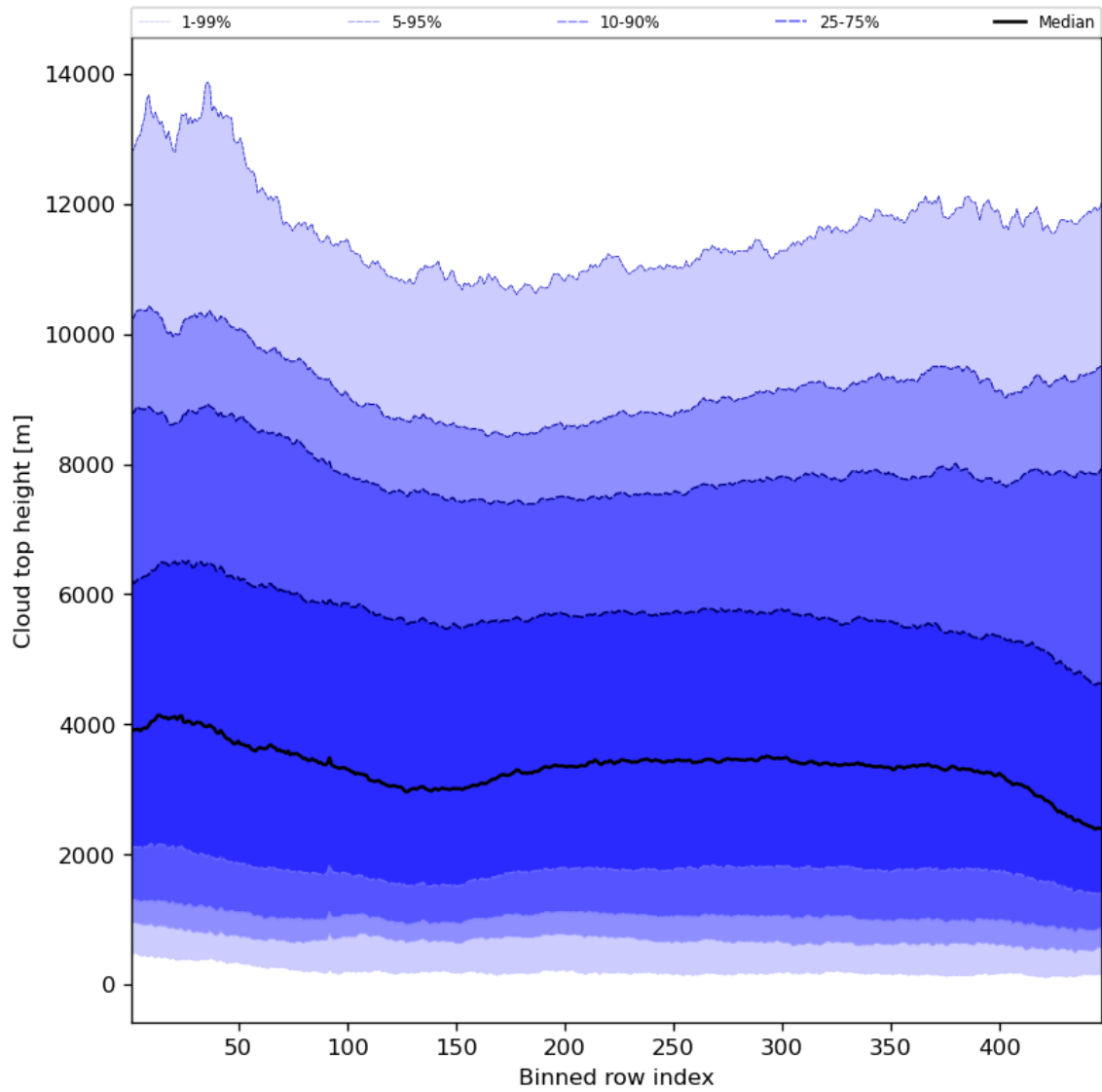
Figure 56: Along track statistics of “Cloud top height” for 2023-11-02 to 2023-11-04
