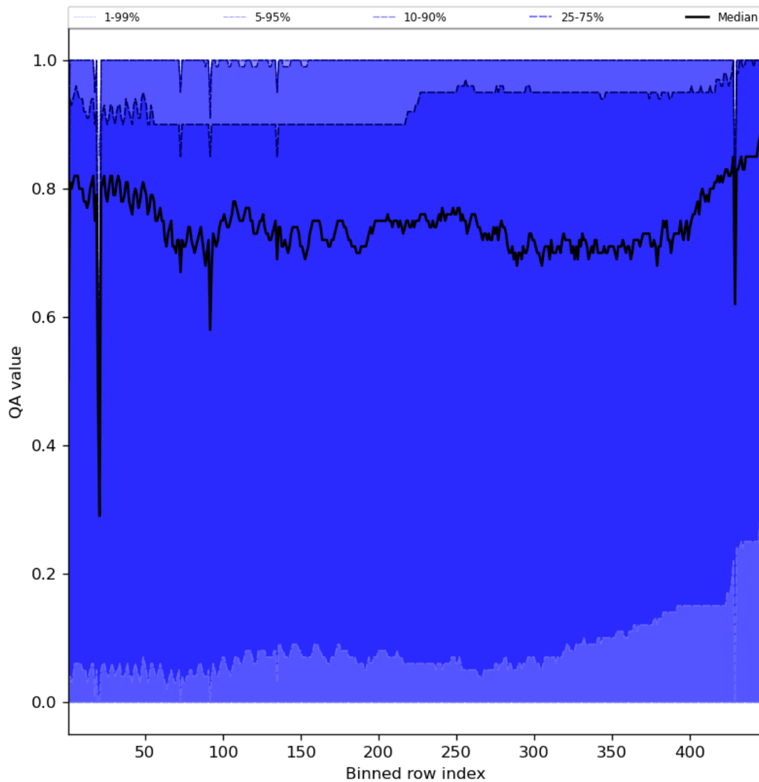
Figure 54: Along track statistics of “QA value” for 2023-11-02 to 2023-11-04
