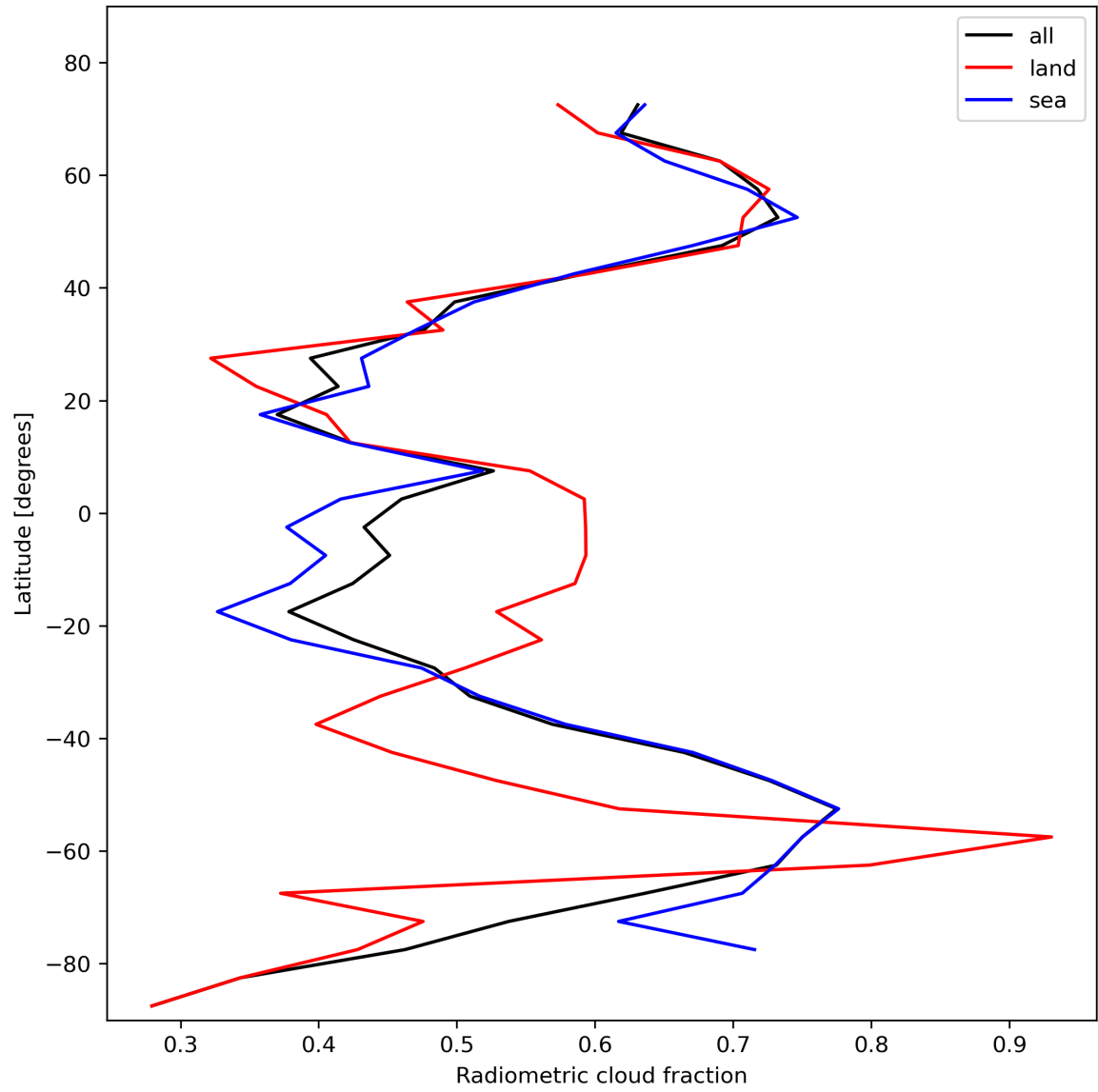
Figure 23: Zonal average of “Radiometric cloud fraction” for 2023-11-02 to 2023-11-04.
