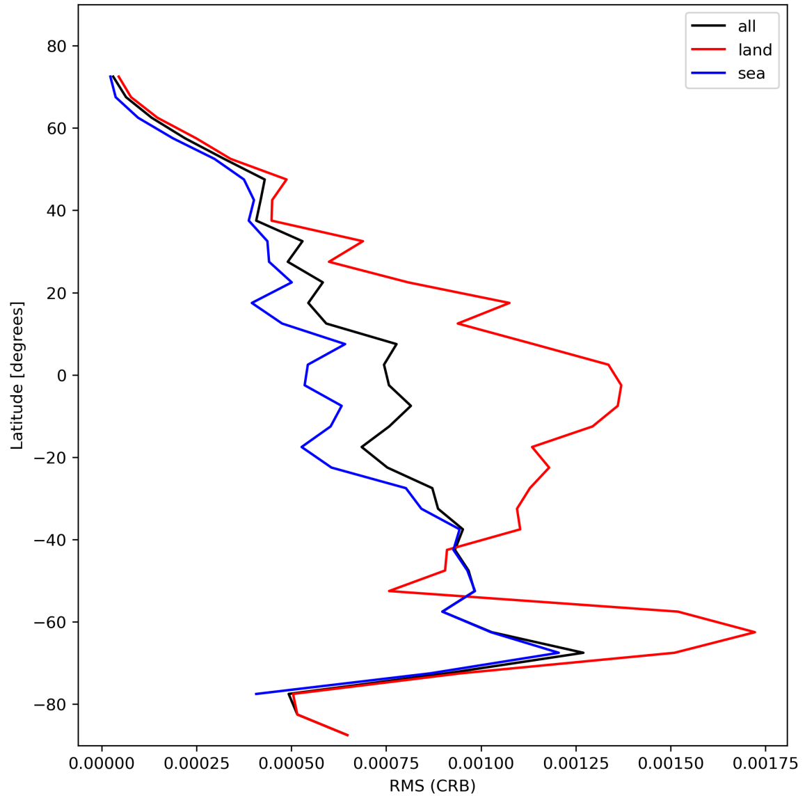
Figure 32: Zonal average of “RMS (CRB)” for 2023-11-02 to 2023-11-04.
