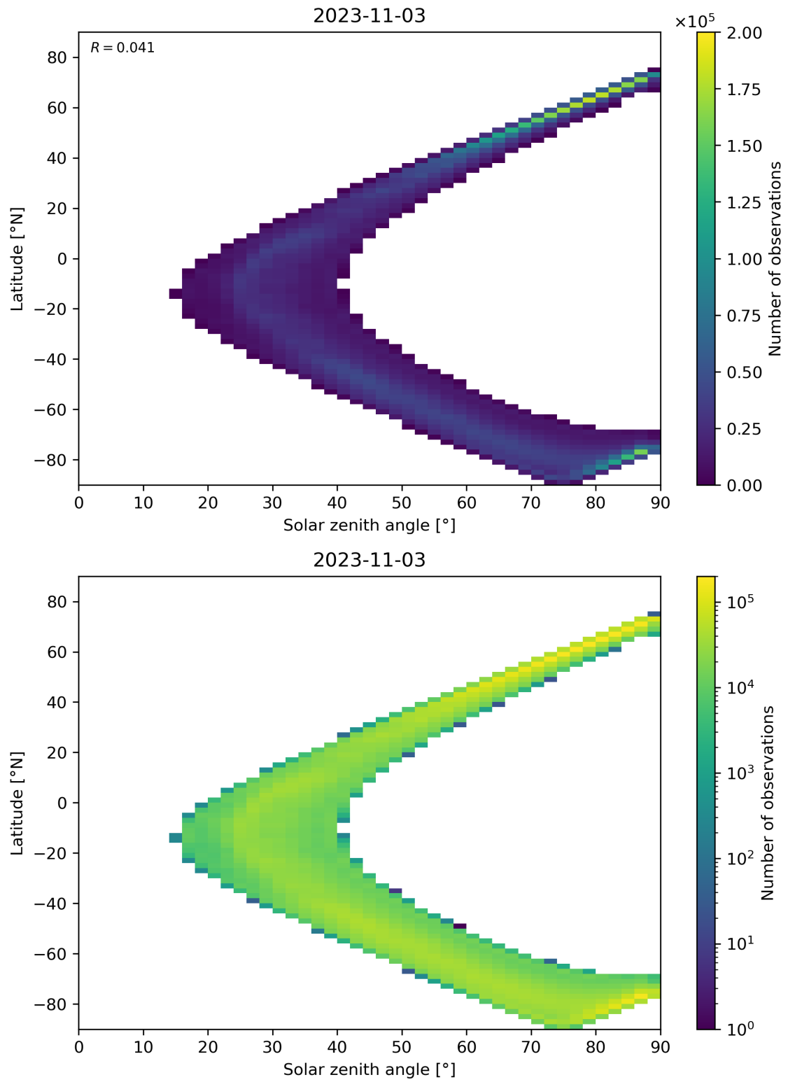
Figure 105: Scatter density plot of “Solar zenith angle” against “Latitude” for 2023-11-02 to 2023-11-04.
