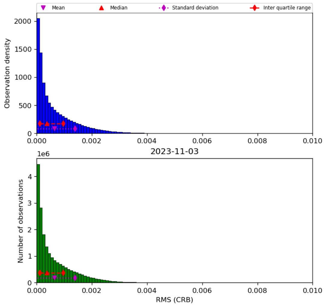
Figure 48: Histogram of “RMS (CRB)” for 2023-11-02 to 2023-11-04
