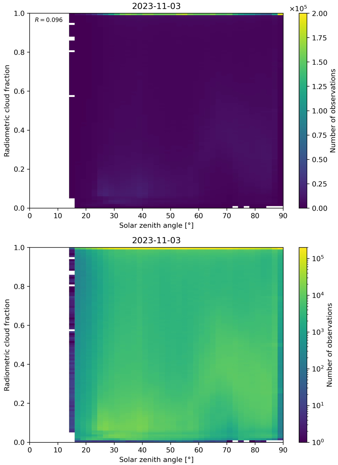
Figure 99: Scatter density plot of “Solar zenith angle” against “Radiometric cloud fraction” for 2023-11-02 to 2023-11-04.
