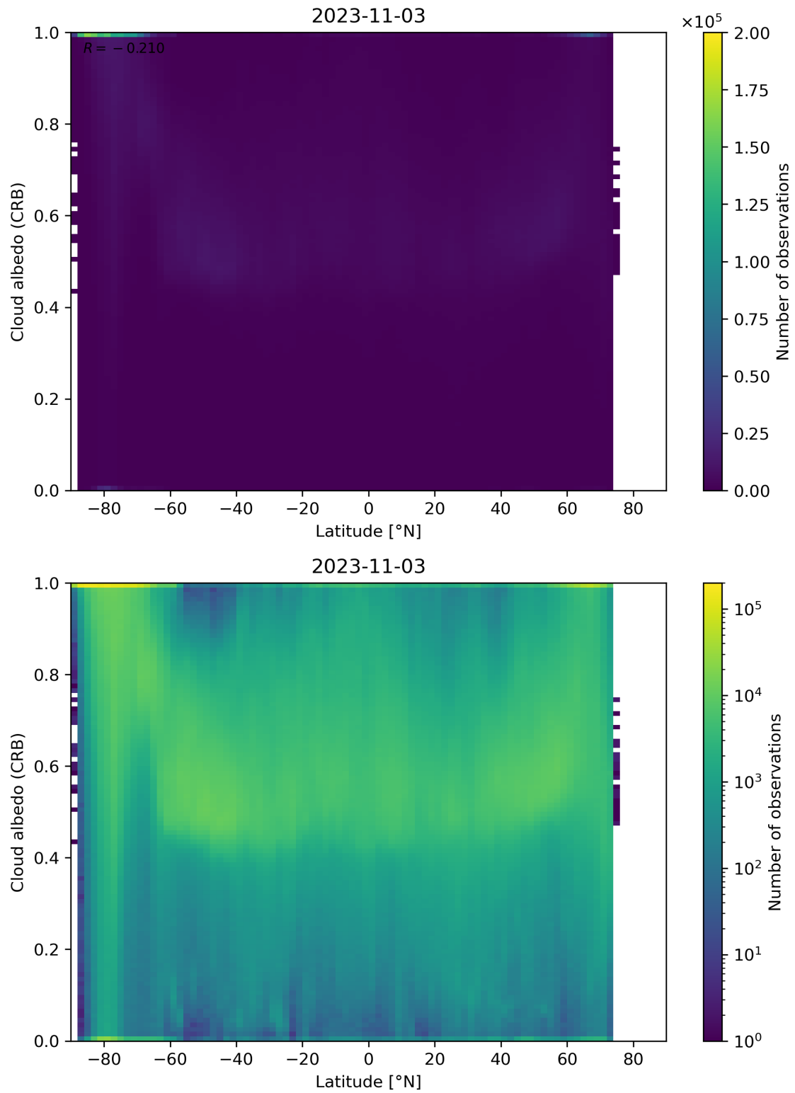
Figure 91: Scatter density plot of “Latitude” against “Cloud albedo (CRB)” for 2023-11-02 to 2023-11-04.
