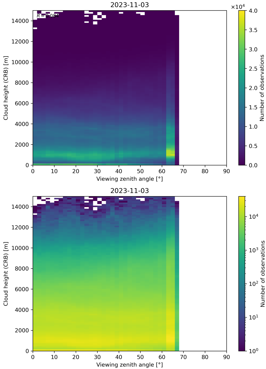
Figure 110: Scatter density plot of “Viewing zenith angle” against “Cloud height (CRB)” for 2023-11-02 to 2023-11-04.
