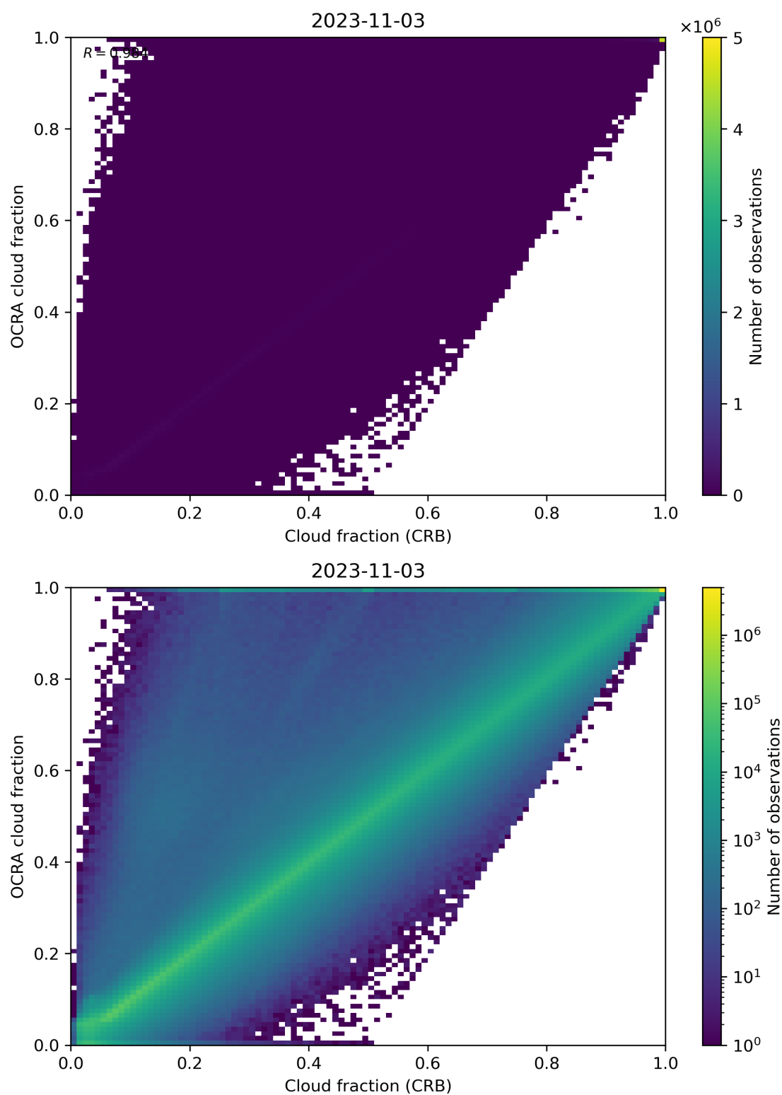
Figure 78: Scatter density plot of “Cloud fraction (CRB)” against “OCRA cloud fraction” for 2023-11-02 to 2023-11-04.
