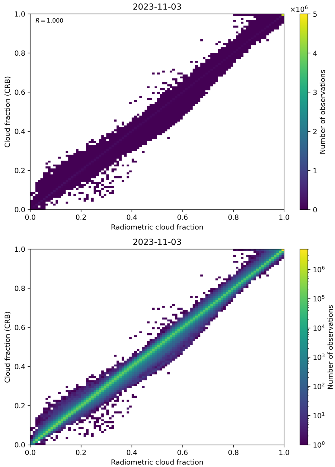
Figure 73: Scatter density plot of “Radiometric cloud fraction” against “Cloud fraction (CRB)” for 2023-11-02 to 2023-11-04.
