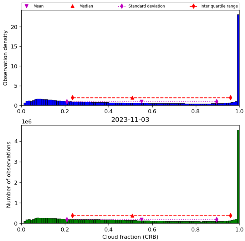
Figure 42: Histogram of “Cloud fraction (CRB)” for 2023-11-02 to 2023-11-04
