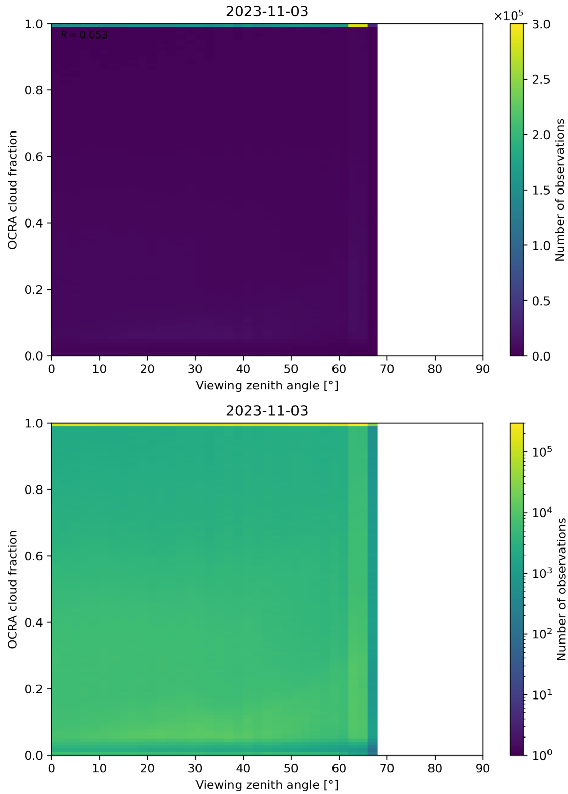
Figure 108: Scatter density plot of “Viewing zenith angle” against “OCRA cloud fraction” for 2023-11-02 to 2023-11-04.
