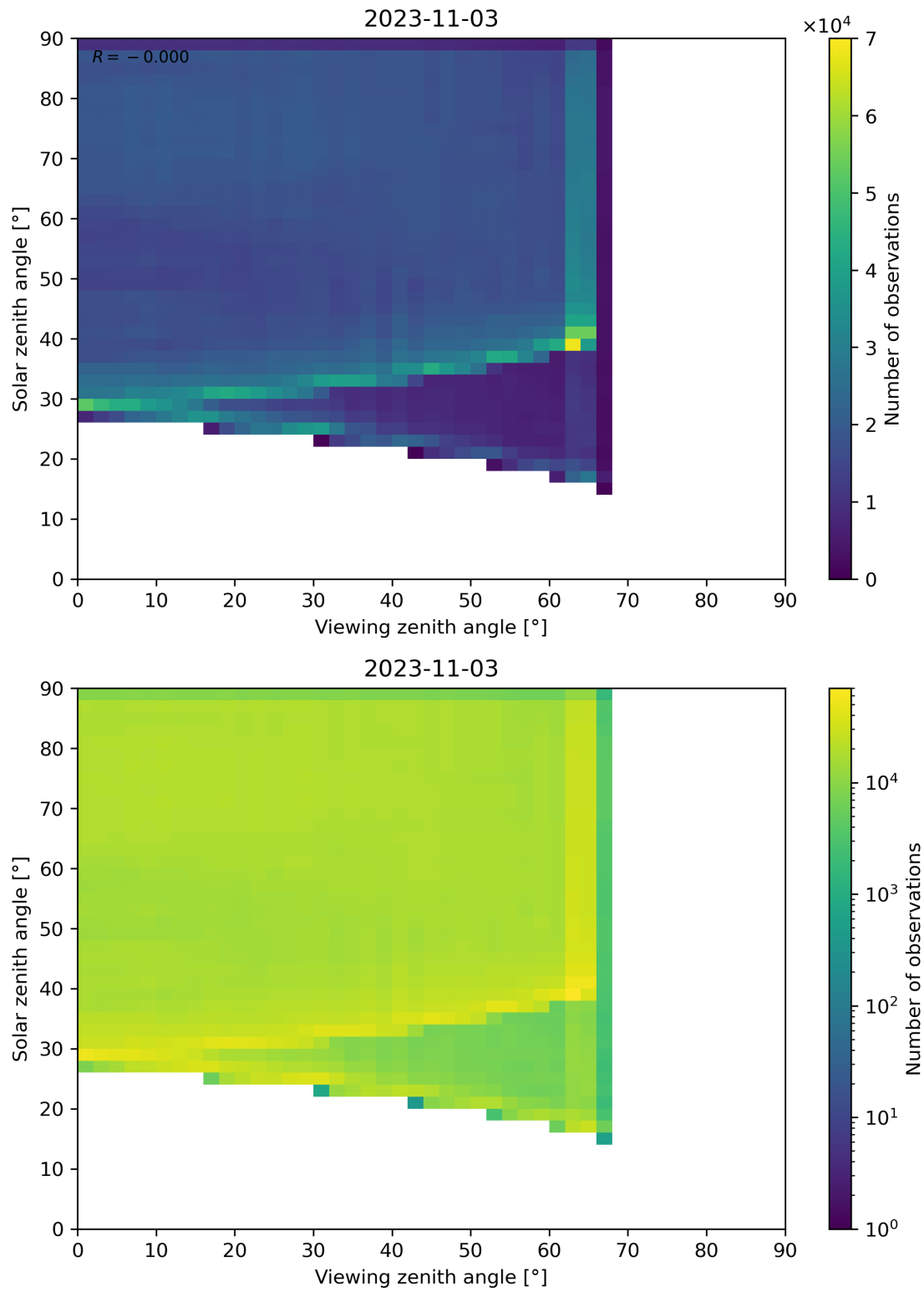
Figure 114: Scatter density plot of “Viewing zenith angle” against “Solar zenith angle” for 2023-11-02 to 2023-11-04.
