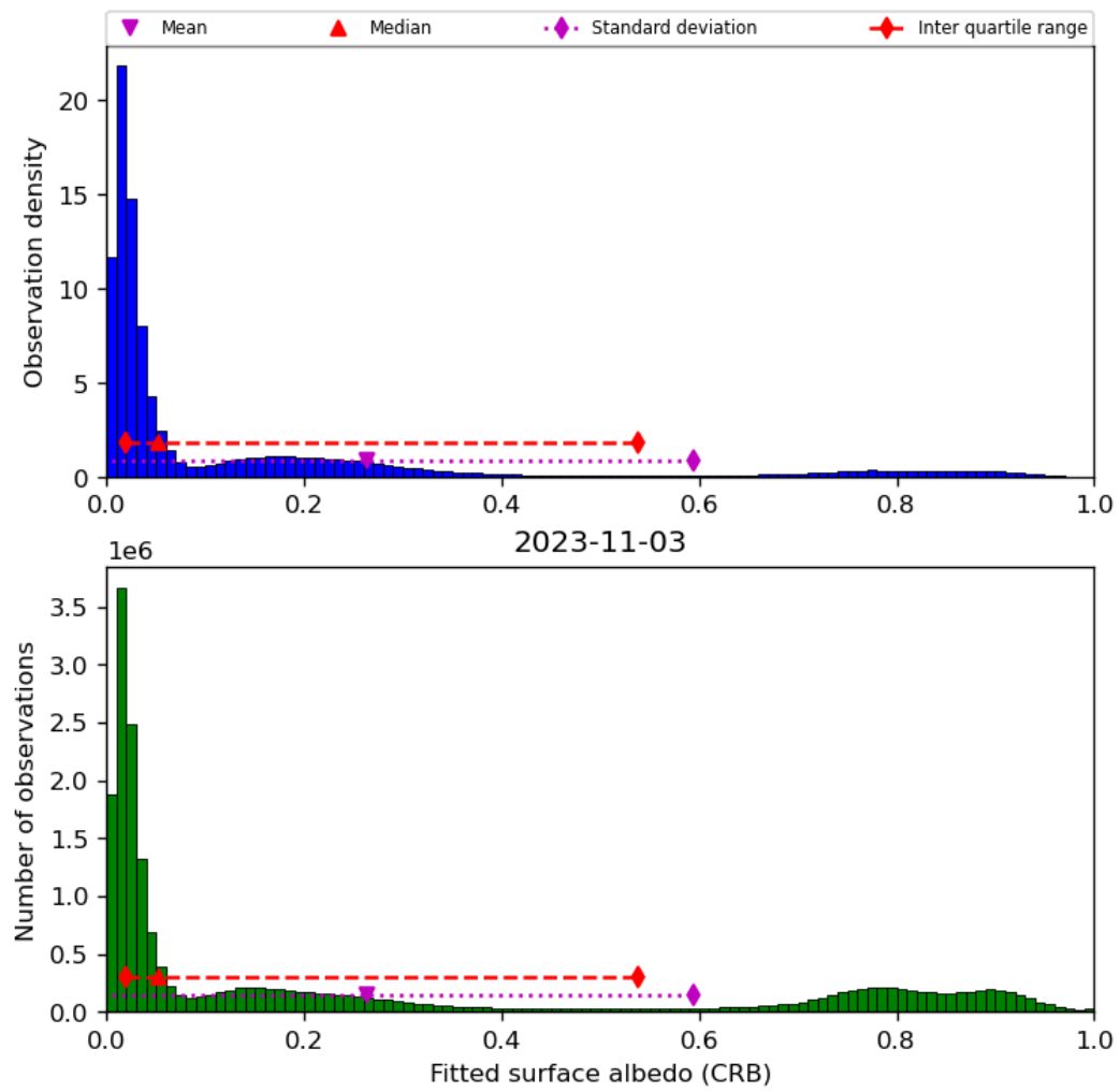
Figure 46: Histogram of “Fitted surface albedo (CRB)” for 2023-11-02 to 2023-11-04
