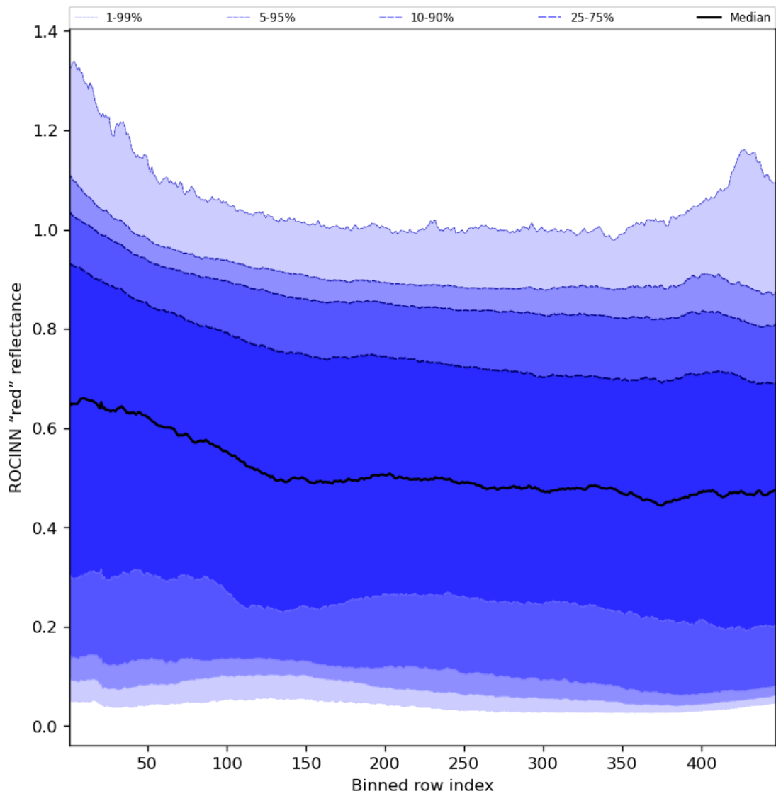
Figure 69: Along track statistics of “ROCINN “red” reflectance” for 2023-11-02 to 2023-11-04
