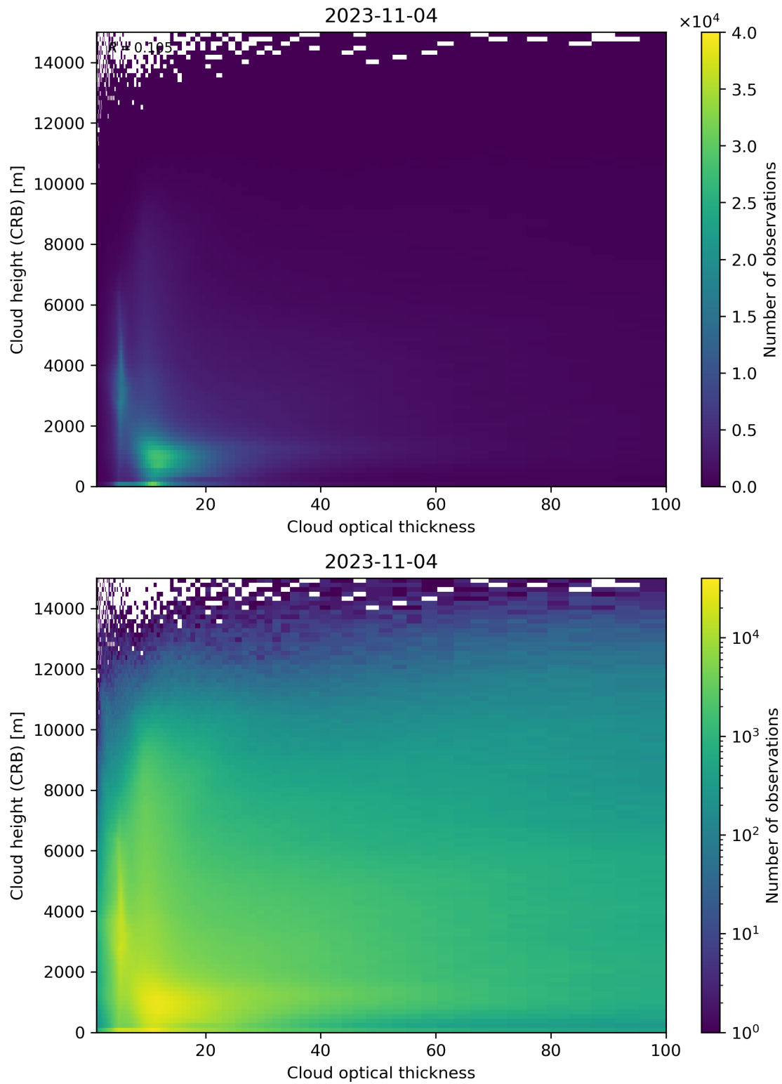
Figure 85: Scatter density plot of “Cloud optical thickness” against “Cloud height (CRB)” for 2023-11-03 to 2023-11-05.
