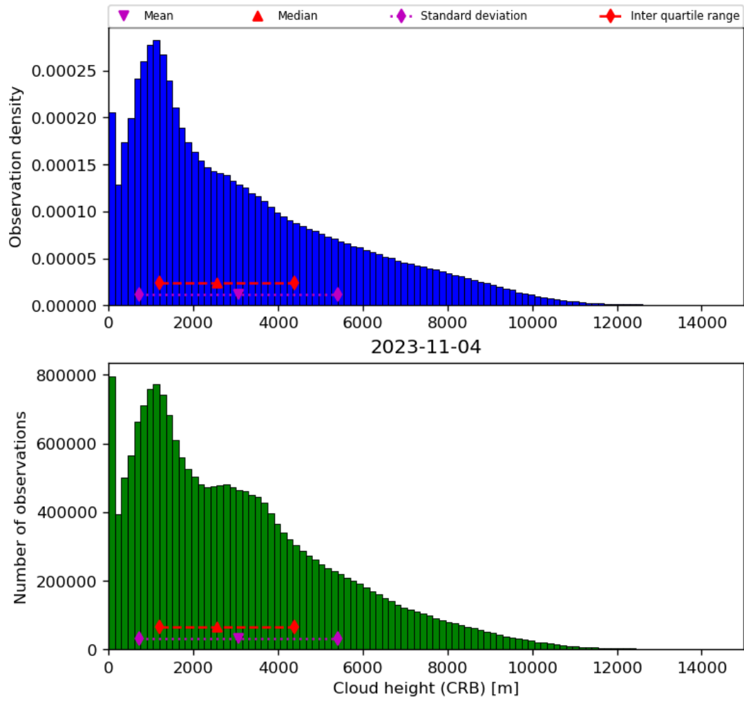
Figure 43: Histogram of “Cloud height (CRB)” for 2023-11-03 to 2023-11-05
