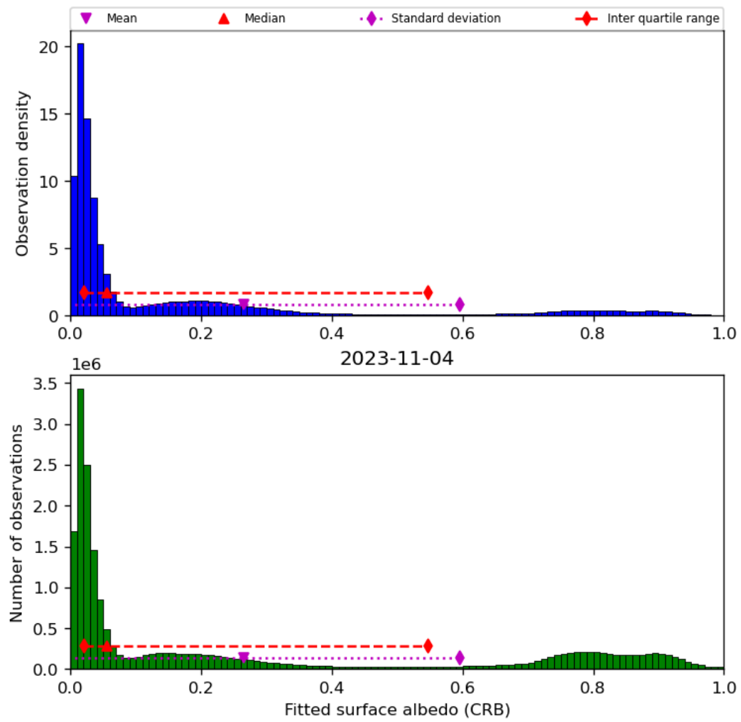
Figure 46: Histogram of “Fitted surface albedo (CRB)” for 2023-11-03 to 2023-11-05
