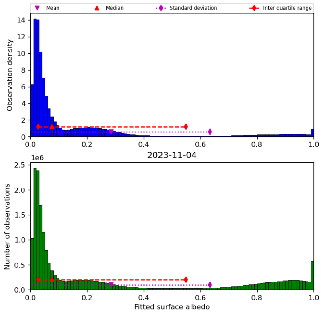
Figure 45: Histogram of “Fitted surface albedo” for 2023-11-03 to 2023-11-05
