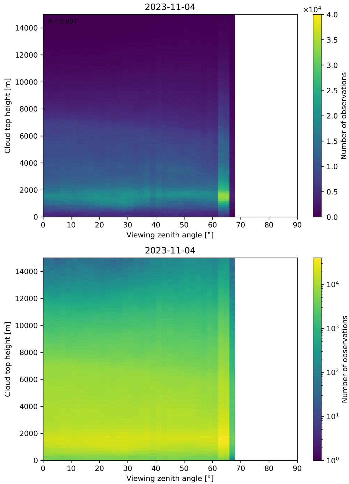
Figure 112: Scatter density plot of “Viewing zenith angle” against “Cloud top height” for 2023-11-03 to 2023-11-05.
