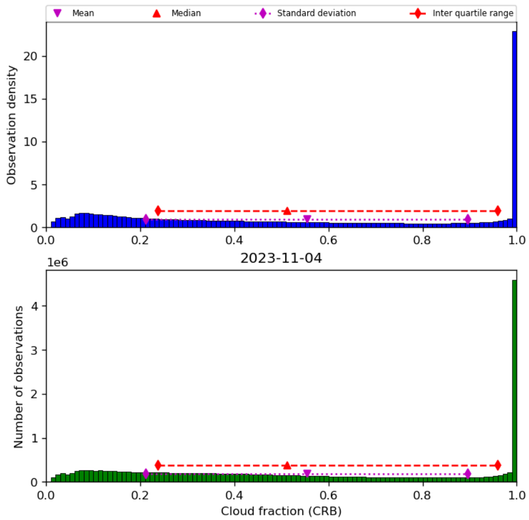
Figure 42: Histogram of “Cloud fraction (CRB)” for 2023-11-03 to 2023-11-05
