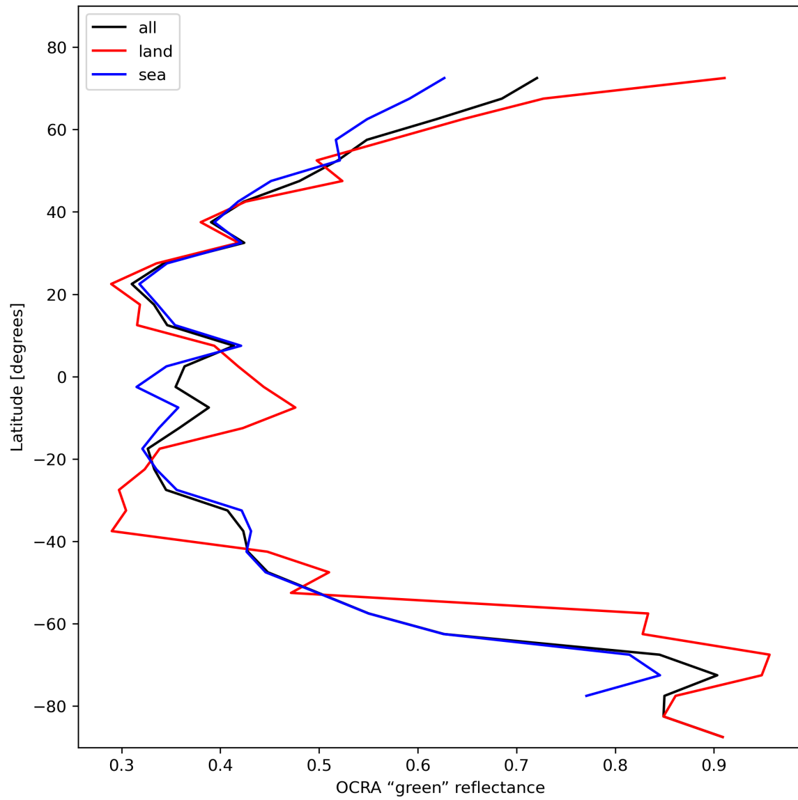
Figure 36: Zonal average of “OCRA “green” reflectance” for 2023-11-03 to 2023-11-05.
