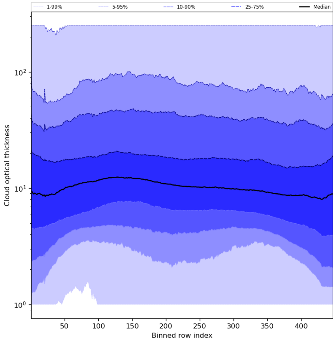
Figure 57: Along track statistics of “Cloud optical thickness” for 2023-11-03 to 2023-11-05
