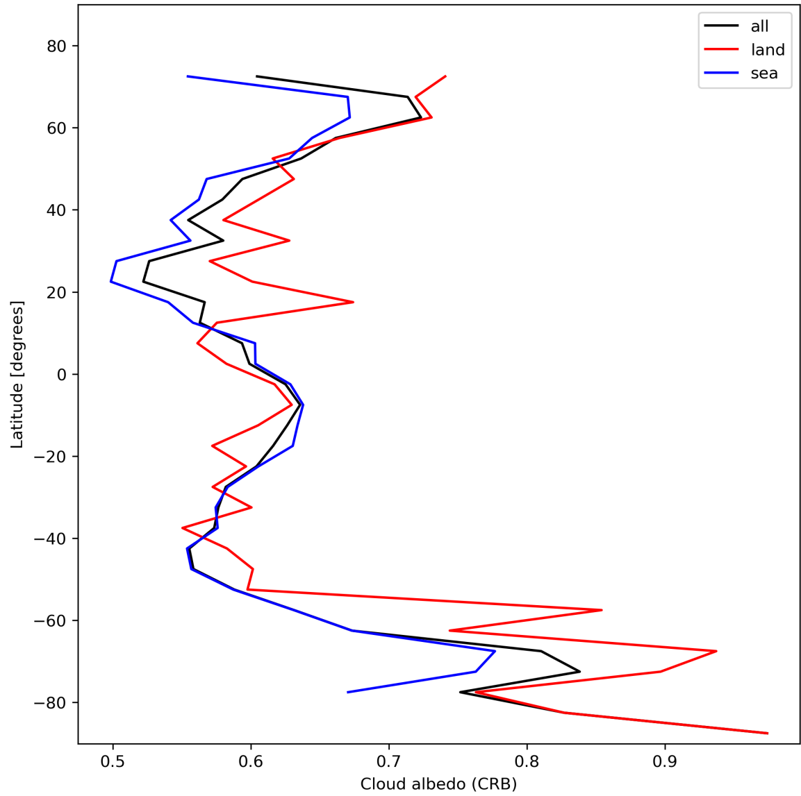
Figure 28: Zonal average of “Cloud albedo (CRB)” for 2023-11-03 to 2023-11-05.
