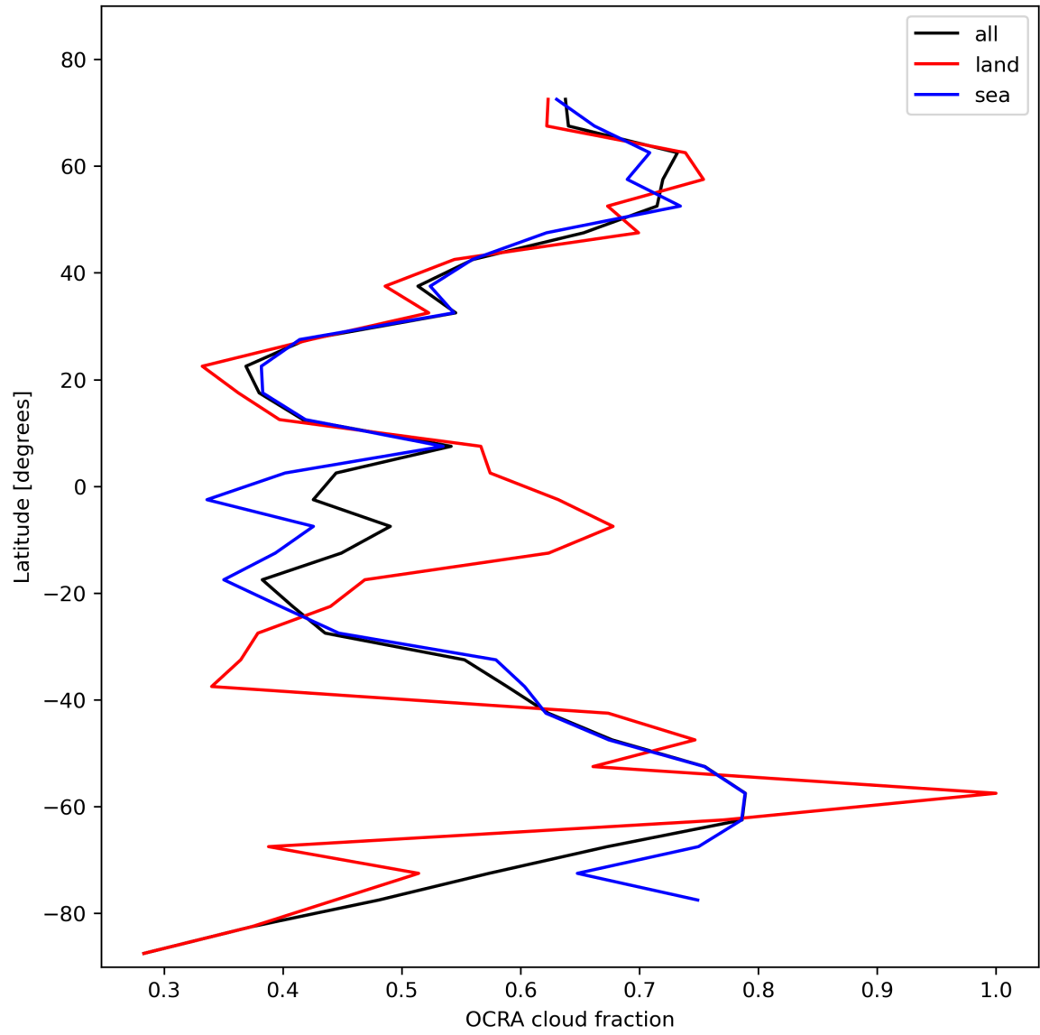
Figure 34: Zonal average of “OCRA cloud fraction” for 2023-11-03 to 2023-11-05.
