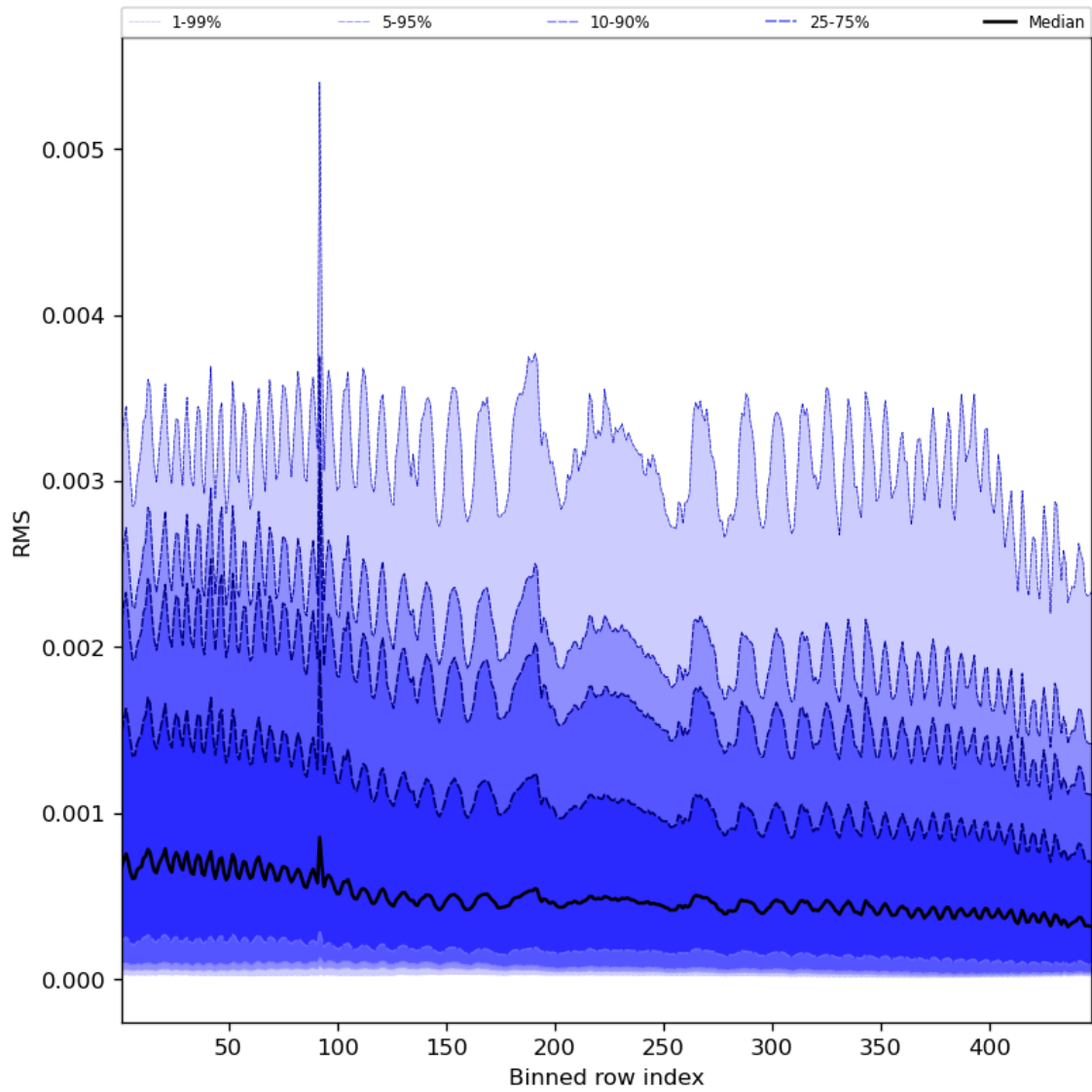
Figure 63: Along track statistics of “RMS” for 2023-11-03 to 2023-11-05
