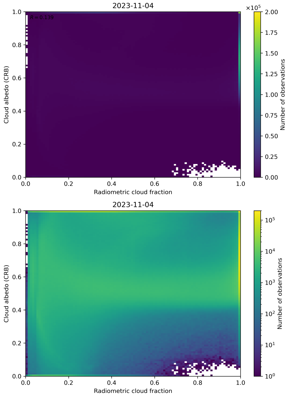
Figure 71: Scatter density plot of “Radiometric cloud fraction” against “Cloud albedo (CRB)” for 2023-11-03 to 2023-11-05.
