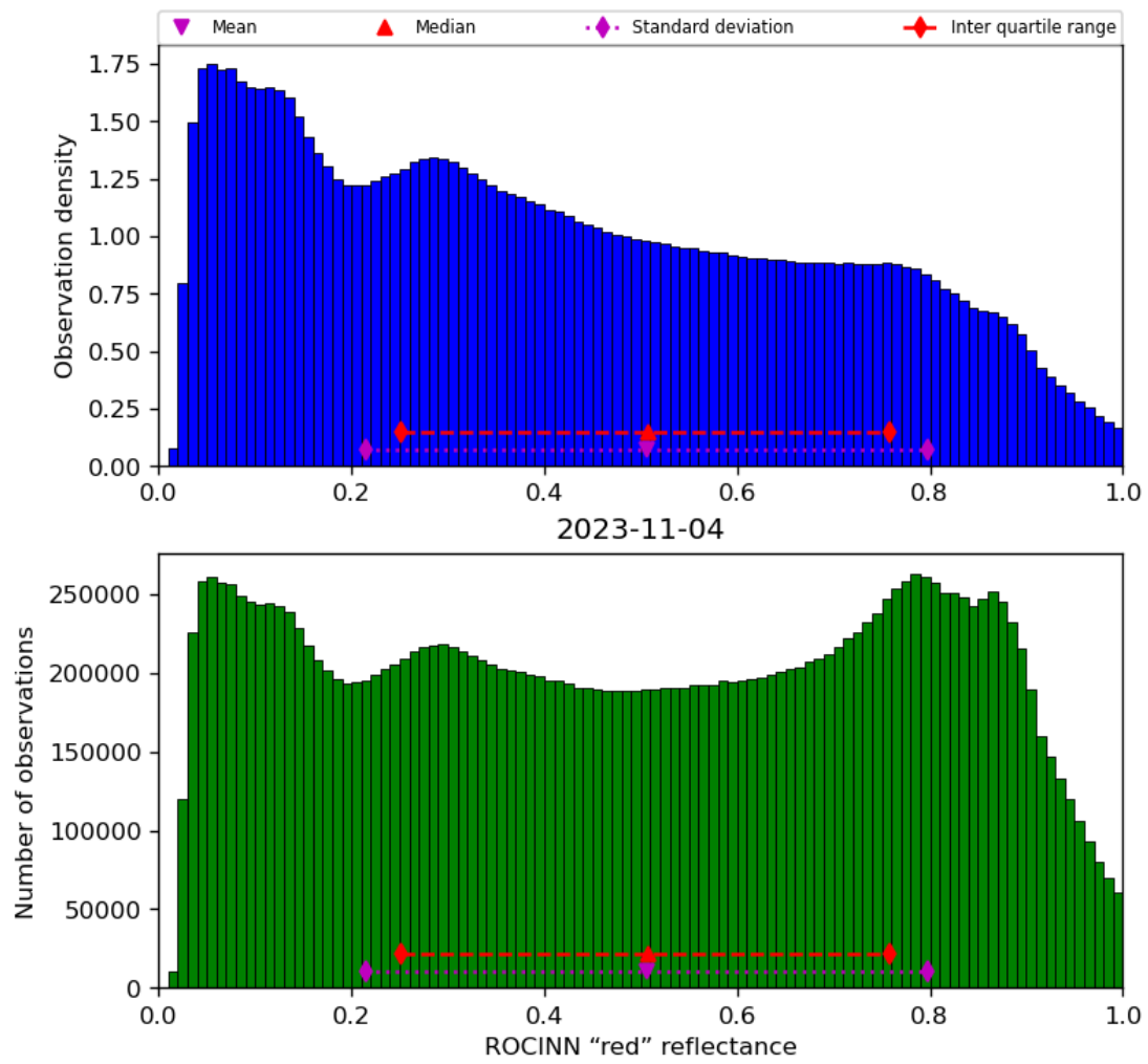
Figure 53: Histogram of “ROCINN “red” reflectance” for 2023-11-03 to 2023-11-05
