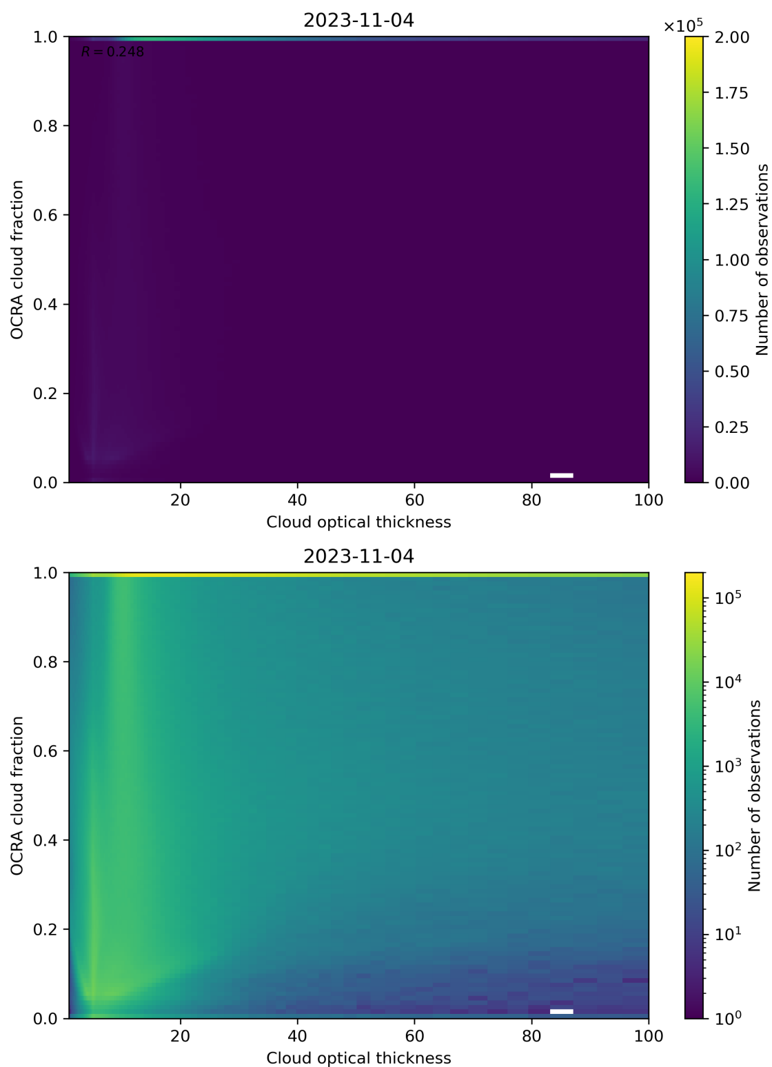
Figure 83: Scatter density plot of “Cloud optical thickness” against “OCRA cloud fraction” for 2023-11-03 to 2023-11-05.
