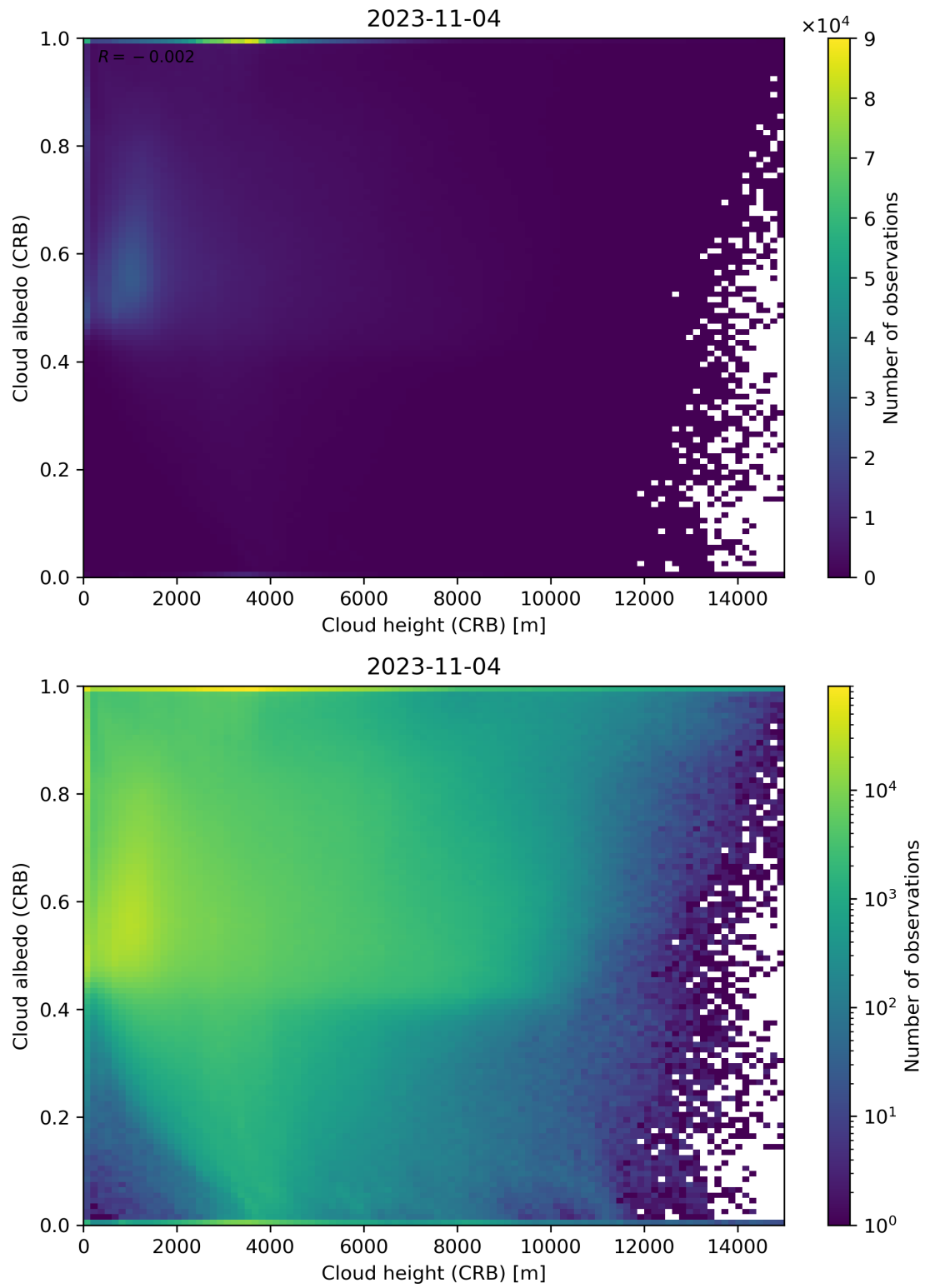
Figure 80: Scatter density plot of “Cloud height (CRB)” against “Cloud albedo (CRB)” for 2023-11-03 to 2023-11-05.
