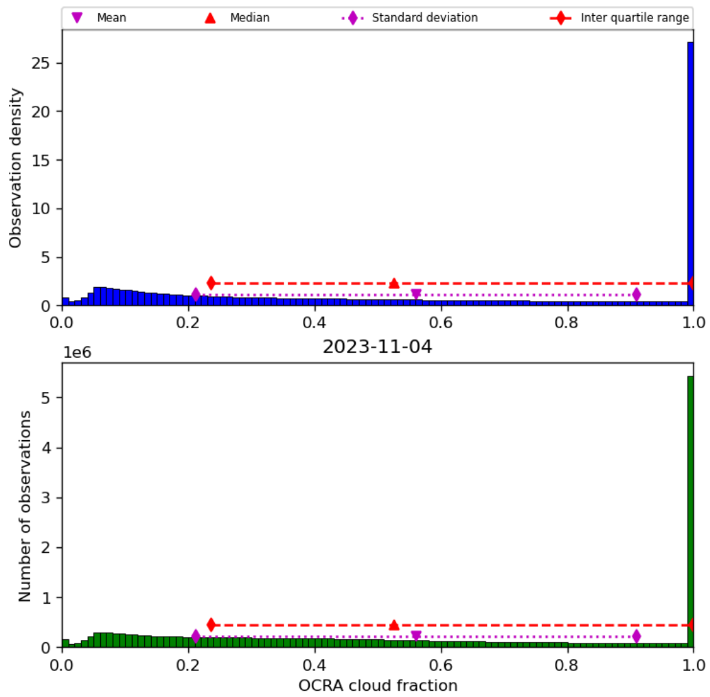
Figure 50: Histogram of “OCRA cloud fraction” for 2023-11-03 to 2023-11-05
