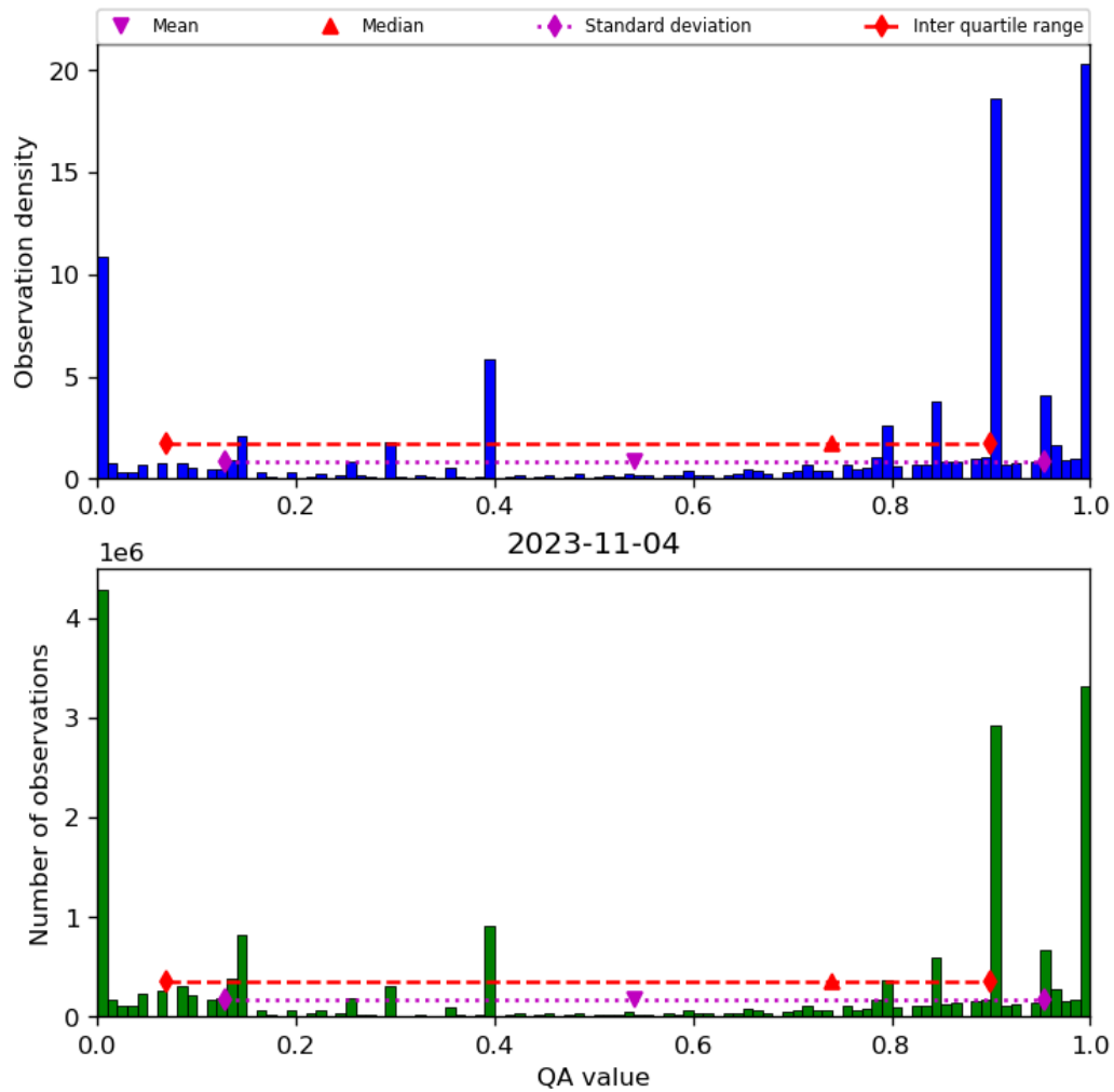
Figure 38: Histogram of “QA value” for 2023-11-03 to 2023-11-05
