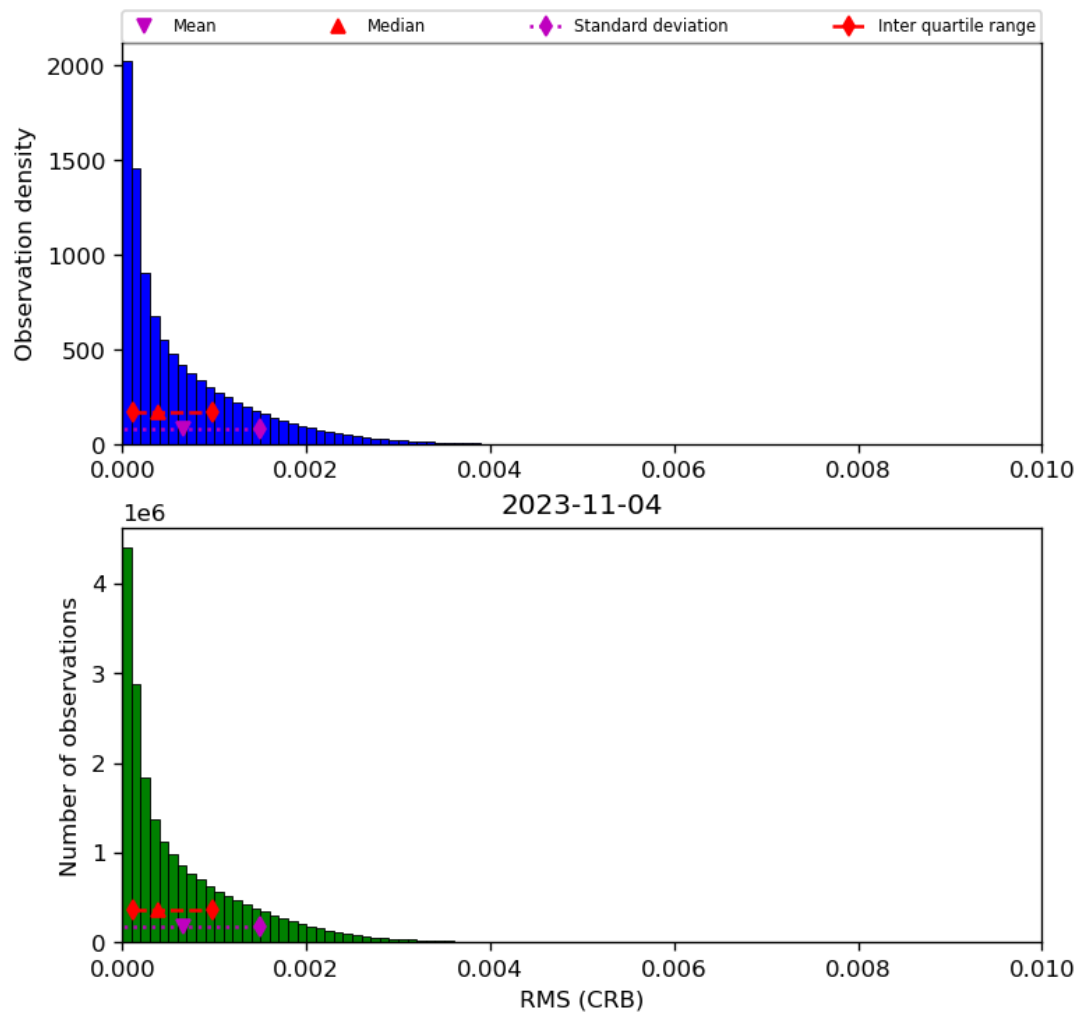
Figure 48: Histogram of “RMS (CRB)” for 2023-11-03 to 2023-11-05
