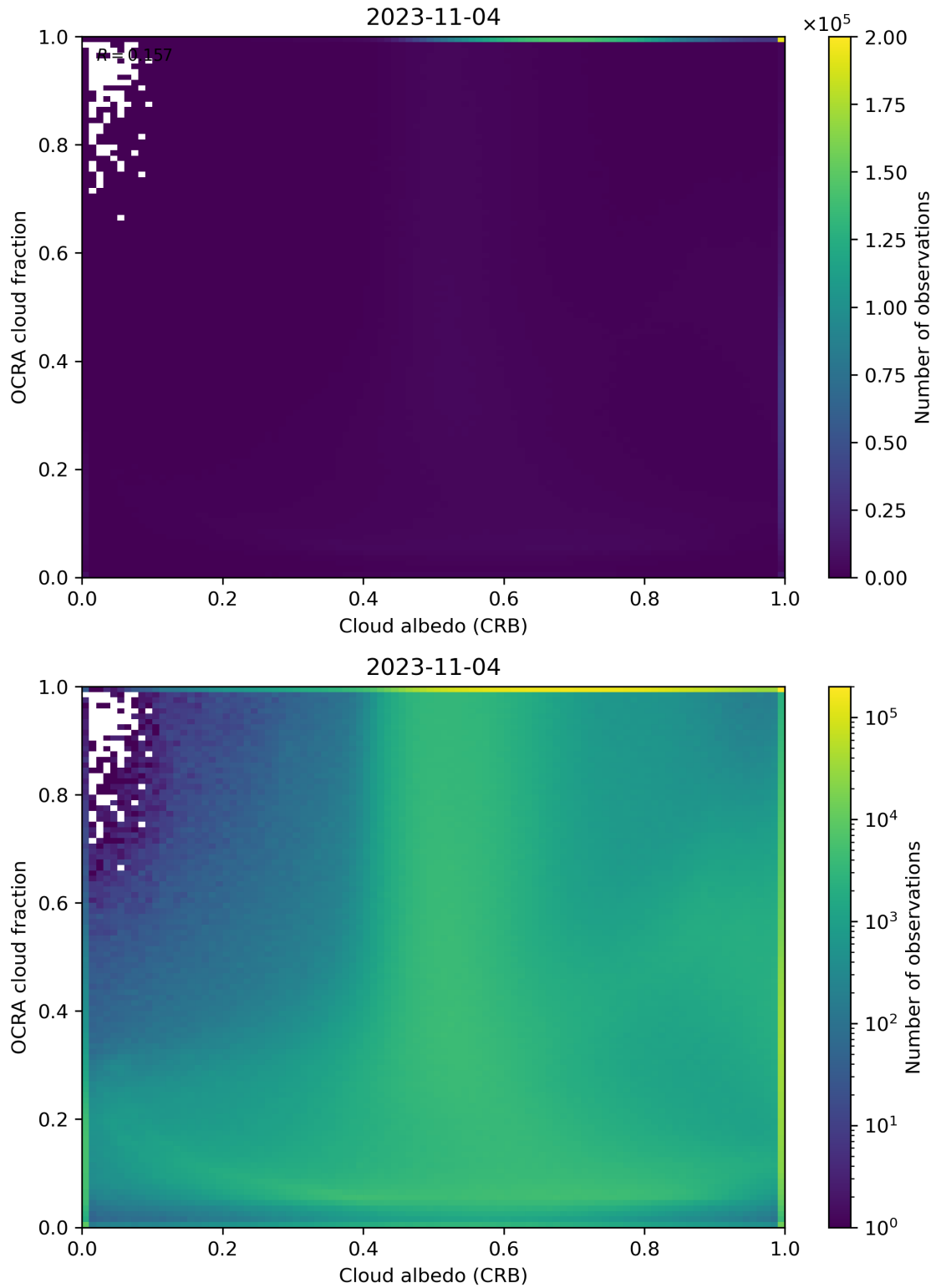
Figure 70: Scatter density plot of “Cloud albedo (CRB)” against “OCRA cloud fraction” for 2023-11-03 to 2023-11-05.
