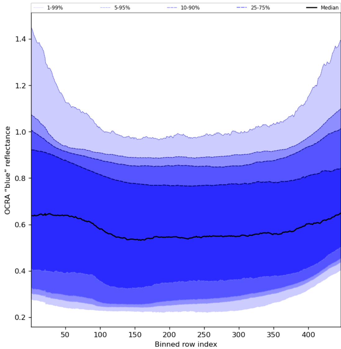
Figure 67: Along track statistics of “OCRA “blue” reflectance” for 2023-11-03 to 2023-11-05
