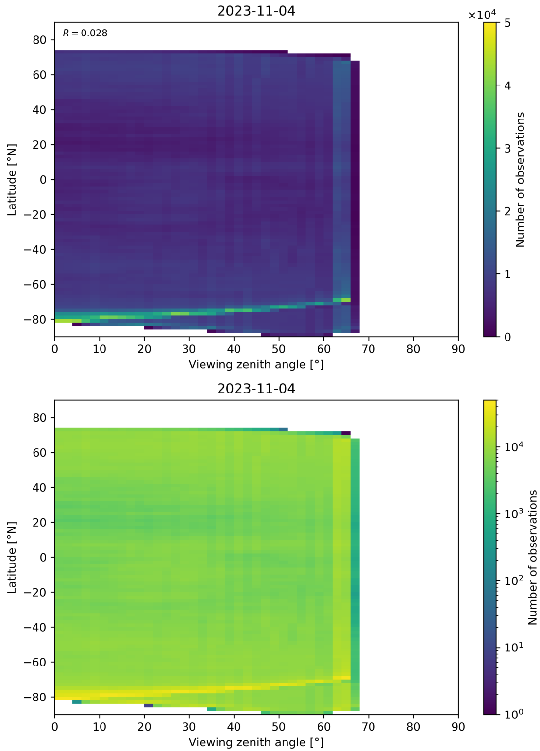
Figure 113: Scatter density plot of “Viewing zenith angle” against “Latitude” for 2023-11-03 to 2023-11-05.
