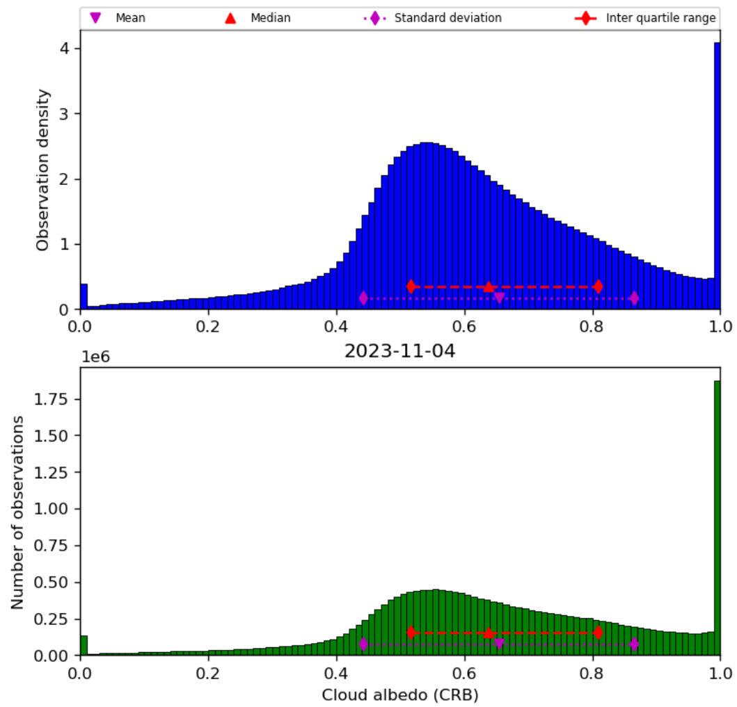
Figure 44: Histogram of “Cloud albedo (CRB)” for 2023-11-03 to 2023-11-05
