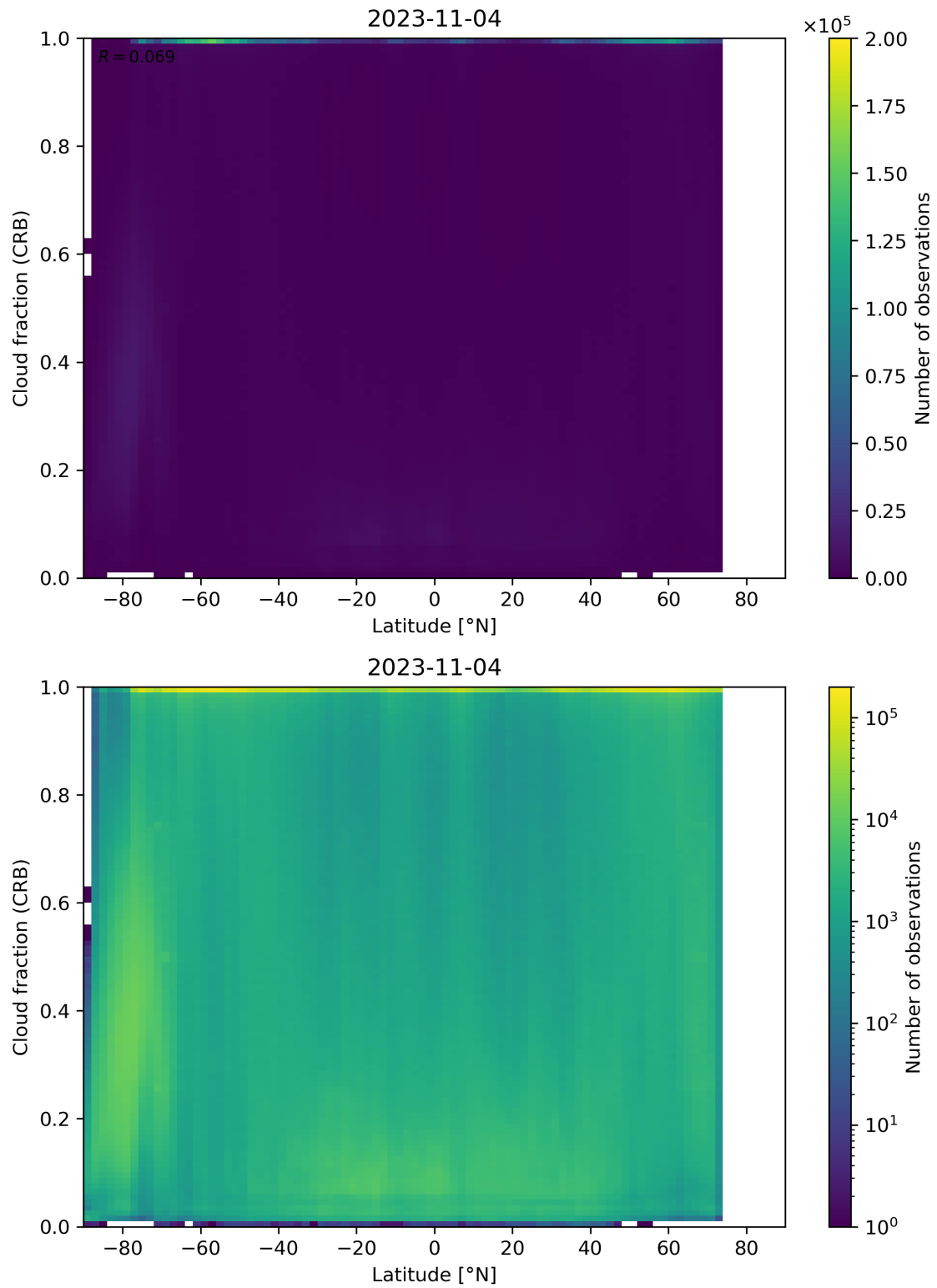
Figure 94: Scatter density plot of “Latitude” against “Cloud fraction (CRB)” for 2023-11-03 to 2023-11-05.
