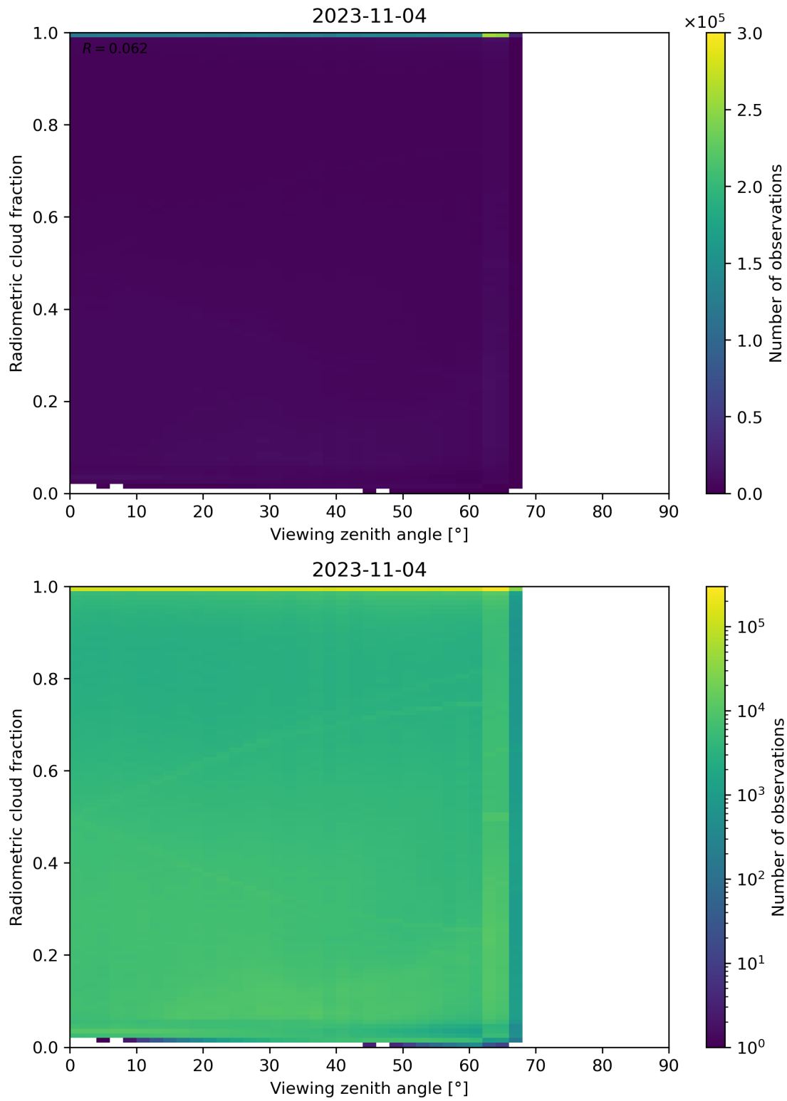
Figure 107: Scatter density plot of “Viewing zenith angle” against “Radiometric cloud fraction” for 2023-11-03 to 2023-11-05.
