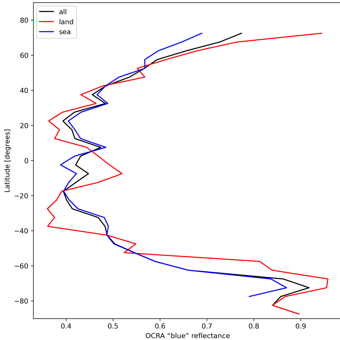
Figure 35: Zonal average of “OCRA “blue” reflectance” for 2023-11-03 to 2023-11-05.
