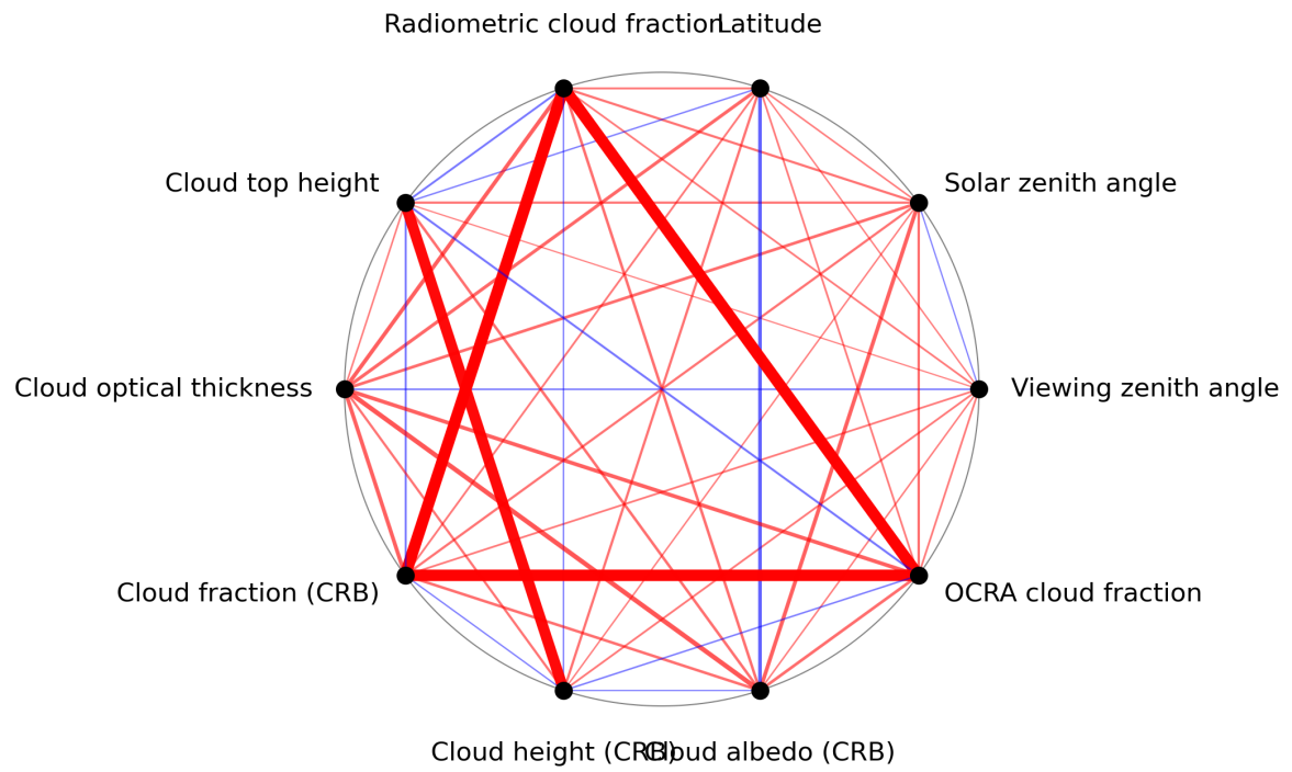
Figure 1: Map of correlation graph for 2023-11-03 to 2023-11-05.
