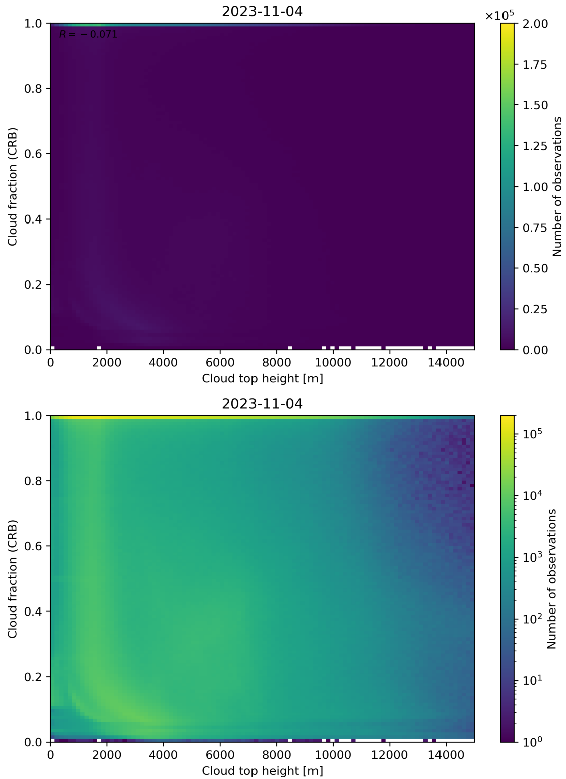
Figure 88: Scatter density plot of “Cloud top height” against “Cloud fraction (CRB)” for 2023-11-03 to 2023-11-05.
