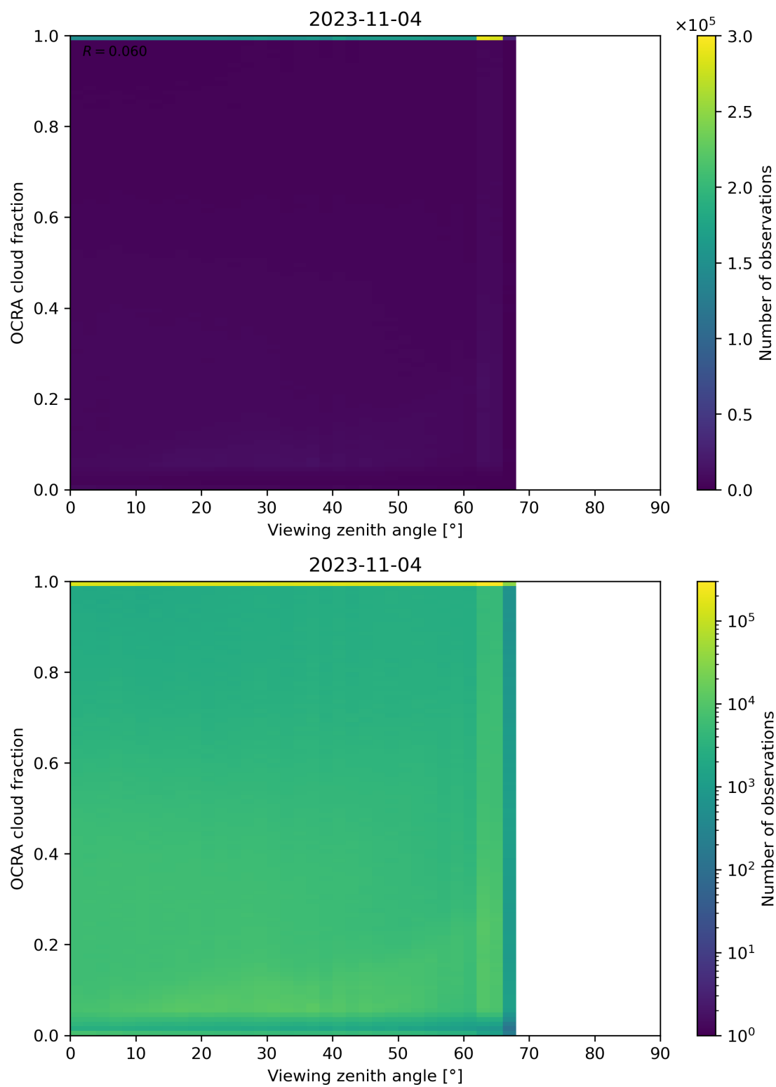
Figure 108: Scatter density plot of “Viewing zenith angle” against “OCRA cloud fraction” for 2023-11-03 to 2023-11-05.
