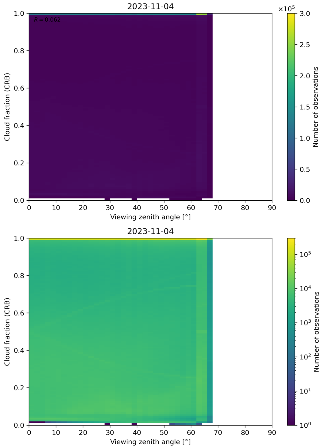
Figure 109: Scatter density plot of “Viewing zenith angle” against “Cloud fraction (CRB)” for 2023-11-03 to 2023-11-05.
