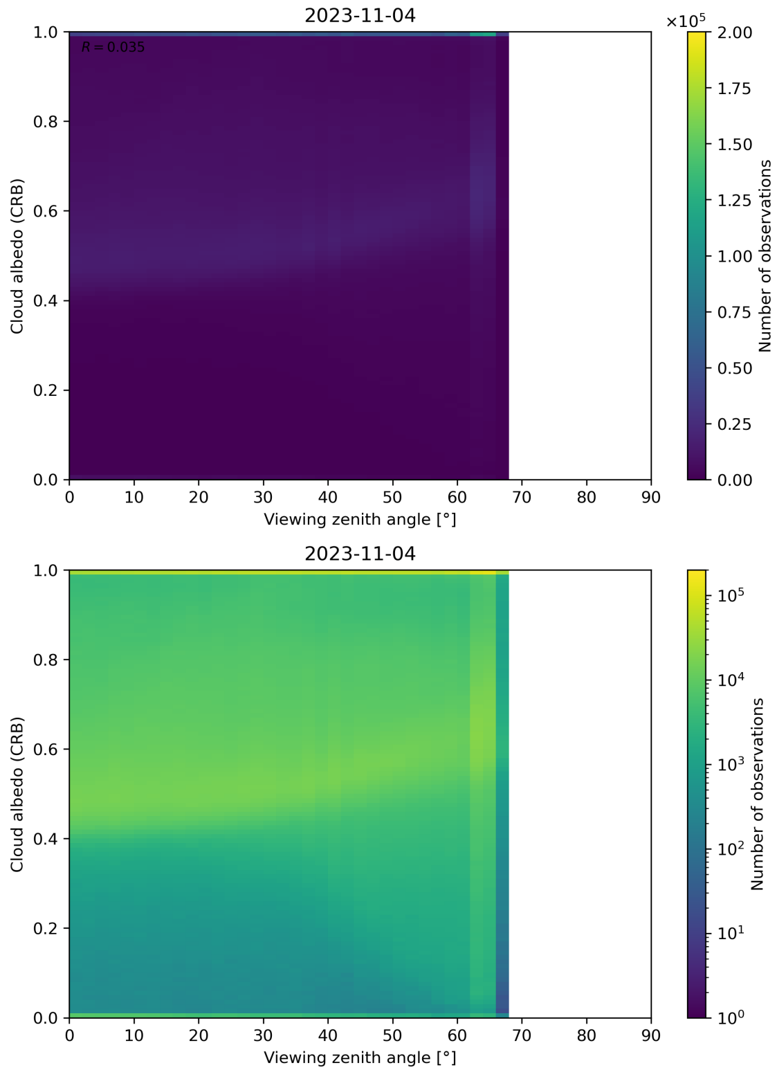
Figure 106: Scatter density plot of “Viewing zenith angle” against “Cloud albedo (CRB)” for 2023-11-03 to 2023-11-05.
