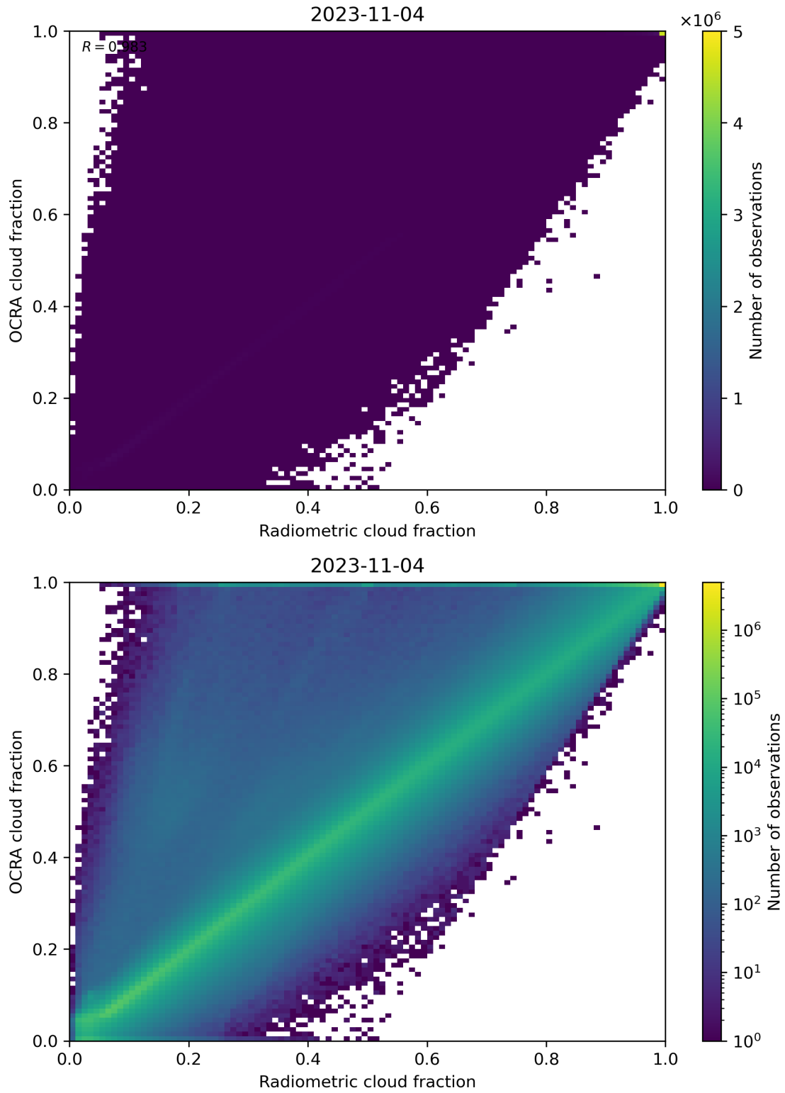
Figure 72: Scatter density plot of “Radiometric cloud fraction” against “OCRA cloud fraction” for 2023-11-03 to 2023-11-05.
