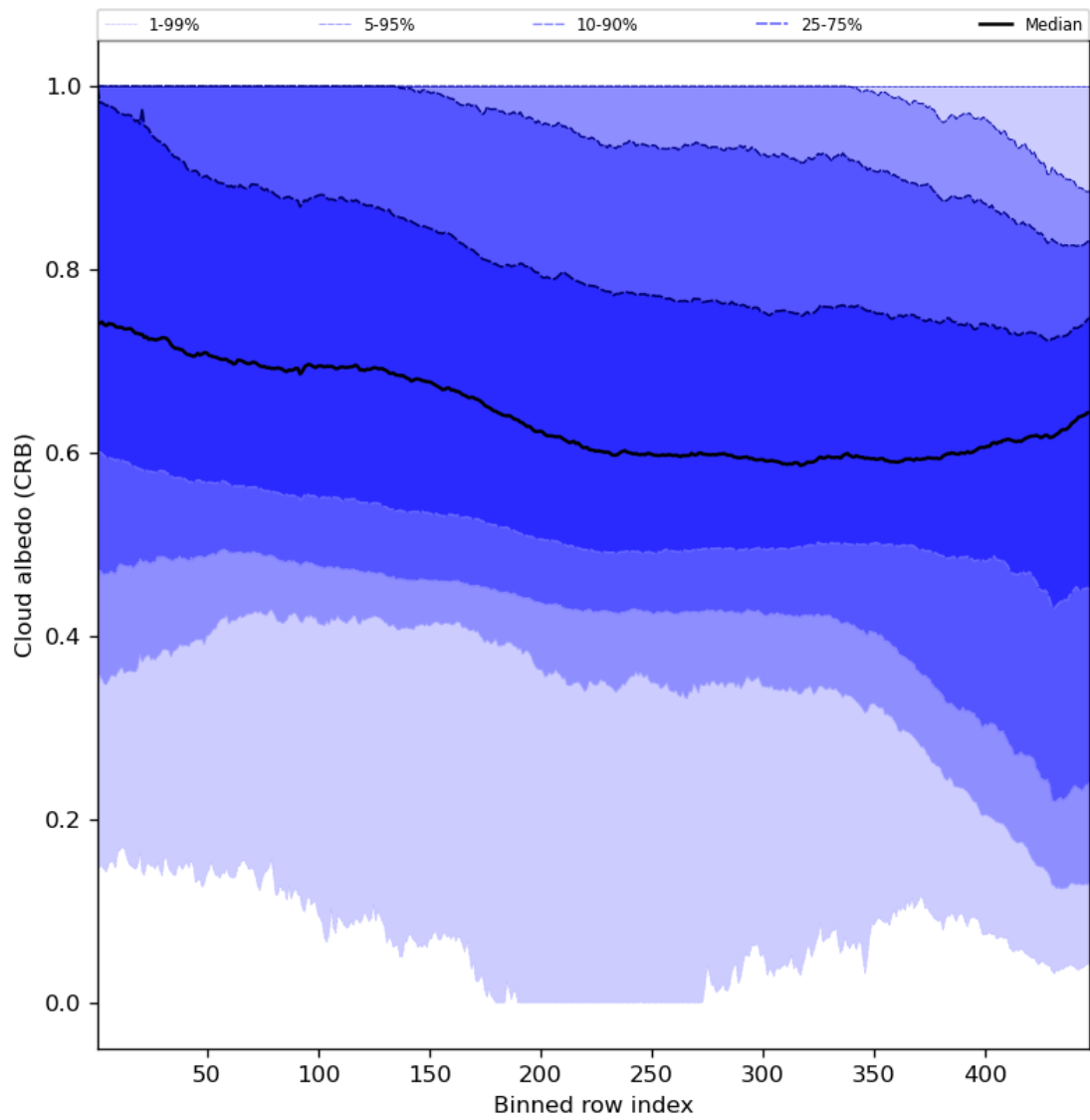
Figure 60: Along track statistics of “Cloud albedo (CRB)” for 2023-11-03 to 2023-11-05
