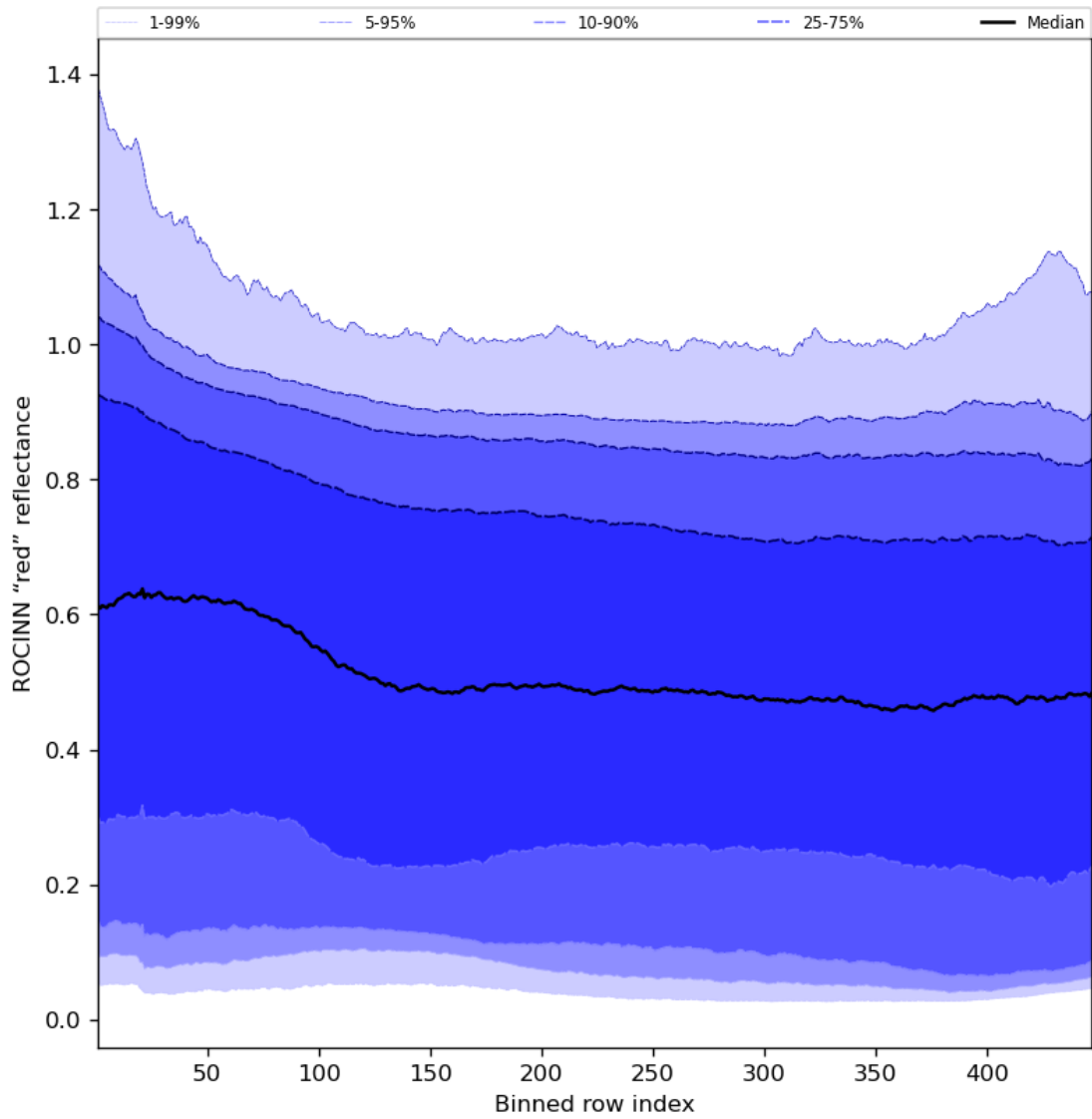
Figure 69: Along track statistics of "ROCINN "red" reflectance" for 2023-11-03 to 2023-11-05
