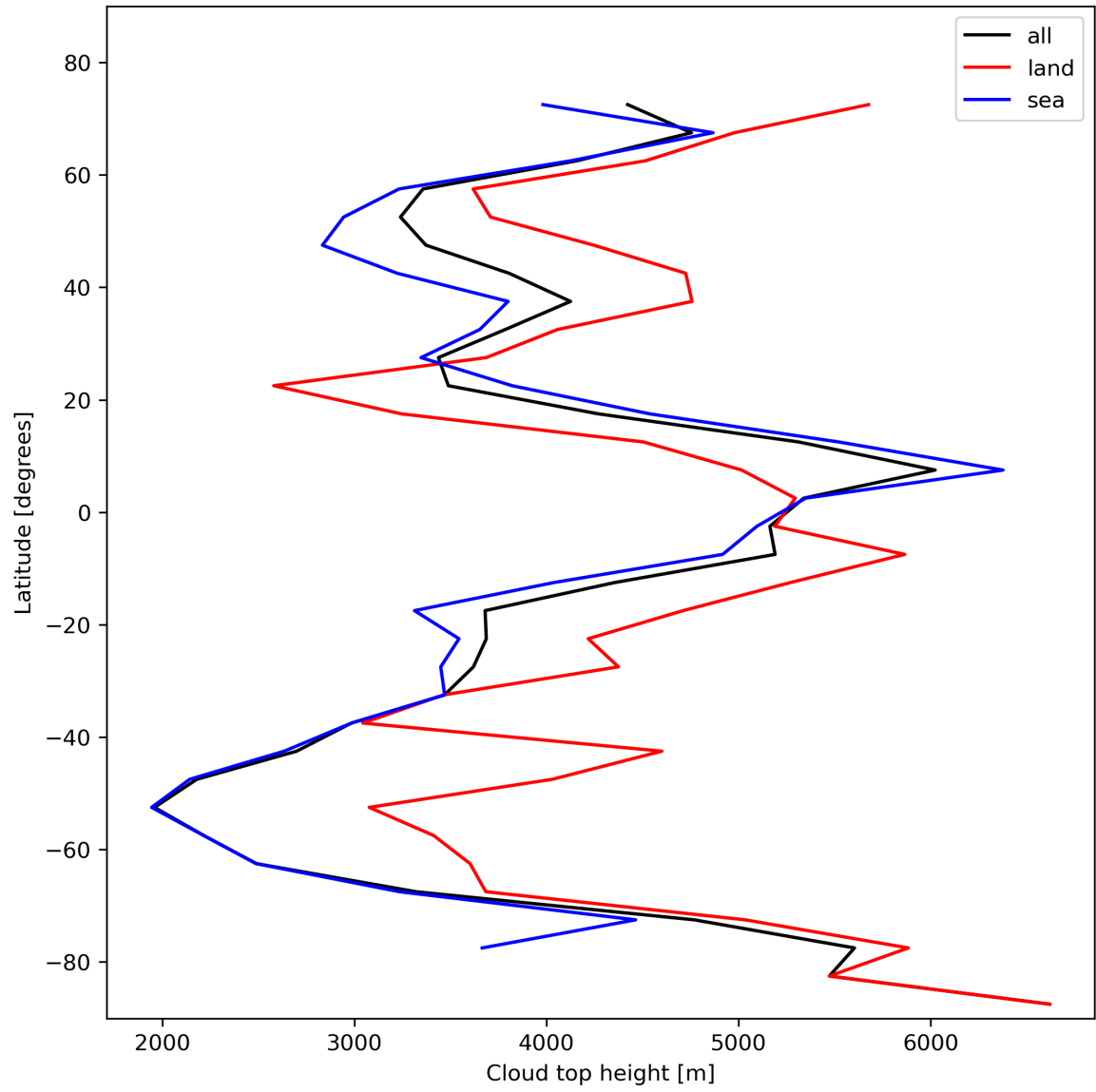
Figure 24: Zonal average of “Cloud top height” for 2023-11-03 to 2023-11-05.
