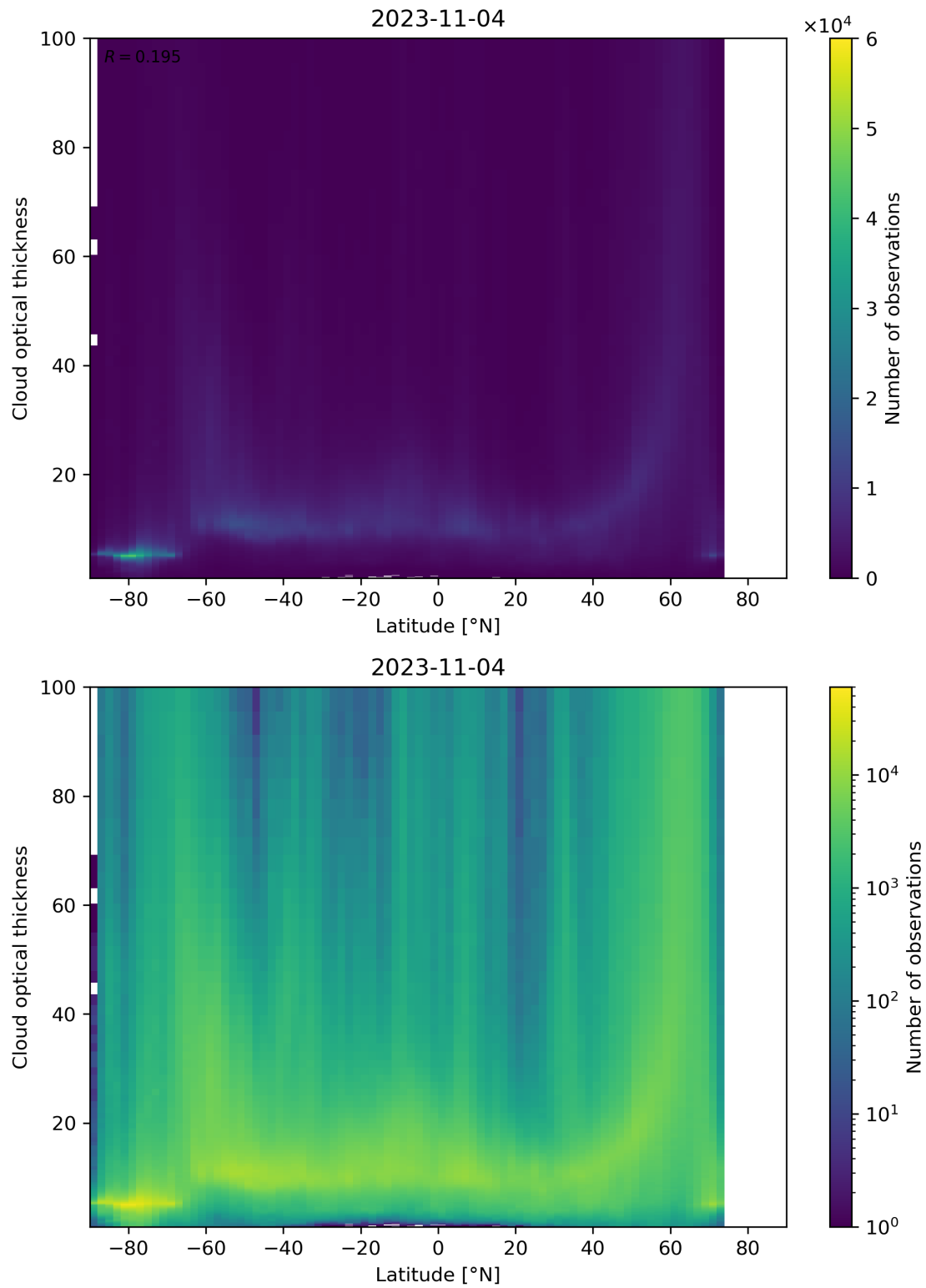
Figure 96: Scatter density plot of “Latitude” against “Cloud optical thickness” for 2023-11-03 to 2023-11-05.
