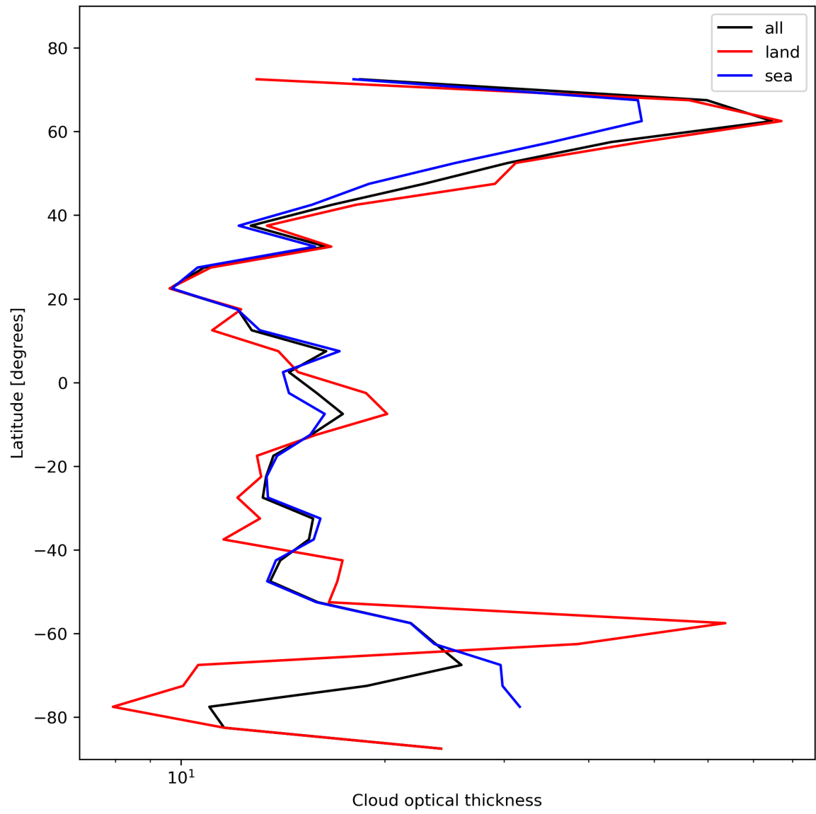
Figure 25: Zonal average of “Cloud optical thickness” for 2023-11-03 to 2023-11-05.
