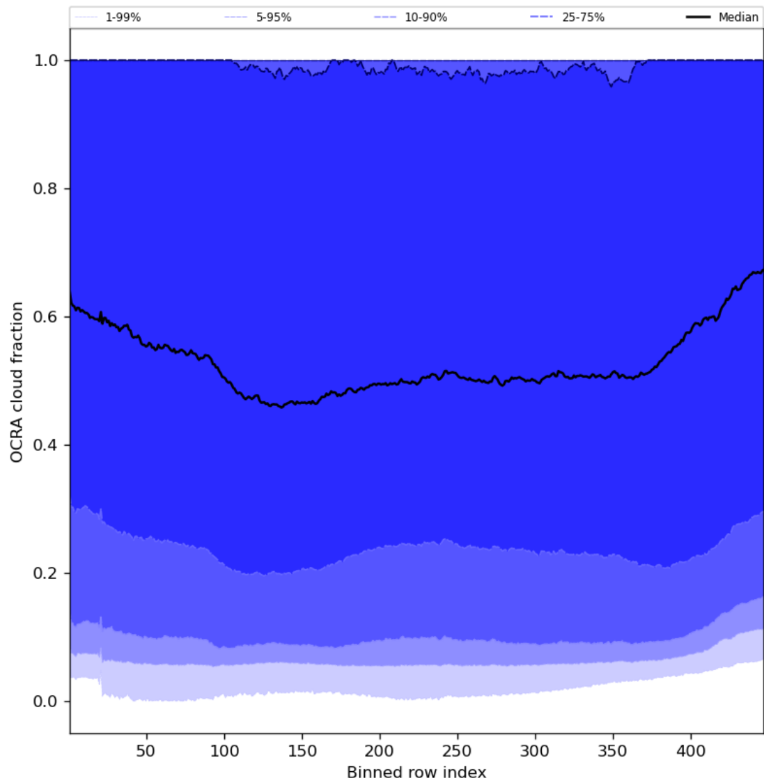
Figure 66: Along track statistics of “OCRA cloud fraction” for 2023-11-03 to 2023-11-05
