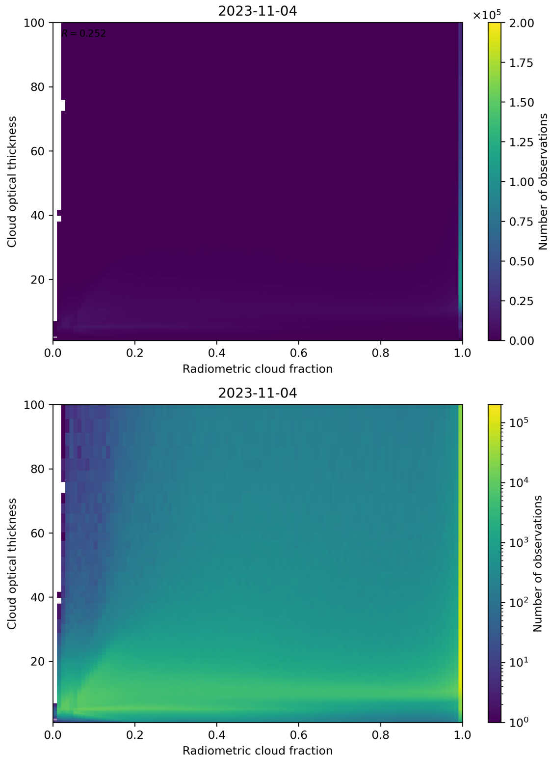
Figure 75: Scatter density plot of “Radiometric cloud fraction” against “Cloud optical thickness” for 2023-11-03 to 2023-11-05.
