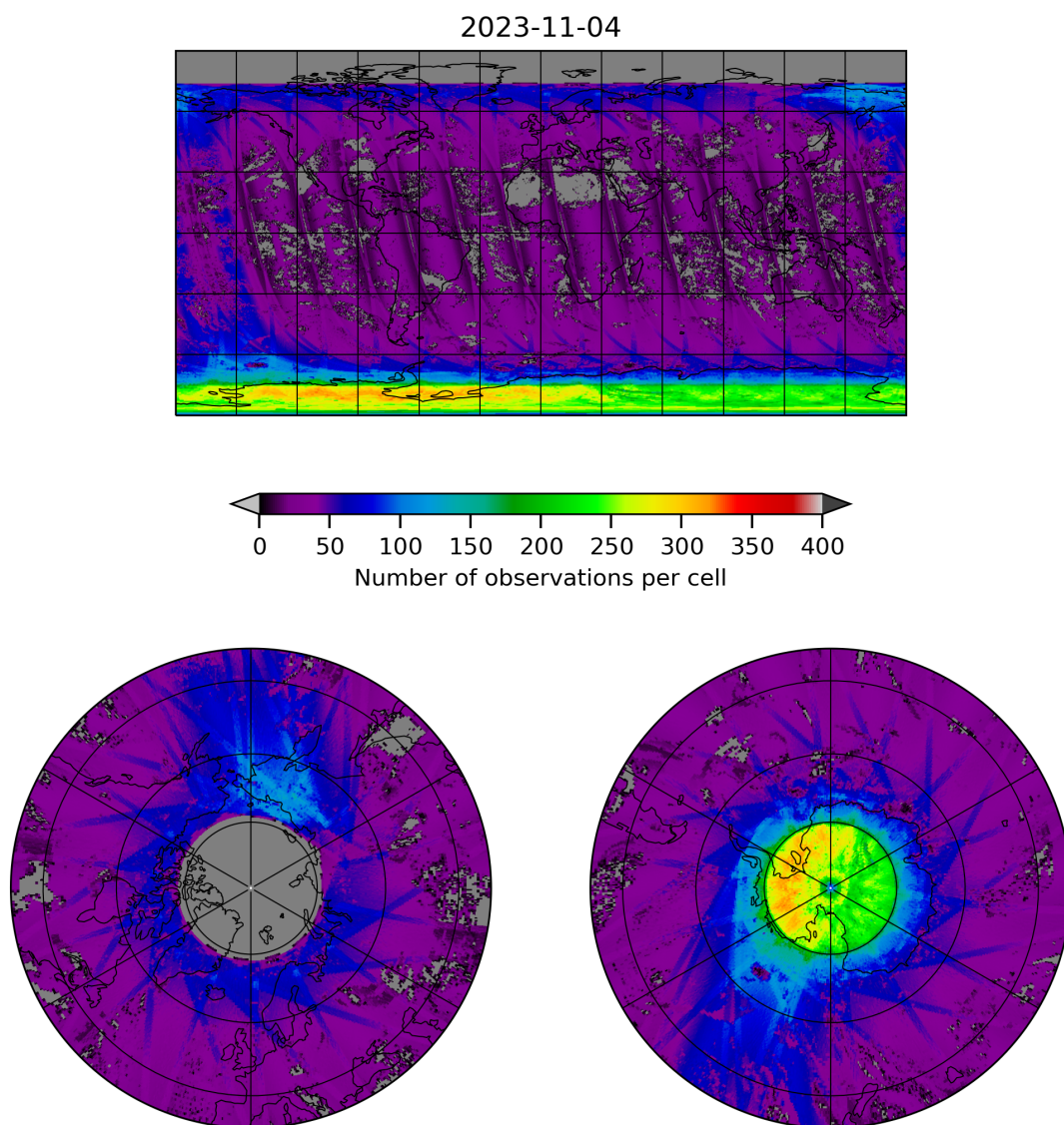
Figure 21: Map of the number of observations for 2023-11-03 to 2023-11-05
