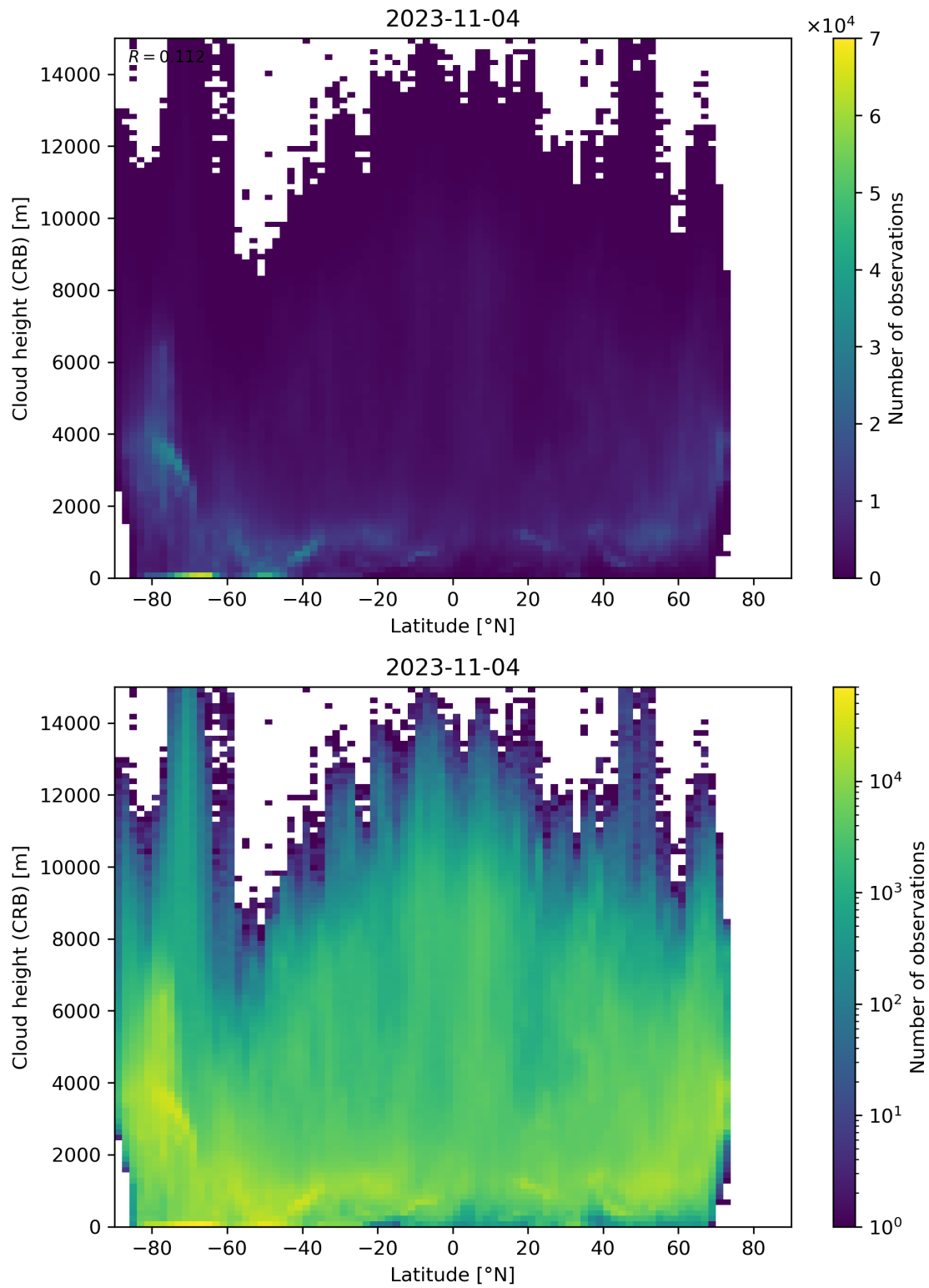
Figure 95: Scatter density plot of “Latitude” against “Cloud height (CRB)” for 2023-11-03 to 2023-11-05.
