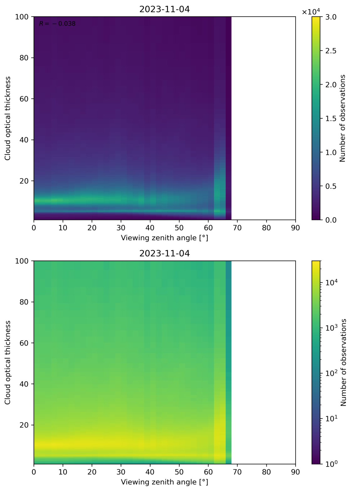
Figure 111: Scatter density plot of “Viewing zenith angle” against “Cloud optical thickness” for 2023-11-03 to 2023-11-05.
