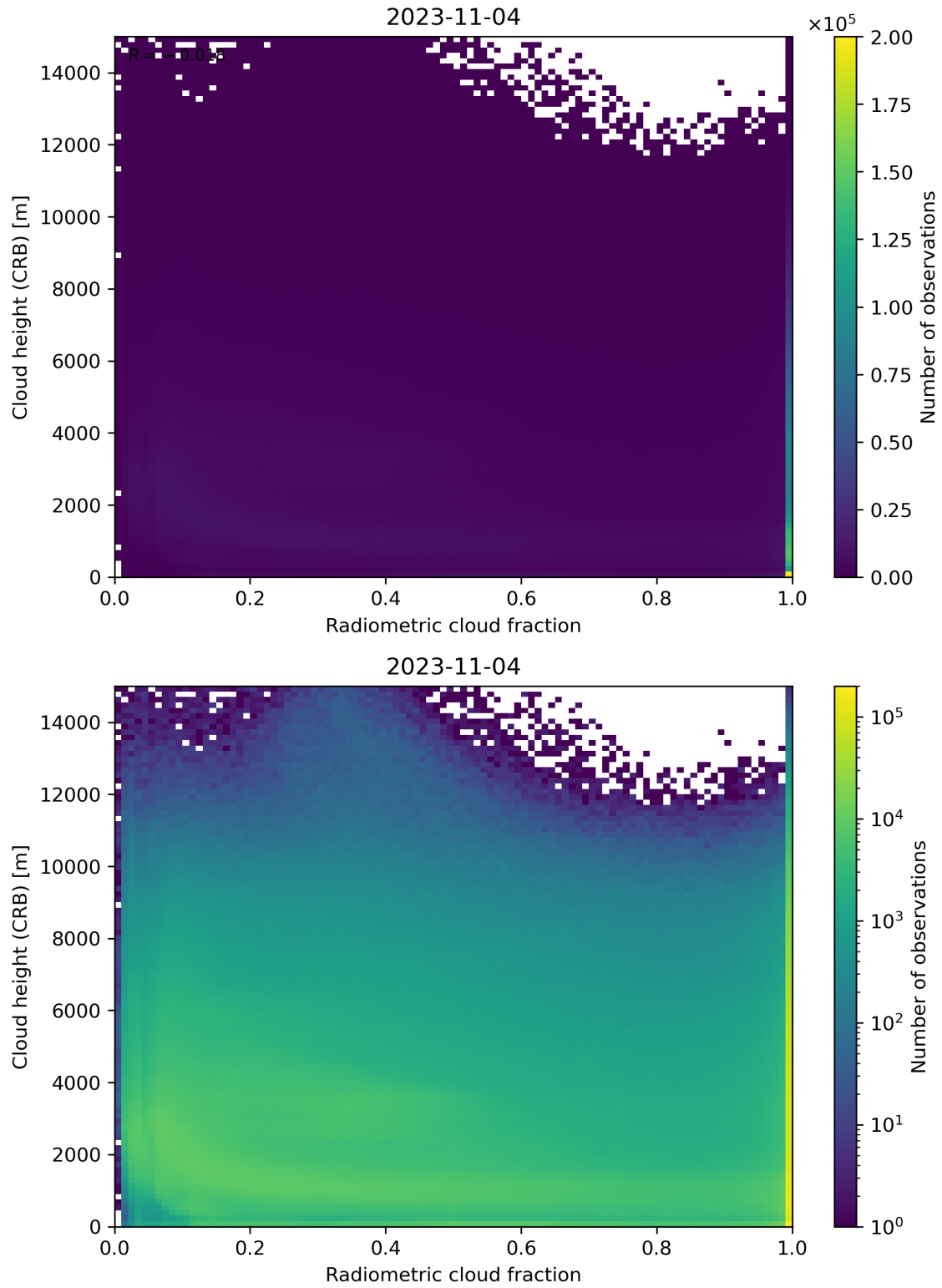
Figure 74: Scatter density plot of “Radiometric cloud fraction” against “Cloud height (CRB)” for 2023-11-03 to 2023-11-05.
