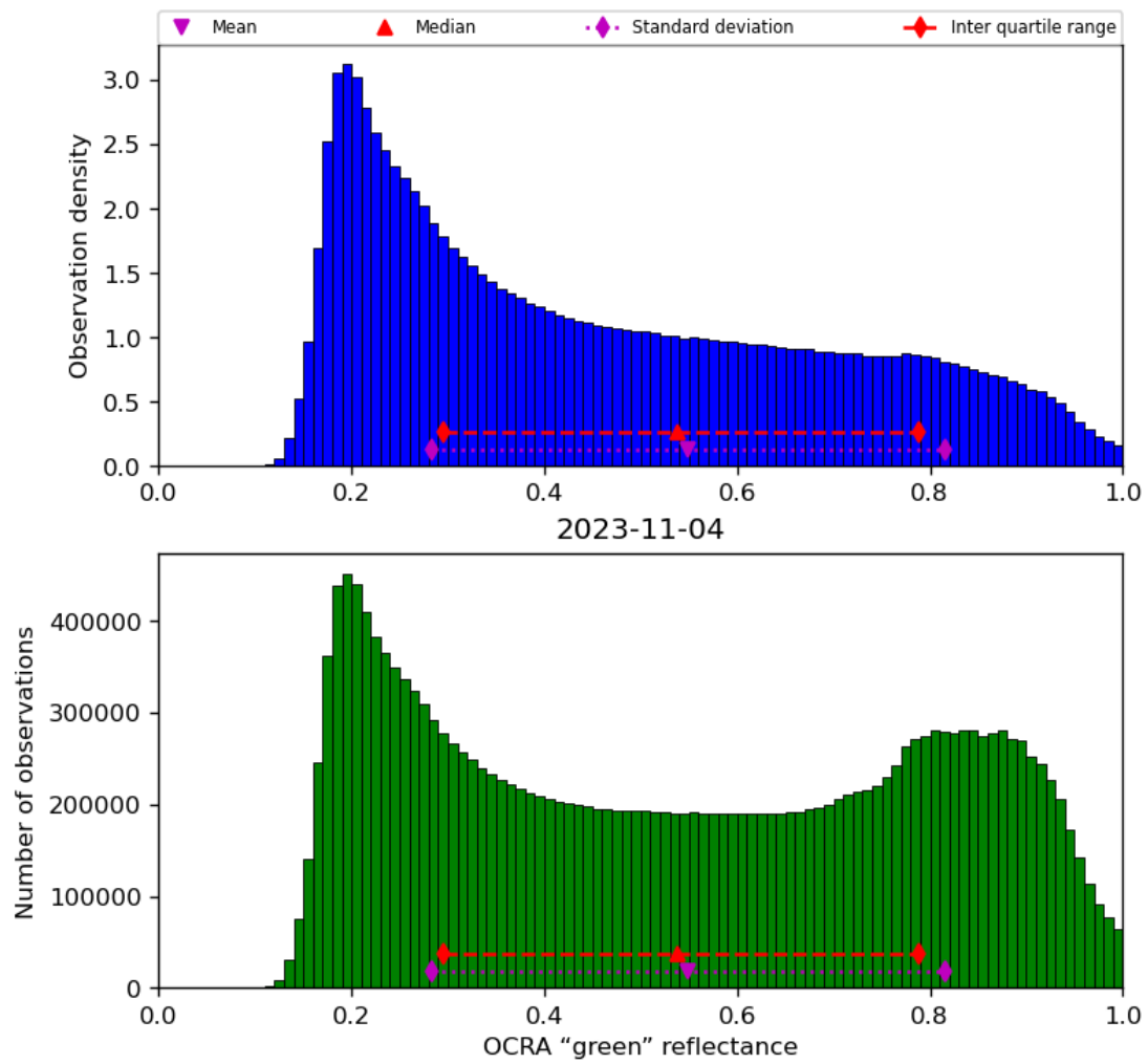
Figure 52: Histogram of “OCRA “green” reflectance” for 2023-11-03 to 2023-11-05
