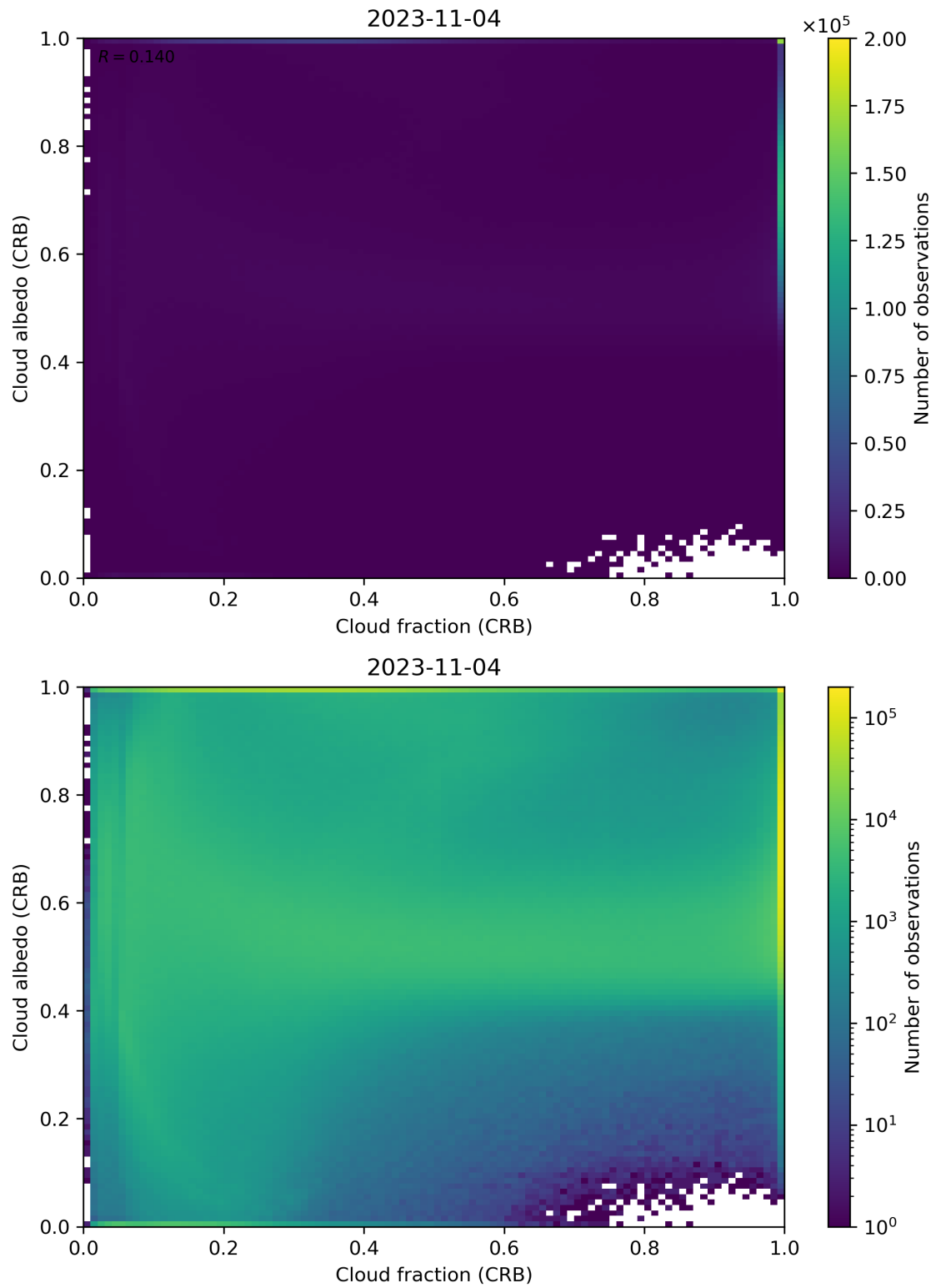
Figure 77: Scatter density plot of “Cloud fraction (CRB)” against “Cloud albedo (CRB)” for 2023-11-03 to 2023-11-05.
