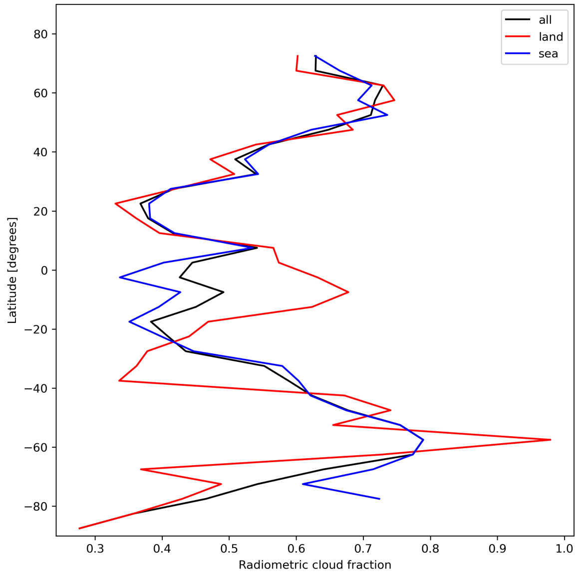
Figure 23: Zonal average of “Radiometric cloud fraction” for 2023-11-03 to 2023-11-05.
