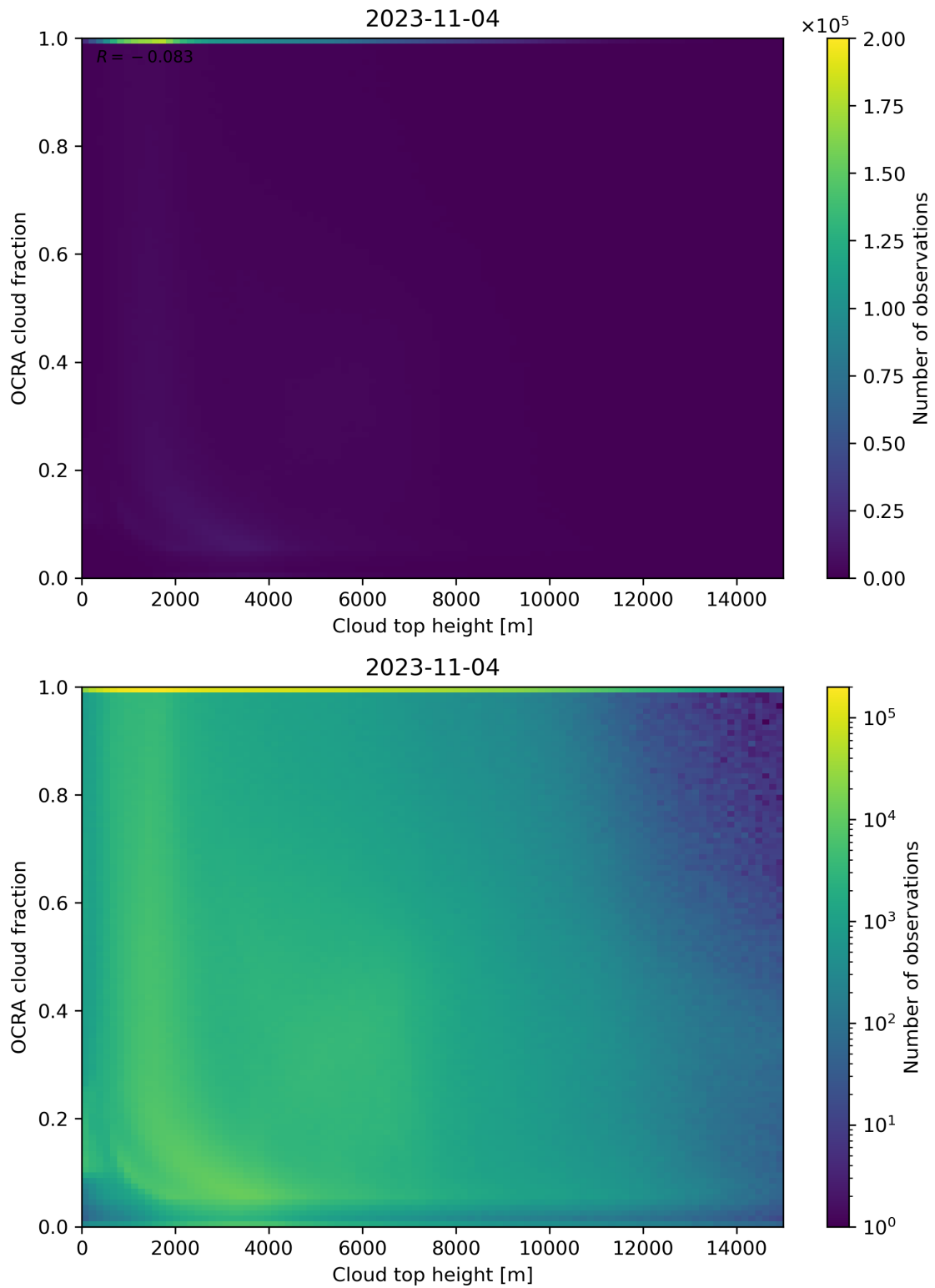
Figure 87: Scatter density plot of “Cloud top height” against “OCRA cloud fraction” for 2023-11-03 to 2023-11-05.
