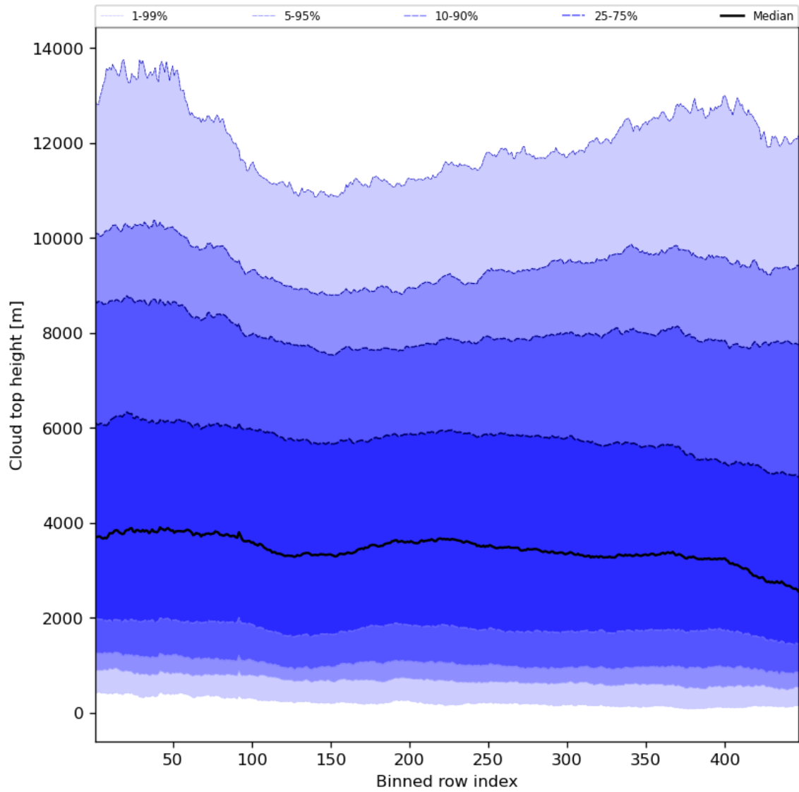
Figure 56: Along track statistics of “Cloud top height” for 2023-11-03 to 2023-11-05
