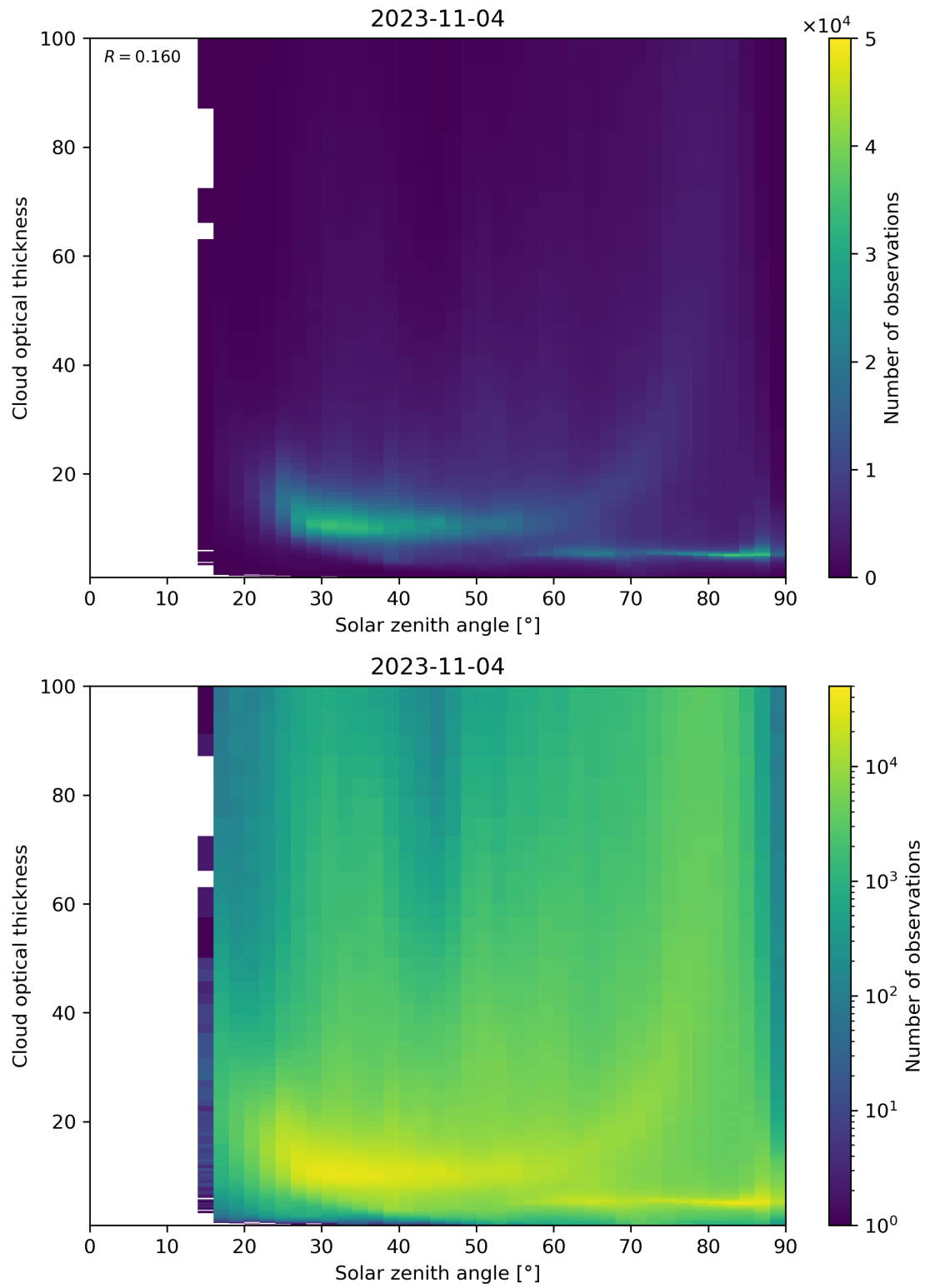
Figure 103: Scatter density plot of “Solar zenith angle” against “Cloud optical thickness” for 2023-11-03 to 2023-11-05.
