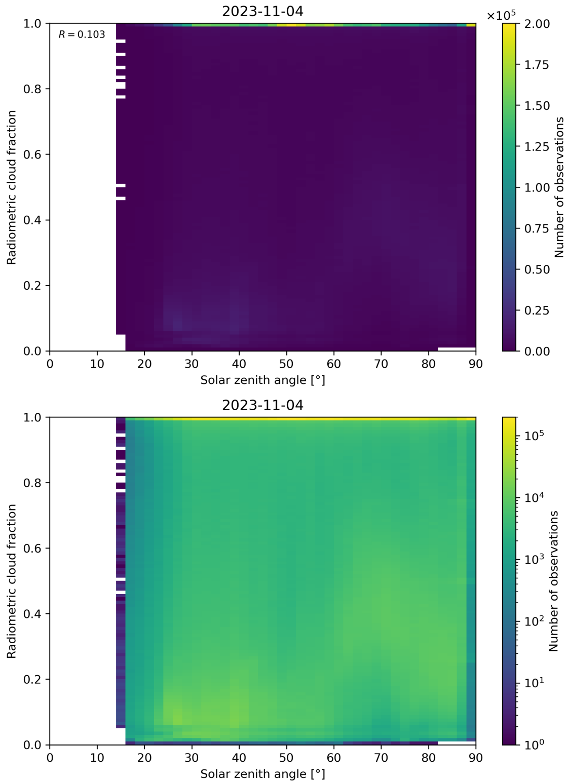
Figure 99: Scatter density plot of “Solar zenith angle” against “Radiometric cloud fraction” for 2023-11-03 to 2023-11-05.
