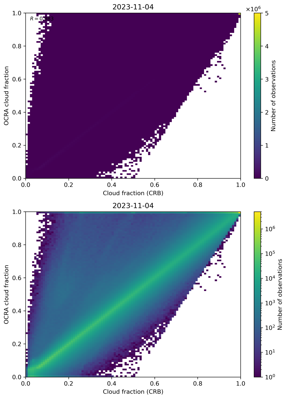
Figure 78: Scatter density plot of “Cloud fraction (CRB)” against “OCRA cloud fraction” for 2023-11-03 to 2023-11-05.
