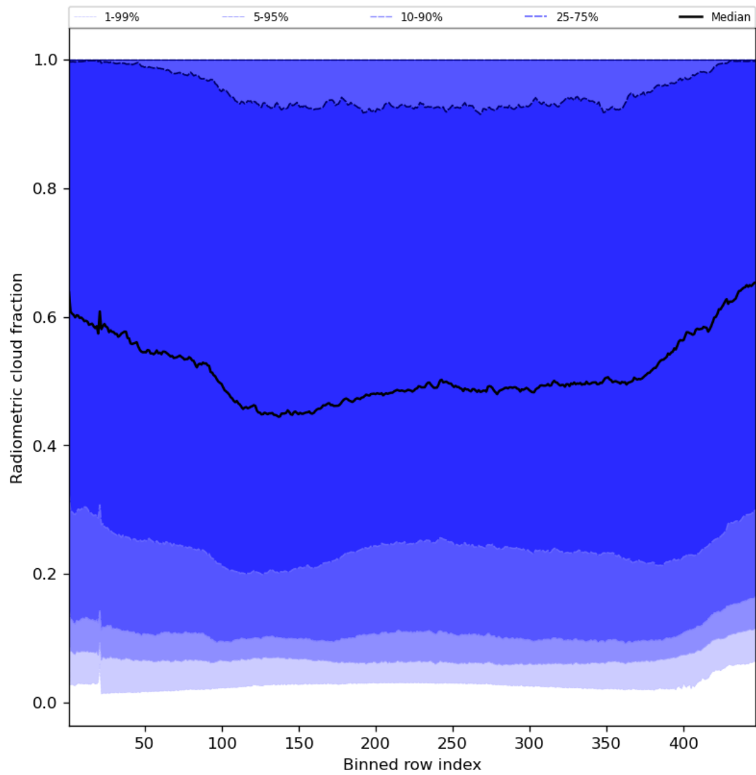
Figure 55: Along track statistics of “Radiometric cloud fraction” for 2023-11-03 to 2023-11-05
