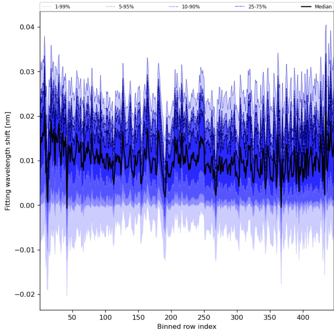
Figure 65: Along track statistics of “Fitting wavelength shift” for 2023-11-03 to 2023-11-05
