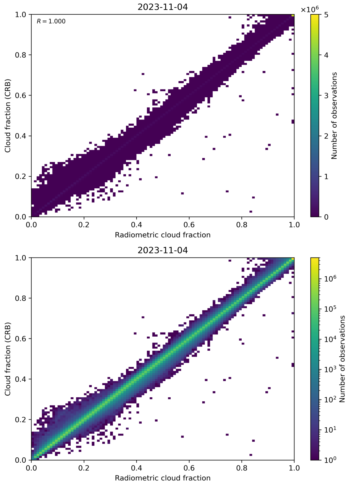
Figure 73: Scatter density plot of “Radiometric cloud fraction” against “Cloud fraction (CRB)” for 2023-11-03 to 2023-11-05.
