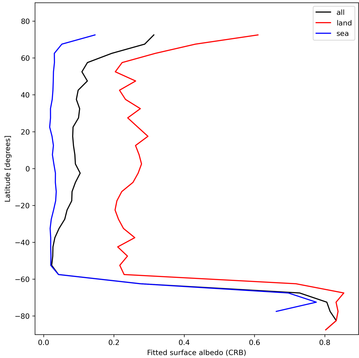
Figure 30: Zonal average of “Fitted surface albedo (CRB)” for 2023-11-03 to 2023-11-05.
