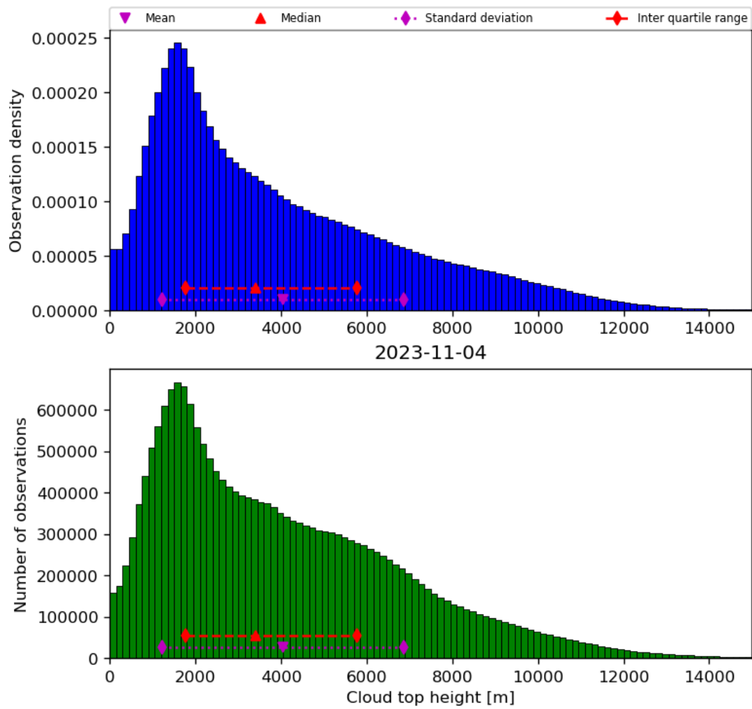
Figure 40: Histogram of “Cloud top height” for 2023-11-03 to 2023-11-05
