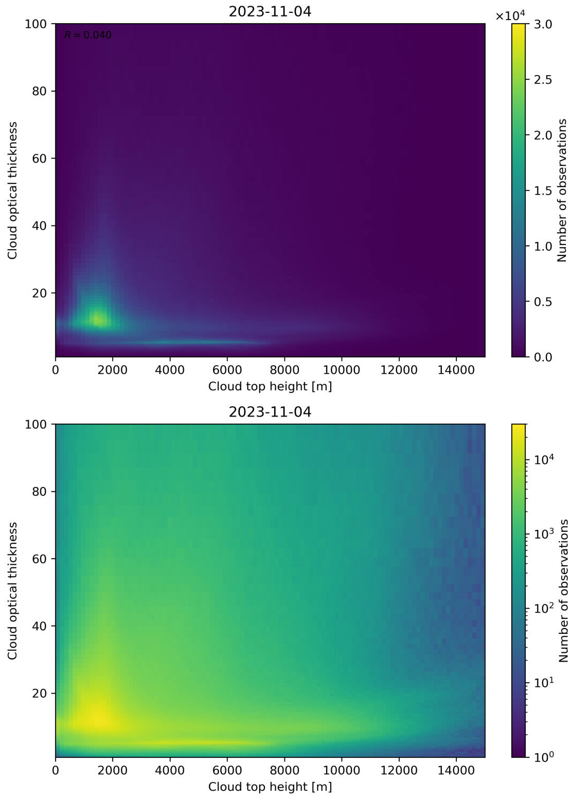
Figure 90: Scatter density plot of “Cloud top height” against “Cloud optical thickness” for 2023-11-03 to 2023-11-05.
