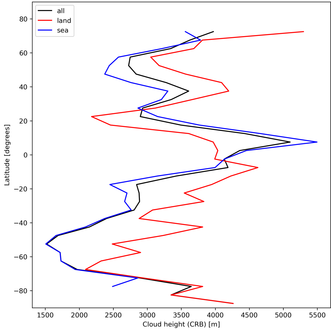
Figure 27: Zonal average of “Cloud height (CRB)” for 2023-11-03 to 2023-11-05.
