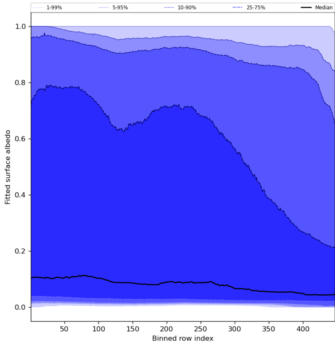
Figure 61: Along track statistics of “Fitted surface albedo” for 2023-11-03 to 2023-11-05
