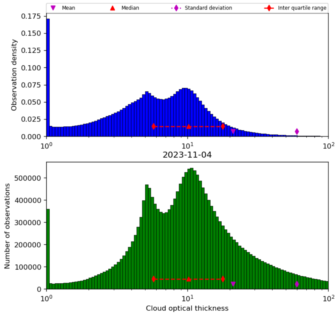
Figure 41: Histogram of “Cloud optical thickness” for 2023-11-03 to 2023-11-05
