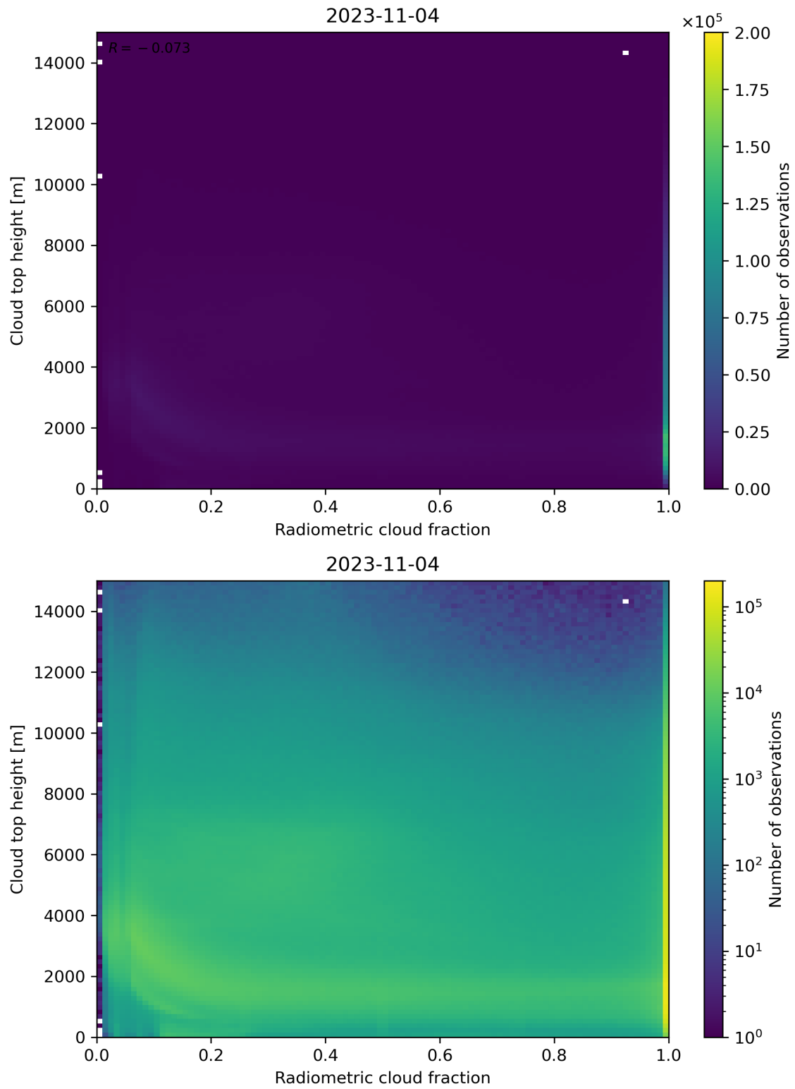
Figure 76: Scatter density plot of “Radiometric cloud fraction” against “Cloud top height” for 2023-11-03 to 2023-11-05.
