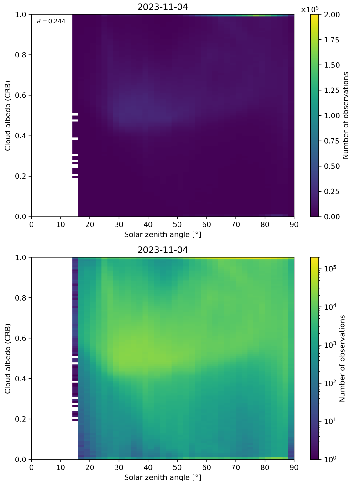
Figure 98: Scatter density plot of “Solar zenith angle” against “Cloud albedo (CRB)” for 2023-11-03 to 2023-11-05.
