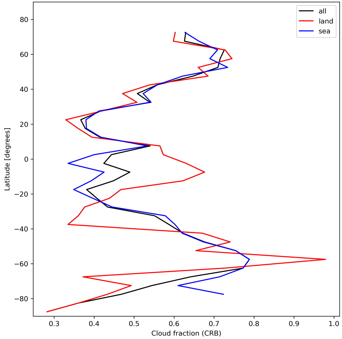
Figure 26: Zonal average of “Cloud fraction (CRB)” for 2023-11-03 to 2023-11-05.
