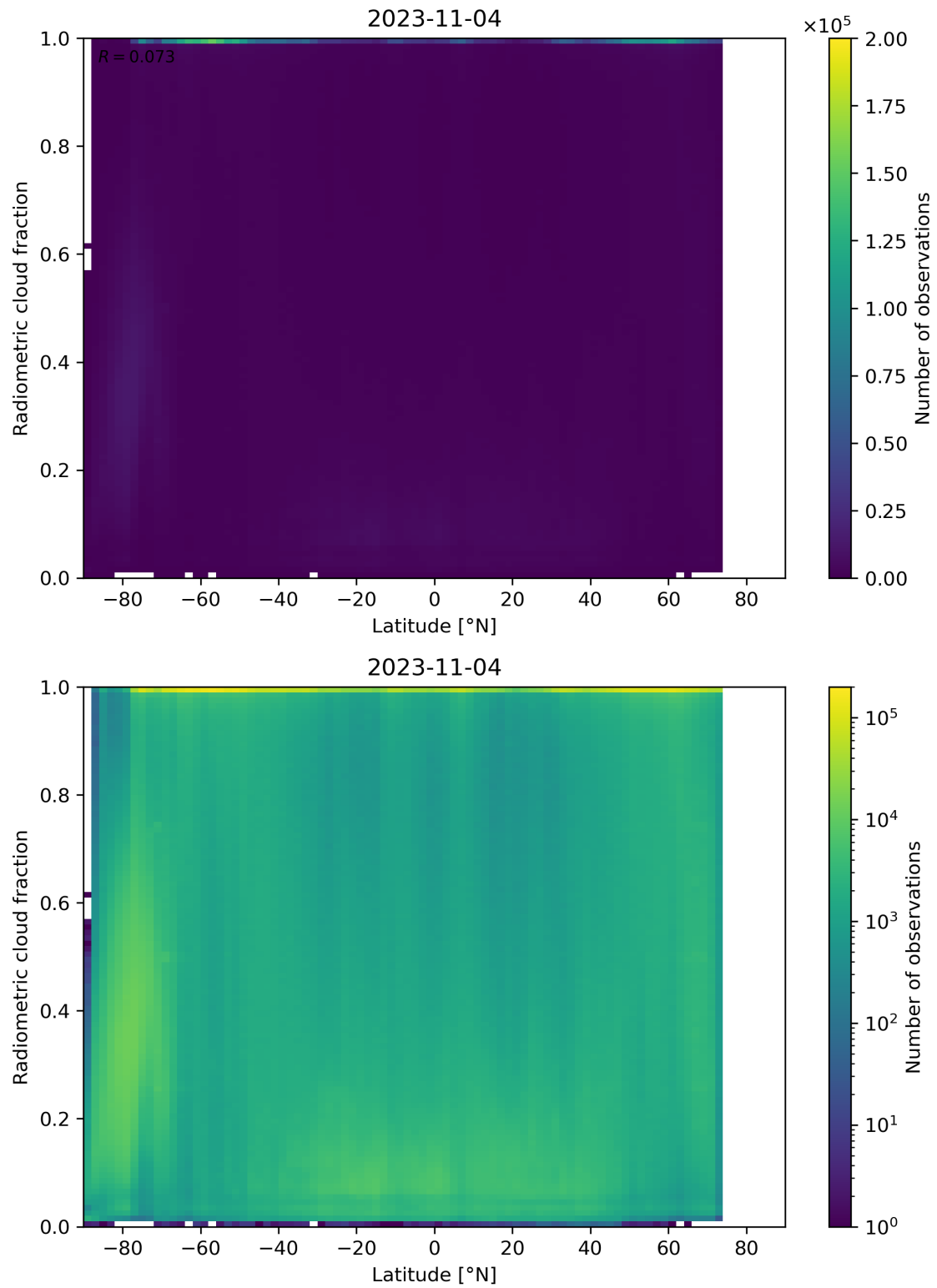
Figure 92: Scatter density plot of “Latitude” against “Radiometric cloud fraction” for 2023-11-03 to 2023-11-05.
