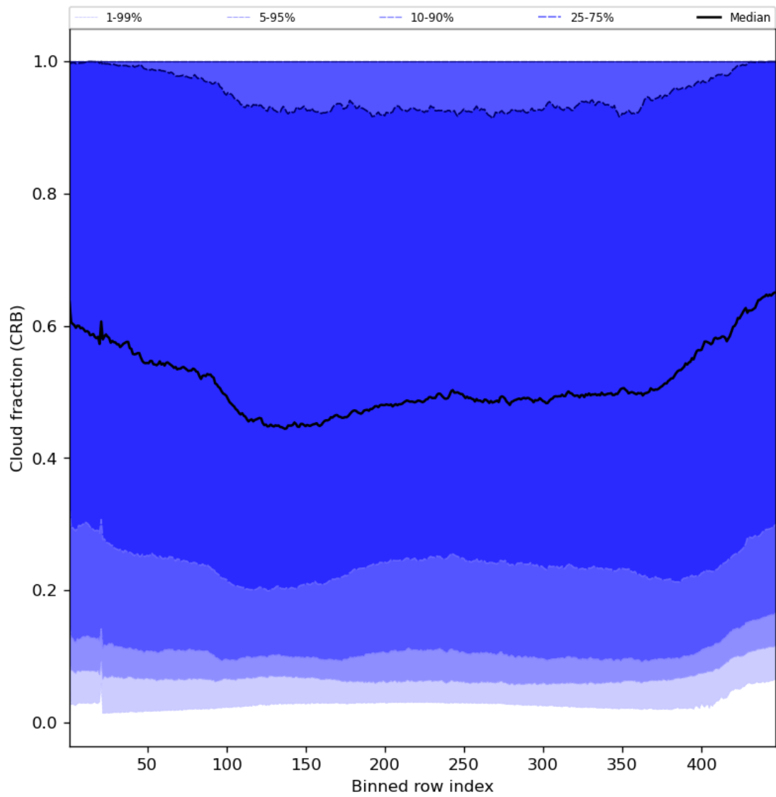
Figure 58: Along track statistics of “Cloud fraction (CRB)” for 2023-11-03 to 2023-11-05
