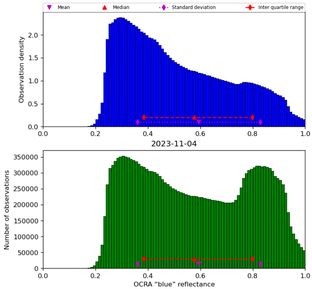
Figure 51: Histogram of “OCRA “blue” reflectance” for 2023-11-03 to 2023-11-05
