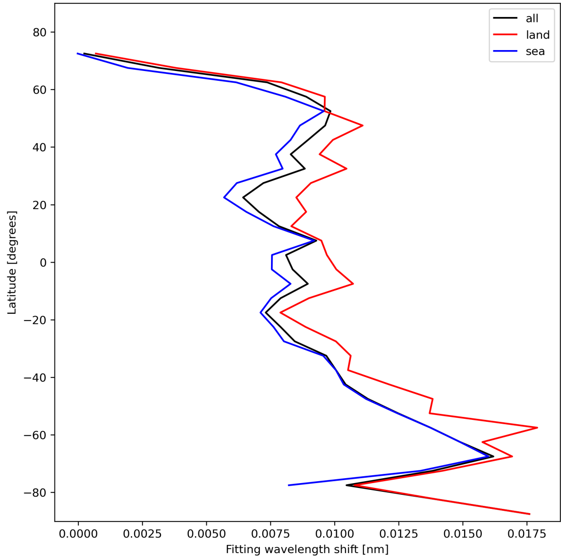
Figure 33: Zonal average of “Fitting wavelength shift” for 2023-11-03 to 2023-11-05.
