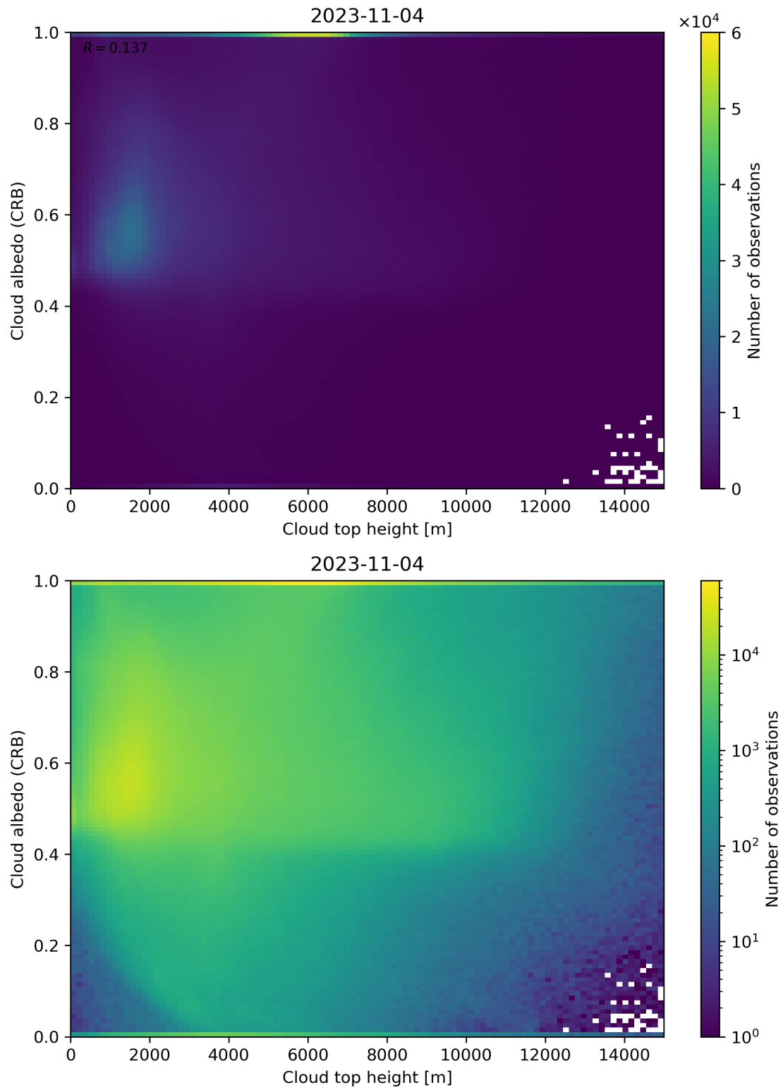
Figure 86: Scatter density plot of “Cloud top height” against “Cloud albedo (CRB)” for 2023-11-03 to 2023-11-05.
