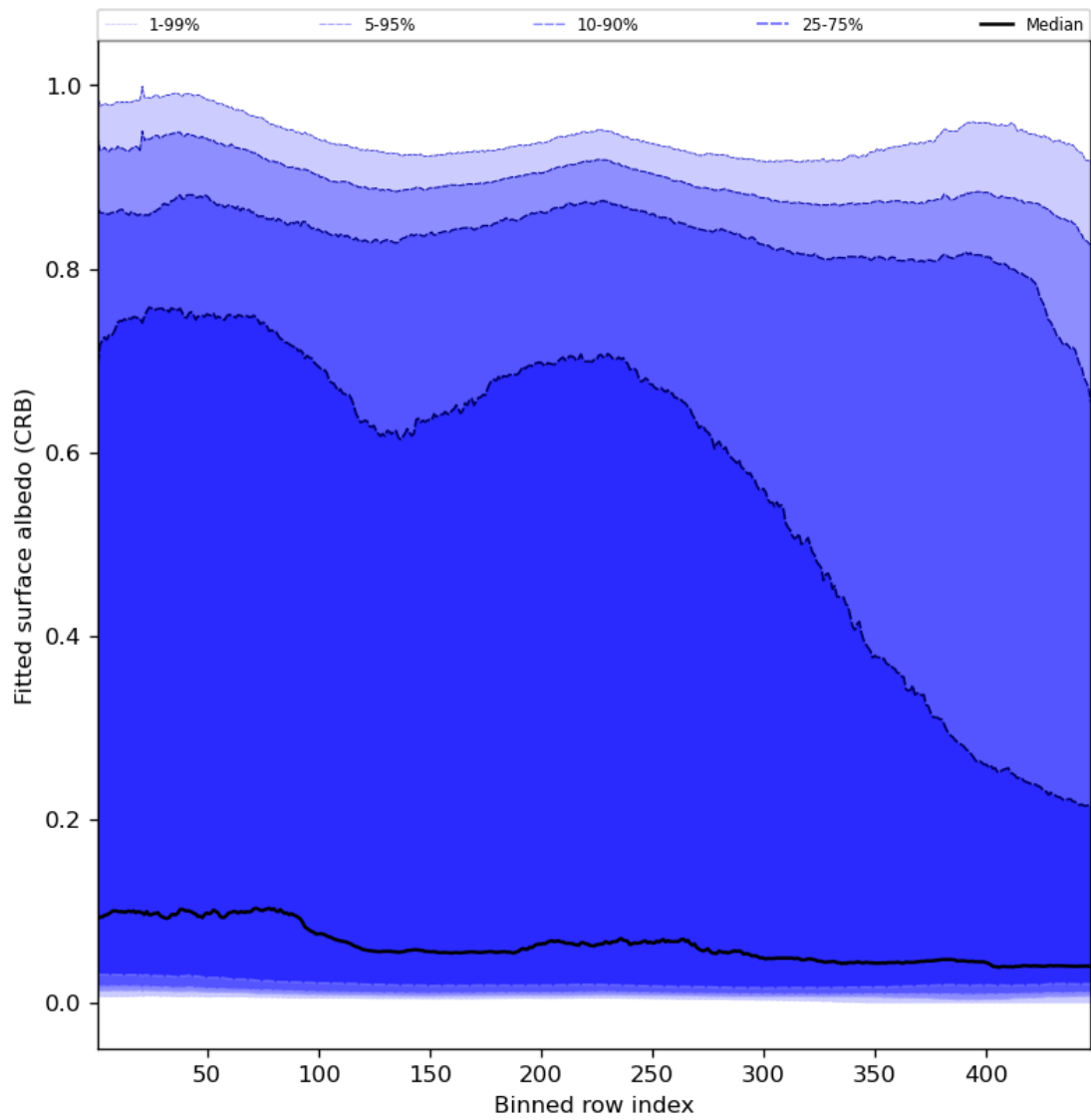
Figure 62: Along track statistics of “Fitted surface albedo (CRB)” for 2023-11-03 to 2023-11-05
