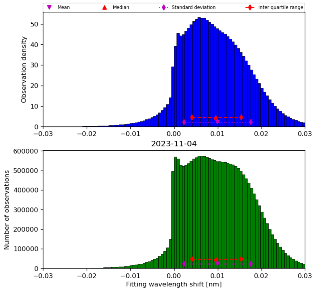
Figure 49: Histogram of “Fitting wavelength shift” for 2023-11-03 to 2023-11-05
