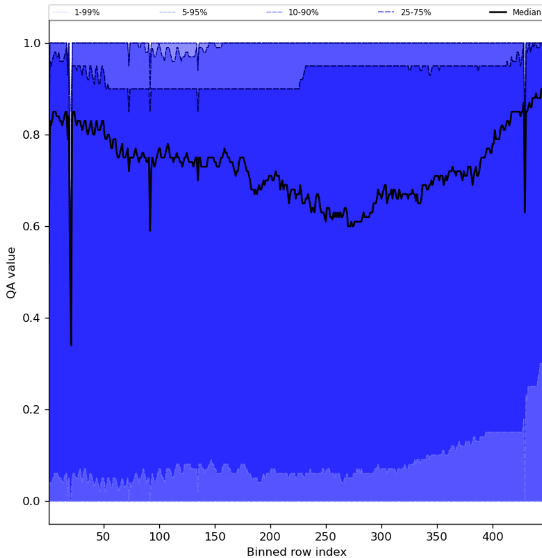
Figure 54: Along track statistics of “QA value” for 2023-11-03 to 2023-11-05
