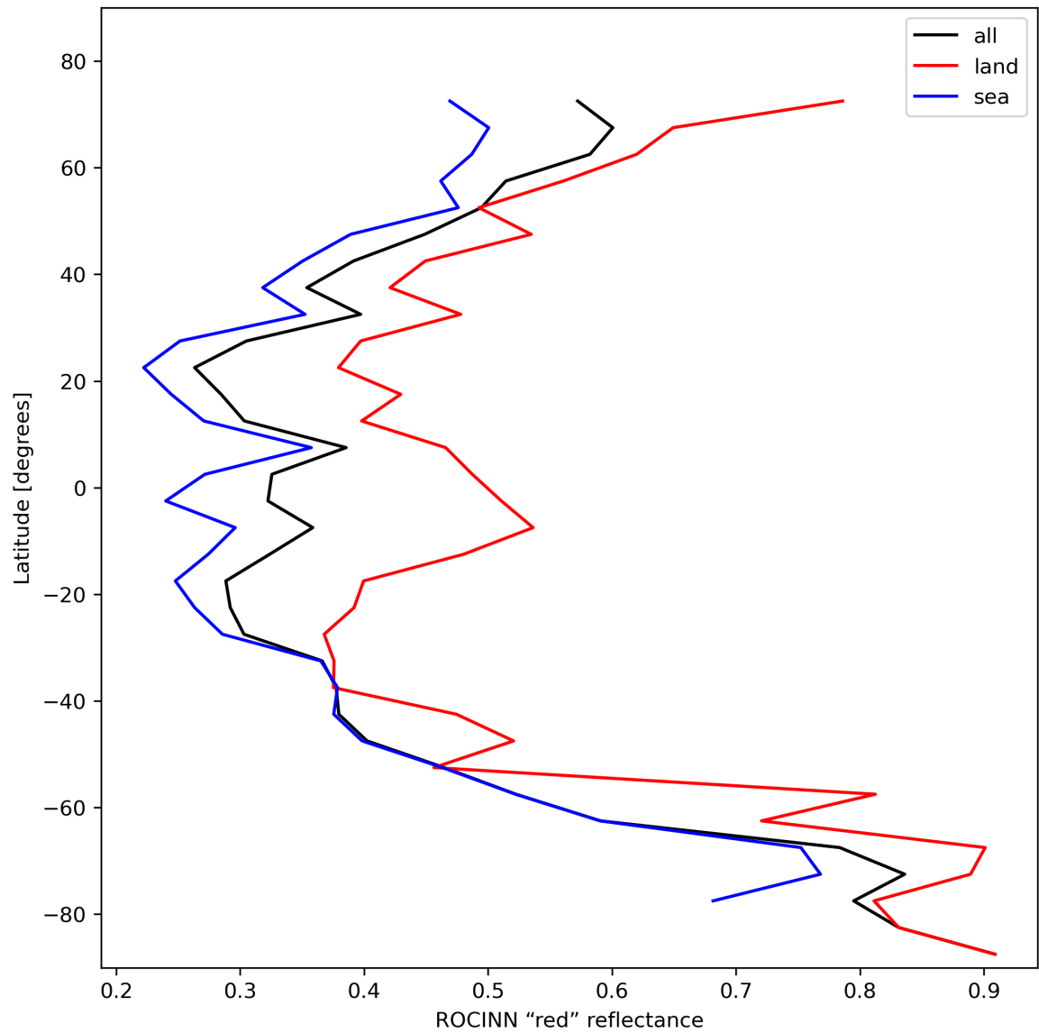
Figure 37: Zonal average of “ROCINN “red” reflectance” for 2023-11-03 to 2023-11-05.
