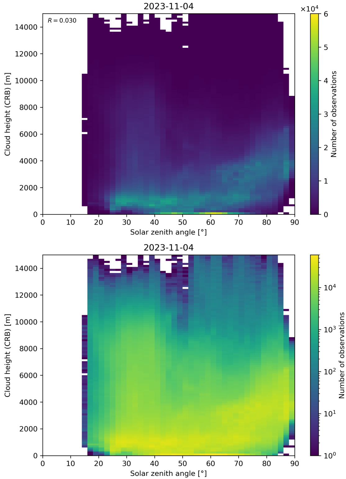
Figure 102: Scatter density plot of “Solar zenith angle” against “Cloud height (CRB)” for 2023-11-03 to 2023-11-05.
