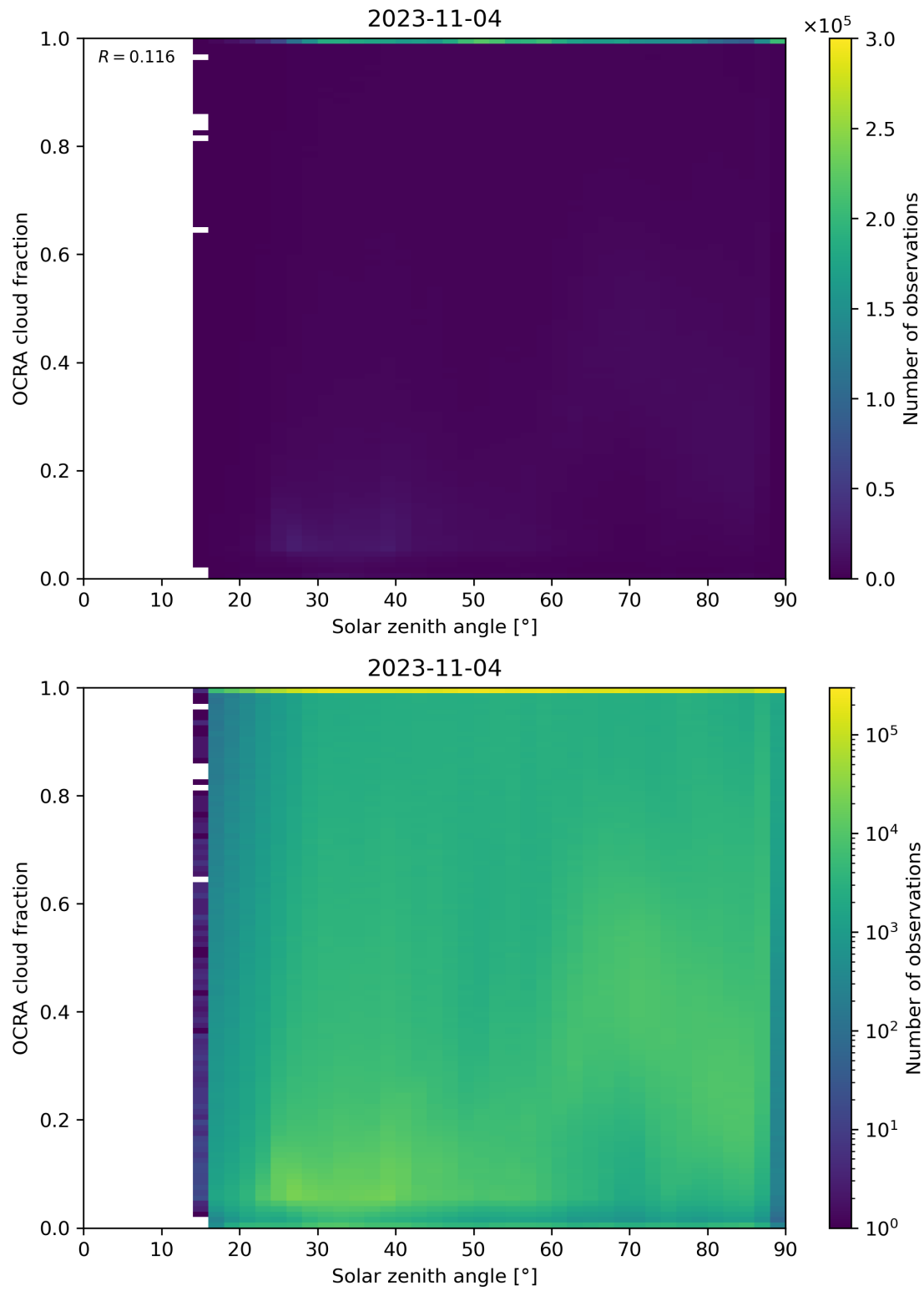
Figure 100: Scatter density plot of “Solar zenith angle” against “OCRA cloud fraction” for 2023-11-03 to 2023-11-05.
