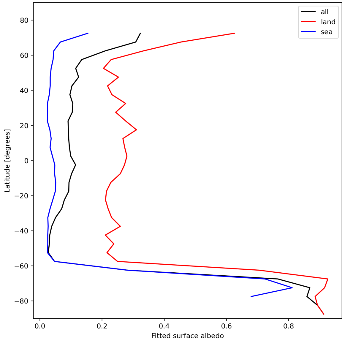
Figure 29: Zonal average of “Fitted surface albedo” for 2023-11-03 to 2023-11-05.
