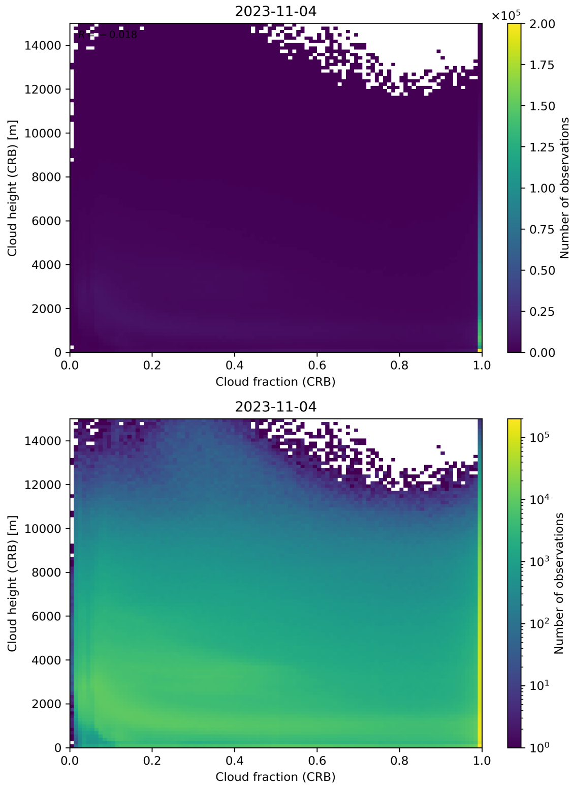
Figure 79: Scatter density plot of “Cloud fraction (CRB)” against “Cloud height (CRB)” for 2023-11-03 to 2023-11-05.
