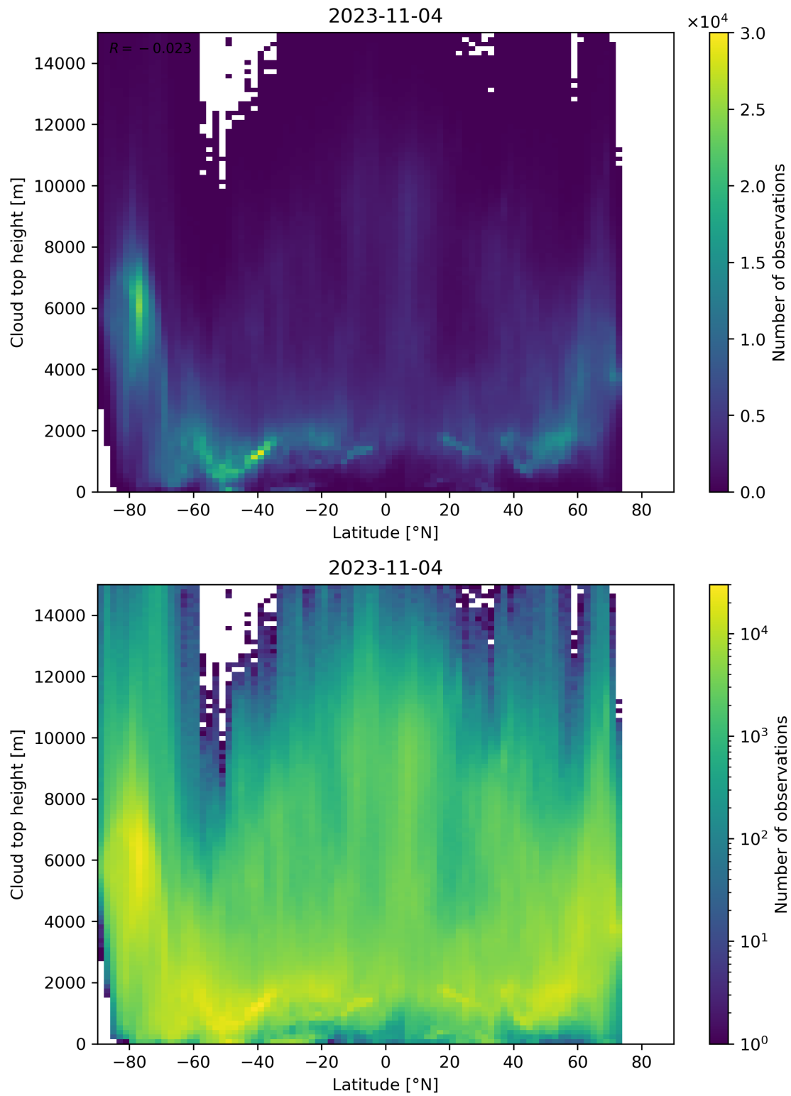
Figure 97: Scatter density plot of “Latitude” against “Cloud top height” for 2023-11-03 to 2023-11-05.
