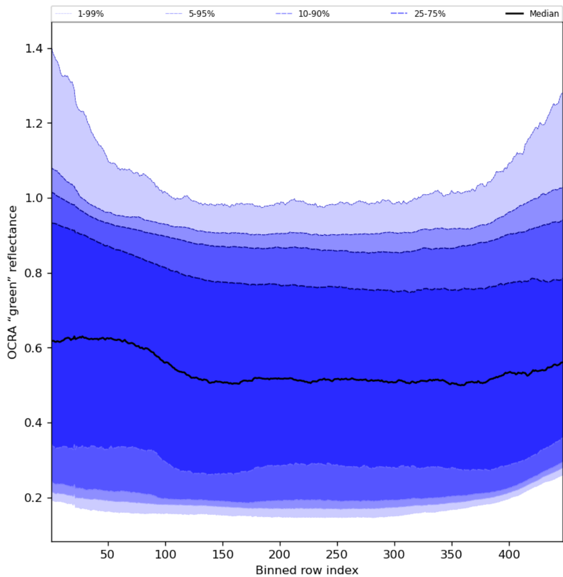
Figure 68: Along track statistics of "OCRA "green" reflectance" for 2023-11-03 to 2023-11-05
