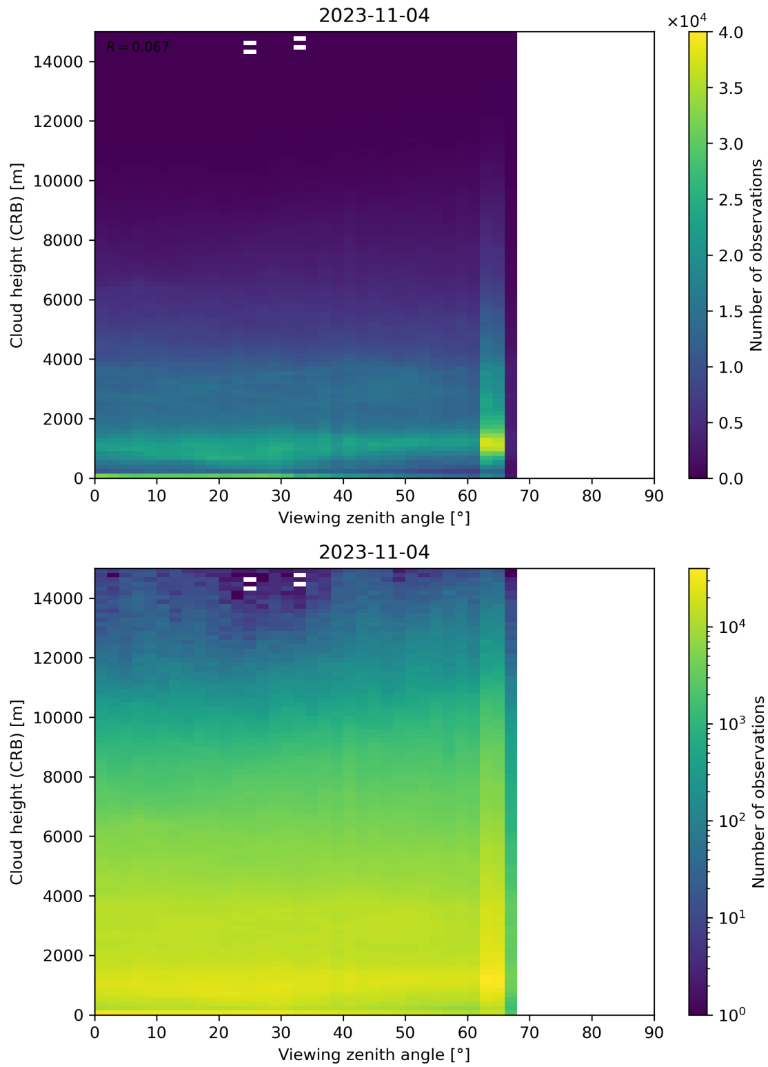
Figure 110: Scatter density plot of “Viewing zenith angle” against “Cloud height (CRB)” for 2023-11-03 to 2023-11-05.
