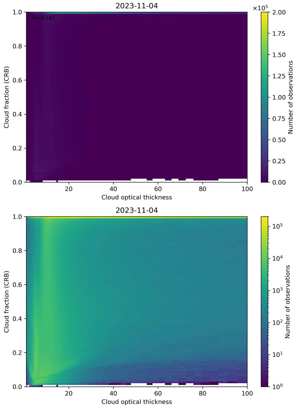
Figure 84: Scatter density plot of “Cloud optical thickness” against “Cloud fraction (CRB)” for 2023-11-03 to 2023-11-05.
