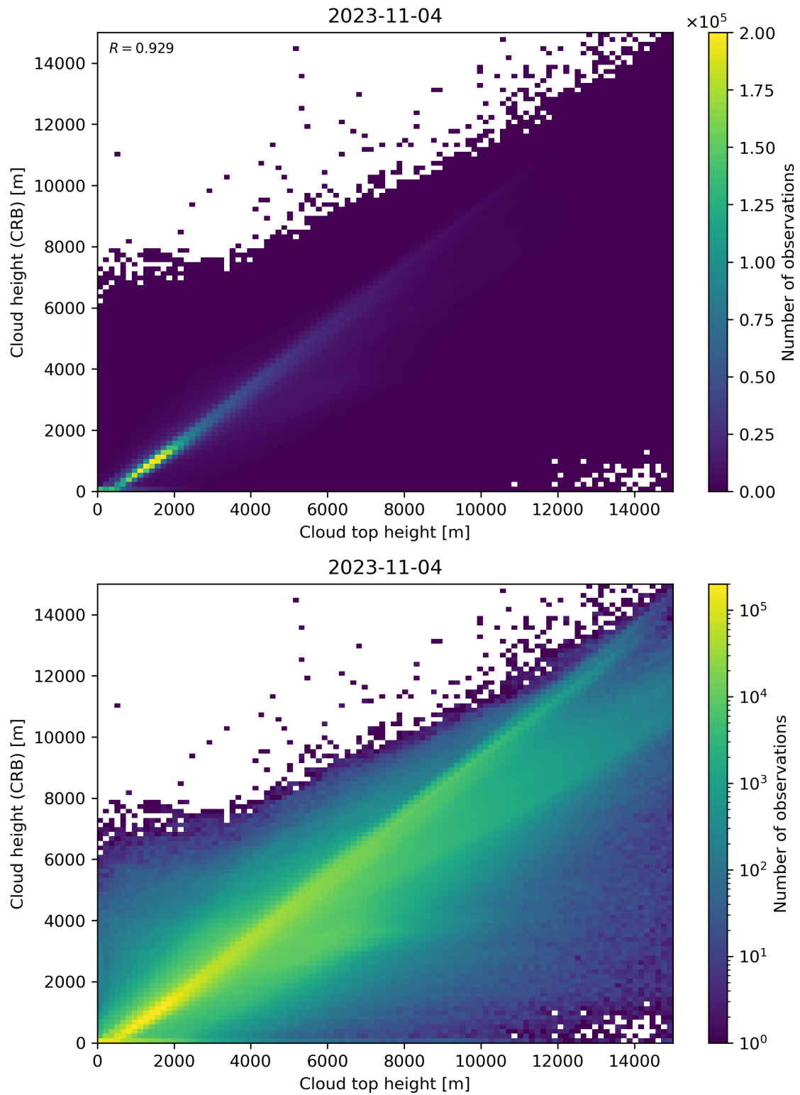
Figure 89: Scatter density plot of “Cloud top height” against “Cloud height (CRB)” for 2023-11-03 to 2023-11-05.
