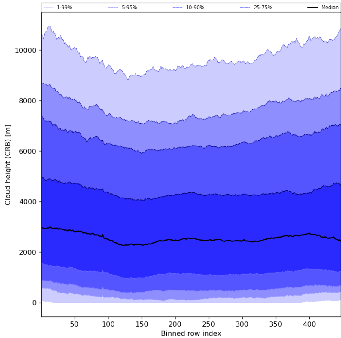
Figure 59: Along track statistics of “Cloud height (CRB)” for 2023-11-03 to 2023-11-05
