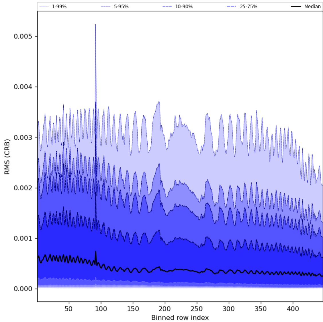
Figure 64: Along track statistics of “RMS (CRB)” for 2023-11-03 to 2023-11-05
