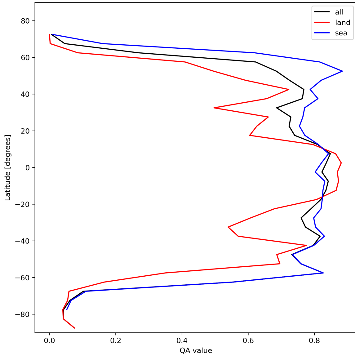
Figure 22: Zonal average of “QA value” for 2023-11-03 to 2023-11-05.
