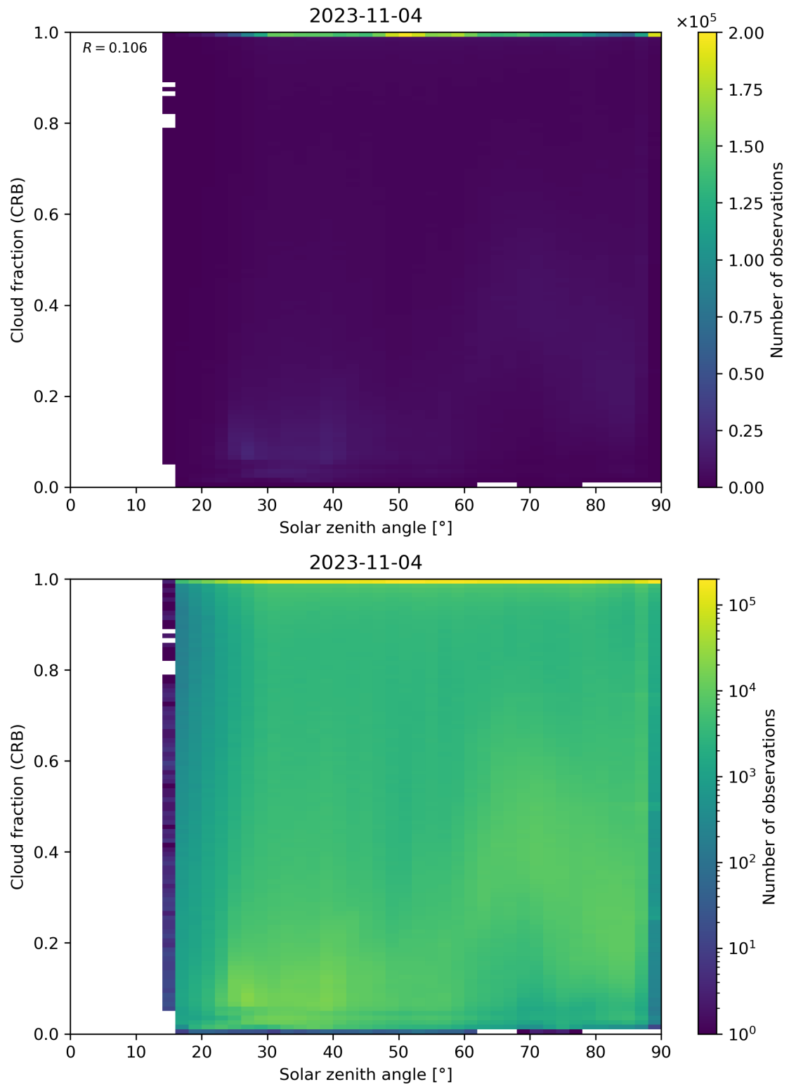
Figure 101: Scatter density plot of “Solar zenith angle” against “Cloud fraction (CRB)” for 2023-11-03 to 2023-11-05.
