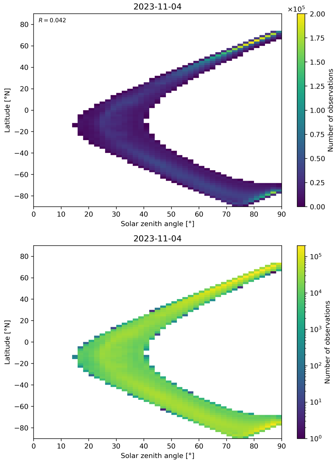
Figure 105: Scatter density plot of “Solar zenith angle” against “Latitude” for 2023-11-03 to 2023-11-05.
