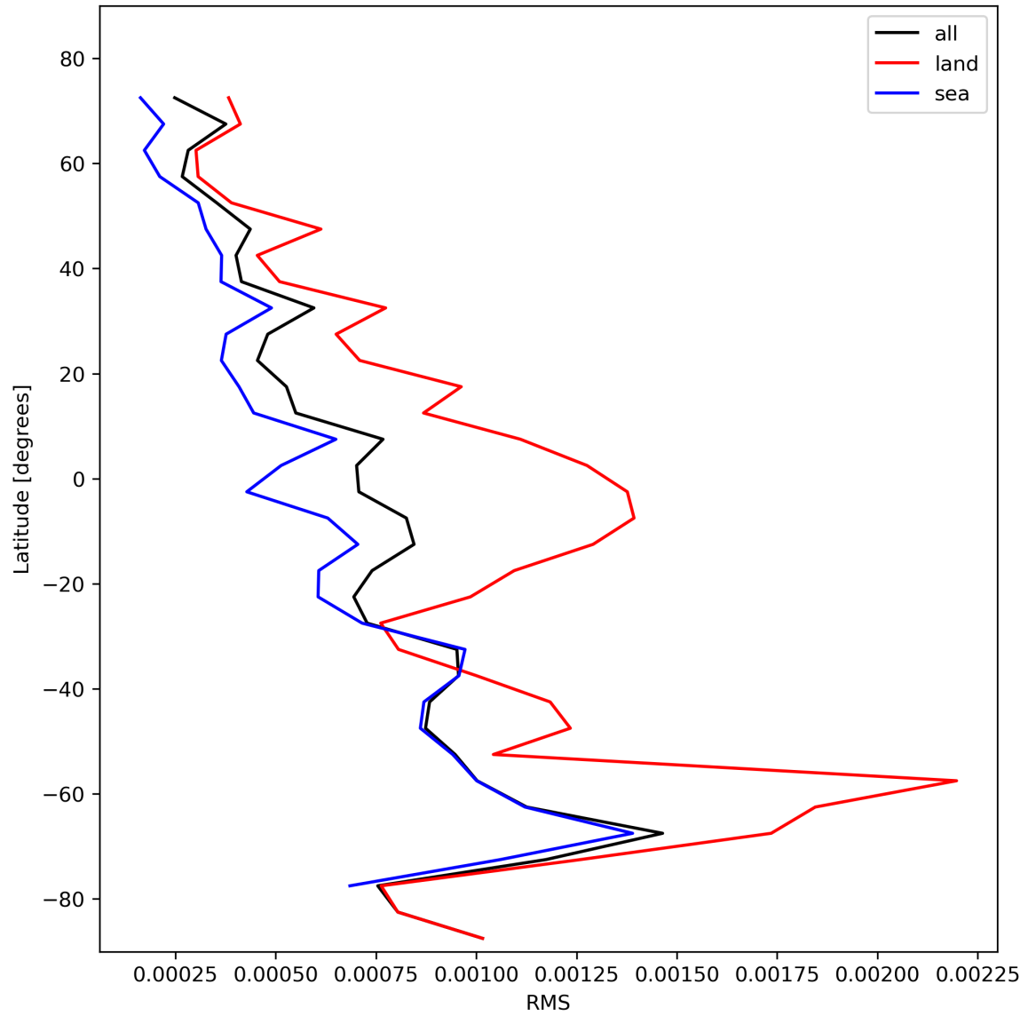
Figure 31: Zonal average of “RMS” for 2023-11-03 to 2023-11-05.
