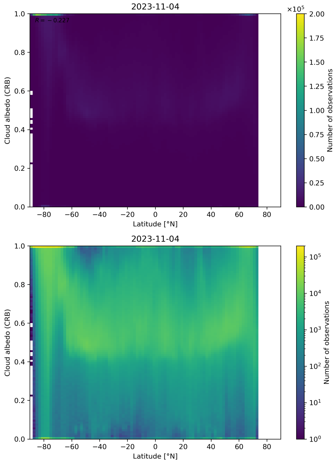
Figure 91: Scatter density plot of “Latitude” against “Cloud albedo (CRB)” for 2023-11-03 to 2023-11-05.
