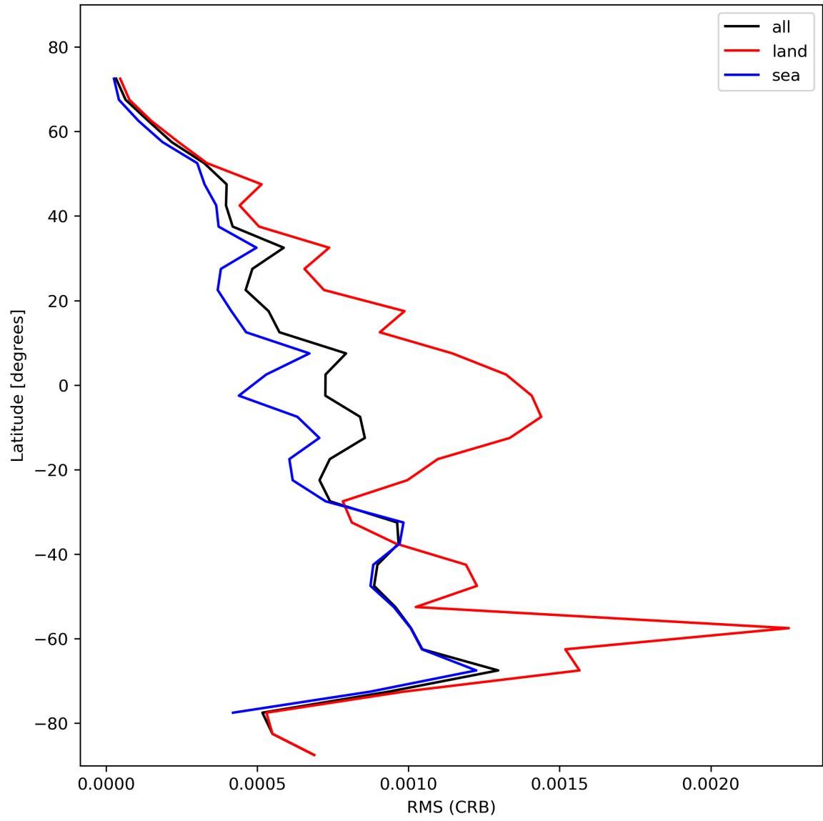
Figure 32: Zonal average of “RMS (CRB)” for 2023-11-03 to 2023-11-05.
