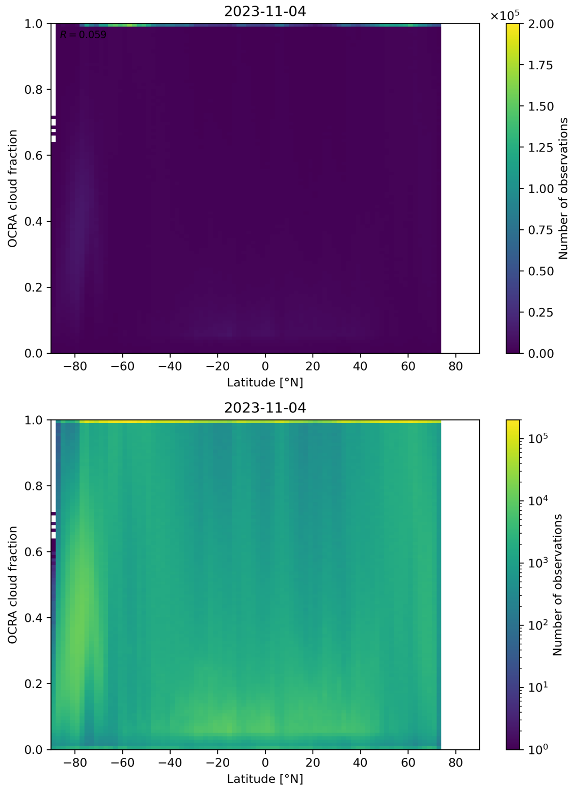
Figure 93: Scatter density plot of “Latitude” against “OCRA cloud fraction” for 2023-11-03 to 2023-11-05.
