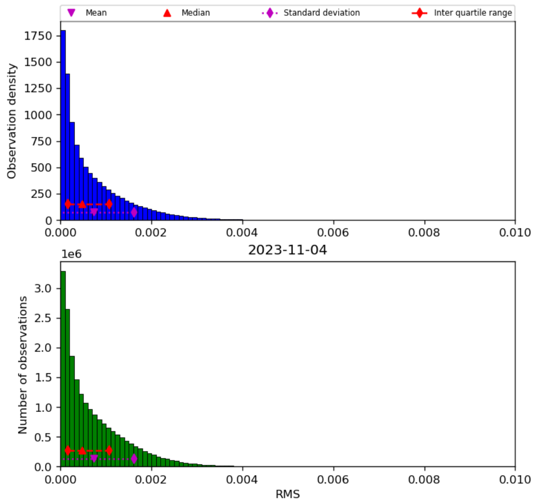
Figure 47: Histogram of “RMS” for 2023-11-03 to 2023-11-05
