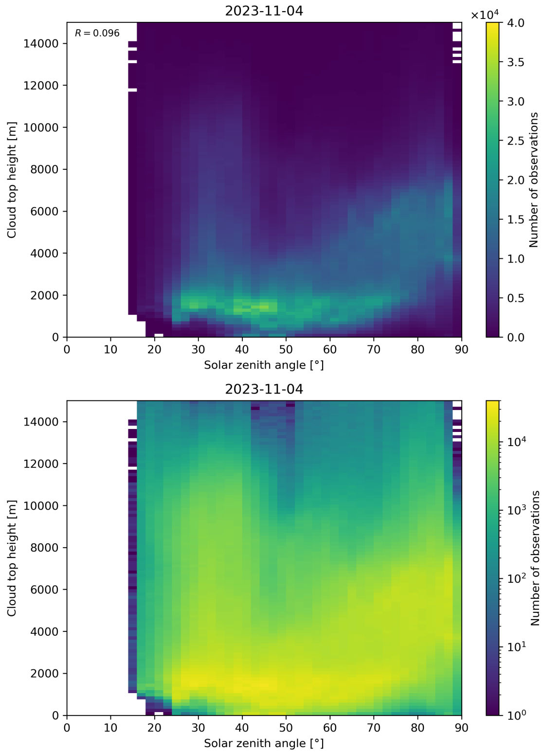
Figure 104: Scatter density plot of “Solar zenith angle” against “Cloud top height” for 2023-11-03 to 2023-11-05.
