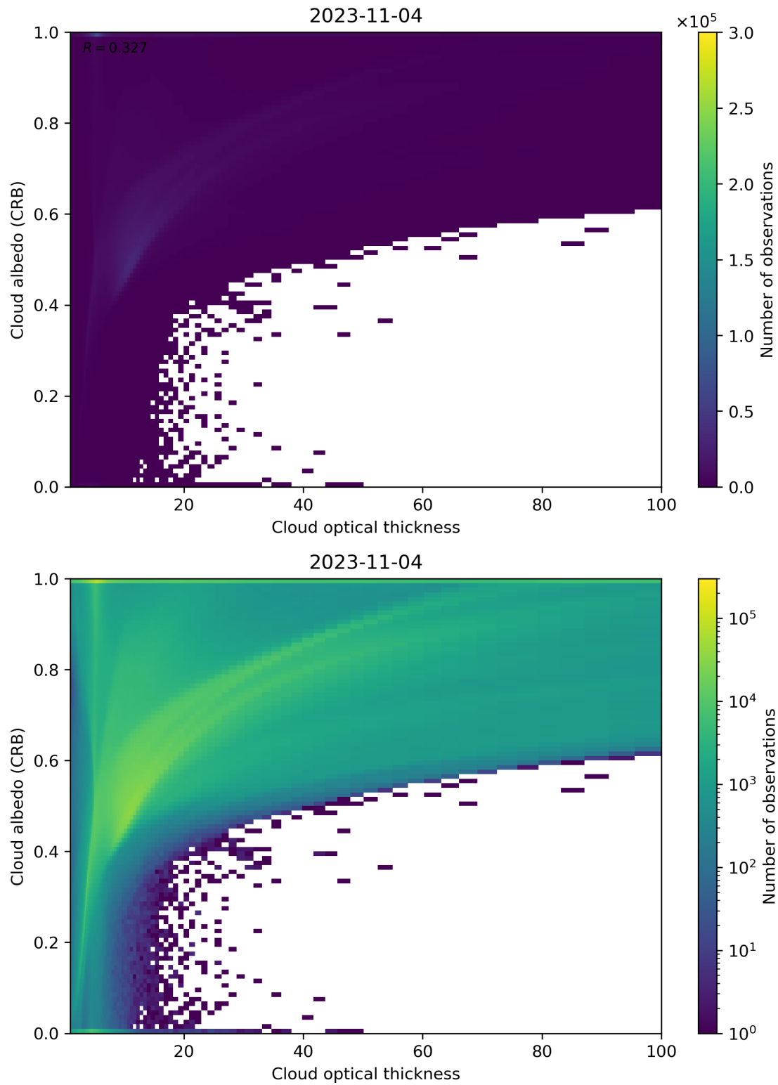
Figure 82: Scatter density plot of “Cloud optical thickness” against “Cloud albedo (CRB)” for 2023-11-03 to 2023-11-05.
