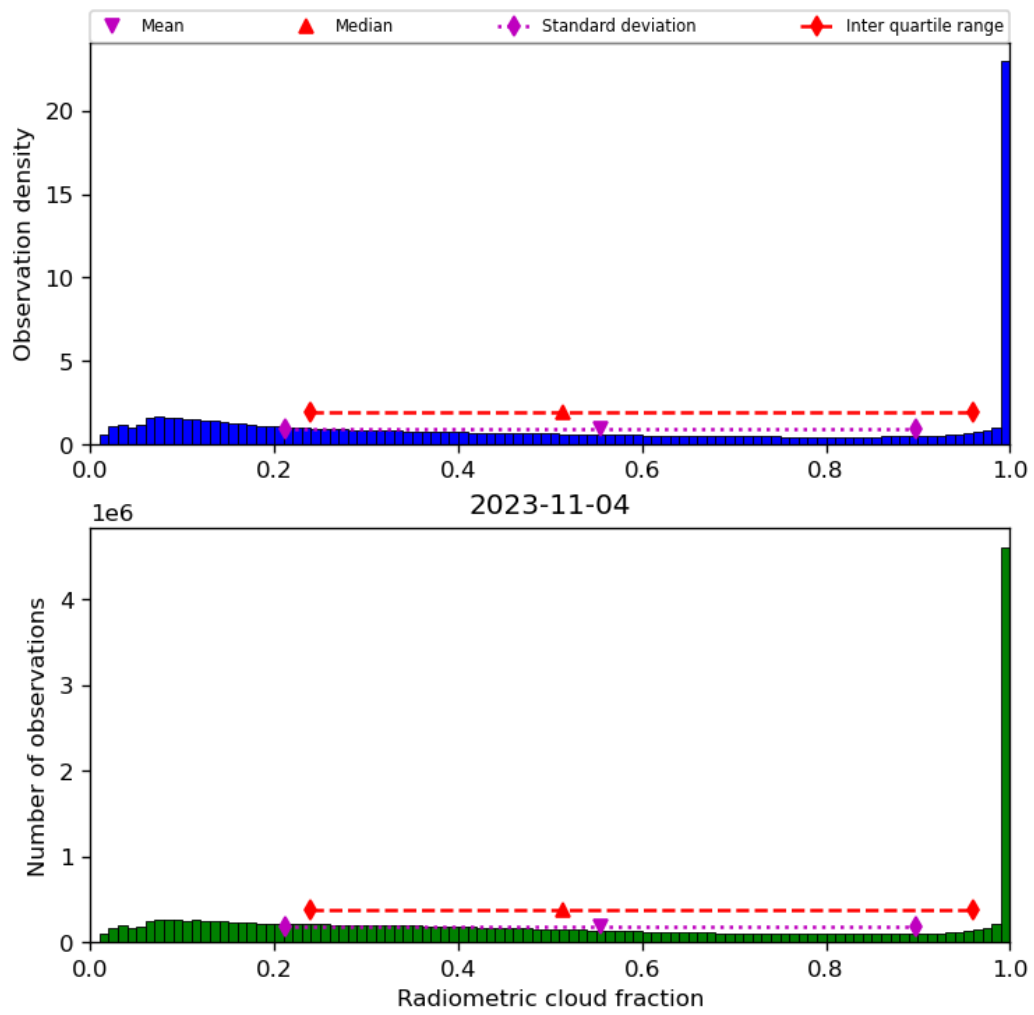
Figure 39: Histogram of “Radiometric cloud fraction” for 2023-11-03 to 2023-11-05
