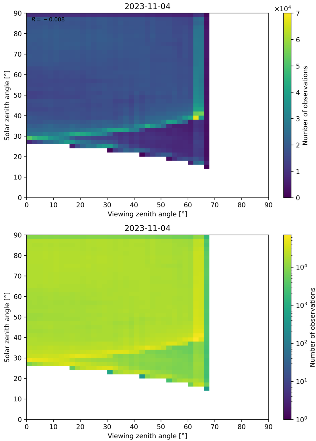
Figure 114: Scatter density plot of “Viewing zenith angle” against “Solar zenith angle” for 2023-11-03 to 2023-11-05.
