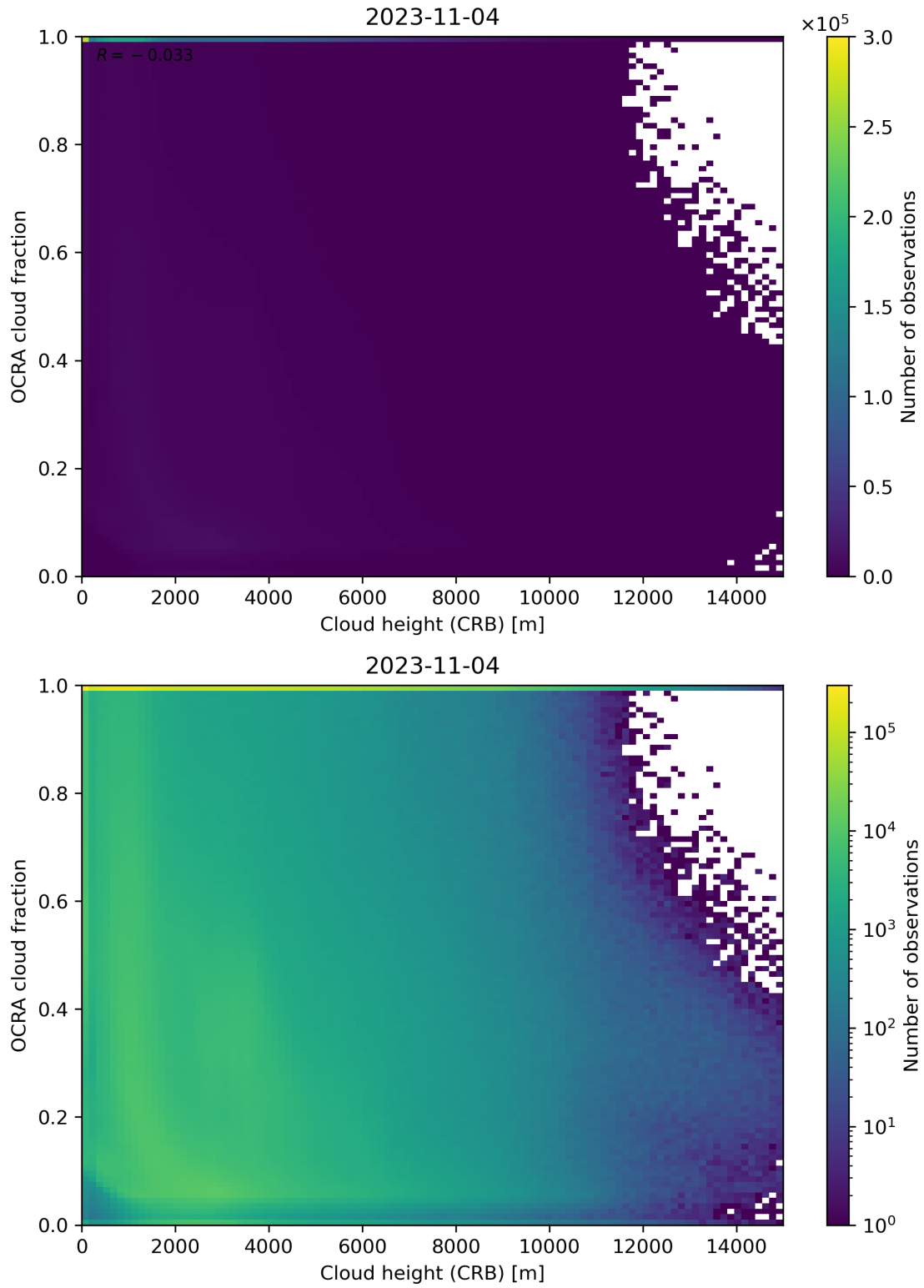
Figure 81: Scatter density plot of “Cloud height (CRB)” against “OCRA cloud fraction” for 2023-11-03 to 2023-11-05.
