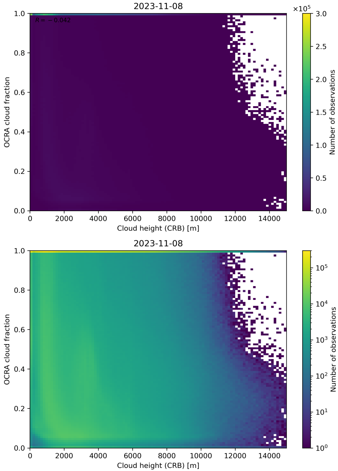
Figure 81: Scatter density plot of “Cloud height (CRB)” against “OCRA cloud fraction” for 2023-11-07 to 2023-11-09.
