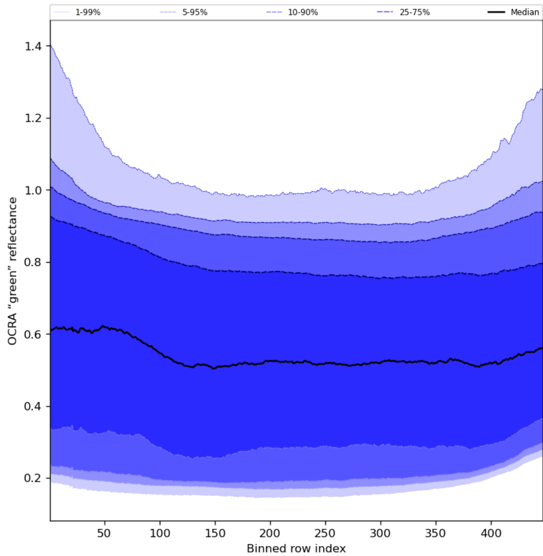
Figure 68: Along track statistics of “OCRA “green” reflectance” for 2023-11-07 to 2023-11-09
