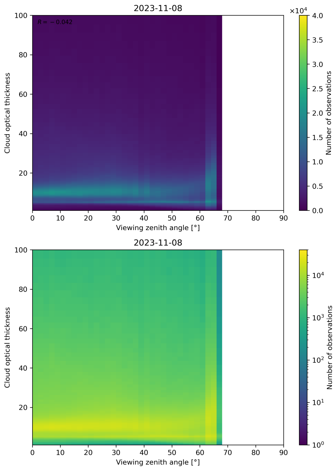
Figure 111: Scatter density plot of “Viewing zenith angle” against “Cloud optical thickness” for 2023-11-07 to 2023-11-09.
