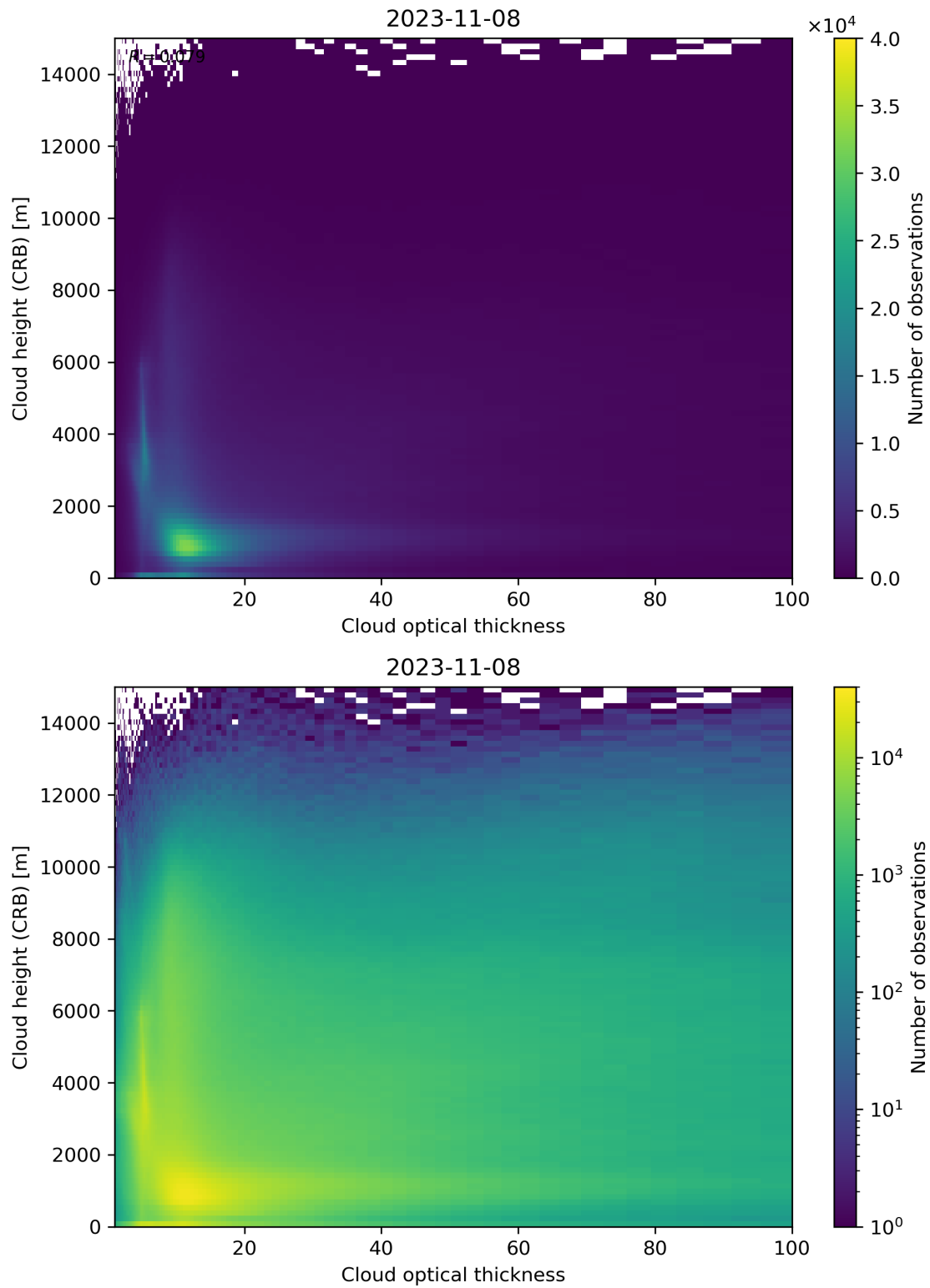
Figure 85: Scatter density plot of “Cloud optical thickness” against “Cloud height (CRB)” for 2023-11-07 to 2023-11-09.
