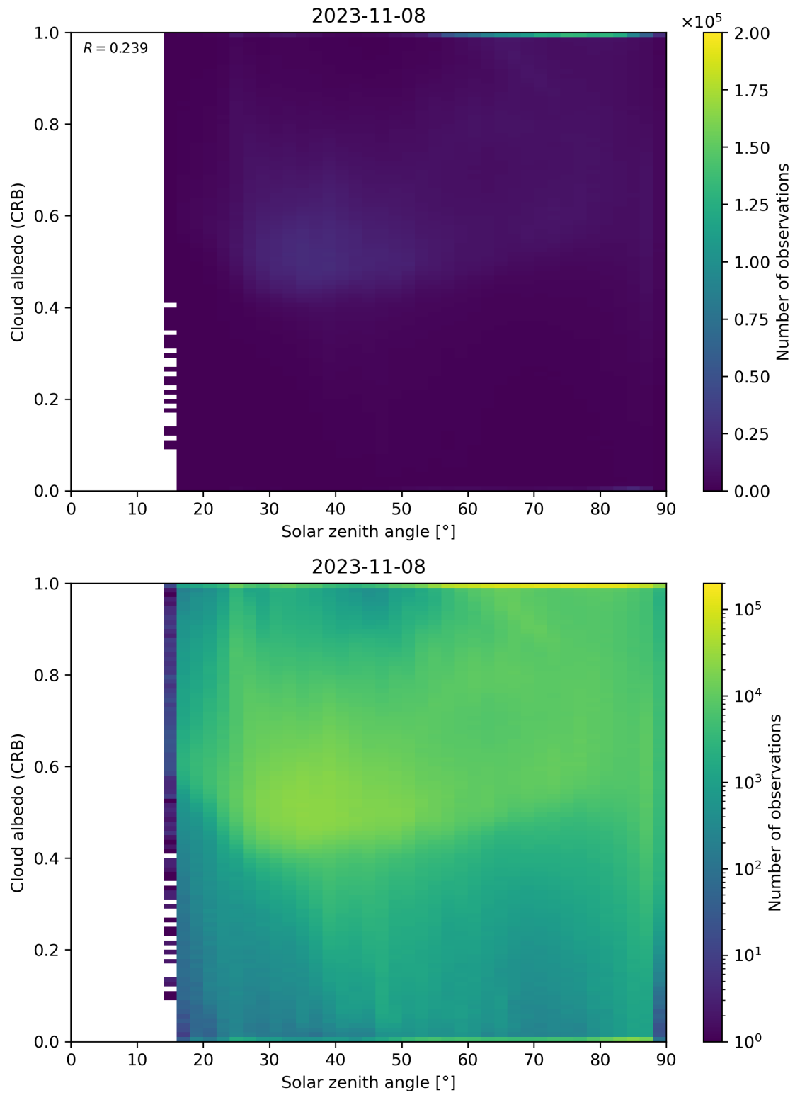
Figure 98: Scatter density plot of “Solar zenith angle” against “Cloud albedo (CRB)” for 2023-11-07 to 2023-11-09.
