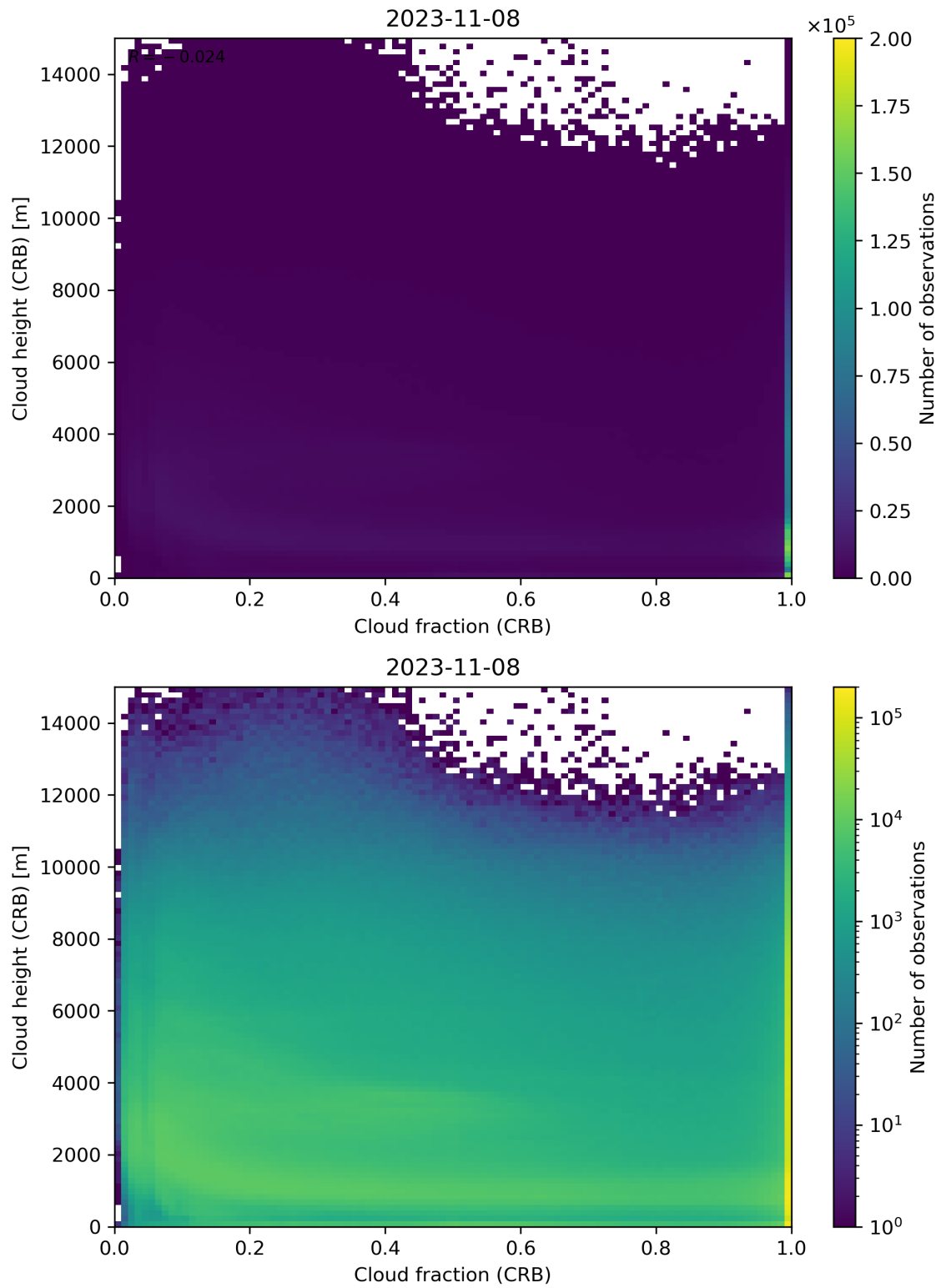
Figure 79: Scatter density plot of “Cloud fraction (CRB)” against “Cloud height (CRB)” for 2023-11-07 to 2023-11-09.
