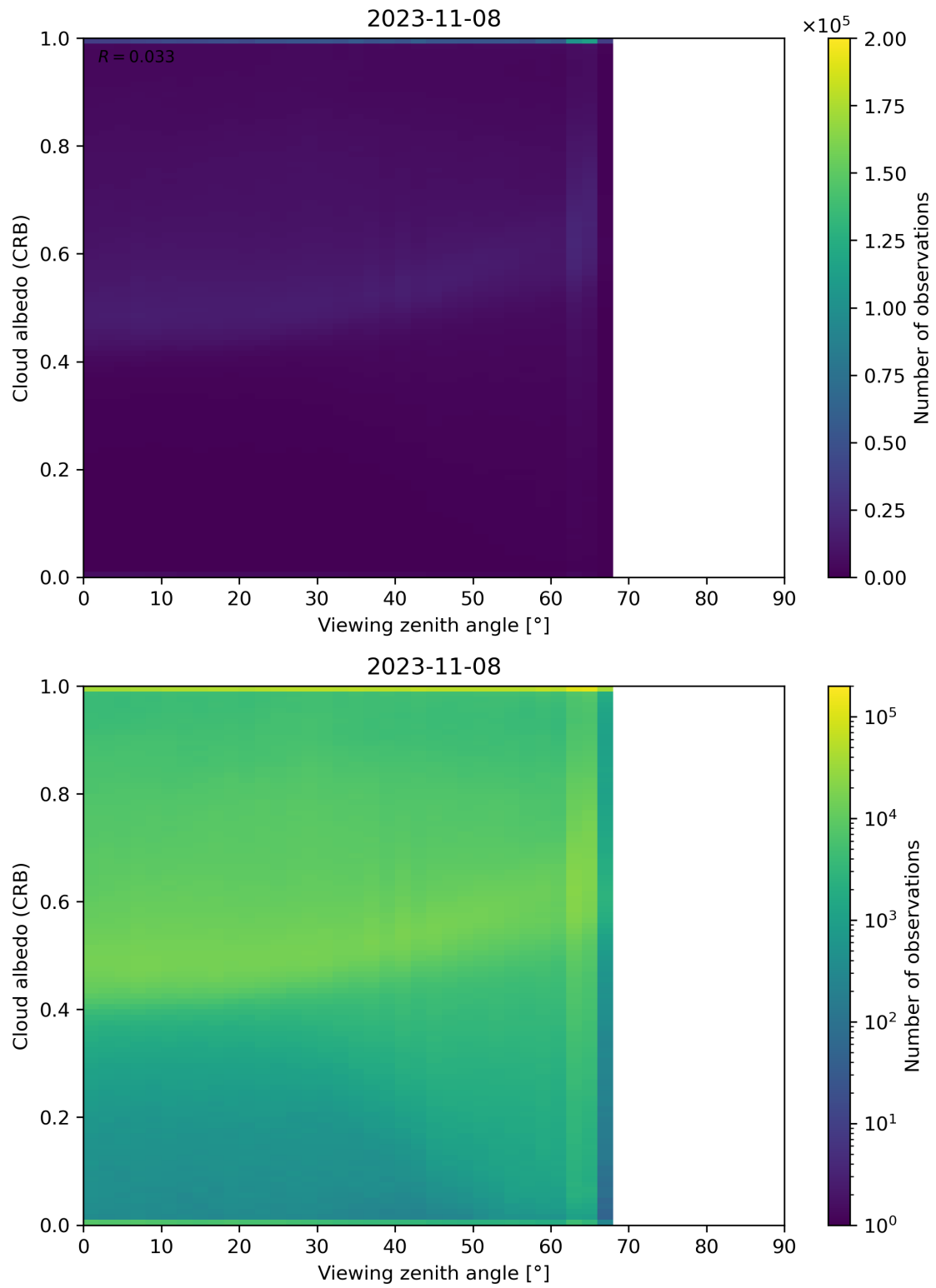
Figure 106: Scatter density plot of “Viewing zenith angle” against “Cloud albedo (CRB)” for 2023-11-07 to 2023-11-09.
