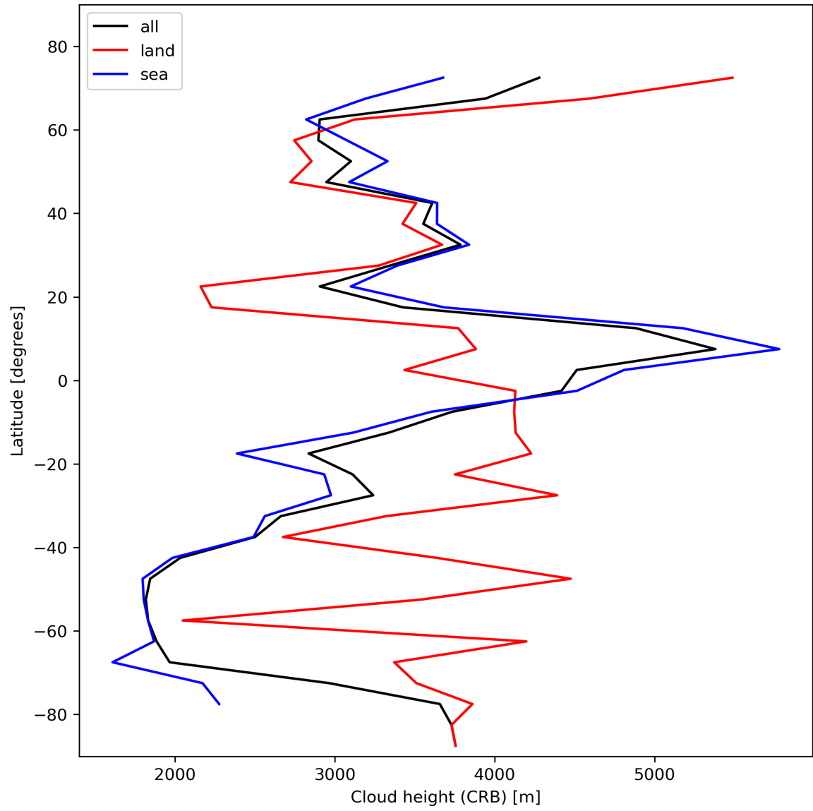
Figure 27: Zonal average of “Cloud height (CRB)” for 2023-11-07 to 2023-11-09.
