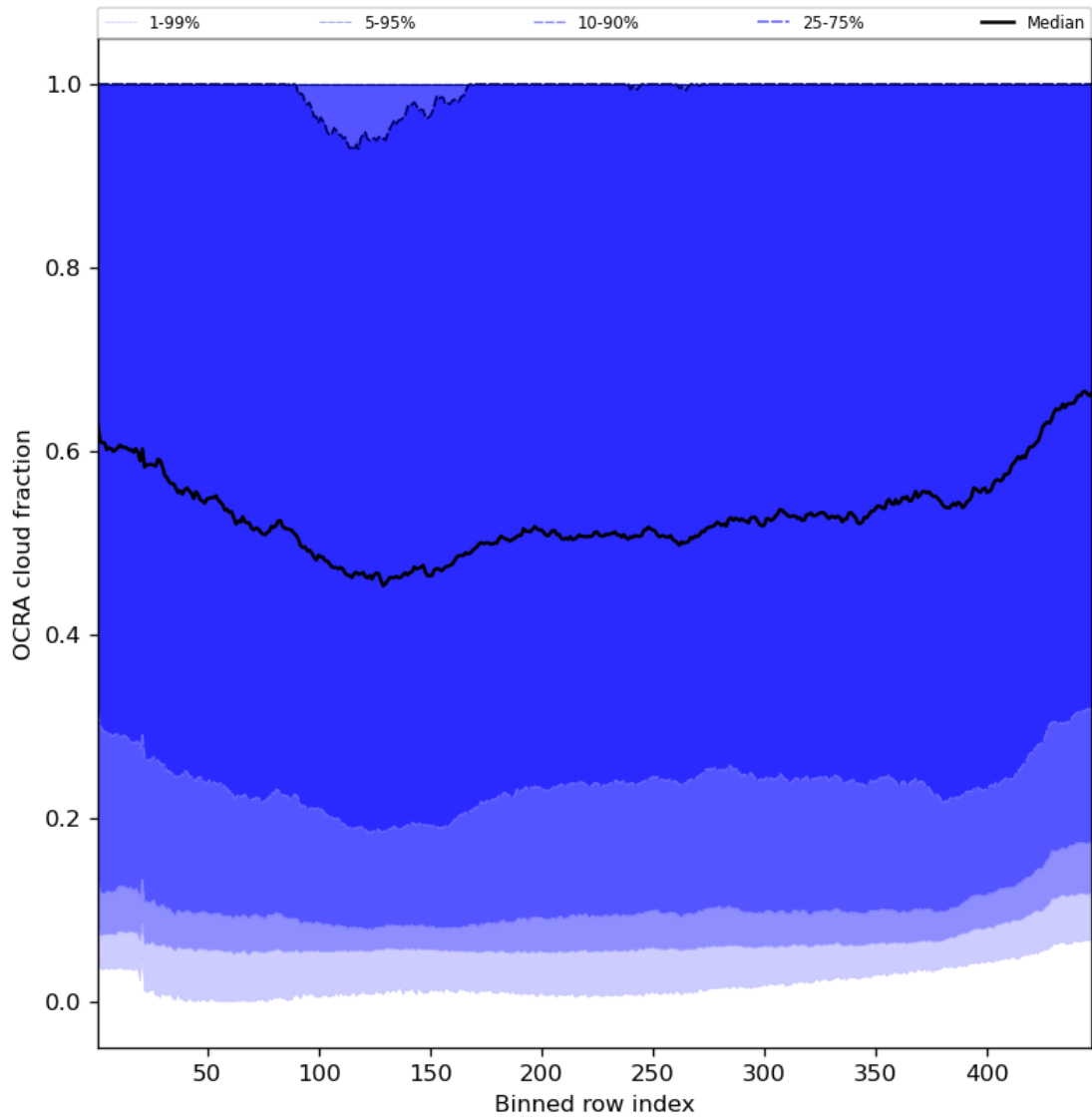
Figure 66: Along track statistics of “OCRA cloud fraction” for 2023-11-07 to 2023-11-09
