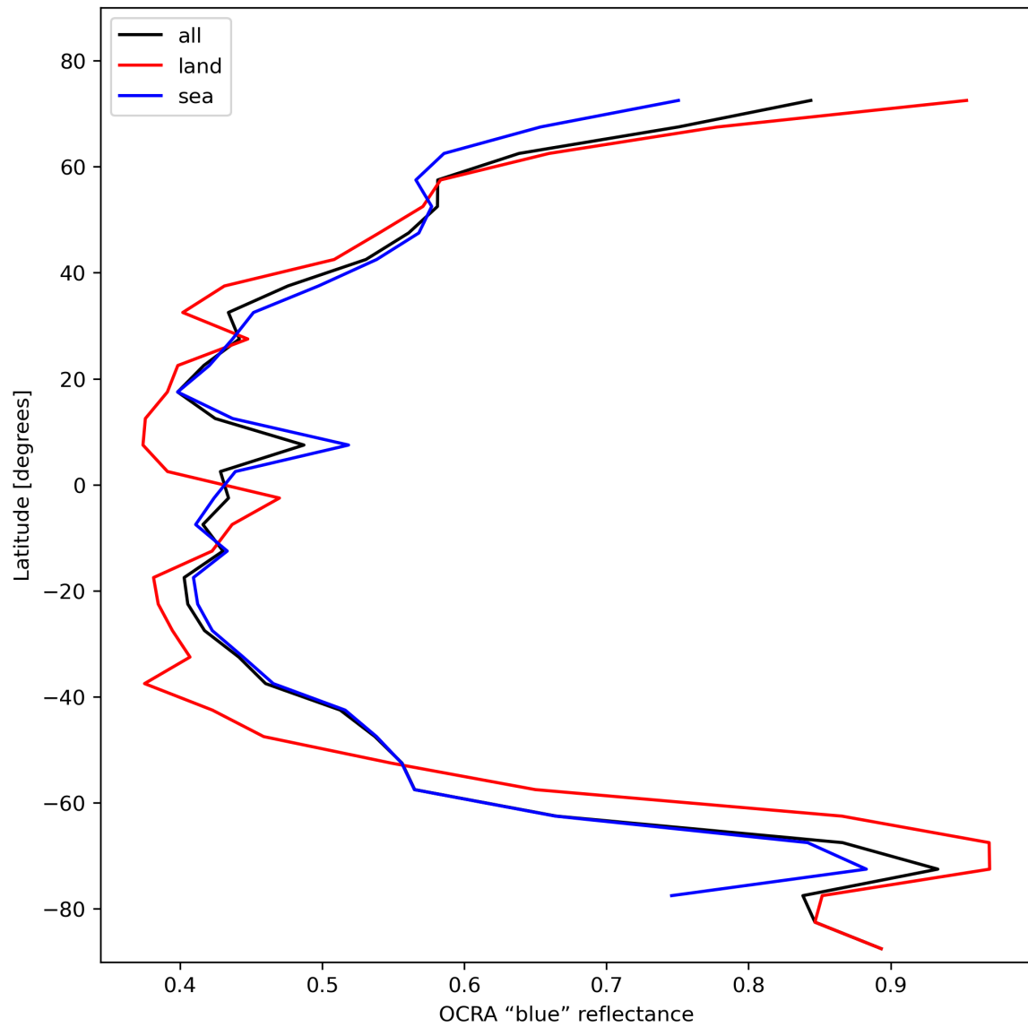
Figure 35: Zonal average of “OCRA “blue” reflectance” for 2023-11-07 to 2023-11-09.
