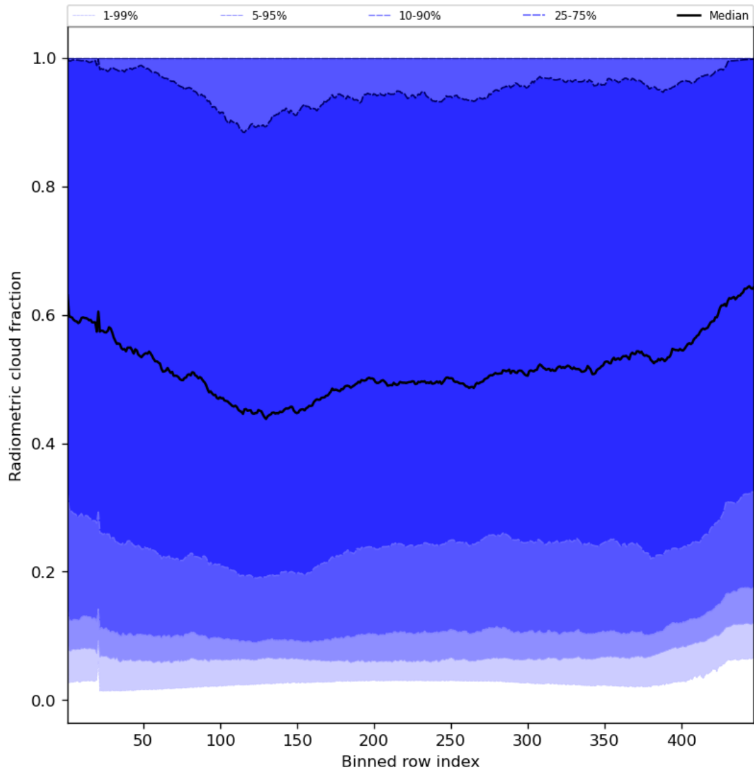
Figure 55: Along track statistics of “Radiometric cloud fraction” for 2023-11-07 to 2023-11-09
