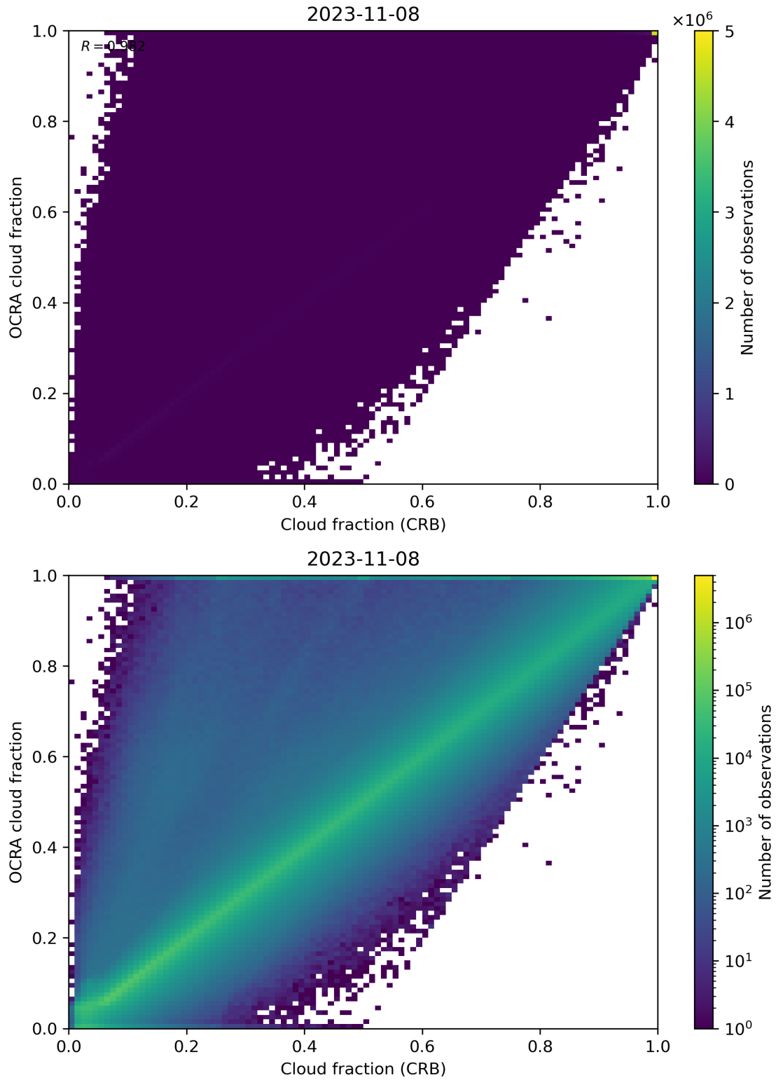
Figure 78: Scatter density plot of “Cloud fraction (CRB)” against “OCRA cloud fraction” for 2023-11-07 to 2023-11-09.
