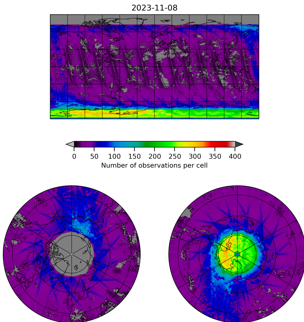
Figure 21: Map of the number of observations for 2023-11-07 to 2023-11-09
