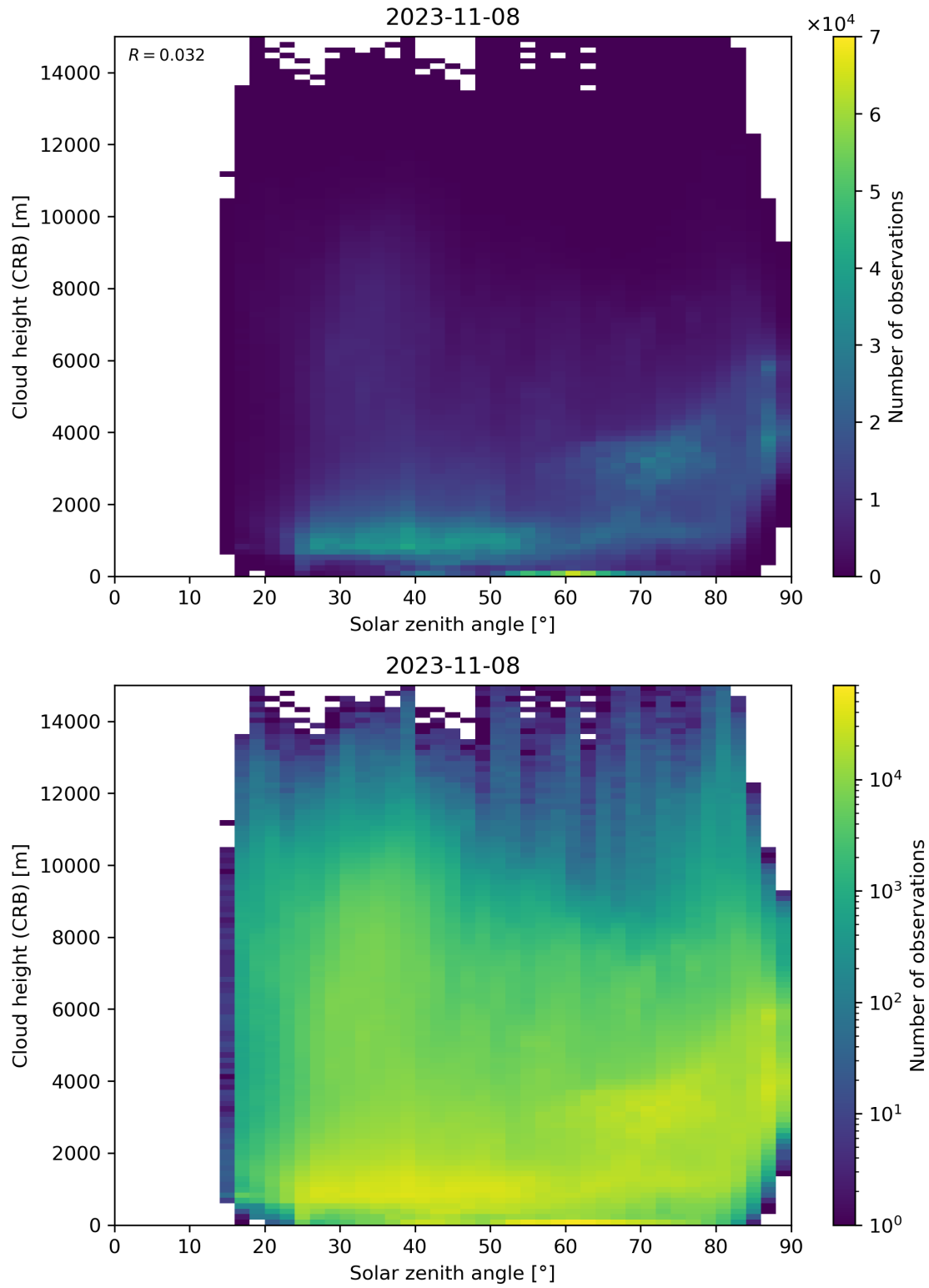
Figure 102: Scatter density plot of “Solar zenith angle” against “Cloud height (CRB)” for 2023-11-07 to 2023-11-09.
