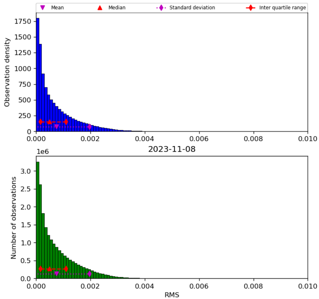
Figure 47: Histogram of “RMS” for 2023-11-07 to 2023-11-09
