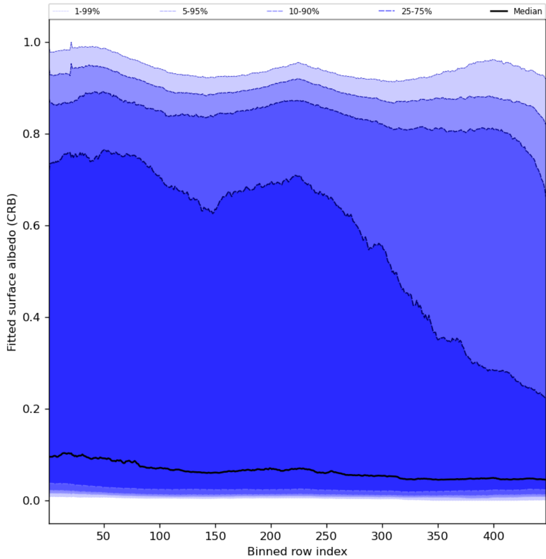
Figure 62: Along track statistics of “Fitted surface albedo (CRB)” for 2023-11-07 to 2023-11-09
