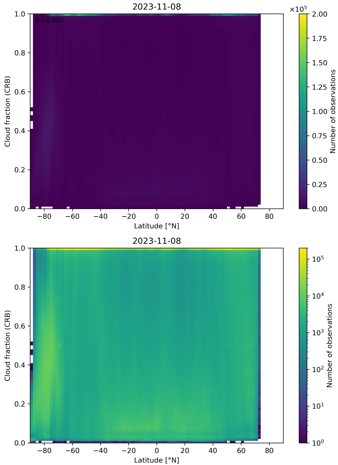
Figure 94: Scatter density plot of “Latitude” against “Cloud fraction (CRB)” for 2023-11-07 to 2023-11-09.
