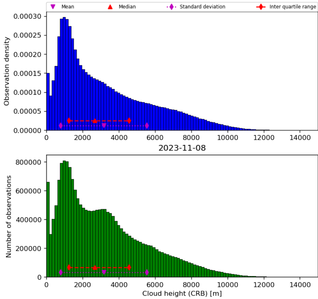
Figure 43: Histogram of “Cloud height (CRB)” for 2023-11-07 to 2023-11-09
