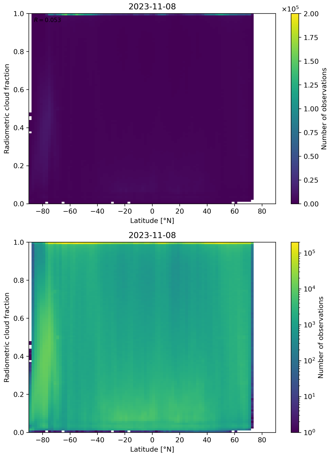
Figure 92: Scatter density plot of “Latitude” against “Radiometric cloud fraction” for 2023-11-07 to 2023-11-09.
