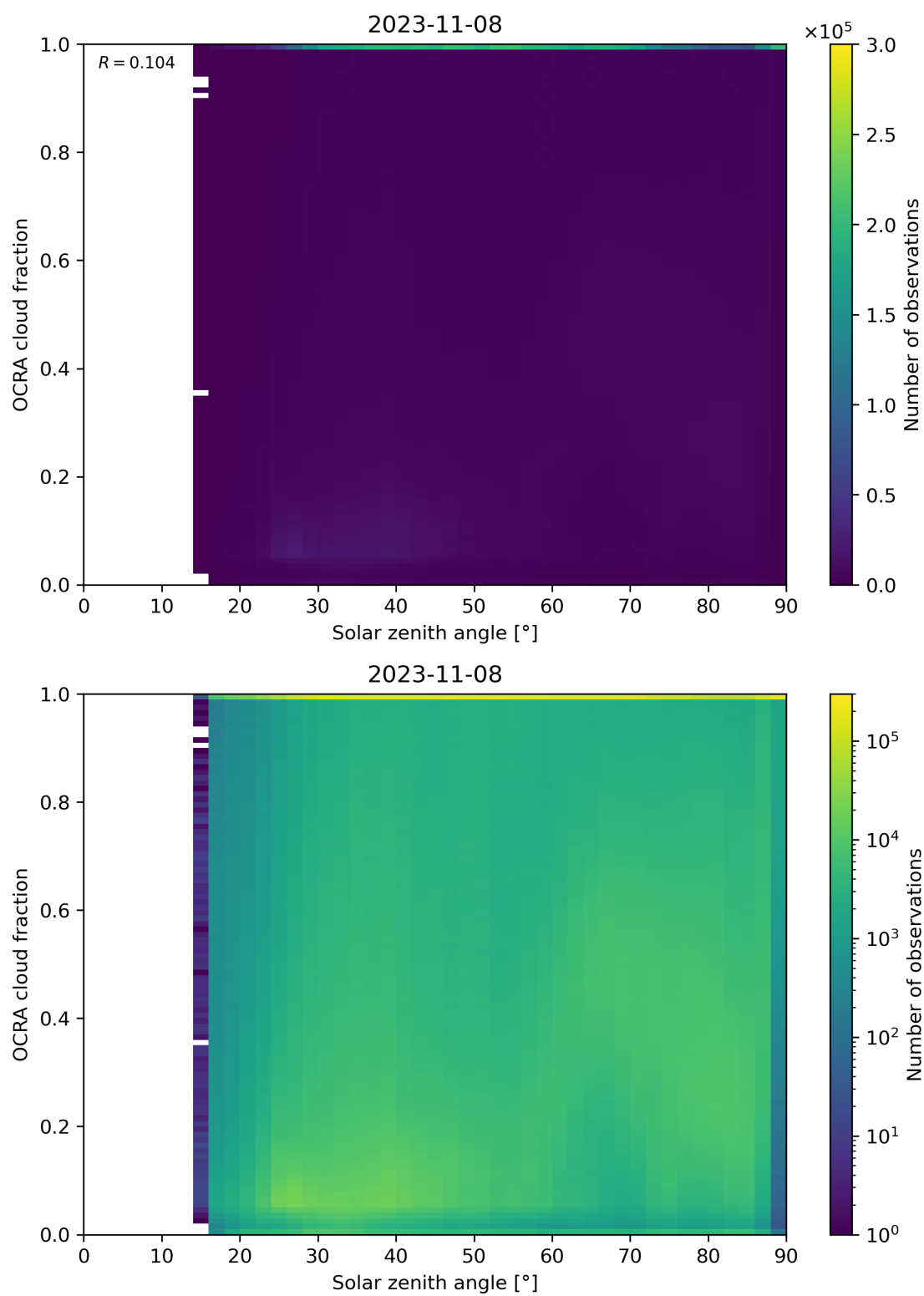
Figure 100: Scatter density plot of “Solar zenith angle” against “OCRA cloud fraction” for 2023-11-07 to 2023-11-09.
