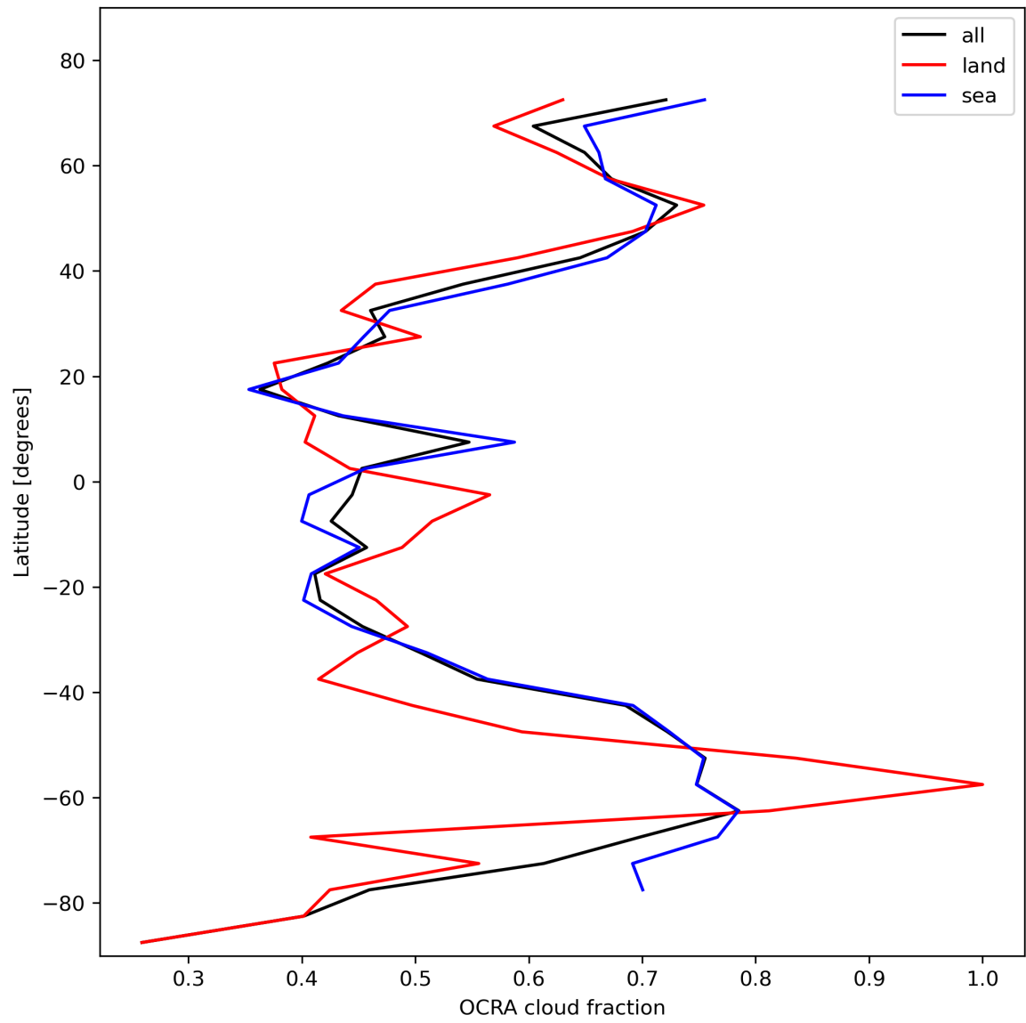
Figure 34: Zonal average of “OCRA cloud fraction” for 2023-11-07 to 2023-11-09.
