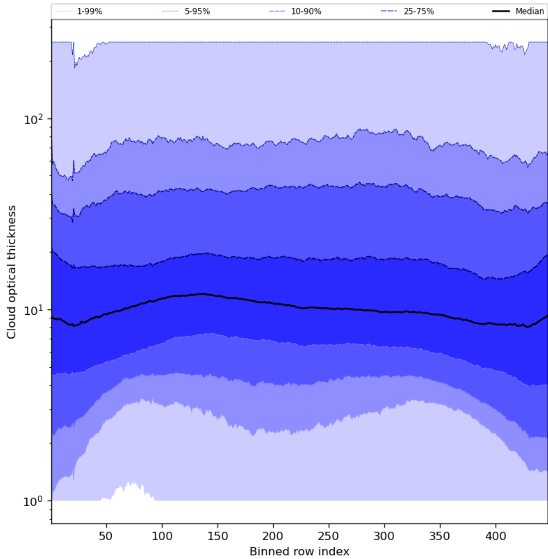
Figure 57: Along track statistics of “Cloud optical thickness” for 2023-11-07 to 2023-11-09
