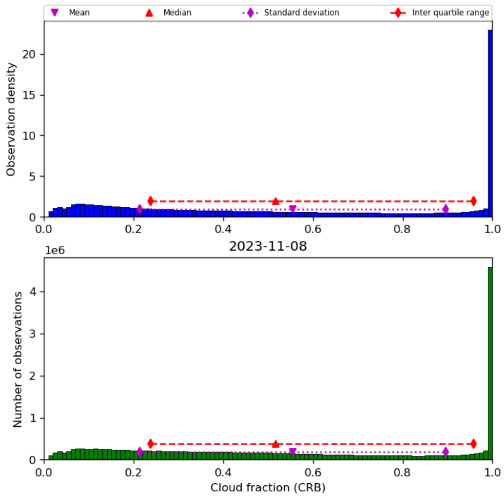
Figure 42: Histogram of “Cloud fraction (CRB)” for 2023-11-07 to 2023-11-09
