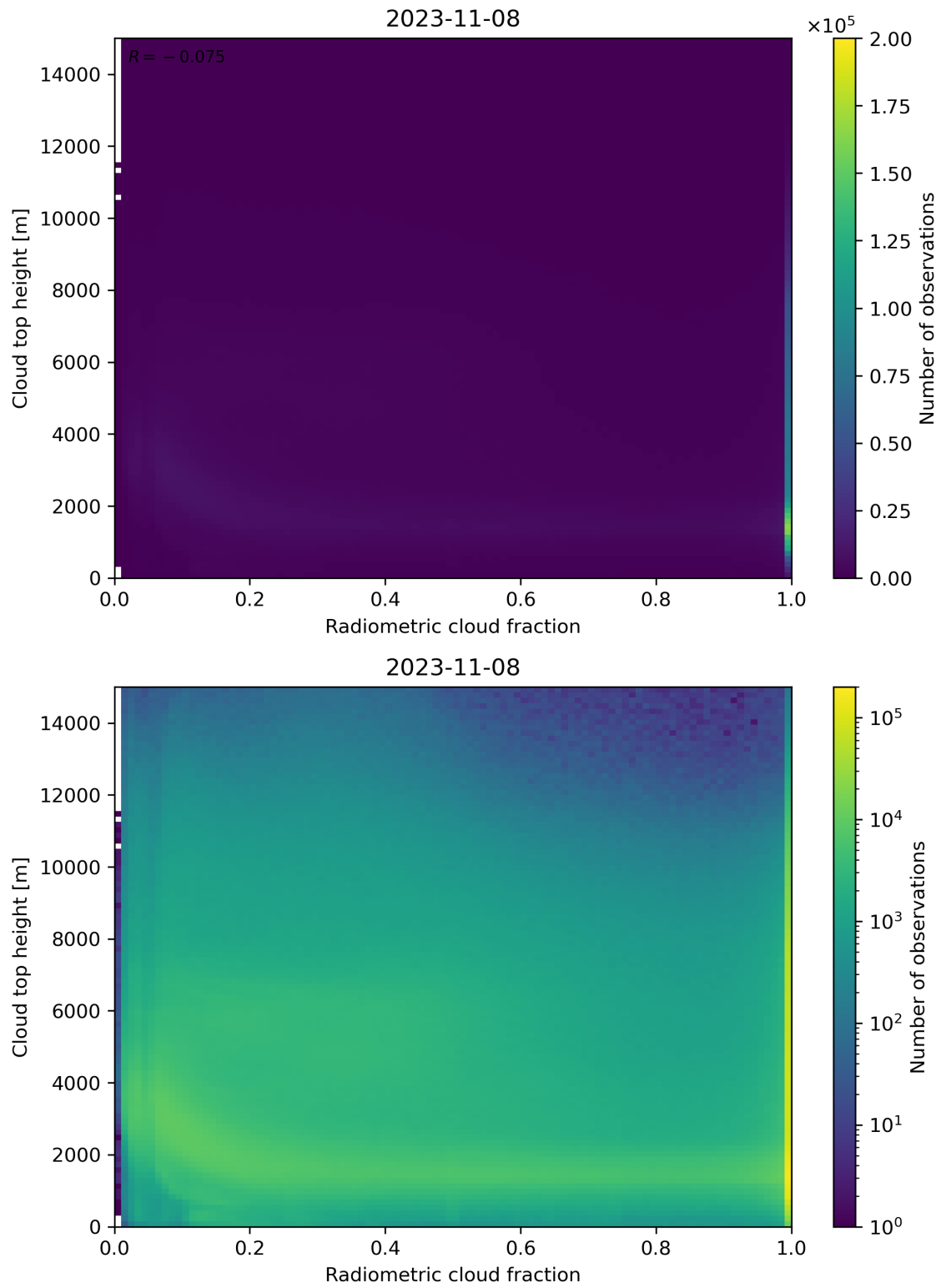
Figure 76: Scatter density plot of “Radiometric cloud fraction” against “Cloud top height” for 2023-11-07 to 2023-11-09.
