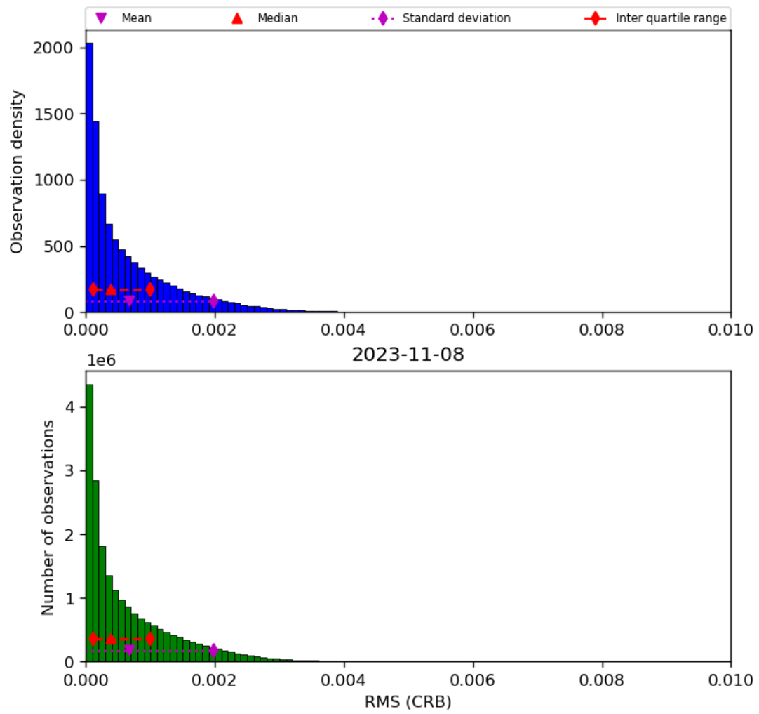
Figure 48: Histogram of “RMS (CRB)” for 2023-11-07 to 2023-11-09
