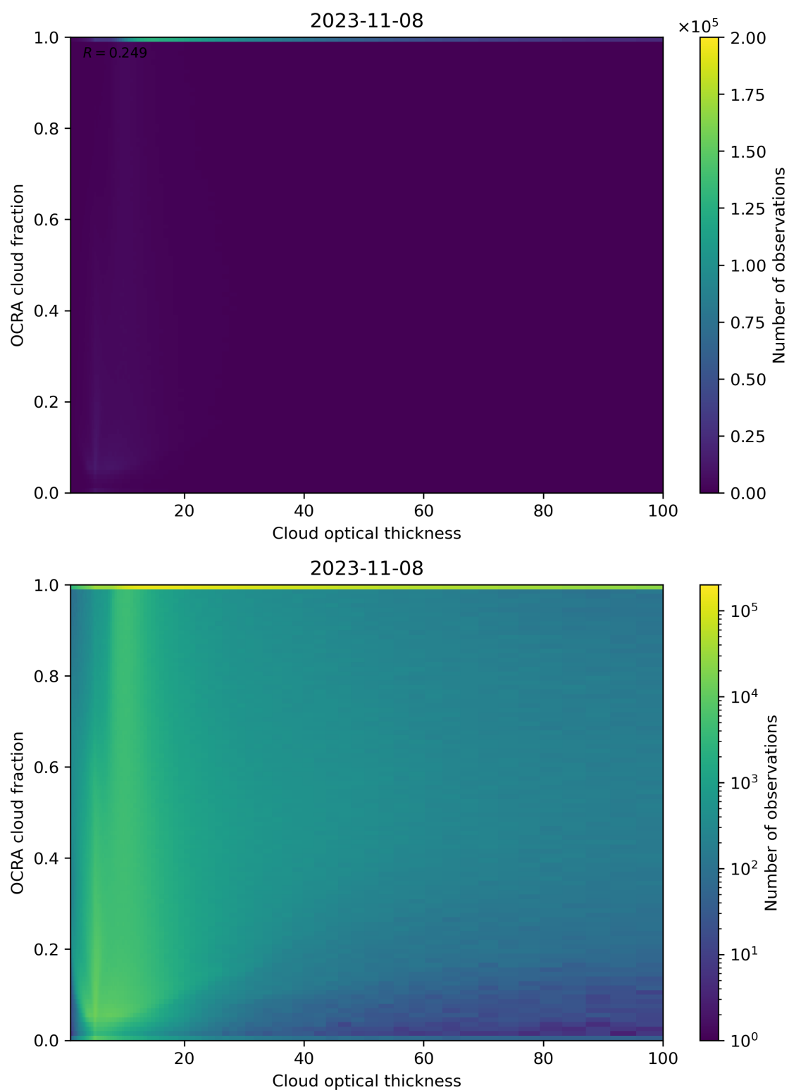
Figure 83: Scatter density plot of “Cloud optical thickness” against “OCRA cloud fraction” for 2023-11-07 to 2023-11-09.
