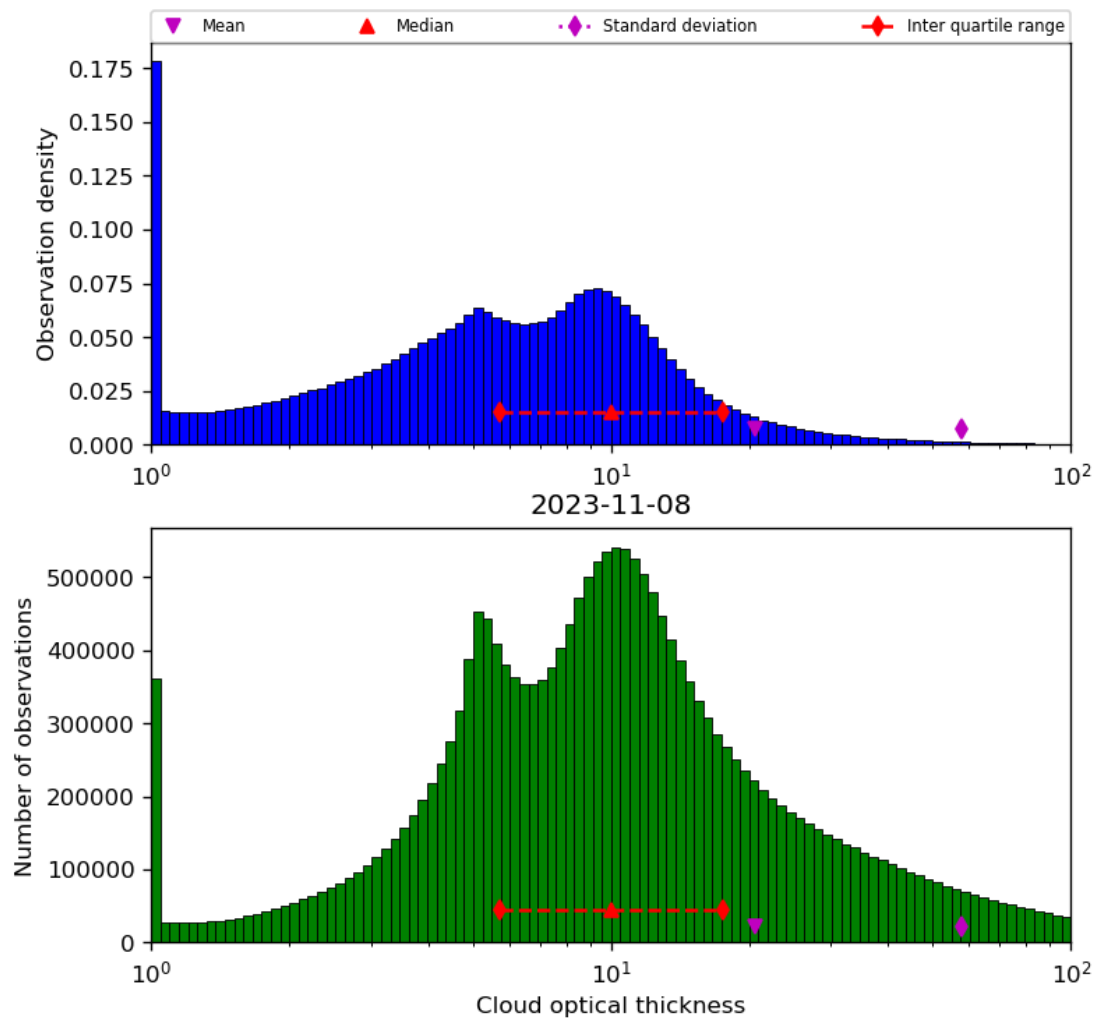
Figure 41: Histogram of “Cloud optical thickness” for 2023-11-07 to 2023-11-09
