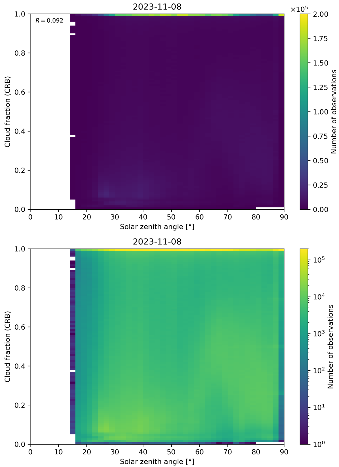
Figure 101: Scatter density plot of “Solar zenith angle” against “Cloud fraction (CRB)” for 2023-11-07 to 2023-11-09.
