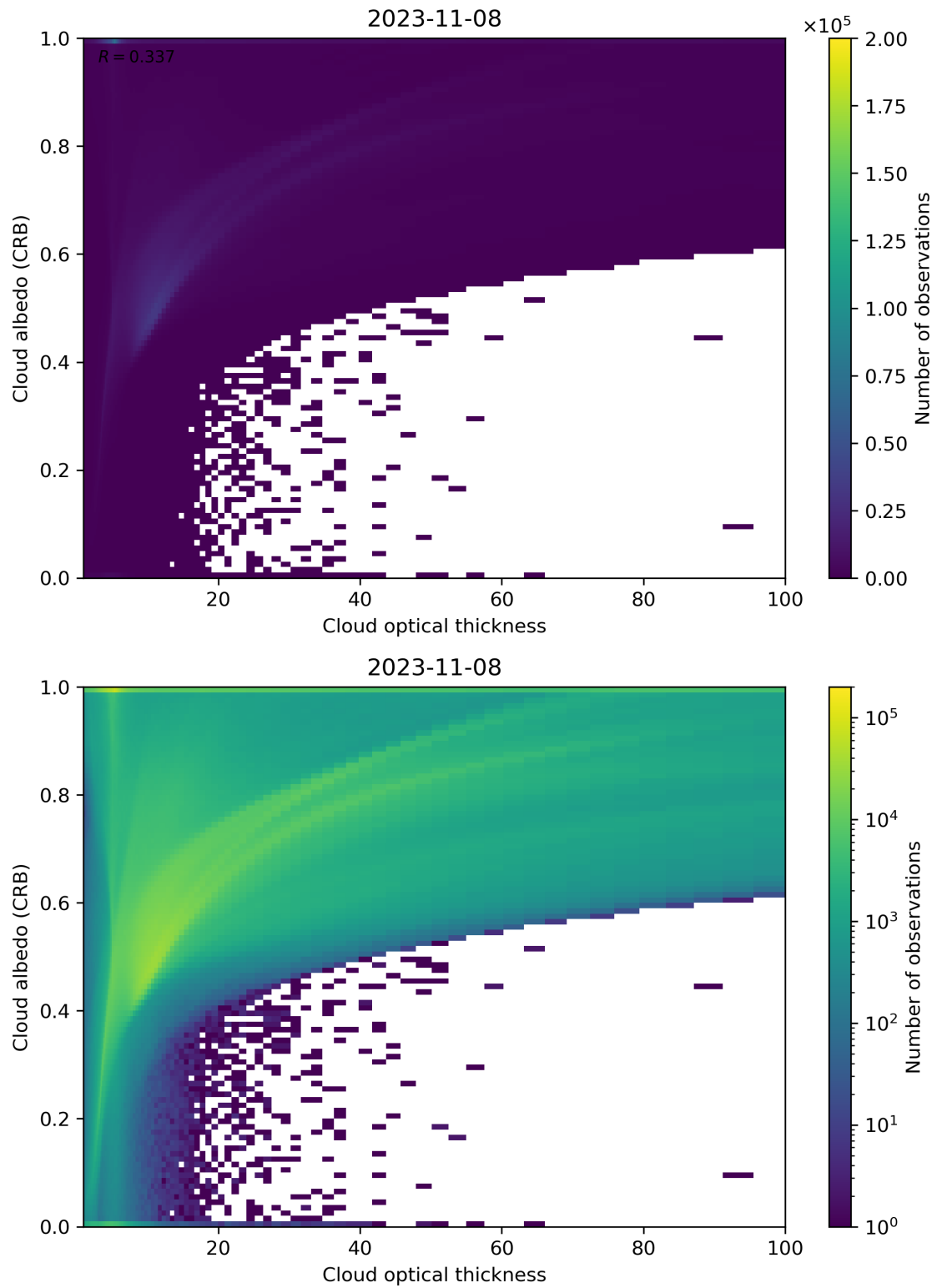
Figure 82: Scatter density plot of “Cloud optical thickness” against “Cloud albedo (CRB)” for 2023-11-07 to 2023-11-09.
