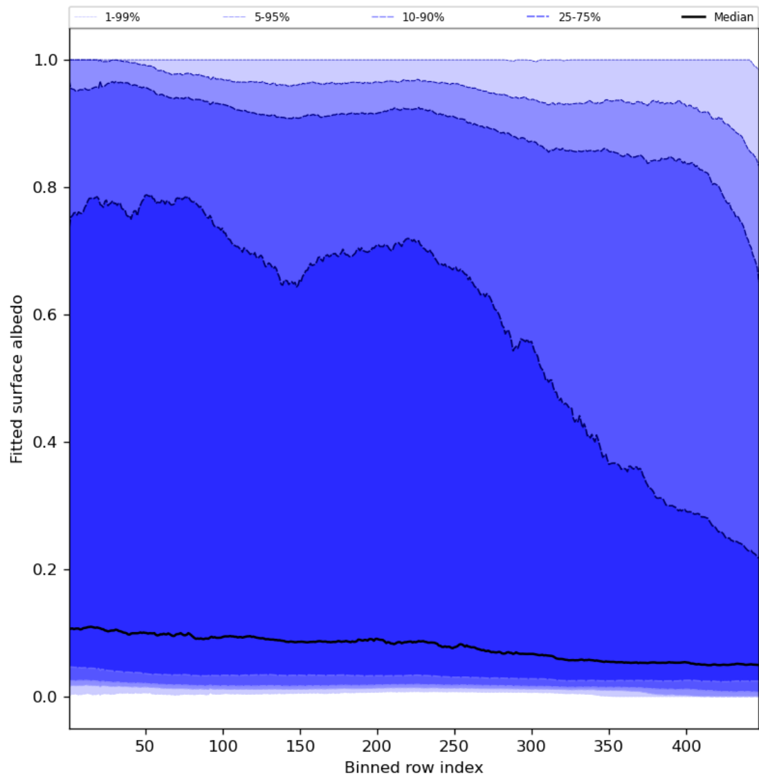
Figure 61: Along track statistics of “Fitted surface albedo” for 2023-11-07 to 2023-11-09
