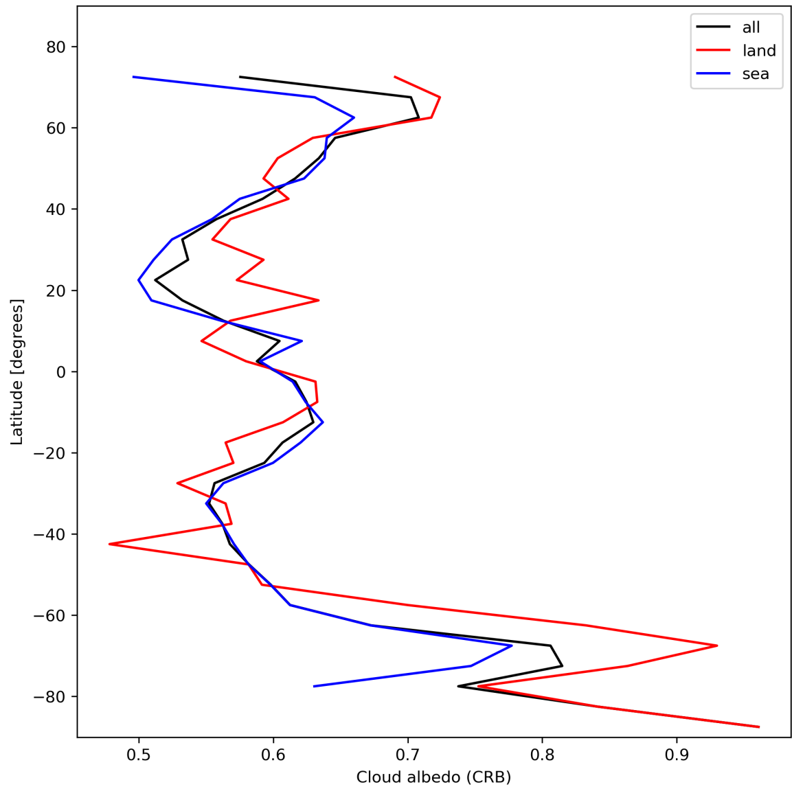
Figure 28: Zonal average of “Cloud albedo (CRB)” for 2023-11-07 to 2023-11-09.
