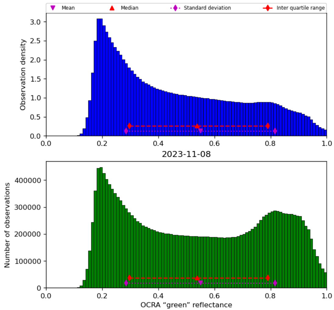
Figure 52: Histogram of “OCRA “green” reflectance” for 2023-11-07 to 2023-11-09
