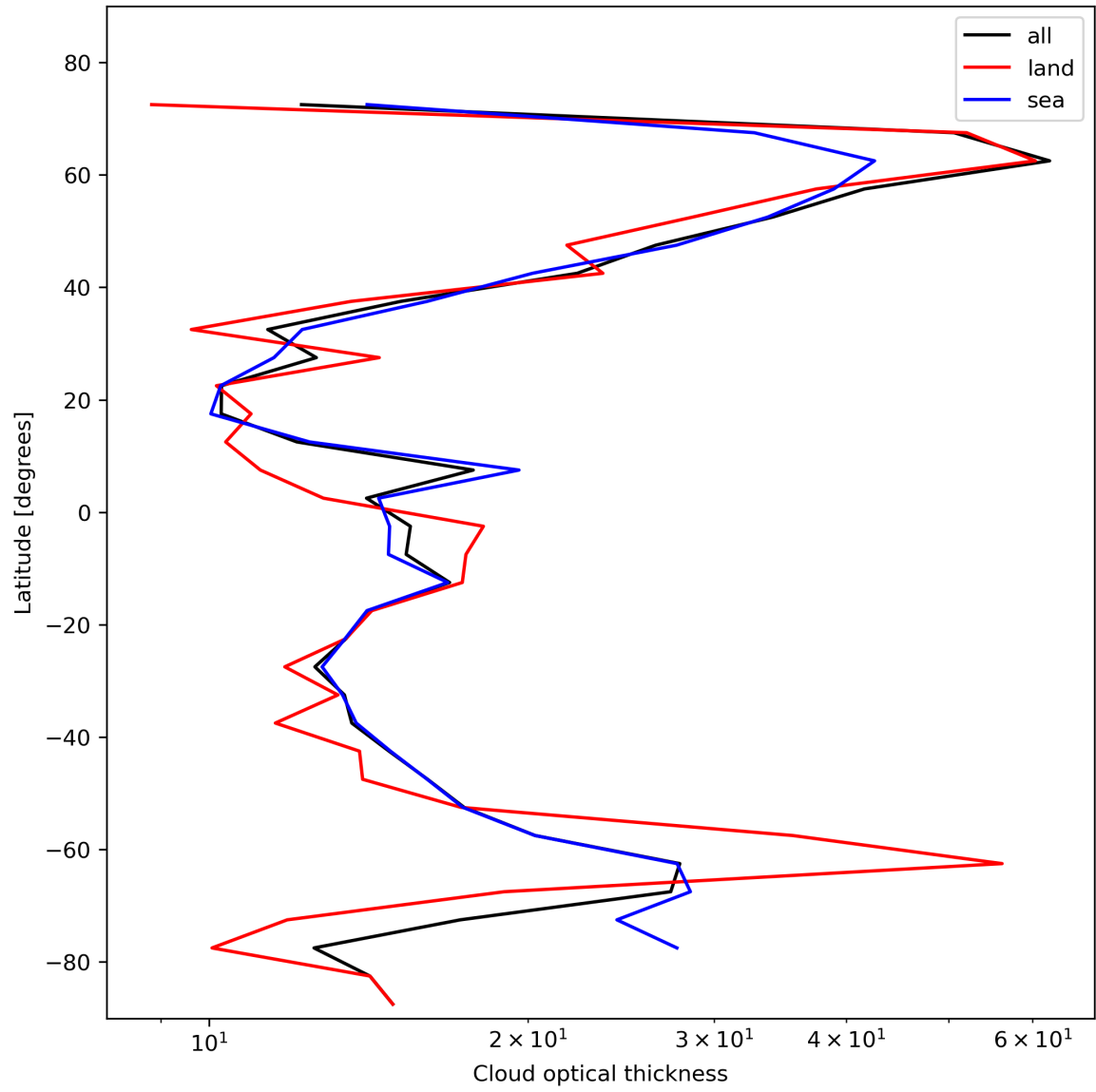
Figure 25: Zonal average of “Cloud optical thickness” for 2023-11-07 to 2023-11-09.
