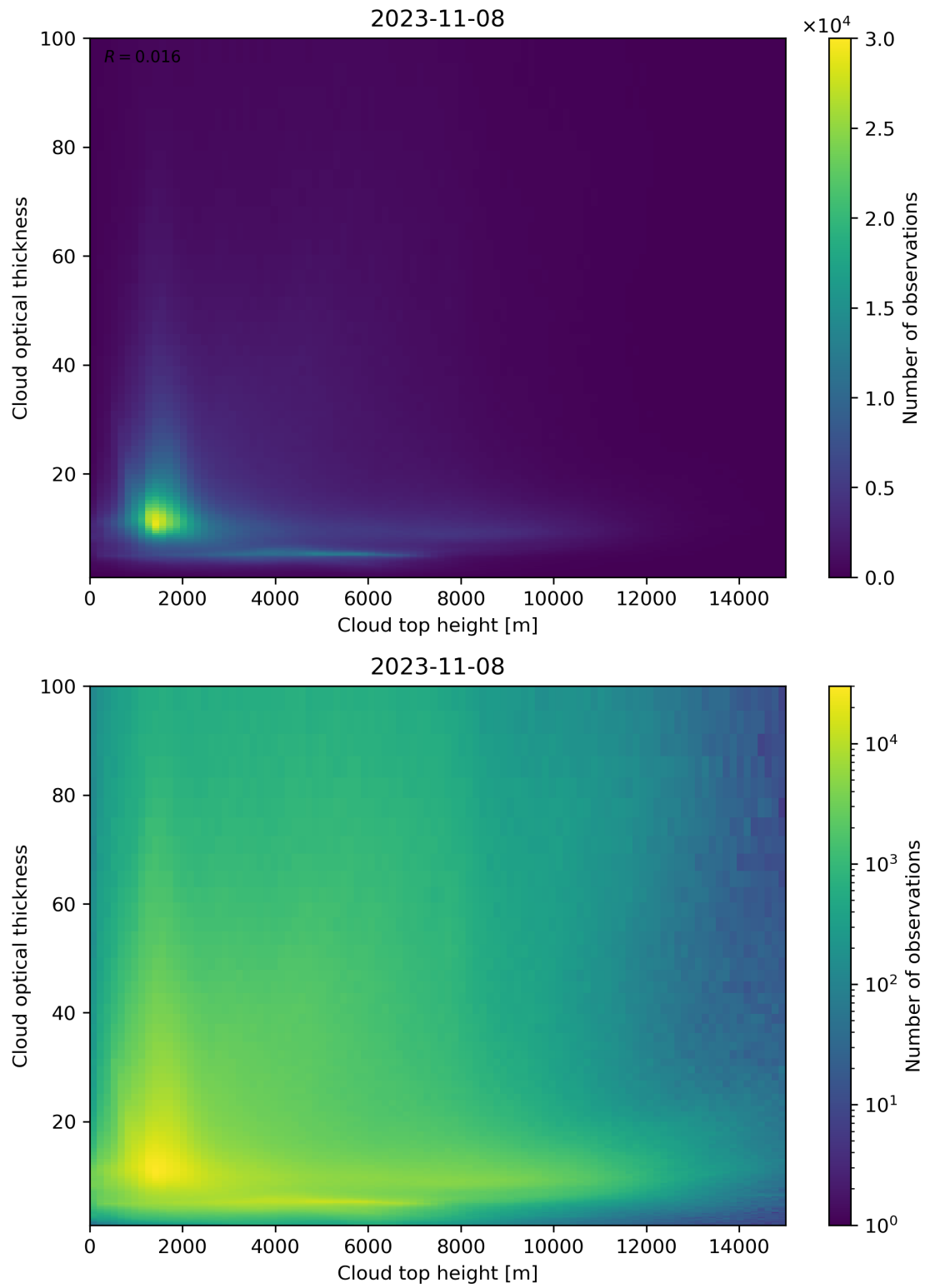
Figure 90: Scatter density plot of “Cloud top height” against “Cloud optical thickness” for 2023-11-07 to 2023-11-09.
