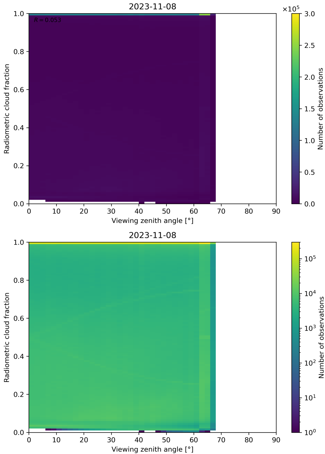
Figure 107: Scatter density plot of “Viewing zenith angle” against “Radiometric cloud fraction” for 2023-11-07 to 2023-11-09.
