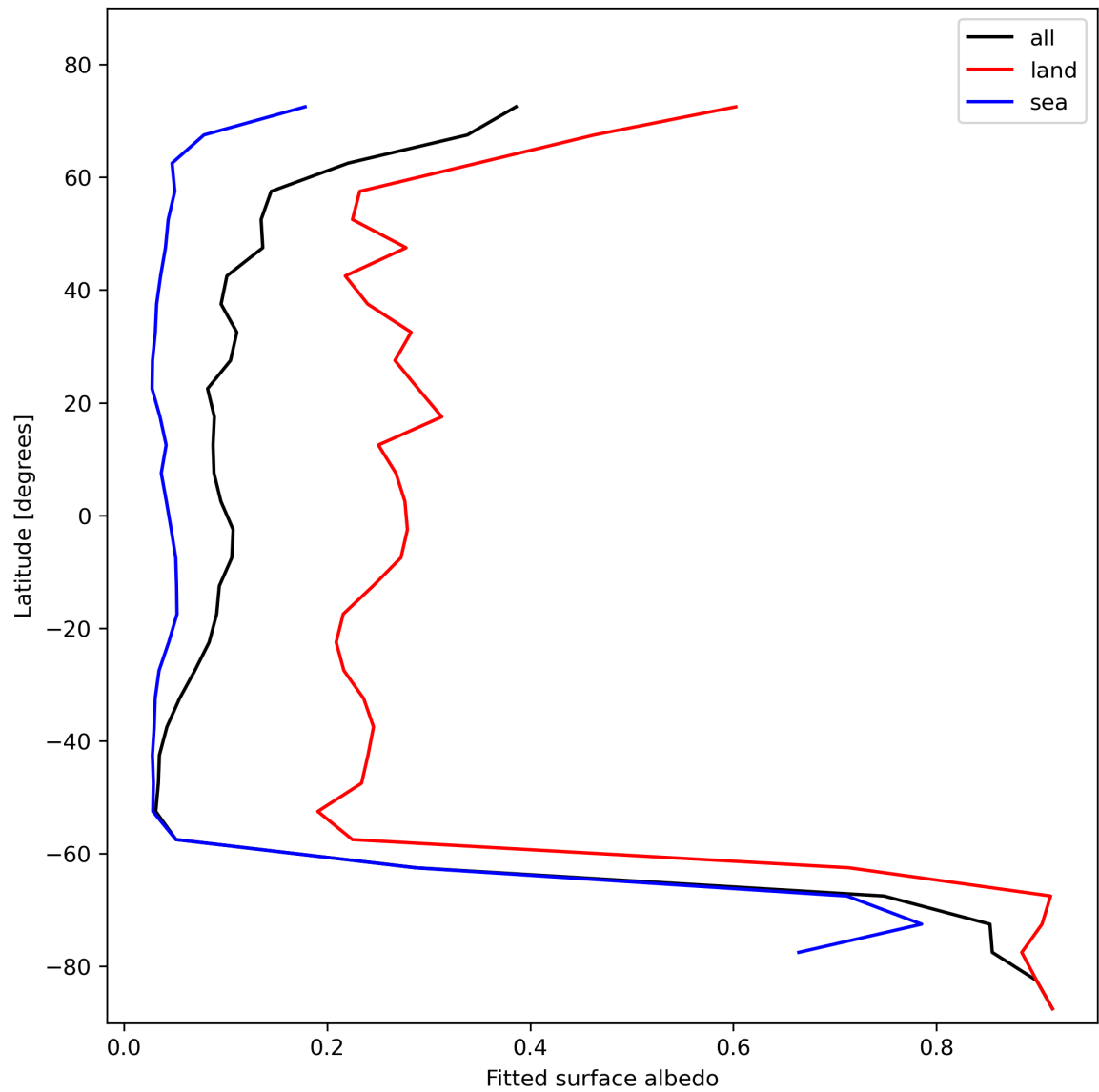
Figure 29: Zonal average of “Fitted surface albedo” for 2023-11-07 to 2023-11-09.
