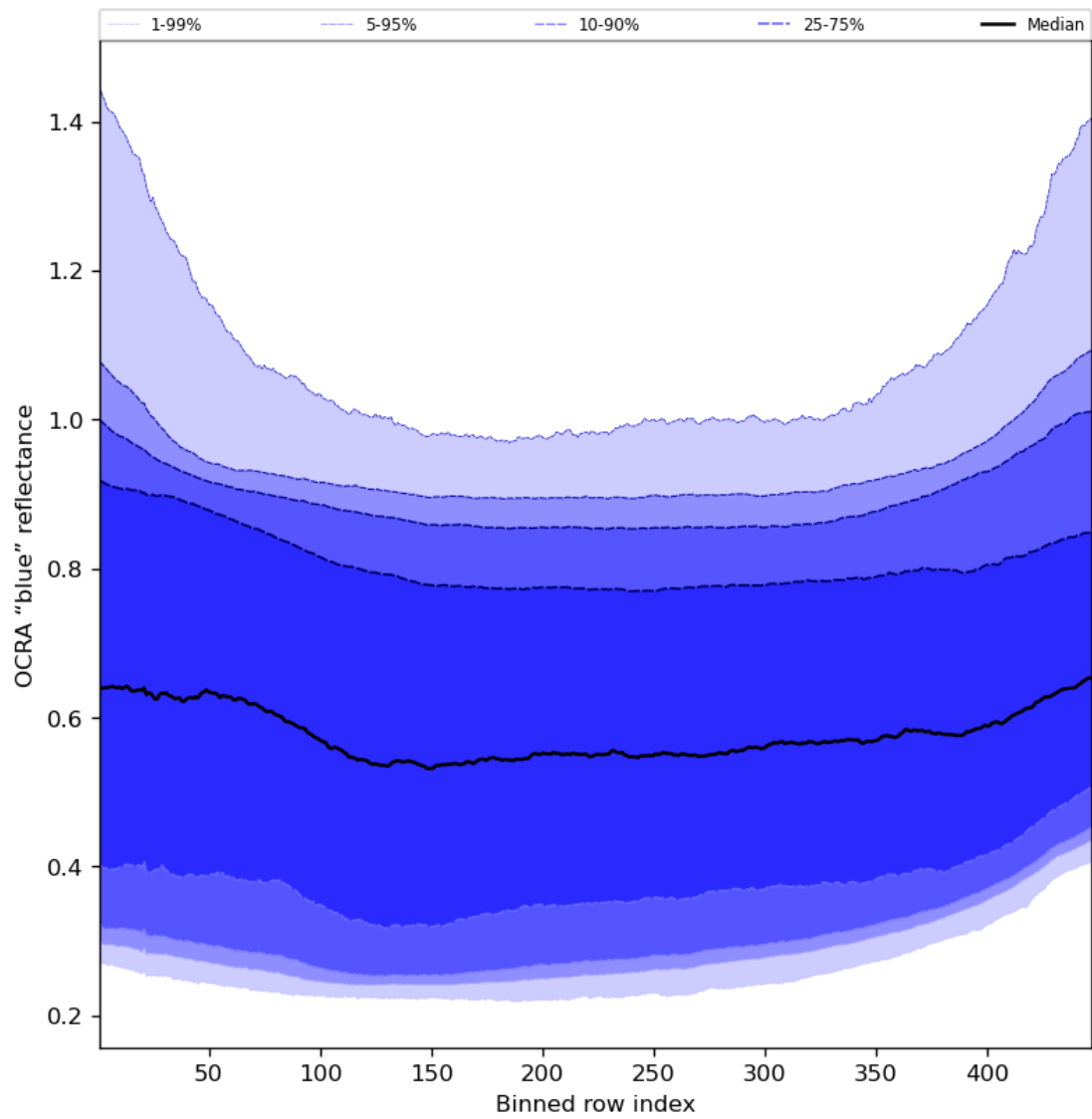
Figure 67: Along track statistics of “OCRA “blue” reflectance” for 2023-11-07 to 2023-11-09
