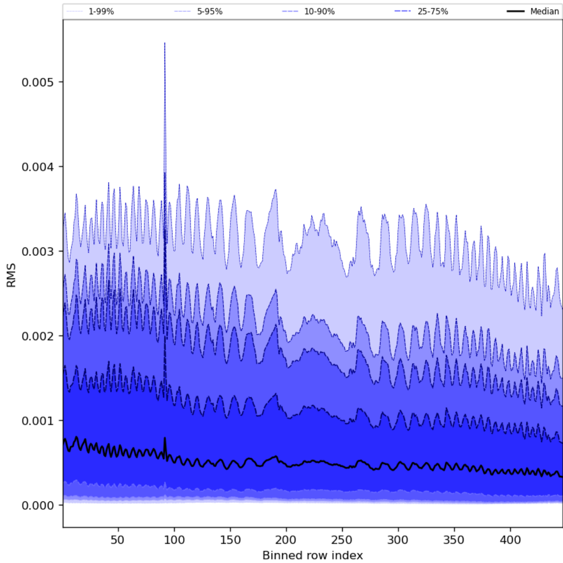
Figure 63: Along track statistics of “RMS” for 2023-11-07 to 2023-11-09
