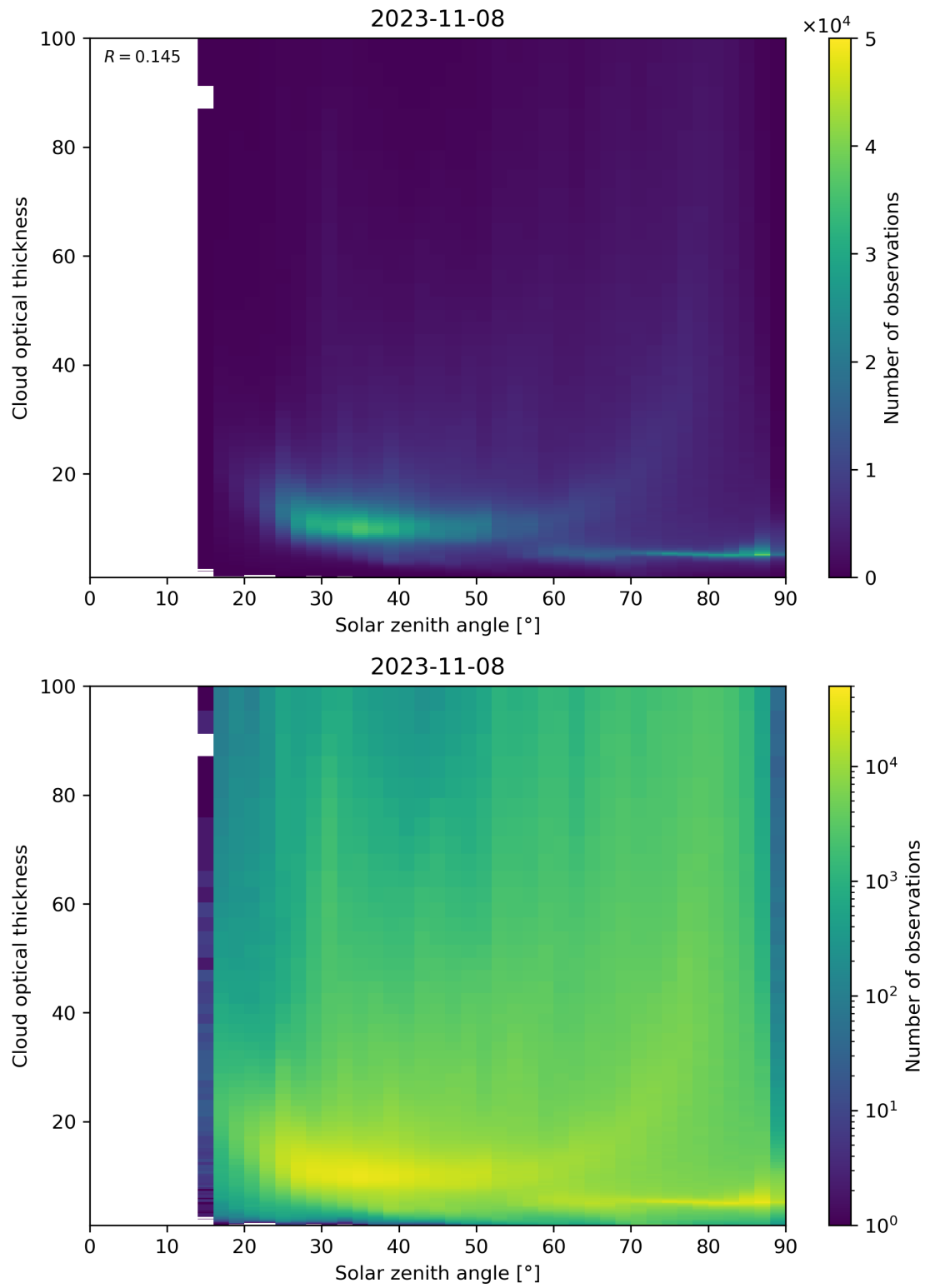
Figure 103: Scatter density plot of “Solar zenith angle” against “Cloud optical thickness” for 2023-11-07 to 2023-11-09.
