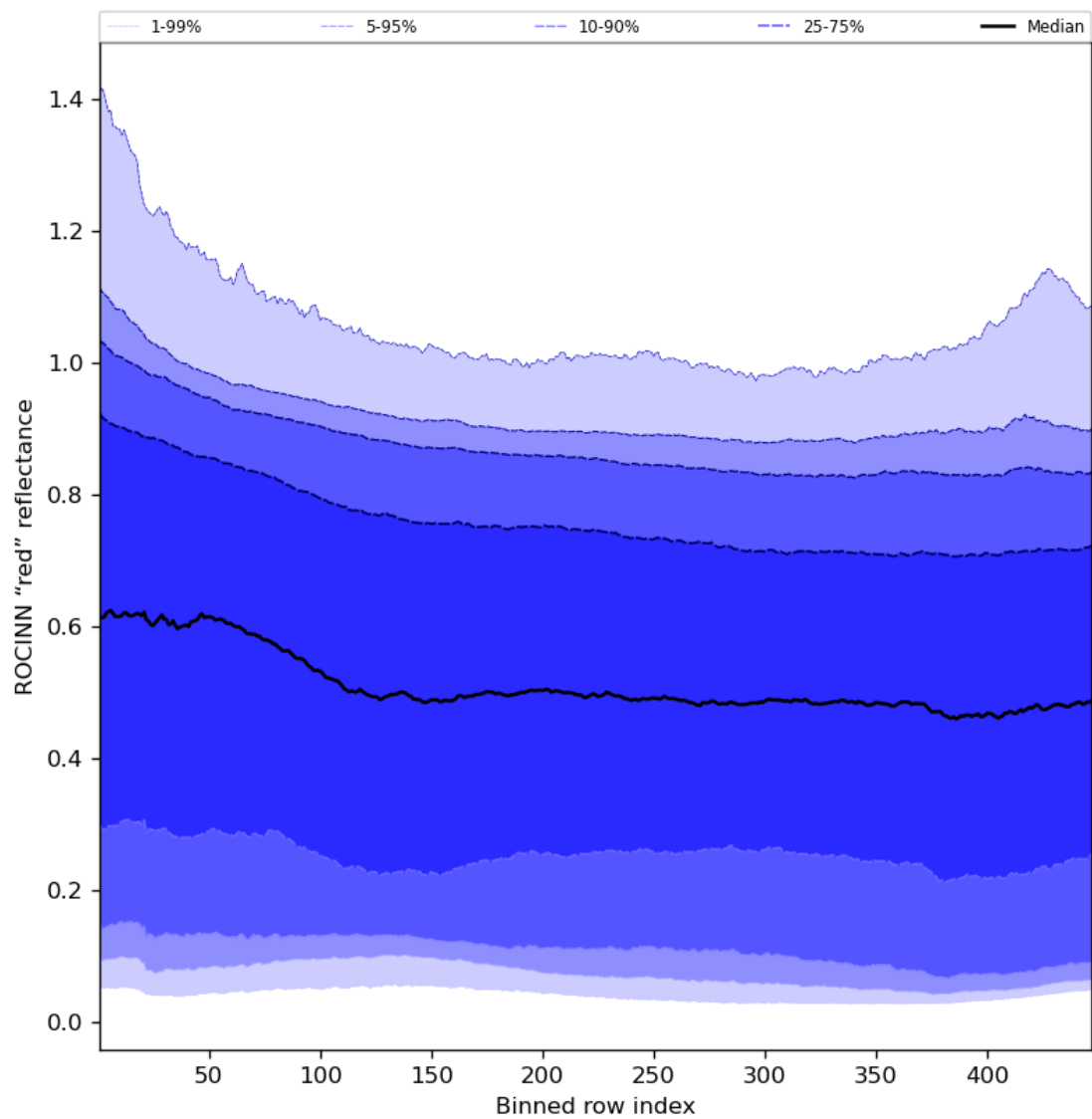
Figure 69: Along track statistics of “ROCINN “red” reflectance” for 2023-11-07 to 2023-11-09
