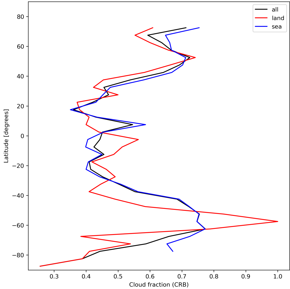
Figure 26: Zonal average of “Cloud fraction (CRB)” for 2023-11-07 to 2023-11-09.
