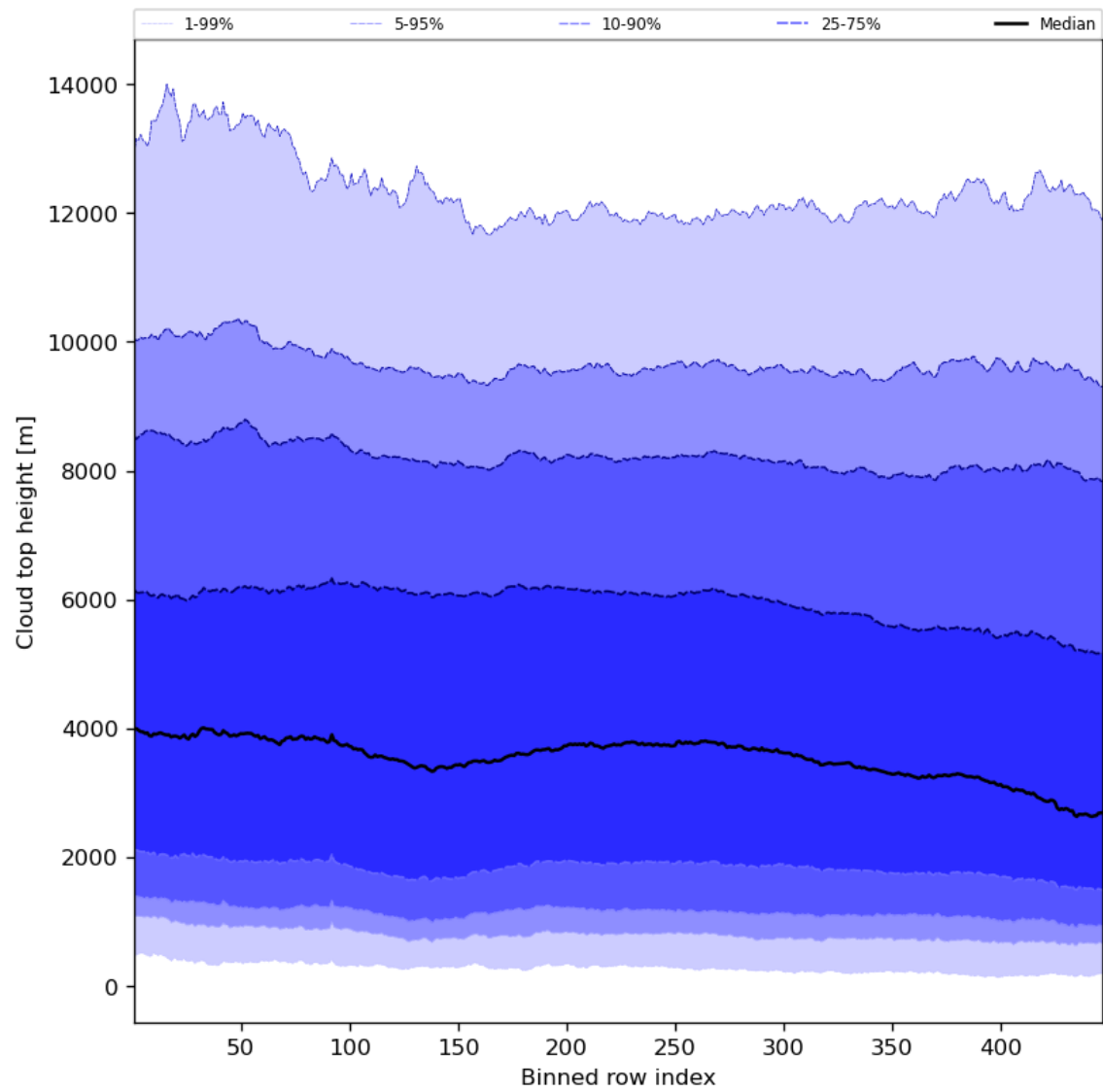
Figure 56: Along track statistics of “Cloud top height” for 2023-11-07 to 2023-11-09
