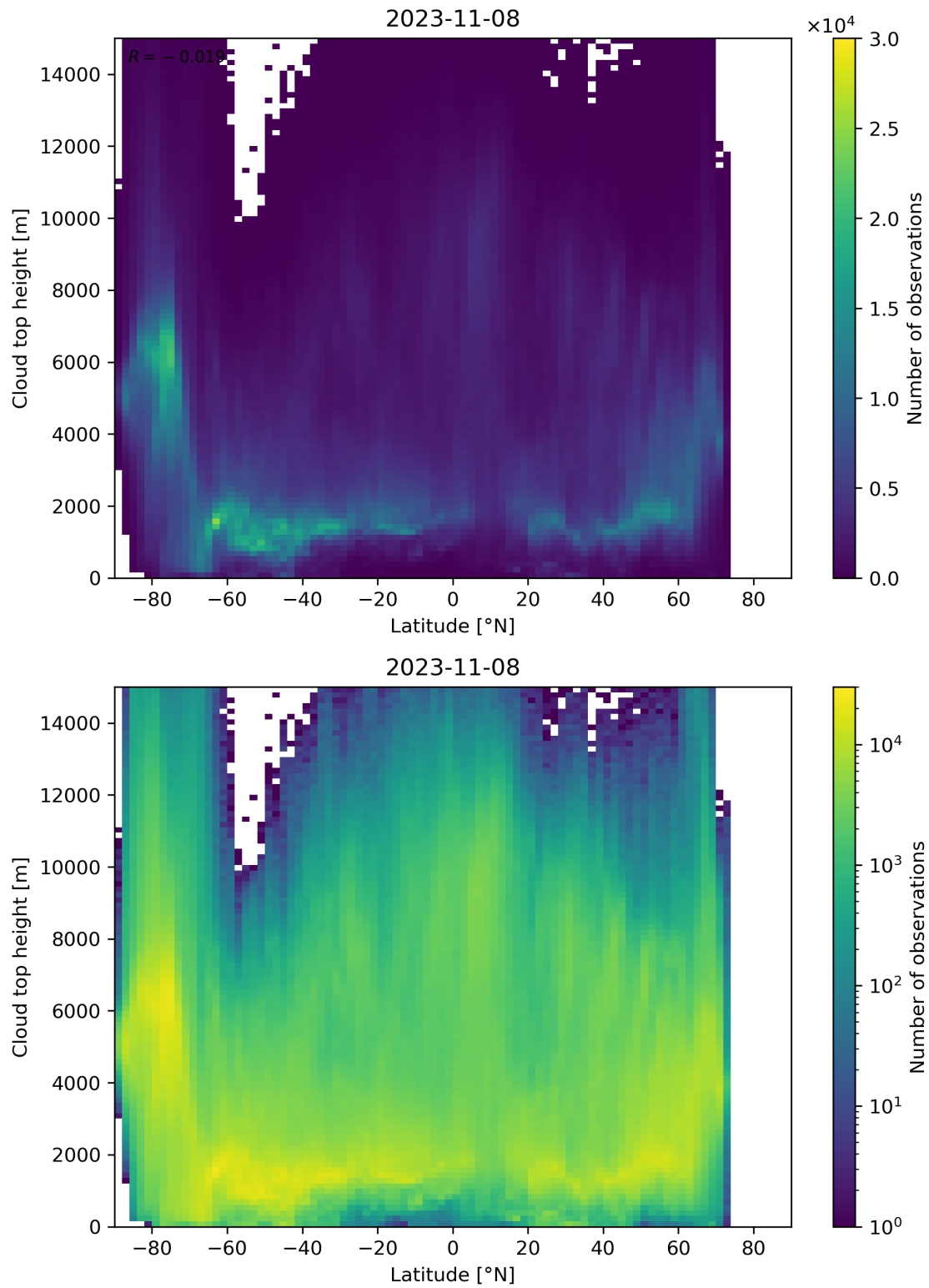
Figure 97: Scatter density plot of “Latitude” against “Cloud top height” for 2023-11-07 to 2023-11-09.
