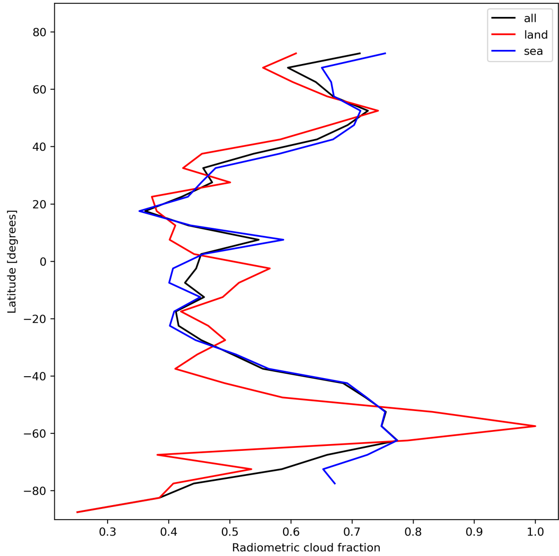
Figure 23: Zonal average of “Radiometric cloud fraction” for 2023-11-07 to 2023-11-09.
