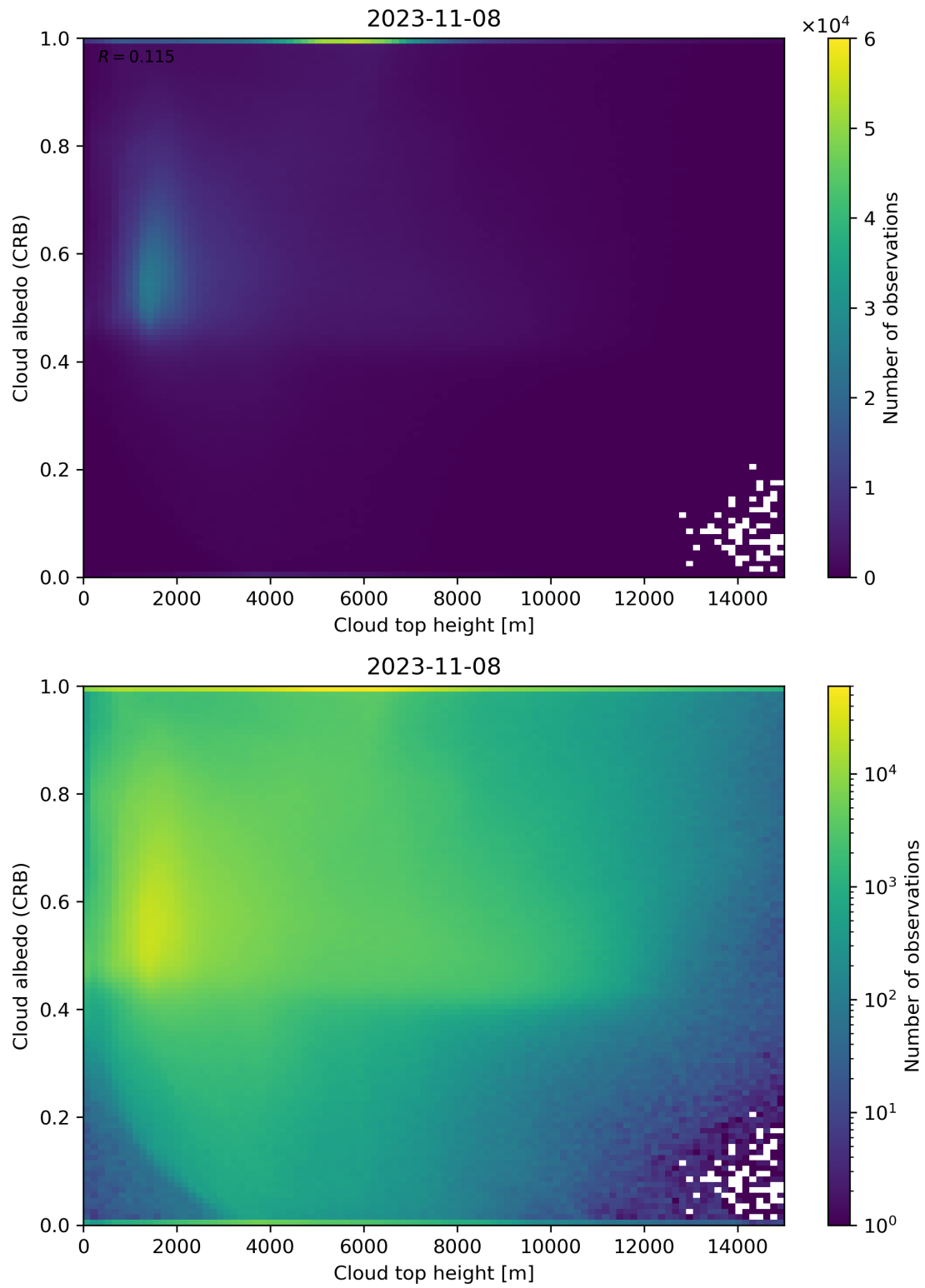
Figure 86: Scatter density plot of “Cloud top height” against “Cloud albedo (CRB)” for 2023-11-07 to 2023-11-09.
