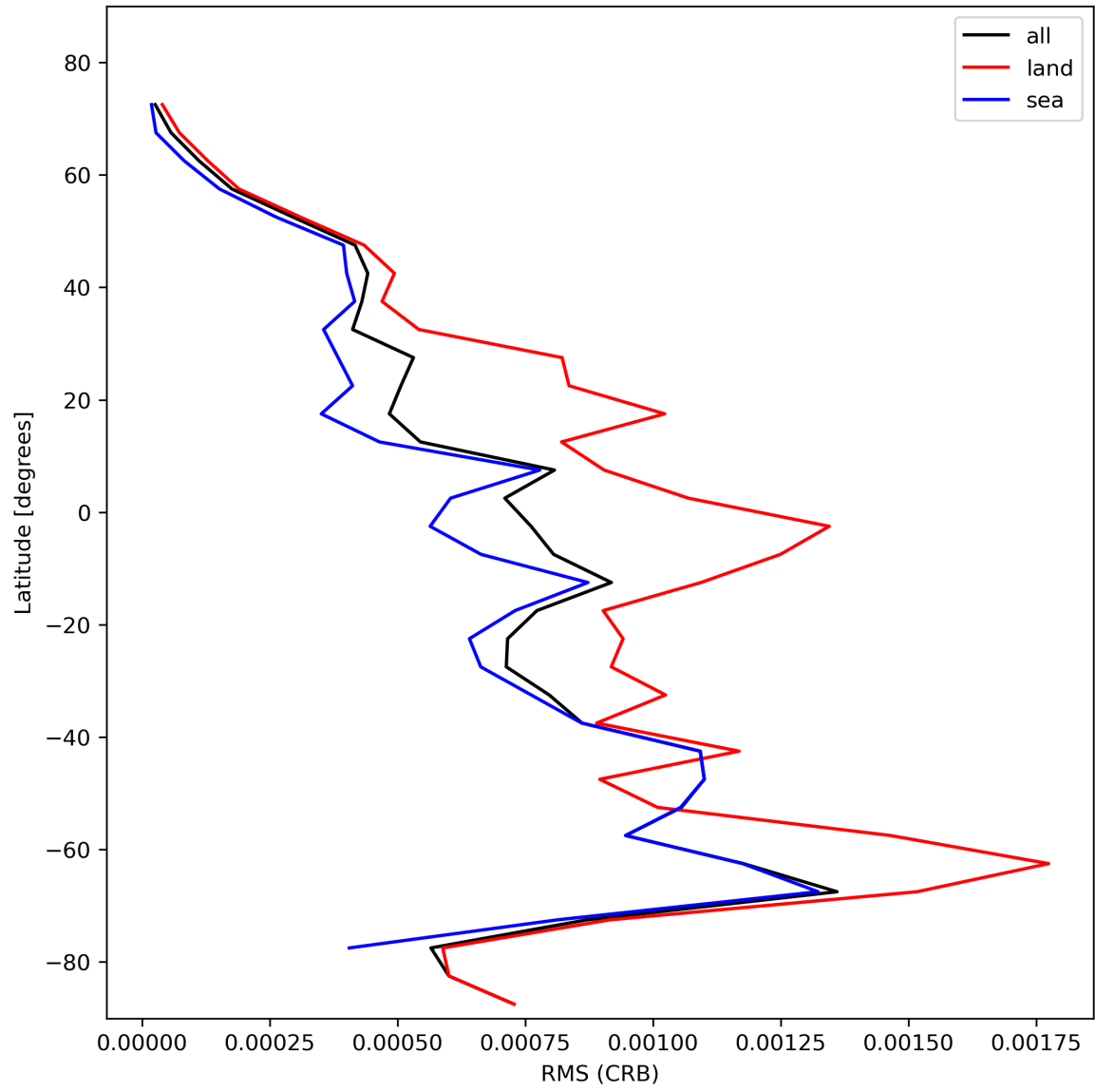
Figure 32: Zonal average of “RMS (CRB)” for 2023-11-07 to 2023-11-09.
