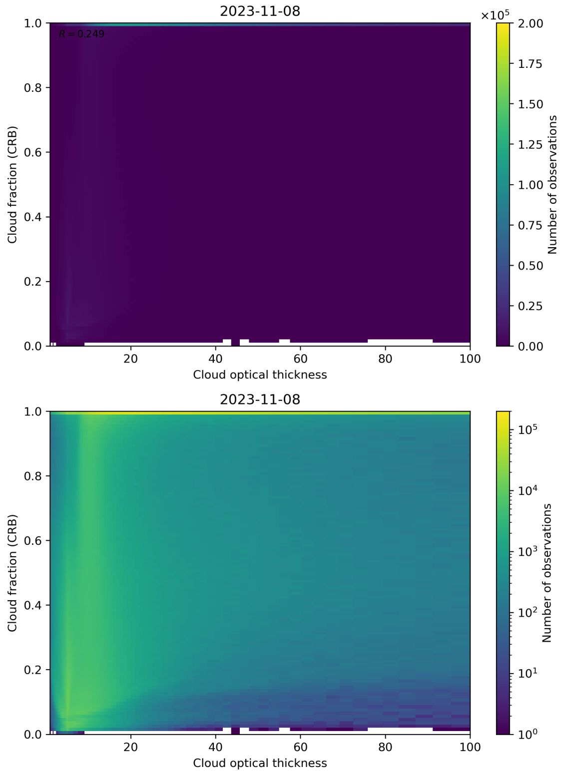
Figure 84: Scatter density plot of “Cloud optical thickness” against “Cloud fraction (CRB)” for 2023-11-07 to 2023-11-09.
