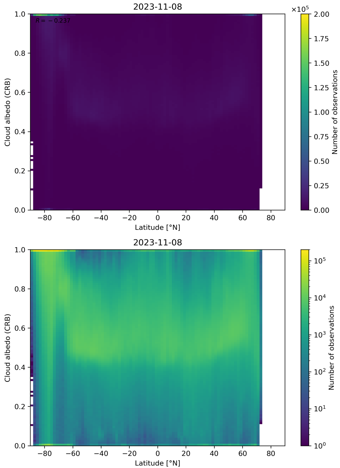
Figure 91: Scatter density plot of “Latitude” against “Cloud albedo (CRB)” for 2023-11-07 to 2023-11-09.
