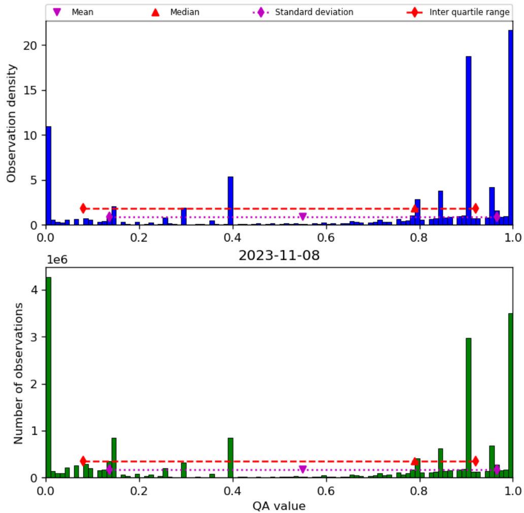
Figure 38: Histogram of “QA value” for 2023-11-07 to 2023-11-09
