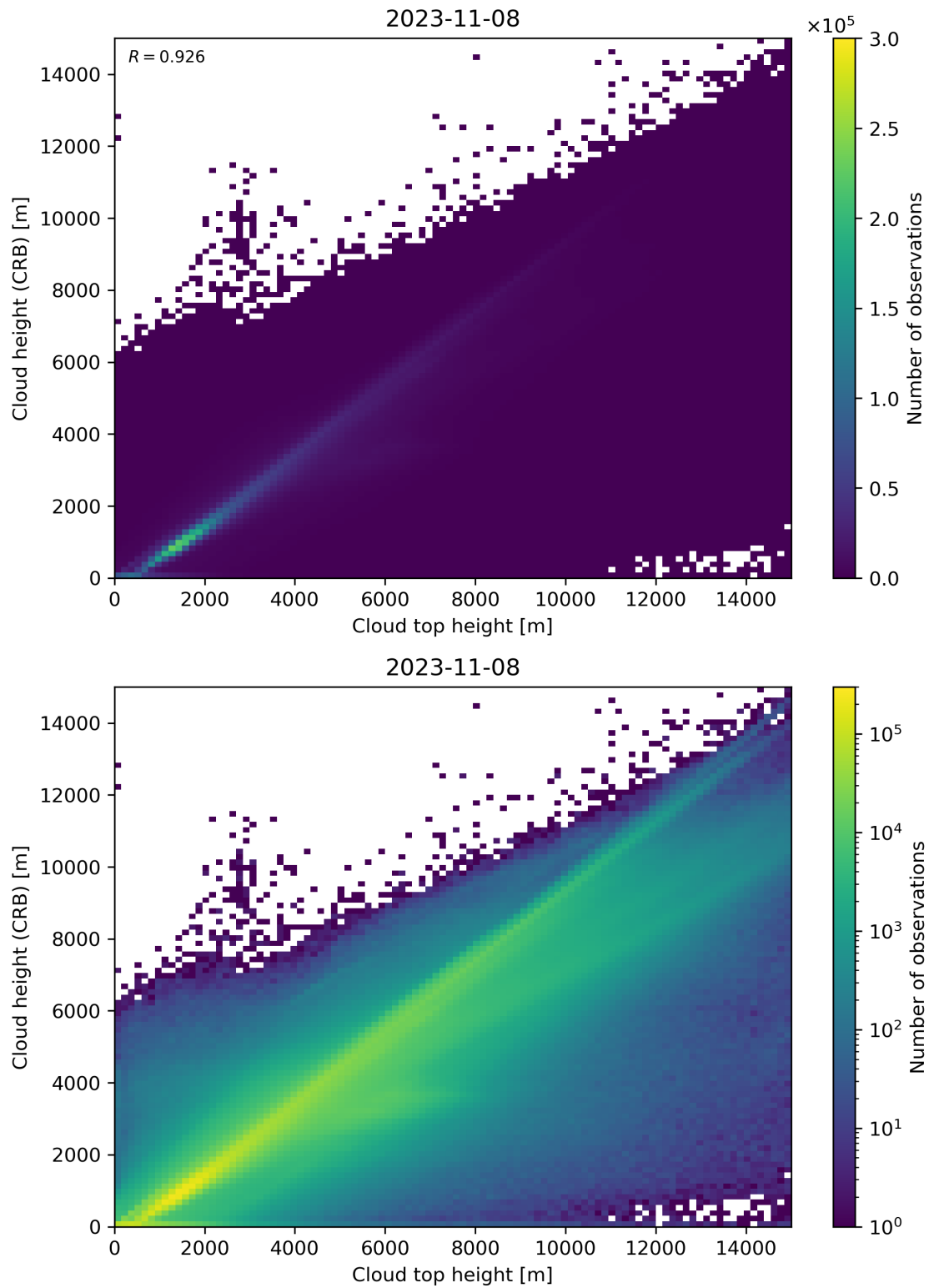
Figure 89: Scatter density plot of “Cloud top height” against “Cloud height (CRB)” for 2023-11-07 to 2023-11-09.
