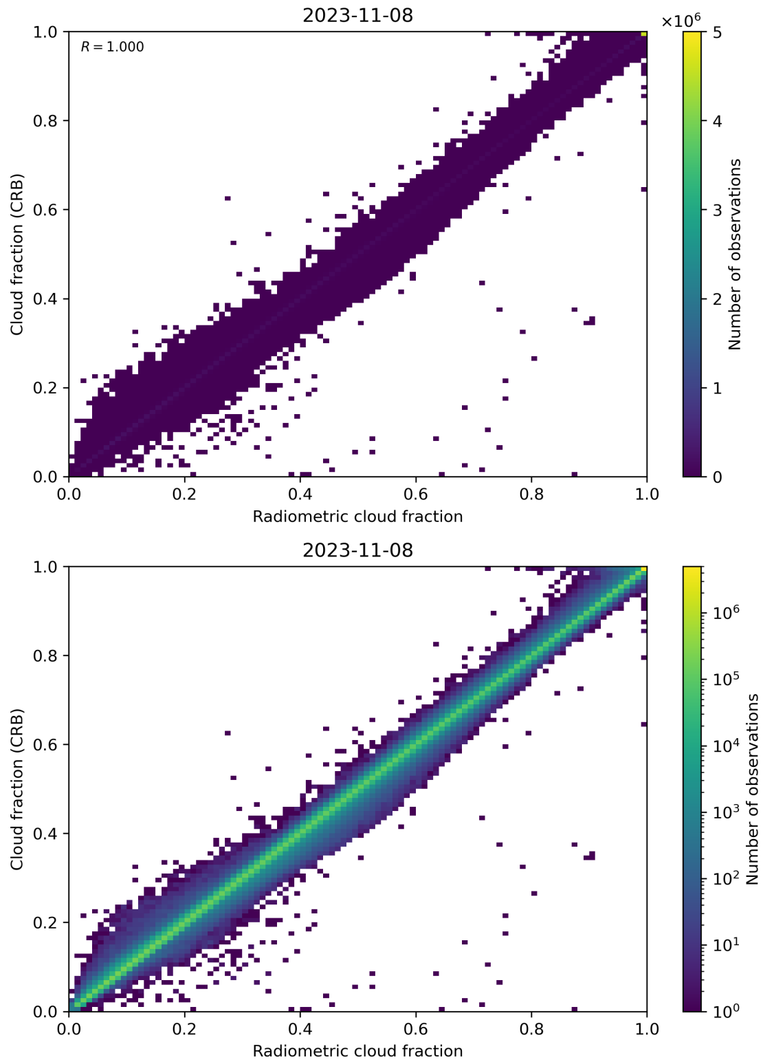
Figure 73: Scatter density plot of “Radiometric cloud fraction” against “Cloud fraction (CRB)” for 2023-11-07 to 2023-11-09.
