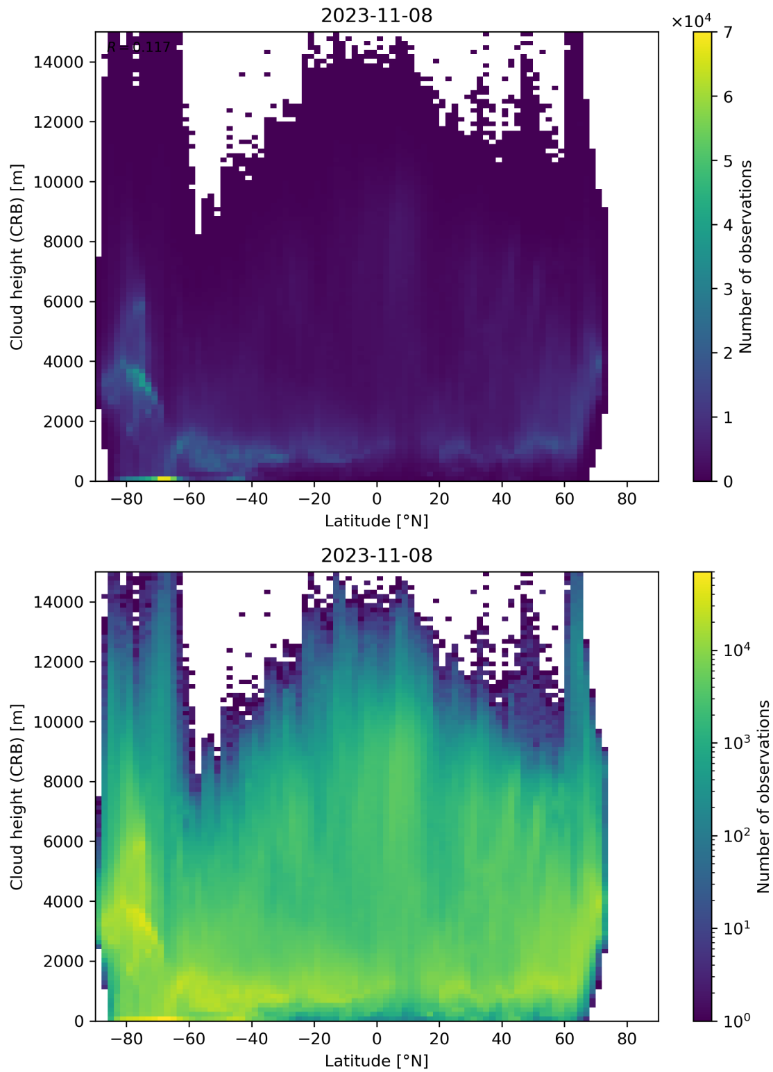
Figure 95: Scatter density plot of “Latitude” against “Cloud height (CRB)” for 2023-11-07 to 2023-11-09.
