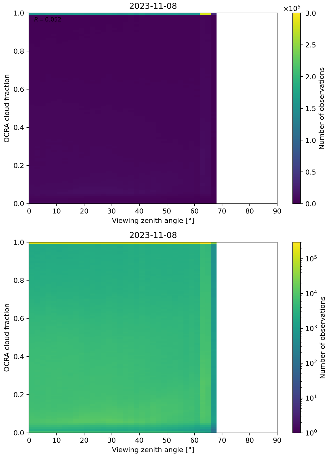
Figure 108: Scatter density plot of “Viewing zenith angle” against “OCRA cloud fraction” for 2023-11-07 to 2023-11-09.
