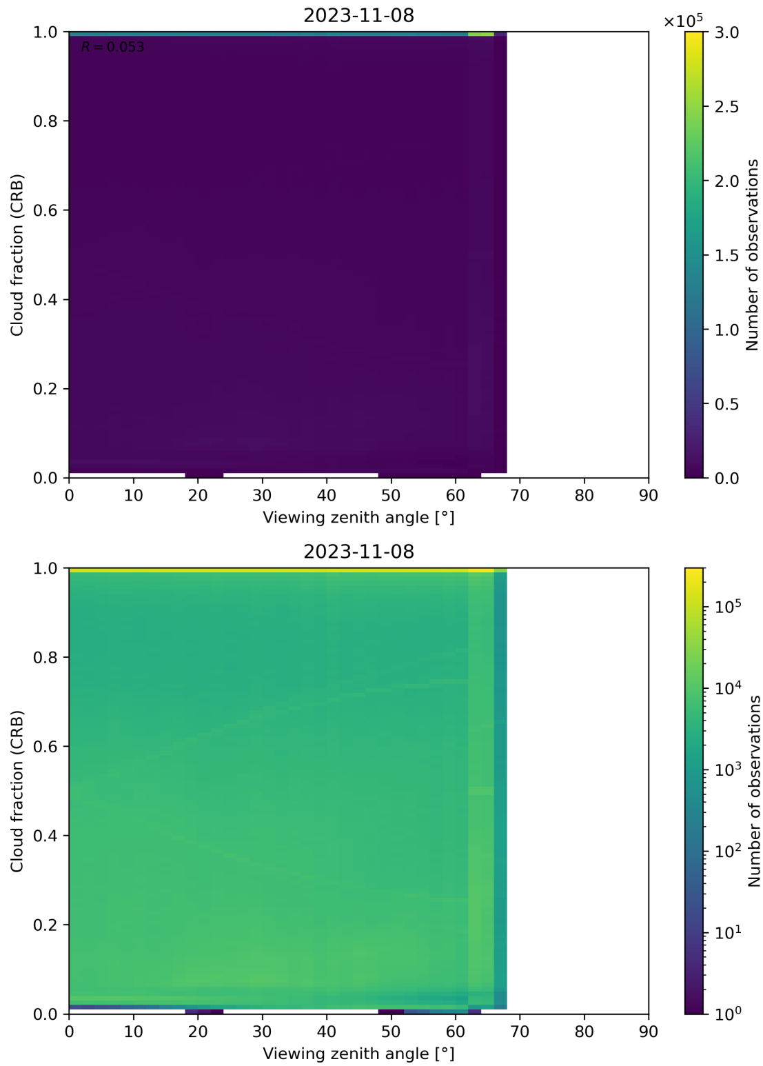
Figure 109: Scatter density plot of “Viewing zenith angle” against “Cloud fraction (CRB)” for 2023-11-07 to 2023-11-09.
