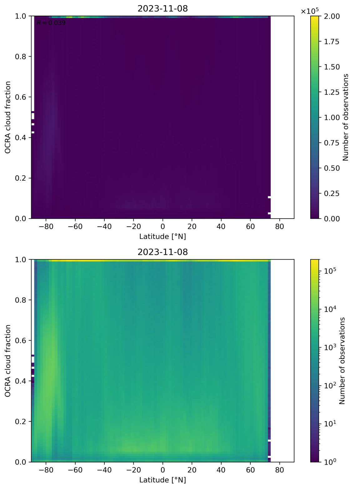
Figure 93: Scatter density plot of “Latitude” against “OCRA cloud fraction” for 2023-11-07 to 2023-11-09.
