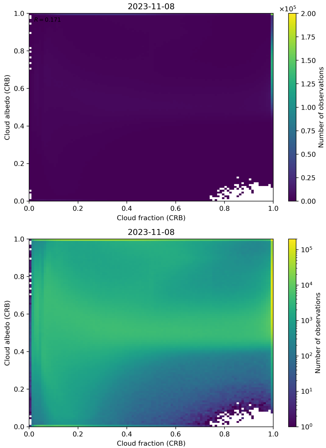
Figure 77: Scatter density plot of “Cloud fraction (CRB)” against “Cloud albedo (CRB)” for 2023-11-07 to 2023-11-09.
