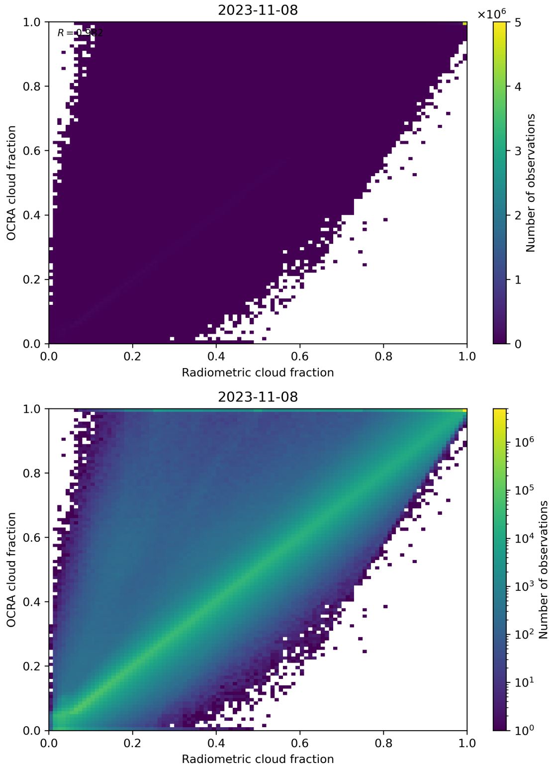
Figure 72: Scatter density plot of “Radiometric cloud fraction” against “OCRA cloud fraction” for 2023-11-07 to 2023-11-09.
