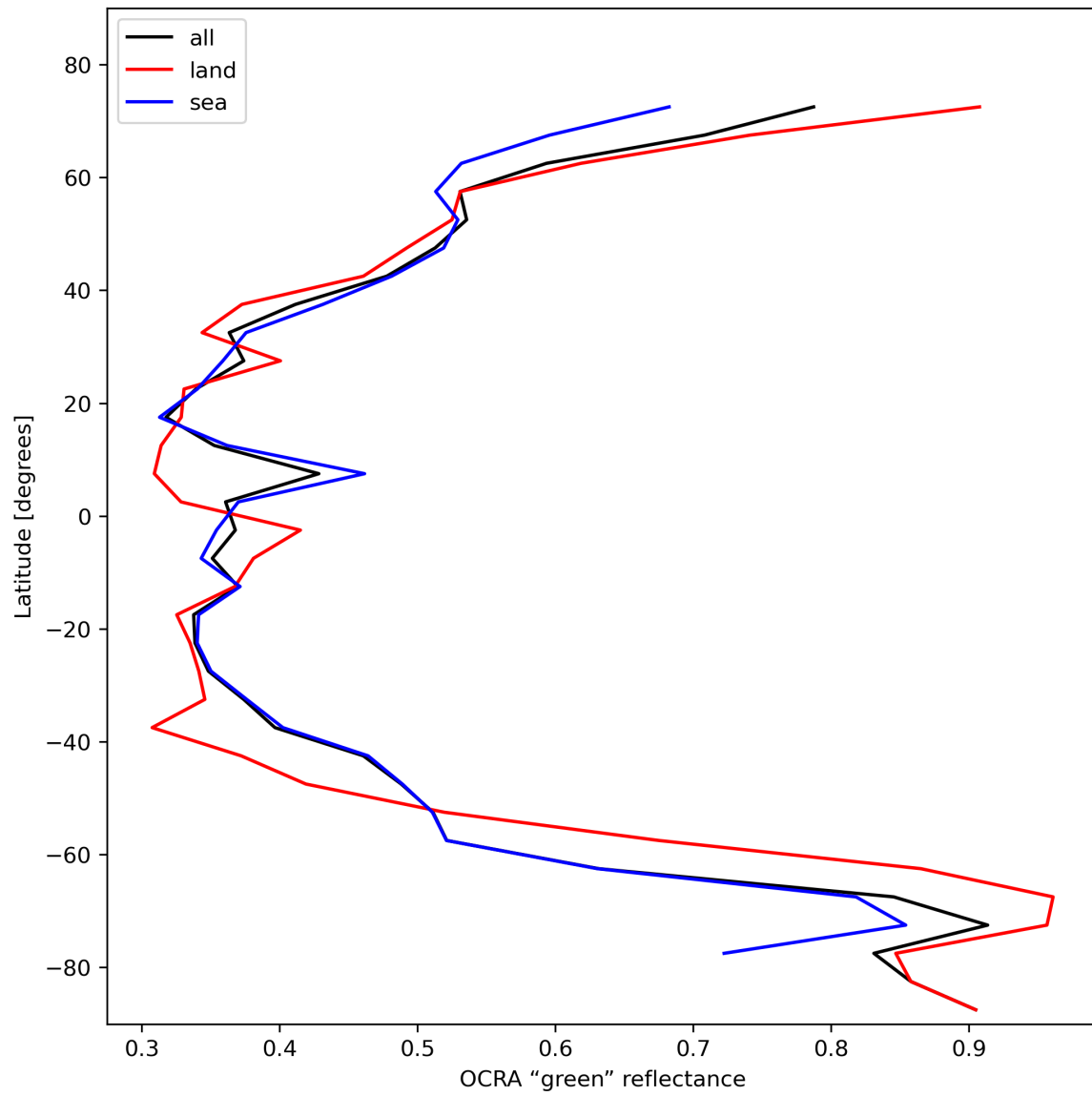
Figure 36: Zonal average of “OCRA “green” reflectance” for 2023-11-07 to 2023-11-09.
