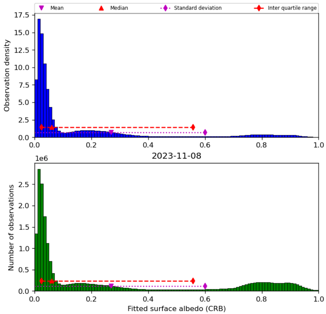
Figure 46: Histogram of “Fitted surface albedo (CRB)” for 2023-11-07 to 2023-11-09
