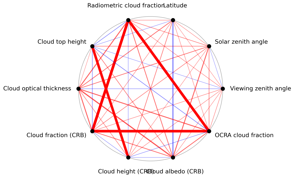
Figure 1: Map of correlation graph for 2023-11-07 to 2023-11-09.
