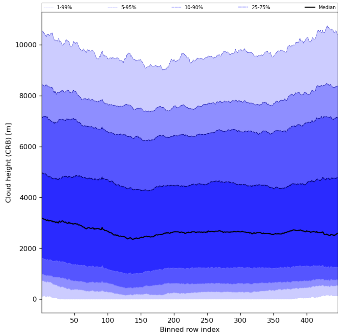
Figure 59: Along track statistics of “Cloud height (CRB)” for 2023-11-07 to 2023-11-09
