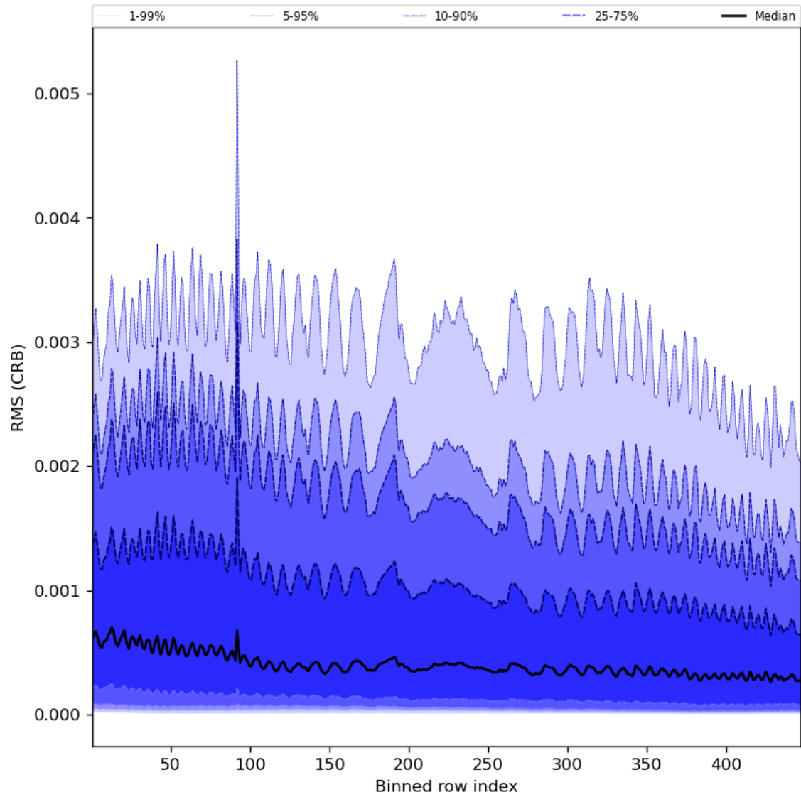
Figure 64: Along track statistics of “RMS (CRB)” for 2023-11-07 to 2023-11-09
