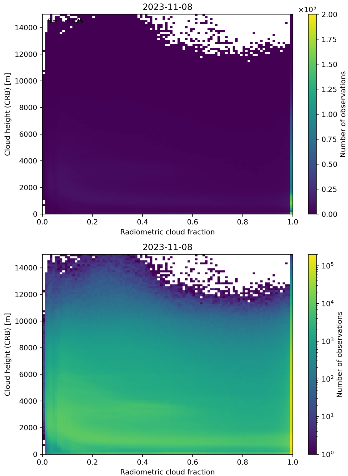
Figure 74: Scatter density plot of “Radiometric cloud fraction” against “Cloud height (CRB)” for 2023-11-07 to 2023-11-09.
