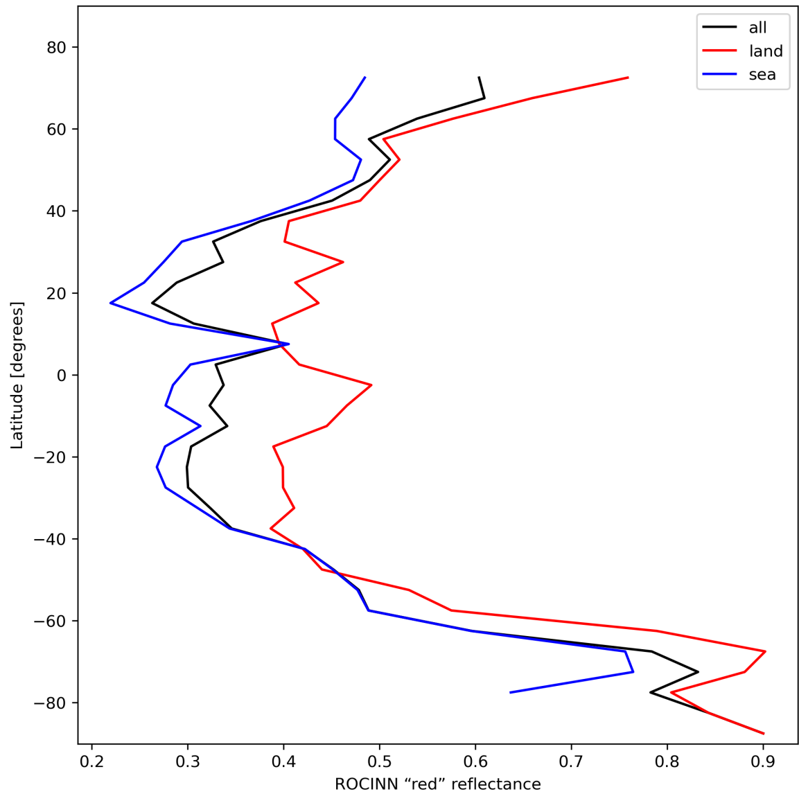
Figure 37: Zonal average of “ROCINN “red” reflectance” for 2023-11-07 to 2023-11-09.
