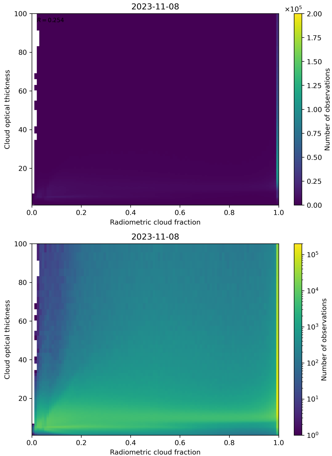
Figure 75: Scatter density plot of “Radiometric cloud fraction” against “Cloud optical thickness” for 2023-11-07 to 2023-11-09.
