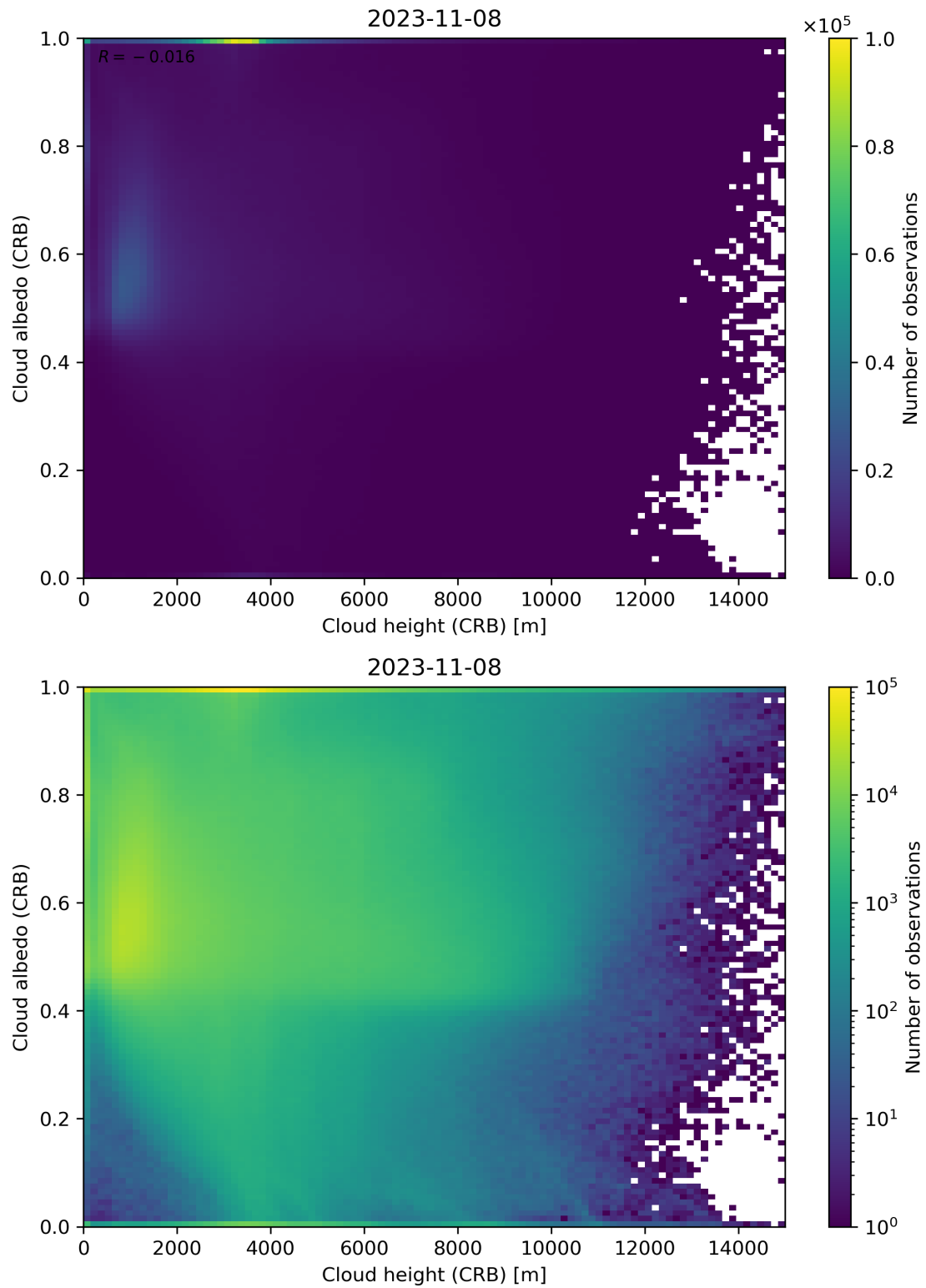
Figure 80: Scatter density plot of “Cloud height (CRB)” against “Cloud albedo (CRB)” for 2023-11-07 to 2023-11-09.
