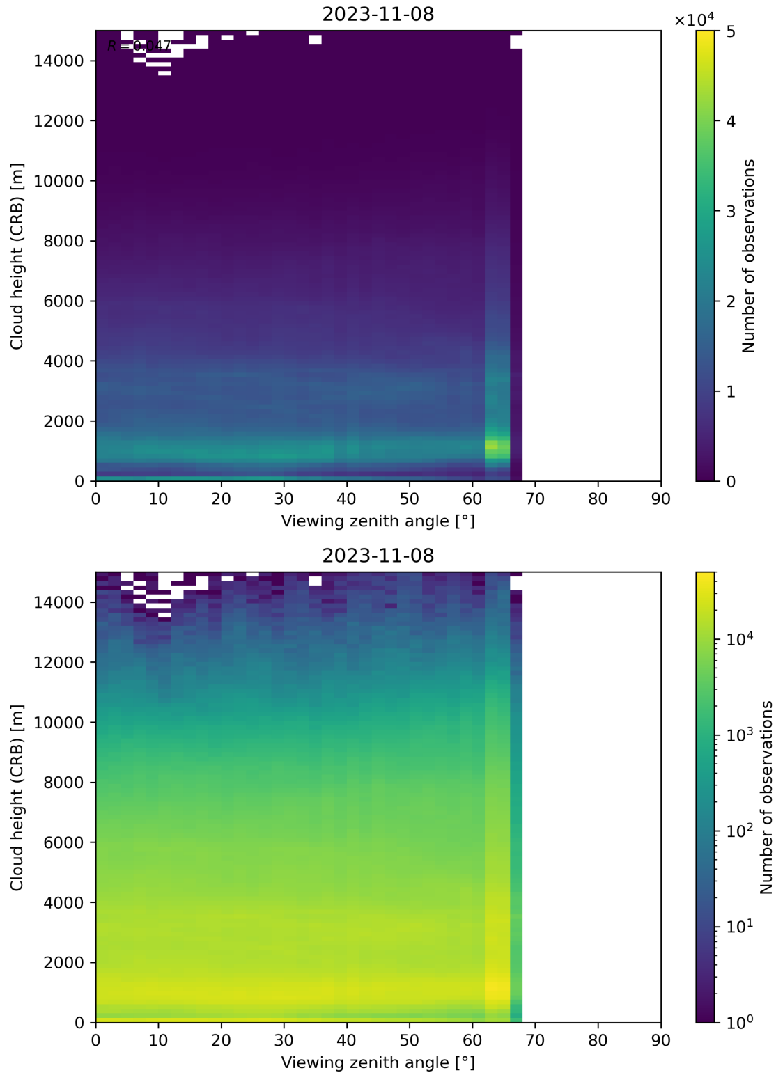
Figure 110: Scatter density plot of “Viewing zenith angle” against “Cloud height (CRB)” for 2023-11-07 to 2023-11-09.
