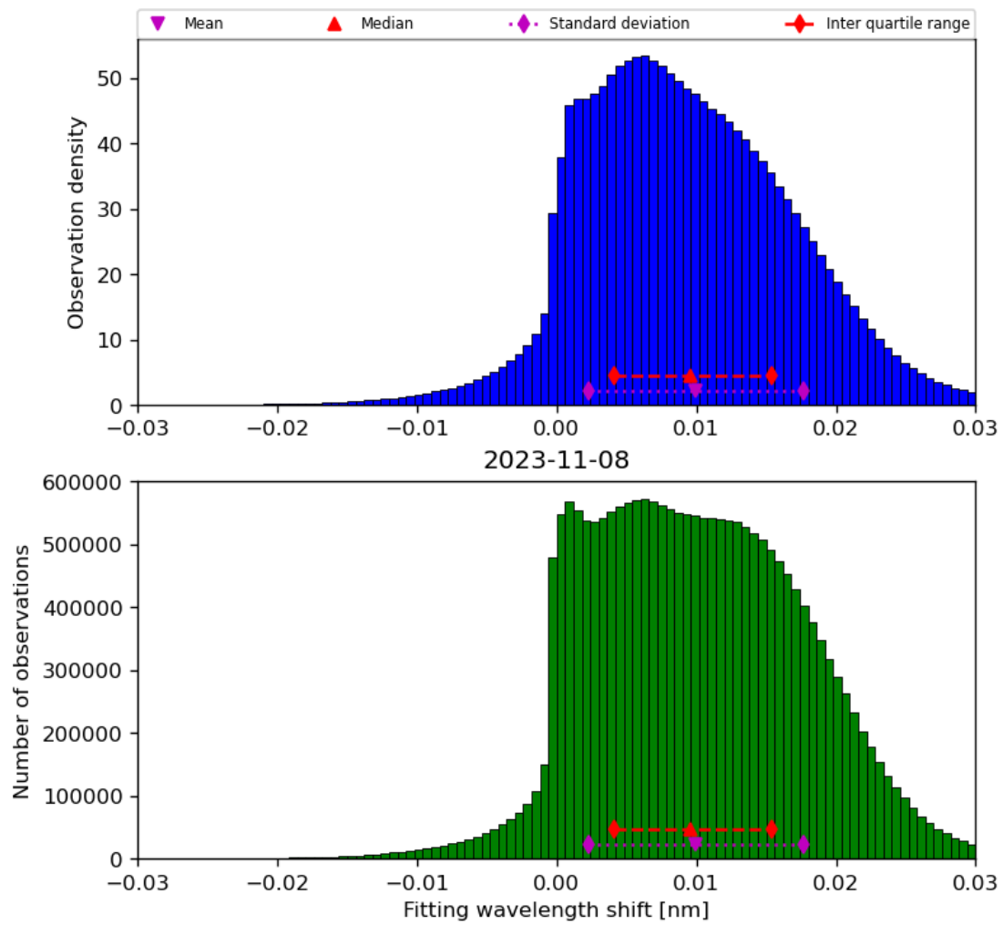
Figure 49: Histogram of “Fitting wavelength shift” for 2023-11-07 to 2023-11-09
