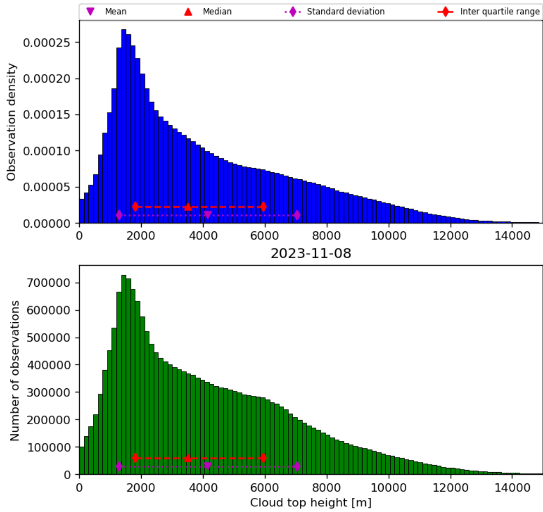
Figure 40: Histogram of “Cloud top height” for 2023-11-07 to 2023-11-09
