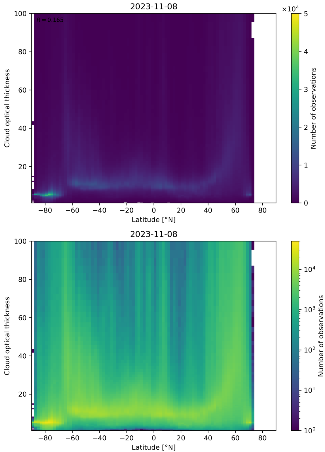
Figure 96: Scatter density plot of “Latitude” against “Cloud optical thickness” for 2023-11-07 to 2023-11-09.
