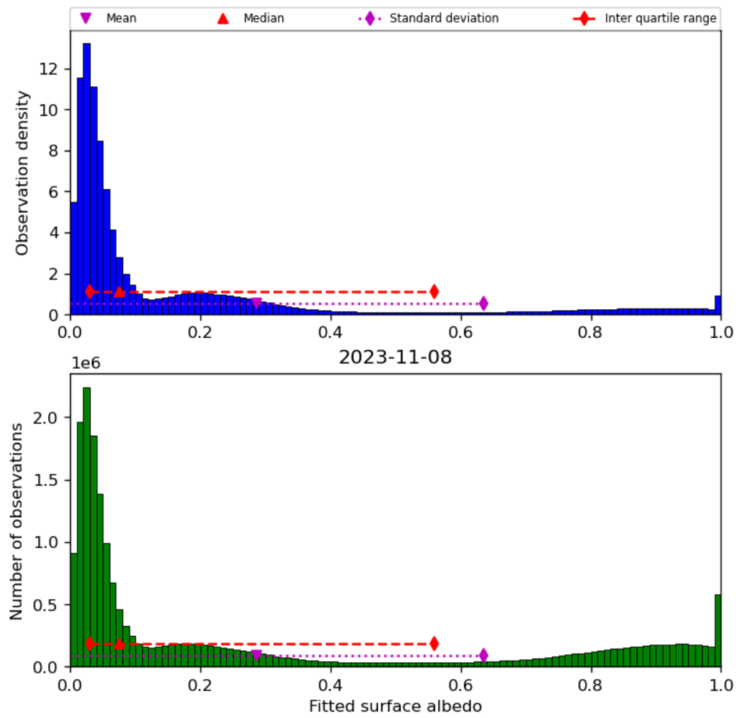
Figure 45: Histogram of “Fitted surface albedo” for 2023-11-07 to 2023-11-09
