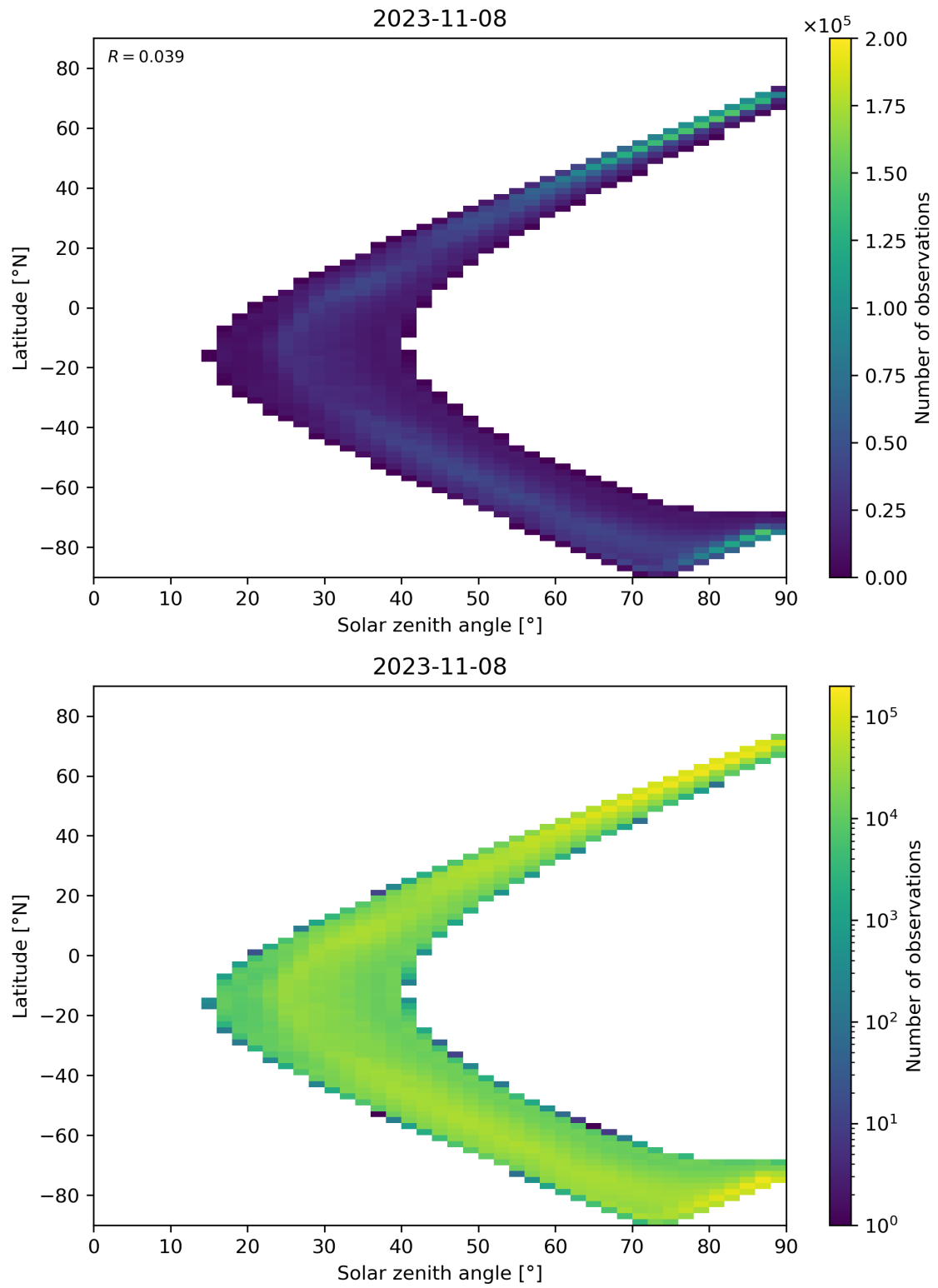
Figure 105: Scatter density plot of “Solar zenith angle” against “Latitude” for 2023-11-07 to 2023-11-09.
