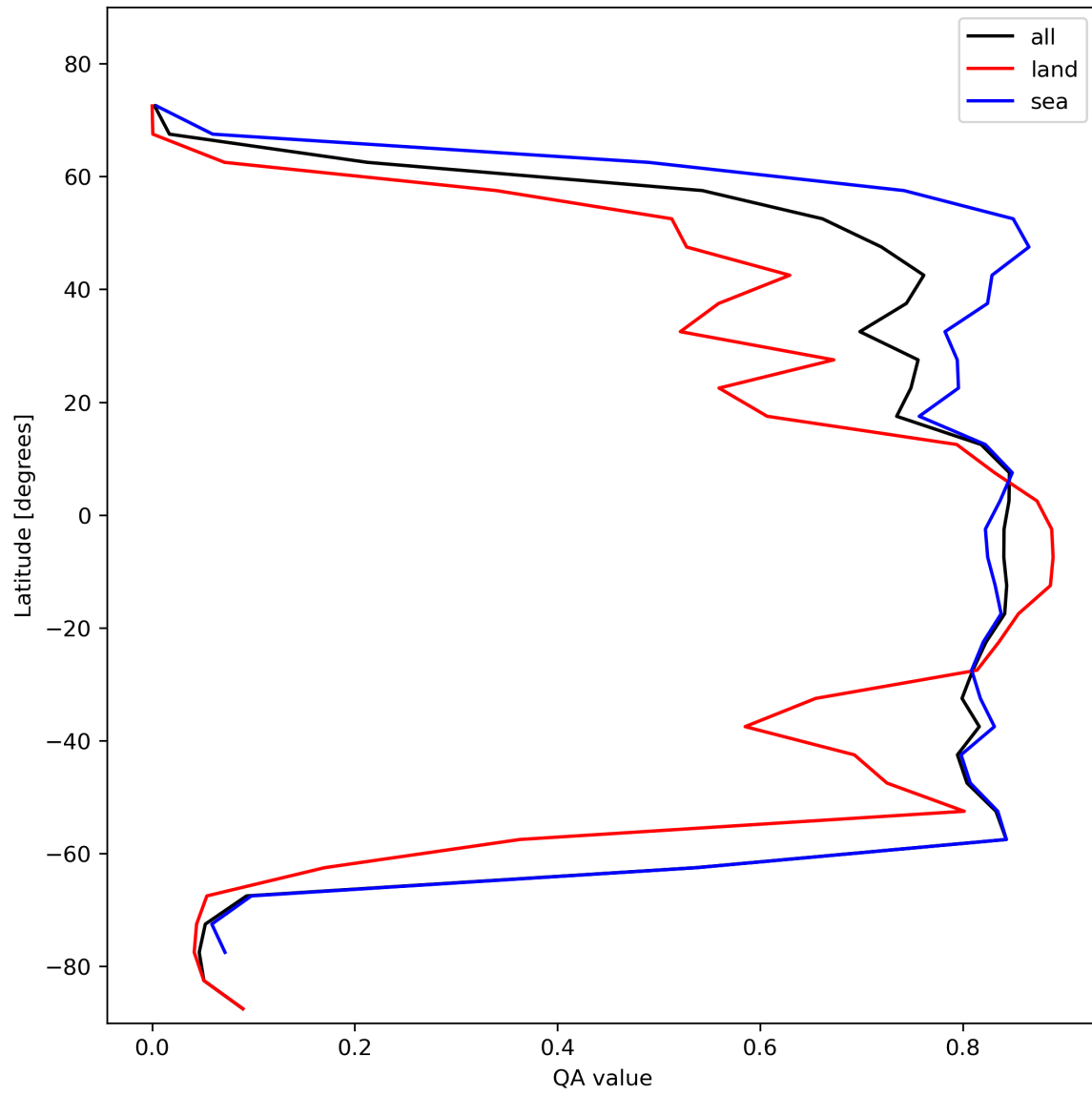
Figure 22: Zonal average of “QA value” for 2023-11-07 to 2023-11-09.
