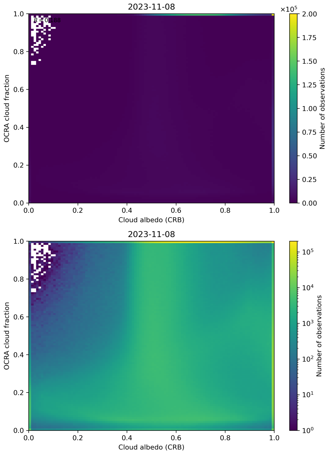
Figure 70: Scatter density plot of “Cloud albedo (CRB)” against “OCRA cloud fraction” for 2023-11-07 to 2023-11-09.
