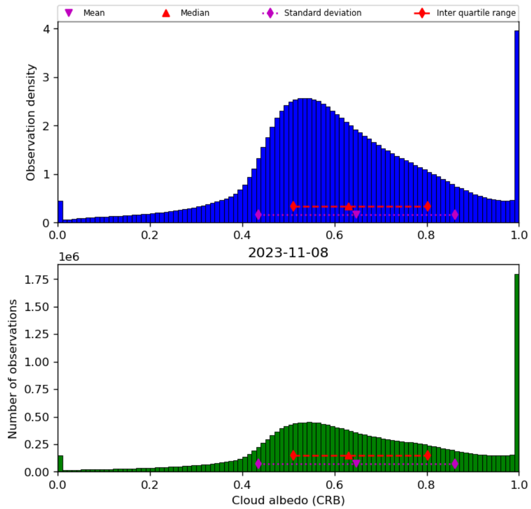
Figure 44: Histogram of “Cloud albedo (CRB)” for 2023-11-07 to 2023-11-09
