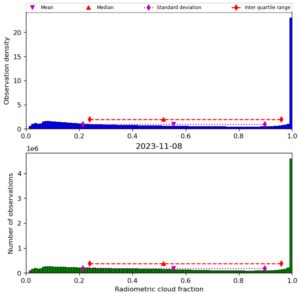
Figure 39: Histogram of “Radiometric cloud fraction” for 2023-11-07 to 2023-11-09
