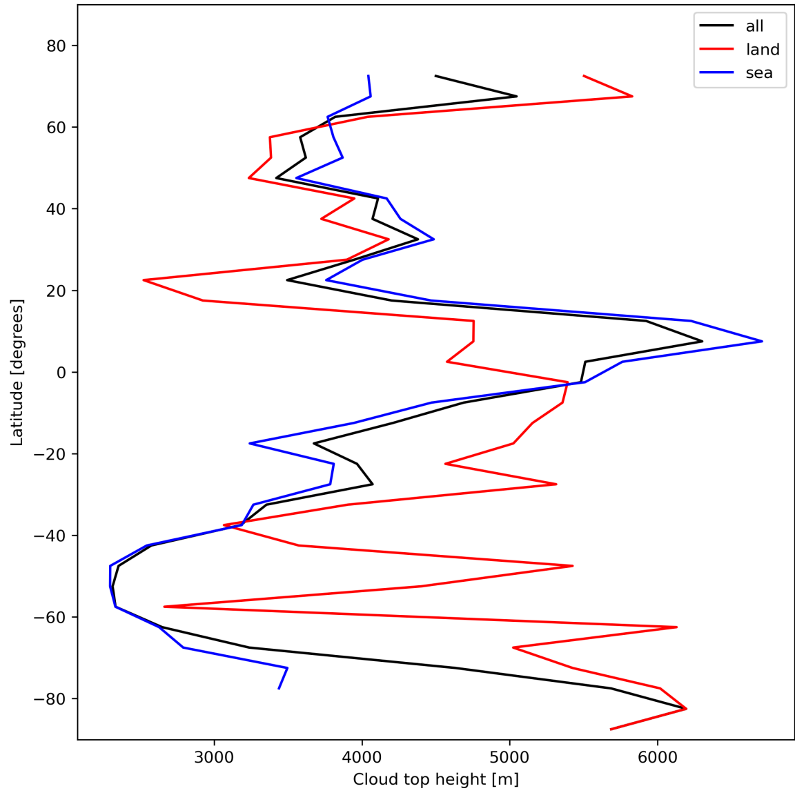
Figure 24: Zonal average of “Cloud top height” for 2023-11-07 to 2023-11-09.
