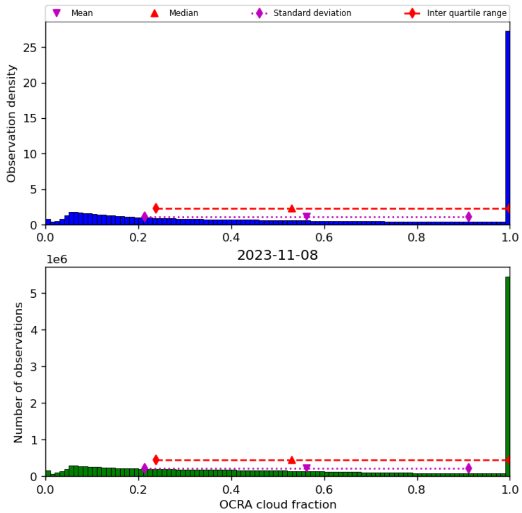
Figure 50: Histogram of “OCRA cloud fraction” for 2023-11-07 to 2023-11-09
