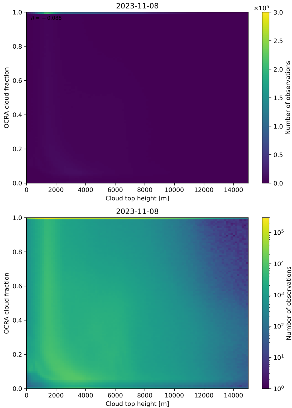
Figure 87: Scatter density plot of “Cloud top height” against “OCRA cloud fraction” for 2023-11-07 to 2023-11-09.
