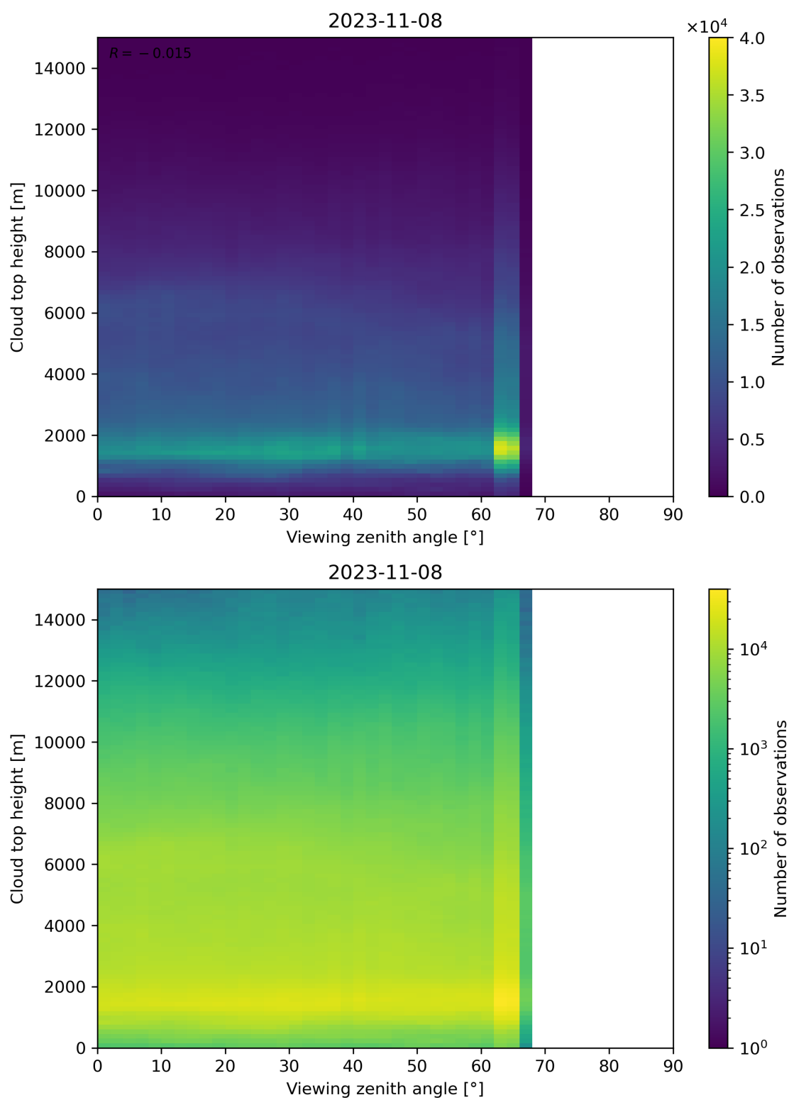
Figure 112: Scatter density plot of “Viewing zenith angle” against “Cloud top height” for 2023-11-07 to 2023-11-09.
