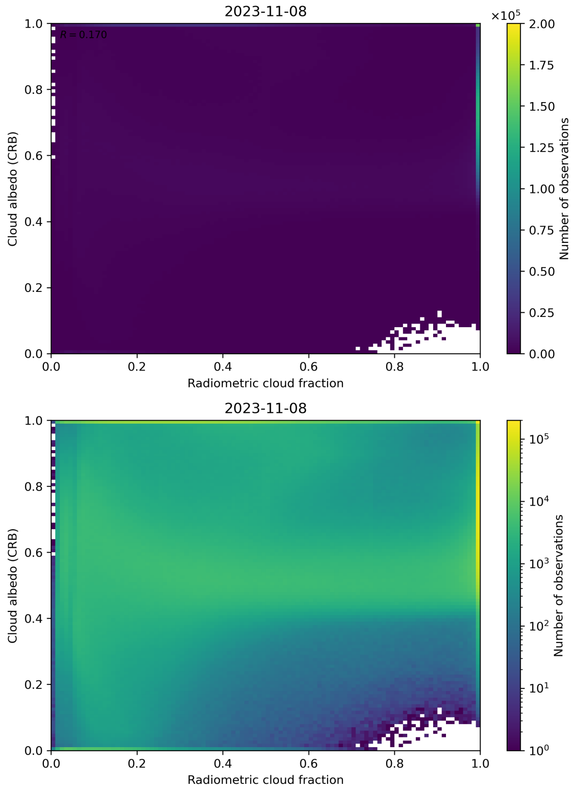
Figure 71: Scatter density plot of “Radiometric cloud fraction” against “Cloud albedo (CRB)” for 2023-11-07 to 2023-11-09.
