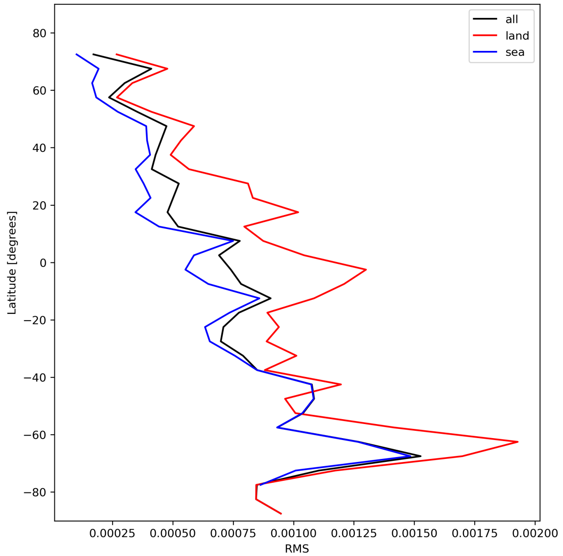
Figure 31: Zonal average of “RMS” for 2023-11-07 to 2023-11-09.
