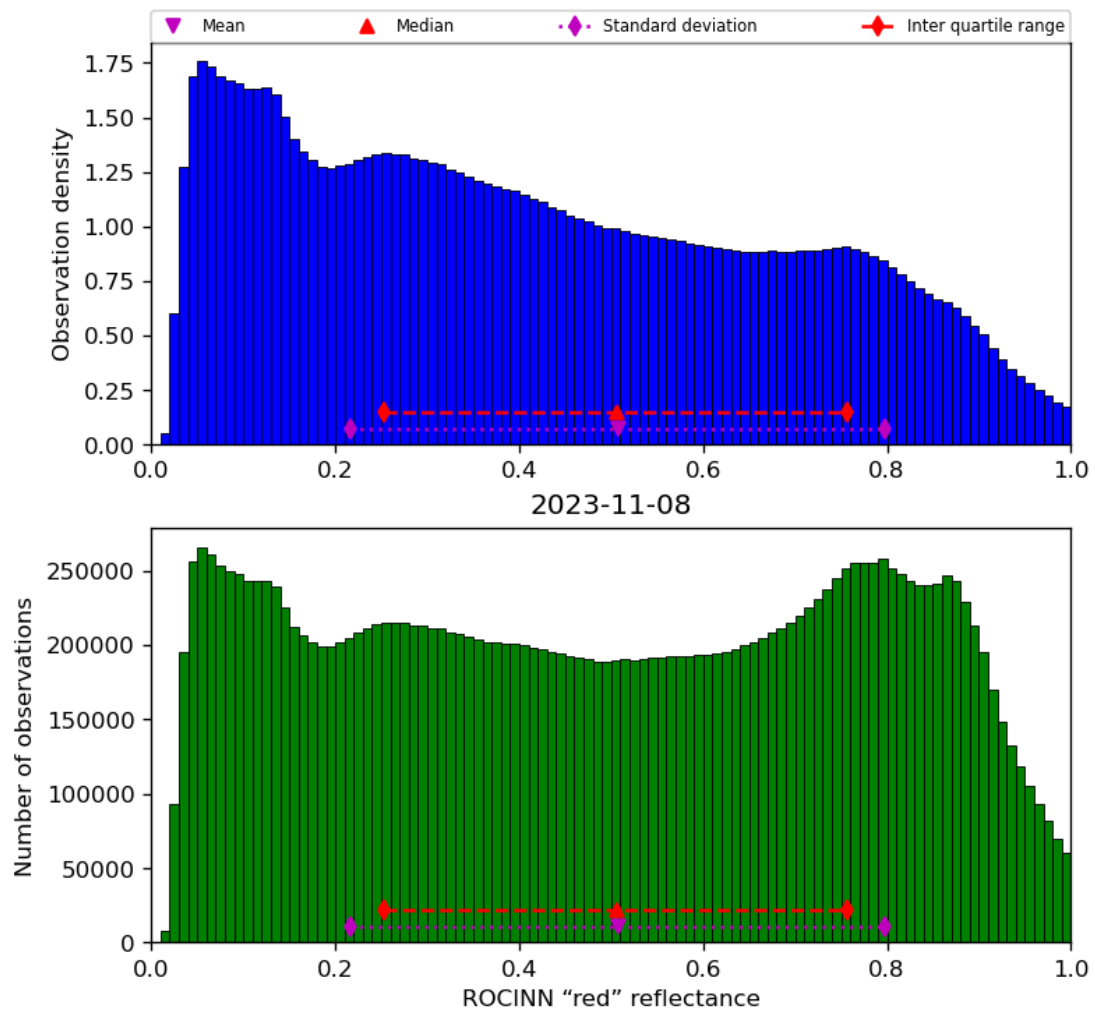
Figure 53: Histogram of “ROCINN “red” reflectance” for 2023-11-07 to 2023-11-09
