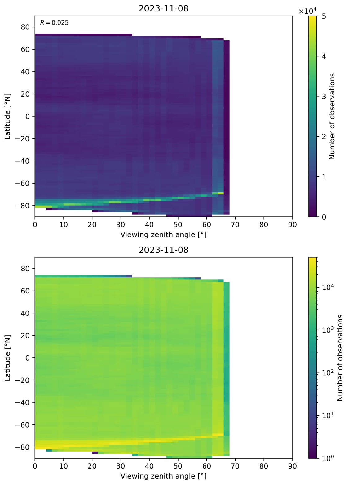
Figure 113: Scatter density plot of “Viewing zenith angle” against “Latitude” for 2023-11-07 to 2023-11-09.
