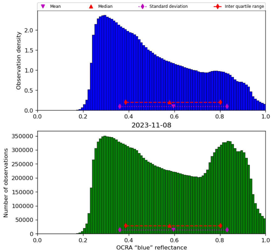
Figure 51: Histogram of “OCRA “blue” reflectance” for 2023-11-07 to 2023-11-09
