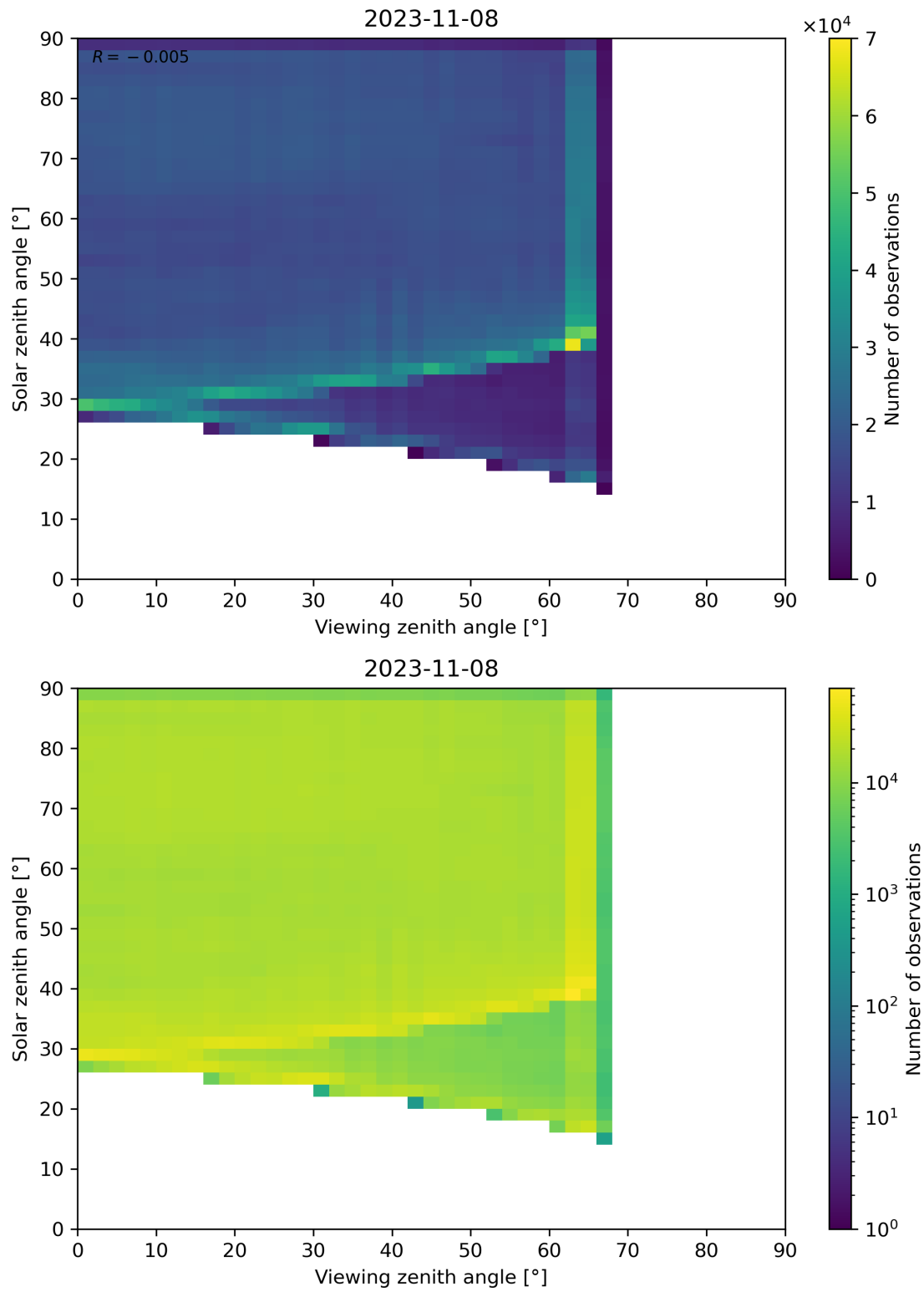
Figure 114: Scatter density plot of “Viewing zenith angle” against “Solar zenith angle” for 2023-11-07 to 2023-11-09.
