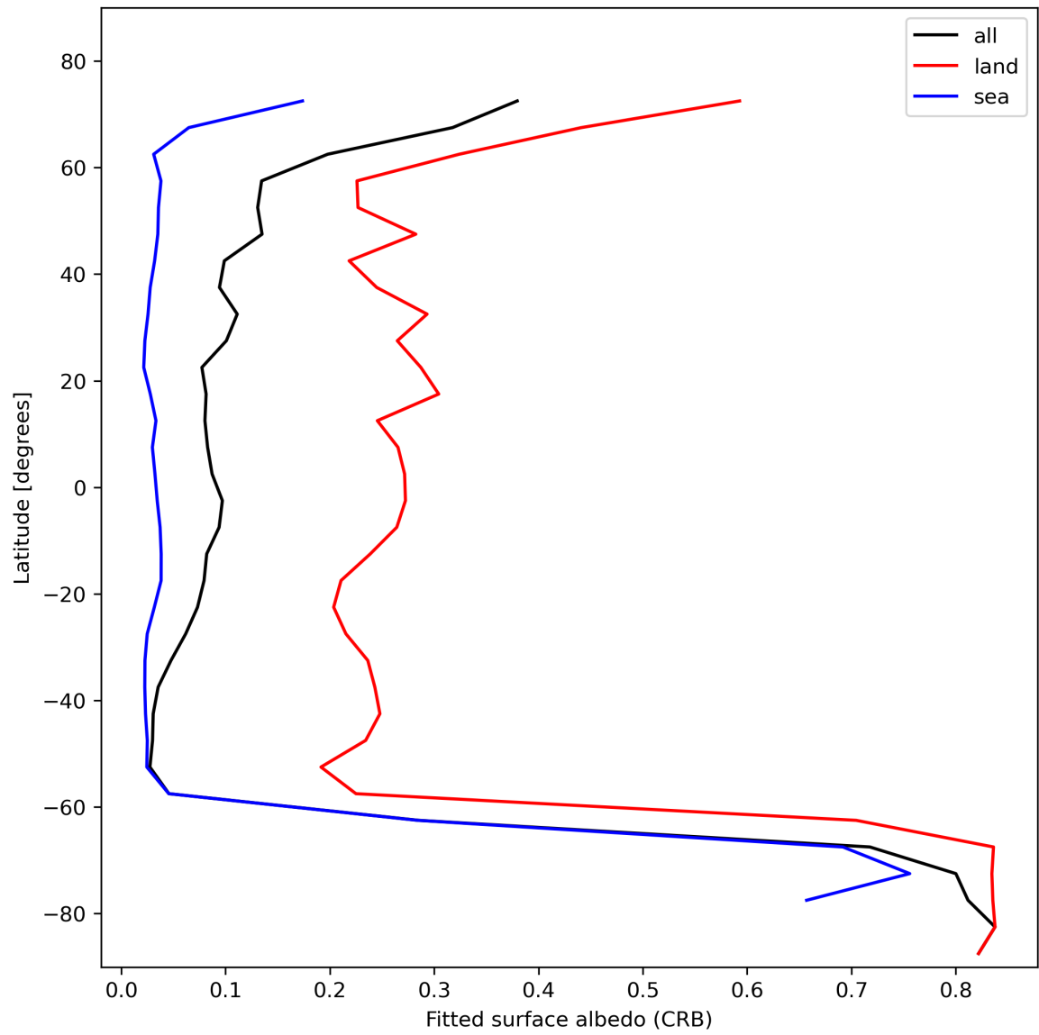
Figure 30: Zonal average of “Fitted surface albedo (CRB)” for 2023-11-07 to 2023-11-09.
