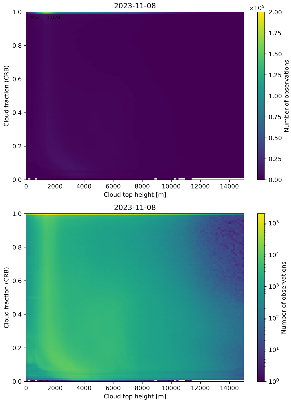
Figure 88: Scatter density plot of “Cloud top height” against “Cloud fraction (CRB)” for 2023-11-07 to 2023-11-09.
