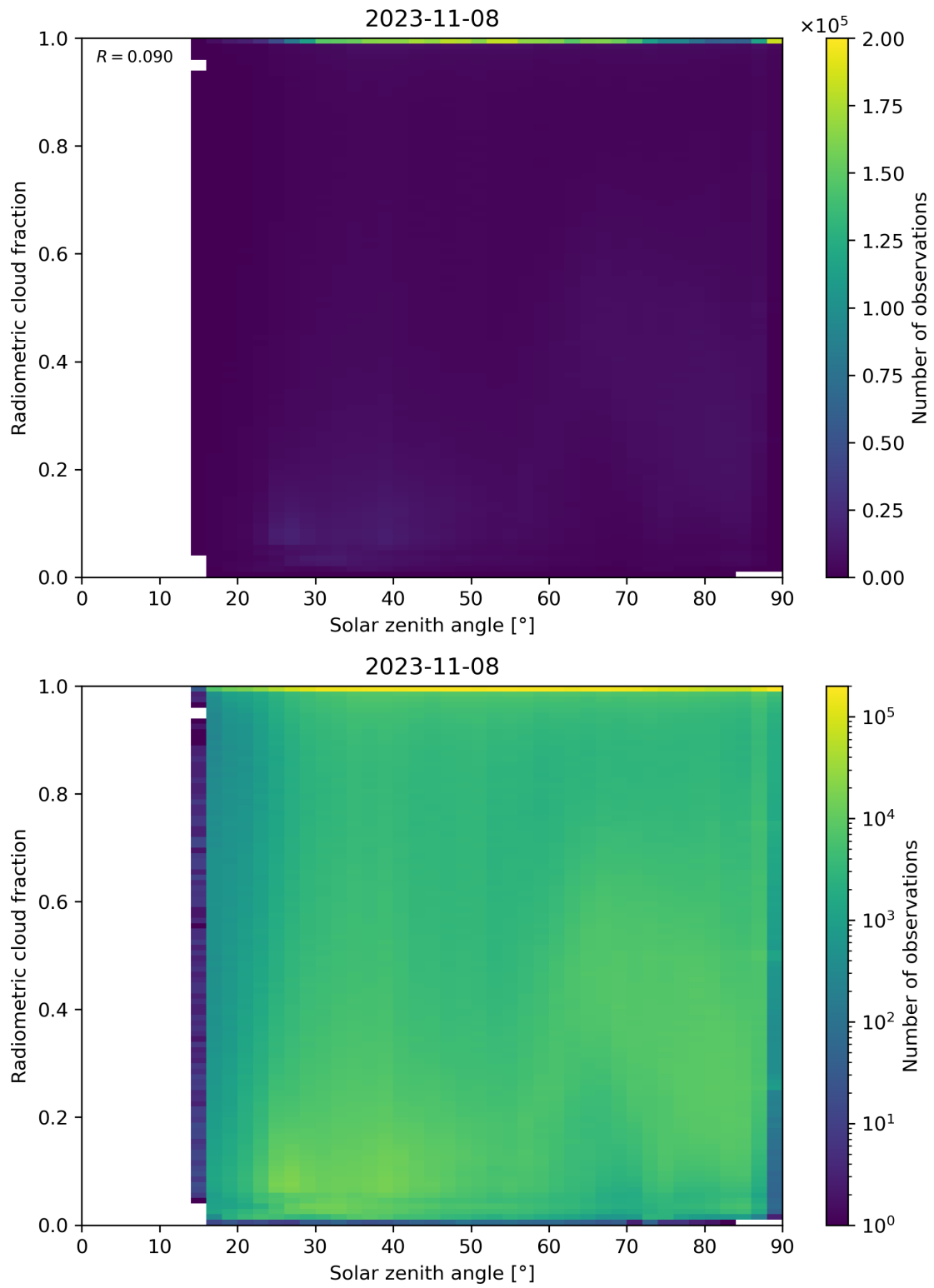
Figure 99: Scatter density plot of “Solar zenith angle” against “Radiometric cloud fraction” for 2023-11-07 to 2023-11-09.
