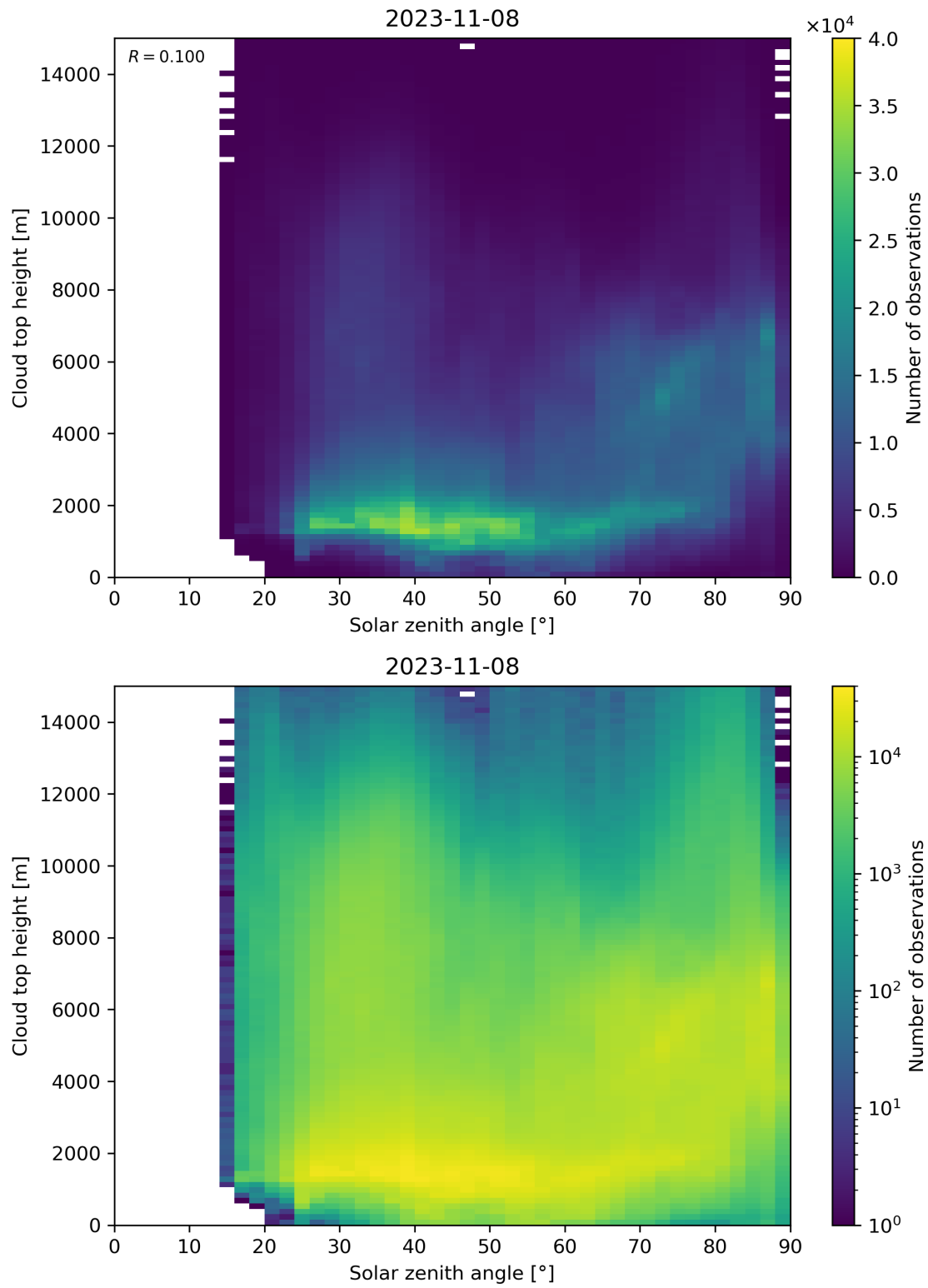
Figure 104: Scatter density plot of “Solar zenith angle” against “Cloud top height” for 2023-11-07 to 2023-11-09.
