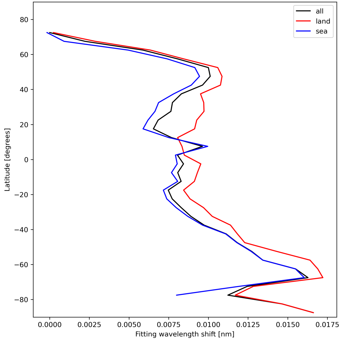
Figure 33: Zonal average of “Fitting wavelength shift” for 2023-11-07 to 2023-11-09.
