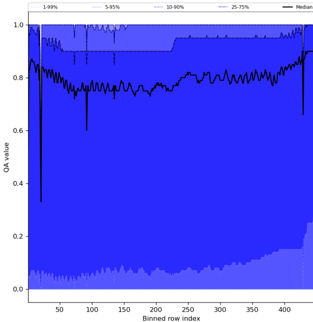
Figure 54: Along track statistics of “QA value” for 2023-11-07 to 2023-11-09
