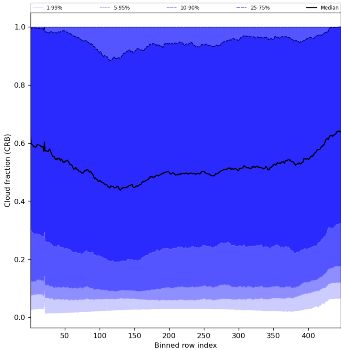
Figure 58: Along track statistics of “Cloud fraction (CRB)” for 2023-11-07 to 2023-11-09
