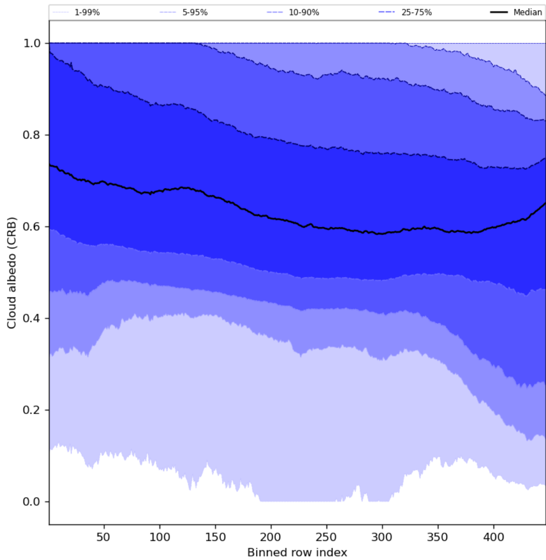
Figure 60: Along track statistics of “Cloud albedo (CRB)” for 2023-11-07 to 2023-11-09
