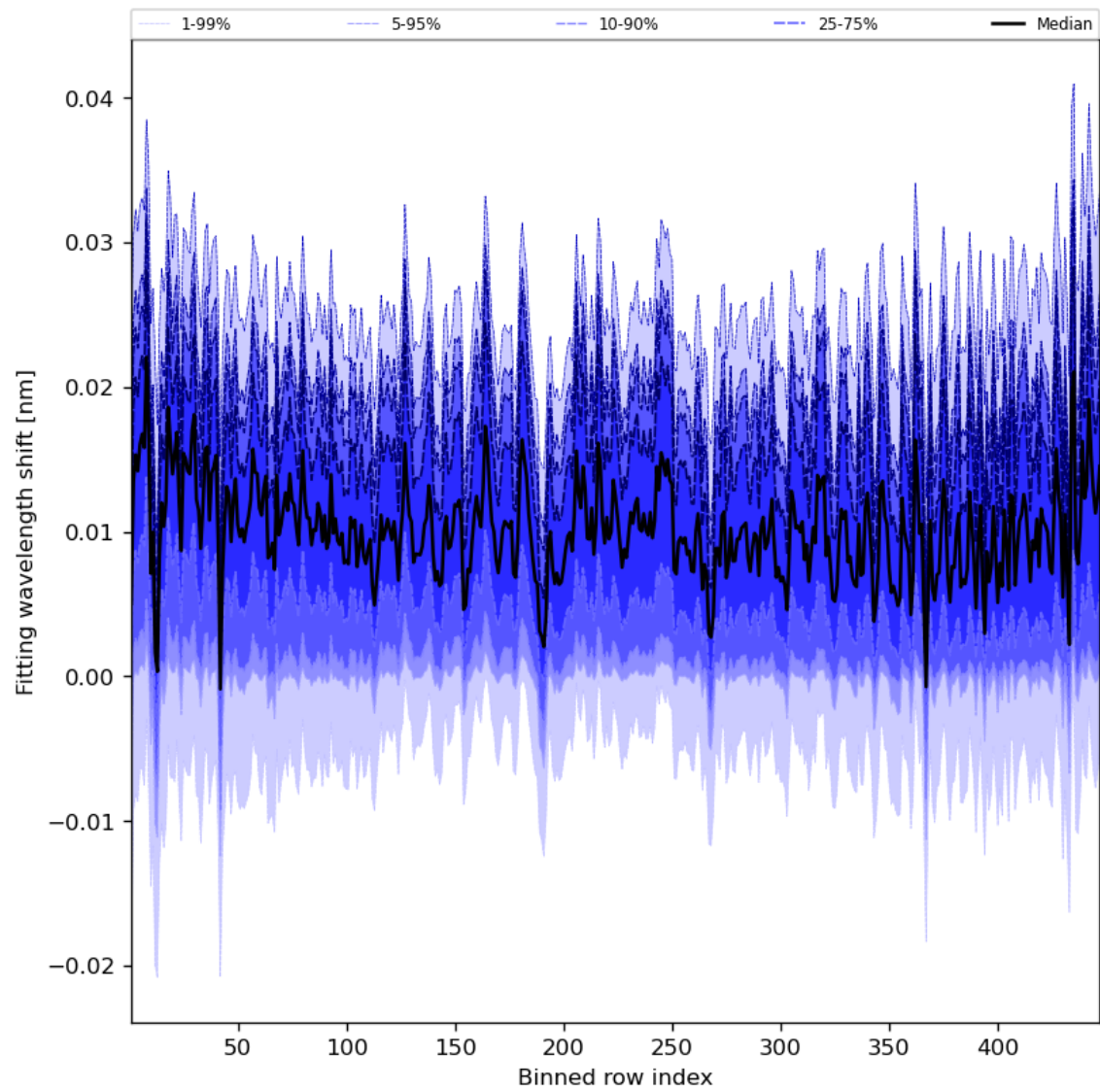
Figure 65: Along track statistics of “Fitting wavelength shift” for 2023-11-07 to 2023-11-09
