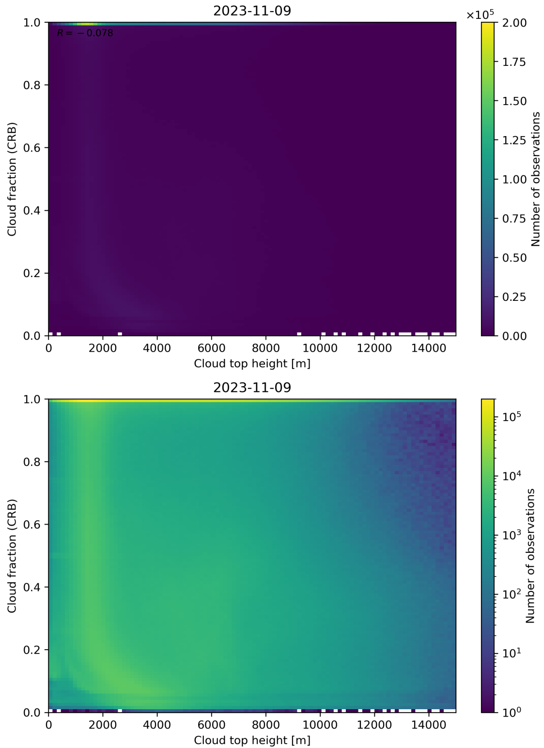
Figure 88: Scatter density plot of “Cloud top height” against “Cloud fraction (CRB)” for 2023-11-08 to 2023-11-10.
