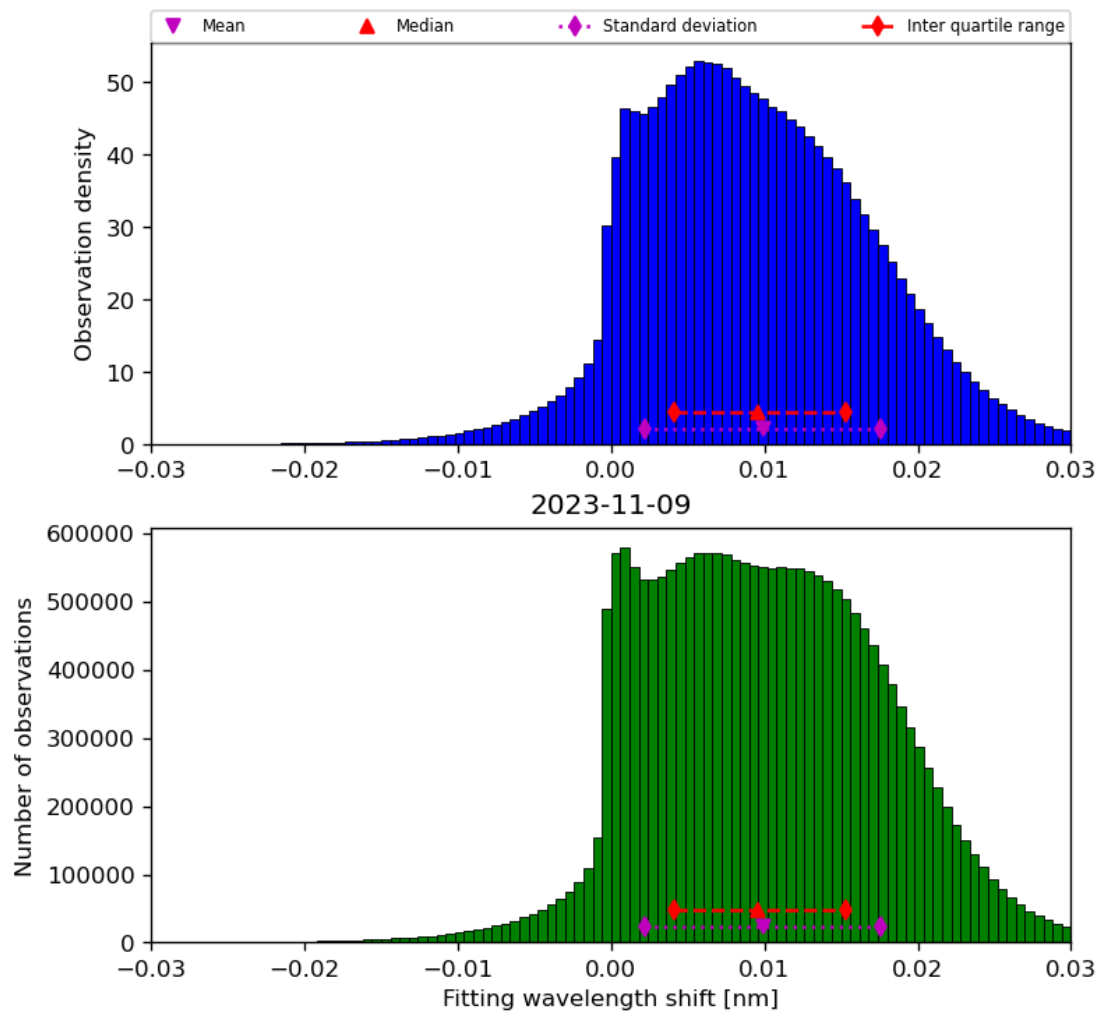
Figure 49: Histogram of “Fitting wavelength shift” for 2023-11-08 to 2023-11-10
