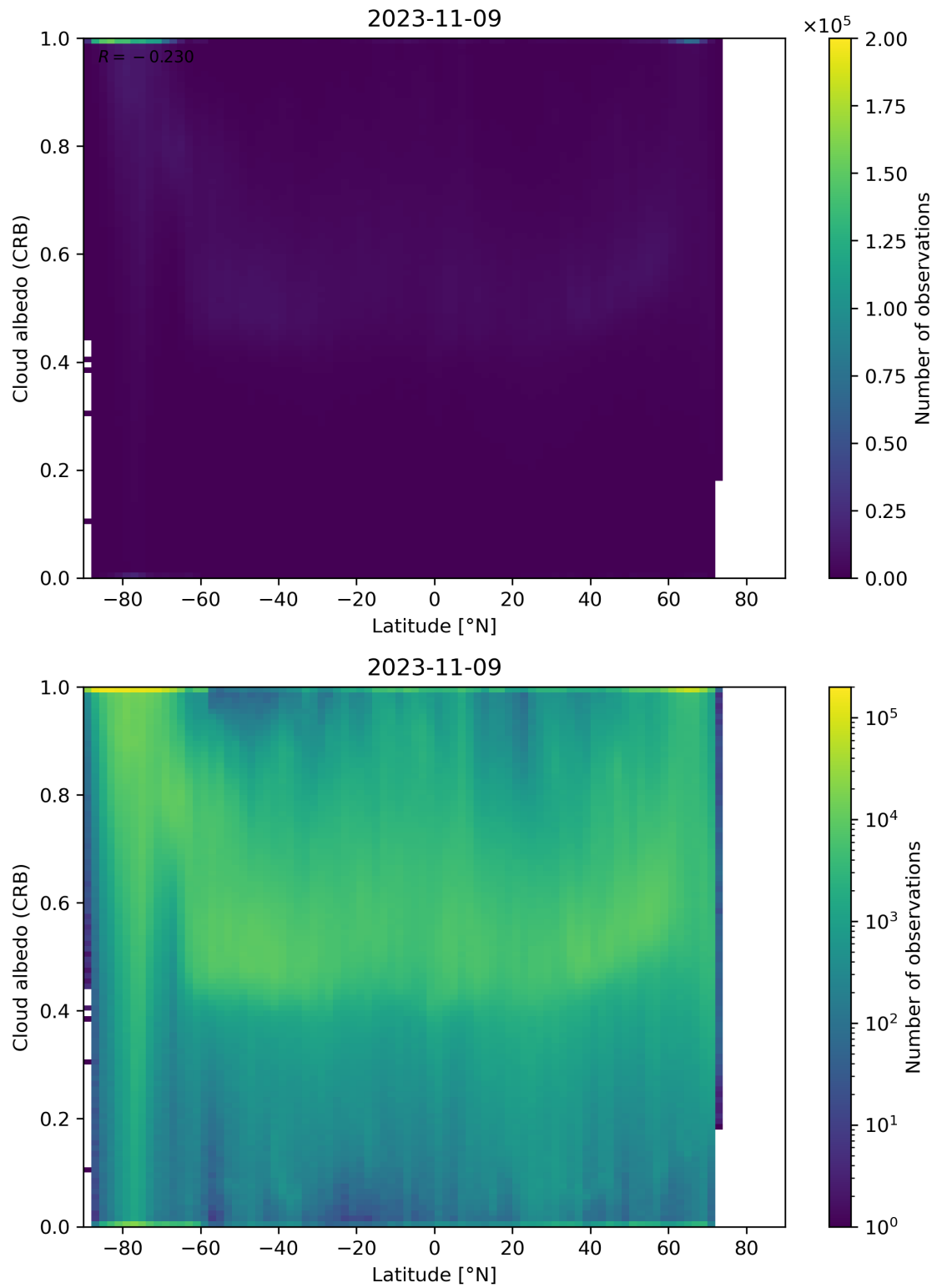
Figure 91: Scatter density plot of “Latitude” against “Cloud albedo (CRB)” for 2023-11-08 to 2023-11-10.
