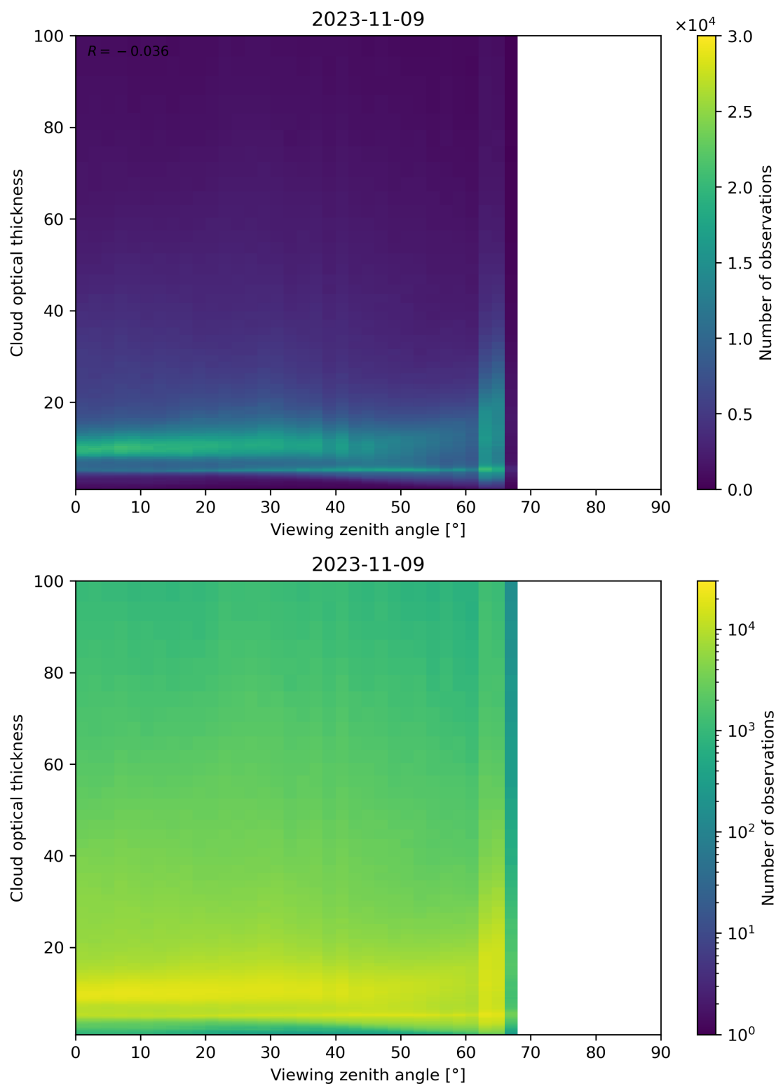
Figure 111: Scatter density plot of “Viewing zenith angle” against “Cloud optical thickness” for 2023-11-08 to 2023-11-10.
