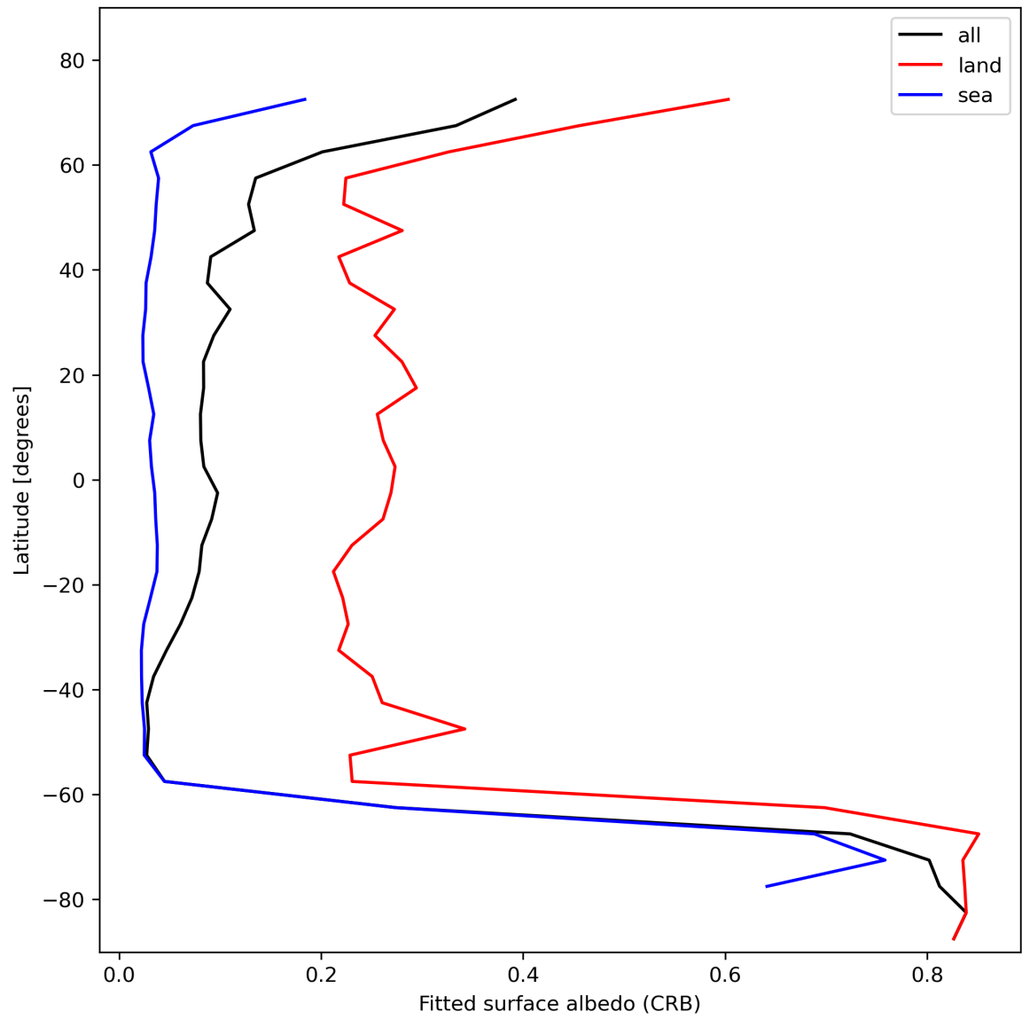
Figure 30: Zonal average of “Fitted surface albedo (CRB)” for 2023-11-08 to 2023-11-10.
