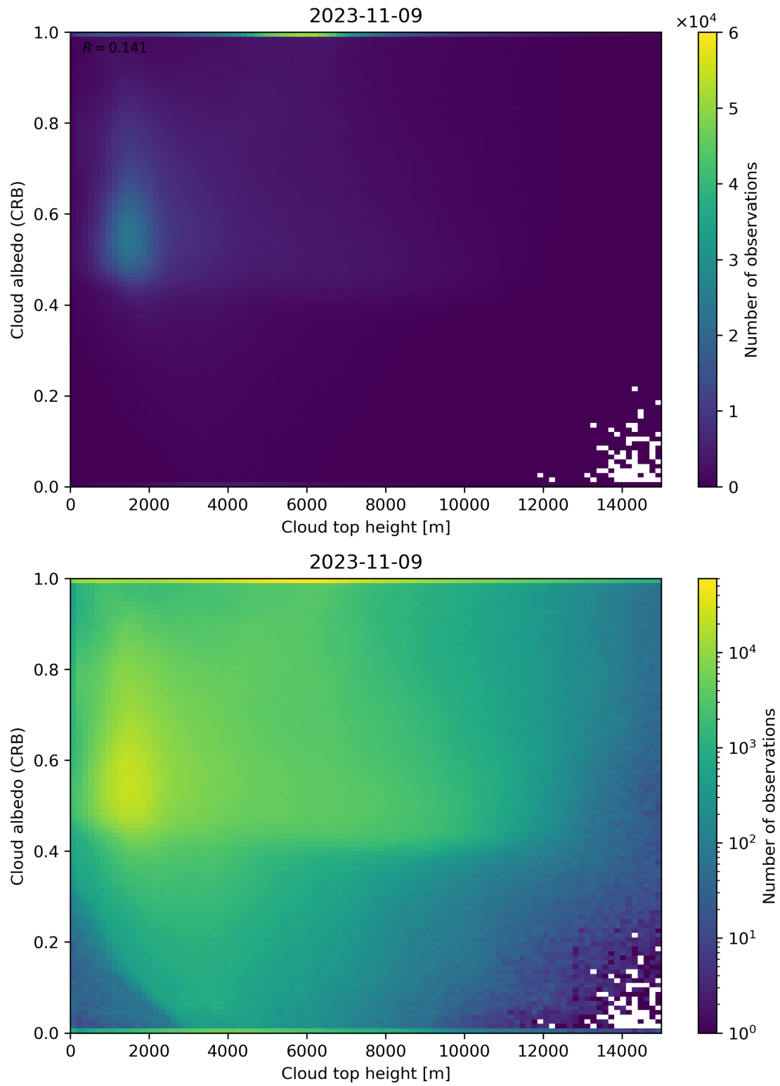
Figure 86: Scatter density plot of “Cloud top height” against “Cloud albedo (CRB)” for 2023-11-08 to 2023-11-10.
