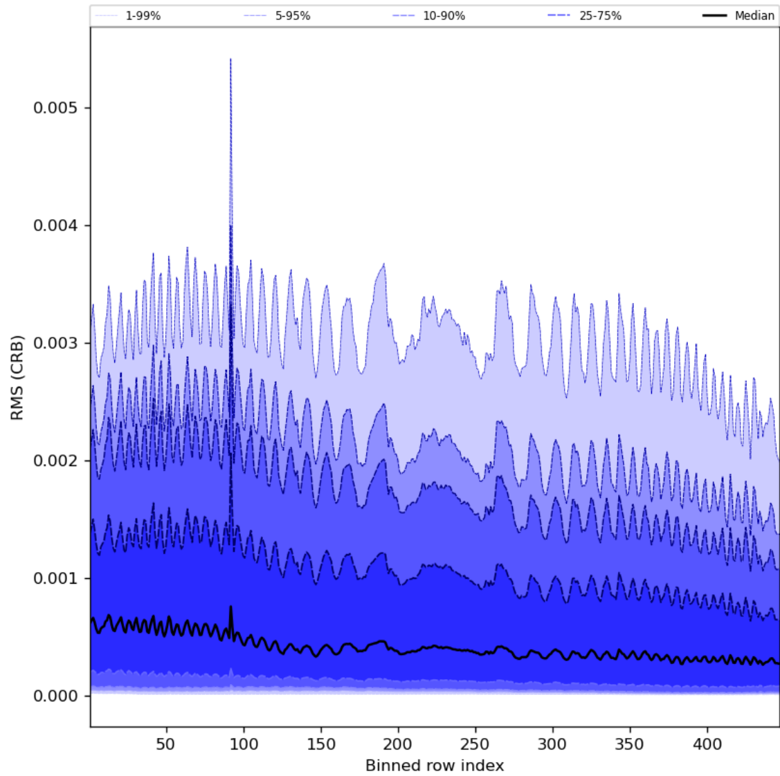
Figure 64: Along track statistics of “RMS (CRB)” for 2023-11-08 to 2023-11-10
