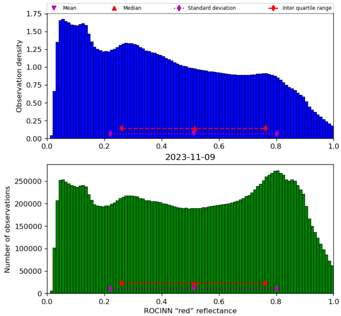
Figure 53: Histogram of “ROCINN “red” reflectance” for 2023-11-08 to 2023-11-10
