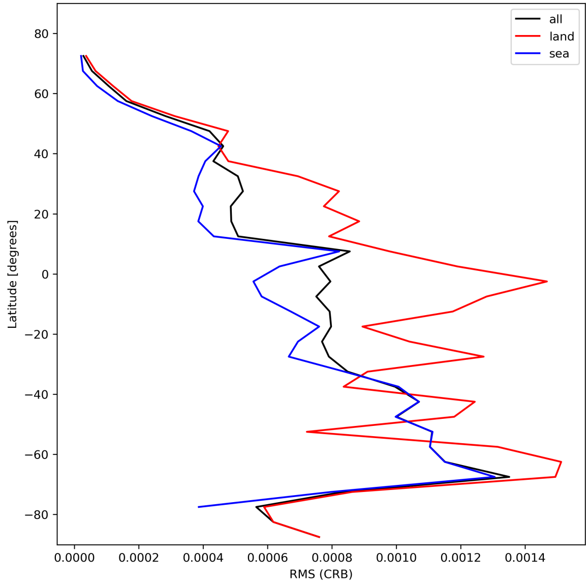
Figure 32: Zonal average of “RMS (CRB)” for 2023-11-08 to 2023-11-10.
