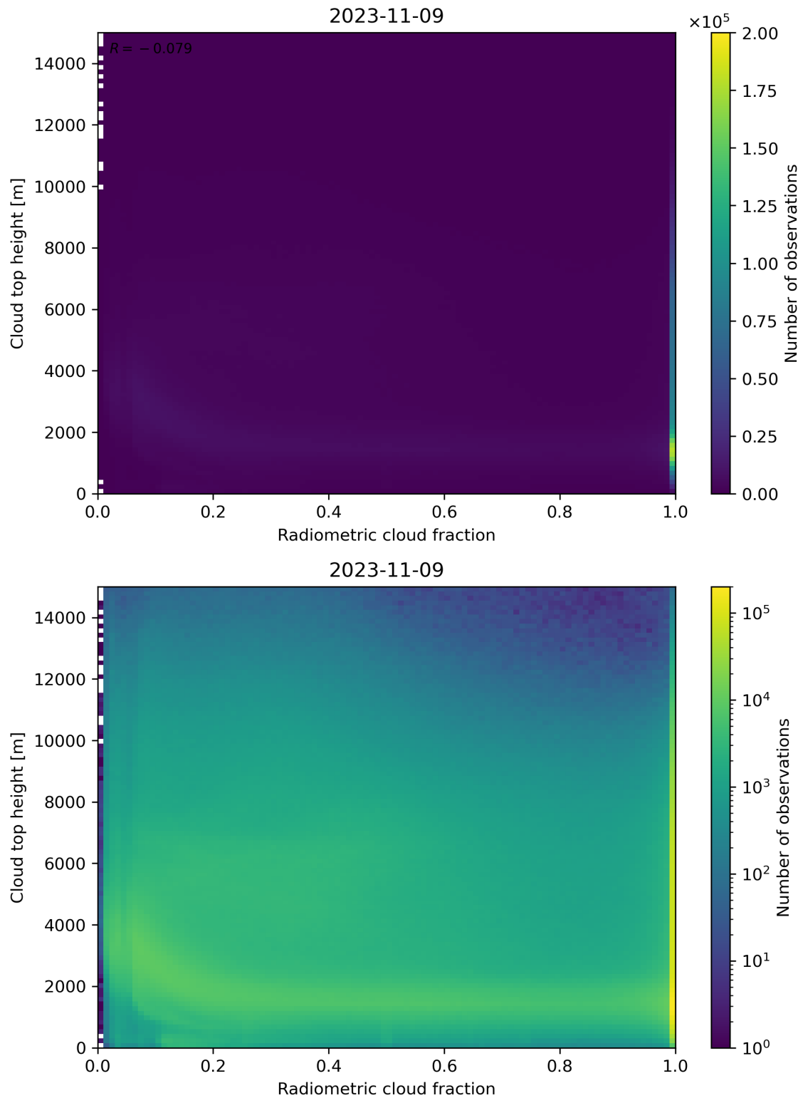
Figure 76: Scatter density plot of “Radiometric cloud fraction” against “Cloud top height” for 2023-11-08 to 2023-11-10.
