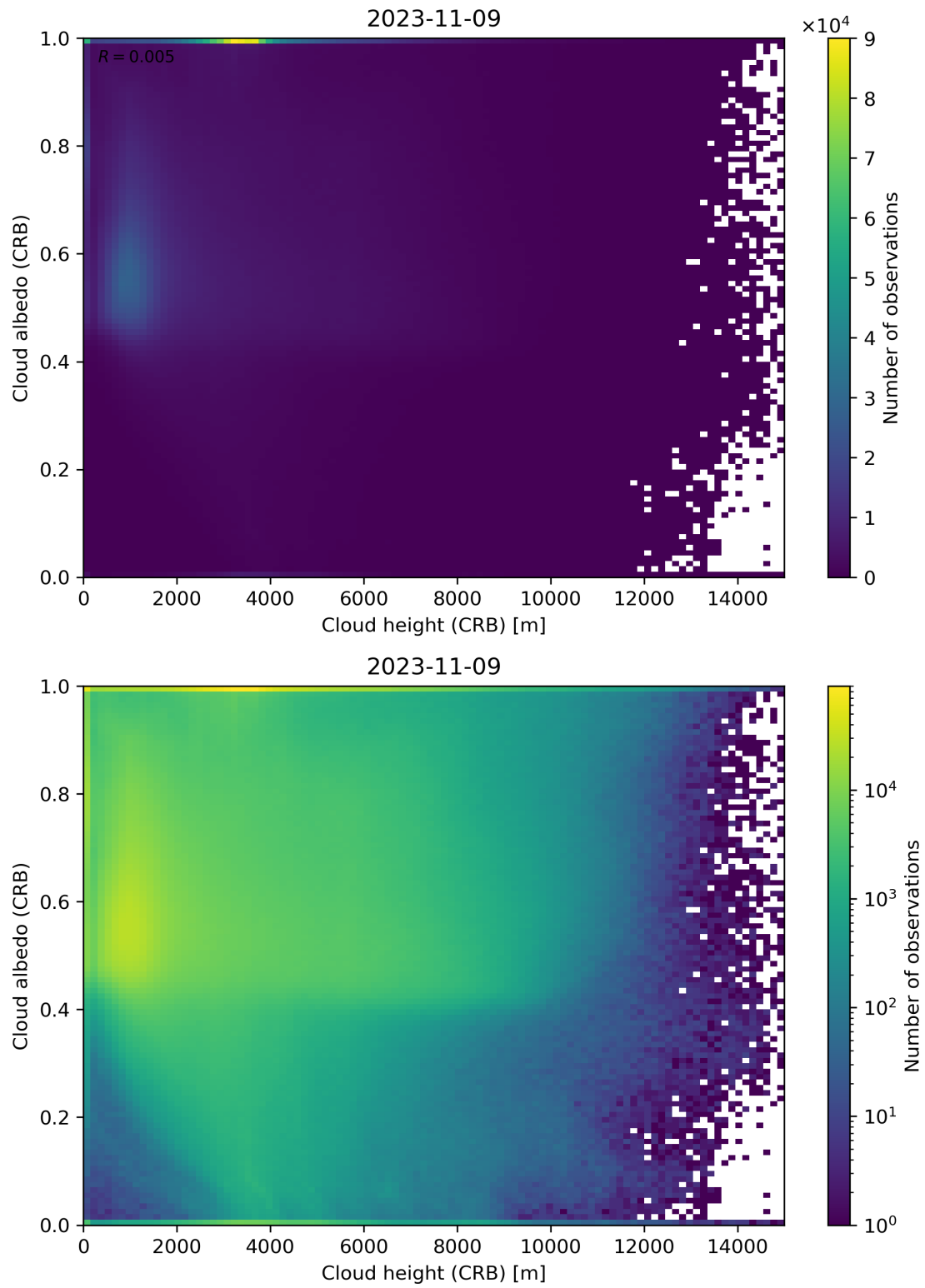
Figure 80: Scatter density plot of “Cloud height (CRB)” against “Cloud albedo (CRB)” for 2023-11-08 to 2023-11-10.
