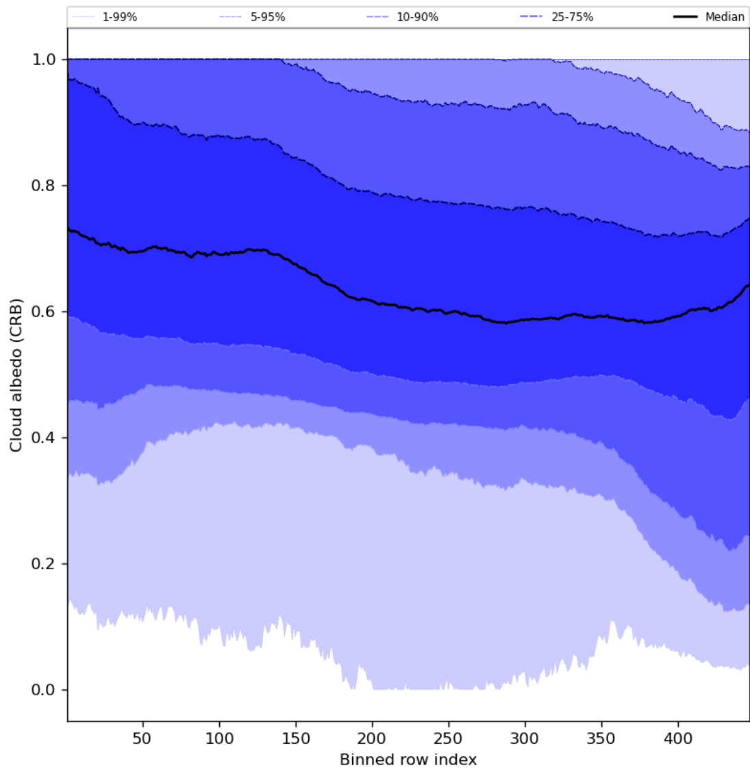
Figure 60: Along track statistics of “Cloud albedo (CRB)” for 2023-11-08 to 2023-11-10
