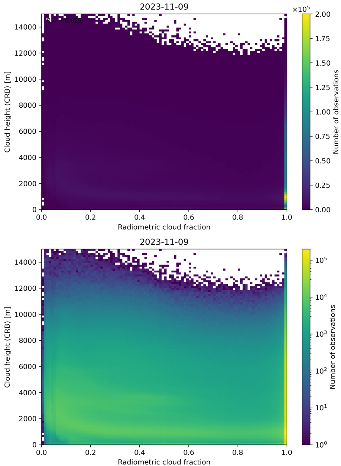
Figure 74: Scatter density plot of “Radiometric cloud fraction” against “Cloud height (CRB)” for 2023-11-08 to 2023-11-10.
