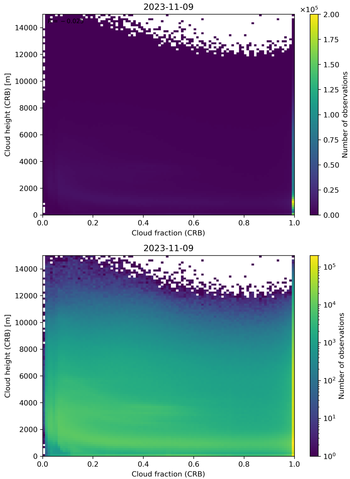
Figure 79: Scatter density plot of “Cloud fraction (CRB)” against “Cloud height (CRB)” for 2023-11-08 to 2023-11-10.
