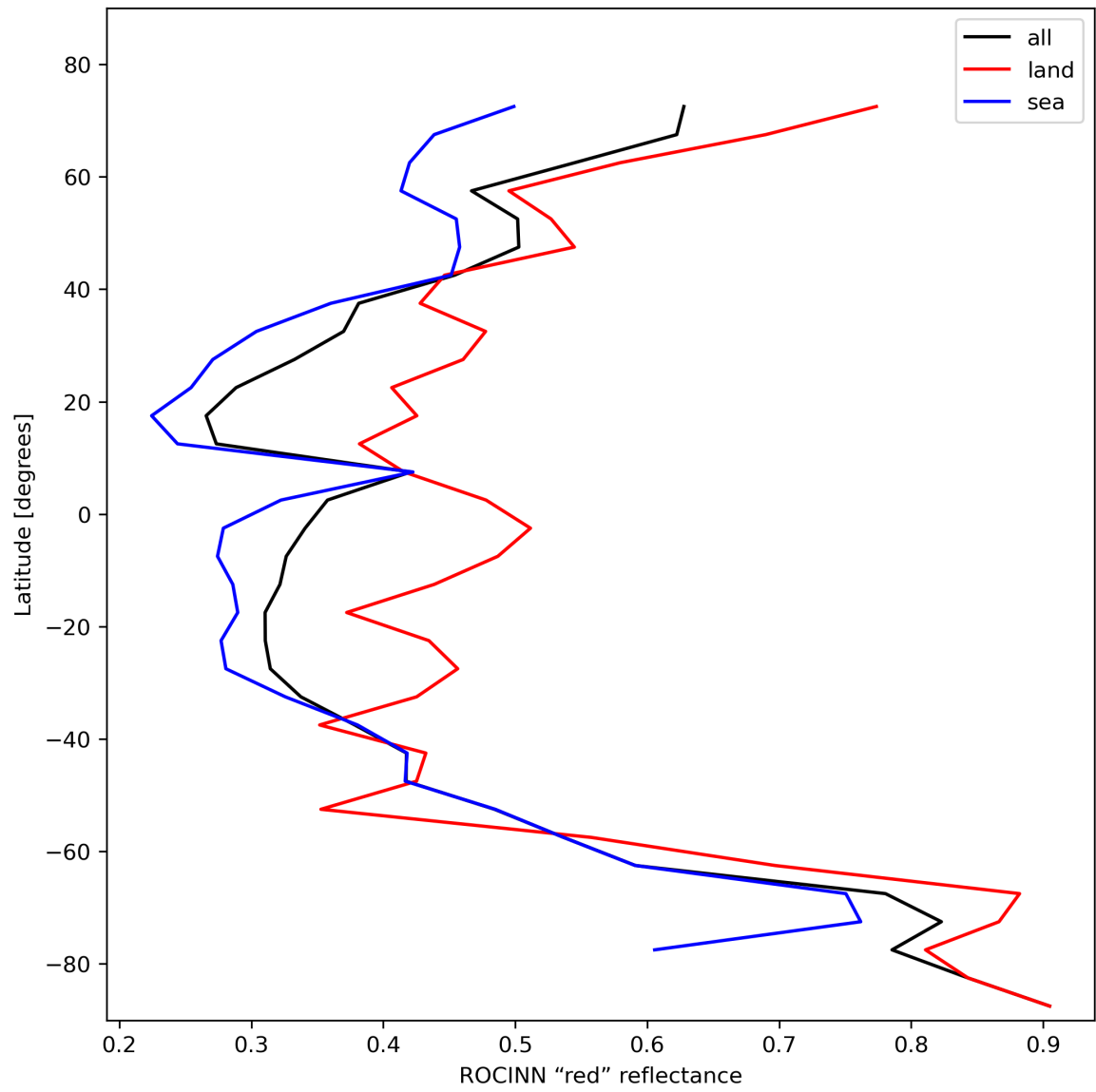
Figure 37: Zonal average of “ROCINN “red” reflectance” for 2023-11-08 to 2023-11-10.
