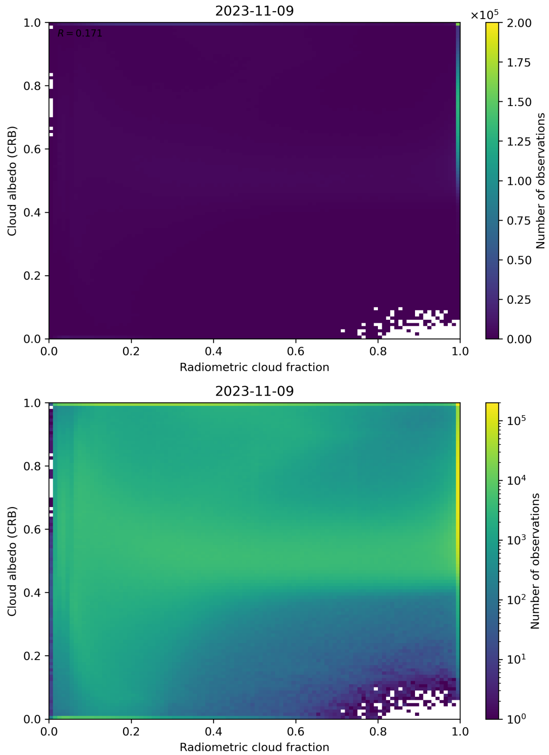
Figure 71: Scatter density plot of “Radiometric cloud fraction” against “Cloud albedo (CRB)” for 2023-11-08 to 2023-11-10.
