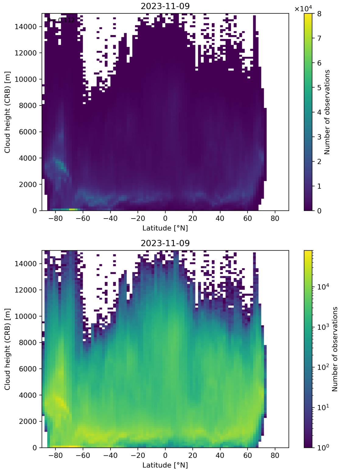
Figure 95: Scatter density plot of “Latitude” against “Cloud height (CRB)” for 2023-11-08 to 2023-11-10.
