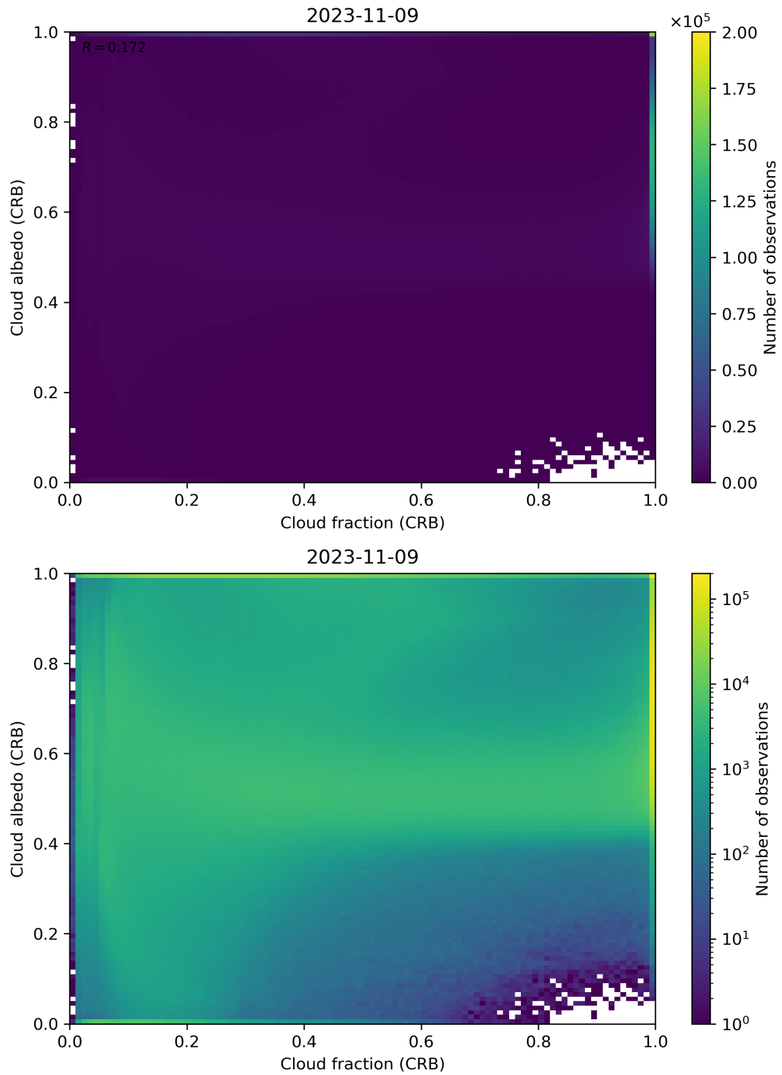
Figure 77: Scatter density plot of “Cloud fraction (CRB)” against “Cloud albedo (CRB)” for 2023-11-08 to 2023-11-10.
