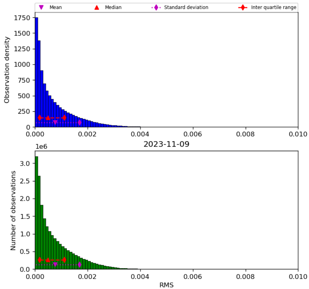
Figure 47: Histogram of “RMS” for 2023-11-08 to 2023-11-10
