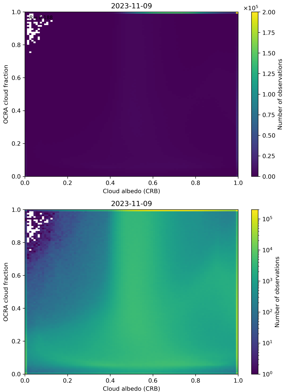
Figure 70: Scatter density plot of “Cloud albedo (CRB)” against “OCRA cloud fraction” for 2023-11-08 to 2023-11-10.
