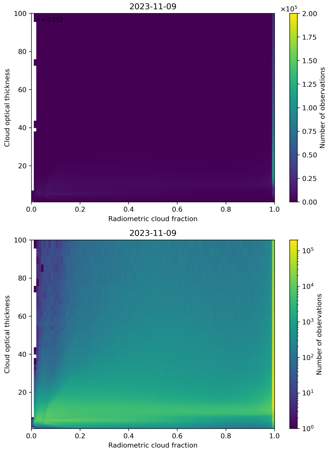
Figure 75: Scatter density plot of “Radiometric cloud fraction” against “Cloud optical thickness” for 2023-11-08 to 2023-11-10.
