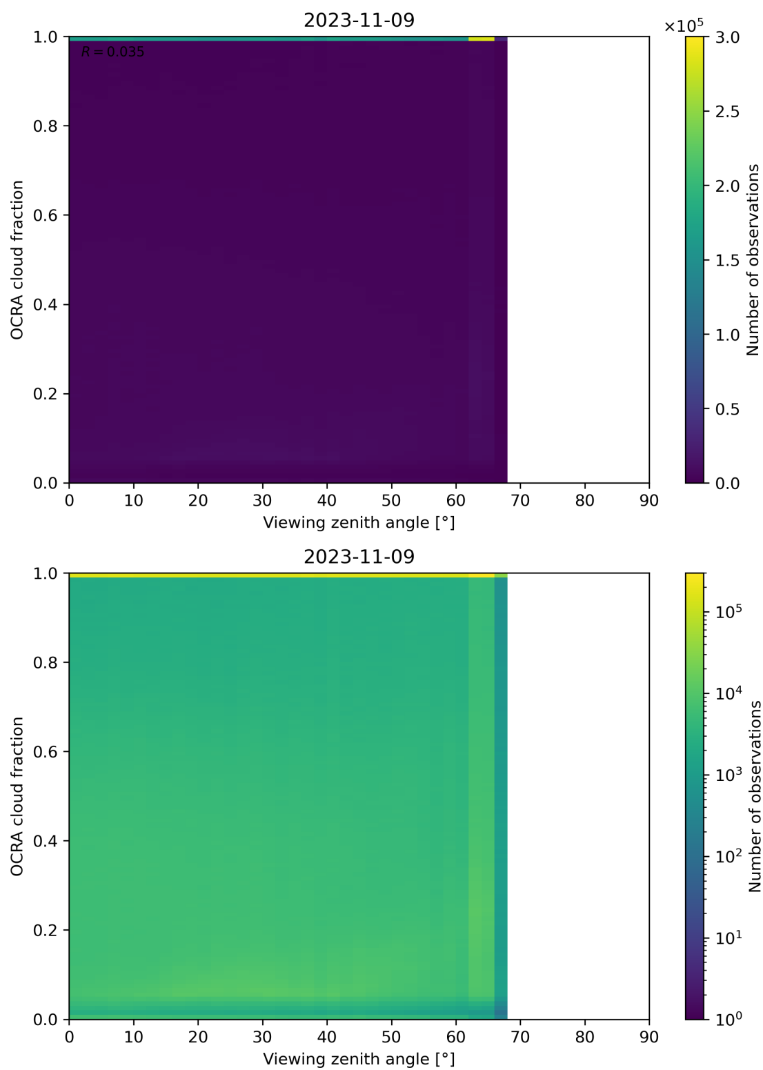
Figure 108: Scatter density plot of “Viewing zenith angle” against “OCRA cloud fraction” for 2023-11-08 to 2023-11-10.
