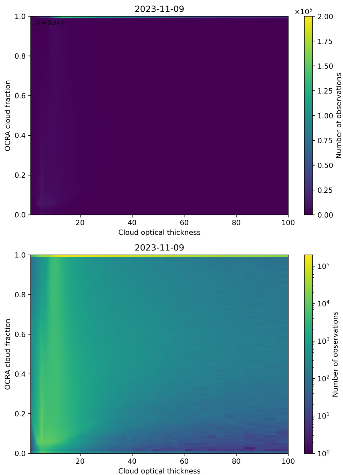
Figure 83: Scatter density plot of “Cloud optical thickness” against “OCRA cloud fraction” for 2023-11-08 to 2023-11-10.
