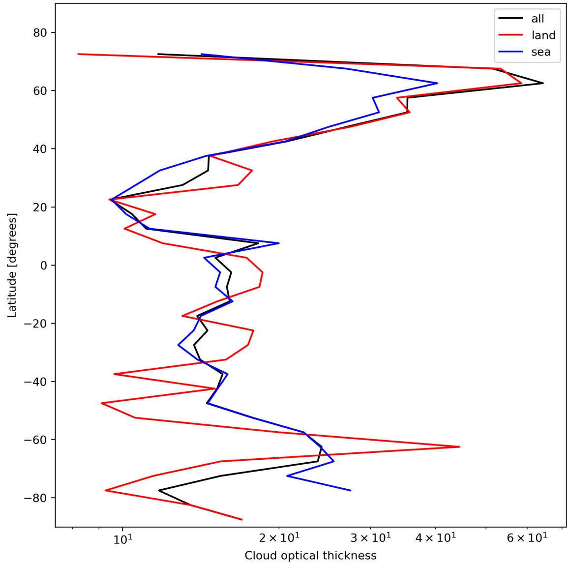
Figure 25: Zonal average of “Cloud optical thickness” for 2023-11-08 to 2023-11-10.
