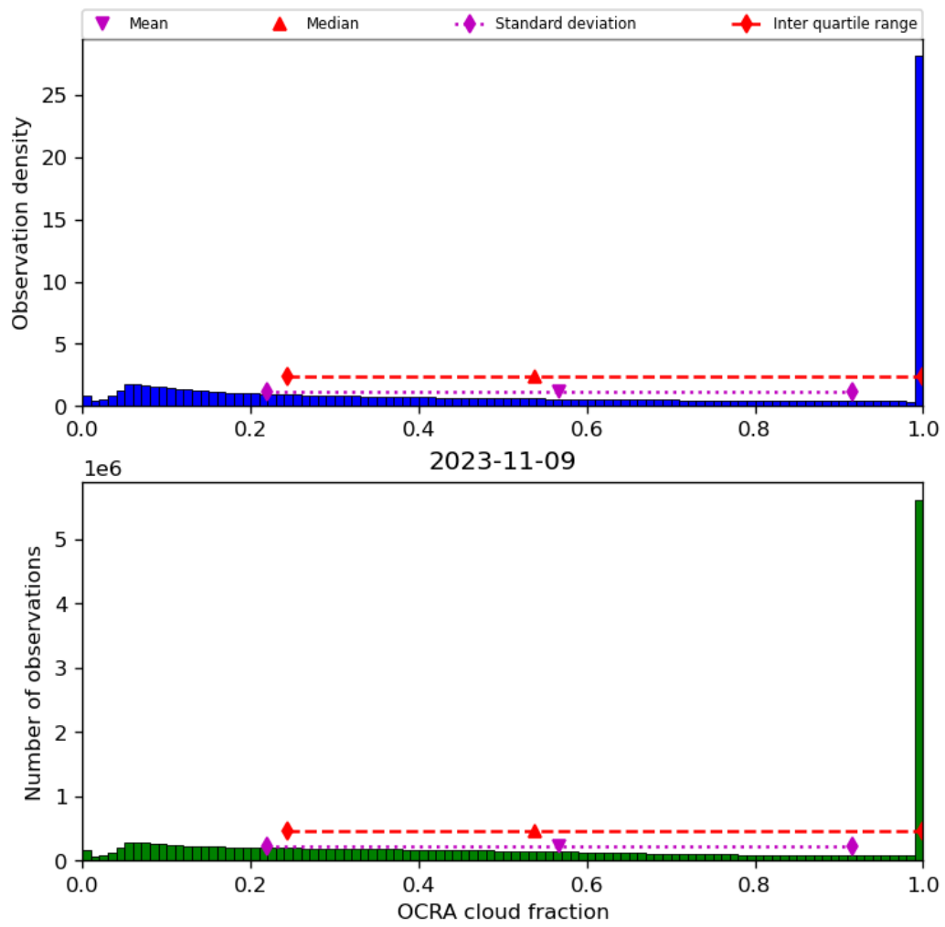
Figure 50: Histogram of “OCRA cloud fraction” for 2023-11-08 to 2023-11-10
