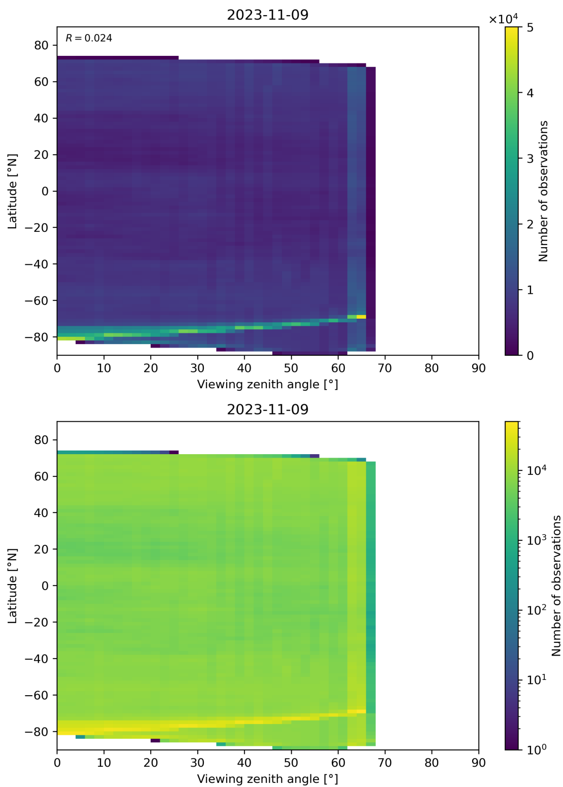
Figure 113: Scatter density plot of “Viewing zenith angle” against “Latitude” for 2023-11-08 to 2023-11-10.
