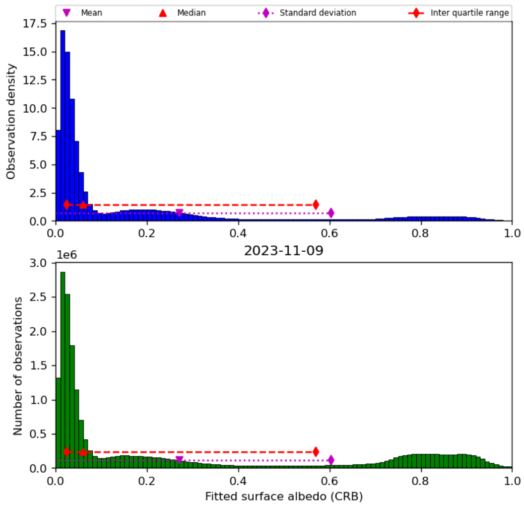
Figure 46: Histogram of “Fitted surface albedo (CRB)” for 2023-11-08 to 2023-11-10
