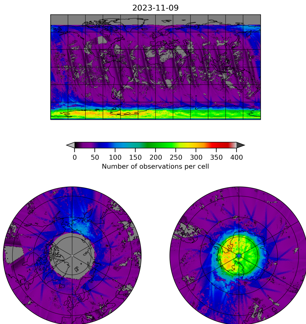
Figure 21: Map of the number of observations for 2023-11-08 to 2023-11-10
