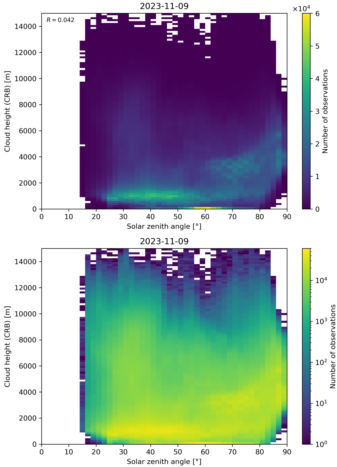
Figure 102: Scatter density plot of “Solar zenith angle” against “Cloud height (CRB)” for 2023-11-08 to 2023-11-10.
