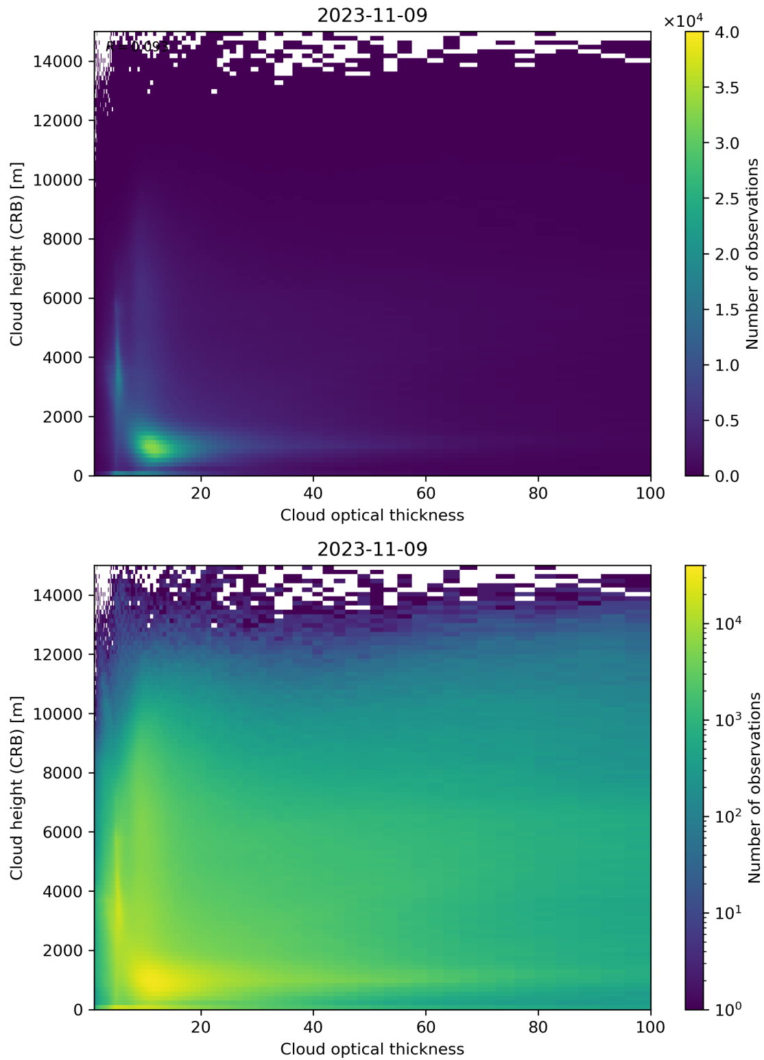
Figure 85: Scatter density plot of “Cloud optical thickness” against “Cloud height (CRB)” for 2023-11-08 to 2023-11-10.
