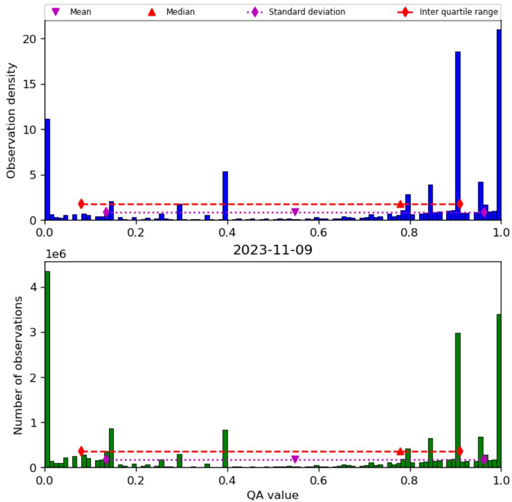
Figure 38: Histogram of “QA value” for 2023-11-08 to 2023-11-10
