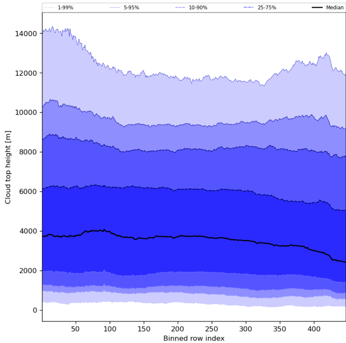
Figure 56: Along track statistics of “Cloud top height” for 2023-11-08 to 2023-11-10
