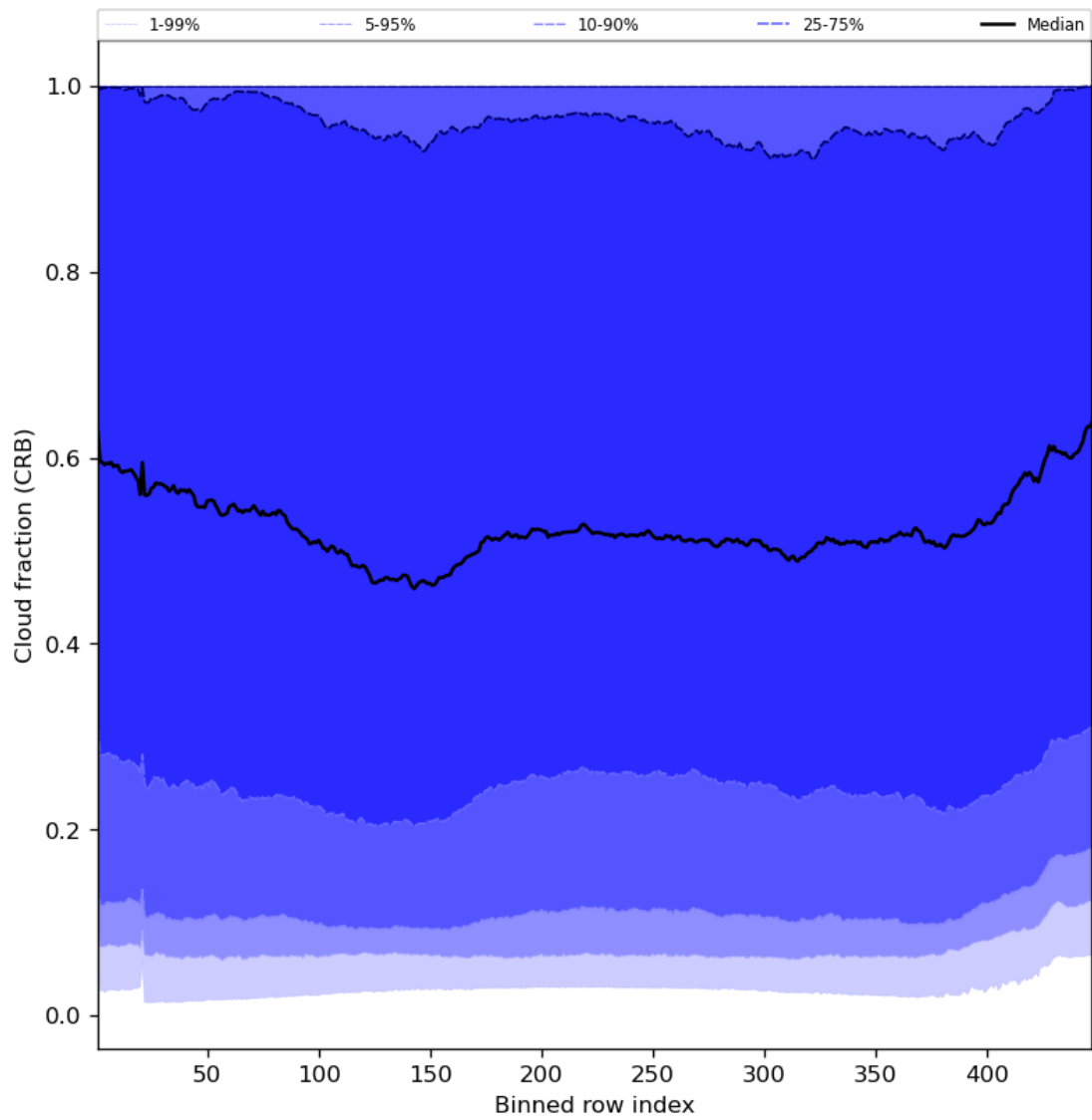
Figure 58: Along track statistics of “Cloud fraction (CRB)” for 2023-11-08 to 2023-11-10
