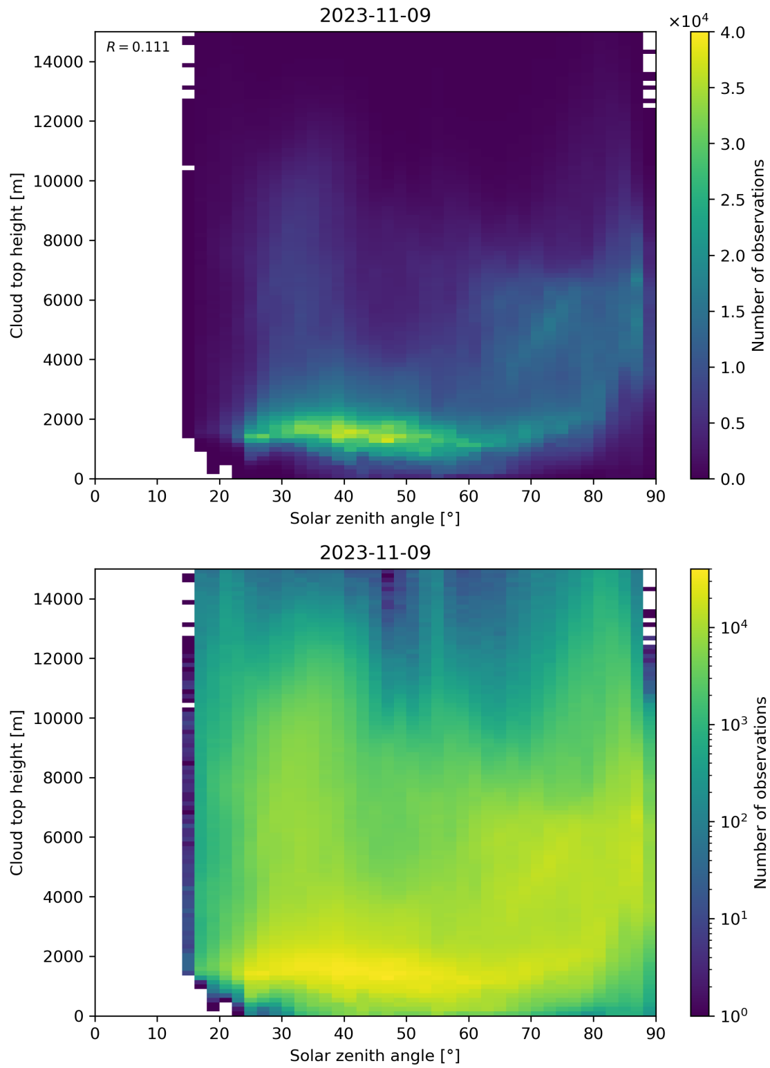
Figure 104: Scatter density plot of “Solar zenith angle” against “Cloud top height” for 2023-11-08 to 2023-11-10.
