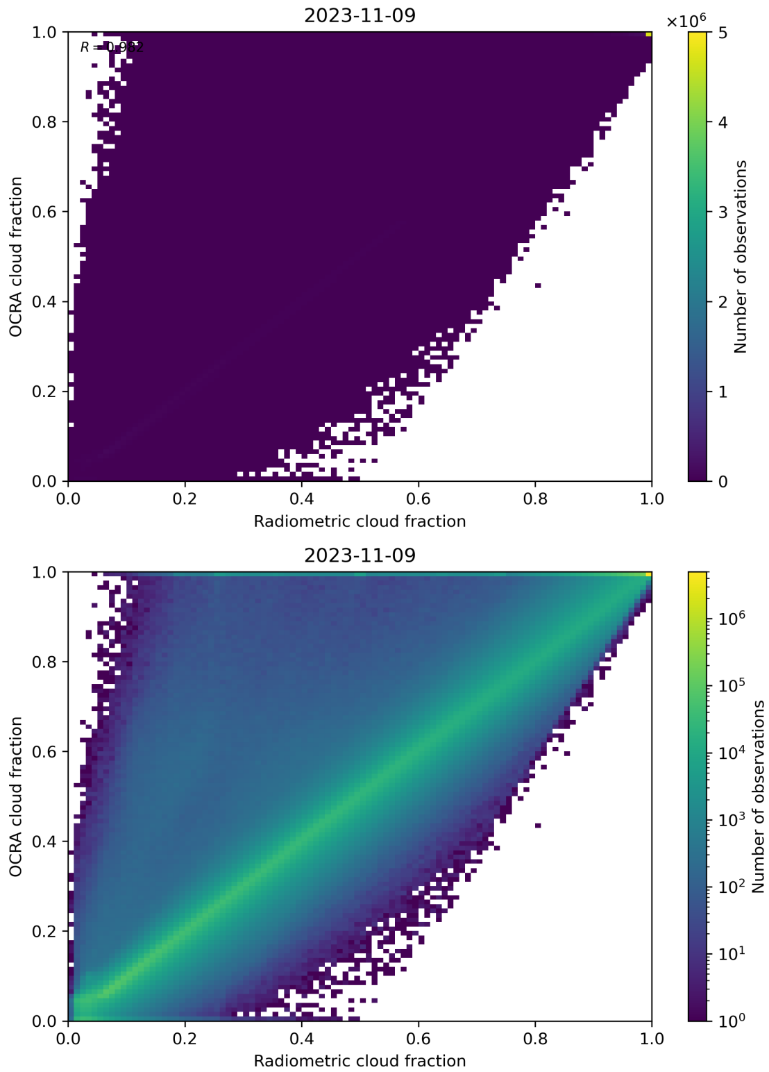
Figure 72: Scatter density plot of “Radiometric cloud fraction” against “OCRA cloud fraction” for 2023-11-08 to 2023-11-10.
