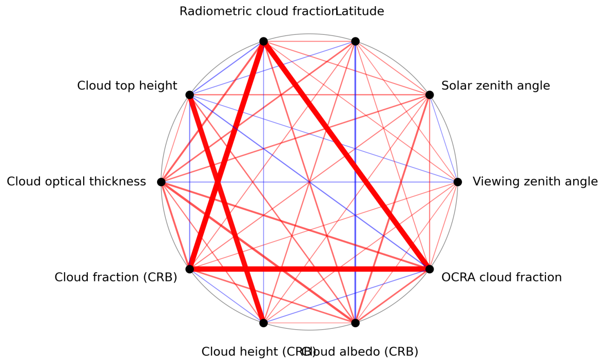
Figure 1: Map of correlation graph for 2023-11-08 to 2023-11-10.
