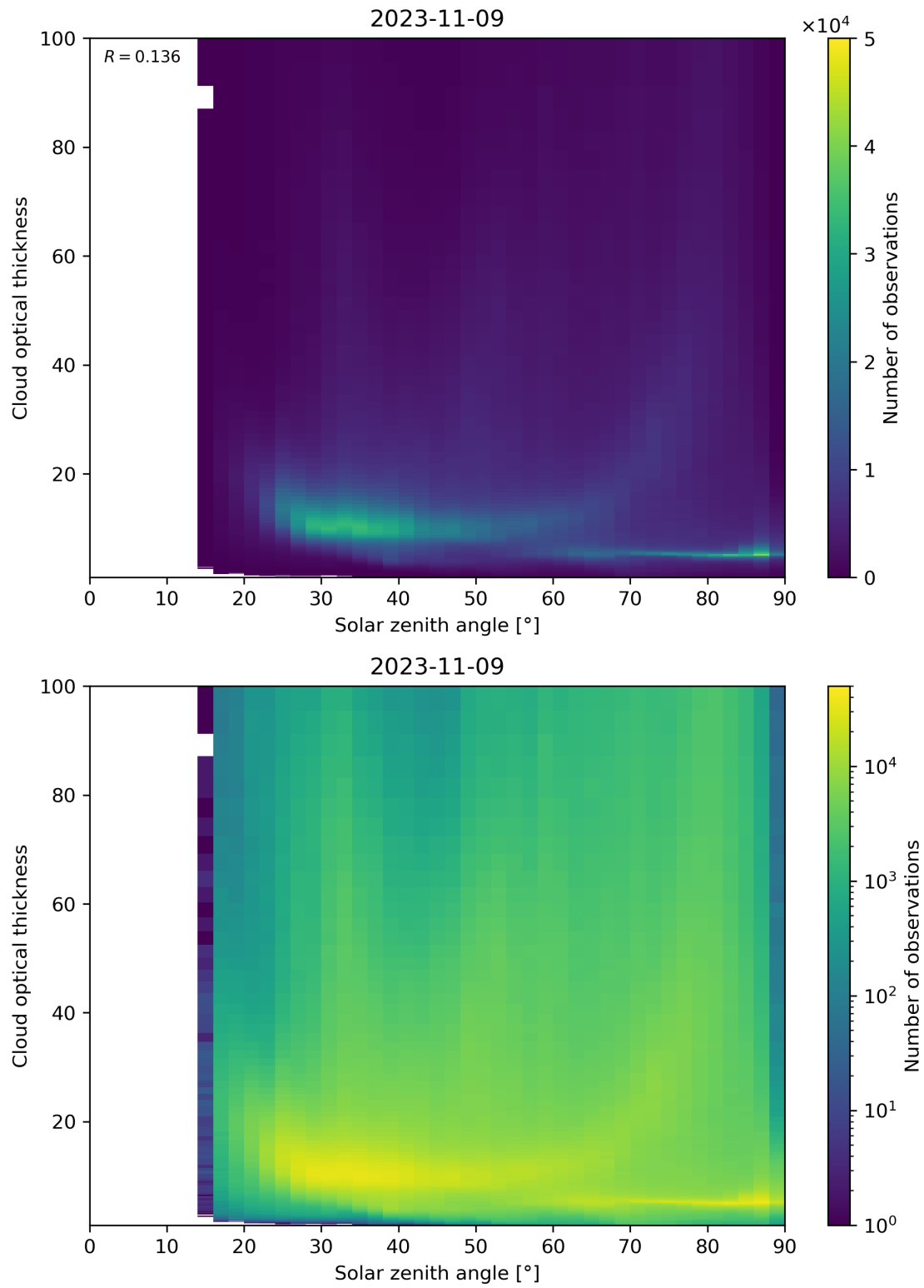
Figure 103: Scatter density plot of “Solar zenith angle” against “Cloud optical thickness” for 2023-11-08 to 2023-11-10.
