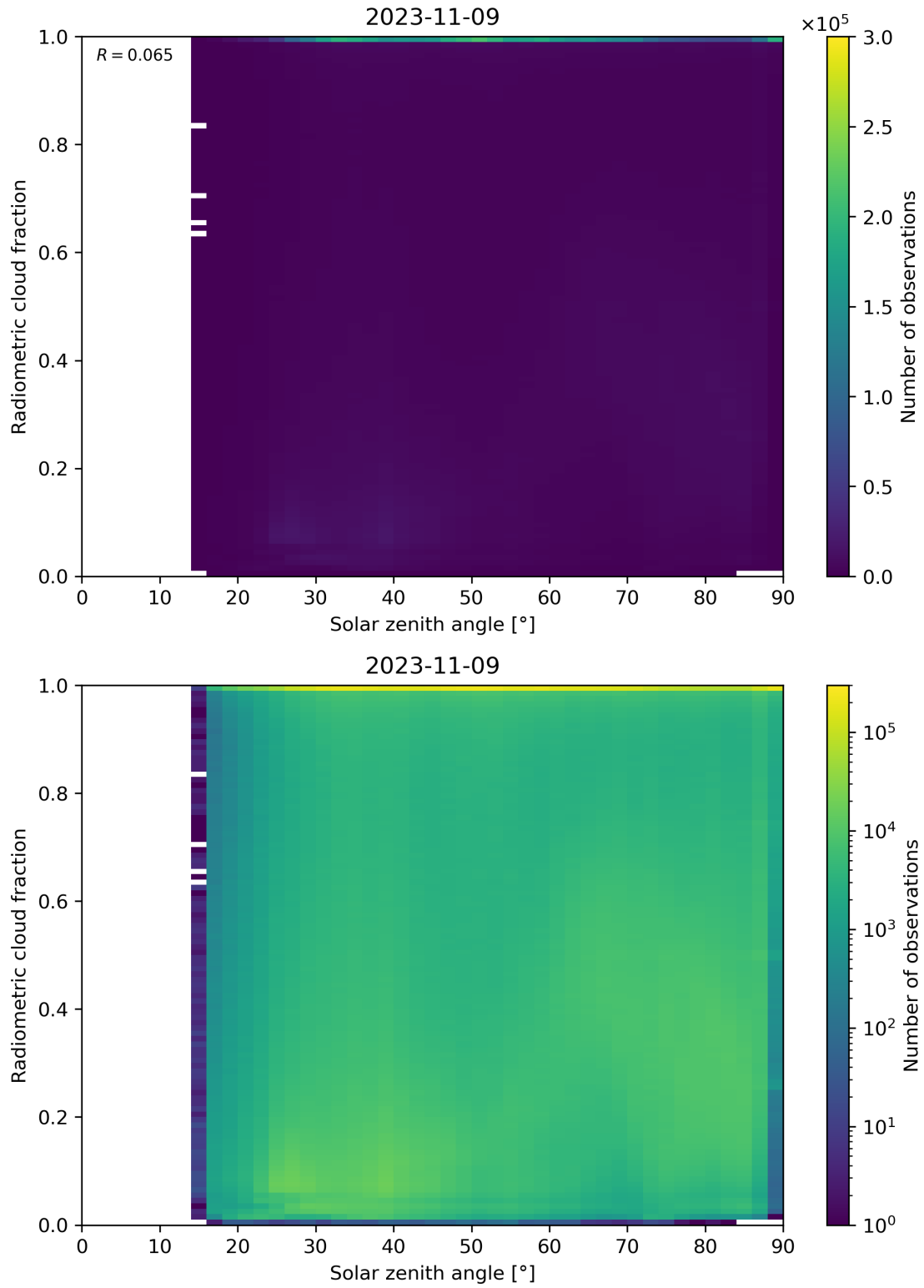
Figure 99: Scatter density plot of “Solar zenith angle” against “Radiometric cloud fraction” for 2023-11-08 to 2023-11-10.
