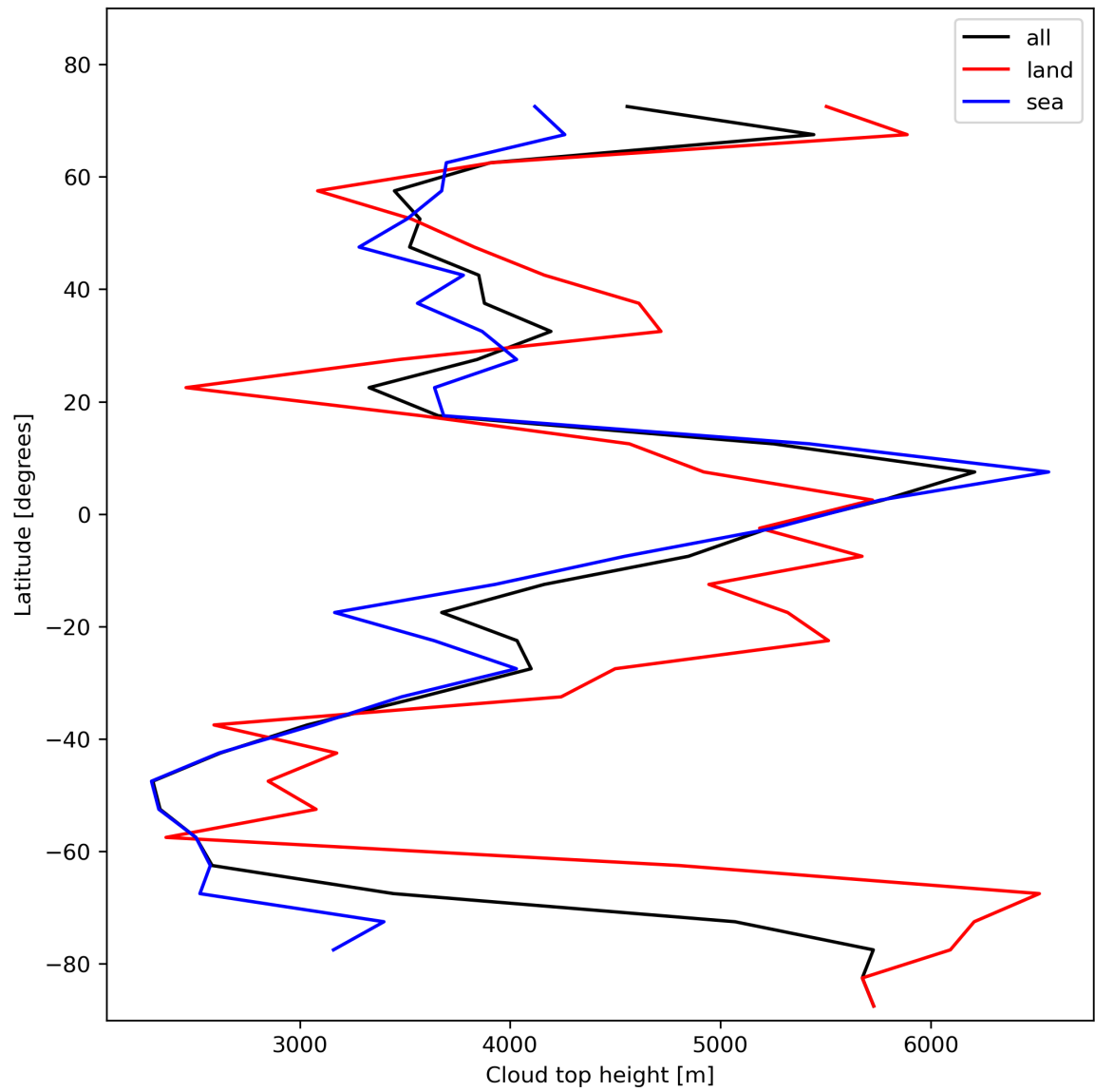
Figure 24: Zonal average of “Cloud top height” for 2023-11-08 to 2023-11-10.
