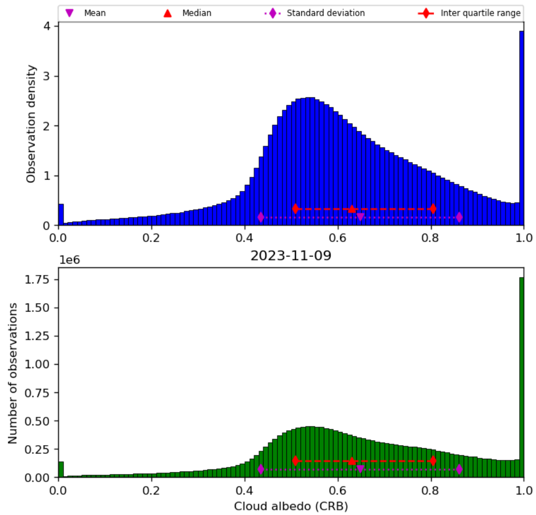
Figure 44: Histogram of “Cloud albedo (CRB)” for 2023-11-08 to 2023-11-10
