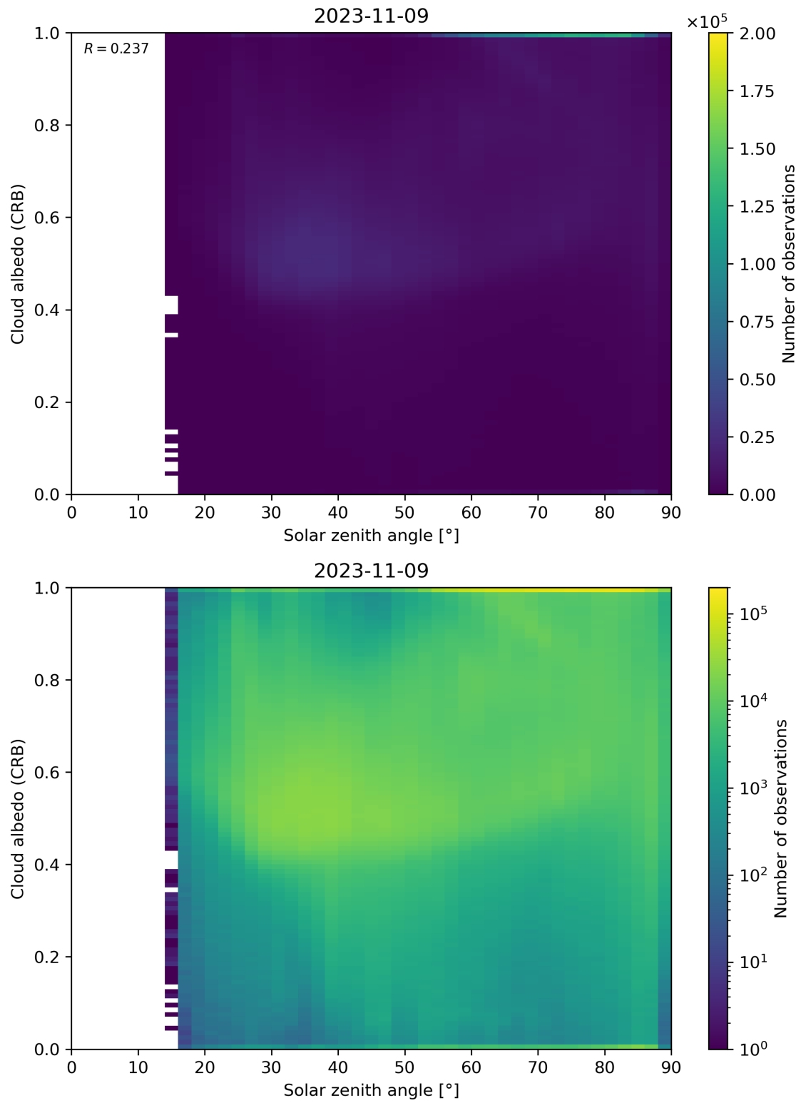
Figure 98: Scatter density plot of “Solar zenith angle” against “Cloud albedo (CRB)” for 2023-11-08 to 2023-11-10.
