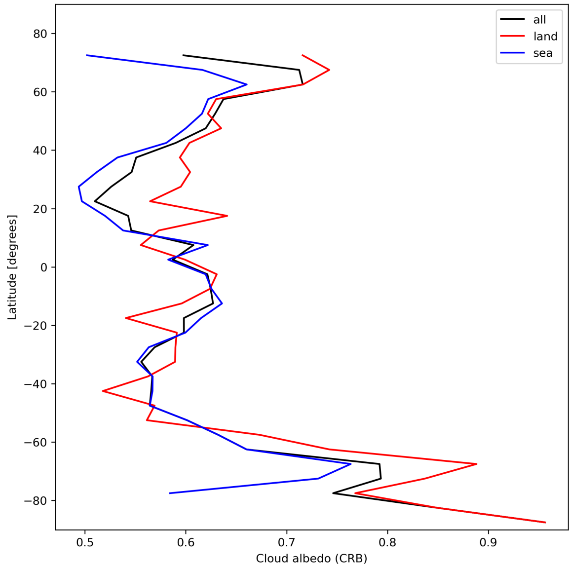
Figure 28: Zonal average of “Cloud albedo (CRB)” for 2023-11-08 to 2023-11-10.
