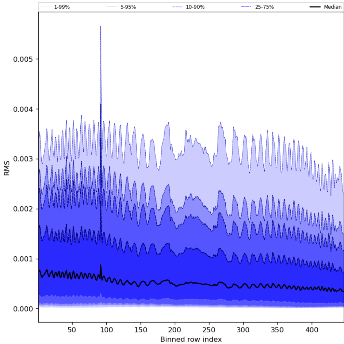
Figure 63: Along track statistics of “RMS” for 2023-11-08 to 2023-11-10
