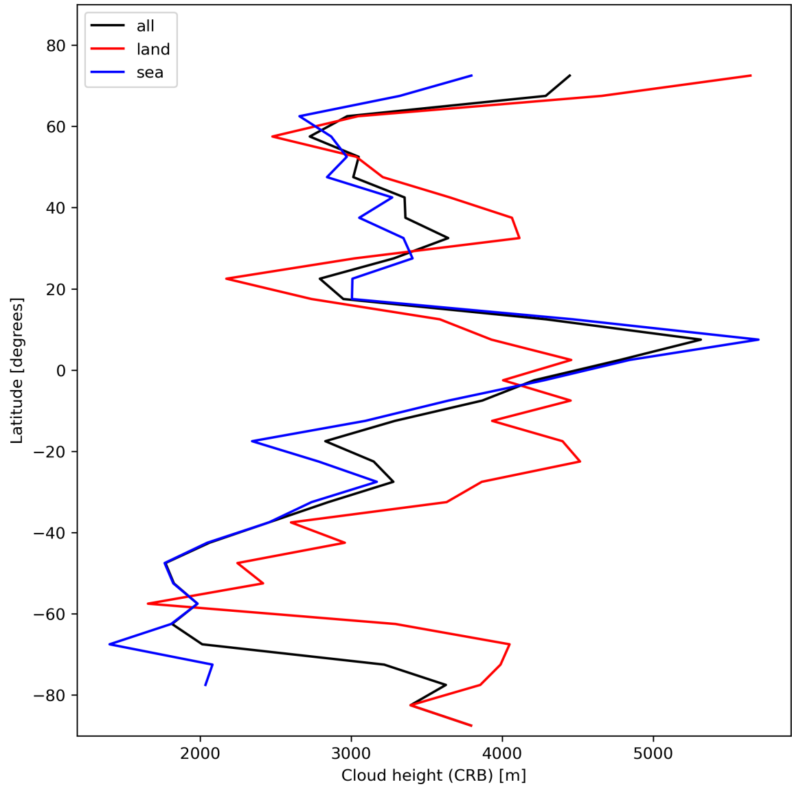
Figure 27: Zonal average of “Cloud height (CRB)” for 2023-11-08 to 2023-11-10.
