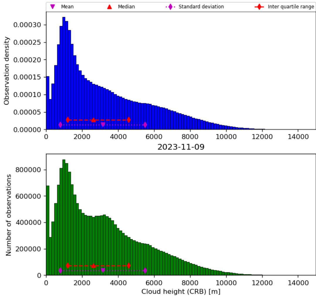
Figure 43: Histogram of “Cloud height (CRB)” for 2023-11-08 to 2023-11-10
