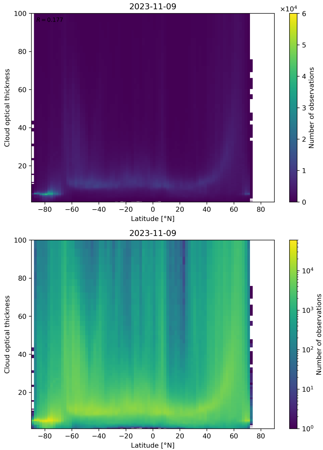
Figure 96: Scatter density plot of “Latitude” against “Cloud optical thickness” for 2023-11-08 to 2023-11-10.
