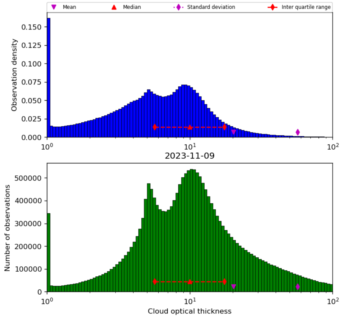
Figure 41: Histogram of “Cloud optical thickness” for 2023-11-08 to 2023-11-10
