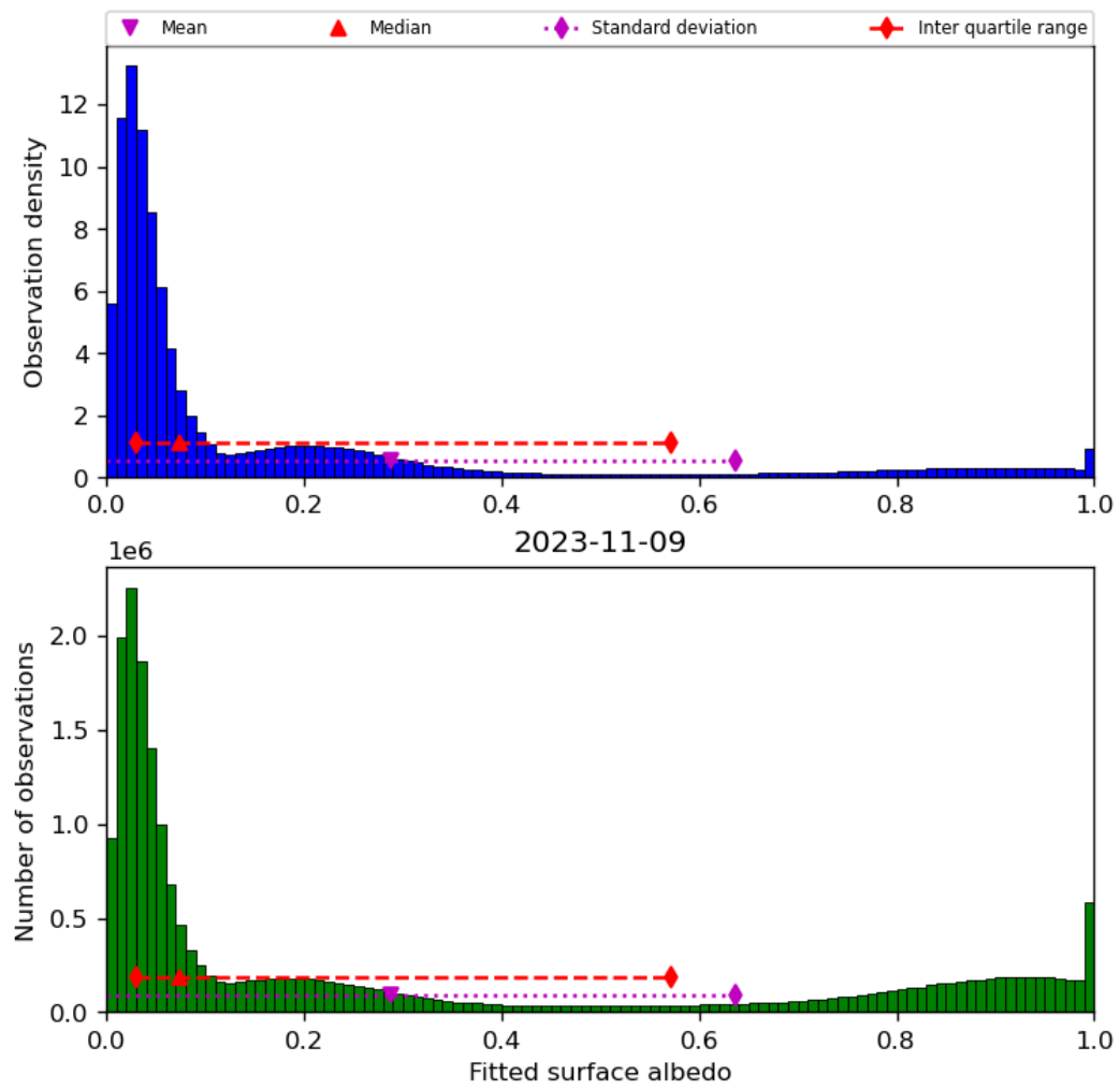
Figure 45: Histogram of “Fitted surface albedo” for 2023-11-08 to 2023-11-10
