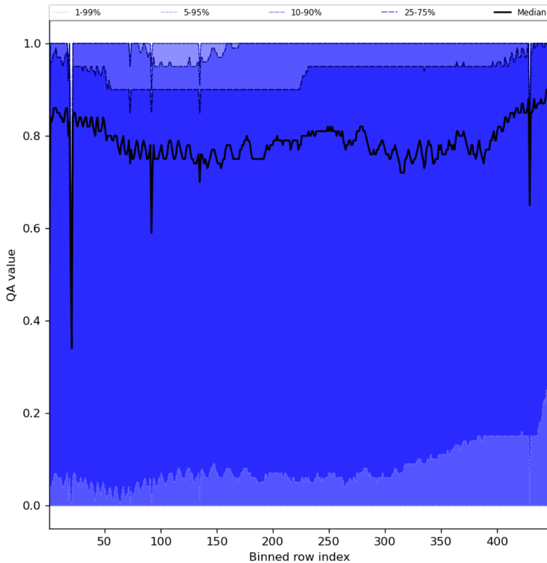
Figure 54: Along track statistics of “QA value” for 2023-11-08 to 2023-11-10
