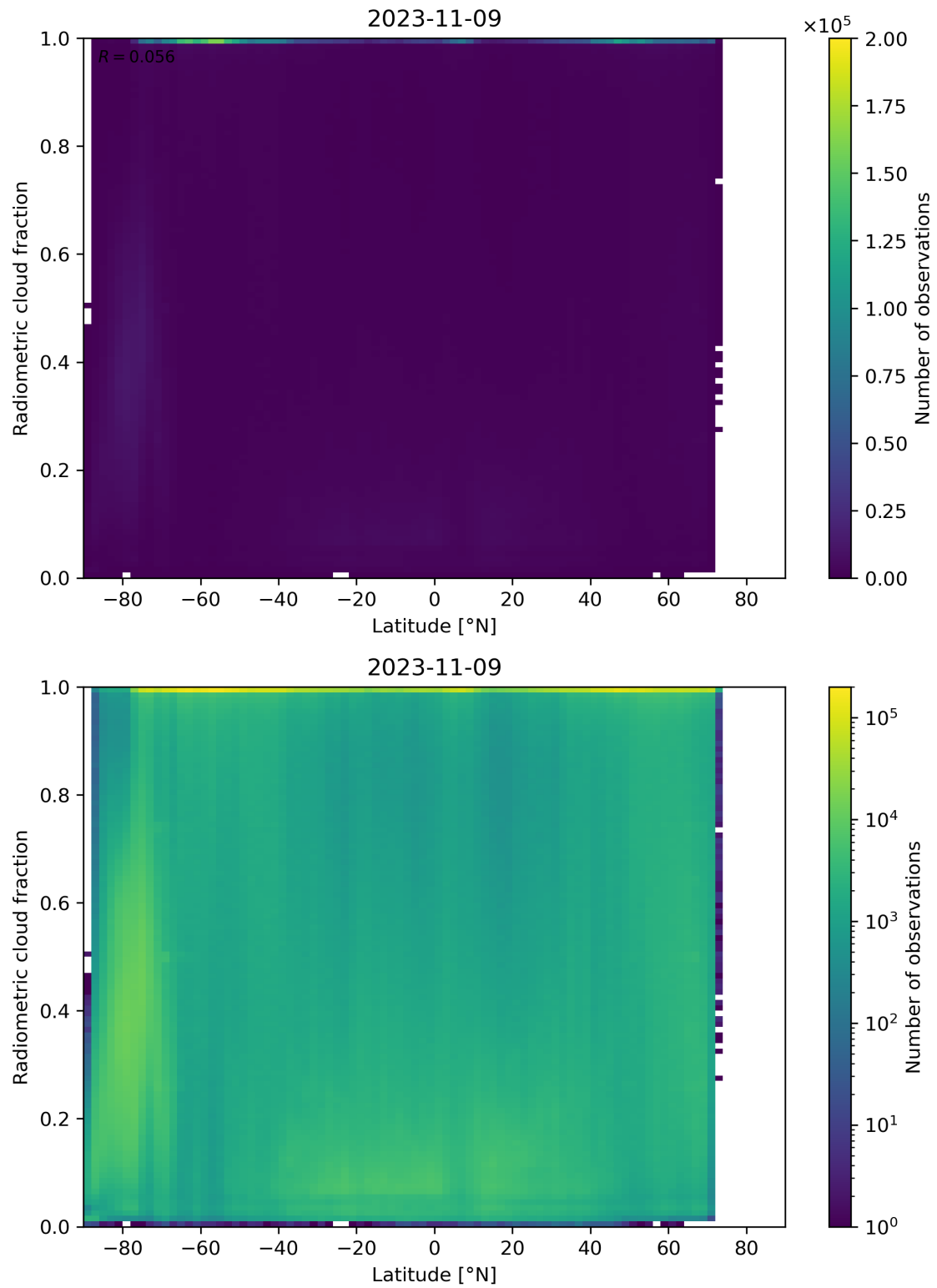
Figure 92: Scatter density plot of “Latitude” against “Radiometric cloud fraction” for 2023-11-08 to 2023-11-10.
