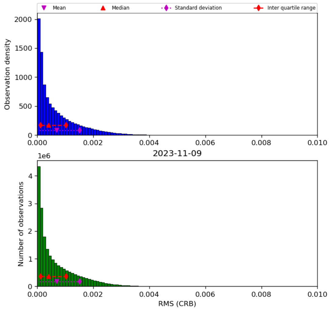
Figure 48: Histogram of “RMS (CRB)” for 2023-11-08 to 2023-11-10
