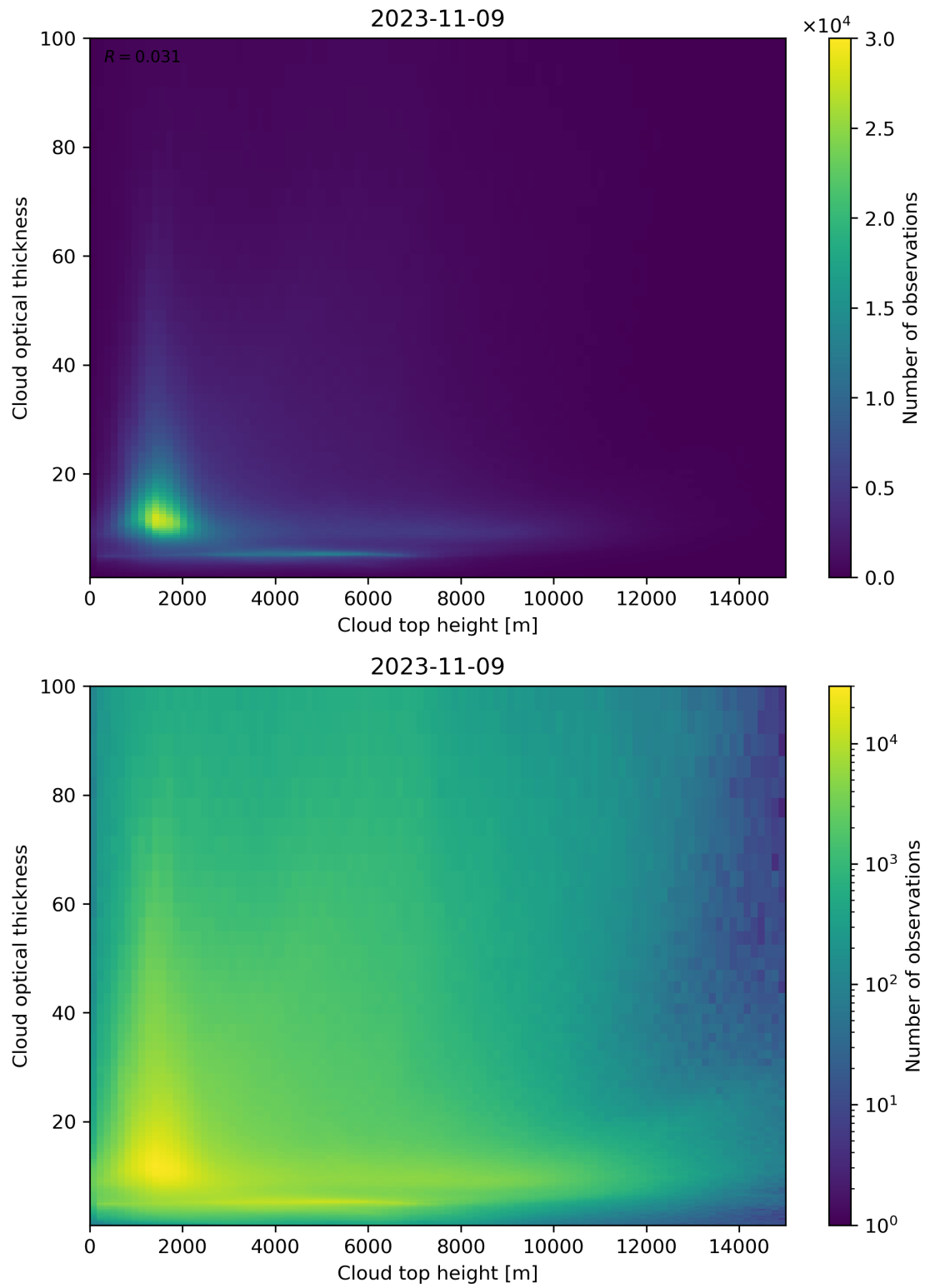
Figure 90: Scatter density plot of “Cloud top height” against “Cloud optical thickness” for 2023-11-08 to 2023-11-10.
