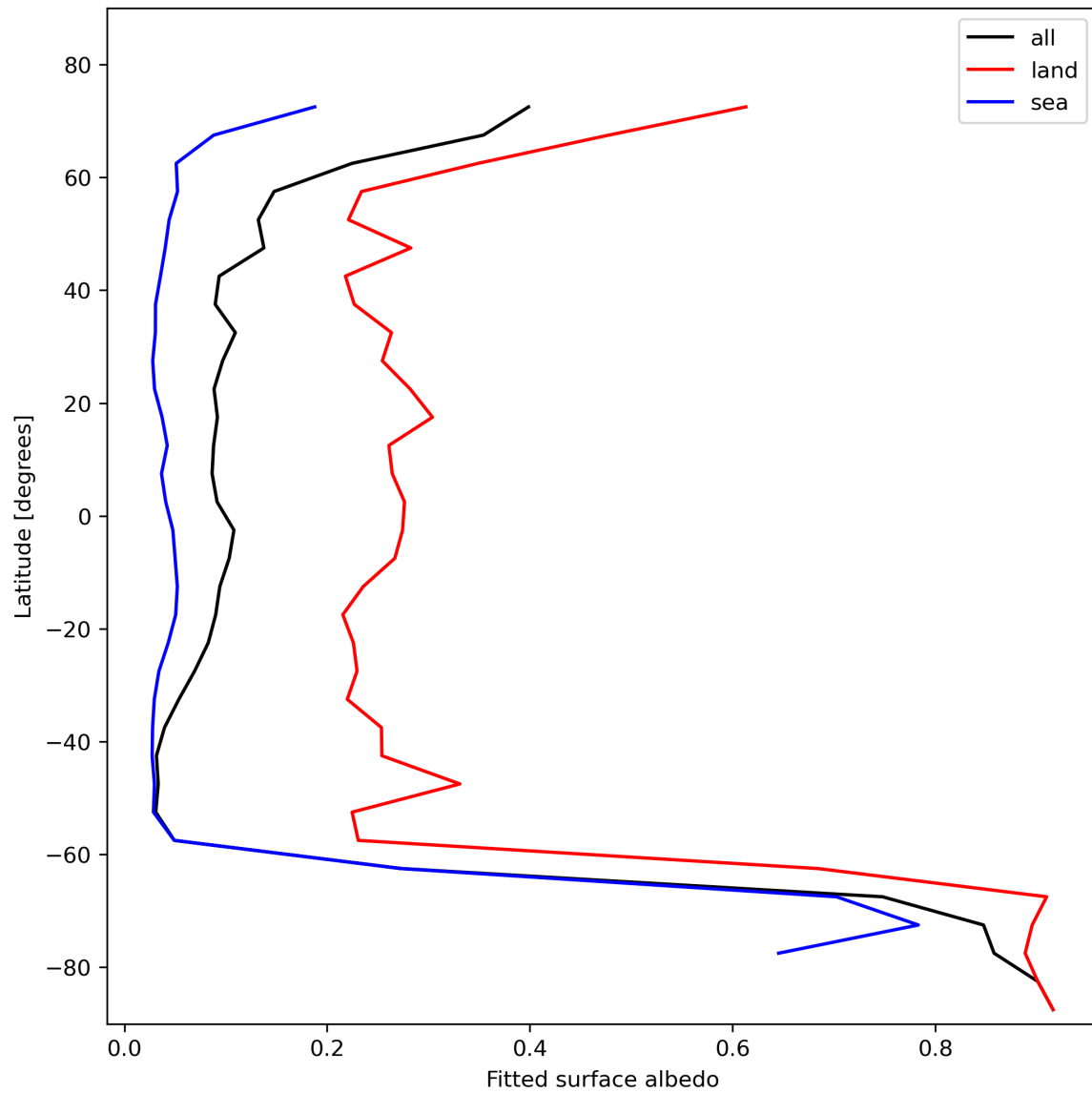
Figure 29: Zonal average of “Fitted surface albedo” for 2023-11-08 to 2023-11-10.
