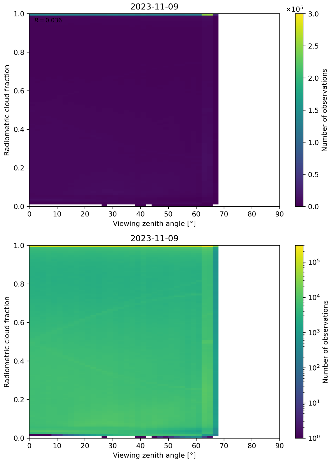
Figure 107: Scatter density plot of “Viewing zenith angle” against “Radiometric cloud fraction” for 2023-11-08 to 2023-11-10.
