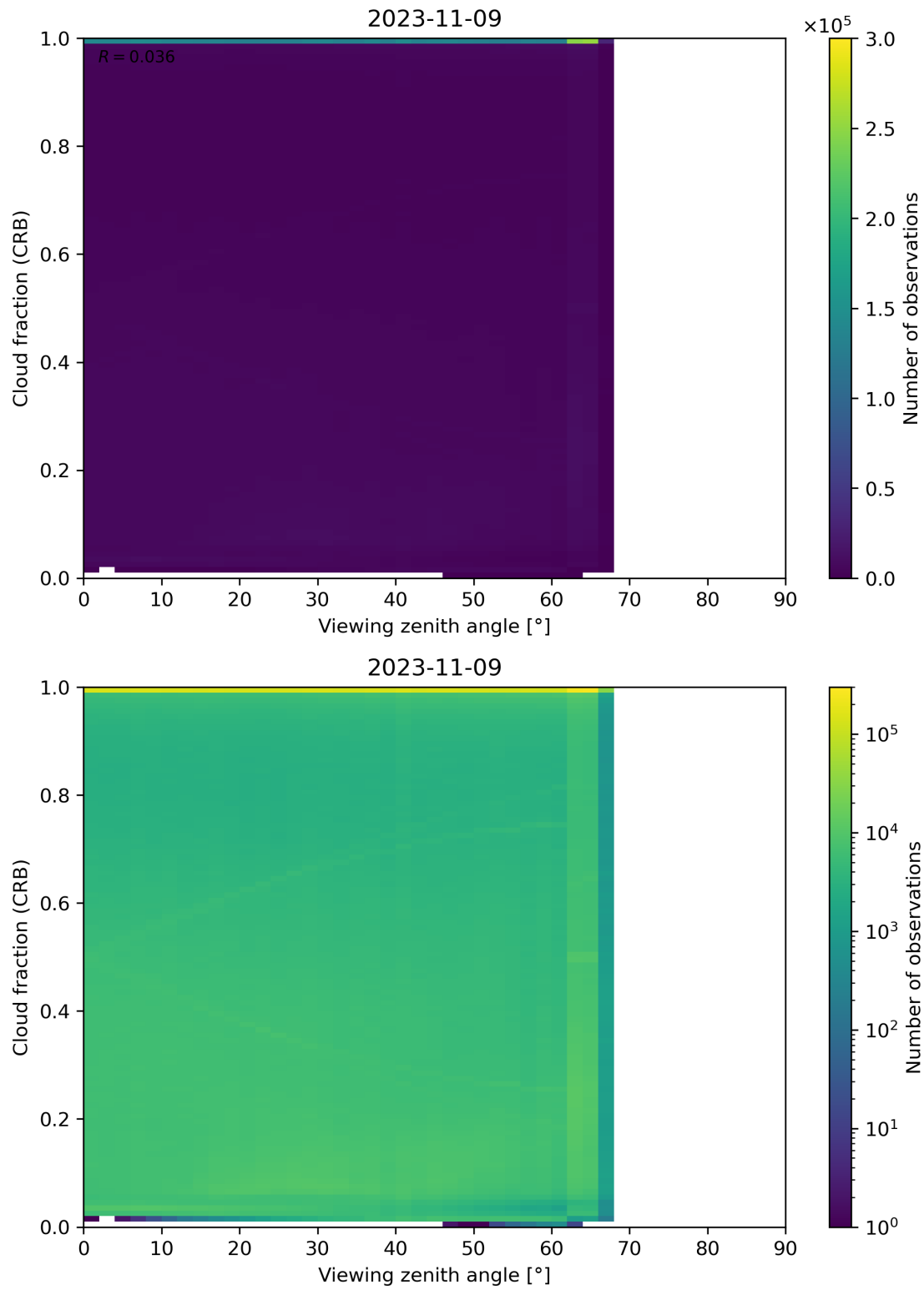
Figure 109: Scatter density plot of “Viewing zenith angle” against “Cloud fraction (CRB)” for 2023-11-08 to 2023-11-10.
