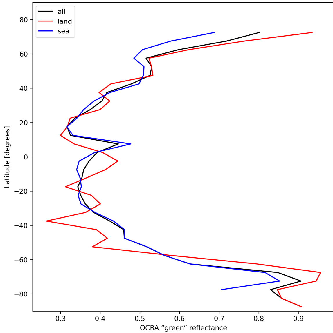
Figure 36: Zonal average of “OCRA “green” reflectance” for 2023-11-08 to 2023-11-10.
