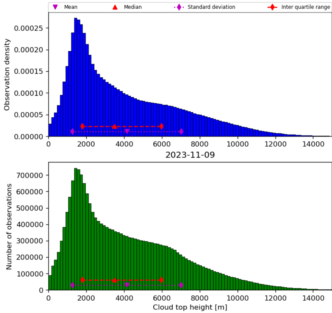
Figure 40: Histogram of “Cloud top height” for 2023-11-08 to 2023-11-10
