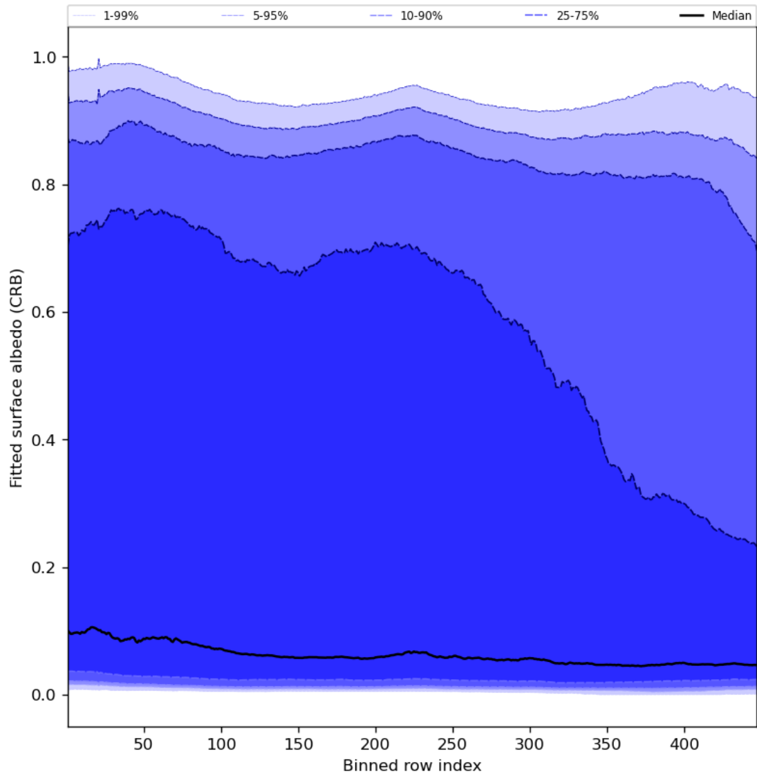
Figure 62: Along track statistics of “Fitted surface albedo (CRB)” for 2023-11-08 to 2023-11-10
