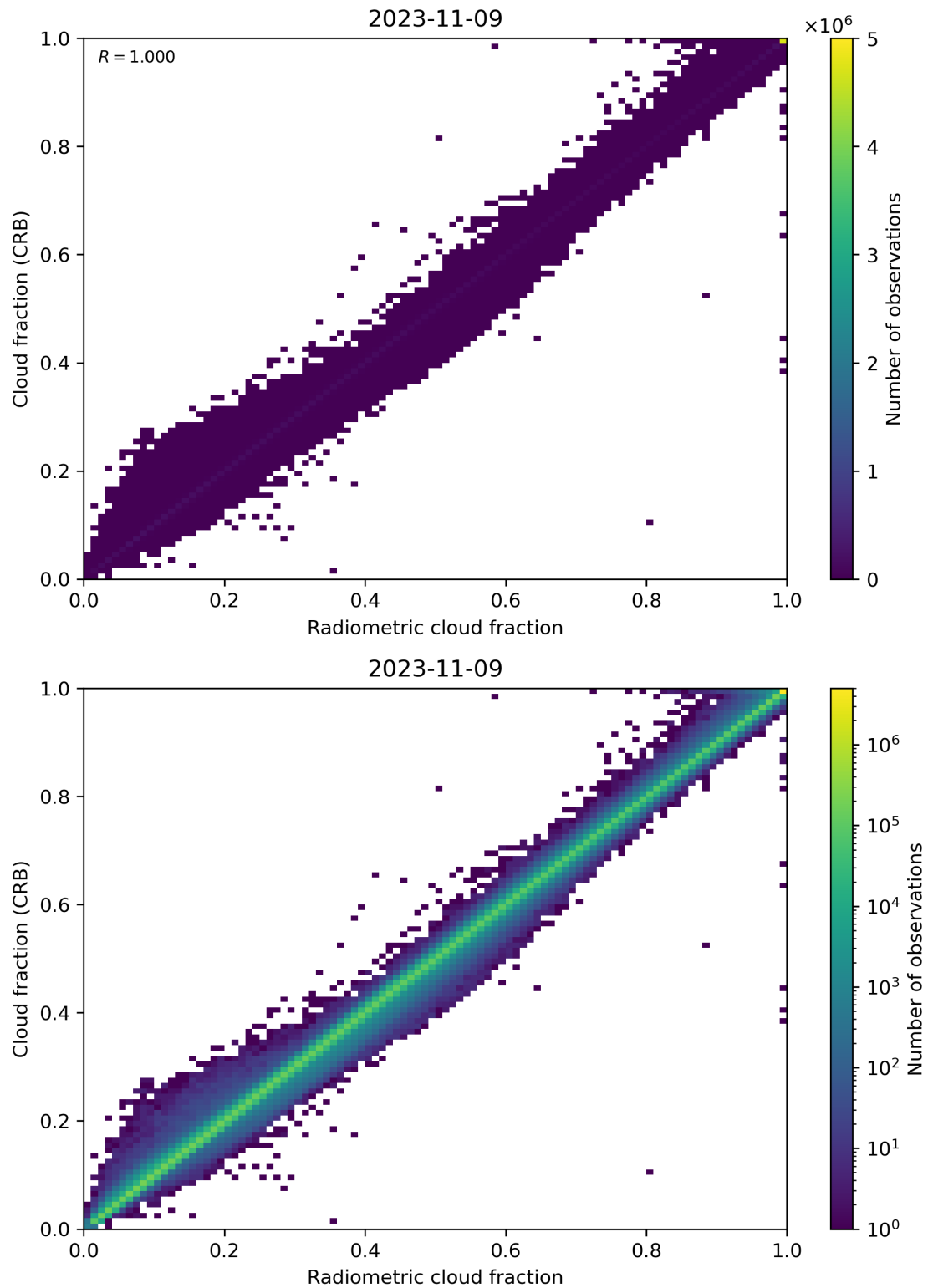
Figure 73: Scatter density plot of “Radiometric cloud fraction” against “Cloud fraction (CRB)” for 2023-11-08 to 2023-11-10.
