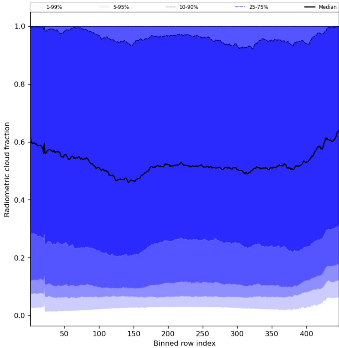
Figure 55: Along track statistics of “Radiometric cloud fraction” for 2023-11-08 to 2023-11-10
