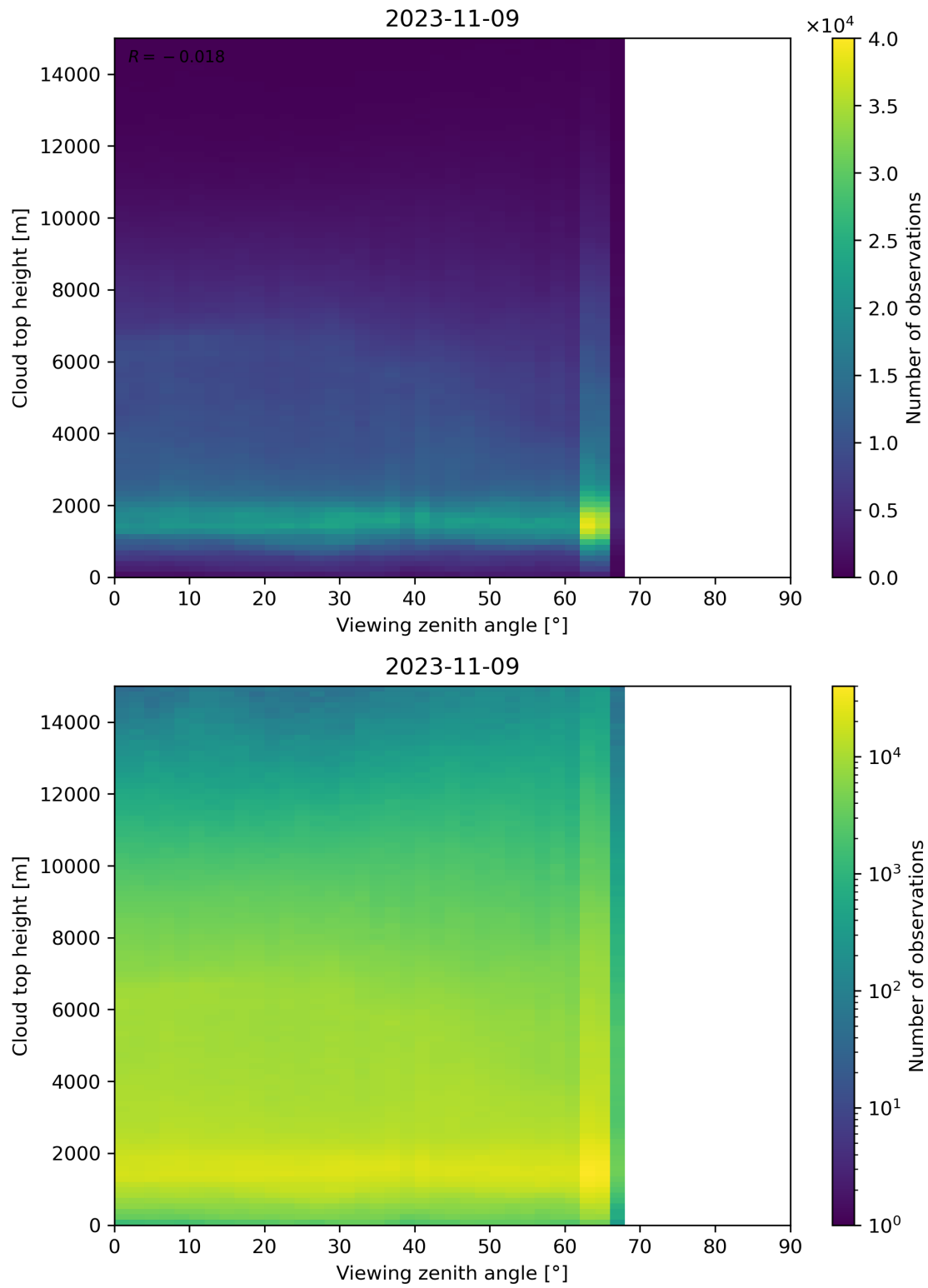
Figure 112: Scatter density plot of “Viewing zenith angle” against “Cloud top height” for 2023-11-08 to 2023-11-10.
