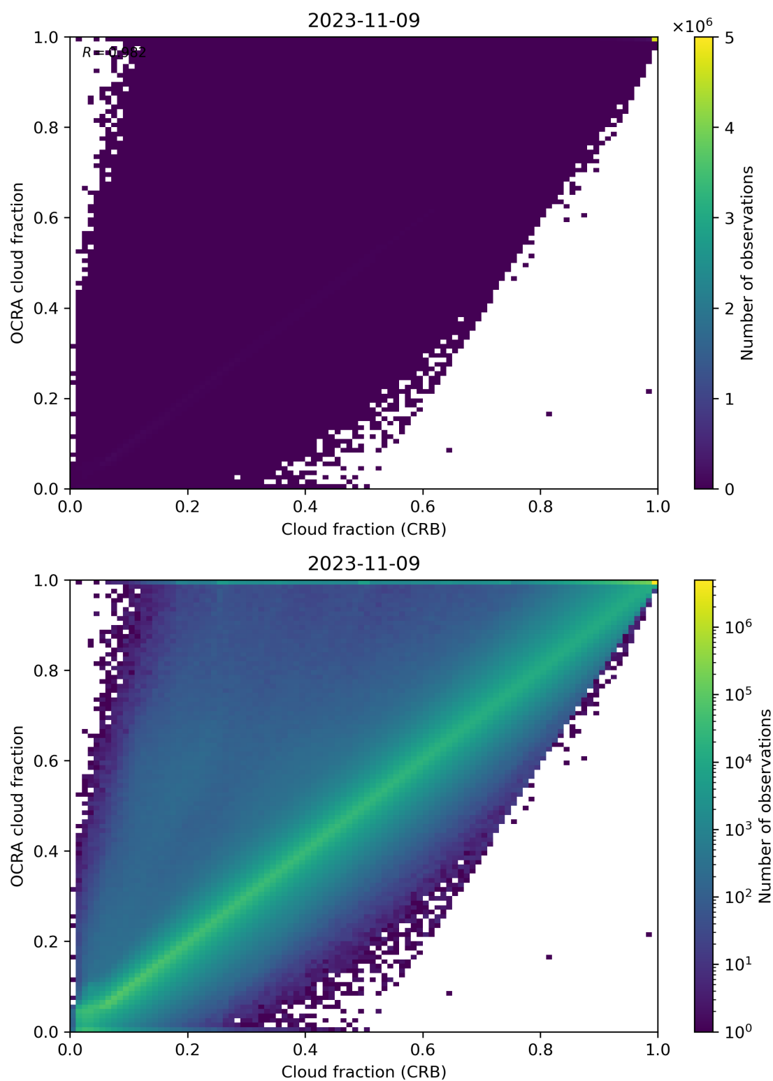
Figure 78: Scatter density plot of “Cloud fraction (CRB)” against “OCRA cloud fraction” for 2023-11-08 to 2023-11-10.
