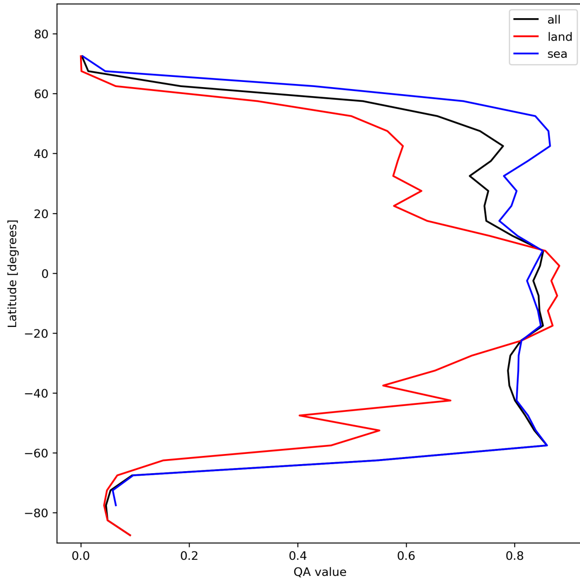
Figure 22: Zonal average of “QA value” for 2023-11-08 to 2023-11-10.
