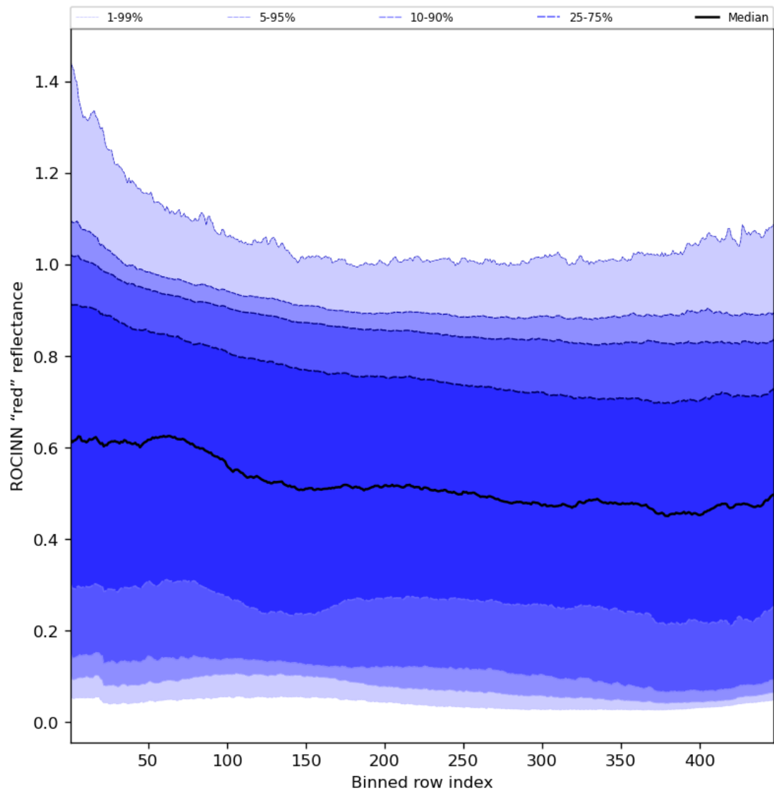
Figure 69: Along track statistics of “ROCINN “red” reflectance” for 2023-11-08 to 2023-11-10
