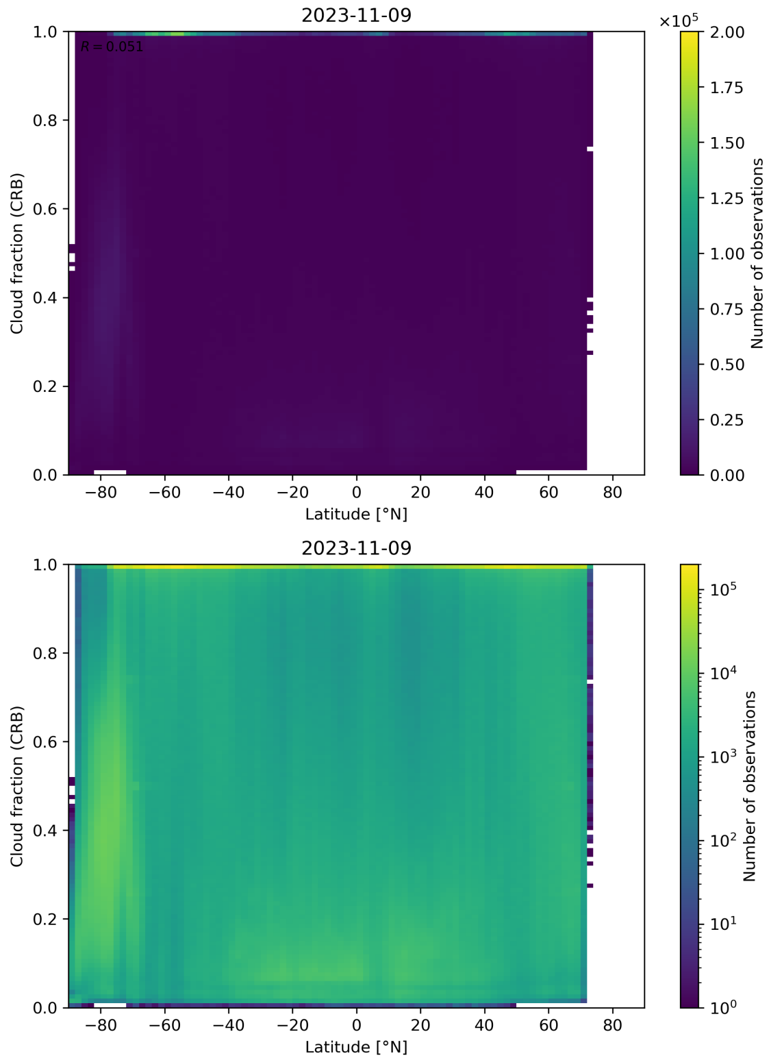
Figure 94: Scatter density plot of “Latitude” against “Cloud fraction (CRB)” for 2023-11-08 to 2023-11-10.
