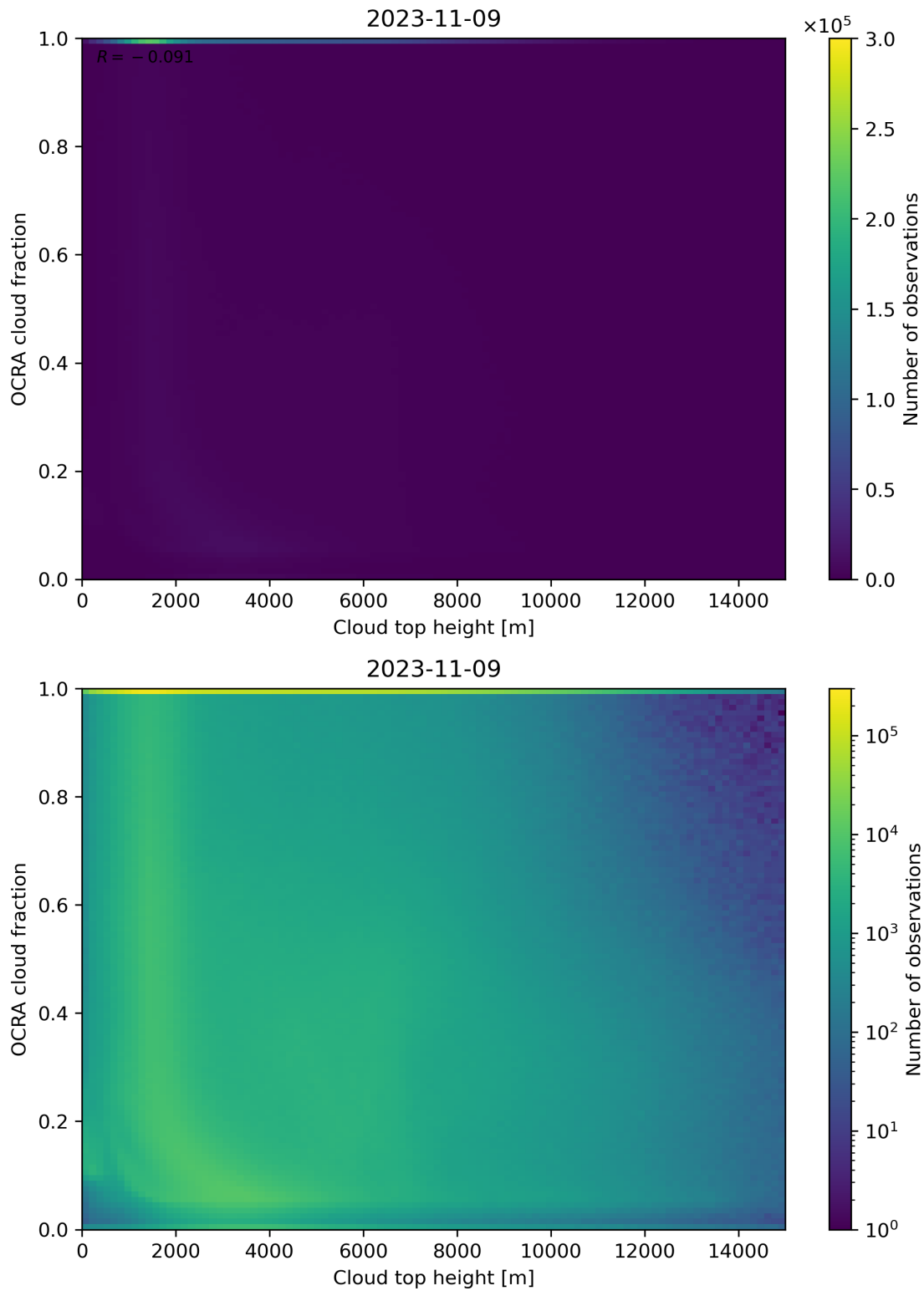
Figure 87: Scatter density plot of “Cloud top height” against “OCRA cloud fraction” for 2023-11-08 to 2023-11-10.
