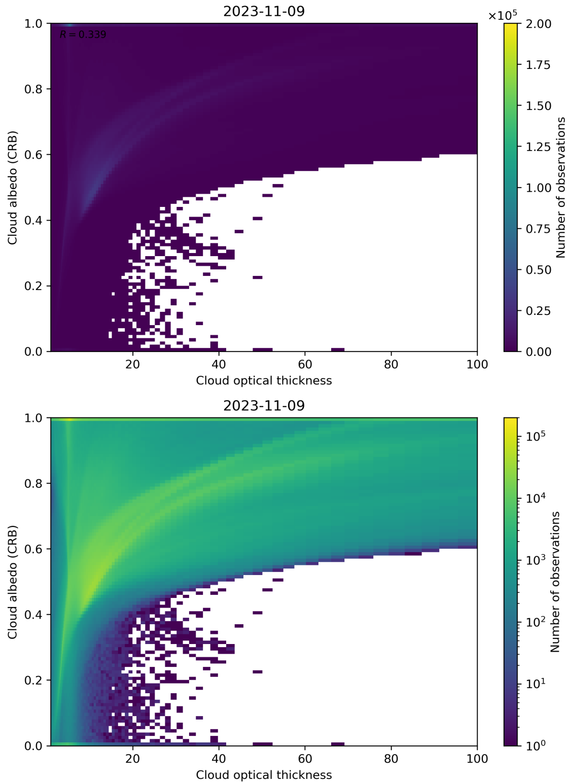
Figure 82: Scatter density plot of “Cloud optical thickness” against “Cloud albedo (CRB)” for 2023-11-08 to 2023-11-10.
