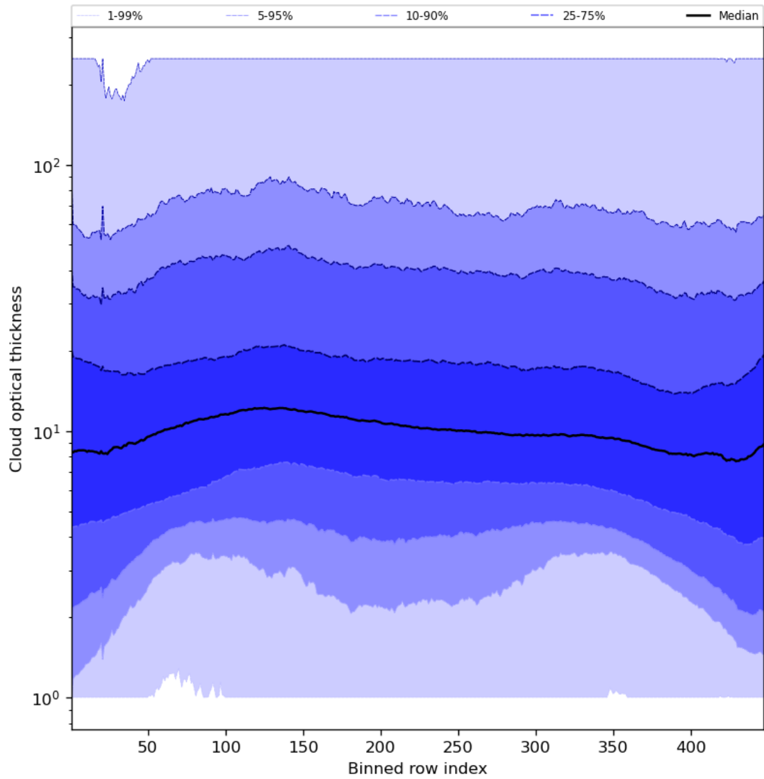
Figure 57: Along track statistics of “Cloud optical thickness” for 2023-11-08 to 2023-11-10
