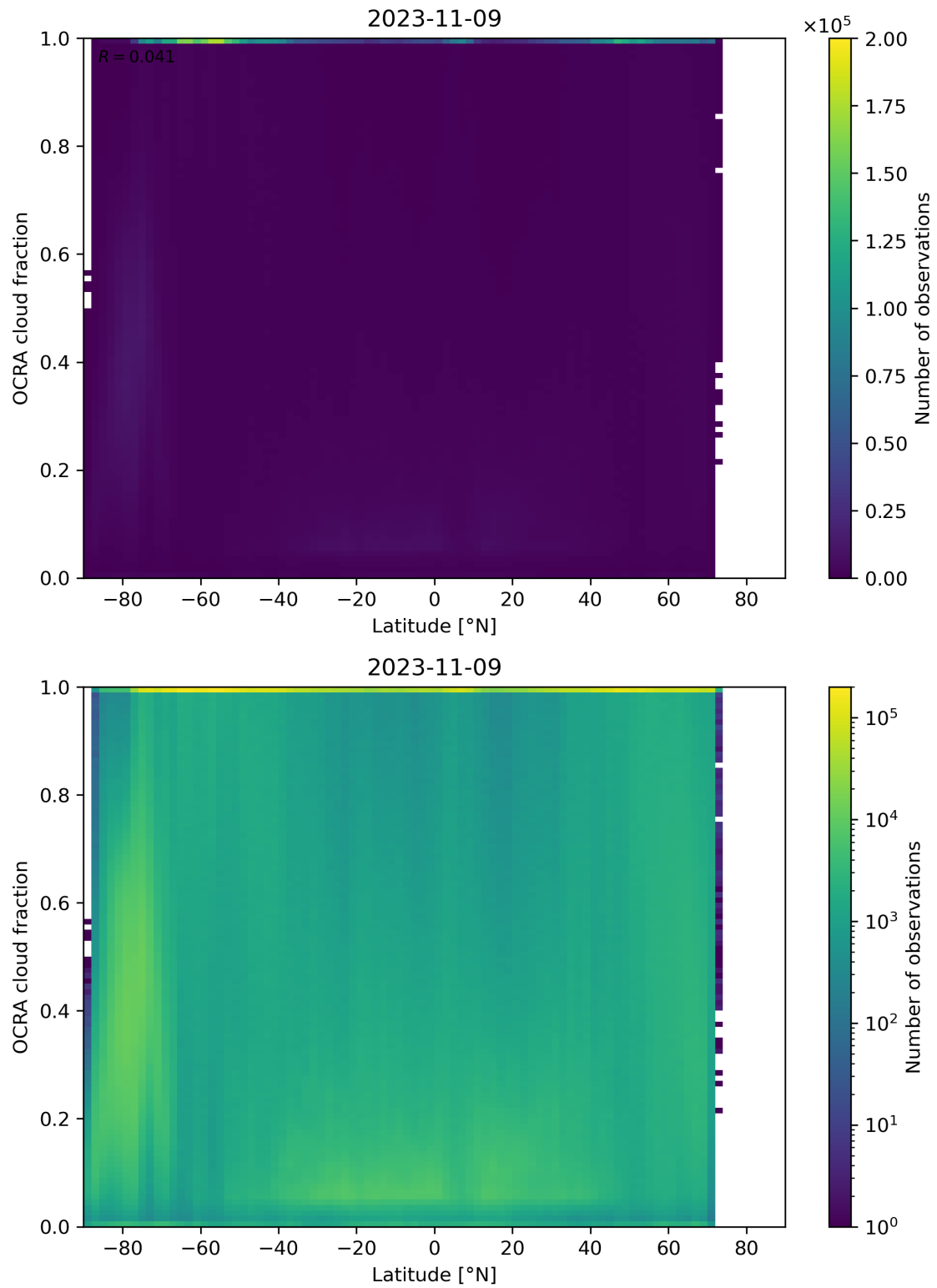
Figure 93: Scatter density plot of “Latitude” against “OCRA cloud fraction” for 2023-11-08 to 2023-11-10.
