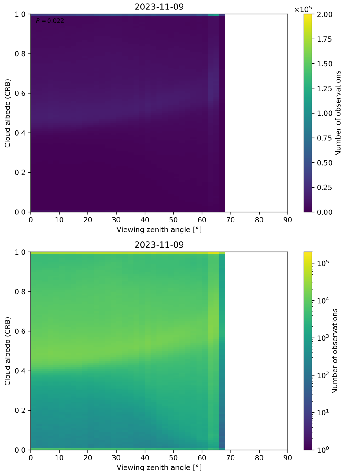
Figure 106: Scatter density plot of “Viewing zenith angle” against “Cloud albedo (CRB)” for 2023-11-08 to 2023-11-10.
