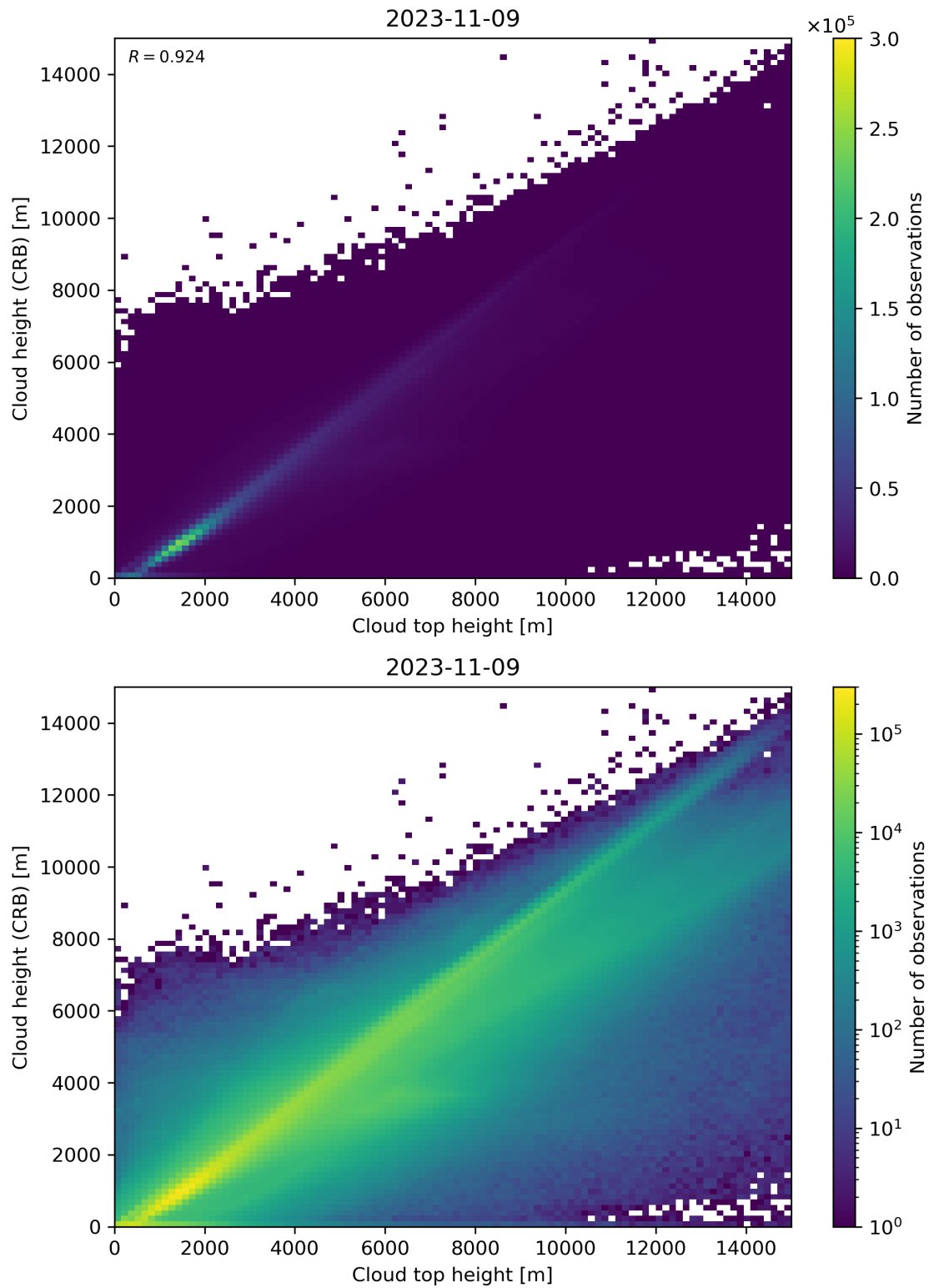
Figure 89: Scatter density plot of “Cloud top height” against “Cloud height (CRB)” for 2023-11-08 to 2023-11-10.
