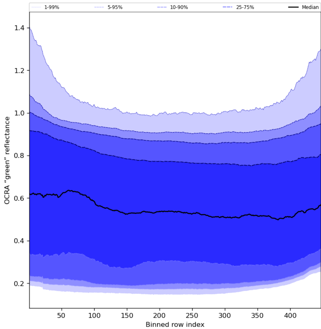
Figure 68: Along track statistics of "OCRA "green" reflectance" for 2023-11-08 to 2023-11-10
