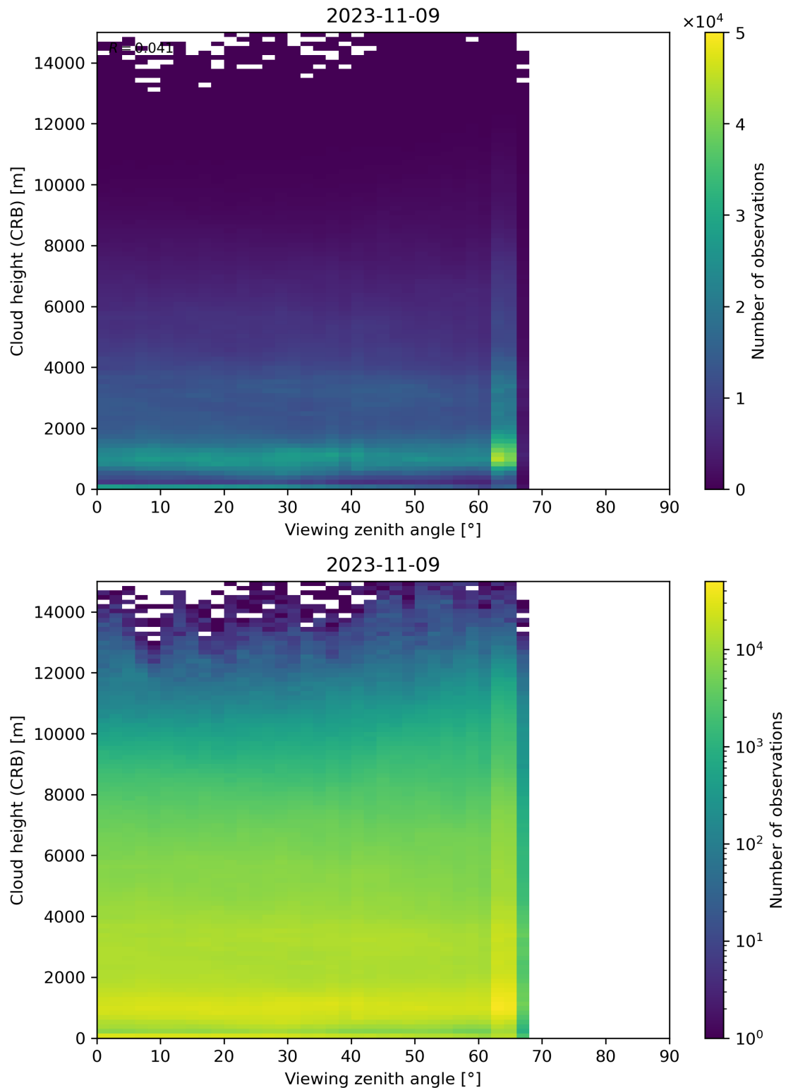
Figure 110: Scatter density plot of “Viewing zenith angle” against “Cloud height (CRB)” for 2023-11-08 to 2023-11-10.
