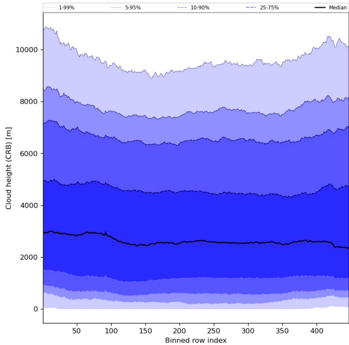
Figure 59: Along track statistics of “Cloud height (CRB)” for 2023-11-08 to 2023-11-10
