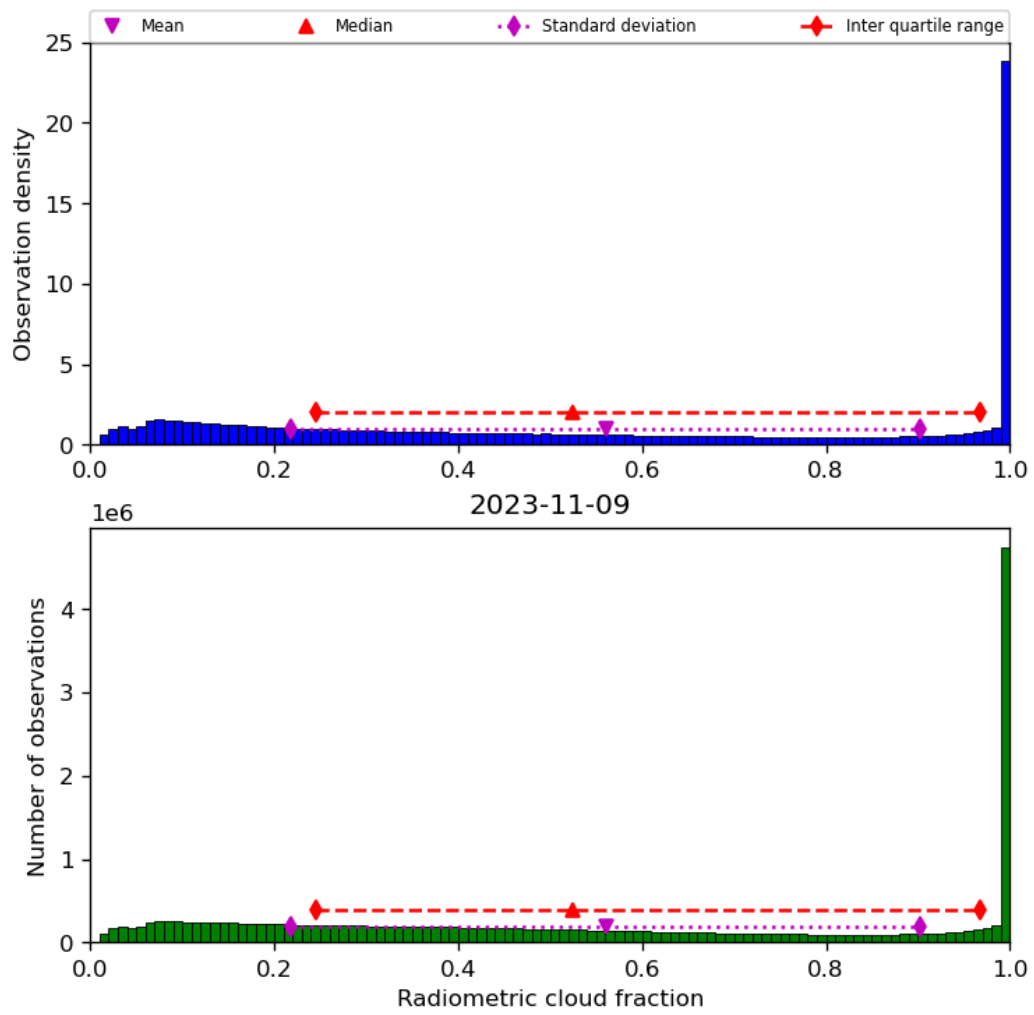
Figure 39: Histogram of “Radiometric cloud fraction” for 2023-11-08 to 2023-11-10
