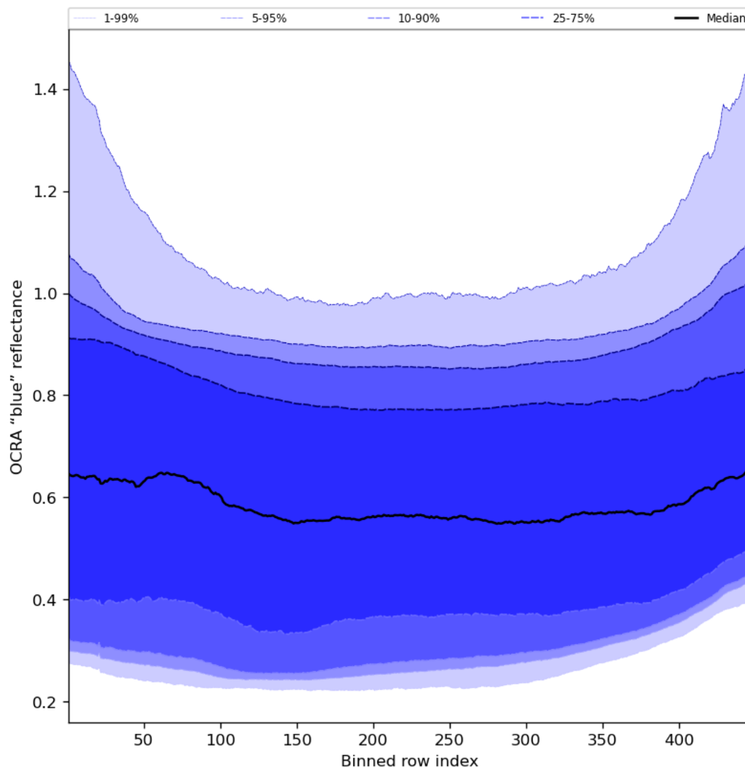
Figure 67: Along track statistics of "OCRA "blue" reflectance" for 2023-11-08 to 2023-11-10
