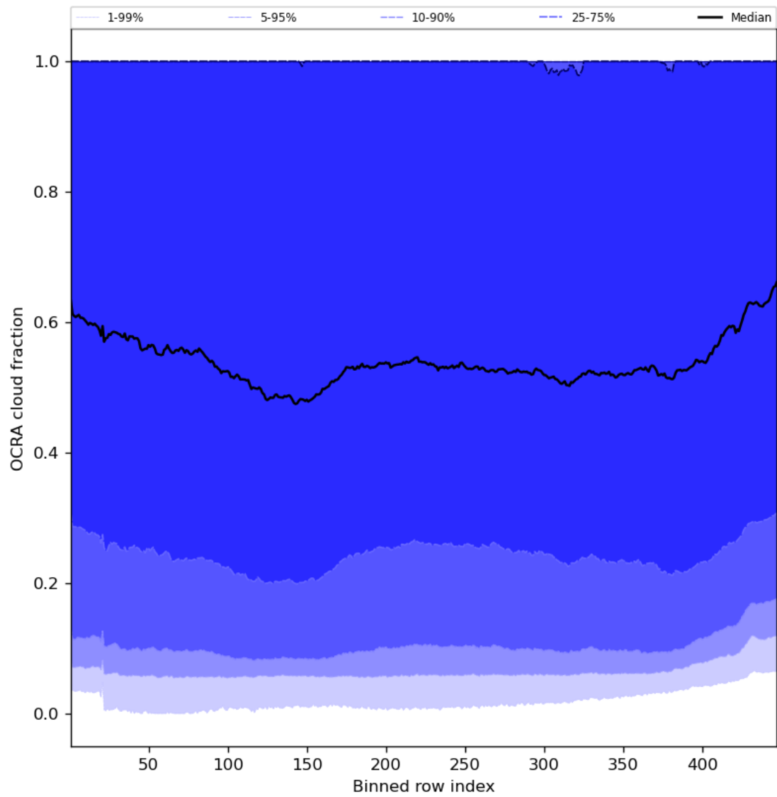
Figure 66: Along track statistics of “OCRA cloud fraction” for 2023-11-08 to 2023-11-10
