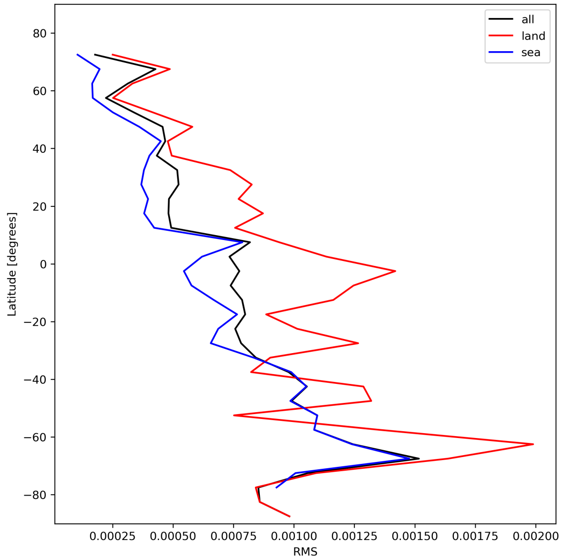
Figure 31: Zonal average of “RMS” for 2023-11-08 to 2023-11-10.
