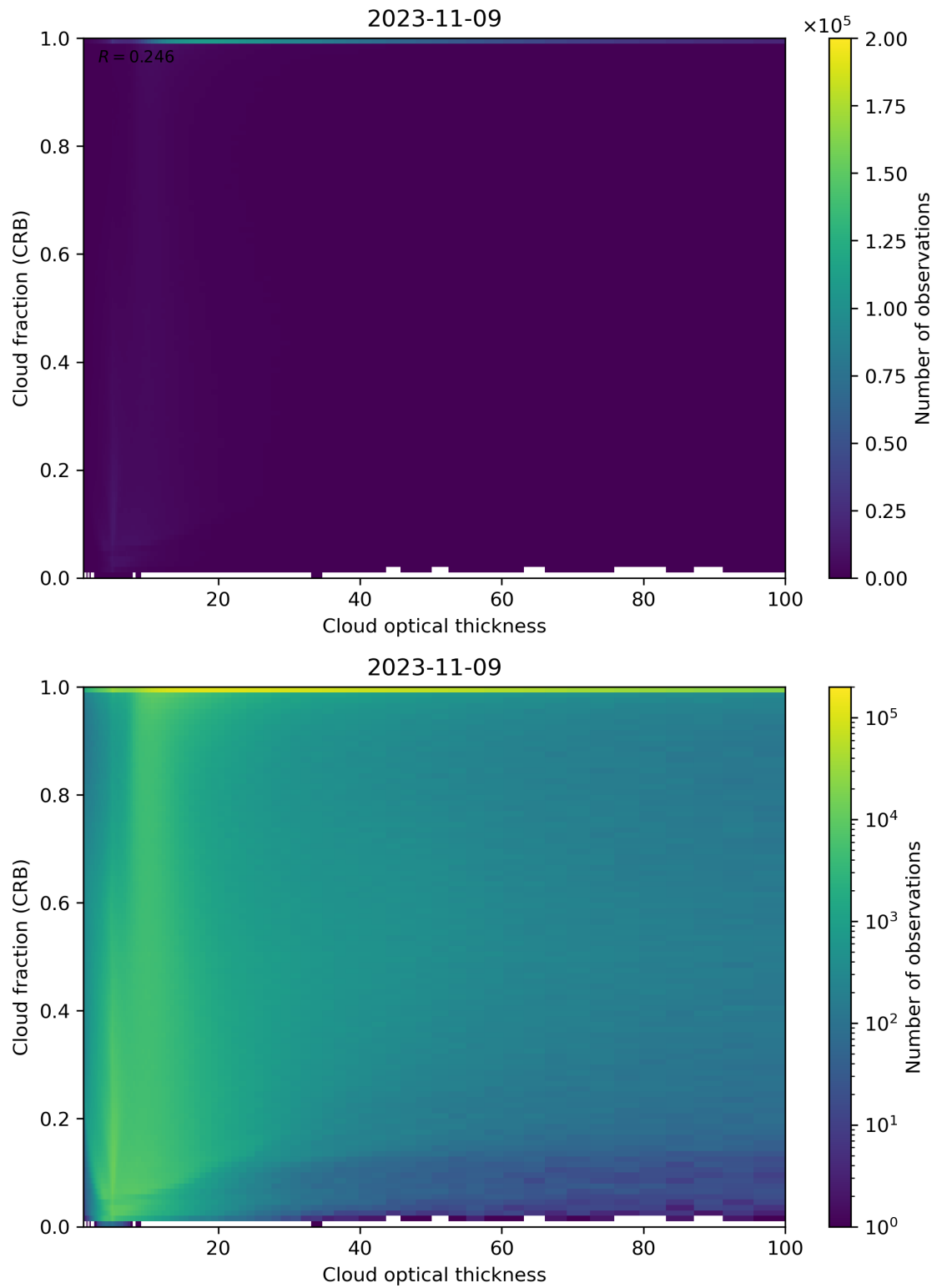
Figure 84: Scatter density plot of “Cloud optical thickness” against “Cloud fraction (CRB)” for 2023-11-08 to 2023-11-10.
