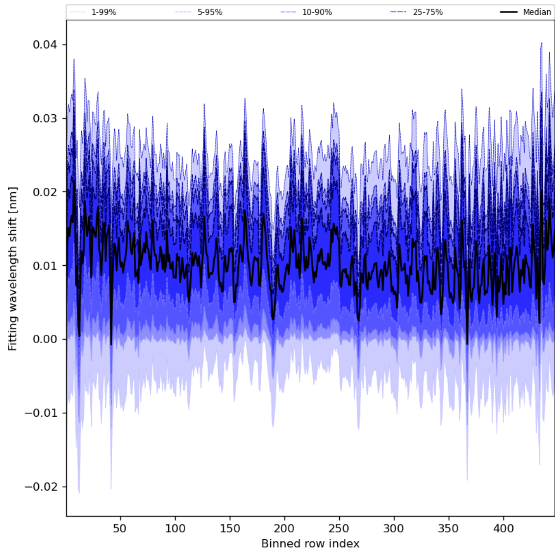
Figure 65: Along track statistics of “Fitting wavelength shift” for 2023-11-08 to 2023-11-10
