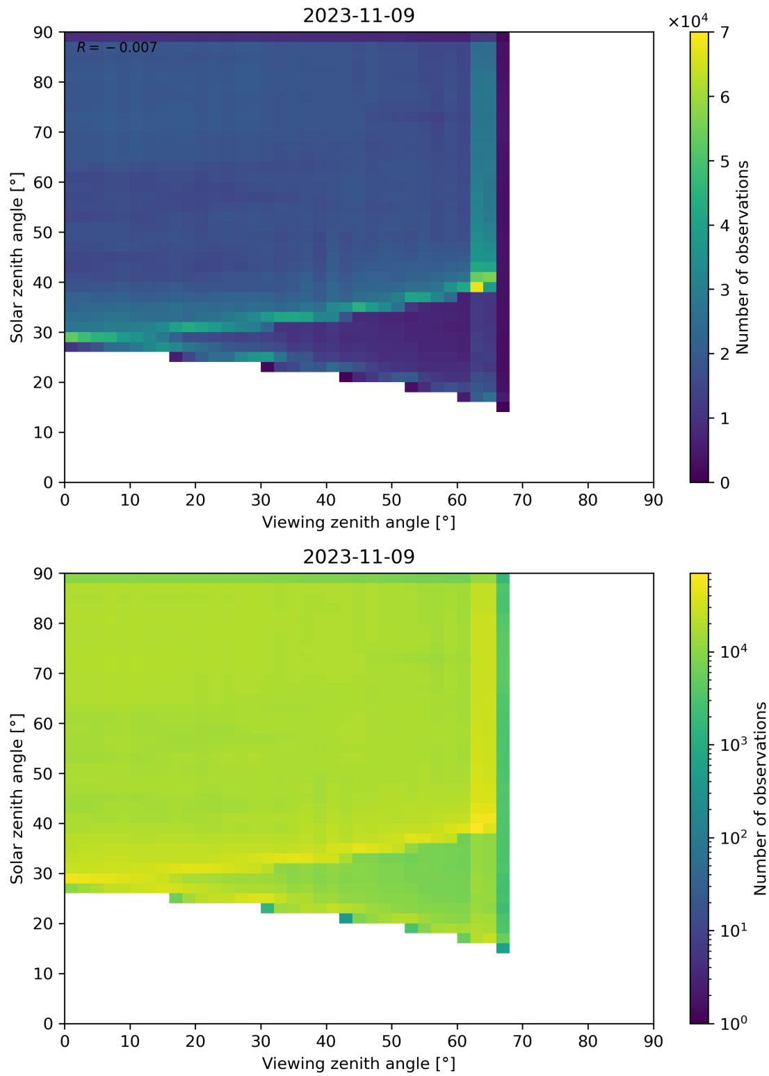
Figure 114: Scatter density plot of “Viewing zenith angle” against “Solar zenith angle” for 2023-11-08 to 2023-11-10.
