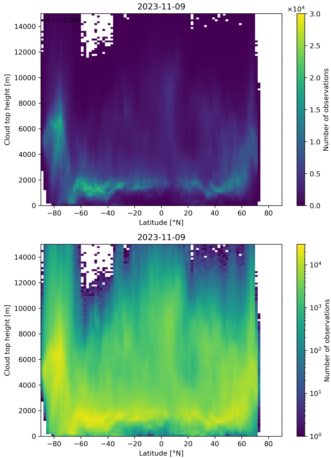
Figure 97: Scatter density plot of “Latitude” against “Cloud top height” for 2023-11-08 to 2023-11-10.
