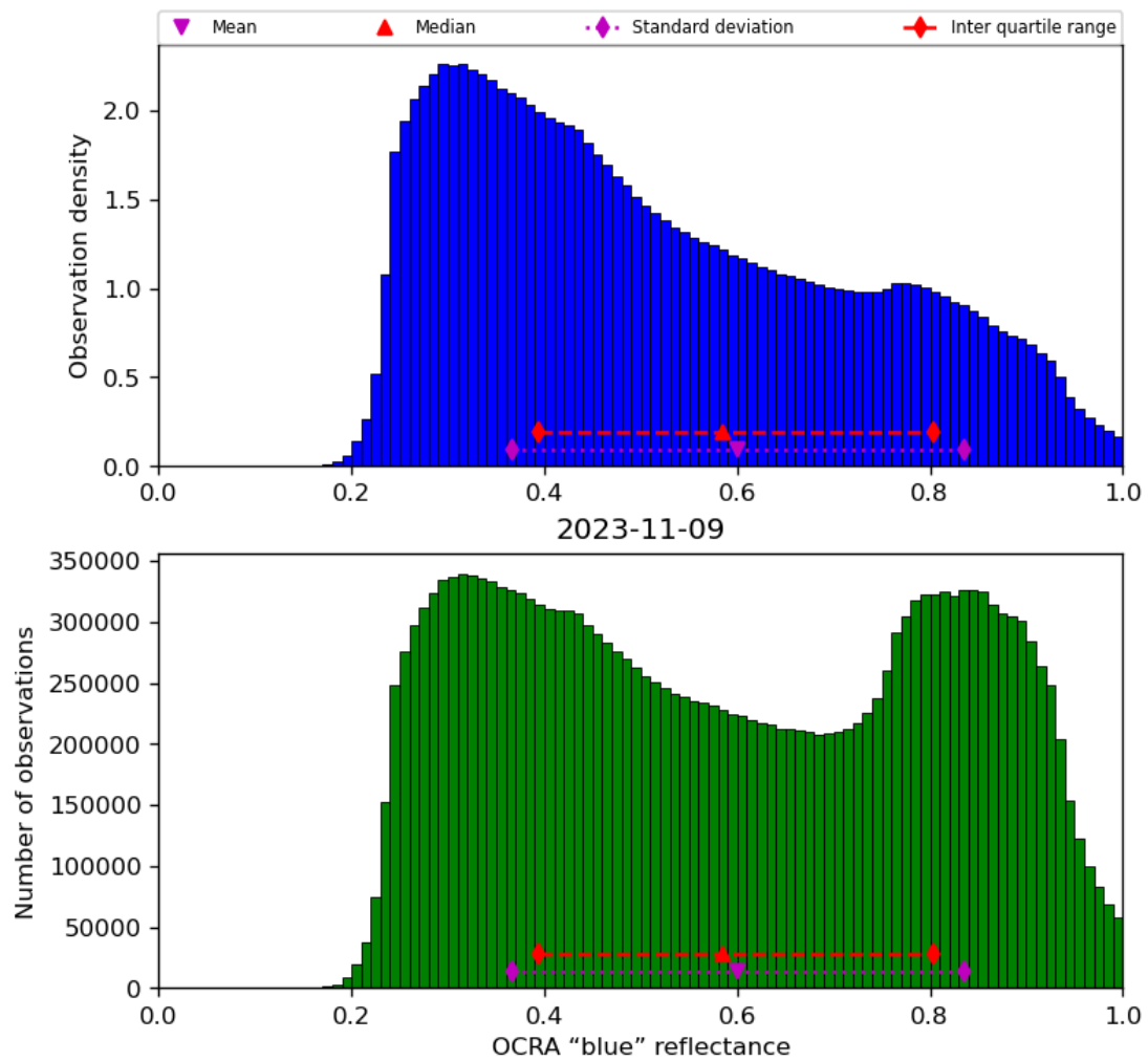
Figure 51: Histogram of “OCRA “blue” reflectance” for 2023-11-08 to 2023-11-10
