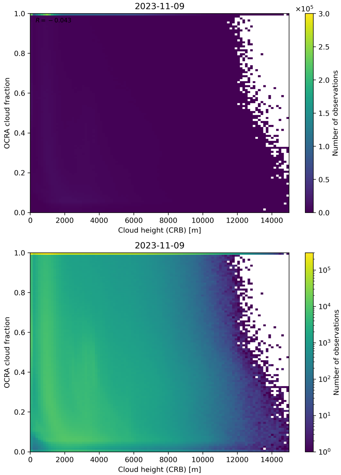
Figure 81: Scatter density plot of “Cloud height (CRB)” against “OCRA cloud fraction” for 2023-11-08 to 2023-11-10.
