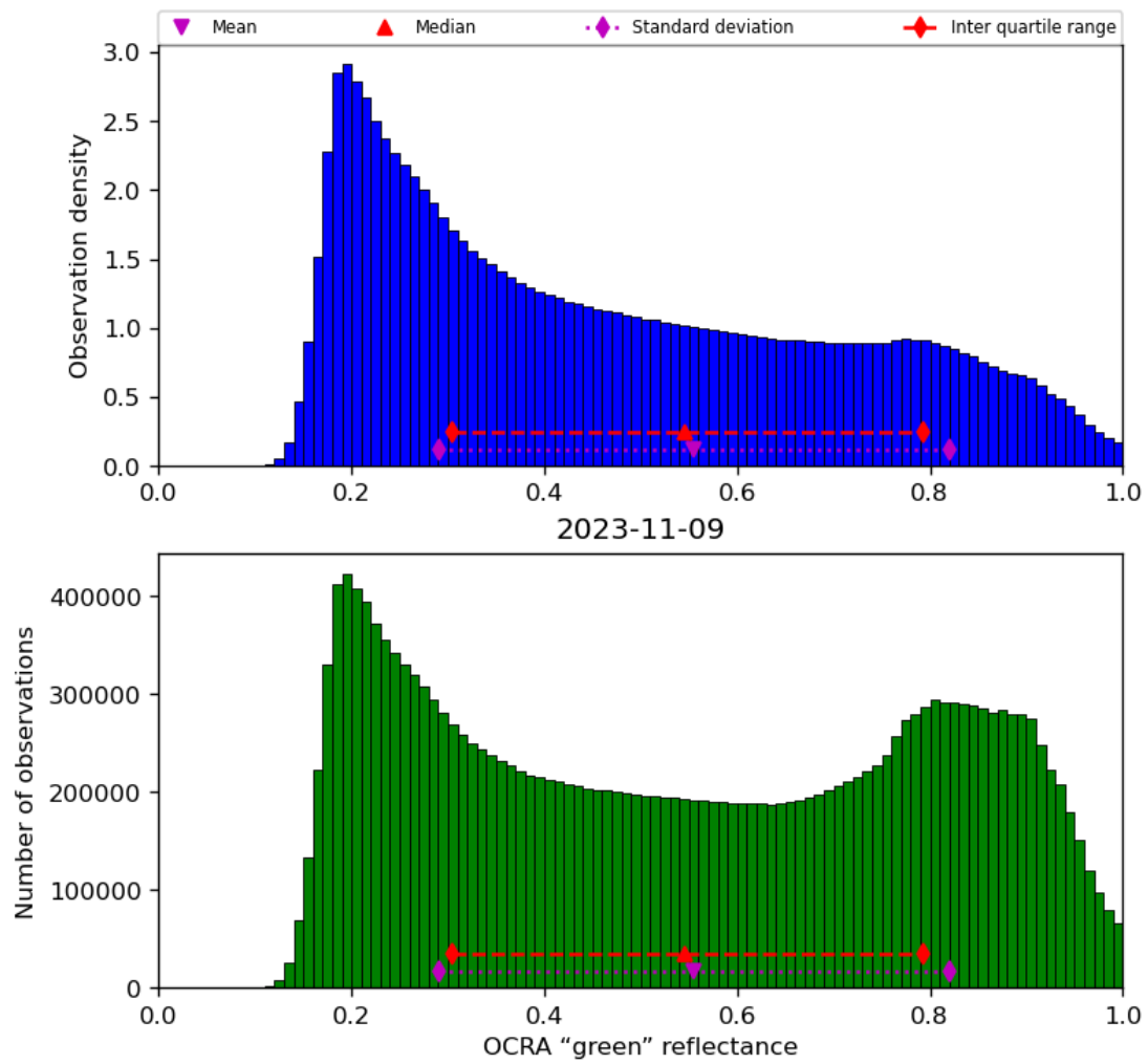
Figure 52: Histogram of “OCRA “green” reflectance” for 2023-11-08 to 2023-11-10
