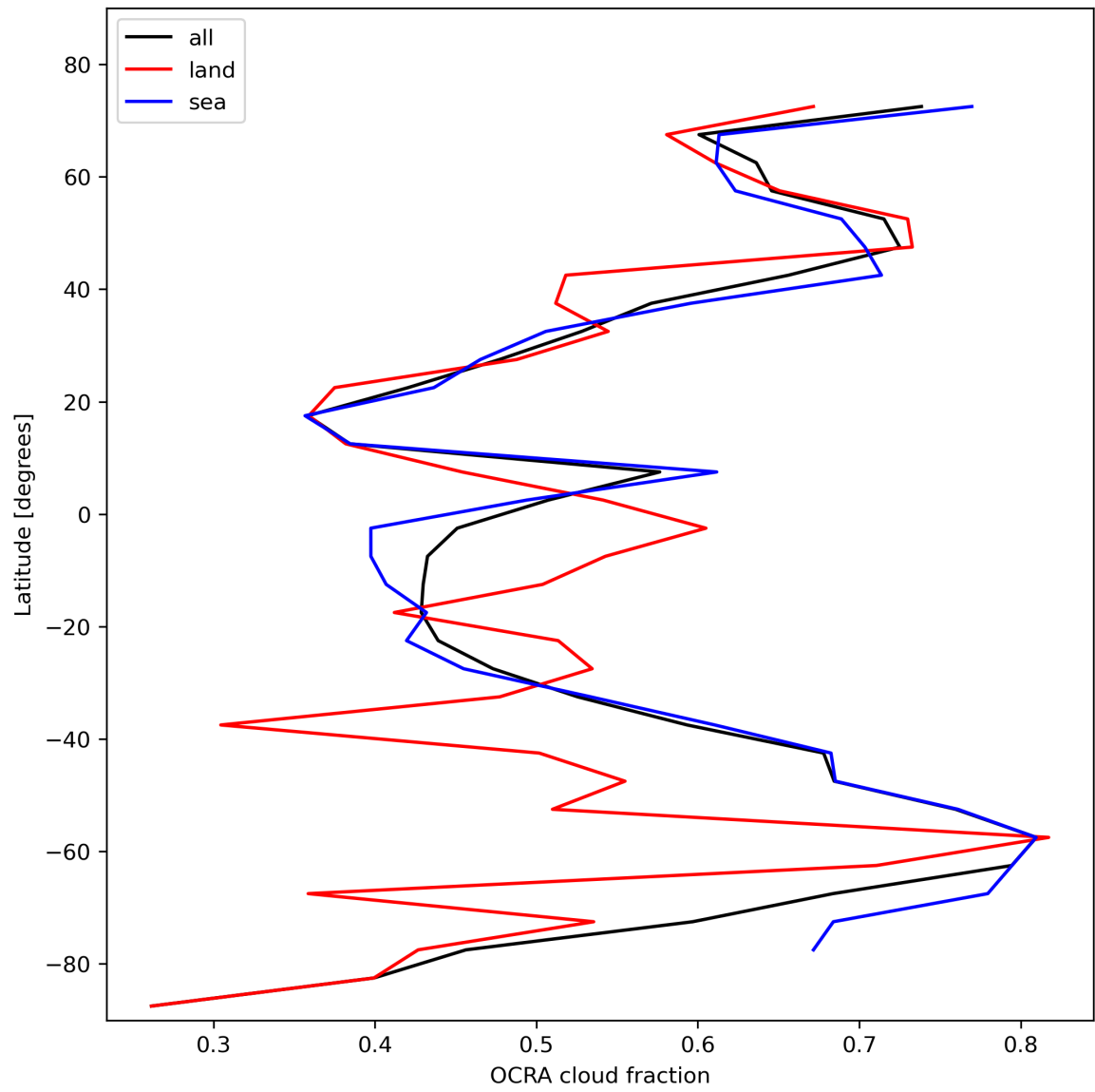
Figure 34: Zonal average of “OCRA cloud fraction” for 2023-11-08 to 2023-11-10.
