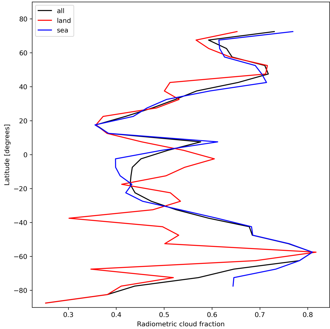
Figure 23: Zonal average of “Radiometric cloud fraction” for 2023-11-08 to 2023-11-10.
