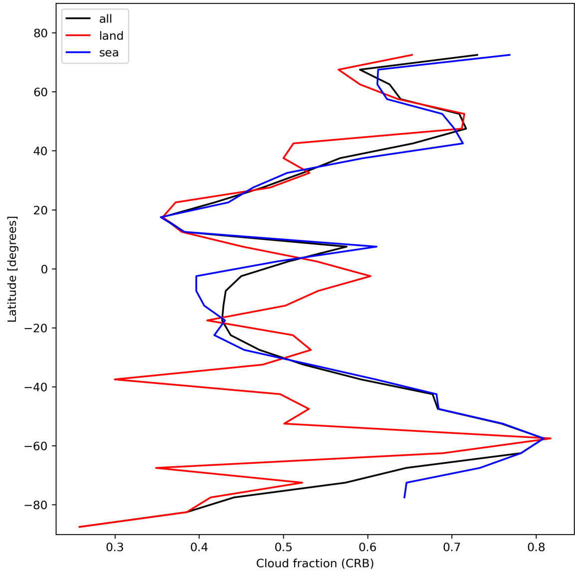
Figure 26: Zonal average of “Cloud fraction (CRB)” for 2023-11-08 to 2023-11-10.
