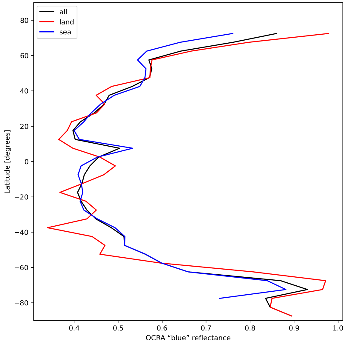
Figure 35: Zonal average of “OCRA “blue” reflectance” for 2023-11-08 to 2023-11-10.
