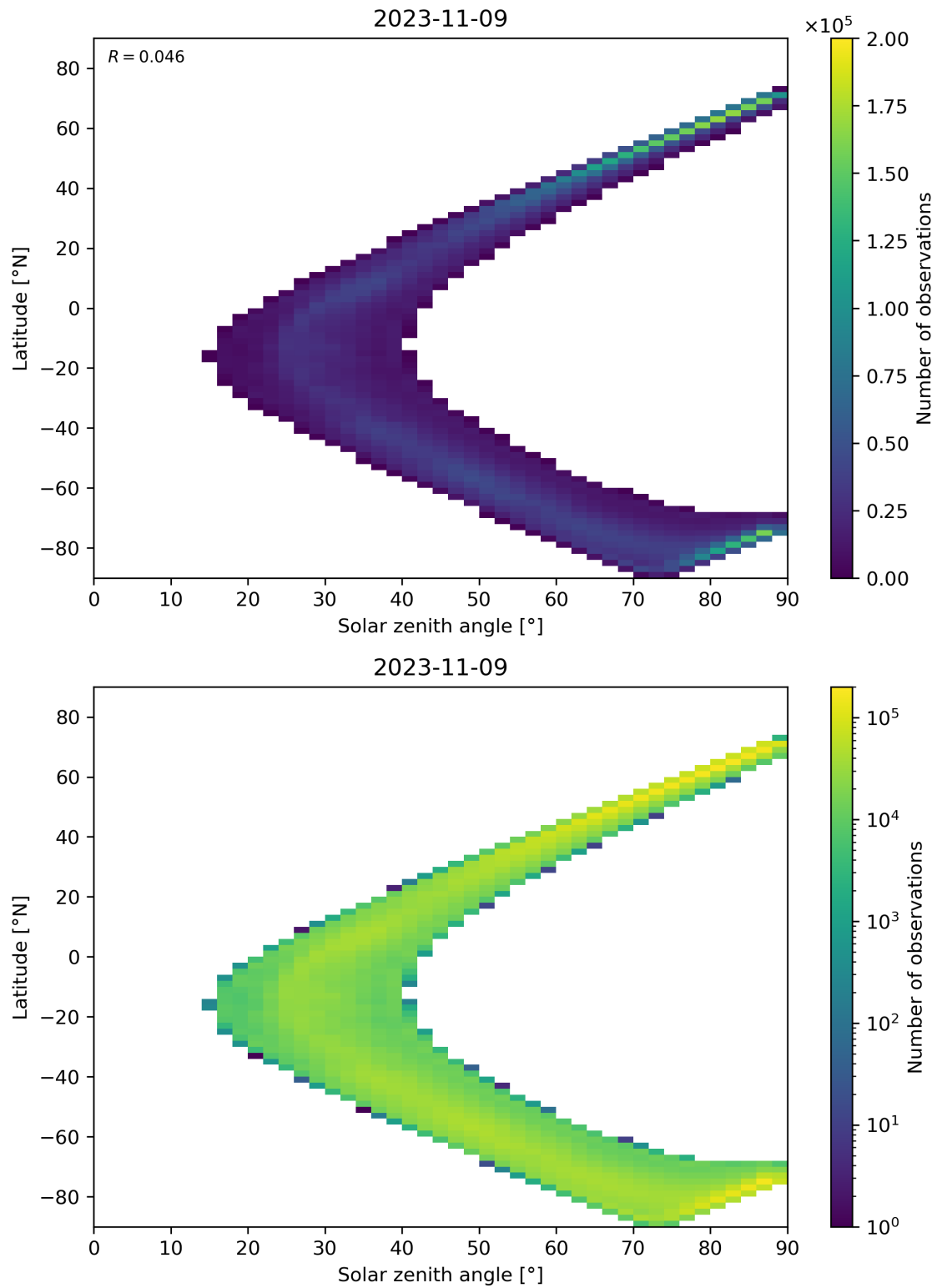
Figure 105: Scatter density plot of “Solar zenith angle” against “Latitude” for 2023-11-08 to 2023-11-10.
