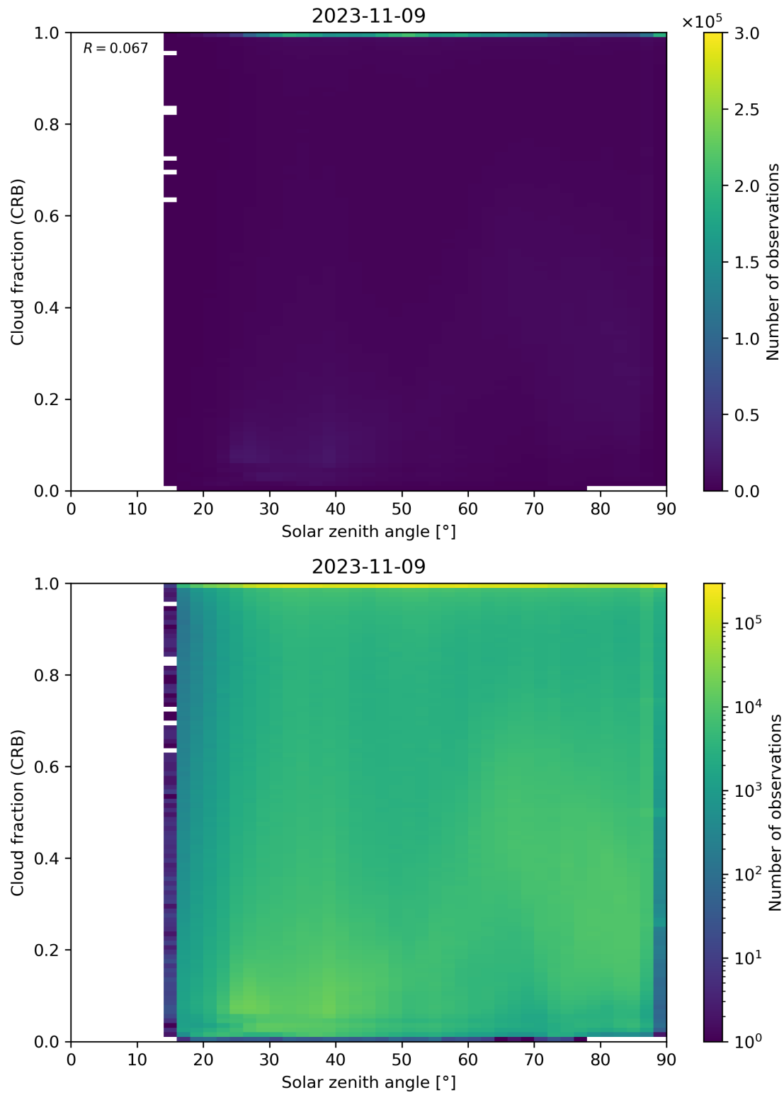
Figure 101: Scatter density plot of “Solar zenith angle” against “Cloud fraction (CRB)” for 2023-11-08 to 2023-11-10.
