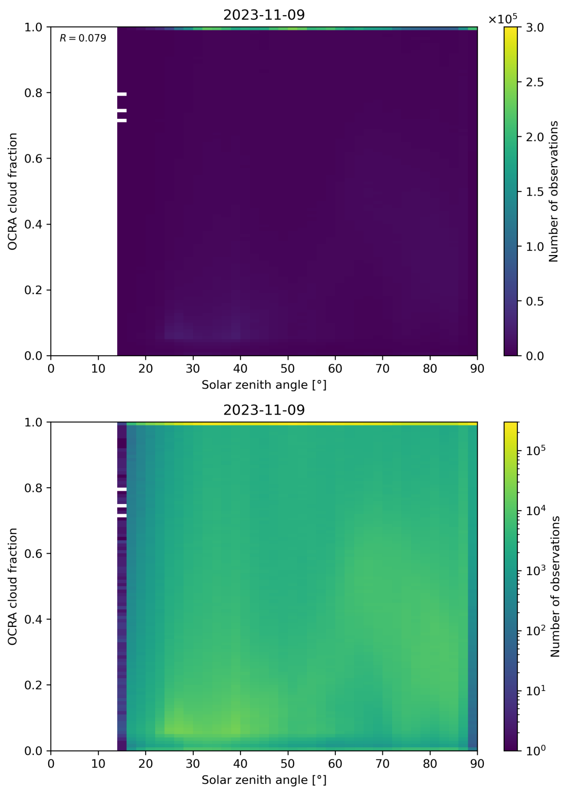
Figure 100: Scatter density plot of “Solar zenith angle” against “OCRA cloud fraction” for 2023-11-08 to 2023-11-10.
