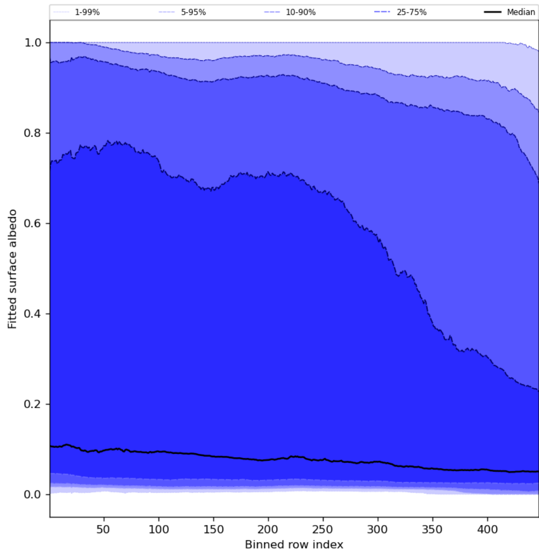
Figure 61: Along track statistics of “Fitted surface albedo” for 2023-11-08 to 2023-11-10
