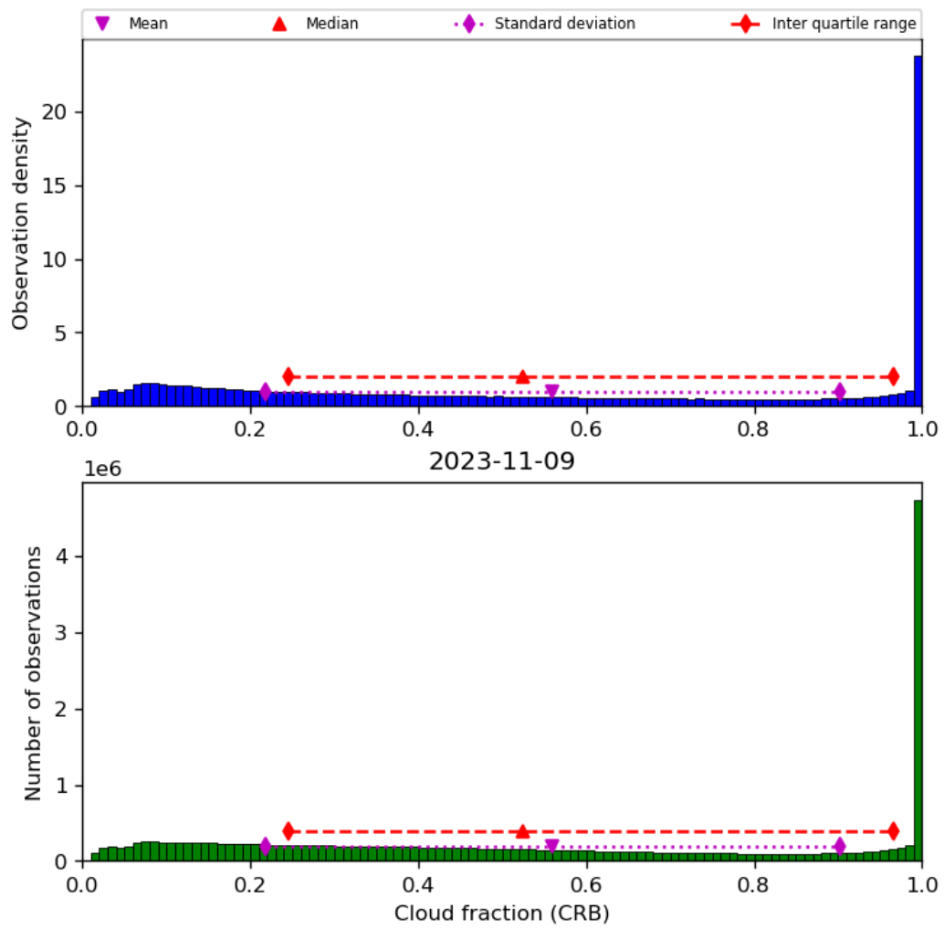
Figure 42: Histogram of “Cloud fraction (CRB)” for 2023-11-08 to 2023-11-10
