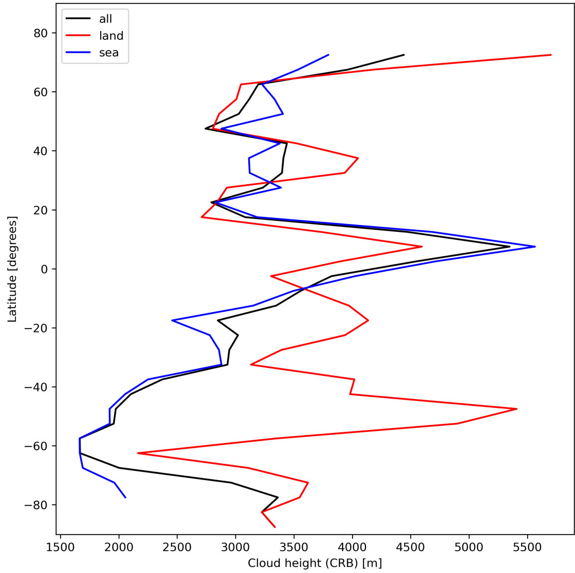
Figure 27: Zonal average of “Cloud height (CRB)” for 2023-11-09 to 2023-11-11.
