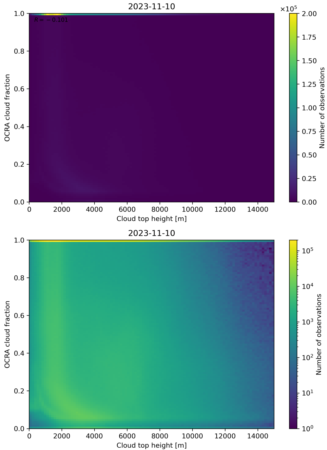
Figure 87: Scatter density plot of “Cloud top height” against “OCRA cloud fraction” for 2023-11-09 to 2023-11-11.
