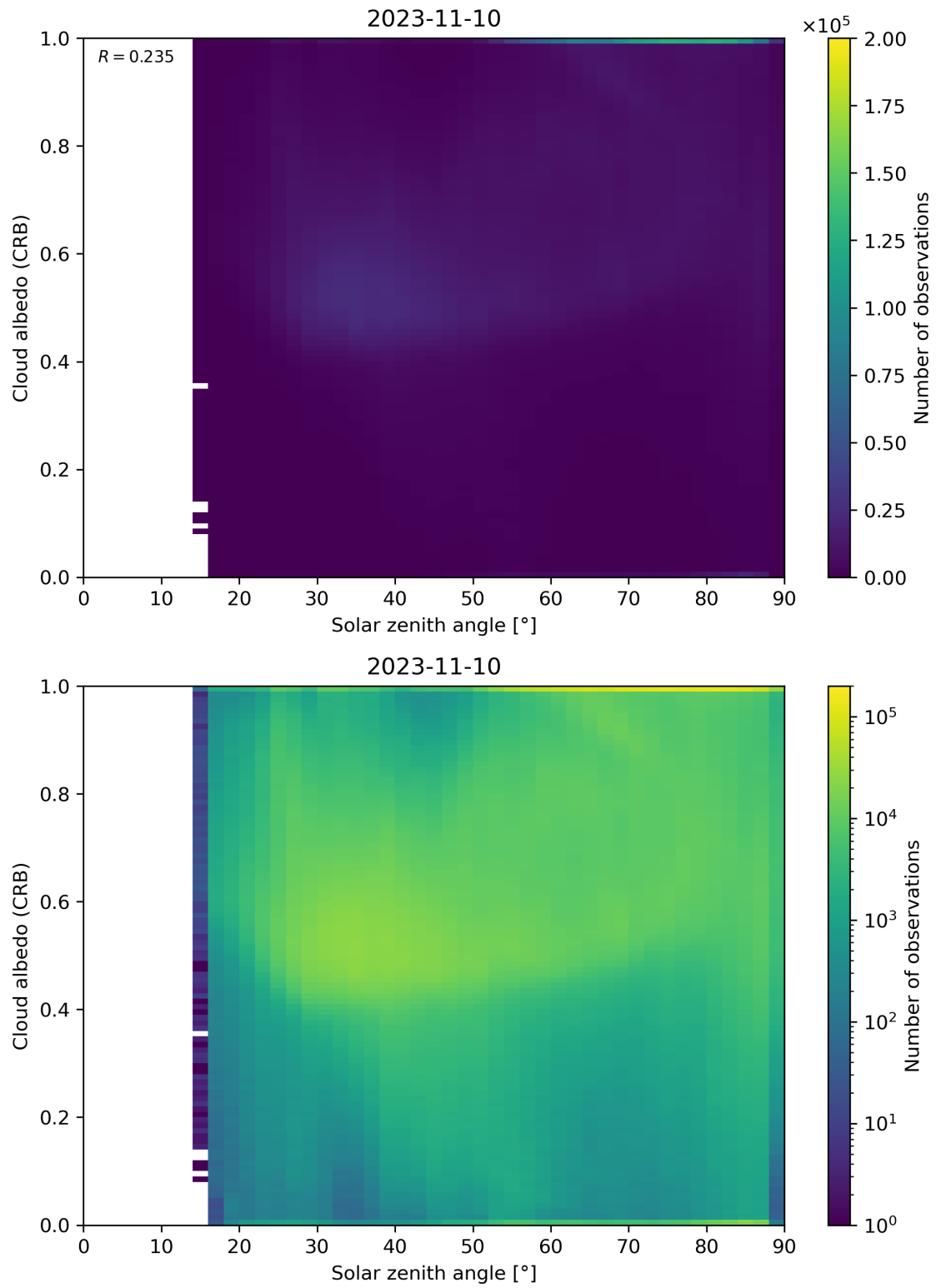
Figure 98: Scatter density plot of “Solar zenith angle” against “Cloud albedo (CRB)” for 2023-11-09 to 2023-11-11.
