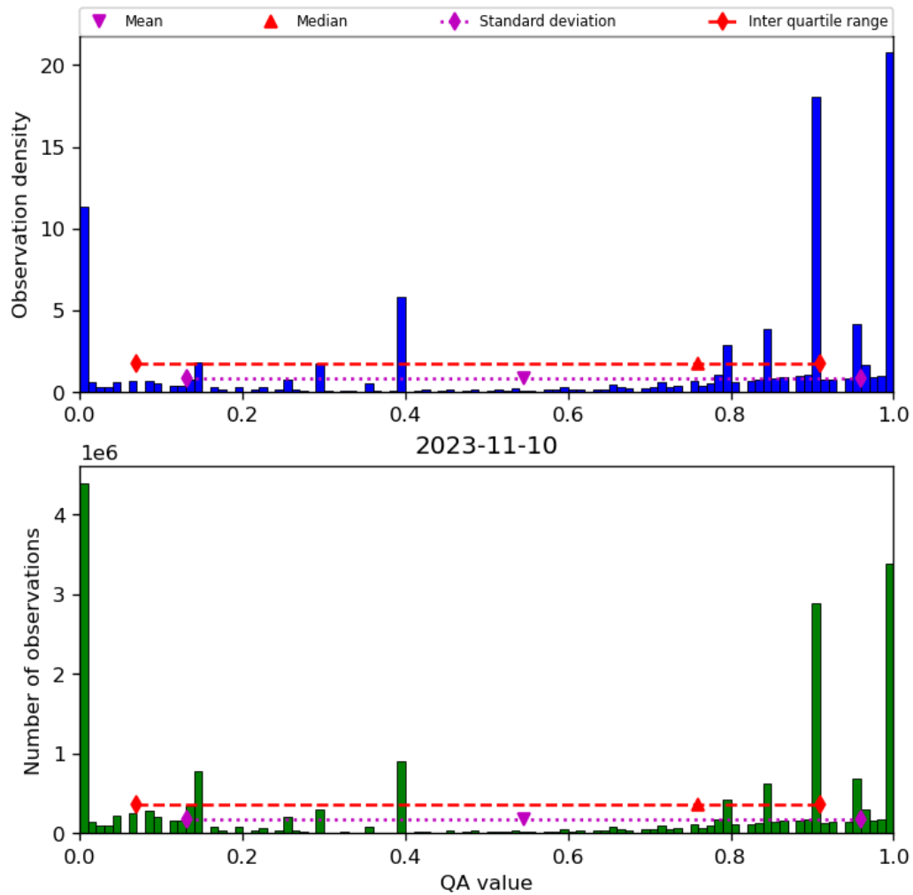
Figure 38: Histogram of “QA value” for 2023-11-09 to 2023-11-11
