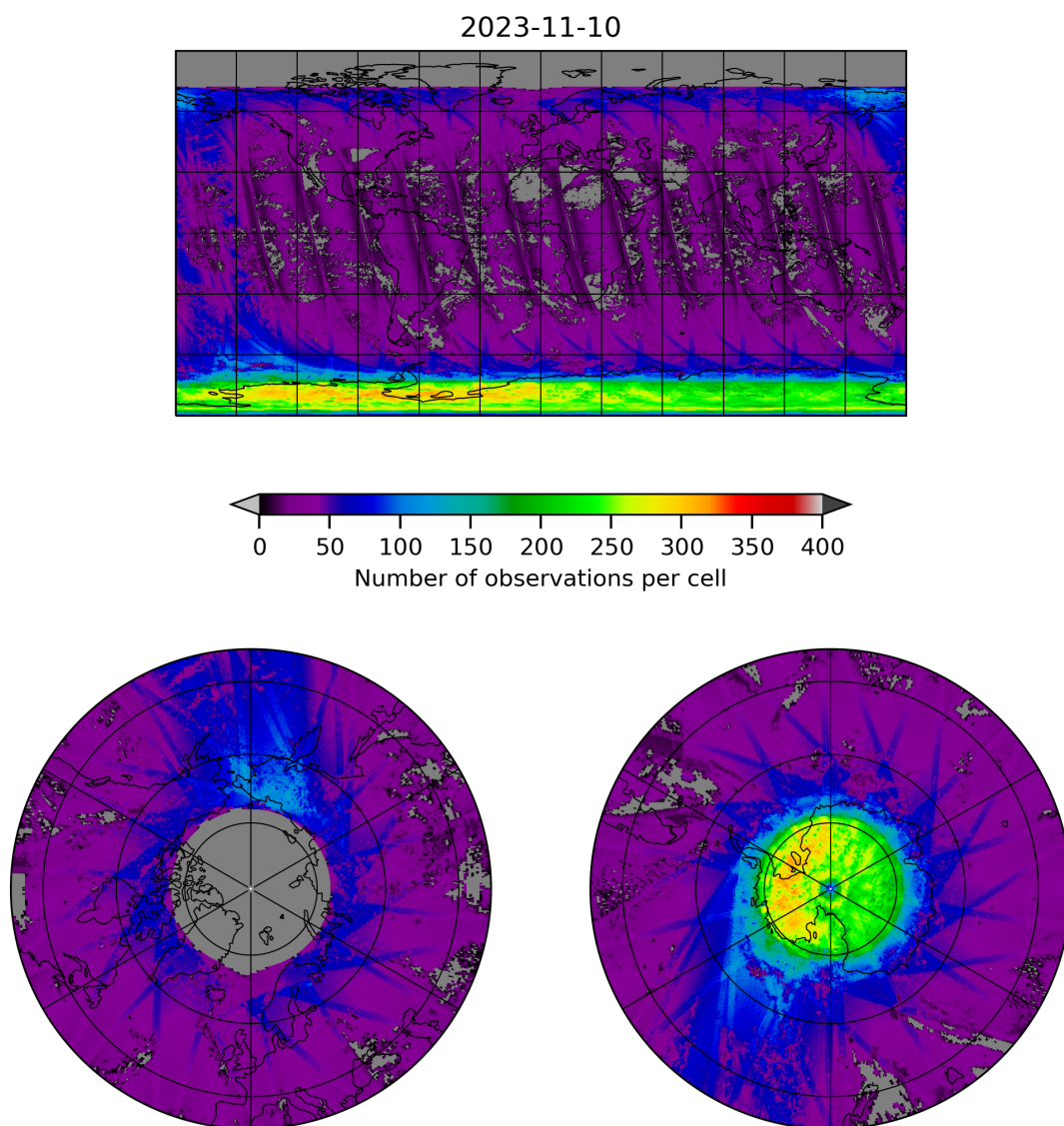
Figure 21: Map of the number of observations for 2023-11-09 to 2023-11-11
