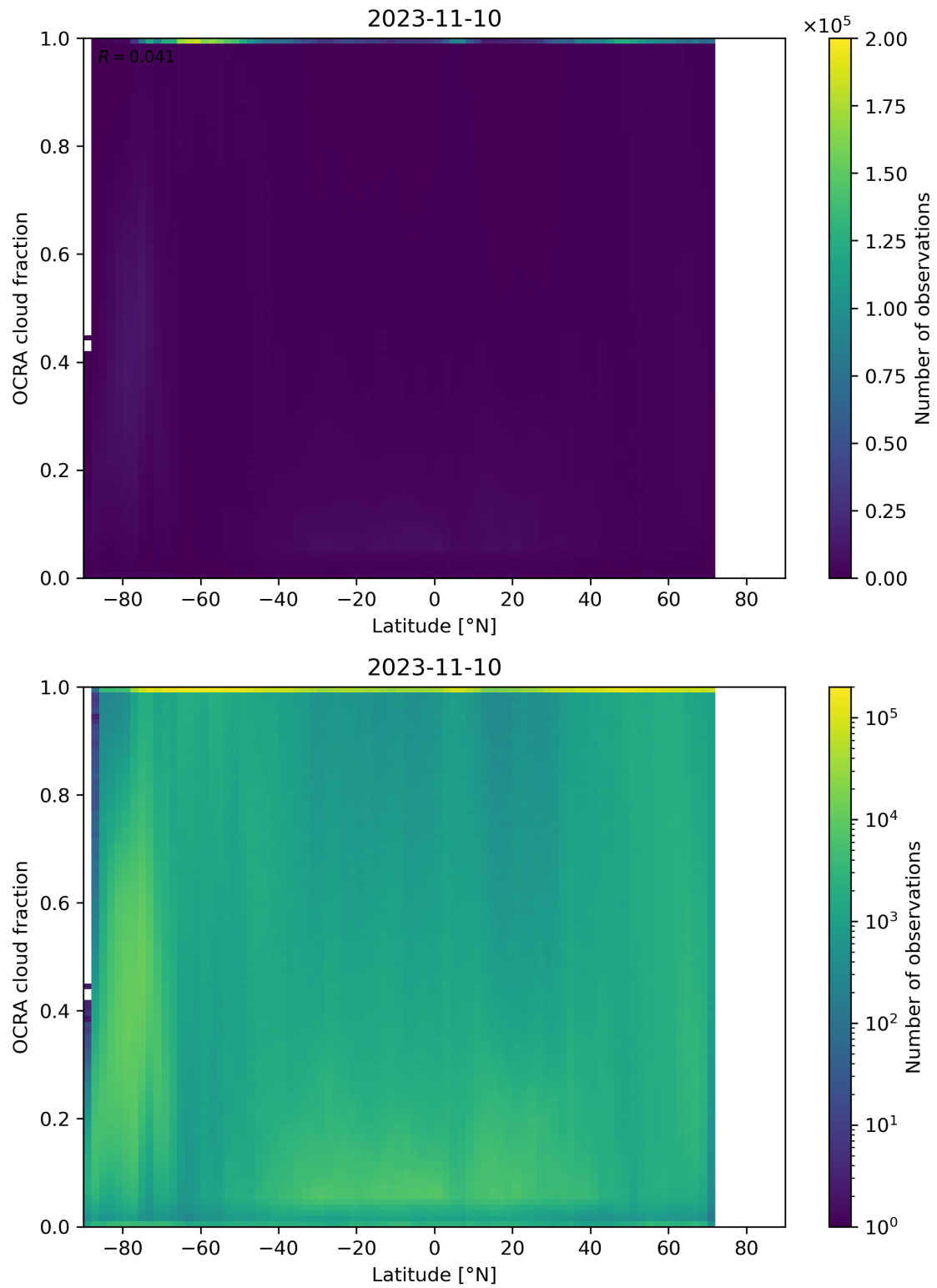
Figure 93: Scatter density plot of “Latitude” against “OCRA cloud fraction” for 2023-11-09 to 2023-11-11.
