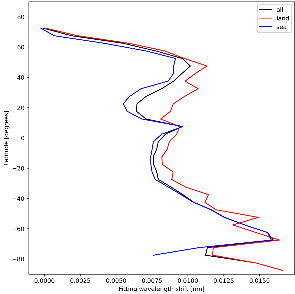
Figure 33: Zonal average of “Fitting wavelength shift” for 2023-11-09 to 2023-11-11.
