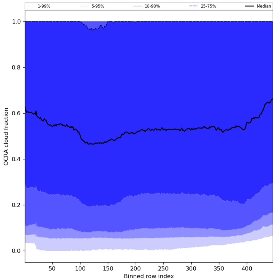
Figure 66: Along track statistics of “OCRA cloud fraction” for 2023-11-09 to 2023-11-11
