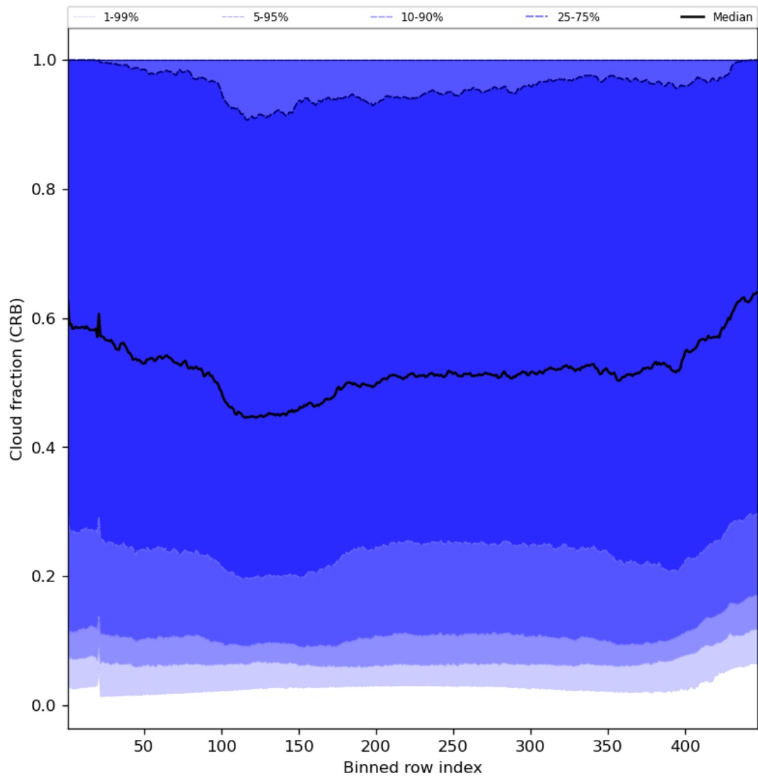
Figure 58: Along track statistics of “Cloud fraction (CRB)” for 2023-11-09 to 2023-11-11
