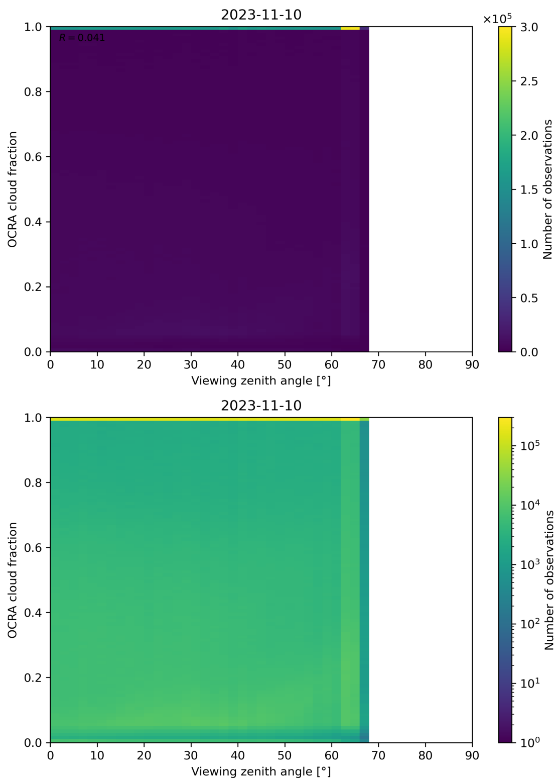
Figure 108: Scatter density plot of “Viewing zenith angle” against “OCRA cloud fraction” for 2023-11-09 to 2023-11-11.
