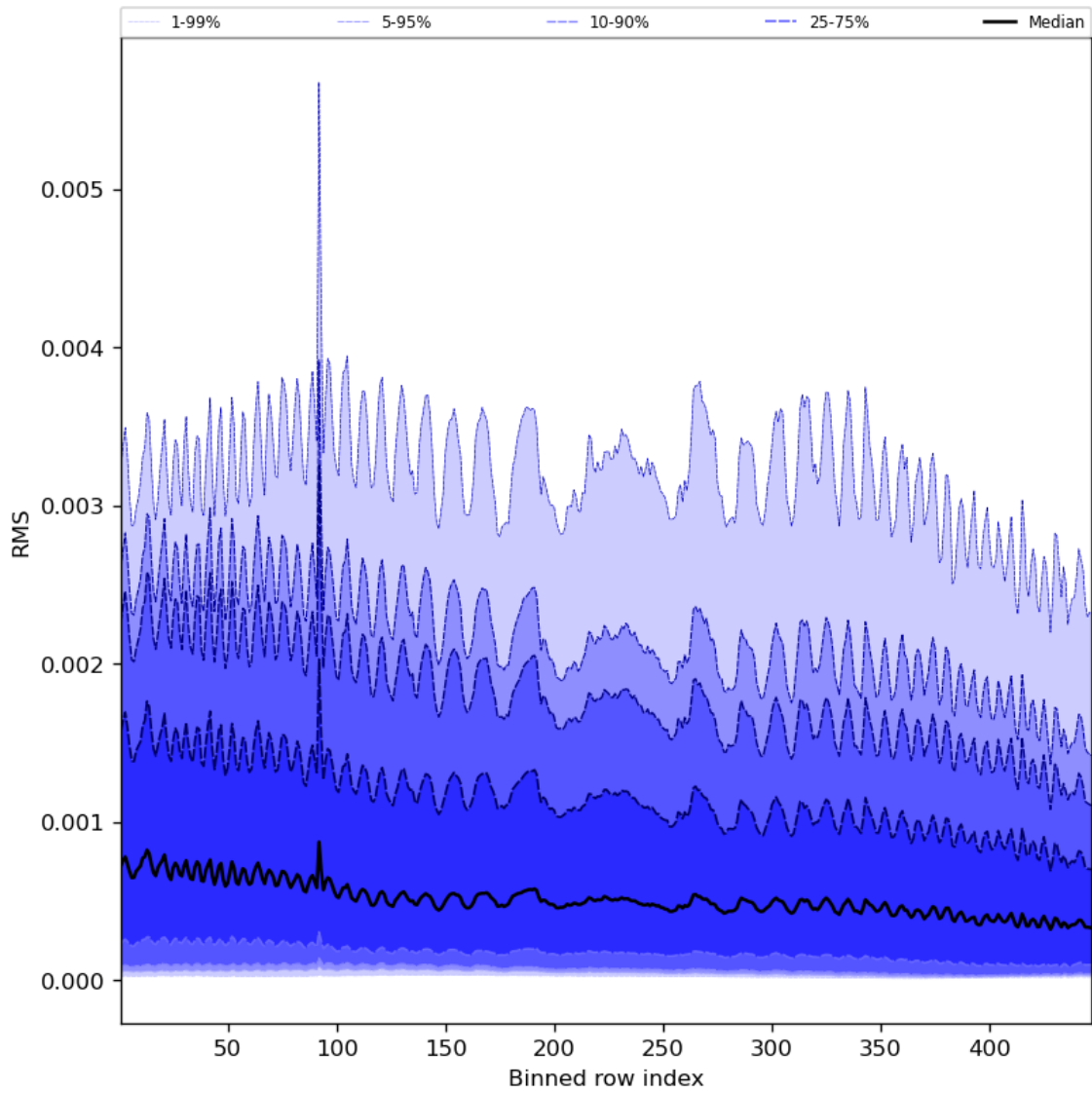
Figure 63: Along track statistics of “RMS” for 2023-11-09 to 2023-11-11
