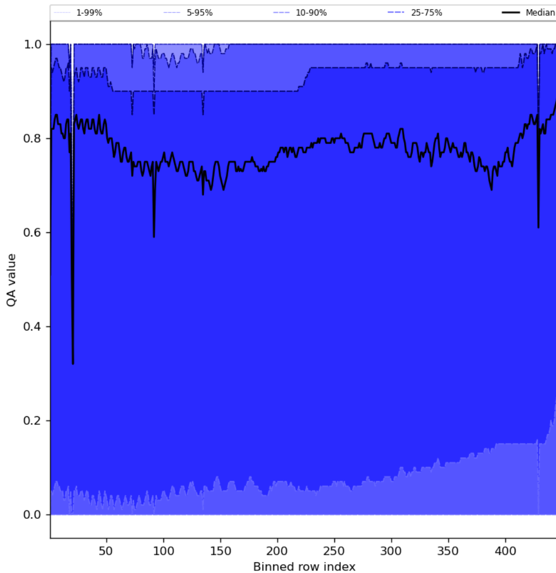
Figure 54: Along track statistics of “QA value” for 2023-11-09 to 2023-11-11
