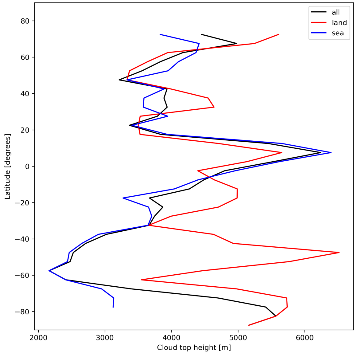
Figure 24: Zonal average of “Cloud top height” for 2023-11-09 to 2023-11-11.
