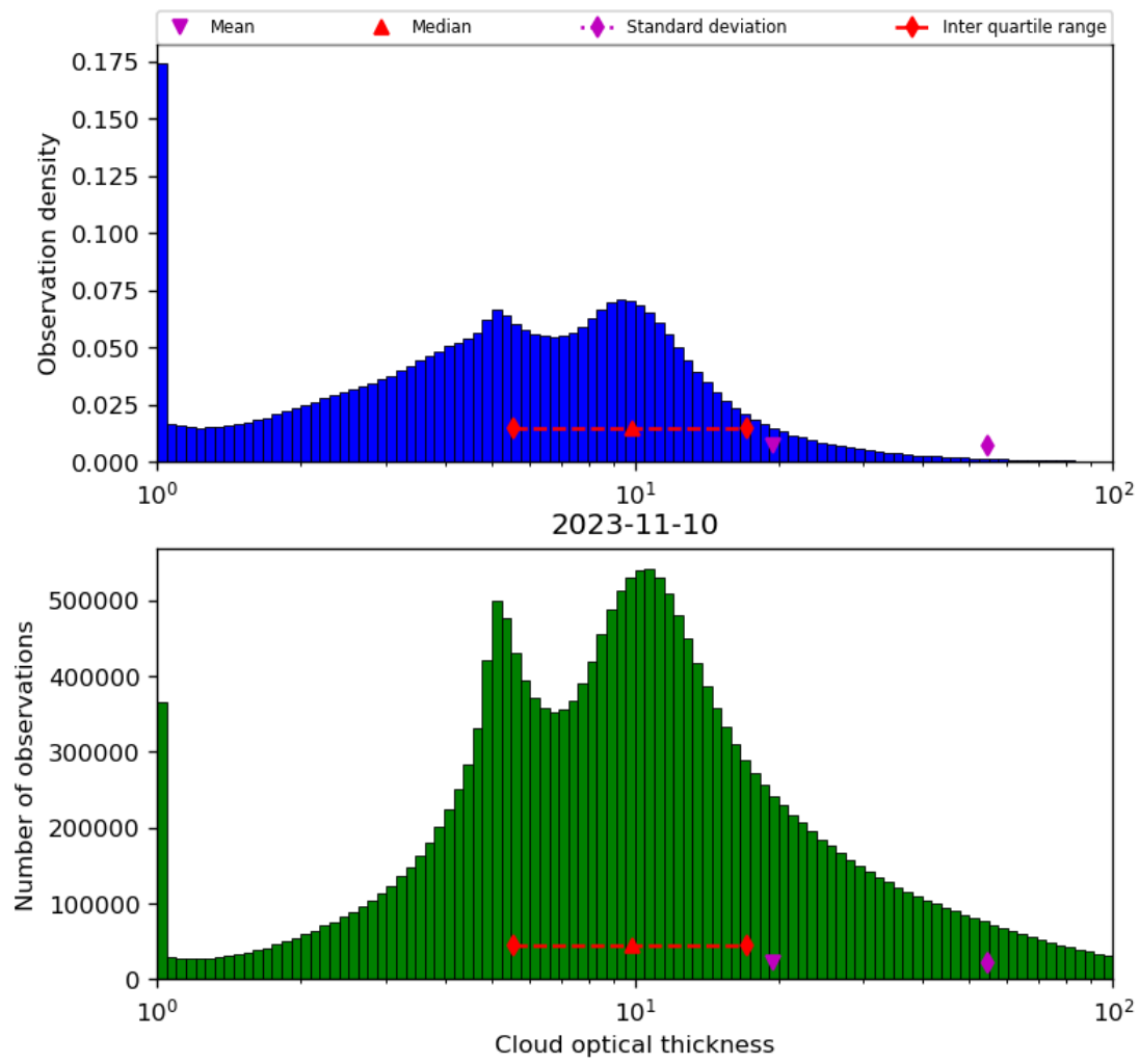
Figure 41: Histogram of “Cloud optical thickness” for 2023-11-09 to 2023-11-11
