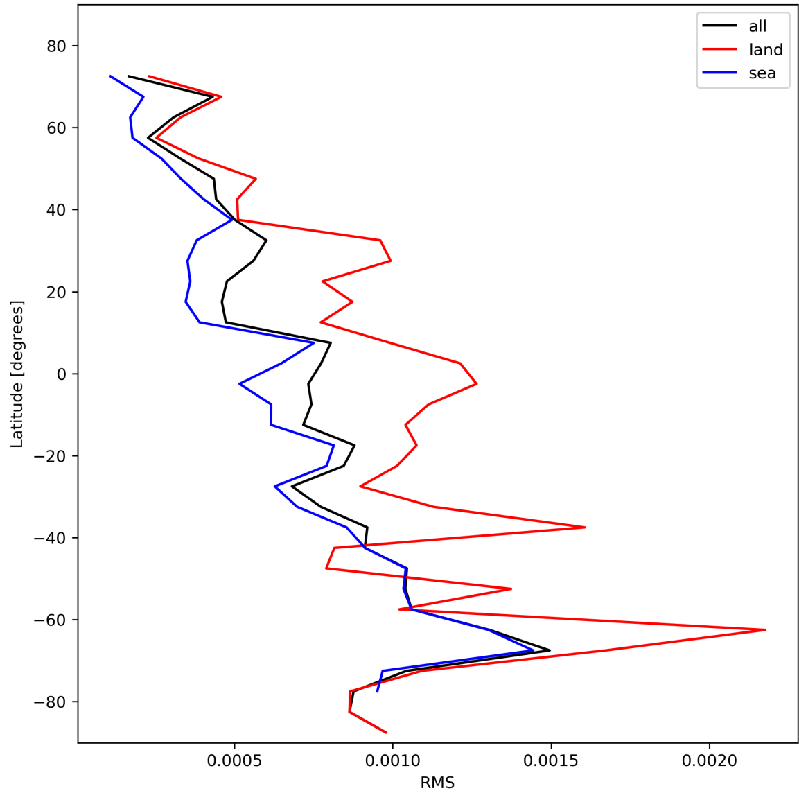
Figure 31: Zonal average of “RMS” for 2023-11-09 to 2023-11-11.
