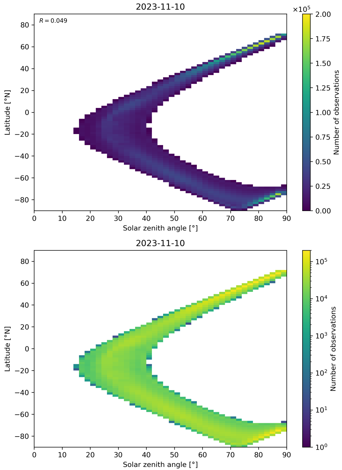
Figure 105: Scatter density plot of “Solar zenith angle” against “Latitude” for 2023-11-09 to 2023-11-11.
