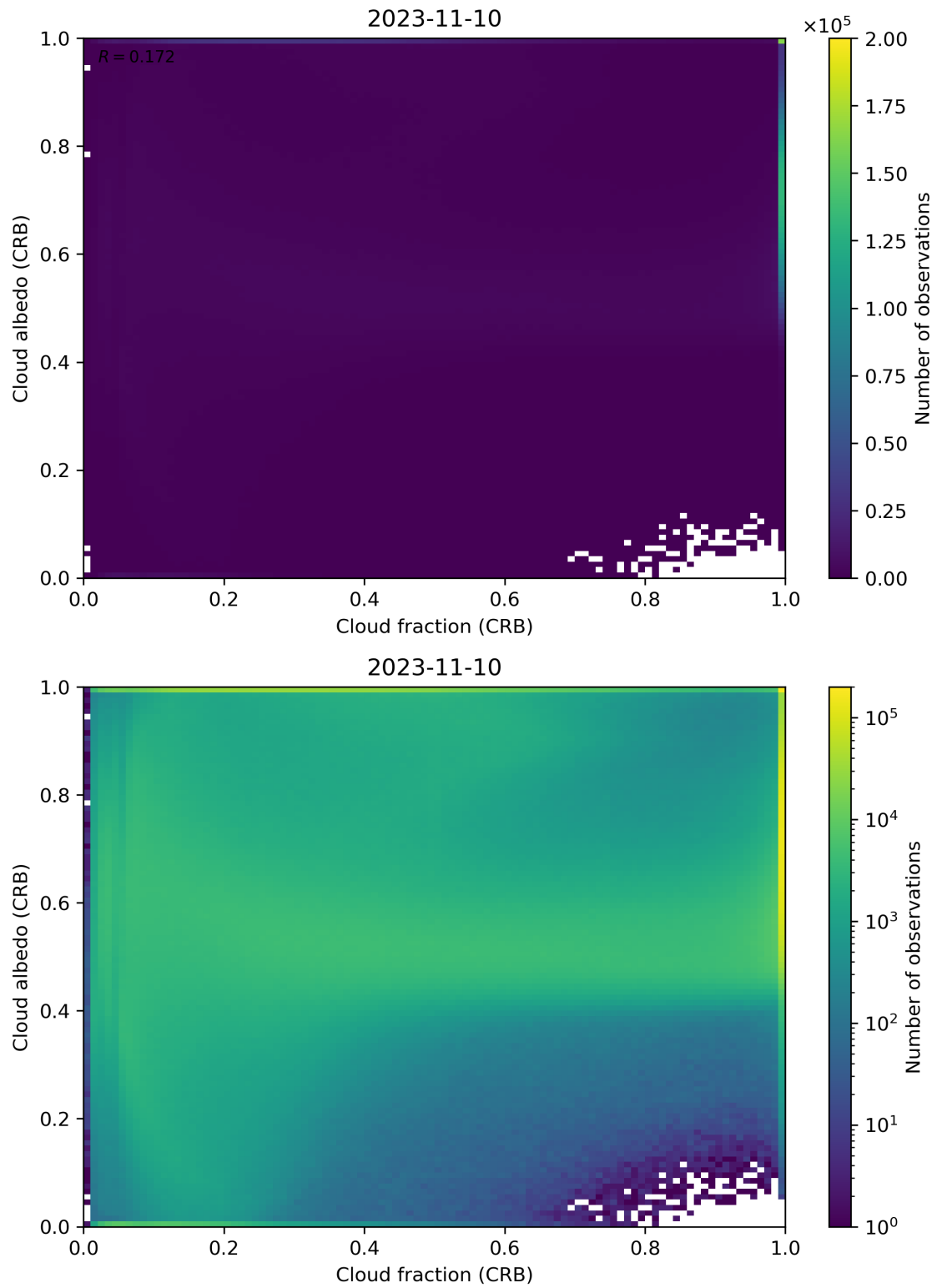
Figure 77: Scatter density plot of “Cloud fraction (CRB)” against “Cloud albedo (CRB)” for 2023-11-09 to 2023-11-11.
