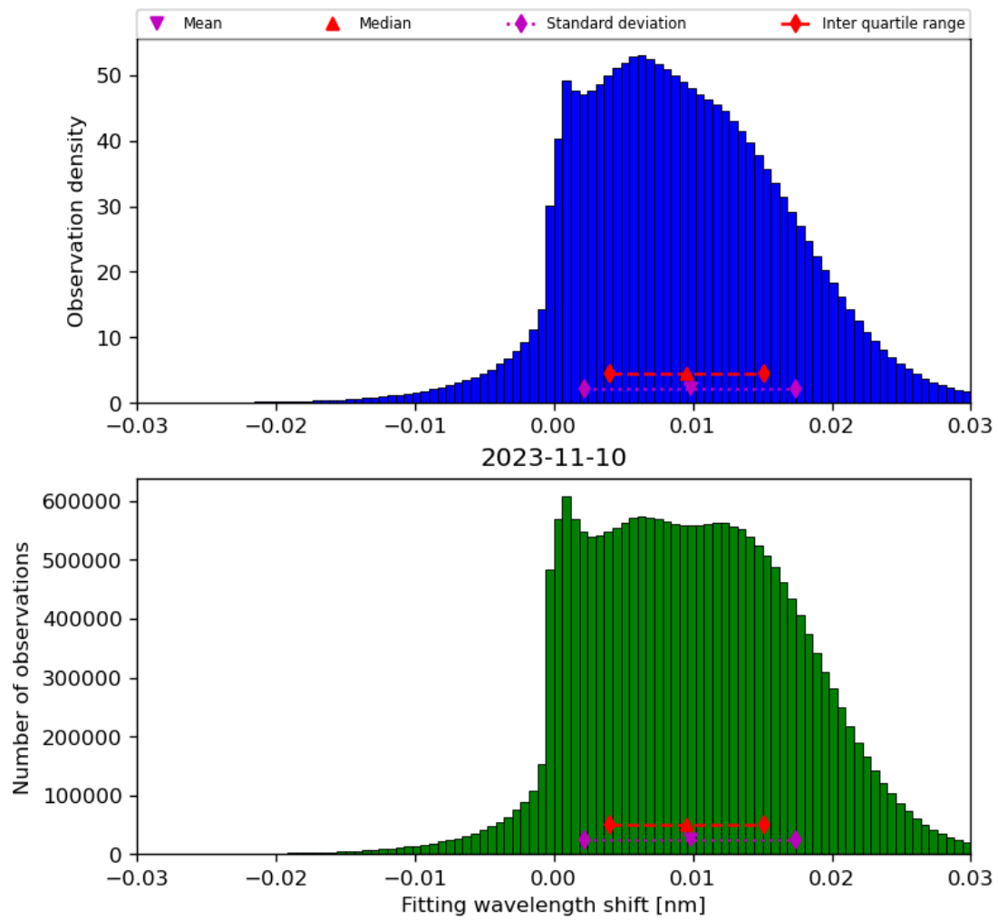
Figure 49: Histogram of “Fitting wavelength shift” for 2023-11-09 to 2023-11-11
