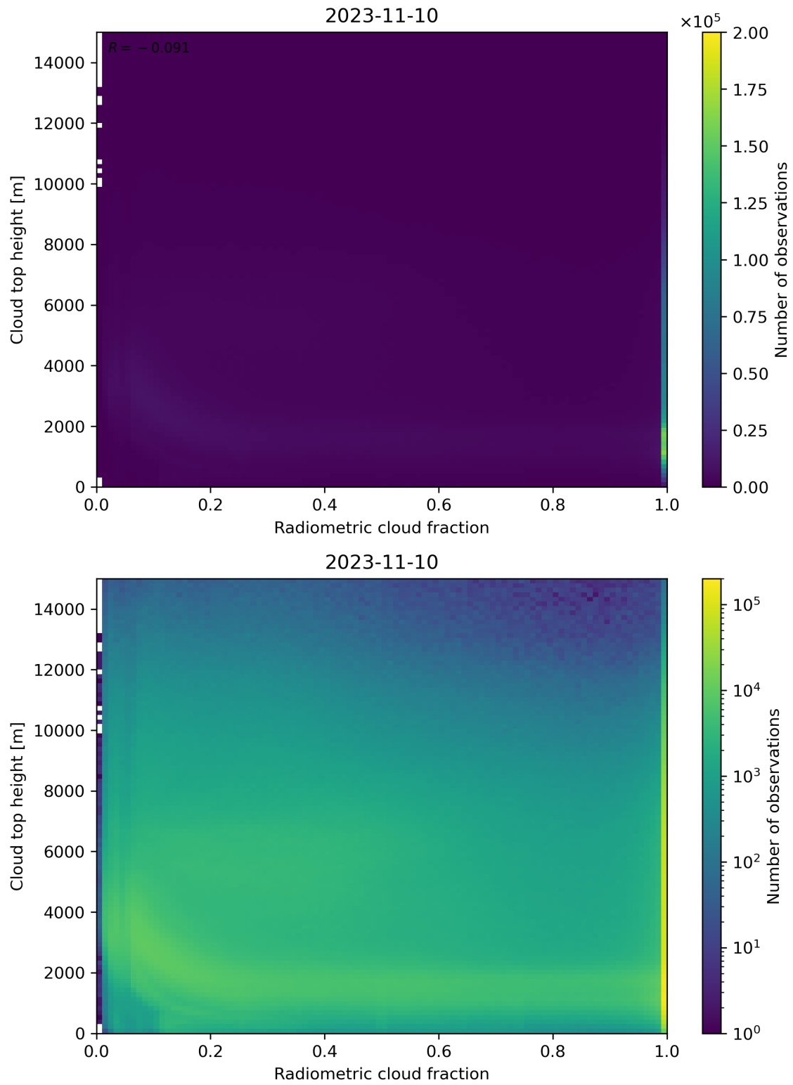
Figure 76: Scatter density plot of “Radiometric cloud fraction” against “Cloud top height” for 2023-11-09 to 2023-11-11.
