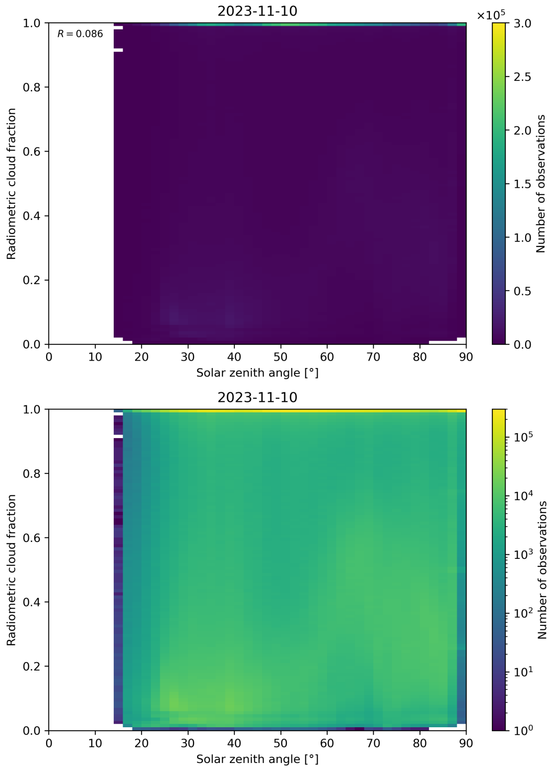
Figure 99: Scatter density plot of “Solar zenith angle” against “Radiometric cloud fraction” for 2023-11-09 to 2023-11-11.
