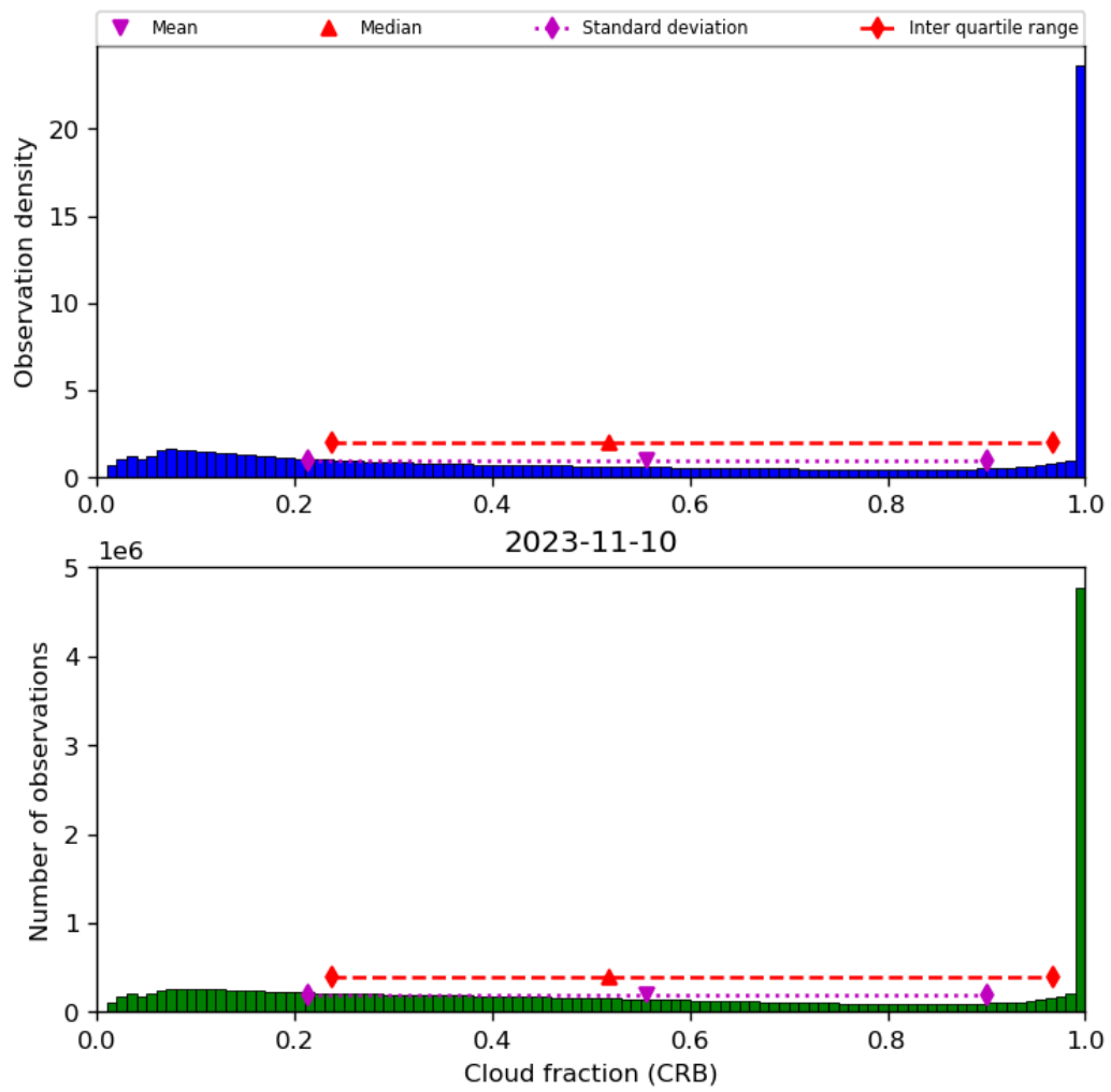
Figure 42: Histogram of “Cloud fraction (CRB)” for 2023-11-09 to 2023-11-11
