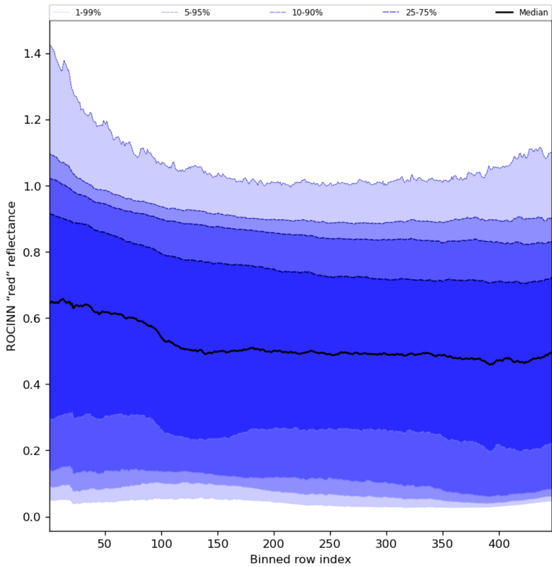
Figure 69: Along track statistics of “ROCINN “red” reflectance” for 2023-11-09 to 2023-11-11
