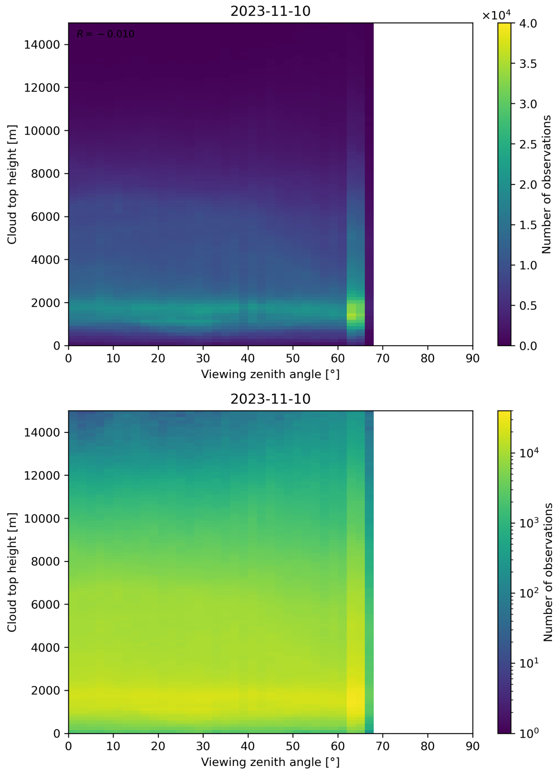
Figure 112: Scatter density plot of “Viewing zenith angle” against “Cloud top height” for 2023-11-09 to 2023-11-11.
