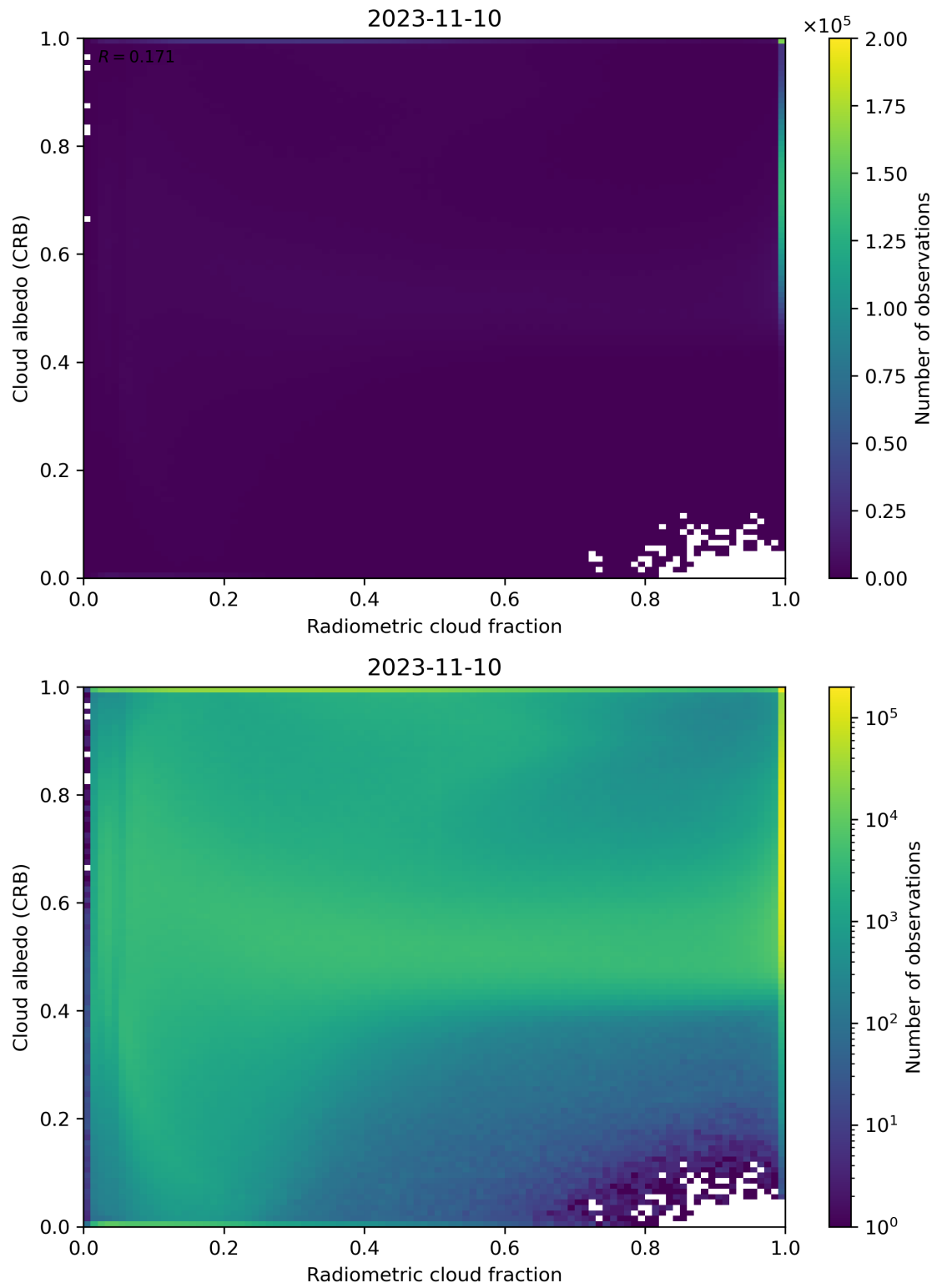
Figure 71: Scatter density plot of “Radiometric cloud fraction” against “Cloud albedo (CRB)” for 2023-11-09 to 2023-11-11.
