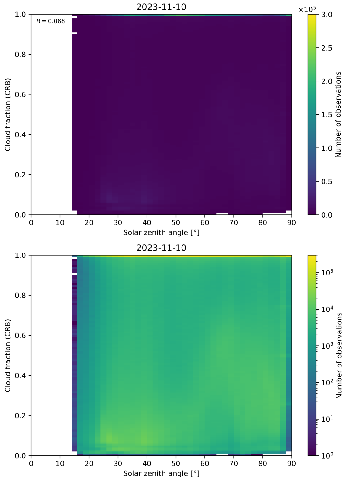
Figure 101: Scatter density plot of “Solar zenith angle” against “Cloud fraction (CRB)” for 2023-11-09 to 2023-11-11.
