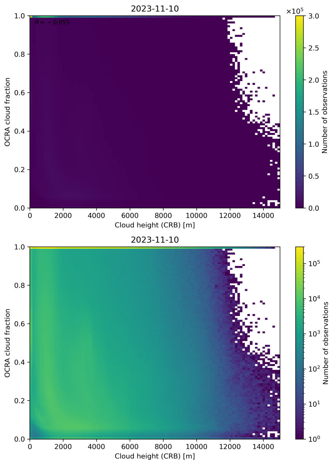
Figure 81: Scatter density plot of “Cloud height (CRB)” against “OCRA cloud fraction” for 2023-11-09 to 2023-11-11.
