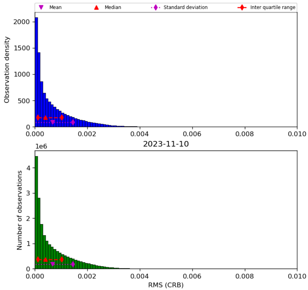
Figure 48: Histogram of “RMS (CRB)” for 2023-11-09 to 2023-11-11
