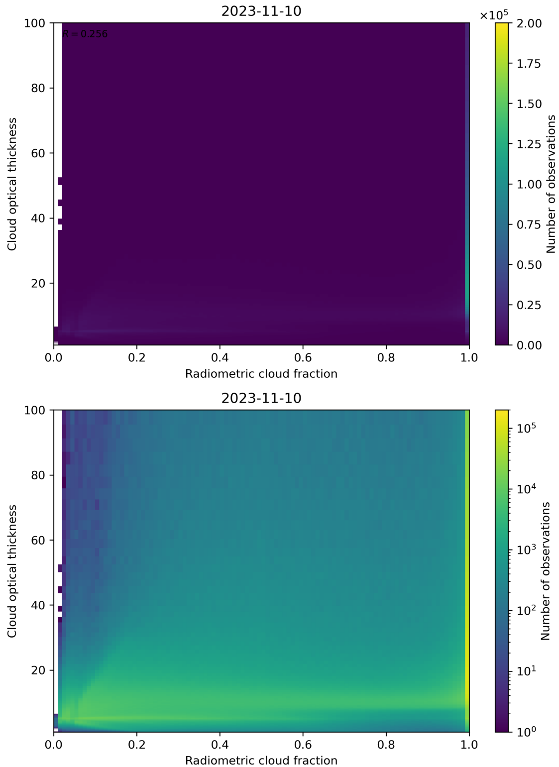
Figure 75: Scatter density plot of “Radiometric cloud fraction” against “Cloud optical thickness” for 2023-11-09 to 2023-11-11.
