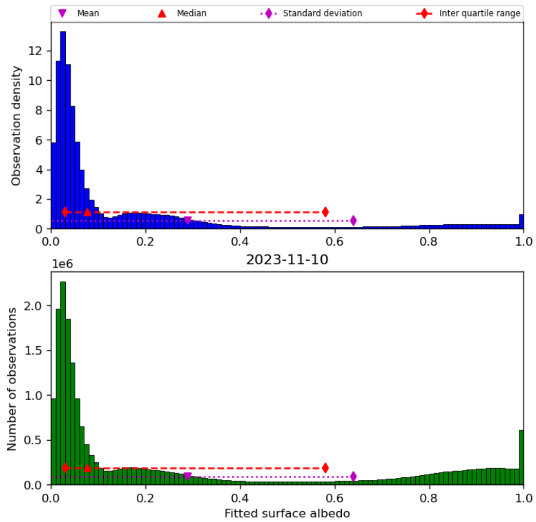
Figure 45: Histogram of “Fitted surface albedo” for 2023-11-09 to 2023-11-11
