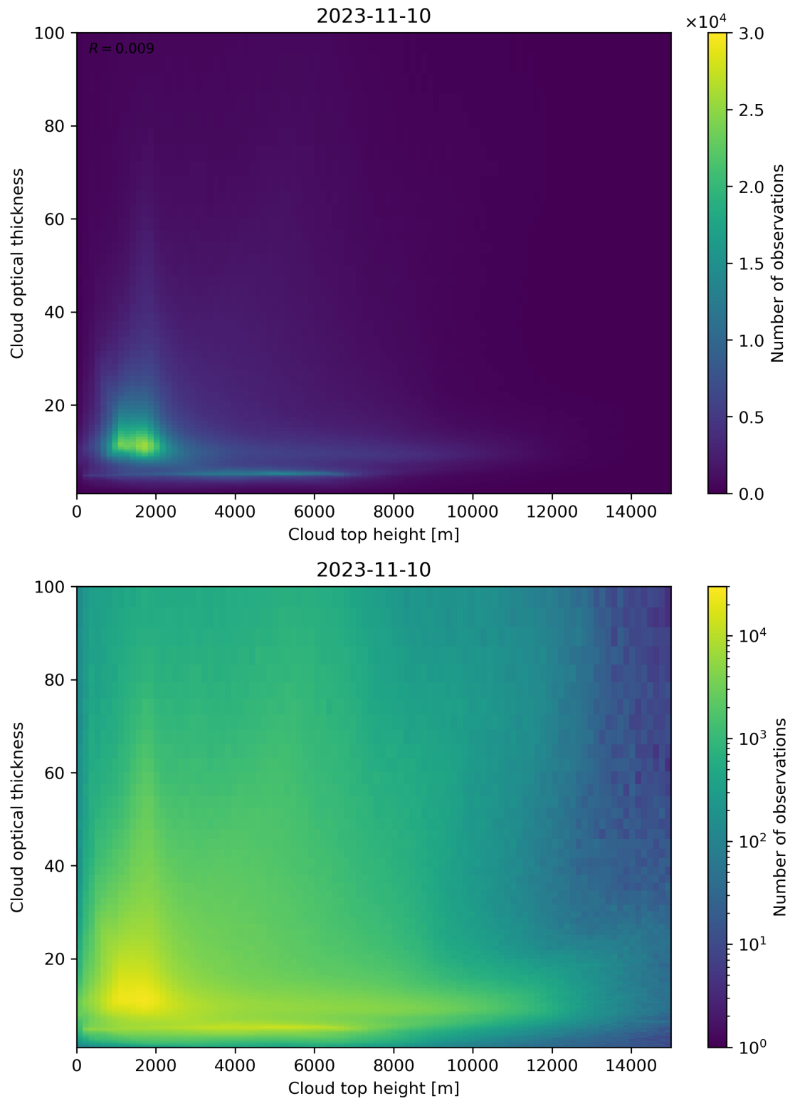
Figure 90: Scatter density plot of “Cloud top height” against “Cloud optical thickness” for 2023-11-09 to 2023-11-11.
