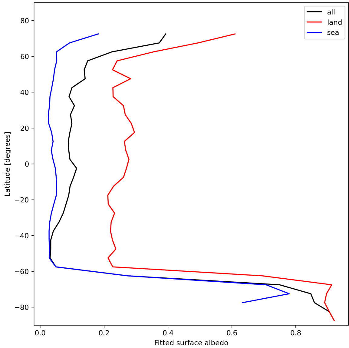
Figure 29: Zonal average of “Fitted surface albedo” for 2023-11-09 to 2023-11-11.
