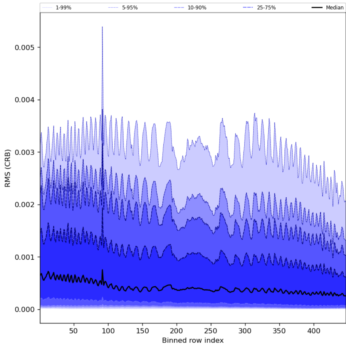
Figure 64: Along track statistics of “RMS (CRB)” for 2023-11-09 to 2023-11-11
