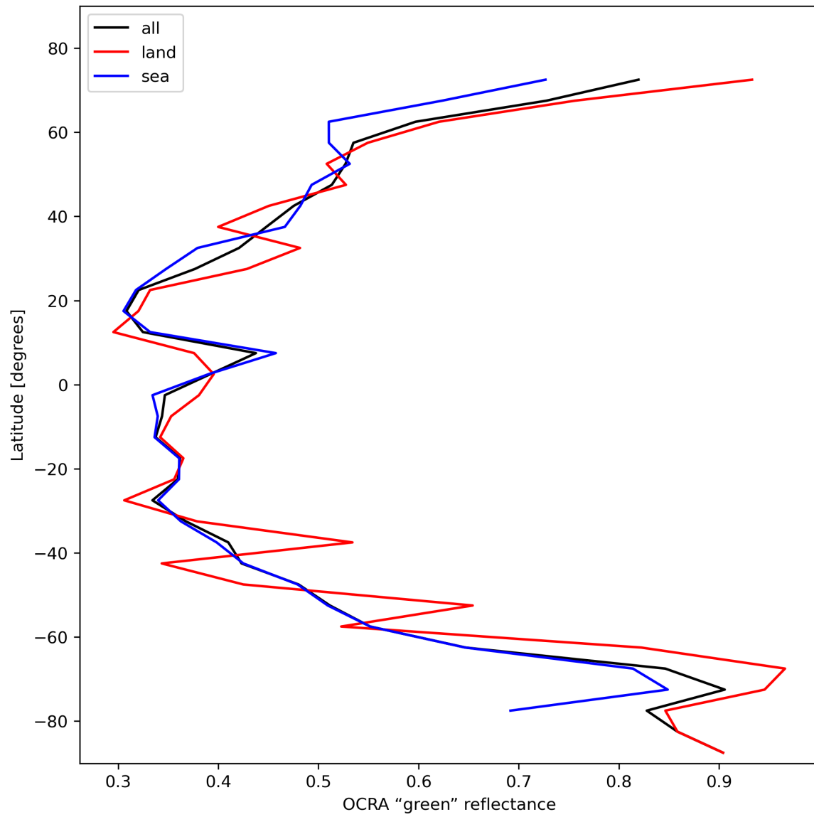
Figure 36: Zonal average of “OCRA “green” reflectance” for 2023-11-09 to 2023-11-11.
