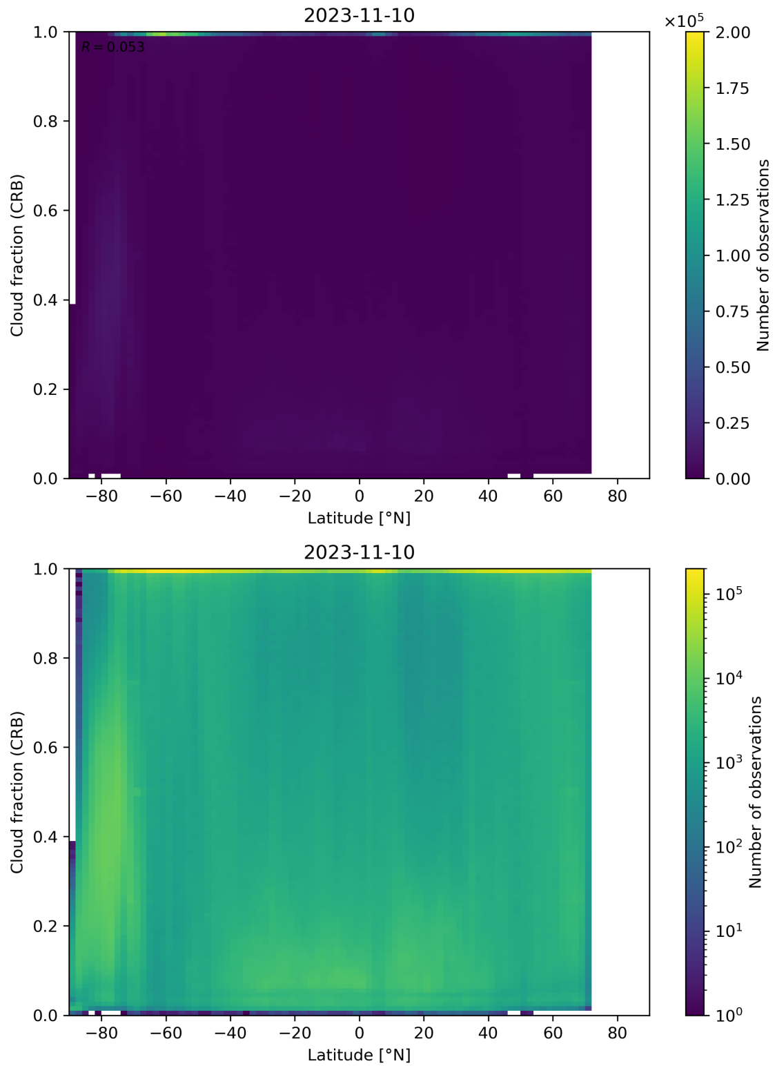
Figure 94: Scatter density plot of “Latitude” against “Cloud fraction (CRB)” for 2023-11-09 to 2023-11-11.
