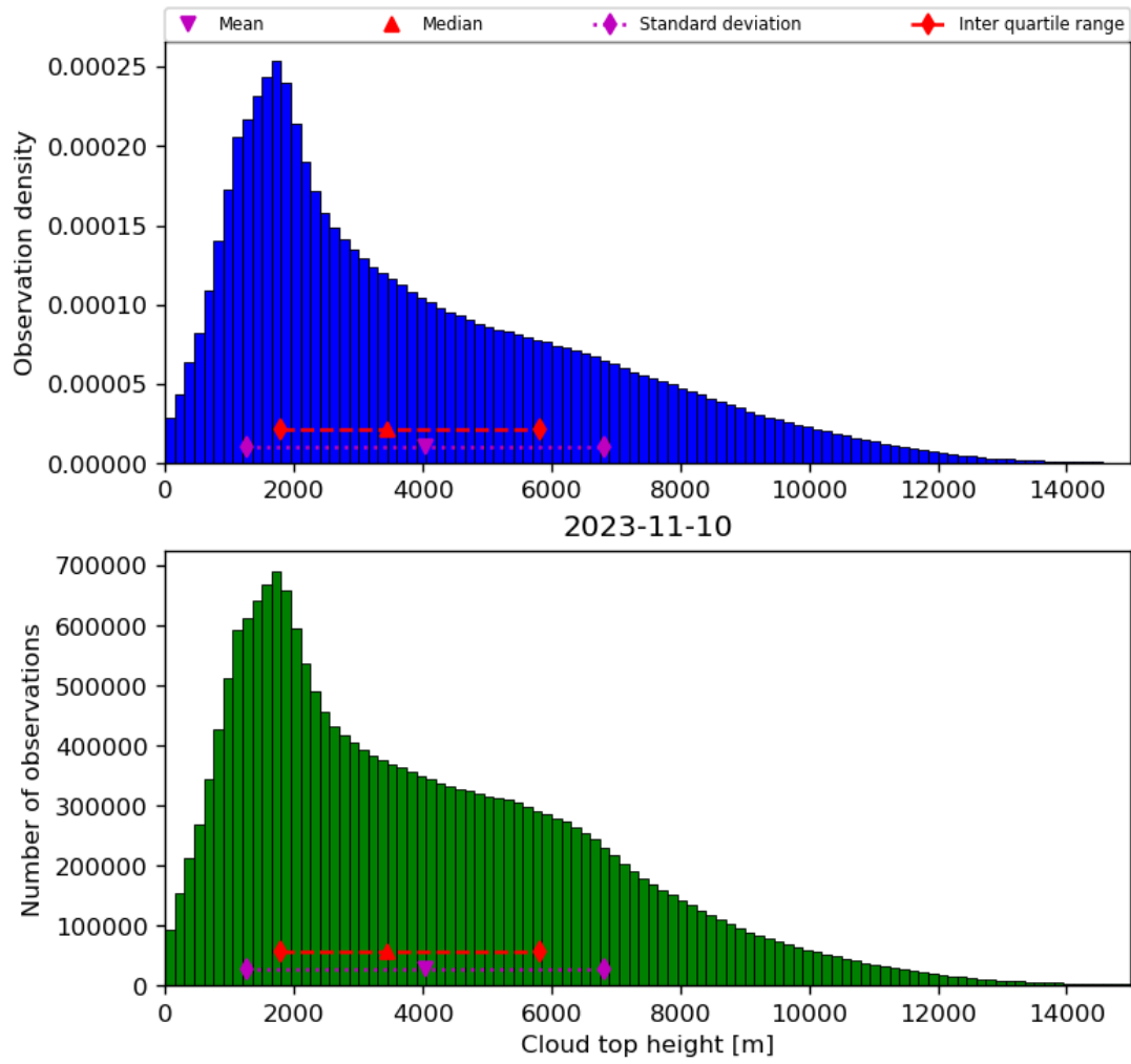
Figure 40: Histogram of “Cloud top height” for 2023-11-09 to 2023-11-11
