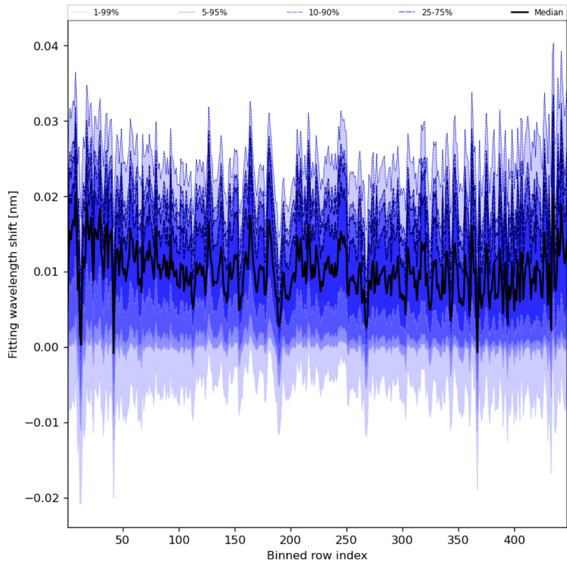
Figure 65: Along track statistics of “Fitting wavelength shift” for 2023-11-09 to 2023-11-11
