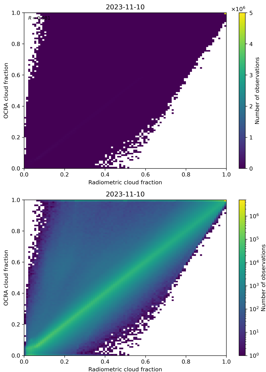
Figure 72: Scatter density plot of “Radiometric cloud fraction” against “OCRA cloud fraction” for 2023-11-09 to 2023-11-11.
