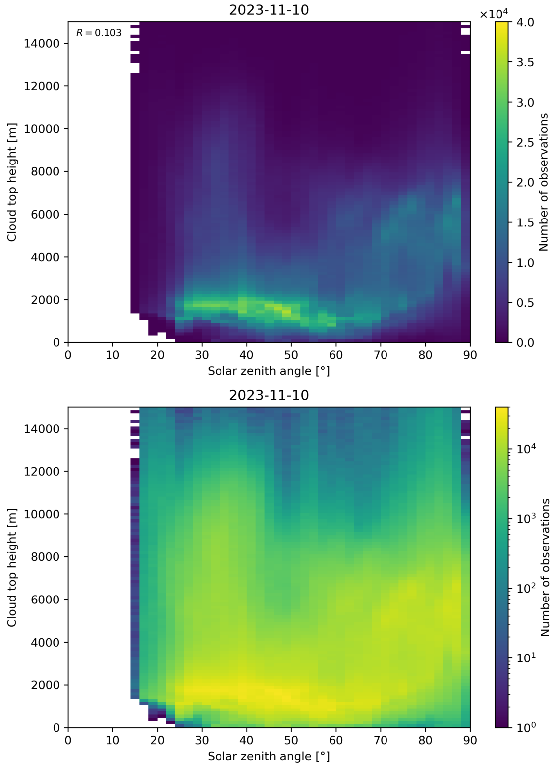
Figure 104: Scatter density plot of “Solar zenith angle” against “Cloud top height” for 2023-11-09 to 2023-11-11.
