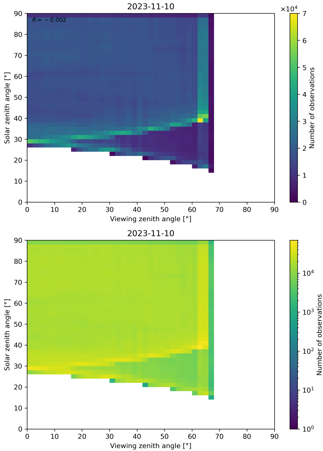
Figure 114: Scatter density plot of “Viewing zenith angle” against “Solar zenith angle” for 2023-11-09 to 2023-11-11.
