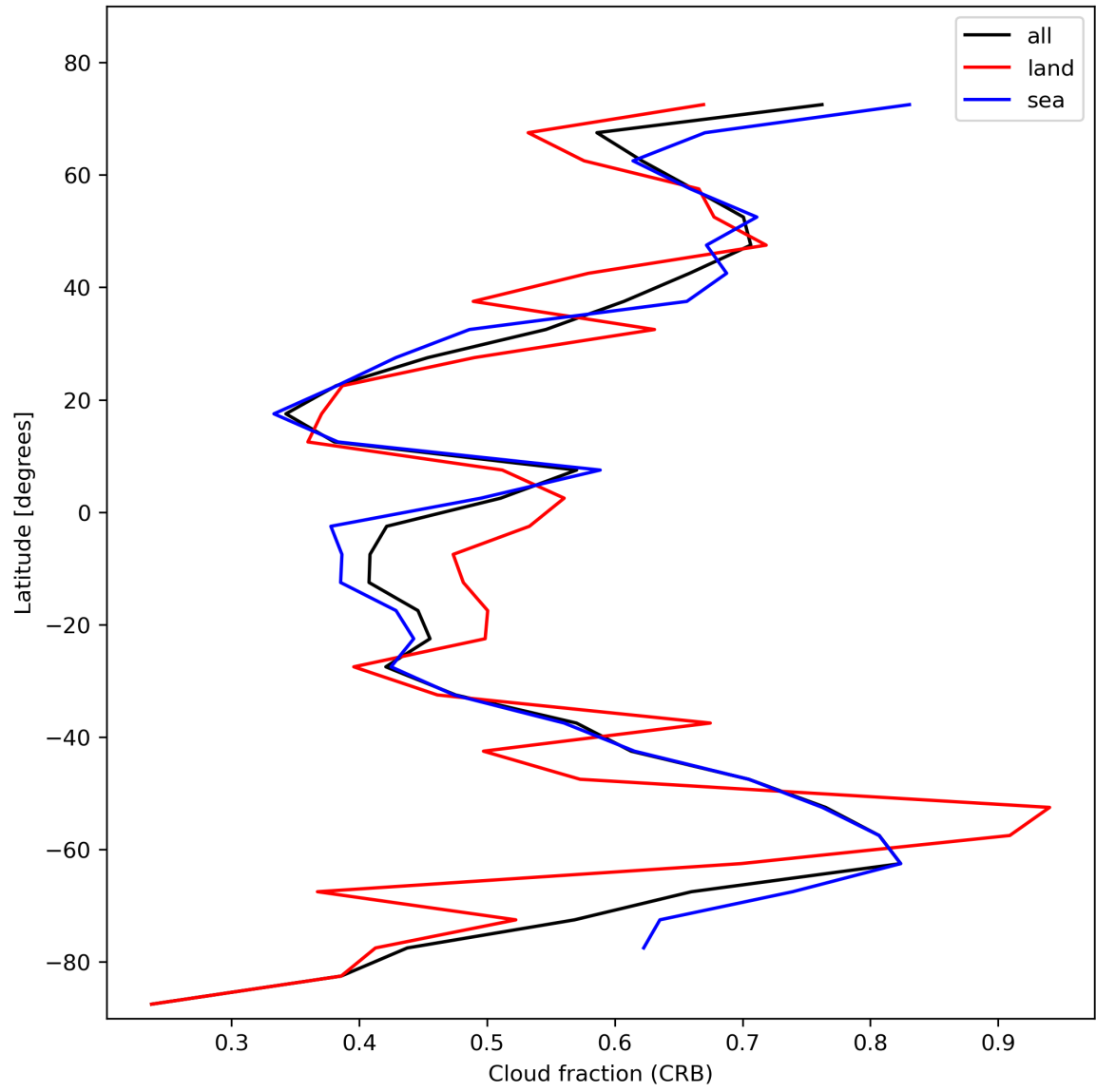
Figure 26: Zonal average of “Cloud fraction (CRB)” for 2023-11-09 to 2023-11-11.
