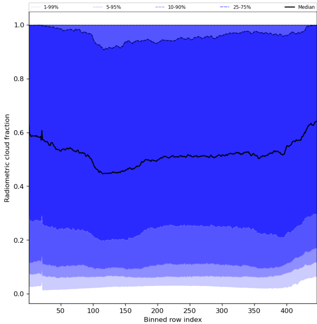
Figure 55: Along track statistics of “Radiometric cloud fraction” for 2023-11-09 to 2023-11-11
