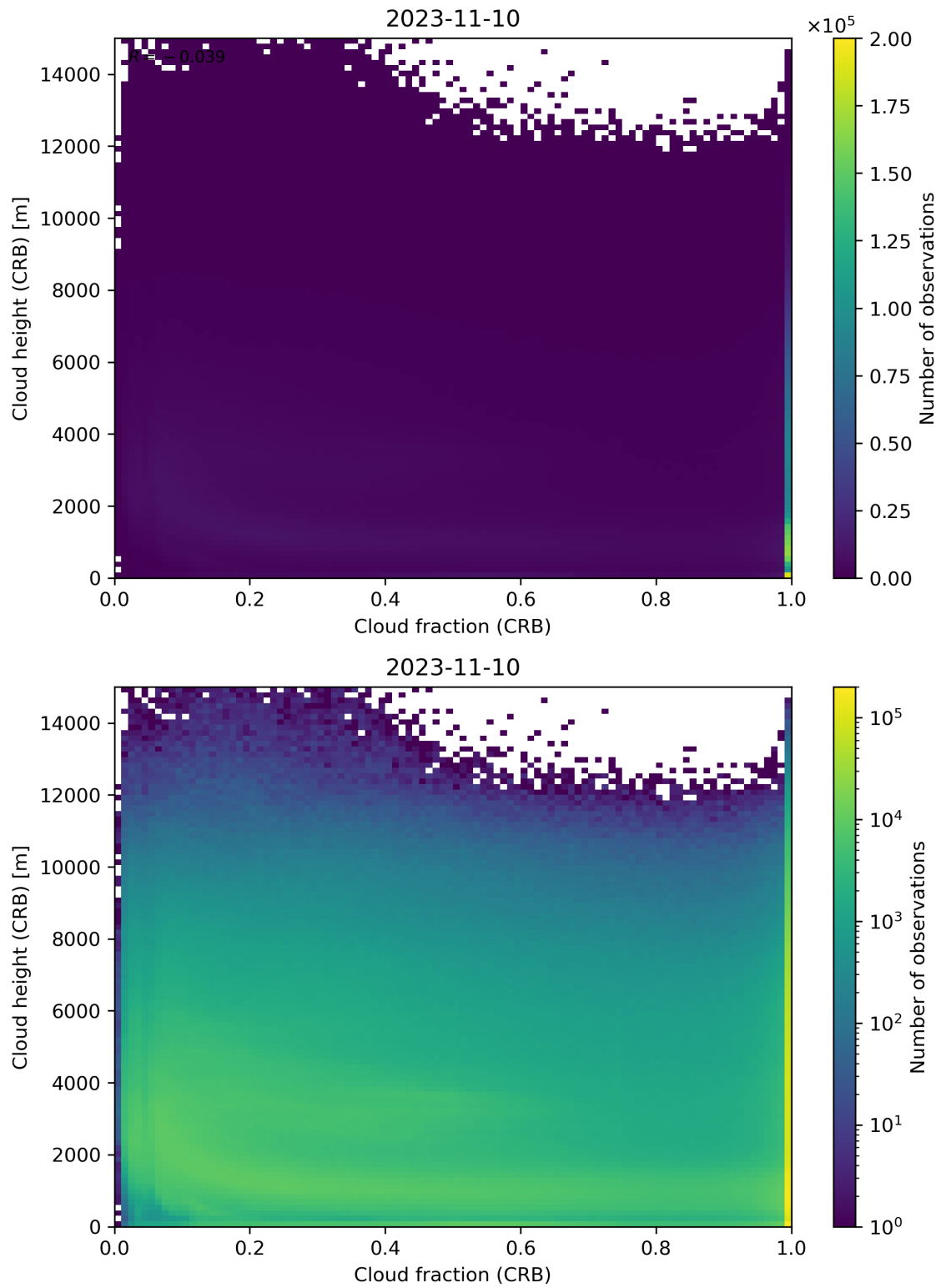
Figure 79: Scatter density plot of “Cloud fraction (CRB)” against “Cloud height (CRB)” for 2023-11-09 to 2023-11-11.
