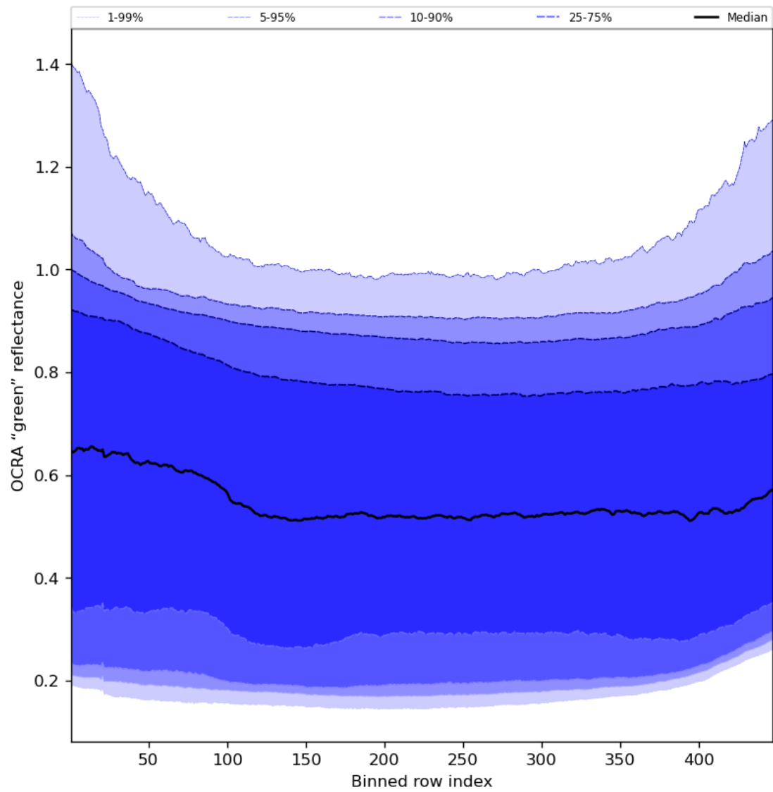
Figure 68: Along track statistics of “OCRA “green” reflectance” for 2023-11-09 to 2023-11-11
