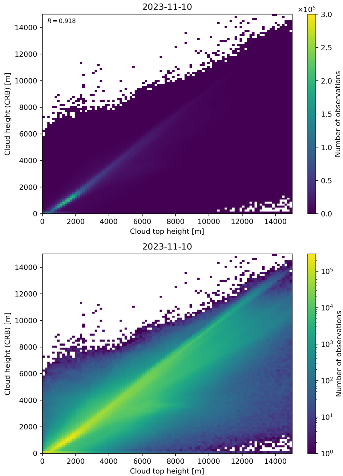
Figure 89: Scatter density plot of “Cloud top height” against “Cloud height (CRB)” for 2023-11-09 to 2023-11-11.
