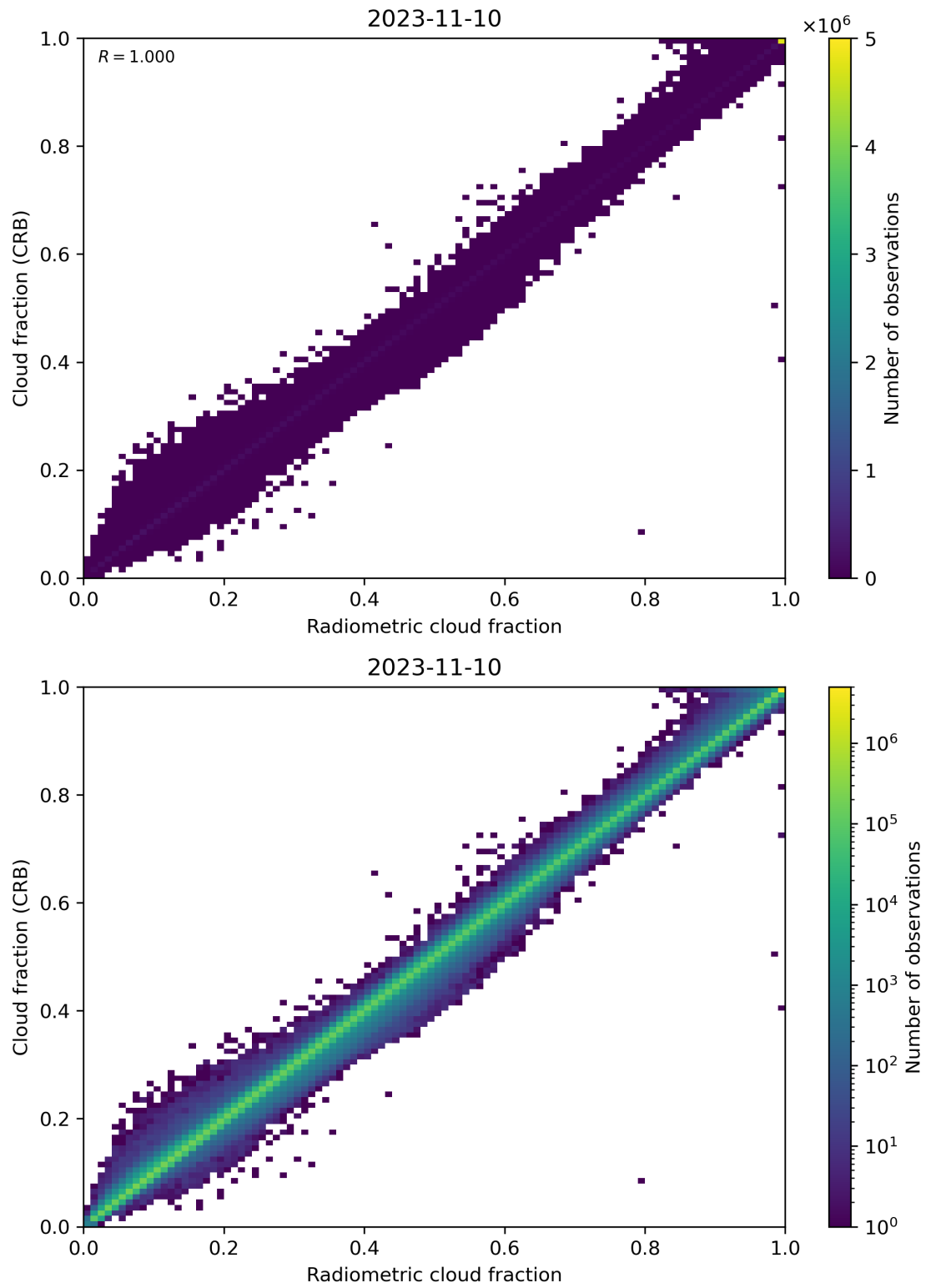
Figure 73: Scatter density plot of “Radiometric cloud fraction” against “Cloud fraction (CRB)” for 2023-11-09 to 2023-11-11.
