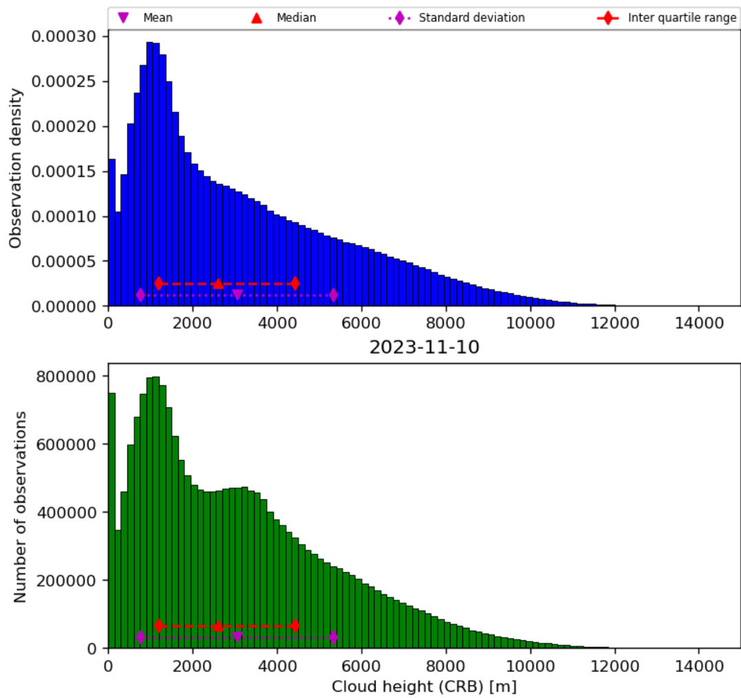
Figure 43: Histogram of “Cloud height (CRB)” for 2023-11-09 to 2023-11-11
