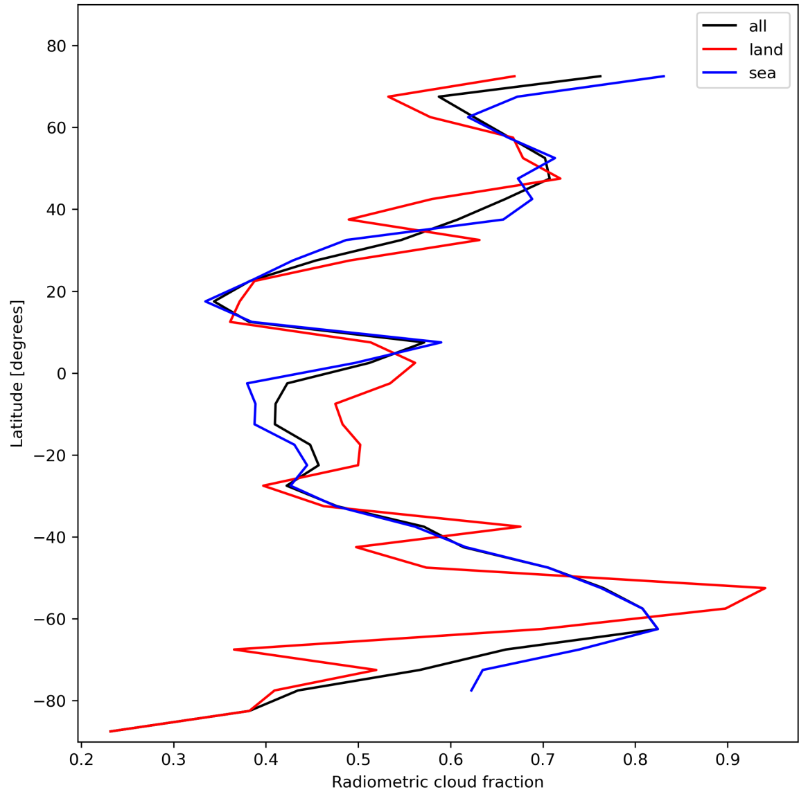
Figure 23: Zonal average of “Radiometric cloud fraction” for 2023-11-09 to 2023-11-11.
