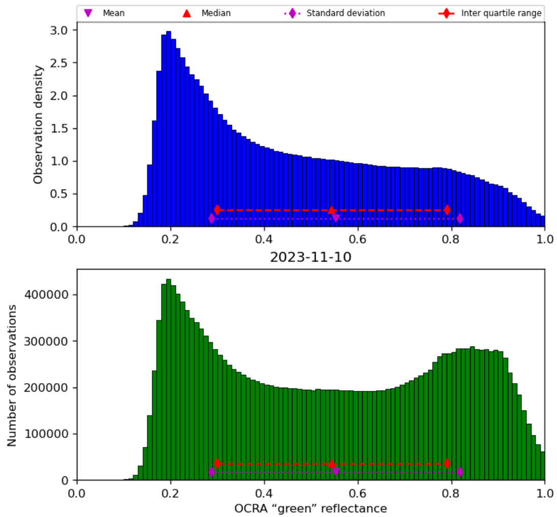
Figure 52: Histogram of “OCRA “green” reflectance” for 2023-11-09 to 2023-11-11
