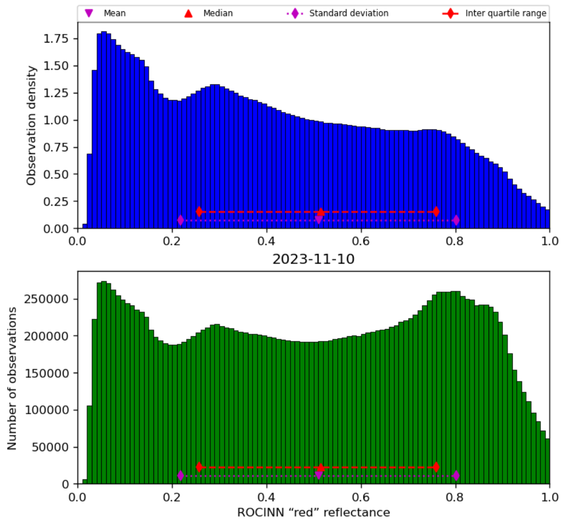
Figure 53: Histogram of “ROCINN “red” reflectance” for 2023-11-09 to 2023-11-11
