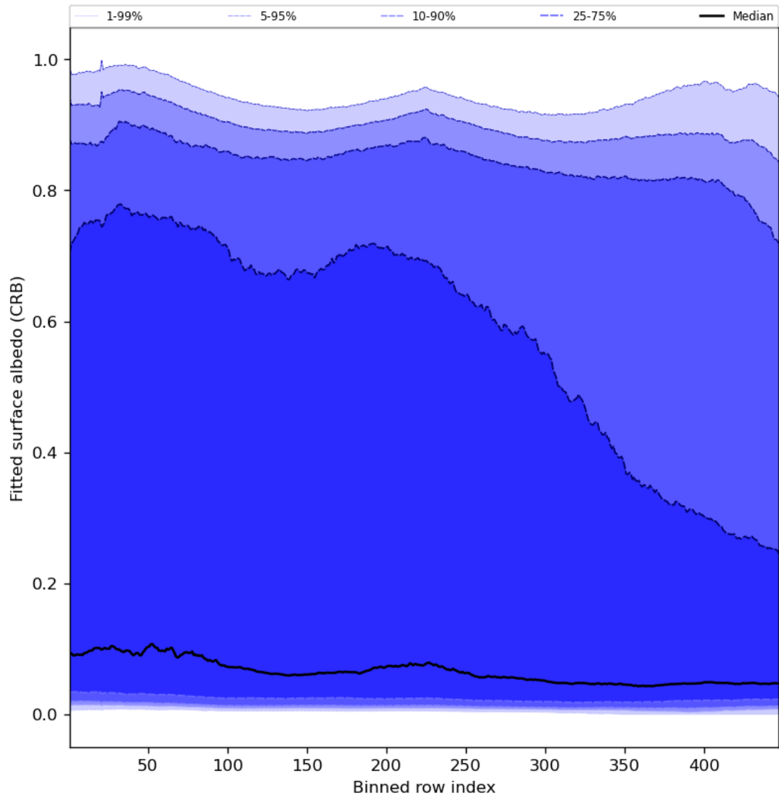
Figure 62: Along track statistics of “Fitted surface albedo (CRB)” for 2023-11-09 to 2023-11-11
