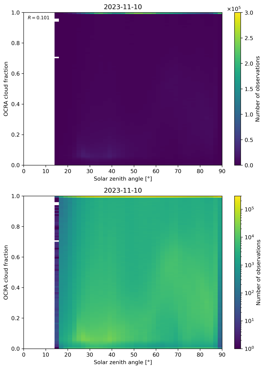
Figure 100: Scatter density plot of “Solar zenith angle” against “OCRA cloud fraction” for 2023-11-09 to 2023-11-11.
