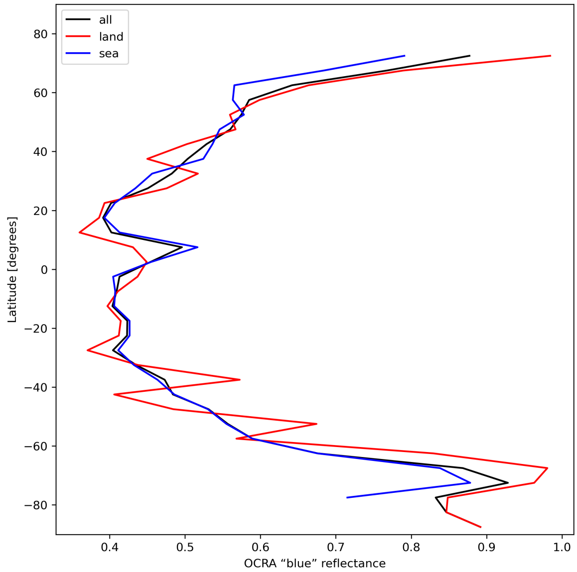
Figure 35: Zonal average of “OCRA “blue” reflectance” for 2023-11-09 to 2023-11-11.
