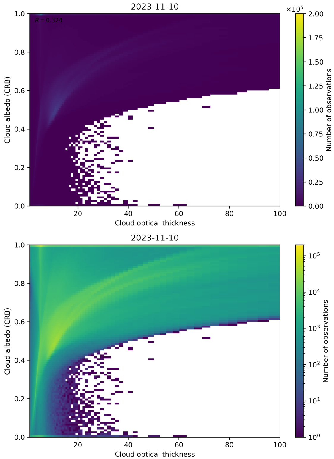
Figure 82: Scatter density plot of “Cloud optical thickness” against “Cloud albedo (CRB)” for 2023-11-09 to 2023-11-11.
