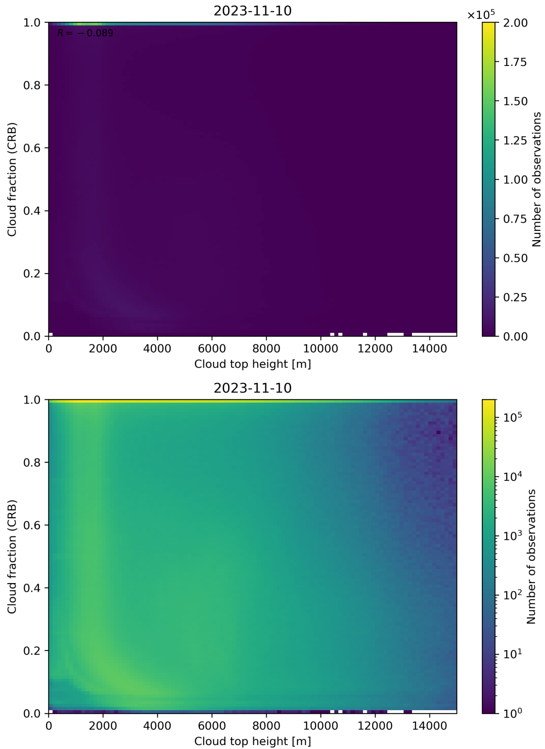
Figure 88: Scatter density plot of “Cloud top height” against “Cloud fraction (CRB)” for 2023-11-09 to 2023-11-11.
