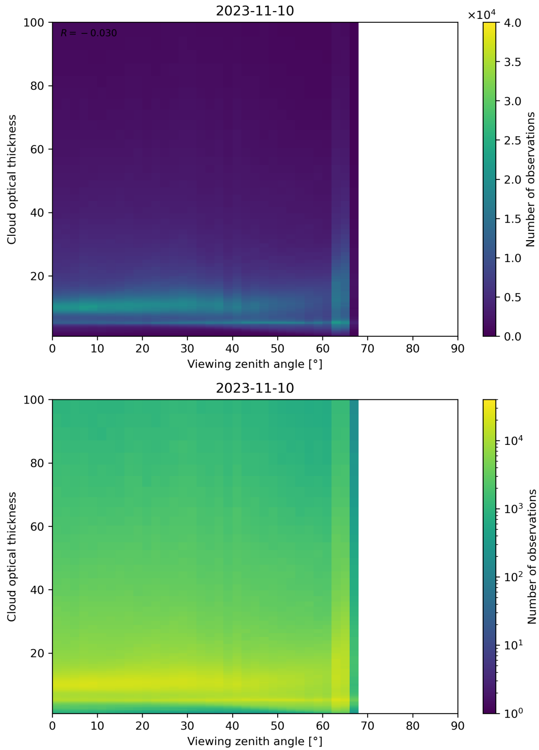
Figure 111: Scatter density plot of “Viewing zenith angle” against “Cloud optical thickness” for 2023-11-09 to 2023-11-11.
