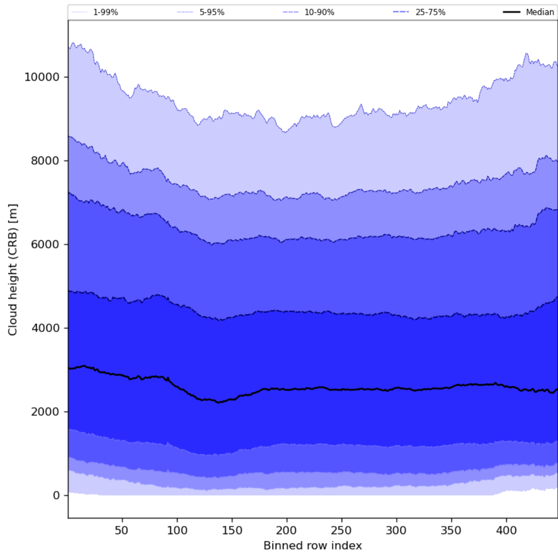
Figure 59: Along track statistics of “Cloud height (CRB)” for 2023-11-09 to 2023-11-11
