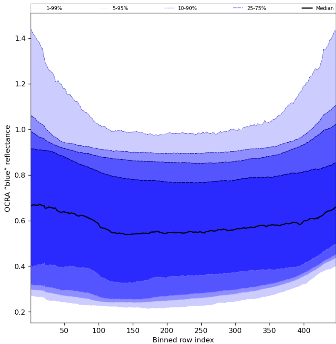
Figure 67: Along track statistics of “OCRA “blue” reflectance” for 2023-11-09 to 2023-11-11
