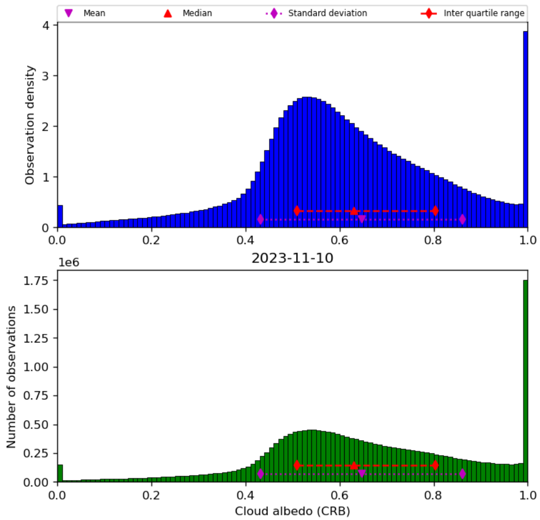
Figure 44: Histogram of “Cloud albedo (CRB)” for 2023-11-09 to 2023-11-11
