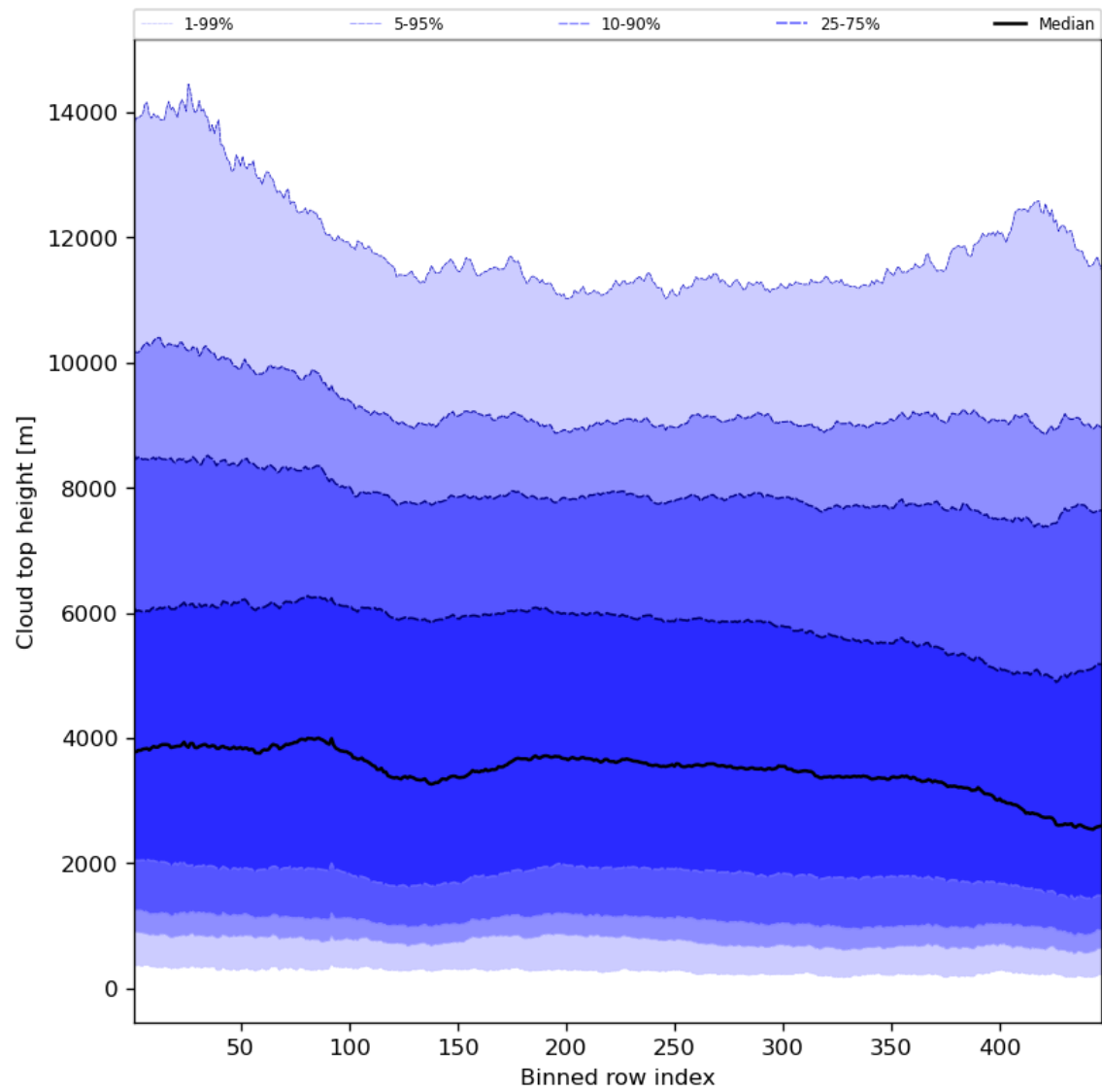
Figure 56: Along track statistics of “Cloud top height” for 2023-11-09 to 2023-11-11
