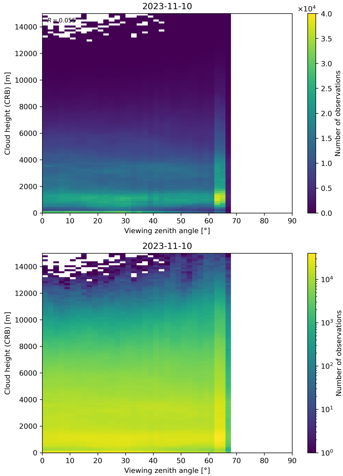
Figure 110: Scatter density plot of “Viewing zenith angle” against “Cloud height (CRB)” for 2023-11-09 to 2023-11-11.
