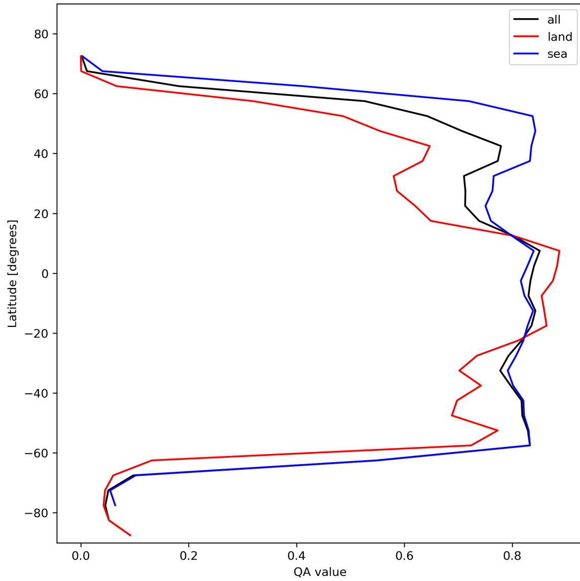
Figure 22: Zonal average of “QA value” for 2023-11-09 to 2023-11-11.
