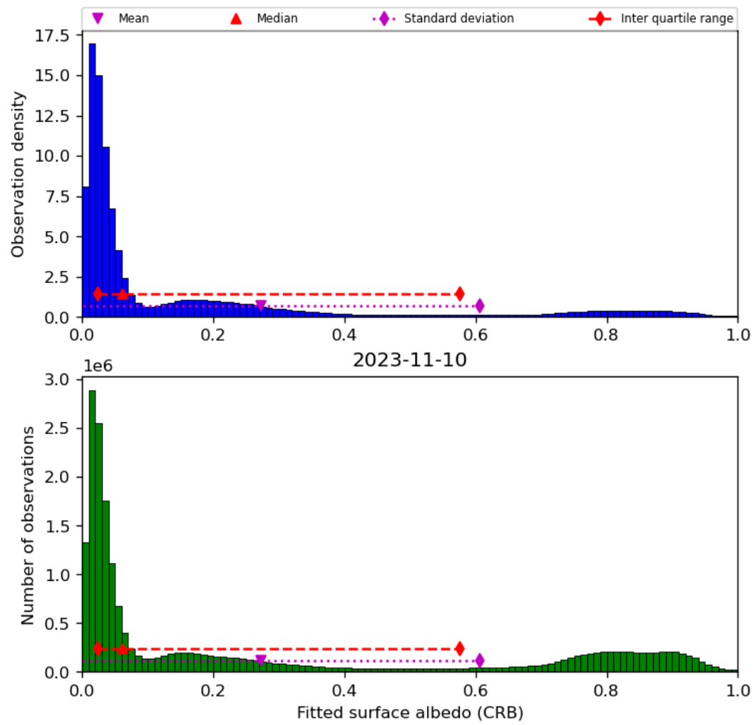
Figure 46: Histogram of “Fitted surface albedo (CRB)” for 2023-11-09 to 2023-11-11
