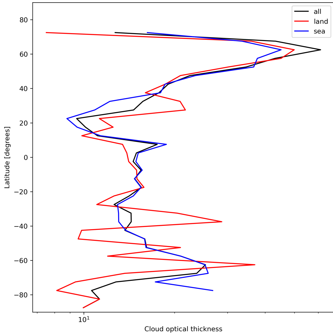
Figure 25: Zonal average of “Cloud optical thickness” for 2023-11-09 to 2023-11-11.
