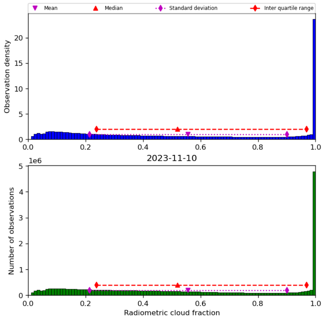
Figure 39: Histogram of "Radiometric cloud fraction" for 2023-11-09 to 2023-11-11
