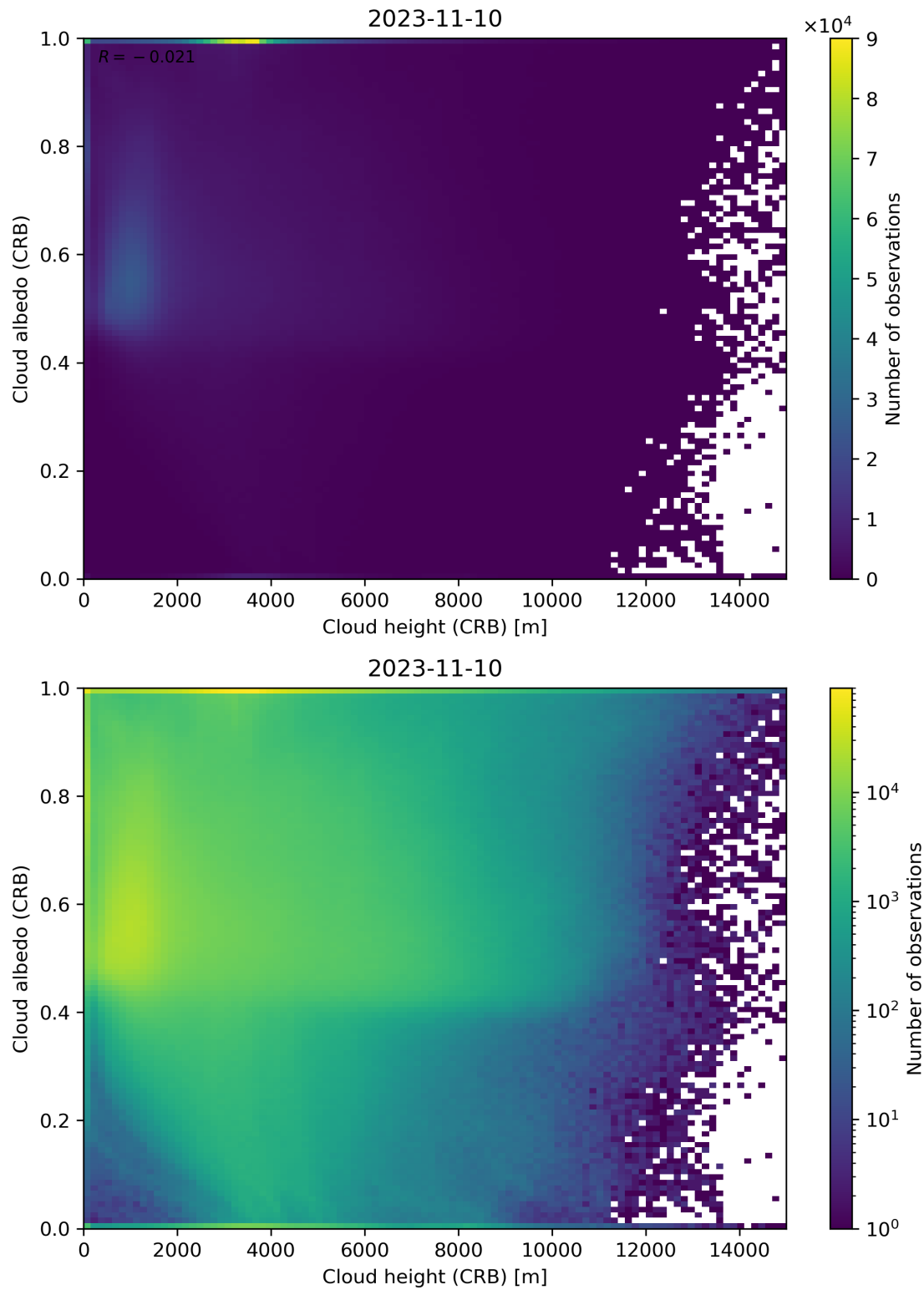
Figure 80: Scatter density plot of “Cloud height (CRB)” against “Cloud albedo (CRB)” for 2023-11-09 to 2023-11-11.
