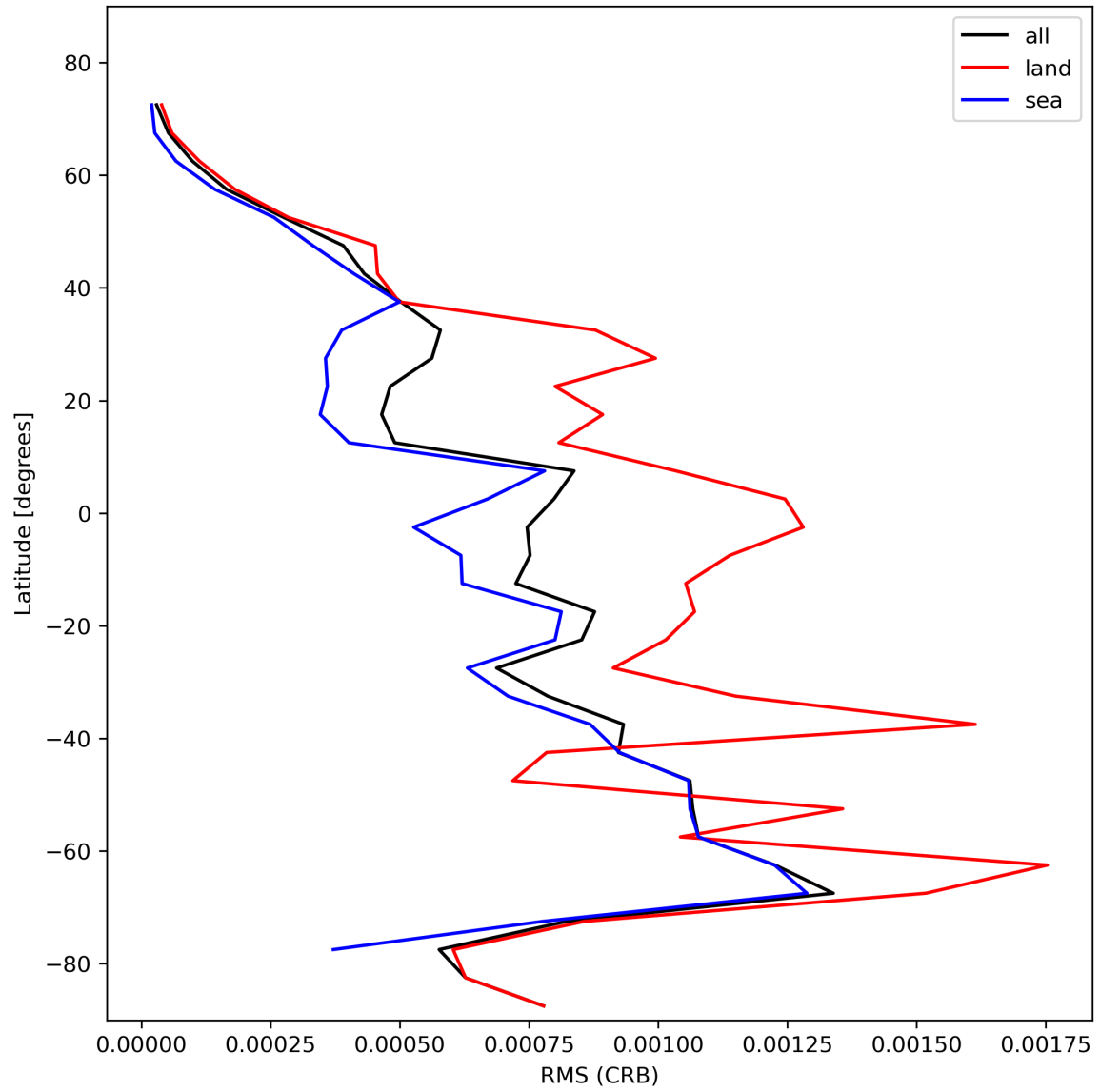
Figure 32: Zonal average of “RMS (CRB)” for 2023-11-09 to 2023-11-11.
