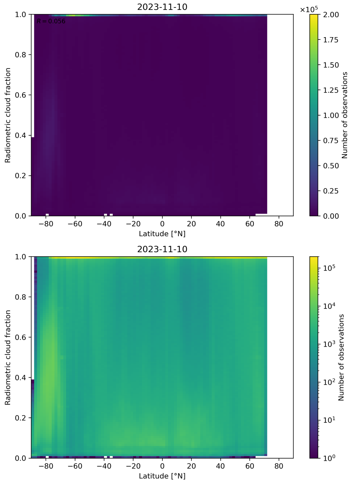
Figure 92: Scatter density plot of “Latitude” against “Radiometric cloud fraction” for 2023-11-09 to 2023-11-11.
