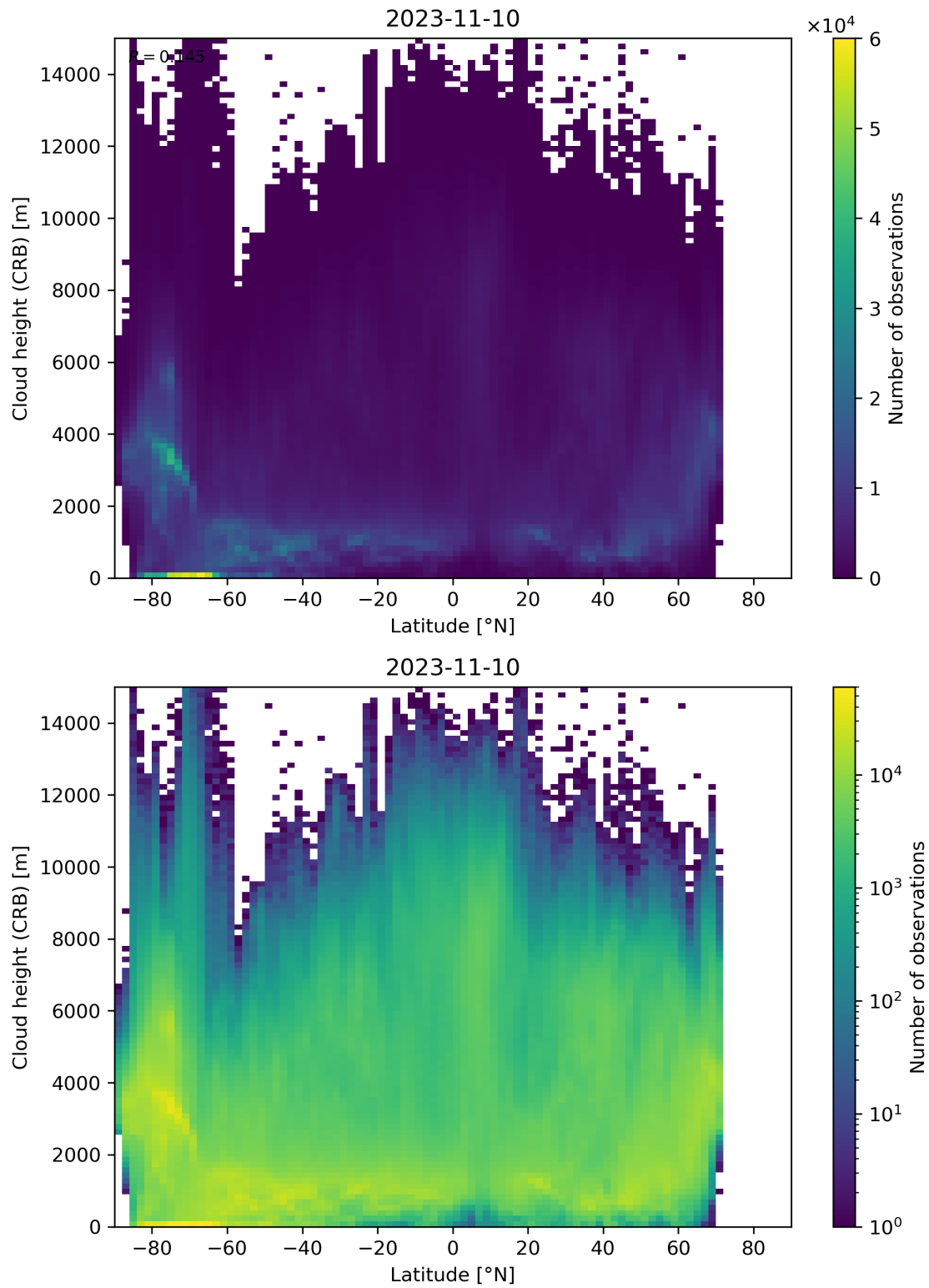
Figure 95: Scatter density plot of “Latitude” against “Cloud height (CRB)” for 2023-11-09 to 2023-11-11.
