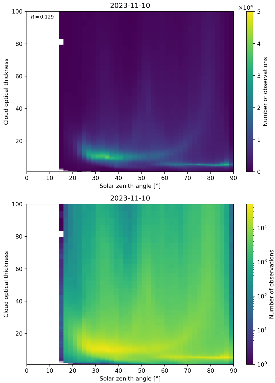
Figure 103: Scatter density plot of “Solar zenith angle” against “Cloud optical thickness” for 2023-11-09 to 2023-11-11.
