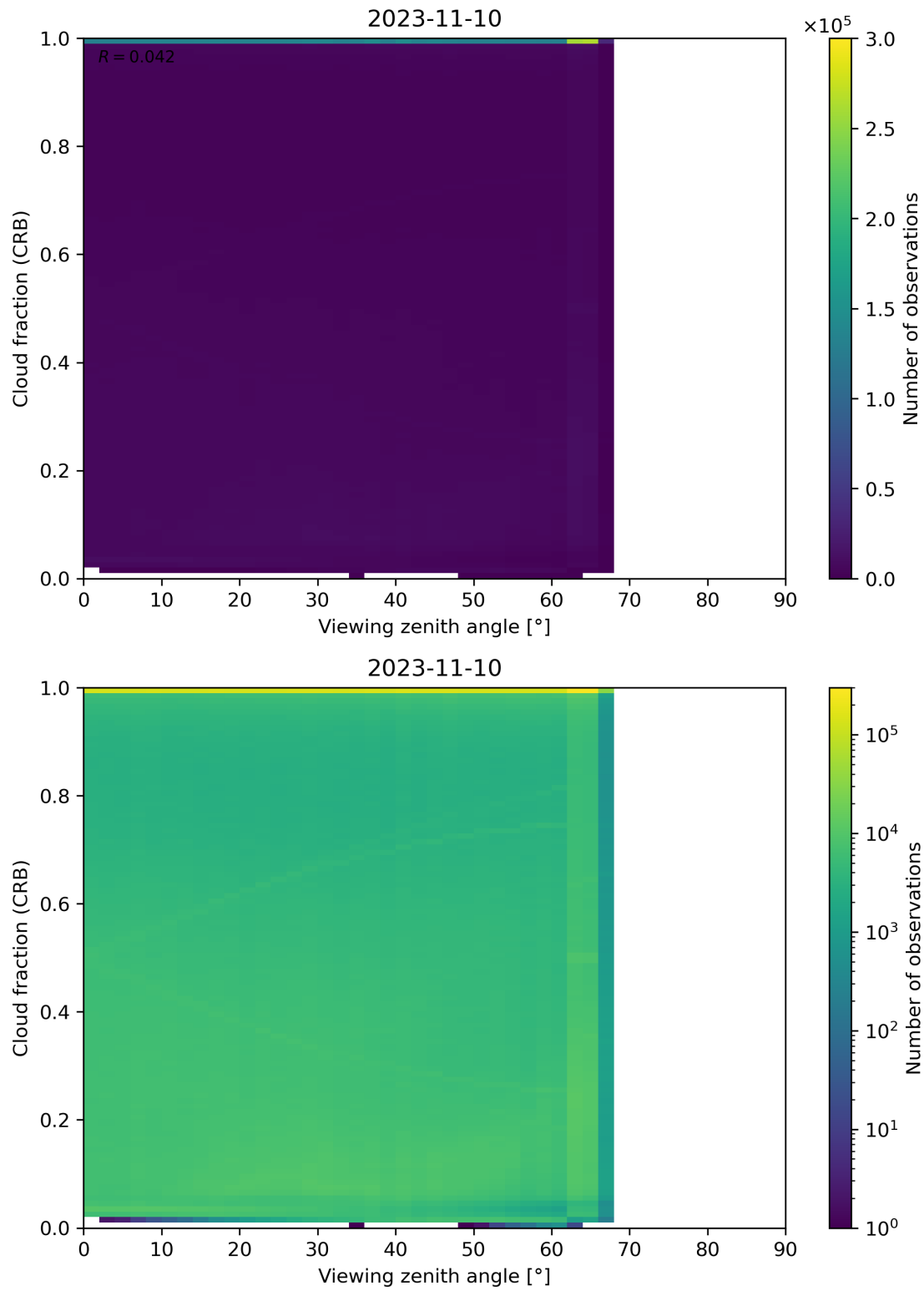
Figure 109: Scatter density plot of “Viewing zenith angle” against “Cloud fraction (CRB)” for 2023-11-09 to 2023-11-11.
