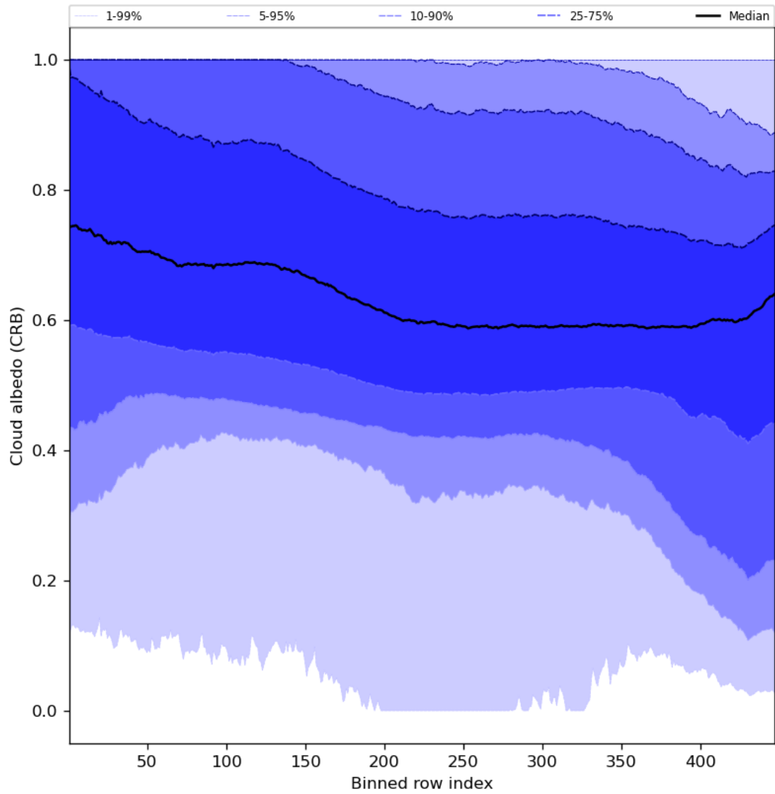
Figure 60: Along track statistics of “Cloud albedo (CRB)” for 2023-11-09 to 2023-11-11
