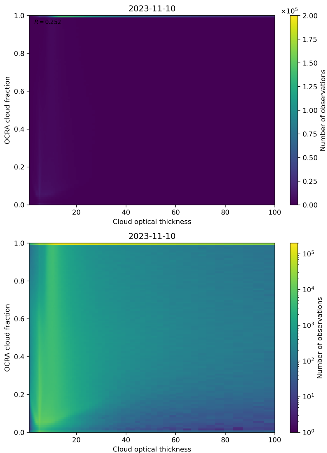
Figure 83: Scatter density plot of “Cloud optical thickness” against “OCRA cloud fraction” for 2023-11-09 to 2023-11-11.
