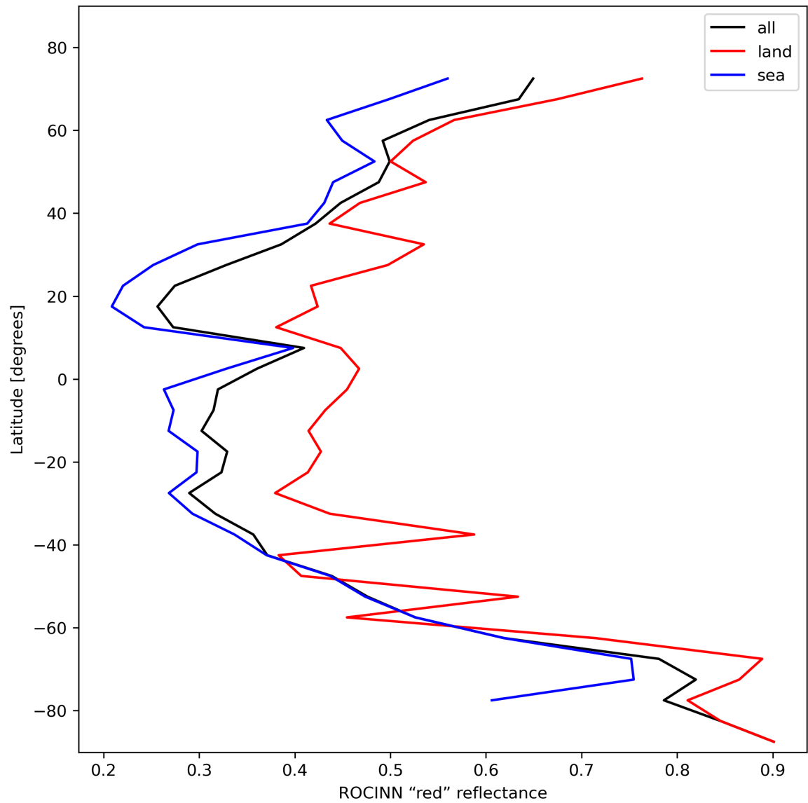
Figure 37: Zonal average of "ROCINN "red" reflectance" for 2023-11-09 to 2023-11-11.
