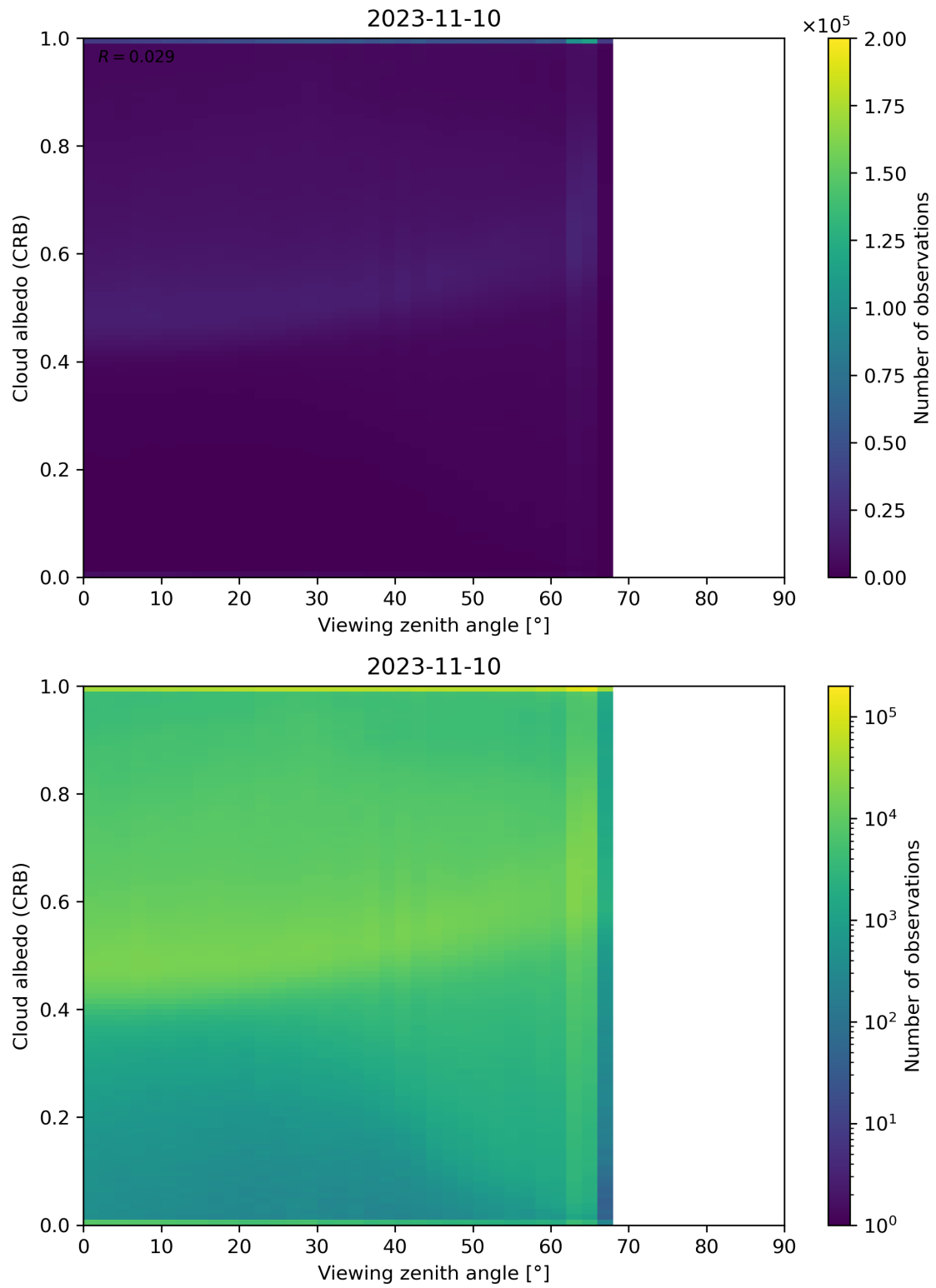
Figure 106: Scatter density plot of “Viewing zenith angle” against “Cloud albedo (CRB)” for 2023-11-09 to 2023-11-11.
