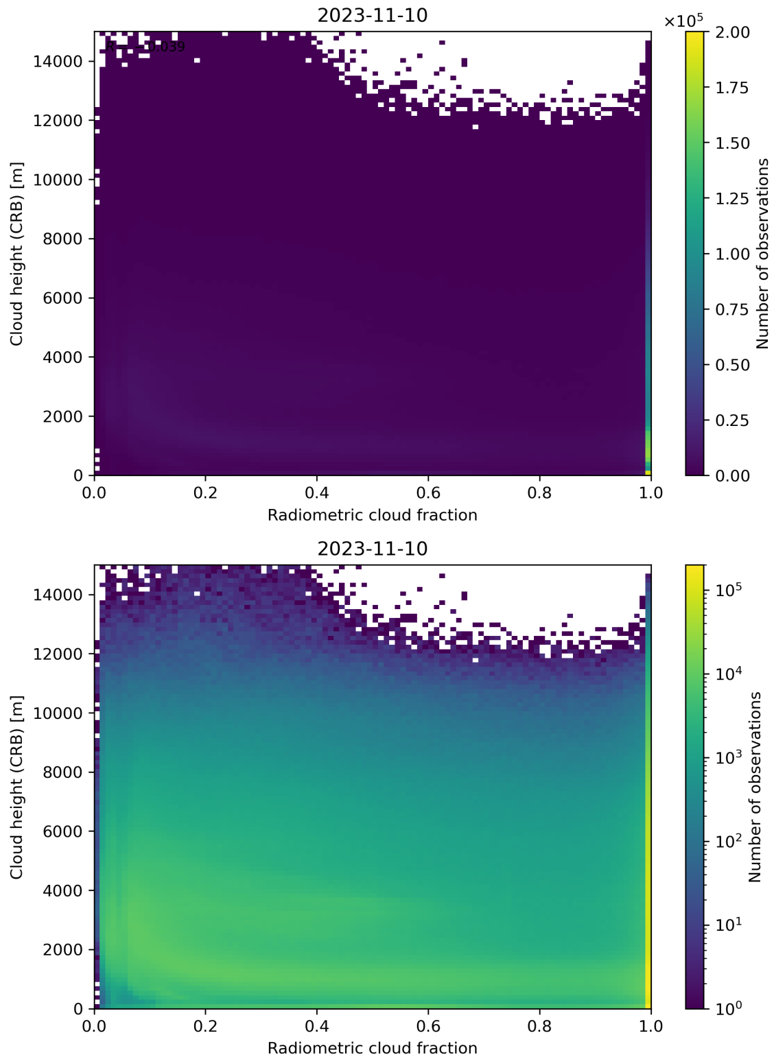
Figure 74: Scatter density plot of “Radiometric cloud fraction” against “Cloud height (CRB)” for 2023-11-09 to 2023-11-11.
