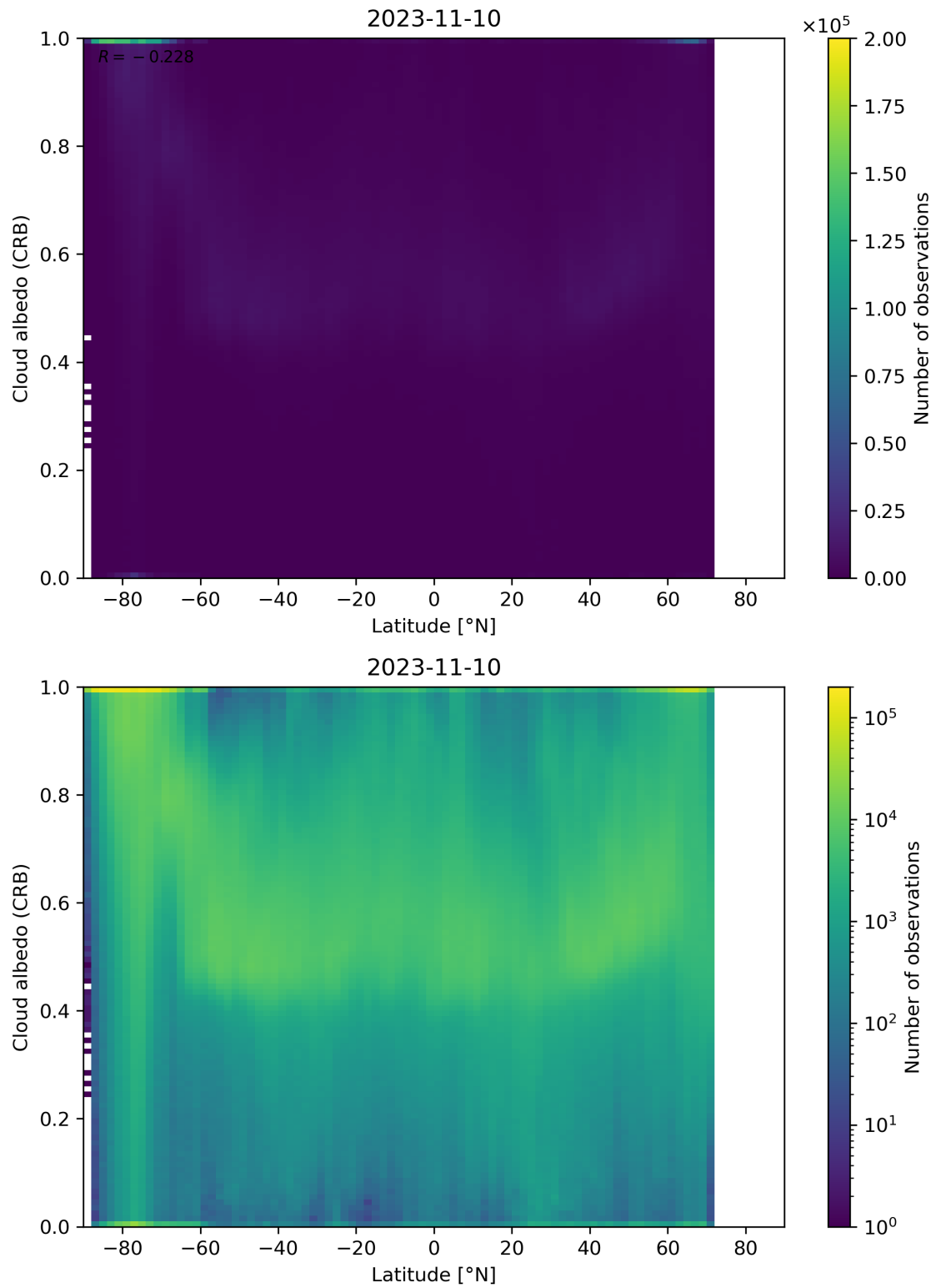
Figure 91: Scatter density plot of “Latitude” against “Cloud albedo (CRB)” for 2023-11-09 to 2023-11-11.
