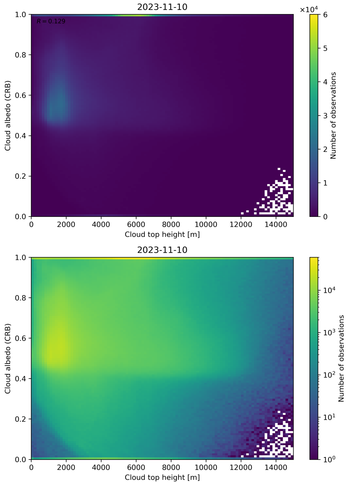
Figure 86: Scatter density plot of “Cloud top height” against “Cloud albedo (CRB)” for 2023-11-09 to 2023-11-11.
