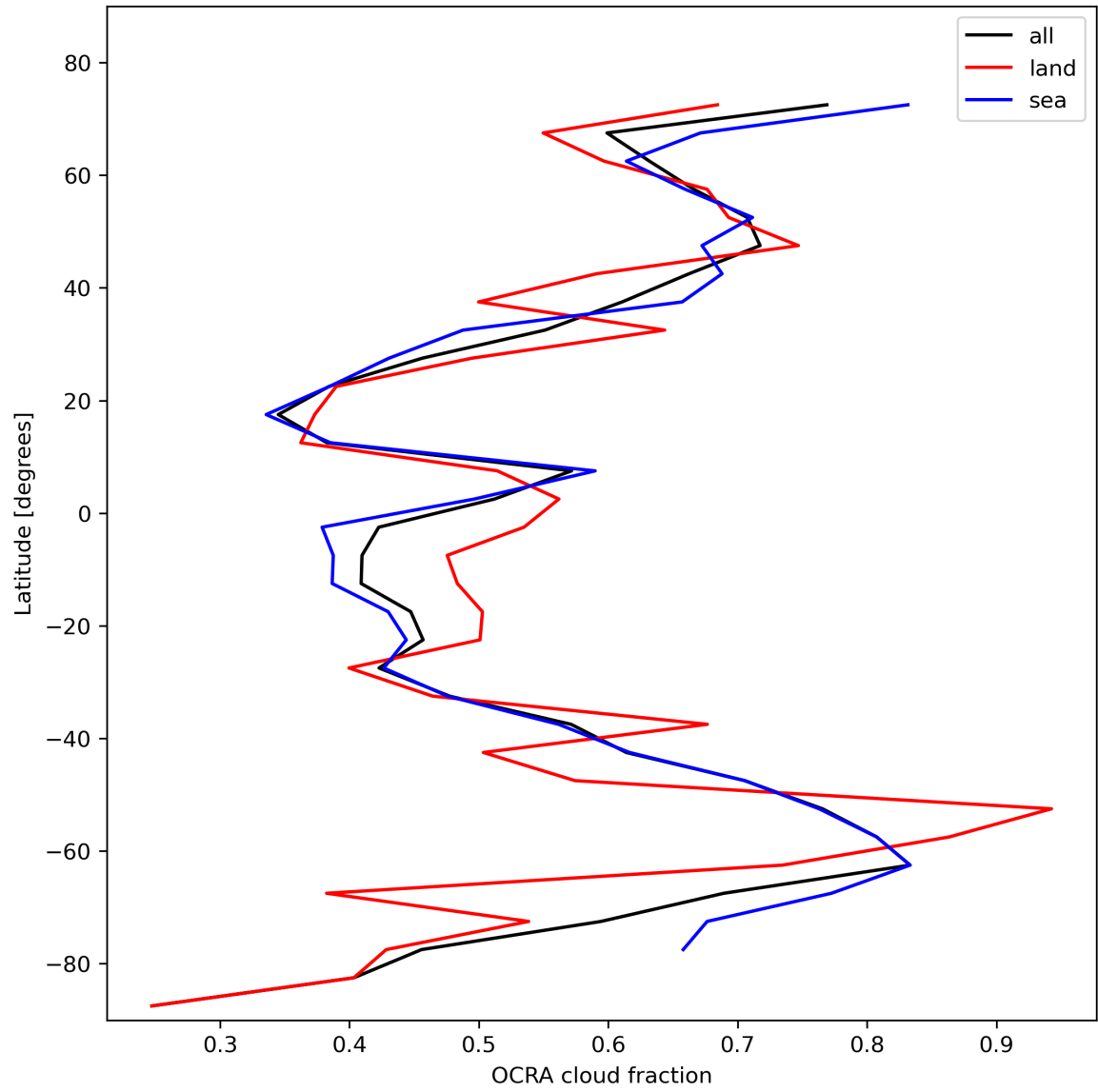
Figure 34: Zonal average of “OCRA cloud fraction” for 2023-11-09 to 2023-11-11.
