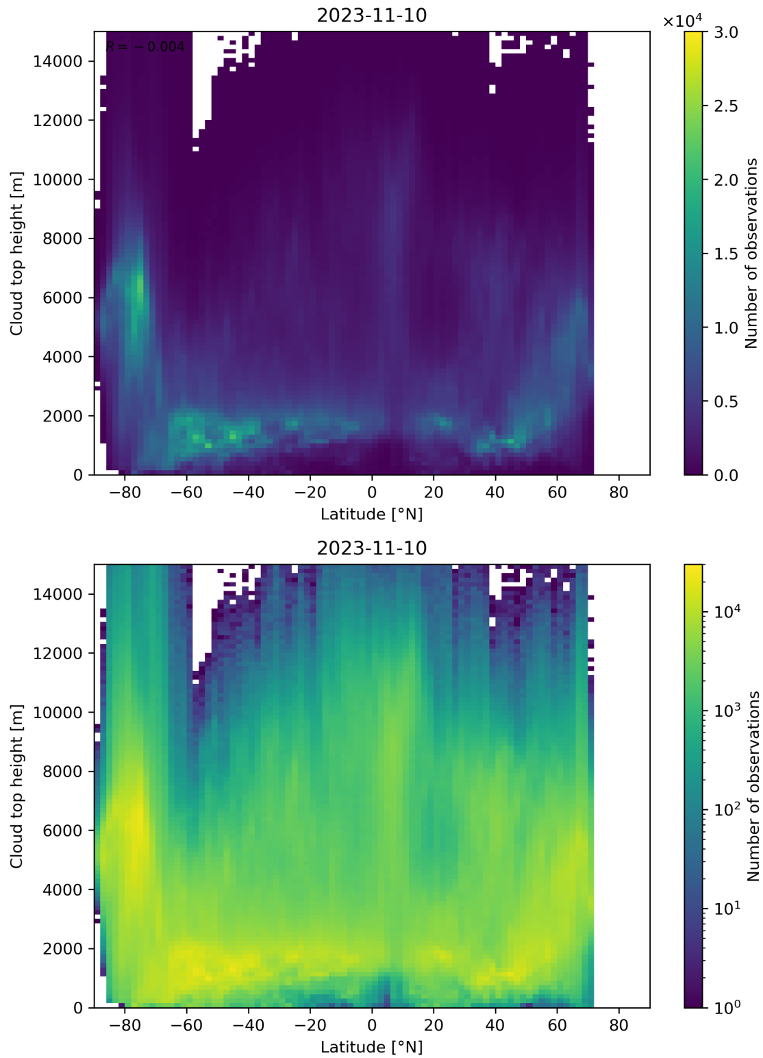
Figure 97: Scatter density plot of “Latitude” against “Cloud top height” for 2023-11-09 to 2023-11-11.
