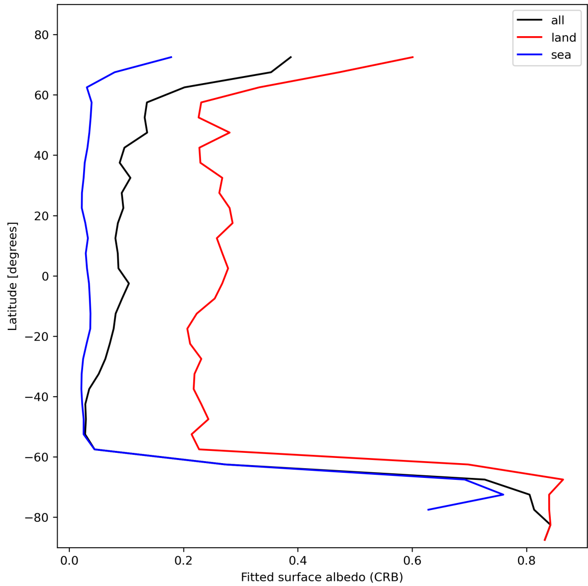
Figure 30: Zonal average of “Fitted surface albedo (CRB)” for 2023-11-09 to 2023-11-11.
