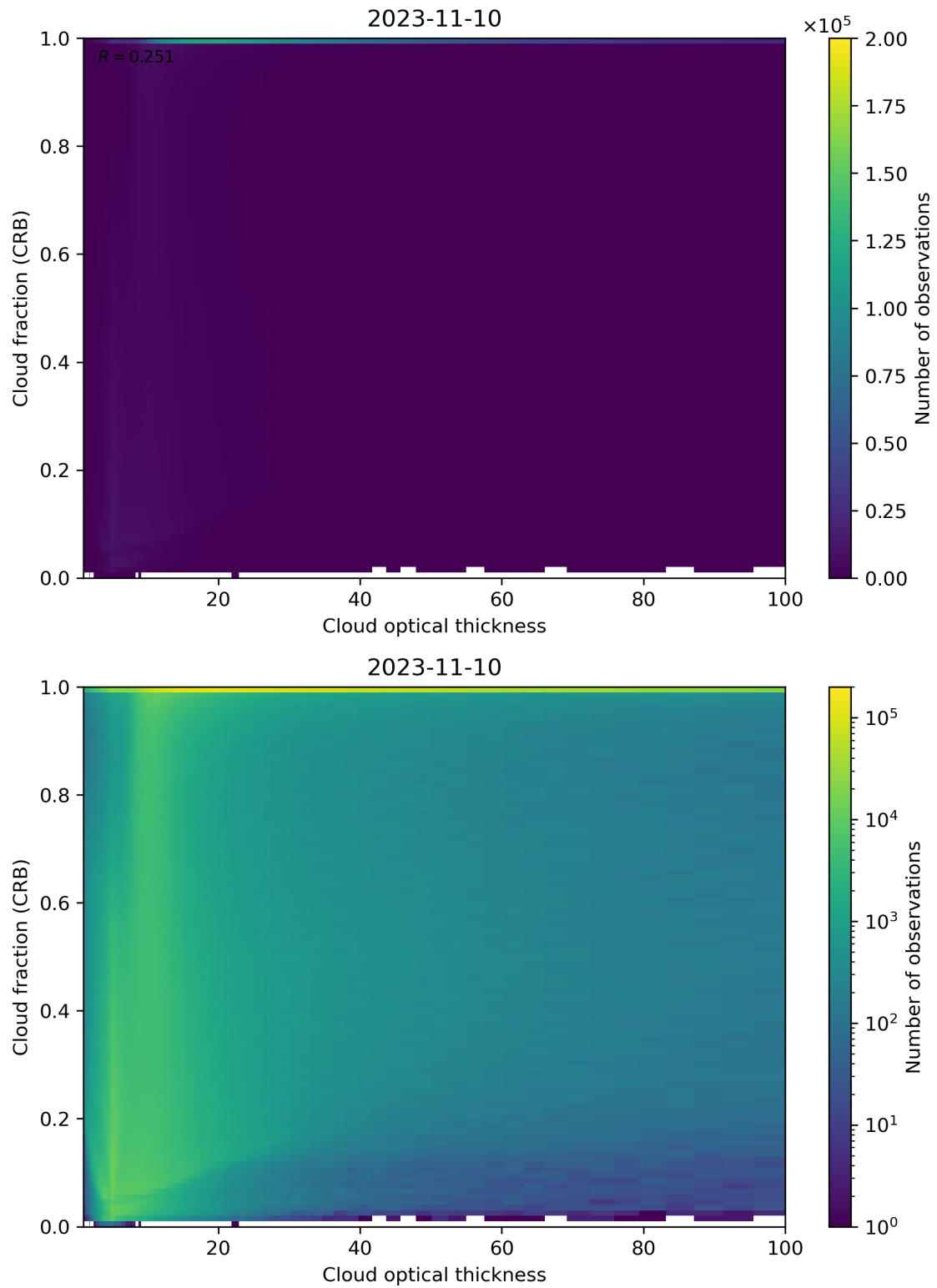
Figure 84: Scatter density plot of “Cloud optical thickness” against “Cloud fraction (CRB)” for 2023-11-09 to 2023-11-11.
