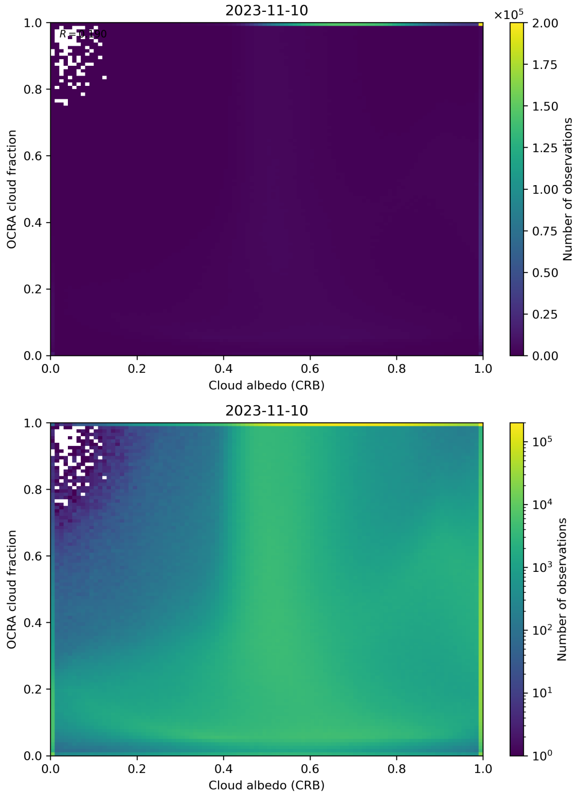
Figure 70: Scatter density plot of “Cloud albedo (CRB)” against “OCRA cloud fraction” for 2023-11-09 to 2023-11-11.
