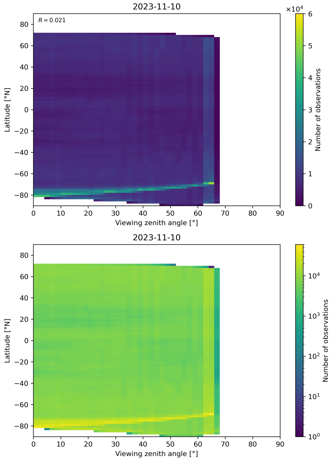
Figure 113: Scatter density plot of “Viewing zenith angle” against “Latitude” for 2023-11-09 to 2023-11-11.
