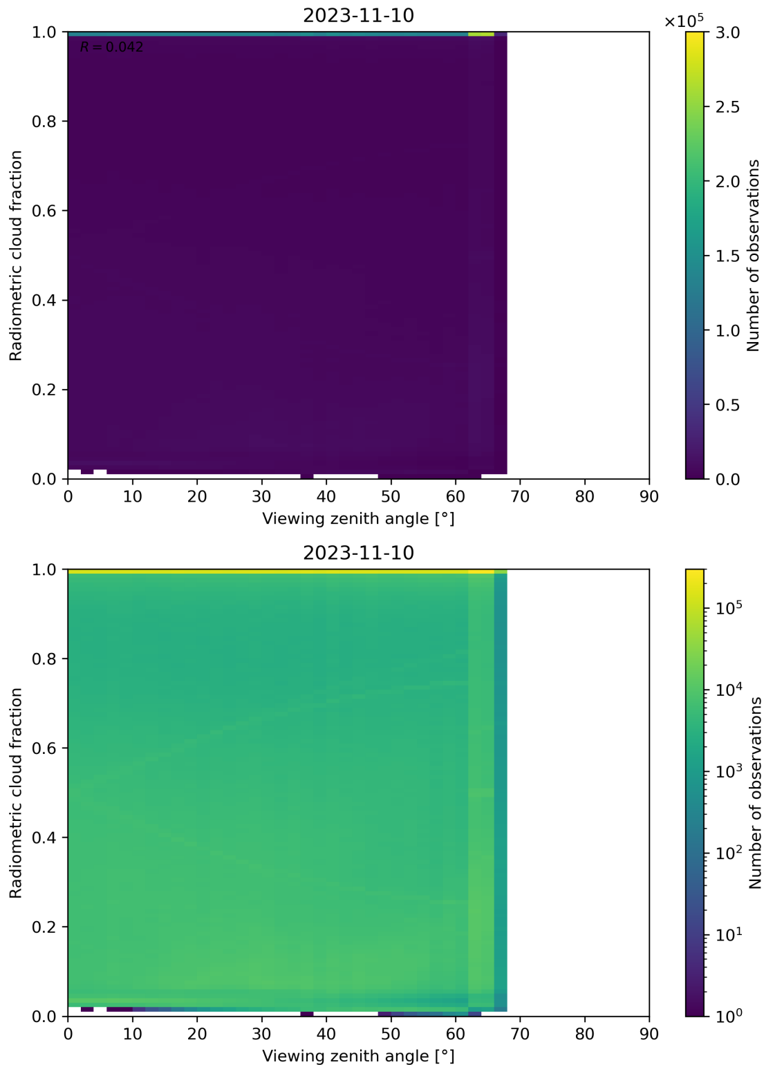
Figure 107: Scatter density plot of “Viewing zenith angle” against “Radiometric cloud fraction” for 2023-11-09 to 2023-11-11.
