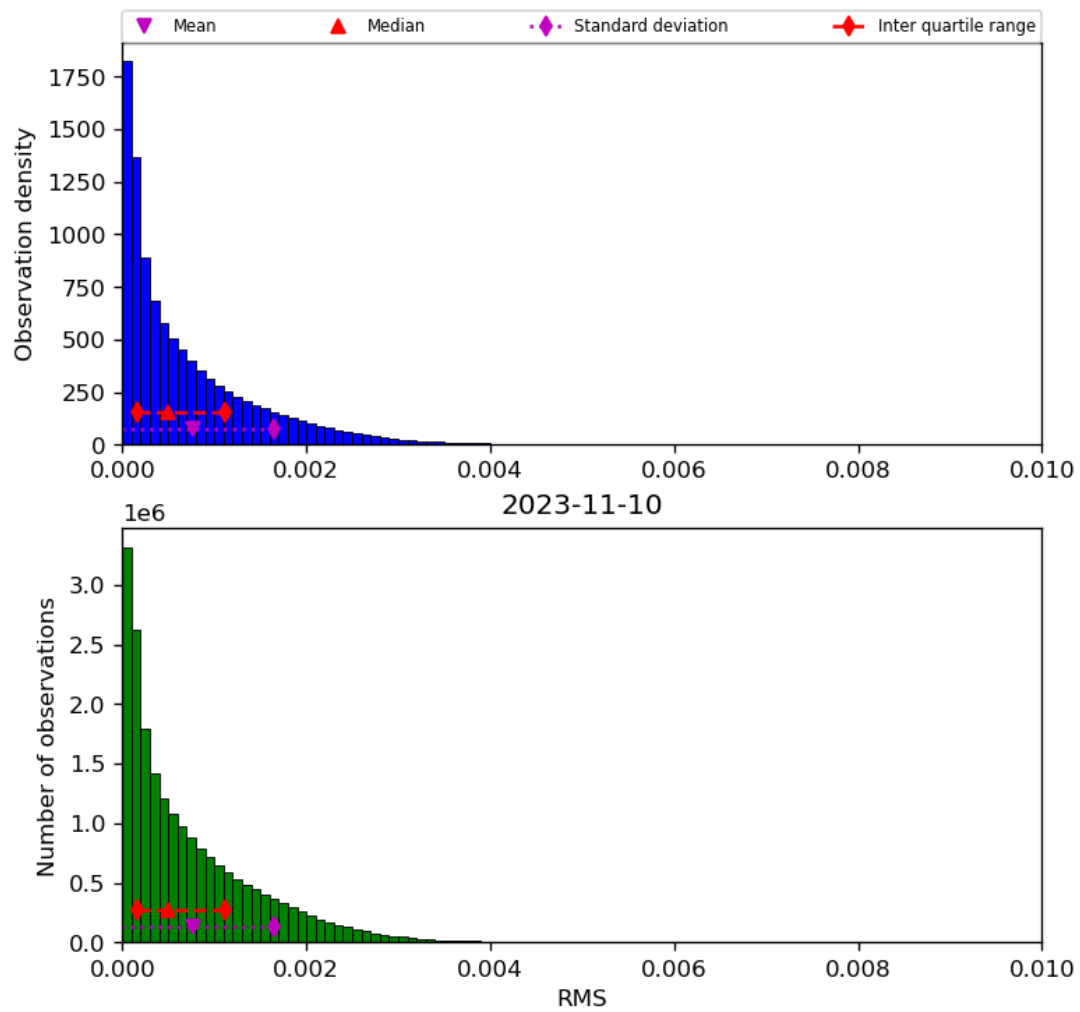
Figure 47: Histogram of “RMS” for 2023-11-09 to 2023-11-11
