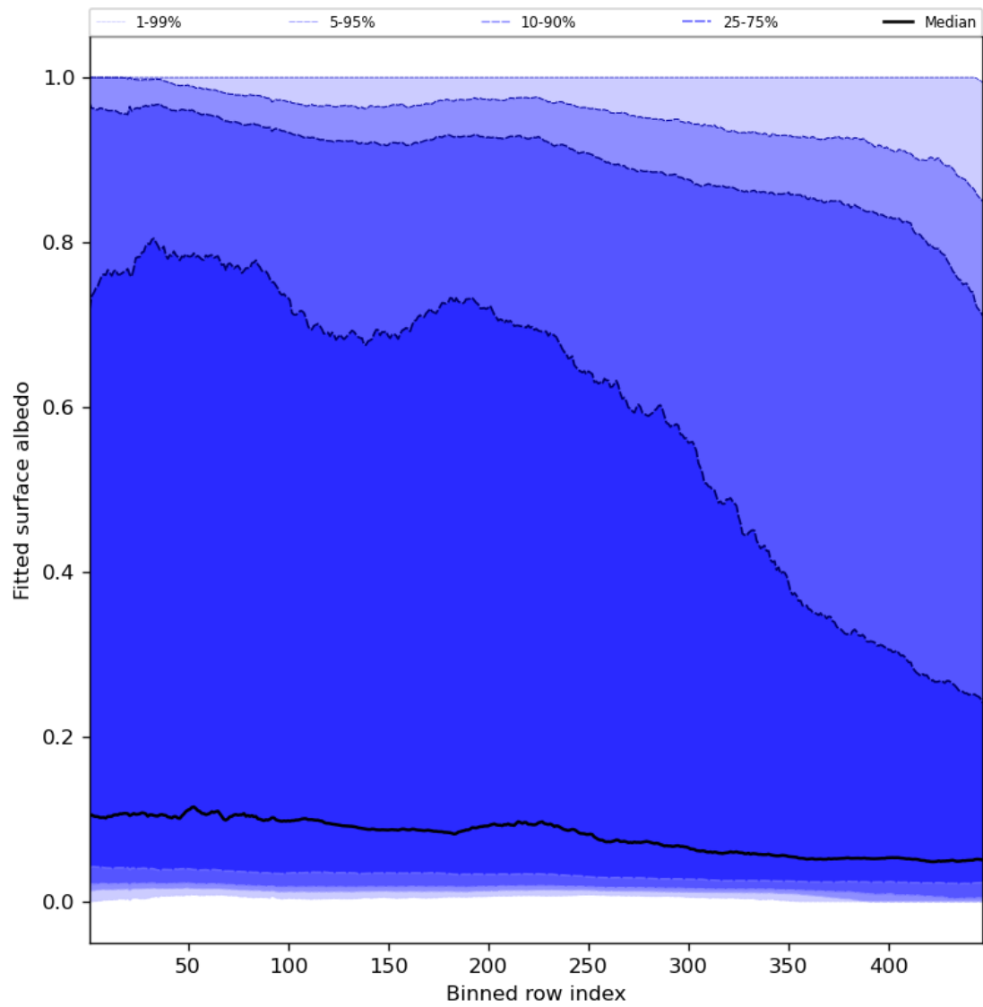
Figure 61: Along track statistics of “Fitted surface albedo” for 2023-11-09 to 2023-11-11
