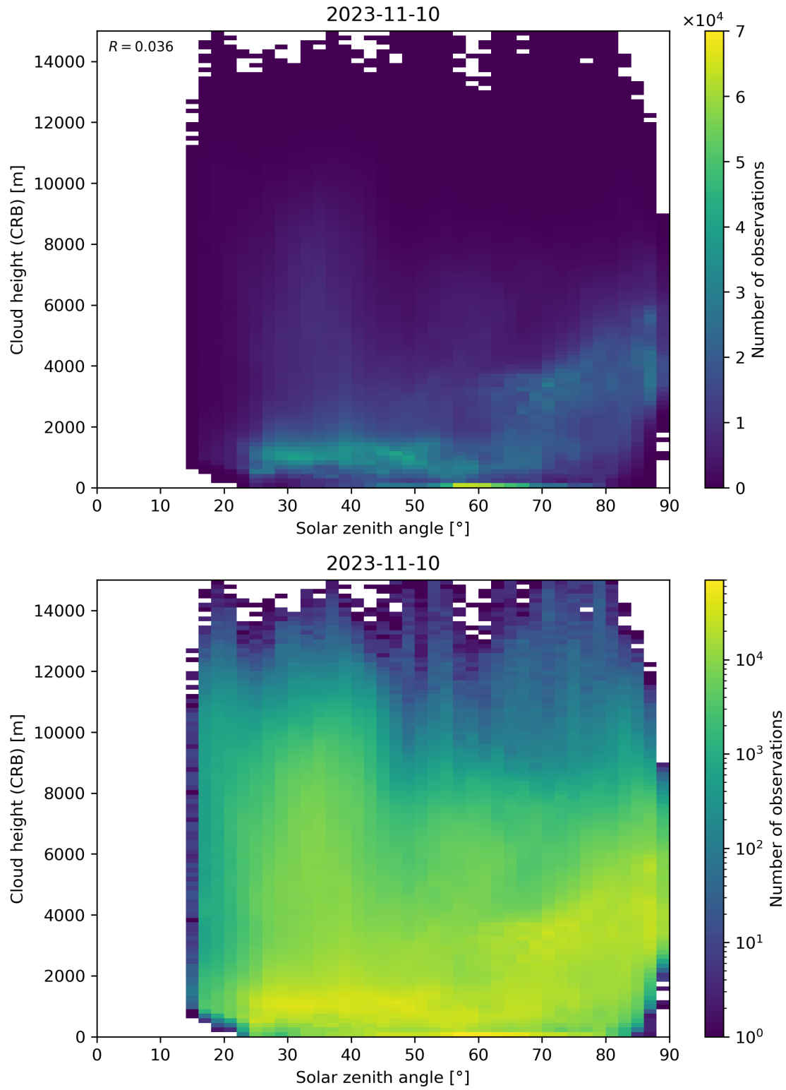
Figure 102: Scatter density plot of “Solar zenith angle” against “Cloud height (CRB)” for 2023-11-09 to 2023-11-11.
