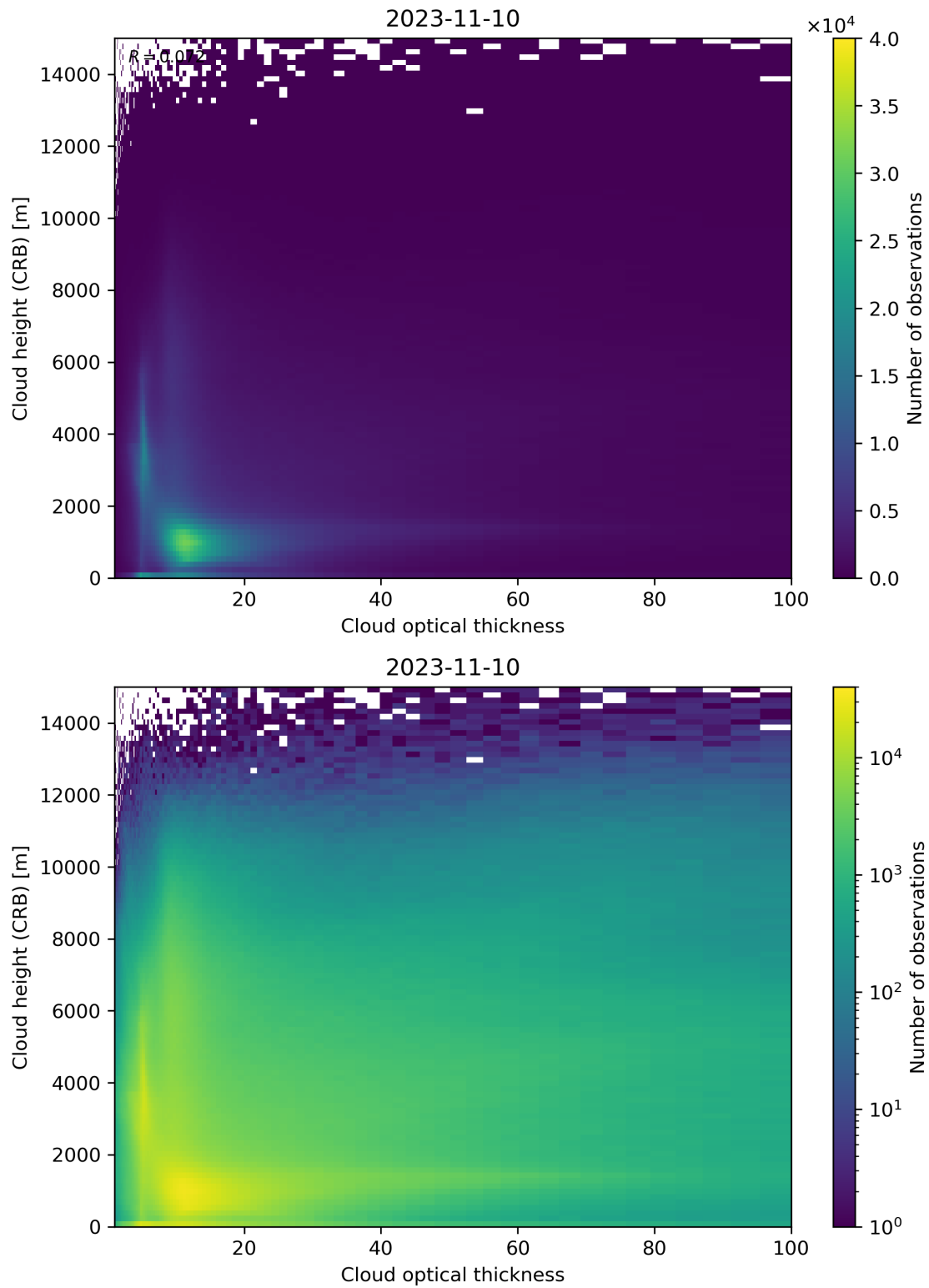
Figure 85: Scatter density plot of “Cloud optical thickness” against “Cloud height (CRB)” for 2023-11-09 to 2023-11-11.
