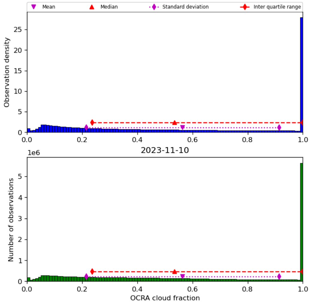
Figure 50: Histogram of “OCRA cloud fraction” for 2023-11-09 to 2023-11-11
