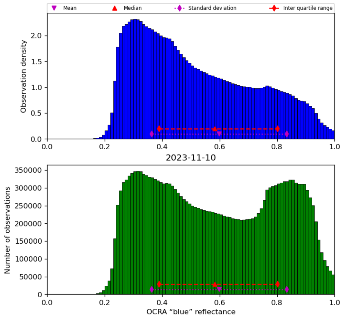
Figure 51: Histogram of “OCRA “blue” reflectance” for 2023-11-09 to 2023-11-11
