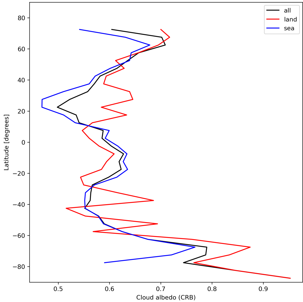
Figure 28: Zonal average of “Cloud albedo (CRB)” for 2023-11-09 to 2023-11-11.
