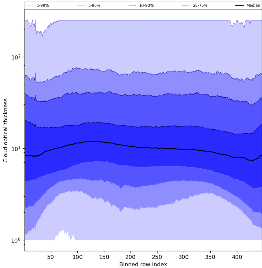
Figure 57: Along track statistics of "Cloud optical thickness" for 2023-11-09 to 2023-11-11
