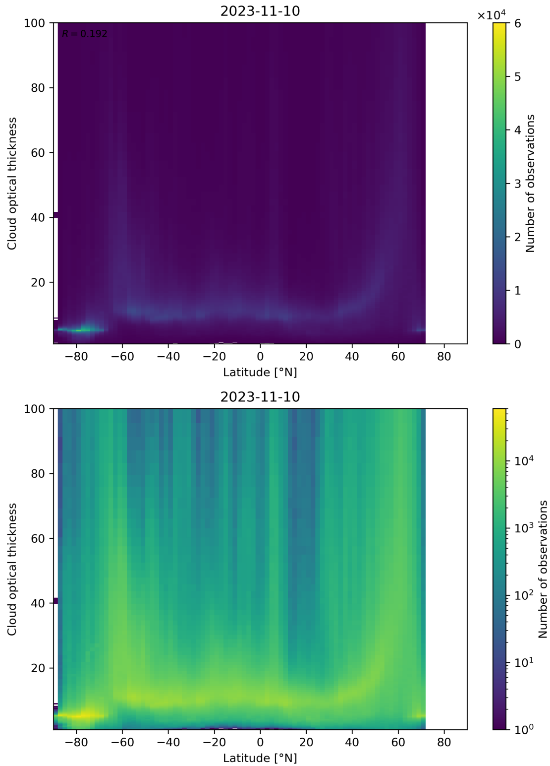
Figure 96: Scatter density plot of “Latitude” against “Cloud optical thickness” for 2023-11-09 to 2023-11-11.
