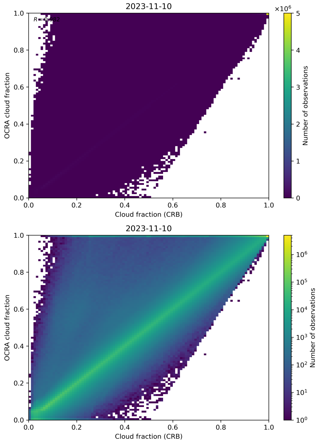
Figure 78: Scatter density plot of “Cloud fraction (CRB)” against “OCRA cloud fraction” for 2023-11-09 to 2023-11-11.
