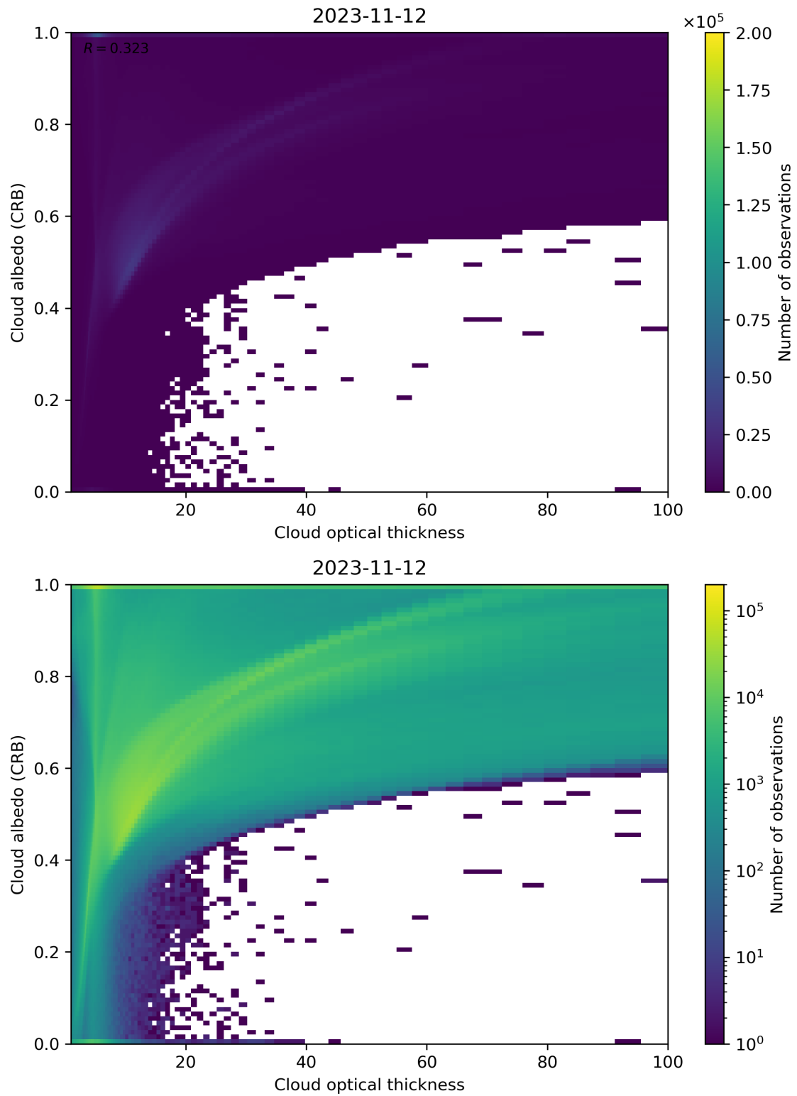
Figure 82: Scatter density plot of “Cloud optical thickness” against “Cloud albedo (CRB)” for 2023-11-12 to 2023-11-13.
