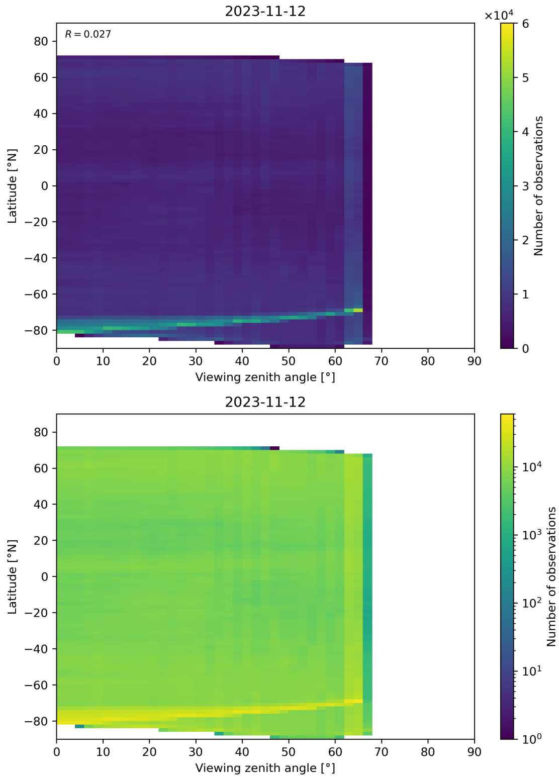
Figure 113: Scatter density plot of “Viewing zenith angle” against “Latitude” for 2023-11-12 to 2023-11-13.
