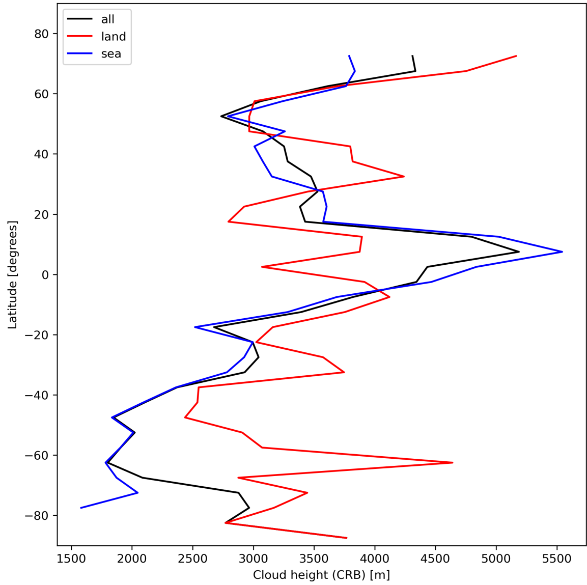
Figure 27: Zonal average of “Cloud height (CRB)” for 2023-11-12 to 2023-11-13.
