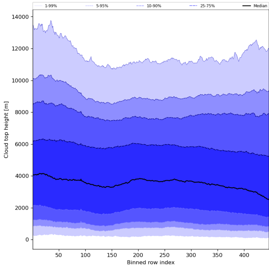
Figure 56: Along track statistics of “Cloud top height” for 2023-11-12 to 2023-11-13
