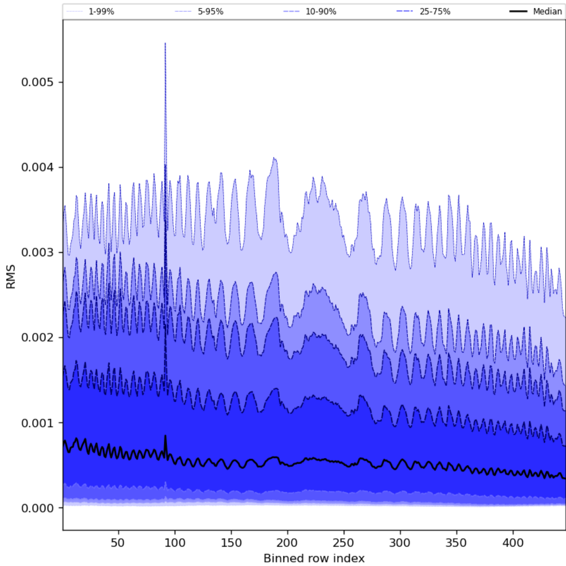
Figure 63: Along track statistics of “RMS” for 2023-11-12 to 2023-11-13
