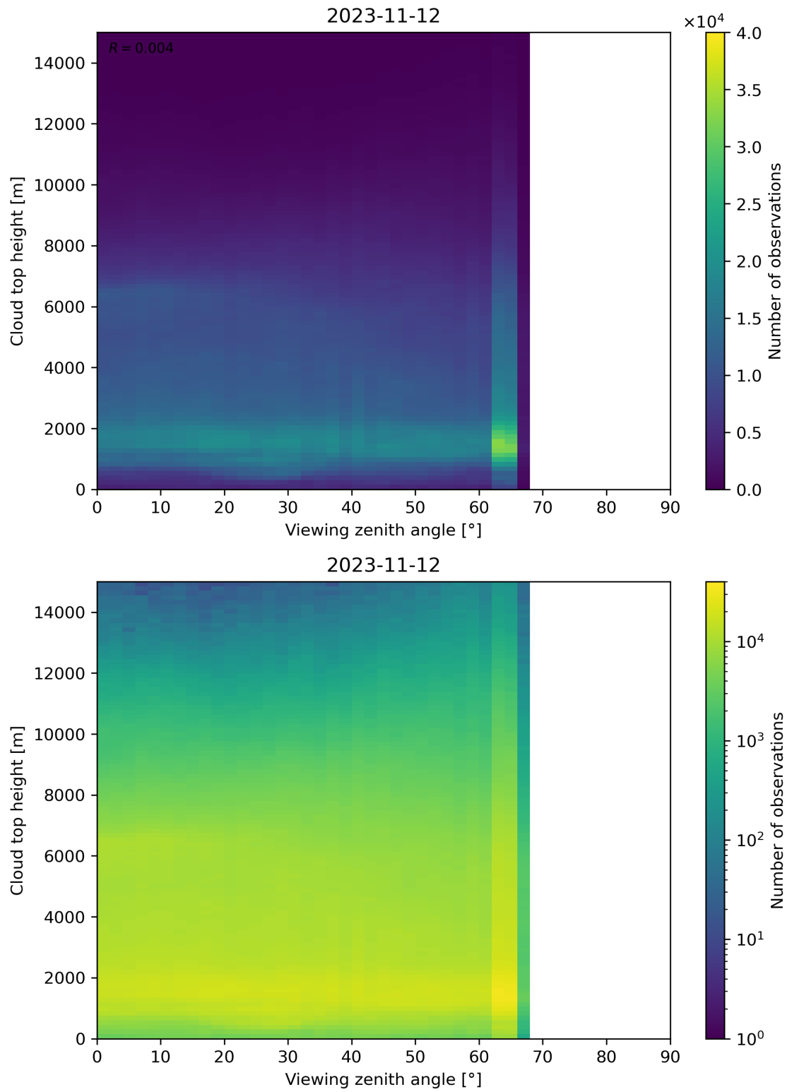
Figure 112: Scatter density plot of “Viewing zenith angle” against “Cloud top height” for 2023-11-12 to 2023-11-13.
