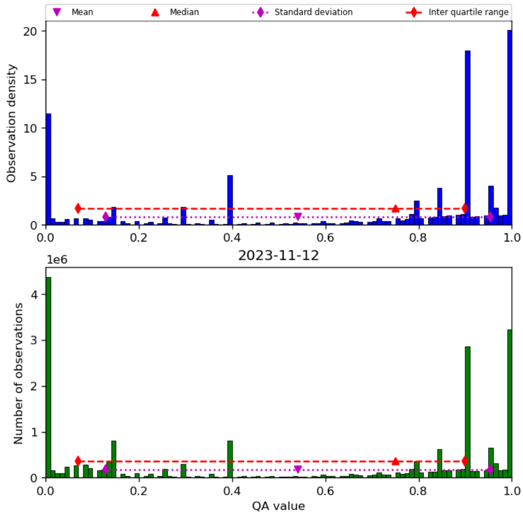
Figure 38: Histogram of “QA value” for 2023-11-12 to 2023-11-13
