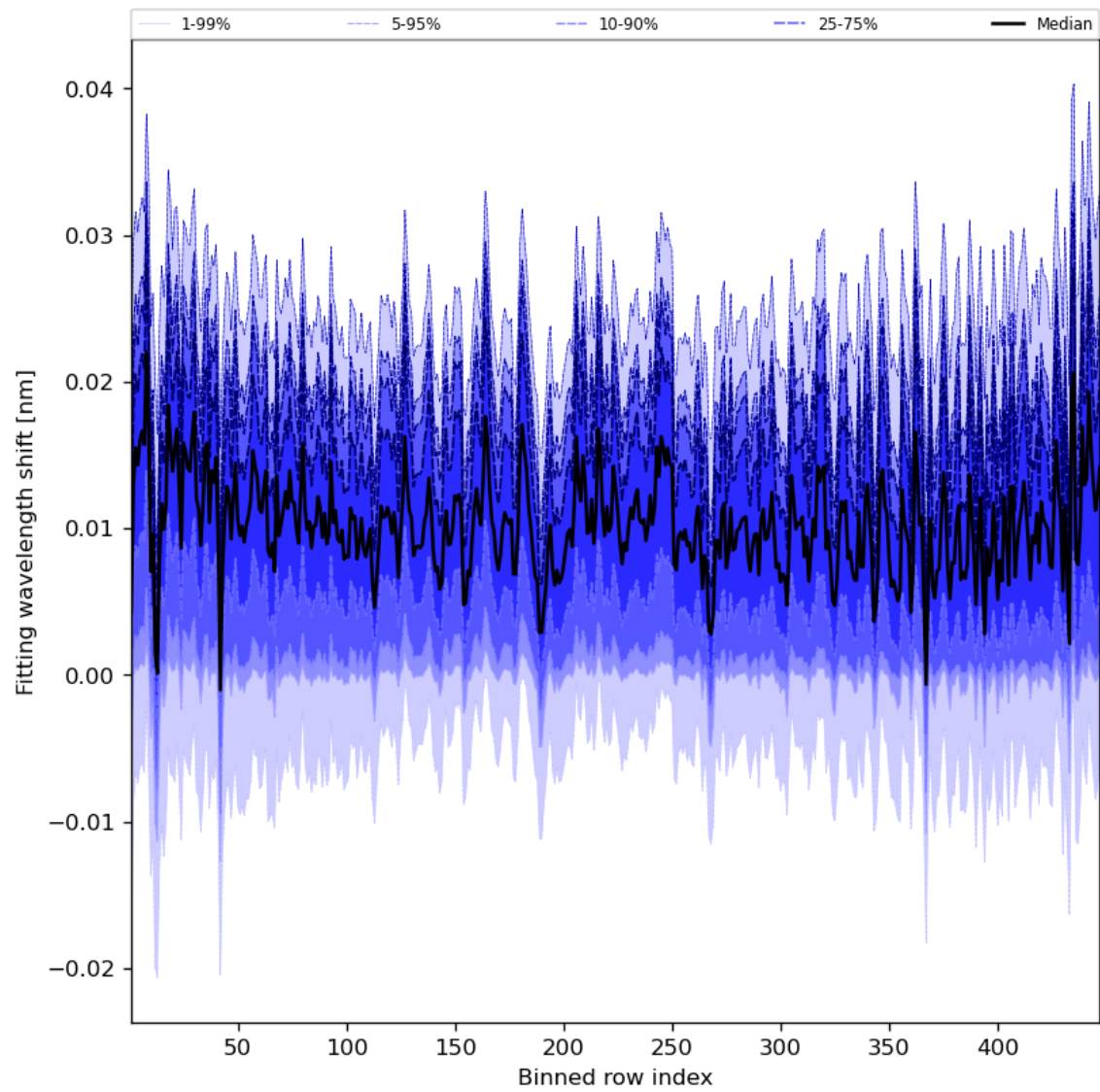
Figure 65: Along track statistics of “Fitting wavelength shift” for 2023-11-12 to 2023-11-13
