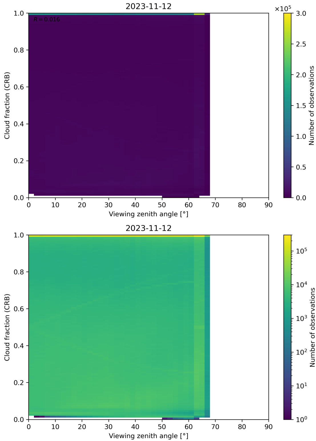
Figure 109: Scatter density plot of “Viewing zenith angle” against “Cloud fraction (CRB)” for 2023-11-12 to 2023-11-13.
