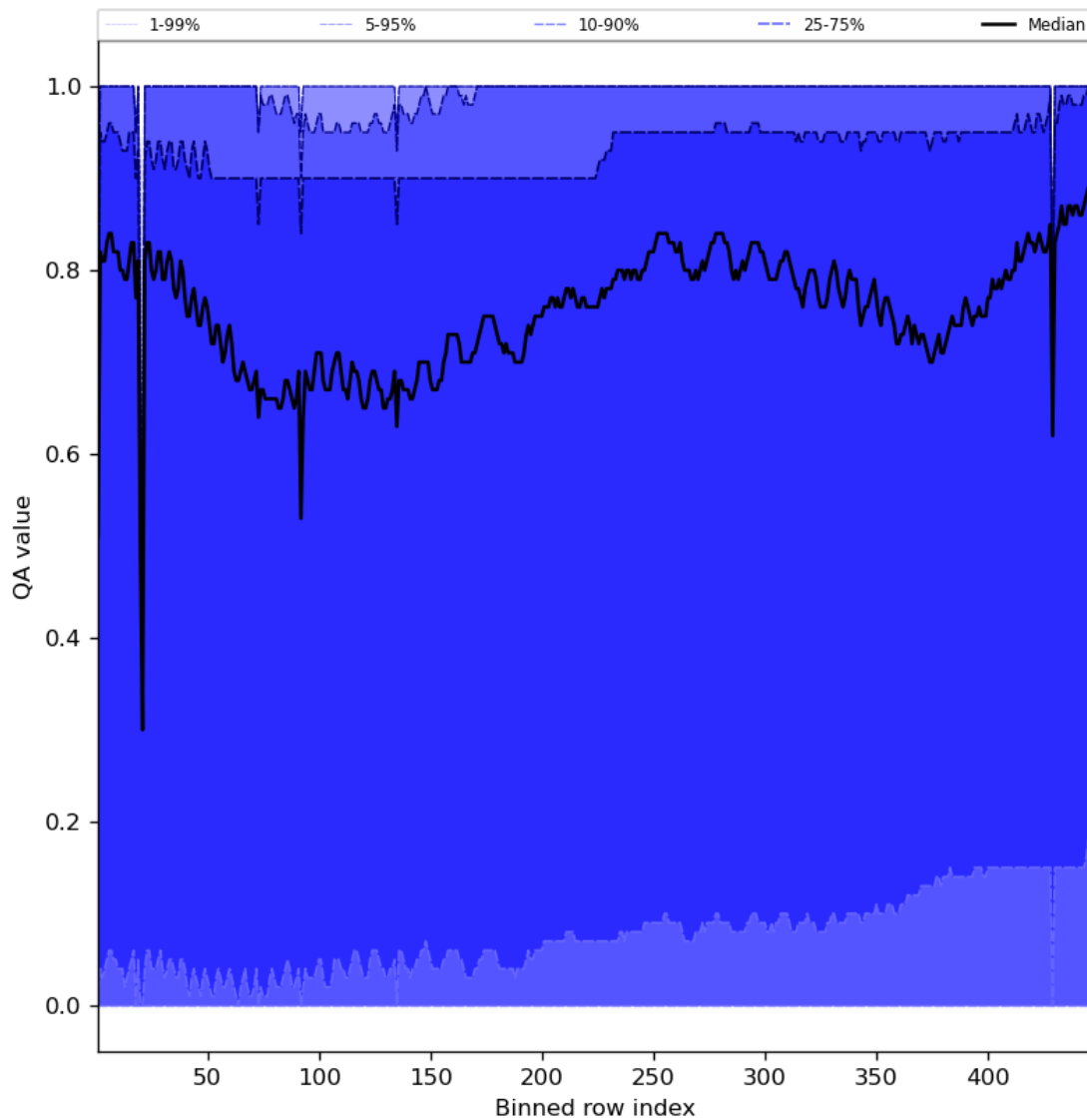
Figure 54: Along track statistics of “QA value” for 2023-11-12 to 2023-11-13
