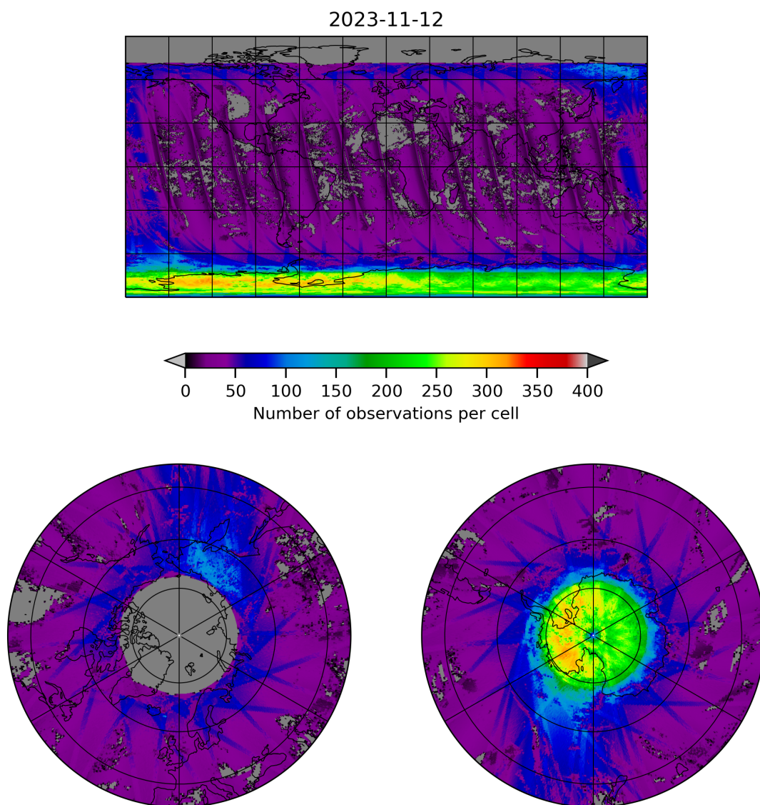
Figure 21: Map of the number of observations for 2023-11-12 to 2023-11-13
