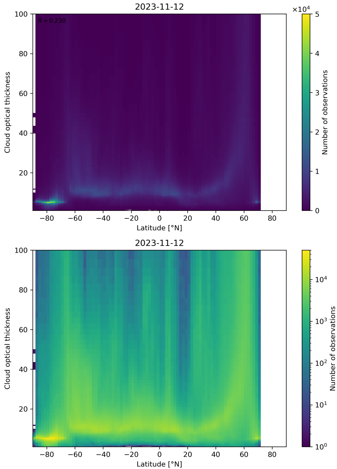
Figure 96: Scatter density plot of “Latitude” against “Cloud optical thickness” for 2023-11-12 to 2023-11-13.
