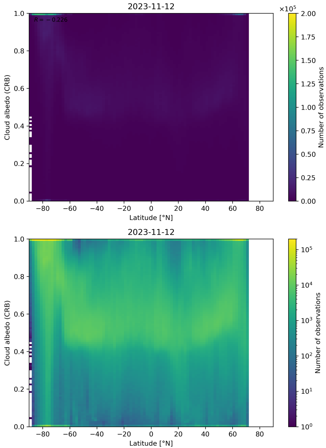
Figure 91: Scatter density plot of “Latitude” against “Cloud albedo (CRB)” for 2023-11-12 to 2023-11-13.
