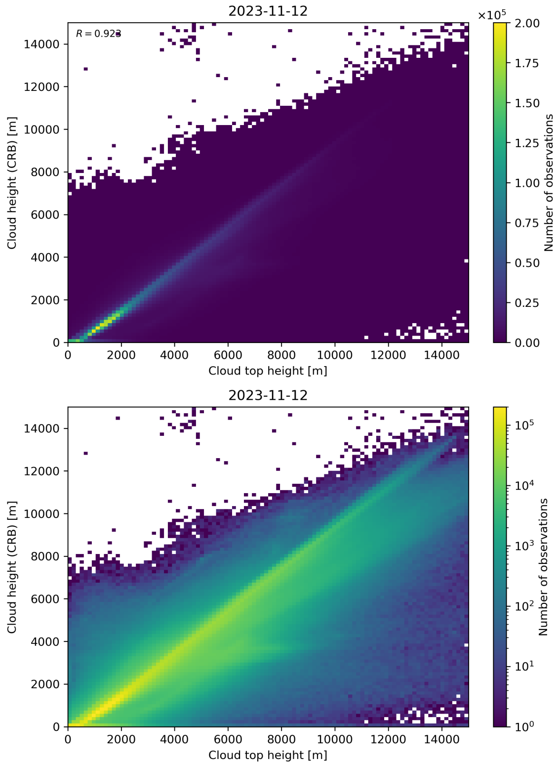
Figure 89: Scatter density plot of “Cloud top height” against “Cloud height (CRB)” for 2023-11-12 to 2023-11-13.
