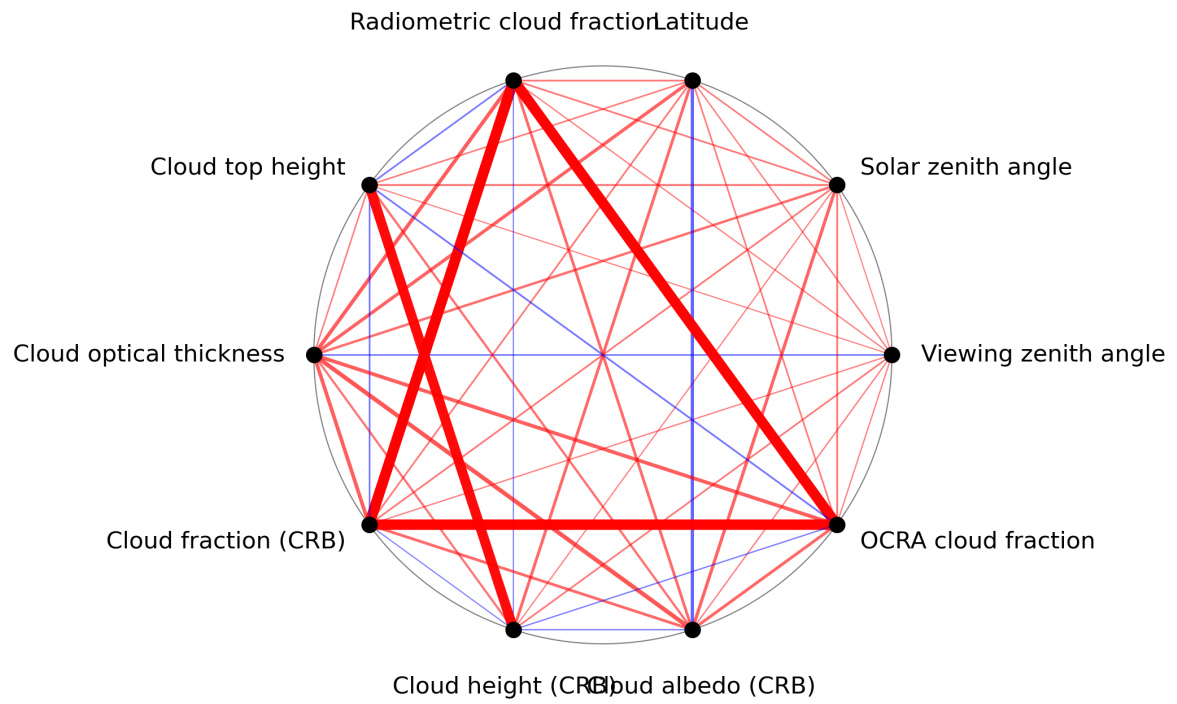
Figure 1: Map of correlation graph for 2023-11-12 to 2023-11-13.
