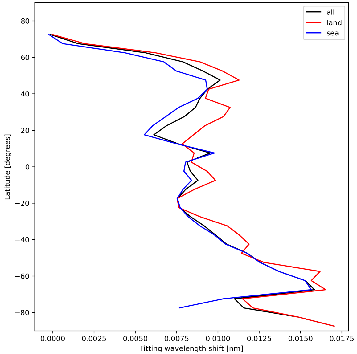
Figure 33: Zonal average of “Fitting wavelength shift” for 2023-11-12 to 2023-11-13.
