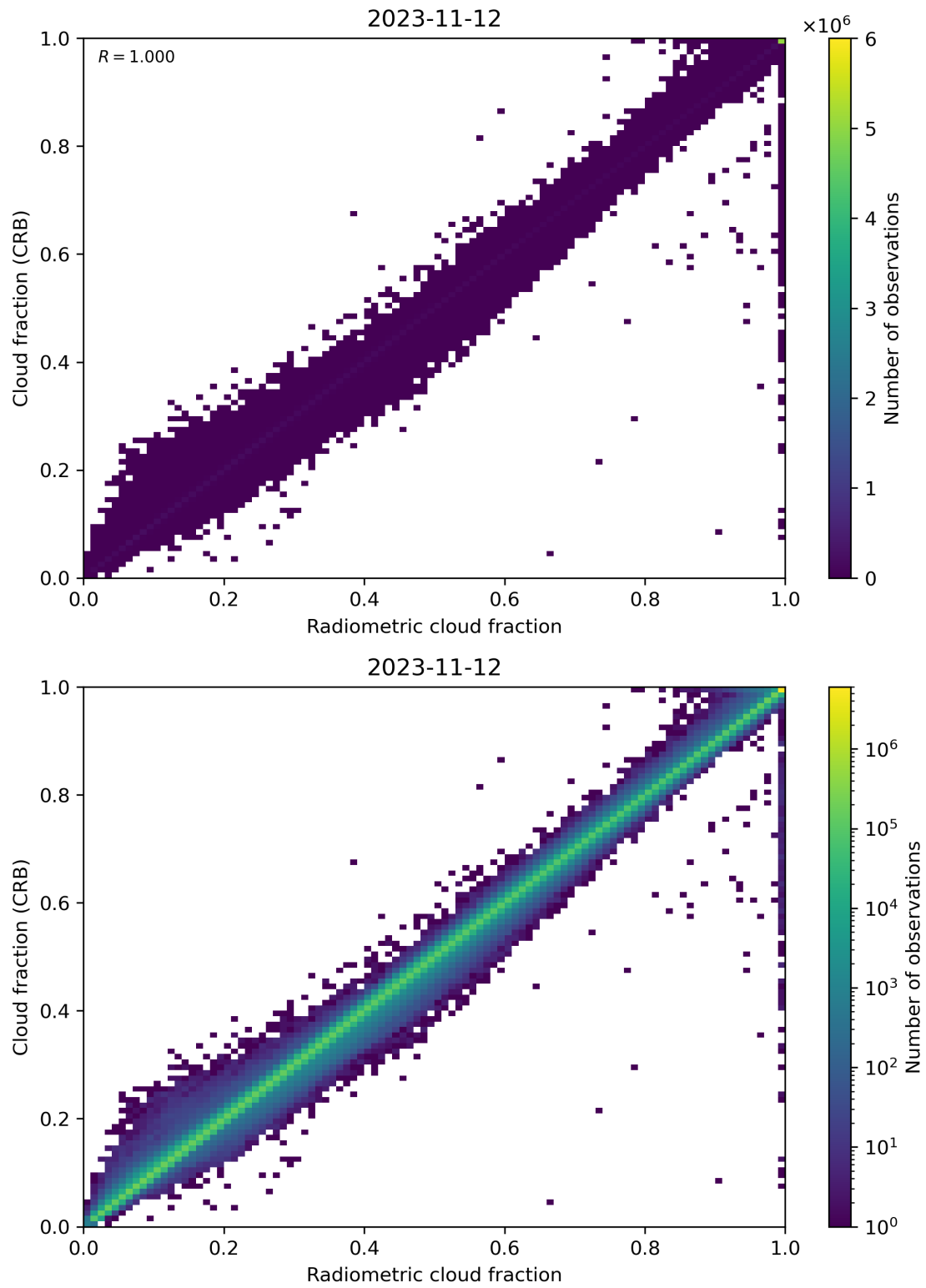
Figure 73: Scatter density plot of “Radiometric cloud fraction” against “Cloud fraction (CRB)” for 2023-11-12 to 2023-11-13.
