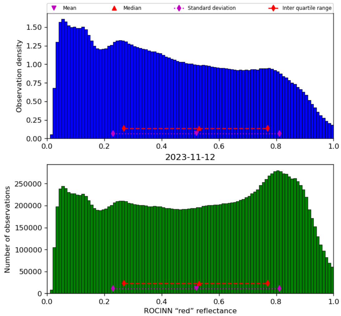
Figure 53: Histogram of “ROCINN “red” reflectance” for 2023-11-12 to 2023-11-13
