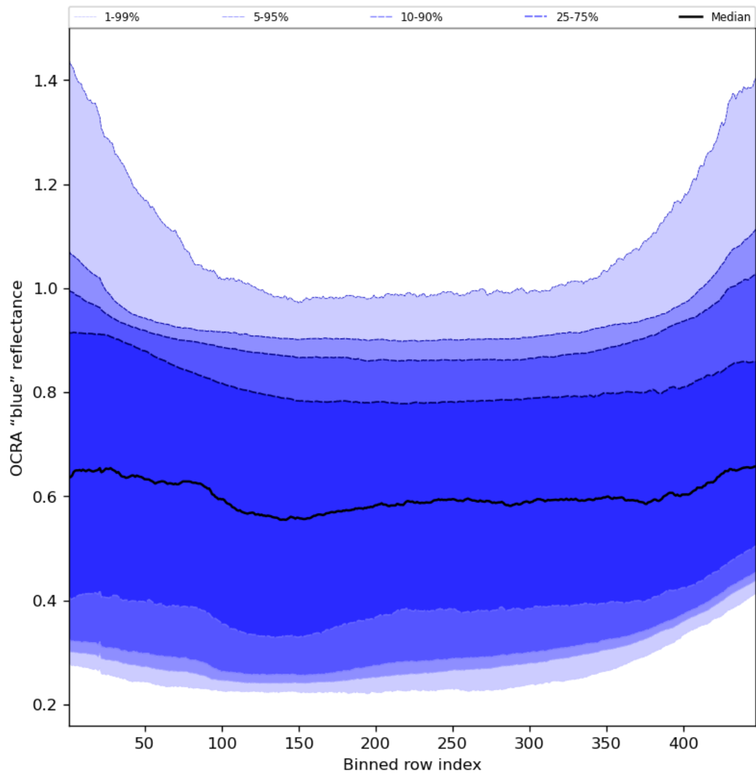
Figure 67: Along track statistics of “OCRA “blue” reflectance” for 2023-11-12 to 2023-11-13
