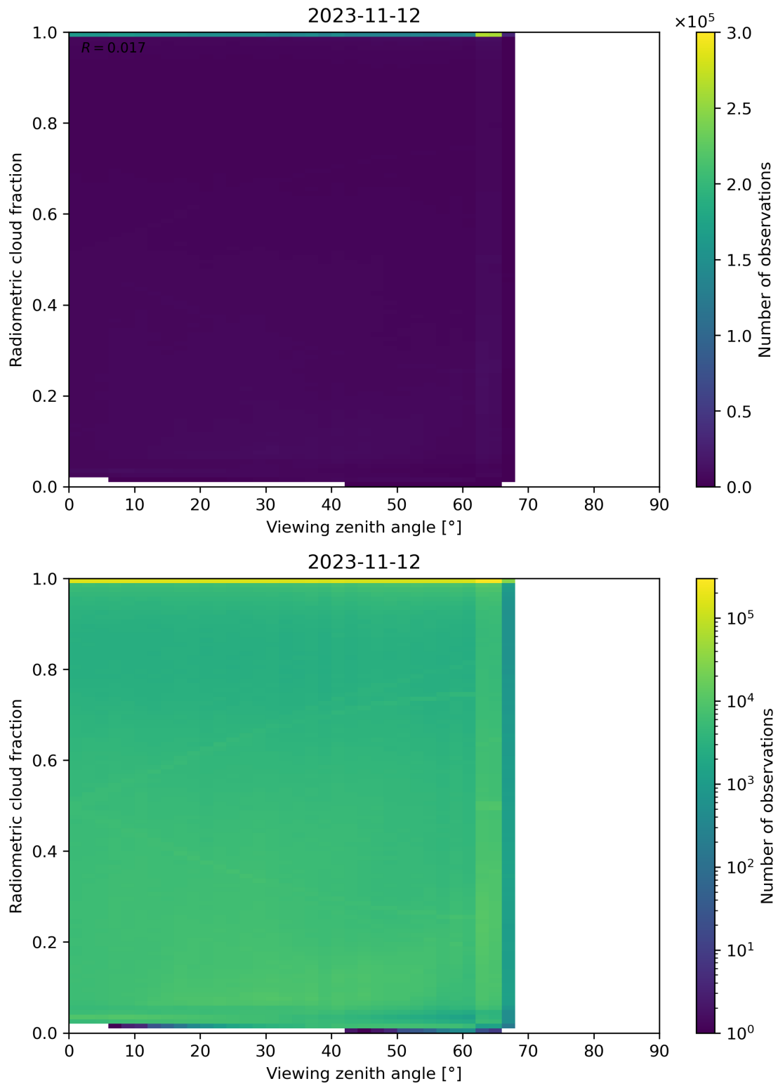
Figure 107: Scatter density plot of “Viewing zenith angle” against “Radiometric cloud fraction” for 2023-11-12 to 2023-11-13.
