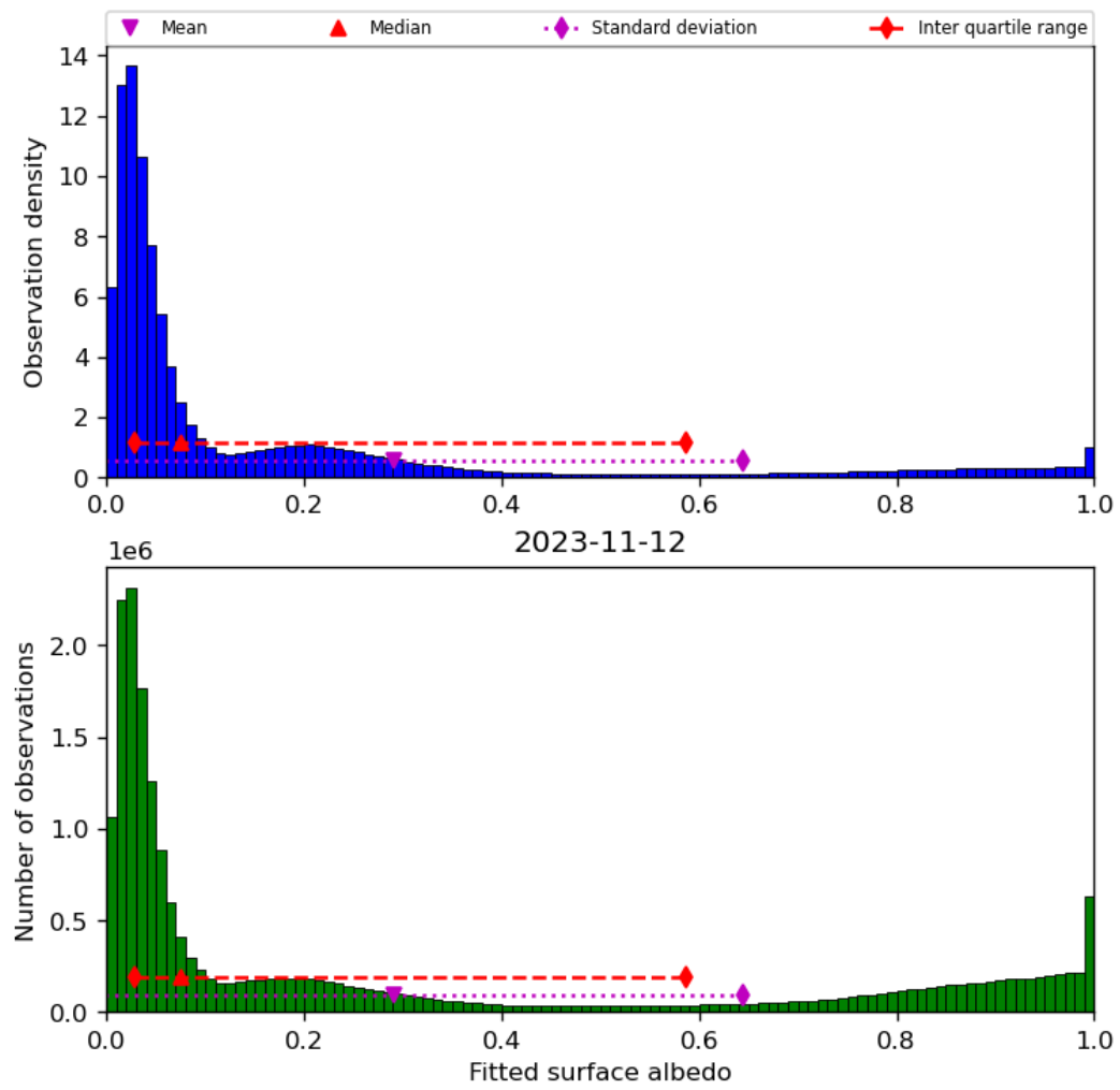
Figure 45: Histogram of “Fitted surface albedo” for 2023-11-12 to 2023-11-13
