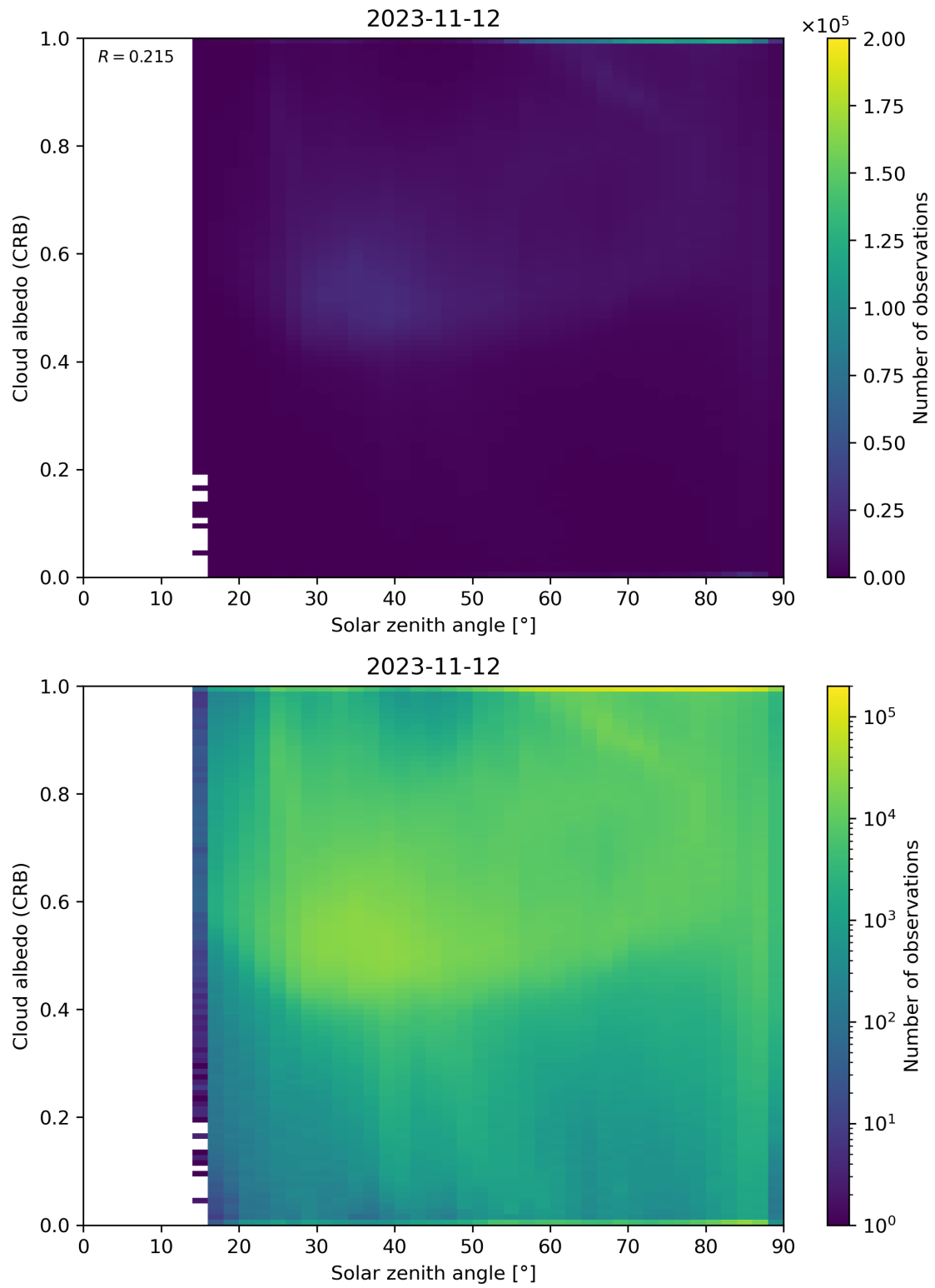
Figure 98: Scatter density plot of “Solar zenith angle” against “Cloud albedo (CRB)” for 2023-11-12 to 2023-11-13.
