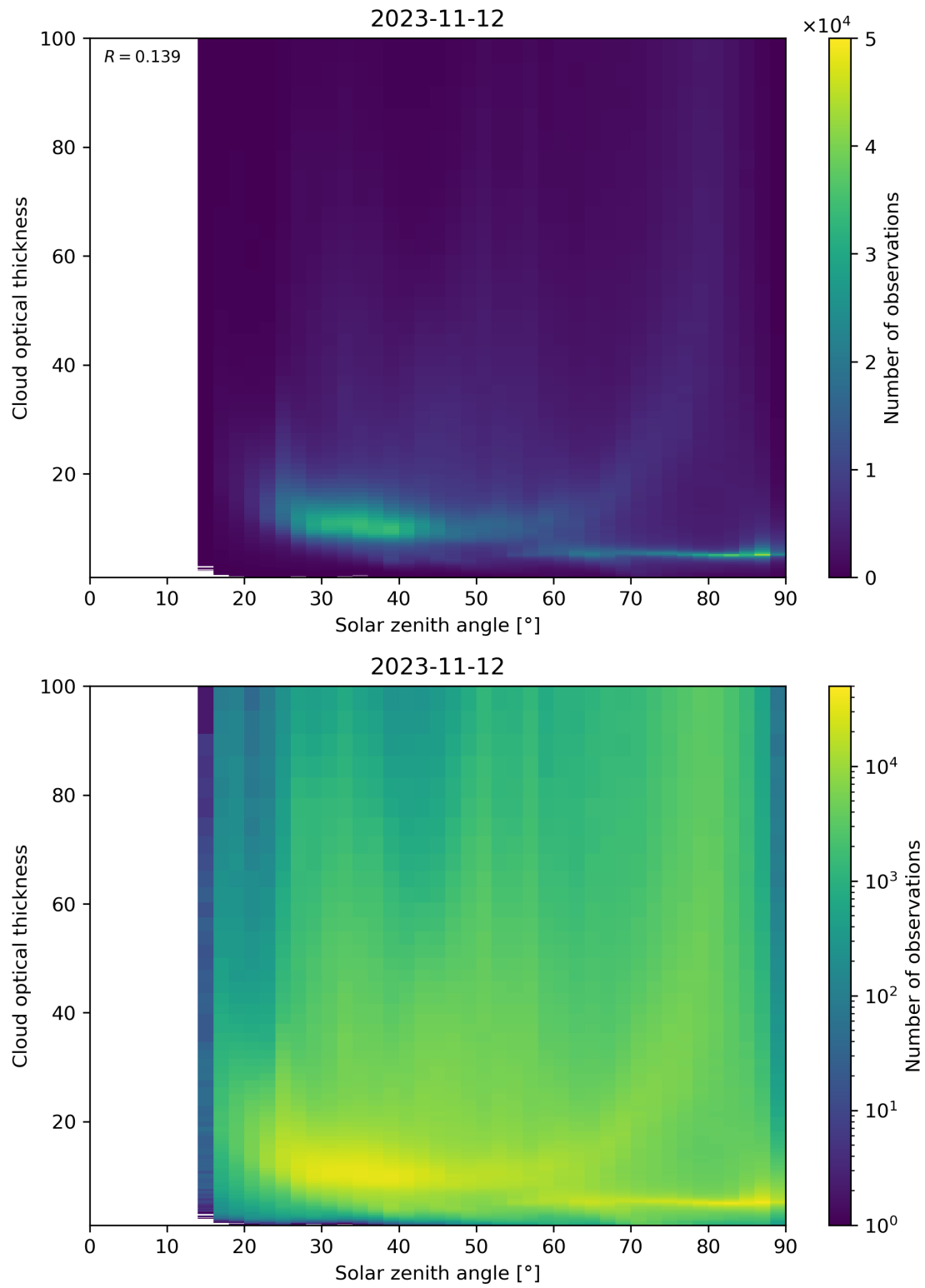
Figure 103: Scatter density plot of “Solar zenith angle” against “Cloud optical thickness” for 2023-11-12 to 2023-11-13.
