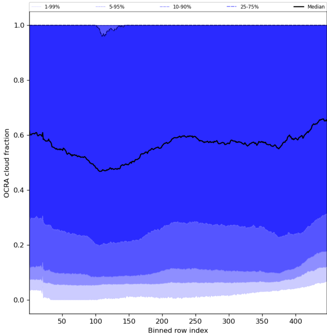
Figure 66: Along track statistics of “OCRA cloud fraction” for 2023-11-12 to 2023-11-13
