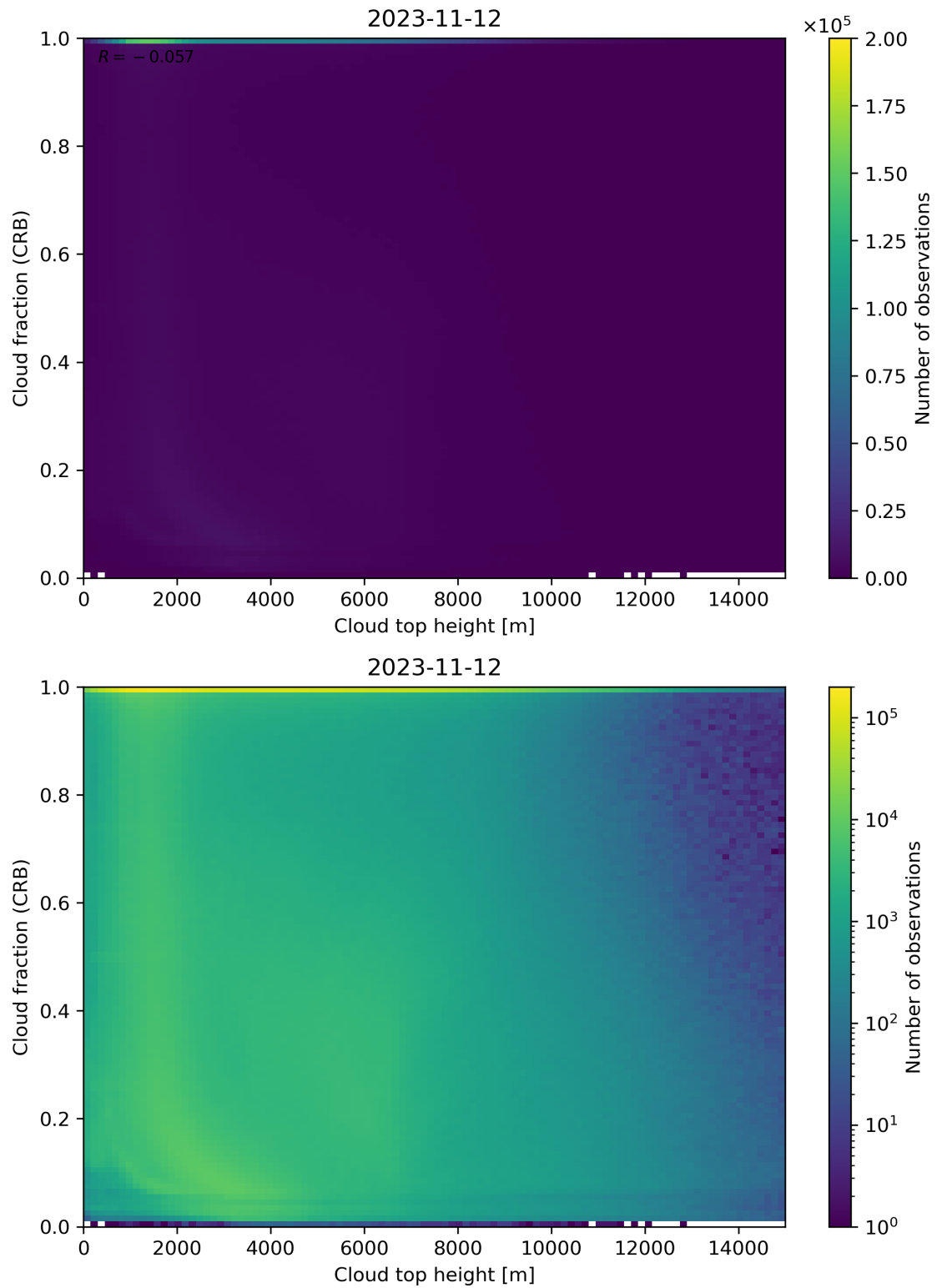
Figure 88: Scatter density plot of “Cloud top height” against “Cloud fraction (CRB)” for 2023-11-12 to 2023-11-13.
