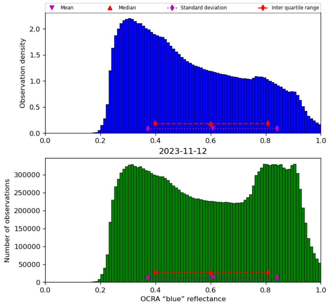
Figure 51: Histogram of "OCRA "blue" reflectance" for 2023-11-12 to 2023-11-13
