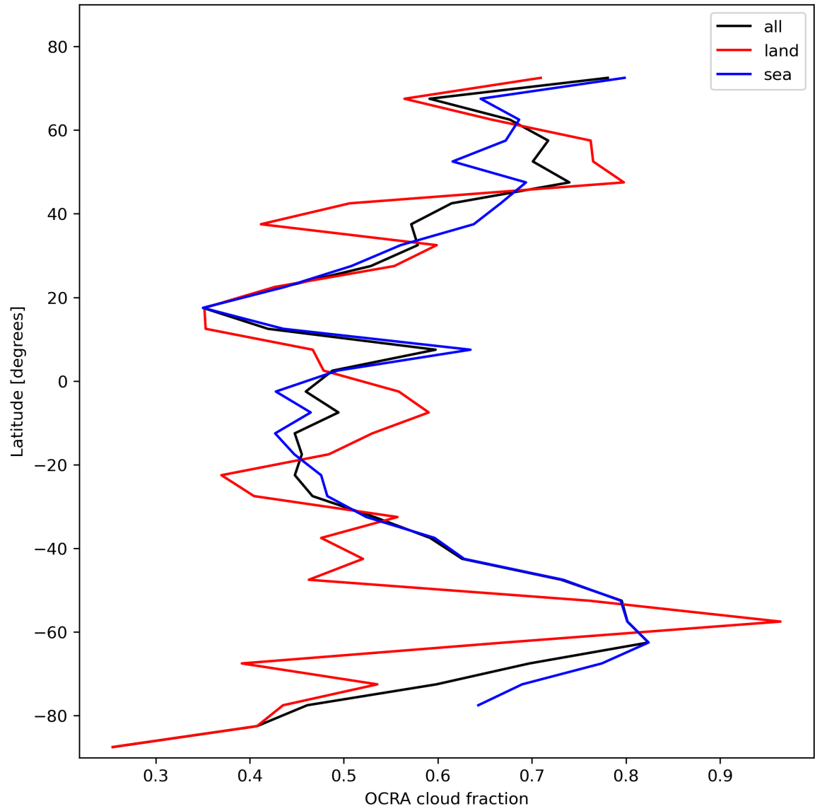
Figure 34: Zonal average of “OCRA cloud fraction” for 2023-11-12 to 2023-11-13.
