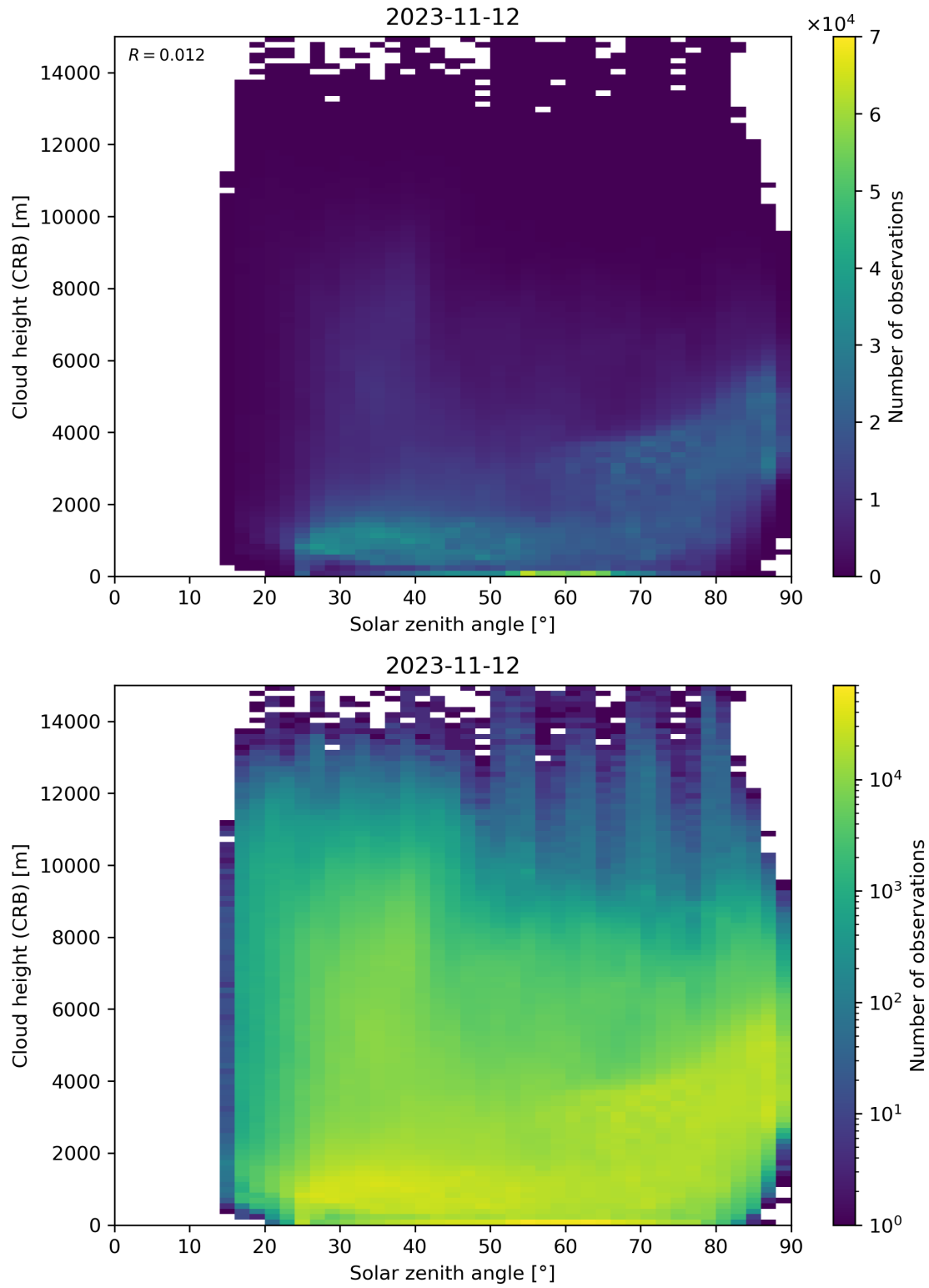
Figure 102: Scatter density plot of “Solar zenith angle” against “Cloud height (CRB)” for 2023-11-12 to 2023-11-13.
