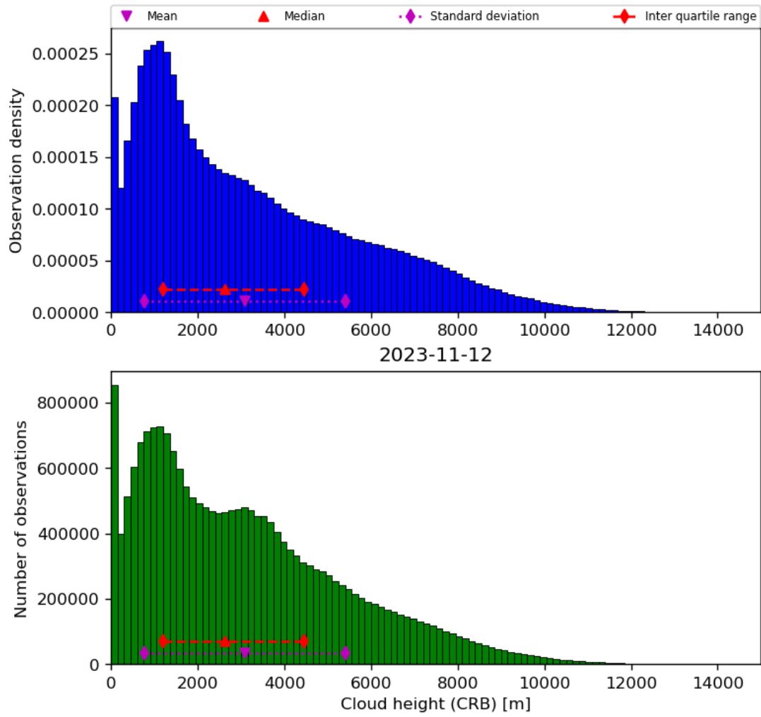
Figure 43: Histogram of “Cloud height (CRB)” for 2023-11-12 to 2023-11-13
