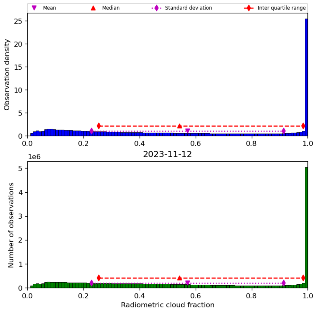
Figure 39: Histogram of “Radiometric cloud fraction” for 2023-11-12 to 2023-11-13
