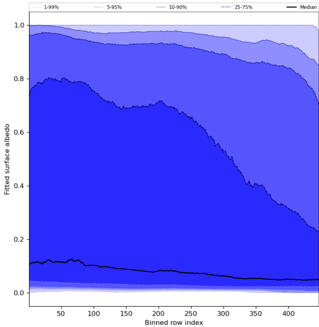
Figure 61: Along track statistics of “Fitted surface albedo” for 2023-11-12 to 2023-11-13
