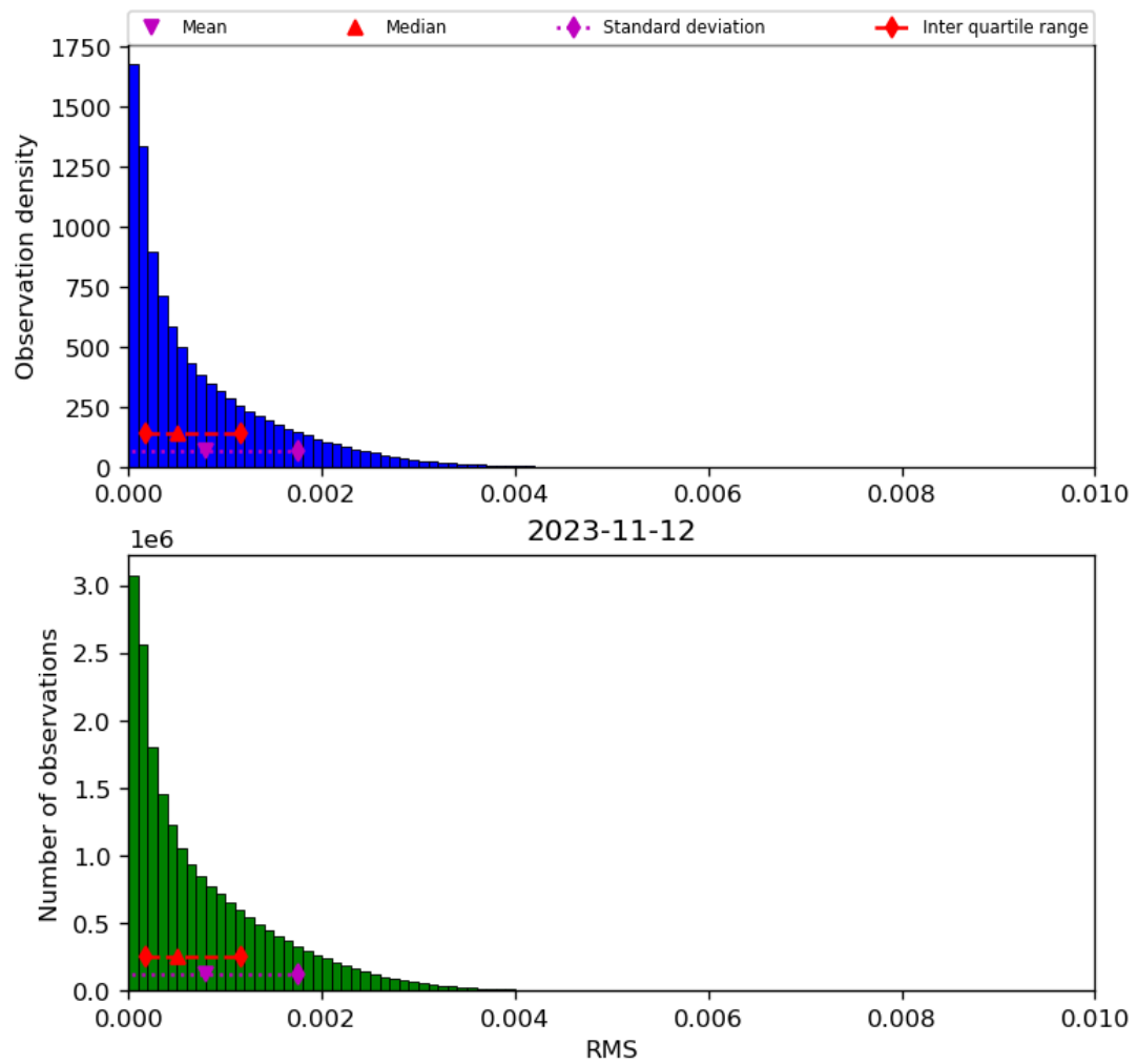
Figure 47: Histogram of “RMS” for 2023-11-12 to 2023-11-13
