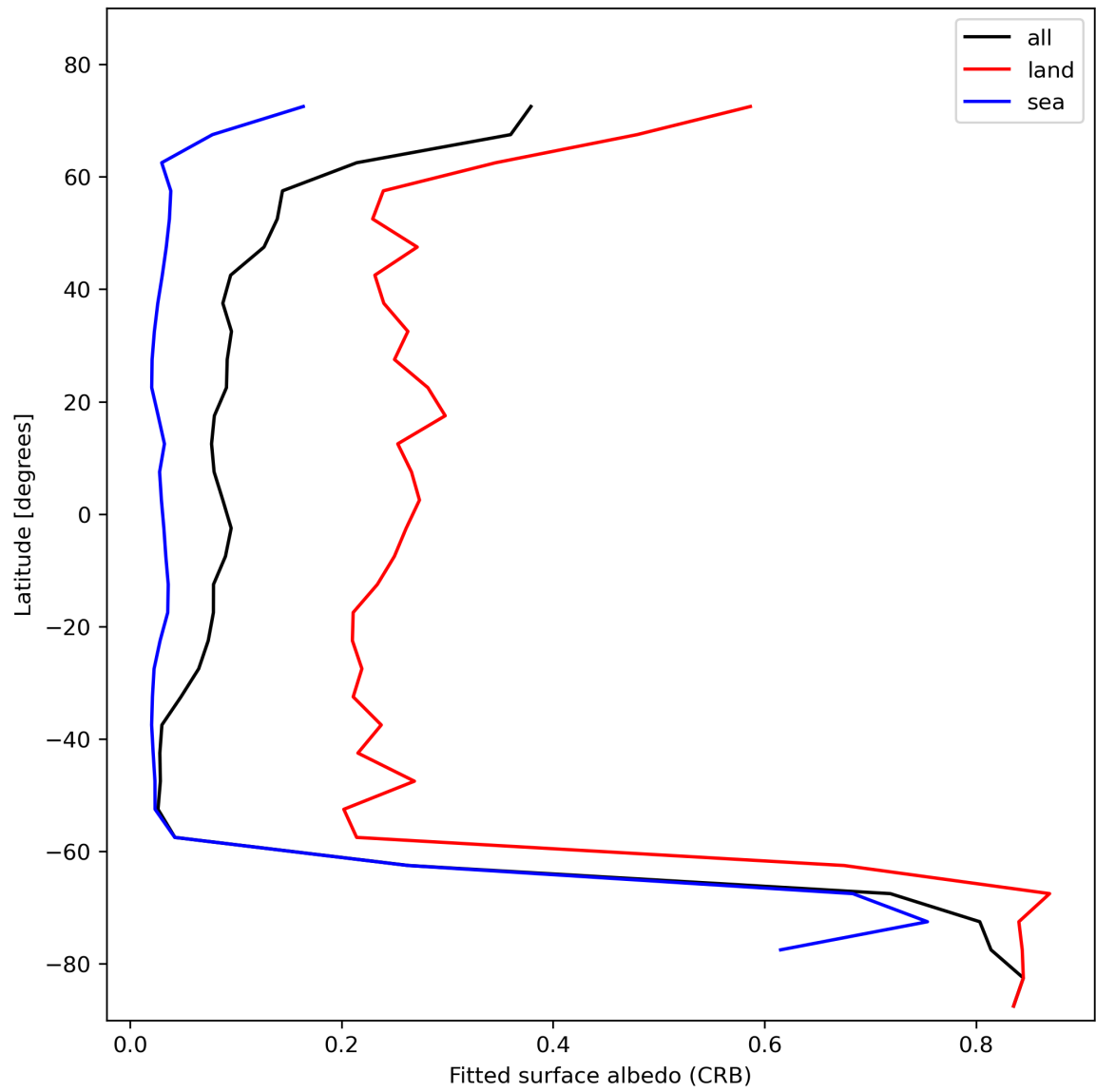
Figure 30: Zonal average of “Fitted surface albedo (CRB)” for 2023-11-12 to 2023-11-13.
