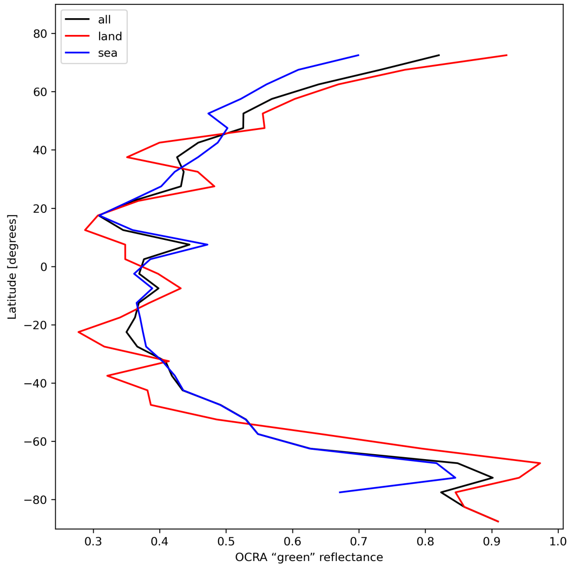
Figure 36: Zonal average of “OCRA “green” reflectance” for 2023-11-12 to 2023-11-13.
