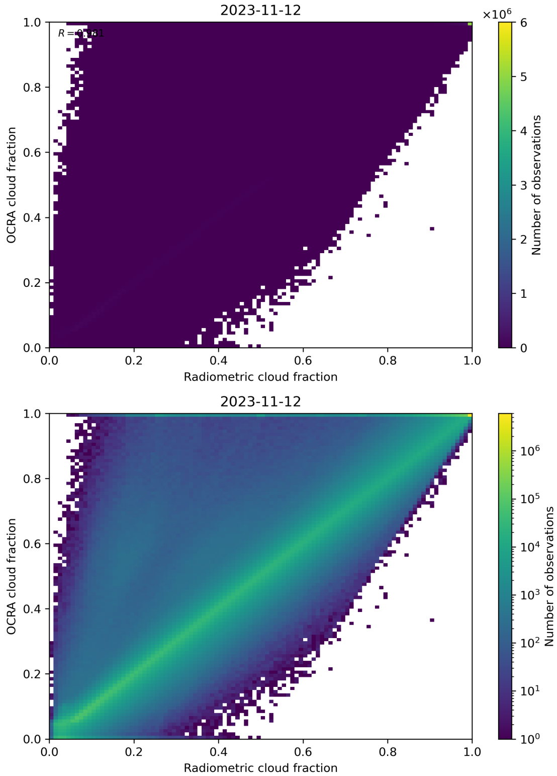
Figure 72: Scatter density plot of “Radiometric cloud fraction” against “OCRA cloud fraction” for 2023-11-12 to 2023-11-13.
