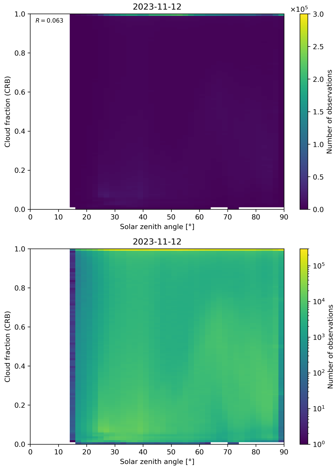
Figure 101: Scatter density plot of “Solar zenith angle” against “Cloud fraction (CRB)” for 2023-11-12 to 2023-11-13.
