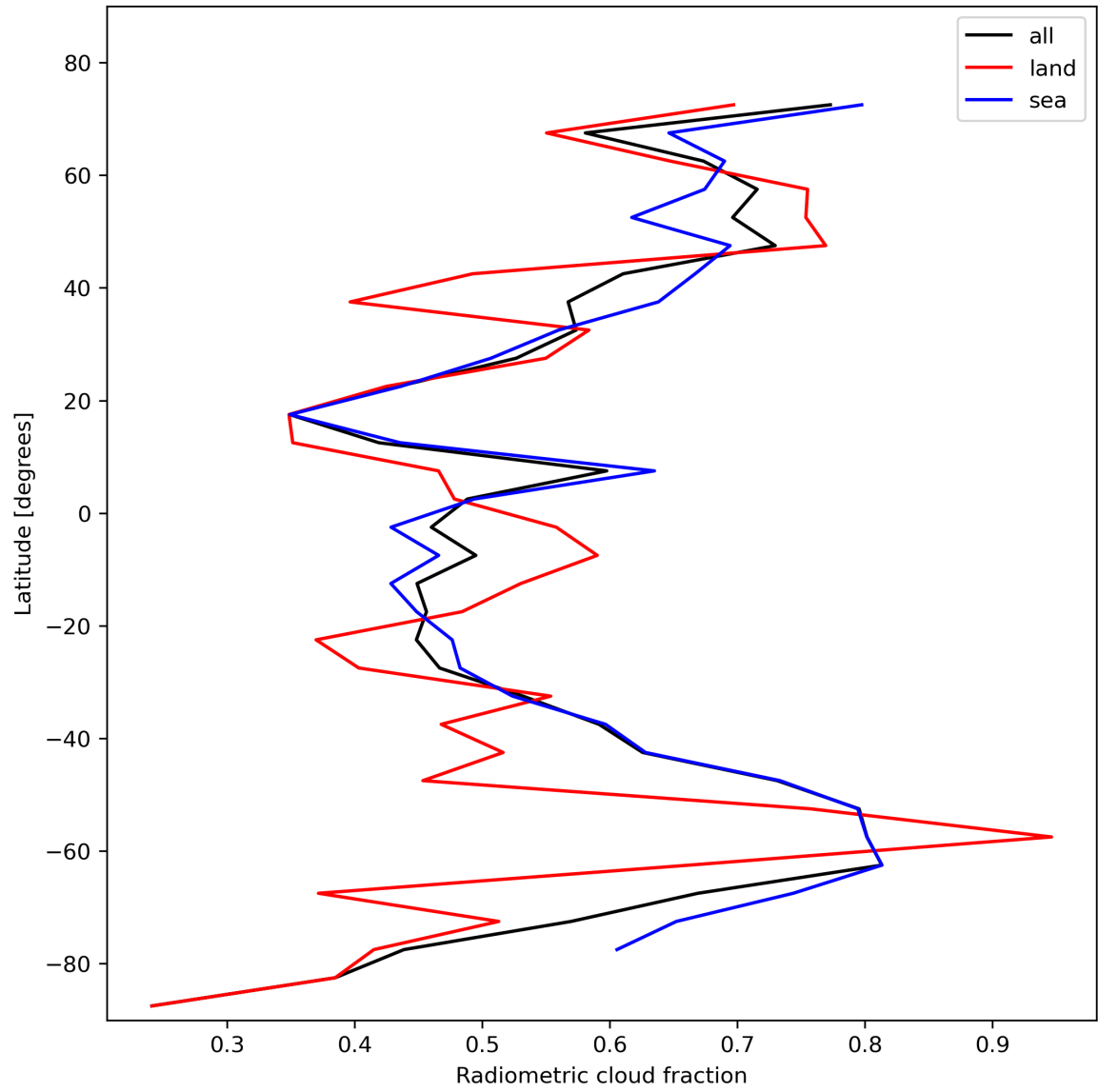
Figure 23: Zonal average of “Radiometric cloud fraction” for 2023-11-12 to 2023-11-13.
