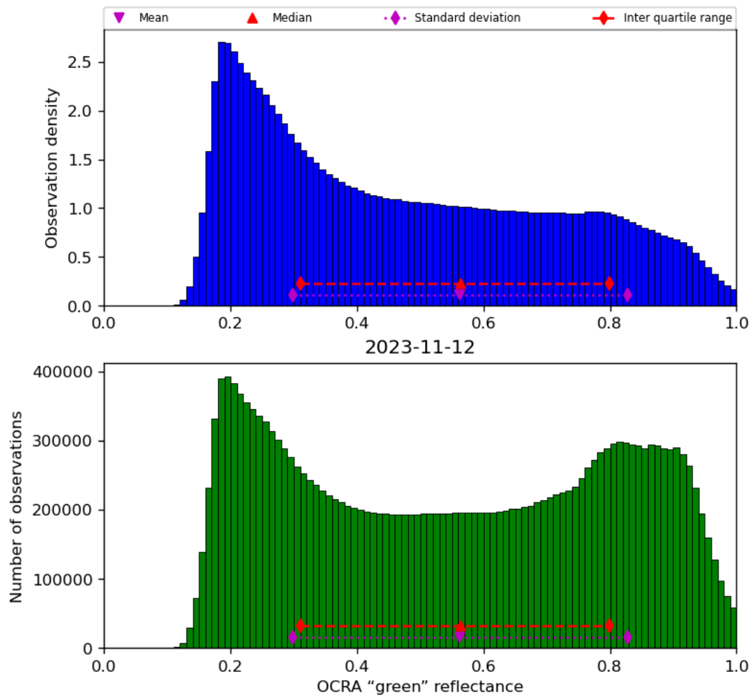
Figure 52: Histogram of “OCRA “green” reflectance” for 2023-11-12 to 2023-11-13
