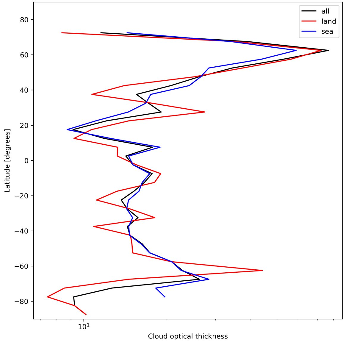
Figure 25: Zonal average of “Cloud optical thickness” for 2023-11-12 to 2023-11-13.
