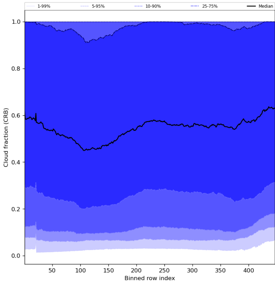
Figure 58: Along track statistics of “Cloud fraction (CRB)” for 2023-11-12 to 2023-11-13
