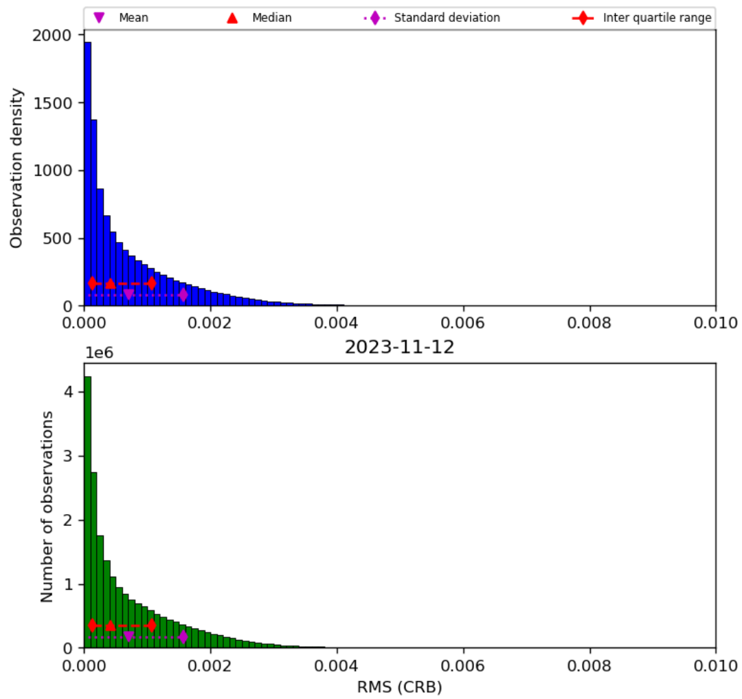
Figure 48: Histogram of “RMS (CRB)” for 2023-11-12 to 2023-11-13
