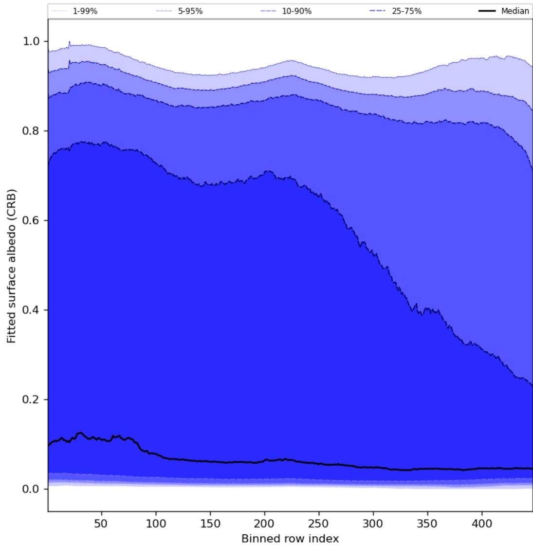
Figure 62: Along track statistics of “Fitted surface albedo (CRB)” for 2023-11-12 to 2023-11-13
