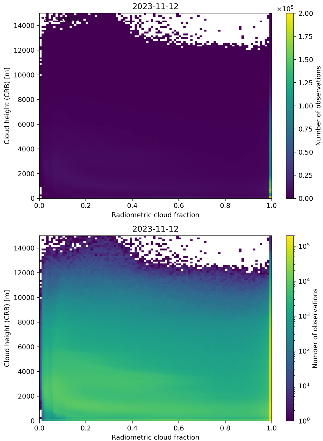
Figure 74: Scatter density plot of “Radiometric cloud fraction” against “Cloud height (CRB)” for 2023-11-12 to 2023-11-13.
