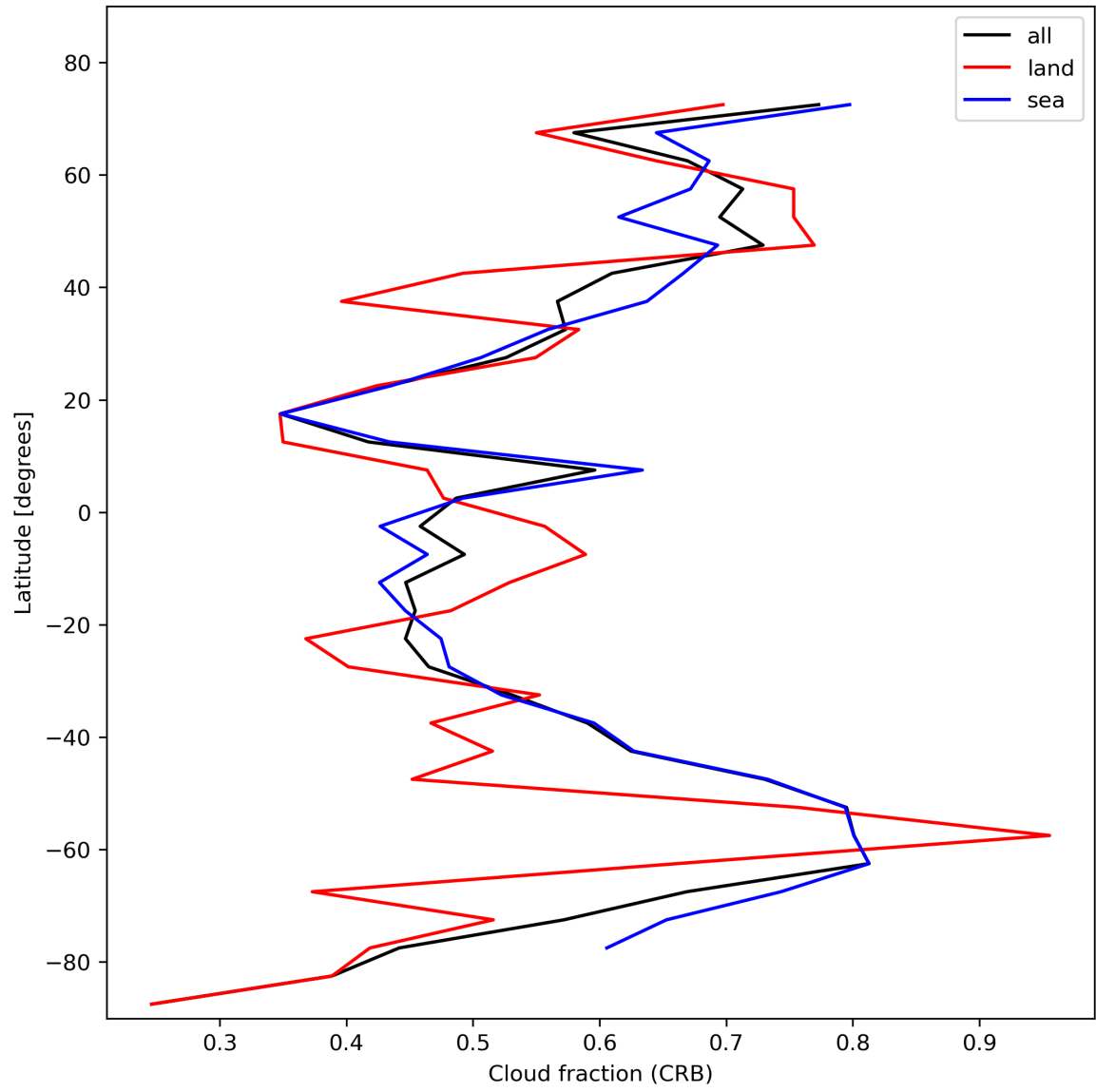
Figure 26: Zonal average of “Cloud fraction (CRB)” for 2023-11-12 to 2023-11-13.
