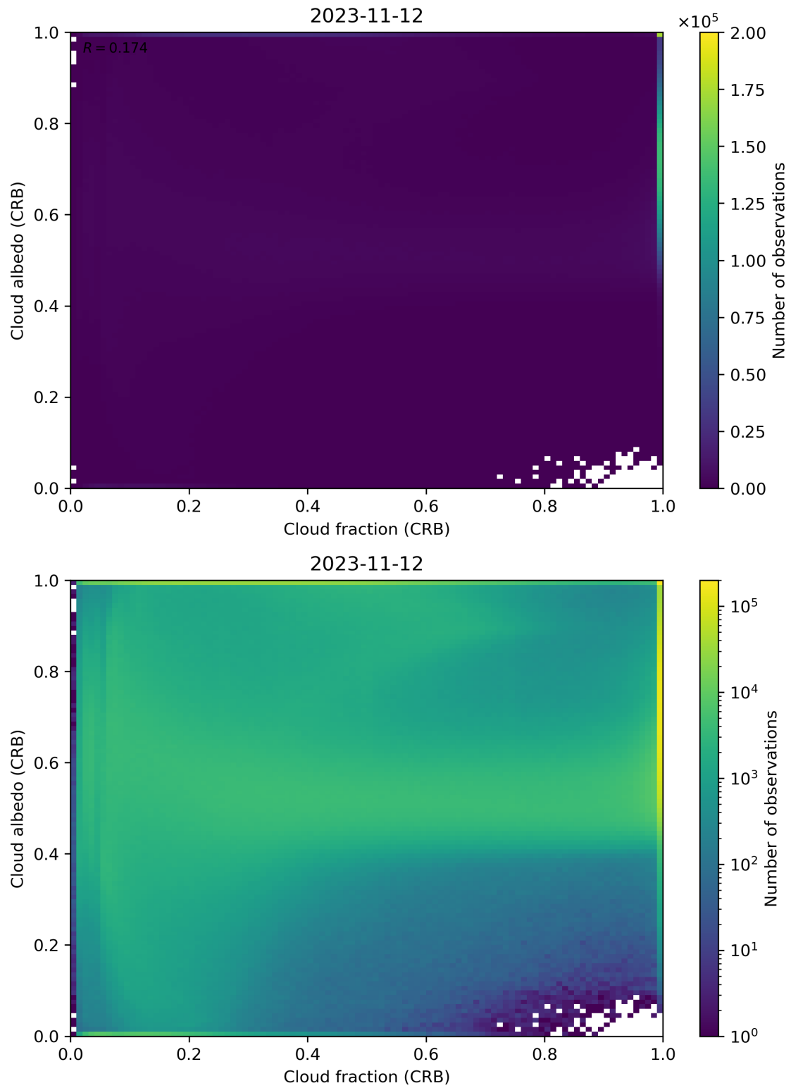
Figure 77: Scatter density plot of “Cloud fraction (CRB)” against “Cloud albedo (CRB)” for 2023-11-12 to 2023-11-13.
