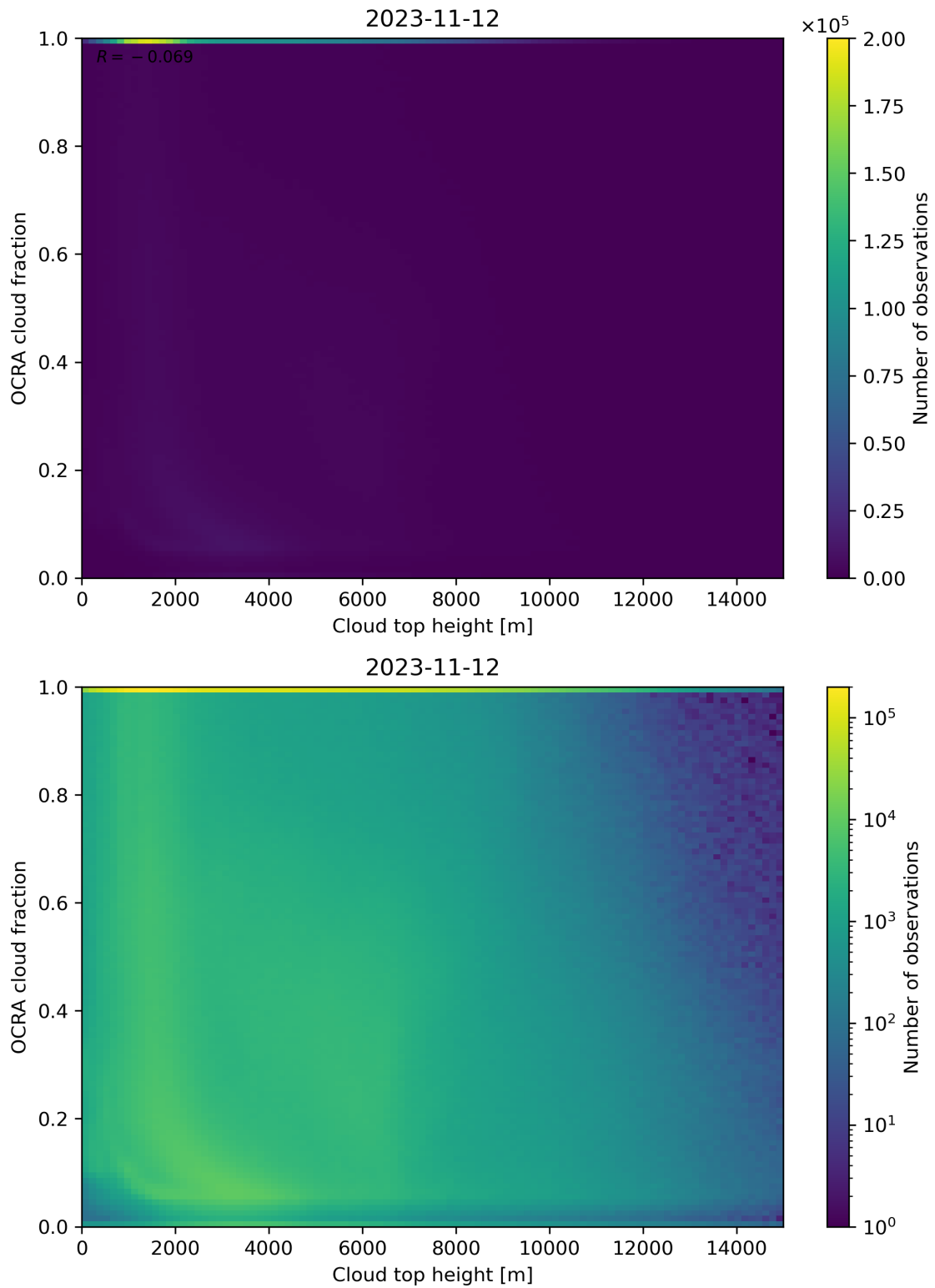
Figure 87: Scatter density plot of “Cloud top height” against “OCRA cloud fraction” for 2023-11-12 to 2023-11-13.
