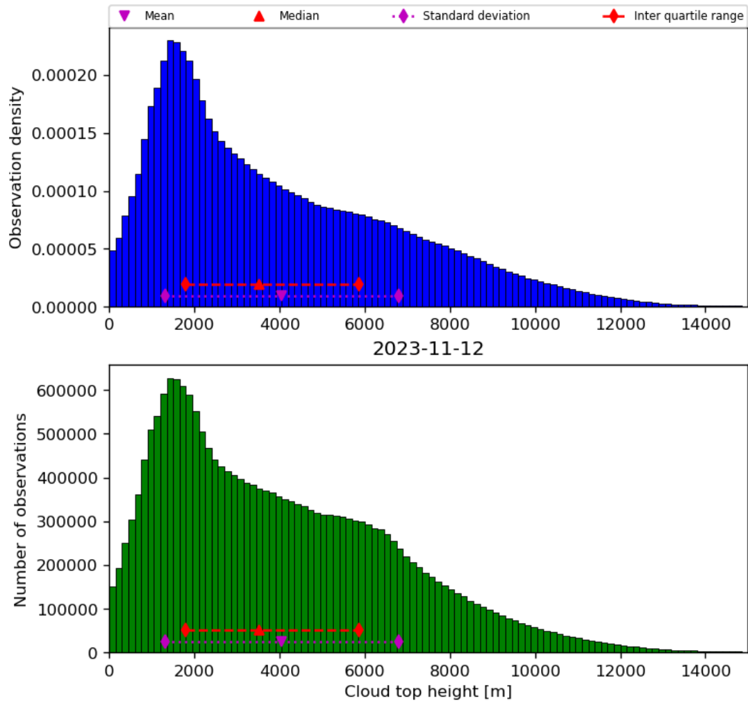
Figure 40: Histogram of “Cloud top height” for 2023-11-12 to 2023-11-13
