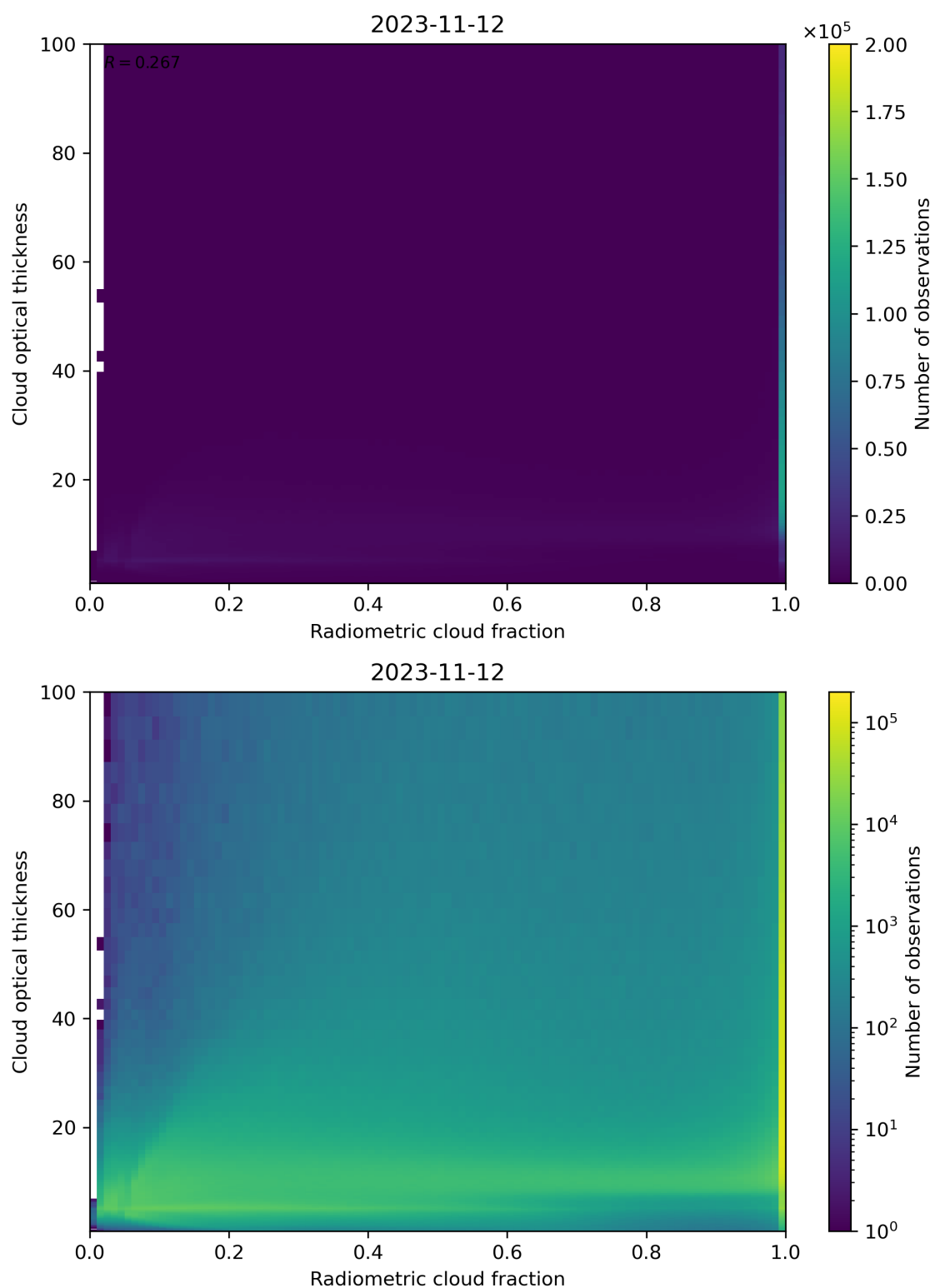
Figure 75: Scatter density plot of “Radiometric cloud fraction” against “Cloud optical thickness” for 2023-11-12 to 2023-11-13.
