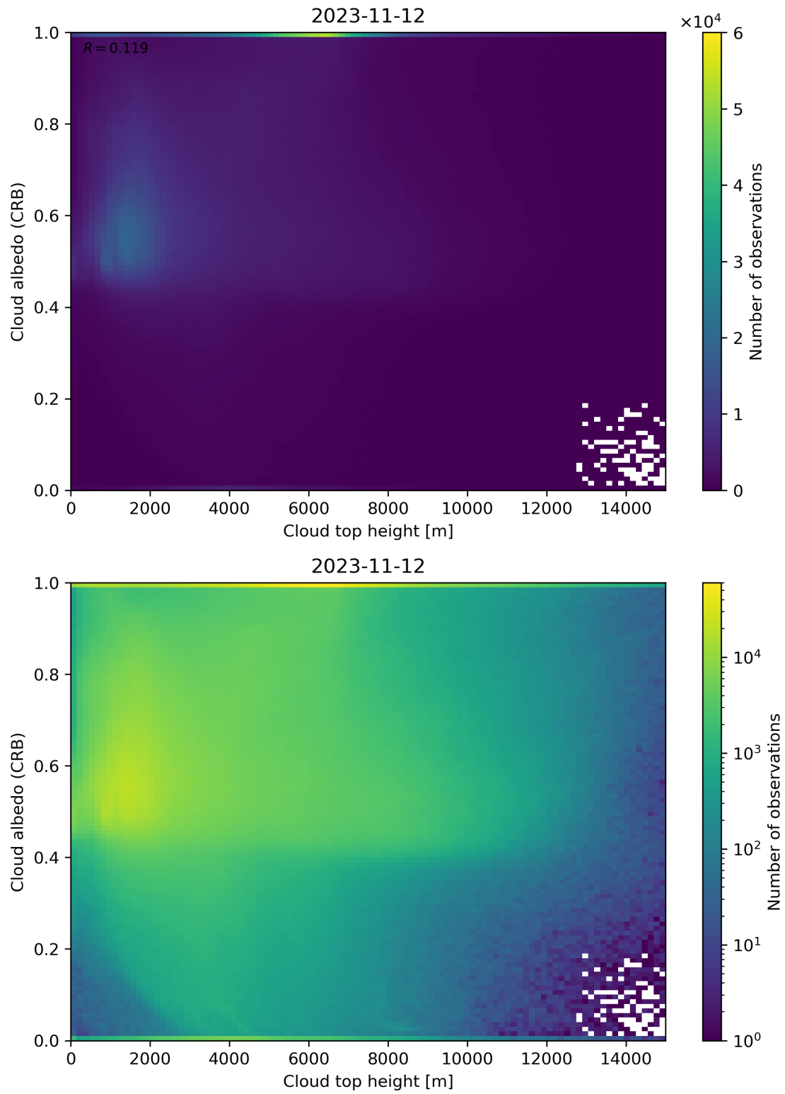
Figure 86: Scatter density plot of “Cloud top height” against “Cloud albedo (CRB)” for 2023-11-12 to 2023-11-13.
