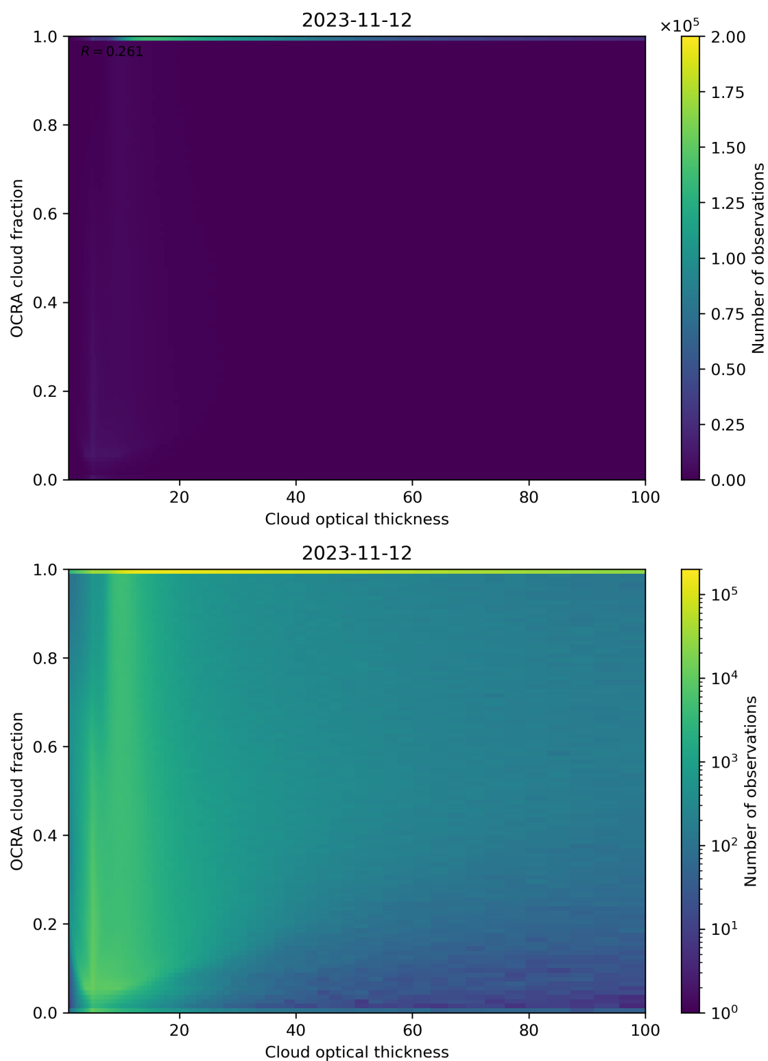
Figure 83: Scatter density plot of “Cloud optical thickness” against “OCRA cloud fraction” for 2023-11-12 to 2023-11-13.
