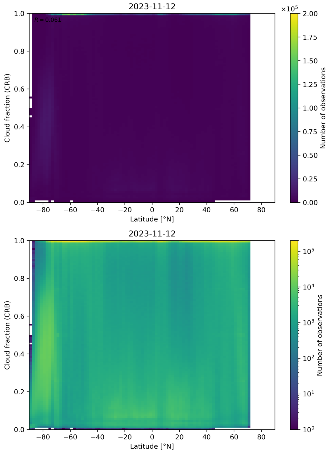
Figure 94: Scatter density plot of “Latitude” against “Cloud fraction (CRB)” for 2023-11-12 to 2023-11-13.
