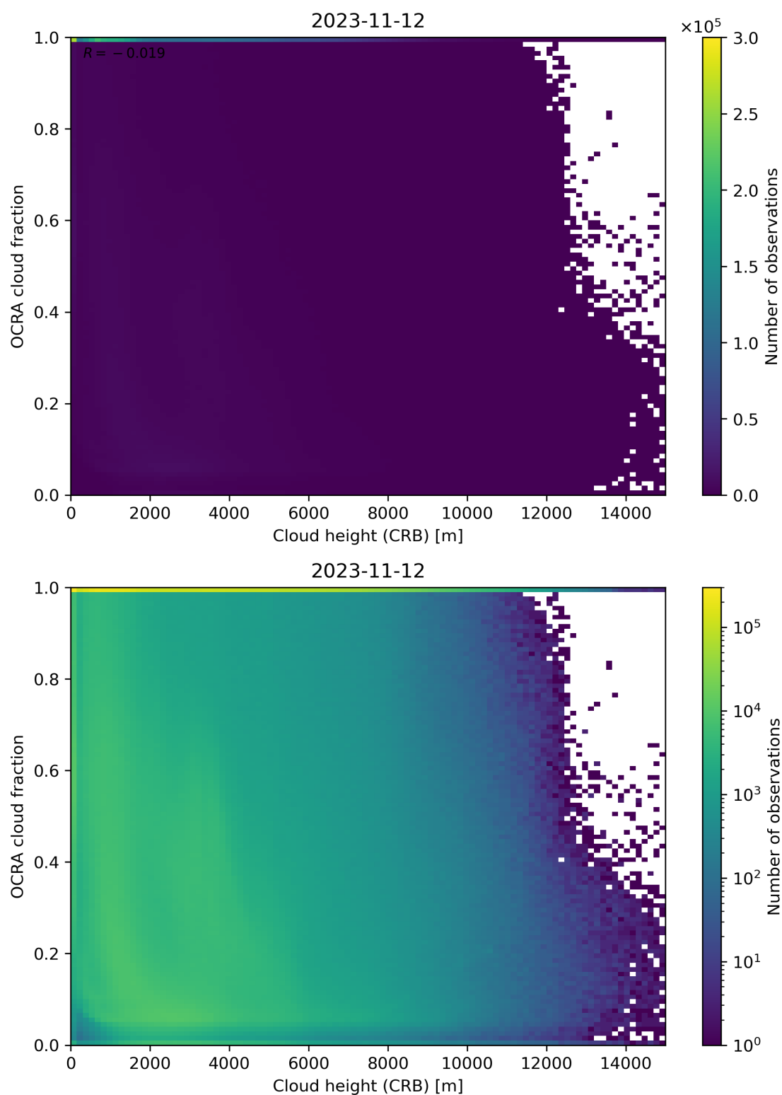
Figure 81: Scatter density plot of “Cloud height (CRB)” against “OCRA cloud fraction” for 2023-11-12 to 2023-11-13.
