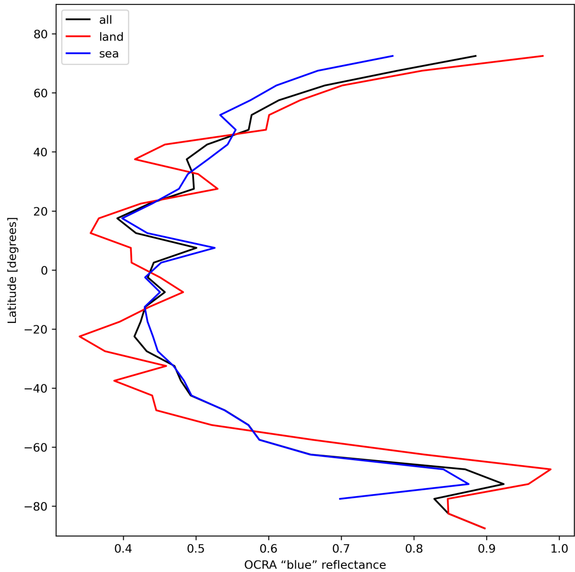
Figure 35: Zonal average of “OCRA “blue” reflectance” for 2023-11-12 to 2023-11-13.
