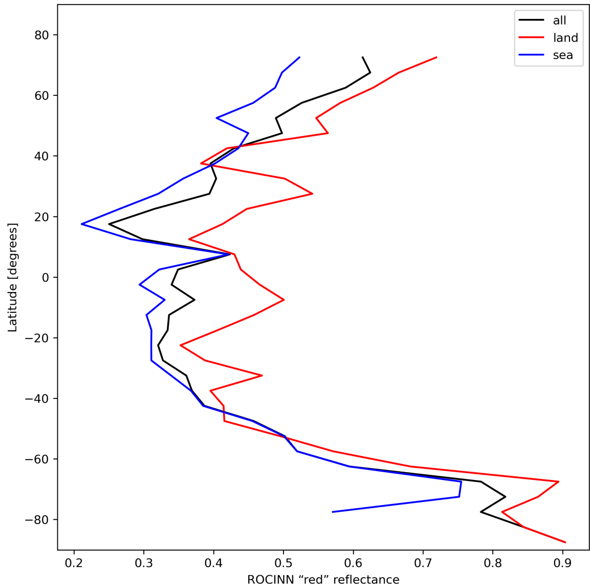
Figure 37: Zonal average of "ROCINN "red" reflectance" for 2023-11-12 to 2023-11-13.
