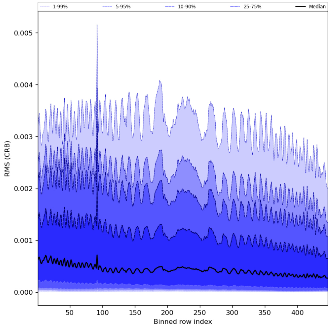
Figure 64: Along track statistics of “RMS (CRB)” for 2023-11-12 to 2023-11-13
