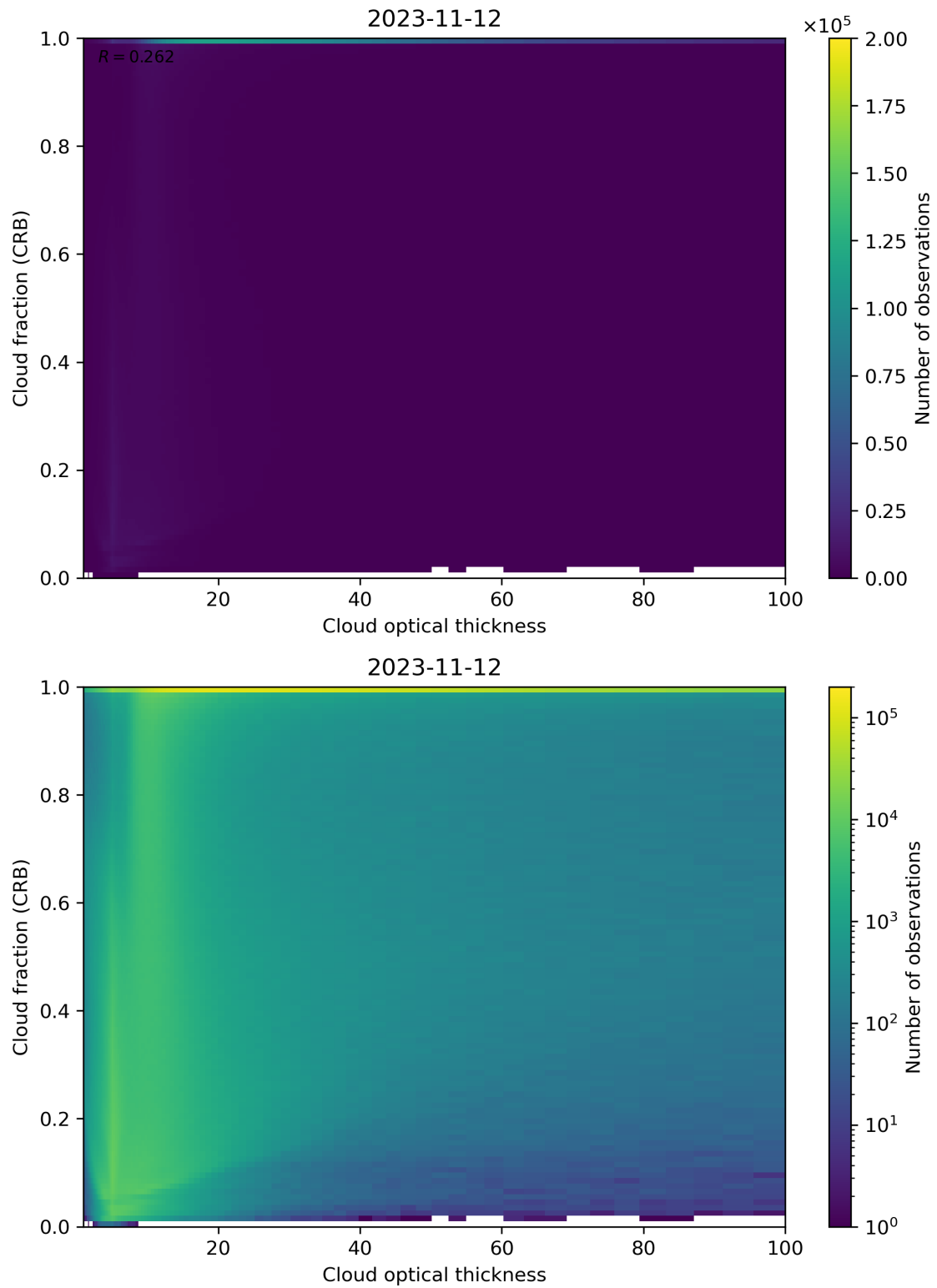
Figure 84: Scatter density plot of “Cloud optical thickness” against “Cloud fraction (CRB)” for 2023-11-12 to 2023-11-13.
