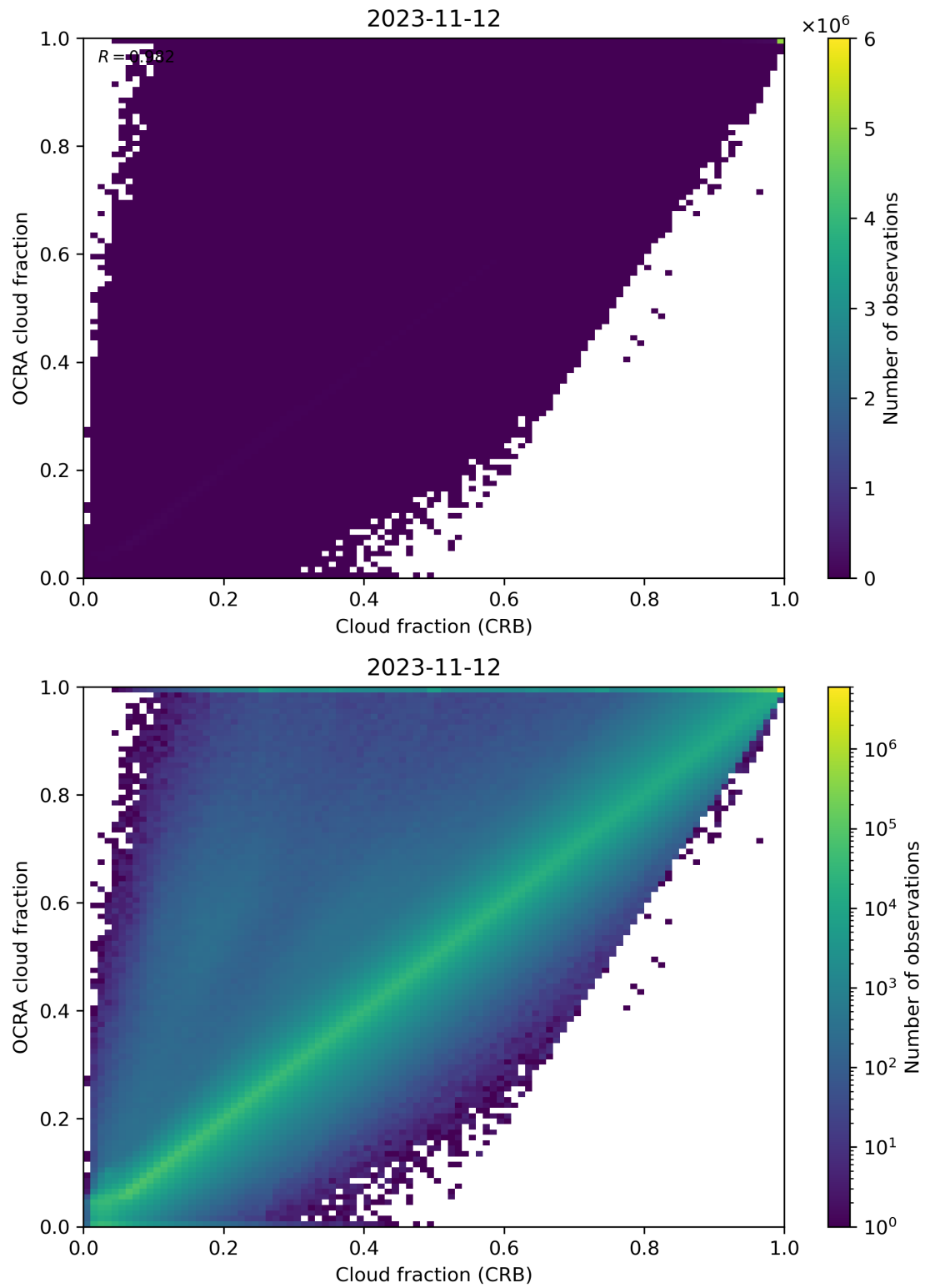
Figure 78: Scatter density plot of “Cloud fraction (CRB)” against “OCRA cloud fraction” for 2023-11-12 to 2023-11-13.
