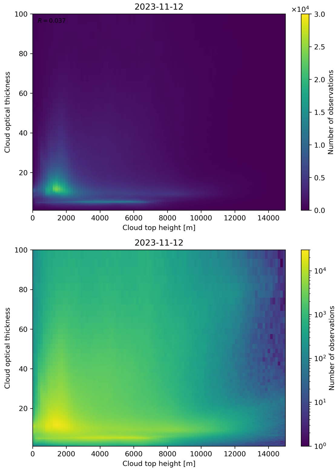
Figure 90: Scatter density plot of “Cloud top height” against “Cloud optical thickness” for 2023-11-12 to 2023-11-13.
