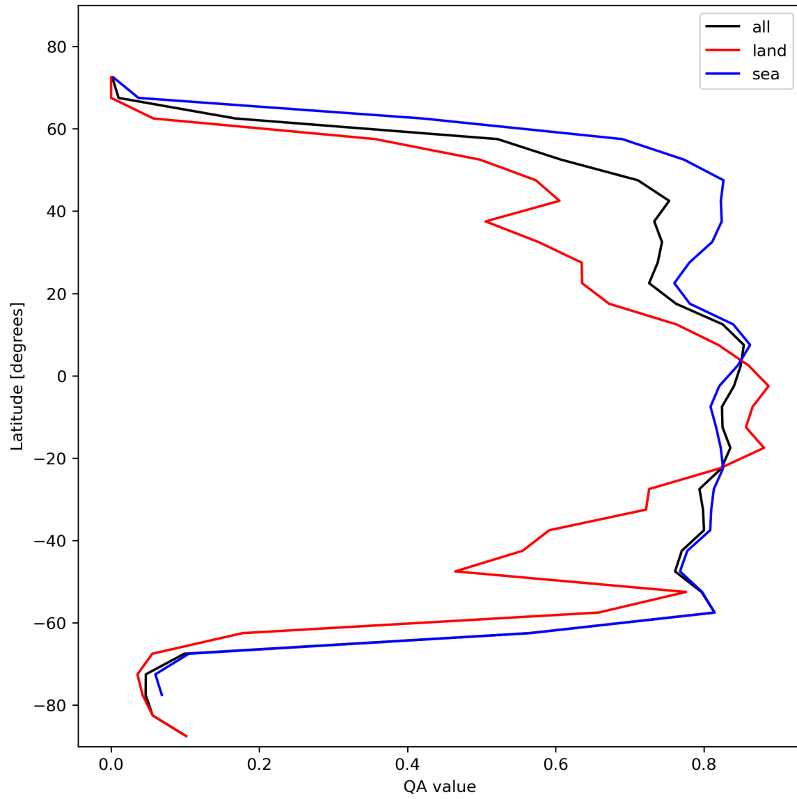
Figure 22: Zonal average of “QA value” for 2023-11-12 to 2023-11-13.
