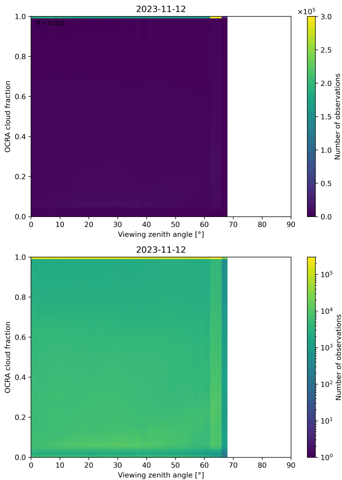
Figure 108: Scatter density plot of “Viewing zenith angle” against “OCRA cloud fraction” for 2023-11-12 to 2023-11-13.
