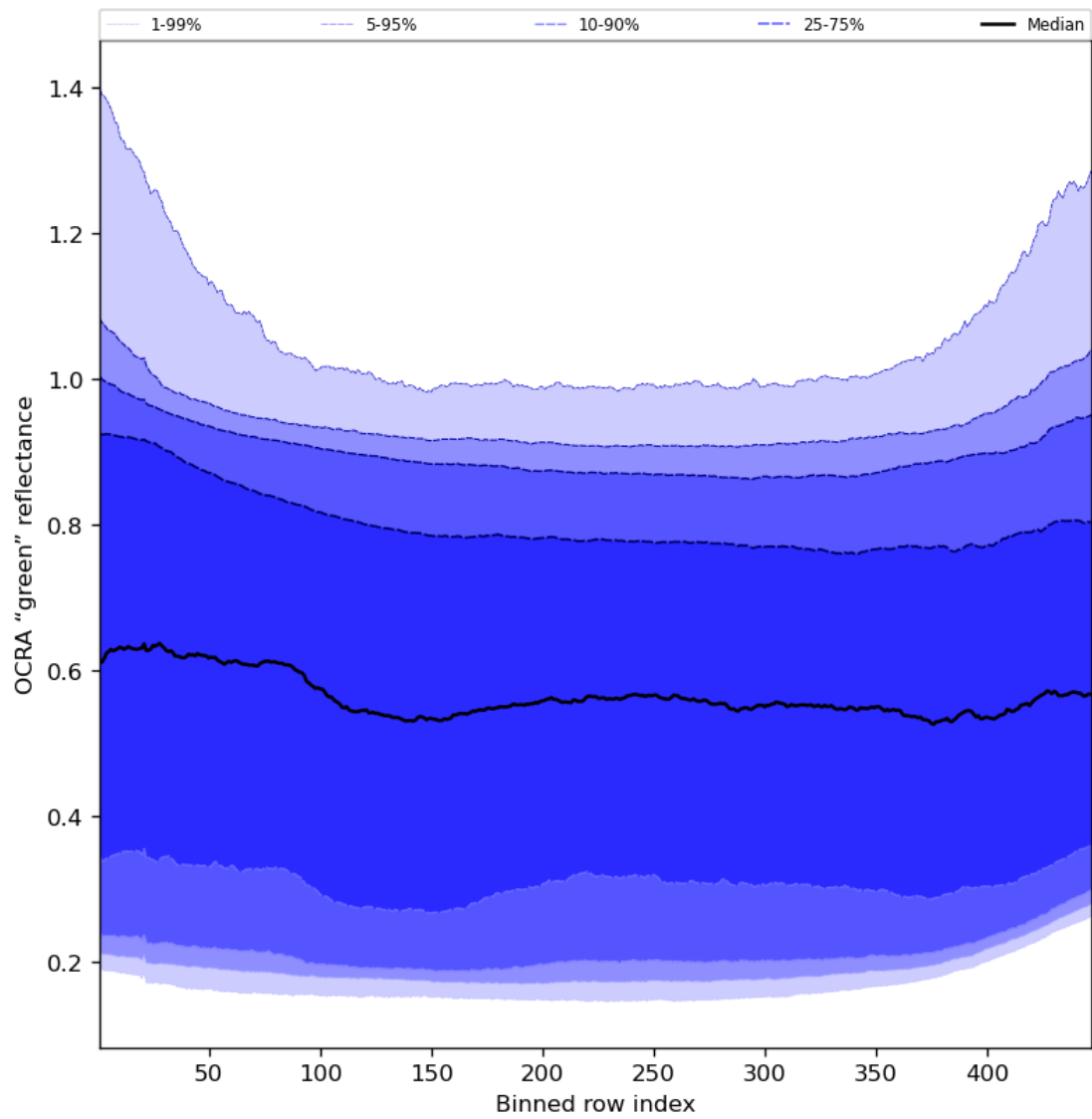
Figure 68: Along track statistics of "OCRA "green" reflectance" for 2023-11-12 to 2023-11-13
