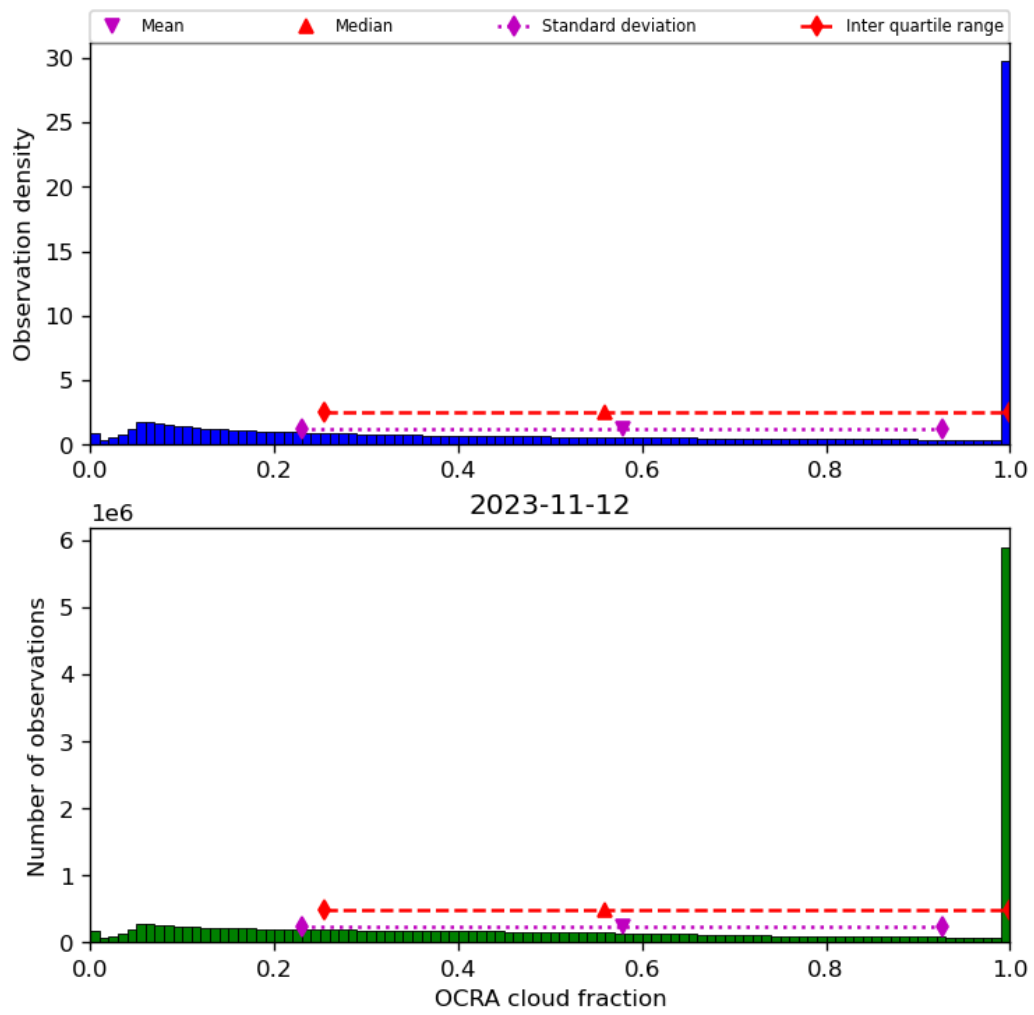
Figure 50: Histogram of “OCRA cloud fraction” for 2023-11-12 to 2023-11-13
