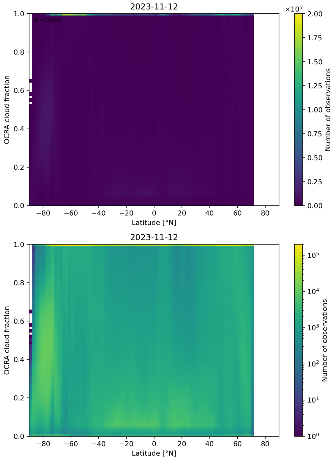
Figure 93: Scatter density plot of “Latitude” against “OCRA cloud fraction” for 2023-11-12 to 2023-11-13.
