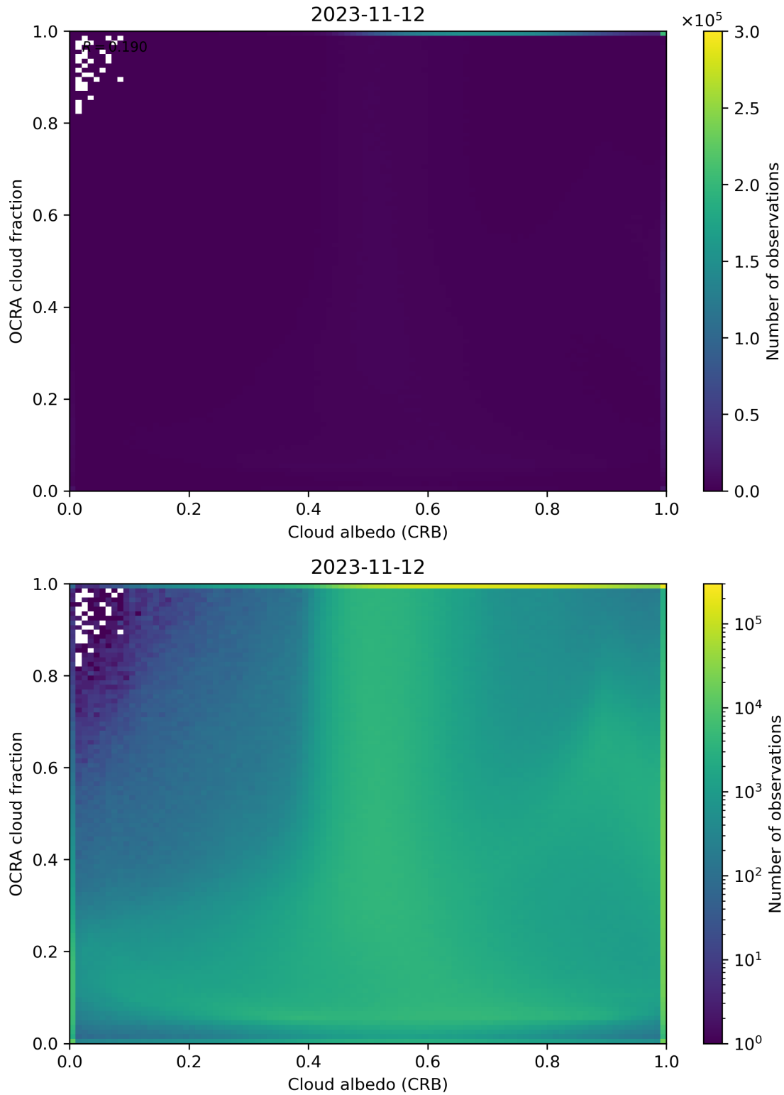
Figure 70: Scatter density plot of “Cloud albedo (CRB)” against “OCRA cloud fraction” for 2023-11-12 to 2023-11-13.
