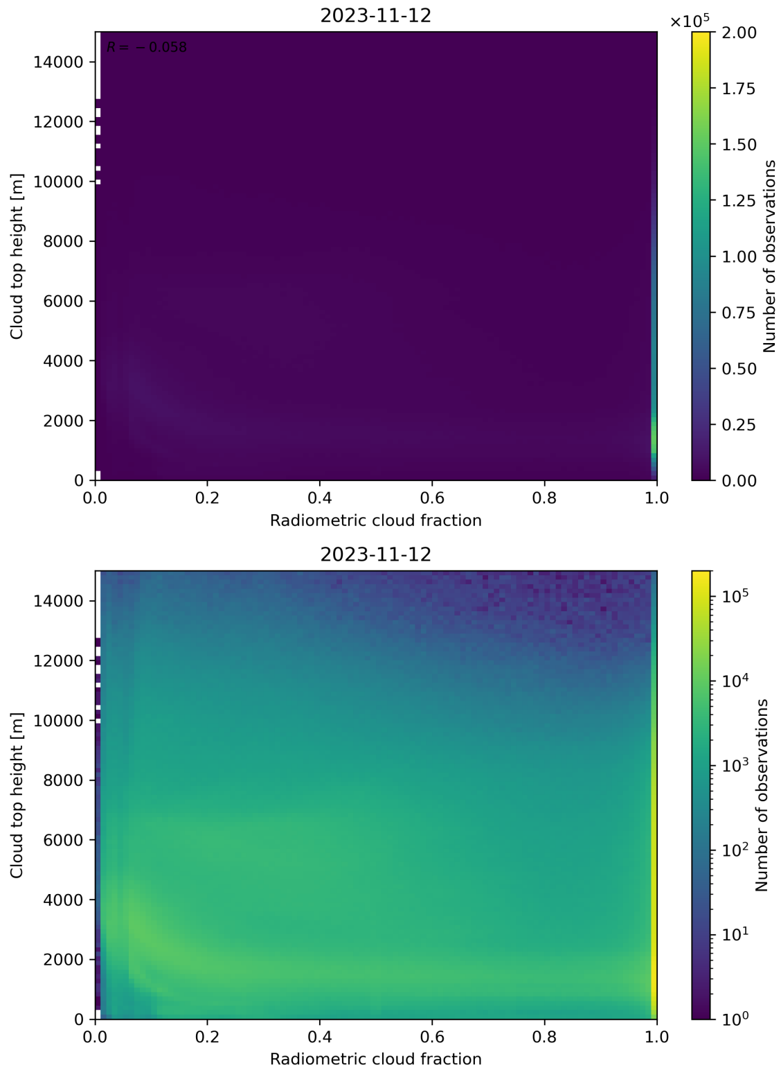
Figure 76: Scatter density plot of “Radiometric cloud fraction” against “Cloud top height” for 2023-11-12 to 2023-11-13.
