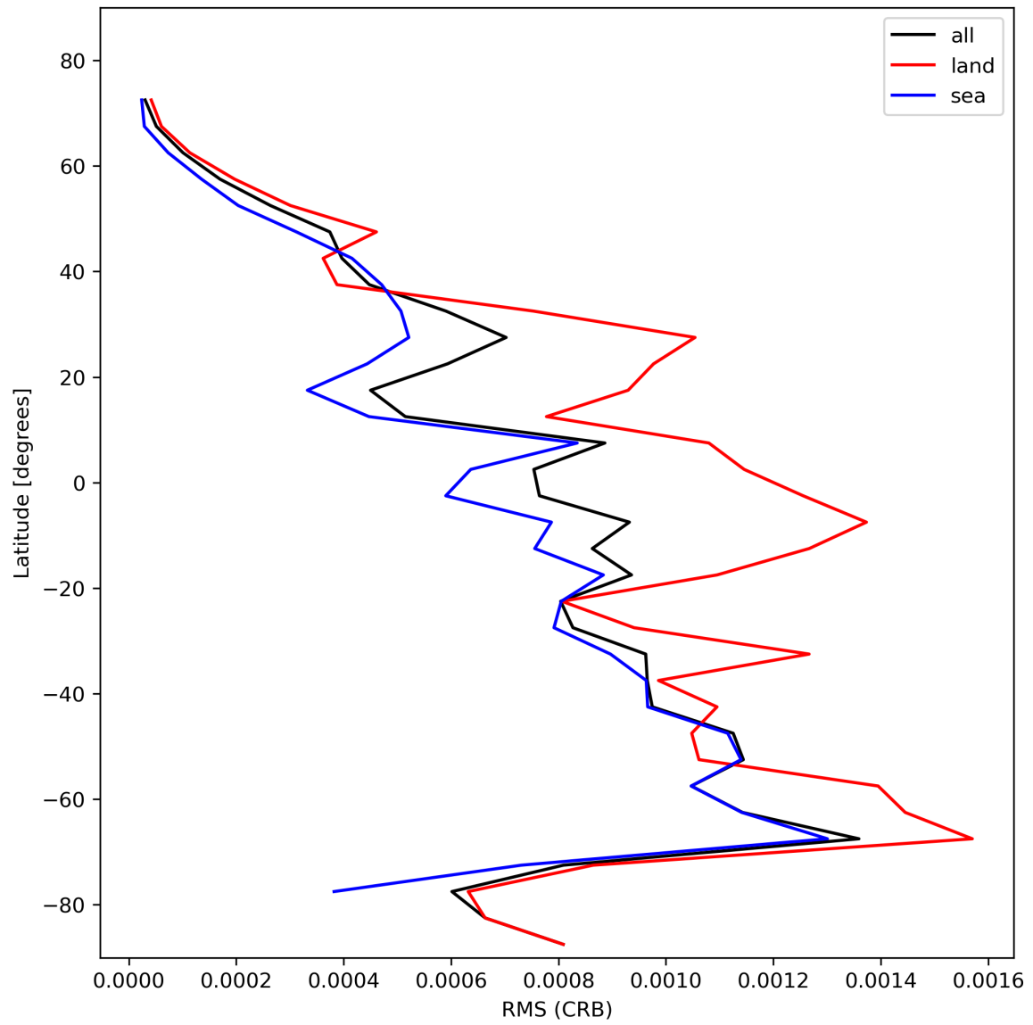
Figure 32: Zonal average of “RMS (CRB)” for 2023-11-12 to 2023-11-13.
