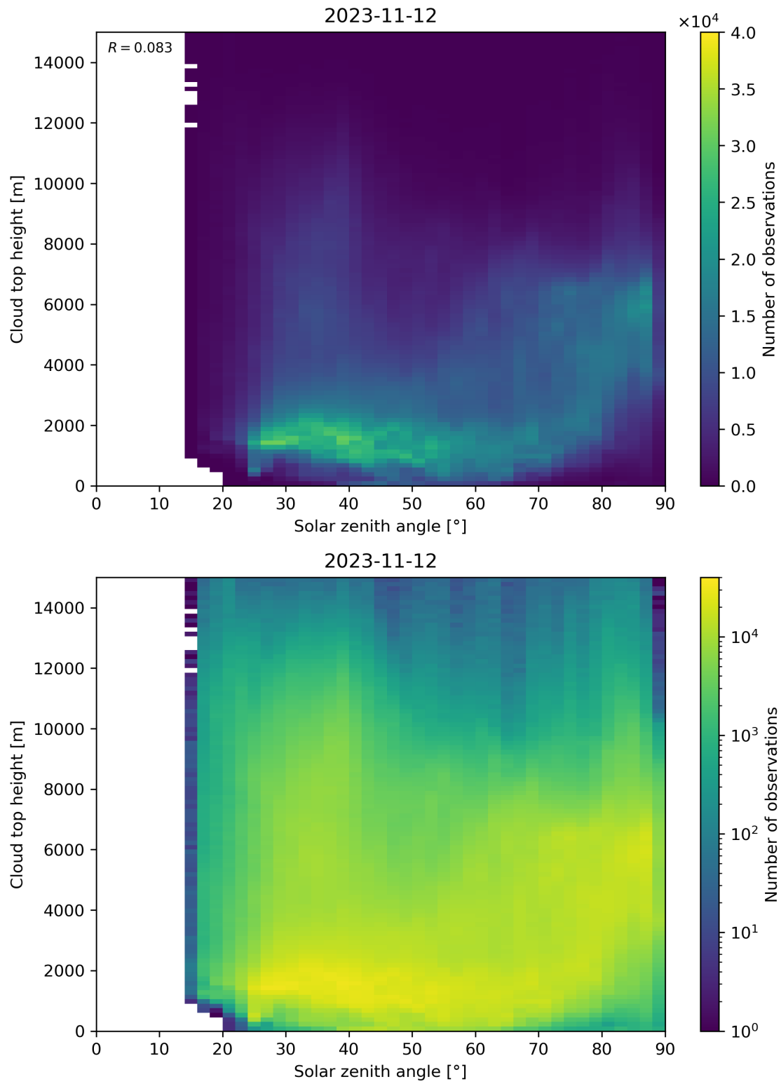
Figure 104: Scatter density plot of “Solar zenith angle” against “Cloud top height” for 2023-11-12 to 2023-11-13.
