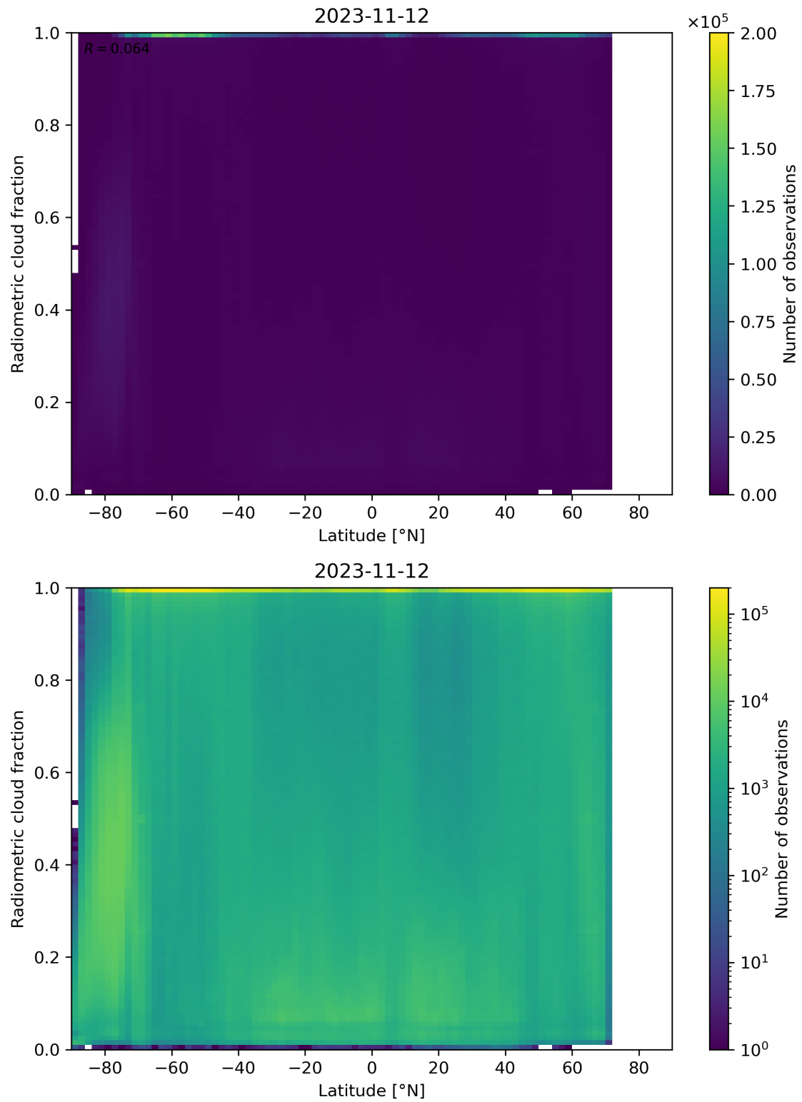
Figure 92: Scatter density plot of “Latitude” against “Radiometric cloud fraction” for 2023-11-12 to 2023-11-13.
