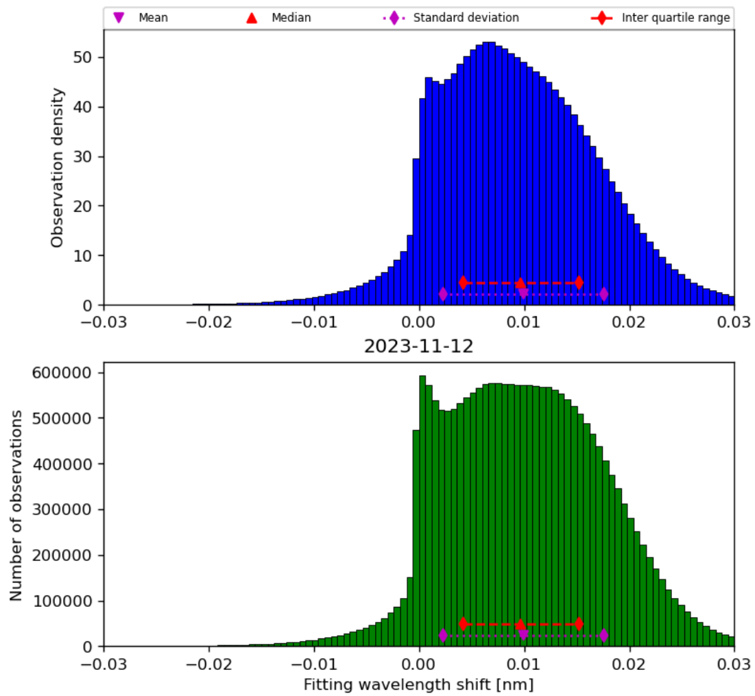
Figure 49: Histogram of “Fitting wavelength shift” for 2023-11-12 to 2023-11-13
