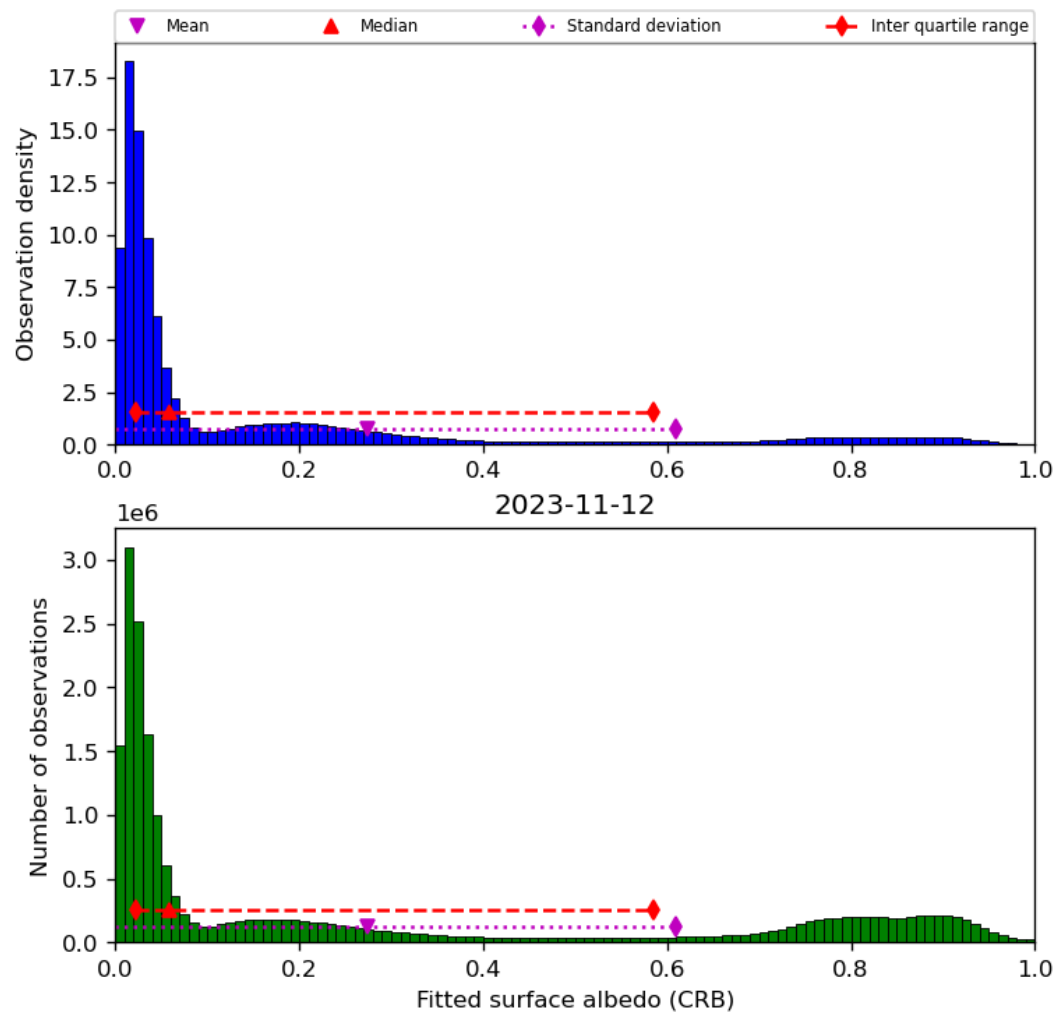
Figure 46: Histogram of “Fitted surface albedo (CRB)” for 2023-11-12 to 2023-11-13
