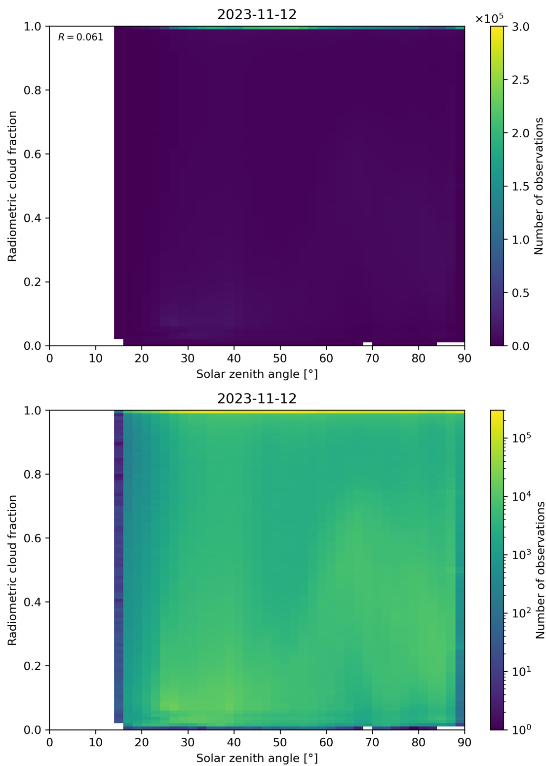
Figure 99: Scatter density plot of “Solar zenith angle” against “Radiometric cloud fraction” for 2023-11-12 to 2023-11-13.
