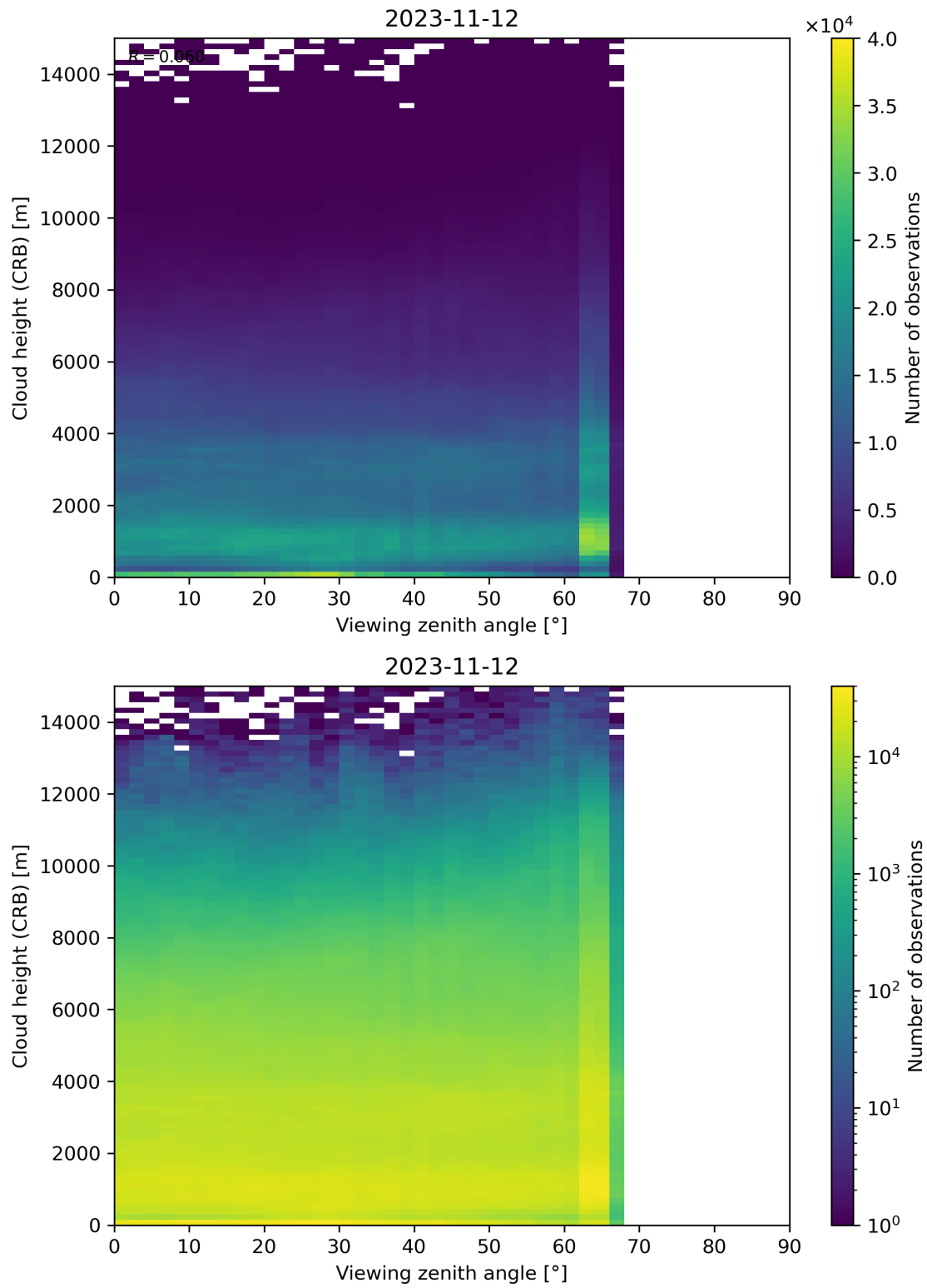
Figure 110: Scatter density plot of “Viewing zenith angle” against “Cloud height (CRB)” for 2023-11-12 to 2023-11-13.
