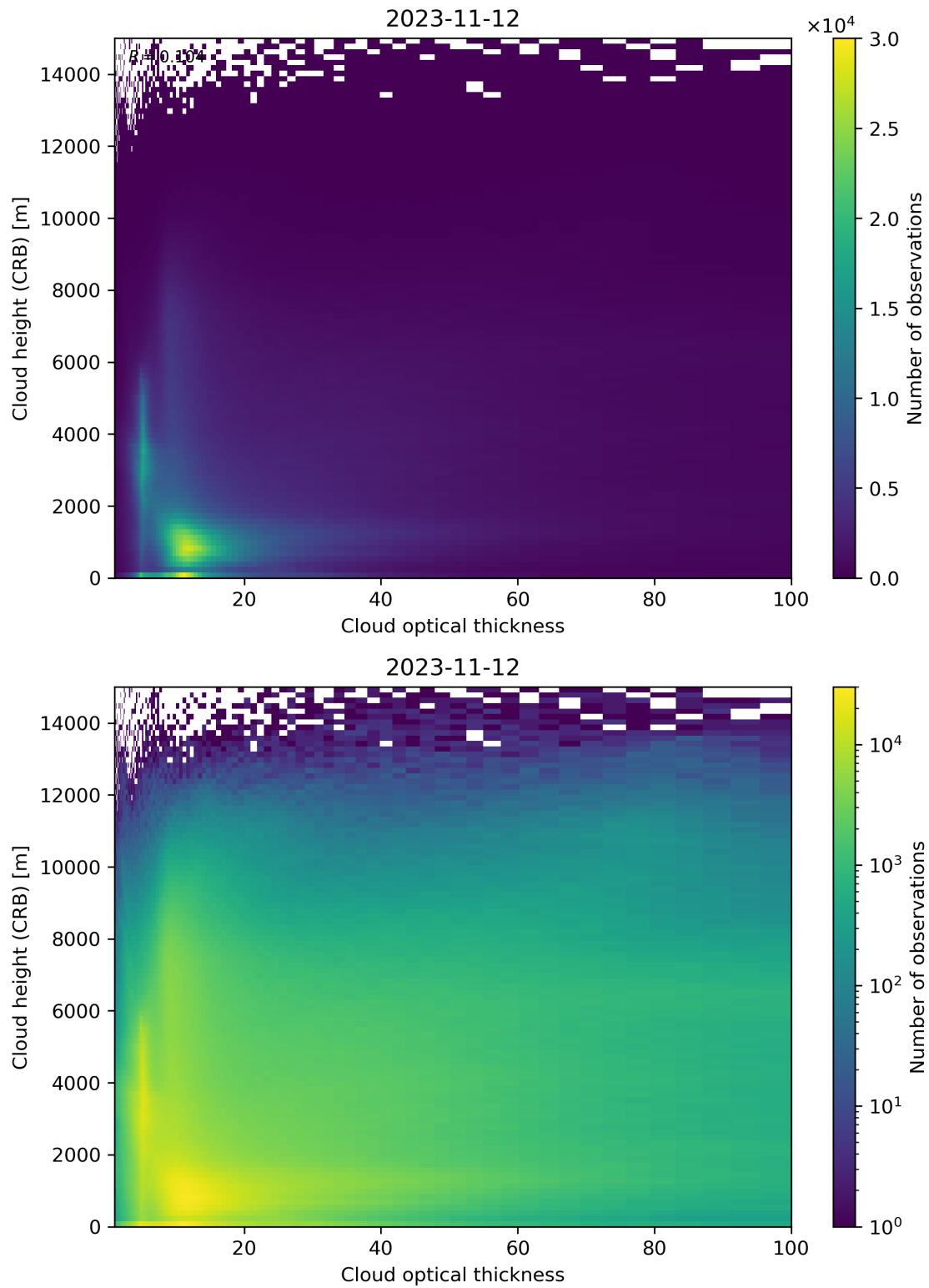
Figure 85: Scatter density plot of “Cloud optical thickness” against “Cloud height (CRB)” for 2023-11-12 to 2023-11-13.
