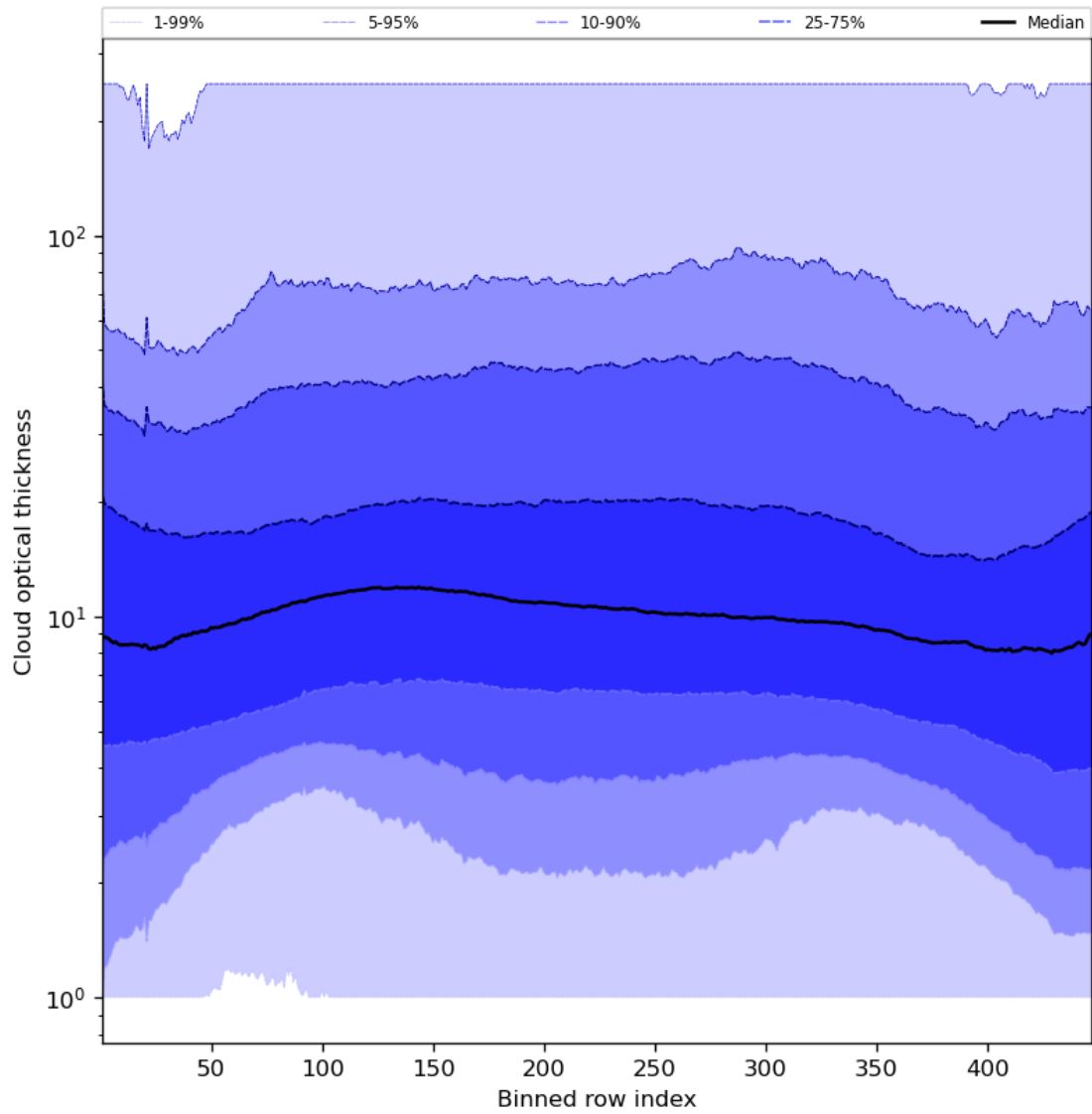
Figure 57: Along track statistics of “Cloud optical thickness” for 2023-11-12 to 2023-11-13
