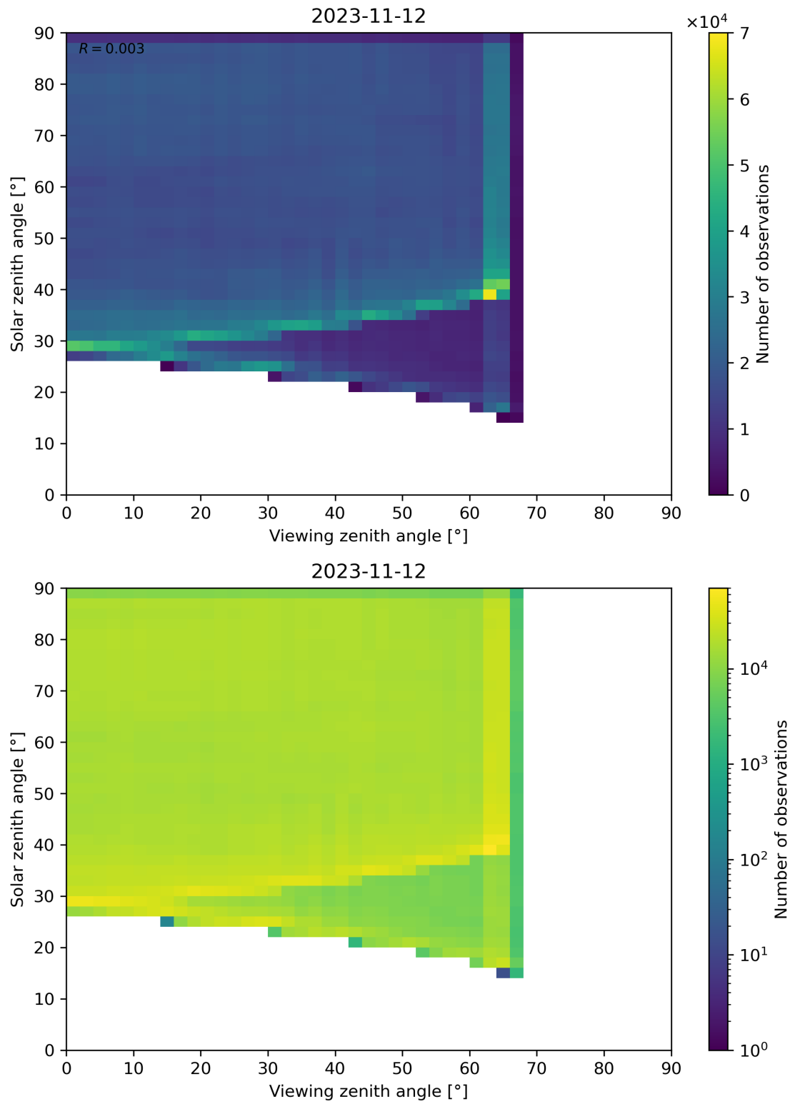
Figure 114: Scatter density plot of “Viewing zenith angle” against “Solar zenith angle” for 2023-11-12 to 2023-11-13.
