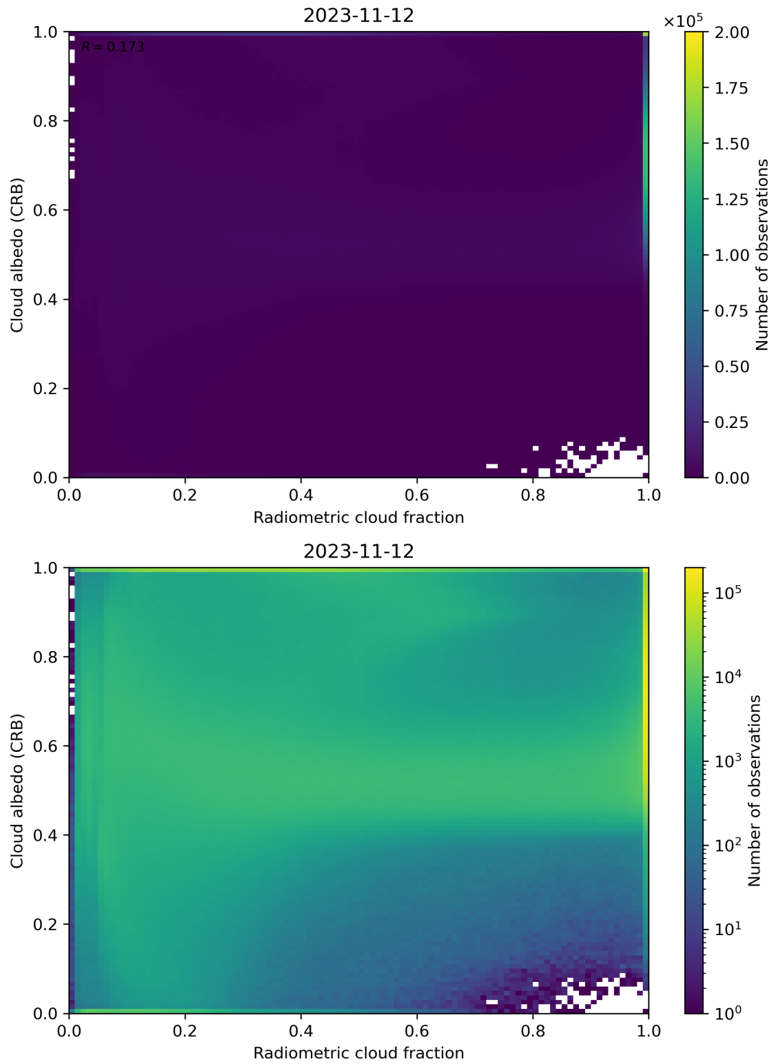
Figure 71: Scatter density plot of “Radiometric cloud fraction” against “Cloud albedo (CRB)” for 2023-11-12 to 2023-11-13.
