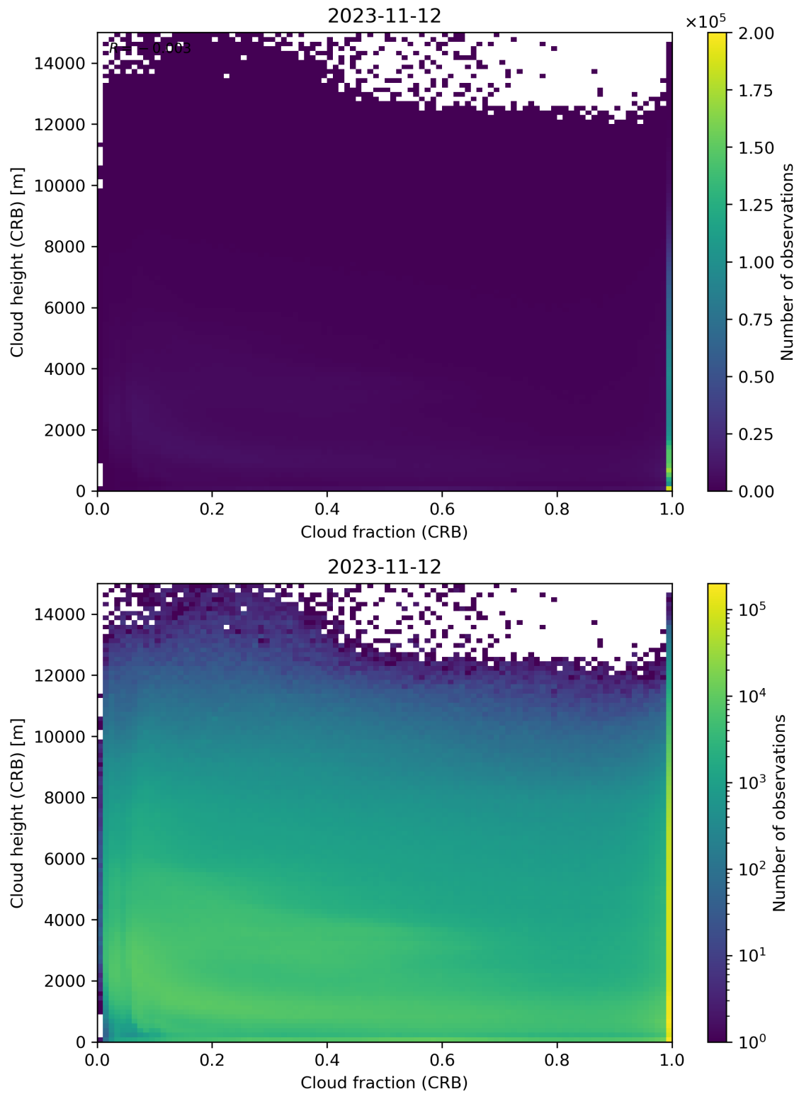
Figure 79: Scatter density plot of “Cloud fraction (CRB)” against “Cloud height (CRB)” for 2023-11-12 to 2023-11-13.
