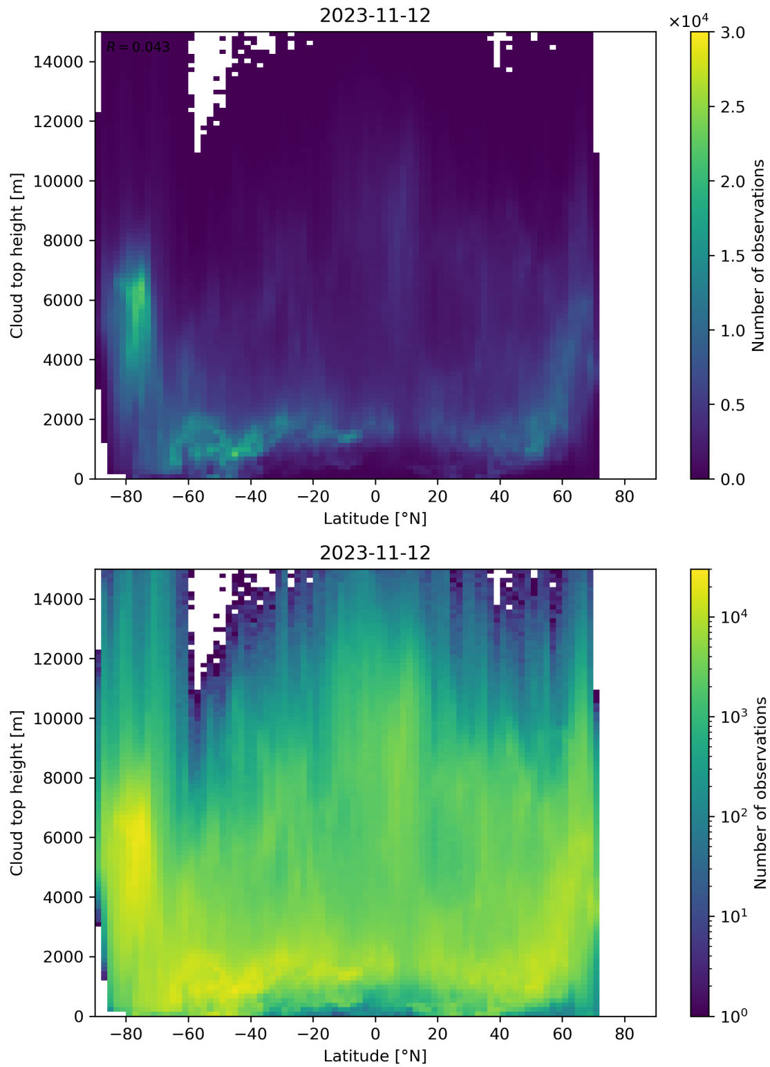
Figure 97: Scatter density plot of “Latitude” against “Cloud top height” for 2023-11-12 to 2023-11-13.
