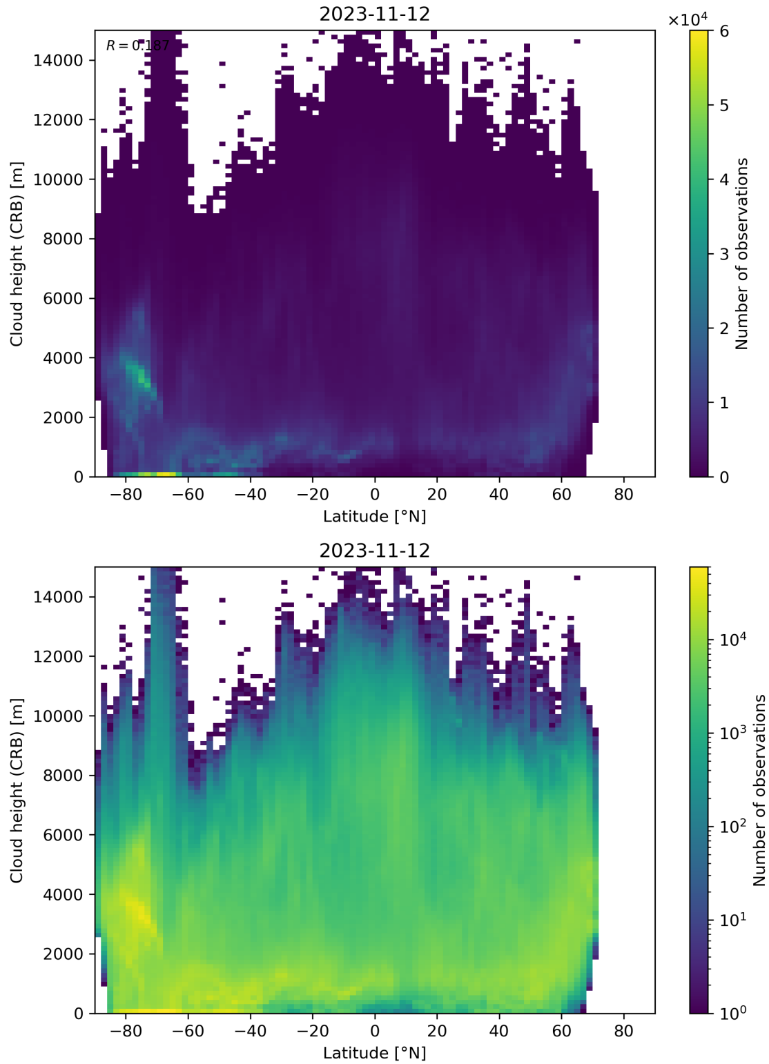
Figure 95: Scatter density plot of “Latitude” against “Cloud height (CRB)” for 2023-11-12 to 2023-11-13.
