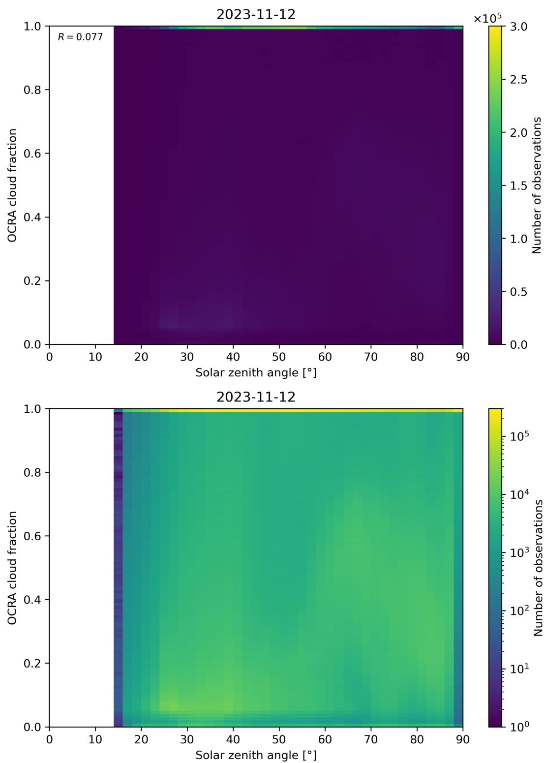
Figure 100: Scatter density plot of “Solar zenith angle” against “OCRA cloud fraction” for 2023-11-12 to 2023-11-13.
