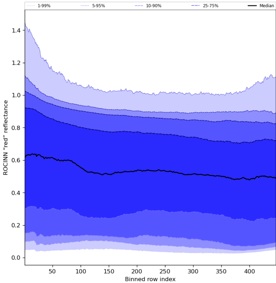
Figure 69: Along track statistics of “ROCINN “red” reflectance” for 2023-11-12 to 2023-11-13
