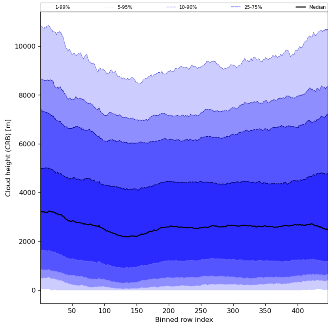
Figure 59: Along track statistics of “Cloud height (CRB)” for 2023-11-12 to 2023-11-13
