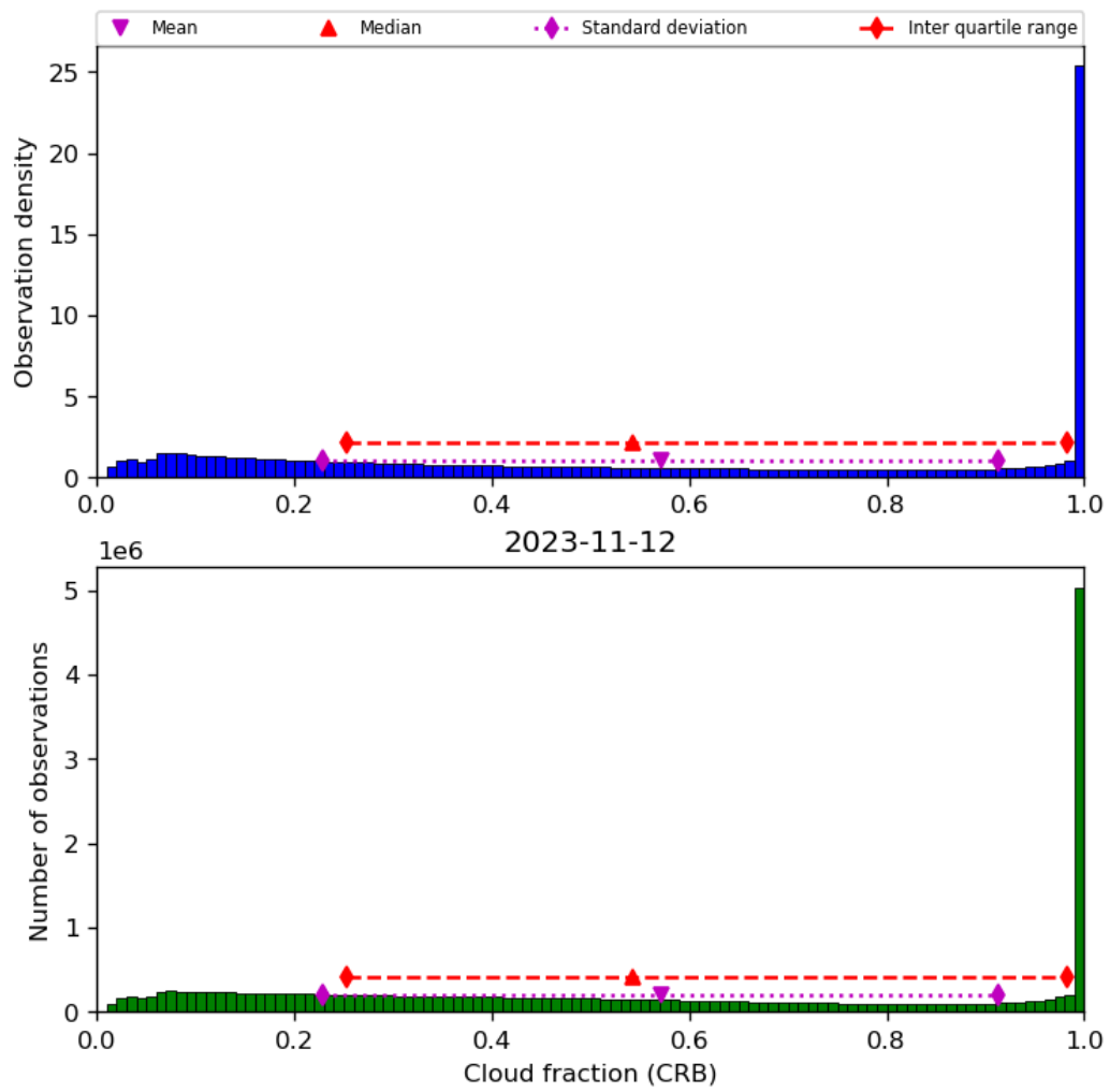
Figure 42: Histogram of “Cloud fraction (CRB)” for 2023-11-12 to 2023-11-13
