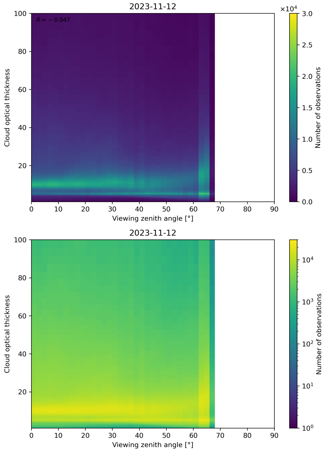
Figure 111: Scatter density plot of “Viewing zenith angle” against “Cloud optical thickness” for 2023-11-12 to 2023-11-13.
