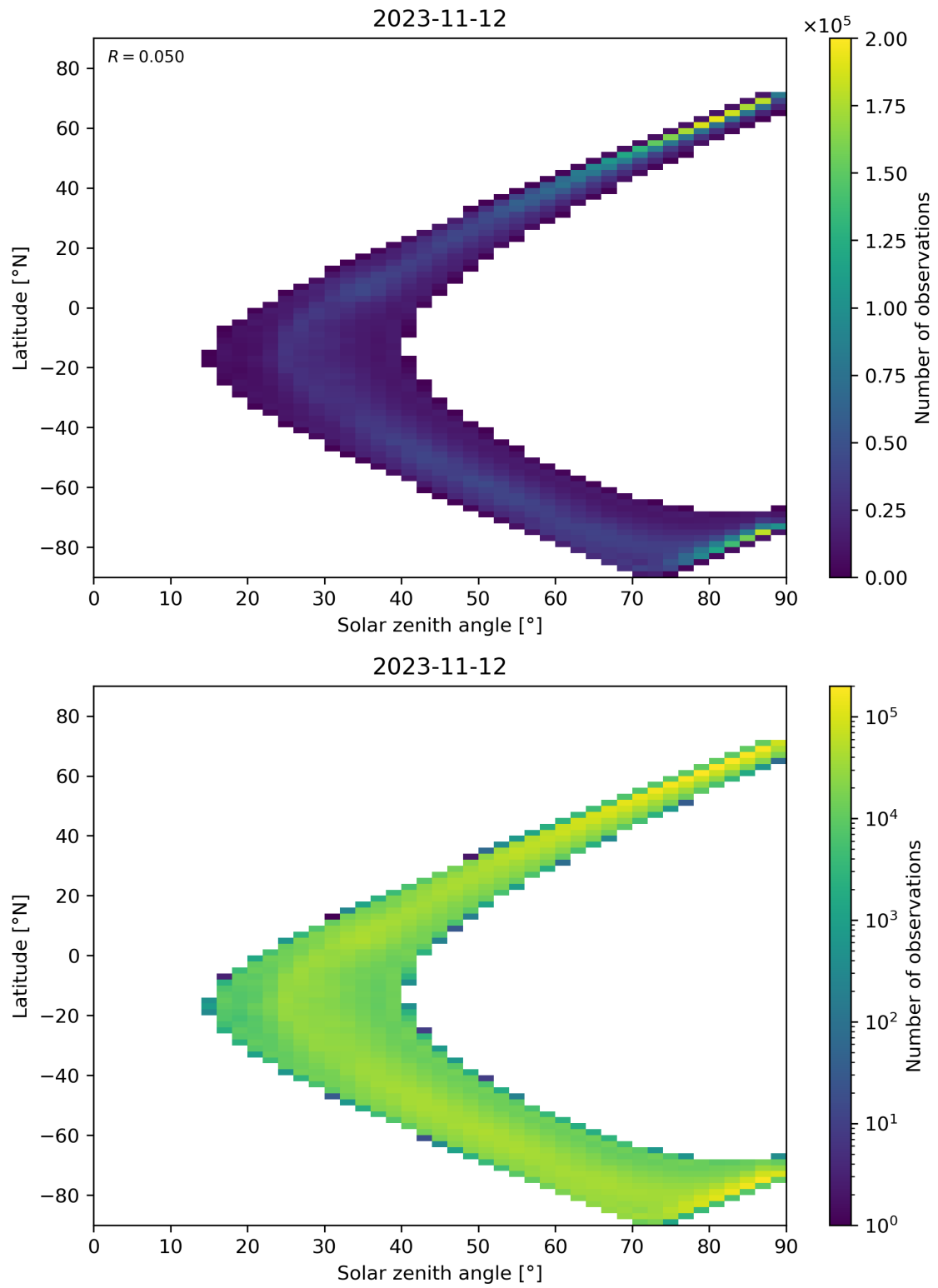
Figure 105: Scatter density plot of “Solar zenith angle” against “Latitude” for 2023-11-12 to 2023-11-13.
