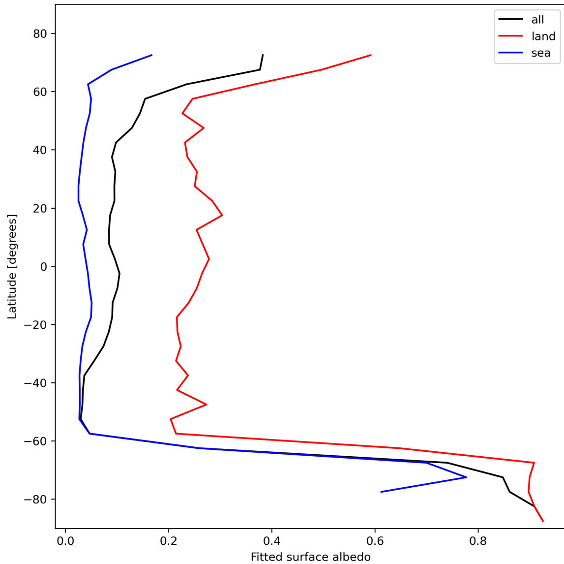
Figure 29: Zonal average of “Fitted surface albedo” for 2023-11-12 to 2023-11-13.
