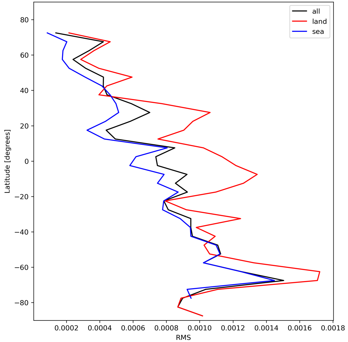
Figure 31: Zonal average of “RMS” for 2023-11-12 to 2023-11-13.
