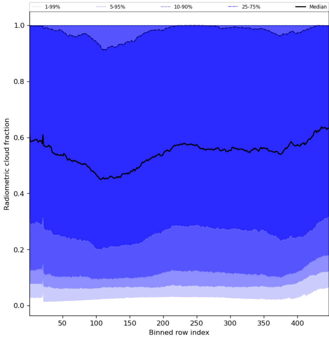
Figure 55: Along track statistics of “Radiometric cloud fraction” for 2023-11-12 to 2023-11-13
