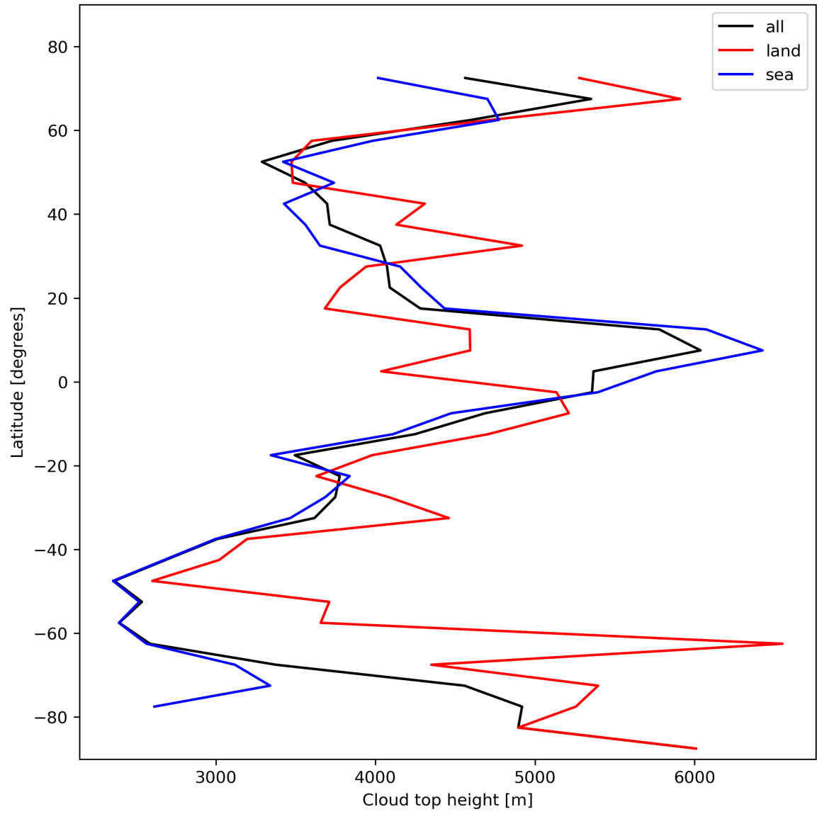
Figure 24: Zonal average of “Cloud top height” for 2023-11-12 to 2023-11-13.
