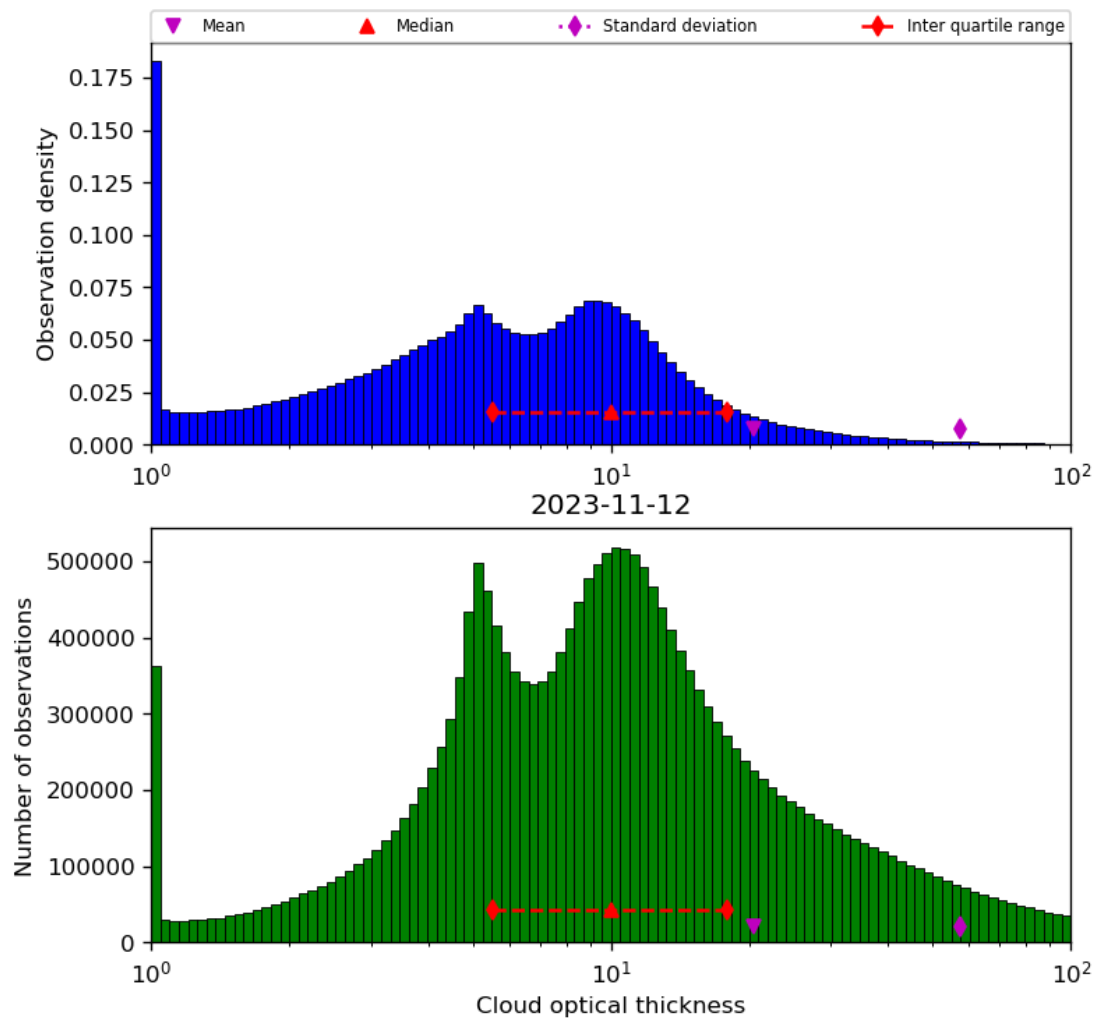
Figure 41: Histogram of “Cloud optical thickness” for 2023-11-12 to 2023-11-13
