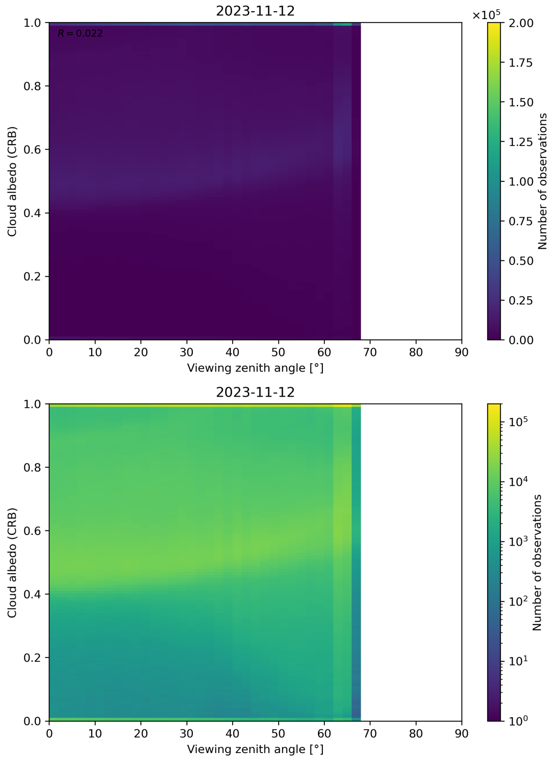
Figure 106: Scatter density plot of “Viewing zenith angle” against “Cloud albedo (CRB)” for 2023-11-12 to 2023-11-13.
