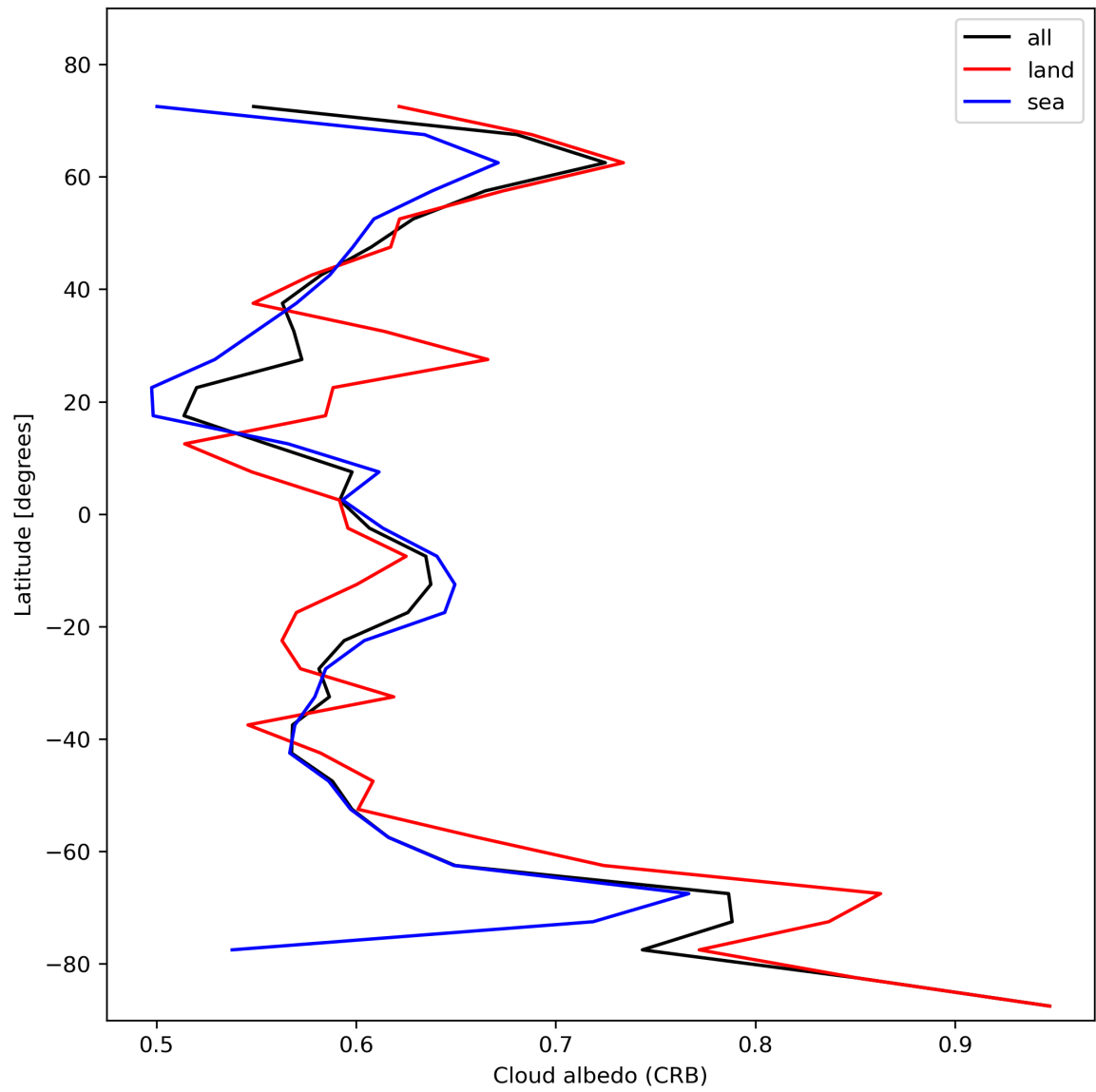
Figure 28: Zonal average of “Cloud albedo (CRB)” for 2023-11-12 to 2023-11-13.
