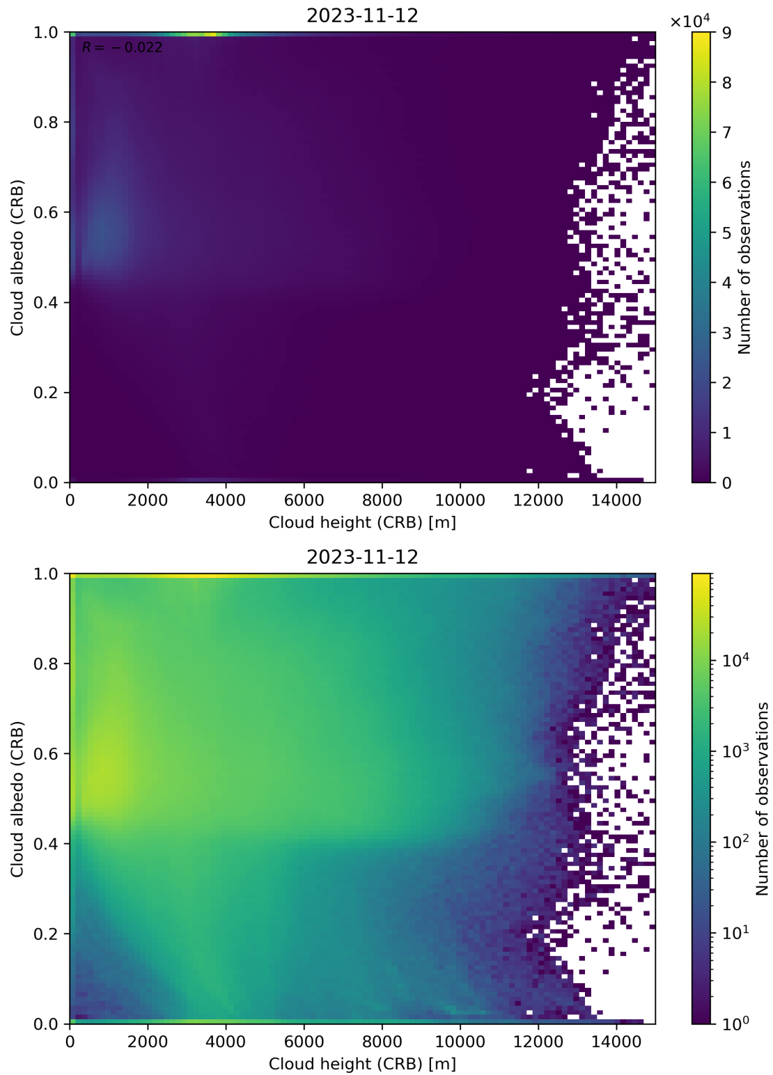
Figure 80: Scatter density plot of “Cloud height (CRB)” against “Cloud albedo (CRB)” for 2023-11-12 to 2023-11-13.
