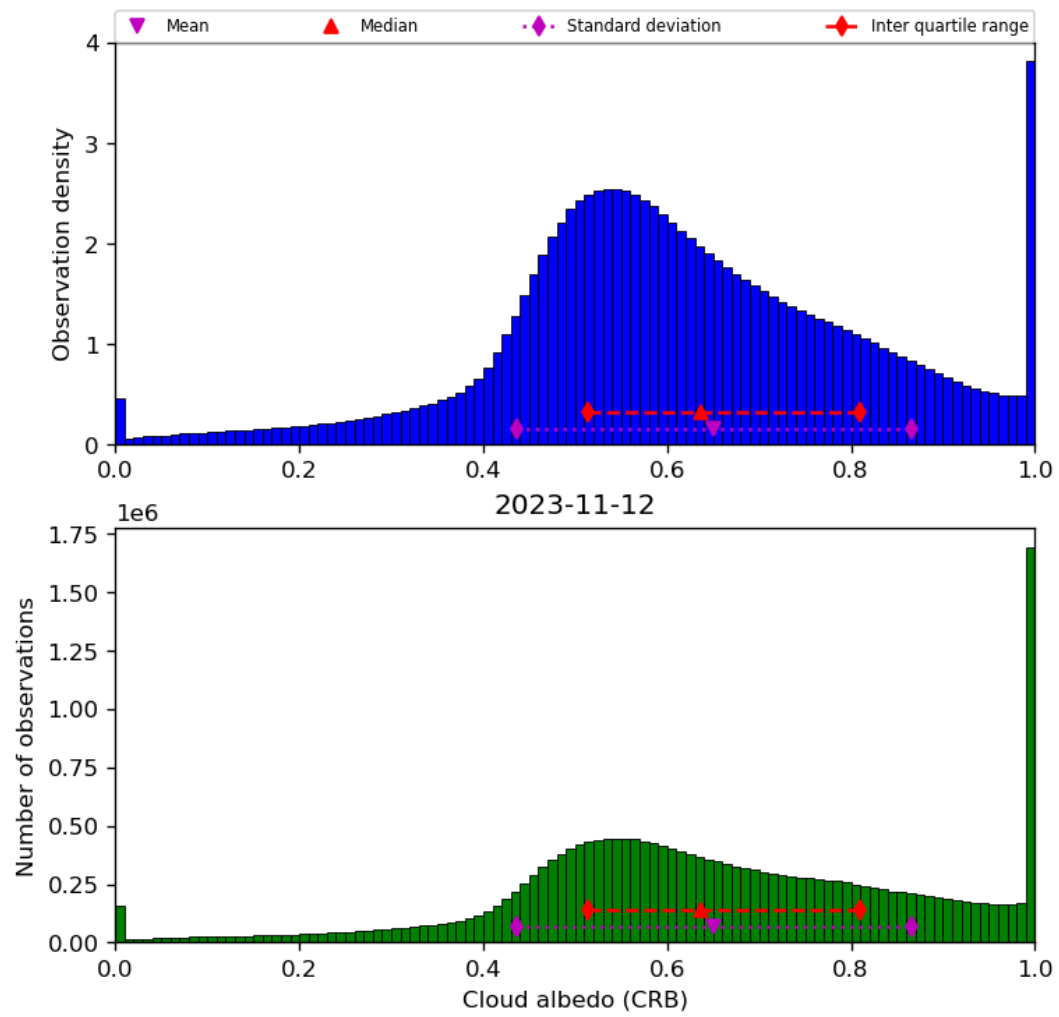
Figure 44: Histogram of “Cloud albedo (CRB)” for 2023-11-12 to 2023-11-13
