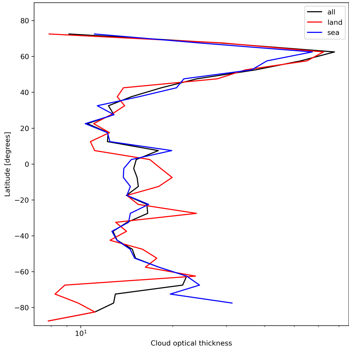
Figure 25: Zonal average of “Cloud optical thickness” for 2023-11-13 to 2023-11-15.
