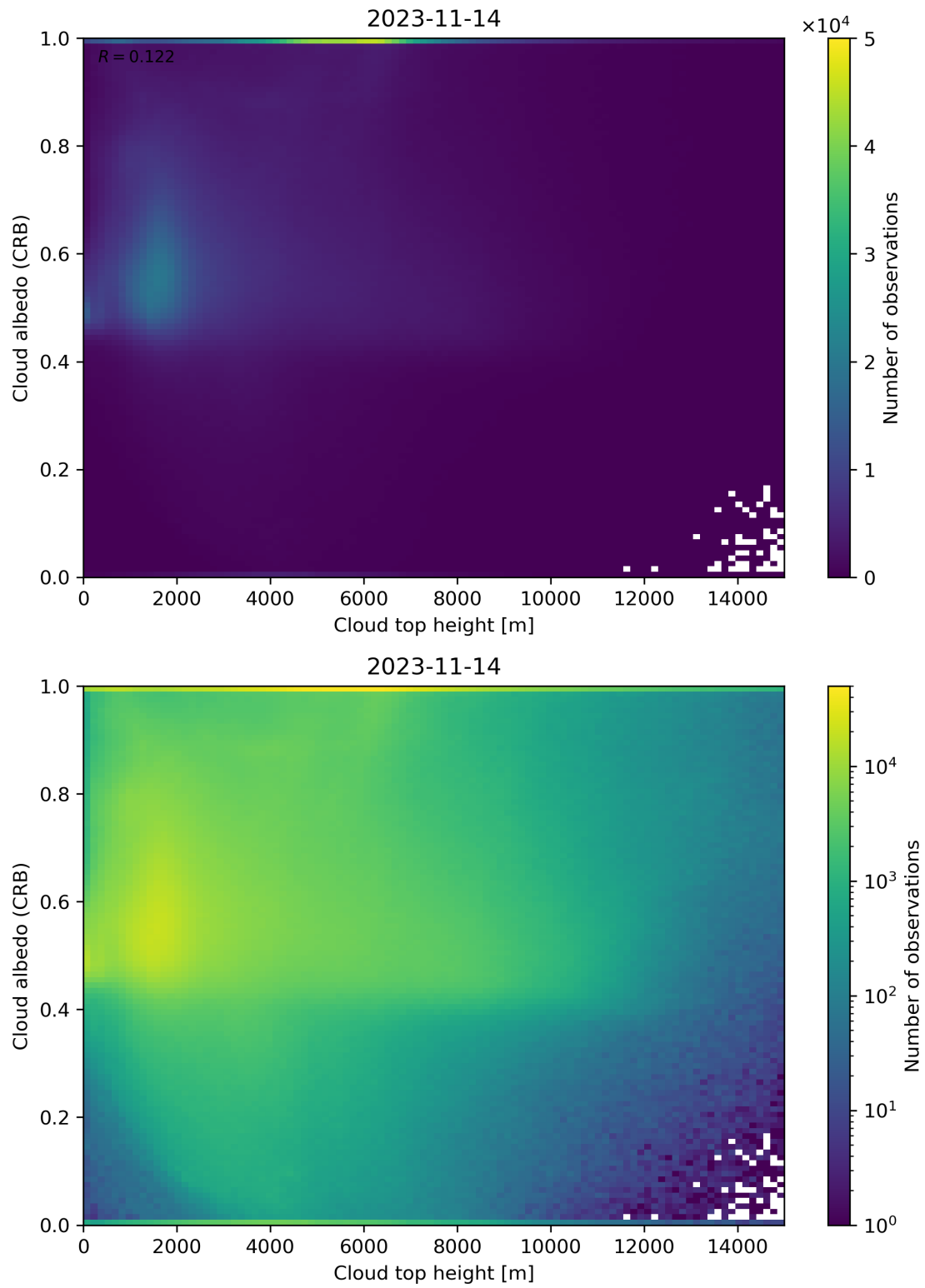
Figure 86: Scatter density plot of “Cloud top height” against “Cloud albedo (CRB)” for 2023-11-13 to 2023-11-15.
