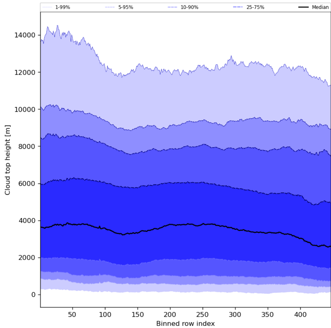
Figure 56: Along track statistics of “Cloud top height” for 2023-11-13 to 2023-11-15
