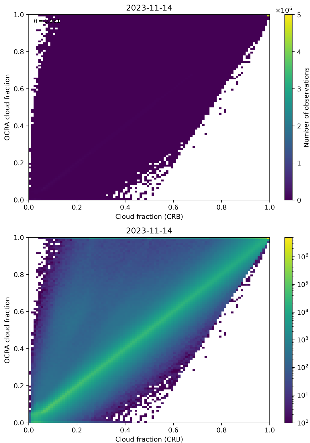
Figure 78: Scatter density plot of “Cloud fraction (CRB)” against “OCRA cloud fraction” for 2023-11-13 to 2023-11-15.
