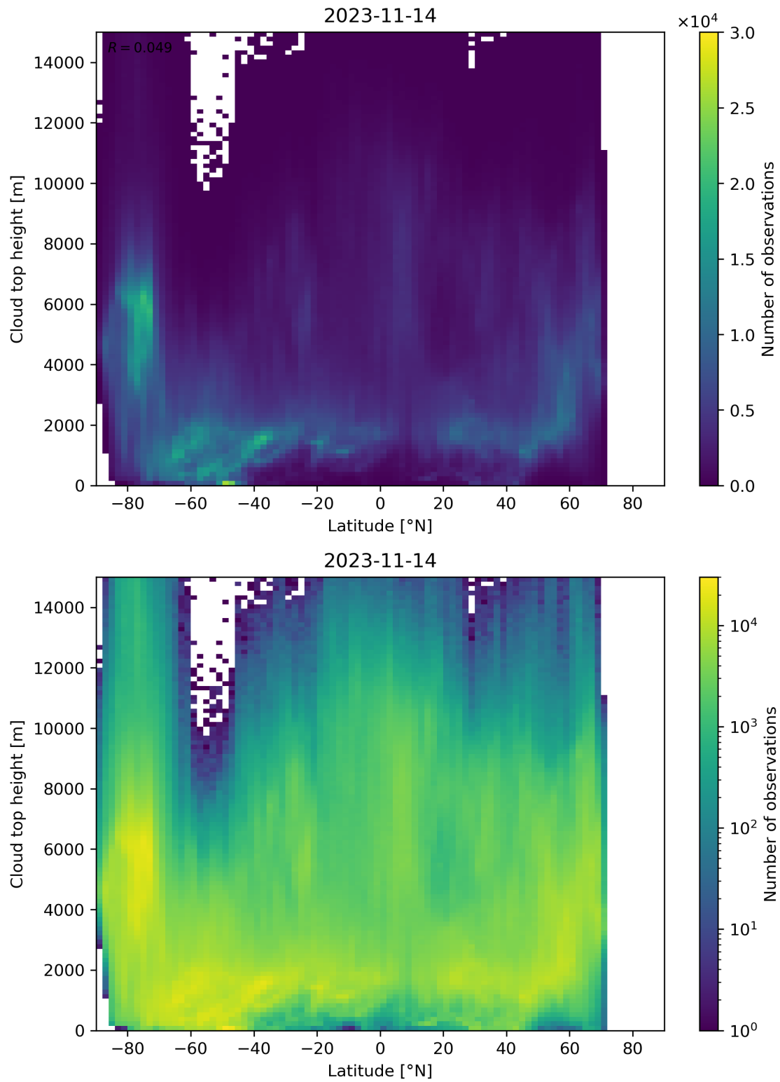
Figure 97: Scatter density plot of “Latitude” against “Cloud top height” for 2023-11-13 to 2023-11-15.
