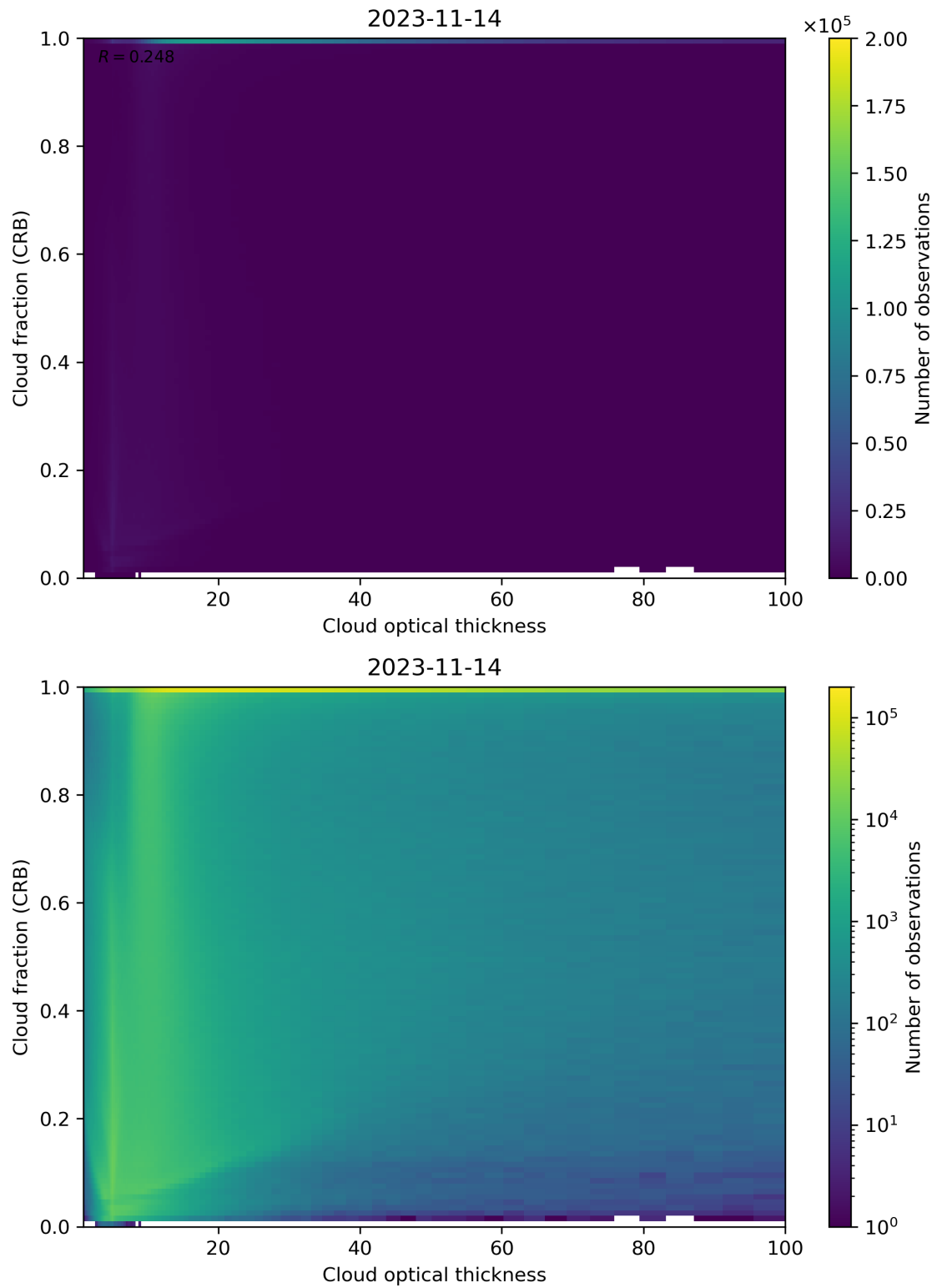
Figure 84: Scatter density plot of “Cloud optical thickness” against “Cloud fraction (CRB)” for 2023-11-13 to 2023-11-15.
