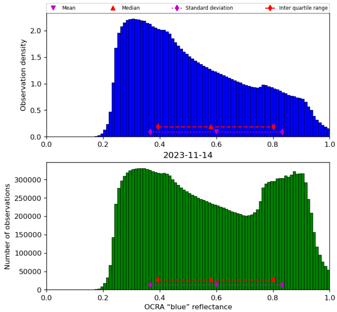
Figure 51: Histogram of “OCRA “blue” reflectance” for 2023-11-13 to 2023-11-15
