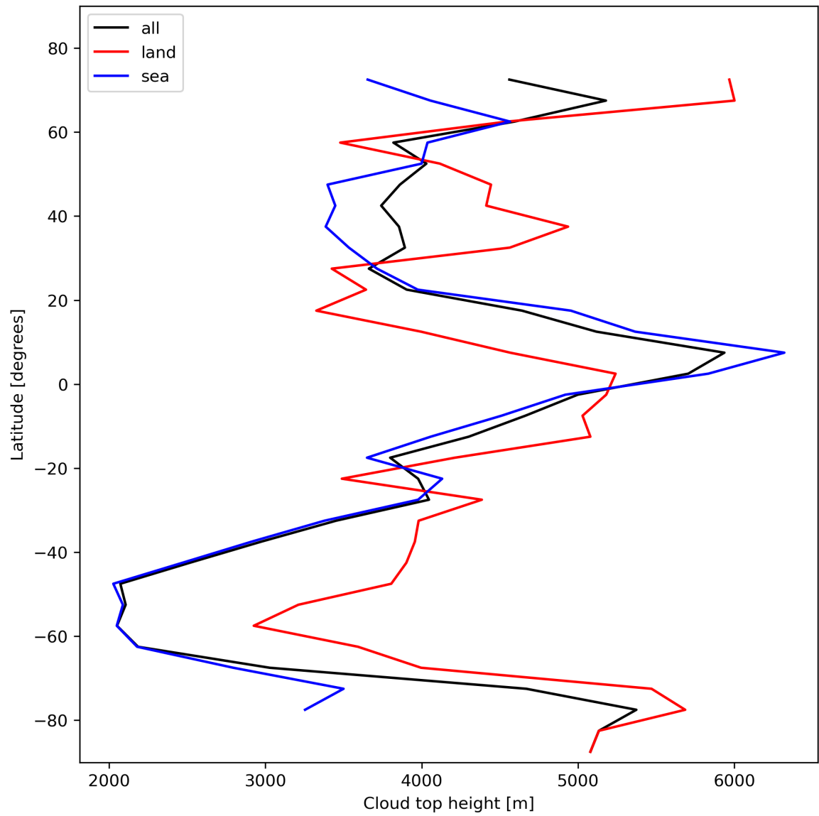
Figure 24: Zonal average of “Cloud top height” for 2023-11-13 to 2023-11-15.
