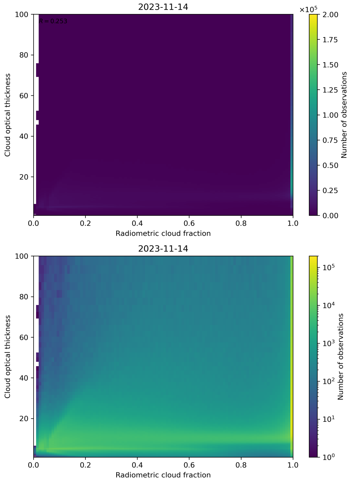
Figure 75: Scatter density plot of “Radiometric cloud fraction” against “Cloud optical thickness” for 2023-11-13 to 2023-11-15.
