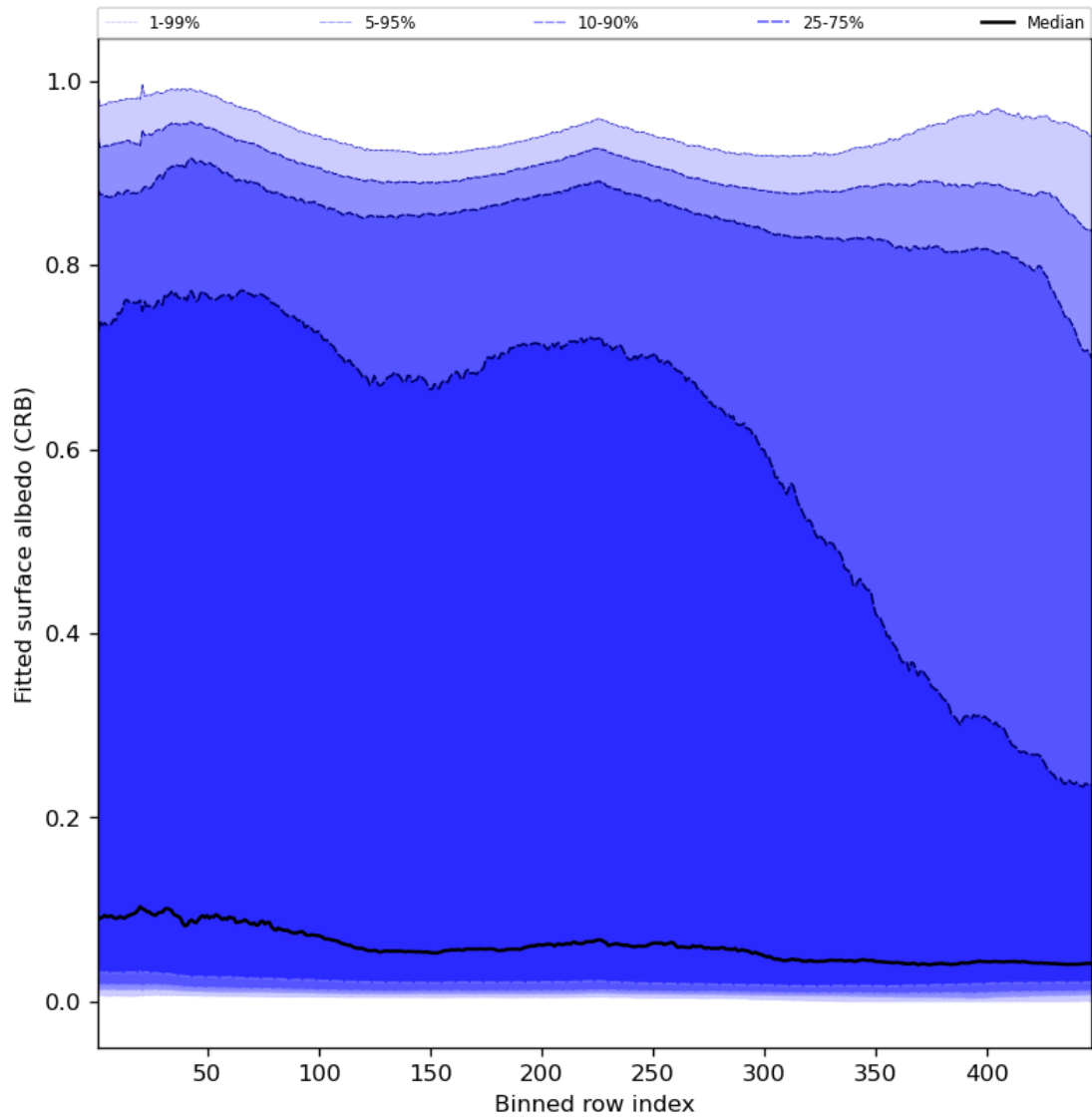
Figure 62: Along track statistics of “Fitted surface albedo (CRB)” for 2023-11-13 to 2023-11-15
