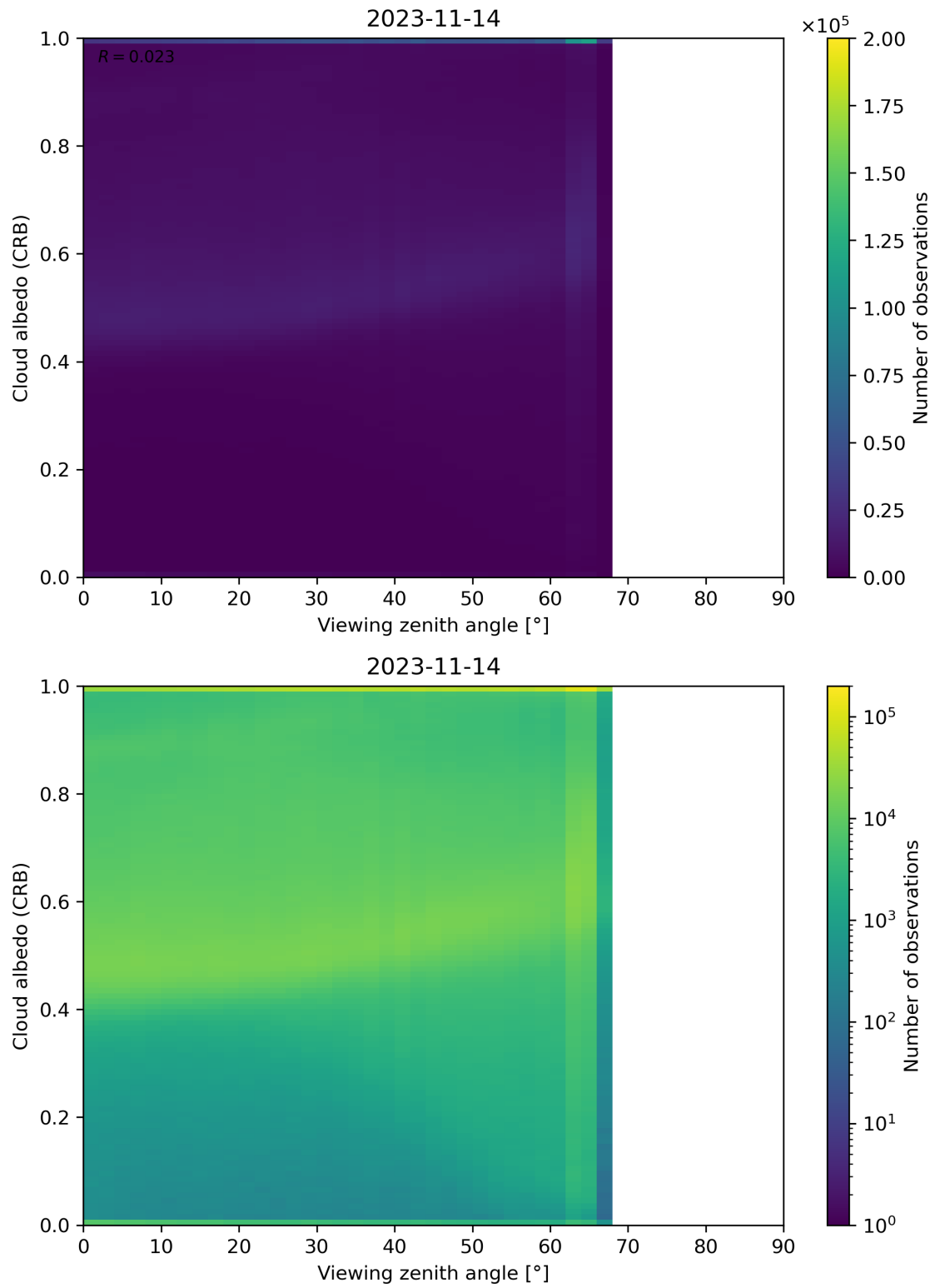
Figure 106: Scatter density plot of “Viewing zenith angle” against “Cloud albedo (CRB)” for 2023-11-13 to 2023-11-15.
