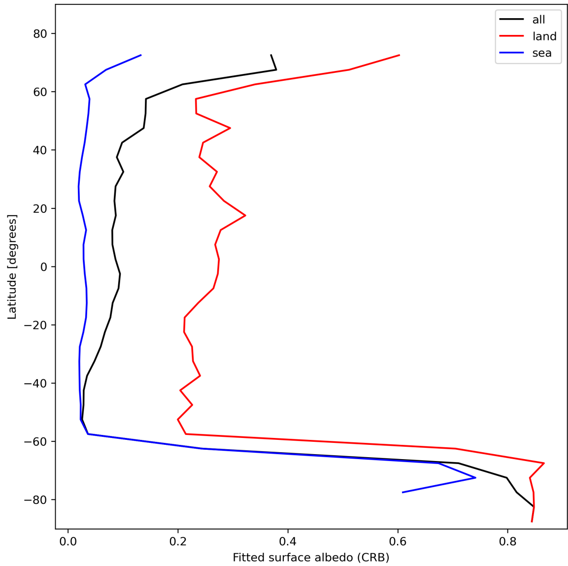
Figure 30: Zonal average of “Fitted surface albedo (CRB)” for 2023-11-13 to 2023-11-15.
