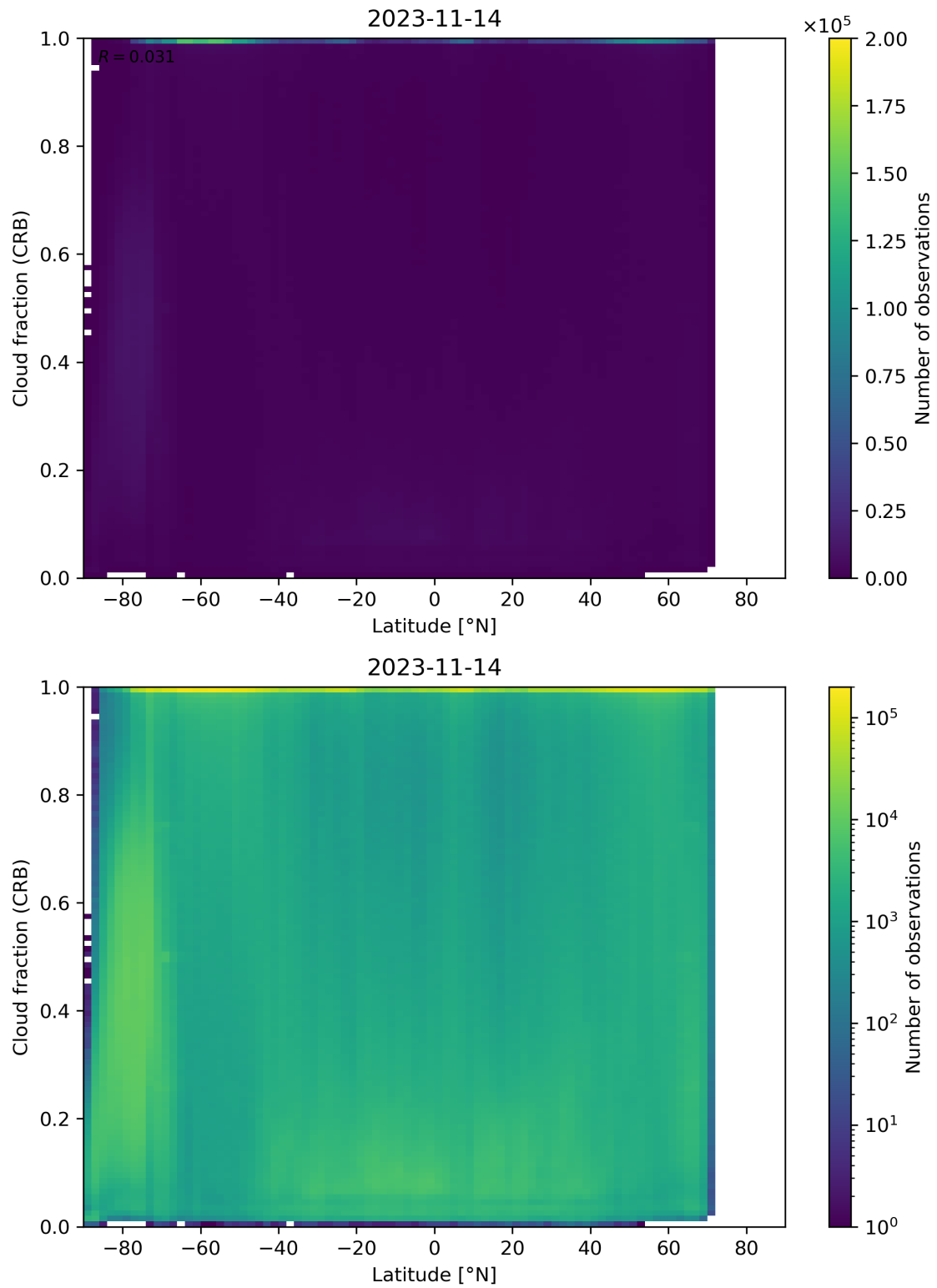
Figure 94: Scatter density plot of “Latitude” against “Cloud fraction (CRB)” for 2023-11-13 to 2023-11-15.
