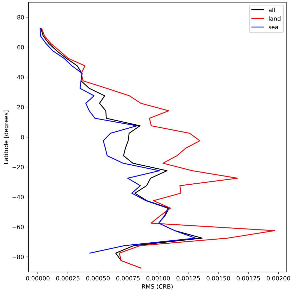
Figure 32: Zonal average of “RMS (CRB)” for 2023-11-13 to 2023-11-15.
