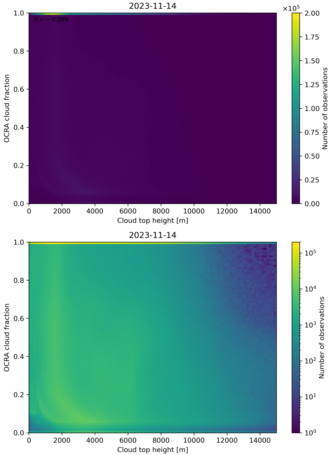
Figure 87: Scatter density plot of “Cloud top height” against “OCRA cloud fraction” for 2023-11-13 to 2023-11-15.
