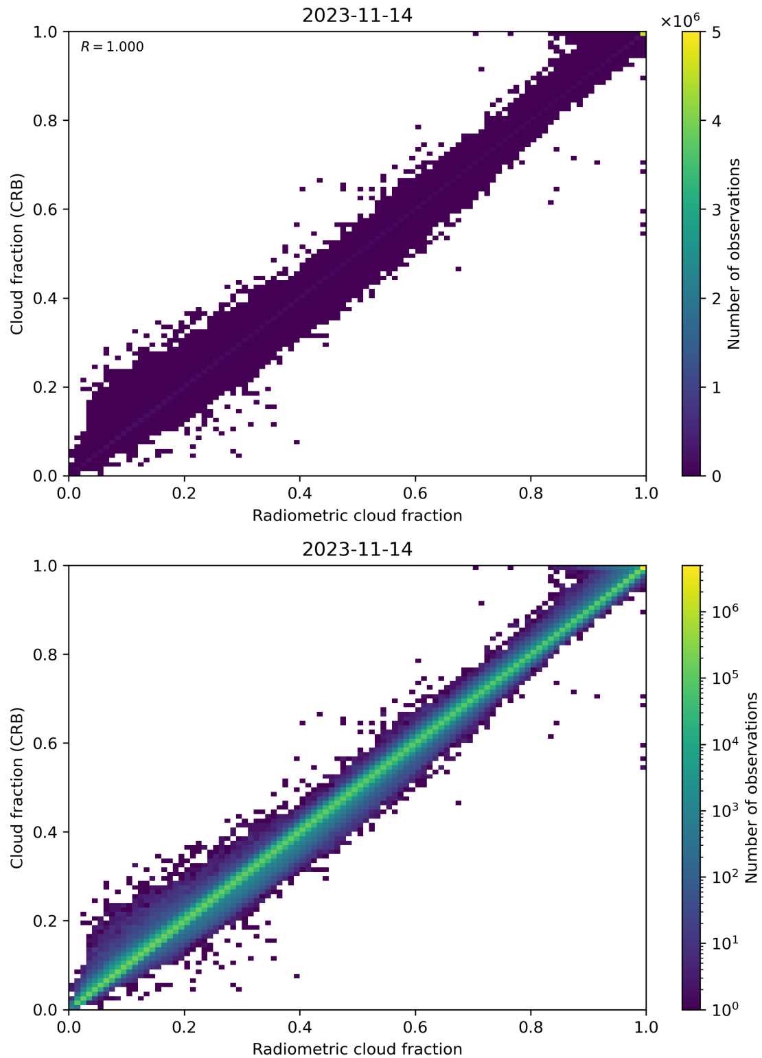
Figure 73: Scatter density plot of “Radiometric cloud fraction” against “Cloud fraction (CRB)” for 2023-11-13 to 2023-11-15.
