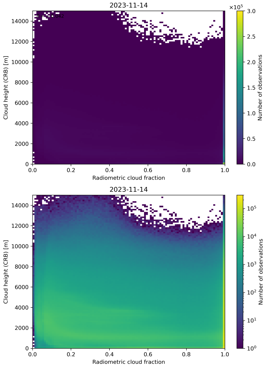
Figure 74: Scatter density plot of “Radiometric cloud fraction” against “Cloud height (CRB)” for 2023-11-13 to 2023-11-15.
