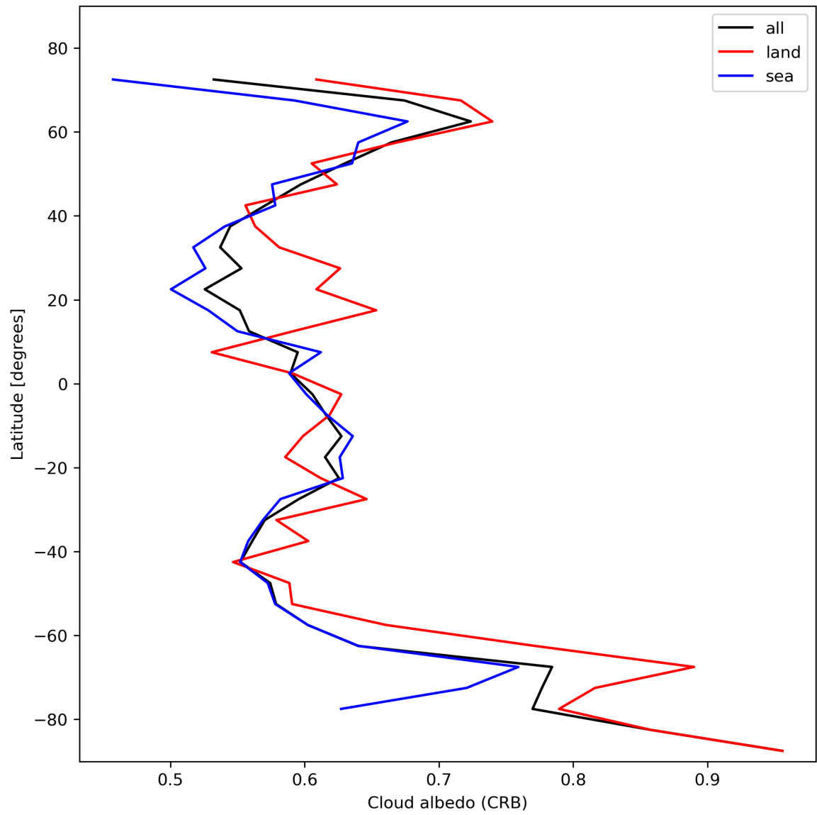
Figure 28: Zonal average of “Cloud albedo (CRB)” for 2023-11-13 to 2023-11-15.
