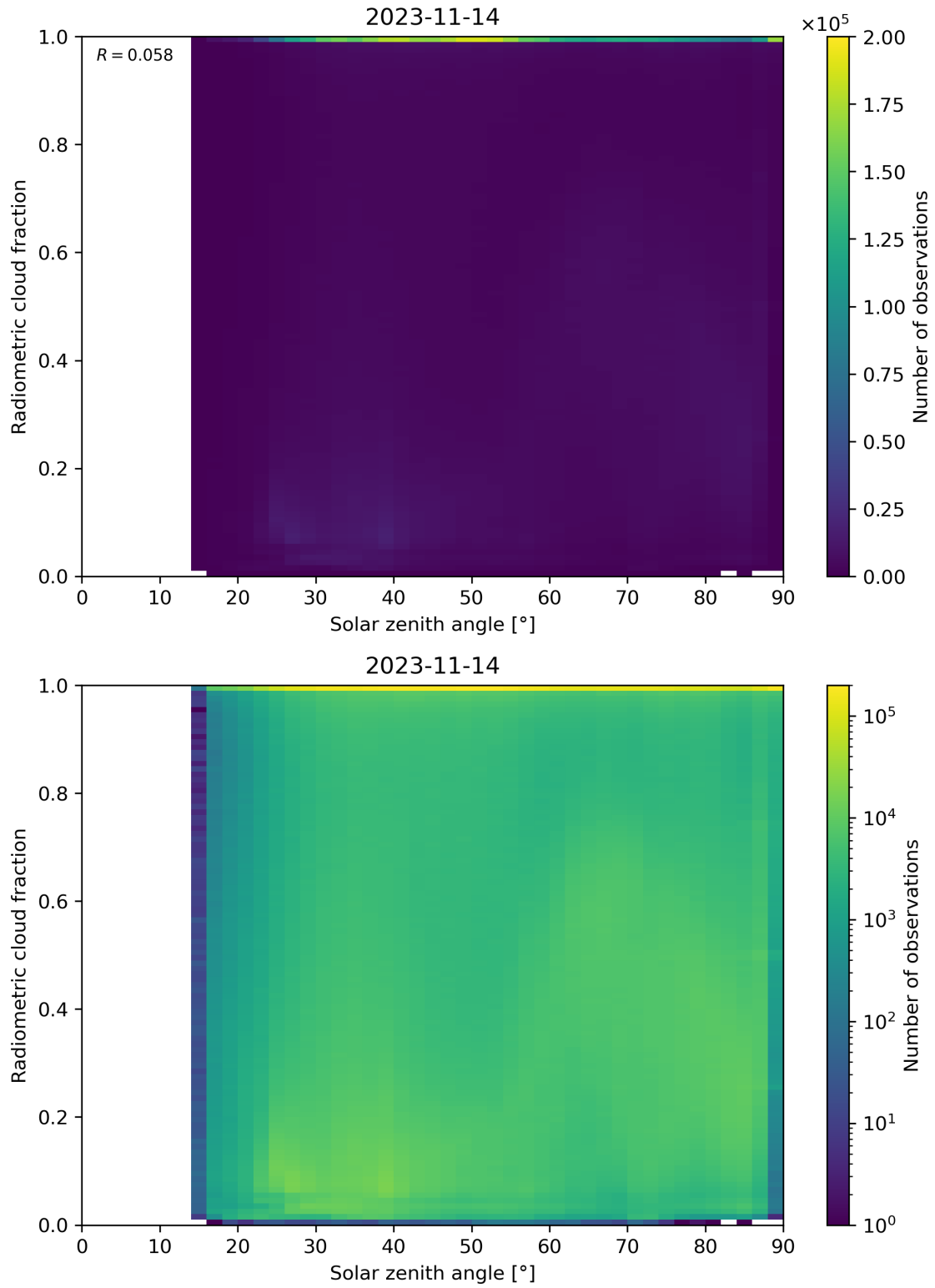
Figure 99: Scatter density plot of “Solar zenith angle” against “Radiometric cloud fraction” for 2023-11-13 to 2023-11-15.
