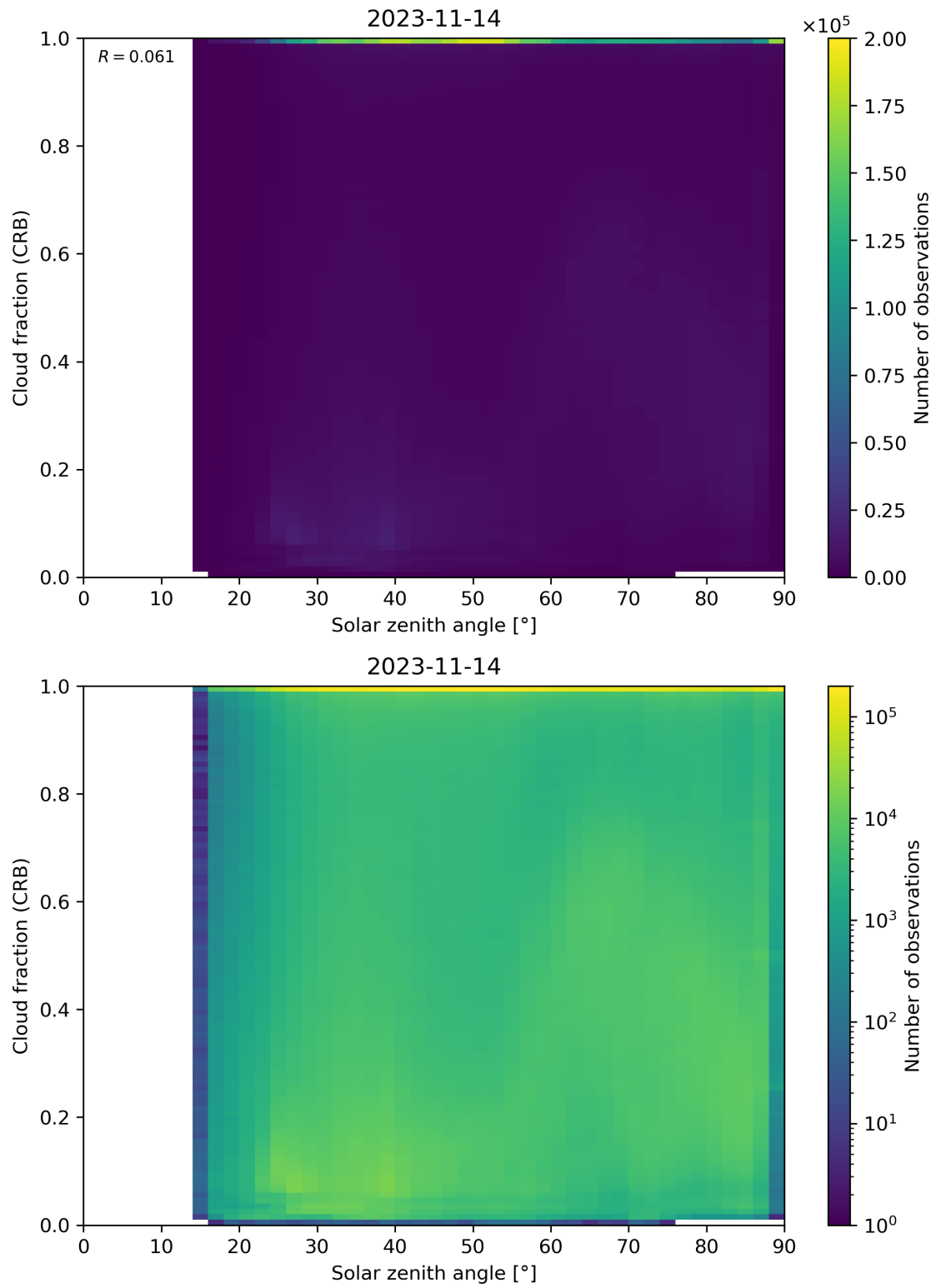
Figure 101: Scatter density plot of “Solar zenith angle” against “Cloud fraction (CRB)” for 2023-11-13 to 2023-11-15.
