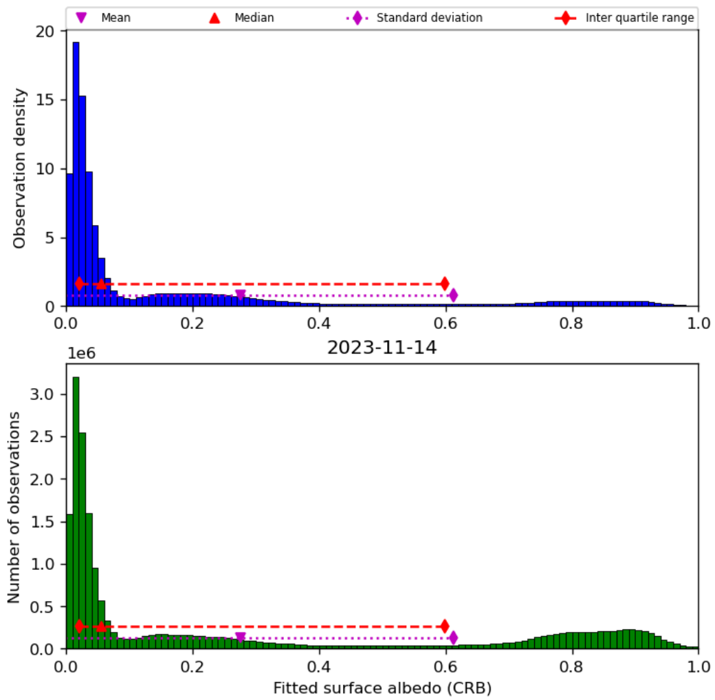
Figure 46: Histogram of “Fitted surface albedo (CRB)” for 2023-11-13 to 2023-11-15
