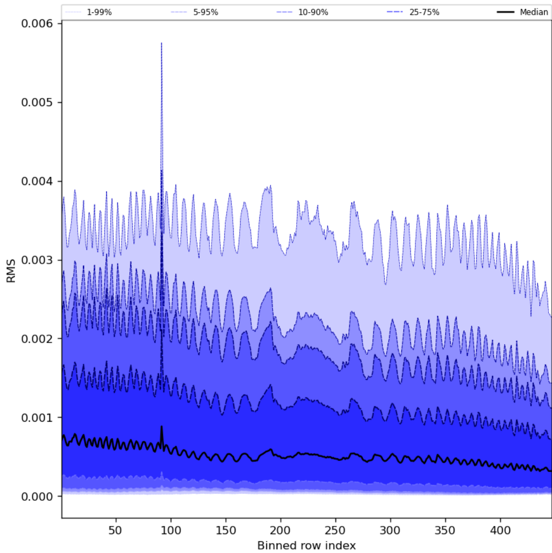
Figure 63: Along track statistics of “RMS” for 2023-11-13 to 2023-11-15
