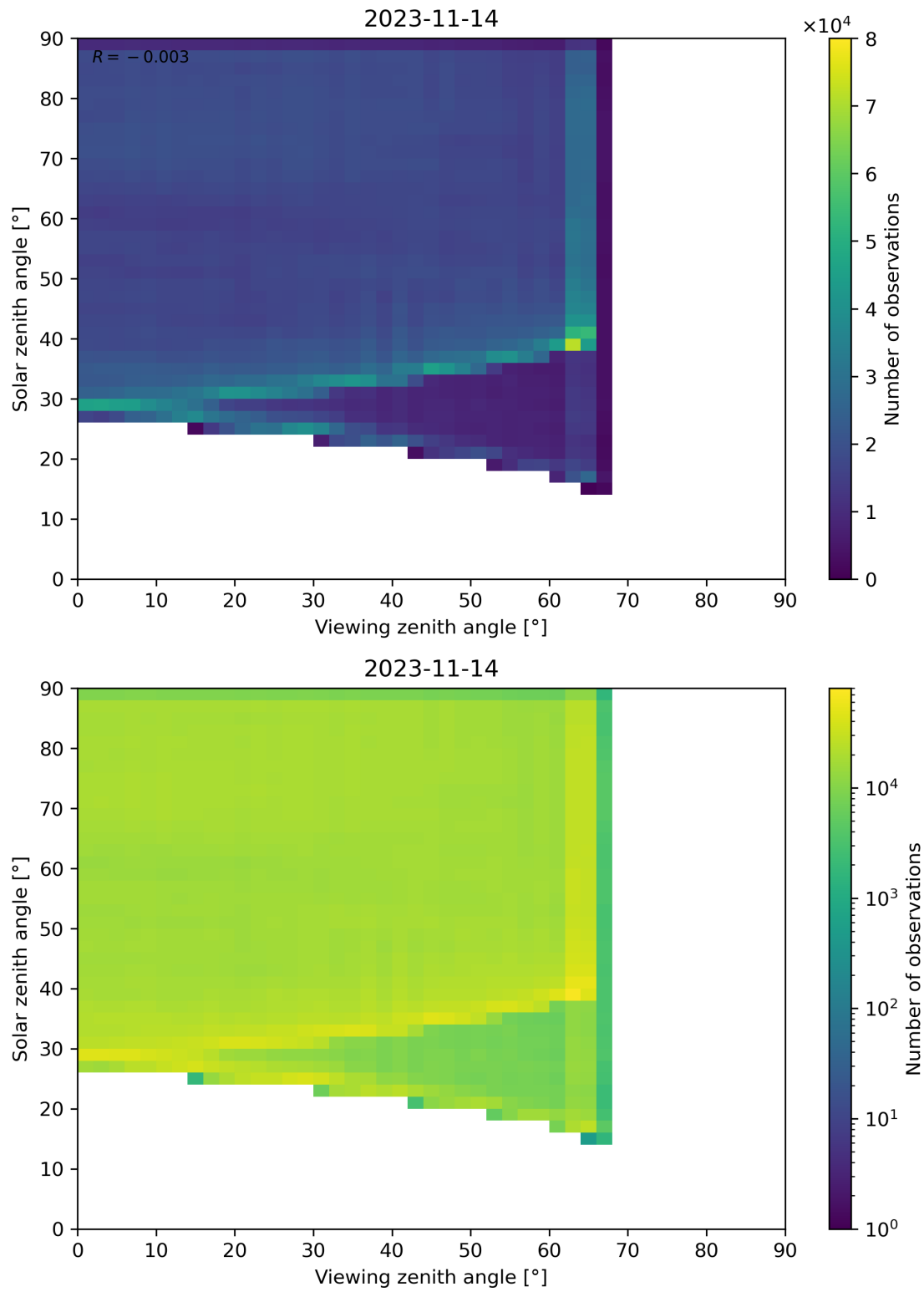
Figure 114: Scatter density plot of “Viewing zenith angle” against “Solar zenith angle” for 2023-11-13 to 2023-11-15.
