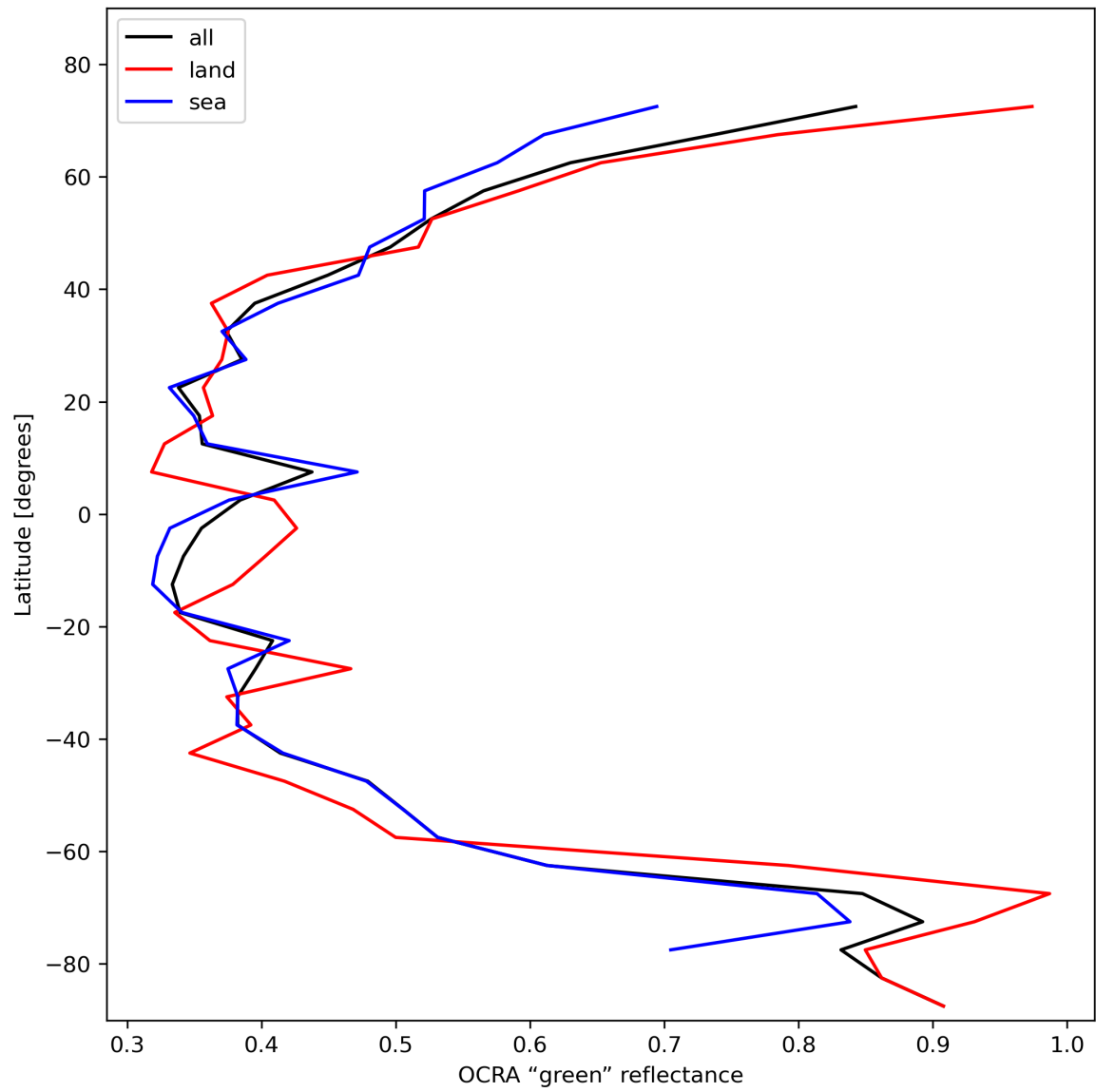
Figure 36: Zonal average of “OCRA “green” reflectance” for 2023-11-13 to 2023-11-15.
