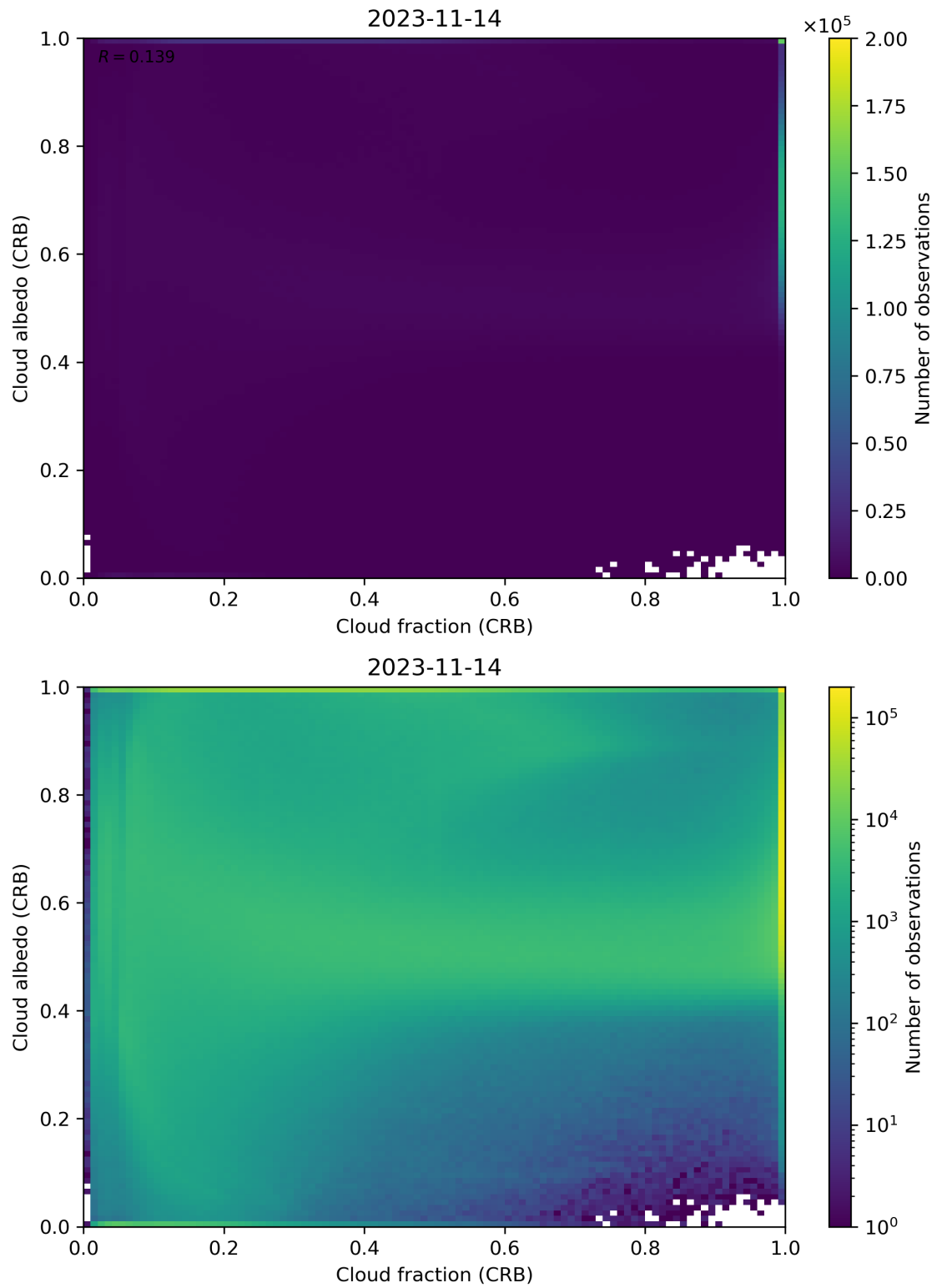
Figure 77: Scatter density plot of “Cloud fraction (CRB)” against “Cloud albedo (CRB)” for 2023-11-13 to 2023-11-15.
