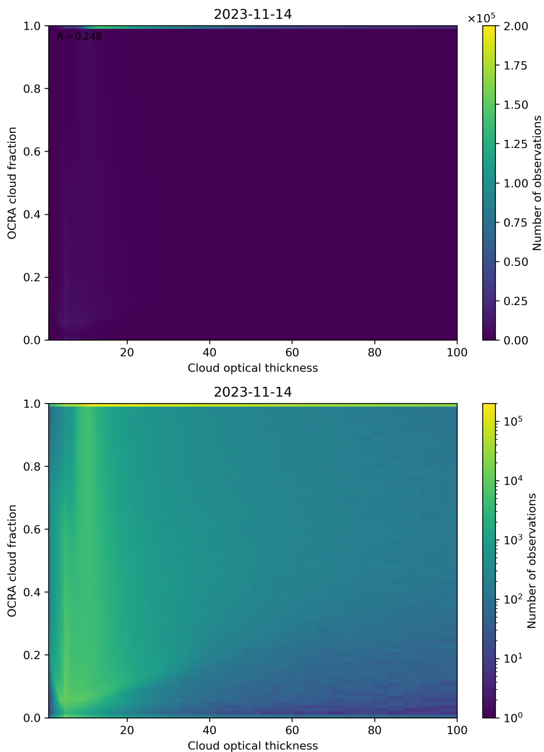
Figure 83: Scatter density plot of “Cloud optical thickness” against “OCRA cloud fraction” for 2023-11-13 to 2023-11-15.
