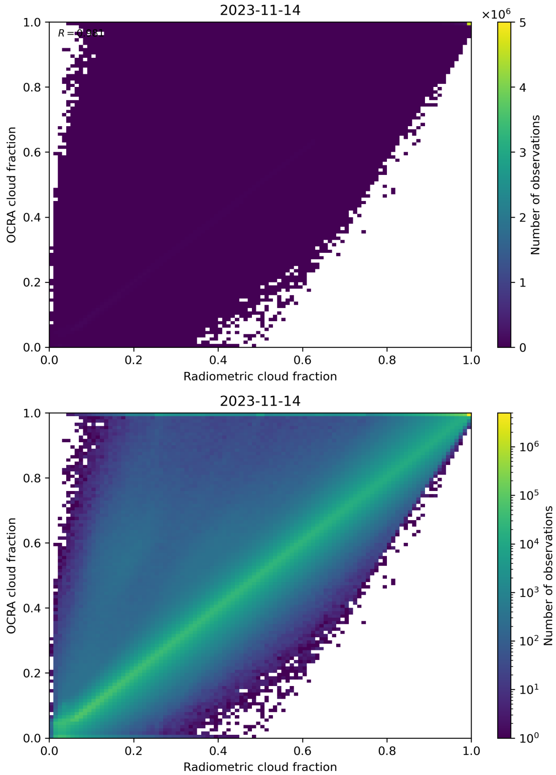
Figure 72: Scatter density plot of “Radiometric cloud fraction” against “OCRA cloud fraction” for 2023-11-13 to 2023-11-15.
