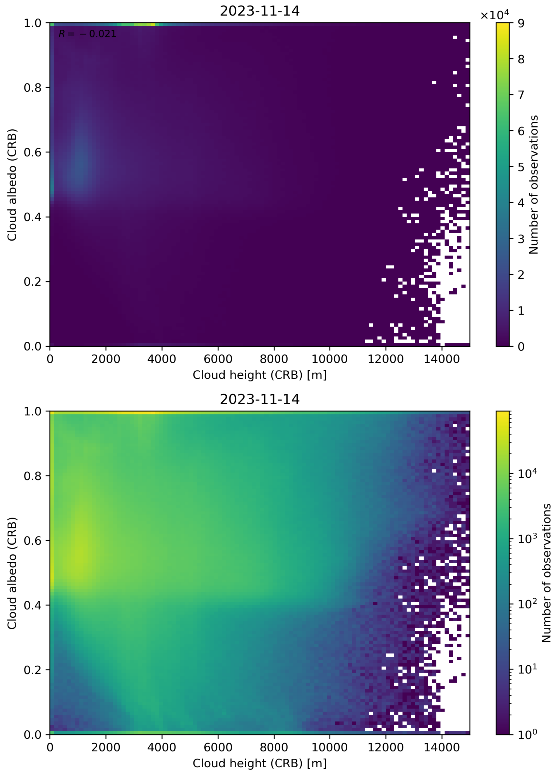
Figure 80: Scatter density plot of “Cloud height (CRB)” against “Cloud albedo (CRB)” for 2023-11-13 to 2023-11-15.
