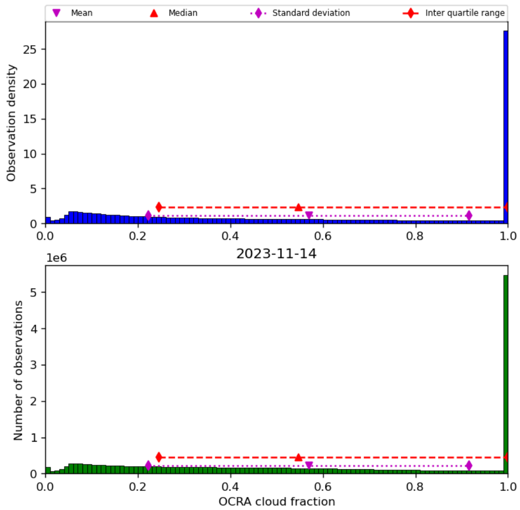
Figure 50: Histogram of “OCRA cloud fraction” for 2023-11-13 to 2023-11-15
