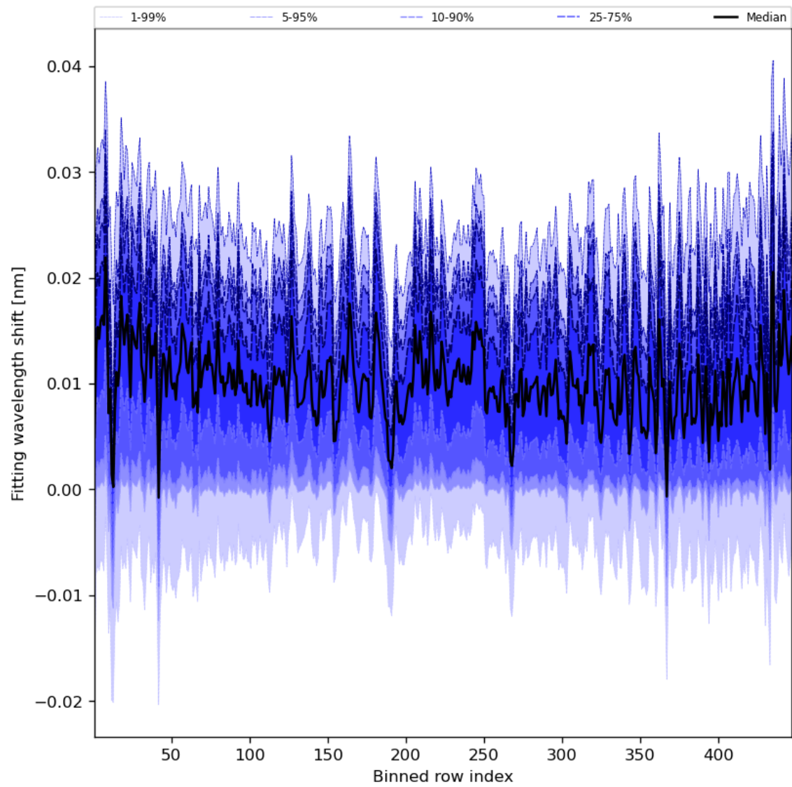
Figure 65: Along track statistics of “Fitting wavelength shift” for 2023-11-13 to 2023-11-15
