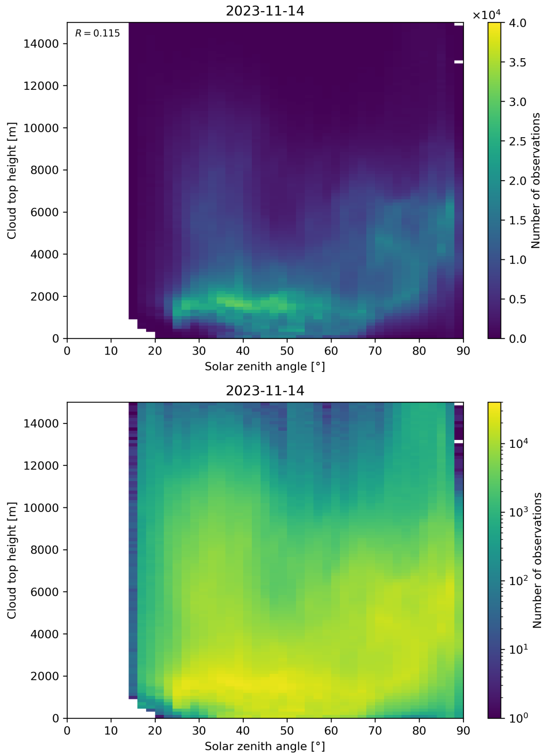
Figure 104: Scatter density plot of “Solar zenith angle” against “Cloud top height” for 2023-11-13 to 2023-11-15.
