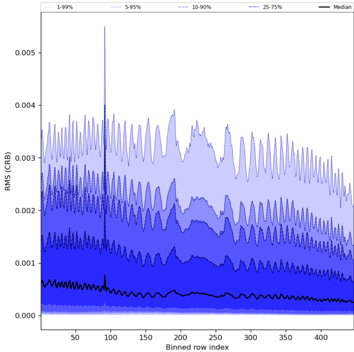
Figure 64: Along track statistics of “RMS (CRB)” for 2023-11-13 to 2023-11-15
