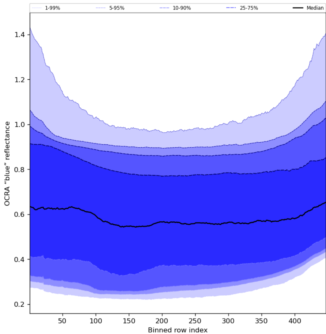
Figure 67: Along track statistics of “OCRA “blue” reflectance” for 2023-11-13 to 2023-11-15
