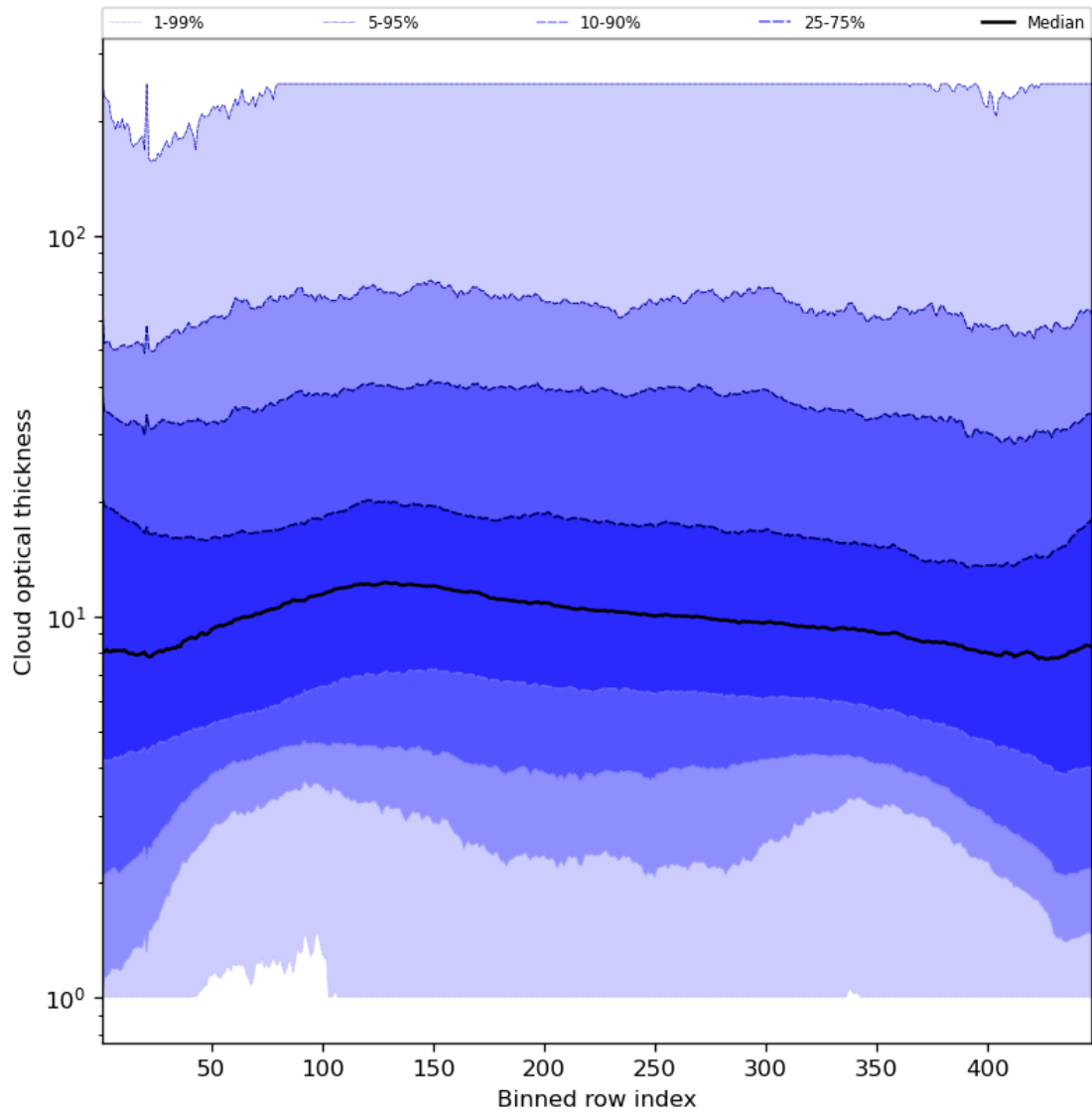
Figure 57: Along track statistics of “Cloud optical thickness” for 2023-11-13 to 2023-11-15
