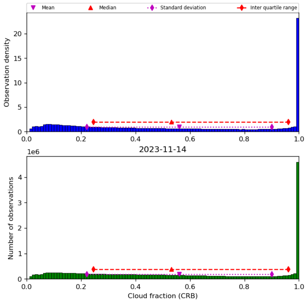
Figure 42: Histogram of “Cloud fraction (CRB)” for 2023-11-13 to 2023-11-15
