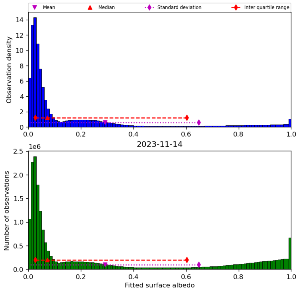
Figure 45: Histogram of “Fitted surface albedo” for 2023-11-13 to 2023-11-15
