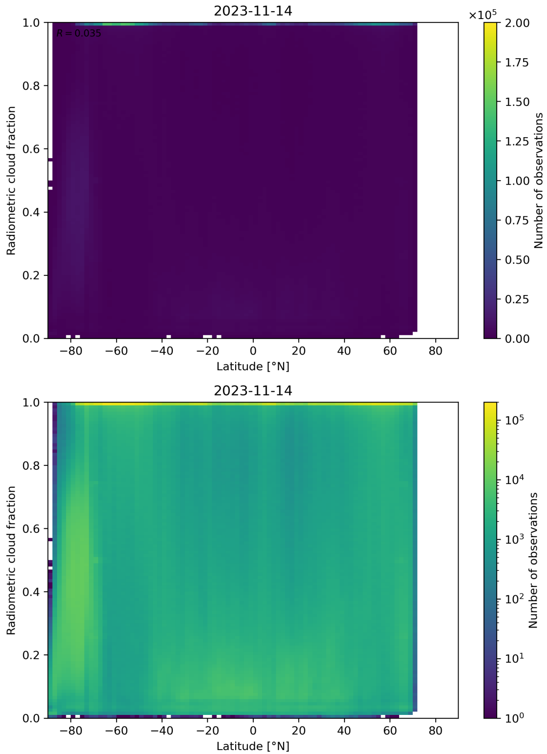
Figure 92: Scatter density plot of “Latitude” against “Radiometric cloud fraction” for 2023-11-13 to 2023-11-15.
