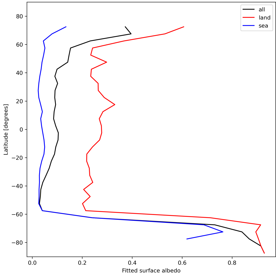
Figure 29: Zonal average of “Fitted surface albedo” for 2023-11-13 to 2023-11-15.
