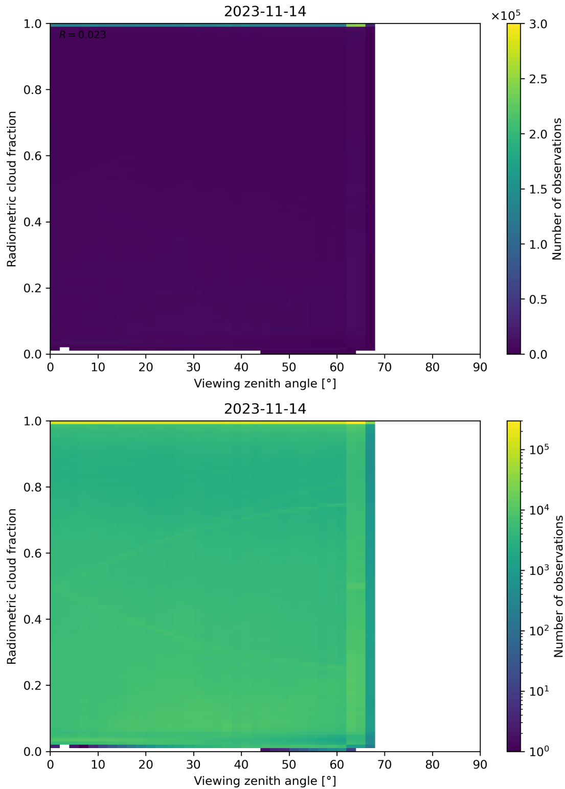
Figure 107: Scatter density plot of “Viewing zenith angle” against “Radiometric cloud fraction” for 2023-11-13 to 2023-11-15.
