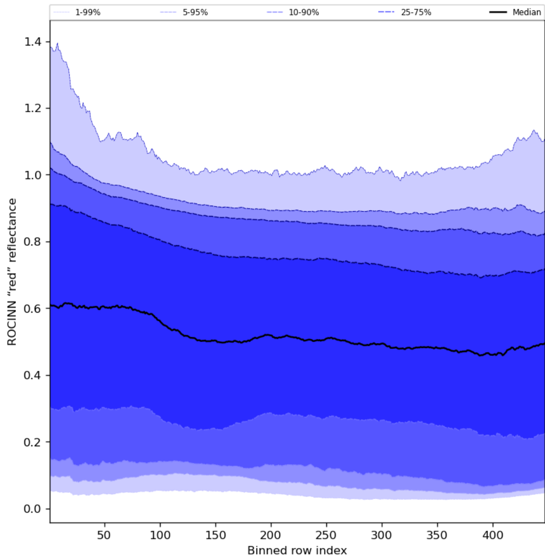
Figure 69: Along track statistics of “ROCINN “red” reflectance” for 2023-11-13 to 2023-11-15
