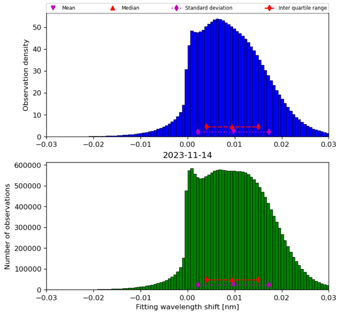
Figure 49: Histogram of “Fitting wavelength shift” for 2023-11-13 to 2023-11-15
