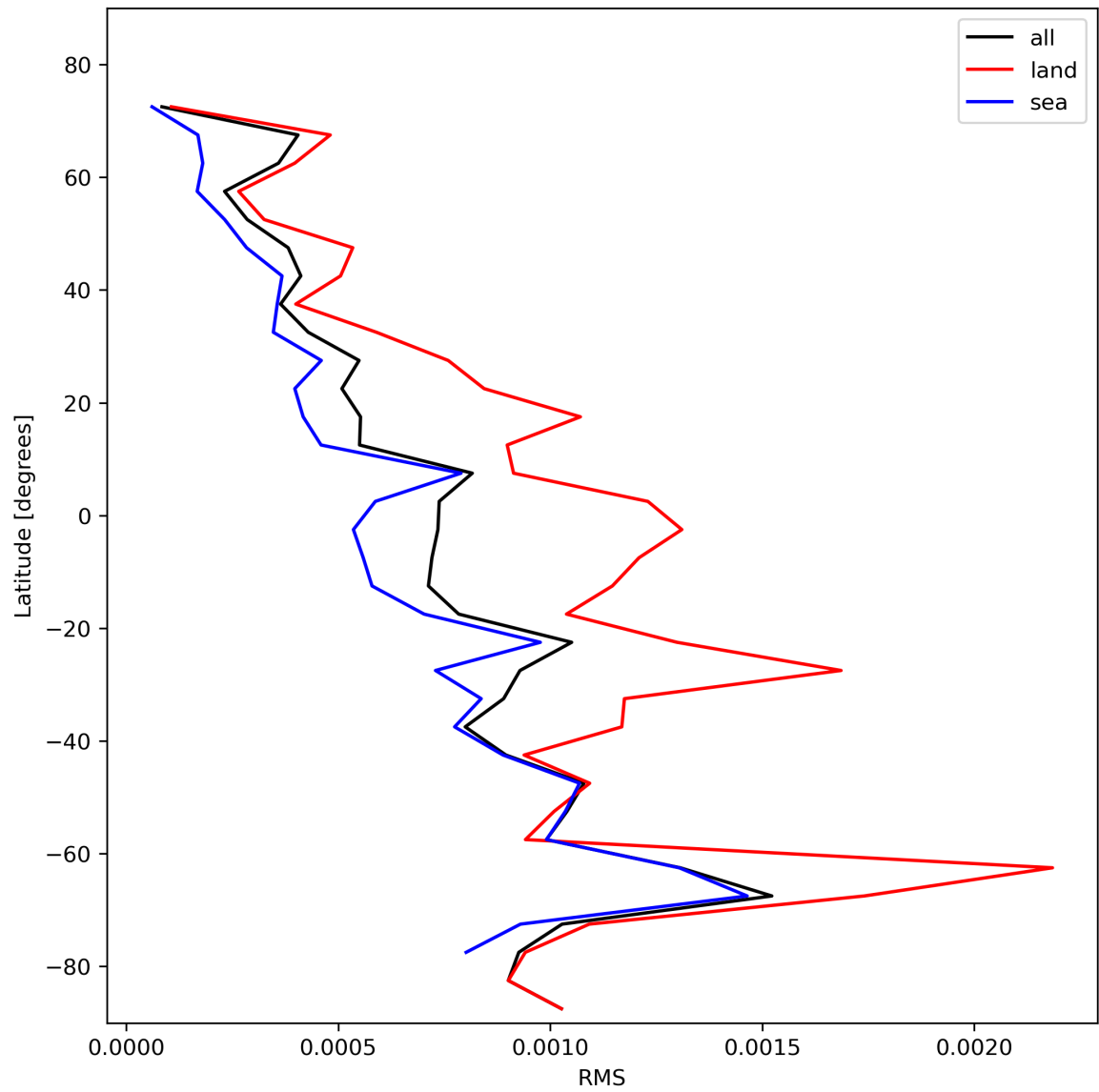
Figure 31: Zonal average of “RMS” for 2023-11-13 to 2023-11-15.
