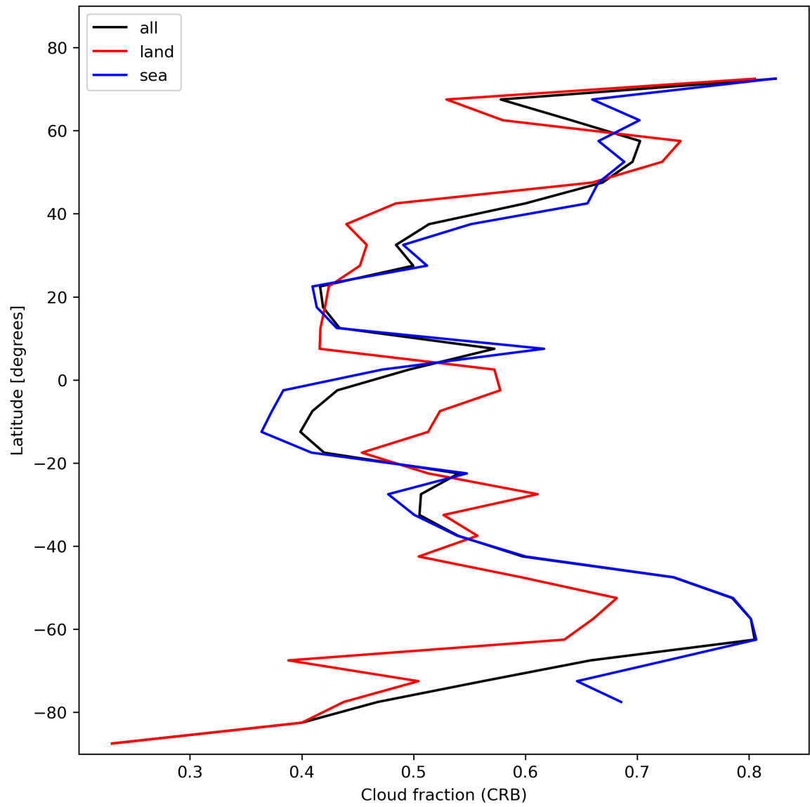
Figure 26: Zonal average of “Cloud fraction (CRB)” for 2023-11-13 to 2023-11-15.
