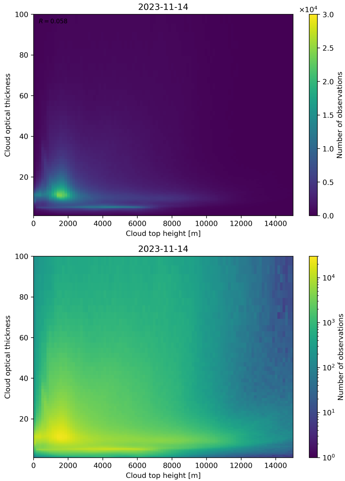
Figure 90: Scatter density plot of “Cloud top height” against “Cloud optical thickness” for 2023-11-13 to 2023-11-15.
