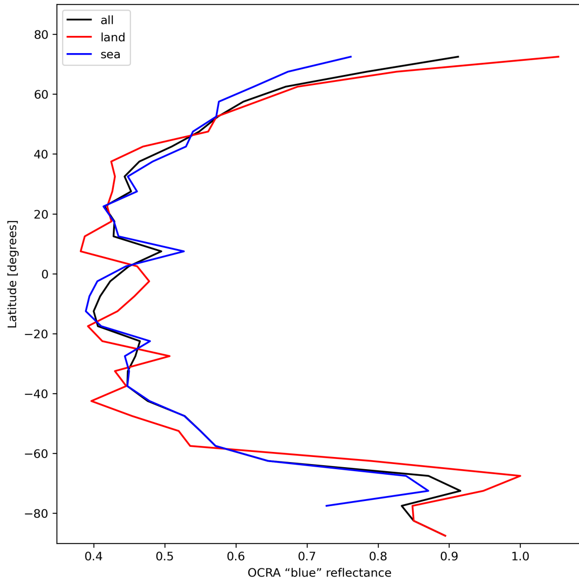
Figure 35: Zonal average of “OCRA “blue” reflectance” for 2023-11-13 to 2023-11-15.
