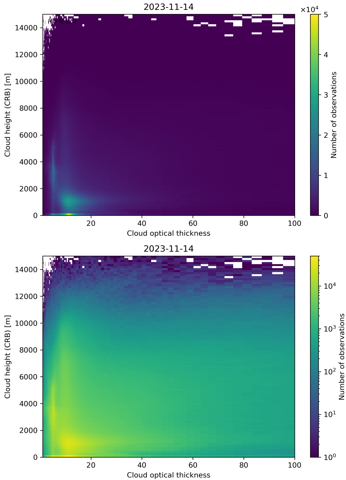
Figure 85: Scatter density plot of “Cloud optical thickness” against “Cloud height (CRB)” for 2023-11-13 to 2023-11-15.
