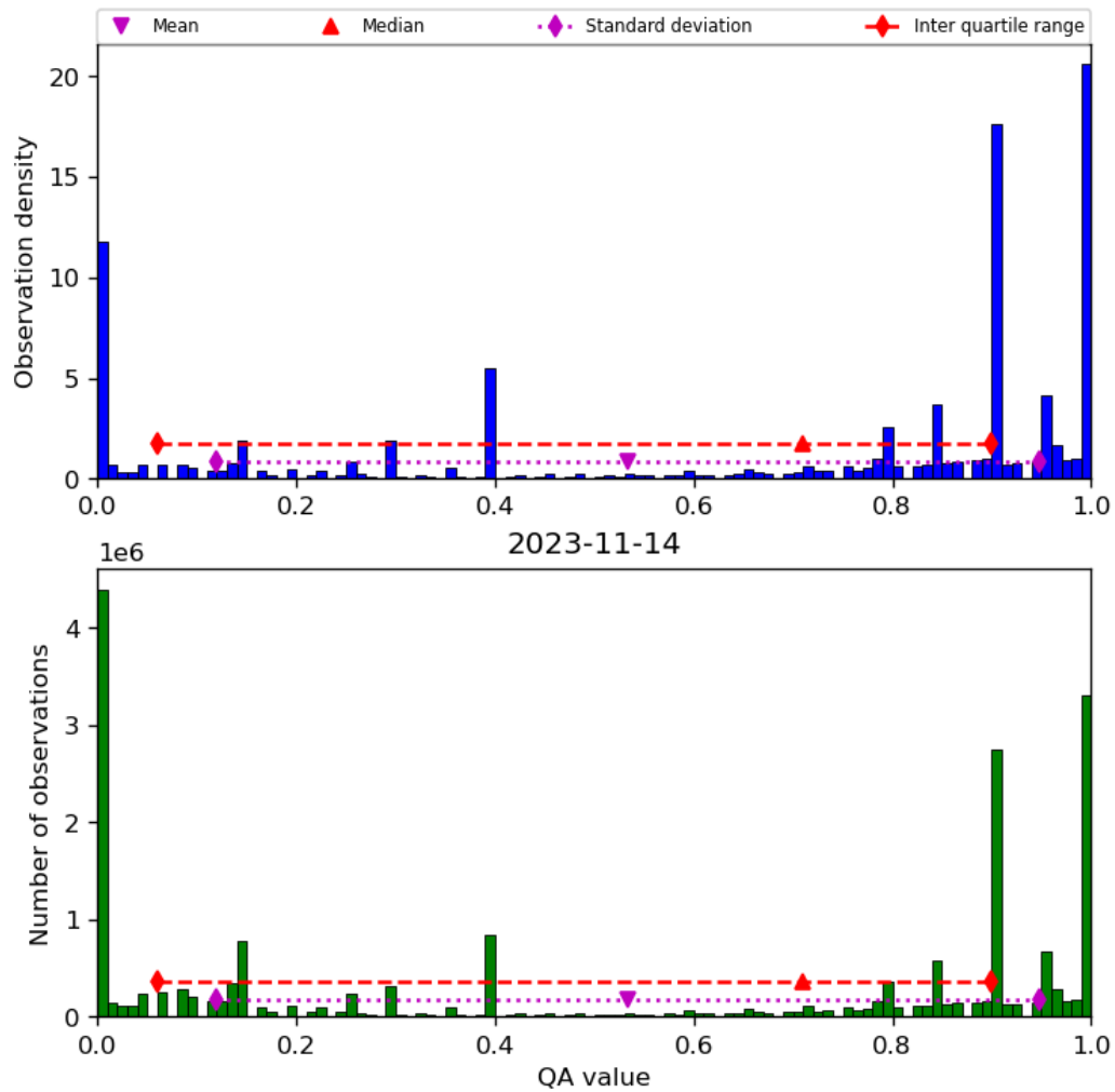
Figure 38: Histogram of “QA value” for 2023-11-13 to 2023-11-15
