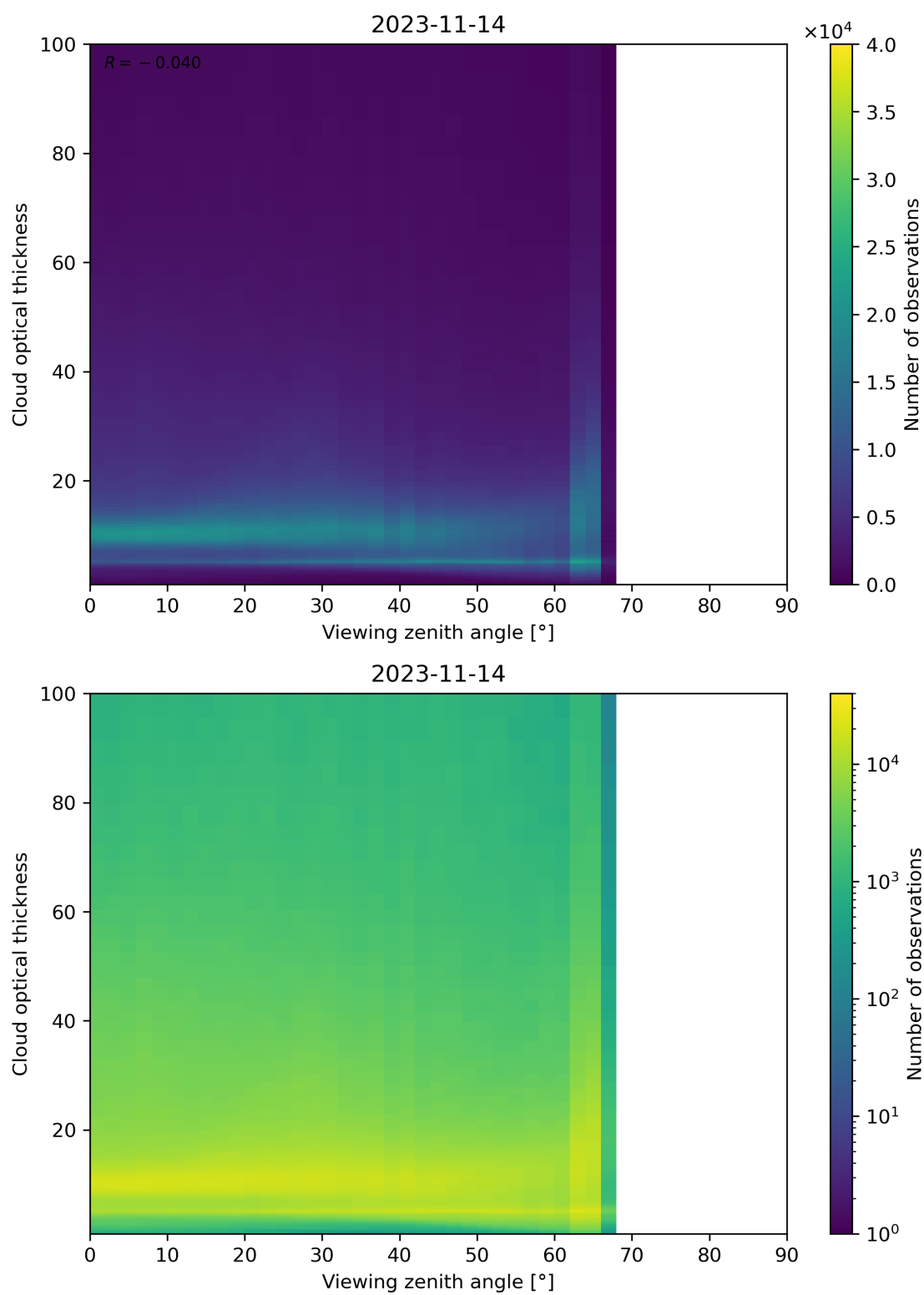
Figure 111: Scatter density plot of “Viewing zenith angle” against “Cloud optical thickness” for 2023-11-13 to 2023-11-15.
