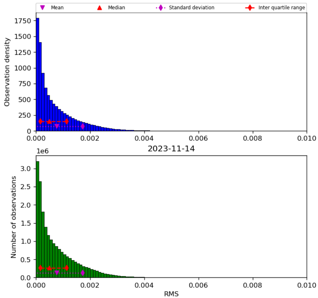
Figure 47: Histogram of “RMS” for 2023-11-13 to 2023-11-15
