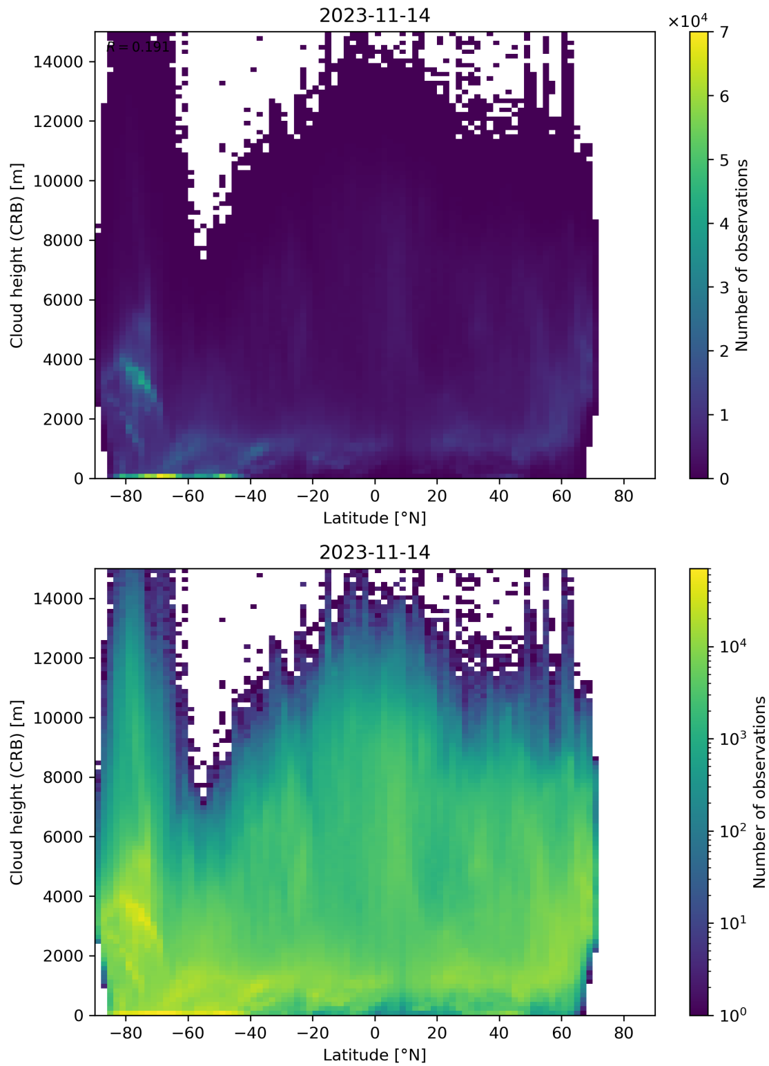
Figure 95: Scatter density plot of “Latitude” against “Cloud height (CRB)” for 2023-11-13 to 2023-11-15.
