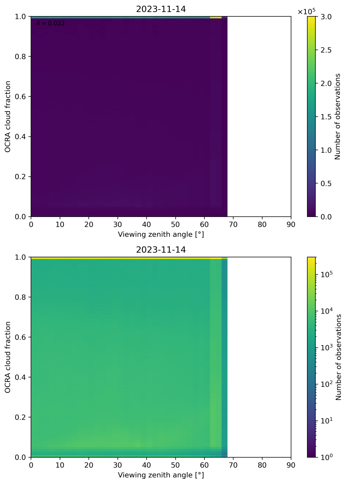
Figure 108: Scatter density plot of “Viewing zenith angle” against “OCRA cloud fraction” for 2023-11-13 to 2023-11-15.
