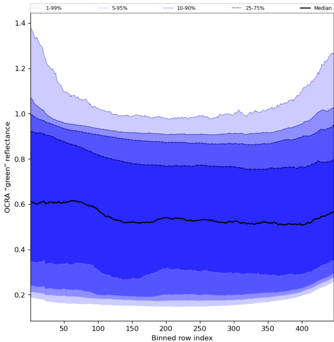
Figure 68: Along track statistics of “OCRA “green” reflectance” for 2023-11-13 to 2023-11-15
