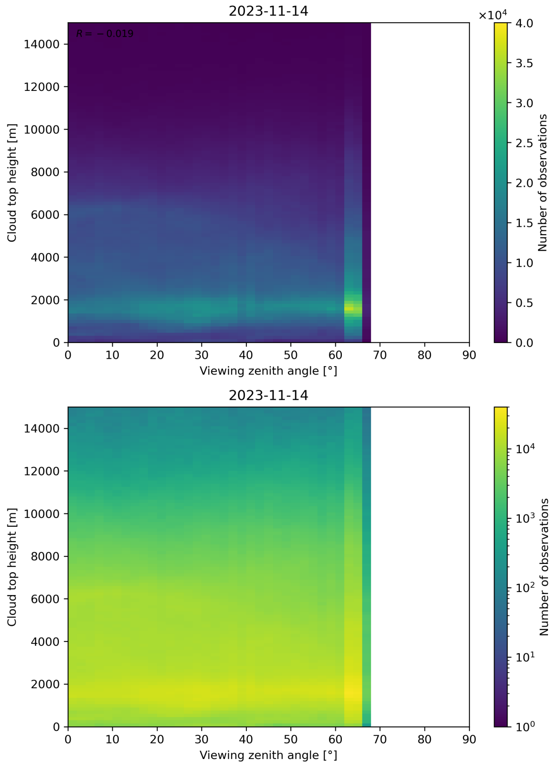
Figure 112: Scatter density plot of “Viewing zenith angle” against “Cloud top height” for 2023-11-13 to 2023-11-15.
