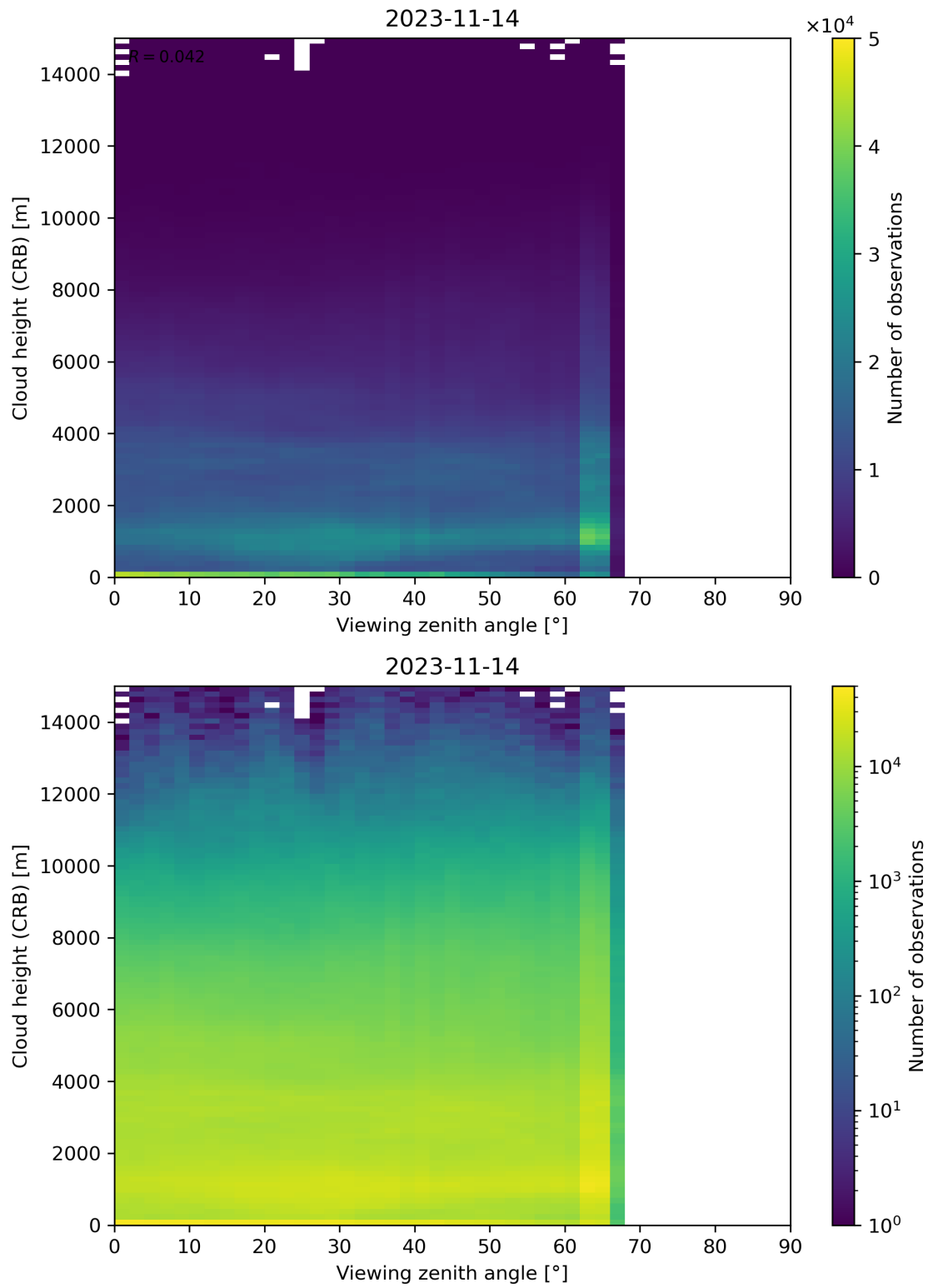
Figure 110: Scatter density plot of “Viewing zenith angle” against “Cloud height (CRB)” for 2023-11-13 to 2023-11-15.
