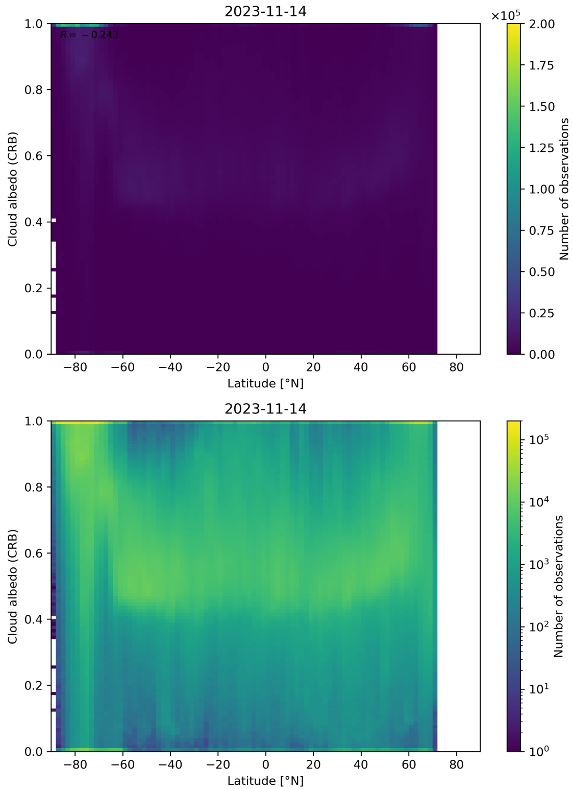
Figure 91: Scatter density plot of “Latitude” against “Cloud albedo (CRB)” for 2023-11-13 to 2023-11-15.
