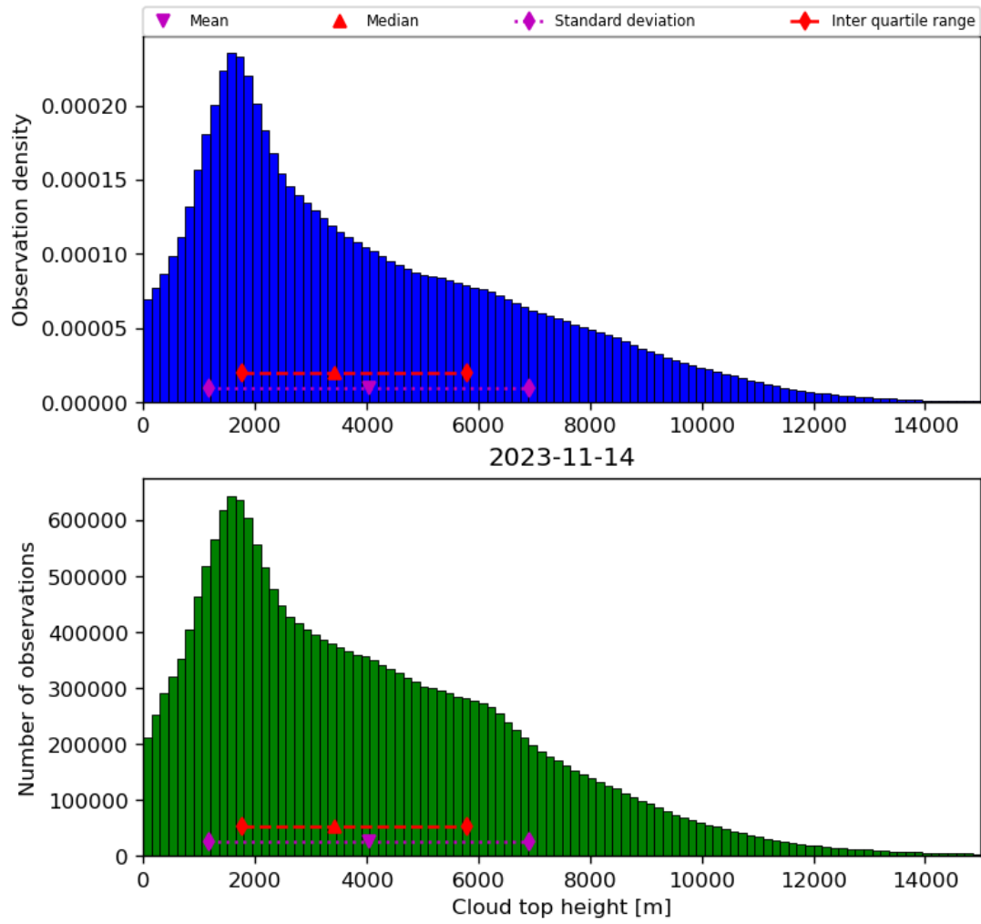
Figure 40: Histogram of “Cloud top height” for 2023-11-13 to 2023-11-15
