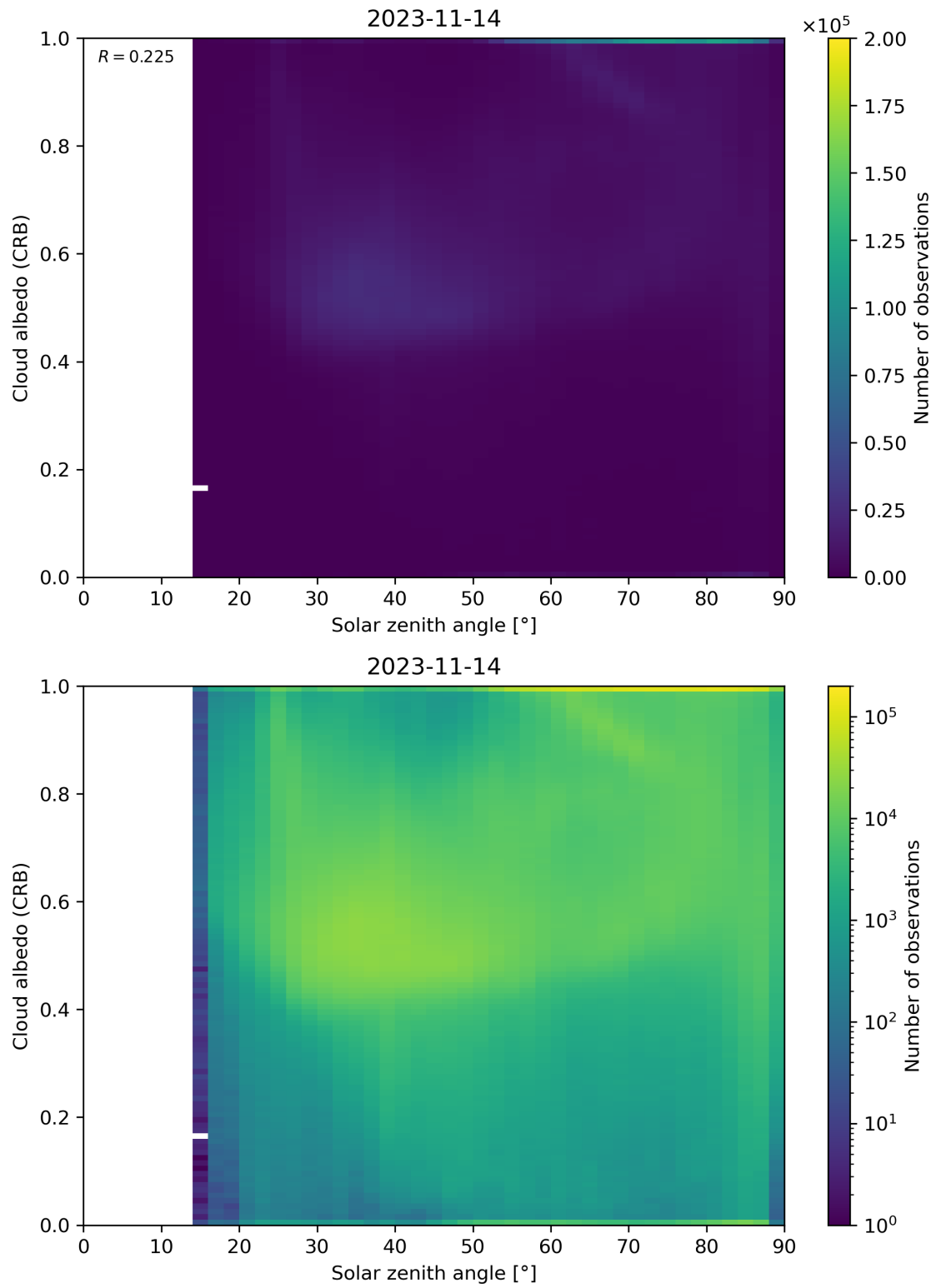
Figure 98: Scatter density plot of “Solar zenith angle” against “Cloud albedo (CRB)” for 2023-11-13 to 2023-11-15.
