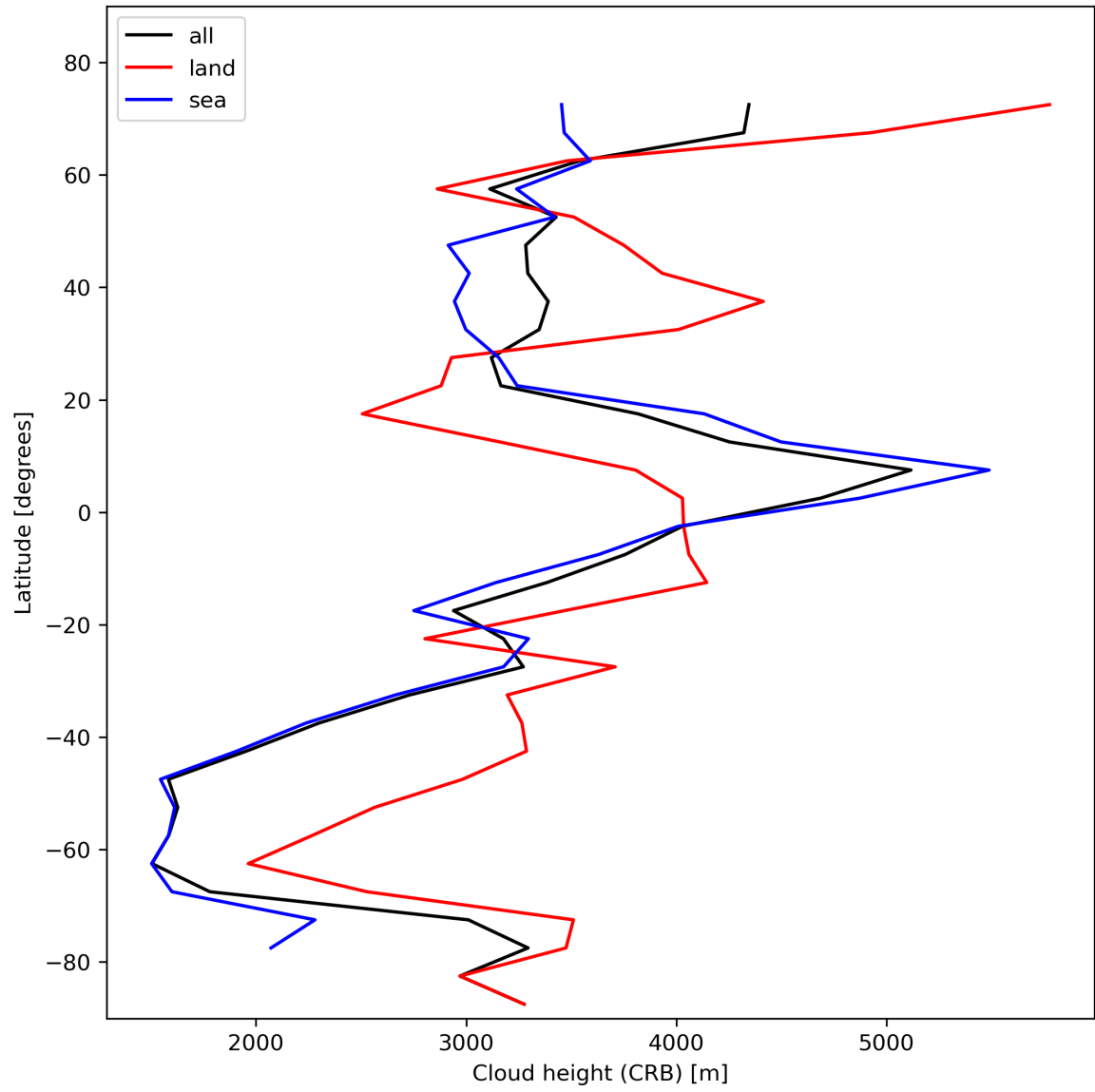
Figure 27: Zonal average of “Cloud height (CRB)” for 2023-11-13 to 2023-11-15.
