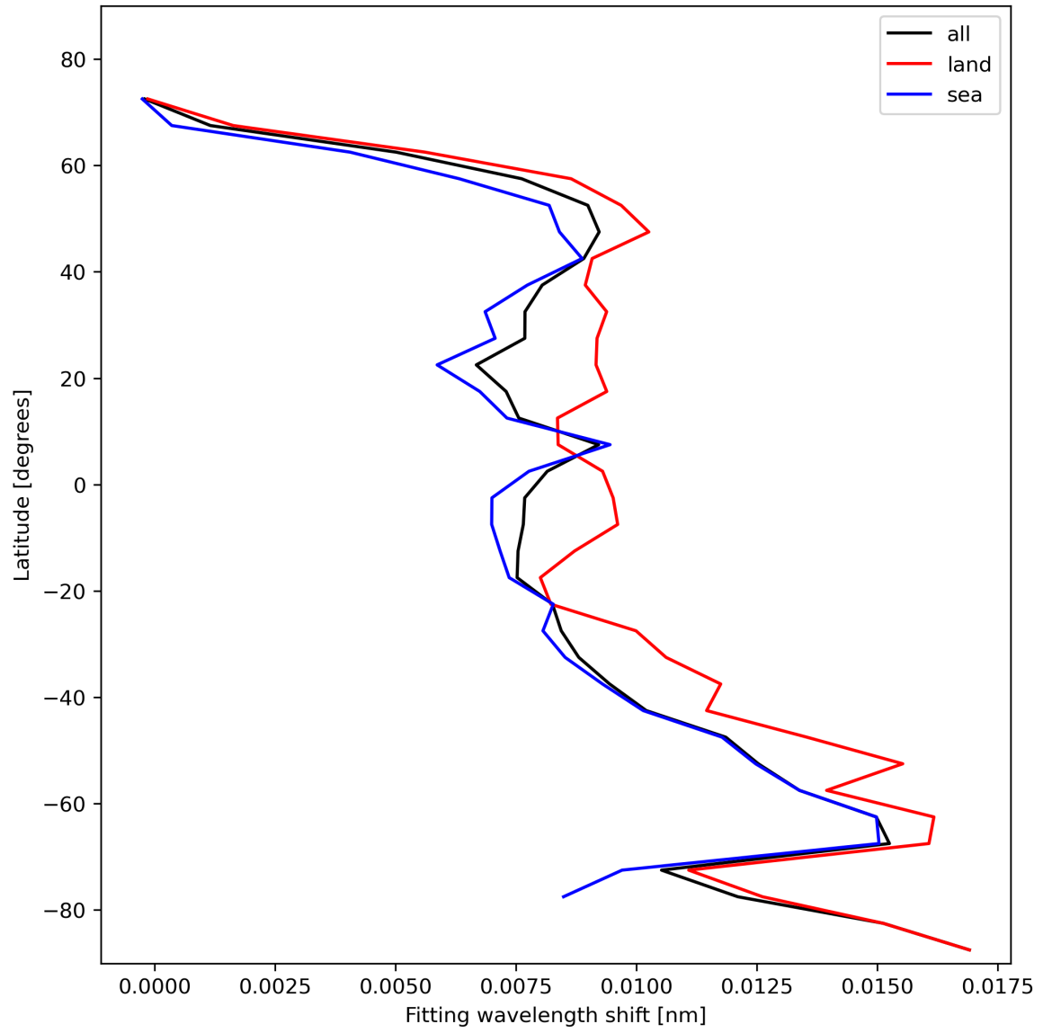
Figure 33: Zonal average of “Fitting wavelength shift” for 2023-11-13 to 2023-11-15.
