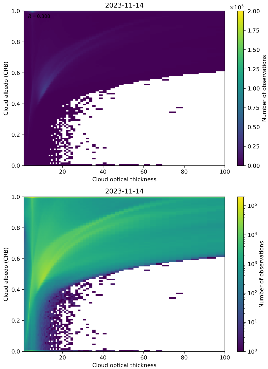
Figure 82: Scatter density plot of “Cloud optical thickness” against “Cloud albedo (CRB)” for 2023-11-13 to 2023-11-15.
