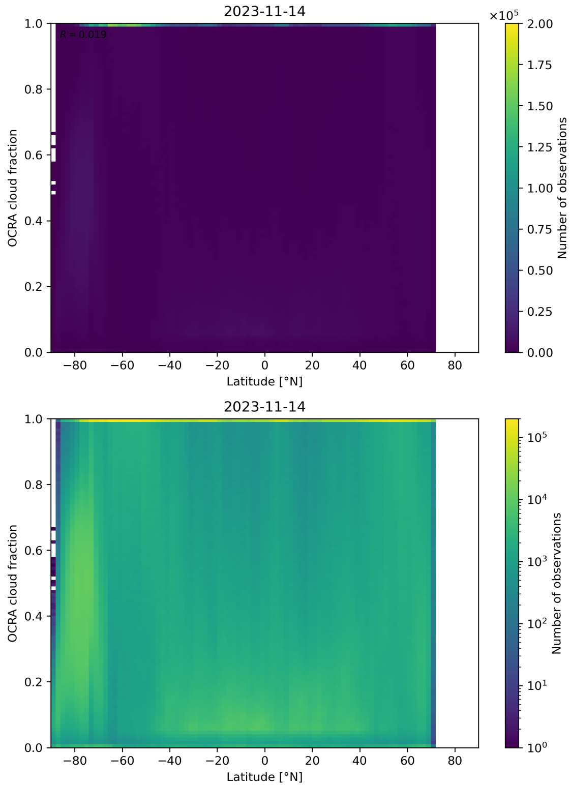
Figure 93: Scatter density plot of “Latitude” against “OCRA cloud fraction” for 2023-11-13 to 2023-11-15.
