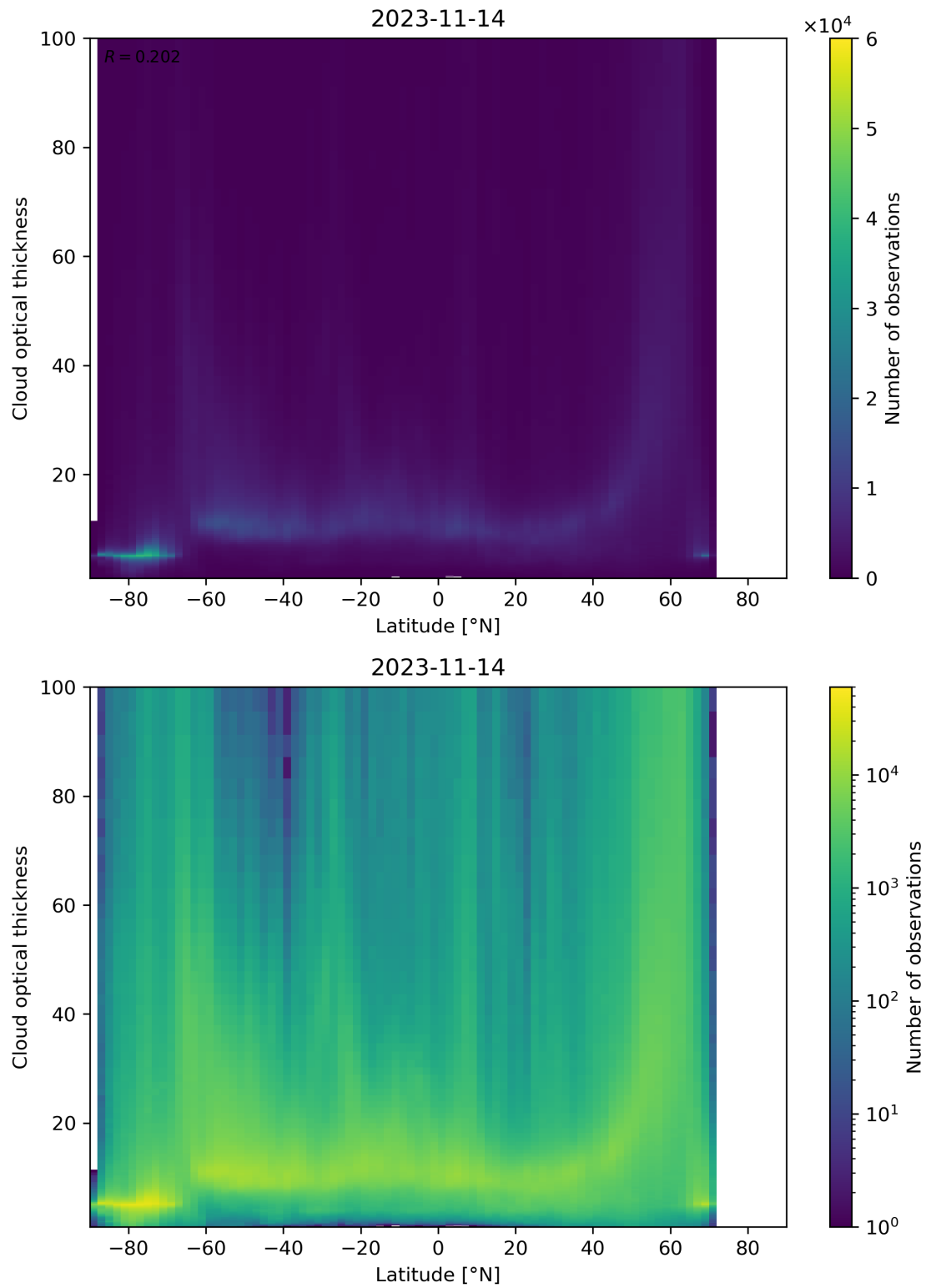
Figure 96: Scatter density plot of “Latitude” against “Cloud optical thickness” for 2023-11-13 to 2023-11-15.
