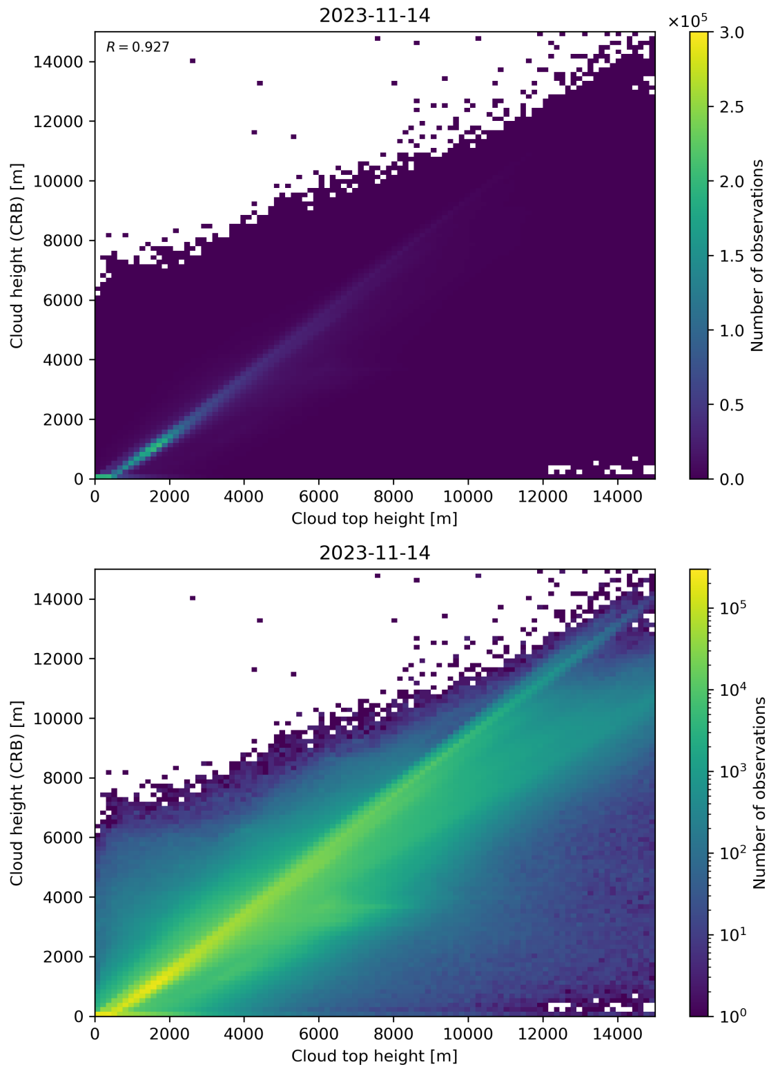
Figure 89: Scatter density plot of “Cloud top height” against “Cloud height (CRB)” for 2023-11-13 to 2023-11-15.
