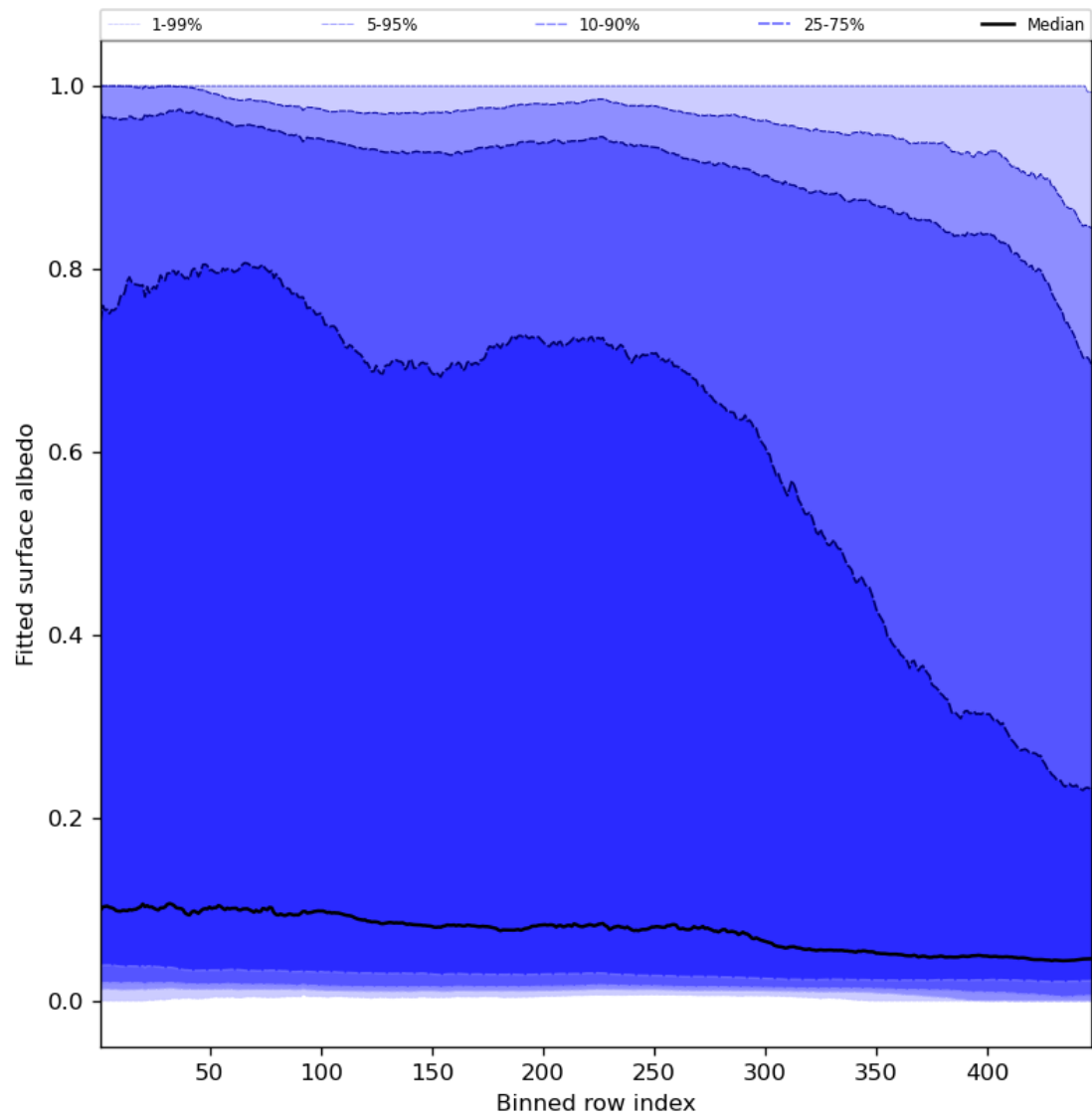
Figure 61: Along track statistics of “Fitted surface albedo” for 2023-11-13 to 2023-11-15
