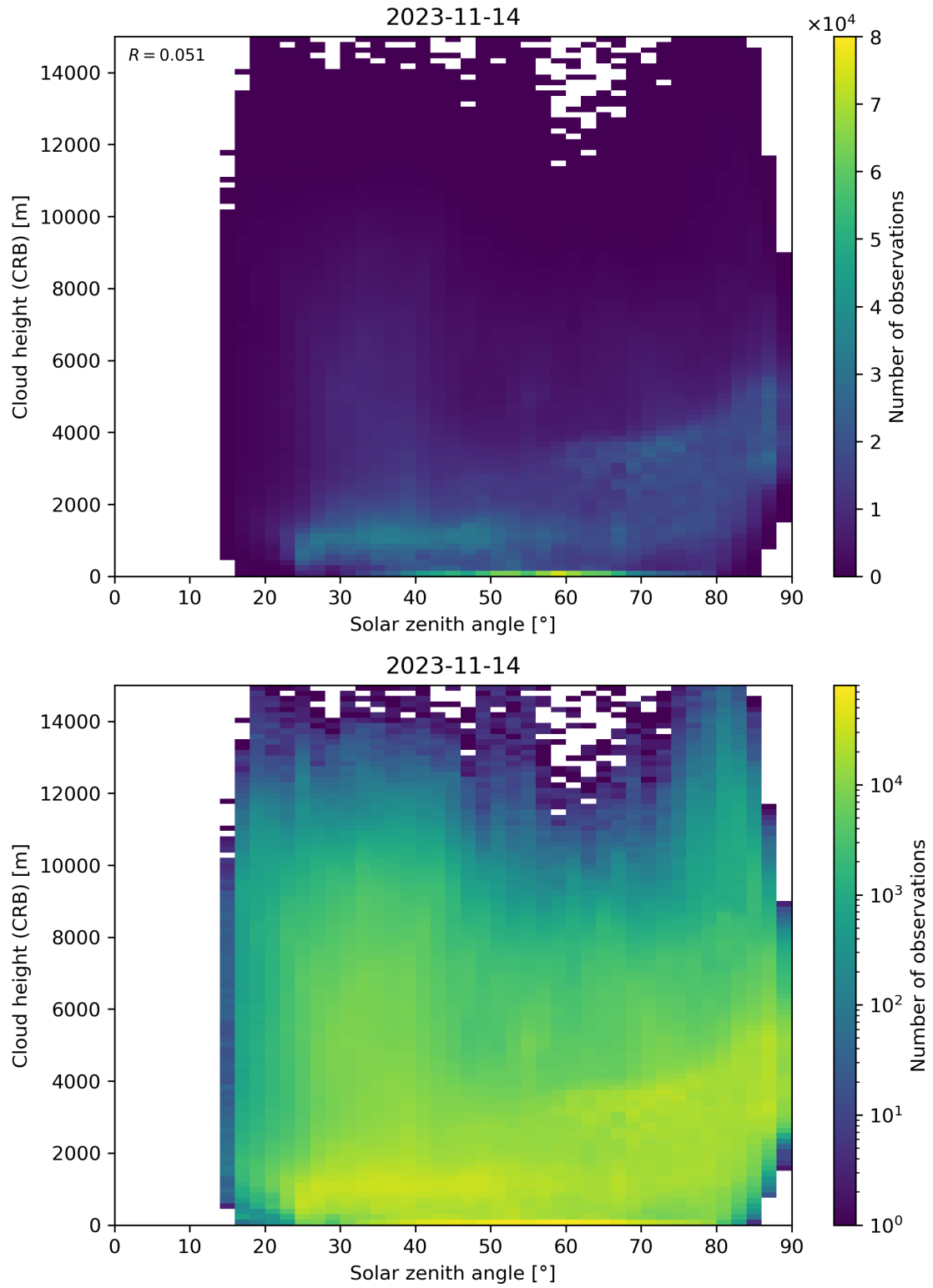
Figure 102: Scatter density plot of “Solar zenith angle” against “Cloud height (CRB)” for 2023-11-13 to 2023-11-15.
