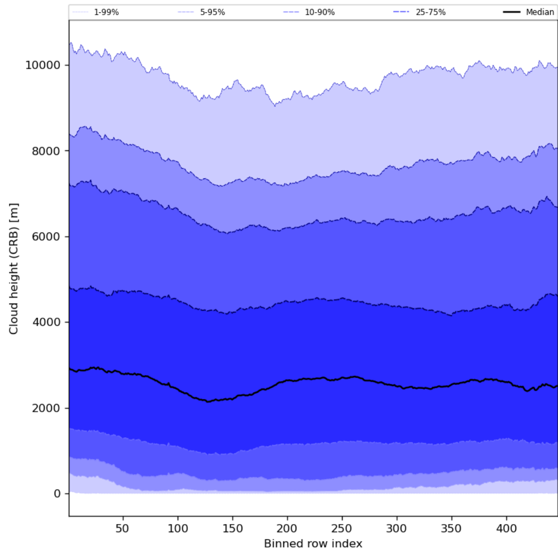
Figure 59: Along track statistics of “Cloud height (CRB)” for 2023-11-13 to 2023-11-15
