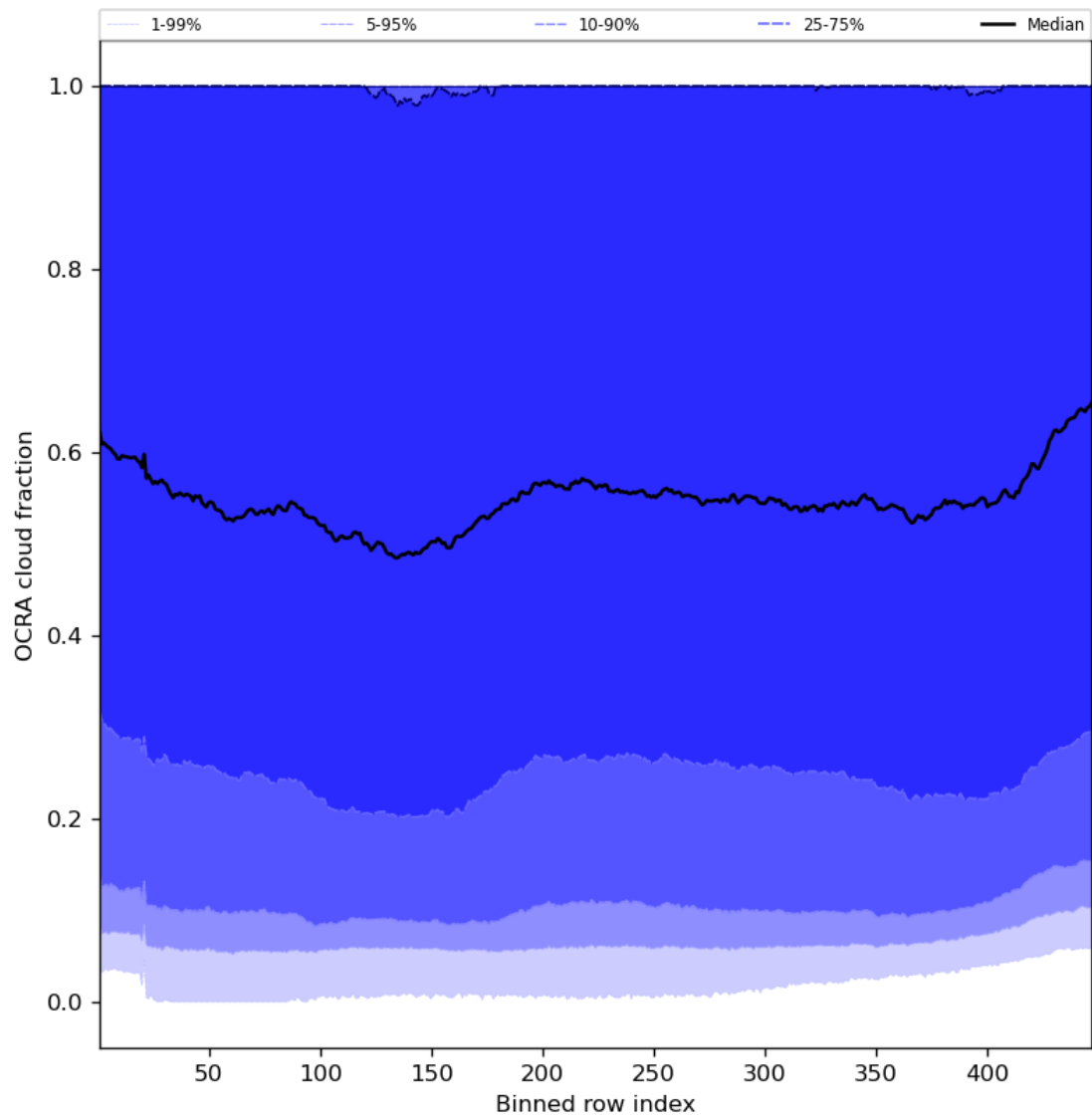
Figure 66: Along track statistics of “OCRA cloud fraction” for 2023-11-13 to 2023-11-15
