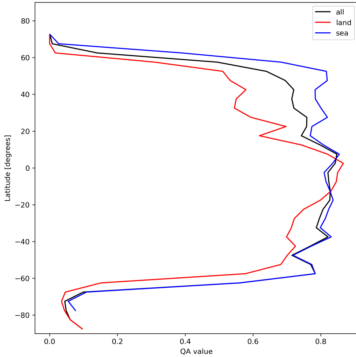
Figure 22: Zonal average of “QA value” for 2023-11-13 to 2023-11-15.
