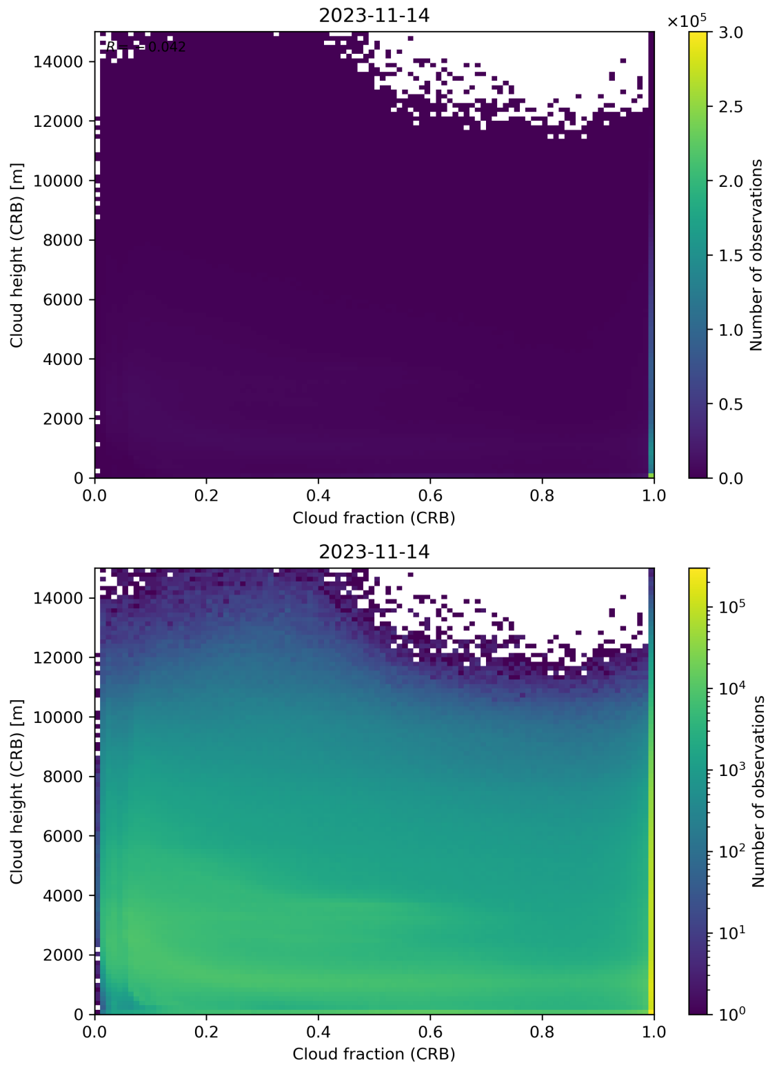
Figure 79: Scatter density plot of “Cloud fraction (CRB)” against “Cloud height (CRB)” for 2023-11-13 to 2023-11-15.
