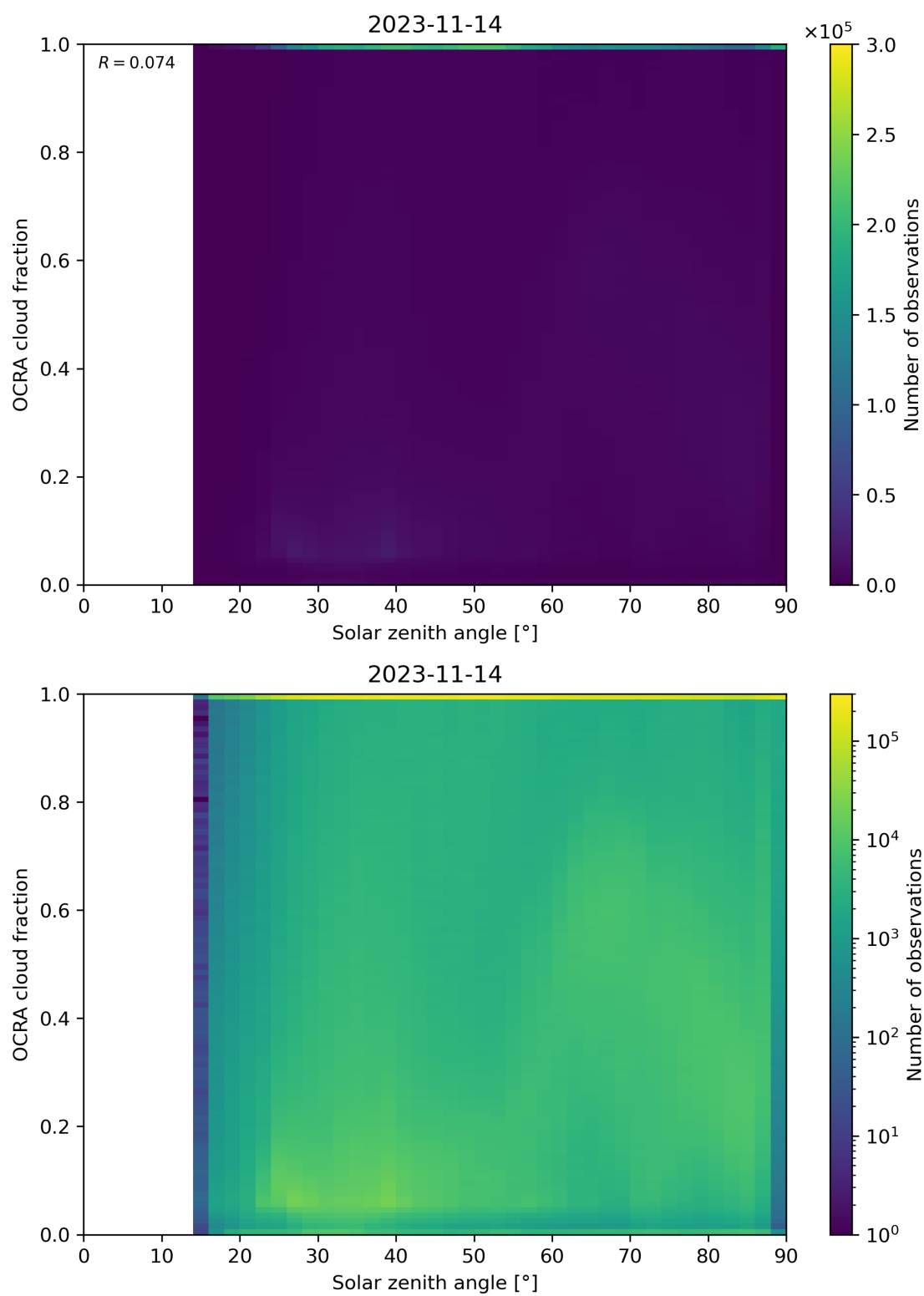
Figure 100: Scatter density plot of “Solar zenith angle” against “OCRA cloud fraction” for 2023-11-13 to 2023-11-15.
