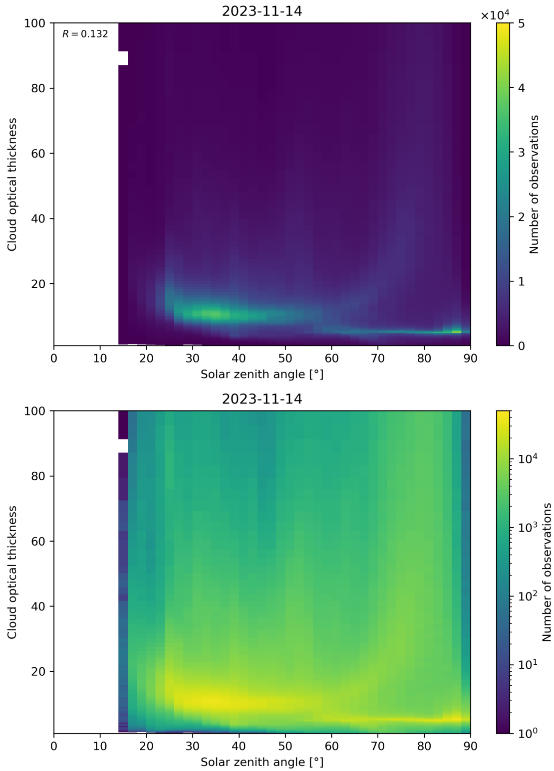
Figure 103: Scatter density plot of “Solar zenith angle” against “Cloud optical thickness” for 2023-11-13 to 2023-11-15.
