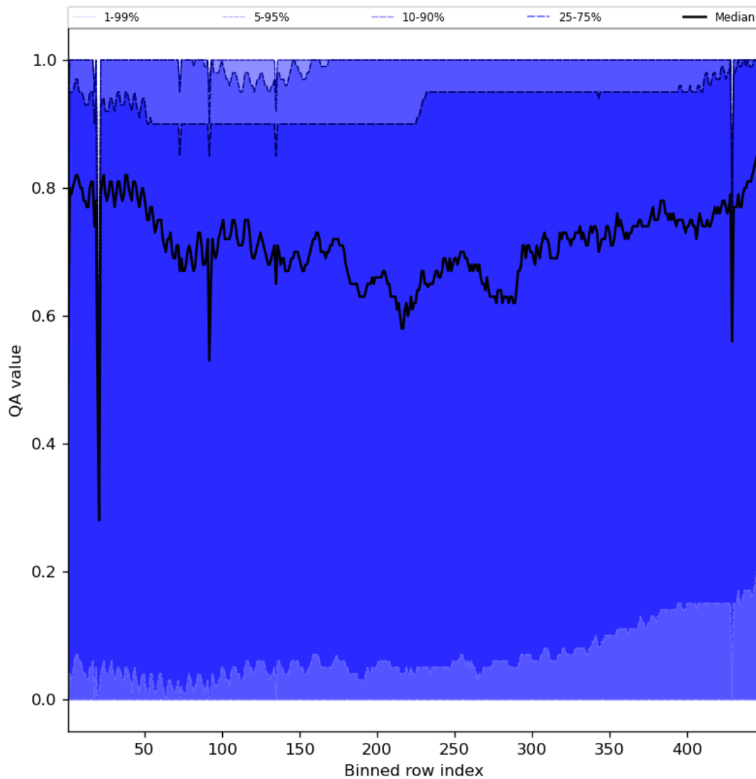
Figure 54: Along track statistics of “QA value” for 2023-11-13 to 2023-11-15
