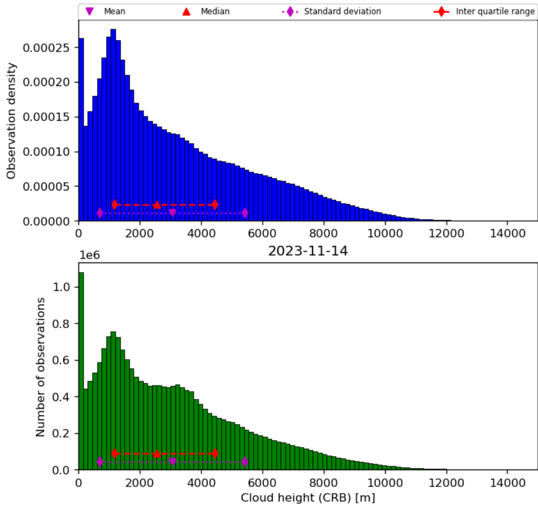
Figure 43: Histogram of “Cloud height (CRB)” for 2023-11-13 to 2023-11-15
