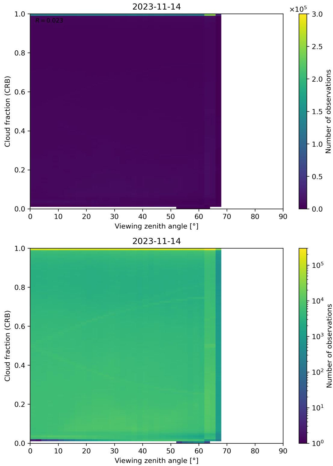
Figure 109: Scatter density plot of “Viewing zenith angle” against “Cloud fraction (CRB)” for 2023-11-13 to 2023-11-15.
