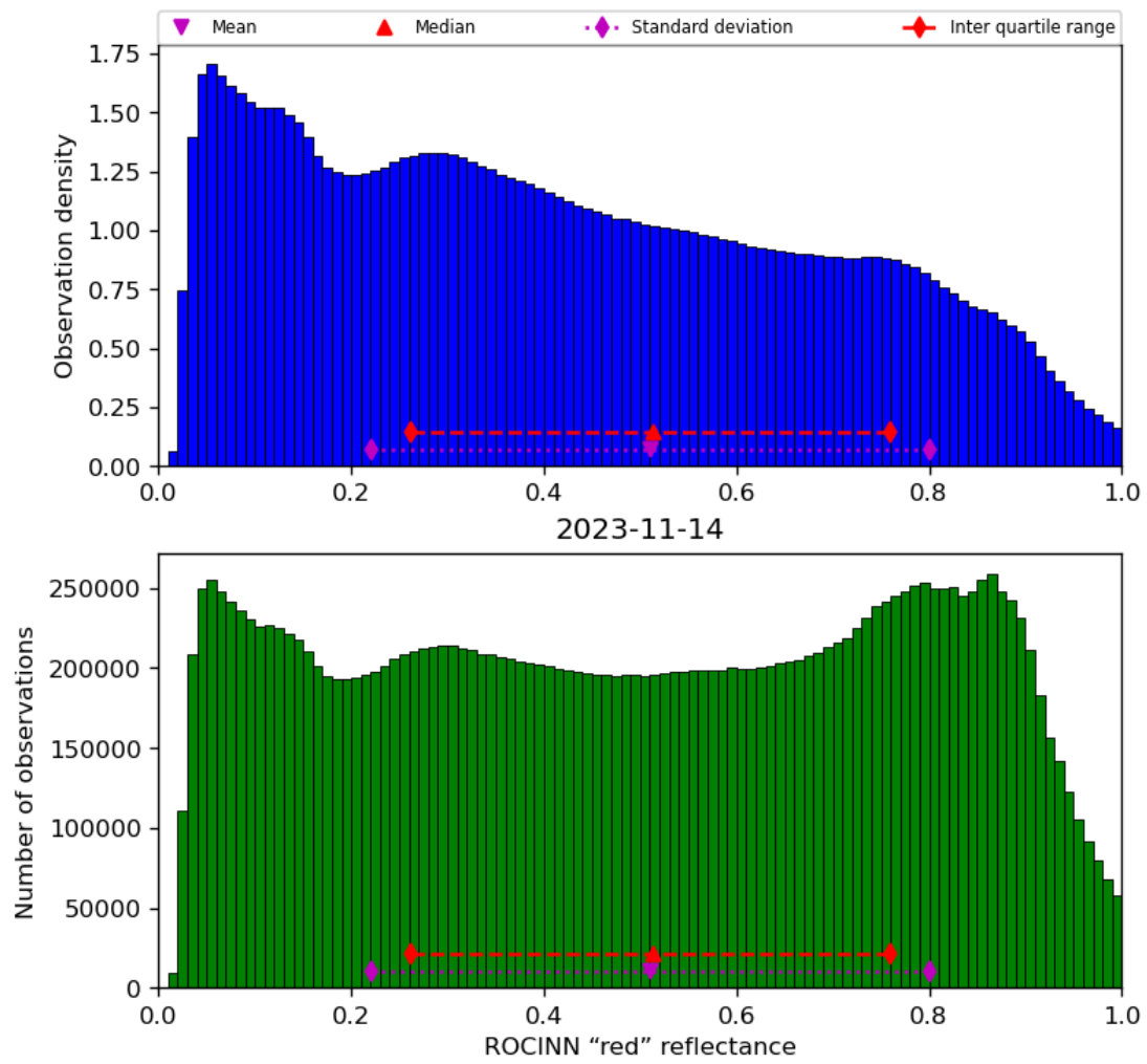
Figure 53: Histogram of “ROCINN “red” reflectance” for 2023-11-13 to 2023-11-15
