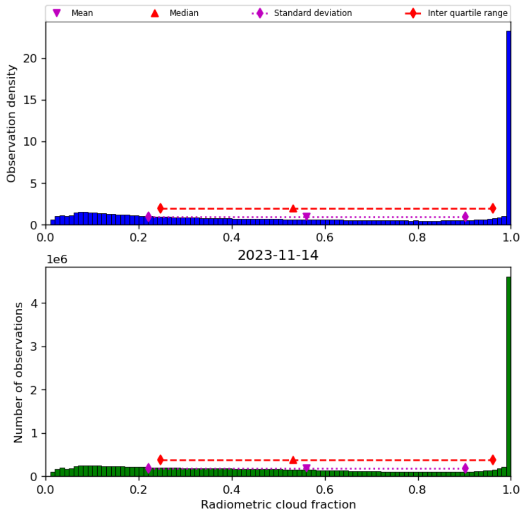
Figure 39: Histogram of “Radiometric cloud fraction” for 2023-11-13 to 2023-11-15
