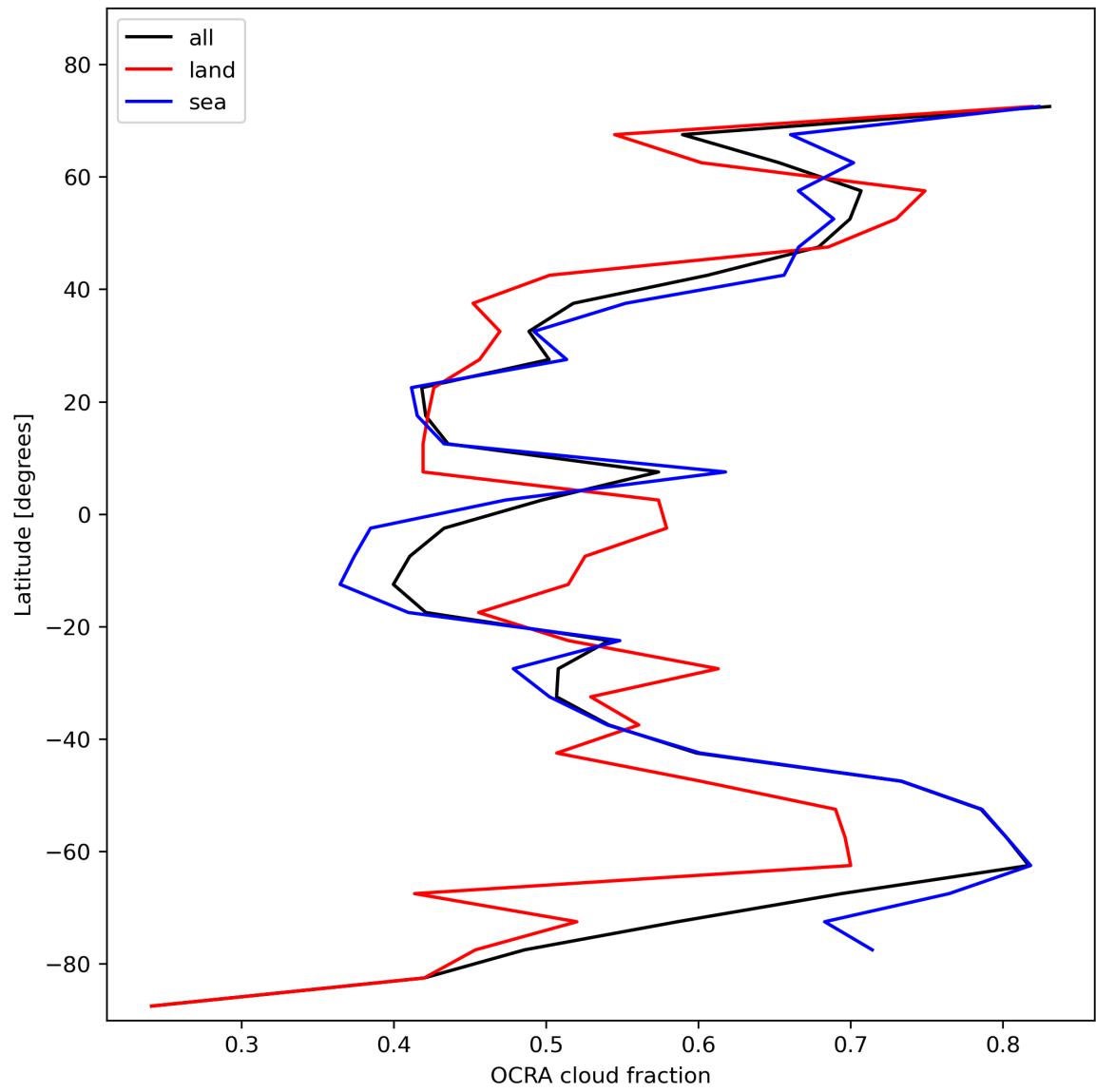
Figure 34: Zonal average of “OCRA cloud fraction” for 2023-11-13 to 2023-11-15.
