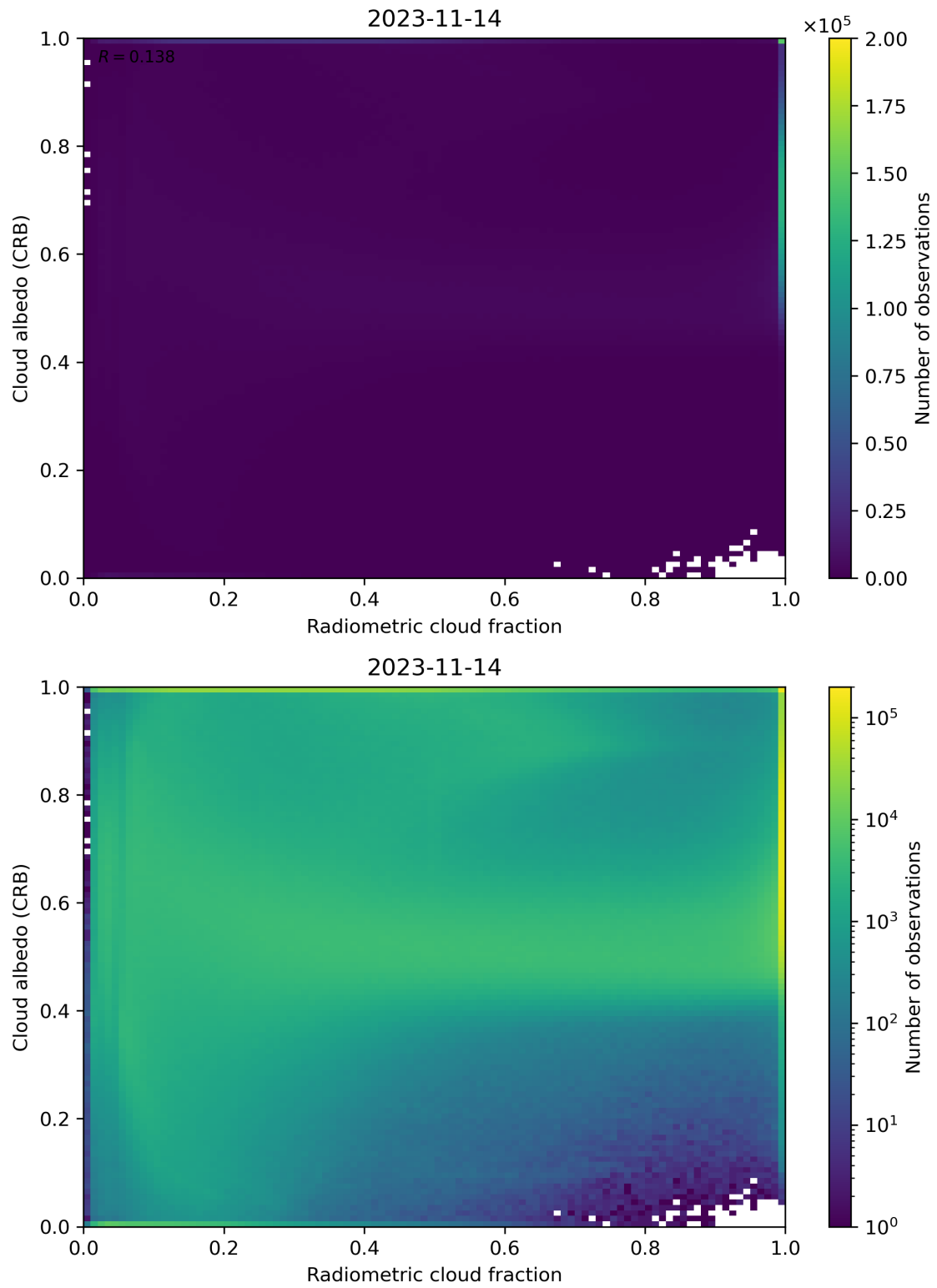
Figure 71: Scatter density plot of “Radiometric cloud fraction” against “Cloud albedo (CRB)” for 2023-11-13 to 2023-11-15.
