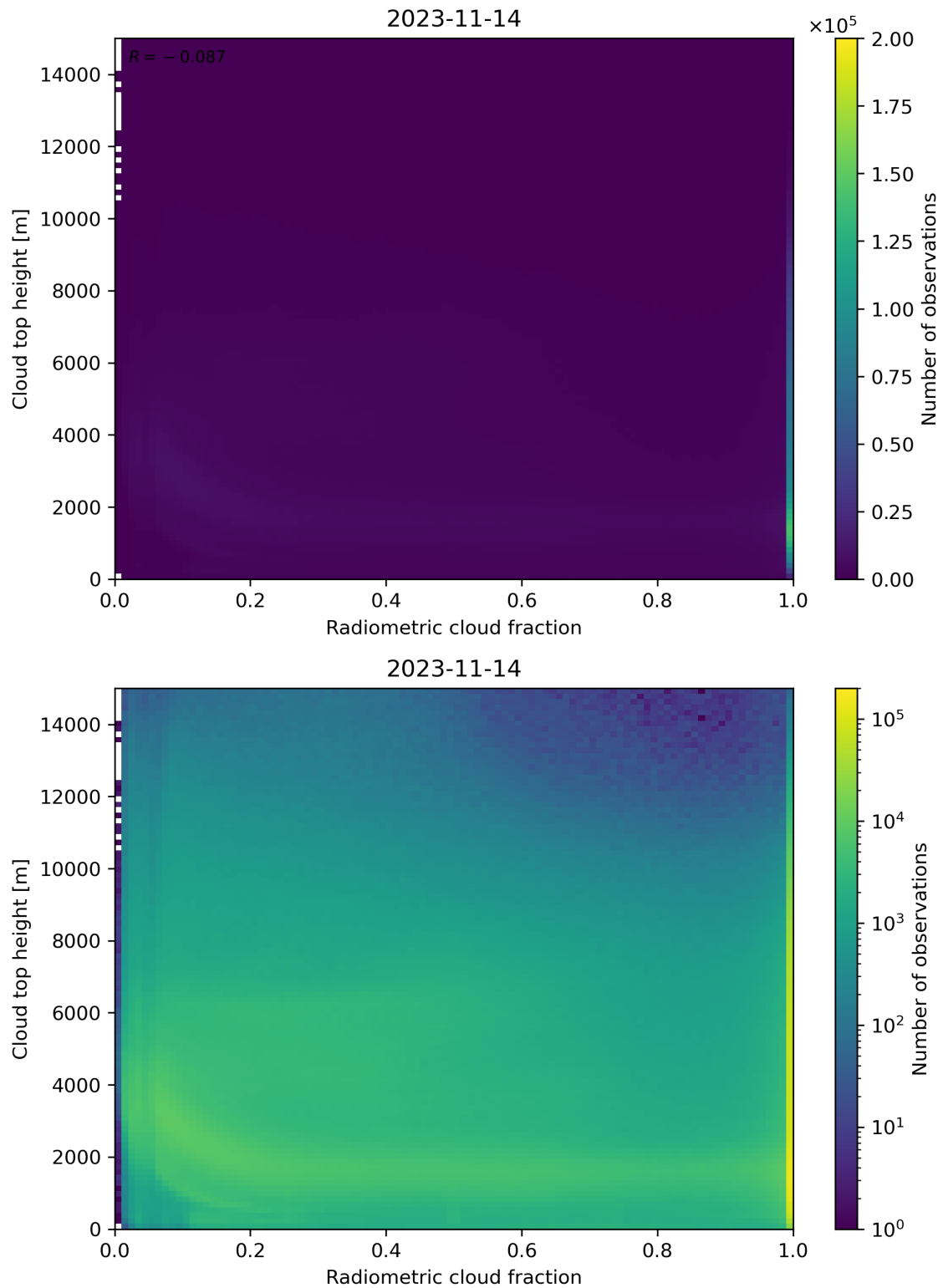
Figure 76: Scatter density plot of “Radiometric cloud fraction” against “Cloud top height” for 2023-11-13 to 2023-11-15.
