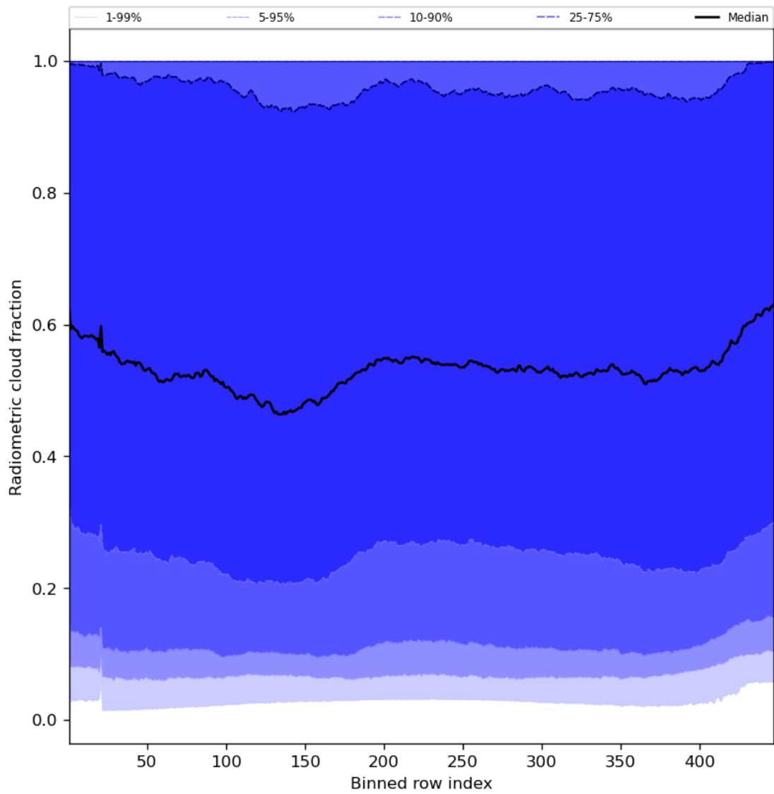
Figure 55: Along track statistics of “Radiometric cloud fraction” for 2023-11-13 to 2023-11-15
