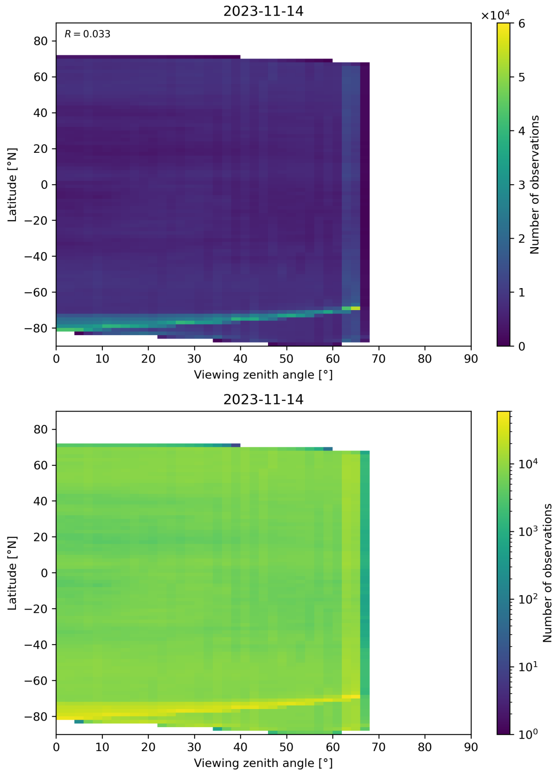
Figure 113: Scatter density plot of “Viewing zenith angle” against “Latitude” for 2023-11-13 to 2023-11-15.
