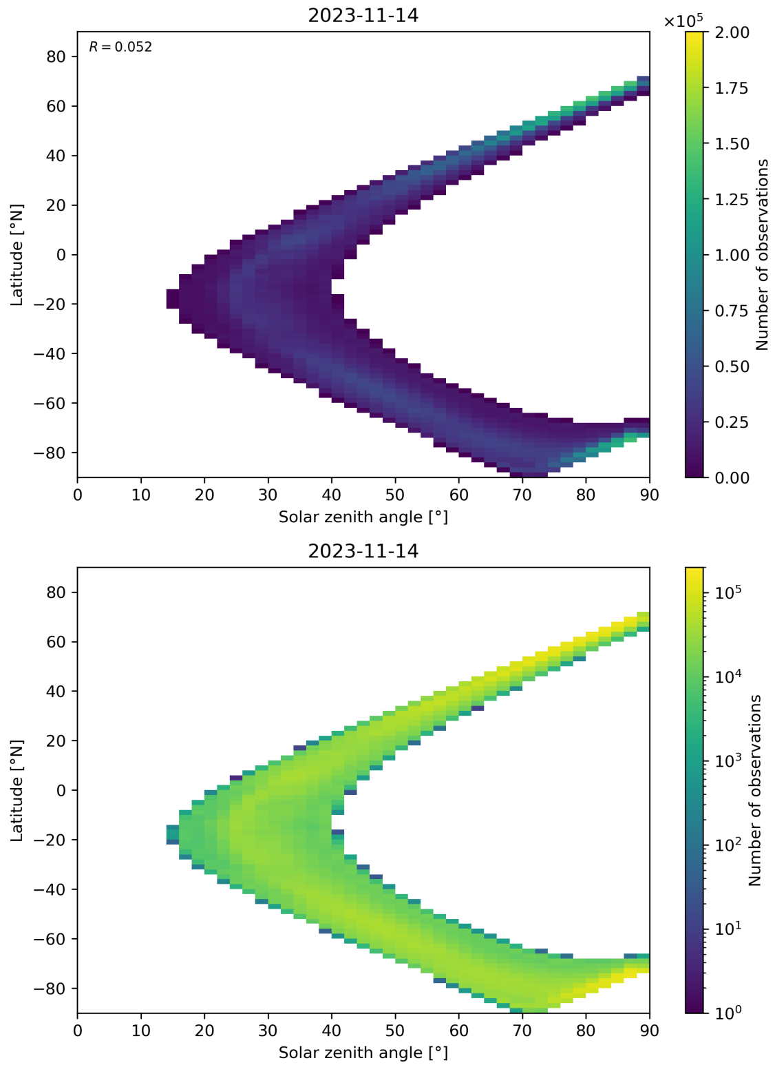
Figure 105: Scatter density plot of “Solar zenith angle” against “Latitude” for 2023-11-13 to 2023-11-15.
