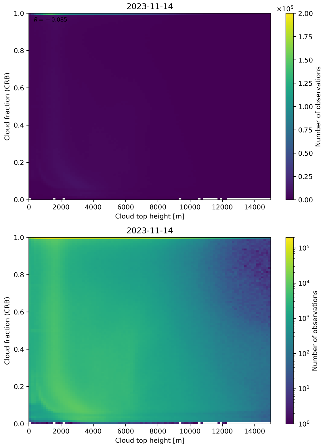
Figure 88: Scatter density plot of “Cloud top height” against “Cloud fraction (CRB)” for 2023-11-13 to 2023-11-15.
