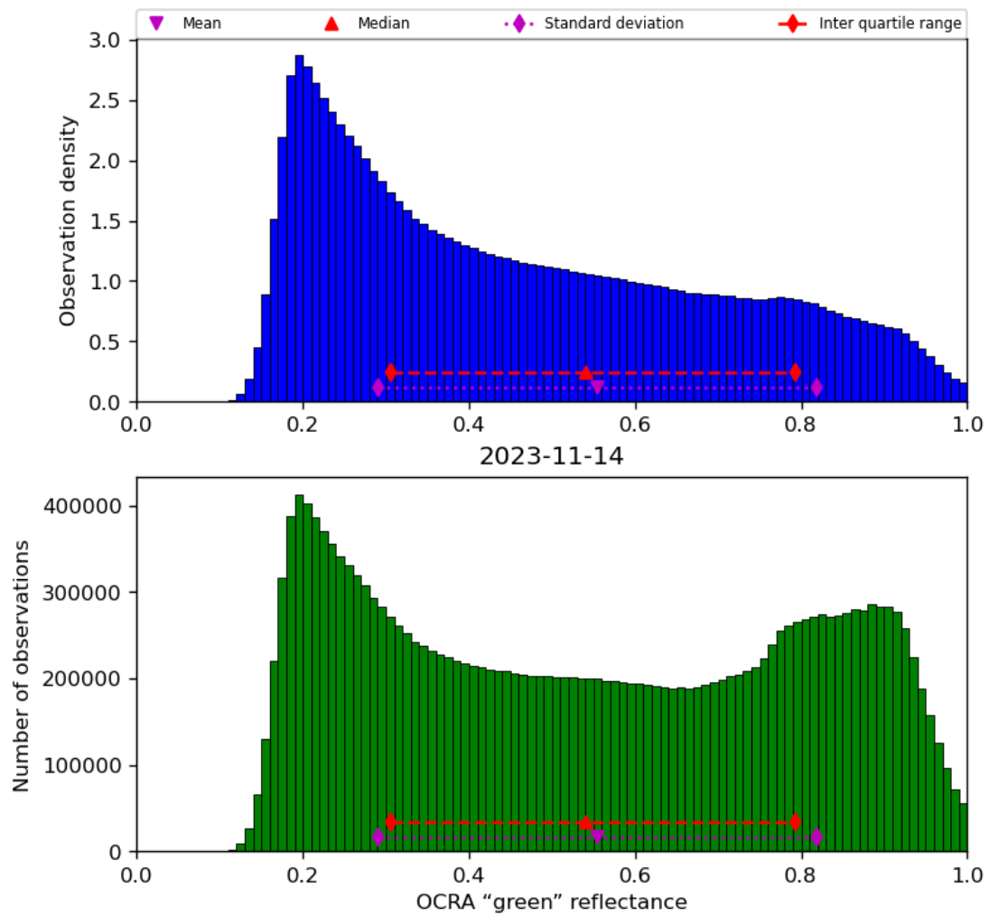
Figure 52: Histogram of “OCRA “green” reflectance” for 2023-11-13 to 2023-11-15
