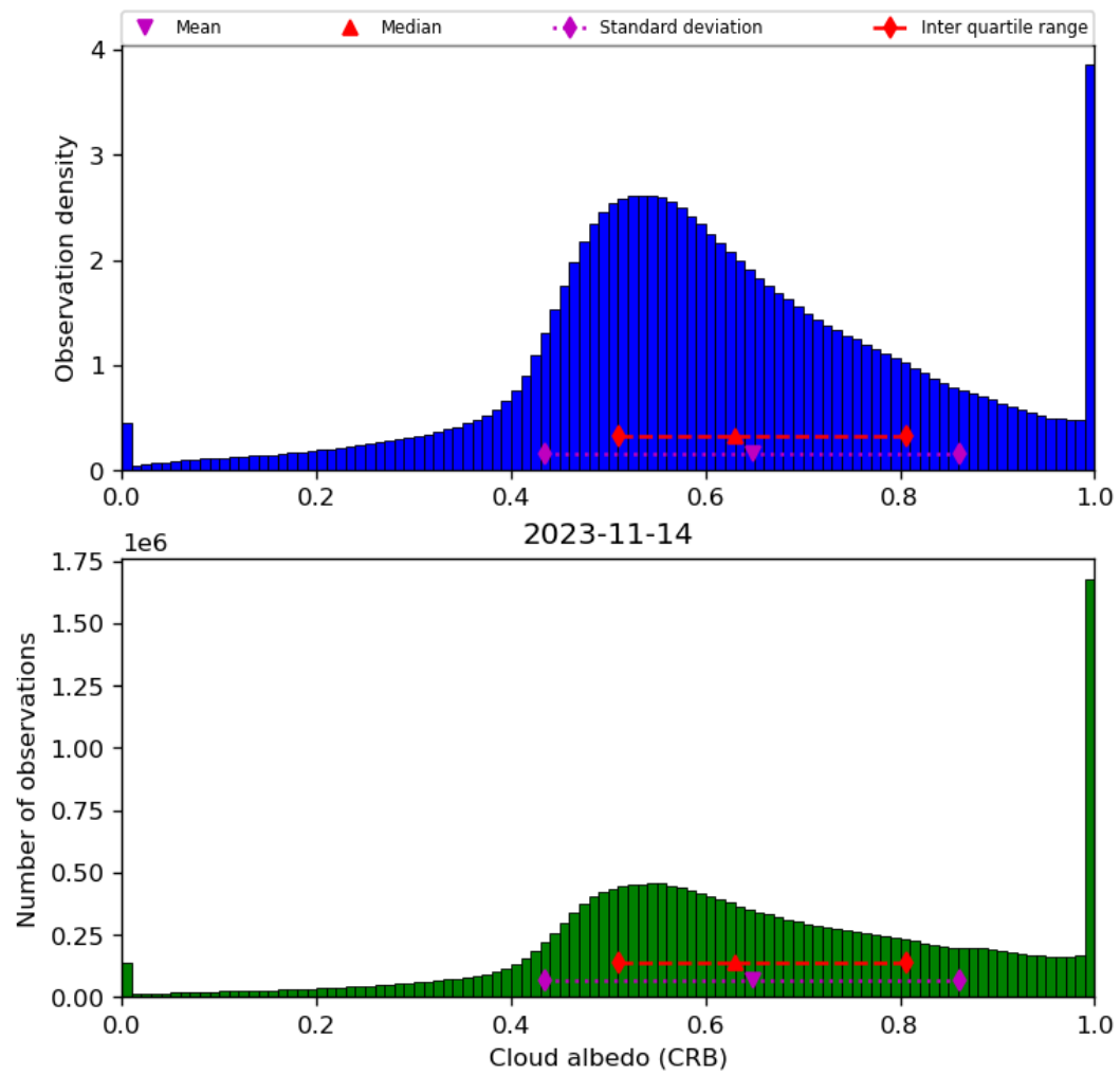
Figure 44: Histogram of “Cloud albedo (CRB)” for 2023-11-13 to 2023-11-15
