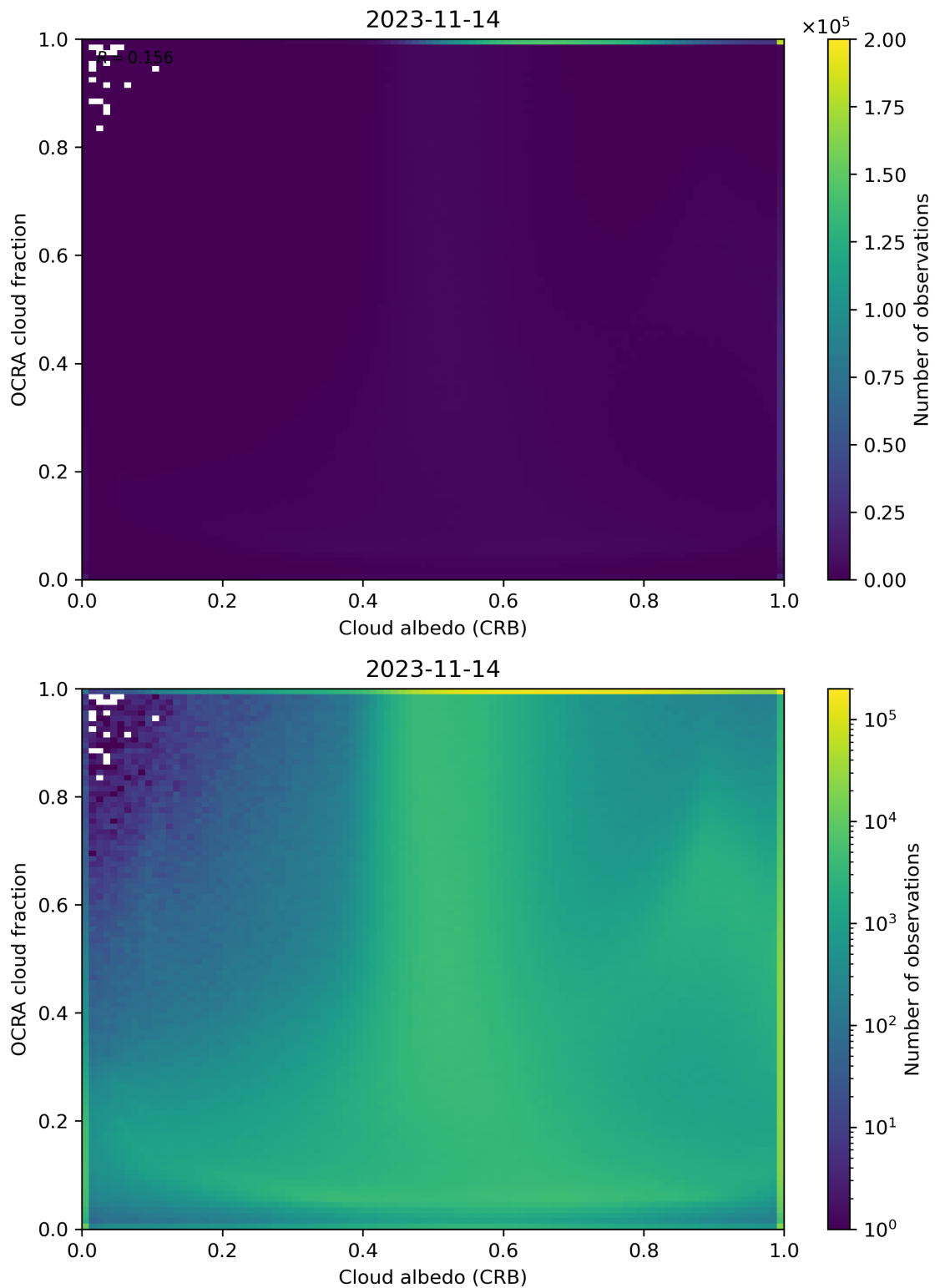
Figure 70: Scatter density plot of “Cloud albedo (CRB)” against “OCRA cloud fraction” for 2023-11-13 to 2023-11-15.
