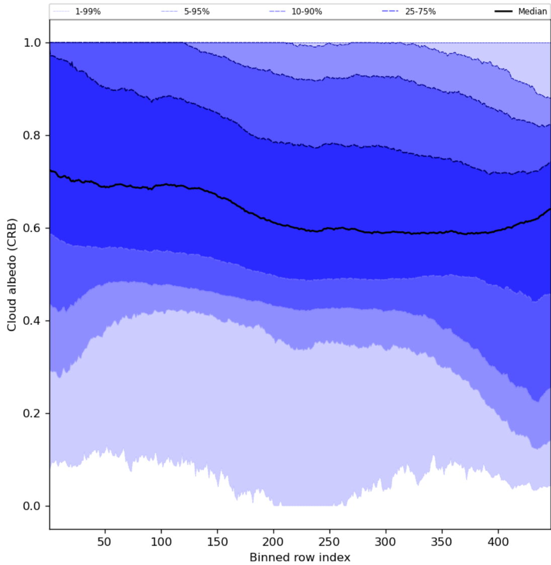
Figure 60: Along track statistics of “Cloud albedo (CRB)” for 2023-11-13 to 2023-11-15
