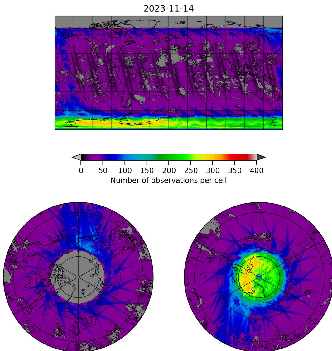
Figure 21: Map of the number of observations for 2023-11-13 to 2023-11-15
