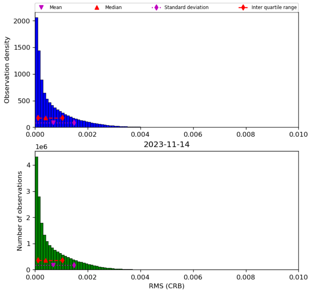
Figure 48: Histogram of “RMS (CRB)” for 2023-11-13 to 2023-11-15
