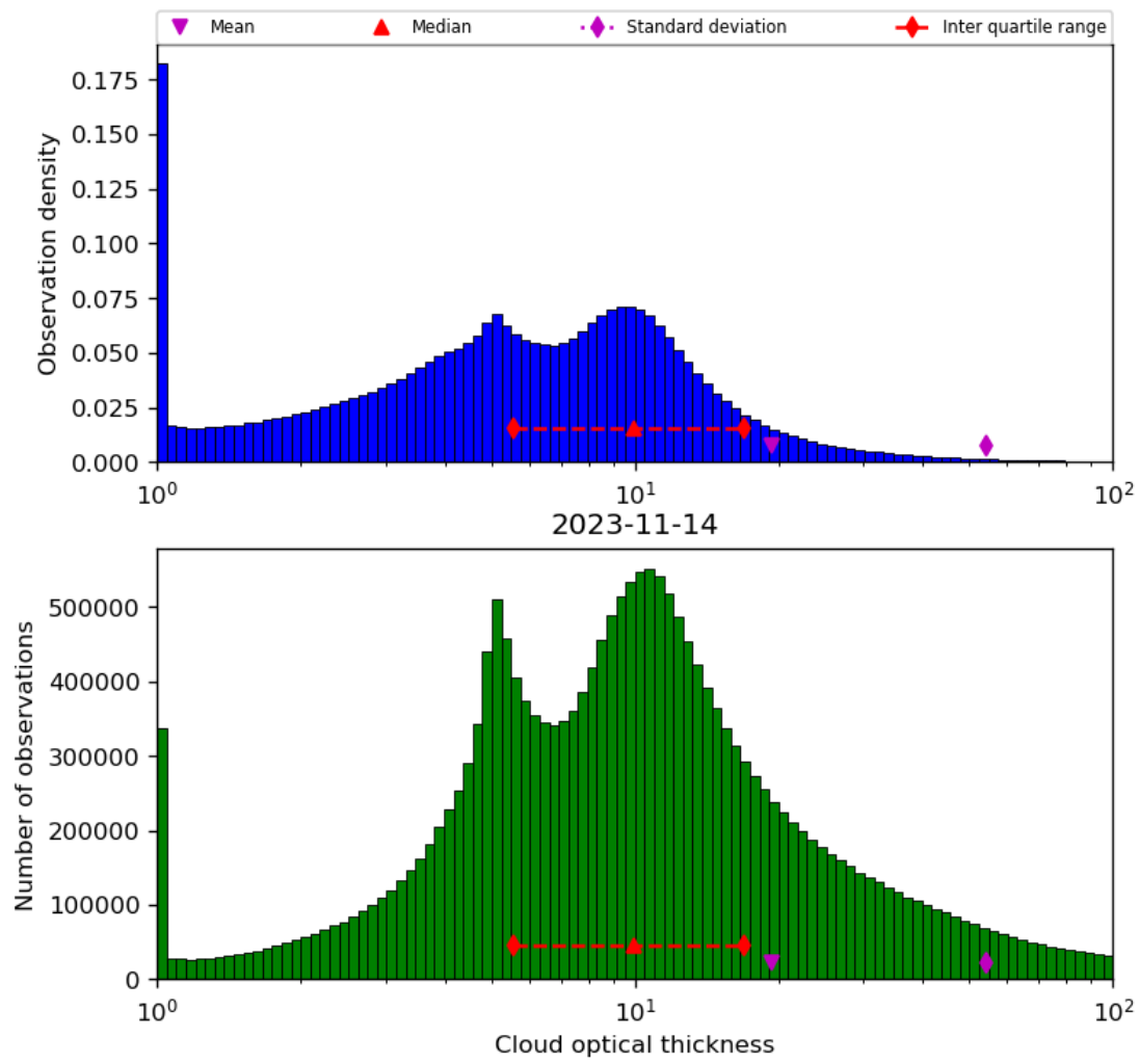
Figure 41: Histogram of “Cloud optical thickness” for 2023-11-13 to 2023-11-15
