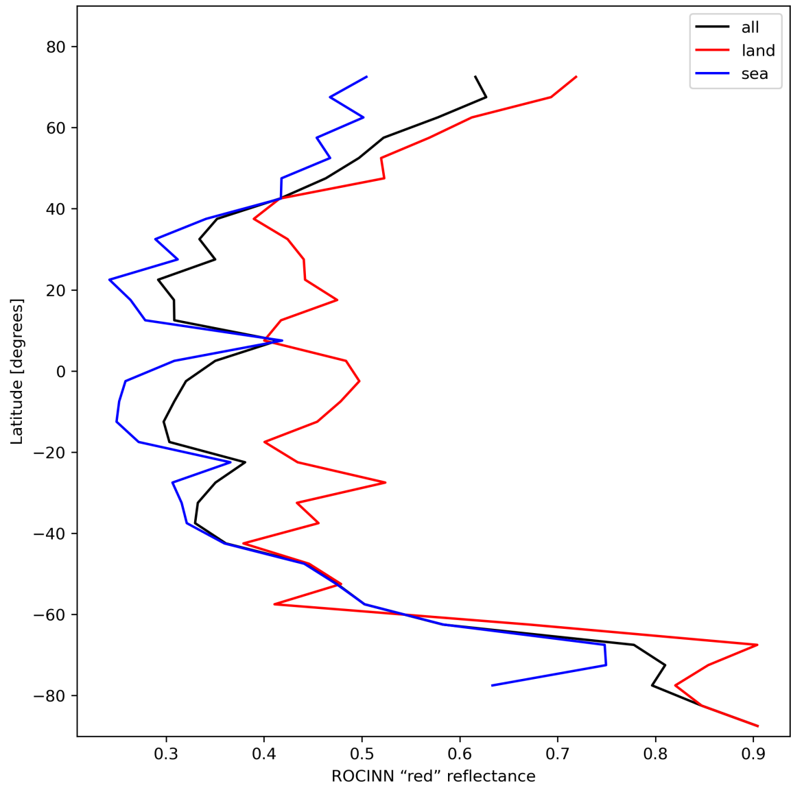
Figure 37: Zonal average of “ROCINN “red” reflectance” for 2023-11-13 to 2023-11-15.
