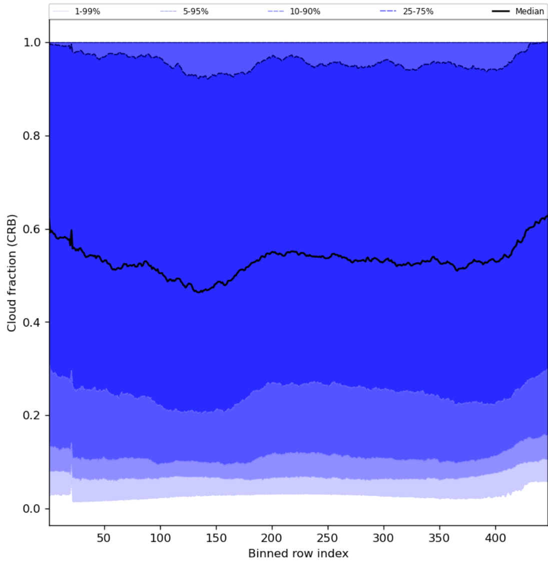
Figure 58: Along track statistics of “Cloud fraction (CRB)” for 2023-11-13 to 2023-11-15
