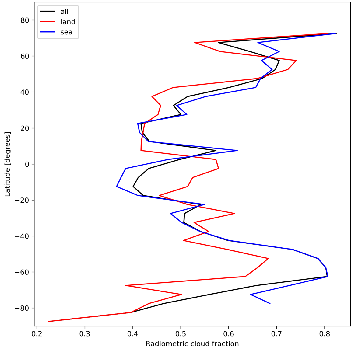
Figure 23: Zonal average of “Radiometric cloud fraction” for 2023-11-13 to 2023-11-15.
