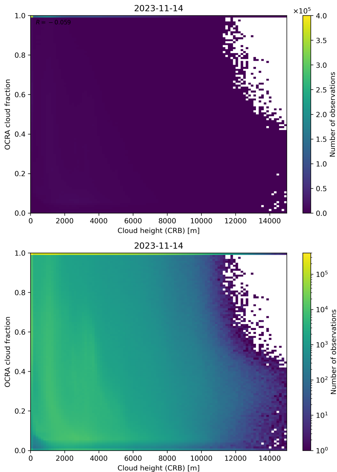
Figure 81: Scatter density plot of “Cloud height (CRB)” against “OCRA cloud fraction” for 2023-11-13 to 2023-11-15.
