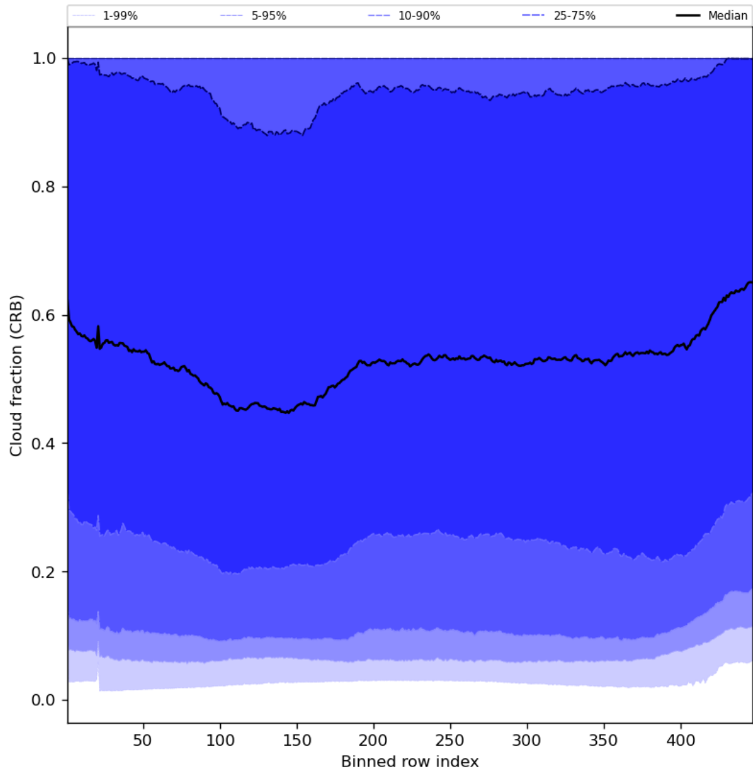
Figure 58: Along track statistics of “Cloud fraction (CRB)” for 2023-11-15 to 2023-11-17
