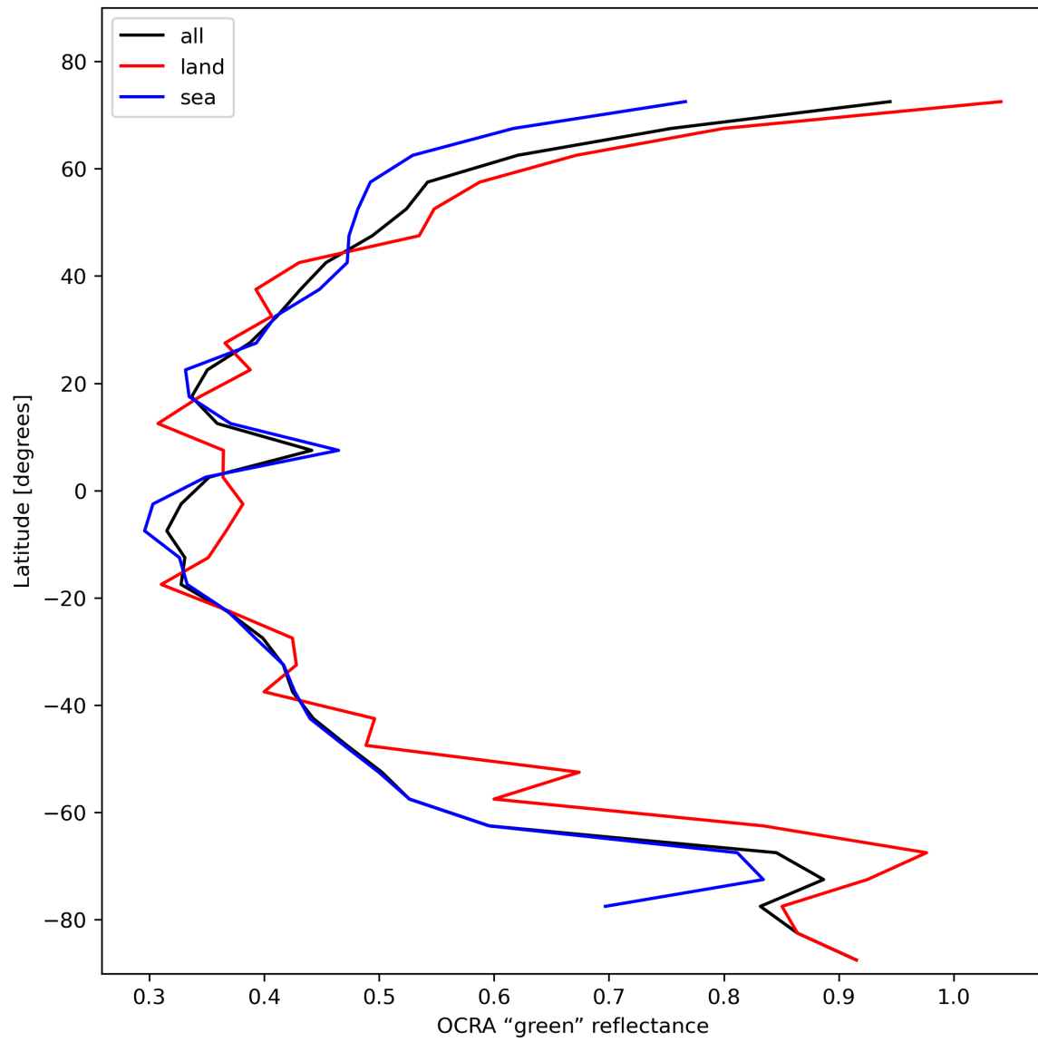
Figure 36: Zonal average of “OCRA “green” reflectance” for 2023-11-15 to 2023-11-17.
