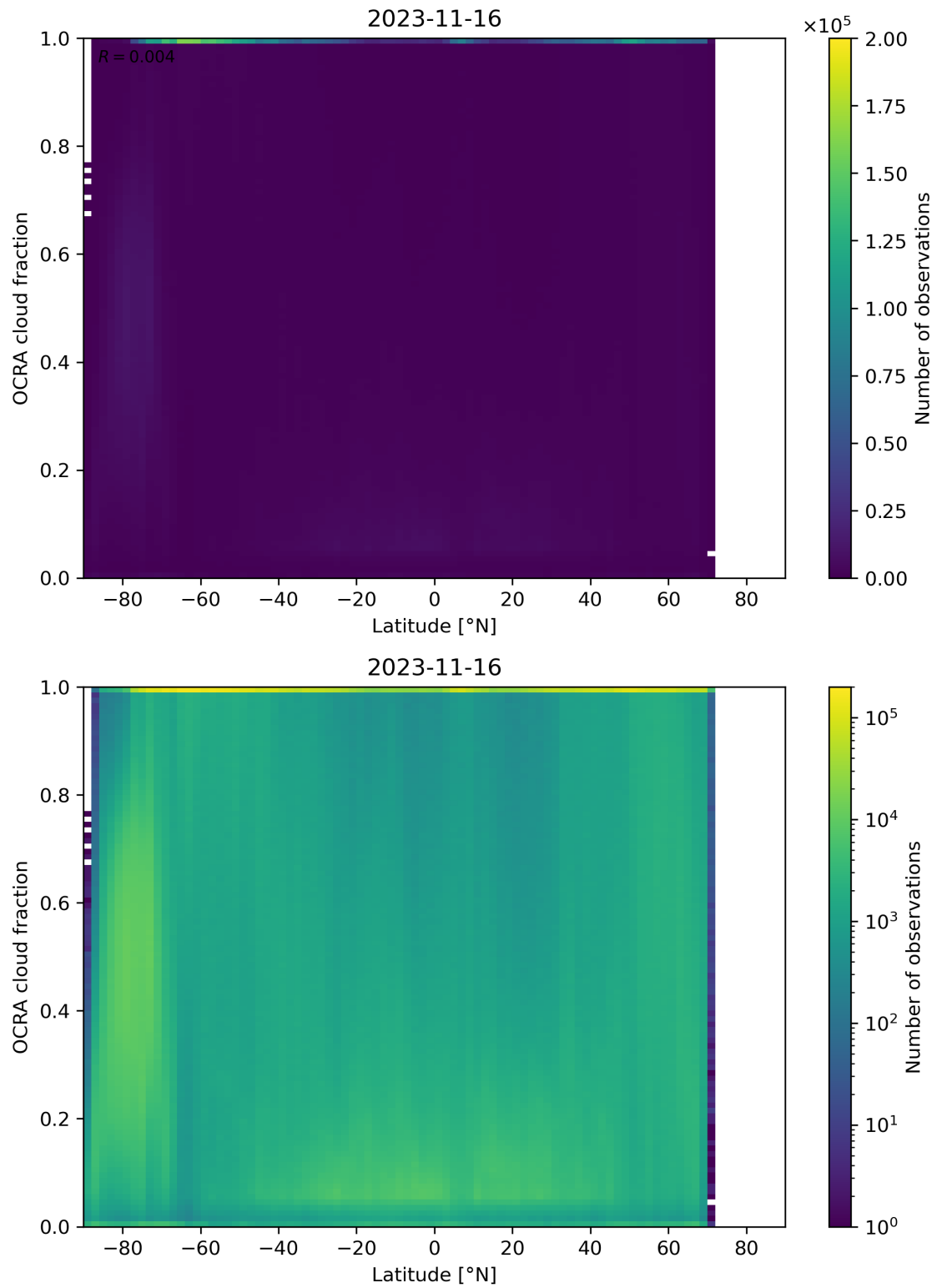
Figure 93: Scatter density plot of “Latitude” against “OCRA cloud fraction” for 2023-11-15 to 2023-11-17.
