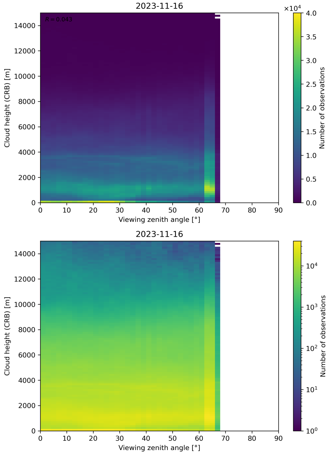
Figure 110: Scatter density plot of “Viewing zenith angle” against “Cloud height (CRB)” for 2023-11-15 to 2023-11-17.
