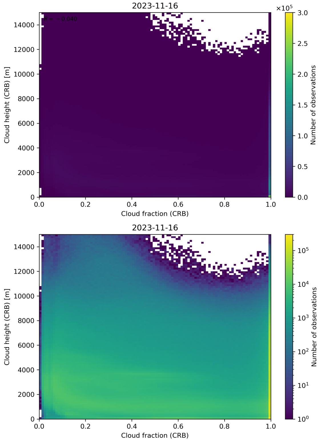
Figure 79: Scatter density plot of “Cloud fraction (CRB)” against “Cloud height (CRB)” for 2023-11-15 to 2023-11-17.
