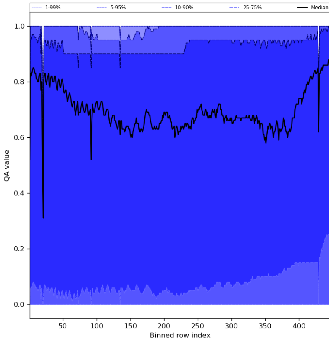
Figure 54: Along track statistics of “QA value” for 2023-11-15 to 2023-11-17
