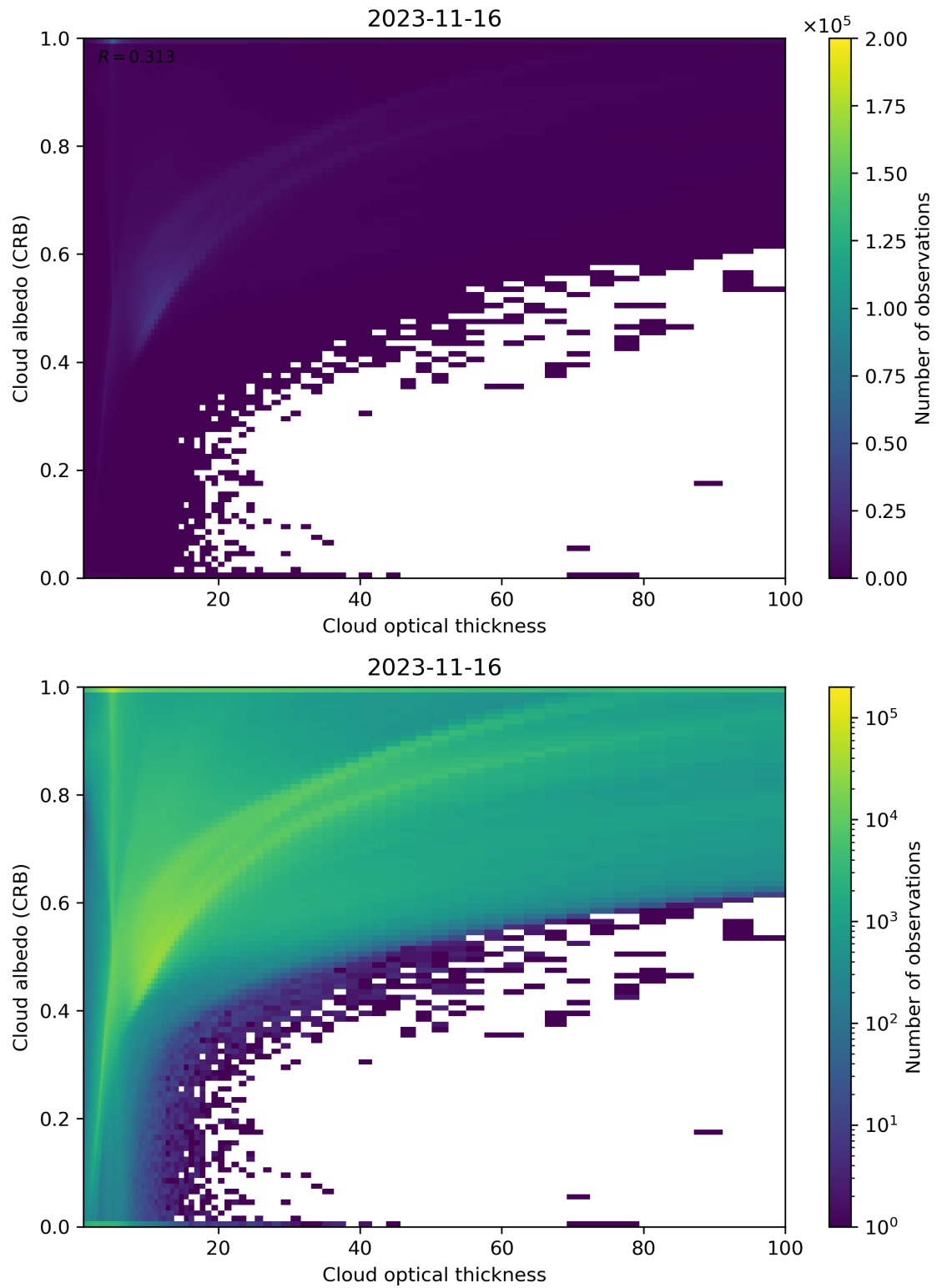
Figure 82: Scatter density plot of “Cloud optical thickness” against “Cloud albedo (CRB)” for 2023-11-15 to 2023-11-17.
