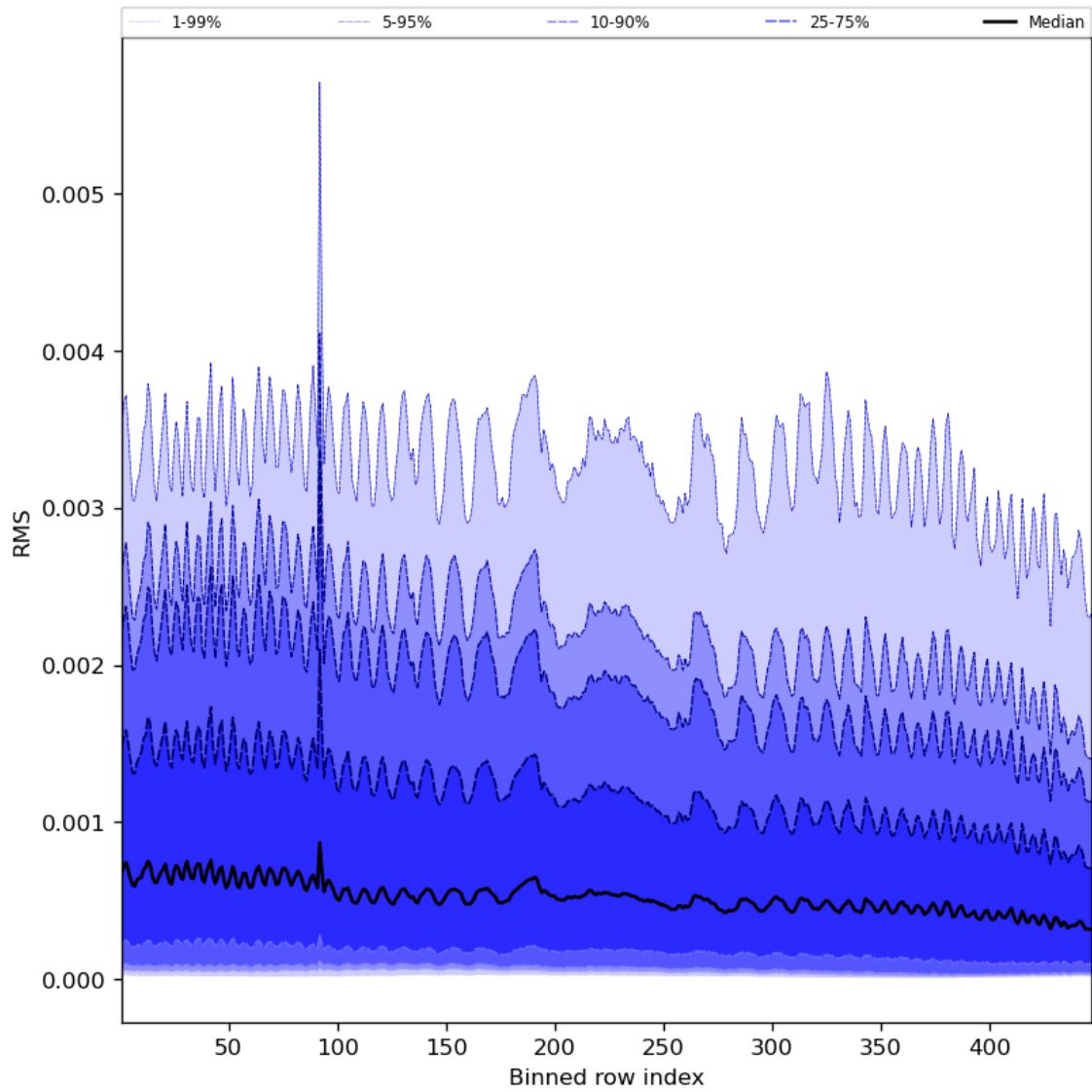
Figure 63: Along track statistics of “RMS” for 2023-11-15 to 2023-11-17
