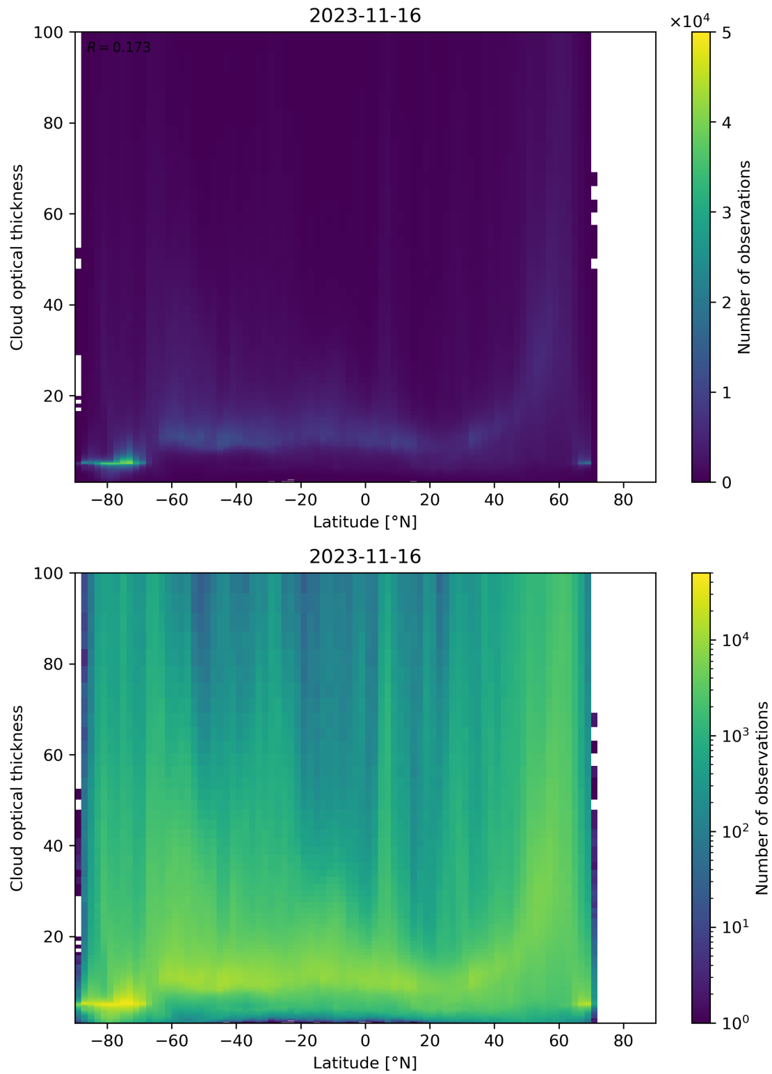
Figure 96: Scatter density plot of “Latitude” against “Cloud optical thickness” for 2023-11-15 to 2023-11-17.
