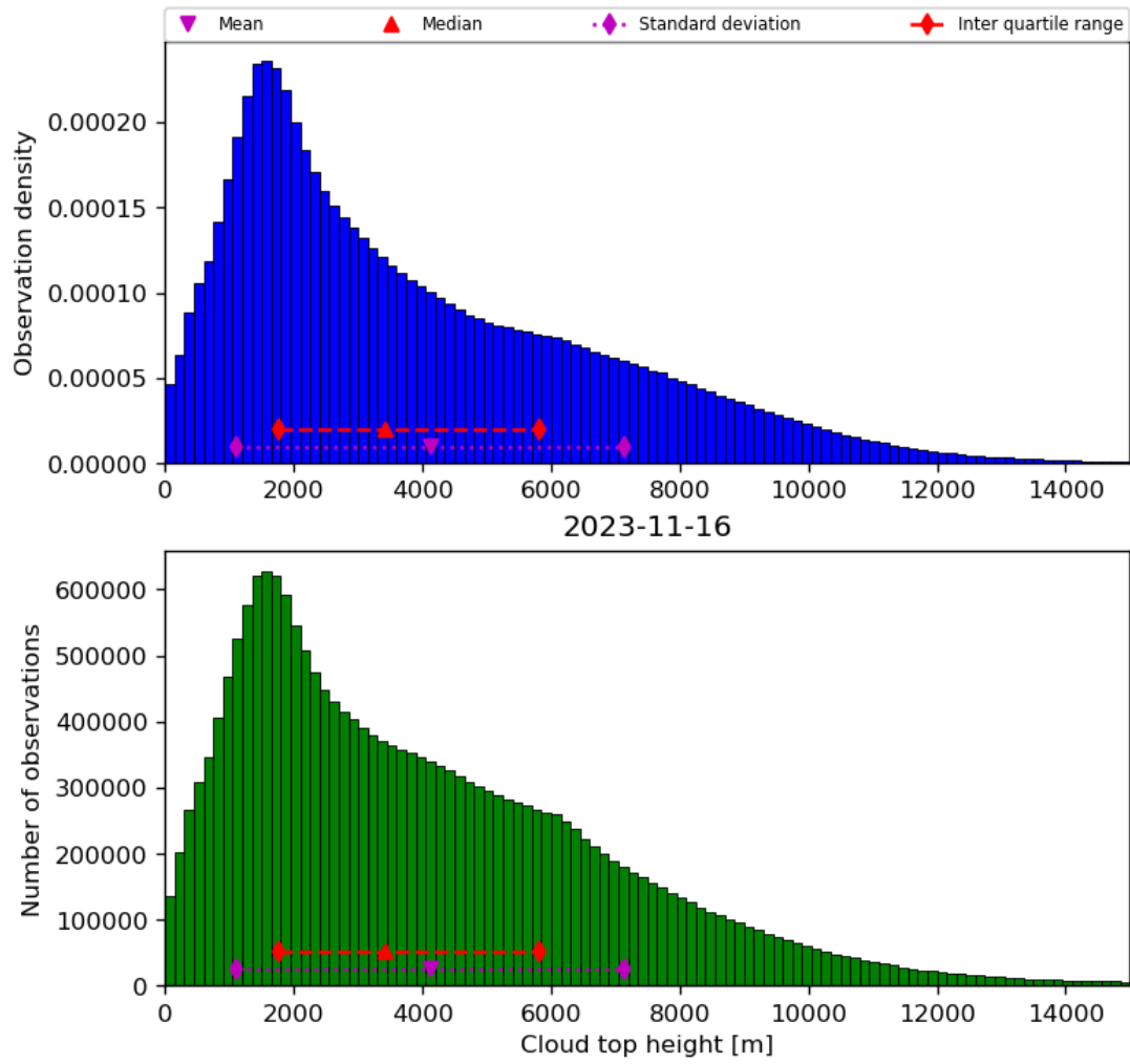
Figure 40: Histogram of “Cloud top height” for 2023-11-15 to 2023-11-17
