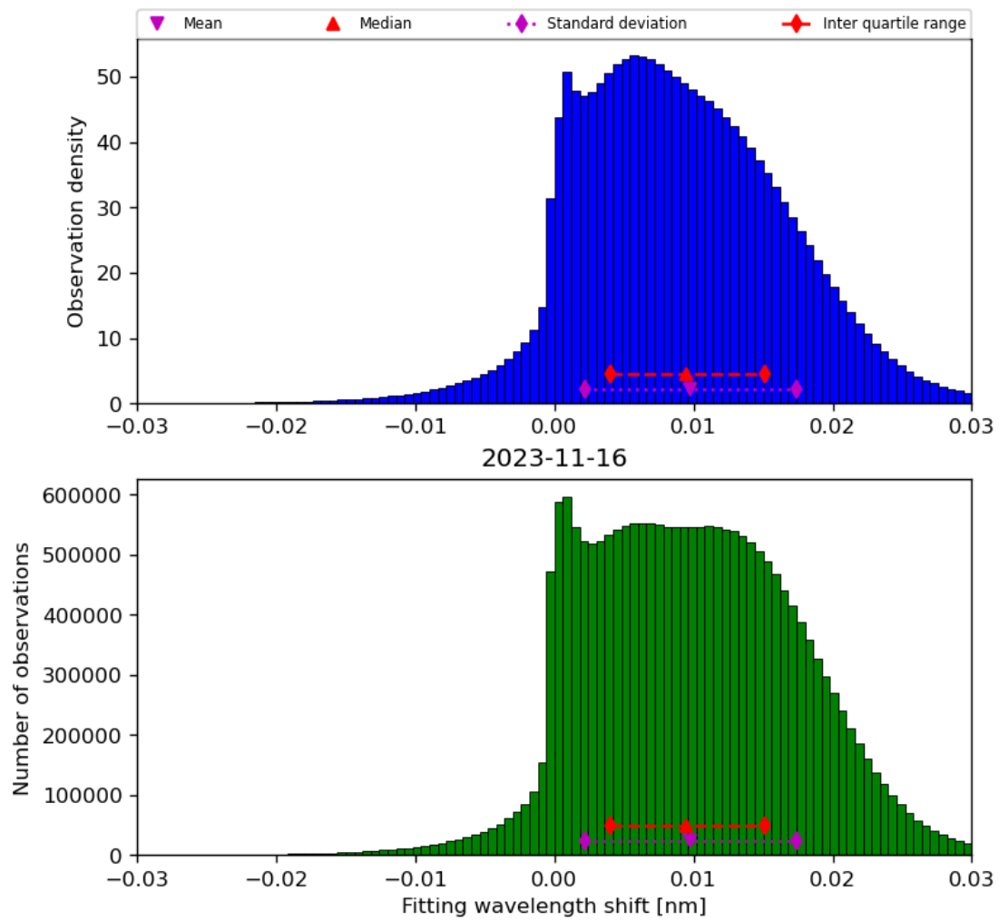
Figure 49: Histogram of “Fitting wavelength shift” for 2023-11-15 to 2023-11-17
