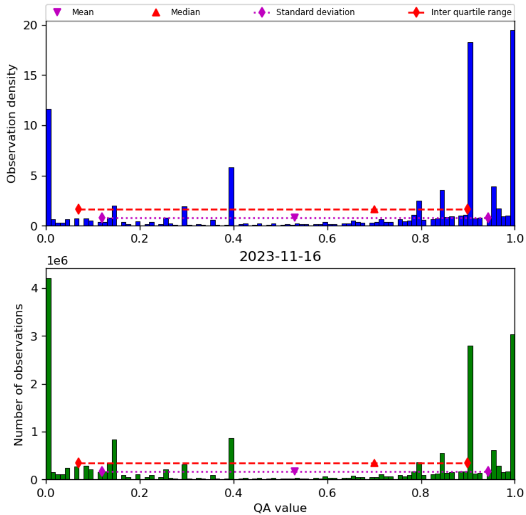
Figure 38: Histogram of “QA value” for 2023-11-15 to 2023-11-17
