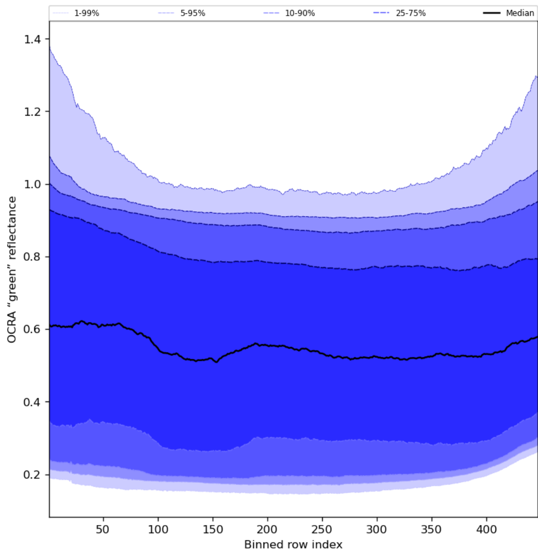
Figure 68: Along track statistics of “OCRA “green” reflectance” for 2023-11-15 to 2023-11-17
