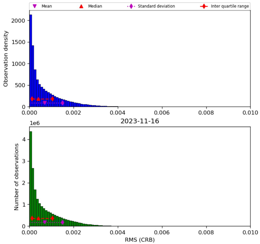
Figure 48: Histogram of “RMS (CRB)” for 2023-11-15 to 2023-11-17
