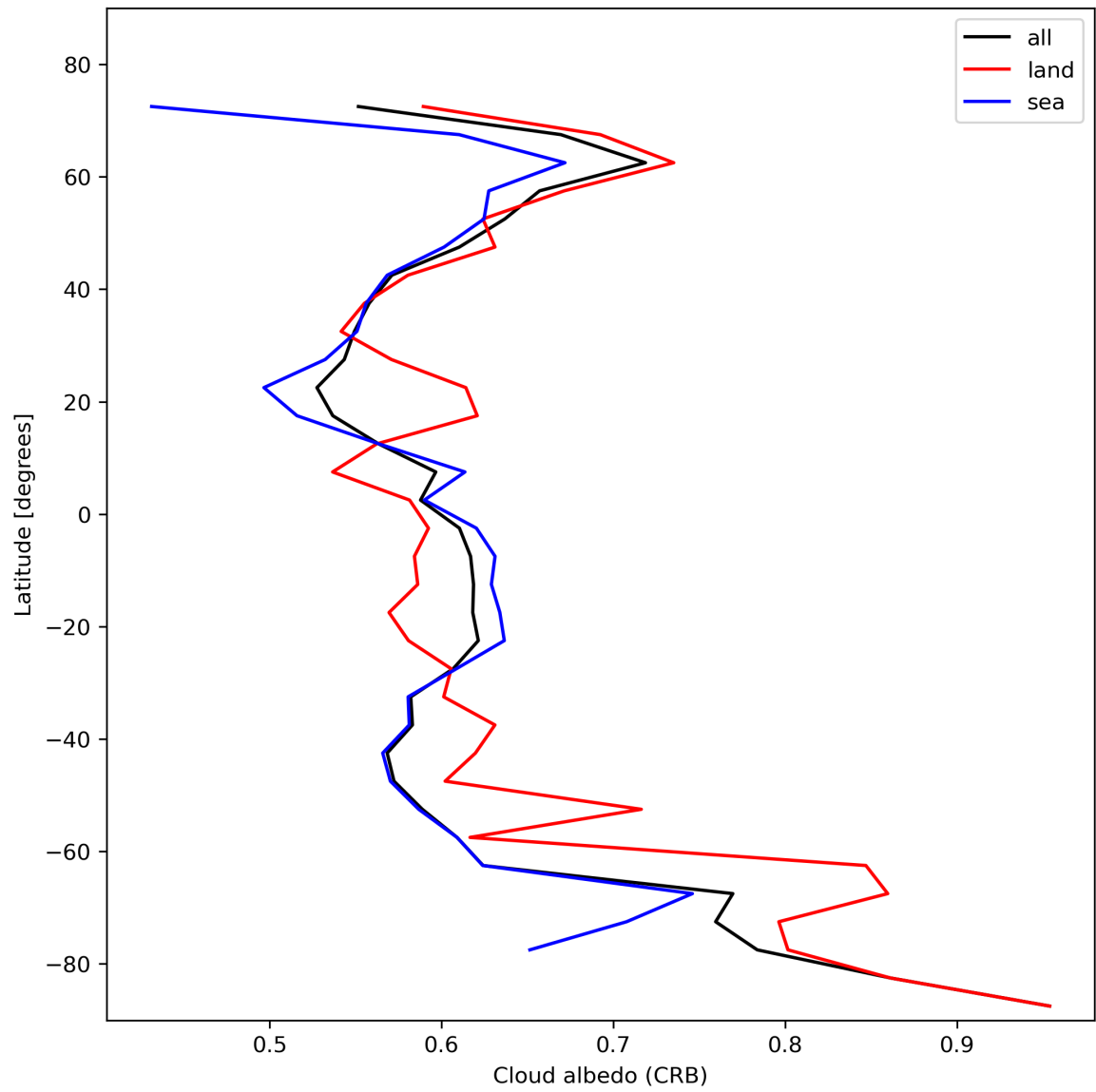
Figure 28: Zonal average of “Cloud albedo (CRB)” for 2023-11-15 to 2023-11-17.
