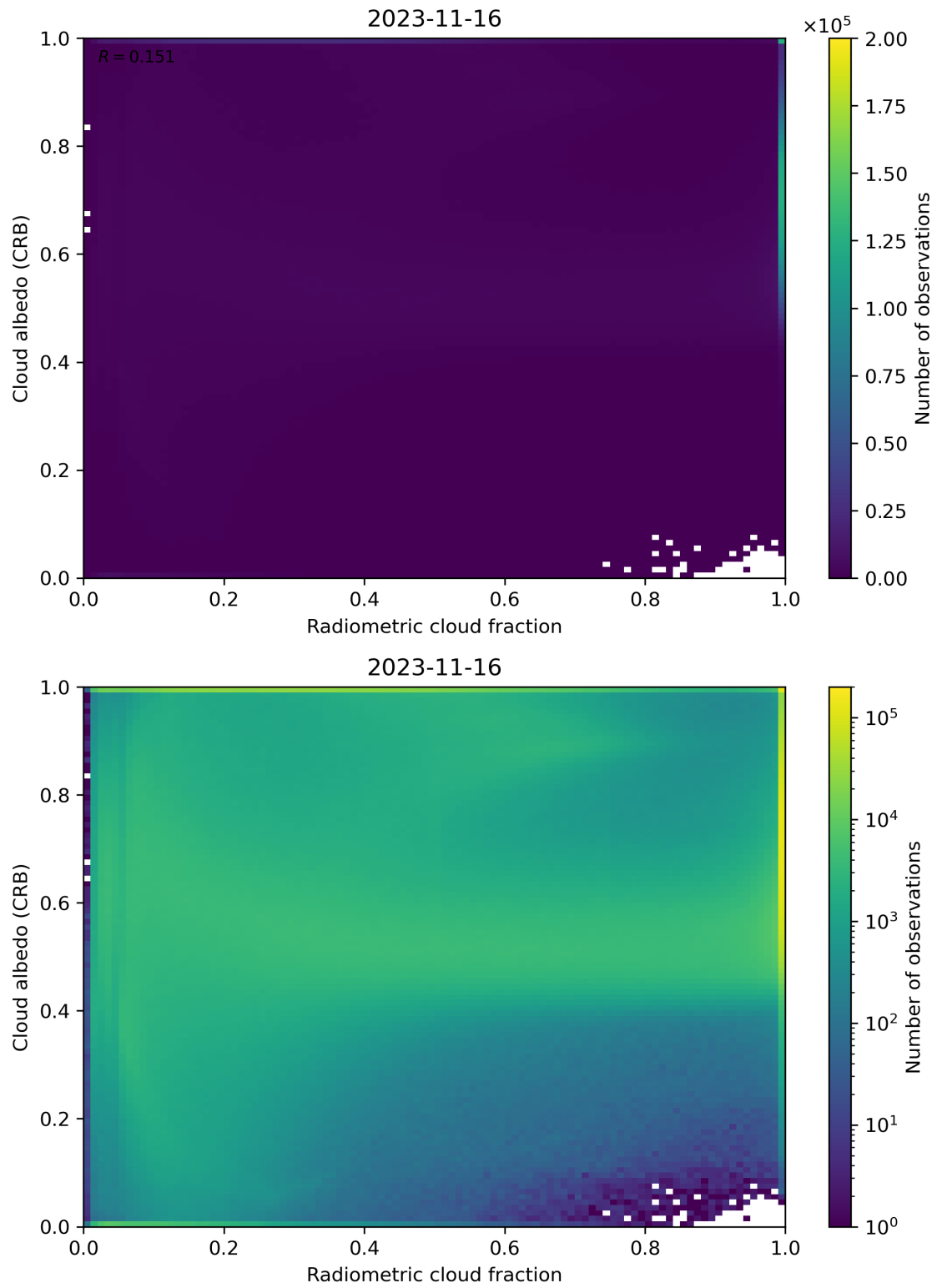
Figure 71: Scatter density plot of “Radiometric cloud fraction” against “Cloud albedo (CRB)” for 2023-11-15 to 2023-11-17.
