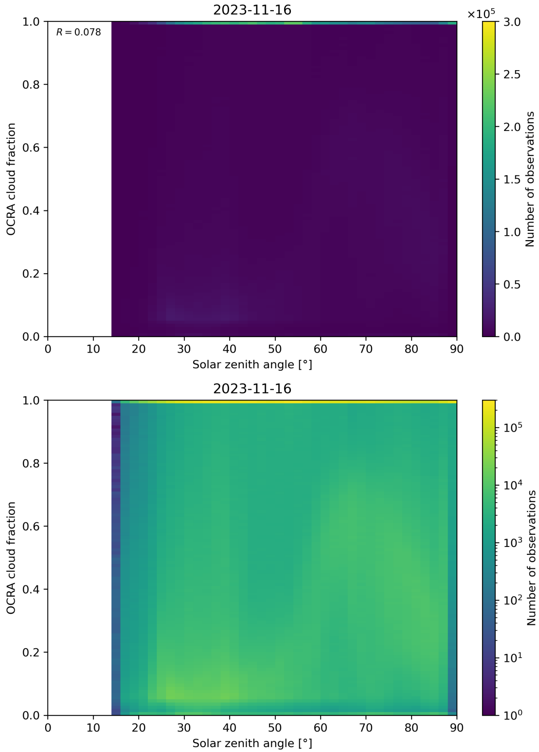
Figure 100: Scatter density plot of “Solar zenith angle” against “OCRA cloud fraction” for 2023-11-15 to 2023-11-17.
