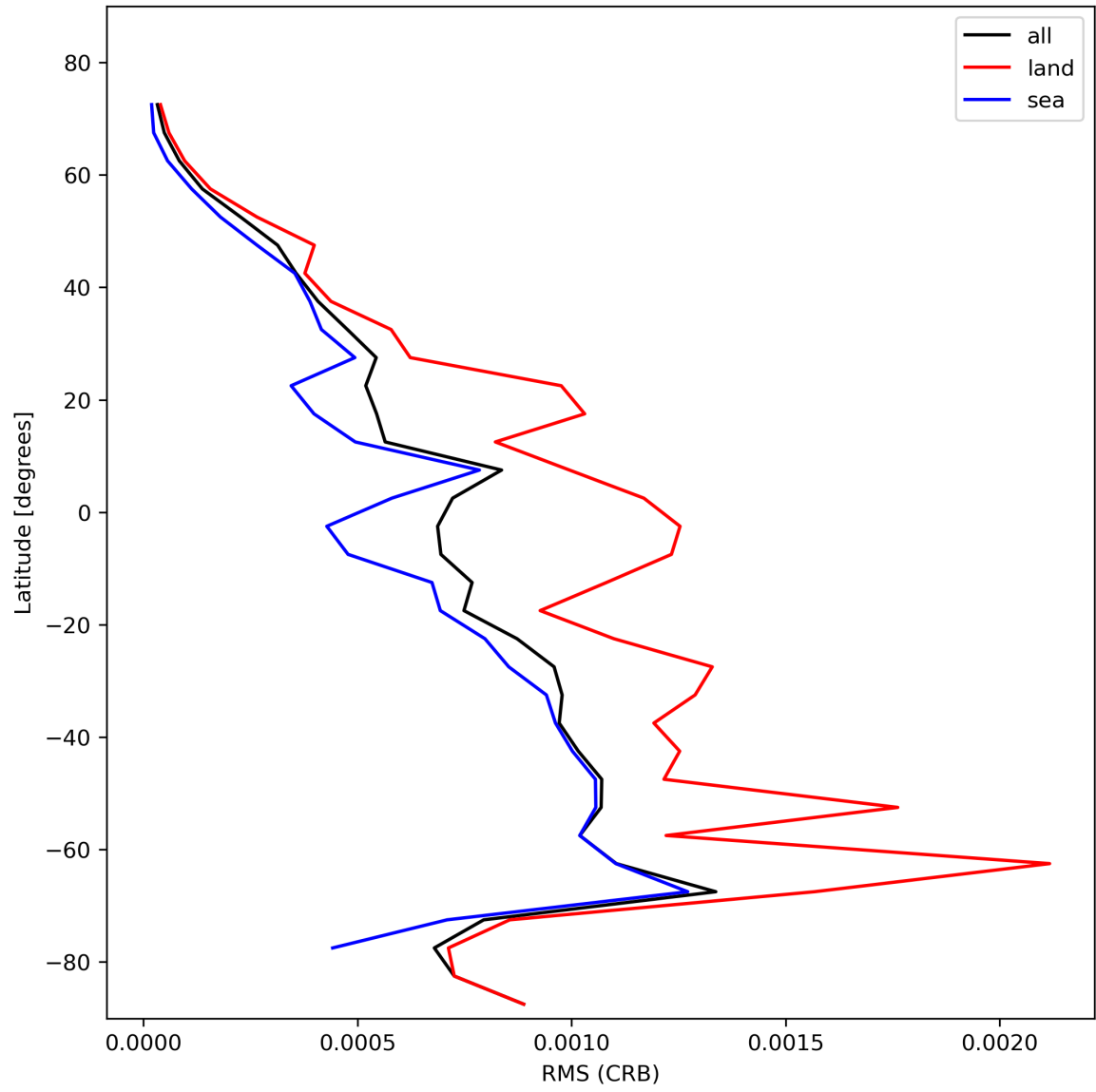
Figure 32: Zonal average of “RMS (CRB)” for 2023-11-15 to 2023-11-17.
