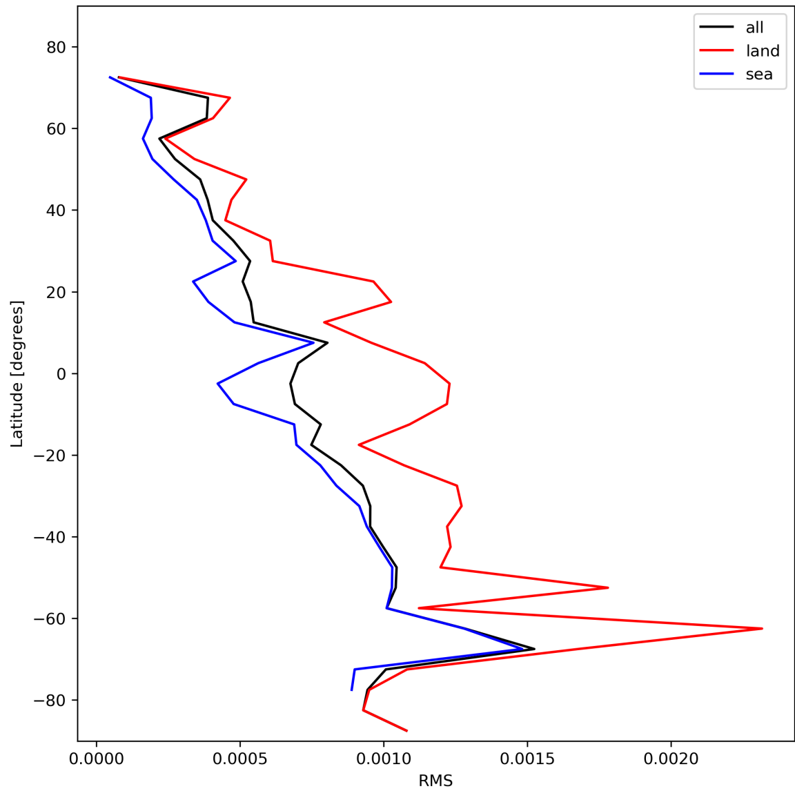
Figure 31: Zonal average of “RMS” for 2023-11-15 to 2023-11-17.
