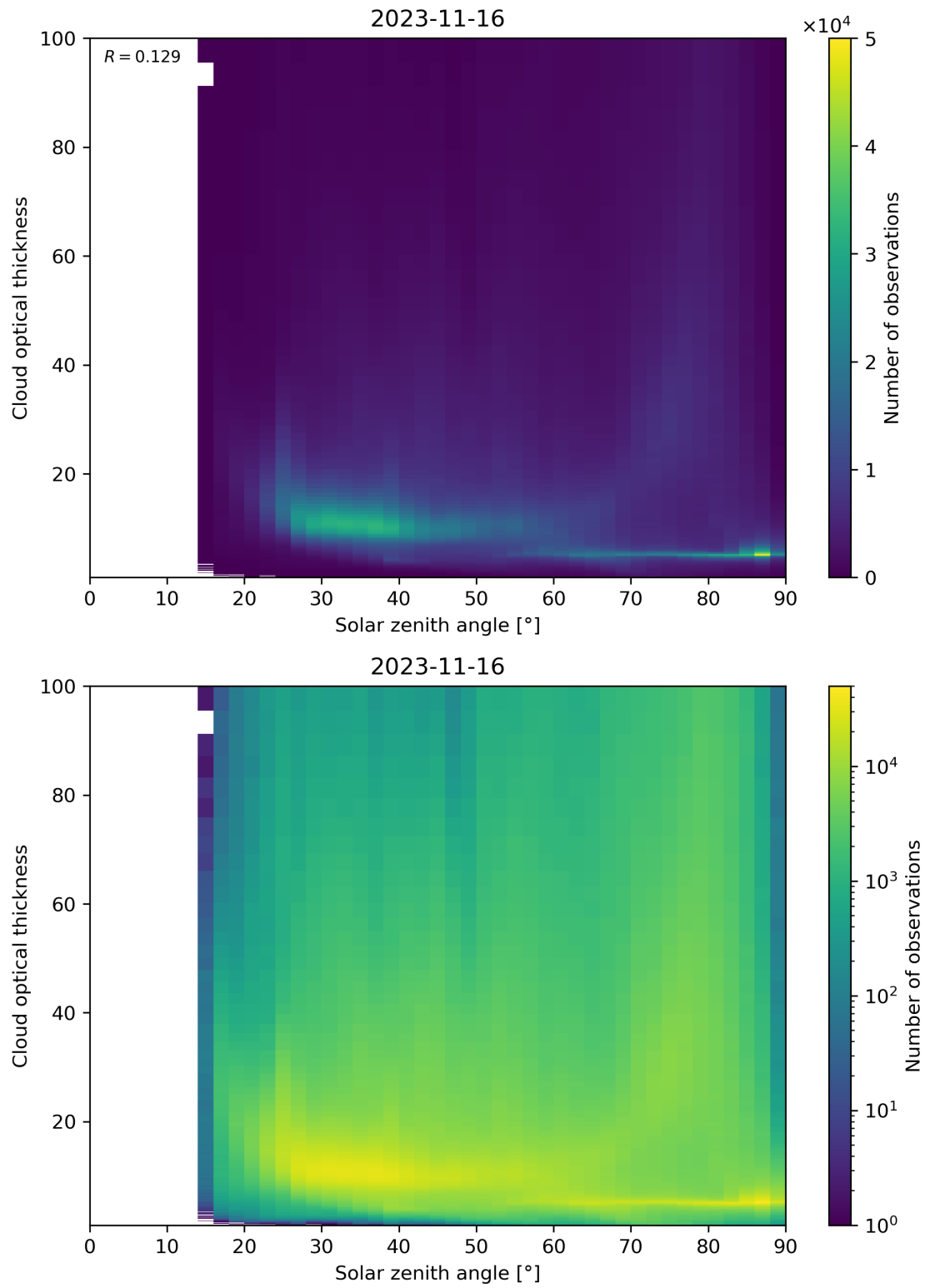
Figure 103: Scatter density plot of “Solar zenith angle” against “Cloud optical thickness” for 2023-11-15 to 2023-11-17.
