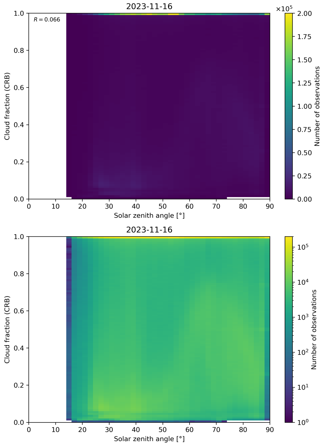
Figure 101: Scatter density plot of “Solar zenith angle” against “Cloud fraction (CRB)” for 2023-11-15 to 2023-11-17.
