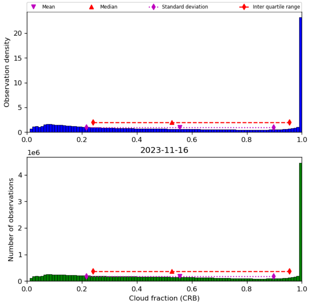
Figure 42: Histogram of “Cloud fraction (CRB)” for 2023-11-15 to 2023-11-17
