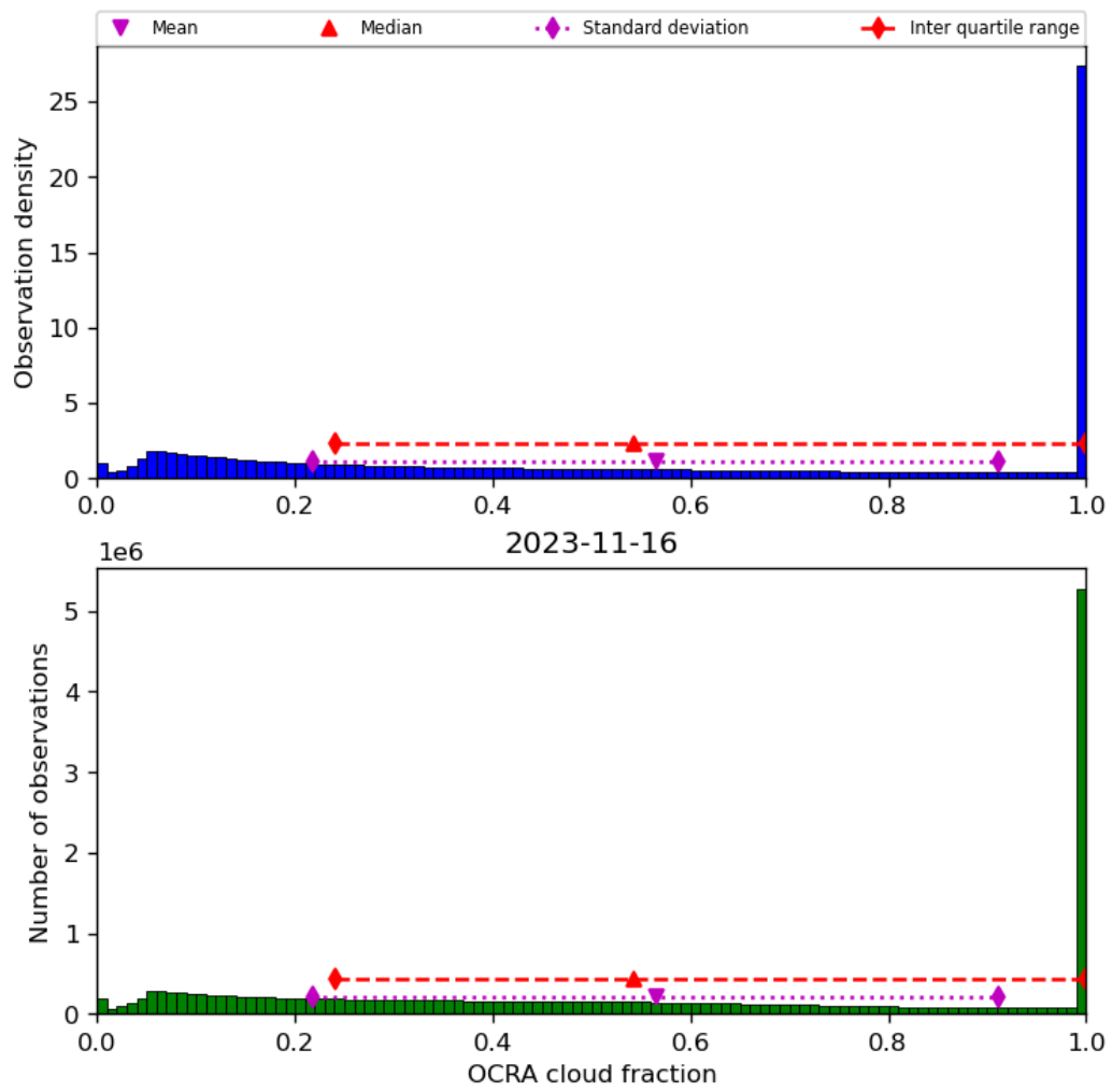
Figure 50: Histogram of “OCRA cloud fraction” for 2023-11-15 to 2023-11-17
