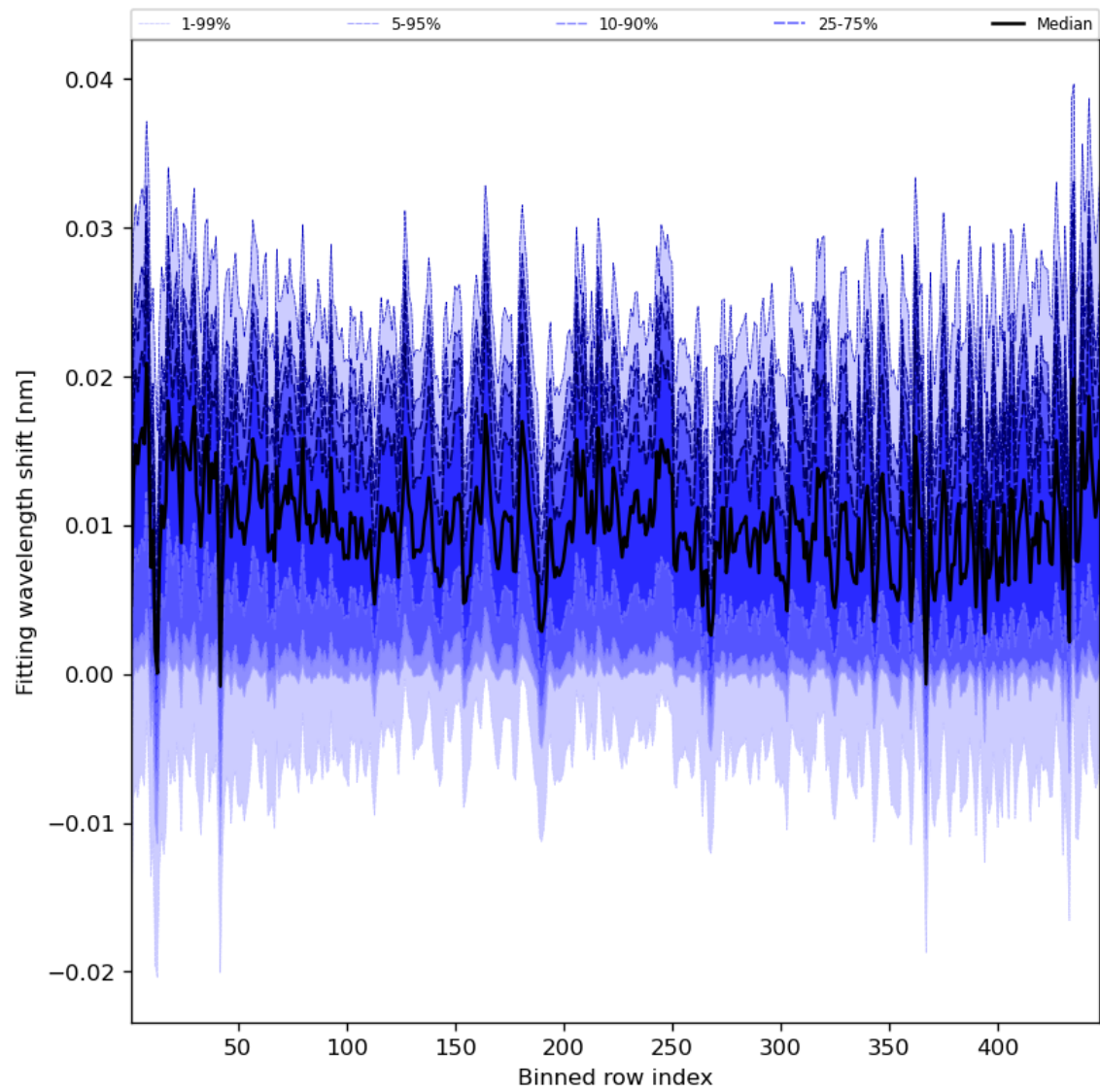
Figure 65: Along track statistics of “Fitting wavelength shift” for 2023-11-15 to 2023-11-17
