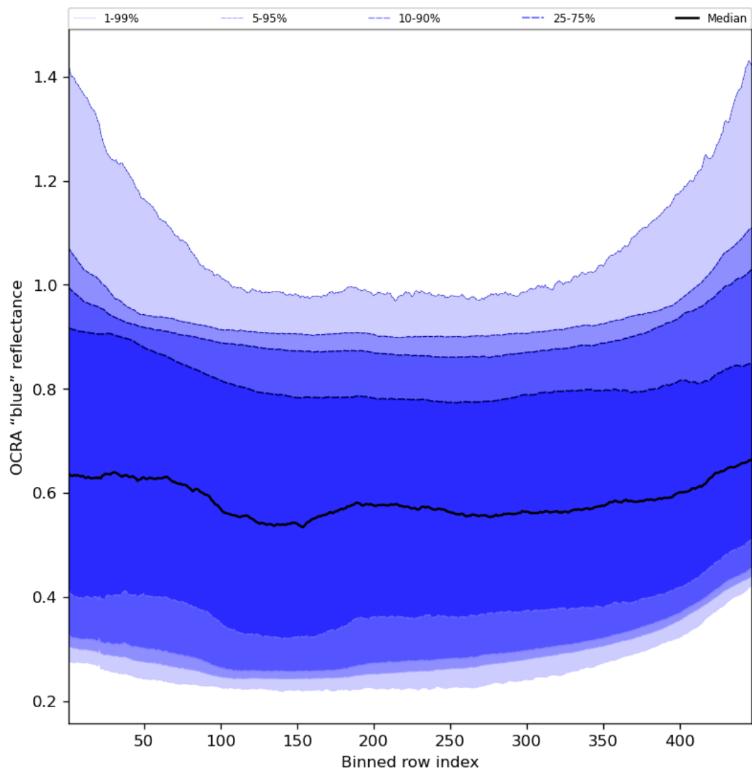
Figure 67: Along track statistics of “OCRA “blue” reflectance” for 2023-11-15 to 2023-11-17
