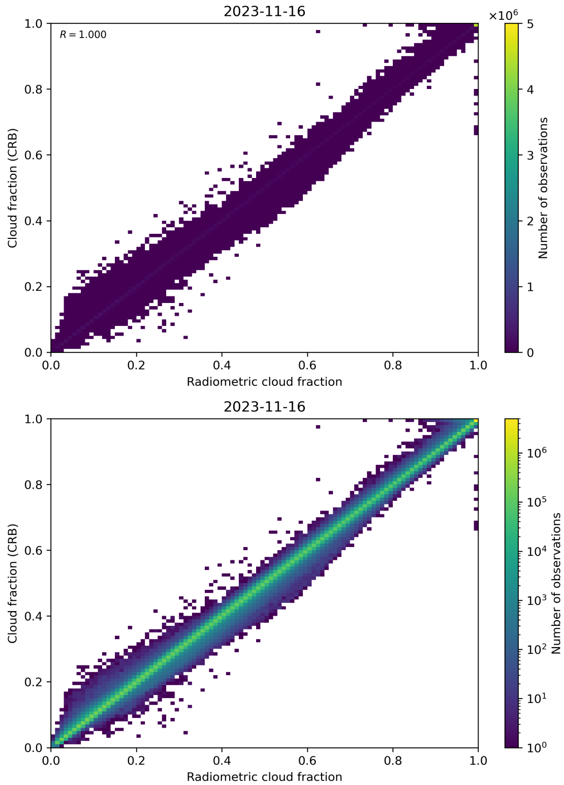
Figure 73: Scatter density plot of “Radiometric cloud fraction” against “Cloud fraction (CRB)” for 2023-11-15 to 2023-11-17.
