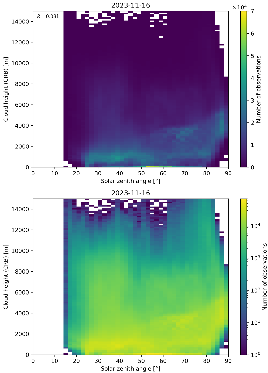
Figure 102: Scatter density plot of “Solar zenith angle” against “Cloud height (CRB)” for 2023-11-15 to 2023-11-17.
