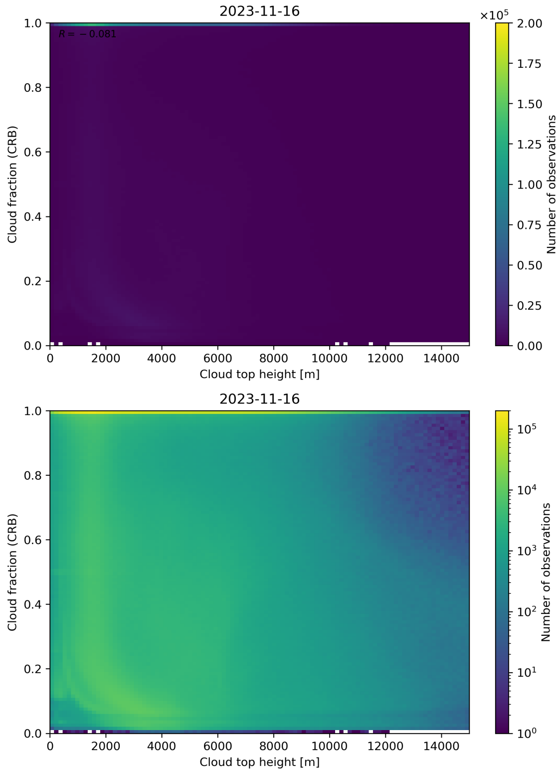
Figure 88: Scatter density plot of “Cloud top height” against “Cloud fraction (CRB)” for 2023-11-15 to 2023-11-17.
