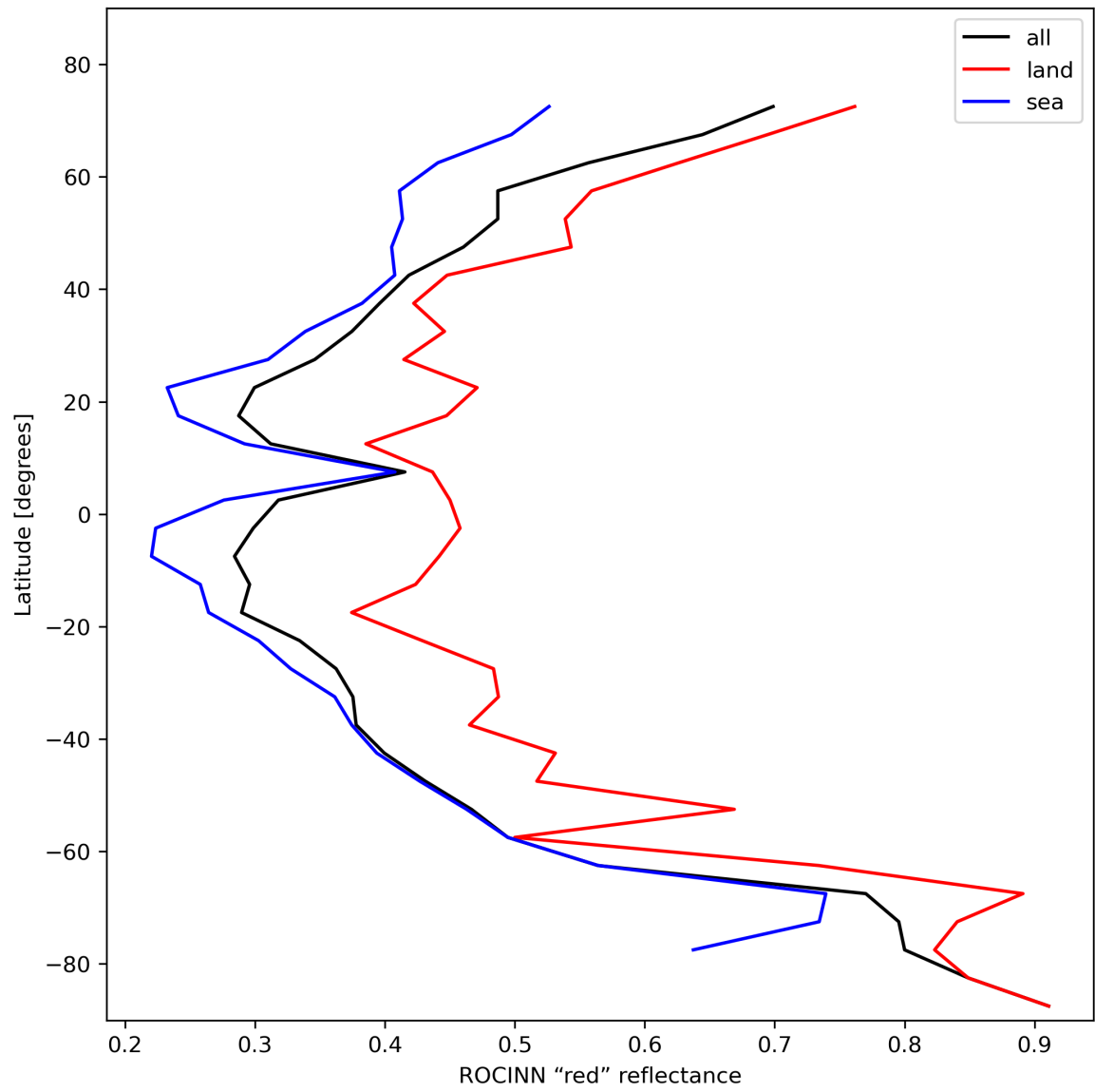
Figure 37: Zonal average of “ROCINN “red” reflectance” for 2023-11-15 to 2023-11-17.
