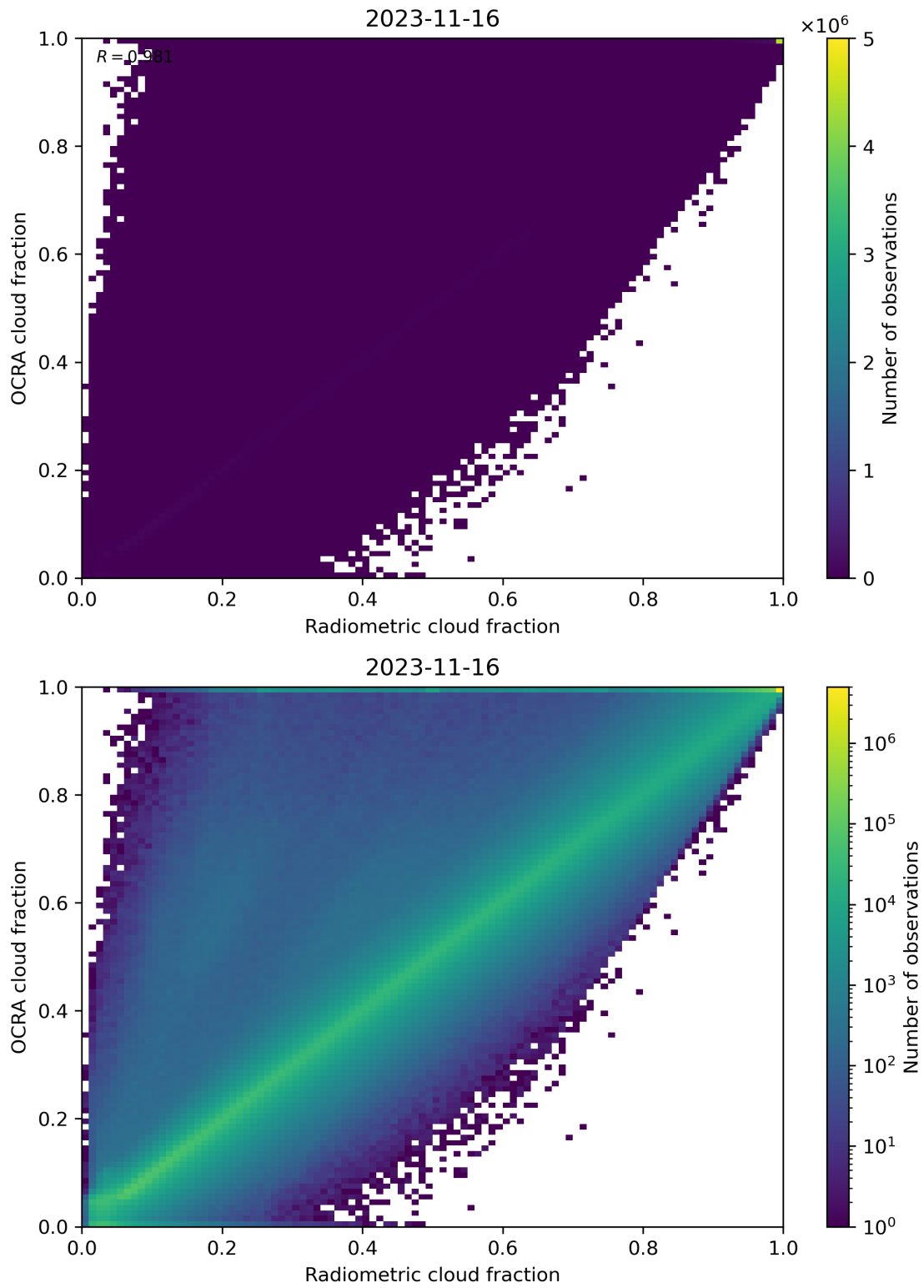
Figure 72: Scatter density plot of “Radiometric cloud fraction” against “OCRA cloud fraction” for 2023-11-15 to 2023-11-17.
