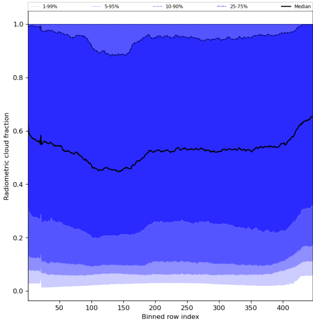
Figure 55: Along track statistics of “Radiometric cloud fraction” for 2023-11-15 to 2023-11-17
