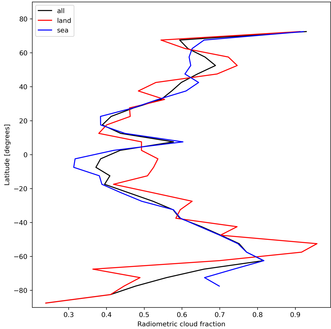
Figure 23: Zonal average of “Radiometric cloud fraction” for 2023-11-15 to 2023-11-17.
