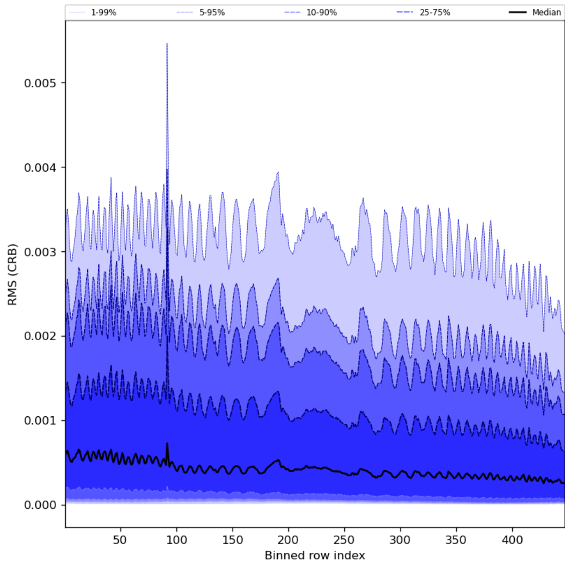
Figure 64: Along track statistics of “RMS (CRB)” for 2023-11-15 to 2023-11-17
