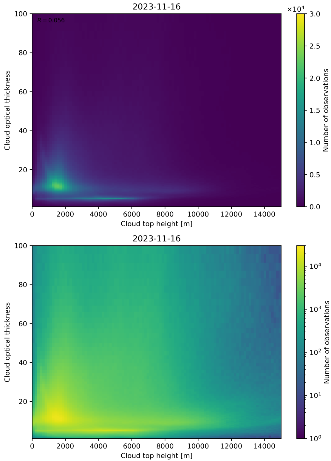
Figure 90: Scatter density plot of “Cloud top height” against “Cloud optical thickness” for 2023-11-15 to 2023-11-17.
