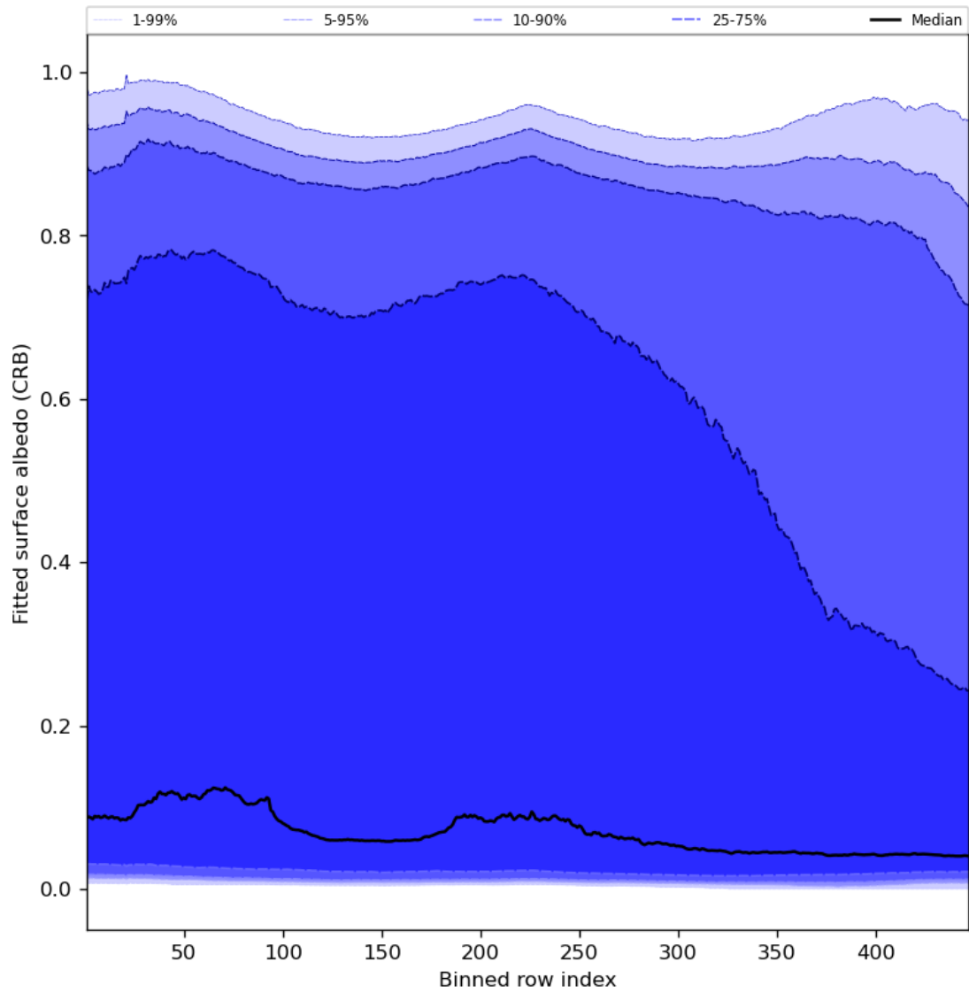
Figure 62: Along track statistics of “Fitted surface albedo (CRB)” for 2023-11-15 to 2023-11-17
