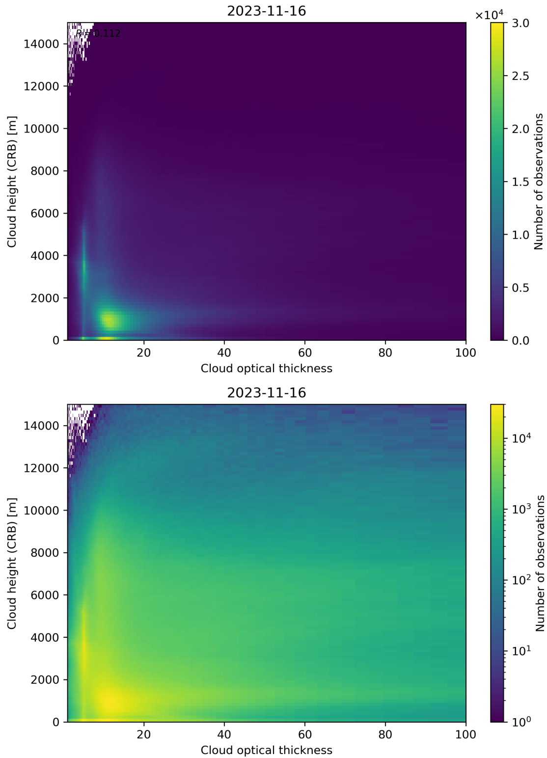
Figure 85: Scatter density plot of “Cloud optical thickness” against “Cloud height (CRB)” for 2023-11-15 to 2023-11-17.
