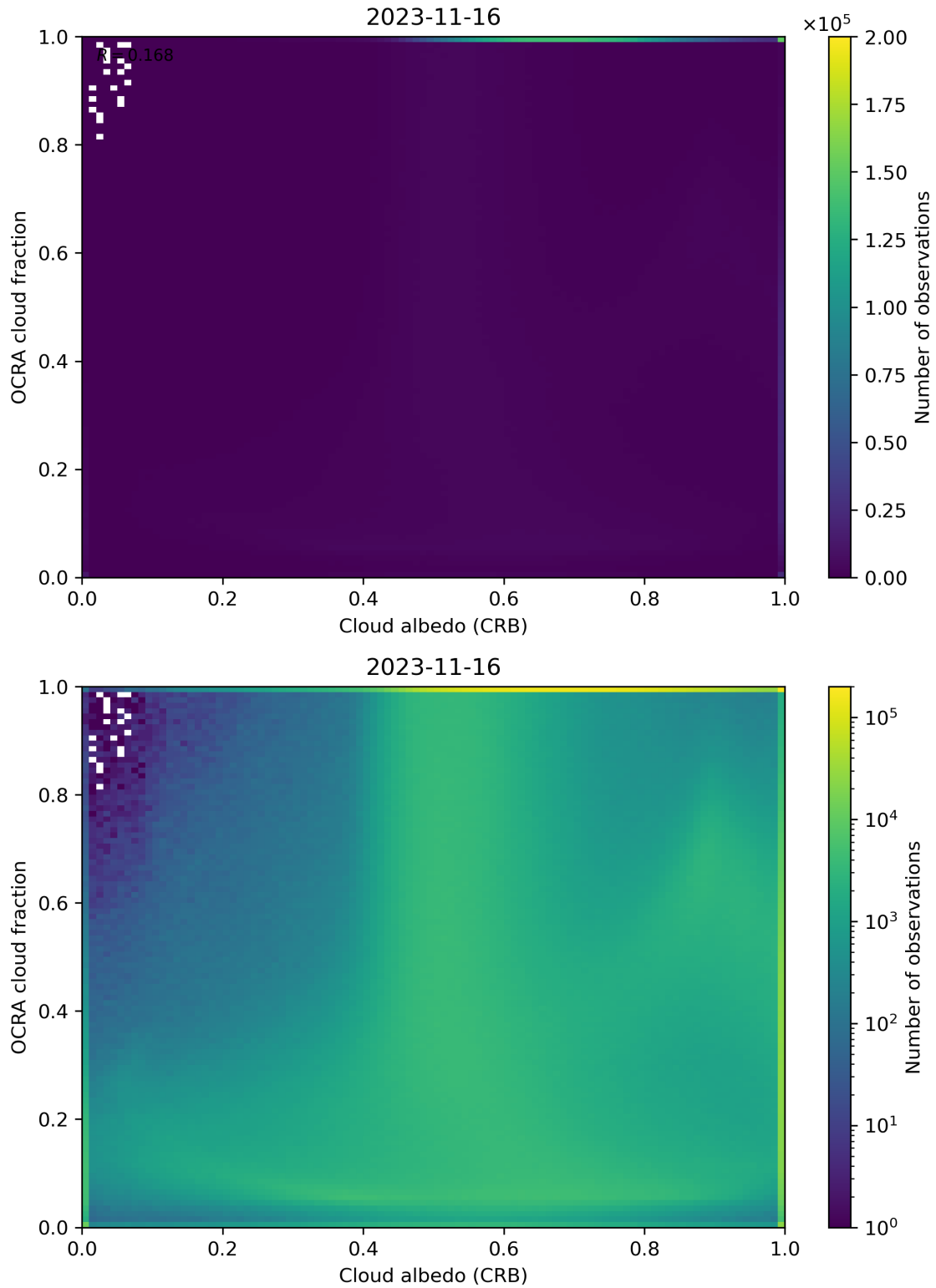
Figure 70: Scatter density plot of “Cloud albedo (CRB)” against “OCRA cloud fraction” for 2023-11-15 to 2023-11-17.
