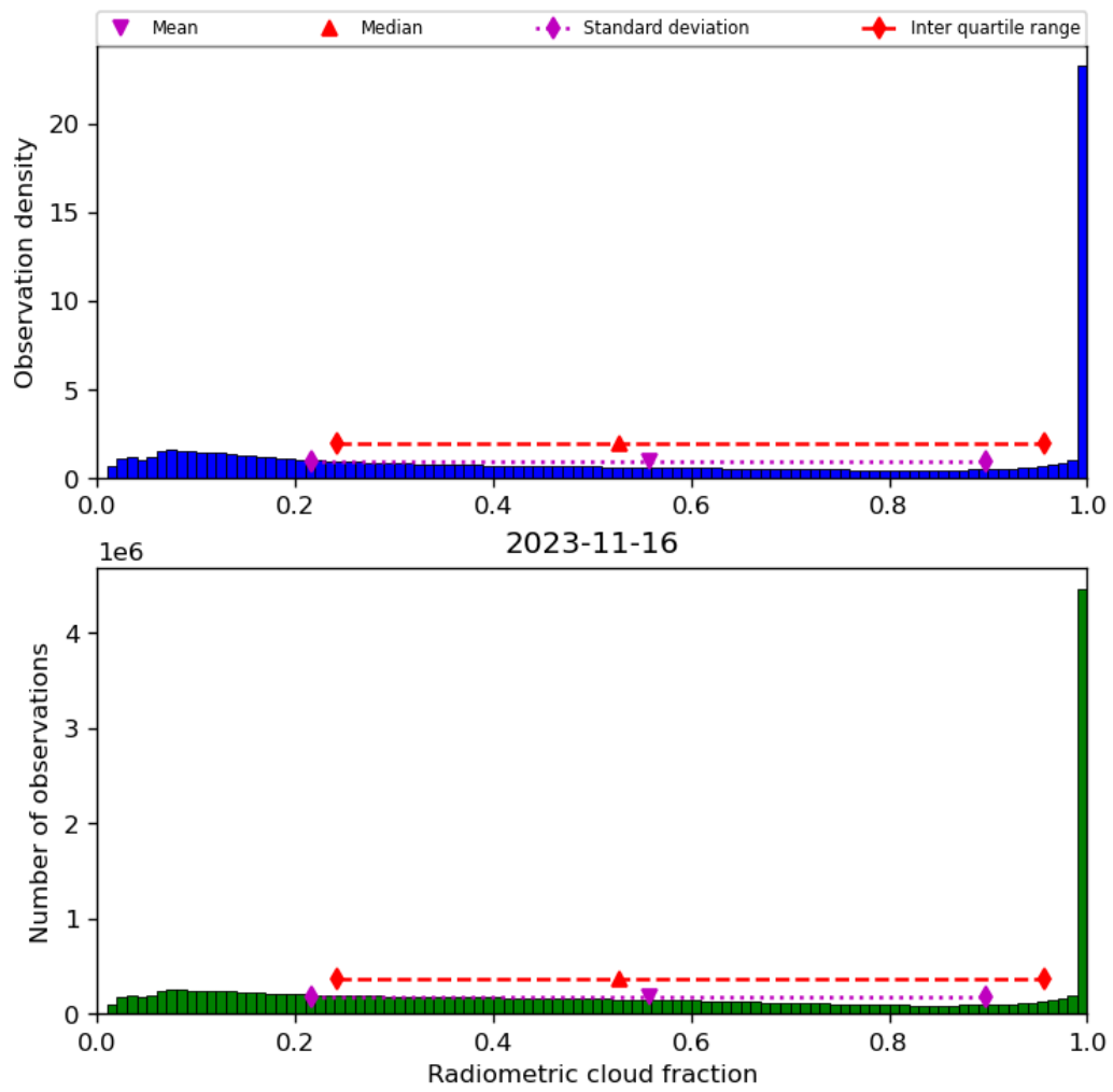
Figure 39: Histogram of “Radiometric cloud fraction” for 2023-11-15 to 2023-11-17
