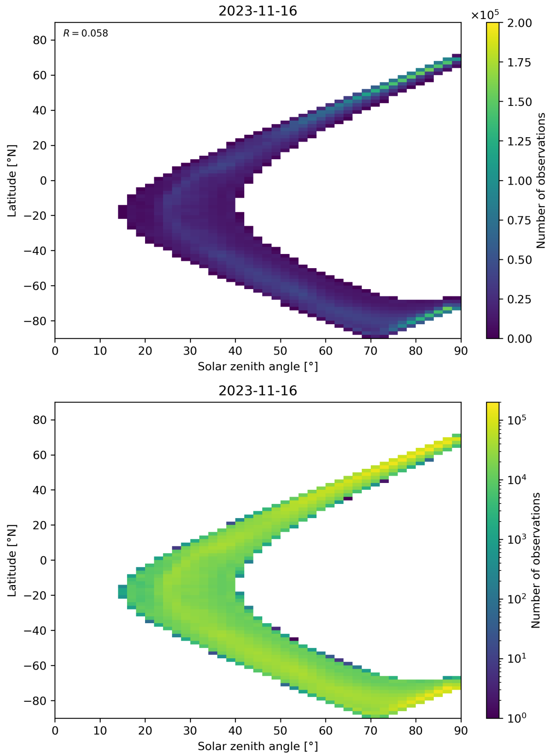
Figure 105: Scatter density plot of “Solar zenith angle” against “Latitude” for 2023-11-15 to 2023-11-17.
