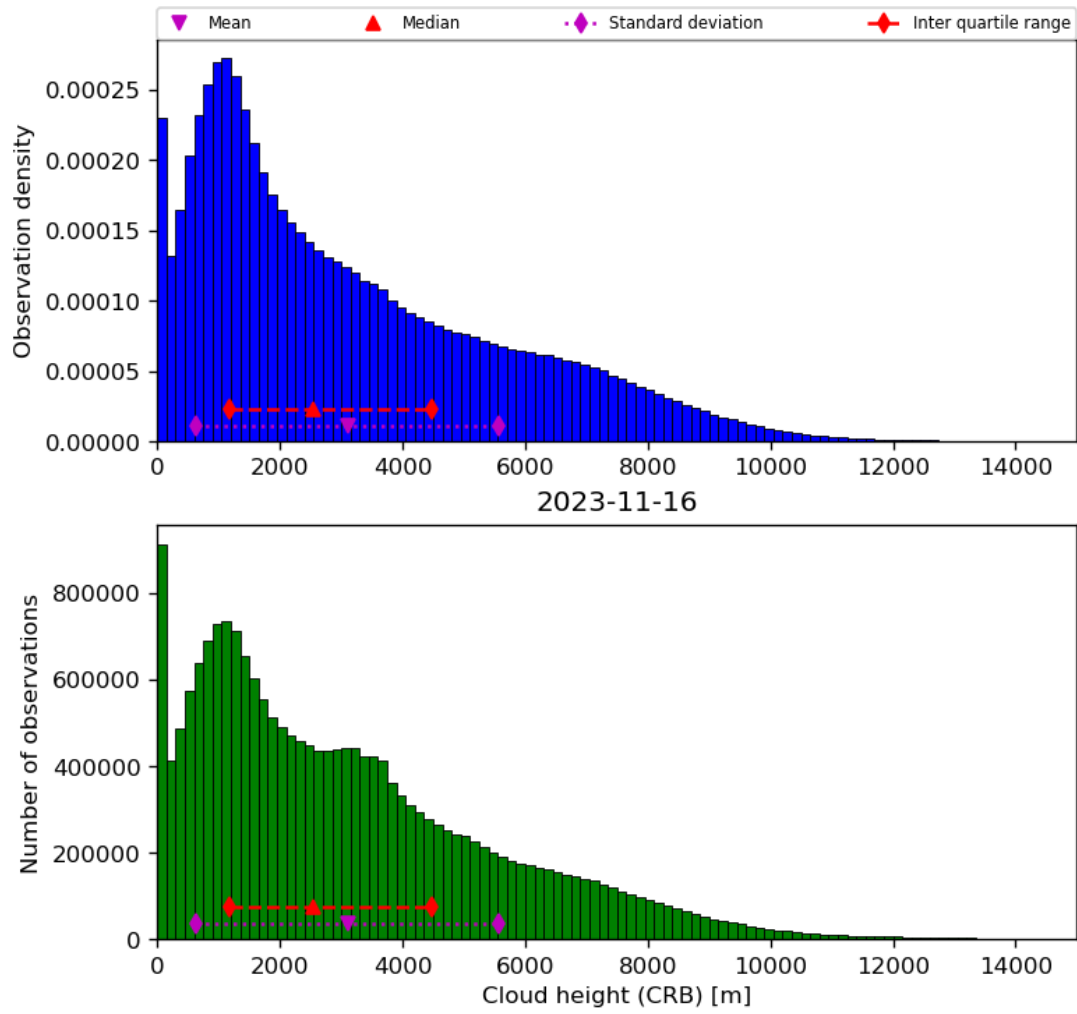
Figure 43: Histogram of “Cloud height (CRB)” for 2023-11-15 to 2023-11-17
