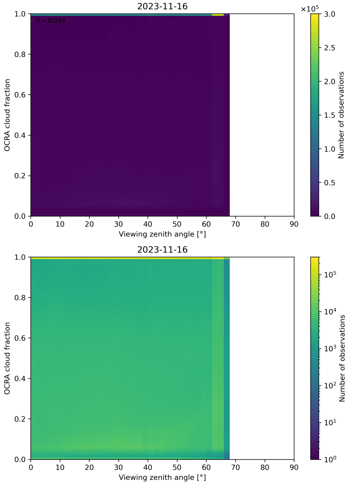
Figure 108: Scatter density plot of “Viewing zenith angle” against “OCRA cloud fraction” for 2023-11-15 to 2023-11-17.
