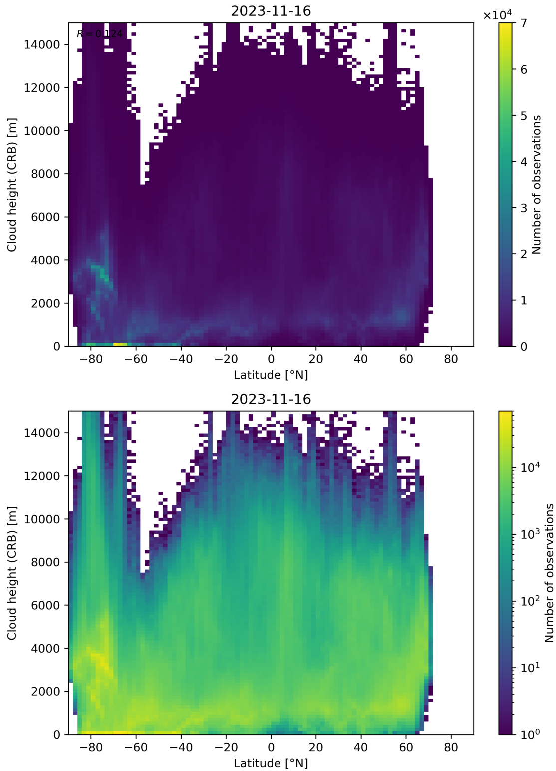
Figure 95: Scatter density plot of “Latitude” against “Cloud height (CRB)” for 2023-11-15 to 2023-11-17.
