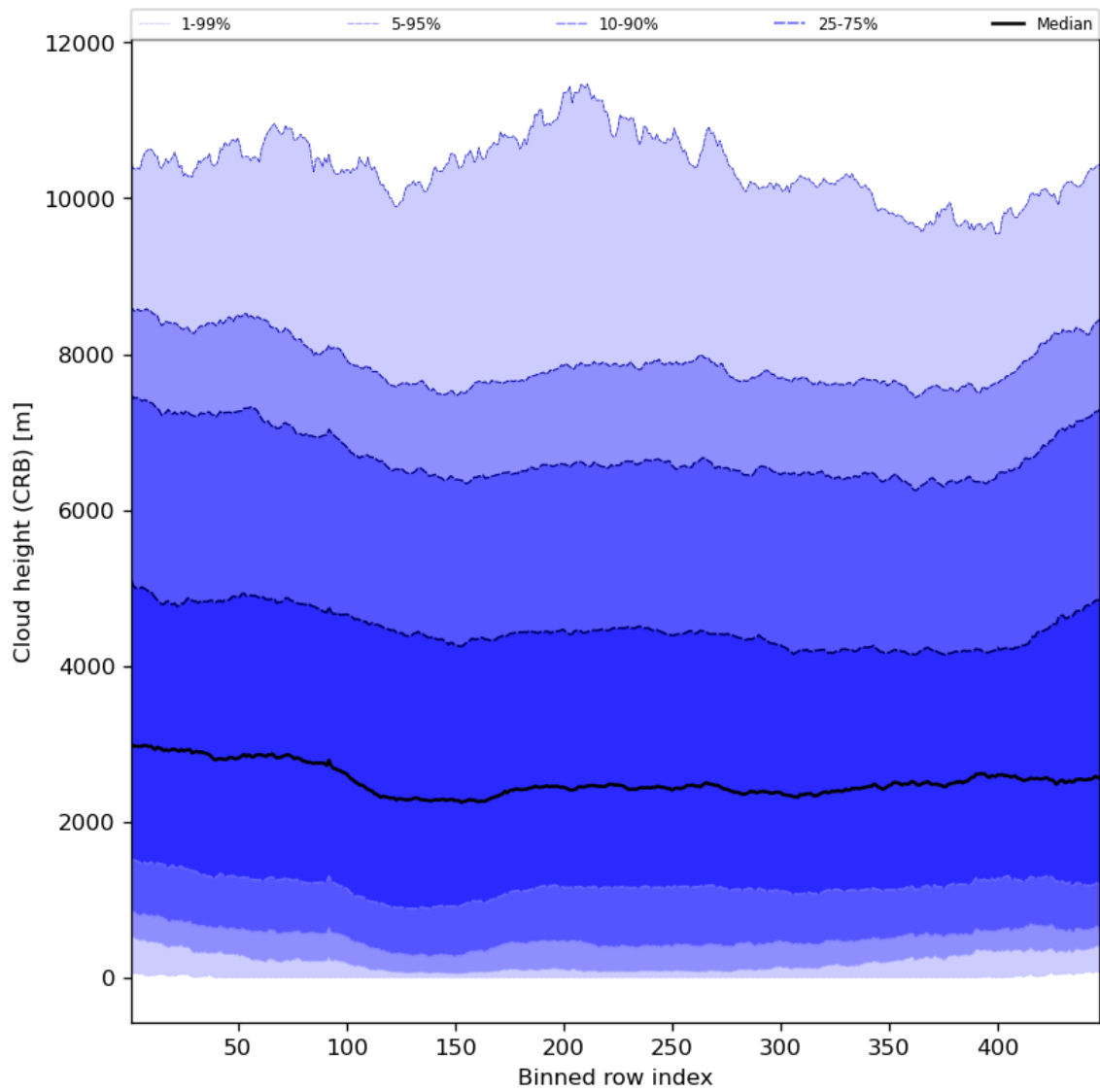
Figure 59: Along track statistics of “Cloud height (CRB)” for 2023-11-15 to 2023-11-17
