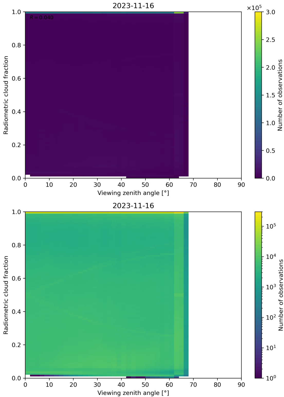
Figure 107: Scatter density plot of “Viewing zenith angle” against “Radiometric cloud fraction” for 2023-11-15 to 2023-11-17.
