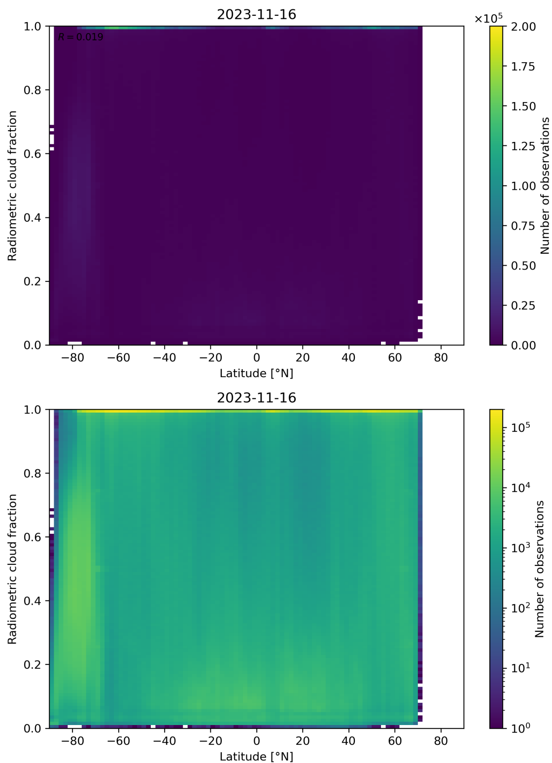
Figure 92: Scatter density plot of “Latitude” against “Radiometric cloud fraction” for 2023-11-15 to 2023-11-17.
