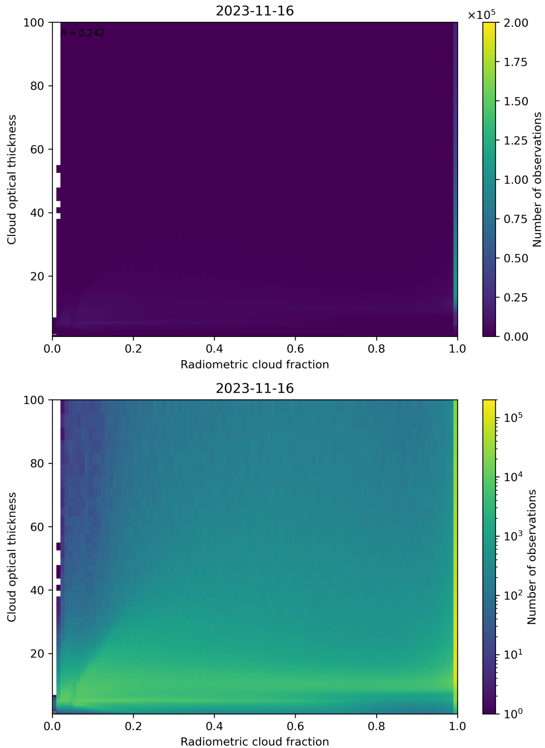
Figure 75: Scatter density plot of “Radiometric cloud fraction” against “Cloud optical thickness” for 2023-11-15 to 2023-11-17.
