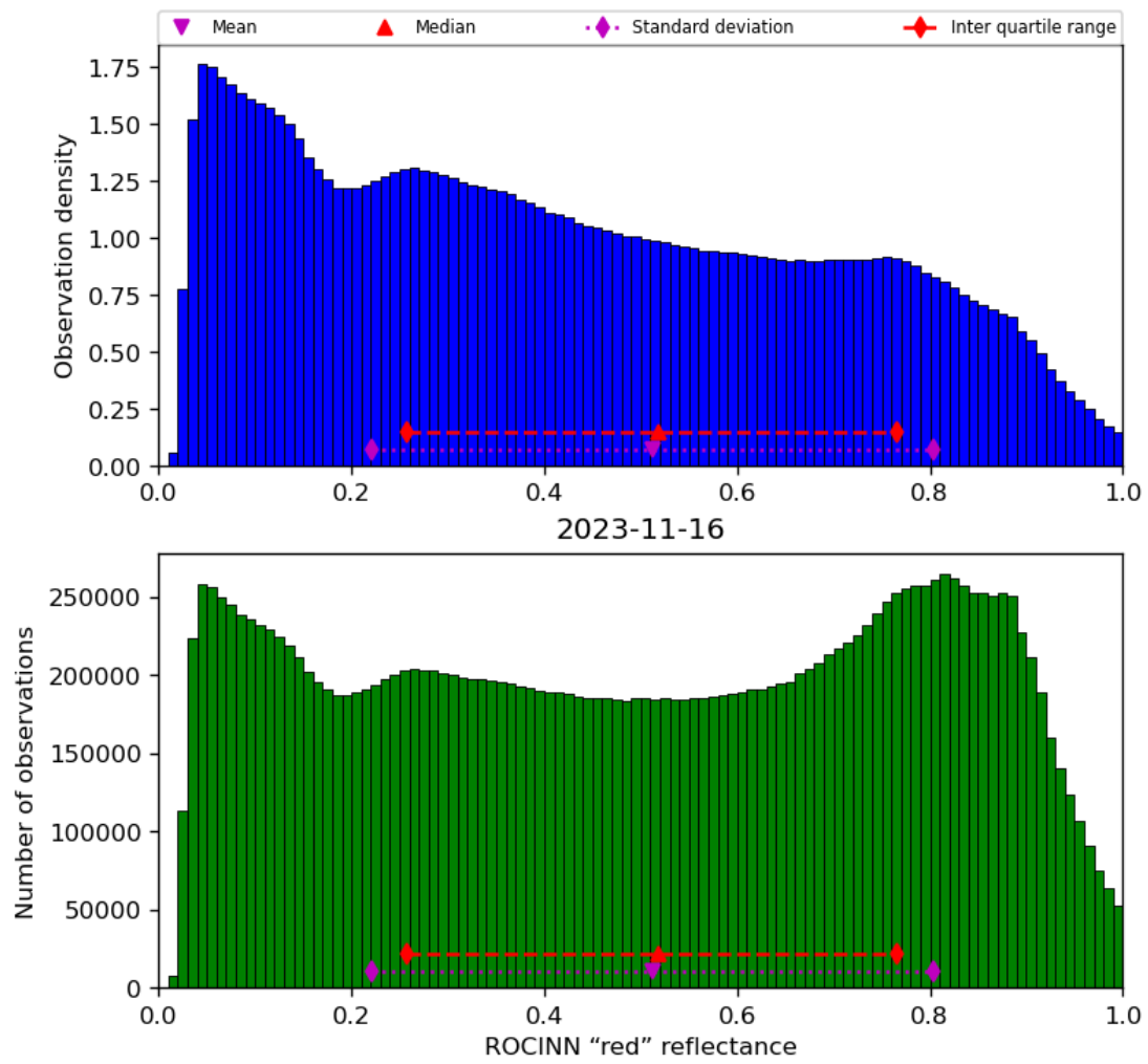
Figure 53: Histogram of “ROCINN “red” reflectance” for 2023-11-15 to 2023-11-17
