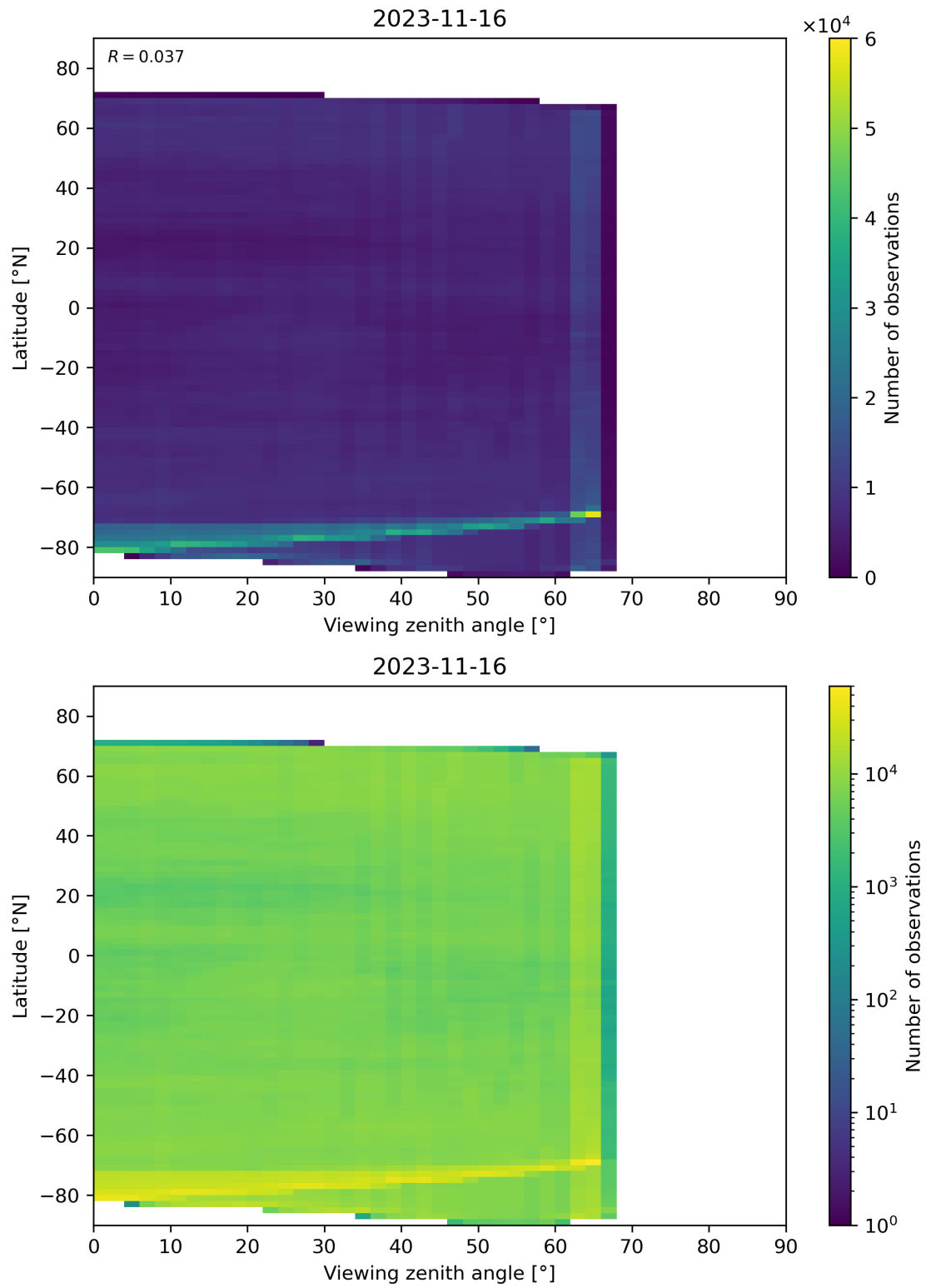
Figure 113: Scatter density plot of “Viewing zenith angle” against “Latitude” for 2023-11-15 to 2023-11-17.
