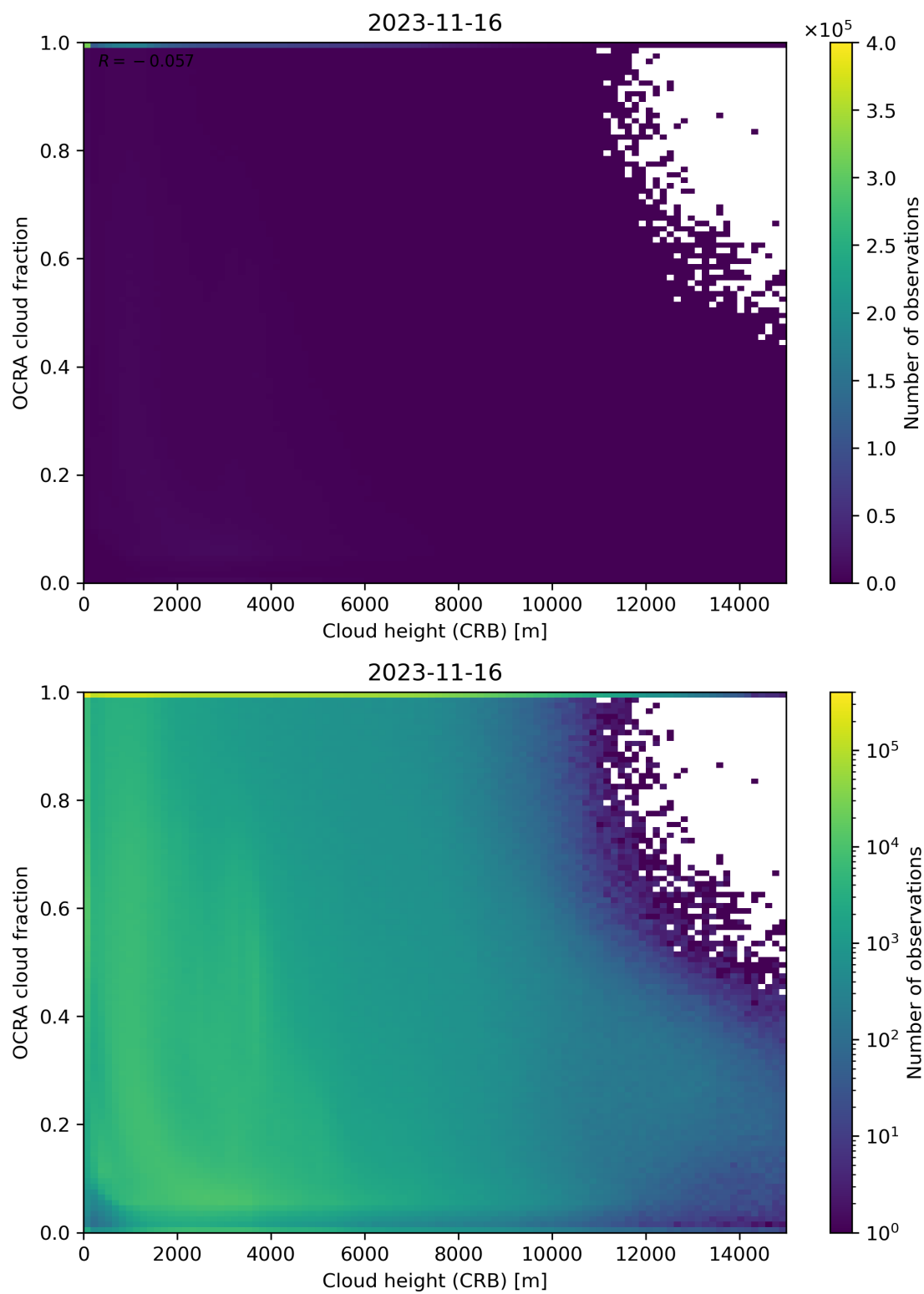
Figure 81: Scatter density plot of “Cloud height (CRB)” against “OCRA cloud fraction” for 2023-11-15 to 2023-11-17.
