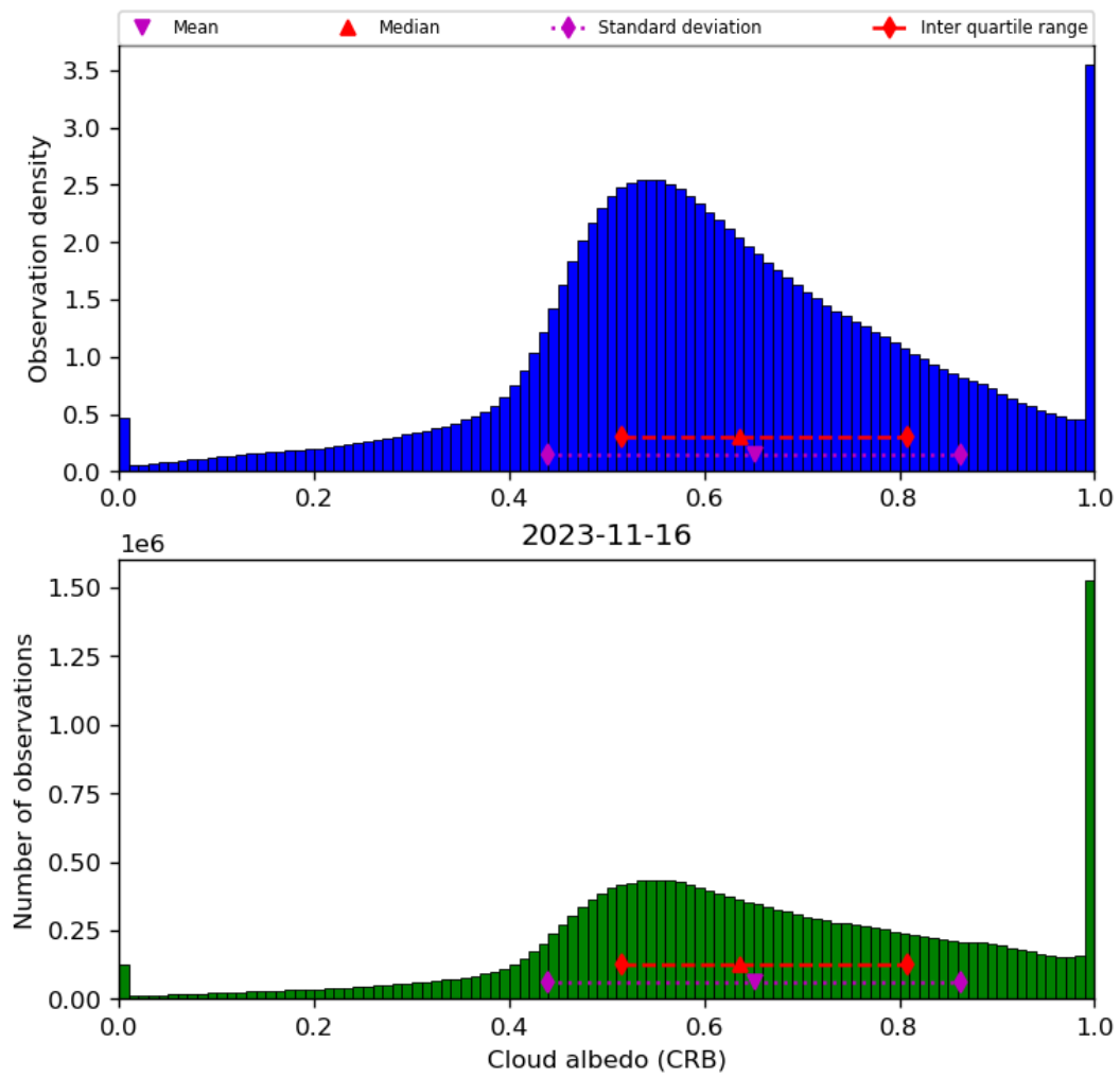
Figure 44: Histogram of “Cloud albedo (CRB)” for 2023-11-15 to 2023-11-17
