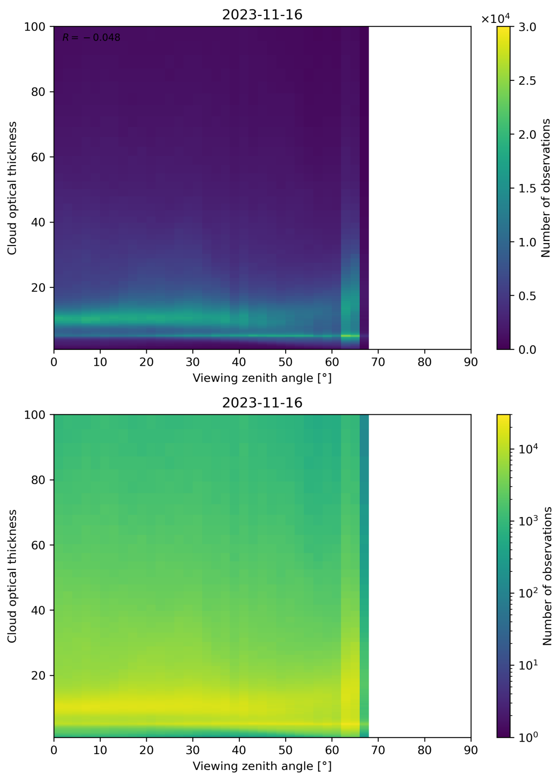
Figure 111: Scatter density plot of “Viewing zenith angle” against “Cloud optical thickness” for 2023-11-15 to 2023-11-17.
