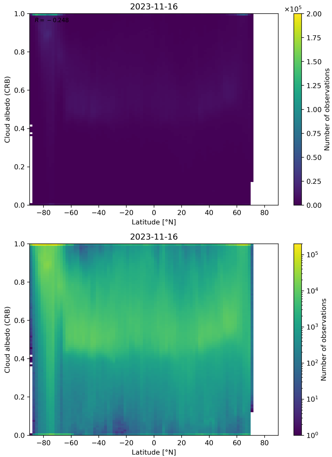
Figure 91: Scatter density plot of “Latitude” against “Cloud albedo (CRB)” for 2023-11-15 to 2023-11-17.
