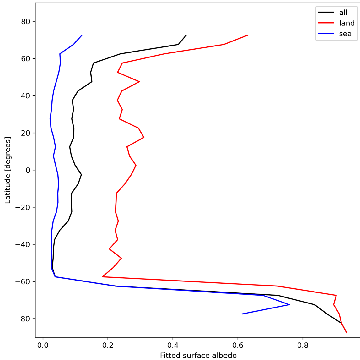
Figure 29: Zonal average of “Fitted surface albedo” for 2023-11-15 to 2023-11-17.
