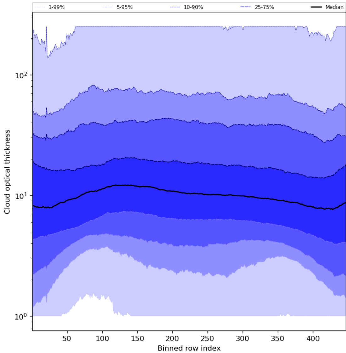
Figure 57: Along track statistics of “Cloud optical thickness” for 2023-11-15 to 2023-11-17
