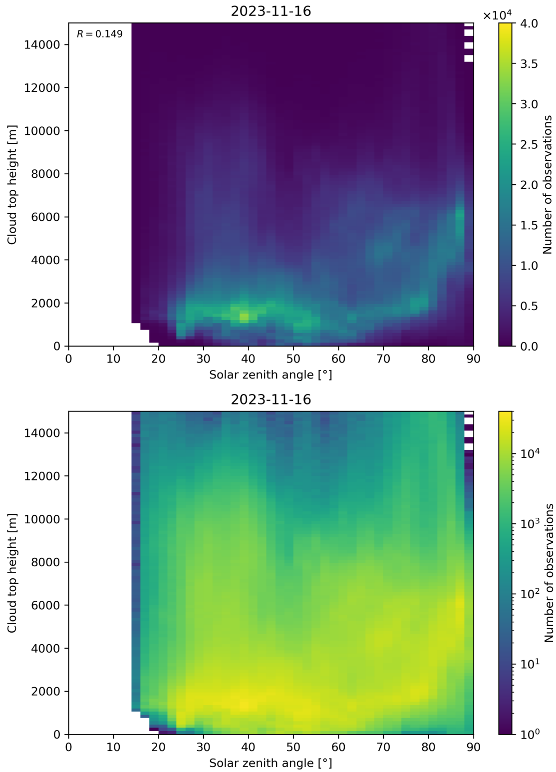
Figure 104: Scatter density plot of “Solar zenith angle” against “Cloud top height” for 2023-11-15 to 2023-11-17.
