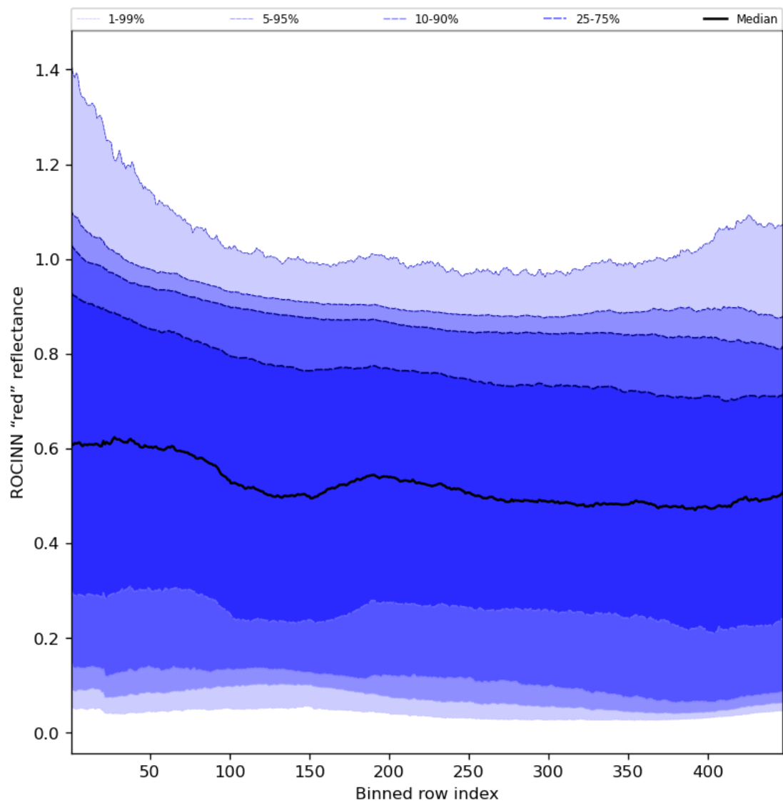
Figure 69: Along track statistics of “ROCINN “red” reflectance” for 2023-11-15 to 2023-11-17
