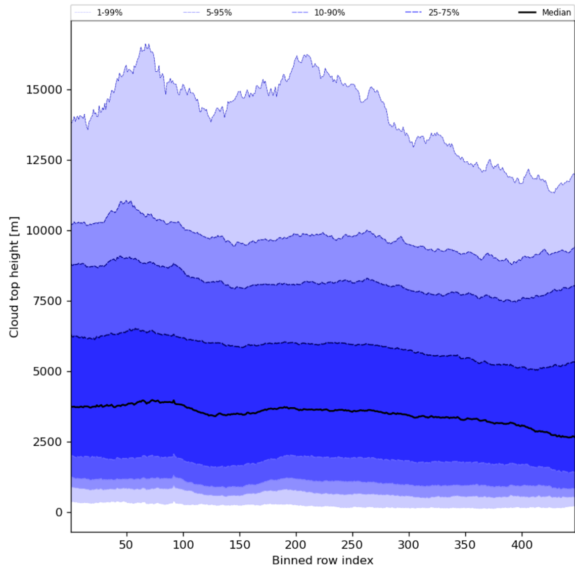
Figure 56: Along track statistics of “Cloud top height” for 2023-11-15 to 2023-11-17
