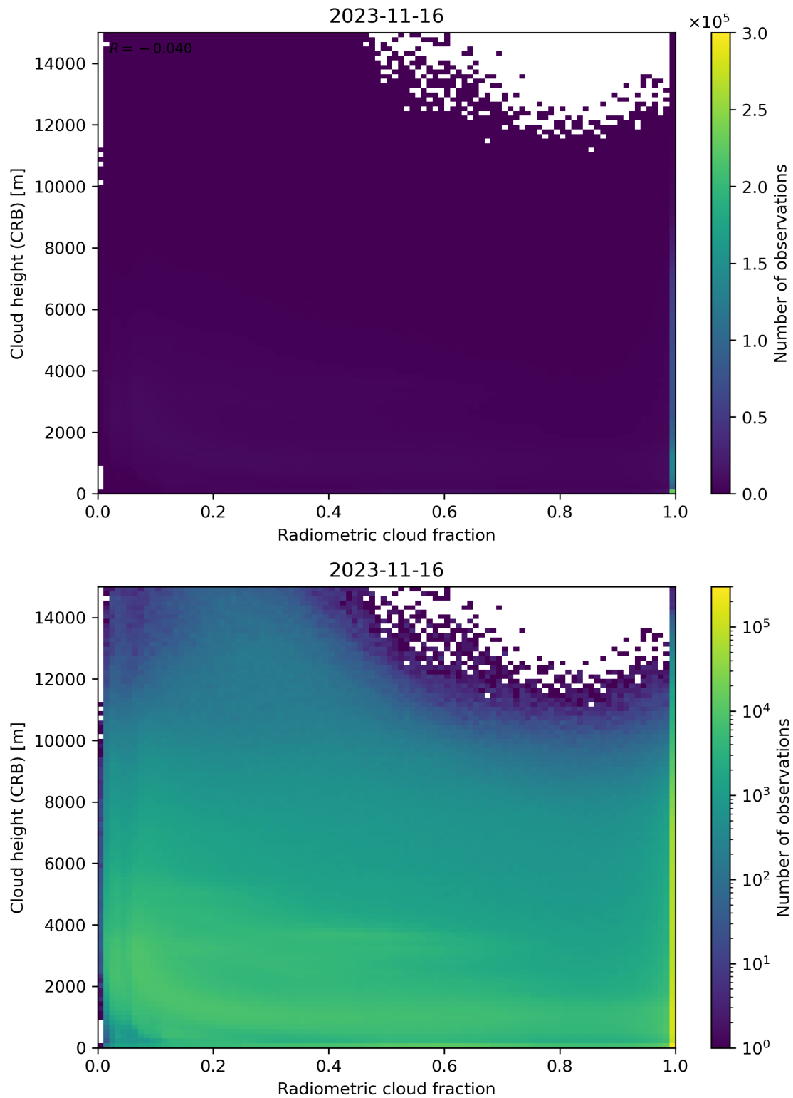
Figure 74: Scatter density plot of “Radiometric cloud fraction” against “Cloud height (CRB)” for 2023-11-15 to 2023-11-17.
