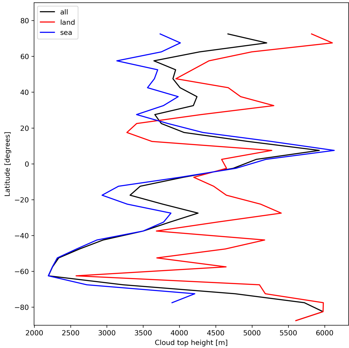
Figure 24: Zonal average of “Cloud top height” for 2023-11-15 to 2023-11-17.
