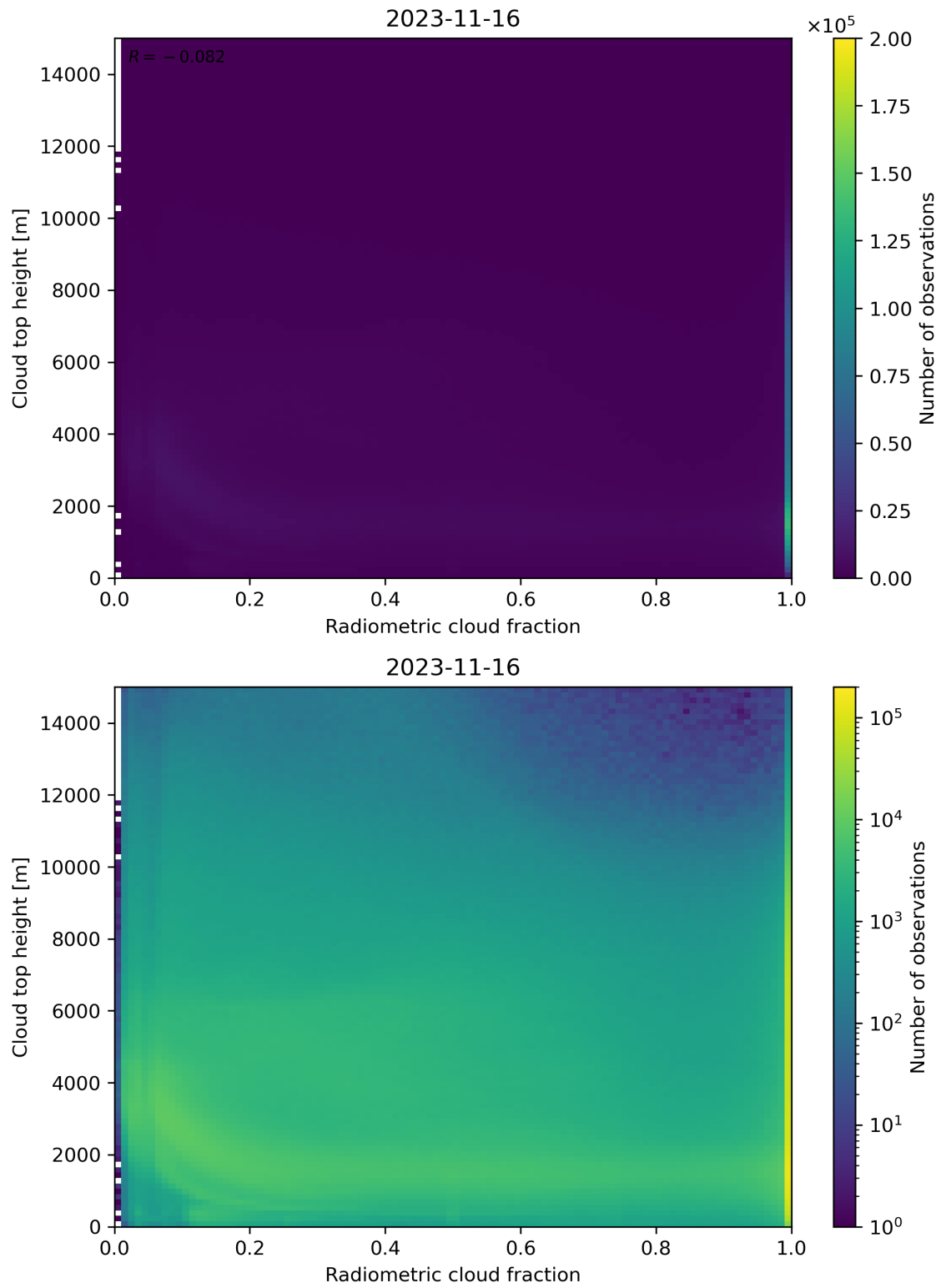
Figure 76: Scatter density plot of “Radiometric cloud fraction” against “Cloud top height” for 2023-11-15 to 2023-11-17.
