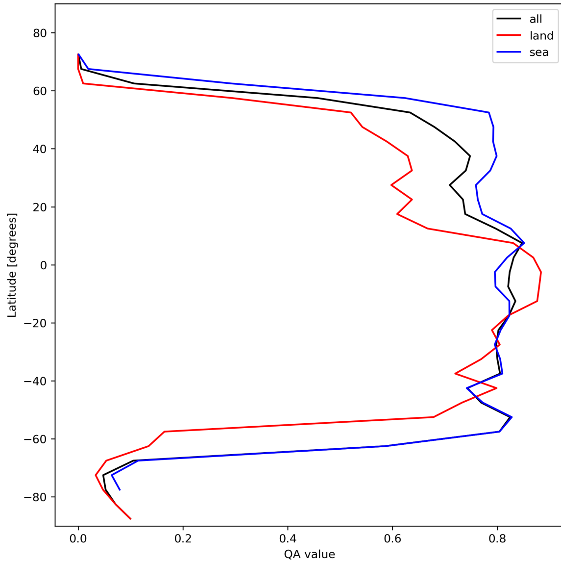
Figure 22: Zonal average of “QA value” for 2023-11-15 to 2023-11-17.
