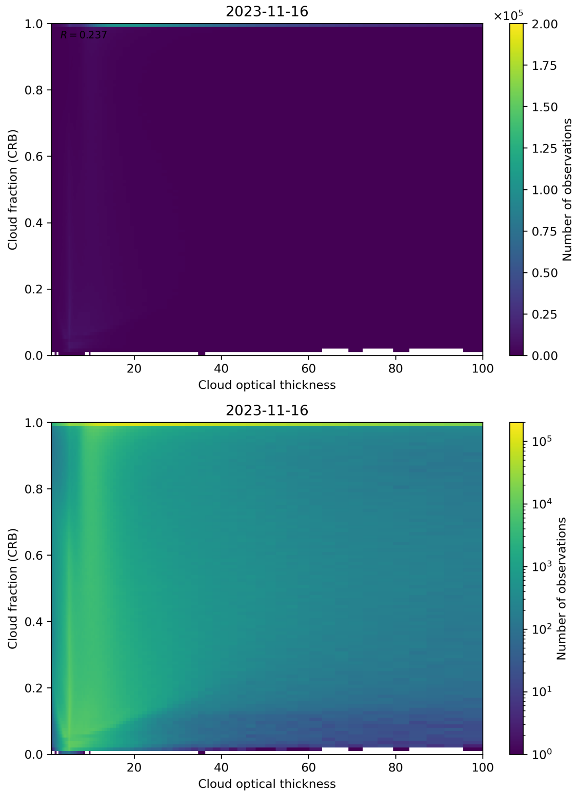
Figure 84: Scatter density plot of “Cloud optical thickness” against “Cloud fraction (CRB)” for 2023-11-15 to 2023-11-17.
