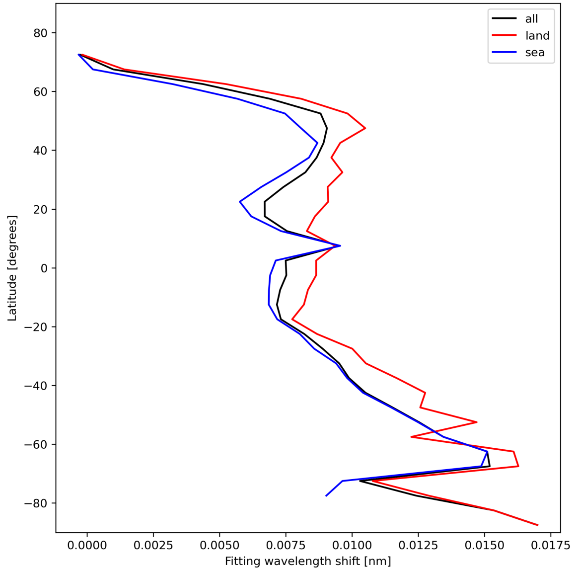
Figure 33: Zonal average of “Fitting wavelength shift” for 2023-11-15 to 2023-11-17.
