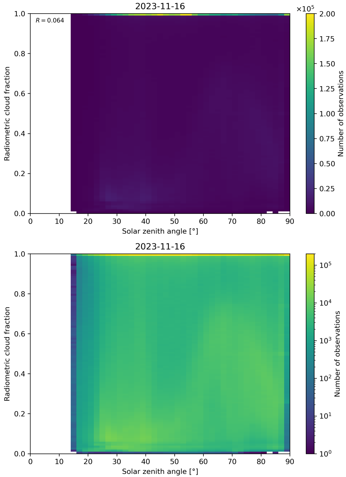
Figure 99: Scatter density plot of “Solar zenith angle” against “Radiometric cloud fraction” for 2023-11-15 to 2023-11-17.
