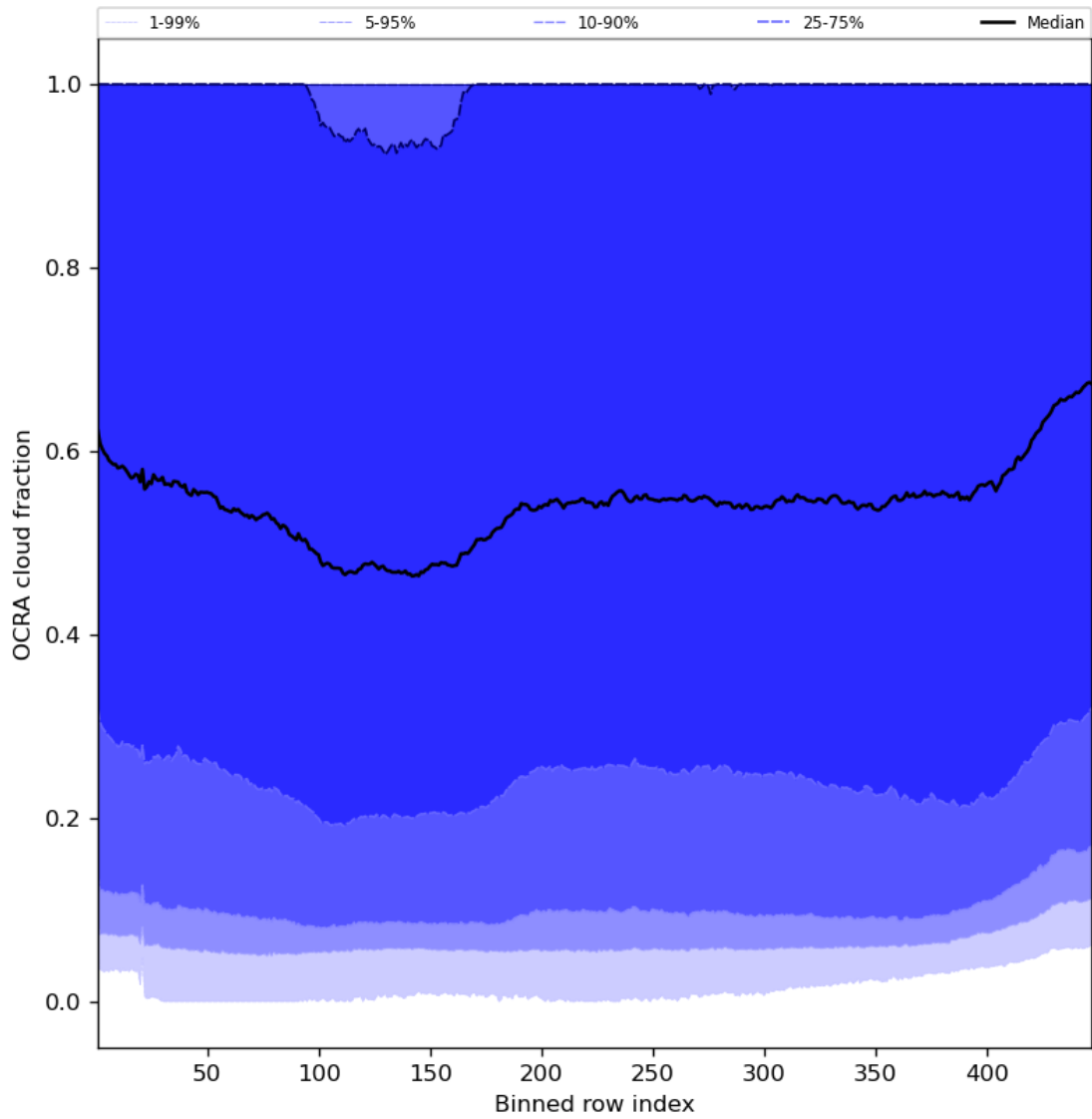
Figure 66: Along track statistics of “OCRA cloud fraction” for 2023-11-15 to 2023-11-17
