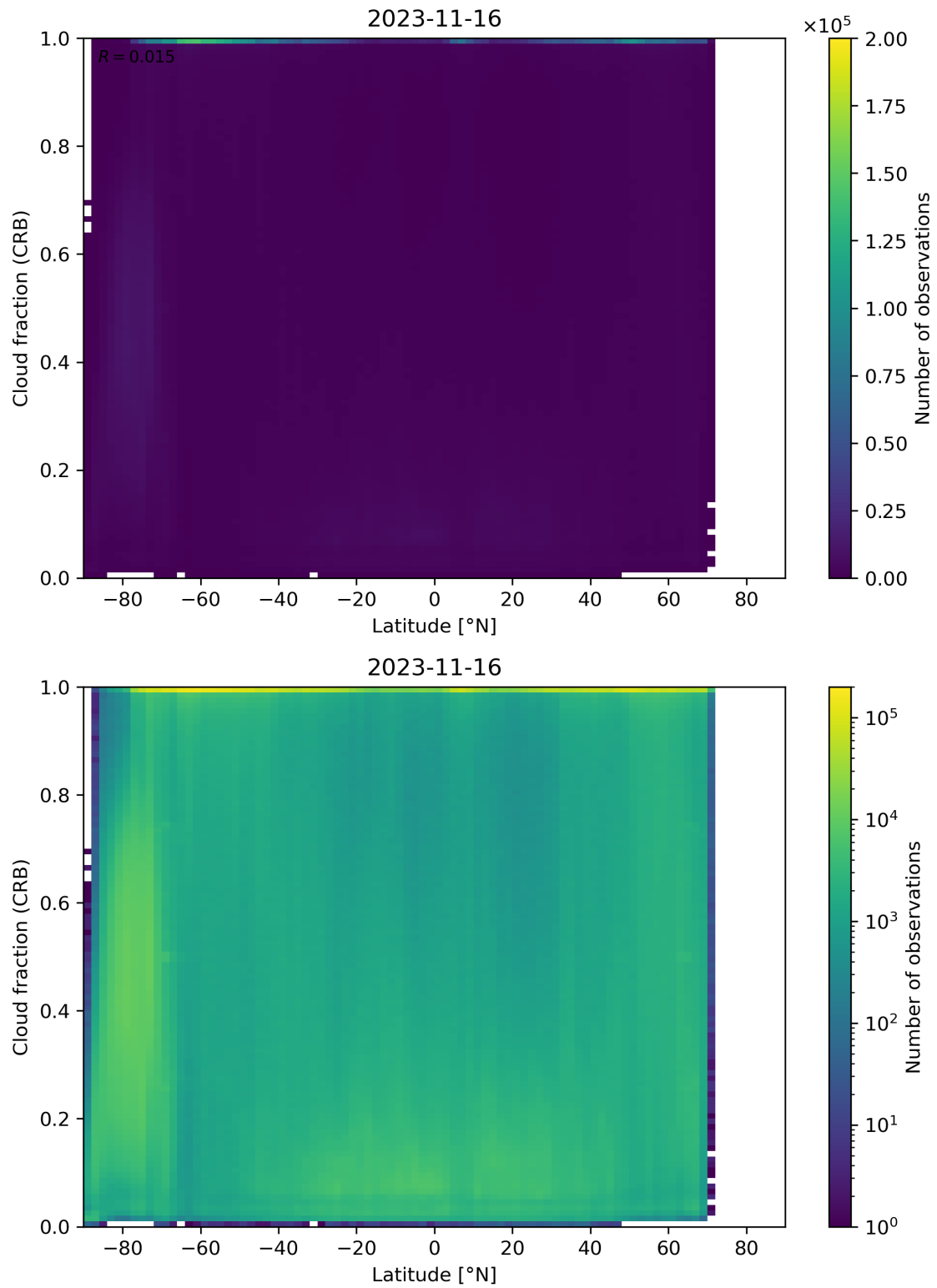
Figure 94: Scatter density plot of “Latitude” against “Cloud fraction (CRB)” for 2023-11-15 to 2023-11-17.
