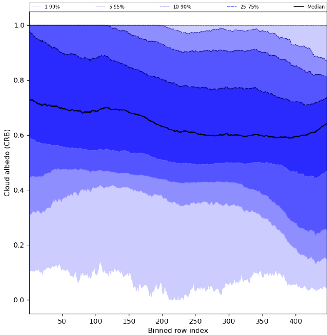
Figure 60: Along track statistics of “Cloud albedo (CRB)” for 2023-11-15 to 2023-11-17
