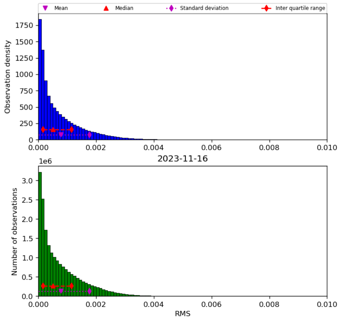
Figure 47: Histogram of “RMS” for 2023-11-15 to 2023-11-17
