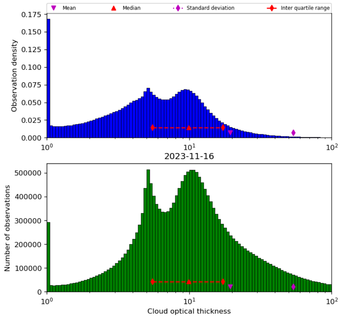
Figure 41: Histogram of “Cloud optical thickness” for 2023-11-15 to 2023-11-17
