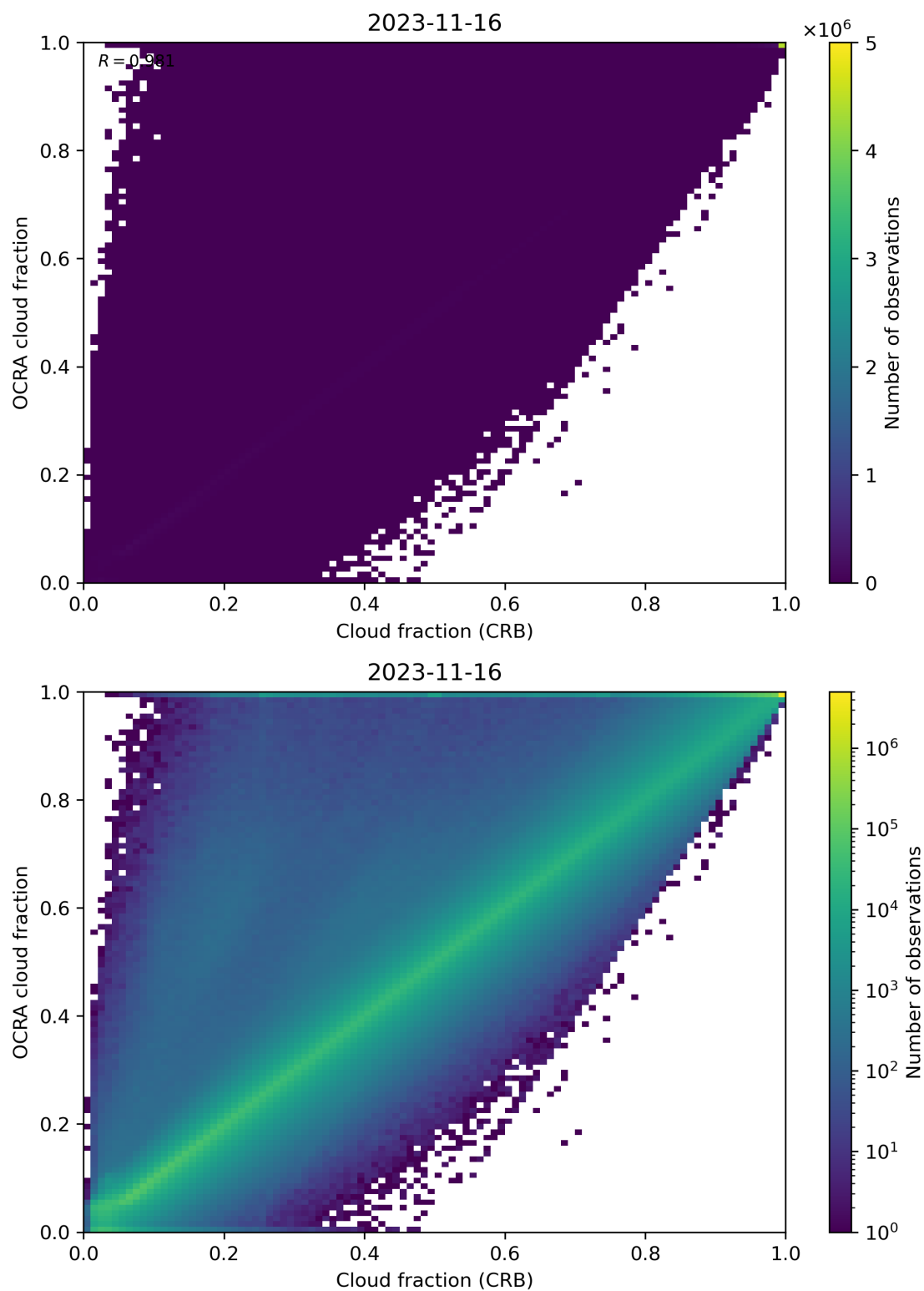
Figure 78: Scatter density plot of “Cloud fraction (CRB)” against “OCRA cloud fraction” for 2023-11-15 to 2023-11-17.
