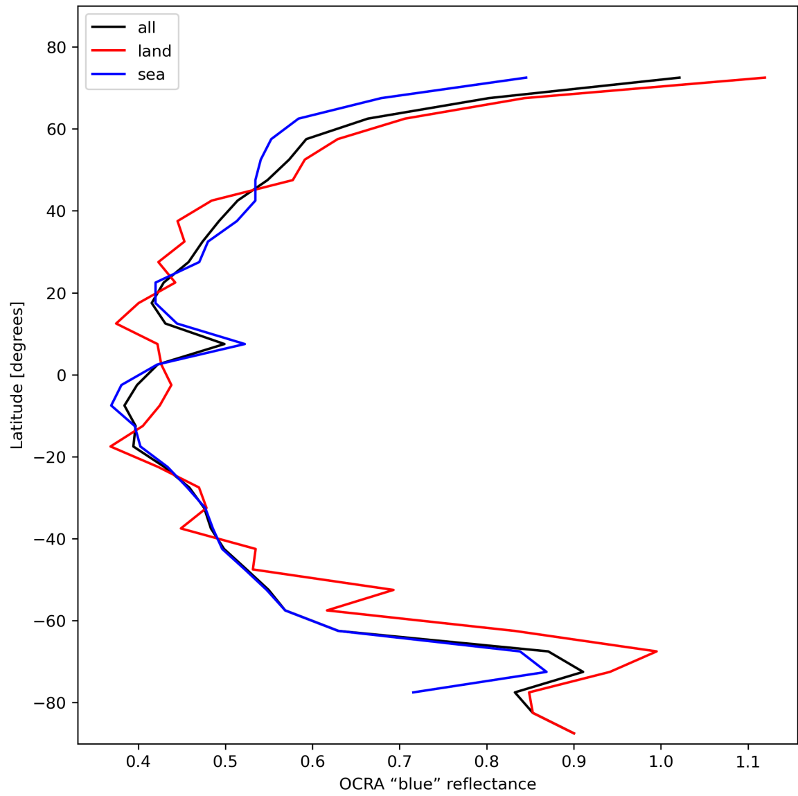
Figure 35: Zonal average of “OCRA “blue” reflectance” for 2023-11-15 to 2023-11-17.
