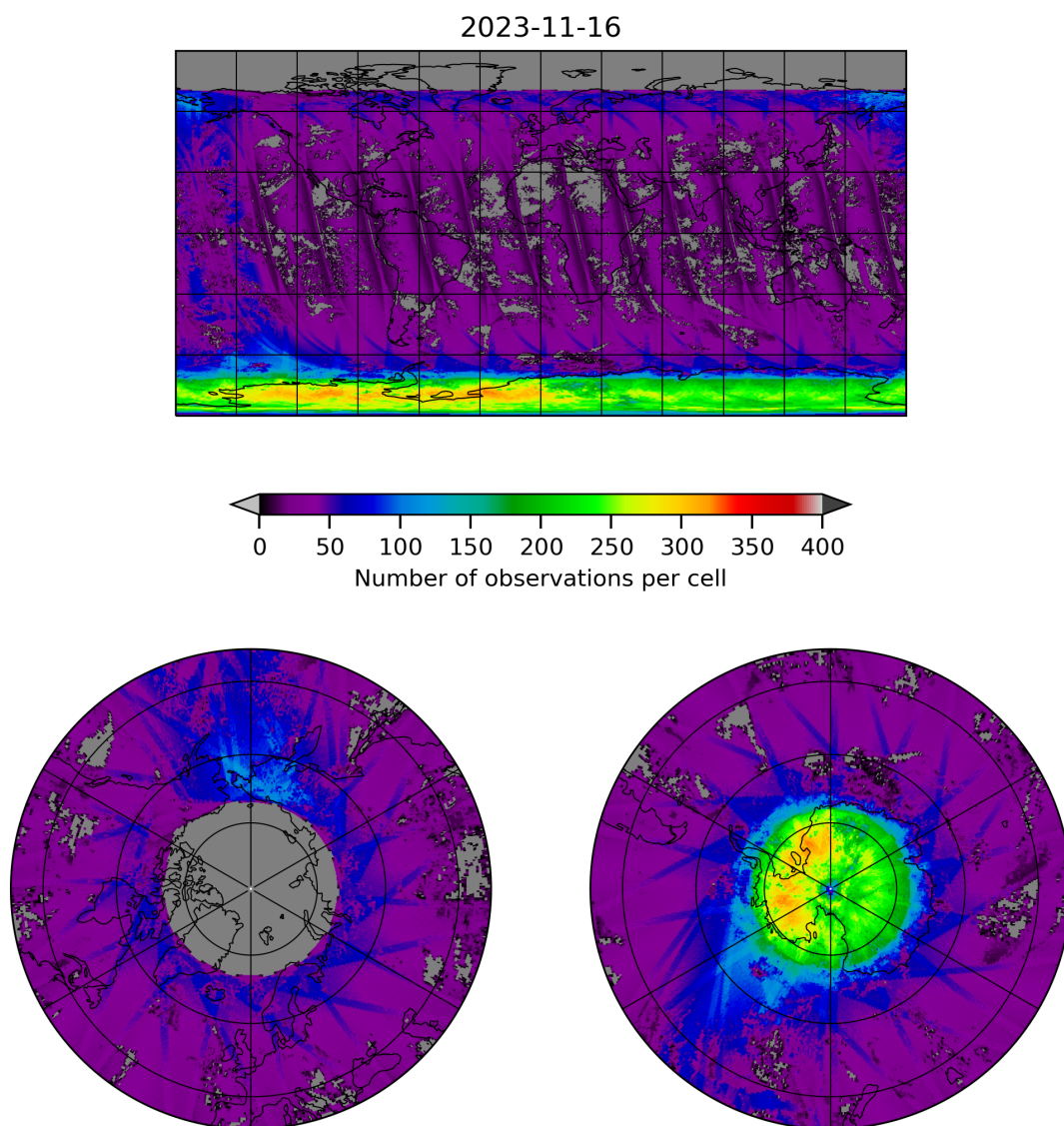
Figure 21: Map of the number of observations for 2023-11-15 to 2023-11-17
