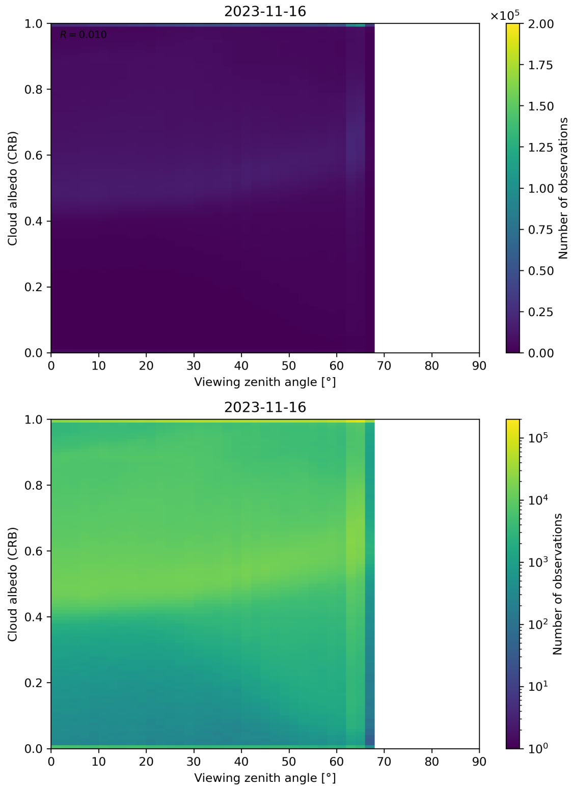
Figure 106: Scatter density plot of “Viewing zenith angle” against “Cloud albedo (CRB)” for 2023-11-15 to 2023-11-17.
