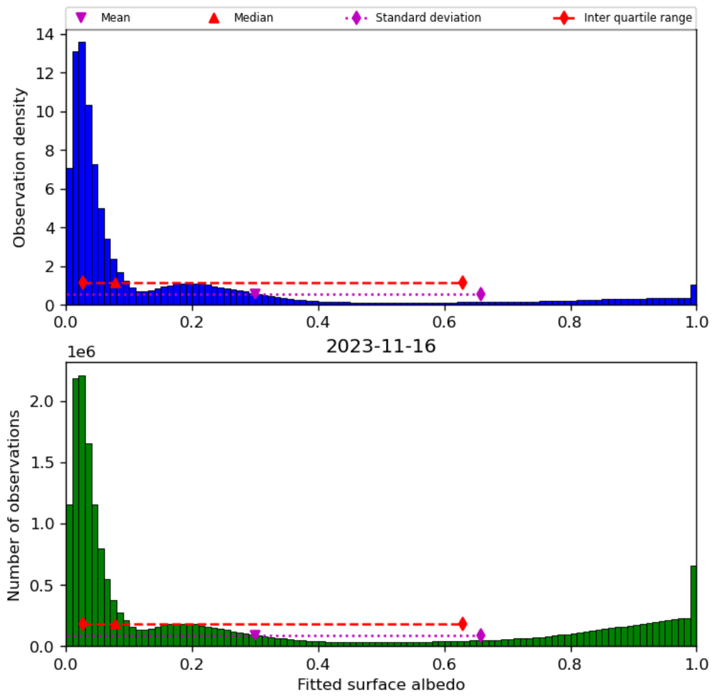
Figure 45: Histogram of “Fitted surface albedo” for 2023-11-15 to 2023-11-17
