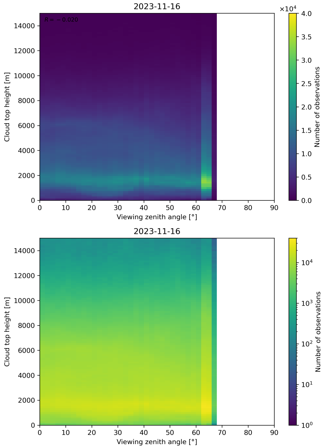
Figure 112: Scatter density plot of “Viewing zenith angle” against “Cloud top height” for 2023-11-15 to 2023-11-17.
