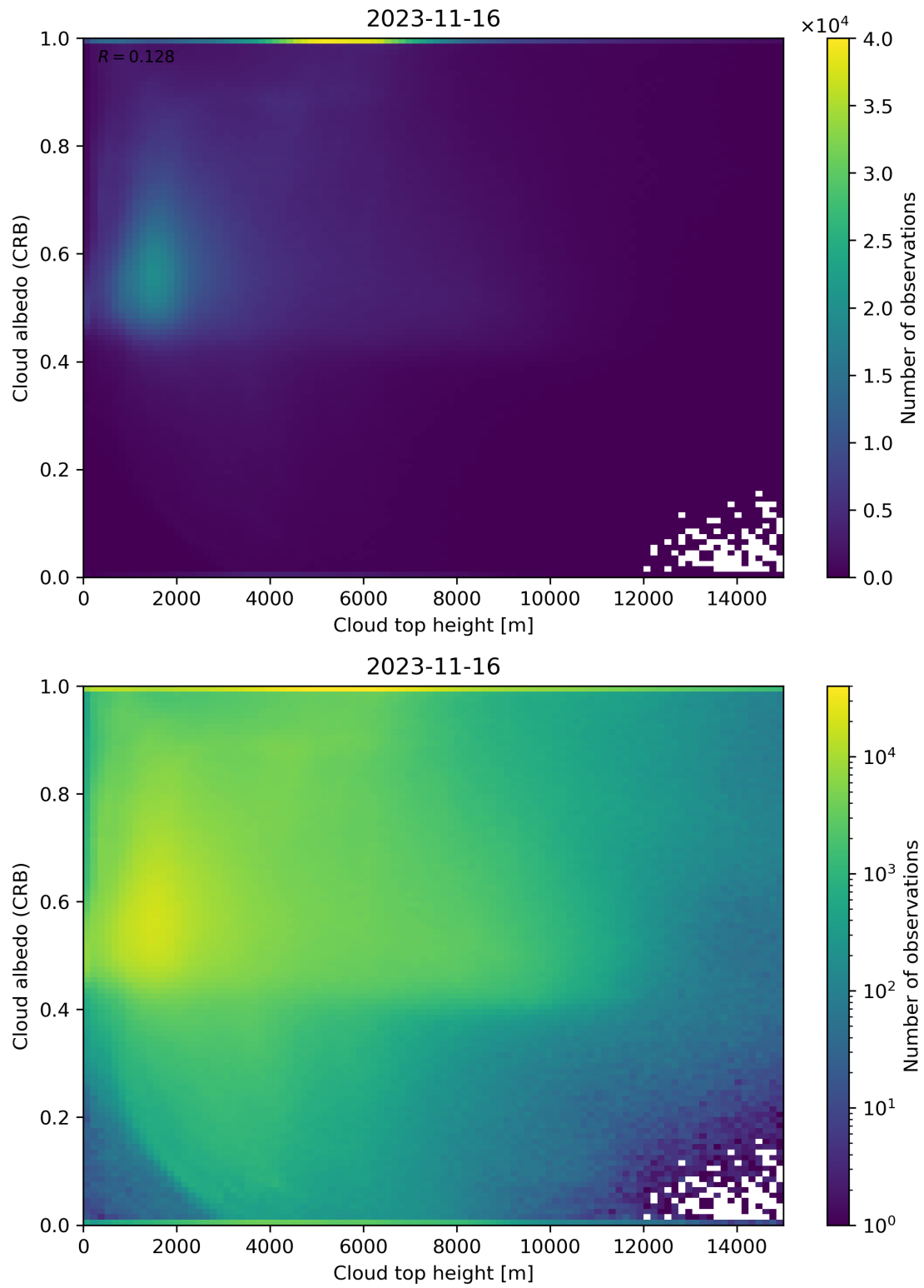
Figure 86: Scatter density plot of “Cloud top height” against “Cloud albedo (CRB)” for 2023-11-15 to 2023-11-17.
