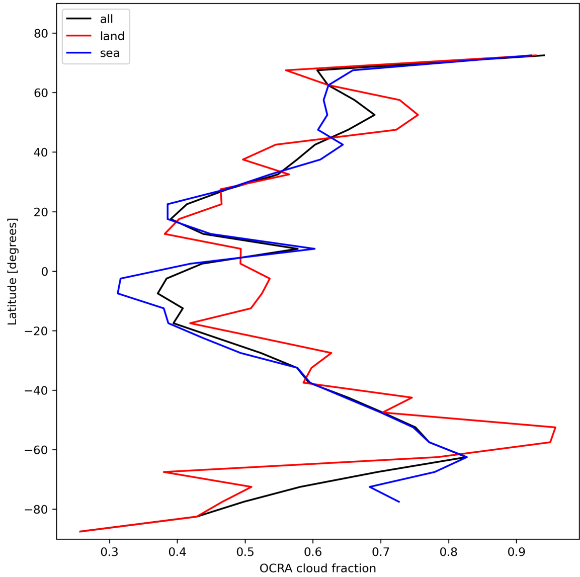
Figure 34: Zonal average of “OCRA cloud fraction” for 2023-11-15 to 2023-11-17.
