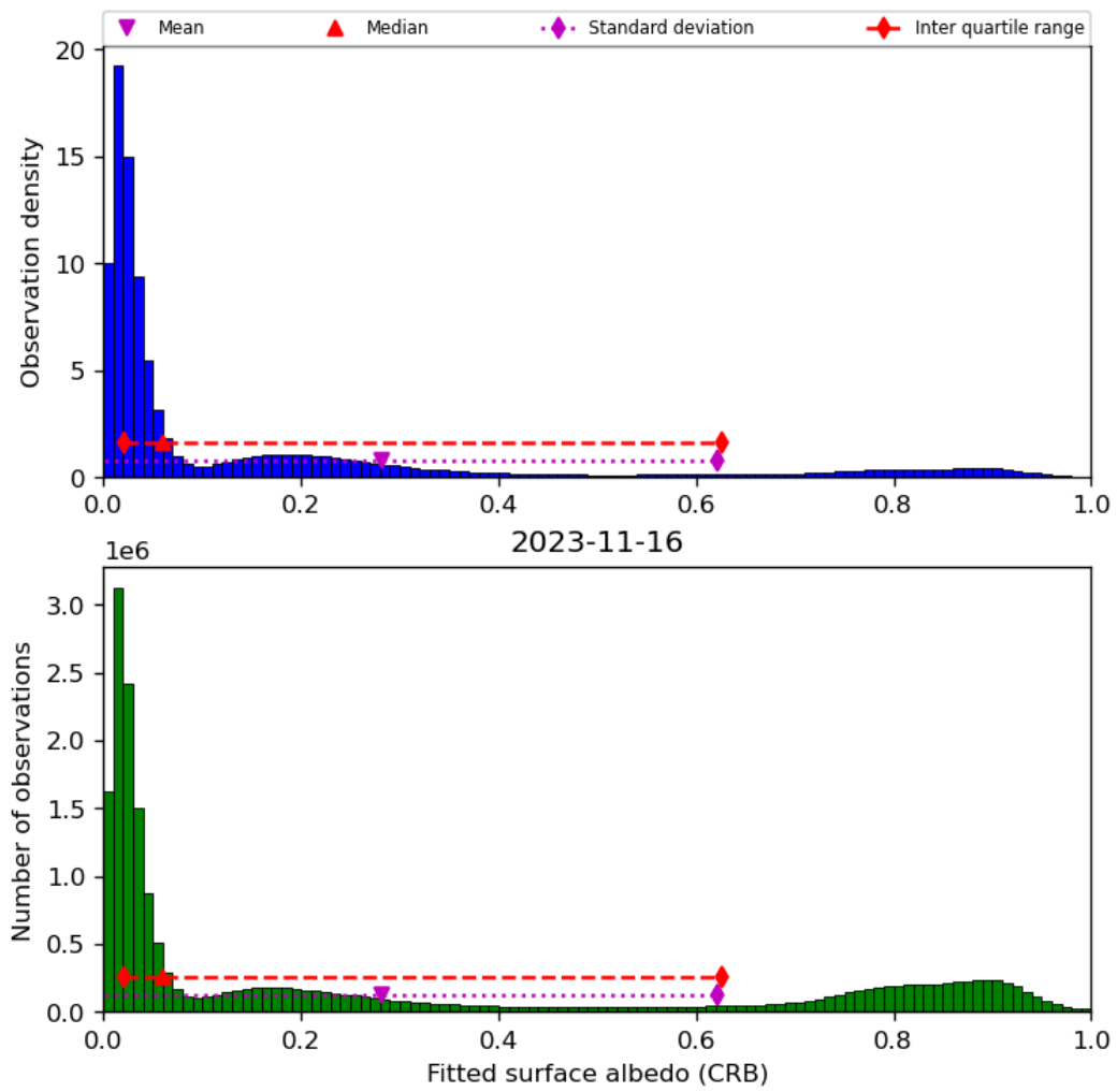
Figure 46: Histogram of “Fitted surface albedo (CRB)” for 2023-11-15 to 2023-11-17
