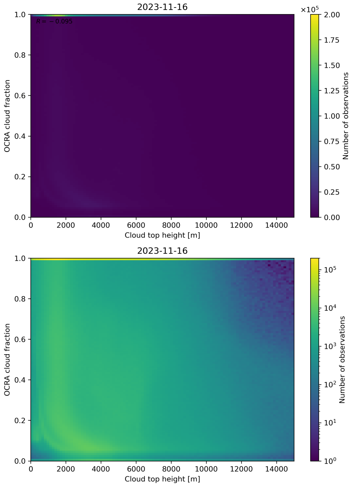
Figure 87: Scatter density plot of “Cloud top height” against “OCRA cloud fraction” for 2023-11-15 to 2023-11-17.
