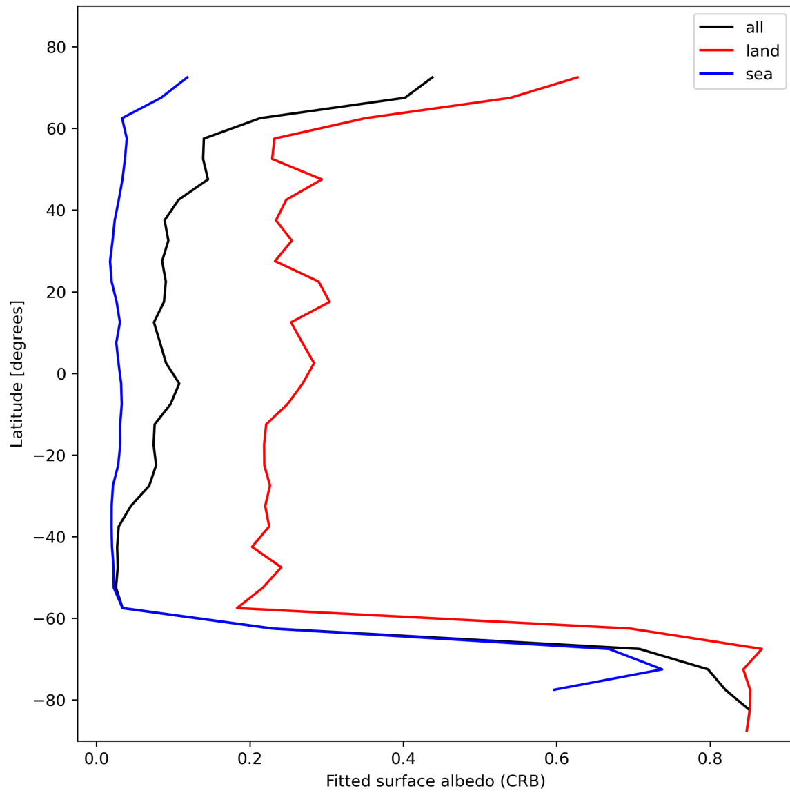
Figure 30: Zonal average of “Fitted surface albedo (CRB)” for 2023-11-15 to 2023-11-17.
