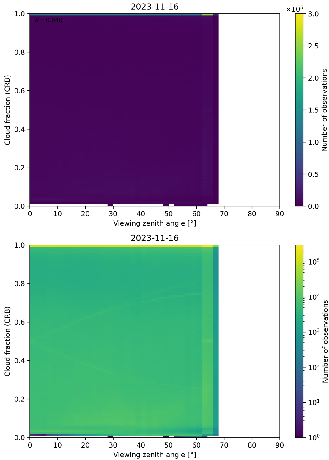
Figure 109: Scatter density plot of “Viewing zenith angle” against “Cloud fraction (CRB)” for 2023-11-15 to 2023-11-17.
