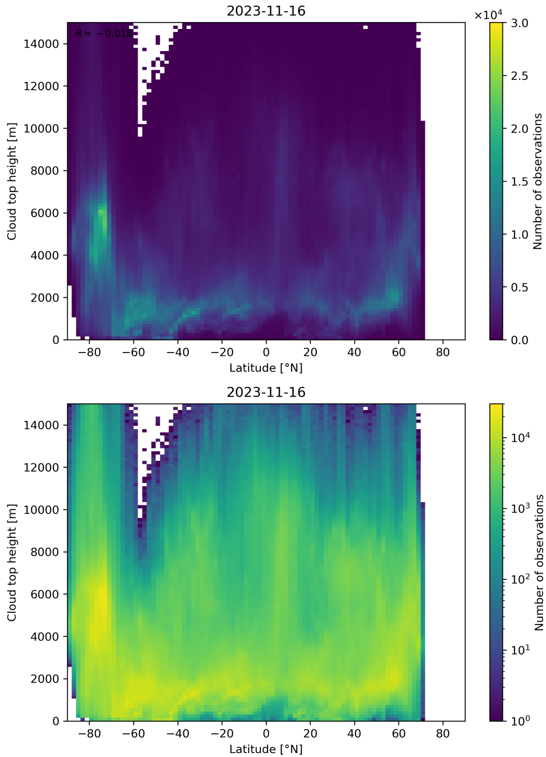
Figure 97: Scatter density plot of “Latitude” against “Cloud top height” for 2023-11-15 to 2023-11-17.
