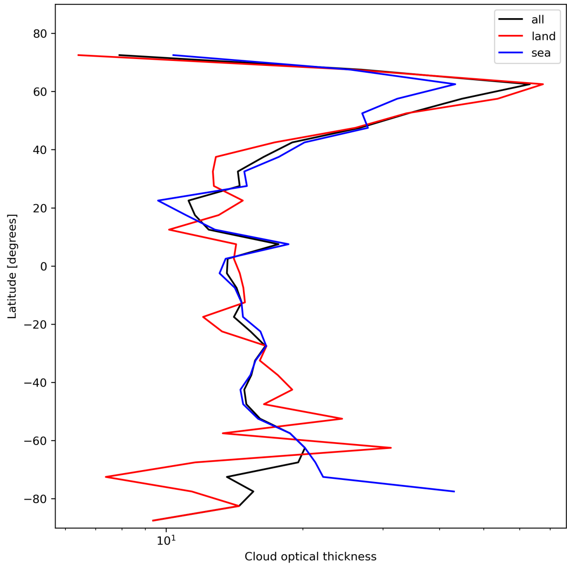
Figure 25: Zonal average of “Cloud optical thickness” for 2023-11-15 to 2023-11-17.
