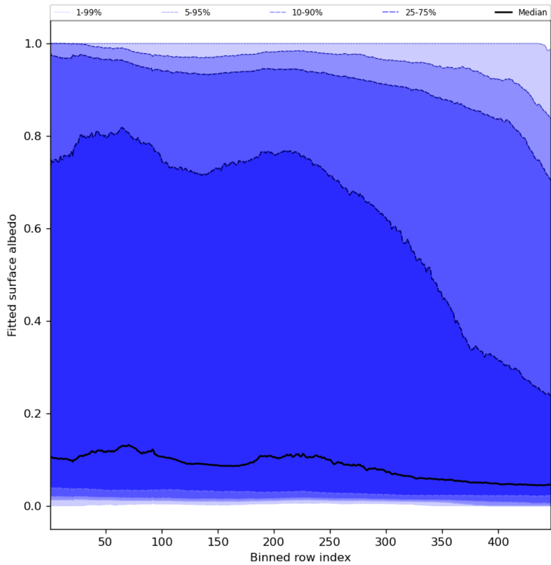
Figure 61: Along track statistics of “Fitted surface albedo” for 2023-11-15 to 2023-11-17
