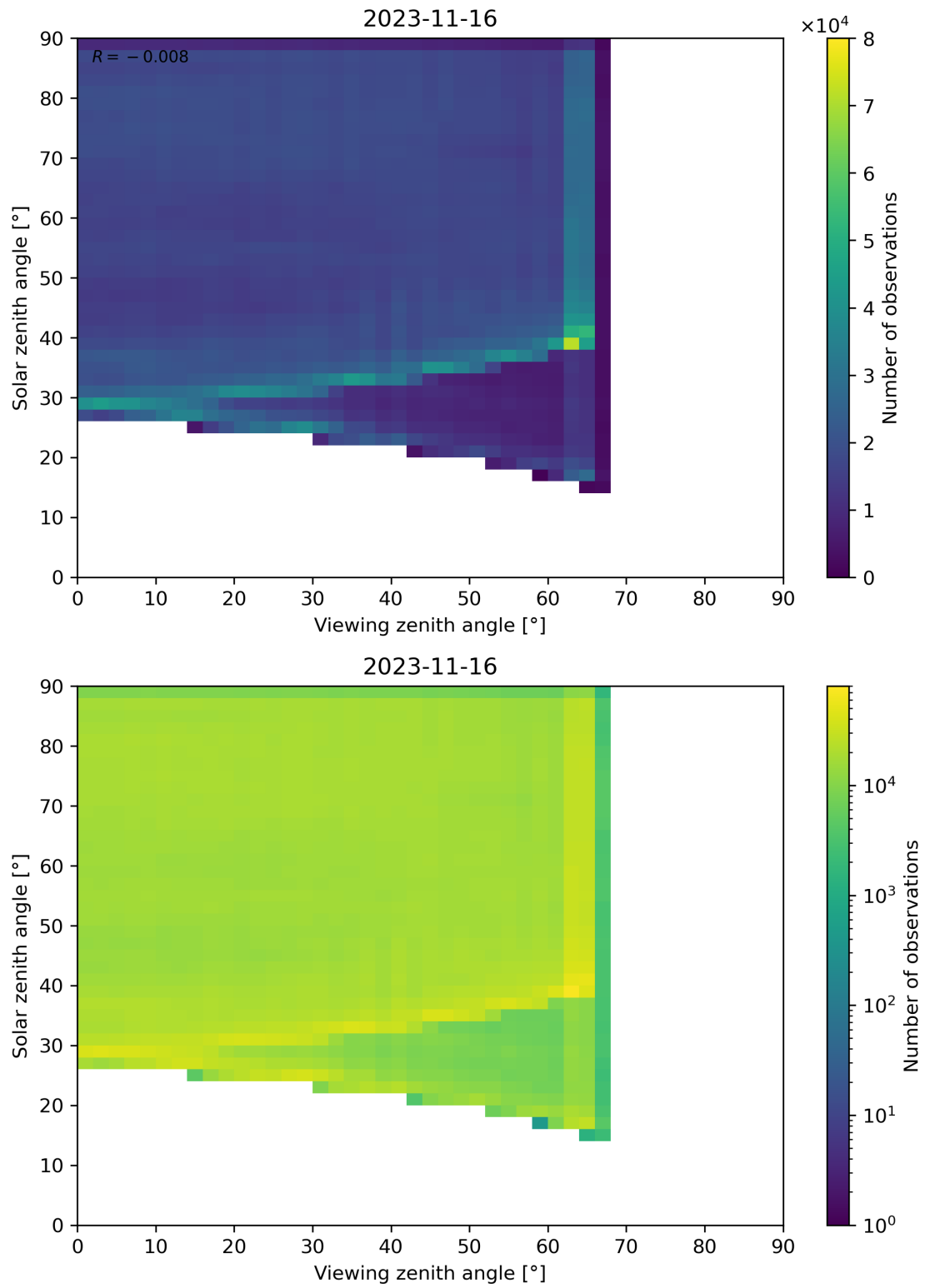
Figure 114: Scatter density plot of “Viewing zenith angle” against “Solar zenith angle” for 2023-11-15 to 2023-11-17.
