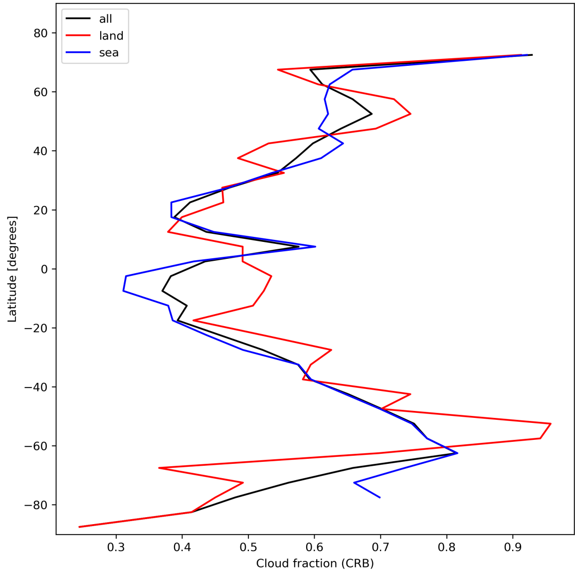
Figure 26: Zonal average of “Cloud fraction (CRB)” for 2023-11-15 to 2023-11-17.
