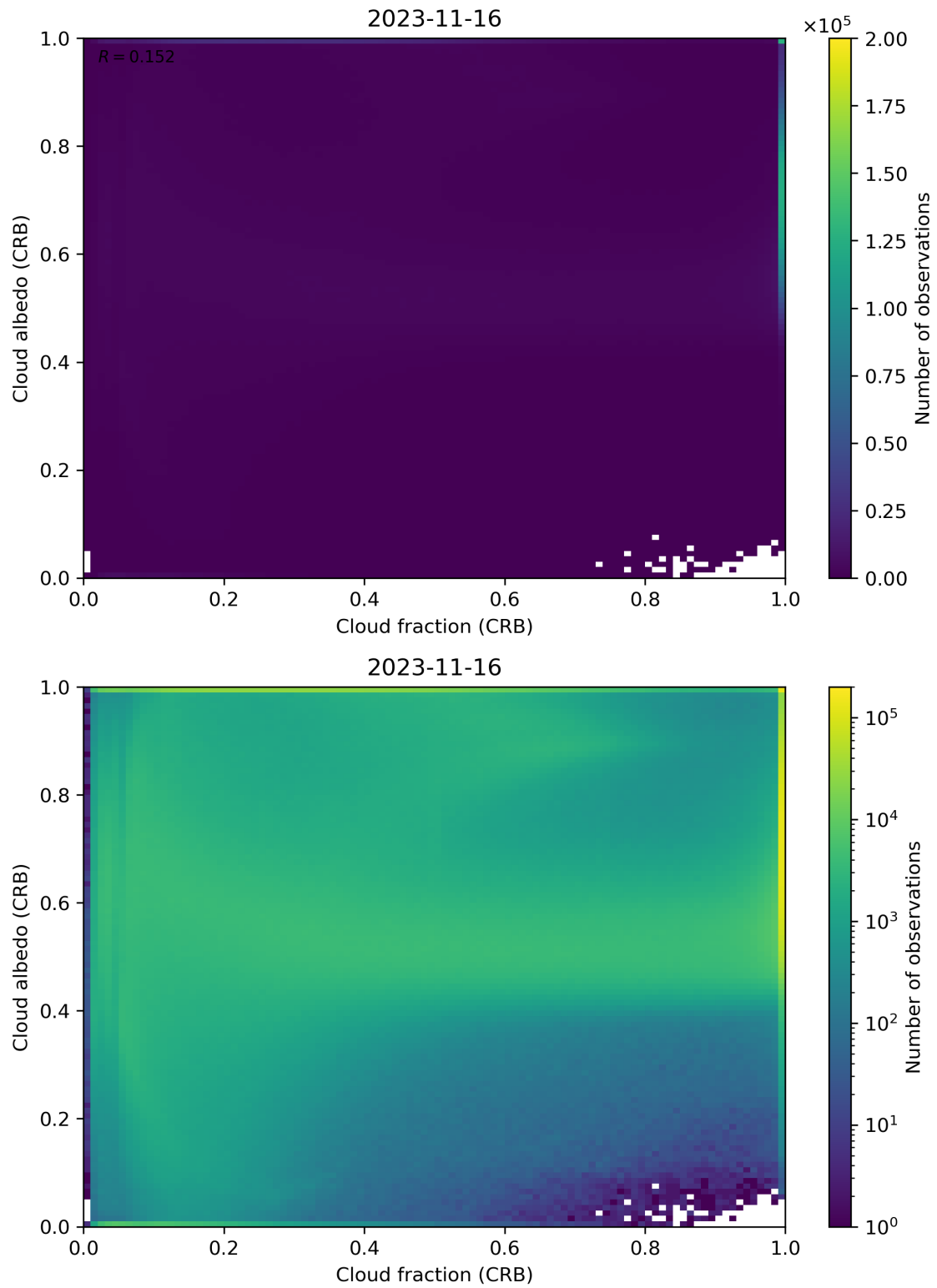
Figure 77: Scatter density plot of “Cloud fraction (CRB)” against “Cloud albedo (CRB)” for 2023-11-15 to 2023-11-17.
