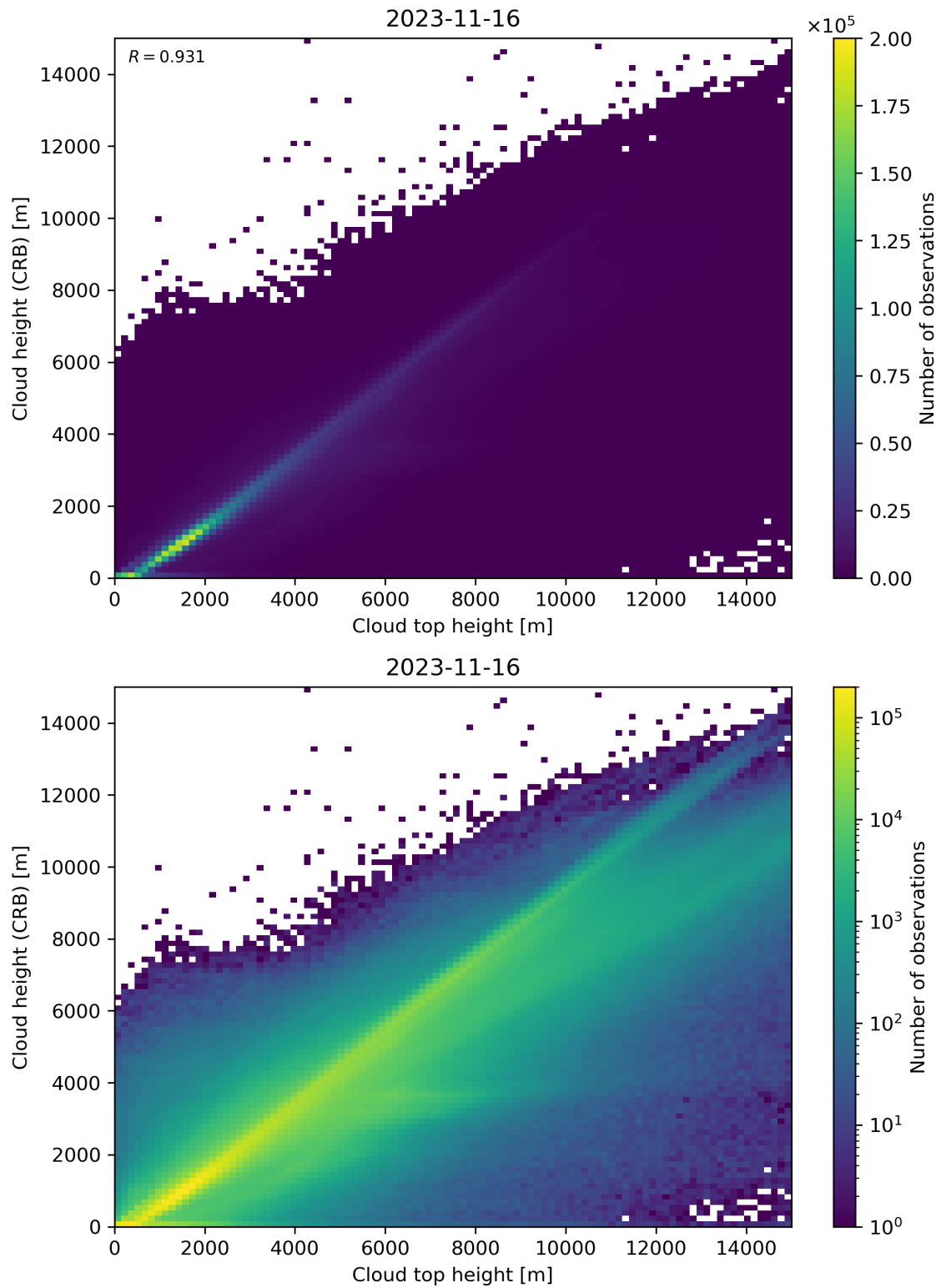
Figure 89: Scatter density plot of “Cloud top height” against “Cloud height (CRB)” for 2023-11-15 to 2023-11-17.
