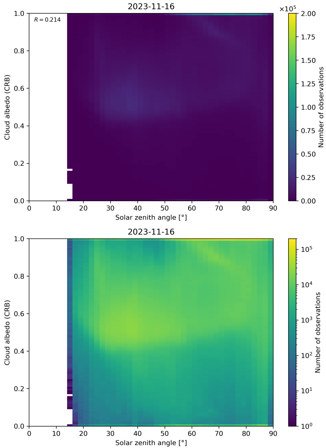
Figure 98: Scatter density plot of “Solar zenith angle” against “Cloud albedo (CRB)” for 2023-11-15 to 2023-11-17.
