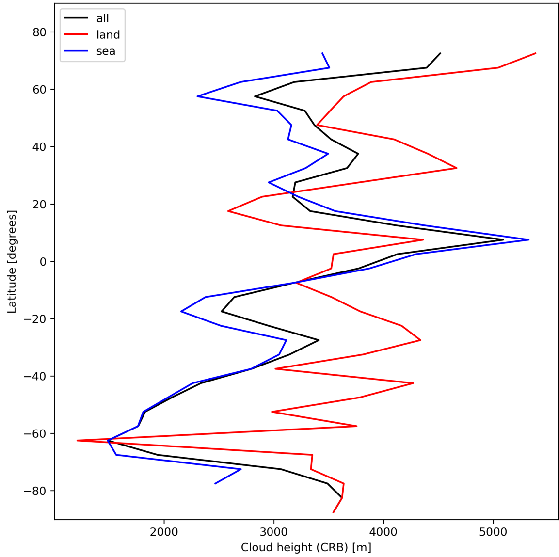
Figure 27: Zonal average of “Cloud height (CRB)” for 2023-11-15 to 2023-11-17.
