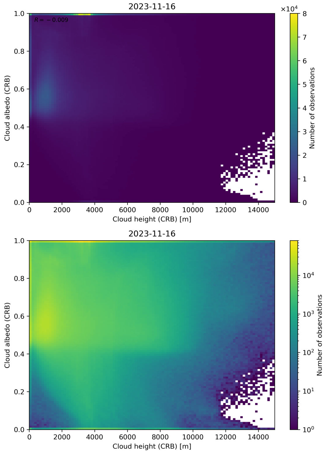
Figure 80: Scatter density plot of “Cloud height (CRB)” against “Cloud albedo (CRB)” for 2023-11-15 to 2023-11-17.
