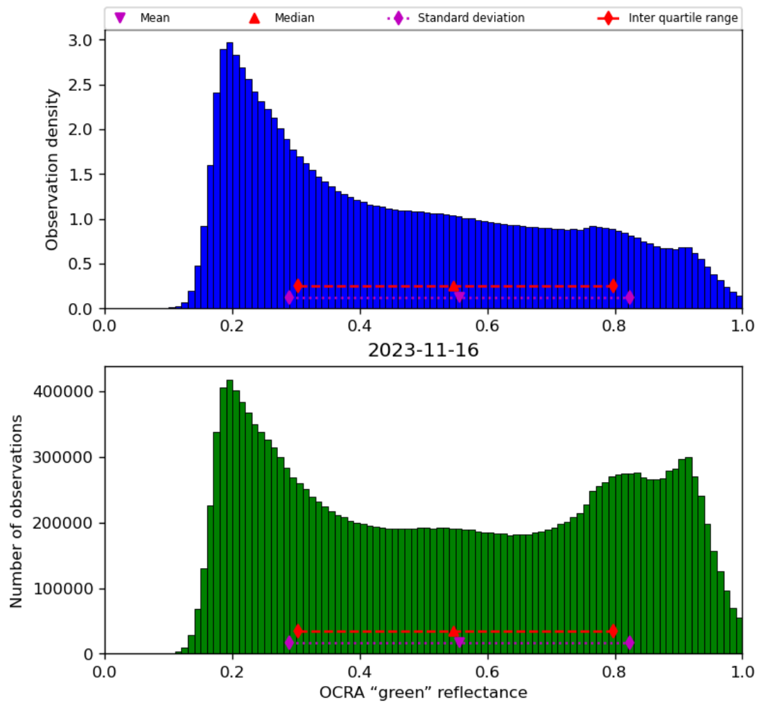
Figure 52: Histogram of “OCRA “green” reflectance” for 2023-11-15 to 2023-11-17
