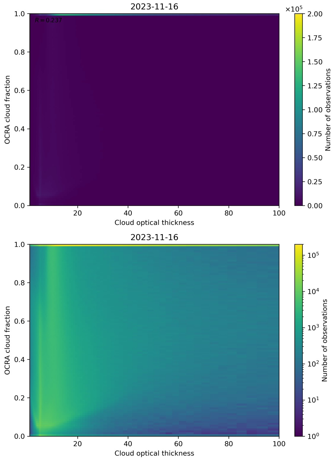
Figure 83: Scatter density plot of “Cloud optical thickness” against “OCRA cloud fraction” for 2023-11-15 to 2023-11-17.
