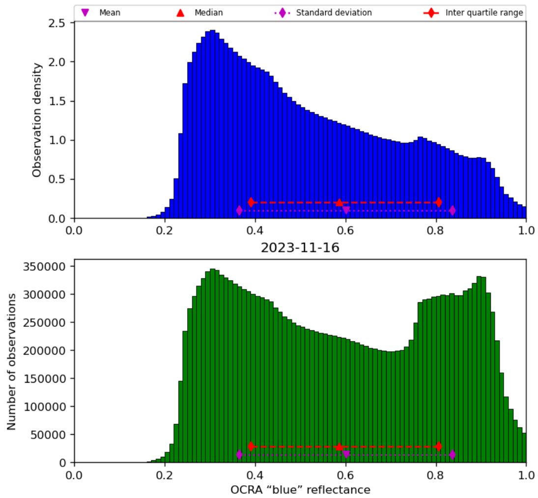
Figure 51: Histogram of “OCRA “blue” reflectance” for 2023-11-15 to 2023-11-17
