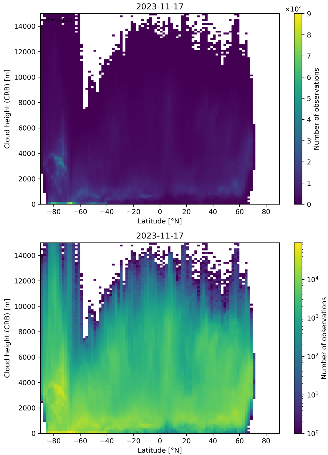
Figure 95: Scatter density plot of “Latitude” against “Cloud height (CRB)” for 2023-11-16 to 2023-11-18.
