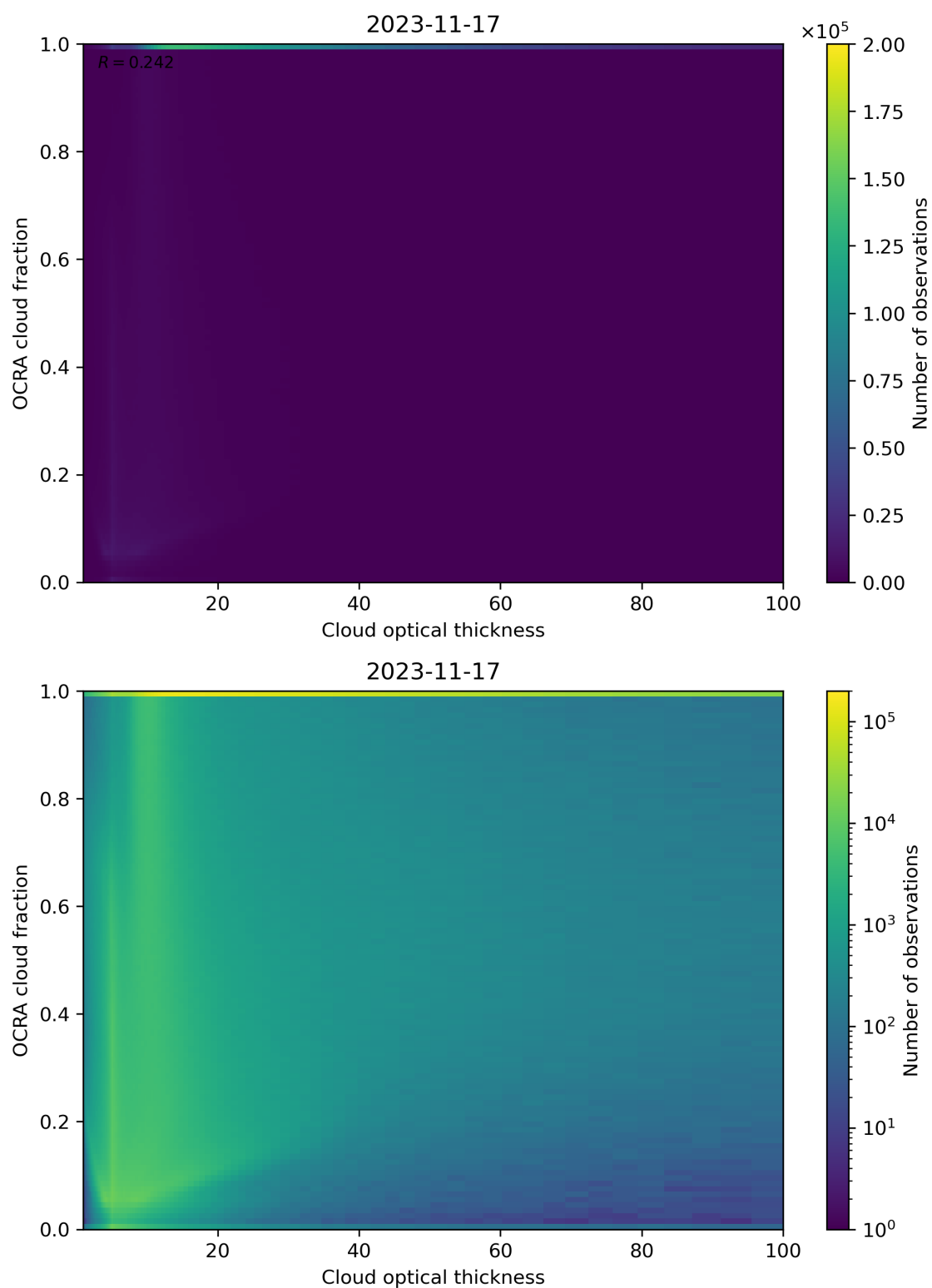
Figure 83: Scatter density plot of “Cloud optical thickness” against “OCRA cloud fraction” for 2023-11-16 to 2023-11-18.
