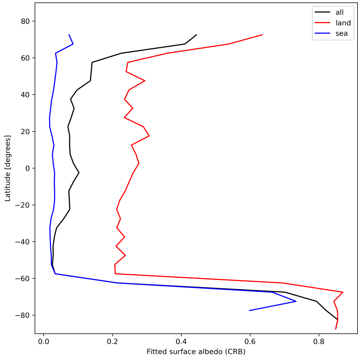
Figure 30: Zonal average of “Fitted surface albedo (CRB)” for 2023-11-16 to 2023-11-18.
