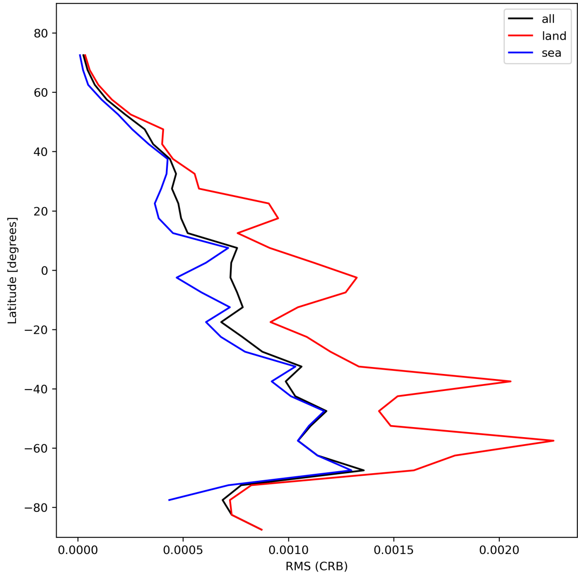
Figure 32: Zonal average of “RMS (CRB)” for 2023-11-16 to 2023-11-18.
