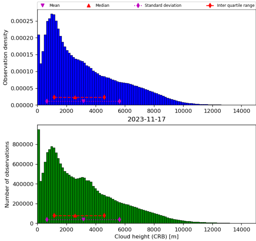
Figure 43: Histogram of “Cloud height (CRB)” for 2023-11-16 to 2023-11-18
