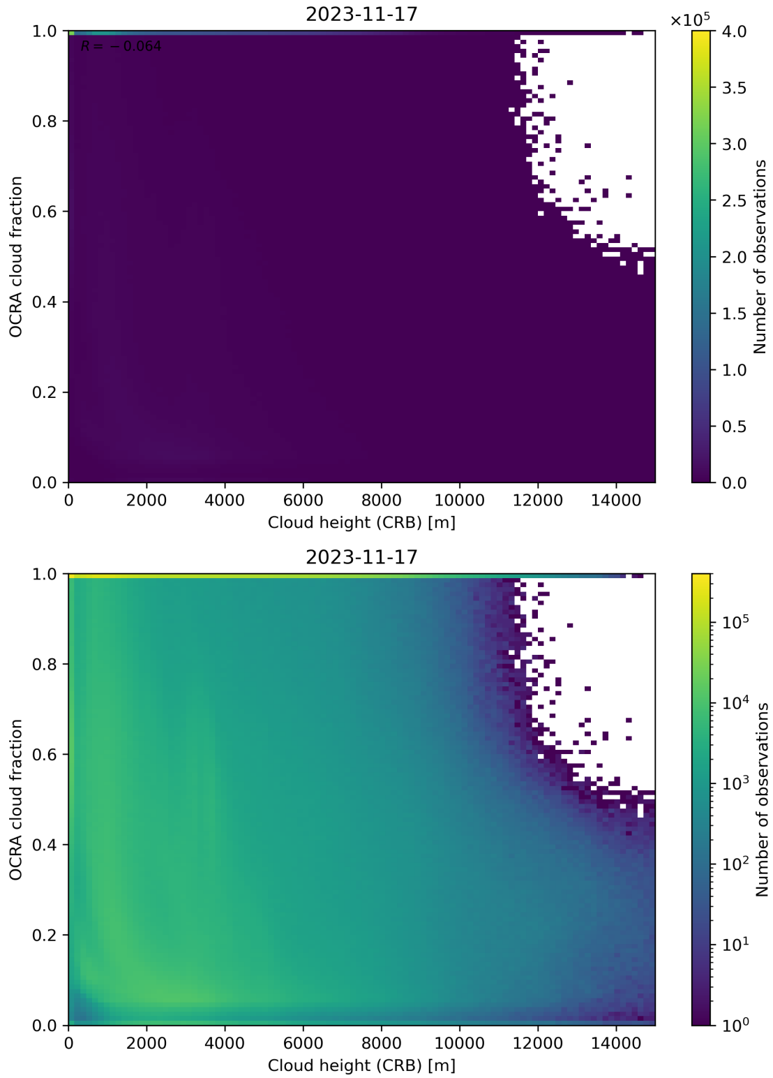
Figure 81: Scatter density plot of “Cloud height (CRB)” against “OCRA cloud fraction” for 2023-11-16 to 2023-11-18.
