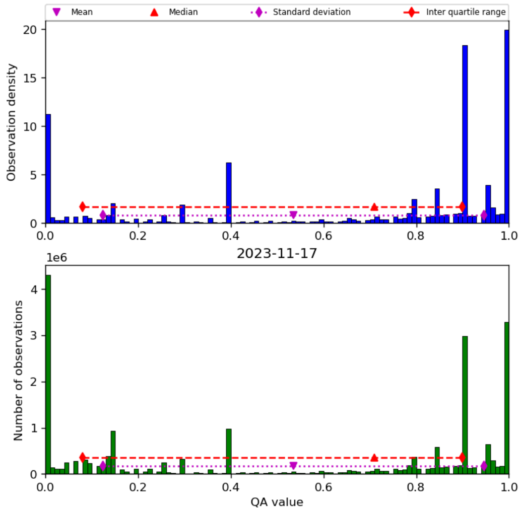
Figure 38: Histogram of “QA value” for 2023-11-16 to 2023-11-18
