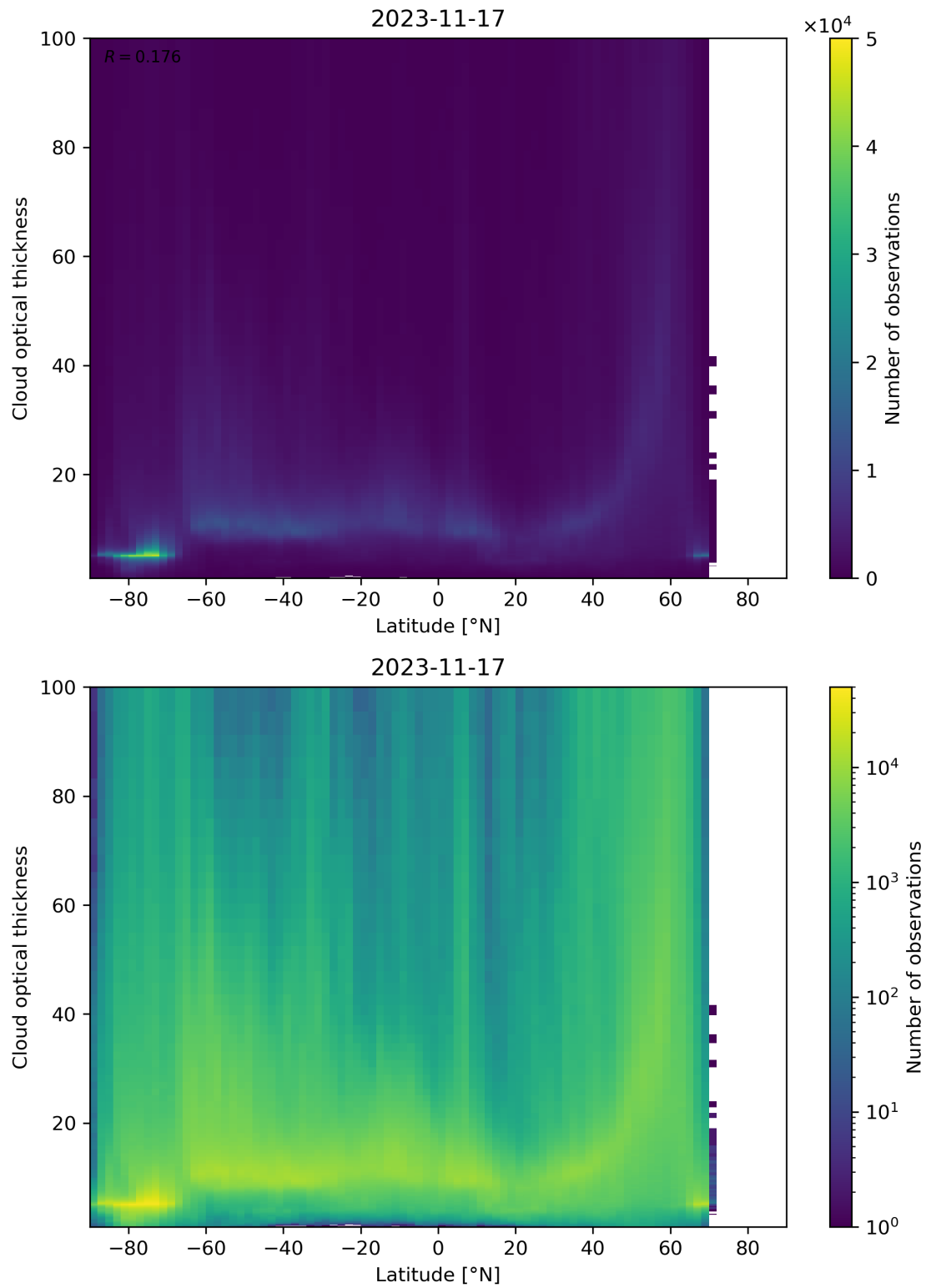
Figure 96: Scatter density plot of “Latitude” against “Cloud optical thickness” for 2023-11-16 to 2023-11-18.
