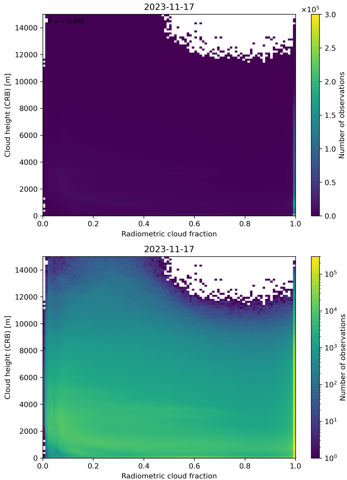
Figure 74: Scatter density plot of “Radiometric cloud fraction” against “Cloud height (CRB)” for 2023-11-16 to 2023-11-18.
