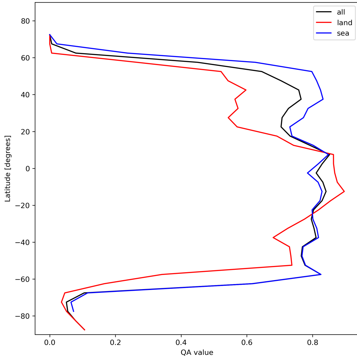
Figure 22: Zonal average of “QA value” for 2023-11-16 to 2023-11-18.
