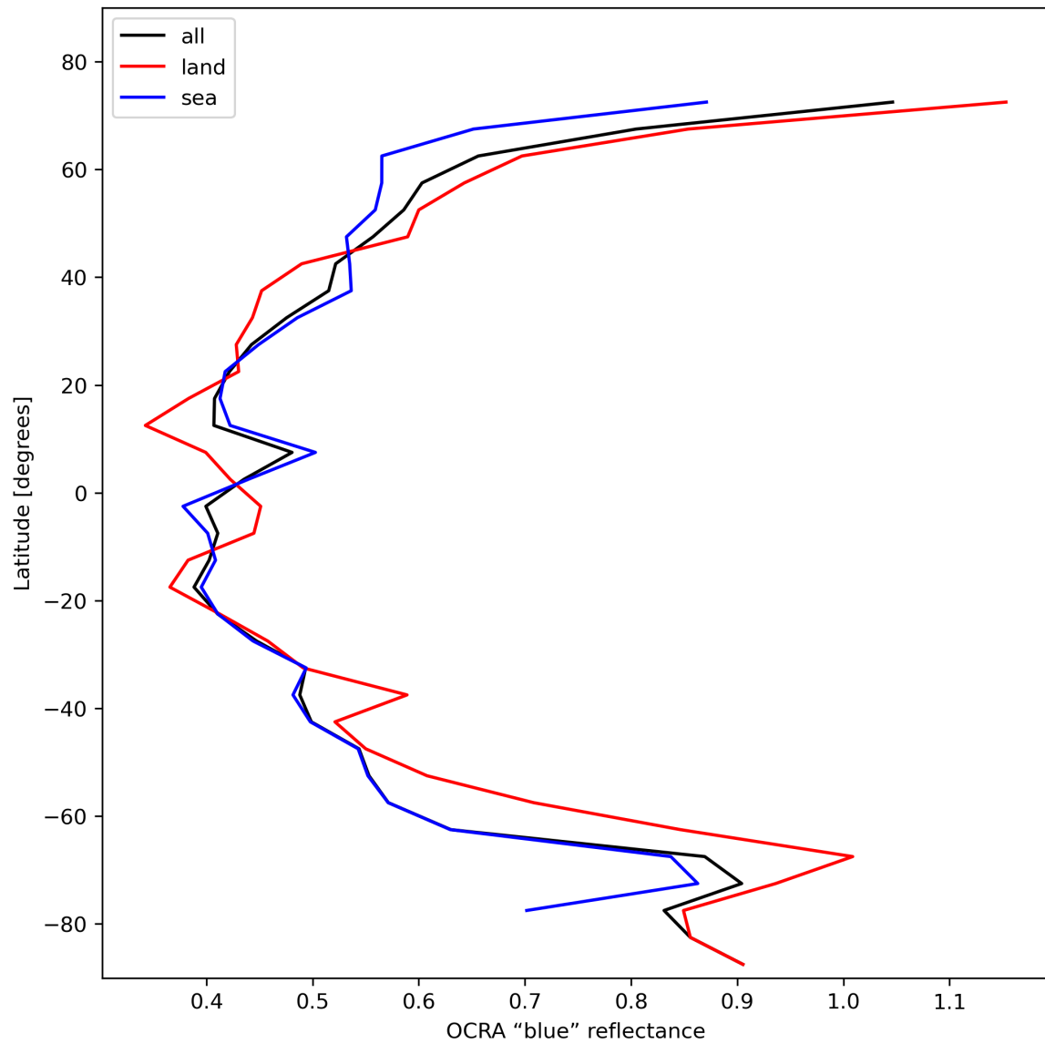
Figure 35: Zonal average of “OCRA “blue” reflectance” for 2023-11-16 to 2023-11-18.
