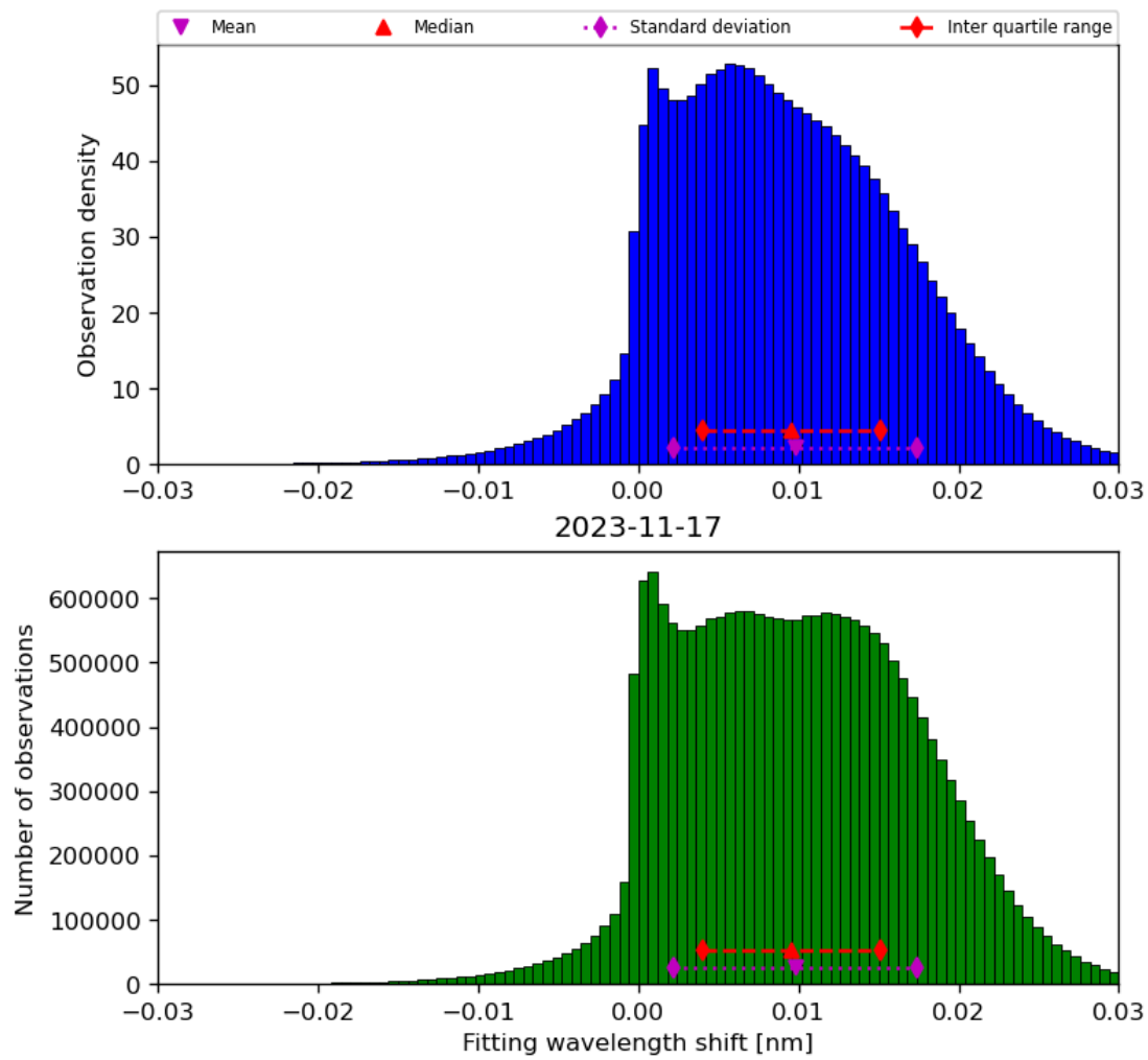
Figure 49: Histogram of “Fitting wavelength shift” for 2023-11-16 to 2023-11-18
