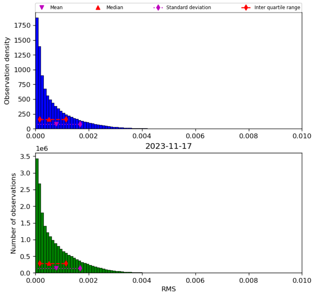
Figure 47: Histogram of “RMS” for 2023-11-16 to 2023-11-18
