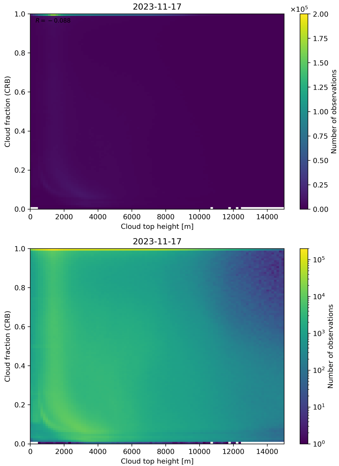
Figure 88: Scatter density plot of “Cloud top height” against “Cloud fraction (CRB)” for 2023-11-16 to 2023-11-18.
