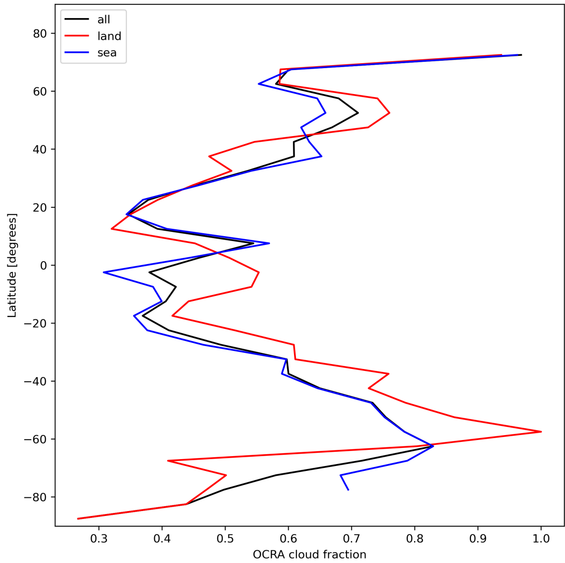
Figure 34: Zonal average of “OCRA cloud fraction” for 2023-11-16 to 2023-11-18.
