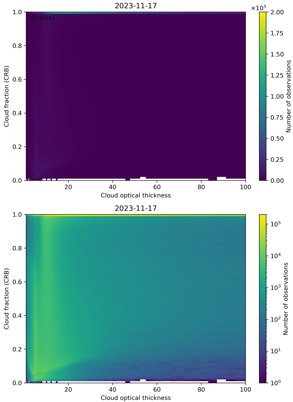
Figure 84: Scatter density plot of “Cloud optical thickness” against “Cloud fraction (CRB)” for 2023-11-16 to 2023-11-18.
