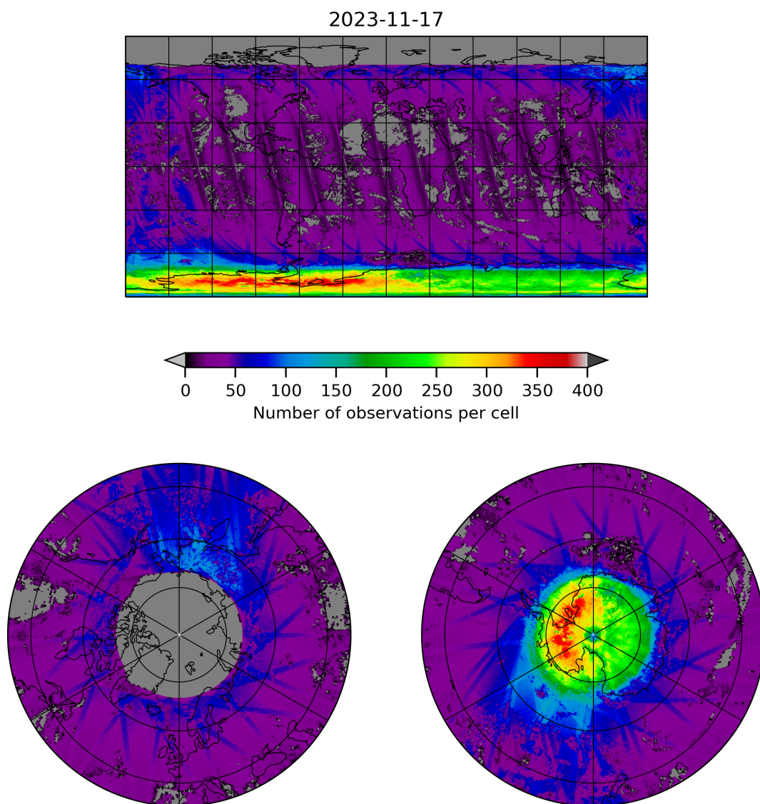
Figure 21: Map of the number of observations for 2023-11-16 to 2023-11-18
