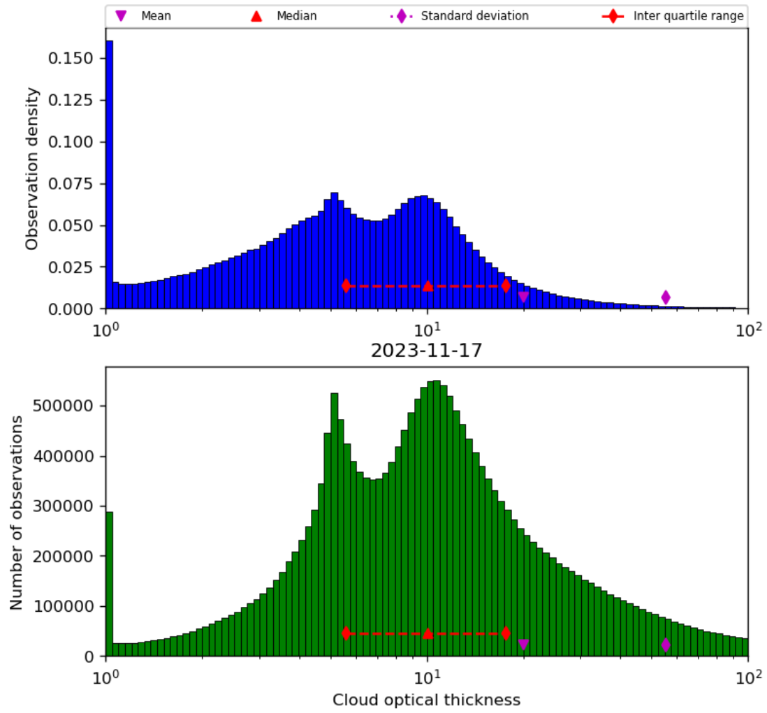
Figure 41: Histogram of “Cloud optical thickness” for 2023-11-16 to 2023-11-18
