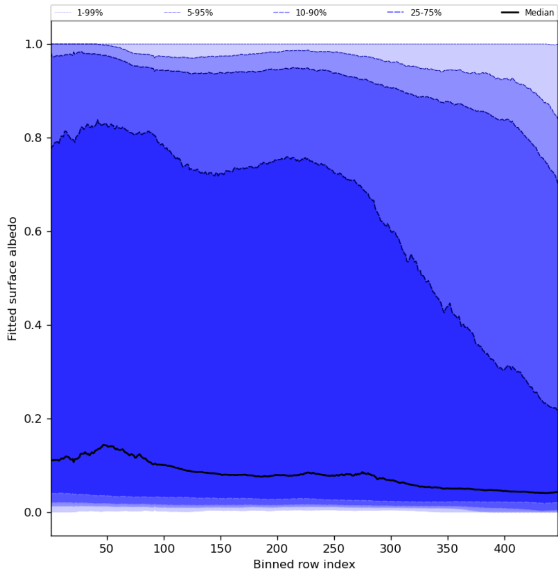
Figure 61: Along track statistics of “Fitted surface albedo” for 2023-11-16 to 2023-11-18
