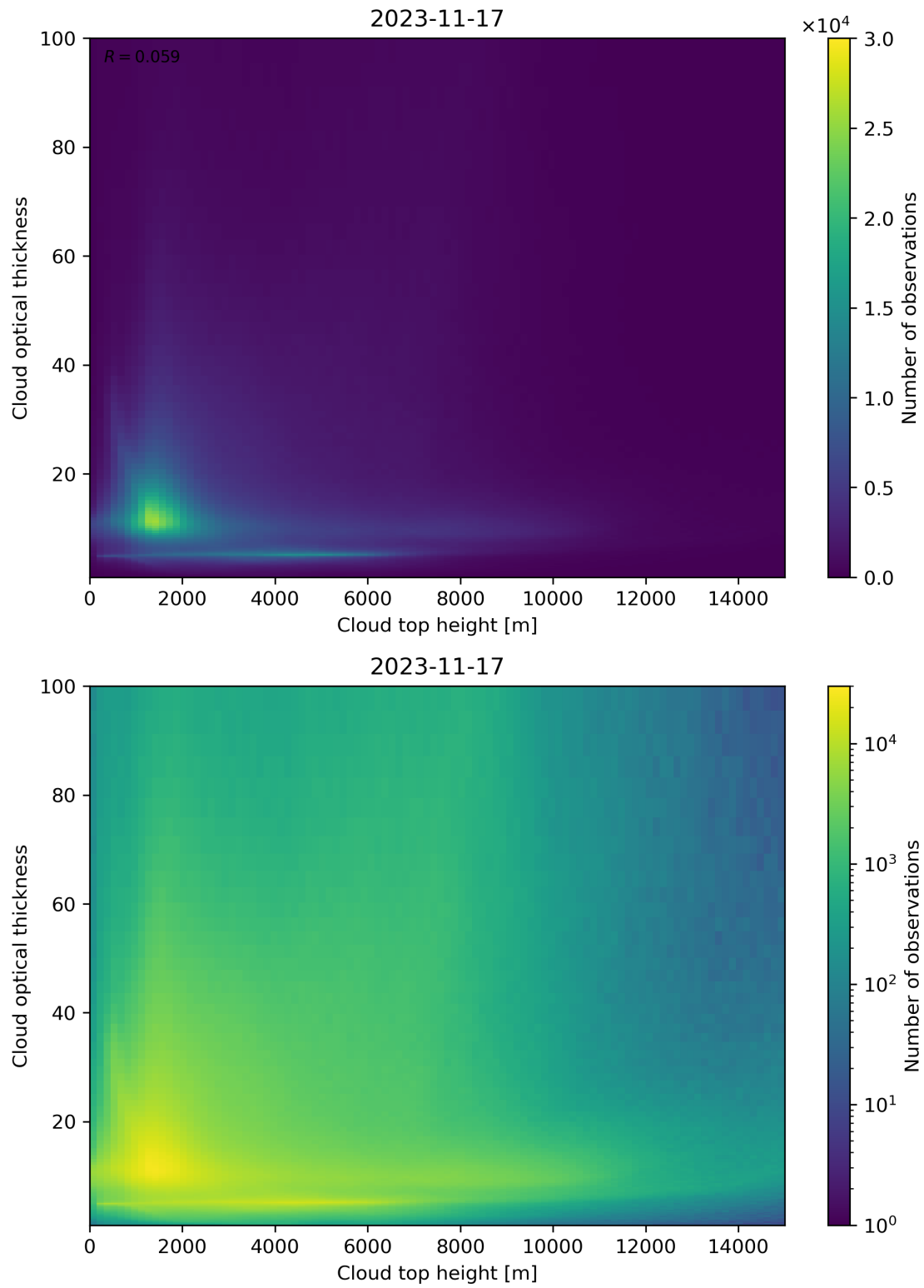
Figure 90: Scatter density plot of “Cloud top height” against “Cloud optical thickness” for 2023-11-16 to 2023-11-18.
