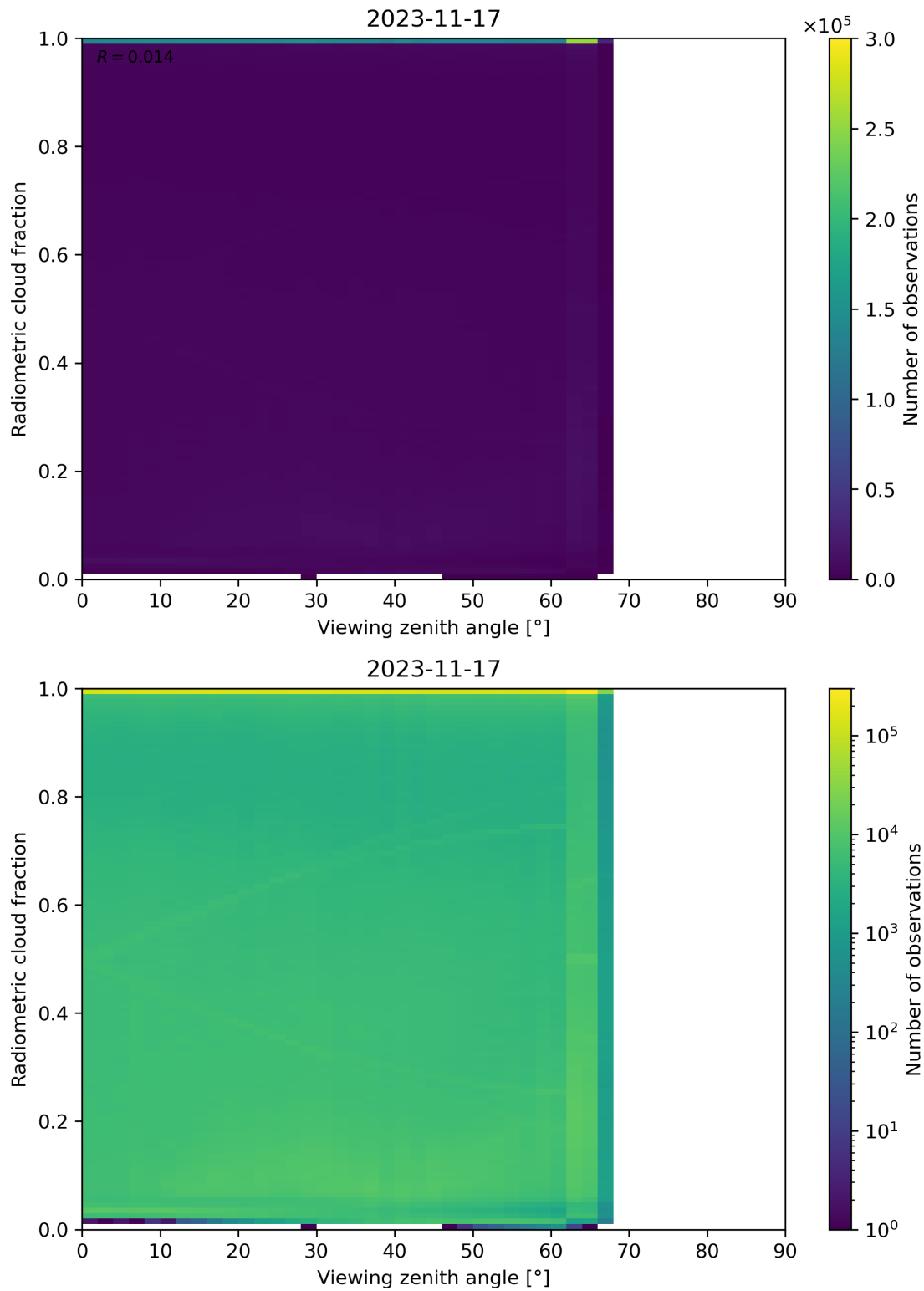
Figure 107: Scatter density plot of “Viewing zenith angle” against “Radiometric cloud fraction” for 2023-11-16 to 2023-11-18.
