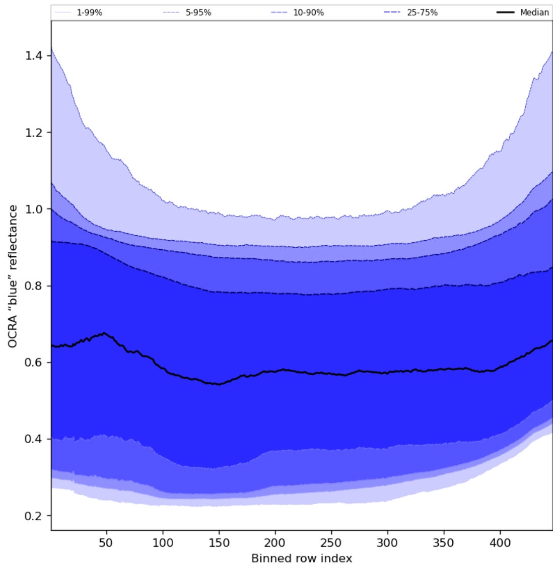
Figure 67: Along track statistics of “OCRA “blue” reflectance” for 2023-11-16 to 2023-11-18
