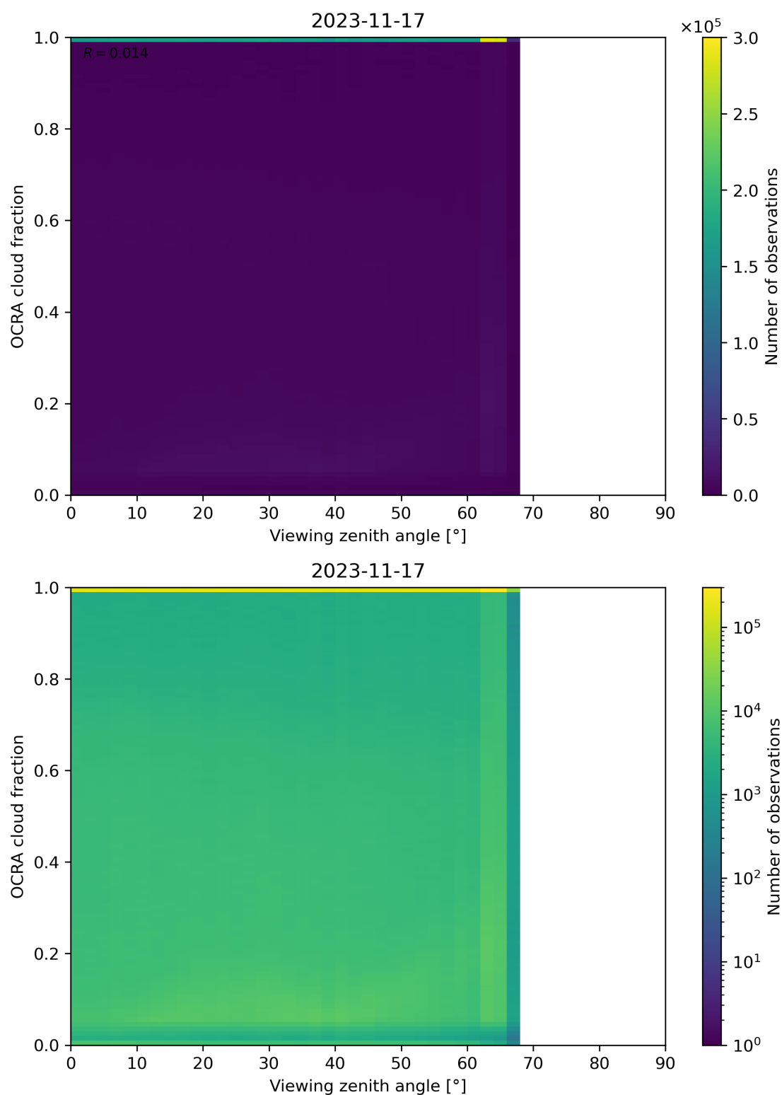
Figure 108: Scatter density plot of “Viewing zenith angle” against “OCRA cloud fraction” for 2023-11-16 to 2023-11-18.
