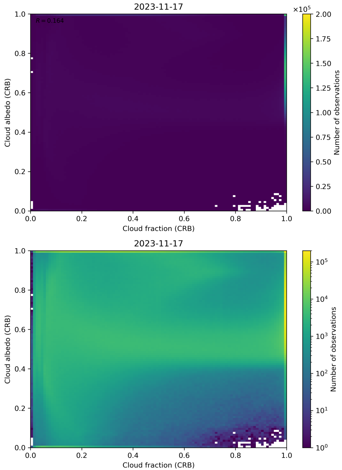
Figure 77: Scatter density plot of “Cloud fraction (CRB)” against “Cloud albedo (CRB)” for 2023-11-16 to 2023-11-18.
