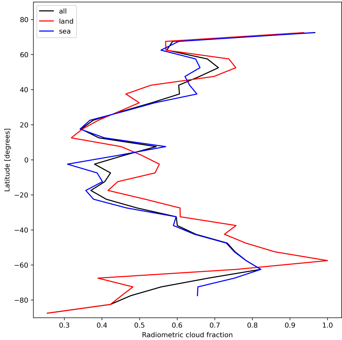
Figure 23: Zonal average of “Radiometric cloud fraction” for 2023-11-16 to 2023-11-18.
