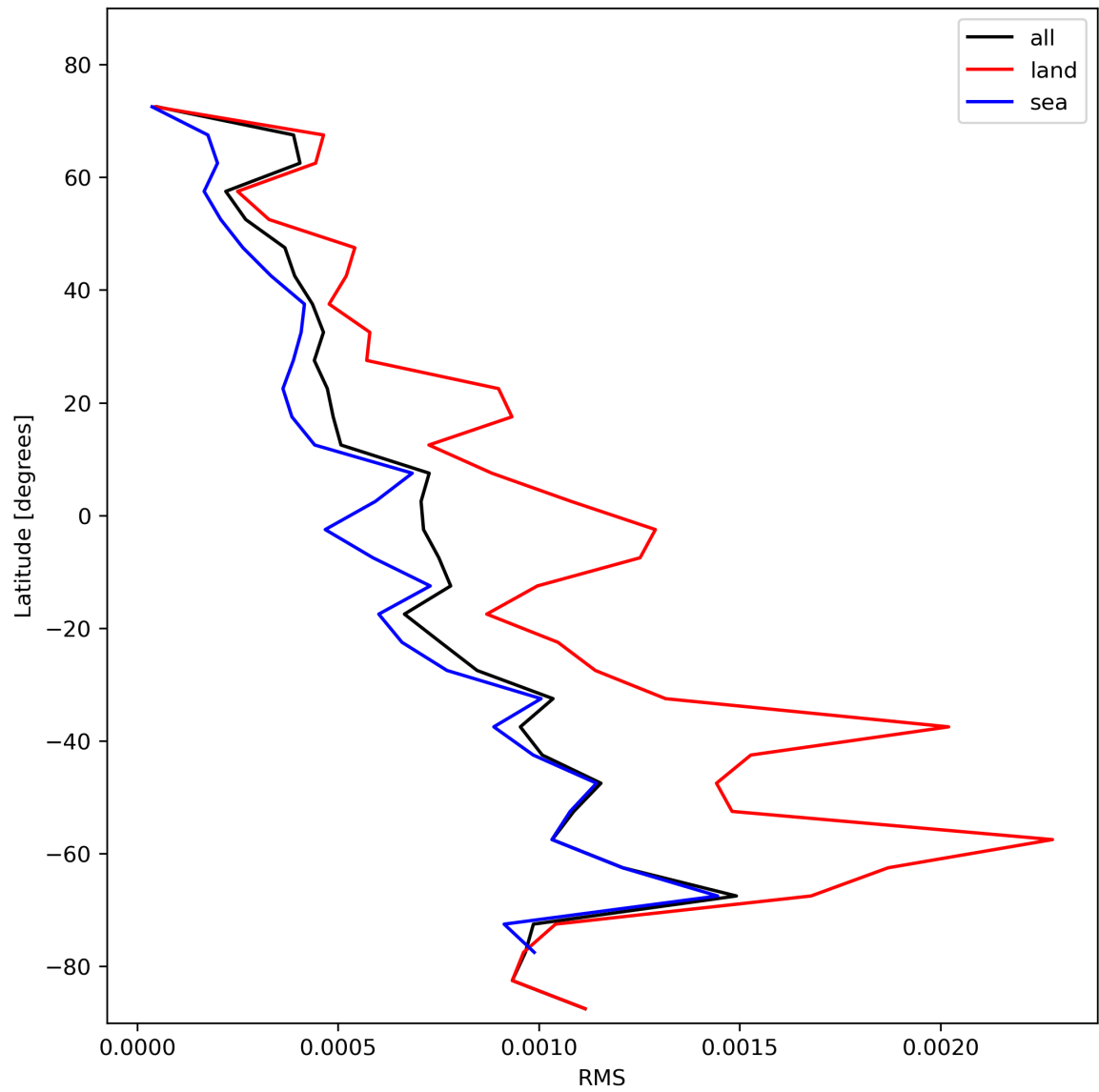
Figure 31: Zonal average of “RMS” for 2023-11-16 to 2023-11-18.
