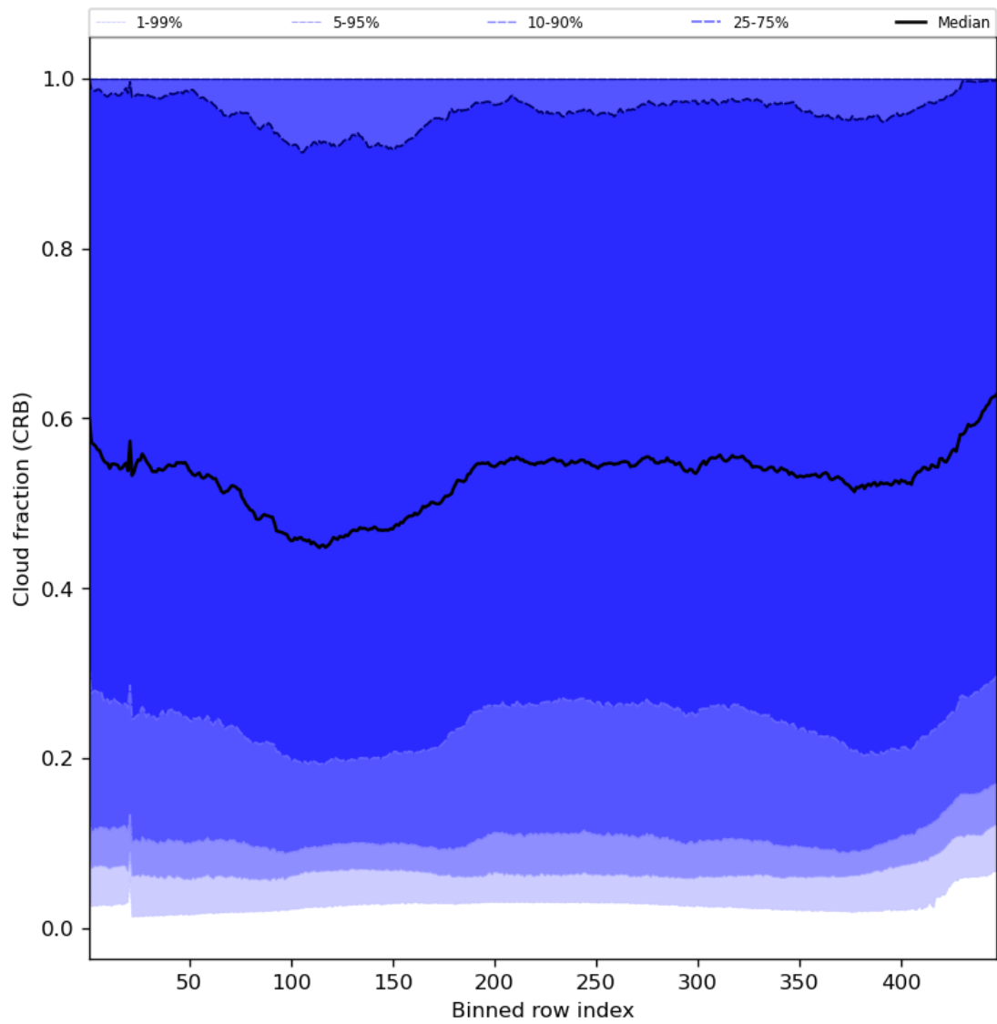
Figure 58: Along track statistics of “Cloud fraction (CRB)” for 2023-11-16 to 2023-11-18
