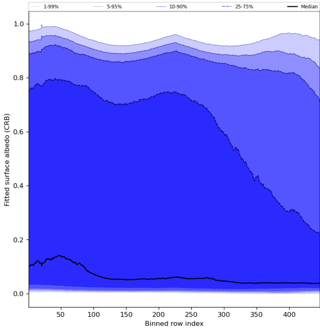
Figure 62: Along track statistics of “Fitted surface albedo (CRB)” for 2023-11-16 to 2023-11-18
