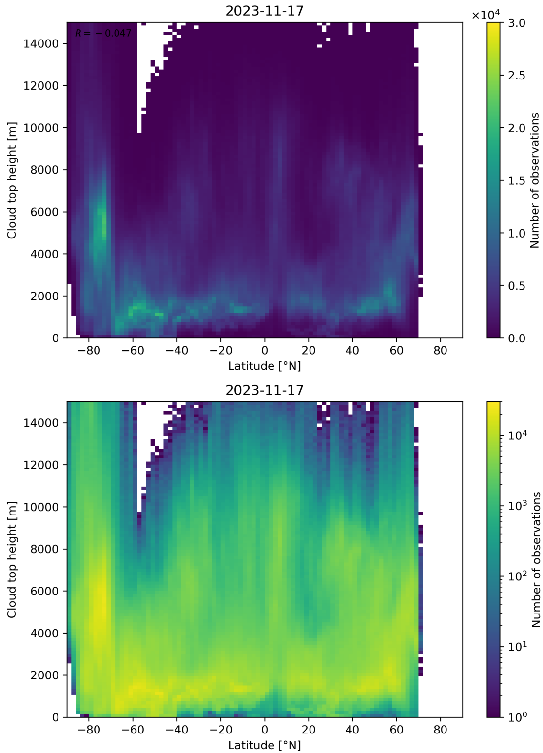
Figure 97: Scatter density plot of “Latitude” against “Cloud top height” for 2023-11-16 to 2023-11-18.
