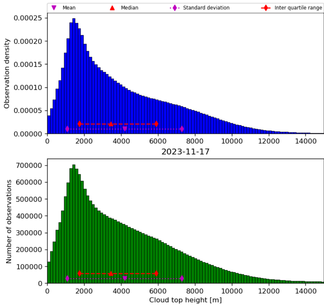
Figure 40: Histogram of “Cloud top height” for 2023-11-16 to 2023-11-18
