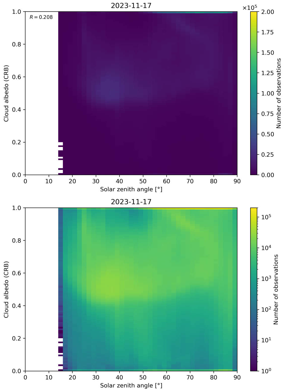
Figure 98: Scatter density plot of “Solar zenith angle” against “Cloud albedo (CRB)” for 2023-11-16 to 2023-11-18.
