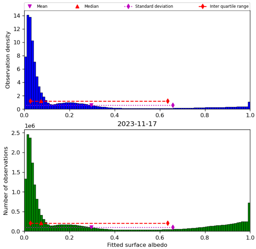
Figure 45: Histogram of “Fitted surface albedo” for 2023-11-16 to 2023-11-18
