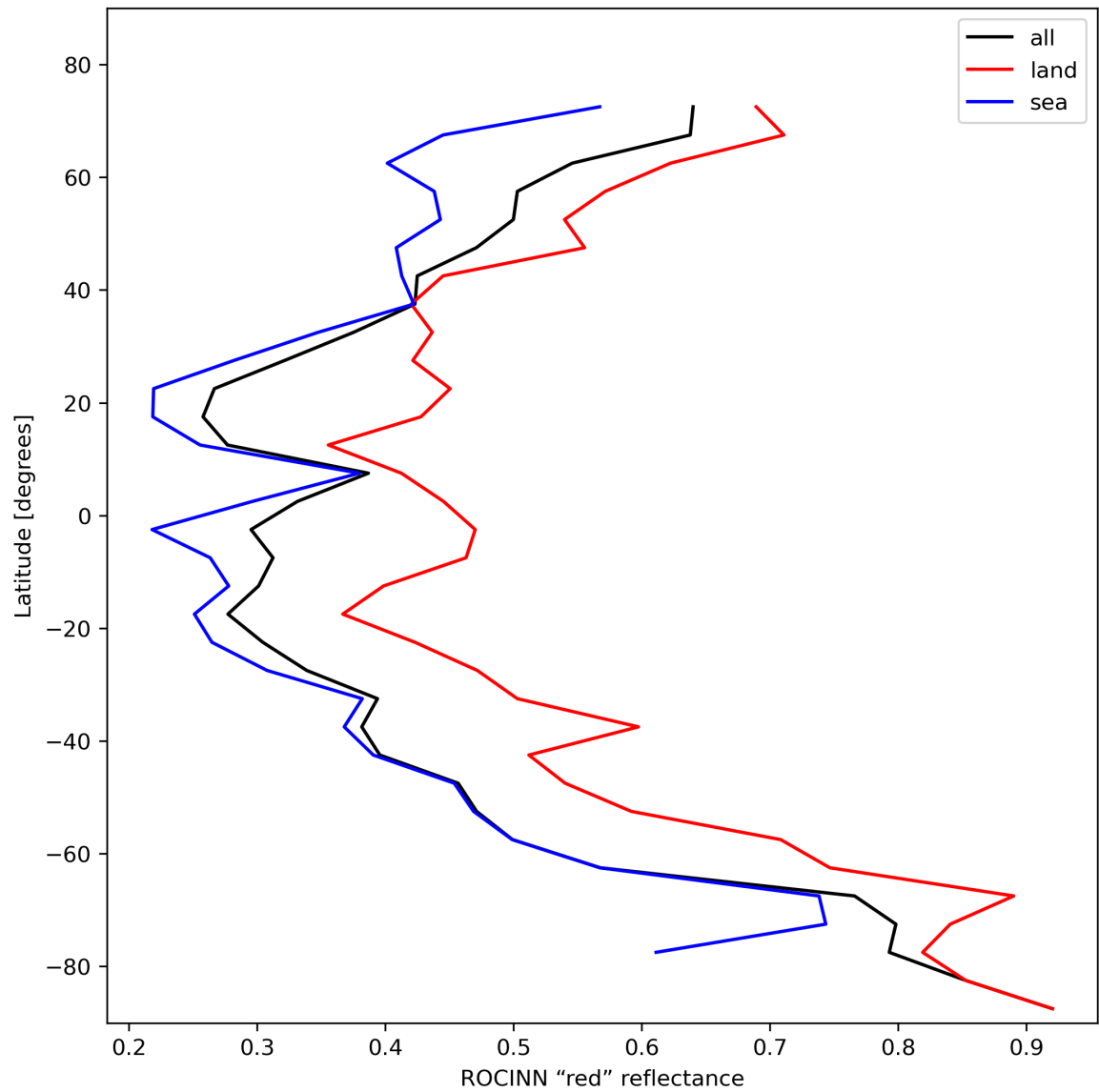
Figure 37: Zonal average of "ROCINN "red" reflectance" for 2023-11-16 to 2023-11-18.
