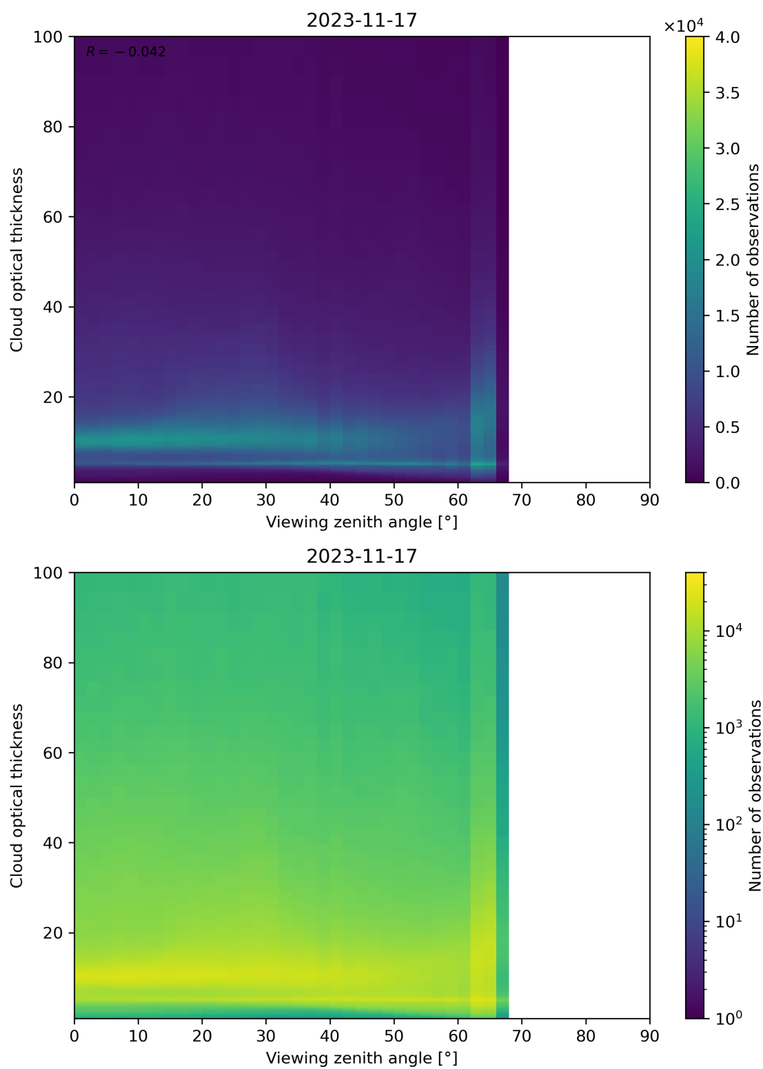
Figure 111: Scatter density plot of “Viewing zenith angle” against “Cloud optical thickness” for 2023-11-16 to 2023-11-18.
