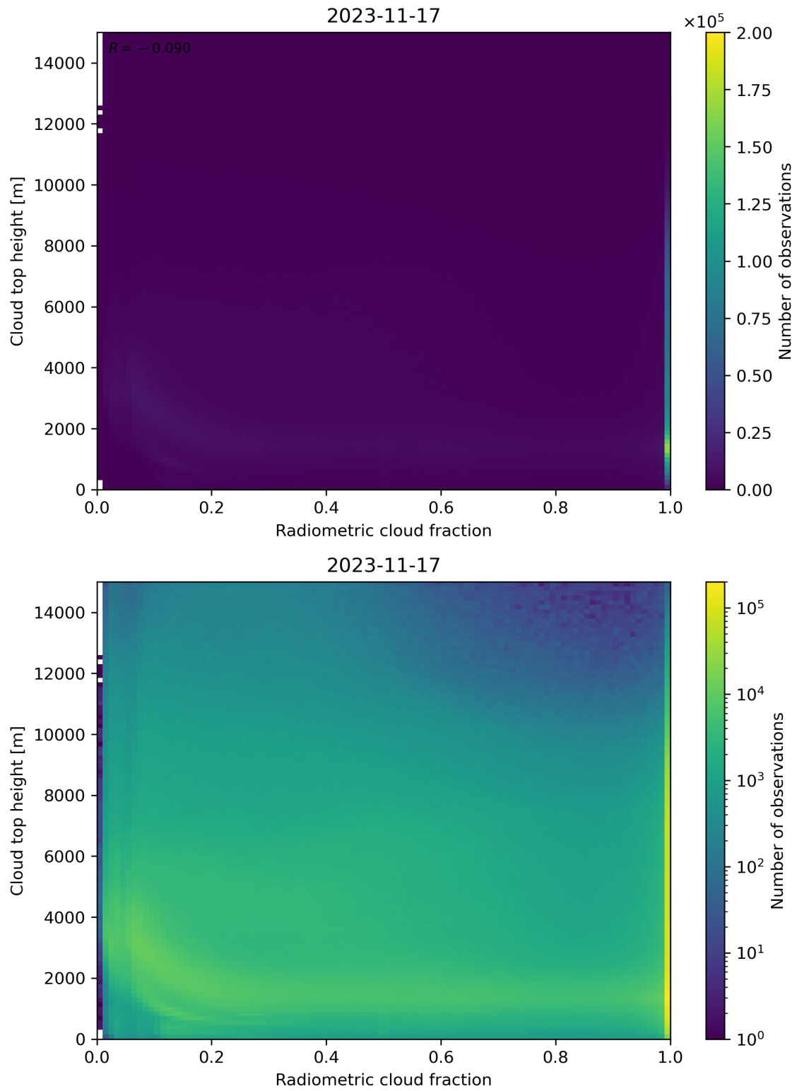
Figure 76: Scatter density plot of “Radiometric cloud fraction” against “Cloud top height” for 2023-11-16 to 2023-11-18.
