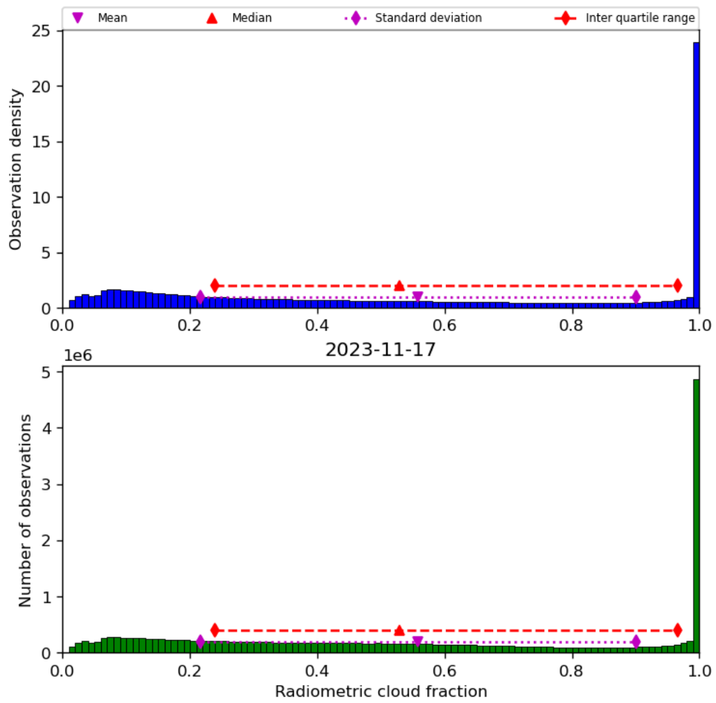
Figure 39: Histogram of “Radiometric cloud fraction” for 2023-11-16 to 2023-11-18
