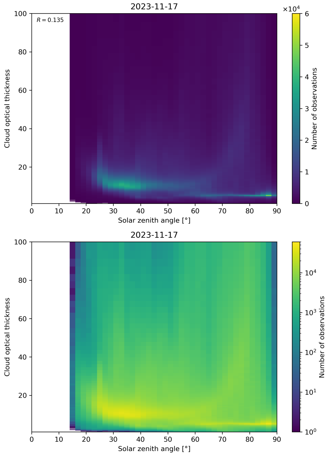
Figure 103: Scatter density plot of “Solar zenith angle” against “Cloud optical thickness” for 2023-11-16 to 2023-11-18.
