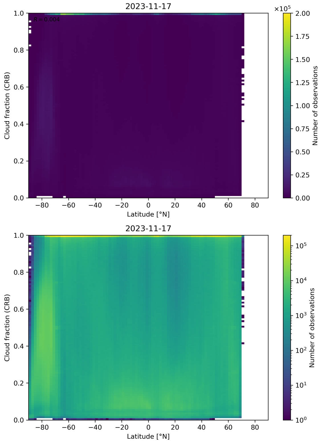
Figure 94: Scatter density plot of “Latitude” against “Cloud fraction (CRB)” for 2023-11-16 to 2023-11-18.
