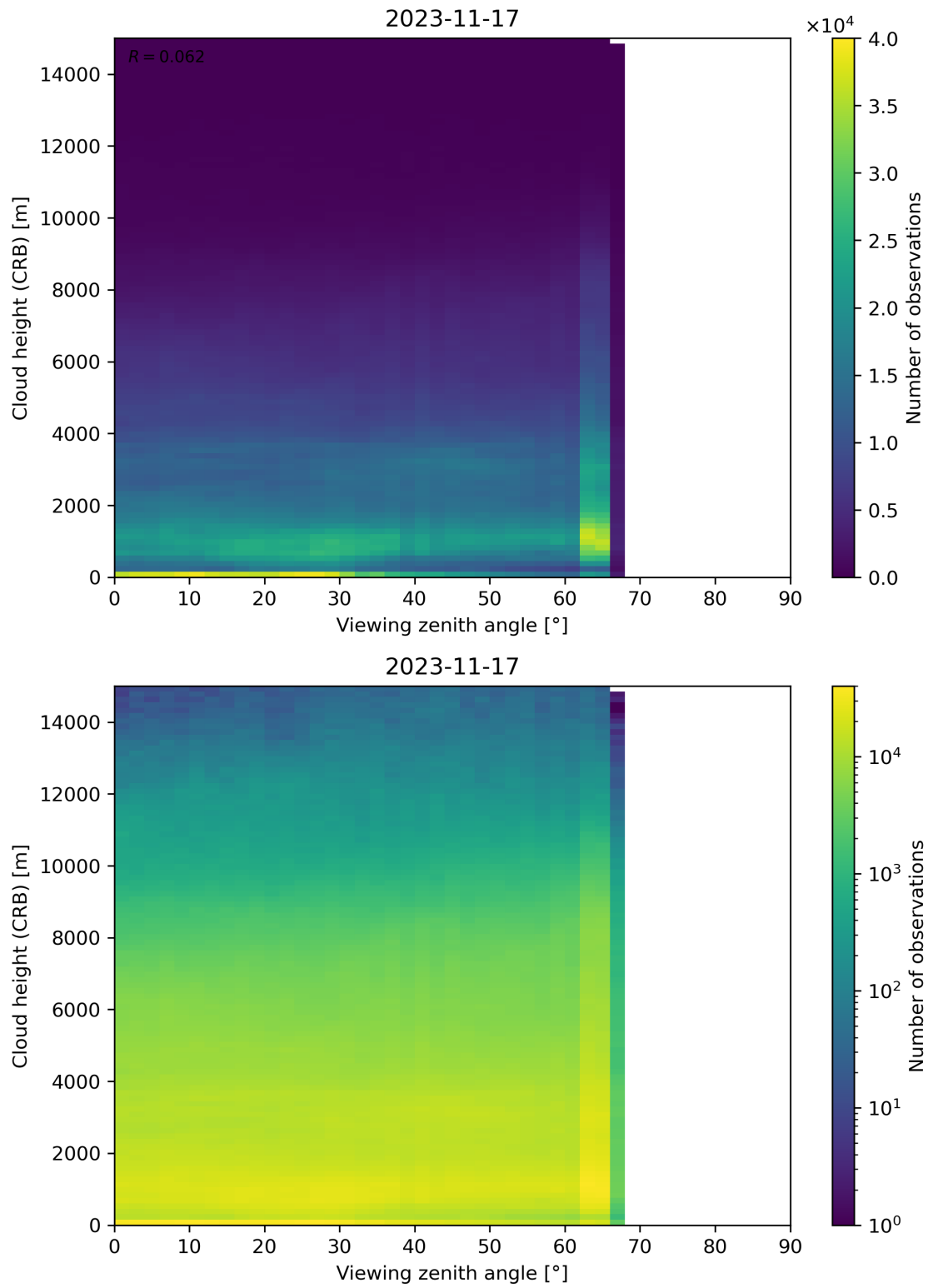
Figure 110: Scatter density plot of “Viewing zenith angle” against “Cloud height (CRB)” for 2023-11-16 to 2023-11-18.
