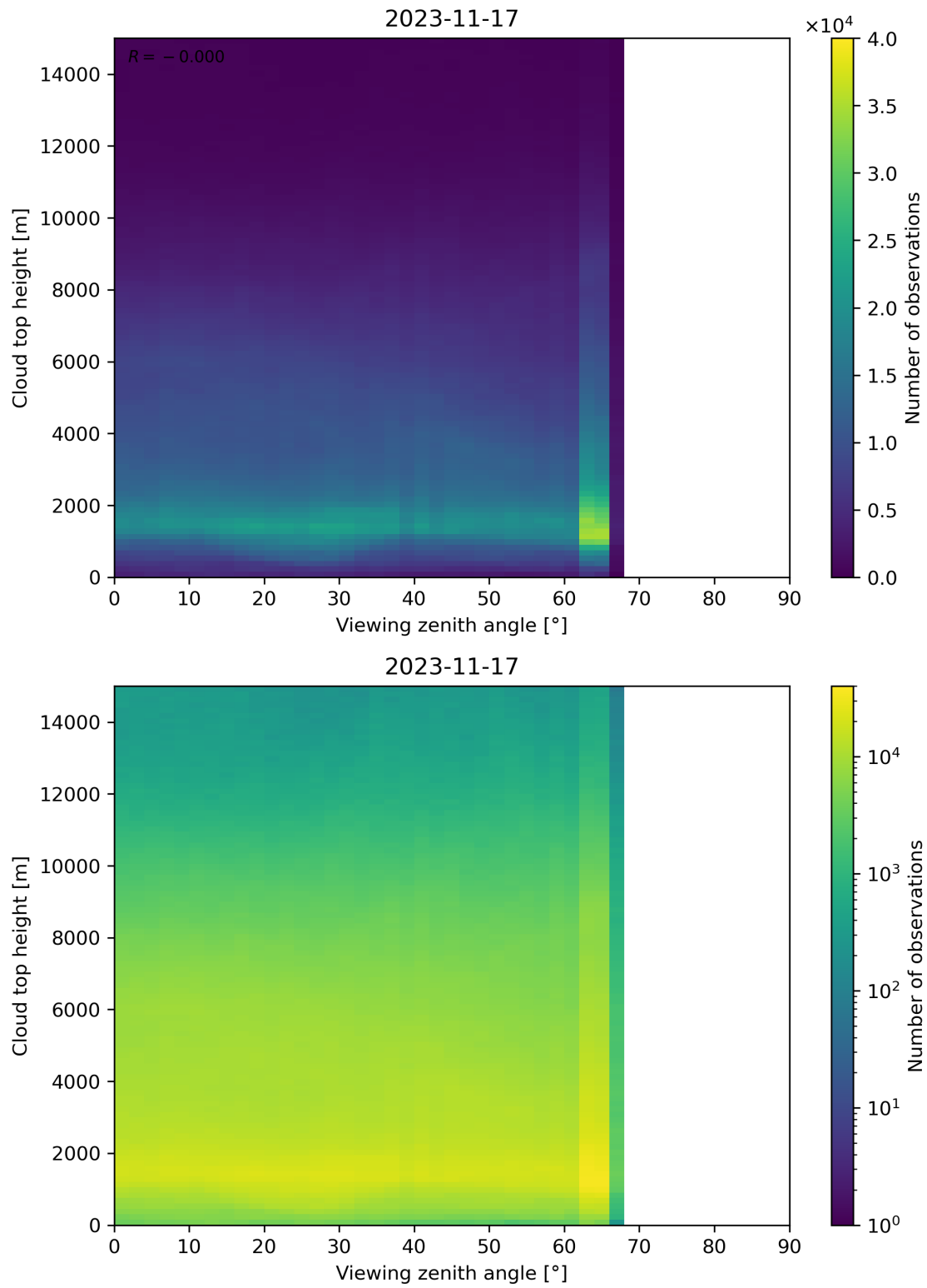
Figure 112: Scatter density plot of “Viewing zenith angle” against “Cloud top height” for 2023-11-16 to 2023-11-18.
