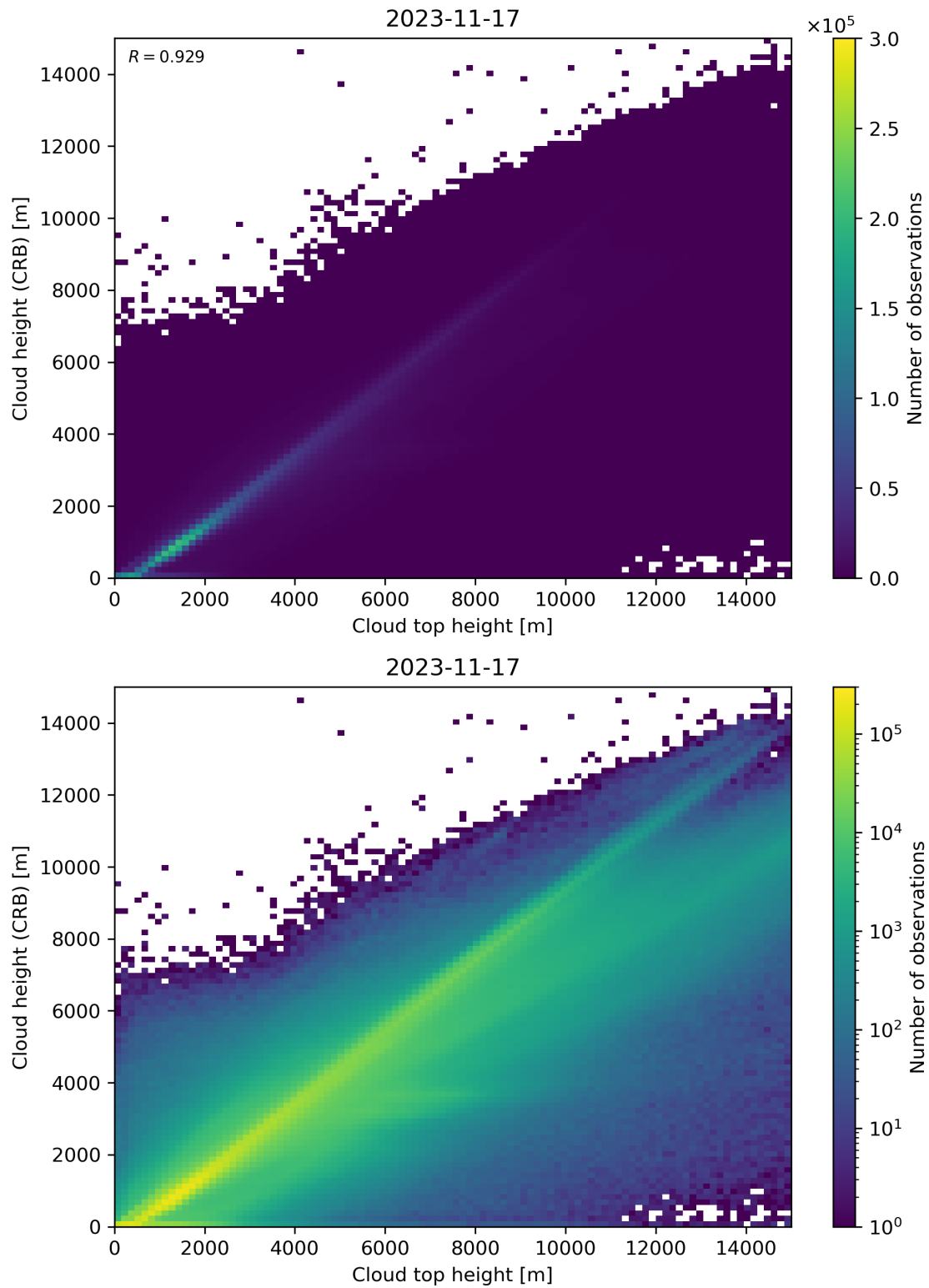
Figure 89: Scatter density plot of “Cloud top height” against “Cloud height (CRB)” for 2023-11-16 to 2023-11-18.
