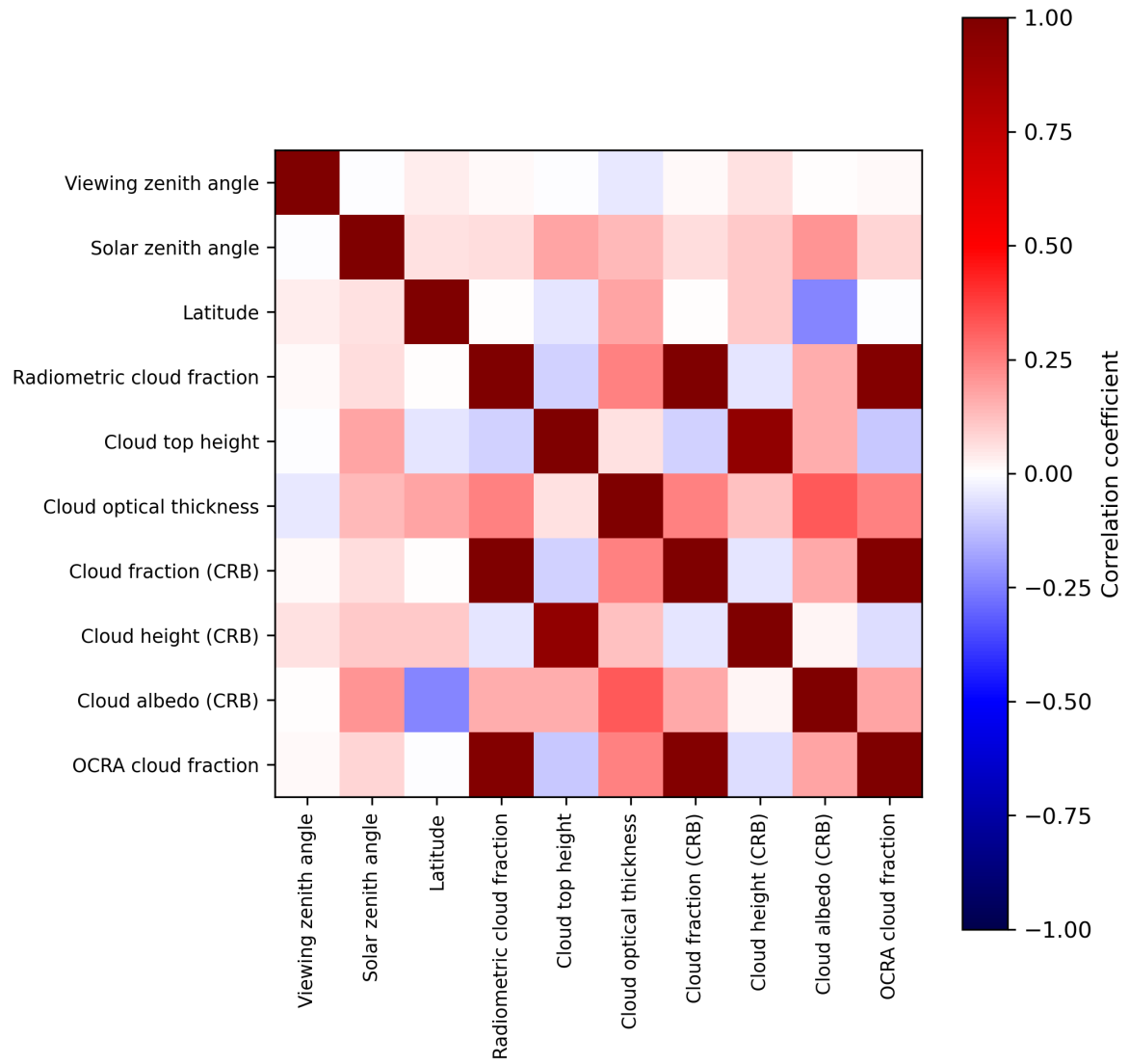
Figure 2: Map of correlation matrix for 2023-11-16 to 2023-11-18.
