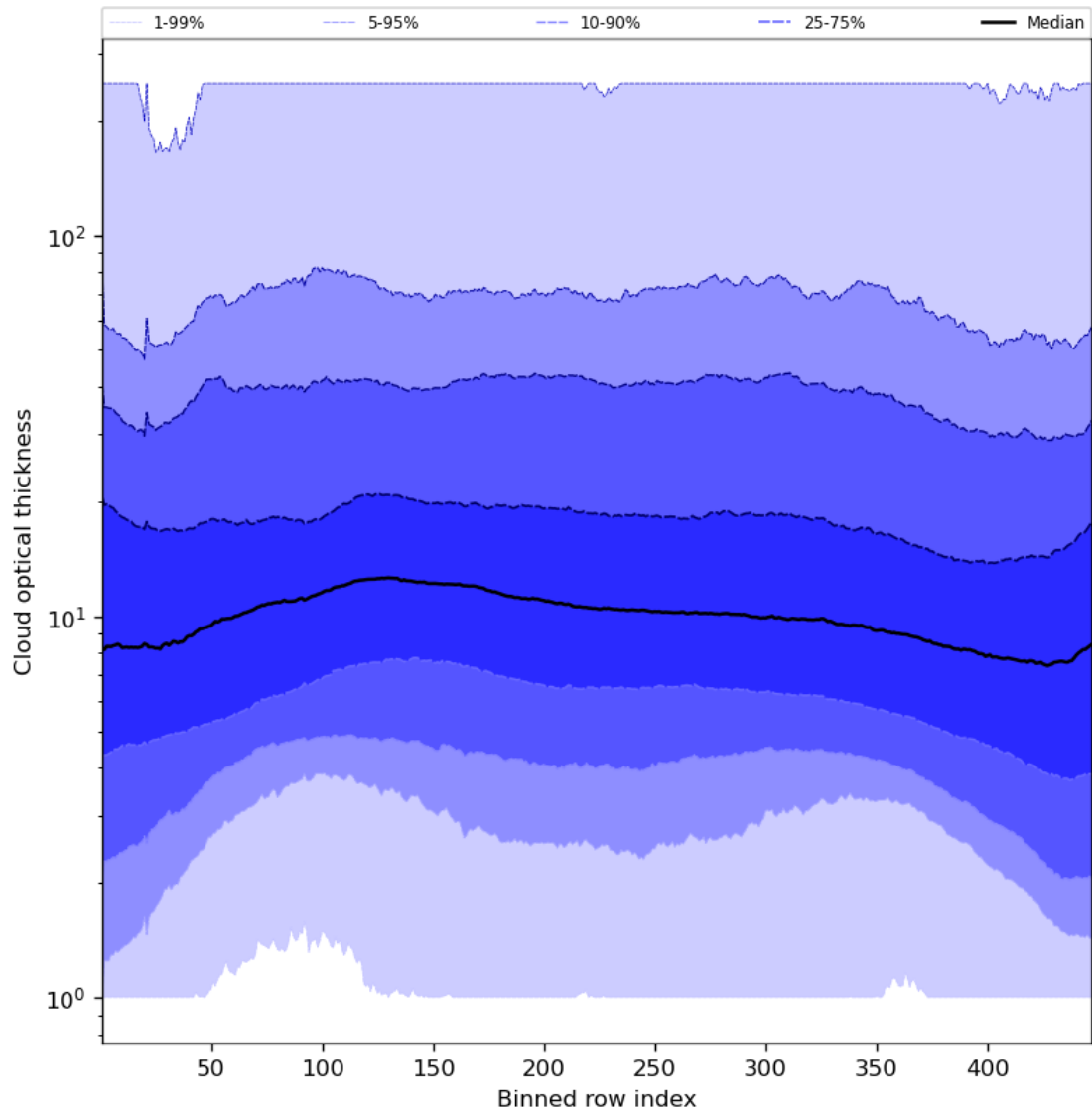
Figure 57: Along track statistics of “Cloud optical thickness” for 2023-11-16 to 2023-11-18
