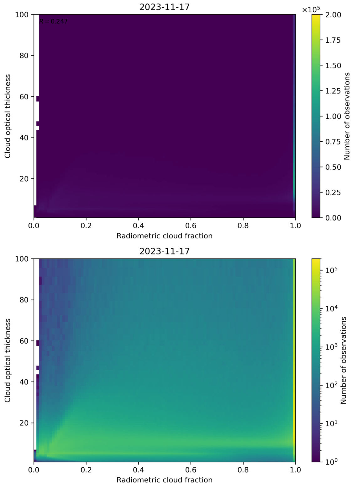
Figure 75: Scatter density plot of “Radiometric cloud fraction” against “Cloud optical thickness” for 2023-11-16 to 2023-11-18.
