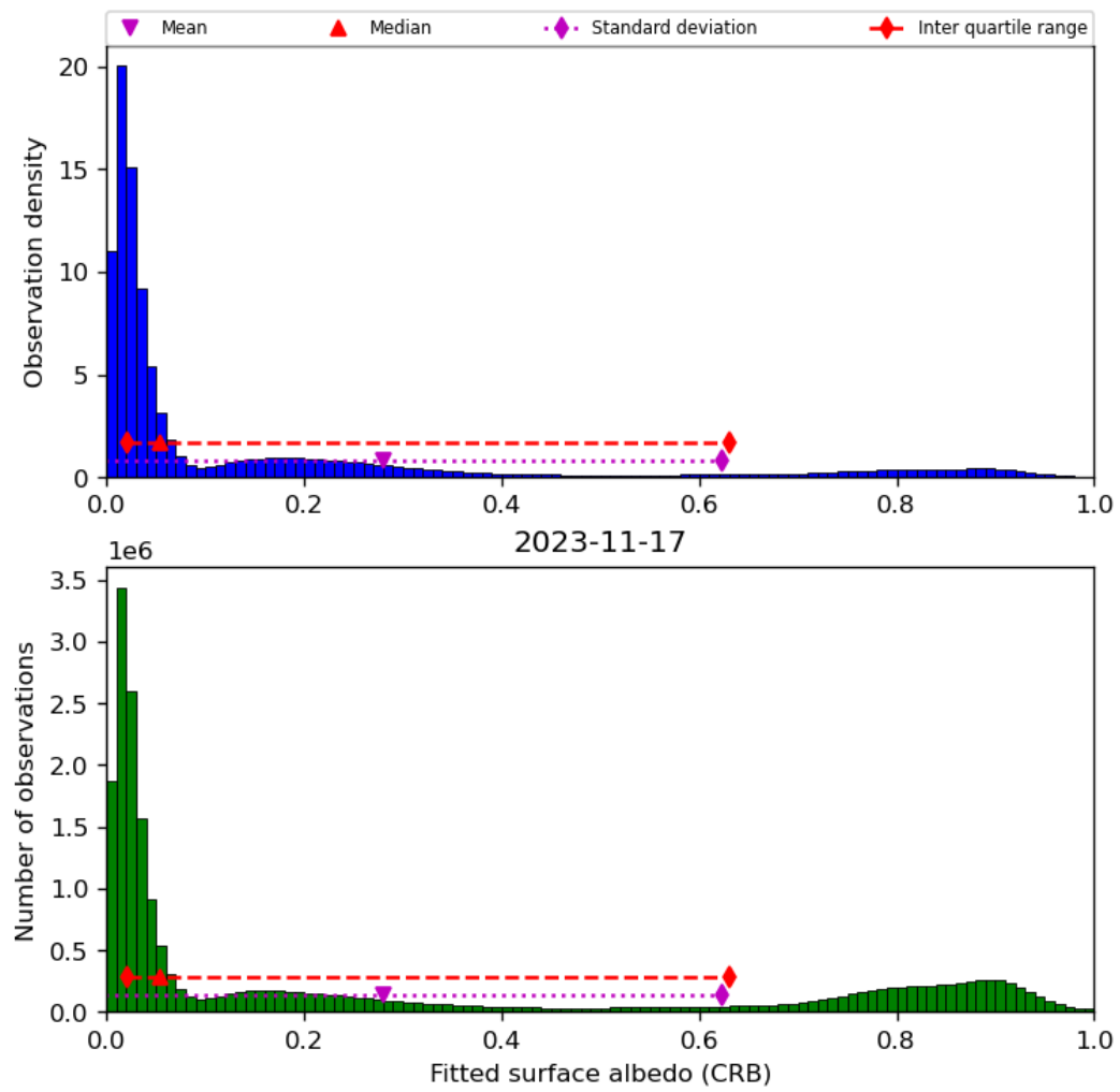
Figure 46: Histogram of “Fitted surface albedo (CRB)” for 2023-11-16 to 2023-11-18
