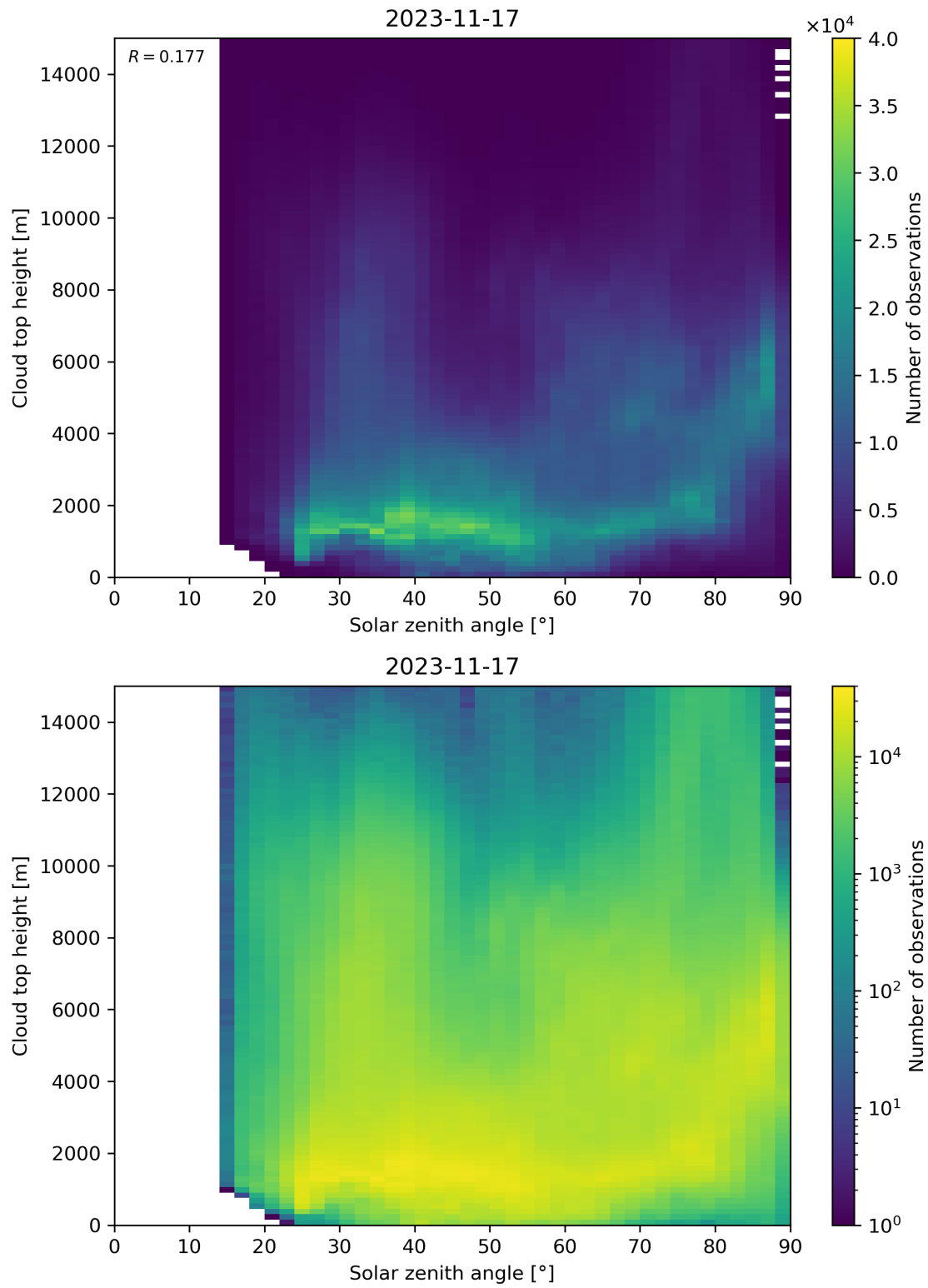
Figure 104: Scatter density plot of “Solar zenith angle” against “Cloud top height” for 2023-11-16 to 2023-11-18.
