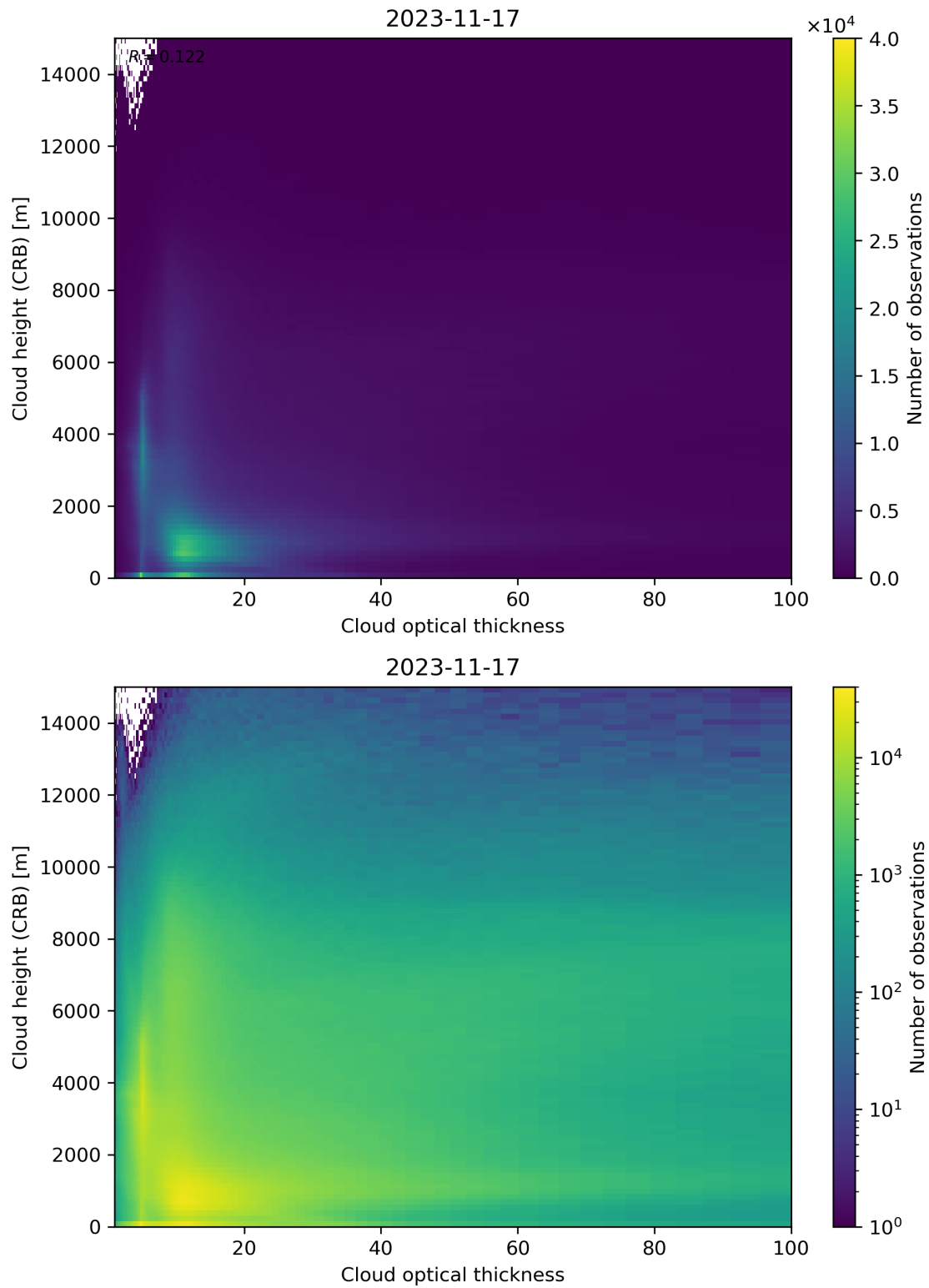
Figure 85: Scatter density plot of “Cloud optical thickness” against “Cloud height (CRB)” for 2023-11-16 to 2023-11-18.
