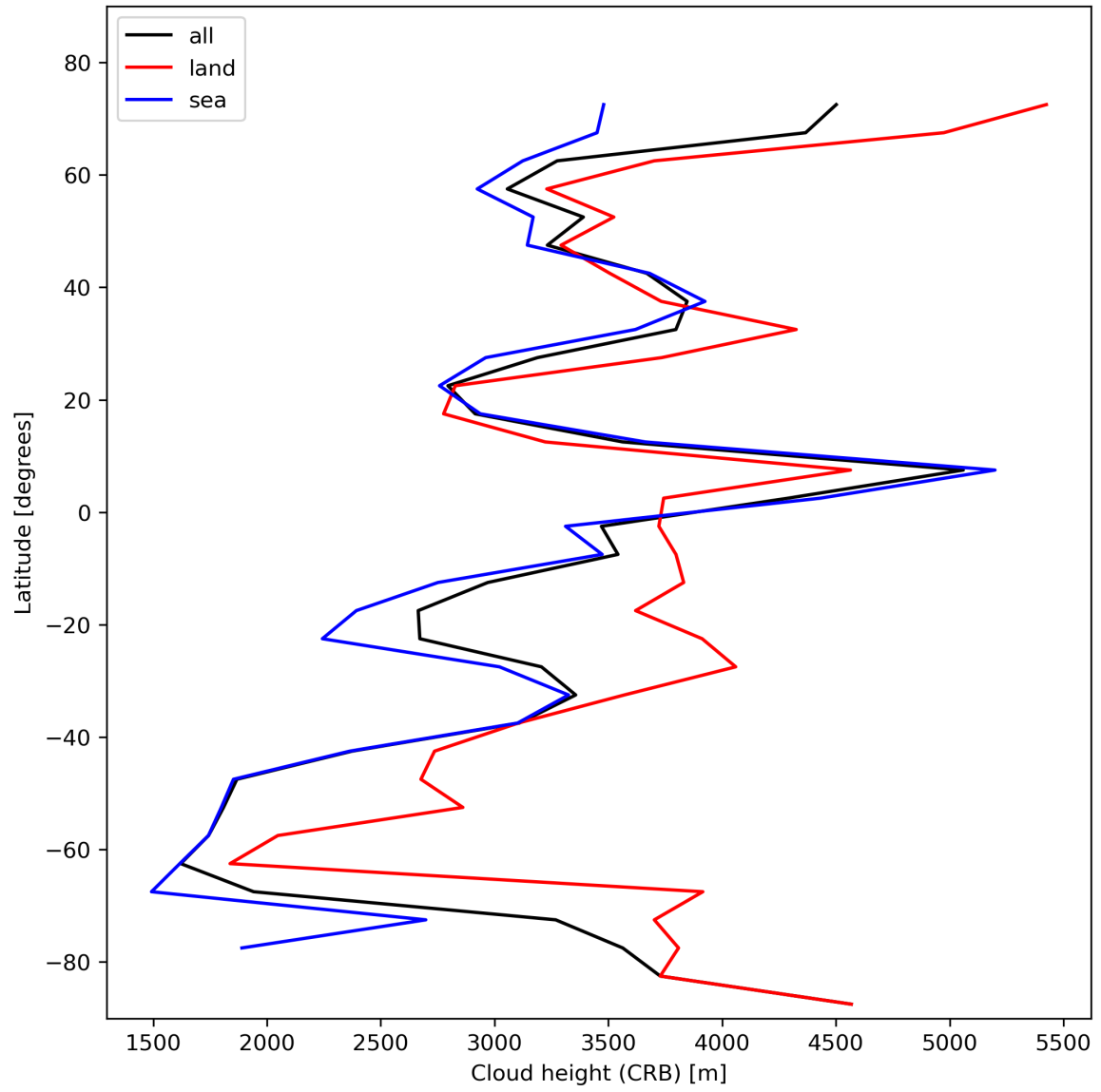
Figure 27: Zonal average of “Cloud height (CRB)” for 2023-11-16 to 2023-11-18.
