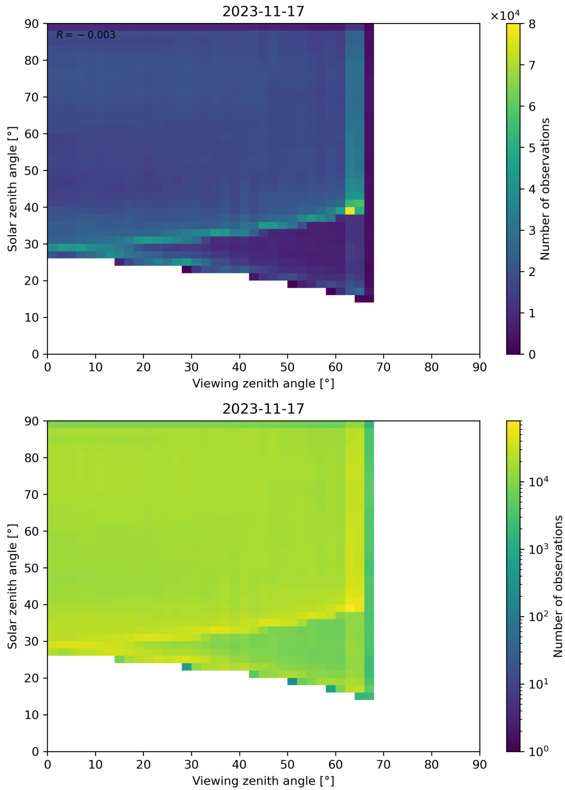
Figure 114: Scatter density plot of “Viewing zenith angle” against “Solar zenith angle” for 2023-11-16 to 2023-11-18.
