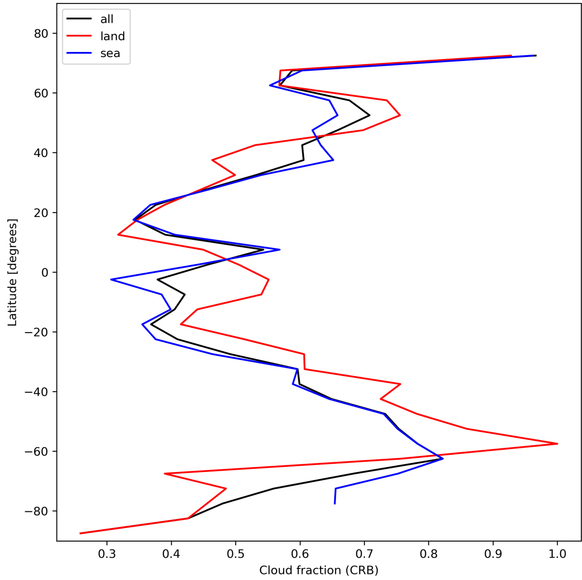
Figure 26: Zonal average of “Cloud fraction (CRB)” for 2023-11-16 to 2023-11-18.
