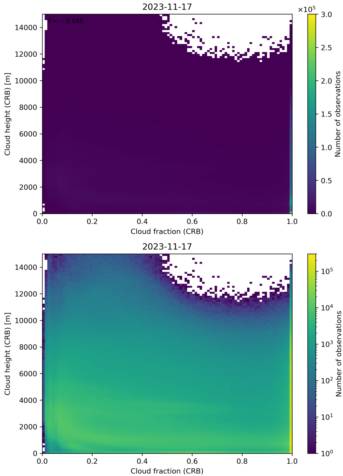
Figure 79: Scatter density plot of “Cloud fraction (CRB)” against “Cloud height (CRB)” for 2023-11-16 to 2023-11-18.
