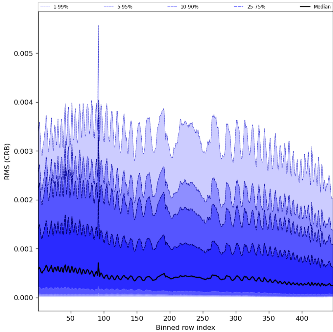
Figure 64: Along track statistics of “RMS (CRB)” for 2023-11-16 to 2023-11-18
