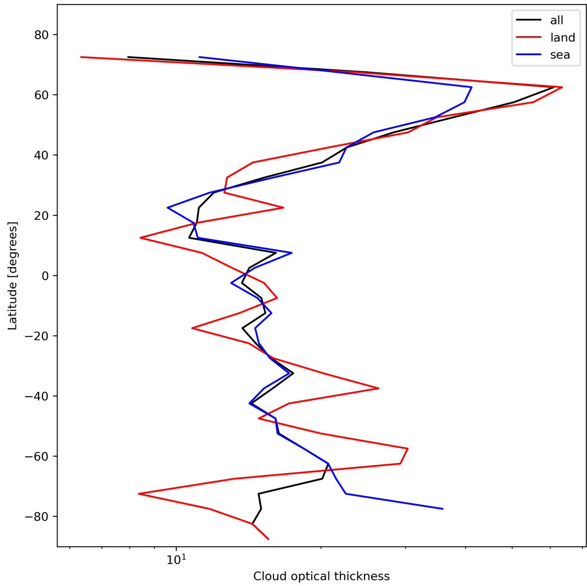
Figure 25: Zonal average of “Cloud optical thickness” for 2023-11-16 to 2023-11-18.
