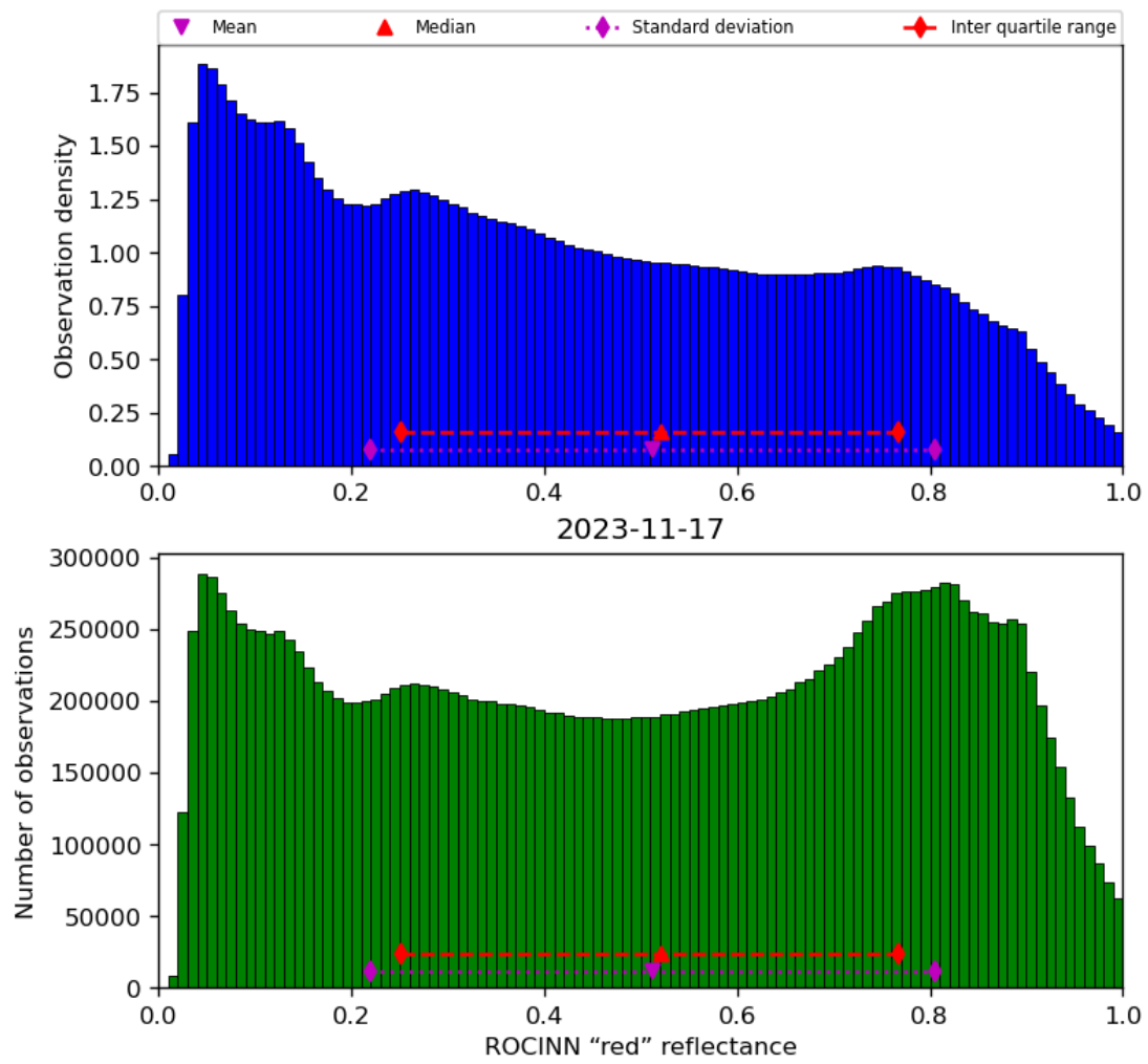
Figure 53: Histogram of “ROCINN “red” reflectance” for 2023-11-16 to 2023-11-18
