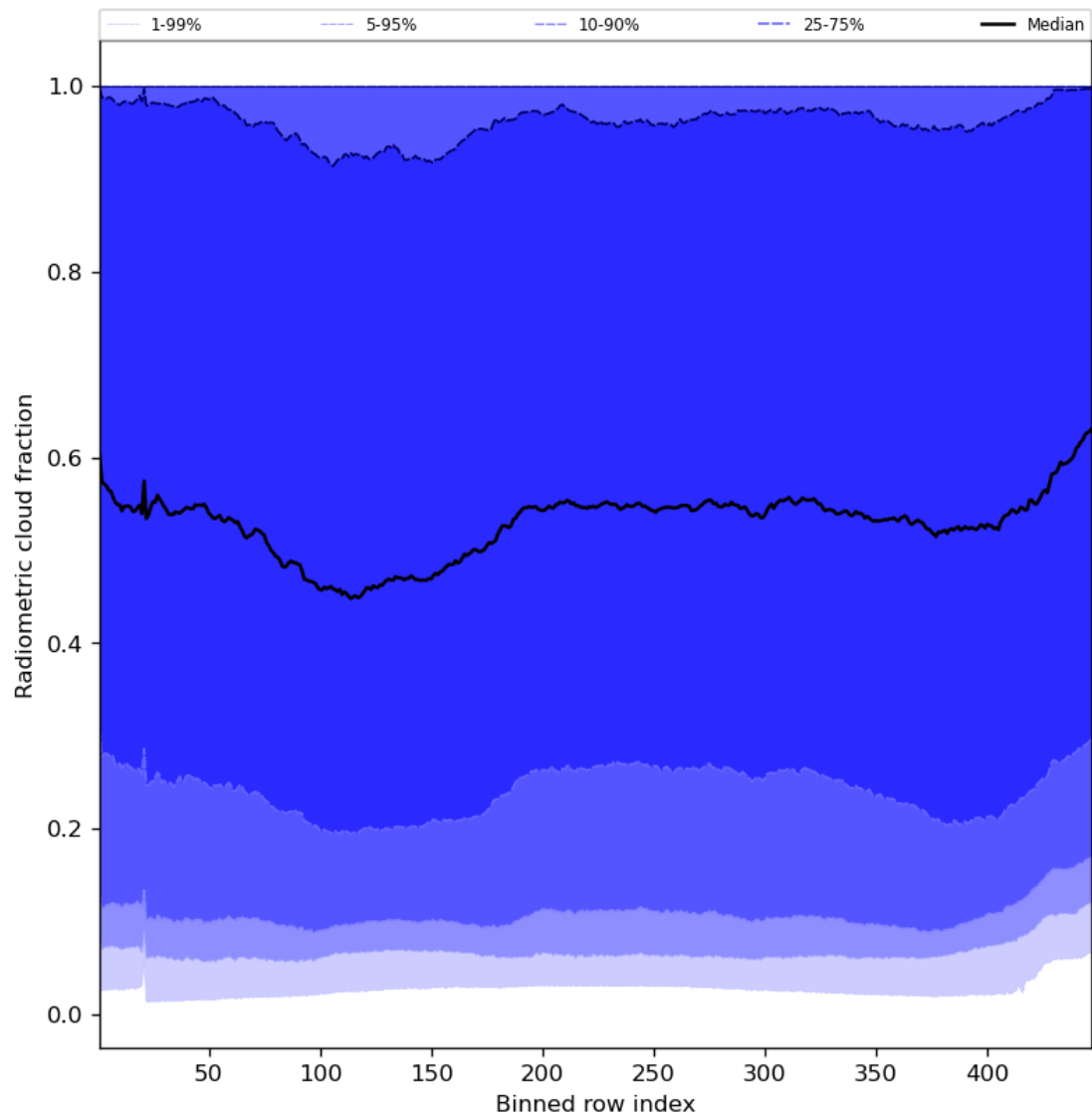
Figure 55: Along track statistics of “Radiometric cloud fraction” for 2023-11-16 to 2023-11-18
