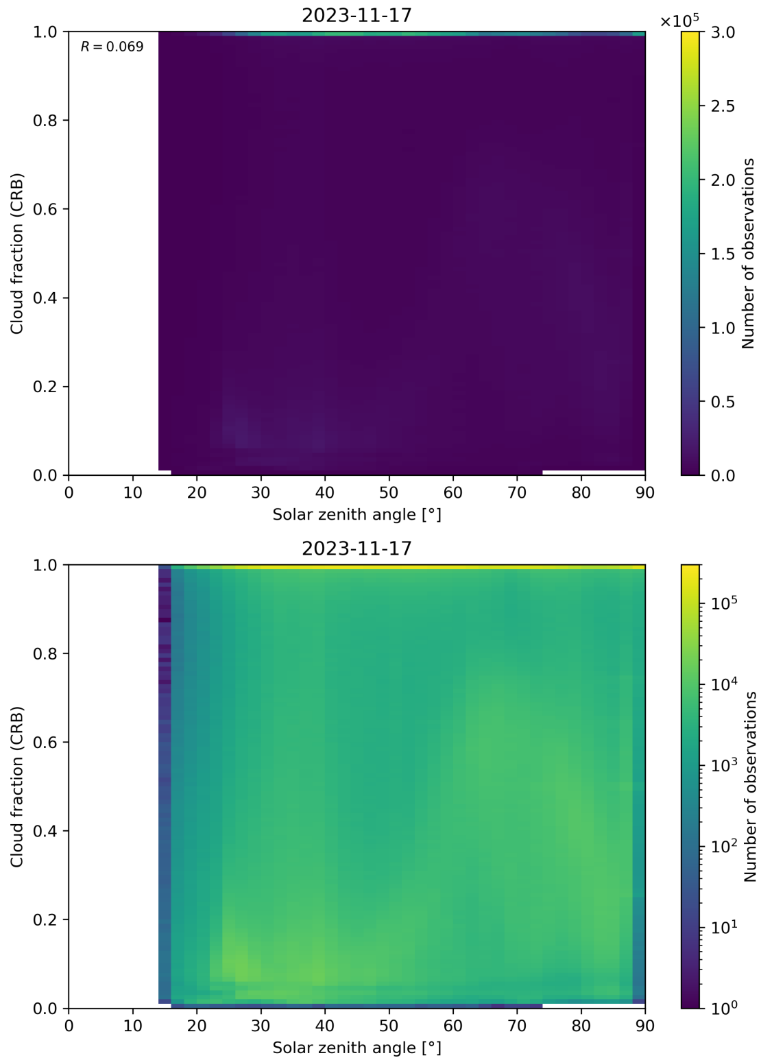
Figure 101: Scatter density plot of “Solar zenith angle” against “Cloud fraction (CRB)” for 2023-11-16 to 2023-11-18.
