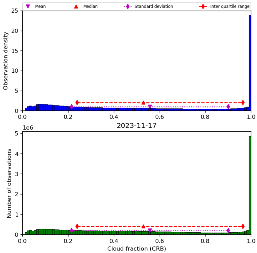
Figure 42: Histogram of “Cloud fraction (CRB)” for 2023-11-16 to 2023-11-18
