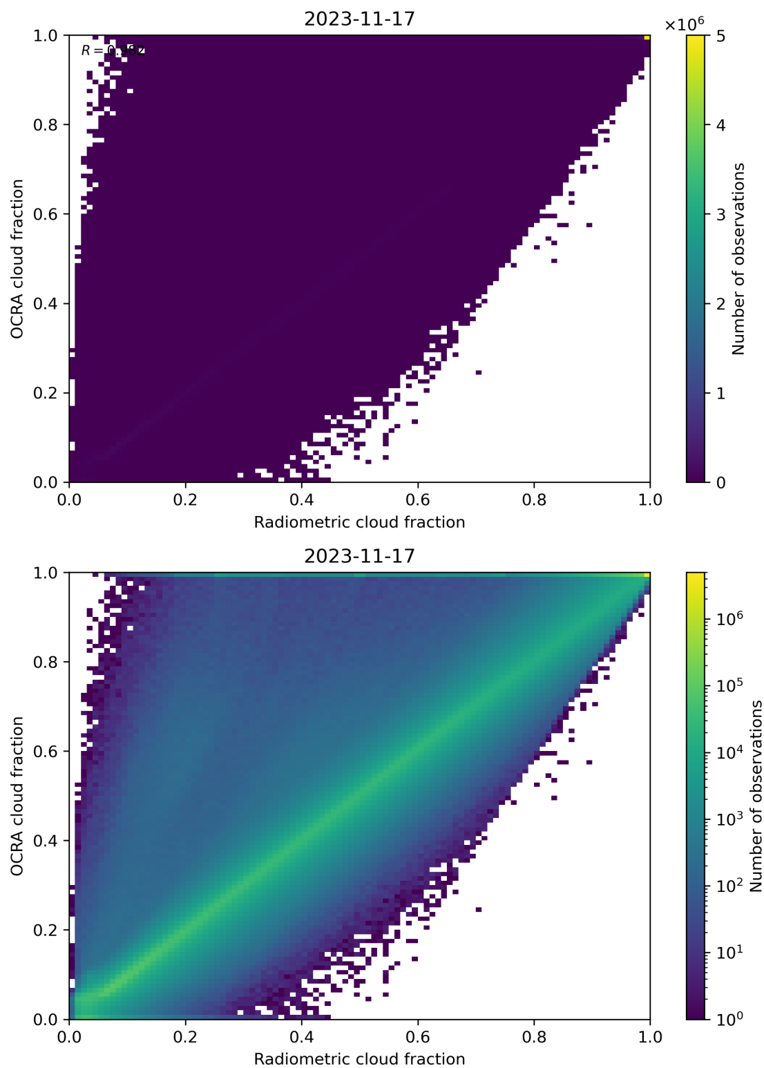
Figure 72: Scatter density plot of “Radiometric cloud fraction” against “OCRA cloud fraction” for 2023-11-16 to 2023-11-18.
