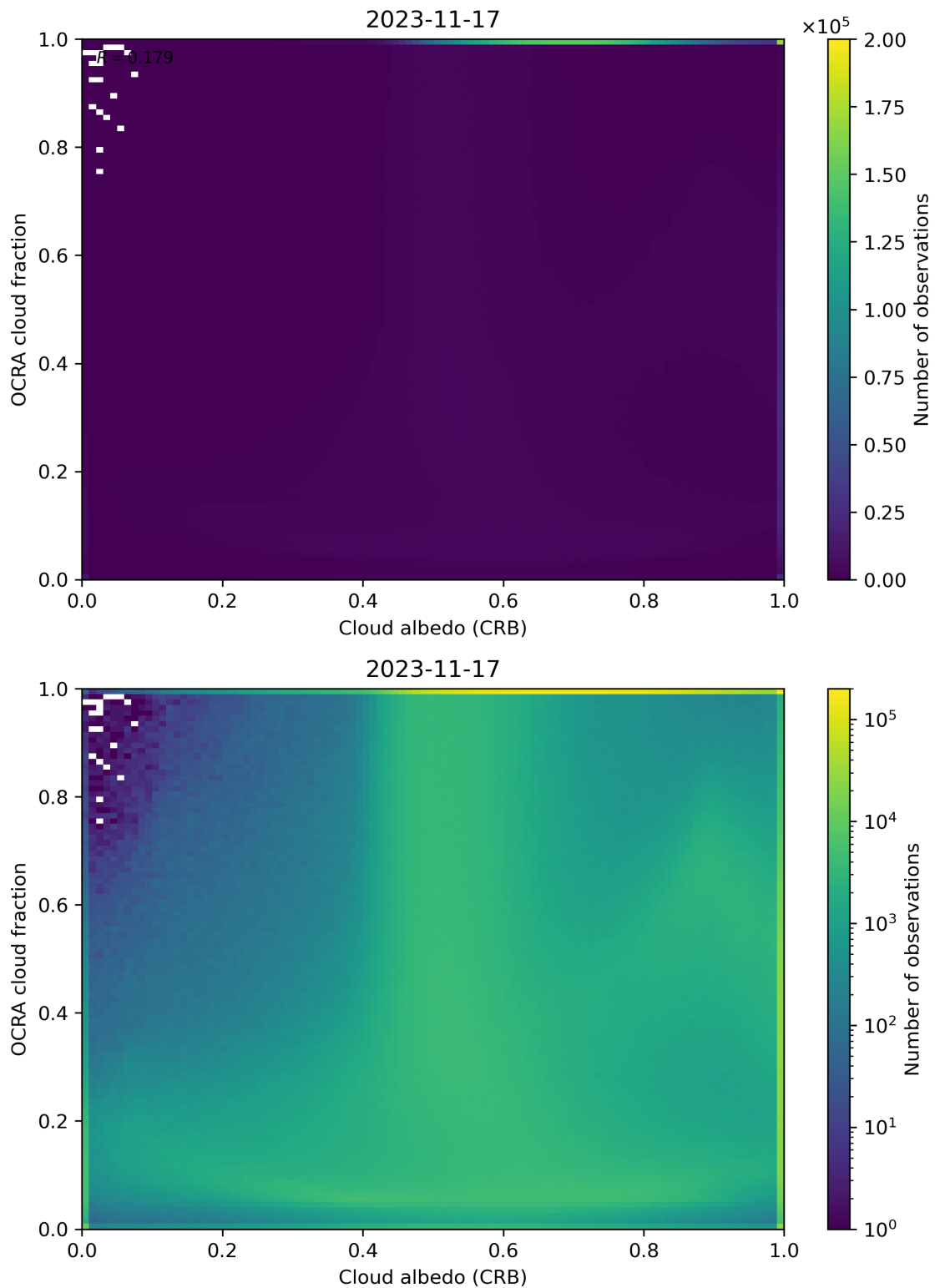
Figure 70: Scatter density plot of “Cloud albedo (CRB)” against “OCRA cloud fraction” for 2023-11-16 to 2023-11-18.
