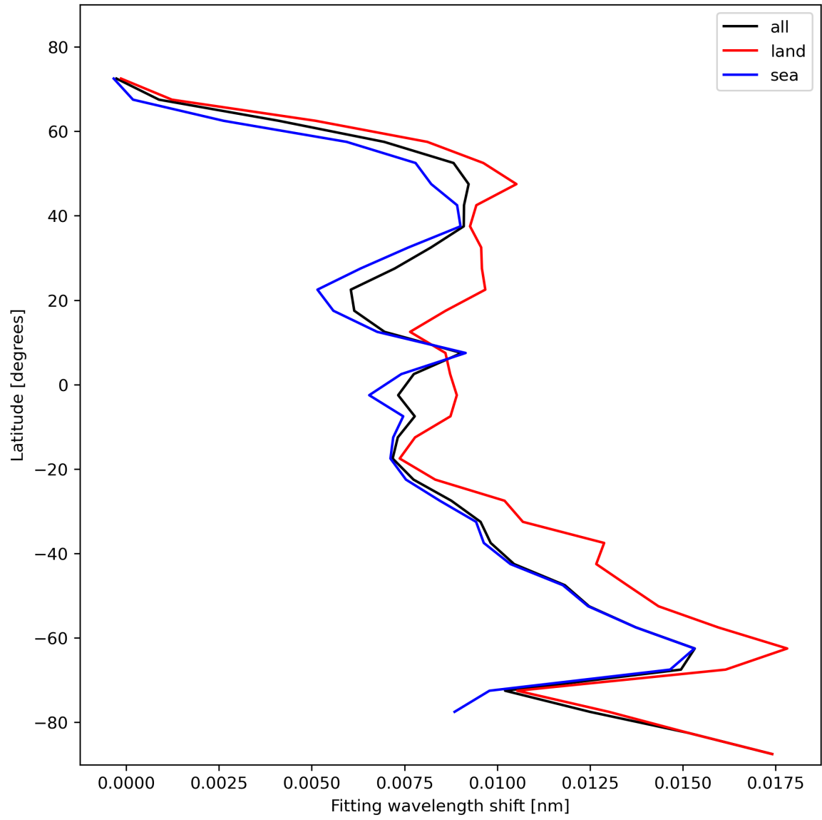
Figure 33: Zonal average of “Fitting wavelength shift” for 2023-11-16 to 2023-11-18.
