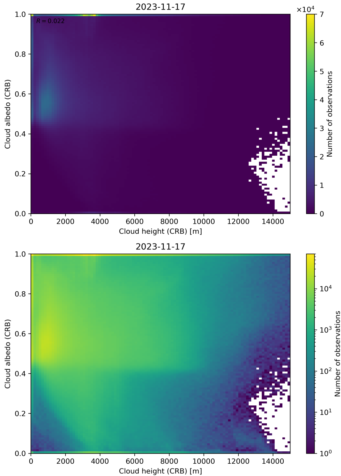
Figure 80: Scatter density plot of “Cloud height (CRB)” against “Cloud albedo (CRB)” for 2023-11-16 to 2023-11-18.
