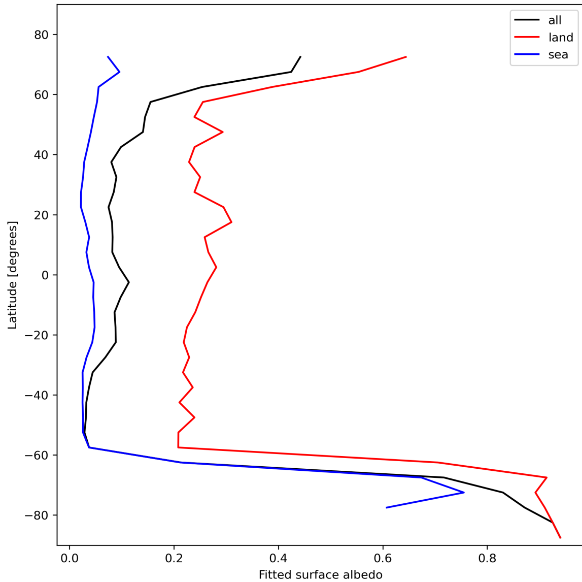
Figure 29: Zonal average of “Fitted surface albedo” for 2023-11-16 to 2023-11-18.
