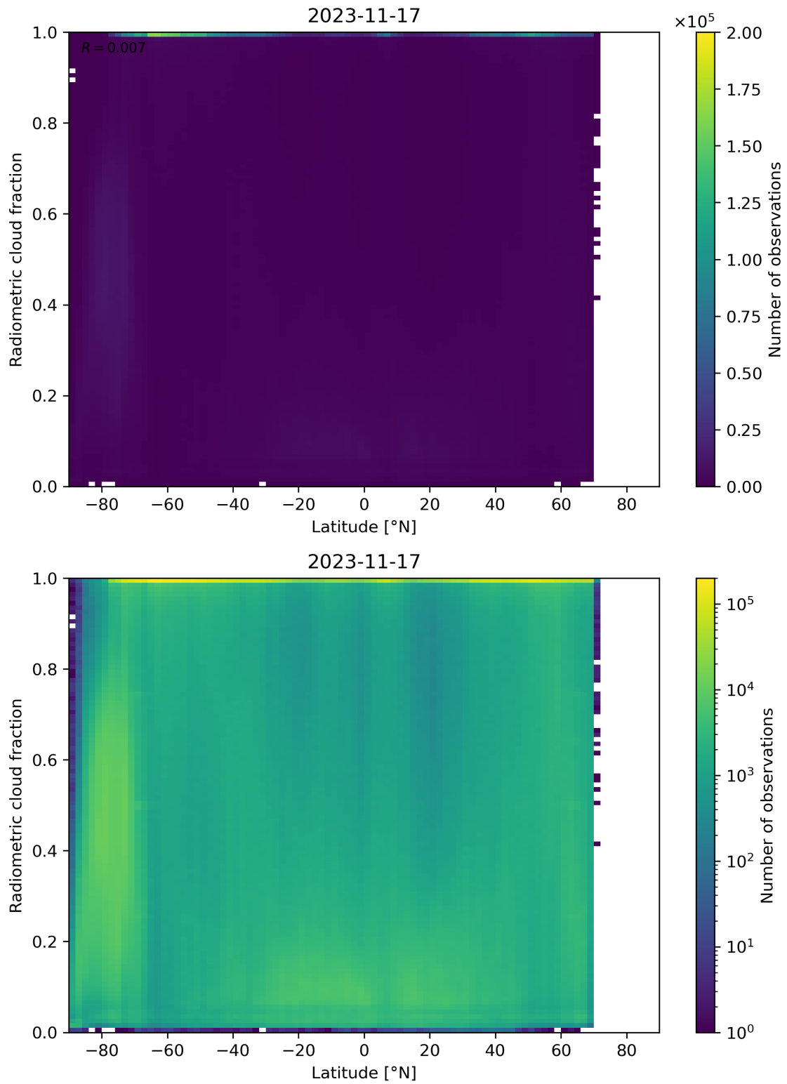
Figure 92: Scatter density plot of “Latitude” against “Radiometric cloud fraction” for 2023-11-16 to 2023-11-18.
