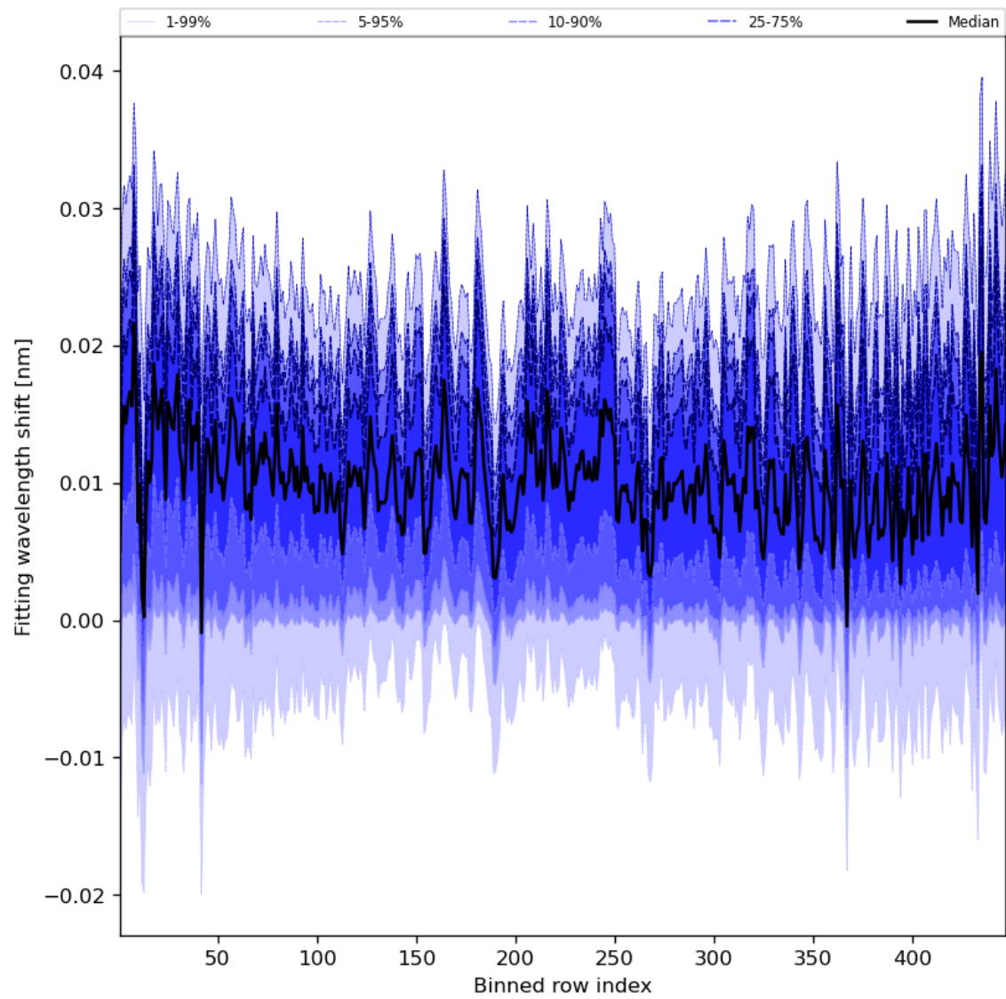
Figure 65: Along track statistics of “Fitting wavelength shift” for 2023-11-16 to 2023-11-18
