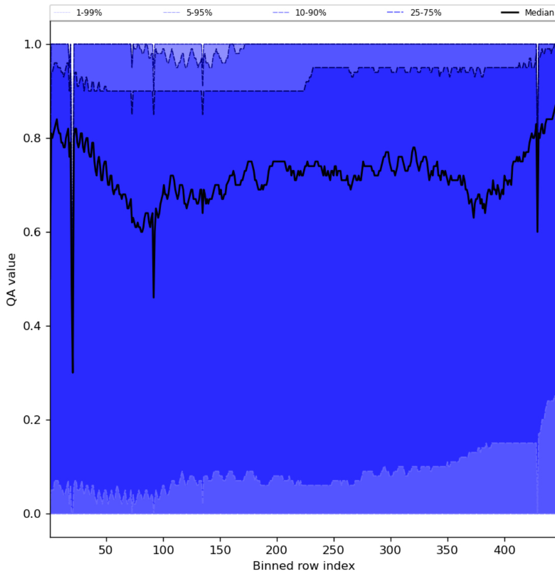
Figure 54: Along track statistics of “QA value” for 2023-11-16 to 2023-11-18
