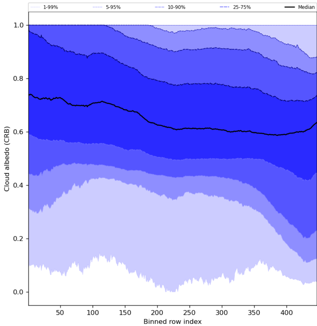
Figure 60: Along track statistics of “Cloud albedo (CRB)” for 2023-11-16 to 2023-11-18
