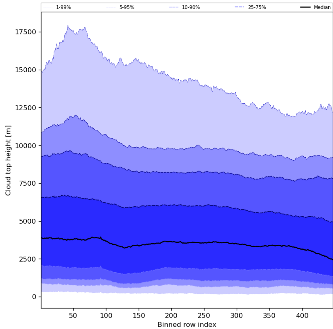
Figure 56: Along track statistics of “Cloud top height” for 2023-11-16 to 2023-11-18
