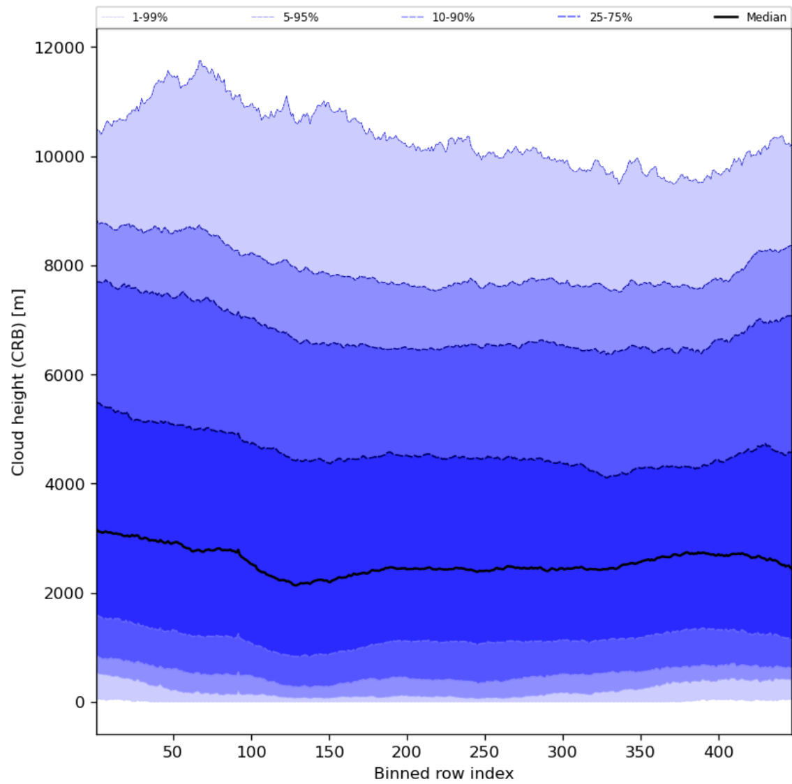
Figure 59: Along track statistics of “Cloud height (CRB)” for 2023-11-16 to 2023-11-18
