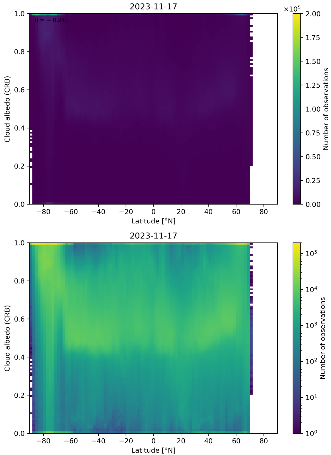
Figure 91: Scatter density plot of “Latitude” against “Cloud albedo (CRB)” for 2023-11-16 to 2023-11-18.
