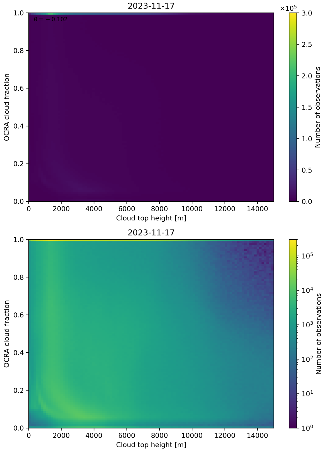
Figure 87: Scatter density plot of “Cloud top height” against “OCRA cloud fraction” for 2023-11-16 to 2023-11-18.
