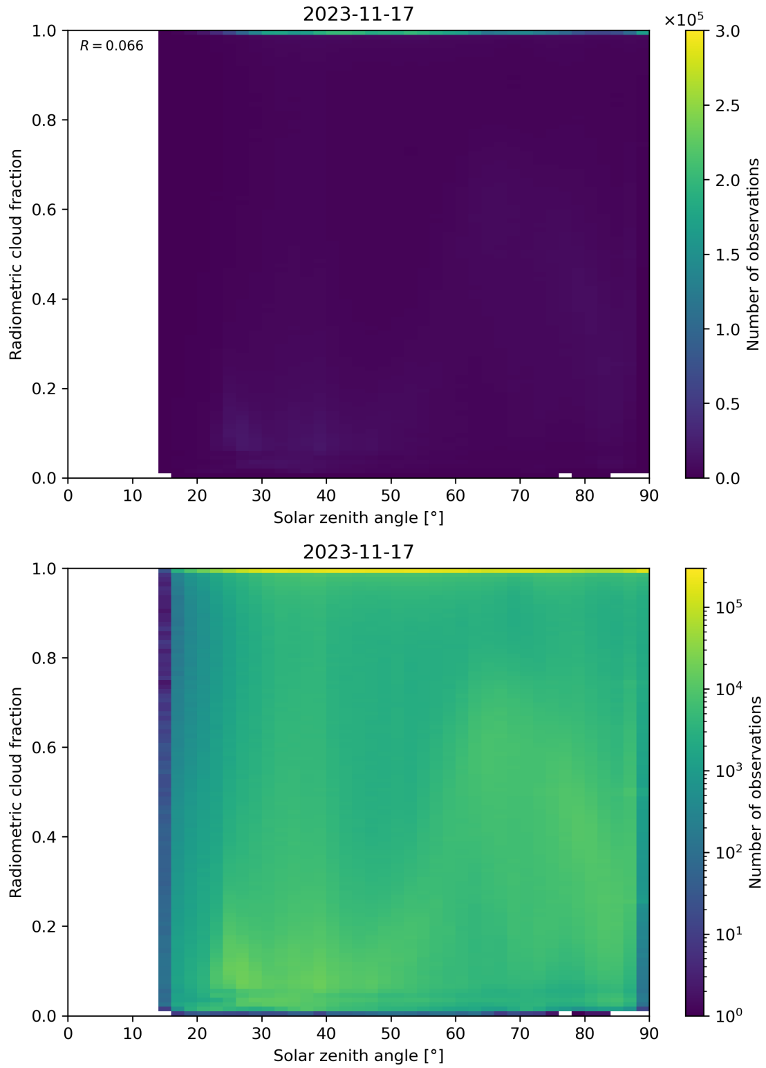
Figure 99: Scatter density plot of “Solar zenith angle” against “Radiometric cloud fraction” for 2023-11-16 to 2023-11-18.
