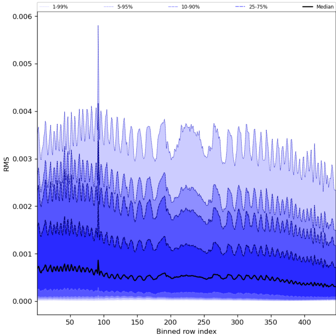
Figure 63: Along track statistics of “RMS” for 2023-11-16 to 2023-11-18
