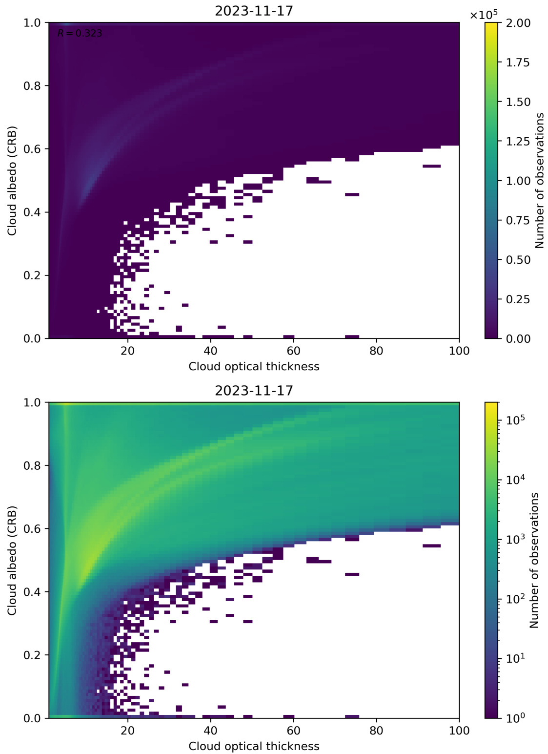
Figure 82: Scatter density plot of “Cloud optical thickness” against “Cloud albedo (CRB)” for 2023-11-16 to 2023-11-18.
