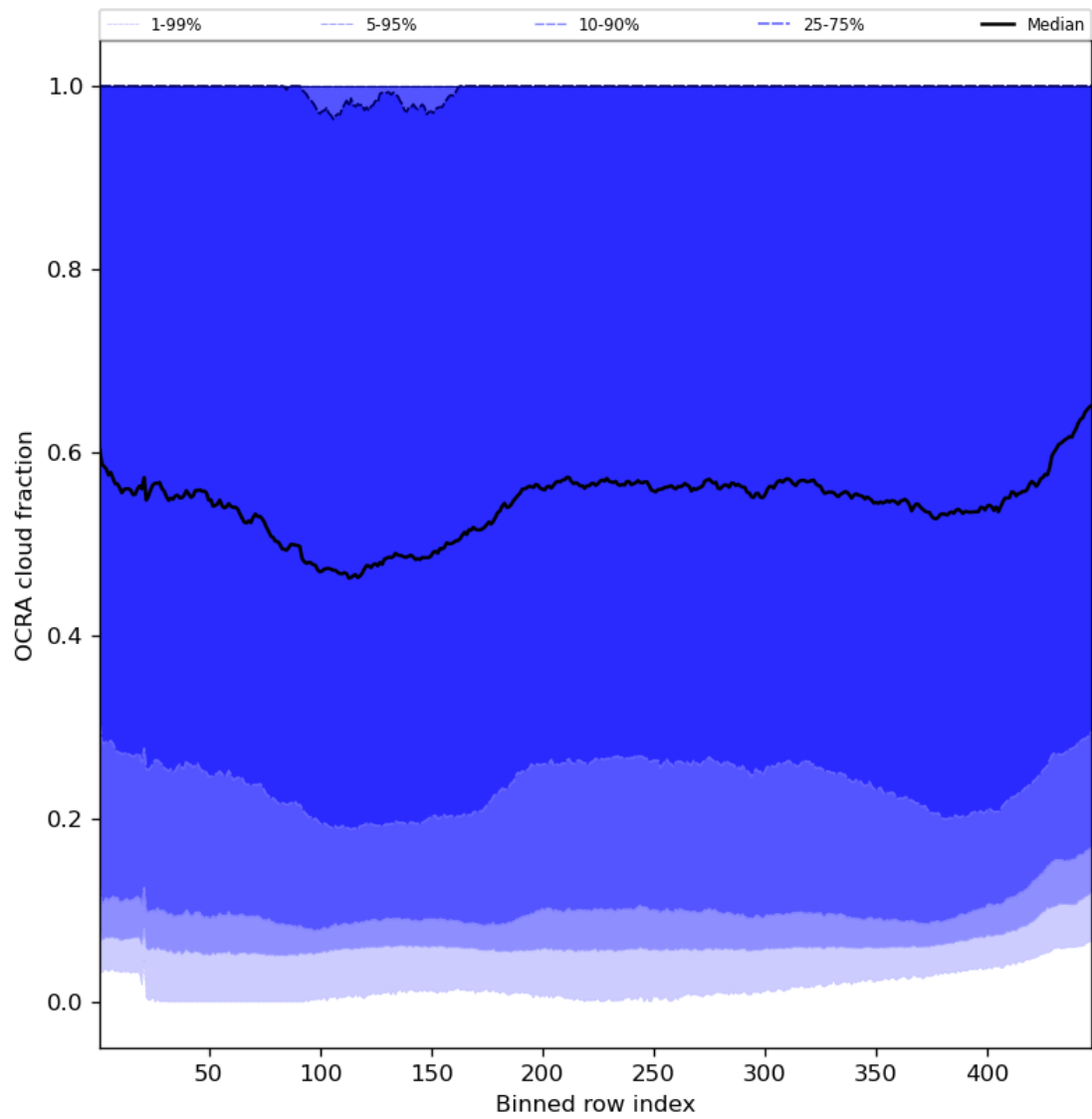
Figure 66: Along track statistics of “OCRA cloud fraction” for 2023-11-16 to 2023-11-18
