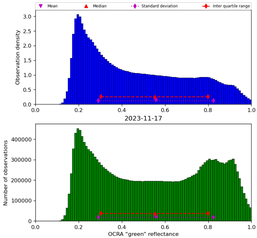
Figure 52: Histogram of “OCRA “green” reflectance” for 2023-11-16 to 2023-11-18
