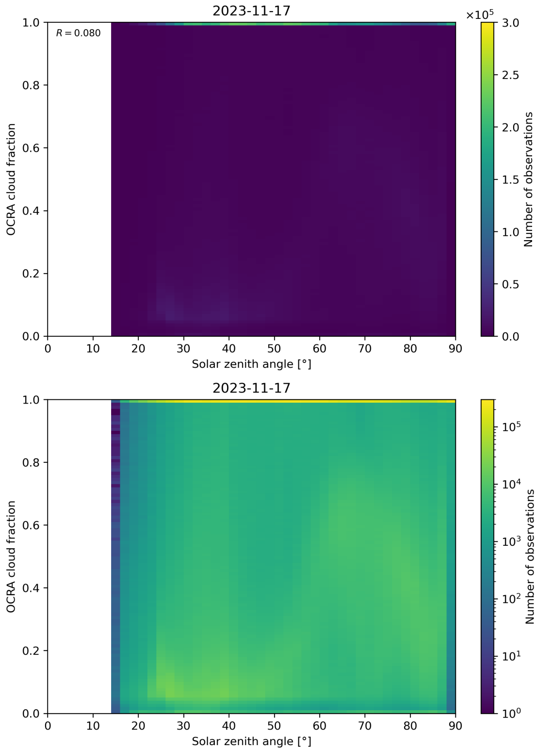
Figure 100: Scatter density plot of “Solar zenith angle” against “OCRA cloud fraction” for 2023-11-16 to 2023-11-18.
