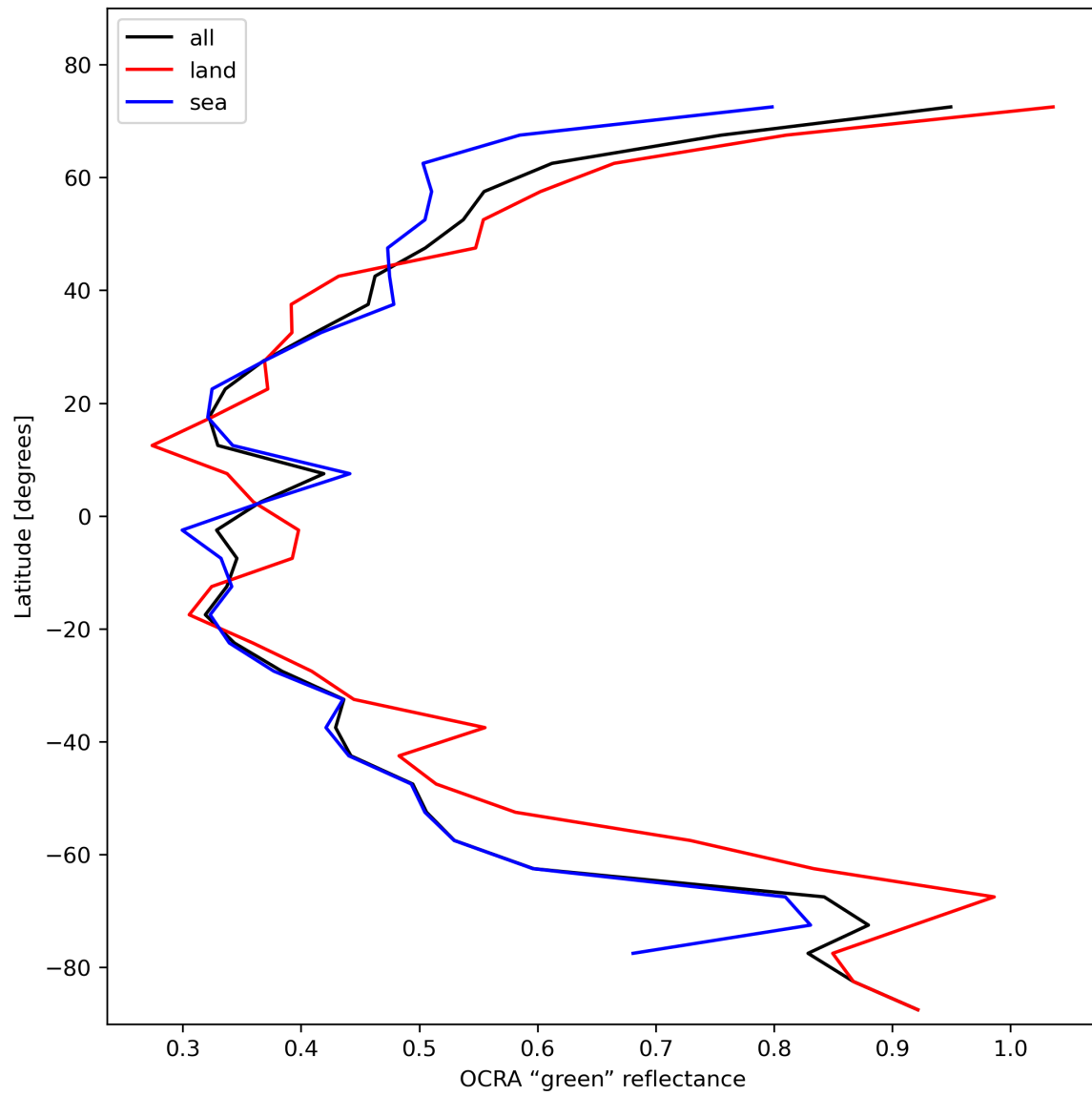
Figure 36: Zonal average of “OCRA “green” reflectance” for 2023-11-16 to 2023-11-18.
