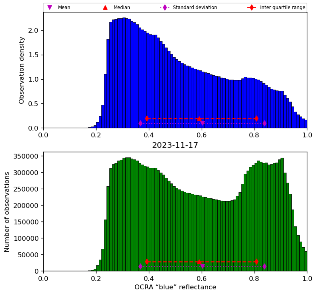
Figure 51: Histogram of “OCRA “blue” reflectance” for 2023-11-16 to 2023-11-18
