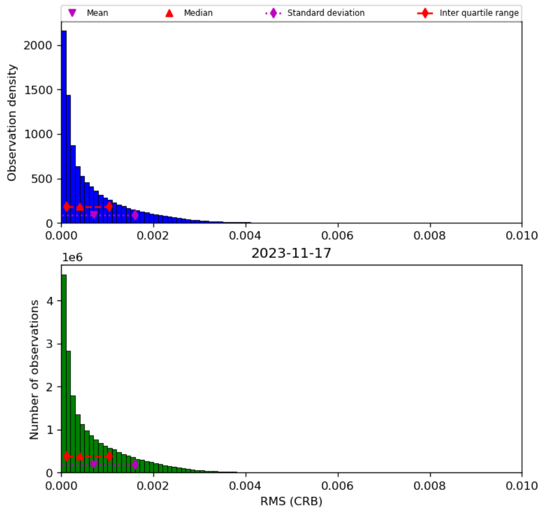
Figure 48: Histogram of “RMS (CRB)” for 2023-11-16 to 2023-11-18
