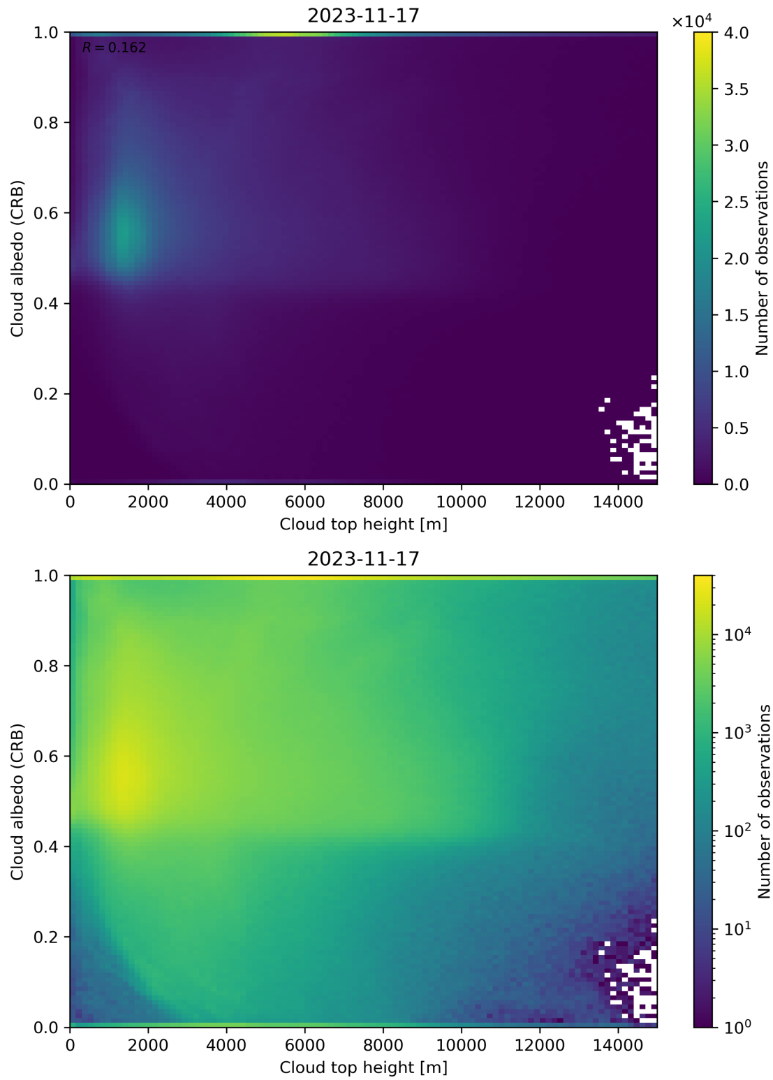
Figure 86: Scatter density plot of “Cloud top height” against “Cloud albedo (CRB)” for 2023-11-16 to 2023-11-18.
