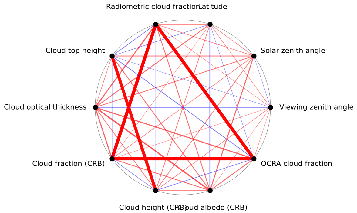
Figure 1: Map of correlation graph for 2023-11-16 to 2023-11-18.
