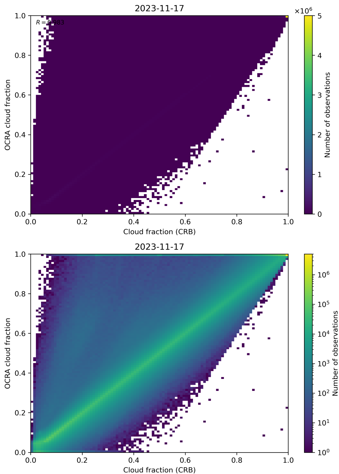
Figure 78: Scatter density plot of “Cloud fraction (CRB)” against “OCRA cloud fraction” for 2023-11-16 to 2023-11-18.
