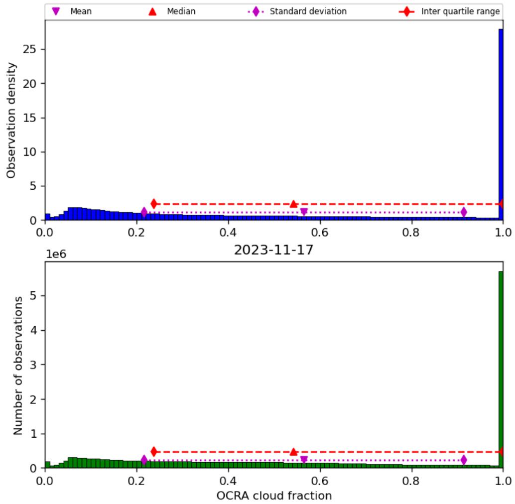
Figure 50: Histogram of “OCRA cloud fraction” for 2023-11-16 to 2023-11-18
