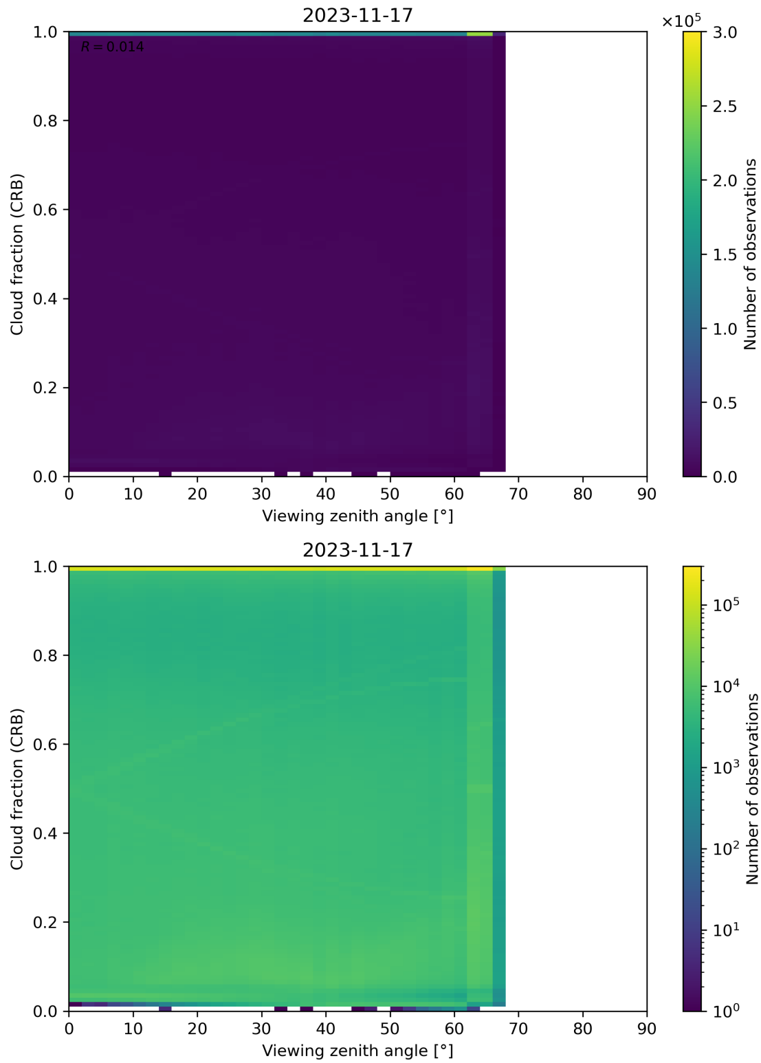
Figure 109: Scatter density plot of “Viewing zenith angle” against “Cloud fraction (CRB)” for 2023-11-16 to 2023-11-18.
