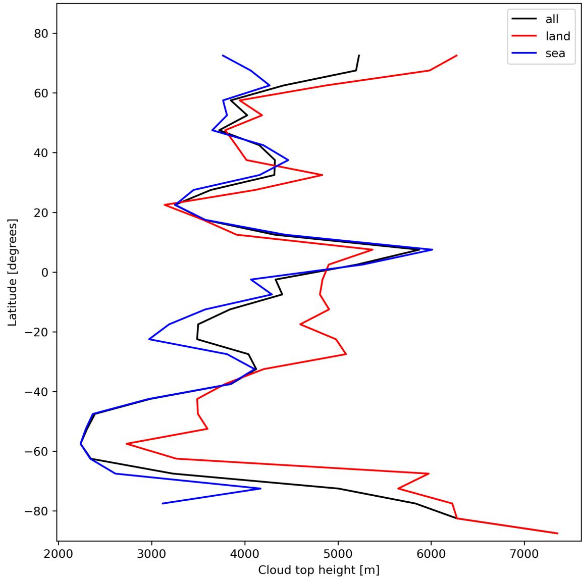
Figure 24: Zonal average of “Cloud top height” for 2023-11-16 to 2023-11-18.
