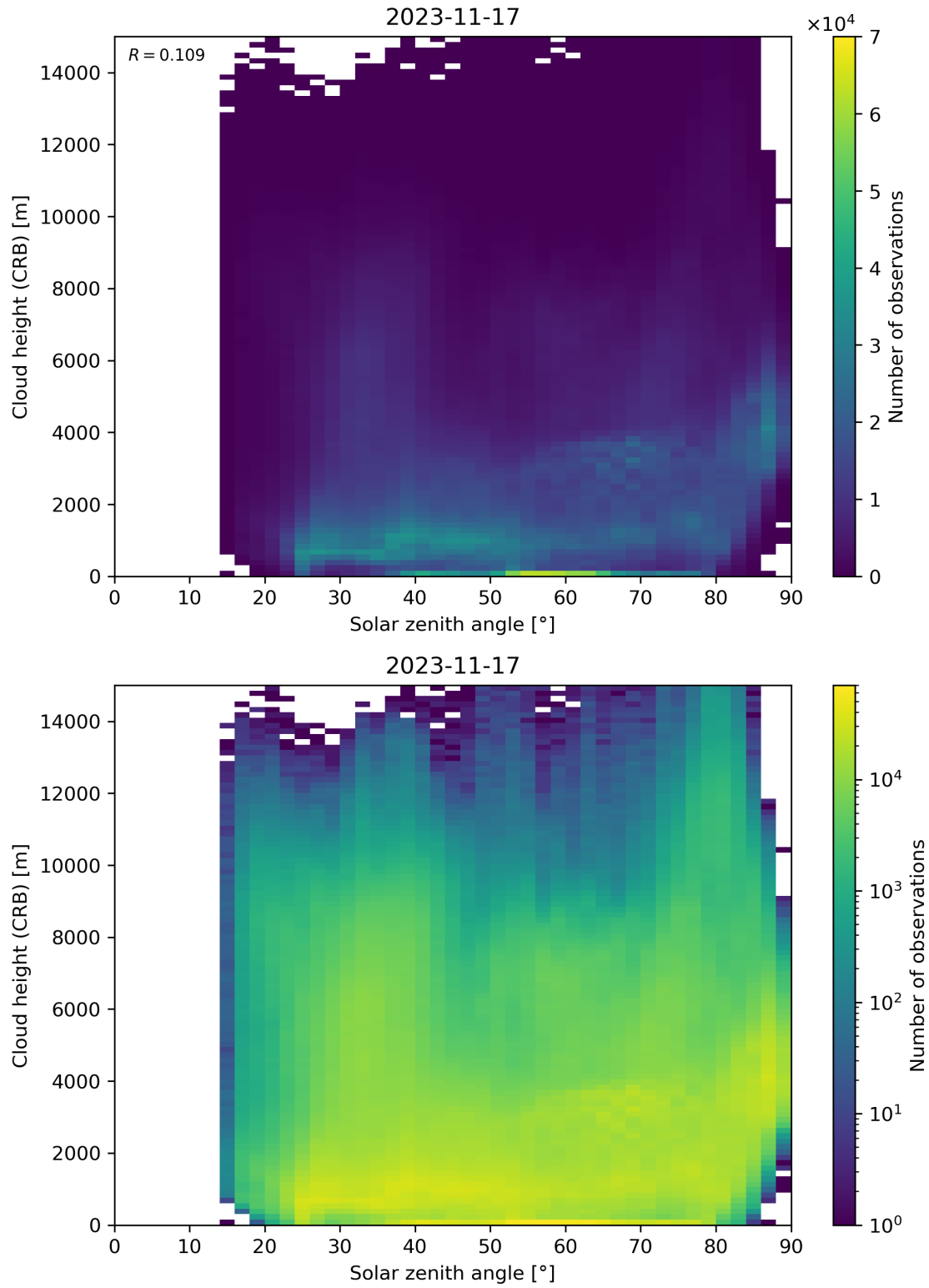
Figure 102: Scatter density plot of “Solar zenith angle” against “Cloud height (CRB)” for 2023-11-16 to 2023-11-18.
