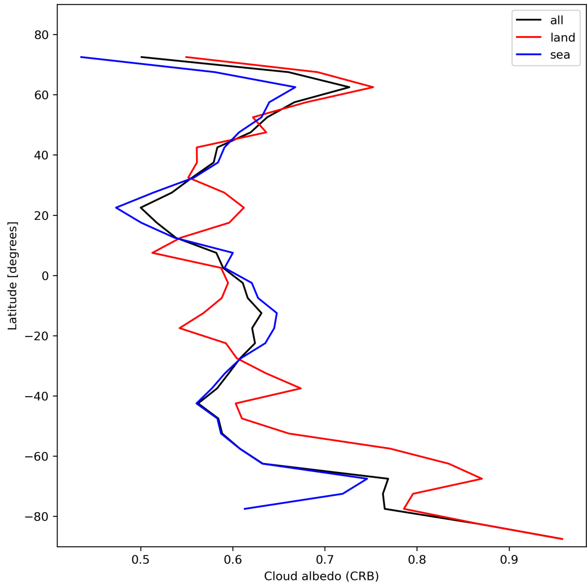
Figure 28: Zonal average of “Cloud albedo (CRB)” for 2023-11-16 to 2023-11-18.
