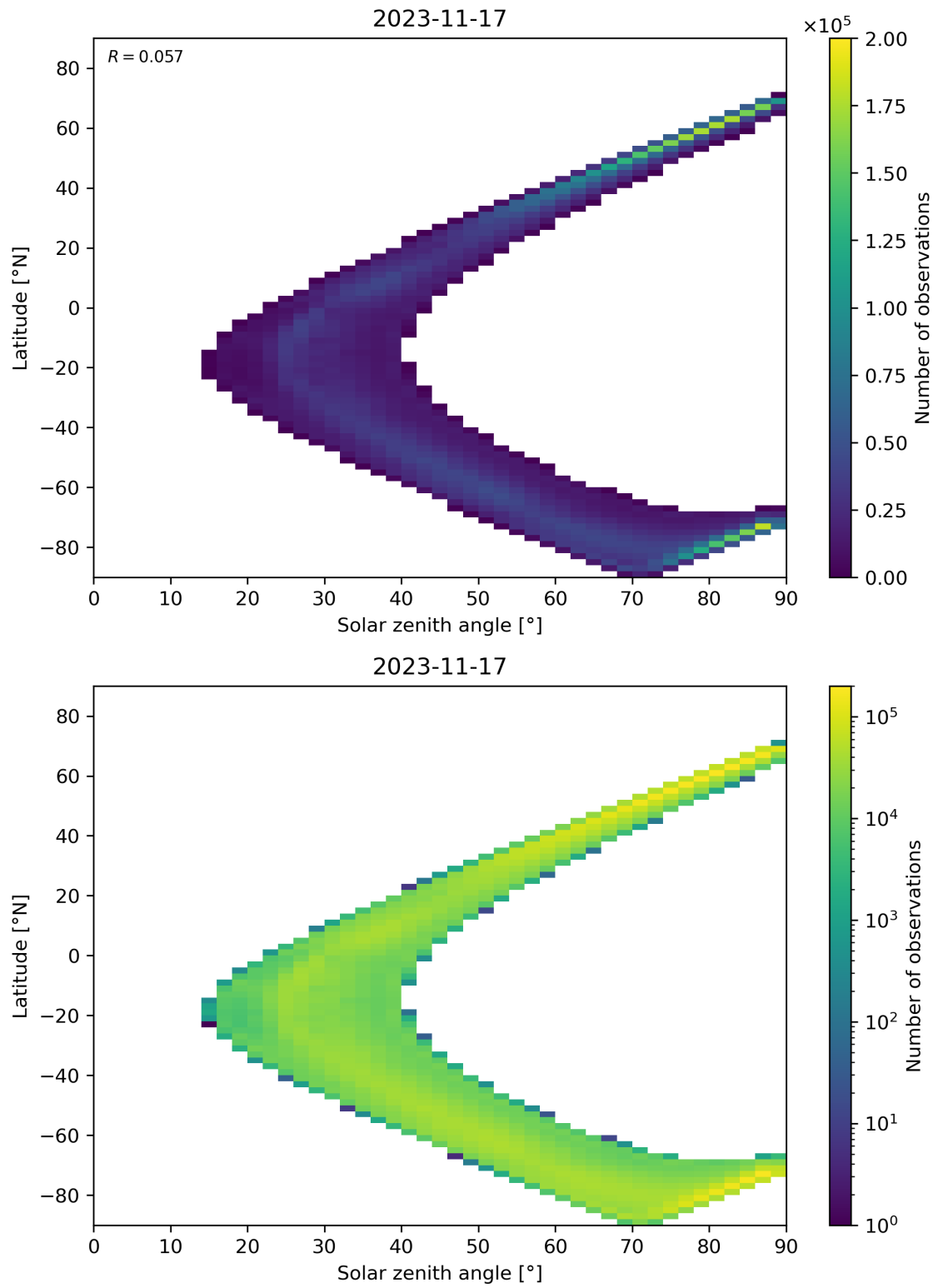
Figure 105: Scatter density plot of “Solar zenith angle” against “Latitude” for 2023-11-16 to 2023-11-18.
