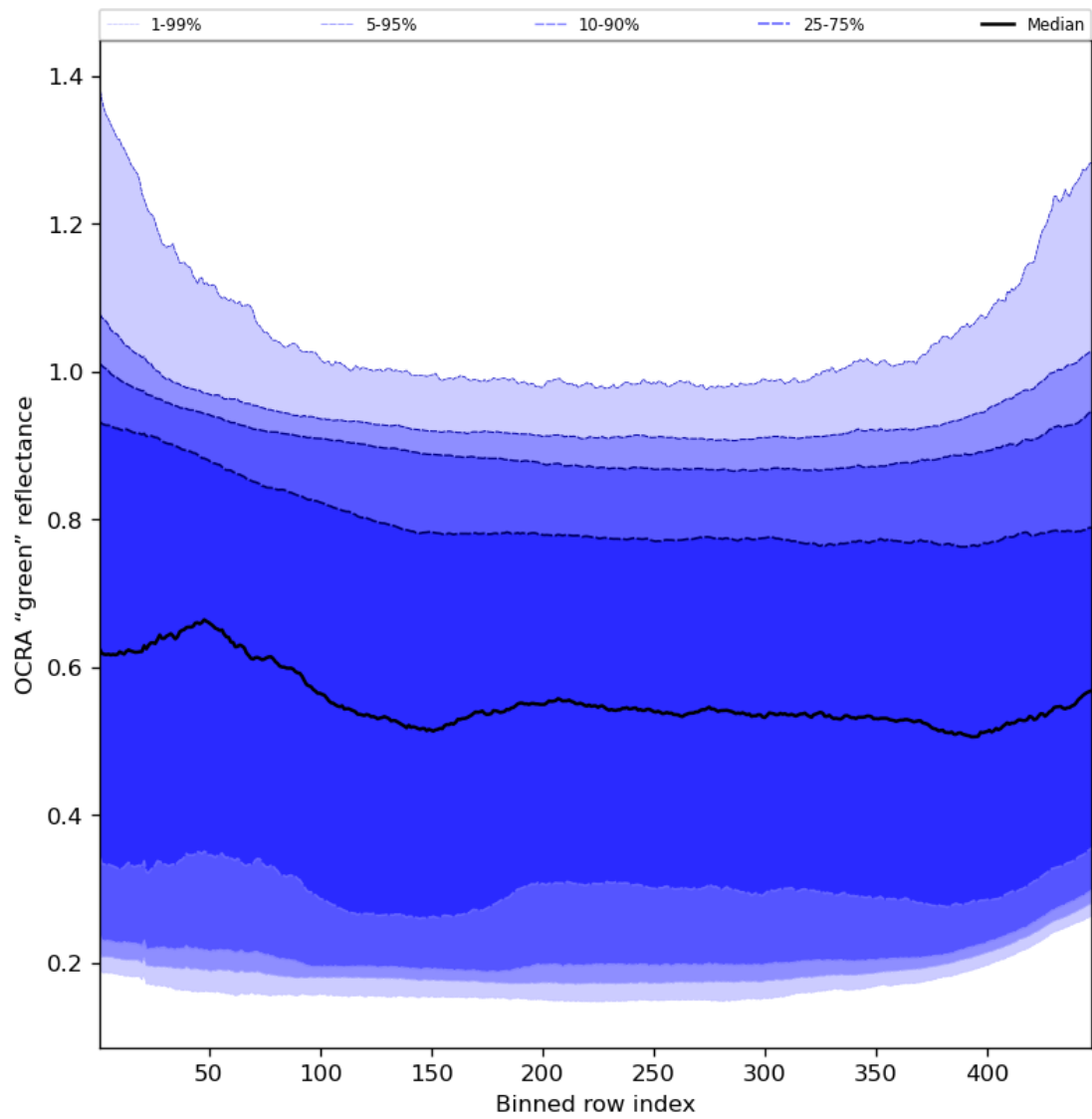
Figure 68: Along track statistics of "OCRA "green" reflectance" for 2023-11-16 to 2023-11-18
