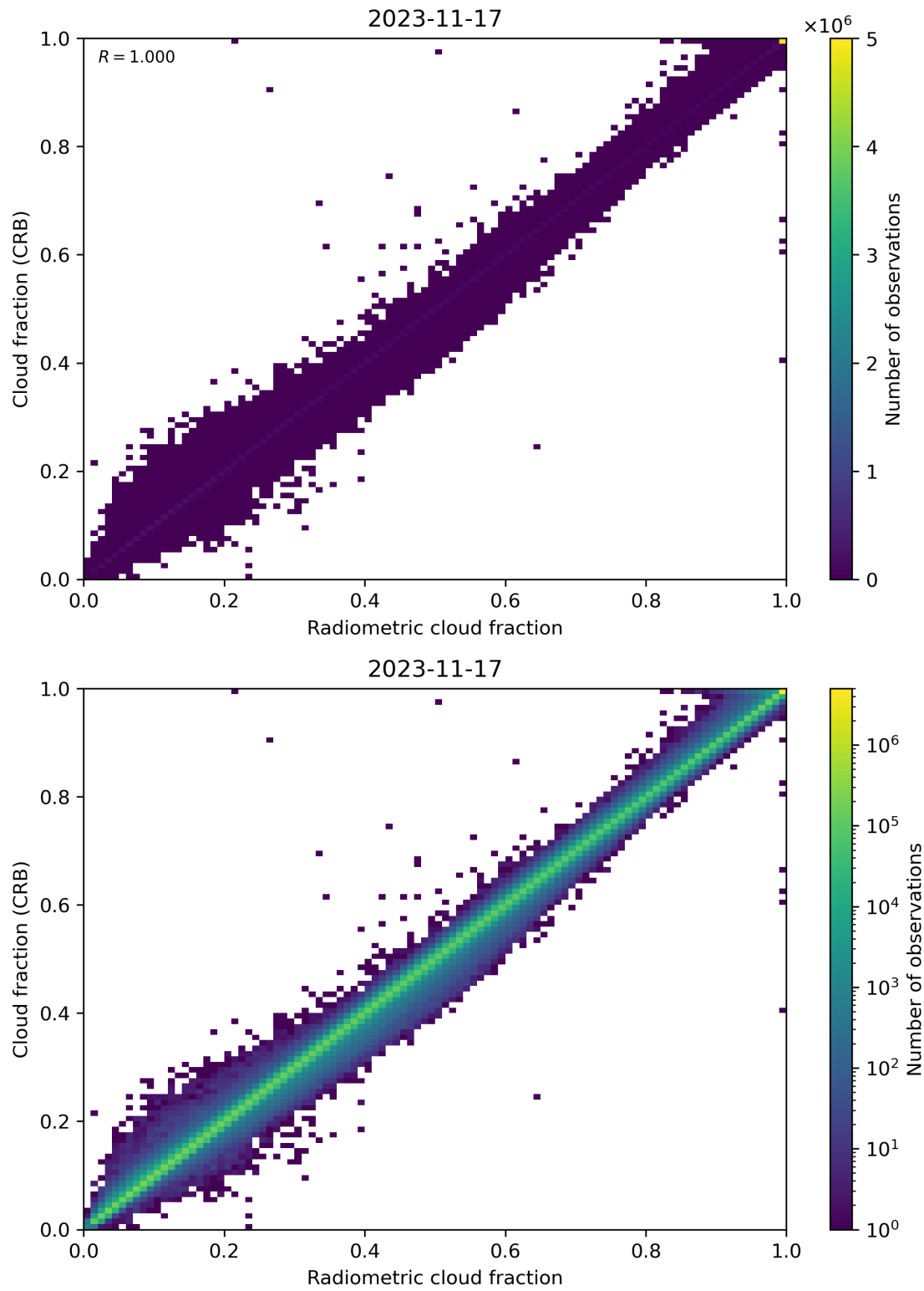
Figure 73: Scatter density plot of “Radiometric cloud fraction” against “Cloud fraction (CRB)” for 2023-11-16 to 2023-11-18.
