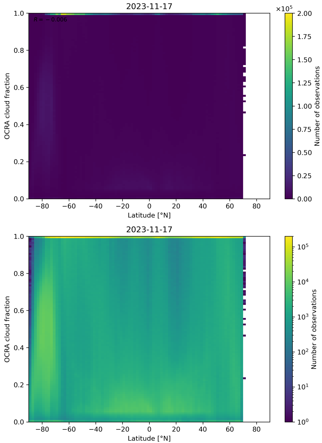
Figure 93: Scatter density plot of “Latitude” against “OCRA cloud fraction” for 2023-11-16 to 2023-11-18.
