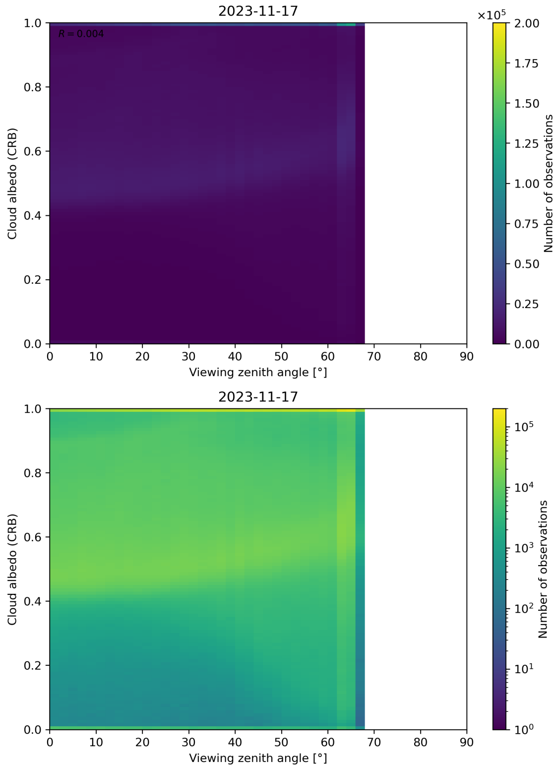
Figure 106: Scatter density plot of “Viewing zenith angle” against “Cloud albedo (CRB)” for 2023-11-16 to 2023-11-18.
