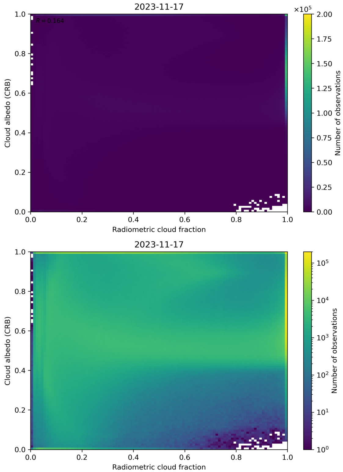
Figure 71: Scatter density plot of “Radiometric cloud fraction” against “Cloud albedo (CRB)” for 2023-11-16 to 2023-11-18.
