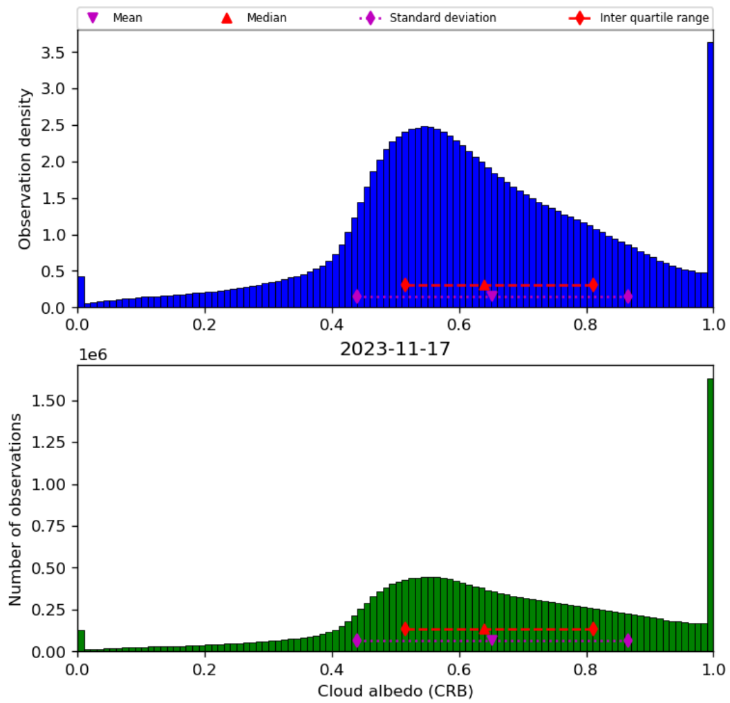
Figure 44: Histogram of “Cloud albedo (CRB)” for 2023-11-16 to 2023-11-18
