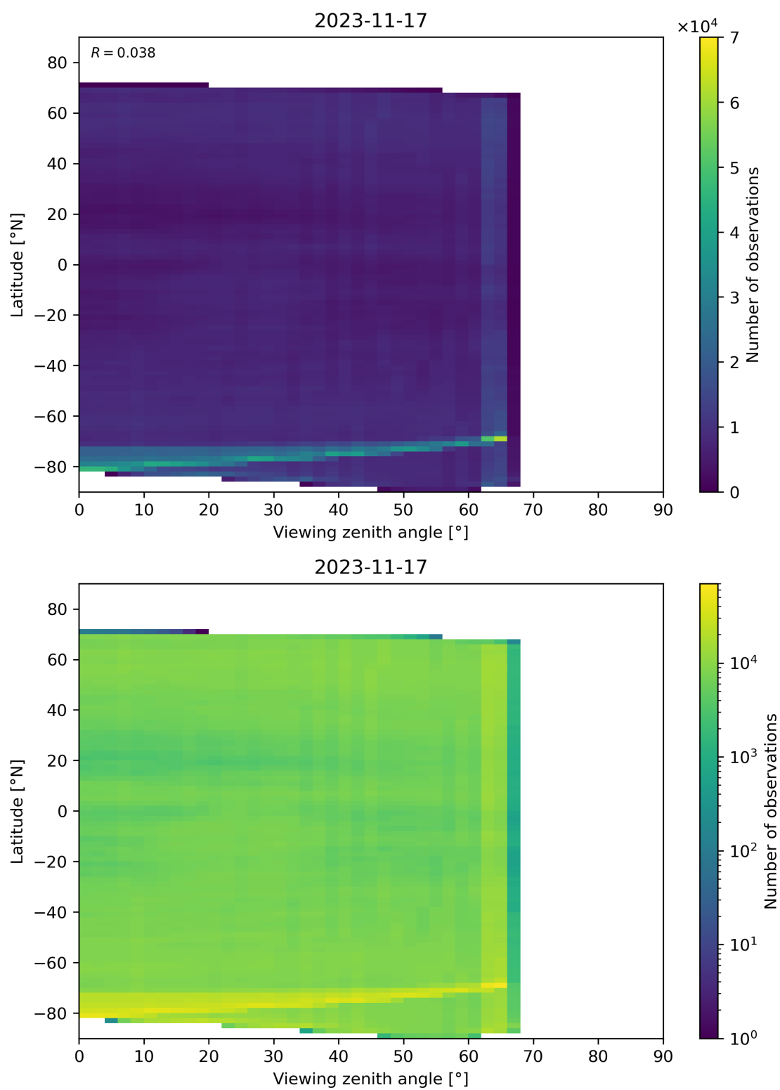
Figure 113: Scatter density plot of “Viewing zenith angle” against “Latitude” for 2023-11-16 to 2023-11-18.
