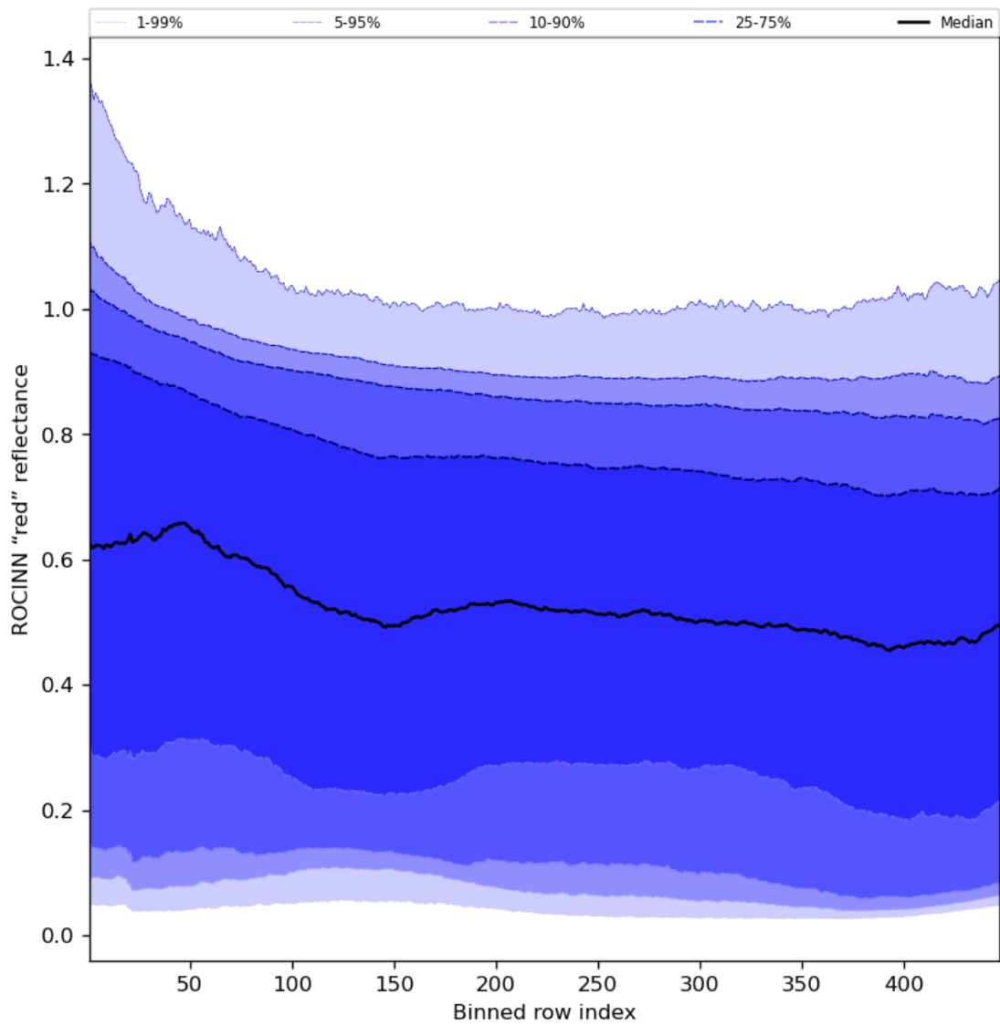
Figure 69: Along track statistics of "ROCINN "red" reflectance" for 2023-11-16 to 2023-11-18
