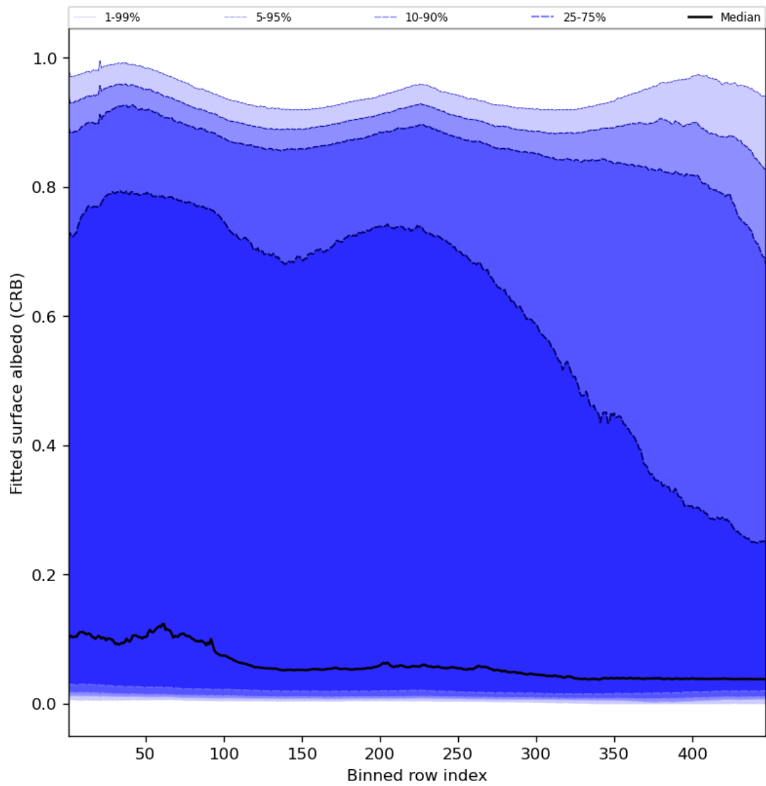
Figure 62: Along track statistics of “Fitted surface albedo (CRB)” for 2023-11-19 to 2023-11-21
