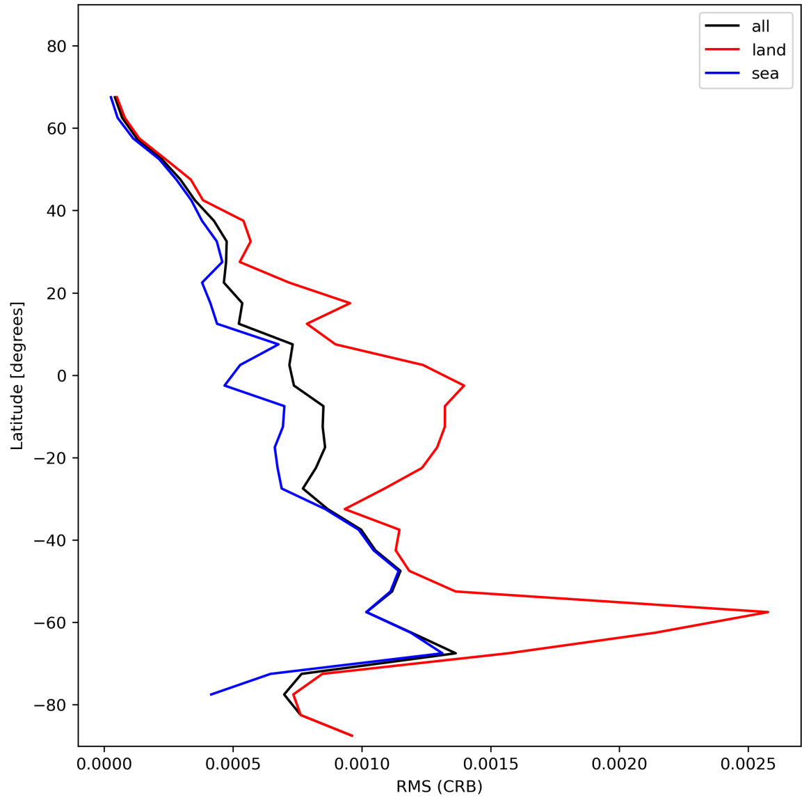
Figure 32: Zonal average of “RMS (CRB)” for 2023-11-19 to 2023-11-21.
