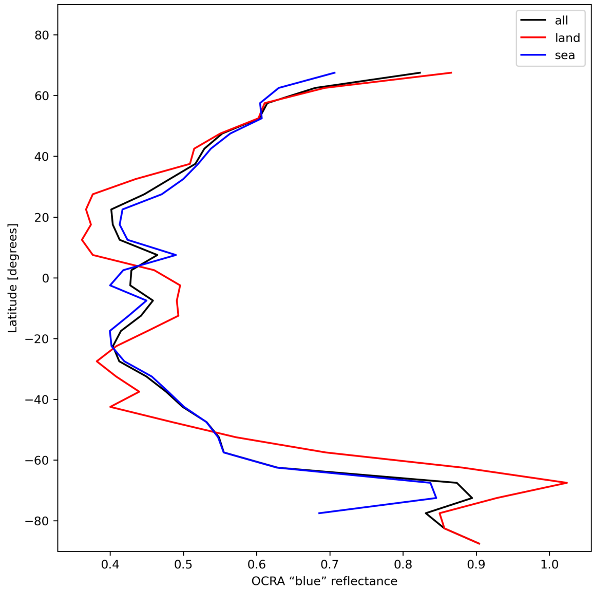
Figure 35: Zonal average of “OCRA “blue” reflectance” for 2023-11-19 to 2023-11-21.
