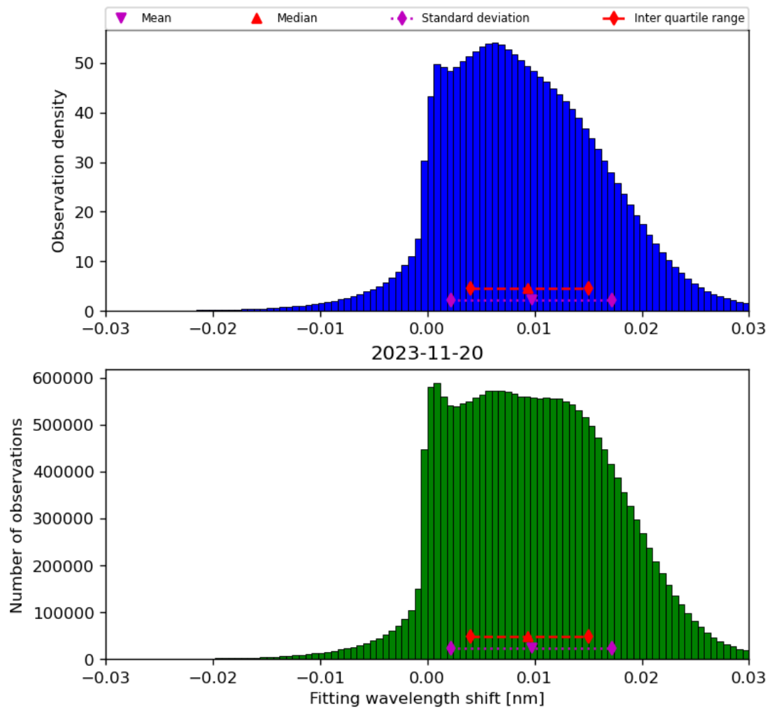
Figure 49: Histogram of “Fitting wavelength shift” for 2023-11-19 to 2023-11-21
