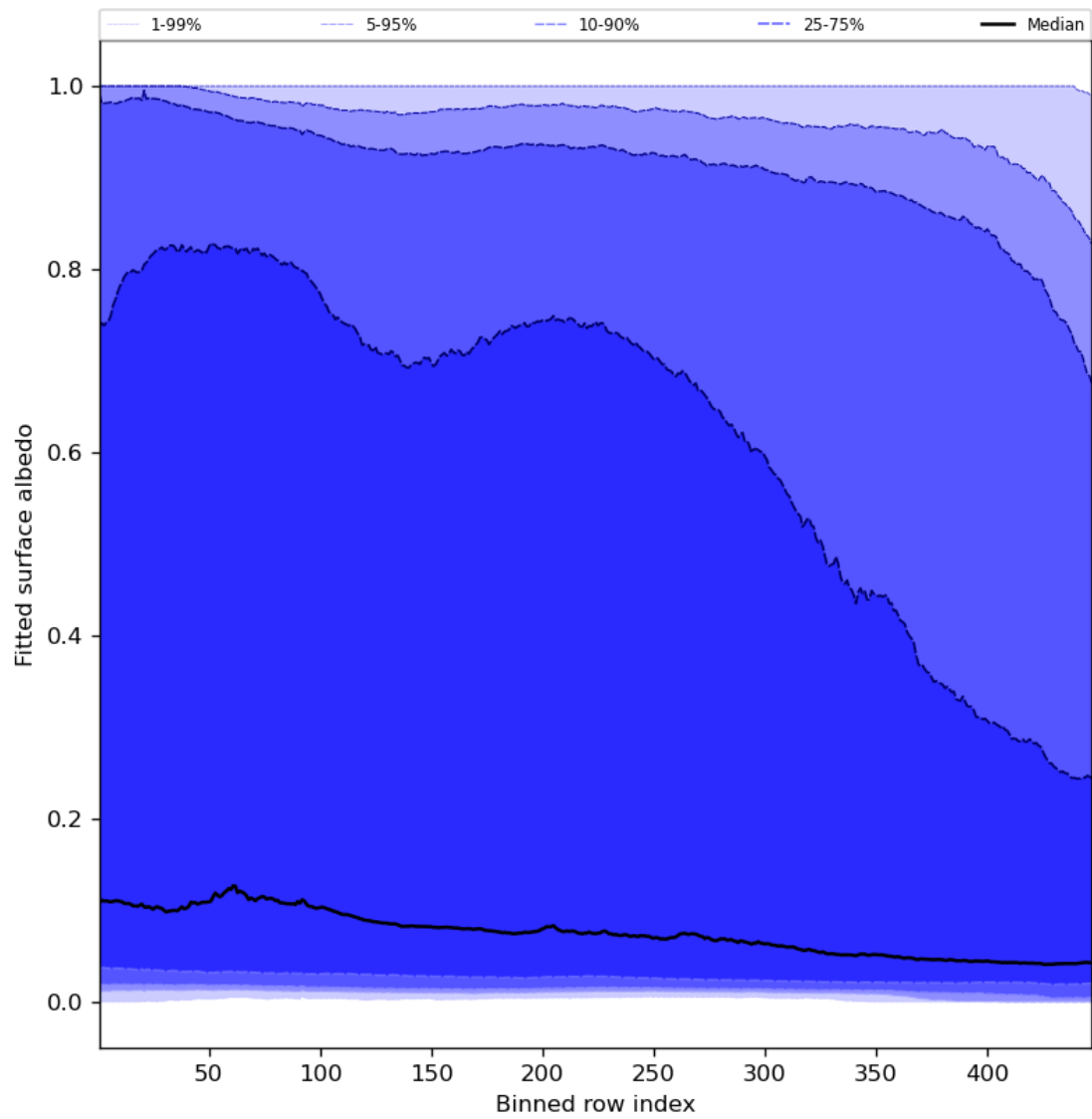
Figure 61: Along track statistics of “Fitted surface albedo” for 2023-11-19 to 2023-11-21
