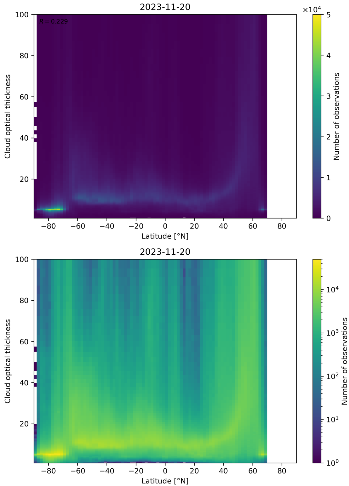
Figure 96: Scatter density plot of “Latitude” against “Cloud optical thickness” for 2023-11-19 to 2023-11-21.
