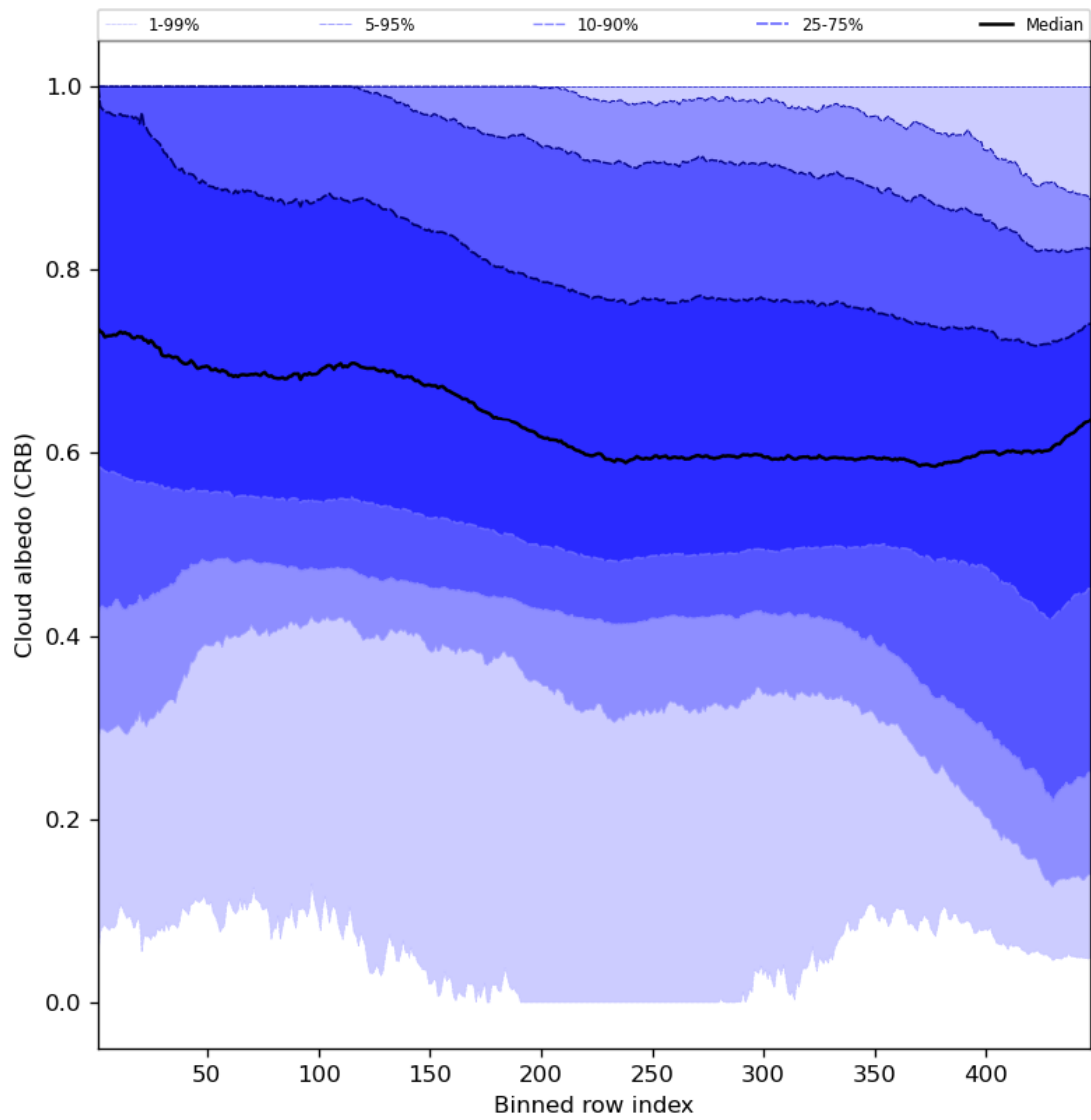
Figure 60: Along track statistics of “Cloud albedo (CRB)” for 2023-11-19 to 2023-11-21
