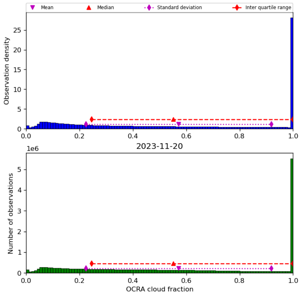
Figure 50: Histogram of “OCRA cloud fraction” for 2023-11-19 to 2023-11-21
