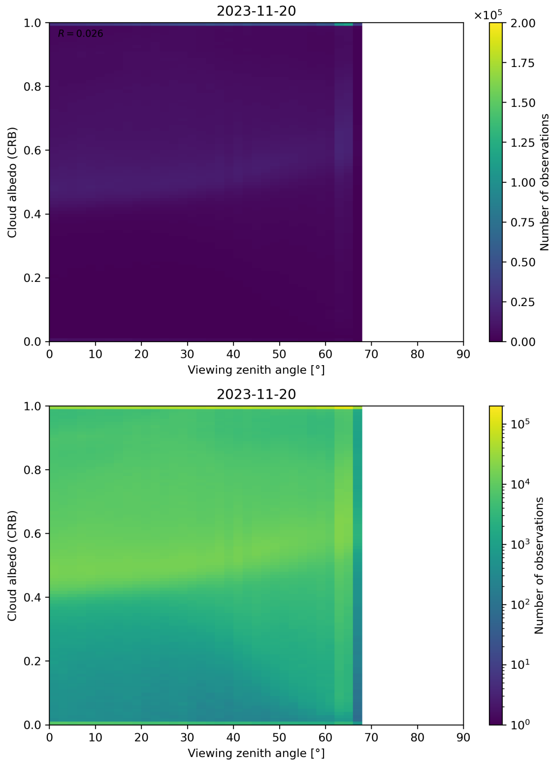
Figure 106: Scatter density plot of “Viewing zenith angle” against “Cloud albedo (CRB)” for 2023-11-19 to 2023-11-21.
