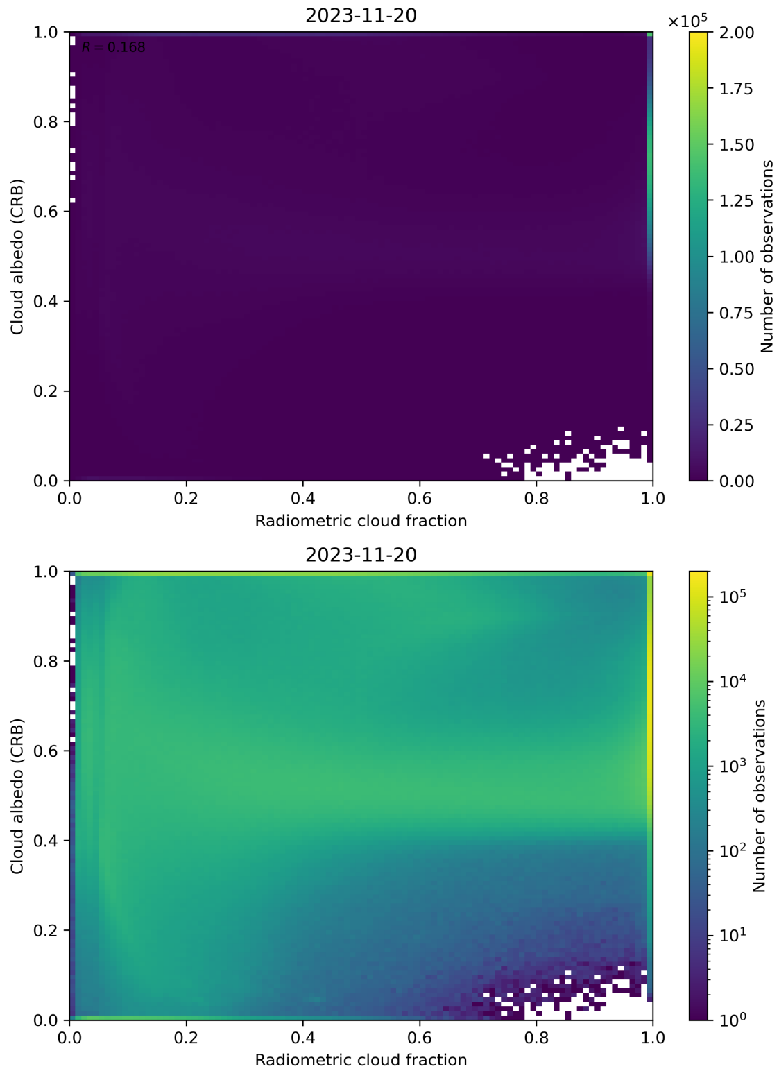
Figure 71: Scatter density plot of “Radiometric cloud fraction” against “Cloud albedo (CRB)” for 2023-11-19 to 2023-11-21.
