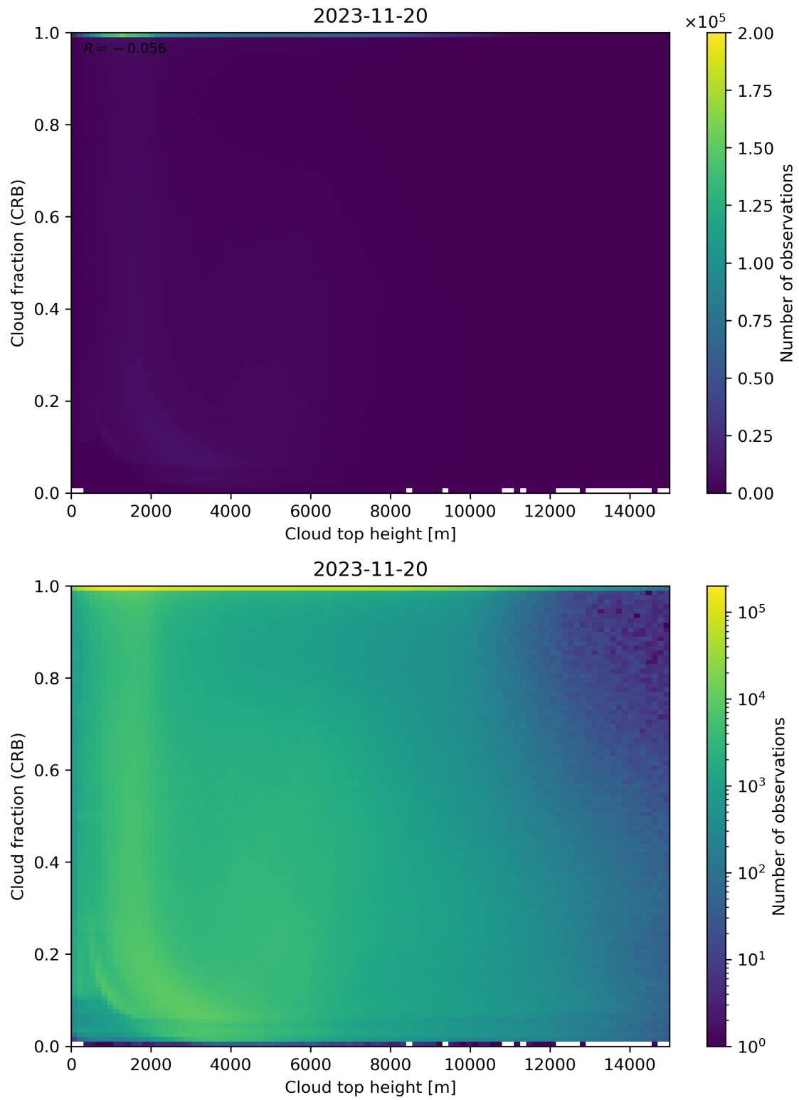
Figure 88: Scatter density plot of “Cloud top height” against “Cloud fraction (CRB)” for 2023-11-19 to 2023-11-21.
