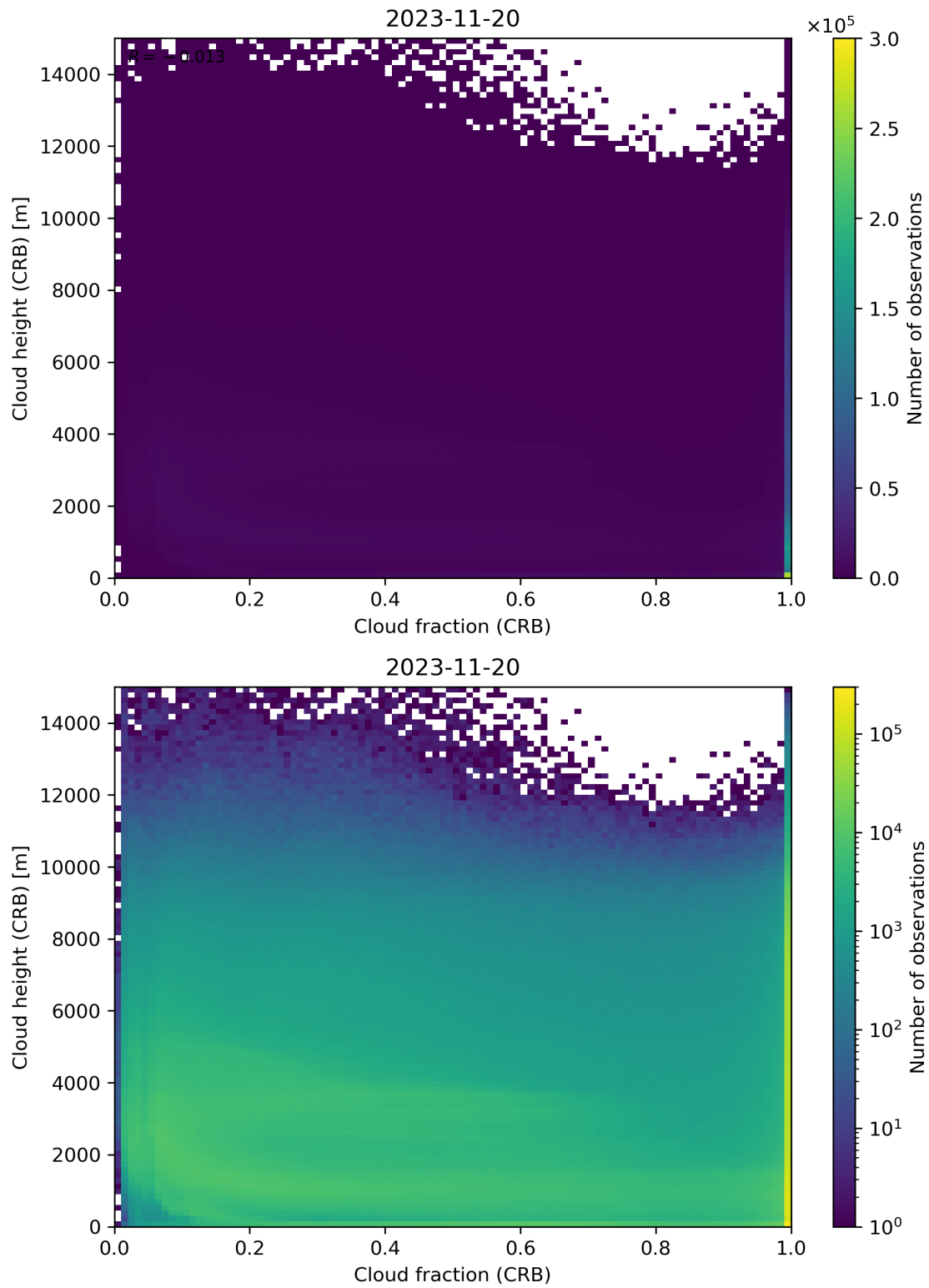
Figure 79: Scatter density plot of “Cloud fraction (CRB)” against “Cloud height (CRB)” for 2023-11-19 to 2023-11-21.
