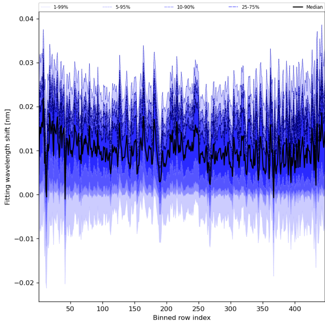
Figure 65: Along track statistics of “Fitting wavelength shift” for 2023-11-19 to 2023-11-21
