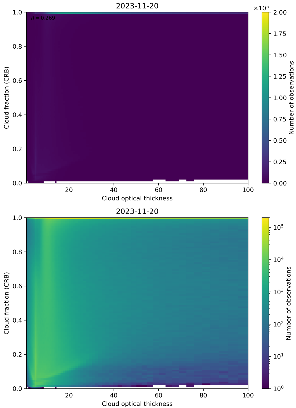
Figure 84: Scatter density plot of “Cloud optical thickness” against “Cloud fraction (CRB)” for 2023-11-19 to 2023-11-21.
