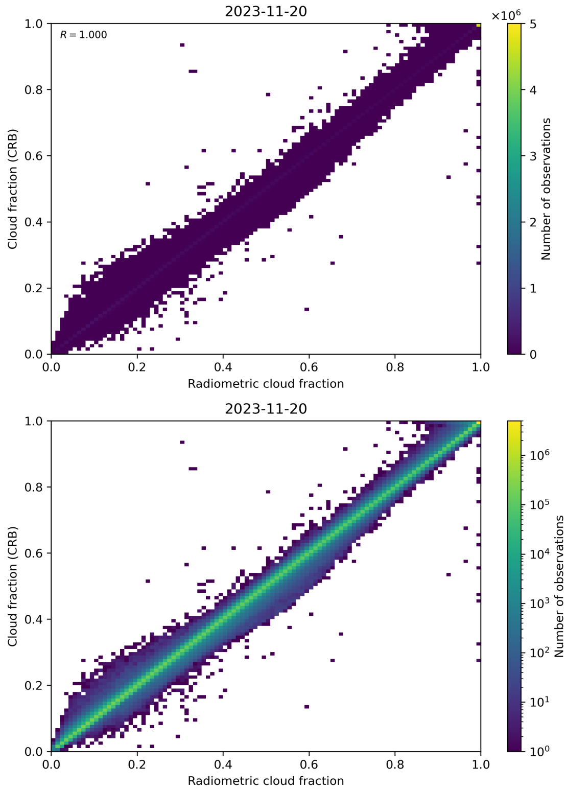
Figure 73: Scatter density plot of “Radiometric cloud fraction” against “Cloud fraction (CRB)” for 2023-11-19 to 2023-11-21.
