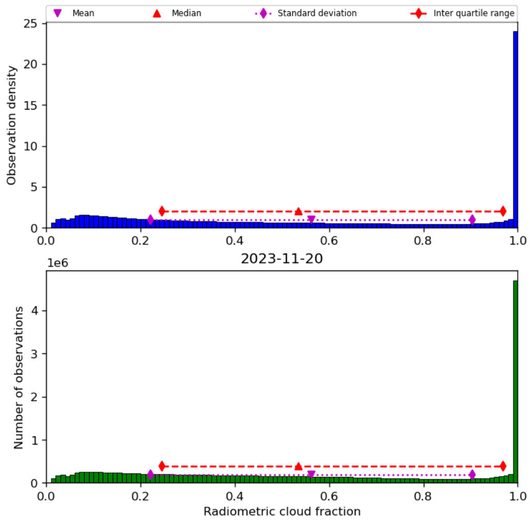
Figure 39: Histogram of “Radiometric cloud fraction” for 2023-11-19 to 2023-11-21
