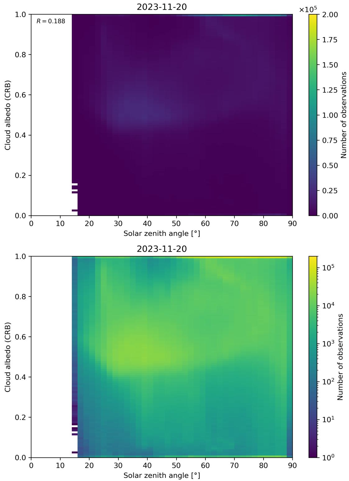
Figure 98: Scatter density plot of “Solar zenith angle” against “Cloud albedo (CRB)” for 2023-11-19 to 2023-11-21.
