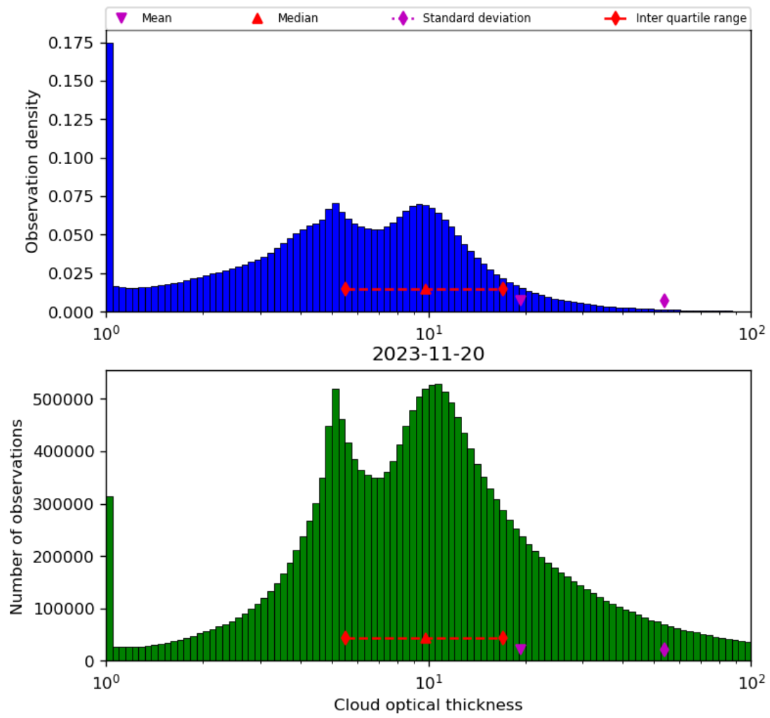
Figure 41: Histogram of “Cloud optical thickness” for 2023-11-19 to 2023-11-21
