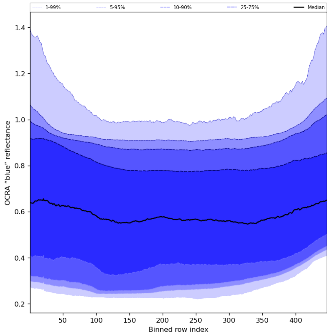
Figure 67: Along track statistics of “OCRA “blue” reflectance” for 2023-11-19 to 2023-11-21
