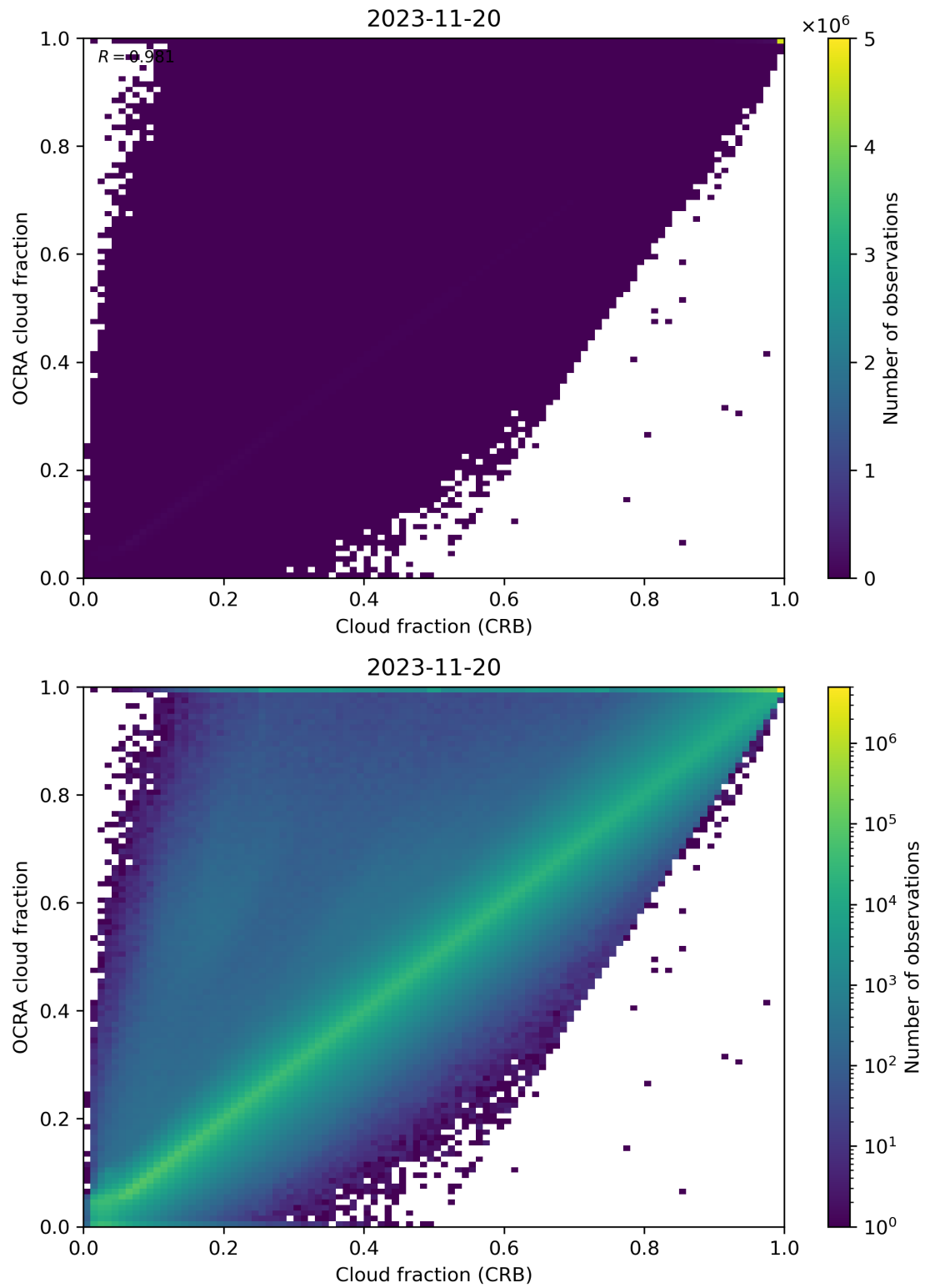
Figure 78: Scatter density plot of “Cloud fraction (CRB)” against “OCRA cloud fraction” for 2023-11-19 to 2023-11-21.
