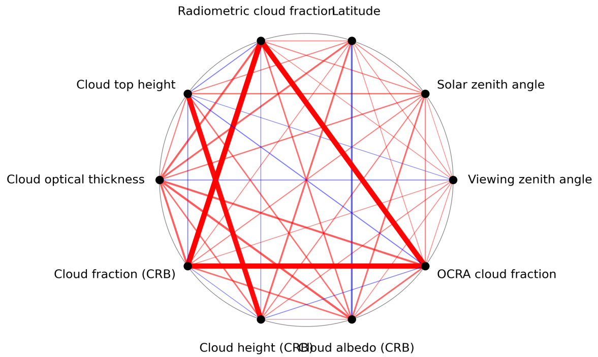
Figure 1: Map of correlation graph for 2023-11-19 to 2023-11-21.
