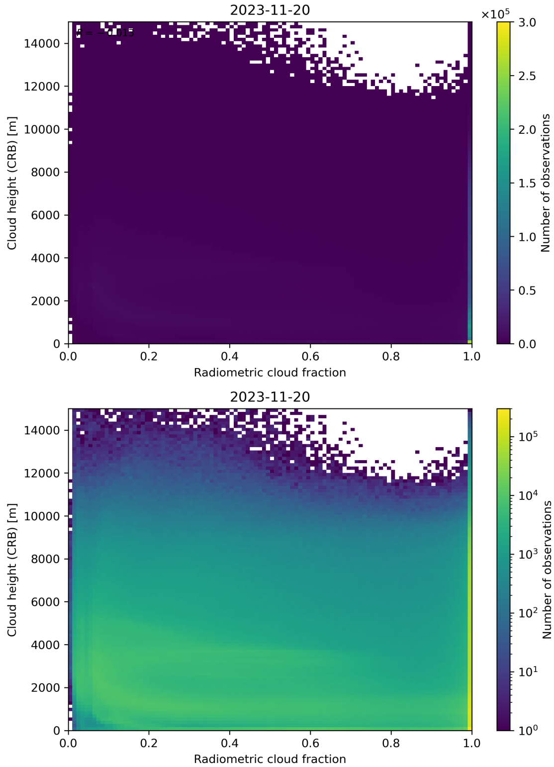
Figure 74: Scatter density plot of “Radiometric cloud fraction” against “Cloud height (CRB)” for 2023-11-19 to 2023-11-21.
