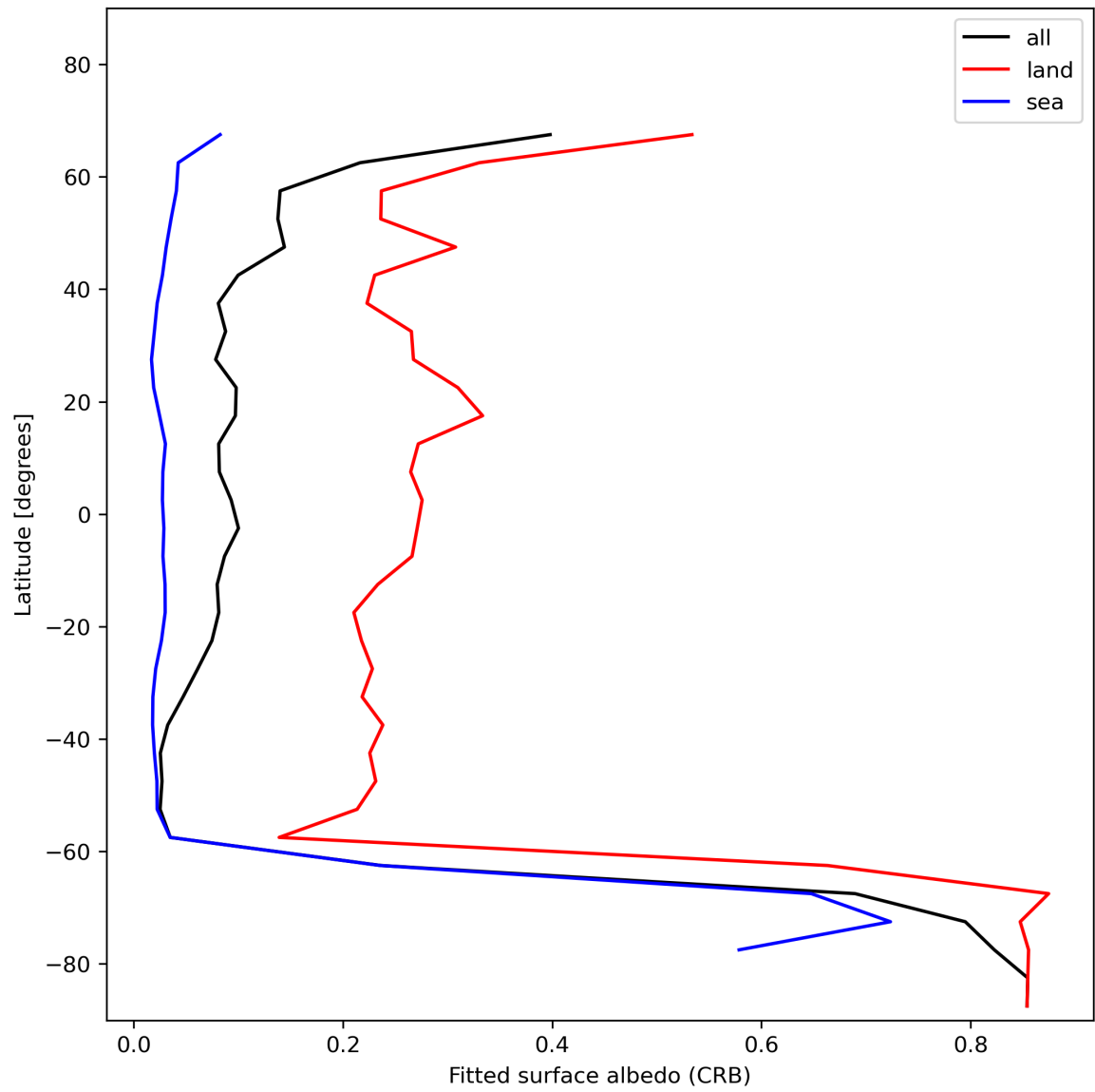
Figure 30: Zonal average of “Fitted surface albedo (CRB)” for 2023-11-19 to 2023-11-21.
