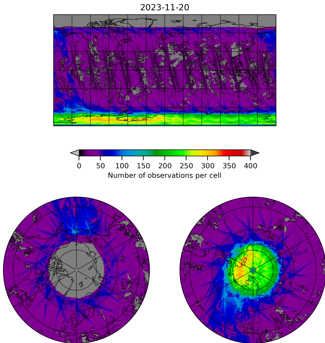
Figure 21: Map of the number of observations for 2023-11-19 to 2023-11-21
