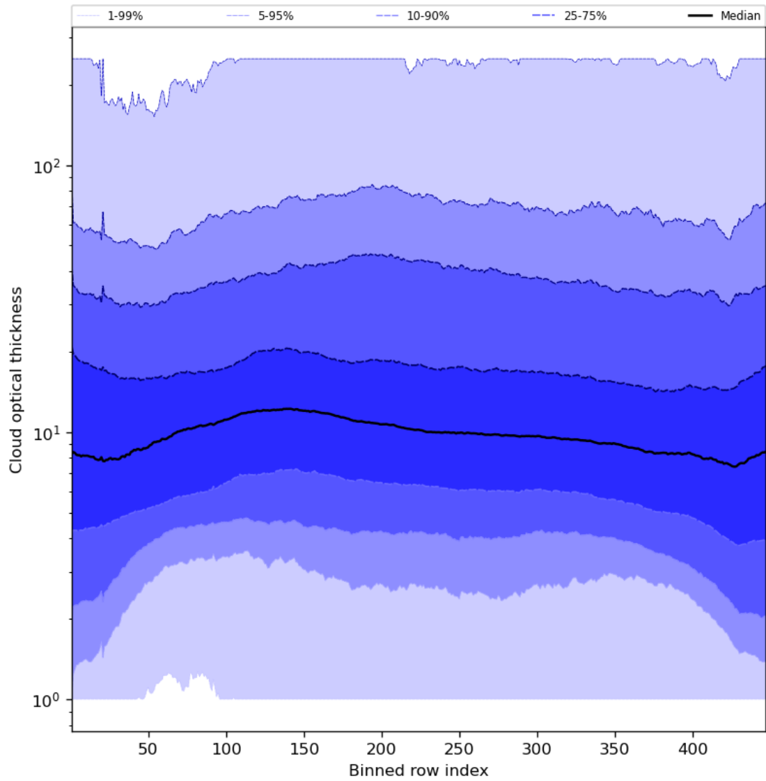
Figure 57: Along track statistics of “Cloud optical thickness” for 2023-11-19 to 2023-11-21
