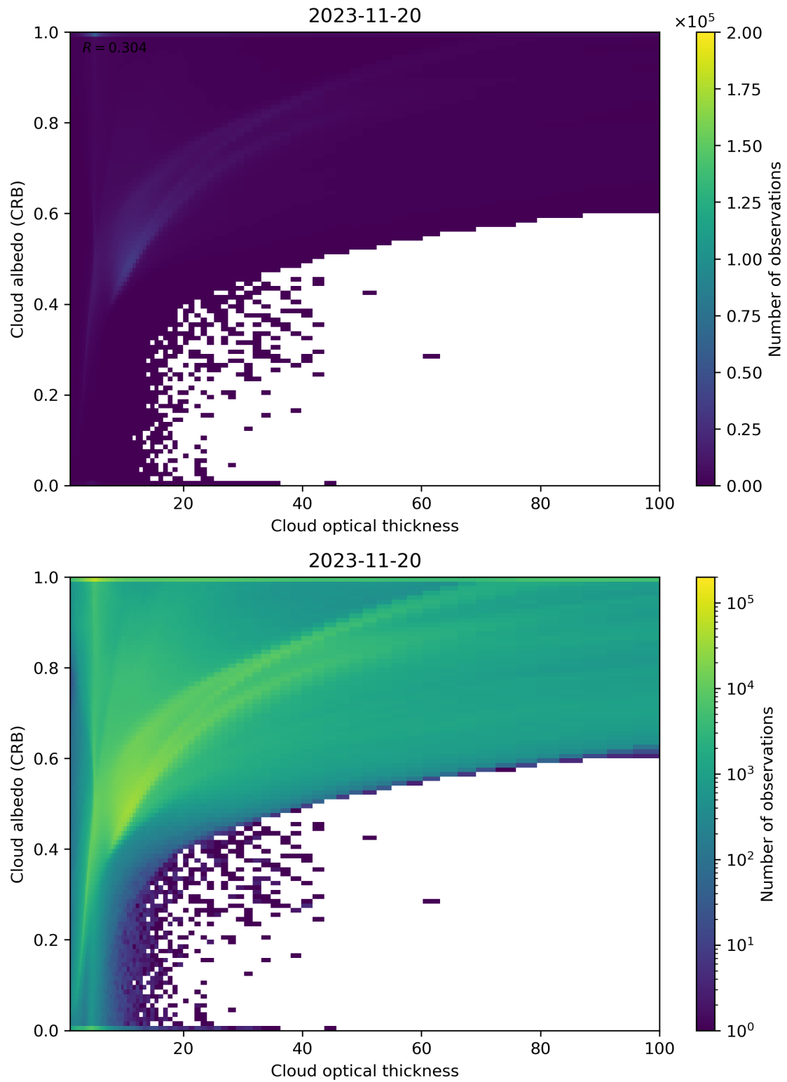
Figure 82: Scatter density plot of “Cloud optical thickness” against “Cloud albedo (CRB)” for 2023-11-19 to 2023-11-21.
