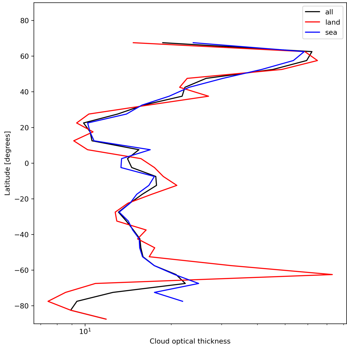
Figure 25: Zonal average of “Cloud optical thickness” for 2023-11-19 to 2023-11-21.
