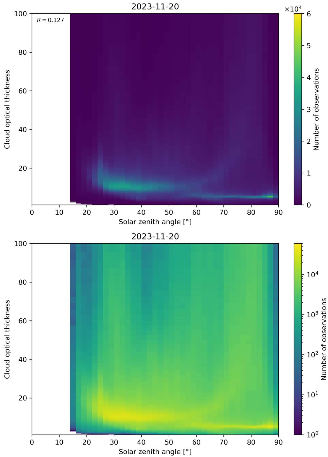
Figure 103: Scatter density plot of “Solar zenith angle” against “Cloud optical thickness” for 2023-11-19 to 2023-11-21.
