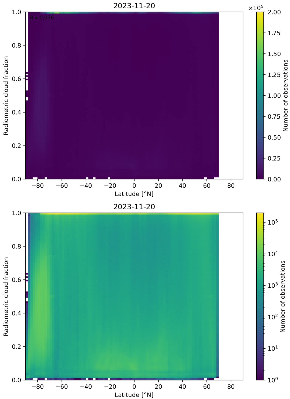
Figure 92: Scatter density plot of “Latitude” against “Radiometric cloud fraction” for 2023-11-19 to 2023-11-21.
