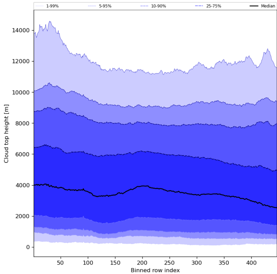
Figure 56: Along track statistics of “Cloud top height” for 2023-11-19 to 2023-11-21
