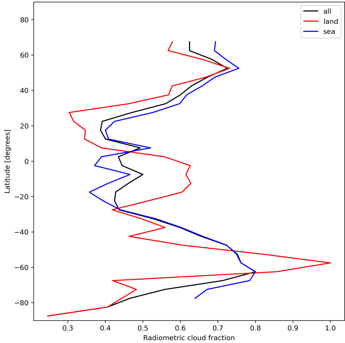
Figure 23: Zonal average of “Radiometric cloud fraction” for 2023-11-19 to 2023-11-21.
