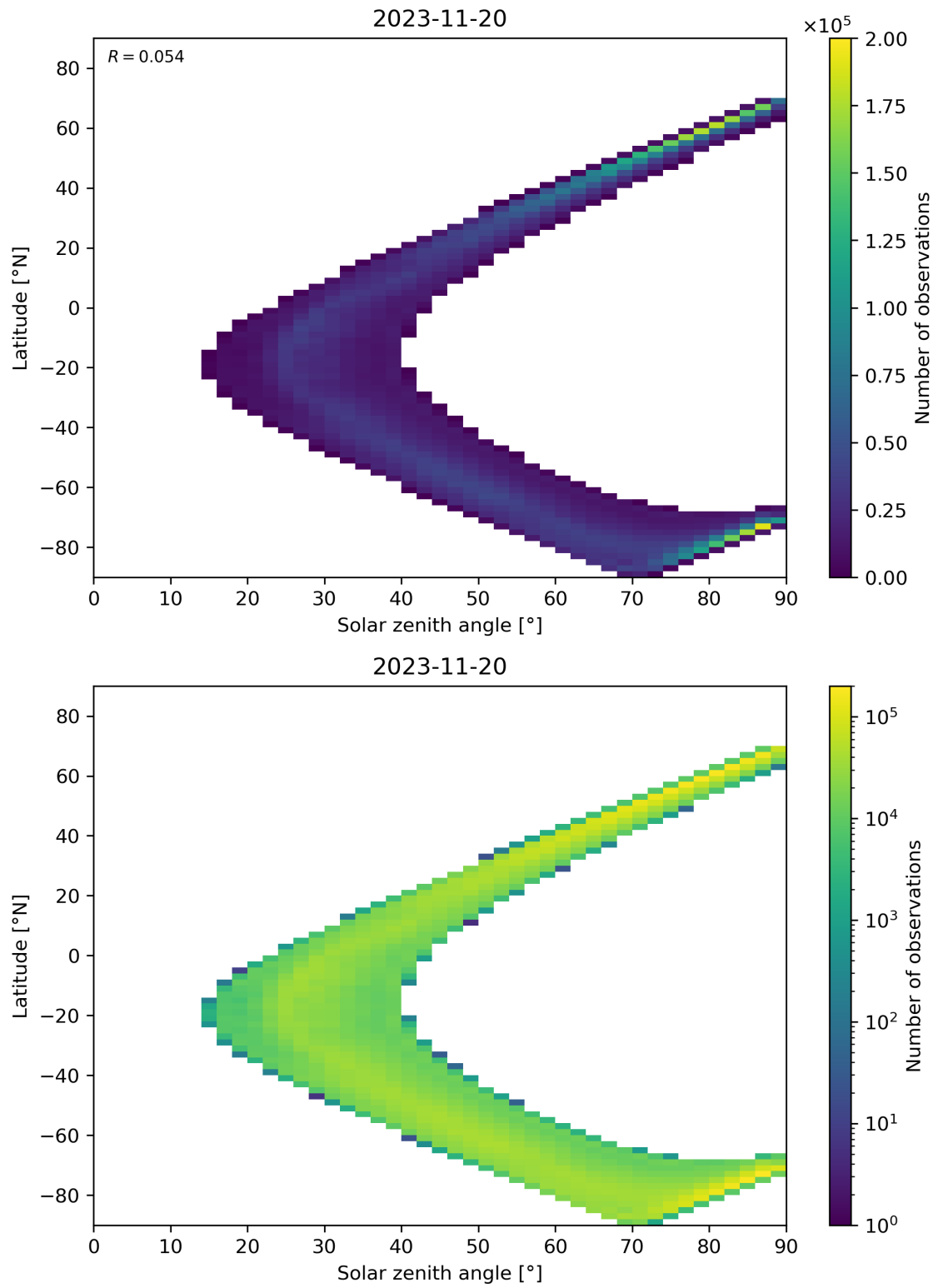
Figure 105: Scatter density plot of “Solar zenith angle” against “Latitude” for 2023-11-19 to 2023-11-21.
