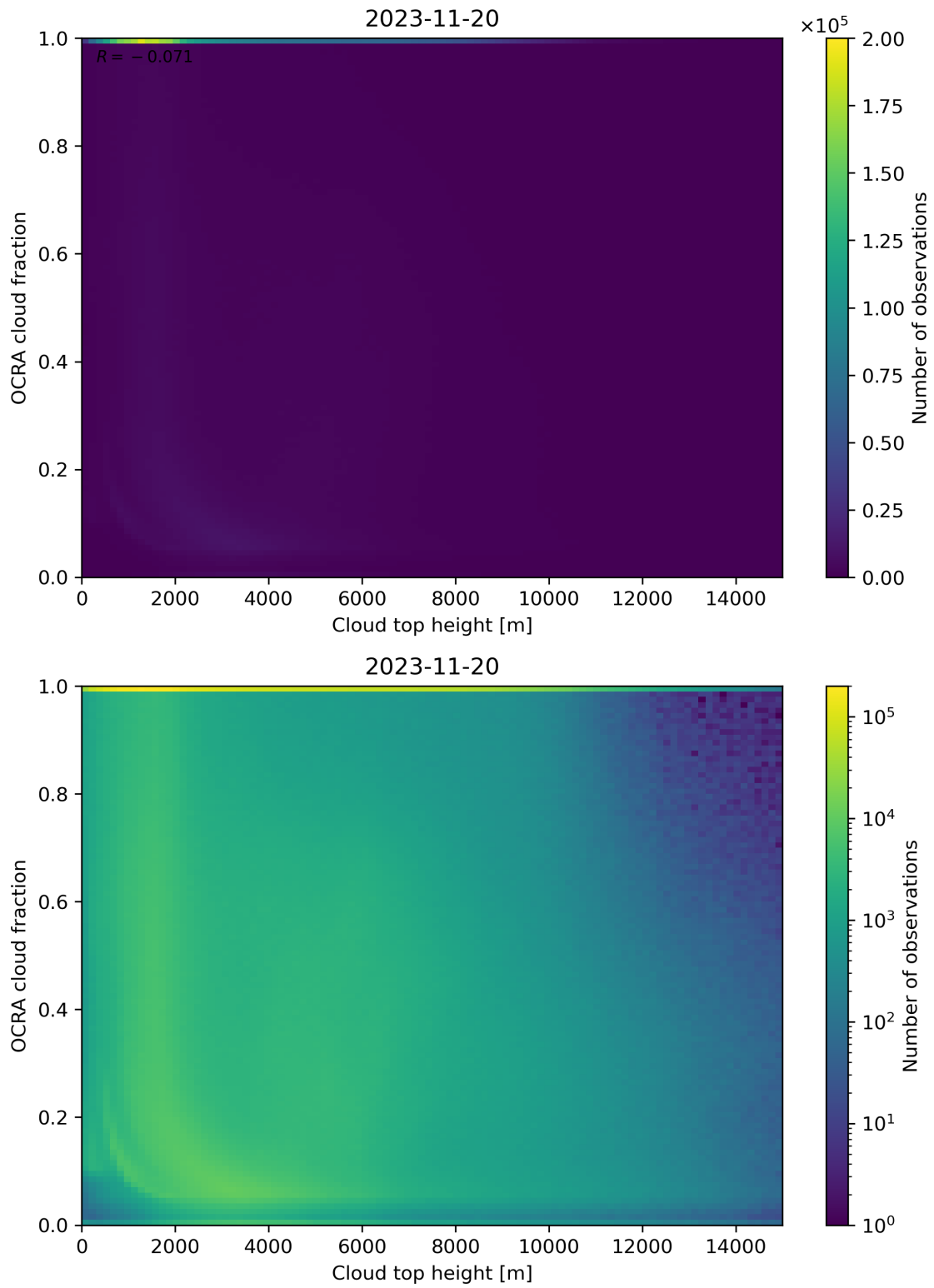
Figure 87: Scatter density plot of “Cloud top height” against “OCRA cloud fraction” for 2023-11-19 to 2023-11-21.
