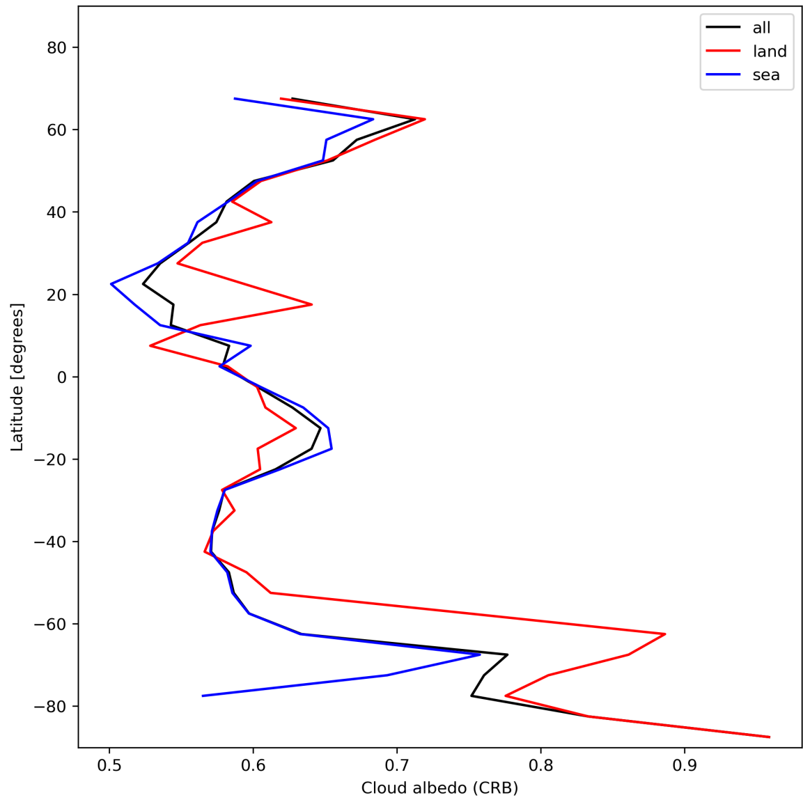
Figure 28: Zonal average of “Cloud albedo (CRB)” for 2023-11-19 to 2023-11-21.
