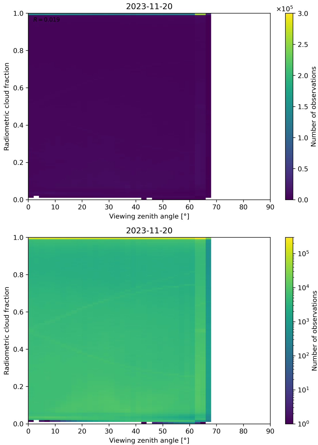
Figure 107: Scatter density plot of “Viewing zenith angle” against “Radiometric cloud fraction” for 2023-11-19 to 2023-11-21.
