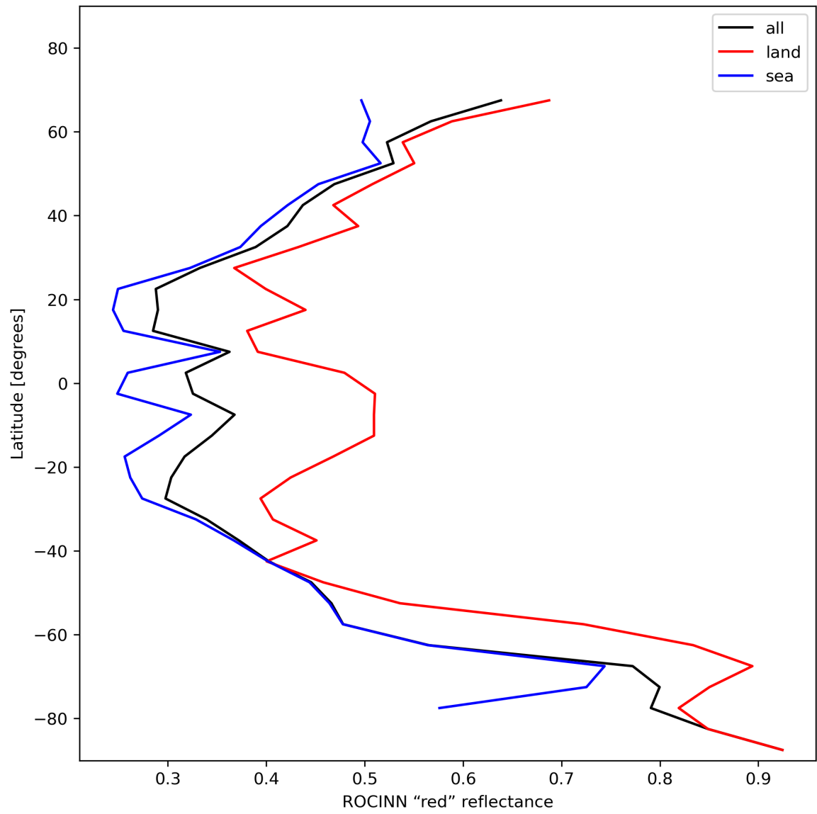
Figure 37: Zonal average of “ROCINN “red” reflectance” for 2023-11-19 to 2023-11-21.
