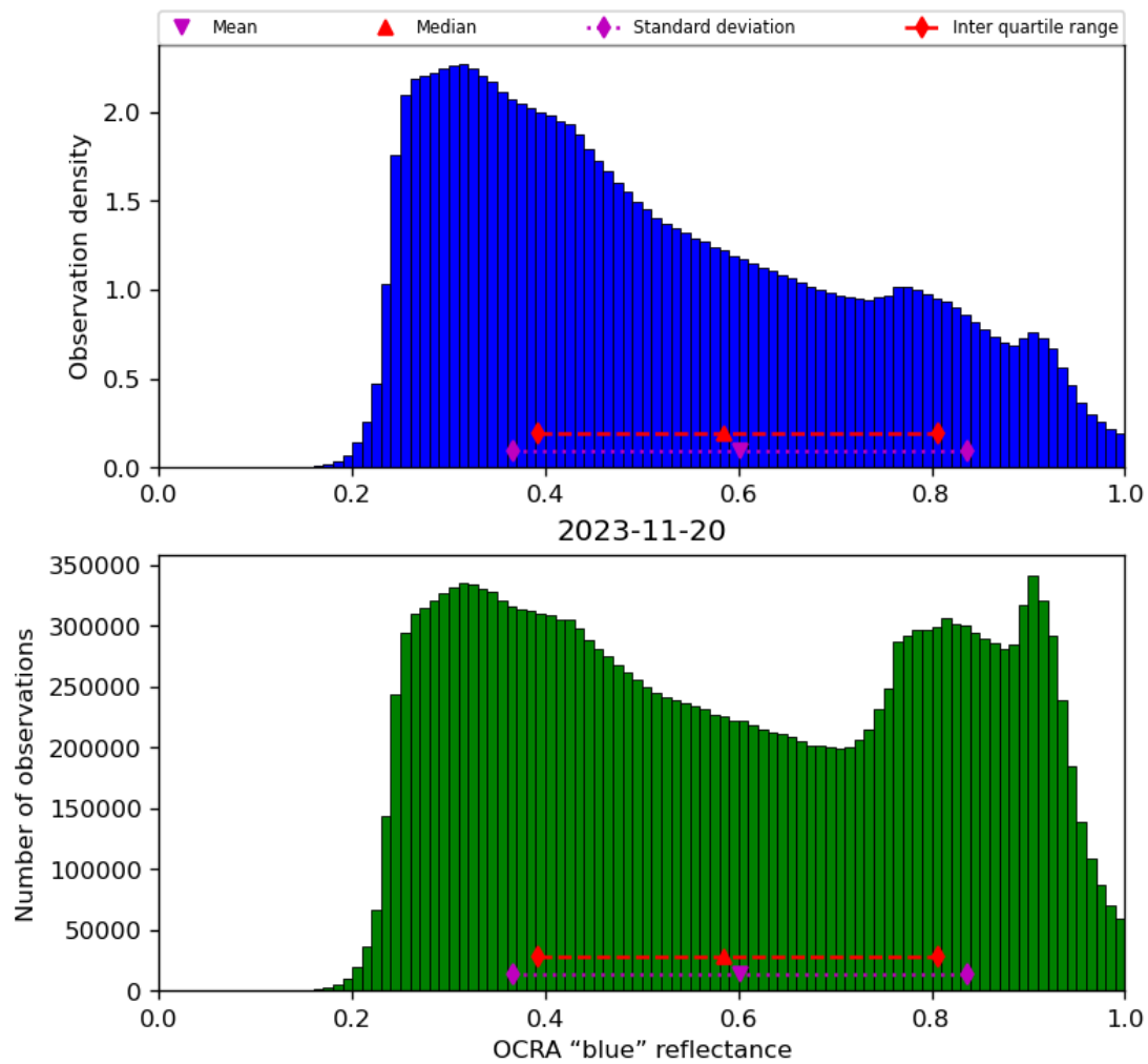
Figure 51: Histogram of “OCRA “blue” reflectance” for 2023-11-19 to 2023-11-21
