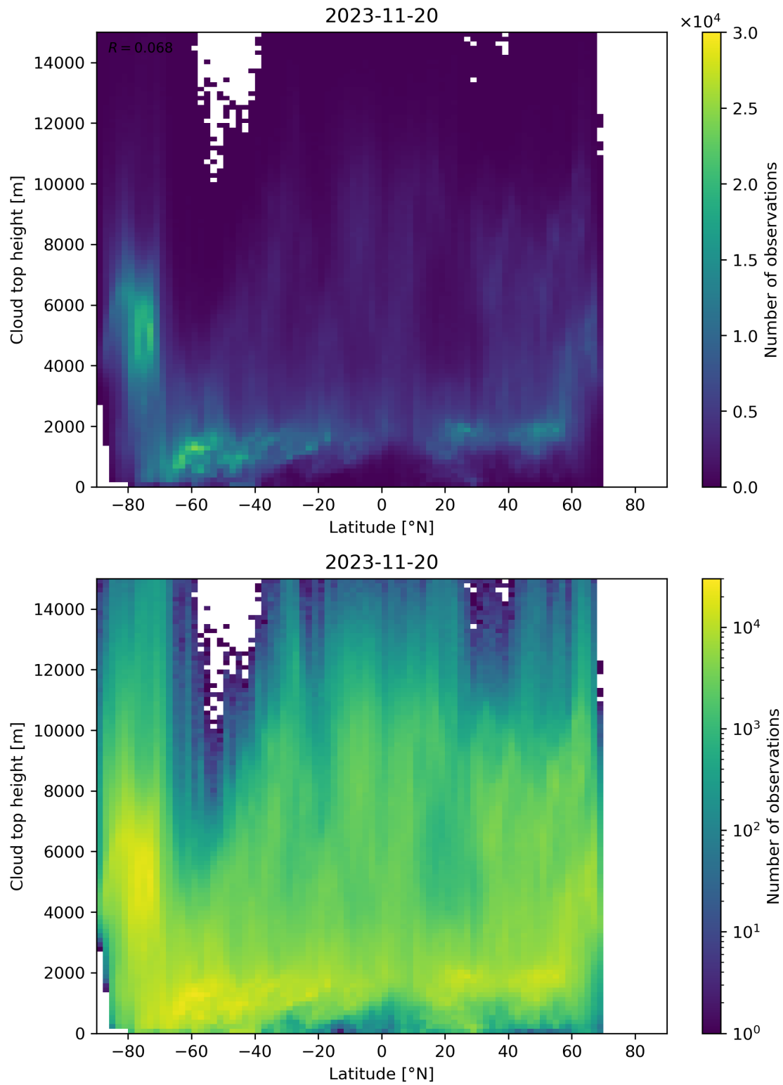
Figure 97: Scatter density plot of “Latitude” against “Cloud top height” for 2023-11-19 to 2023-11-21.
