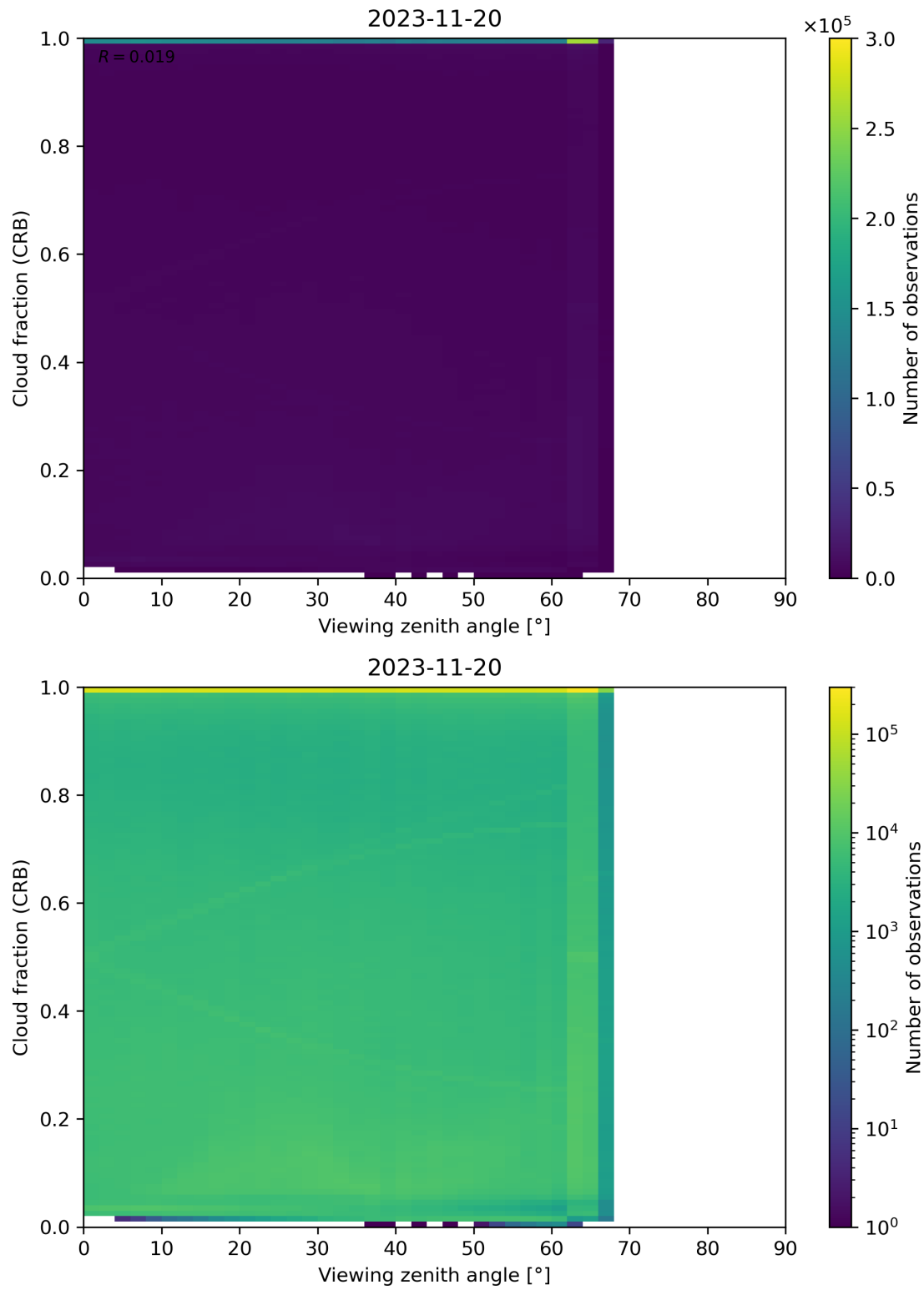
Figure 109: Scatter density plot of “Viewing zenith angle” against “Cloud fraction (CRB)” for 2023-11-19 to 2023-11-21.
