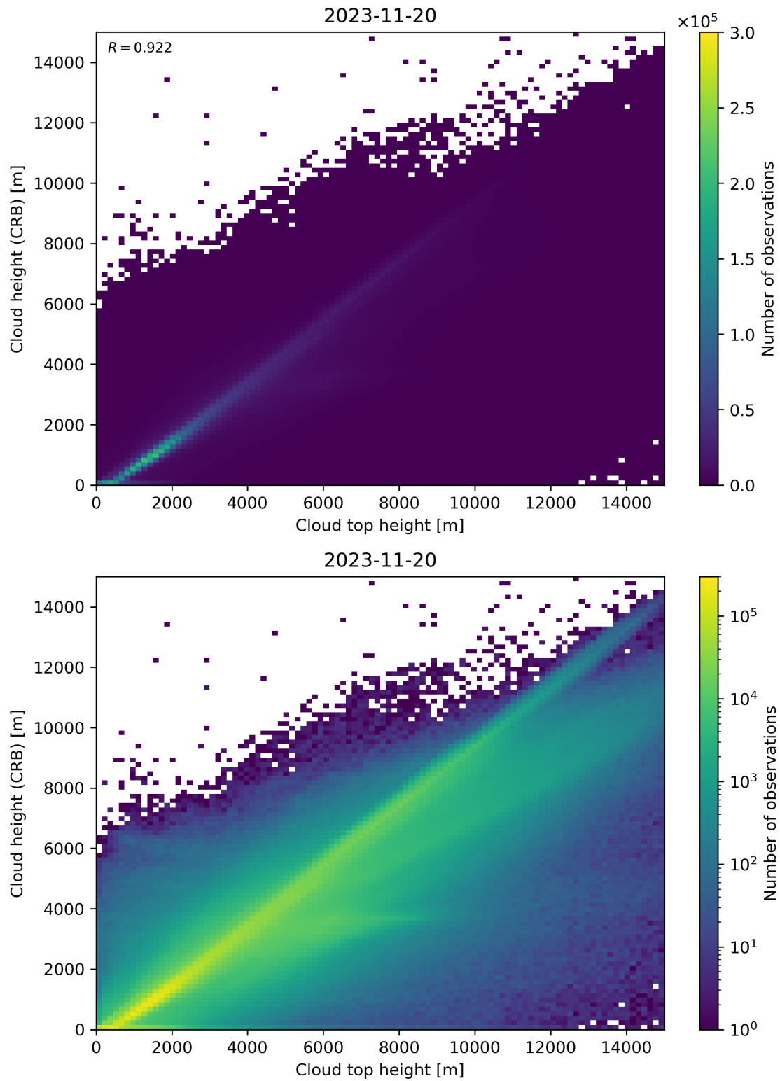
Figure 89: Scatter density plot of “Cloud top height” against “Cloud height (CRB)” for 2023-11-19 to 2023-11-21.
