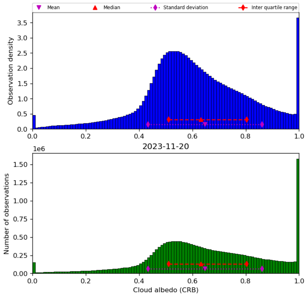
Figure 44: Histogram of “Cloud albedo (CRB)” for 2023-11-19 to 2023-11-21
