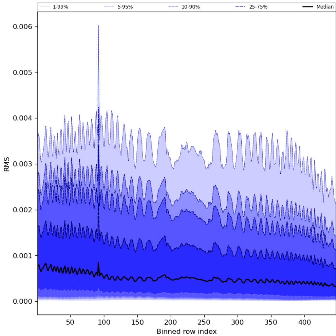
Figure 63: Along track statistics of “RMS” for 2023-11-19 to 2023-11-21
