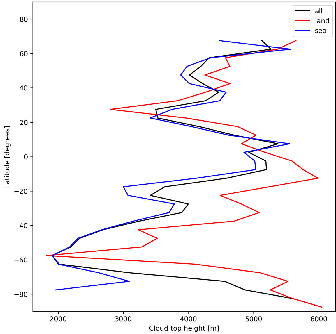
Figure 24: Zonal average of “Cloud top height” for 2023-11-19 to 2023-11-21.
