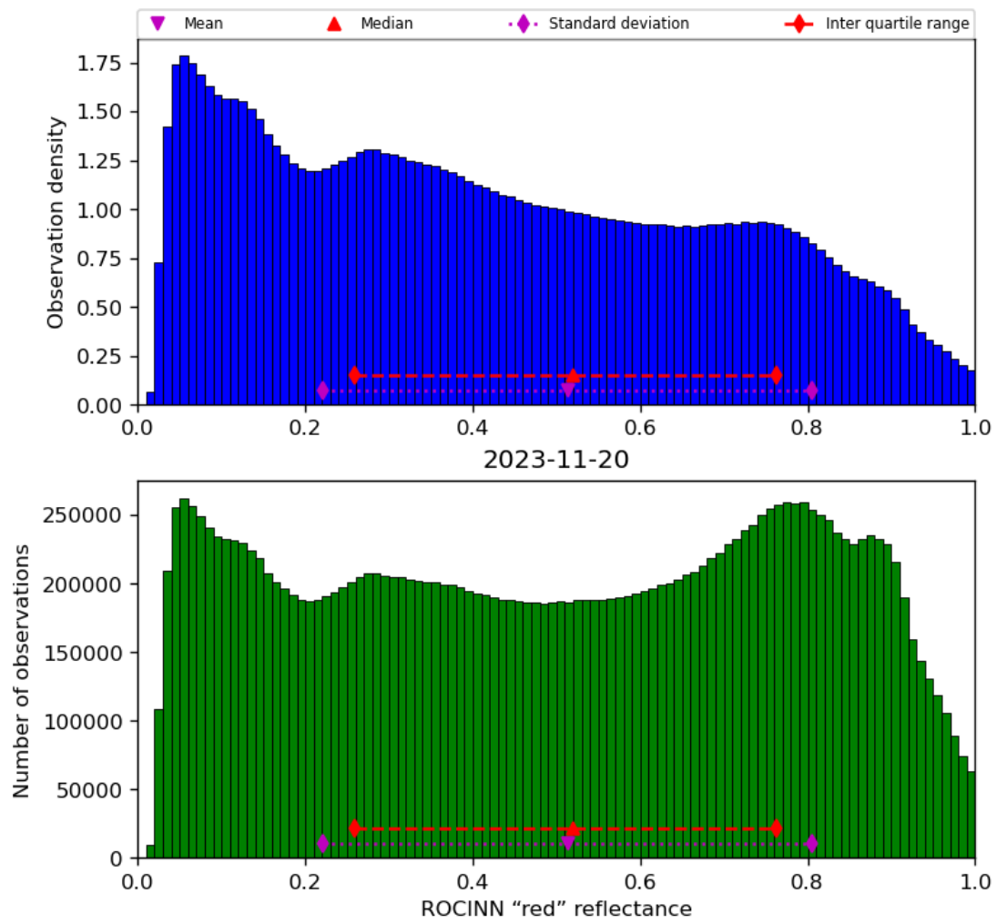
Figure 53: Histogram of “ROCINN “red” reflectance” for 2023-11-19 to 2023-11-21
