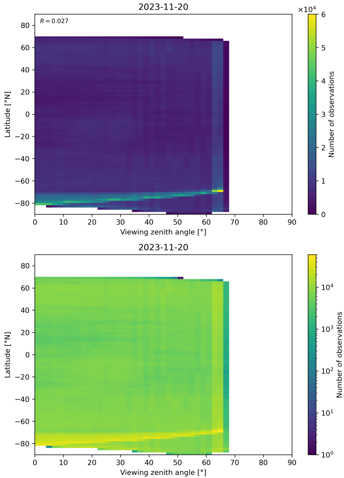
Figure 113: Scatter density plot of “Viewing zenith angle” against “Latitude” for 2023-11-19 to 2023-11-21.
