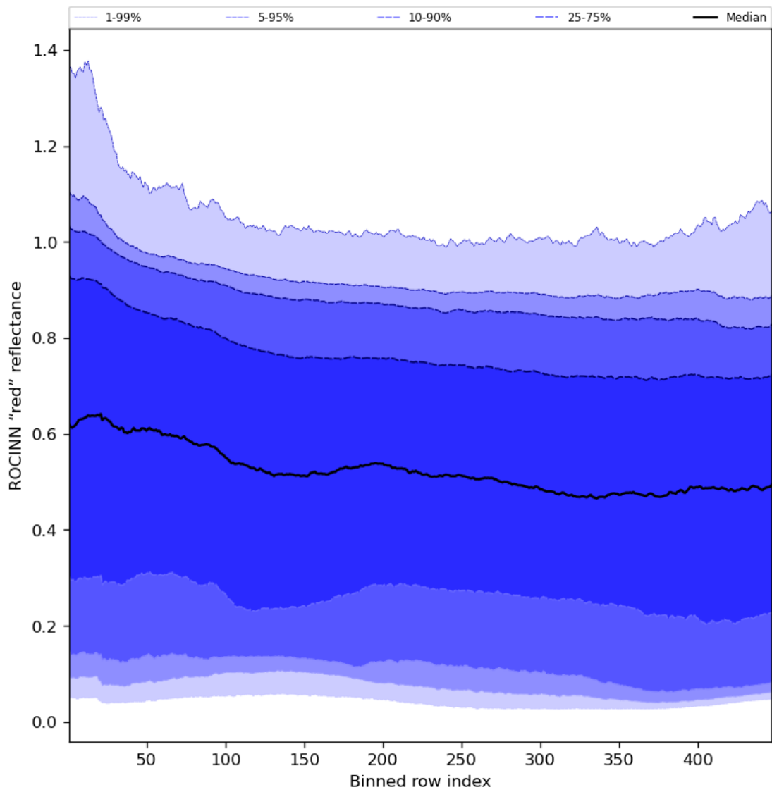
Figure 69: Along track statistics of “ROCINN “red” reflectance” for 2023-11-19 to 2023-11-21
