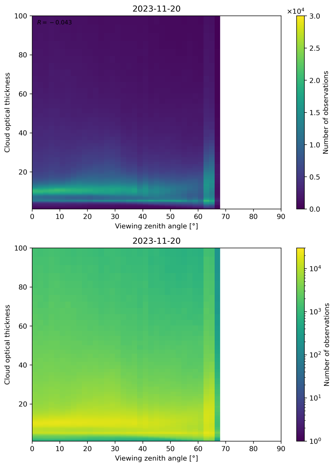
Figure 111: Scatter density plot of “Viewing zenith angle” against “Cloud optical thickness” for 2023-11-19 to 2023-11-21.
