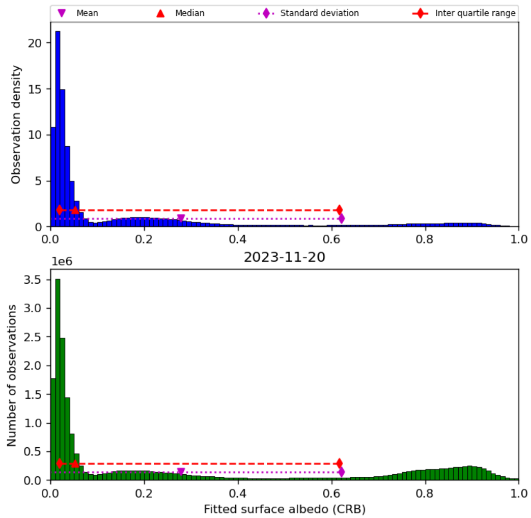
Figure 46: Histogram of “Fitted surface albedo (CRB)” for 2023-11-19 to 2023-11-21
