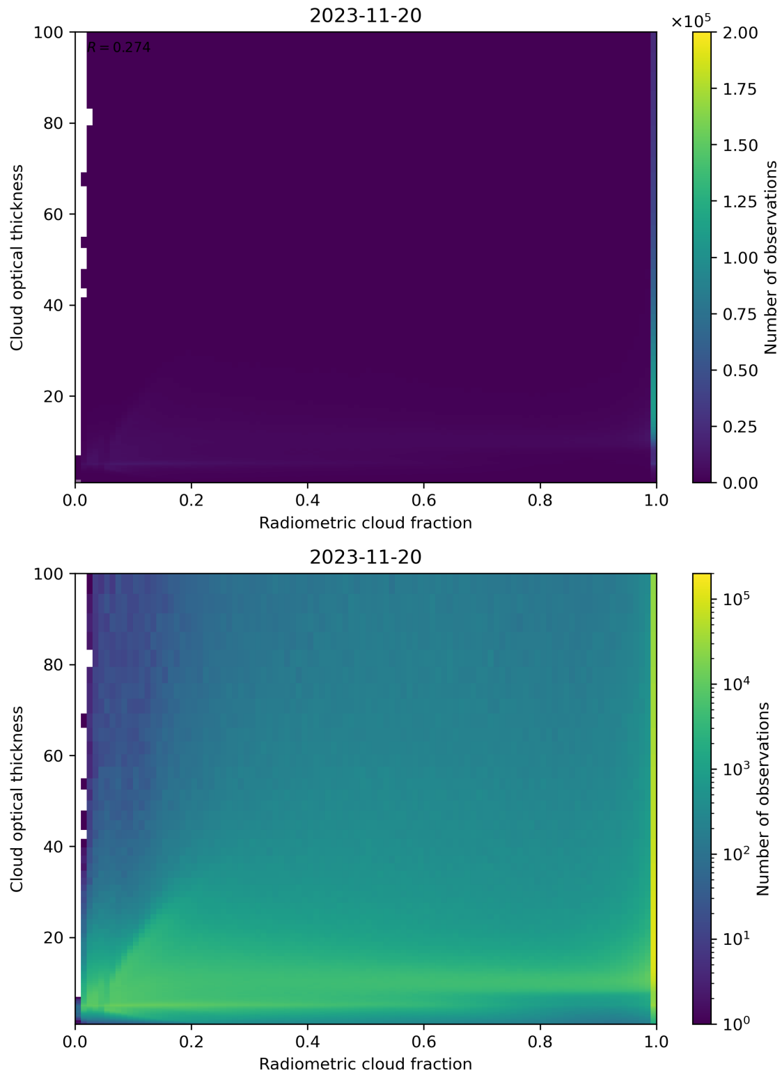
Figure 75: Scatter density plot of “Radiometric cloud fraction” against “Cloud optical thickness” for 2023-11-19 to 2023-11-21.
