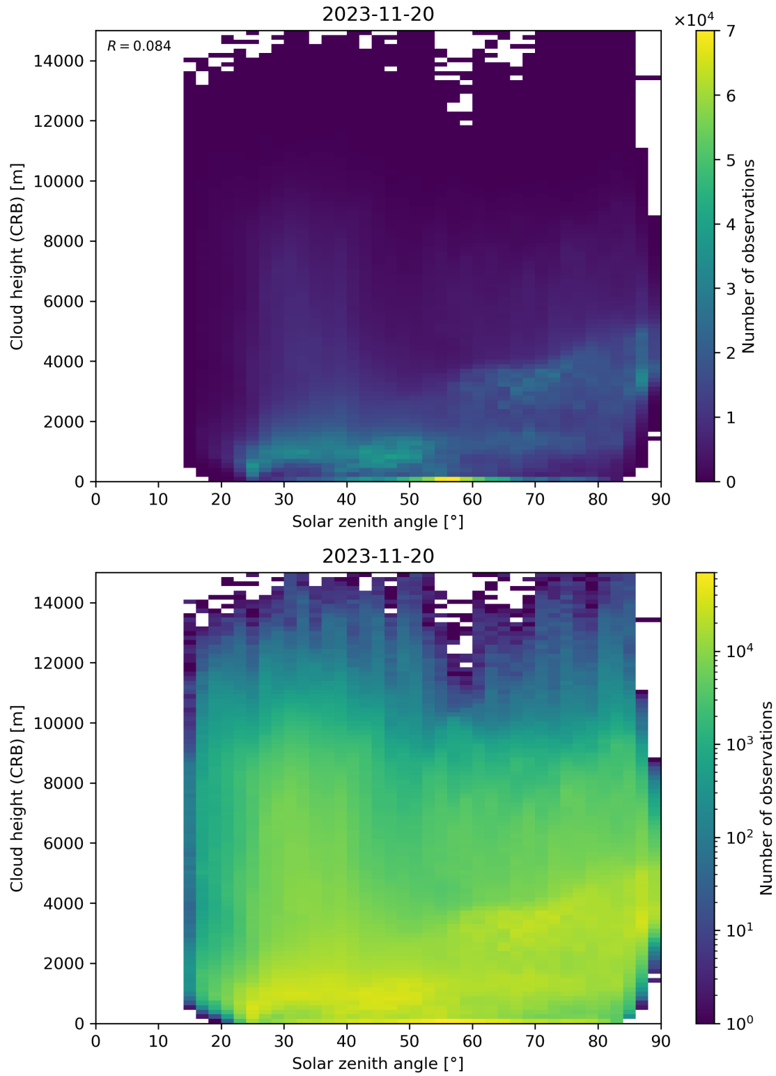
Figure 102: Scatter density plot of “Solar zenith angle” against “Cloud height (CRB)” for 2023-11-19 to 2023-11-21.
