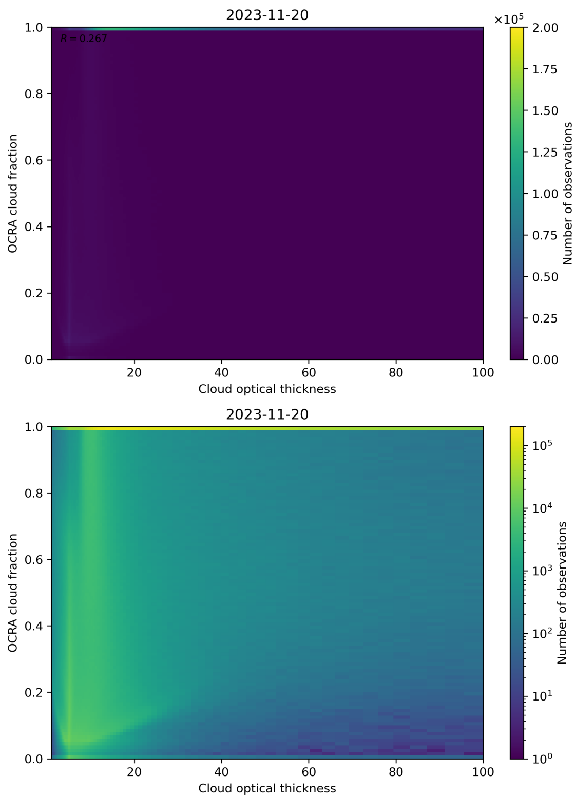
Figure 83: Scatter density plot of “Cloud optical thickness” against “OCRA cloud fraction” for 2023-11-19 to 2023-11-21.
