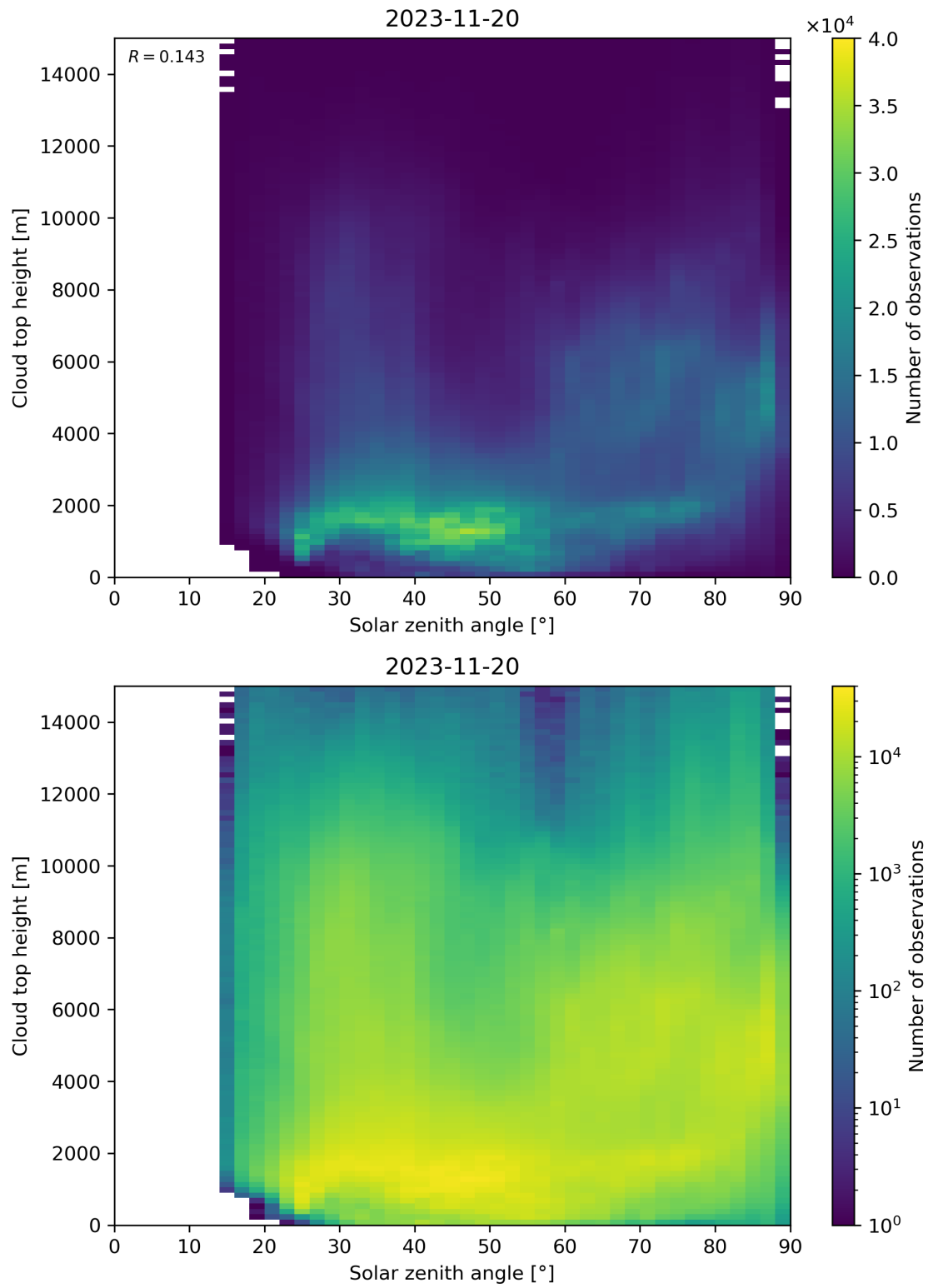
Figure 104: Scatter density plot of “Solar zenith angle” against “Cloud top height” for 2023-11-19 to 2023-11-21.
