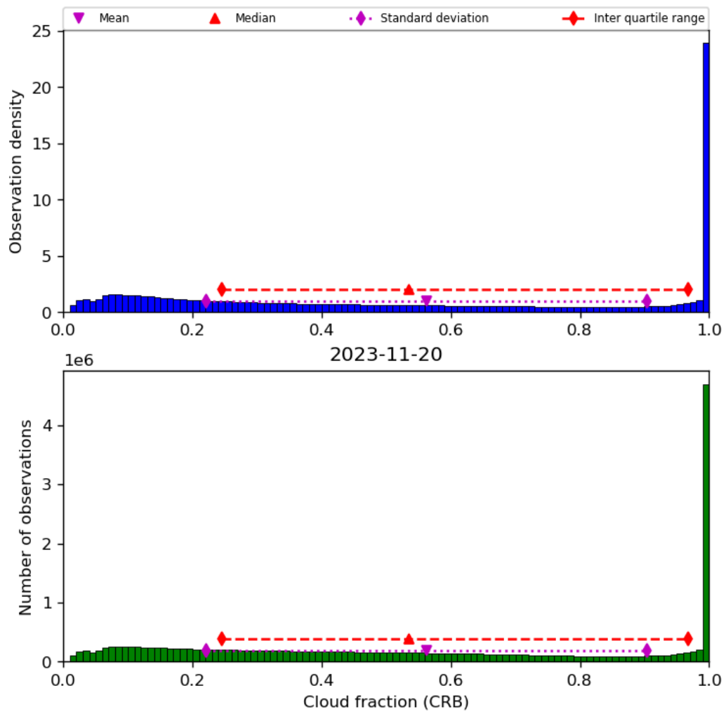
Figure 42: Histogram of “Cloud fraction (CRB)” for 2023-11-19 to 2023-11-21
