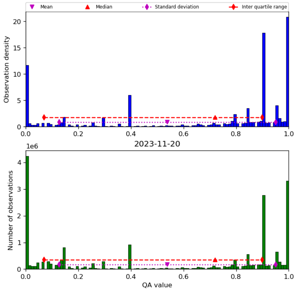
Figure 38: Histogram of “QA value” for 2023-11-19 to 2023-11-21
