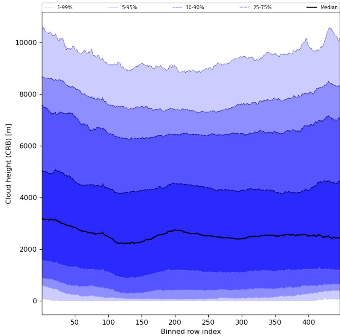
Figure 59: Along track statistics of “Cloud height (CRB)” for 2023-11-19 to 2023-11-21
