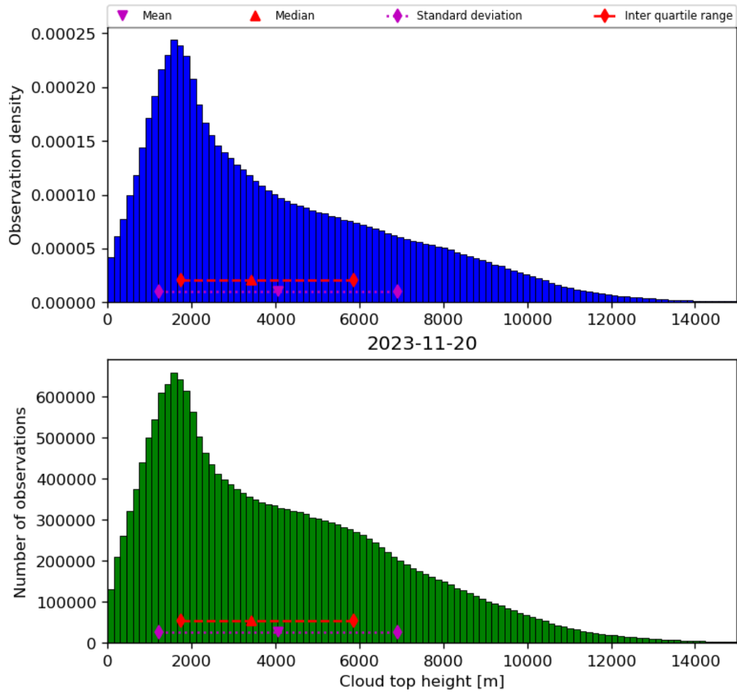
Figure 40: Histogram of “Cloud top height” for 2023-11-19 to 2023-11-21
