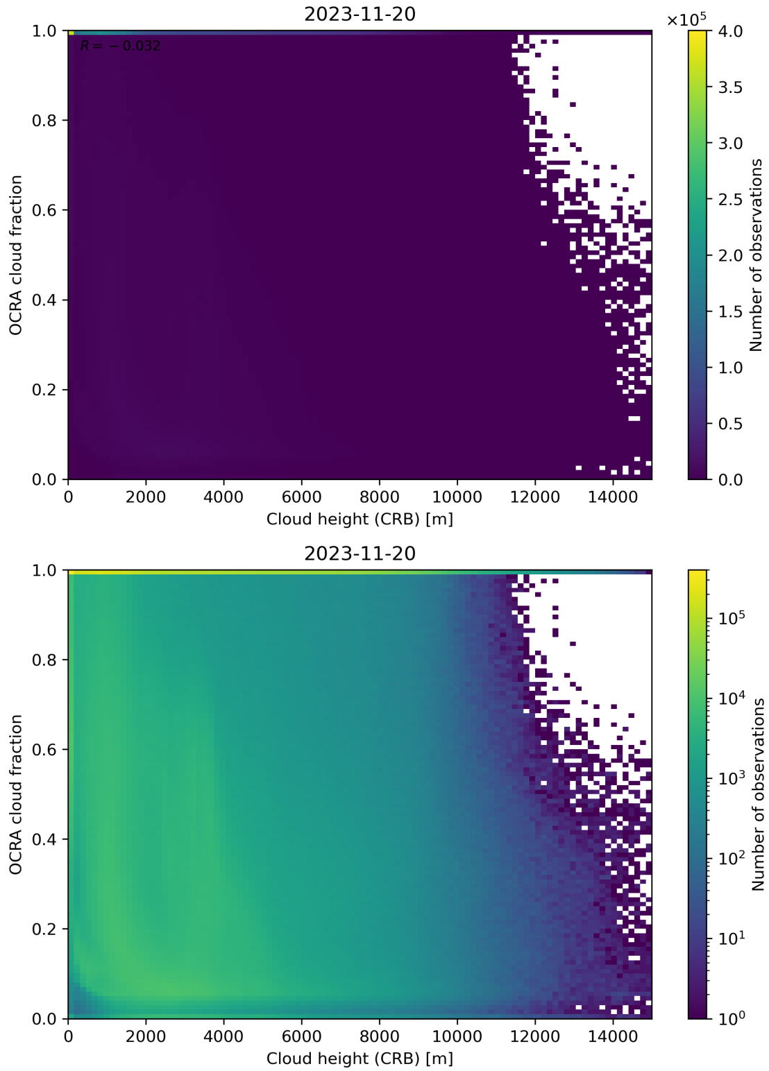
Figure 81: Scatter density plot of “Cloud height (CRB)” against “OCRA cloud fraction” for 2023-11-19 to 2023-11-21.
