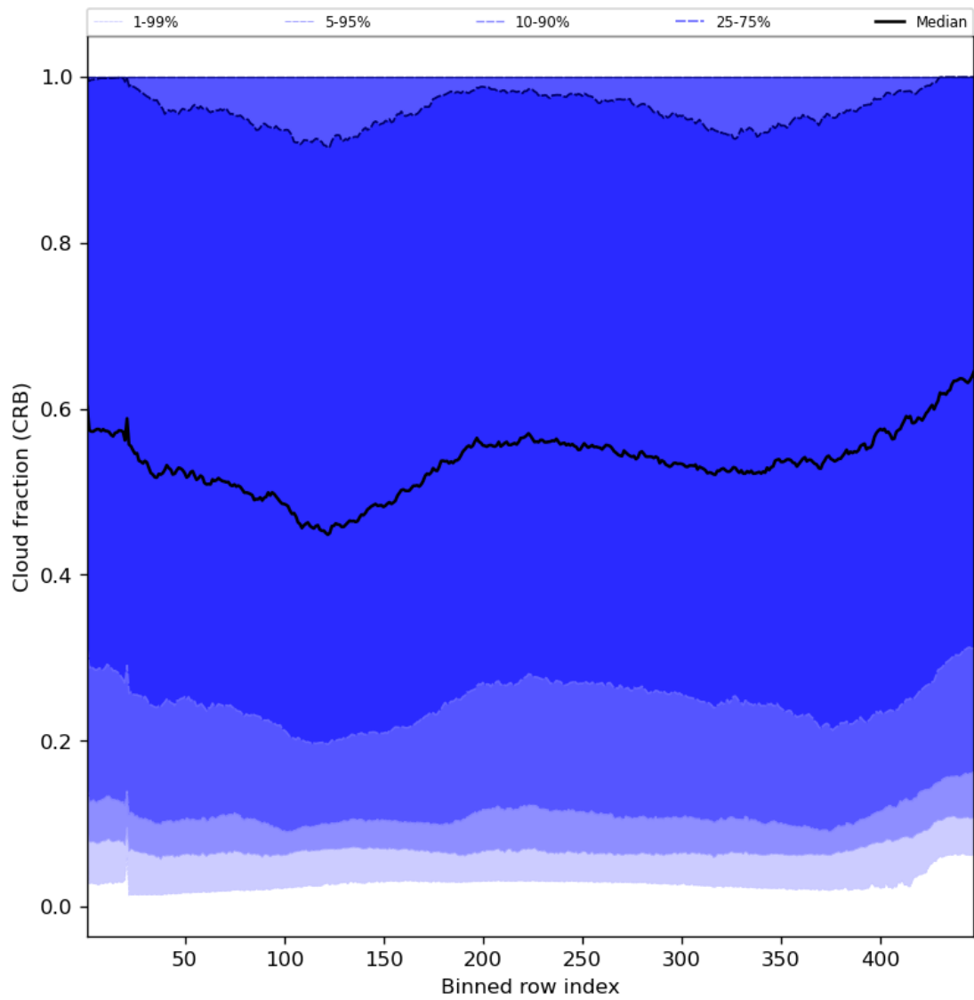
Figure 58: Along track statistics of “Cloud fraction (CRB)” for 2023-11-19 to 2023-11-21
