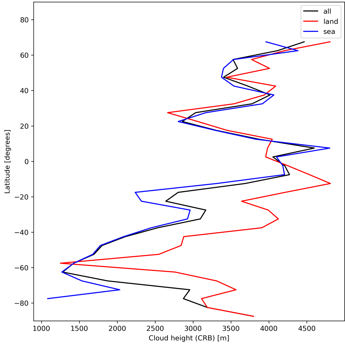
Figure 27: Zonal average of “Cloud height (CRB)” for 2023-11-19 to 2023-11-21.
