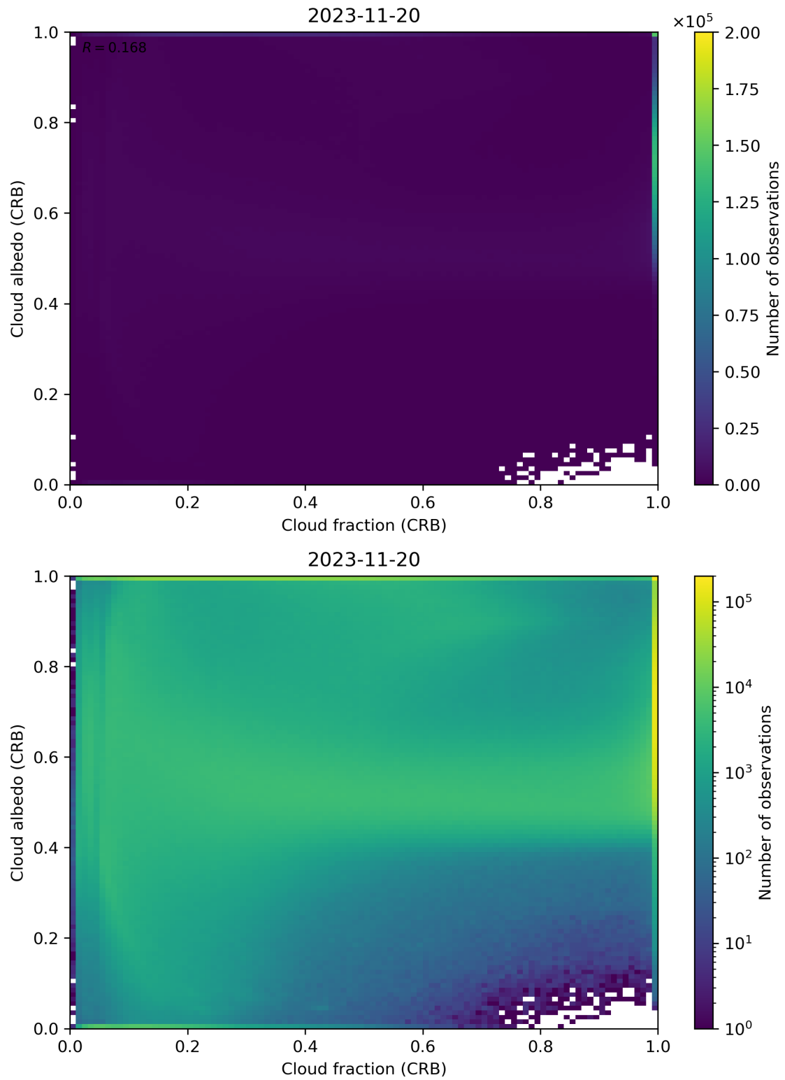
Figure 77: Scatter density plot of “Cloud fraction (CRB)” against “Cloud albedo (CRB)” for 2023-11-19 to 2023-11-21.
