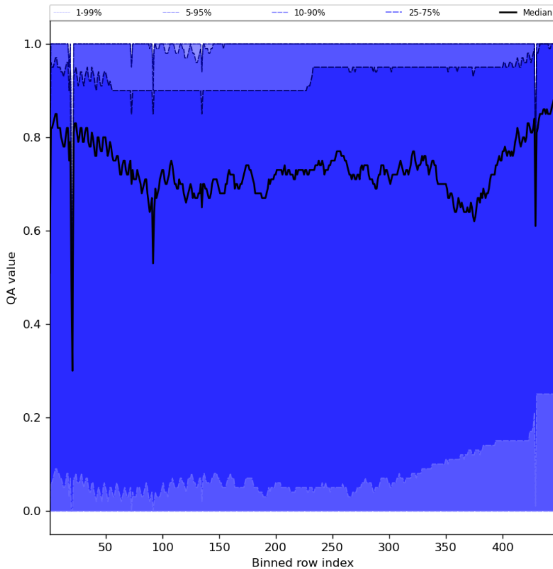
Figure 54: Along track statistics of “QA value” for 2023-11-19 to 2023-11-21
