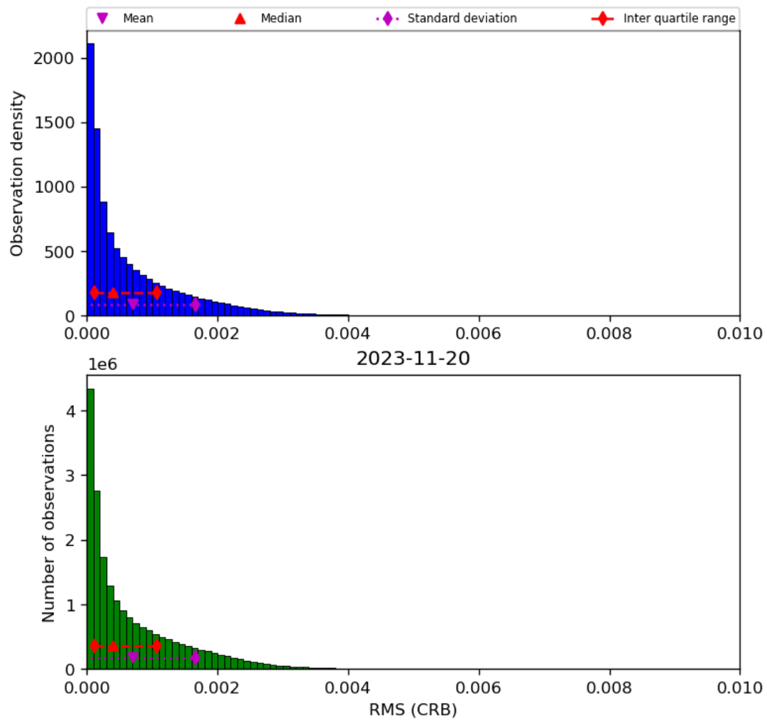
Figure 48: Histogram of “RMS (CRB)” for 2023-11-19 to 2023-11-21
