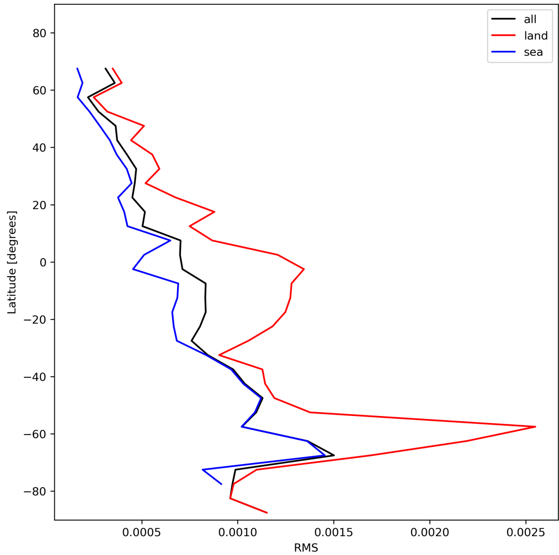
Figure 31: Zonal average of “RMS” for 2023-11-19 to 2023-11-21.
