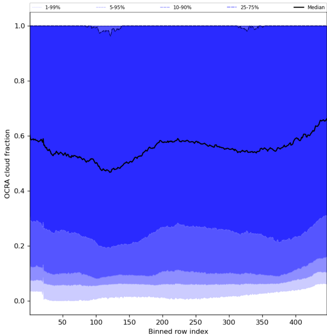
Figure 66: Along track statistics of “OCRA cloud fraction” for 2023-11-19 to 2023-11-21
