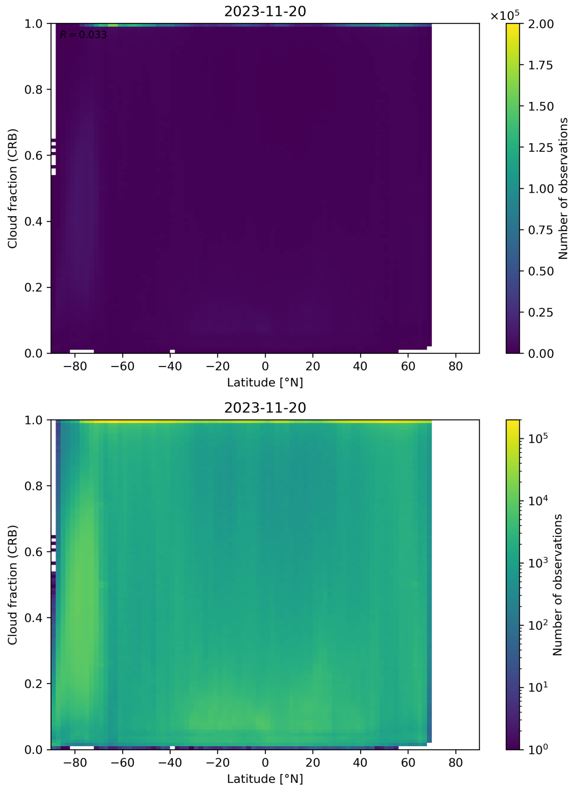
Figure 94: Scatter density plot of “Latitude” against “Cloud fraction (CRB)” for 2023-11-19 to 2023-11-21.
