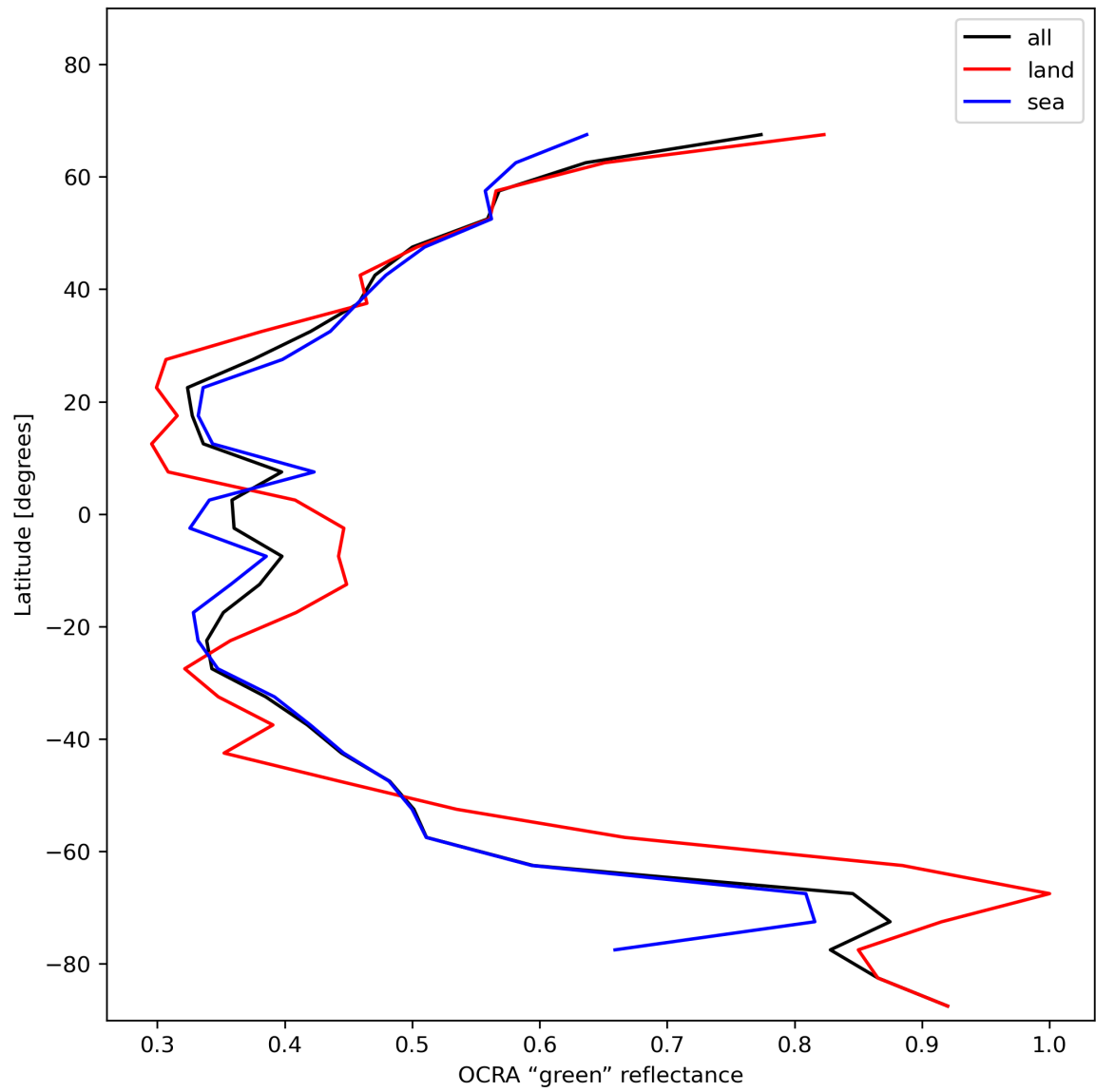
Figure 36: Zonal average of “OCRA “green” reflectance” for 2023-11-19 to 2023-11-21.
