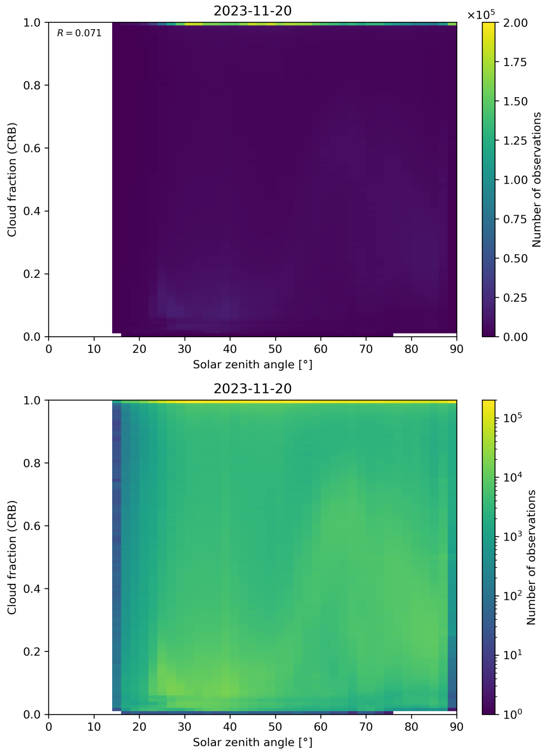
Figure 101: Scatter density plot of “Solar zenith angle” against “Cloud fraction (CRB)” for 2023-11-19 to 2023-11-21.
