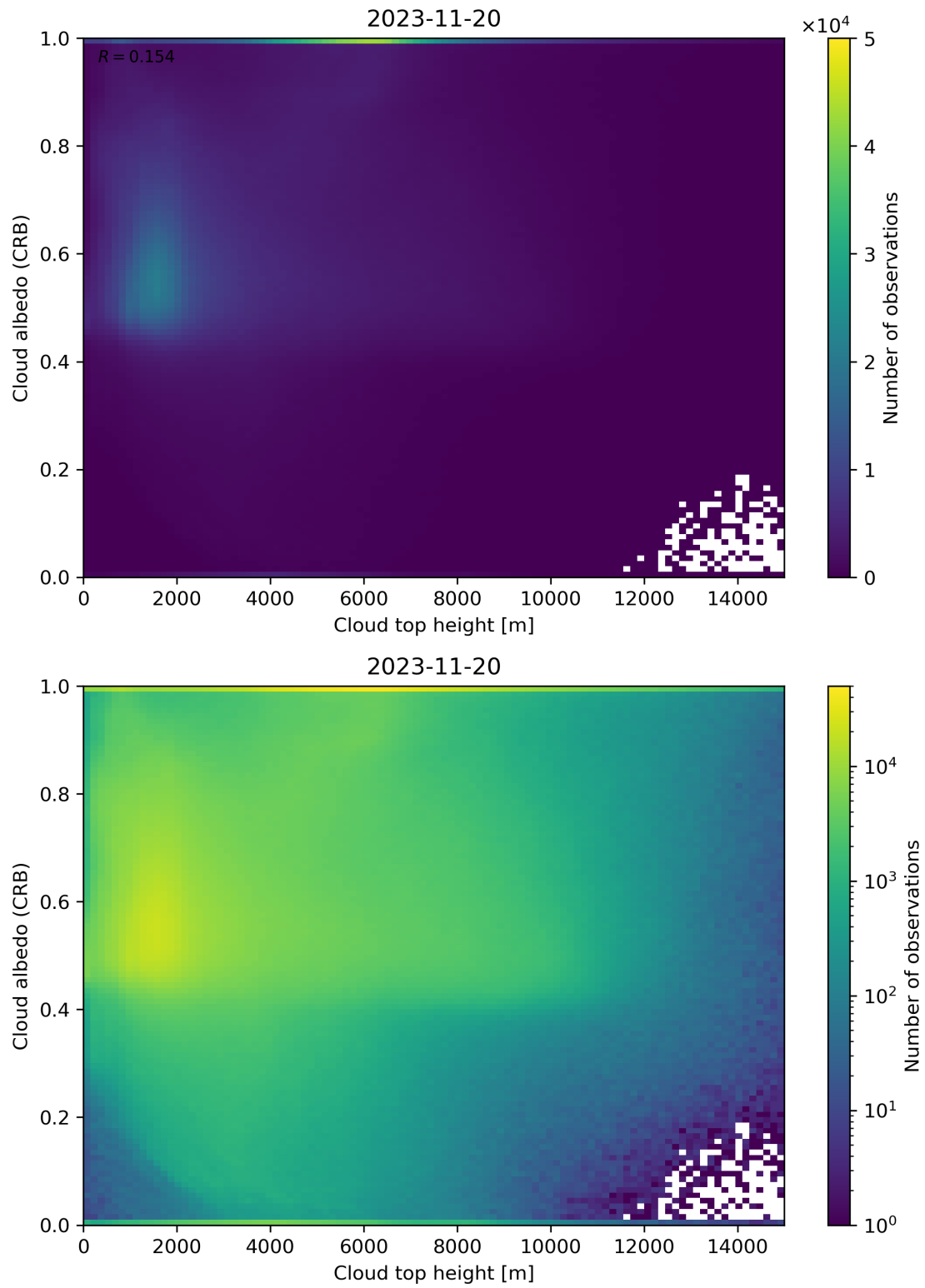
Figure 86: Scatter density plot of “Cloud top height” against “Cloud albedo (CRB)” for 2023-11-19 to 2023-11-21.
