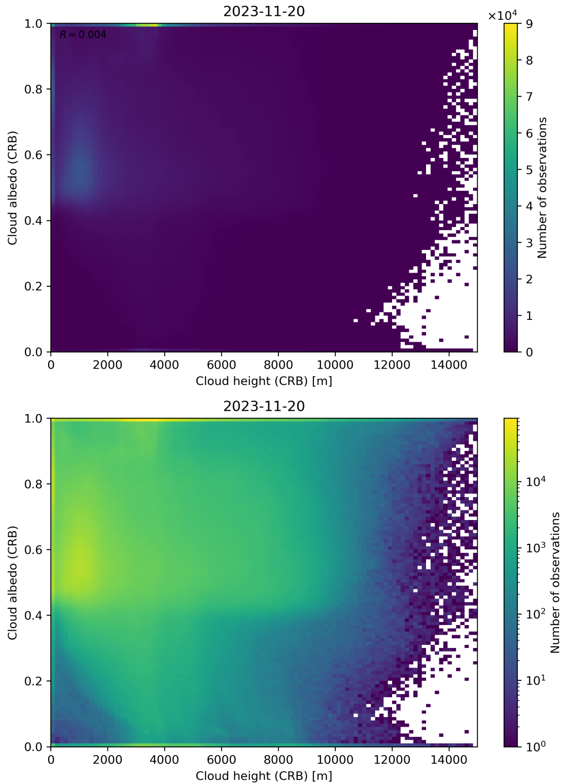
Figure 80: Scatter density plot of “Cloud height (CRB)” against “Cloud albedo (CRB)” for 2023-11-19 to 2023-11-21.
