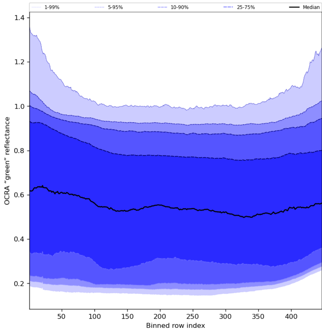
Figure 68: Along track statistics of “OCRA “green” reflectance” for 2023-11-19 to 2023-11-21
