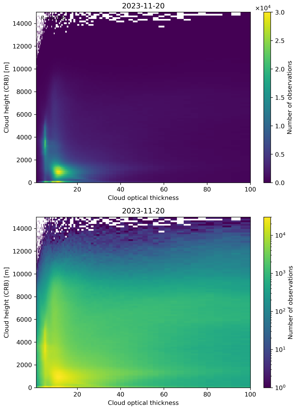
Figure 85: Scatter density plot of “Cloud optical thickness” against “Cloud height (CRB)” for 2023-11-19 to 2023-11-21.
