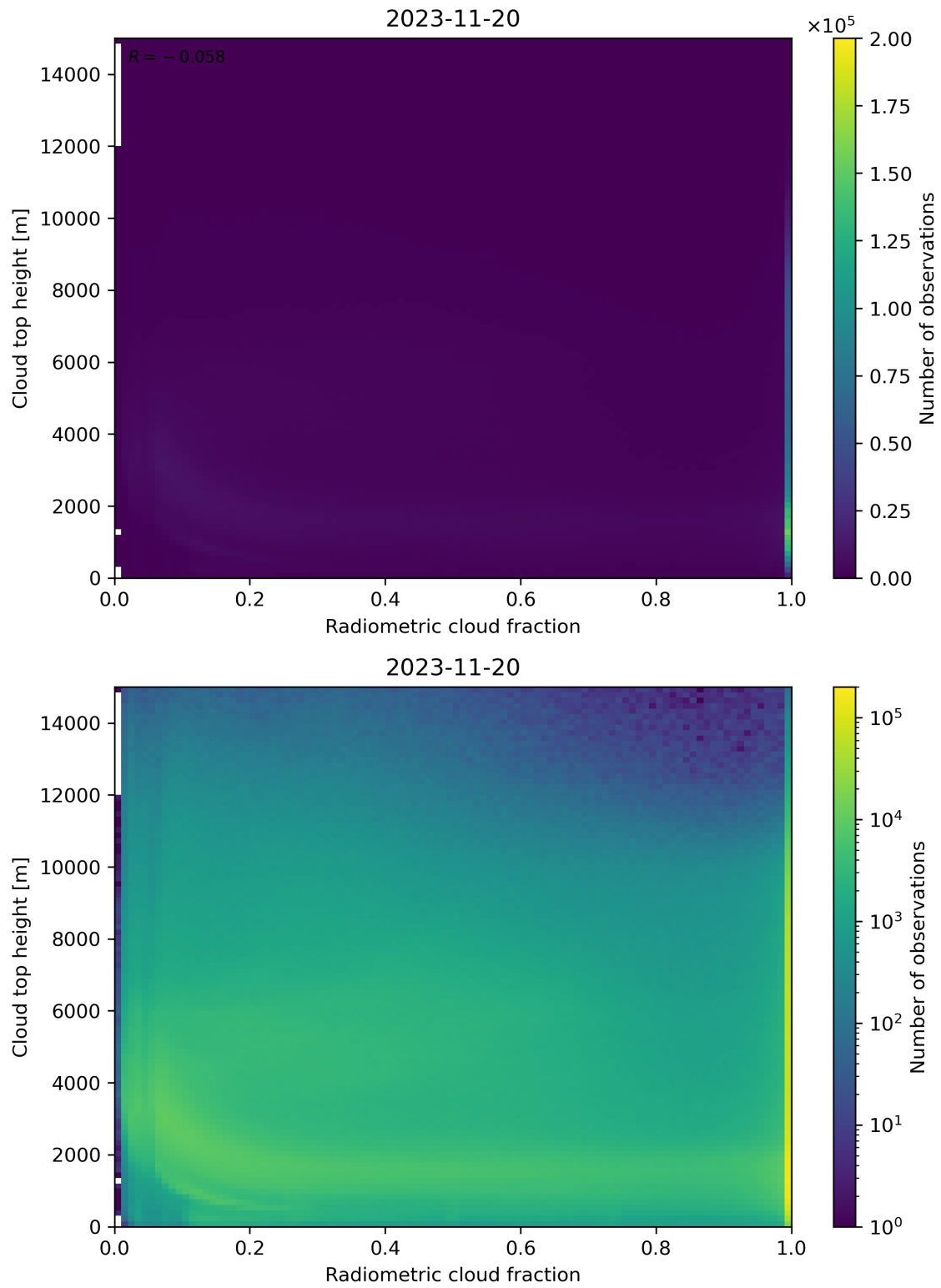
Figure 76: Scatter density plot of “Radiometric cloud fraction” against “Cloud top height” for 2023-11-19 to 2023-11-21.
