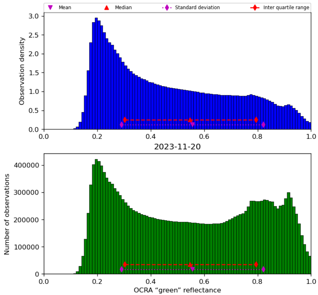
Figure 52: Histogram of “OCRA “green” reflectance” for 2023-11-19 to 2023-11-21
