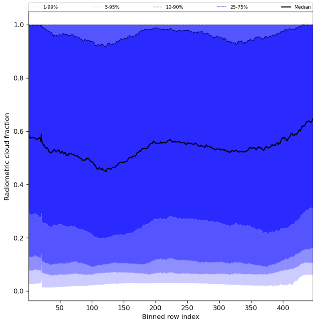
Figure 55: Along track statistics of “Radiometric cloud fraction” for 2023-11-19 to 2023-11-21
