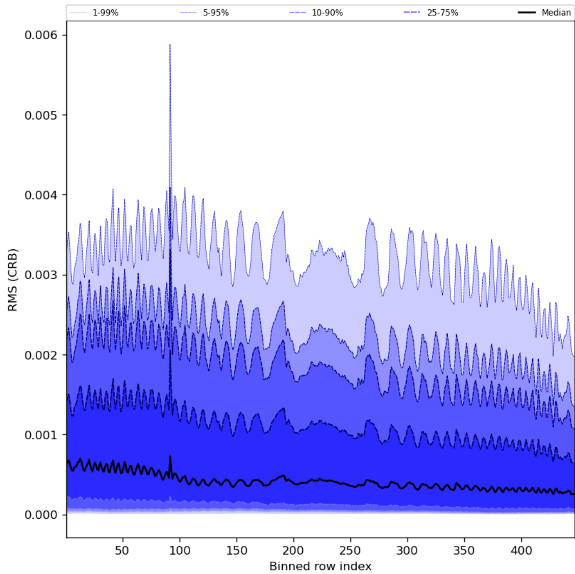
Figure 64: Along track statistics of “RMS (CRB)” for 2023-11-19 to 2023-11-21
