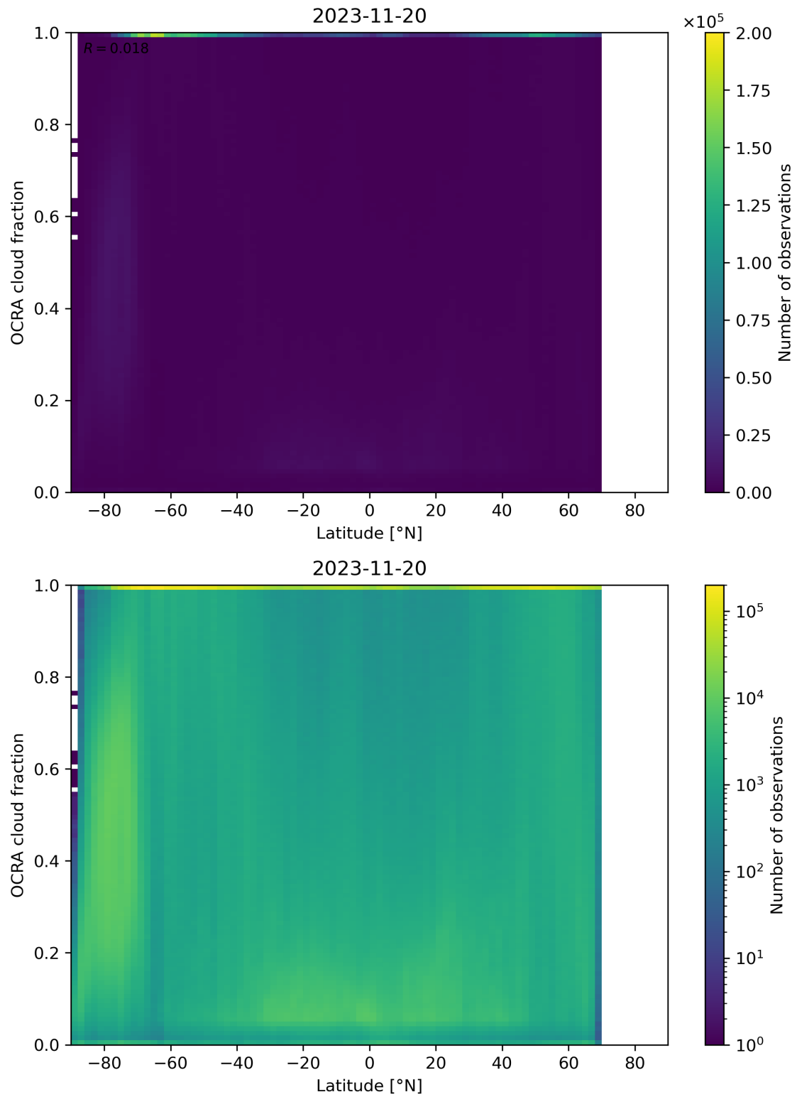
Figure 93: Scatter density plot of “Latitude” against “OCRA cloud fraction” for 2023-11-19 to 2023-11-21.
