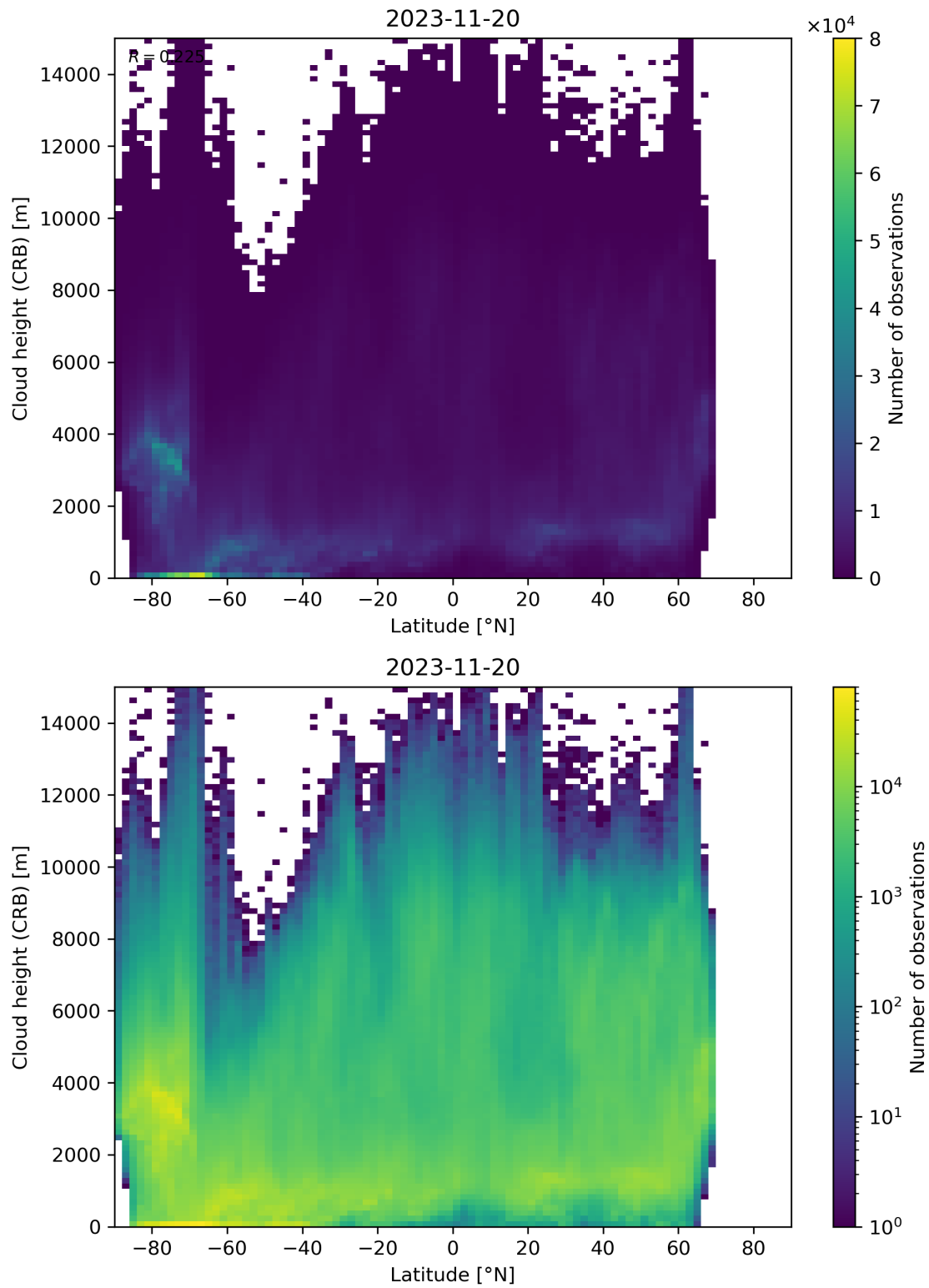
Figure 95: Scatter density plot of “Latitude” against “Cloud height (CRB)” for 2023-11-19 to 2023-11-21.
