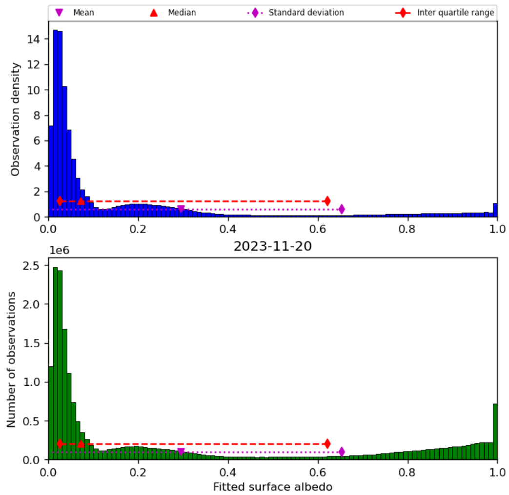
Figure 45: Histogram of “Fitted surface albedo” for 2023-11-19 to 2023-11-21
