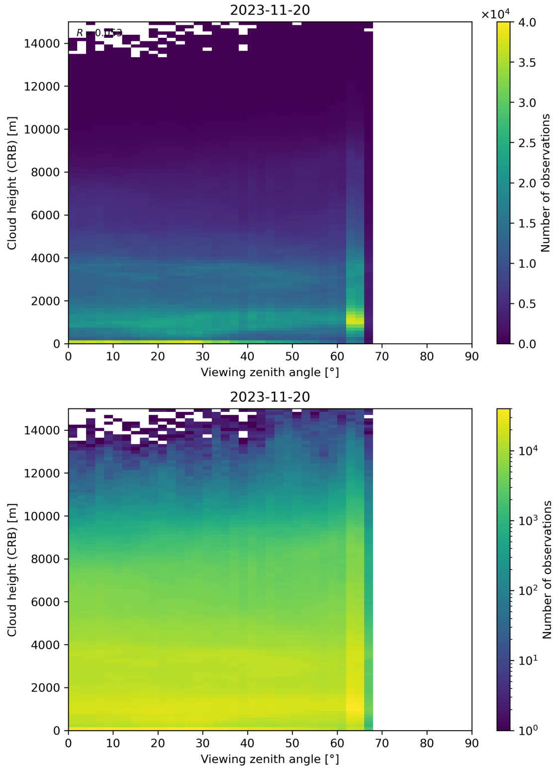
Figure 110: Scatter density plot of “Viewing zenith angle” against “Cloud height (CRB)” for 2023-11-19 to 2023-11-21.
