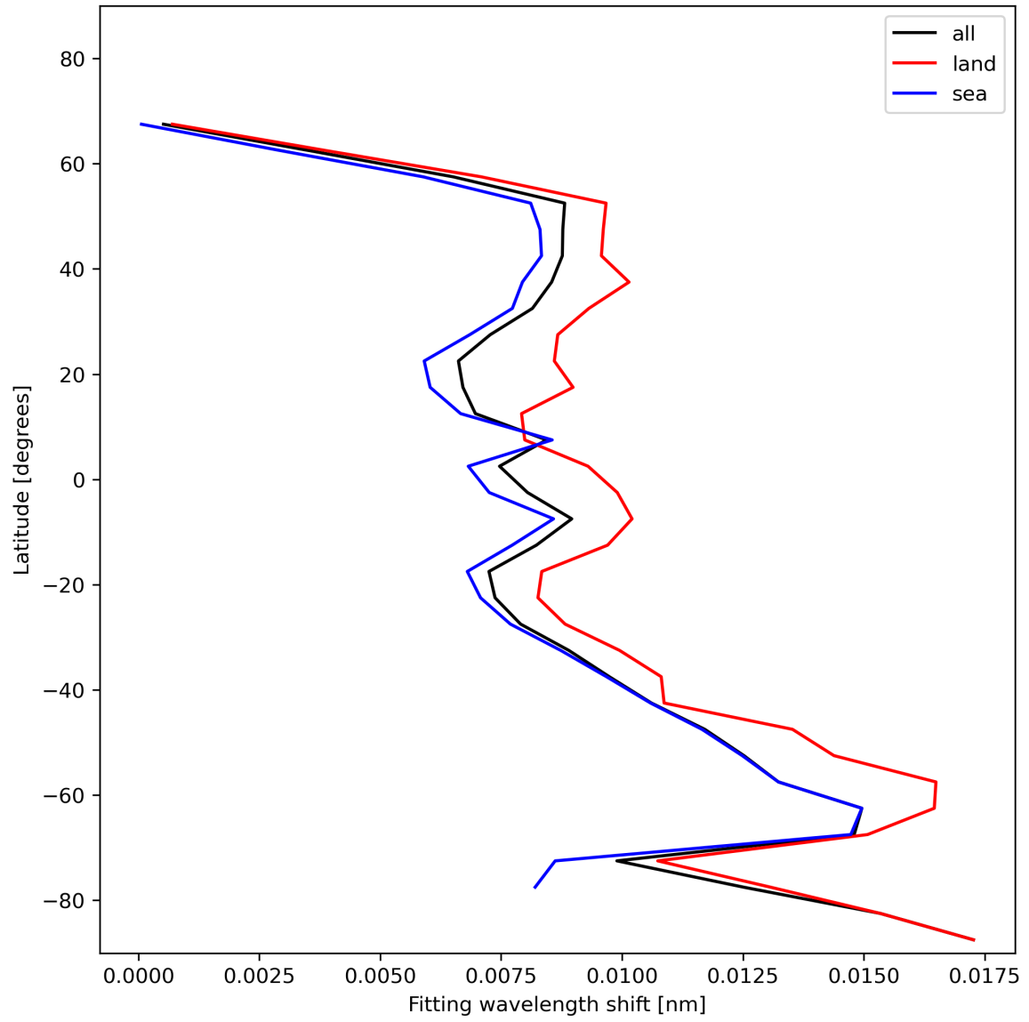
Figure 33: Zonal average of “Fitting wavelength shift” for 2023-11-19 to 2023-11-21.
