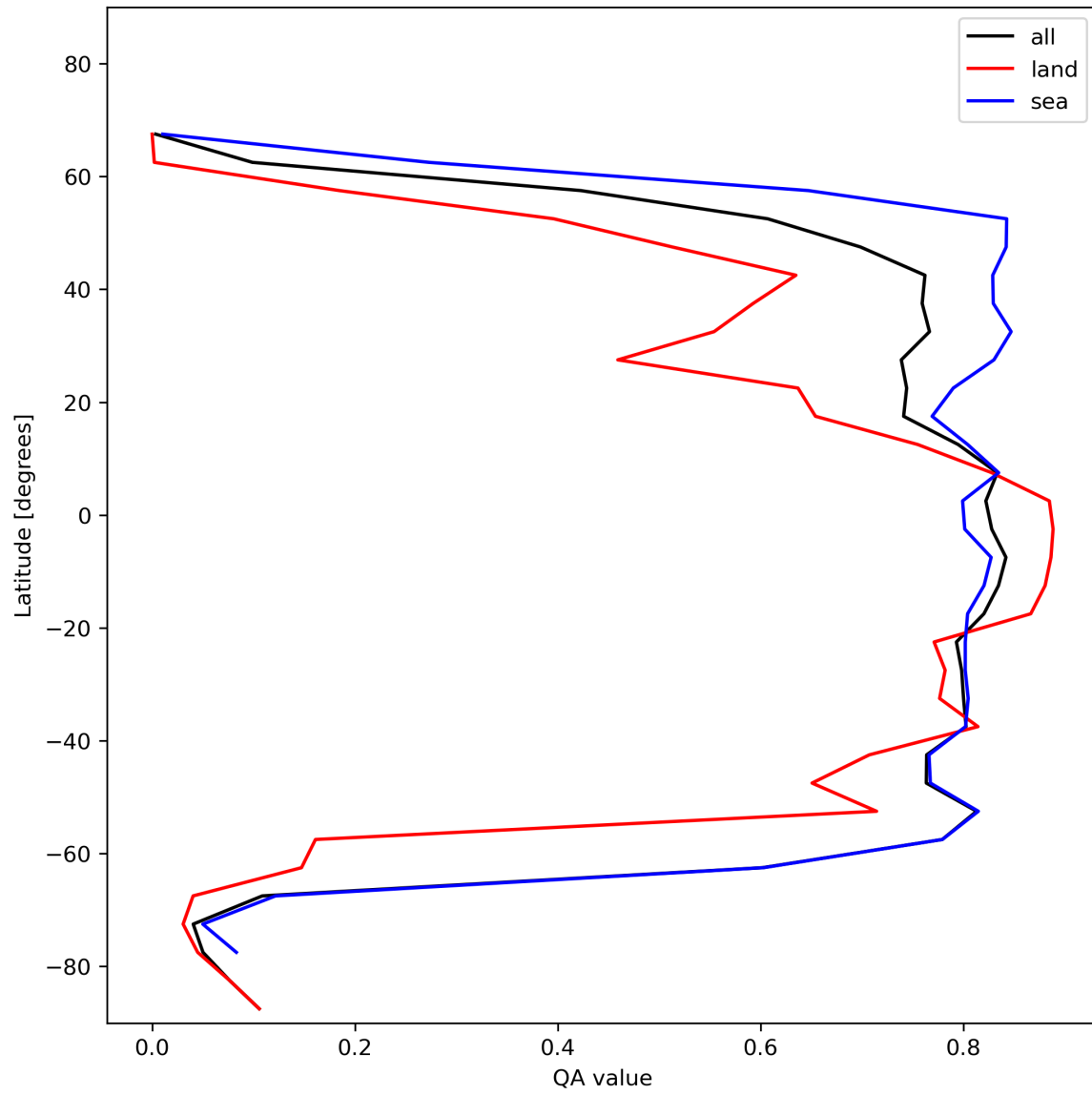
Figure 22: Zonal average of “QA value” for 2023-11-19 to 2023-11-21.
