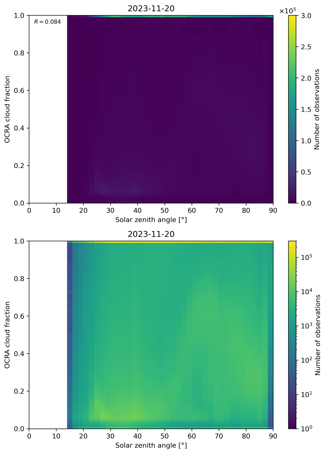
Figure 100: Scatter density plot of “Solar zenith angle” against “OCRA cloud fraction” for 2023-11-19 to 2023-11-21.
