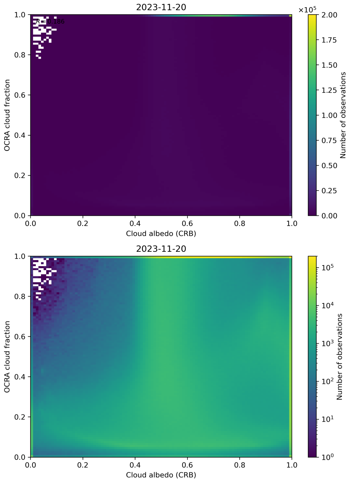
Figure 70: Scatter density plot of “Cloud albedo (CRB)” against “OCRA cloud fraction” for 2023-11-19 to 2023-11-21.
