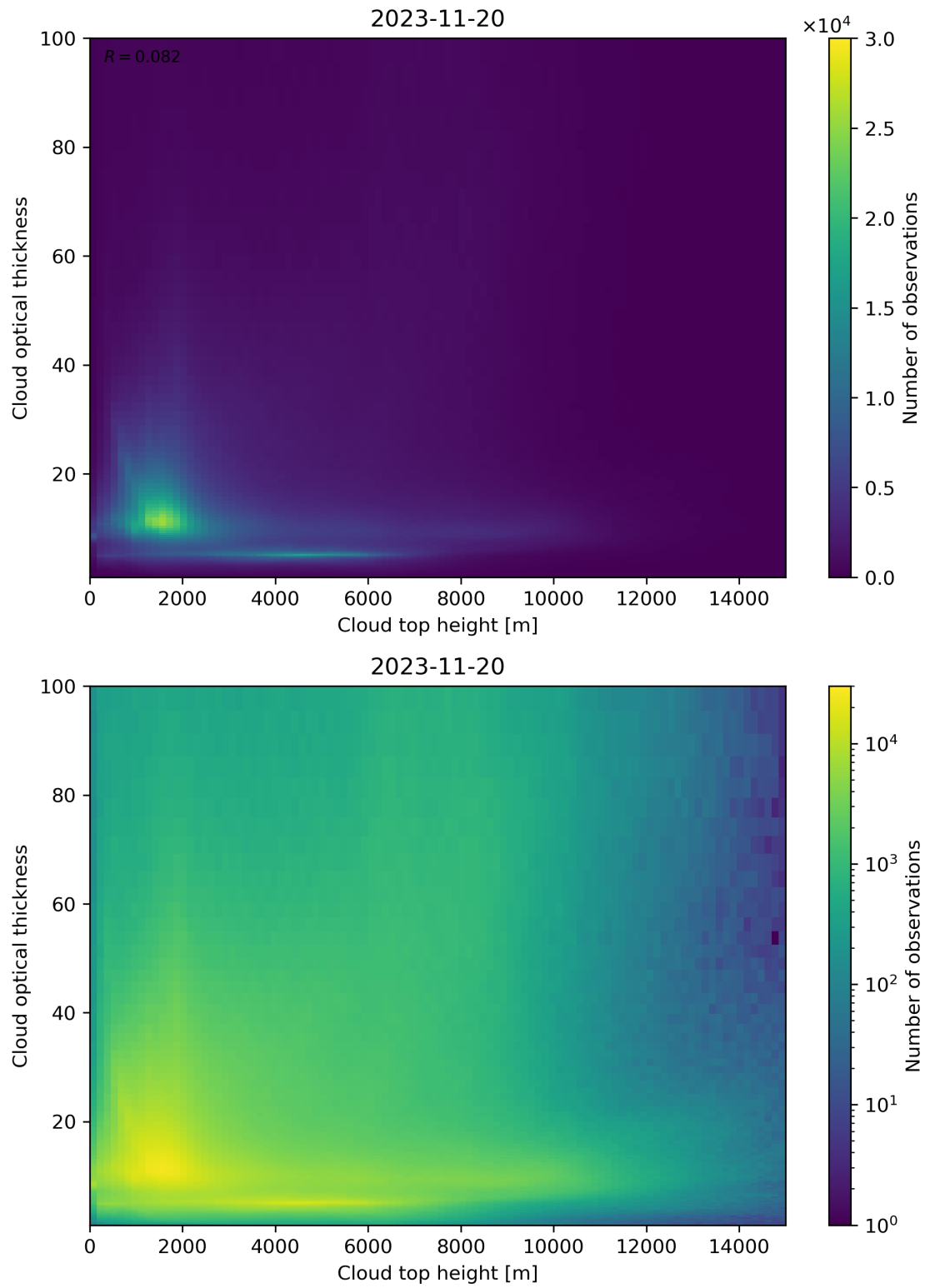
Figure 90: Scatter density plot of “Cloud top height” against “Cloud optical thickness” for 2023-11-19 to 2023-11-21.
