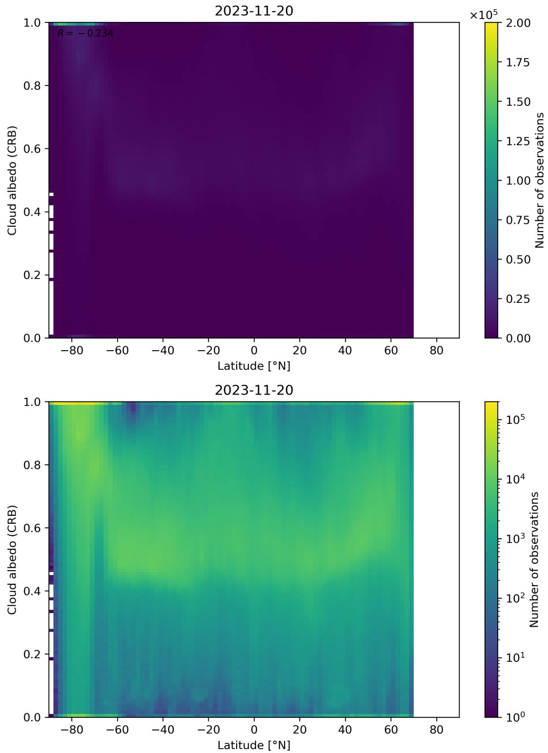
Figure 91: Scatter density plot of “Latitude” against “Cloud albedo (CRB)” for 2023-11-19 to 2023-11-21.
