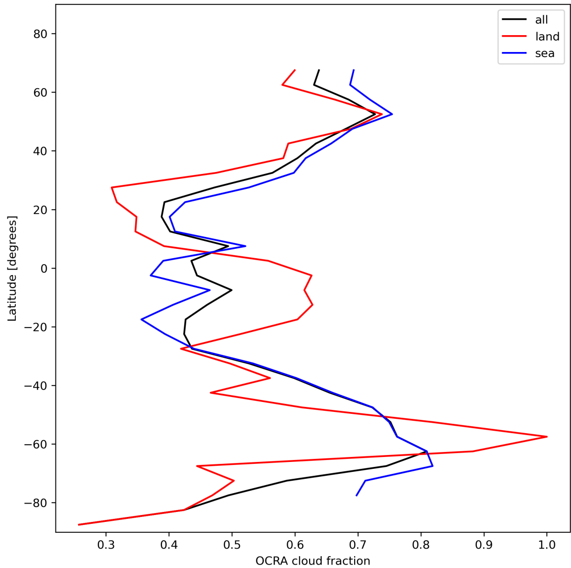
Figure 34: Zonal average of “OCRA cloud fraction” for 2023-11-19 to 2023-11-21.
