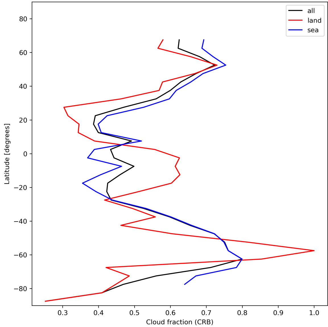
Figure 26: Zonal average of “Cloud fraction (CRB)” for 2023-11-19 to 2023-11-21.
