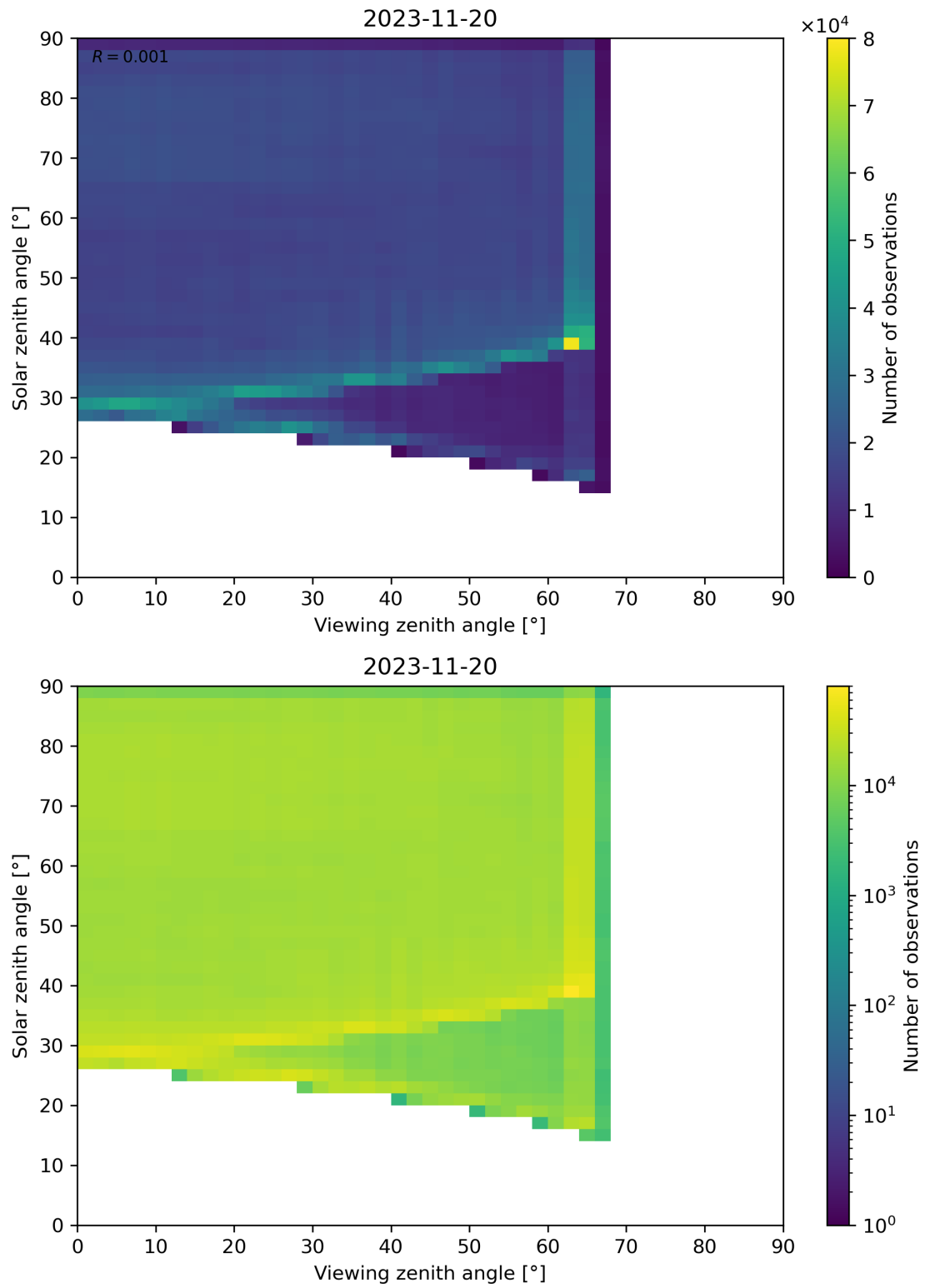
Figure 114: Scatter density plot of “Viewing zenith angle” against “Solar zenith angle” for 2023-11-19 to 2023-11-21.
