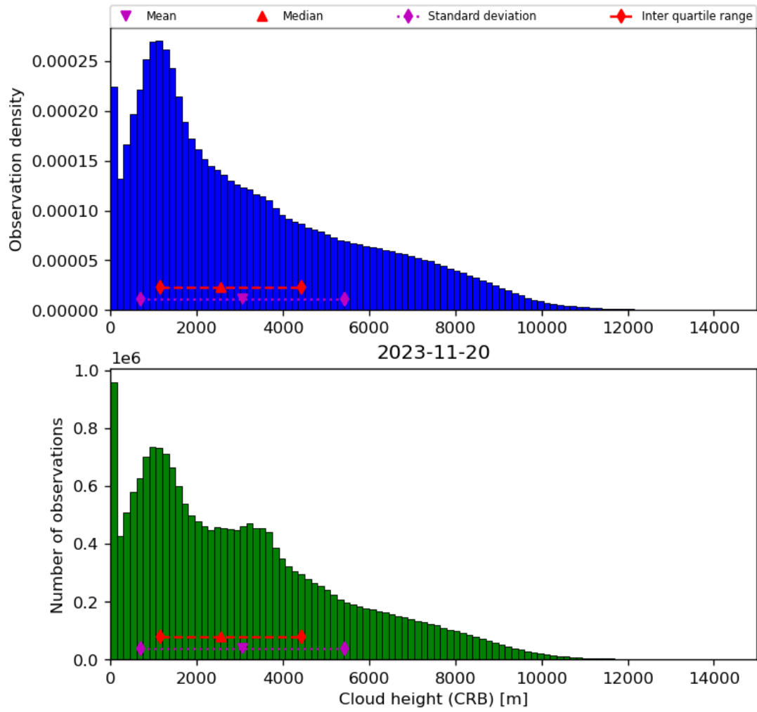
Figure 43: Histogram of “Cloud height (CRB)” for 2023-11-19 to 2023-11-21
