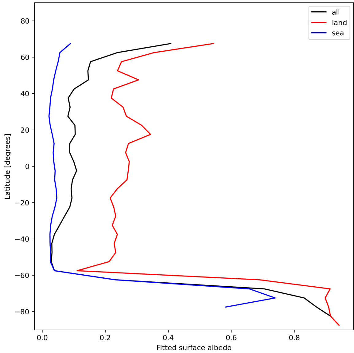
Figure 29: Zonal average of “Fitted surface albedo” for 2023-11-19 to 2023-11-21.
