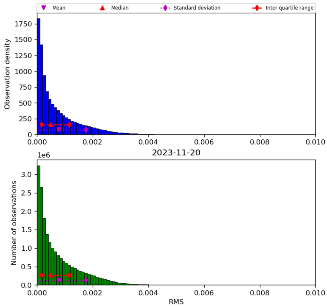
Figure 47: Histogram of “RMS” for 2023-11-19 to 2023-11-21
