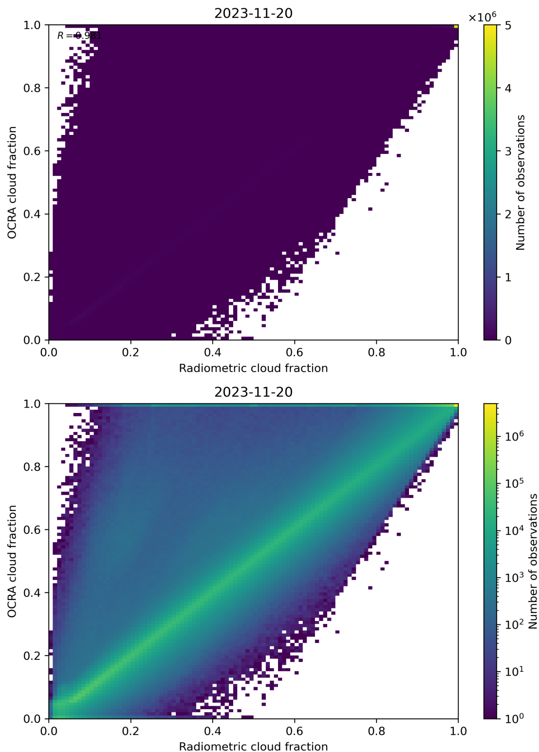
Figure 72: Scatter density plot of “Radiometric cloud fraction” against “OCRA cloud fraction” for 2023-11-19 to 2023-11-21.
