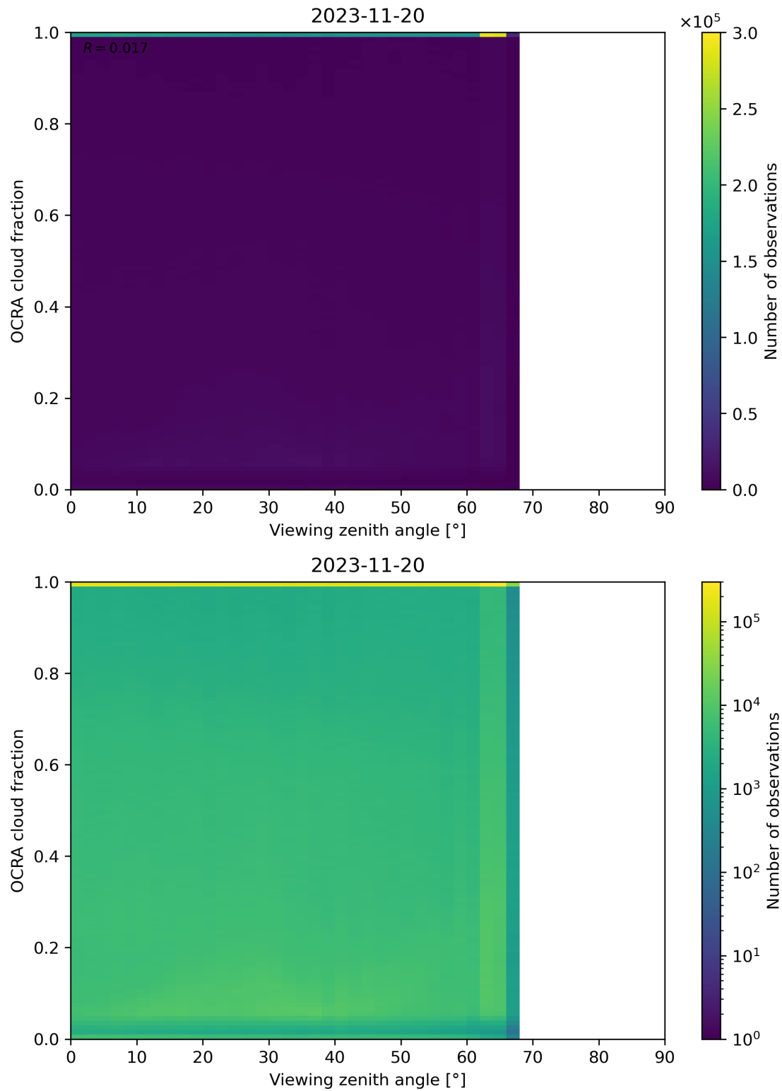
Figure 108: Scatter density plot of “Viewing zenith angle” against “OCRA cloud fraction” for 2023-11-19 to 2023-11-21.
