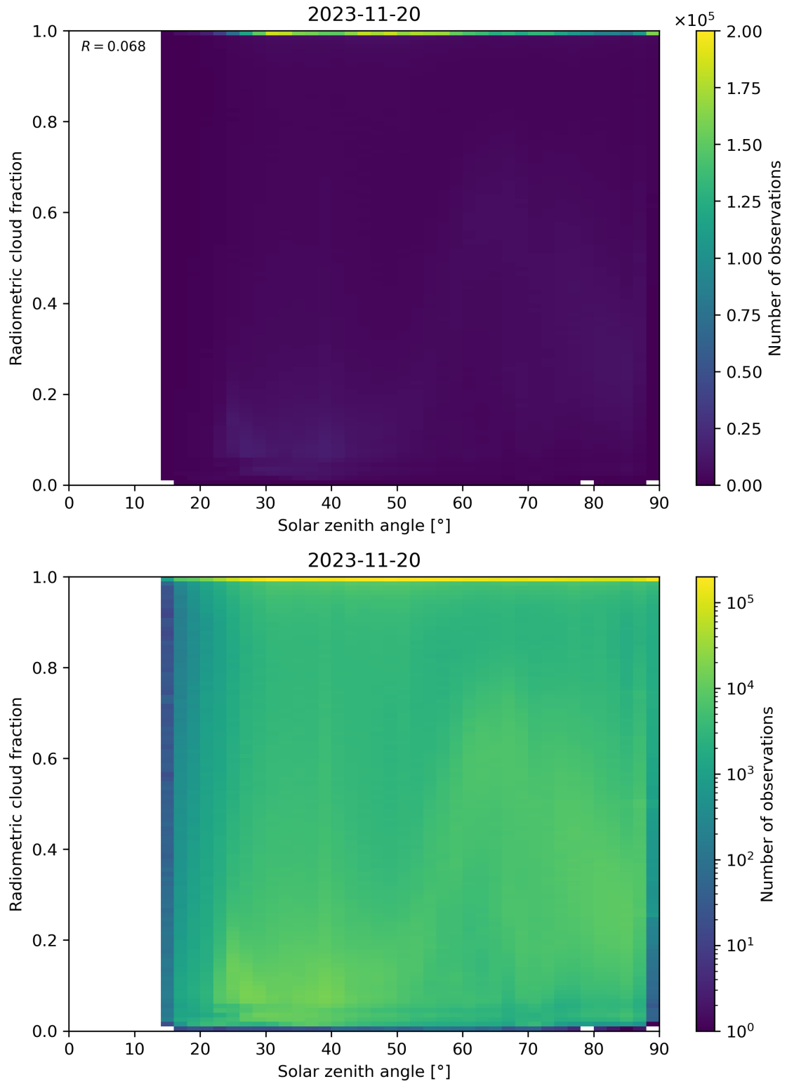
Figure 99: Scatter density plot of “Solar zenith angle” against “Radiometric cloud fraction” for 2023-11-19 to 2023-11-21.
