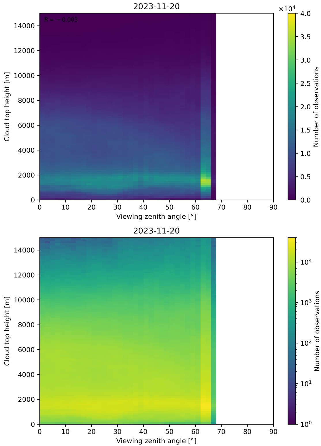
Figure 112: Scatter density plot of “Viewing zenith angle” against “Cloud top height” for 2023-11-19 to 2023-11-21.
