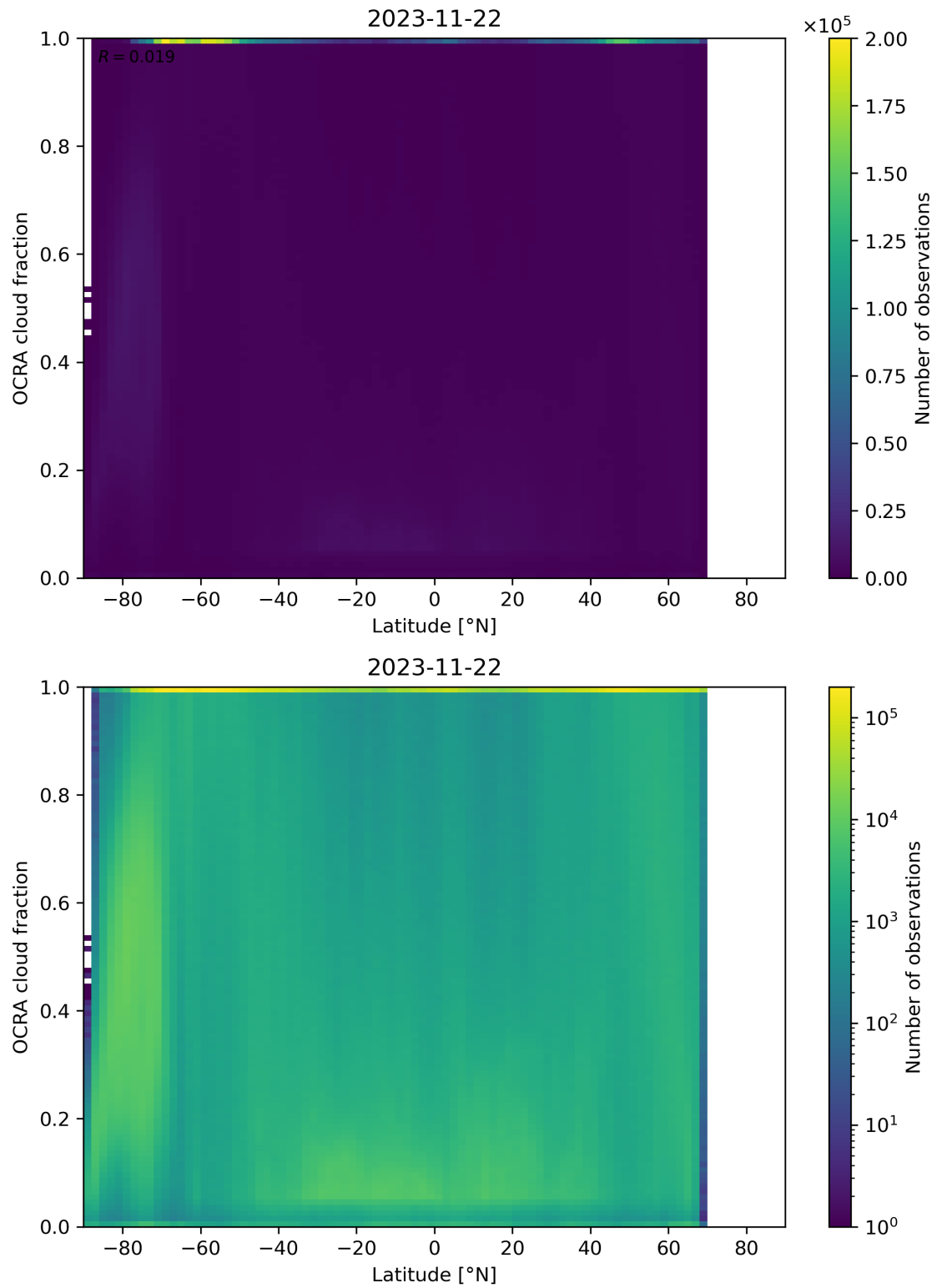
Figure 93: Scatter density plot of “Latitude” against “OCRA cloud fraction” for 2023-11-21 to 2023-11-23.
