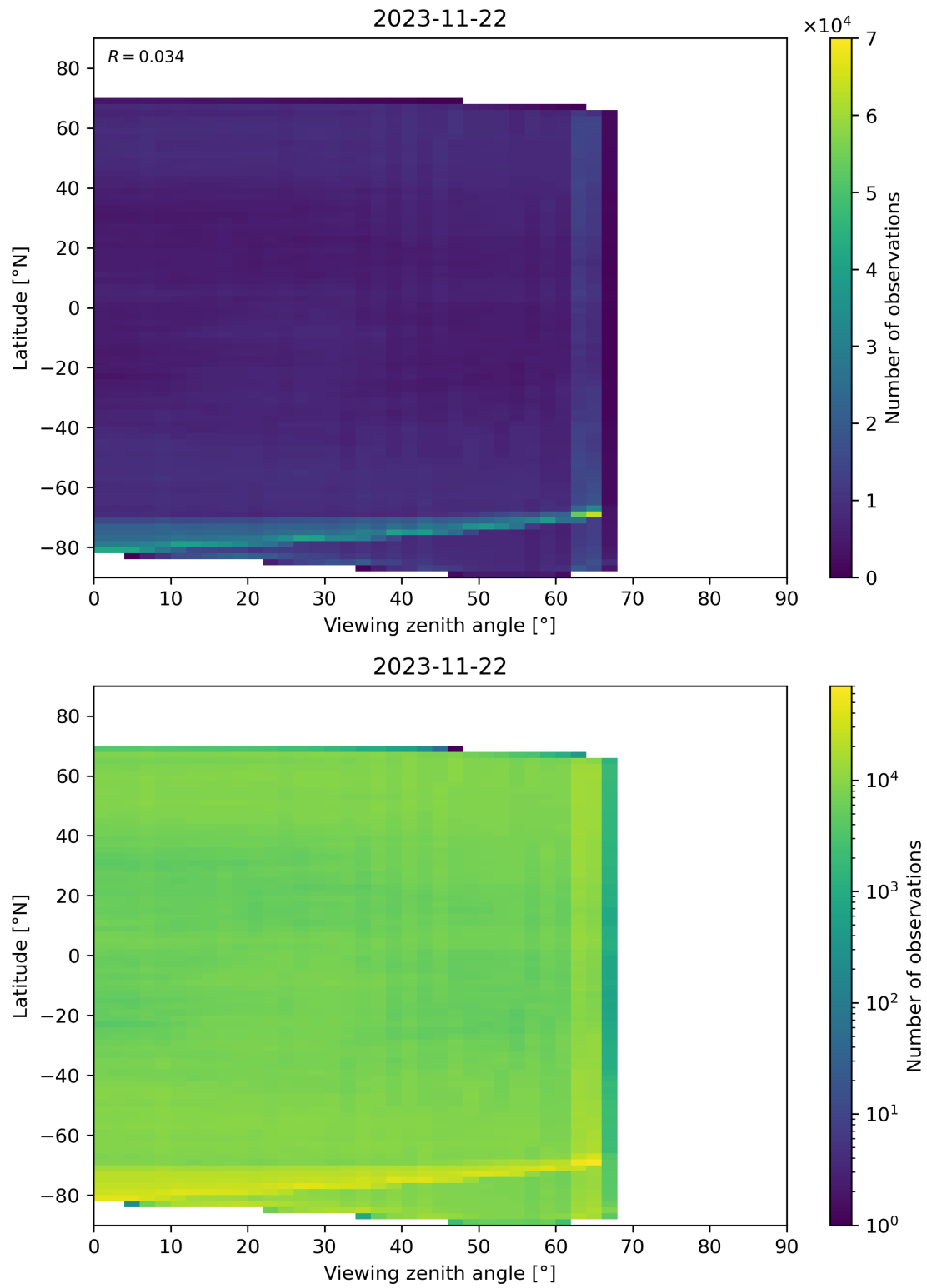
Figure 113: Scatter density plot of “Viewing zenith angle” against “Latitude” for 2023-11-21 to 2023-11-23.
