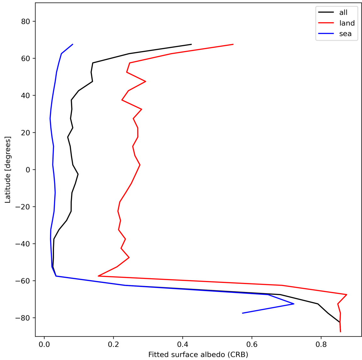
Figure 30: Zonal average of “Fitted surface albedo (CRB)” for 2023-11-21 to 2023-11-23.
