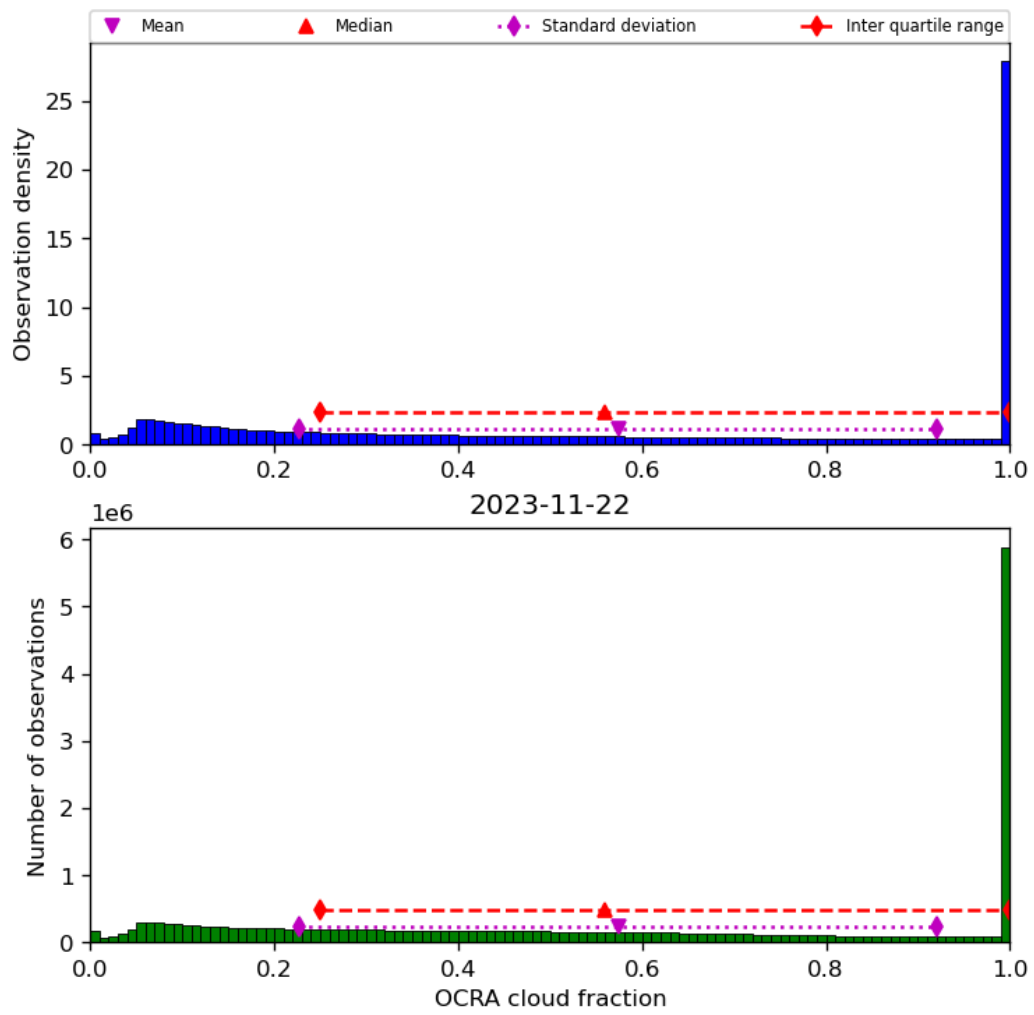
Figure 50: Histogram of “OCRA cloud fraction” for 2023-11-21 to 2023-11-23
