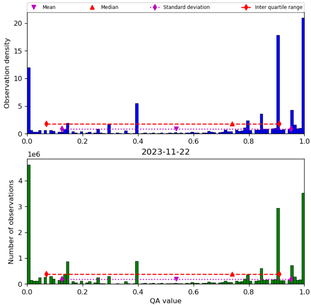
Figure 38: Histogram of “QA value” for 2023-11-21 to 2023-11-23
