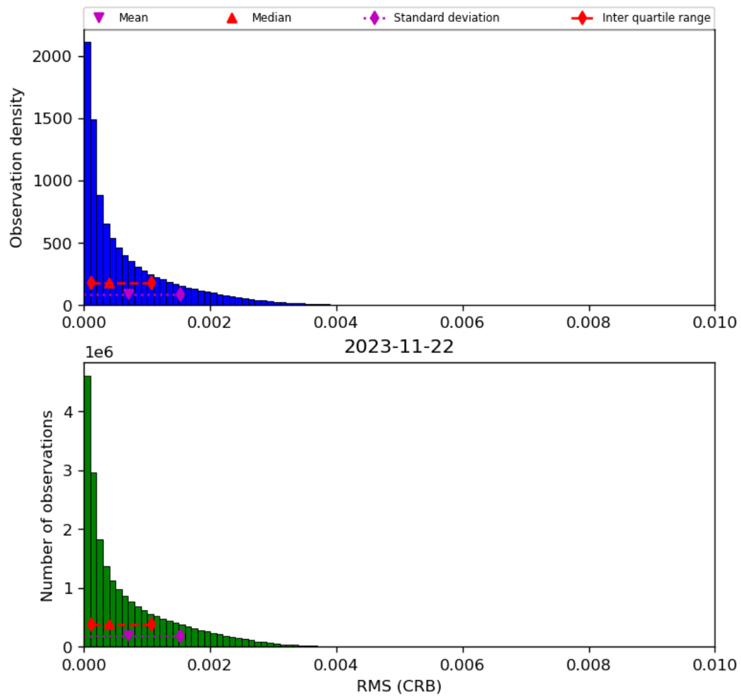
Figure 48: Histogram of “RMS (CRB)” for 2023-11-21 to 2023-11-23
