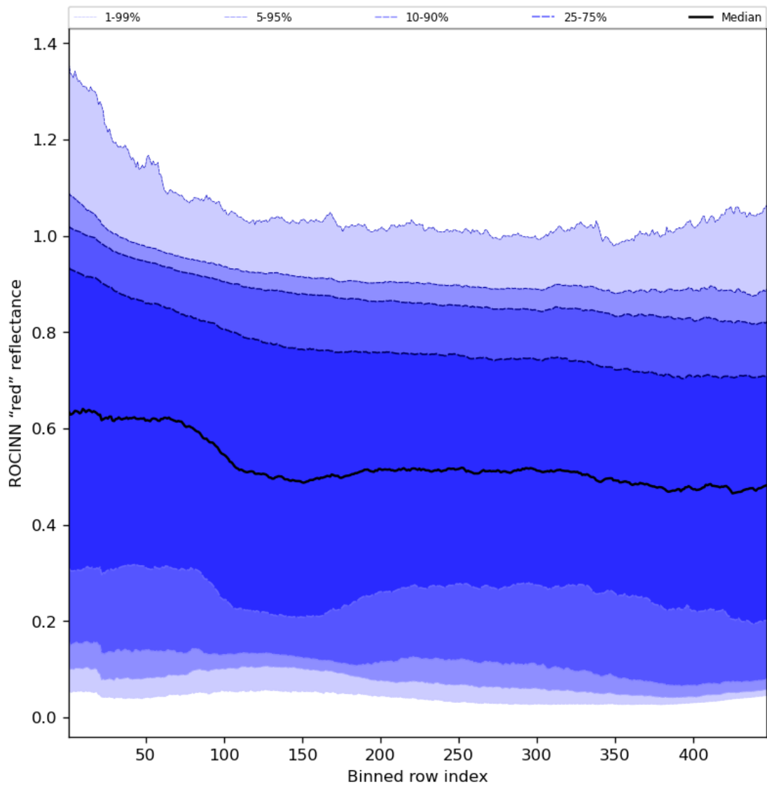
Figure 69: Along track statistics of “ROCINN “red” reflectance” for 2023-11-21 to 2023-11-23
