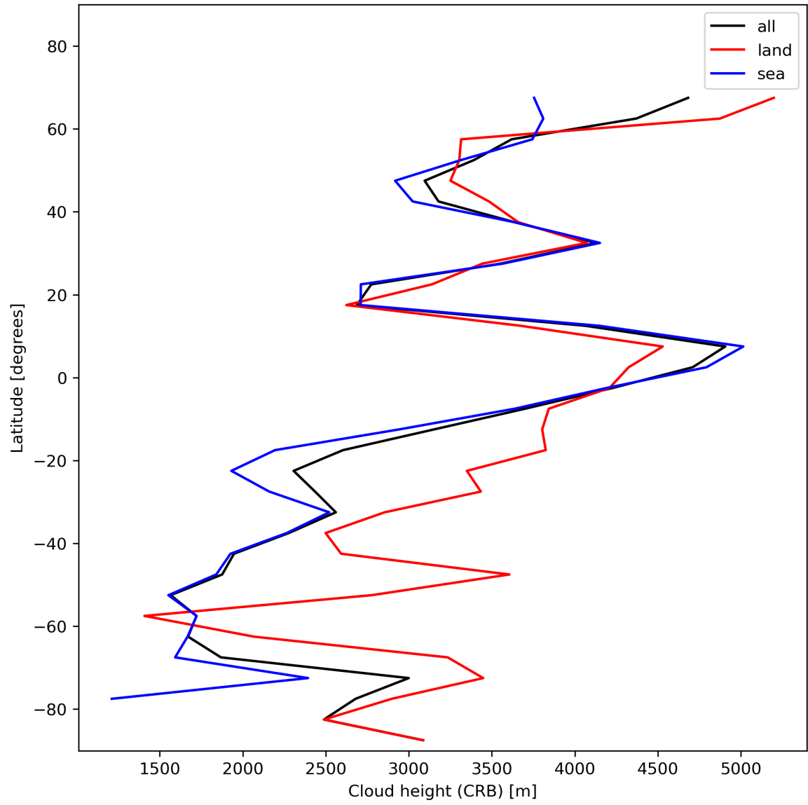
Figure 27: Zonal average of “Cloud height (CRB)” for 2023-11-21 to 2023-11-23.
