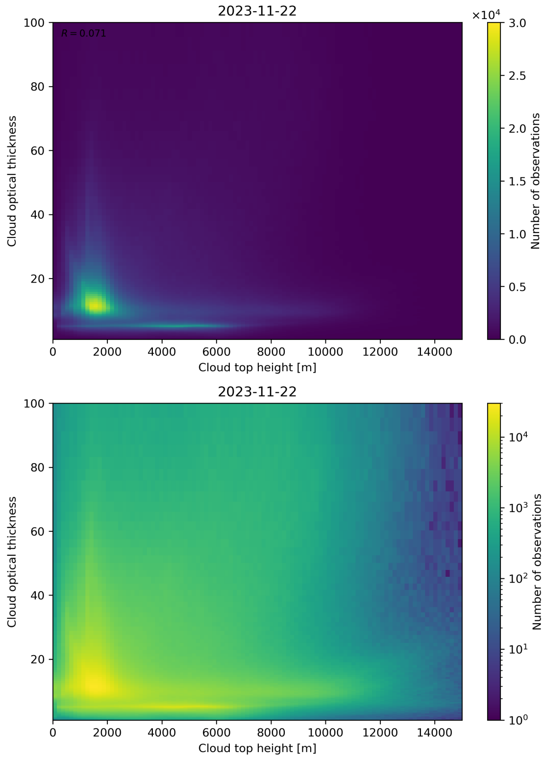
Figure 90: Scatter density plot of “Cloud top height” against “Cloud optical thickness” for 2023-11-21 to 2023-11-23.
