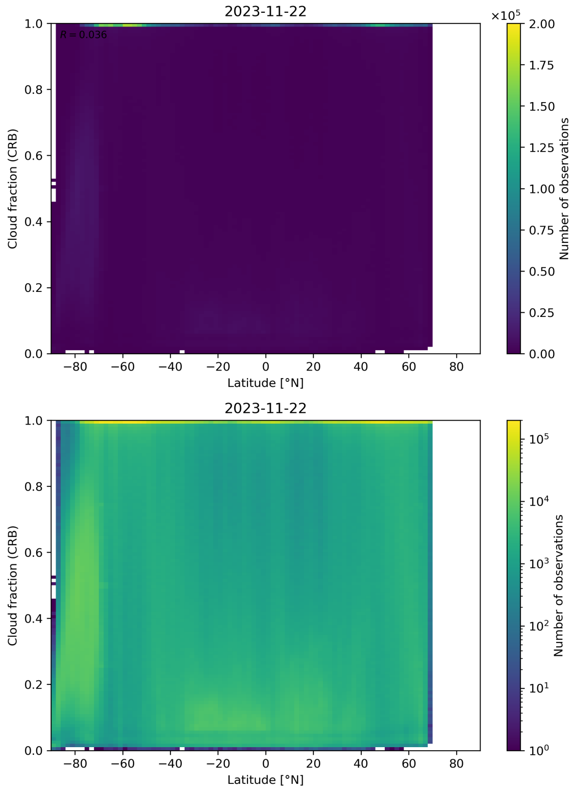
Figure 94: Scatter density plot of “Latitude” against “Cloud fraction (CRB)” for 2023-11-21 to 2023-11-23.
