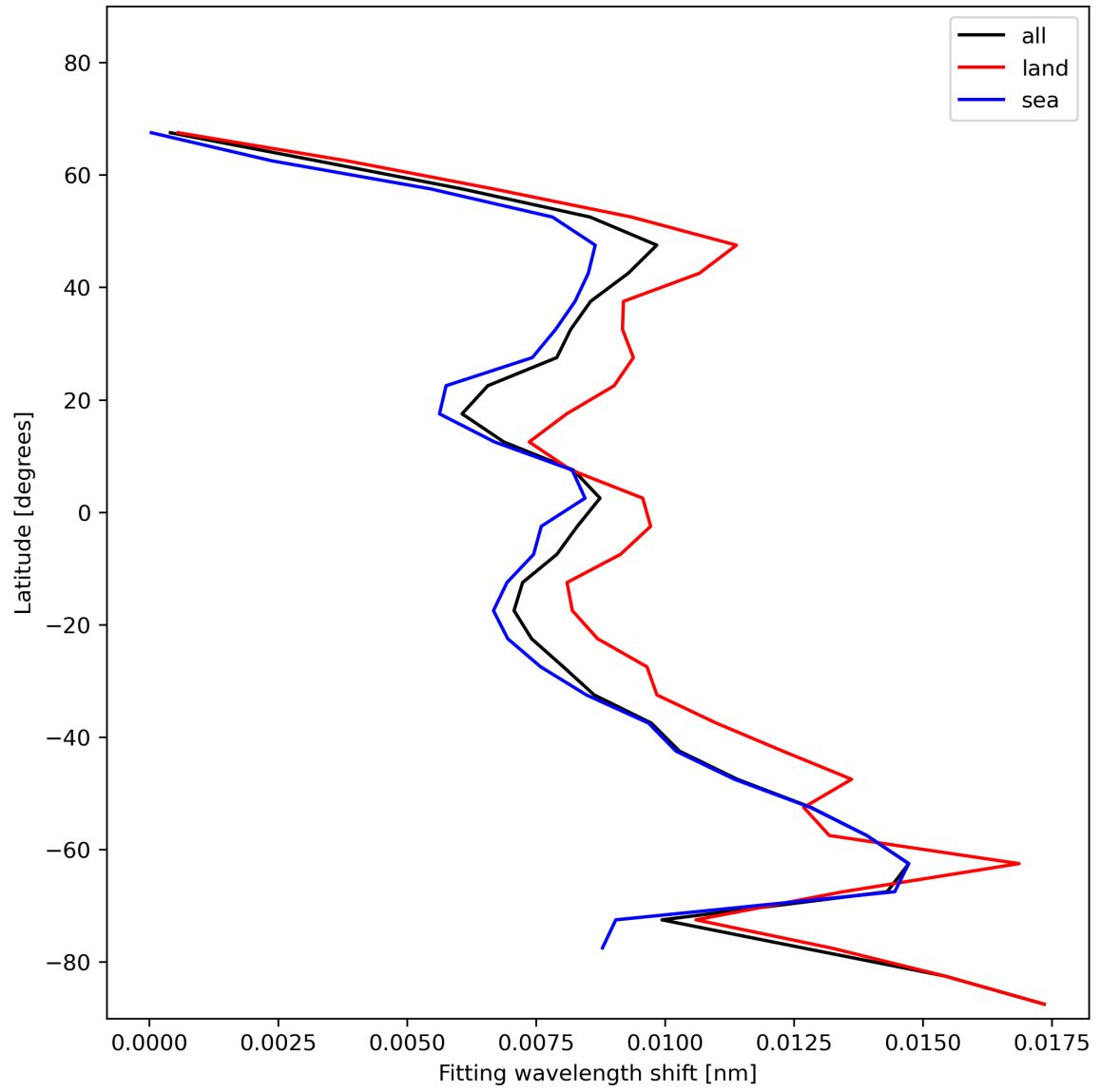
Figure 33: Zonal average of “Fitting wavelength shift” for 2023-11-21 to 2023-11-23.
