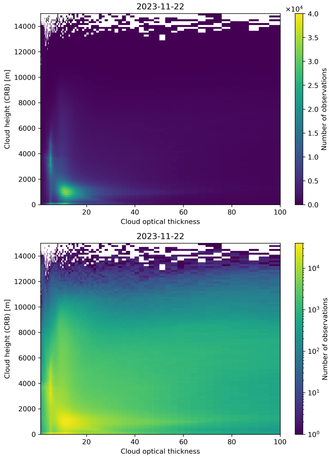
Figure 85: Scatter density plot of “Cloud optical thickness” against “Cloud height (CRB)” for 2023-11-21 to 2023-11-23.
