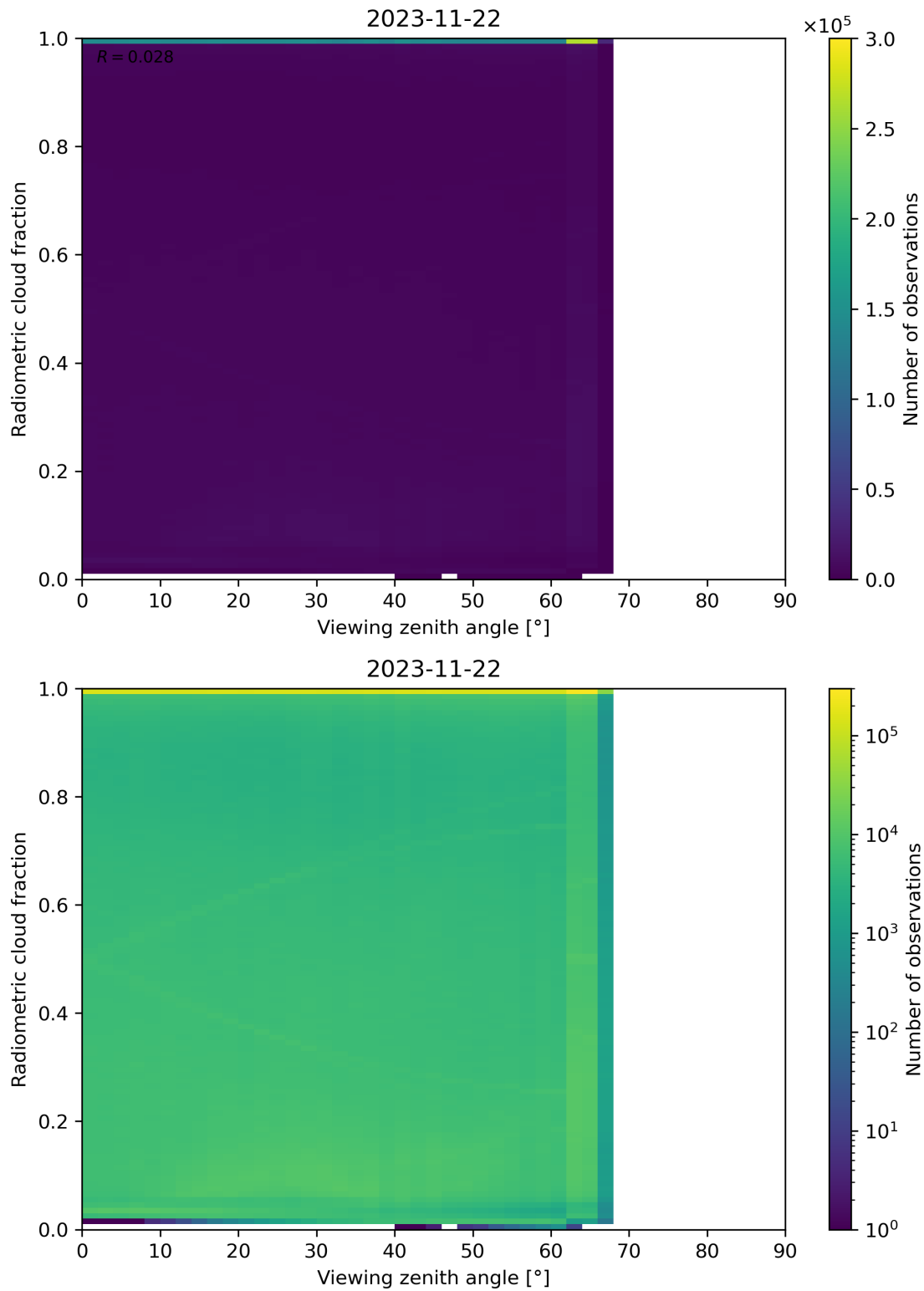
Figure 107: Scatter density plot of “Viewing zenith angle” against “Radiometric cloud fraction” for 2023-11-21 to 2023-11-23.
