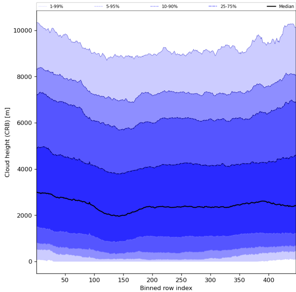
Figure 59: Along track statistics of “Cloud height (CRB)” for 2023-11-21 to 2023-11-23
