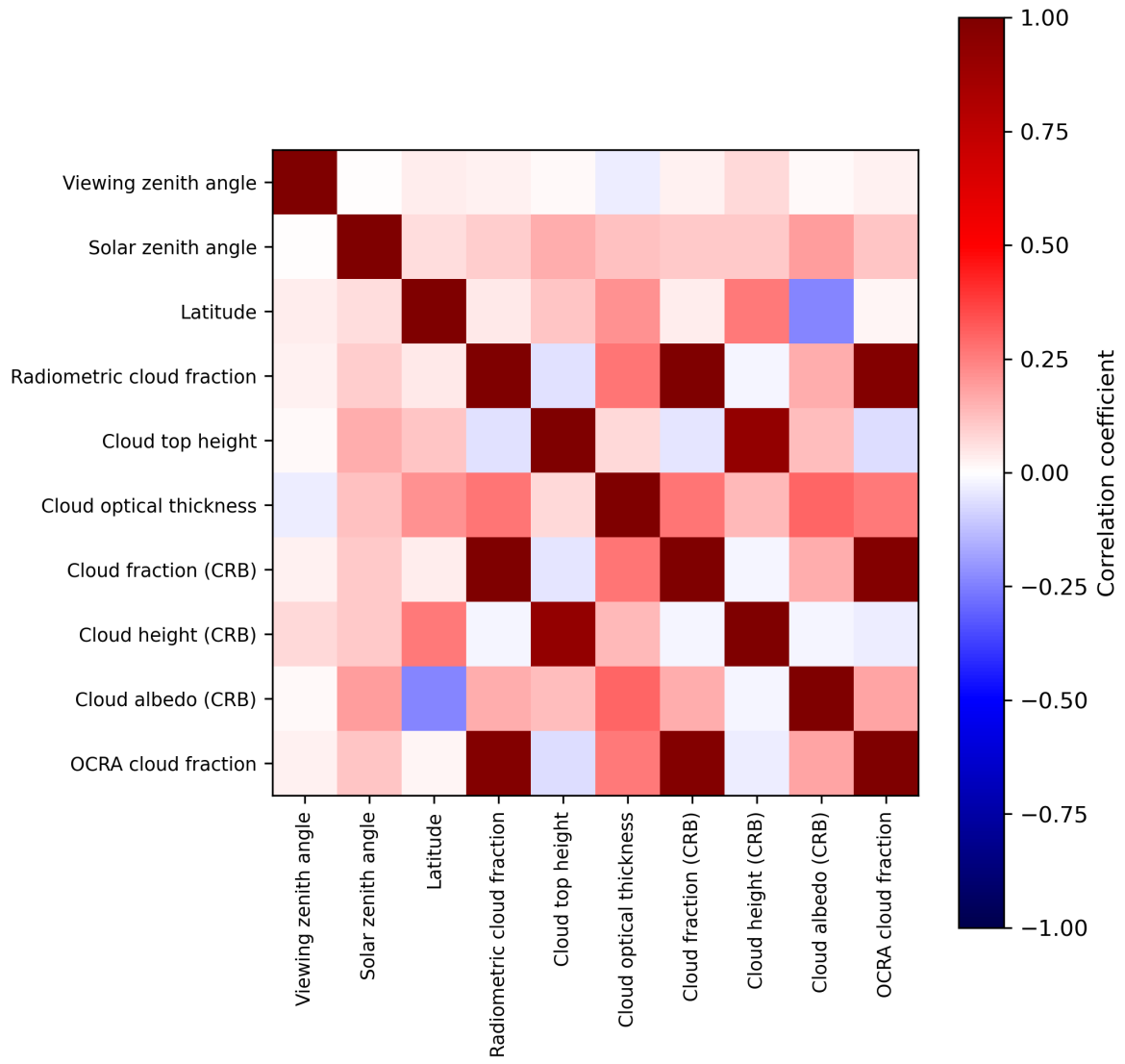
Figure 2: Map of correlation matrix for 2023-11-21 to 2023-11-23.
