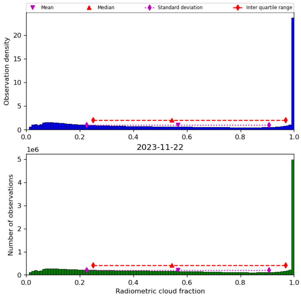
Figure 39: Histogram of “Radiometric cloud fraction” for 2023-11-21 to 2023-11-23
