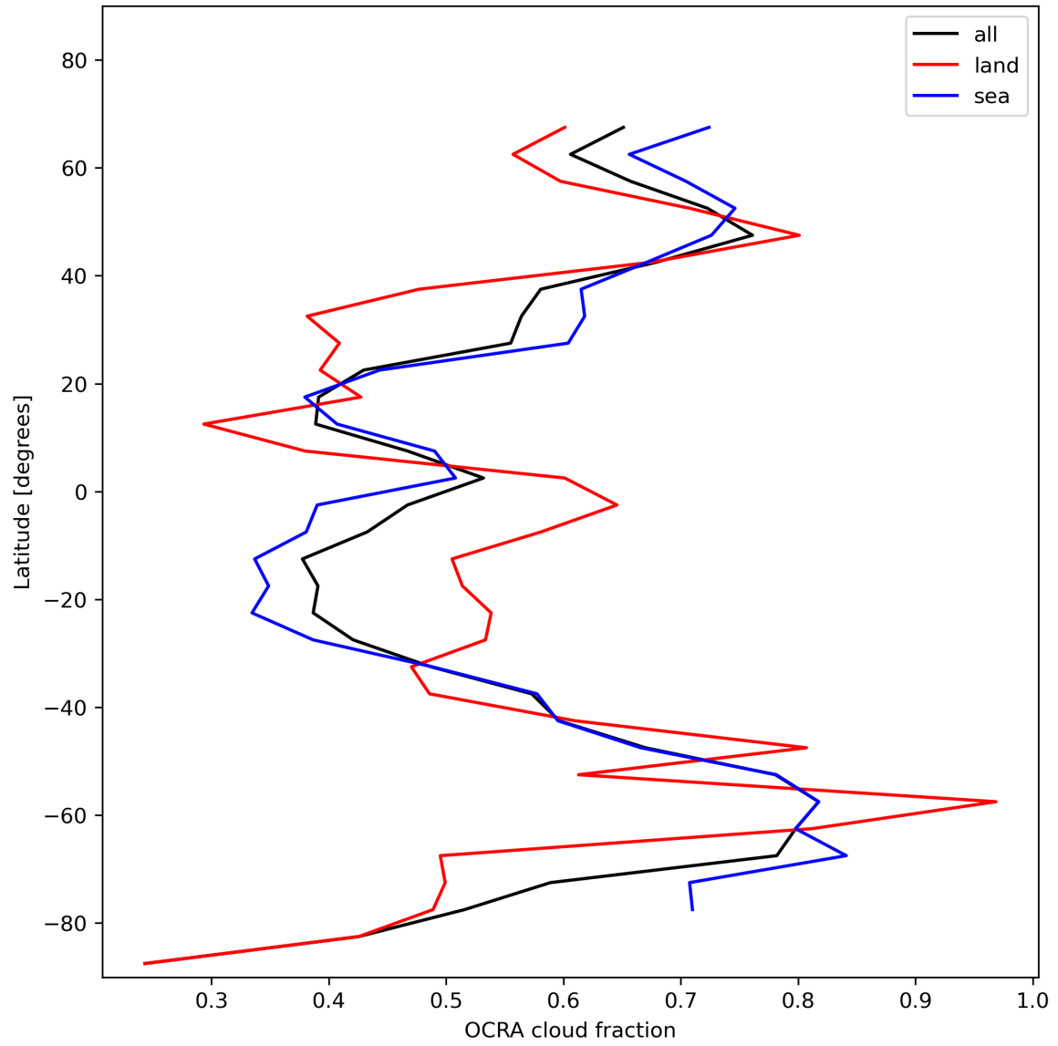
Figure 34: Zonal average of “OCRA cloud fraction” for 2023-11-21 to 2023-11-23.
