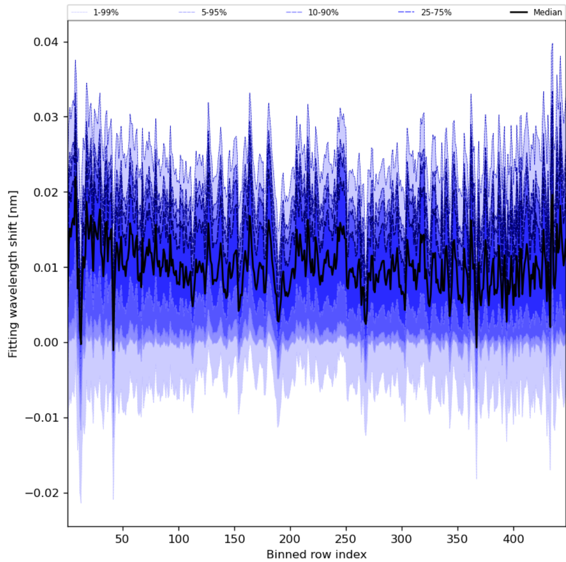
Figure 65: Along track statistics of “Fitting wavelength shift” for 2023-11-21 to 2023-11-23
