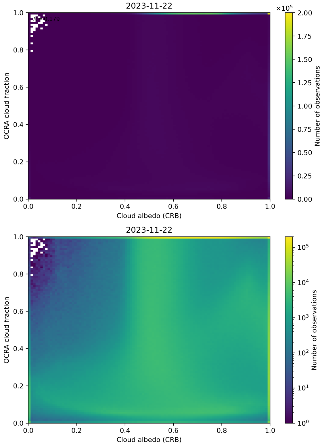
Figure 70: Scatter density plot of “Cloud albedo (CRB)” against “OCRA cloud fraction” for 2023-11-21 to 2023-11-23.
