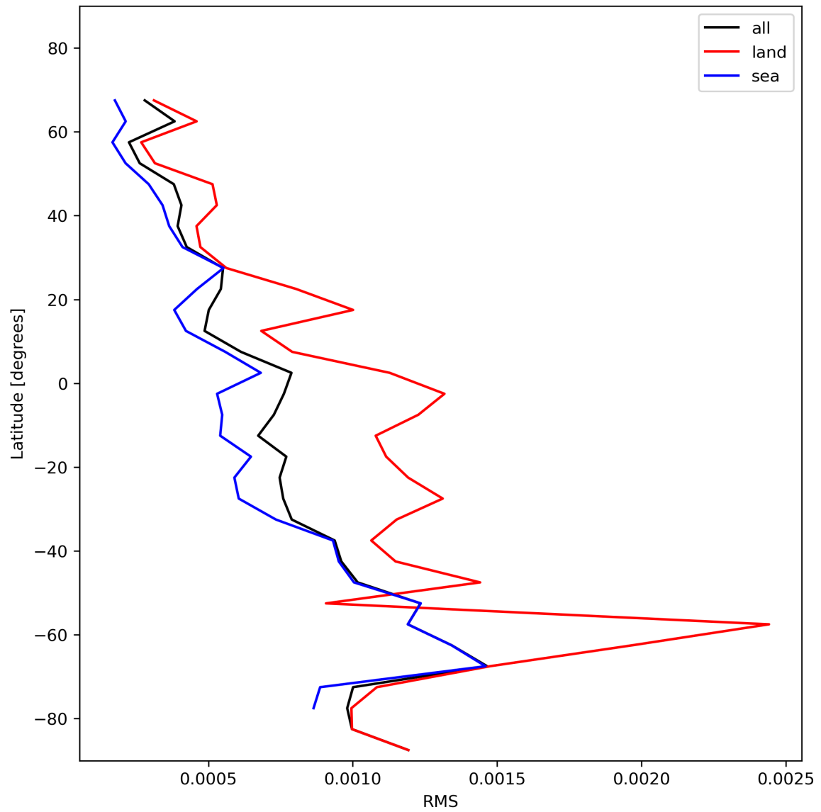
Figure 31: Zonal average of “RMS” for 2023-11-21 to 2023-11-23.
