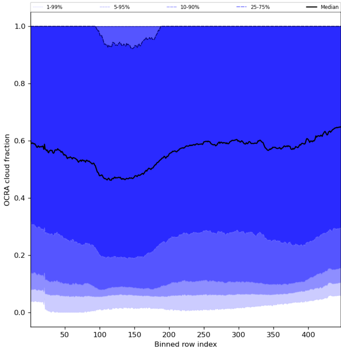
Figure 66: Along track statistics of “OCRA cloud fraction” for 2023-11-21 to 2023-11-23
