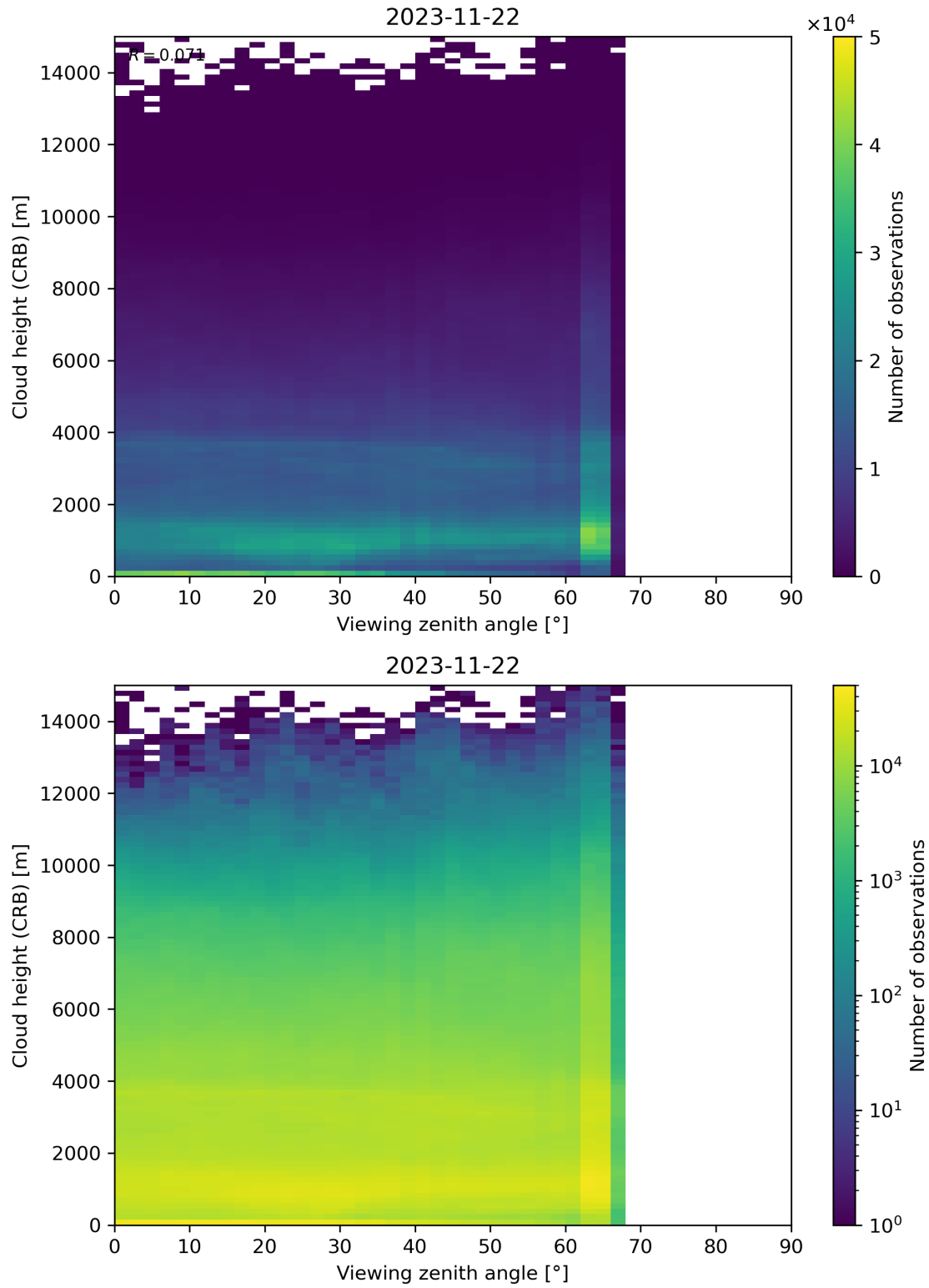
Figure 110: Scatter density plot of “Viewing zenith angle” against “Cloud height (CRB)” for 2023-11-21 to 2023-11-23.
