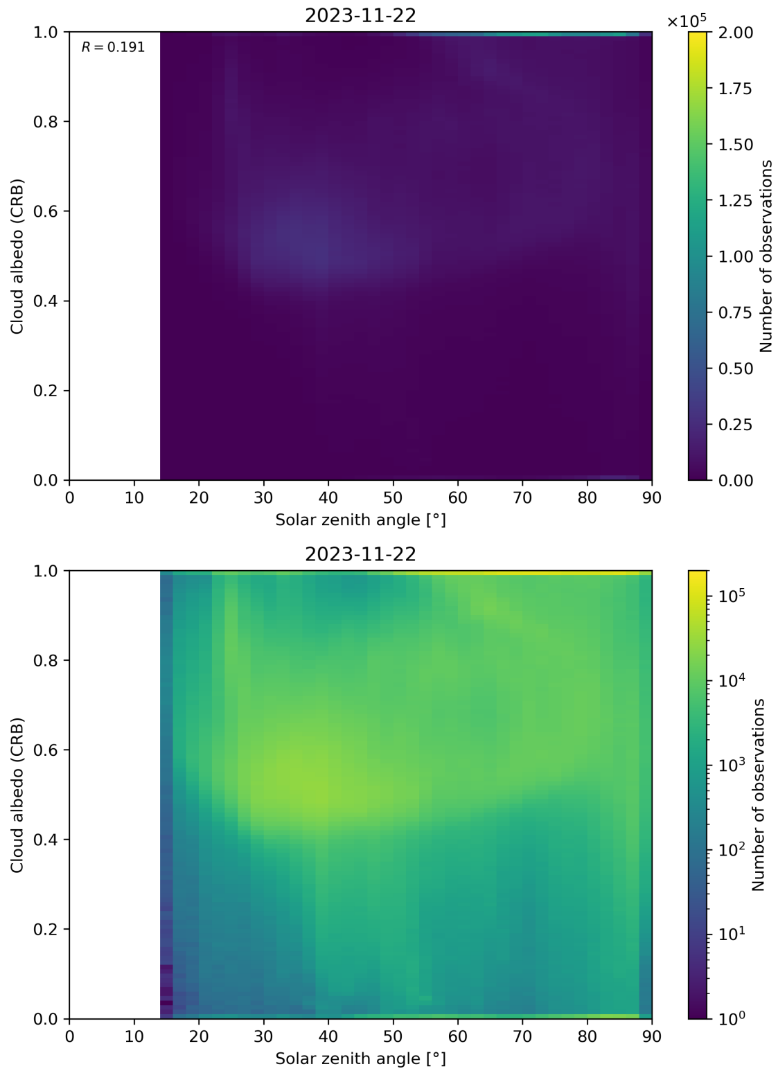
Figure 98: Scatter density plot of “Solar zenith angle” against “Cloud albedo (CRB)” for 2023-11-21 to 2023-11-23.
