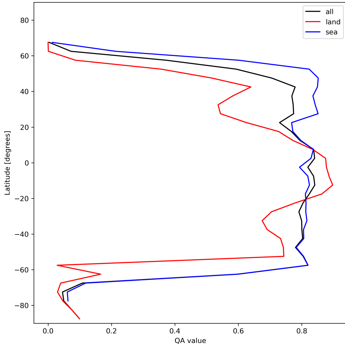
Figure 22: Zonal average of “QA value” for 2023-11-21 to 2023-11-23.
