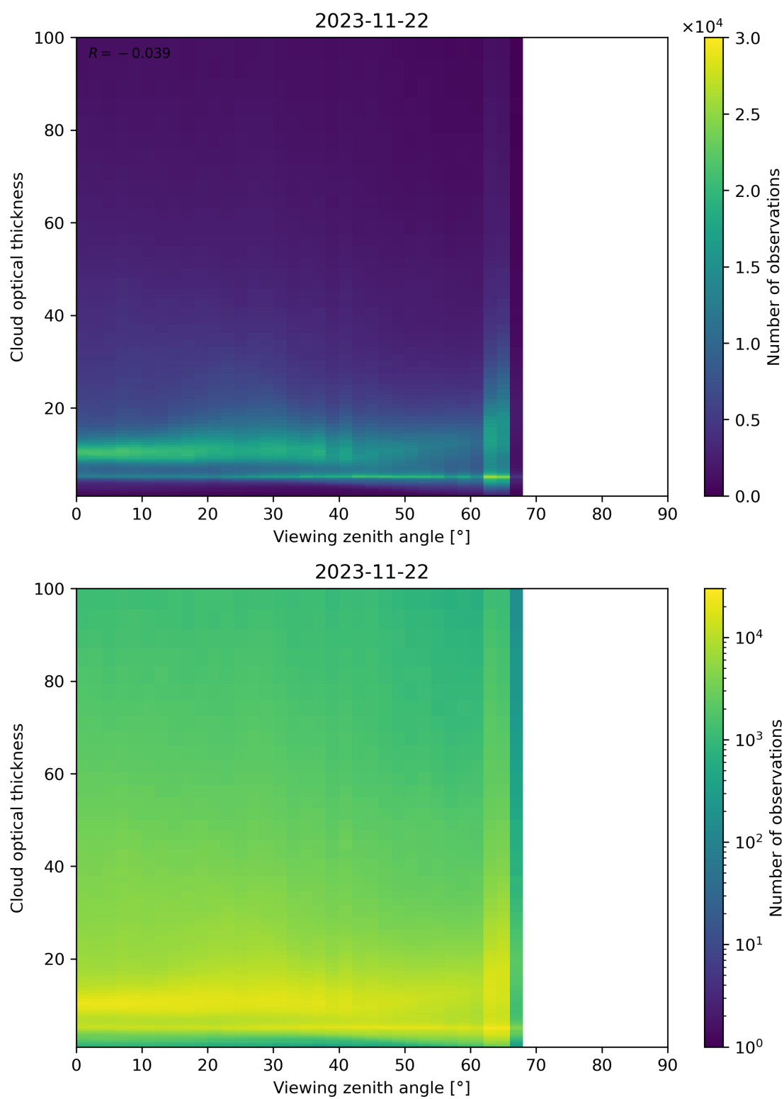
Figure 111: Scatter density plot of “Viewing zenith angle” against “Cloud optical thickness” for 2023-11-21 to 2023-11-23.
