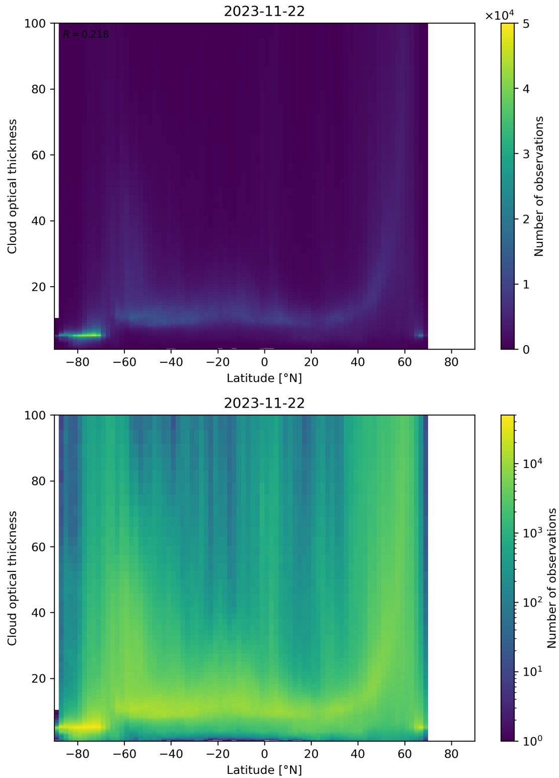
Figure 96: Scatter density plot of “Latitude” against “Cloud optical thickness” for 2023-11-21 to 2023-11-23.
