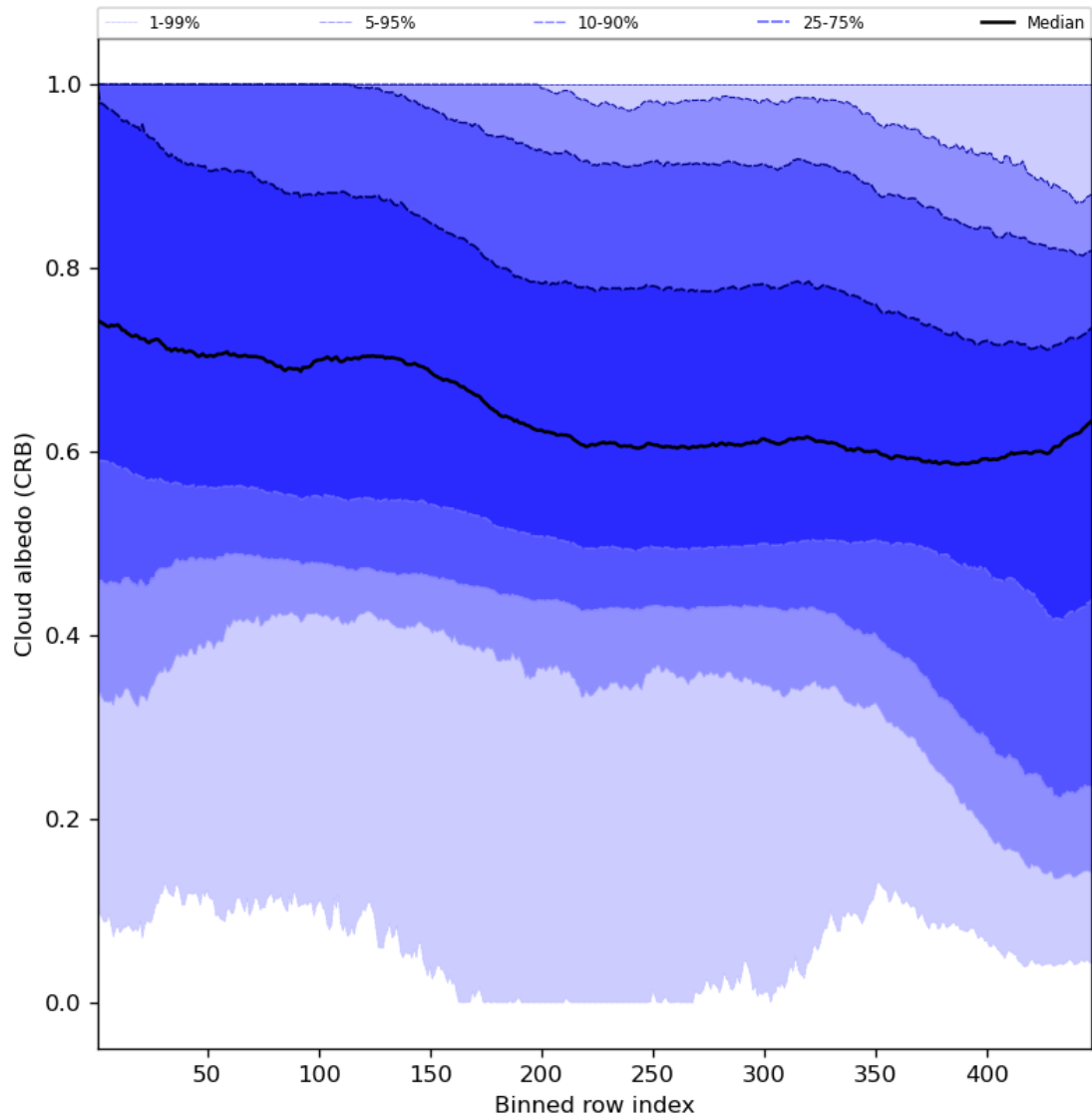
Figure 60: Along track statistics of “Cloud albedo (CRB)” for 2023-11-21 to 2023-11-23
