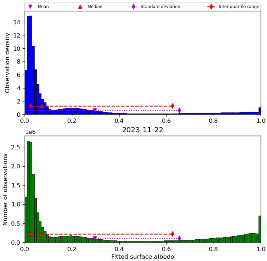
Figure 45: Histogram of “Fitted surface albedo” for 2023-11-21 to 2023-11-23
