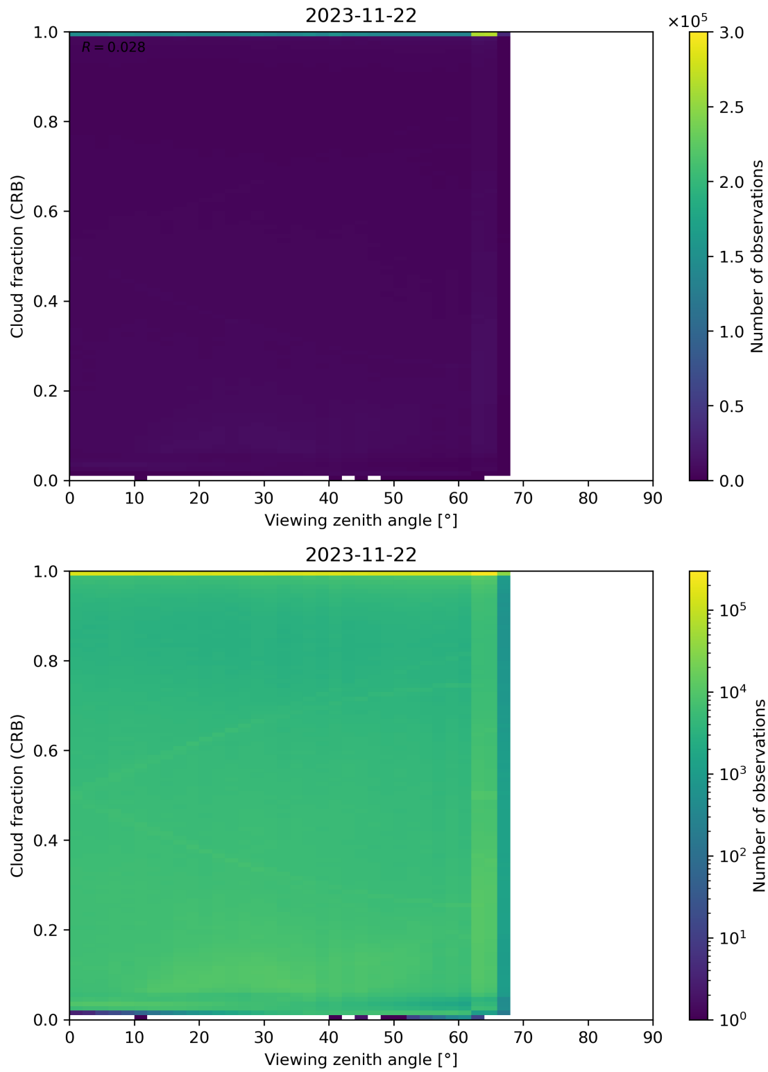
Figure 109: Scatter density plot of “Viewing zenith angle” against “Cloud fraction (CRB)” for 2023-11-21 to 2023-11-23.
