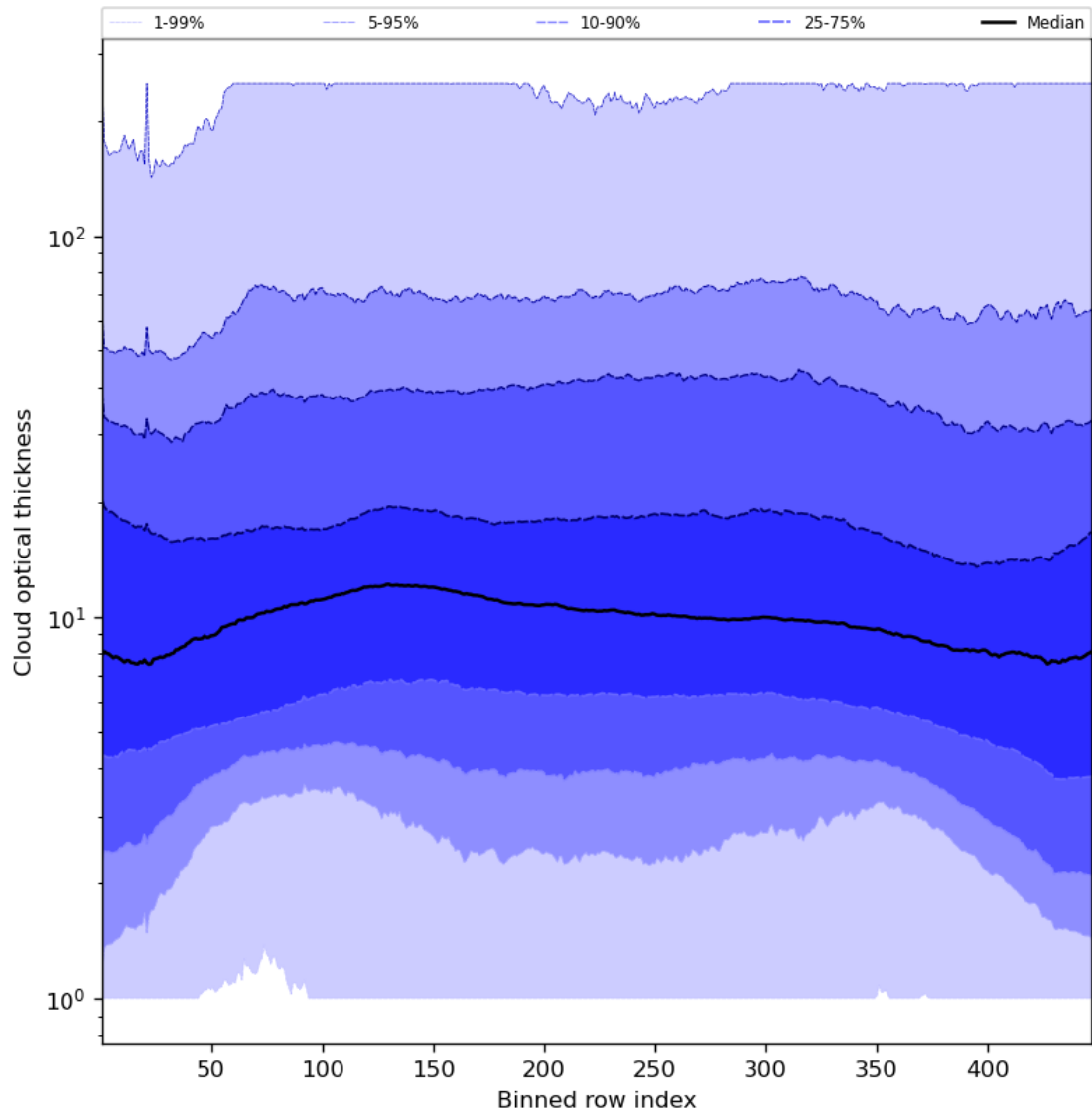
Figure 57: Along track statistics of “Cloud optical thickness” for 2023-11-21 to 2023-11-23
