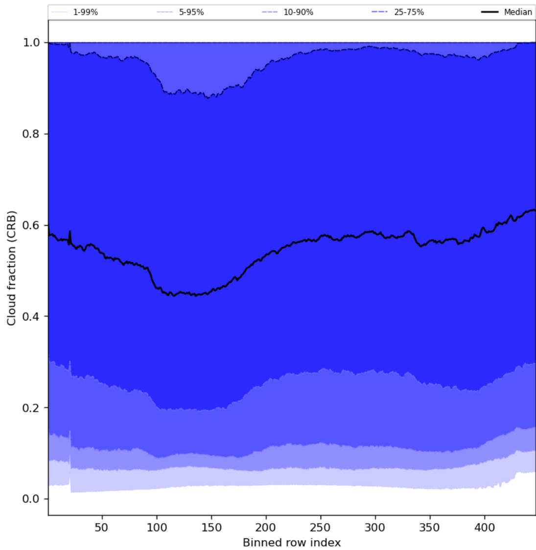
Figure 58: Along track statistics of “Cloud fraction (CRB)” for 2023-11-21 to 2023-11-23
