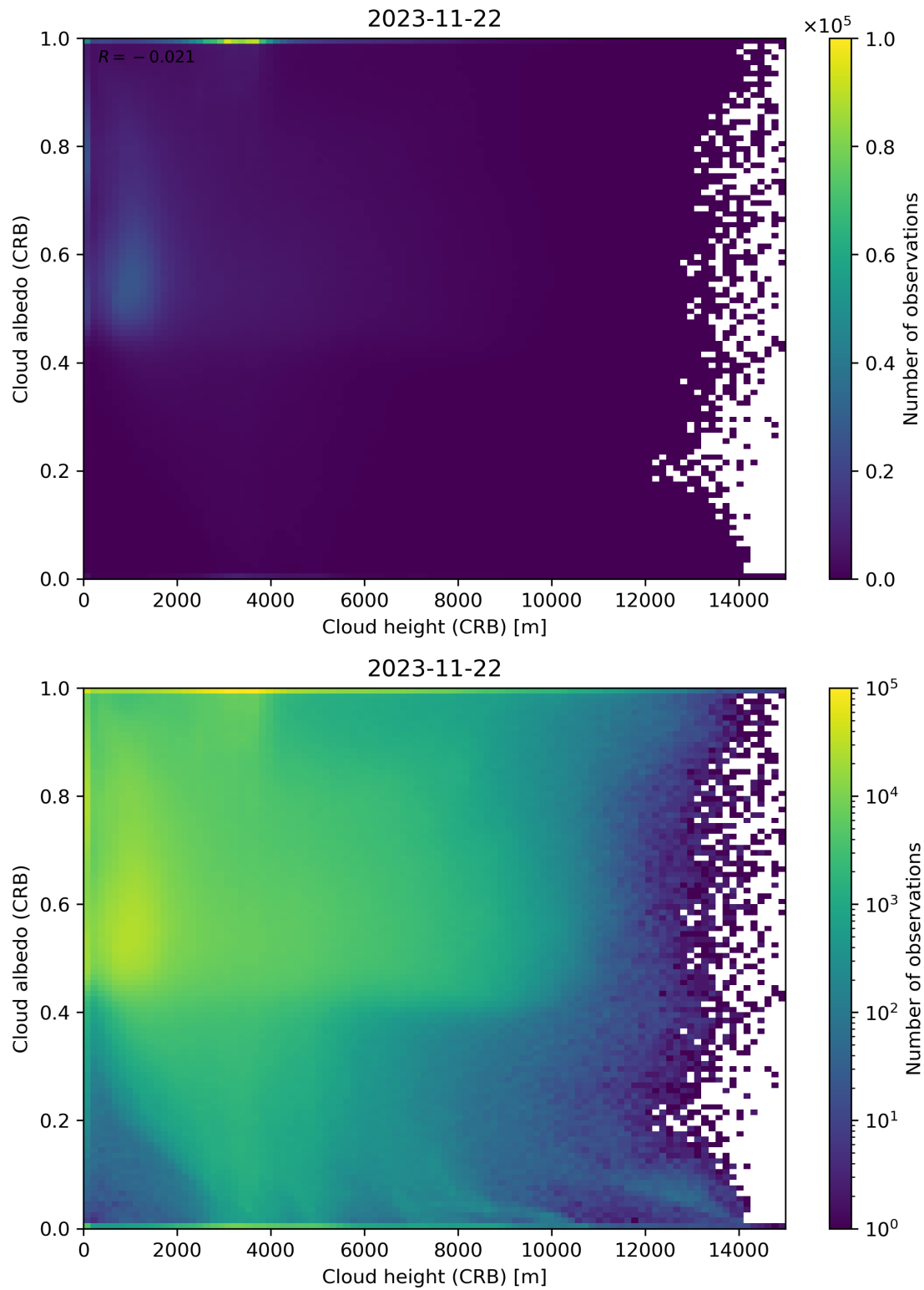
Figure 80: Scatter density plot of “Cloud height (CRB)” against “Cloud albedo (CRB)” for 2023-11-21 to 2023-11-23.
