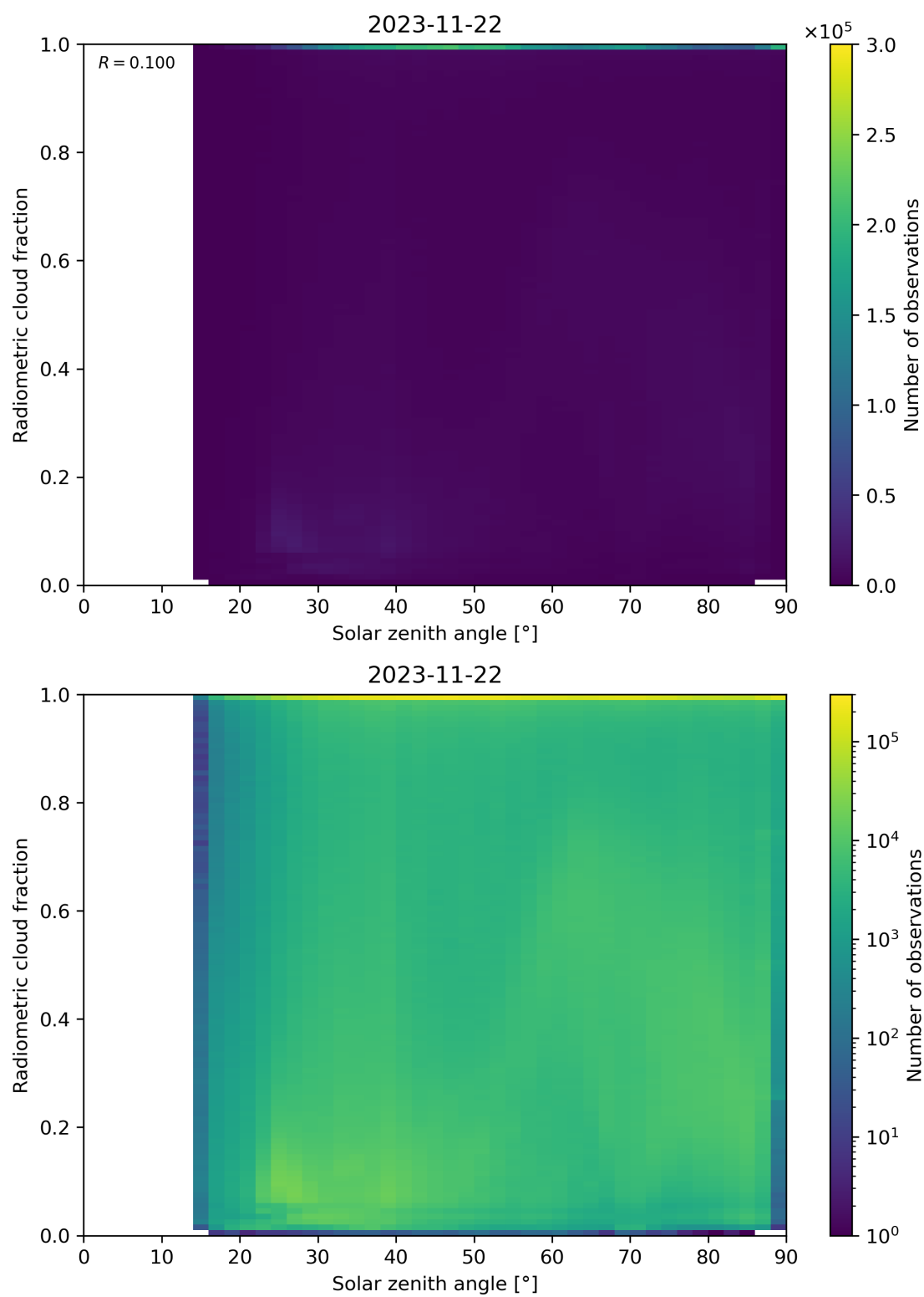
Figure 99: Scatter density plot of “Solar zenith angle” against “Radiometric cloud fraction” for 2023-11-21 to 2023-11-23.
