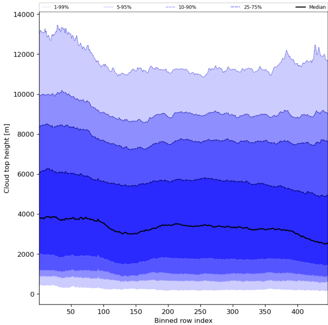
Figure 56: Along track statistics of “Cloud top height” for 2023-11-21 to 2023-11-23
