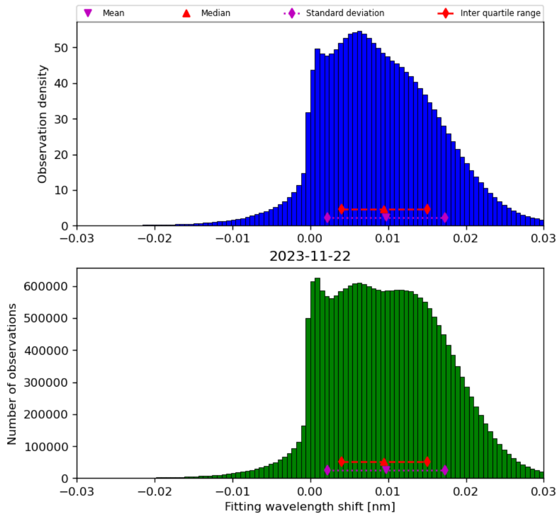
Figure 49: Histogram of “Fitting wavelength shift” for 2023-11-21 to 2023-11-23
