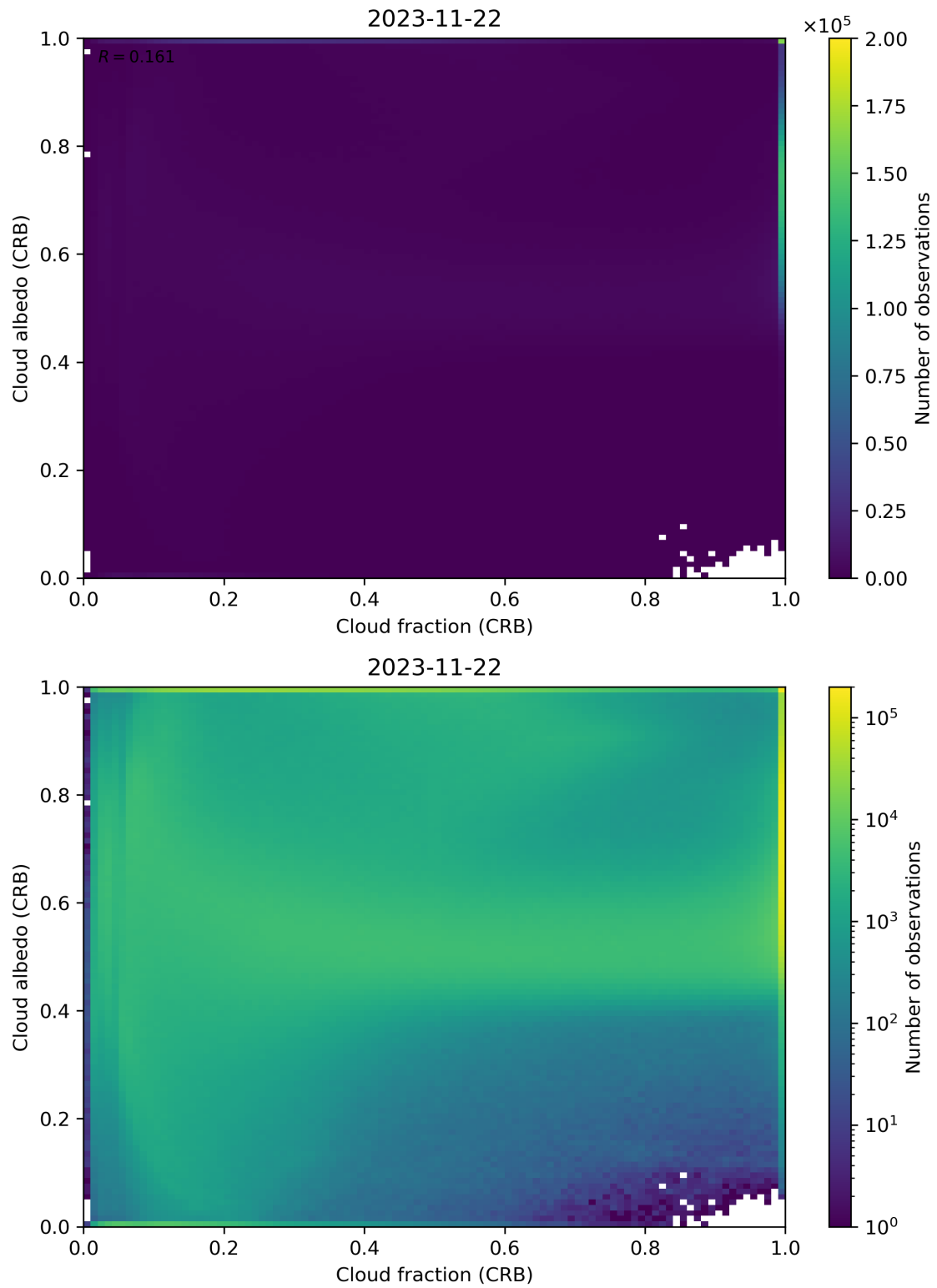
Figure 77: Scatter density plot of “Cloud fraction (CRB)” against “Cloud albedo (CRB)” for 2023-11-21 to 2023-11-23.
