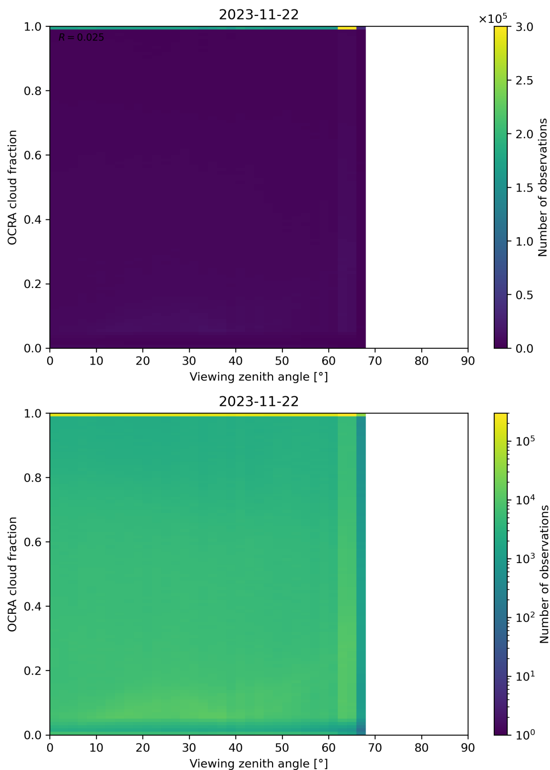
Figure 108: Scatter density plot of “Viewing zenith angle” against “OCRA cloud fraction” for 2023-11-21 to 2023-11-23.
