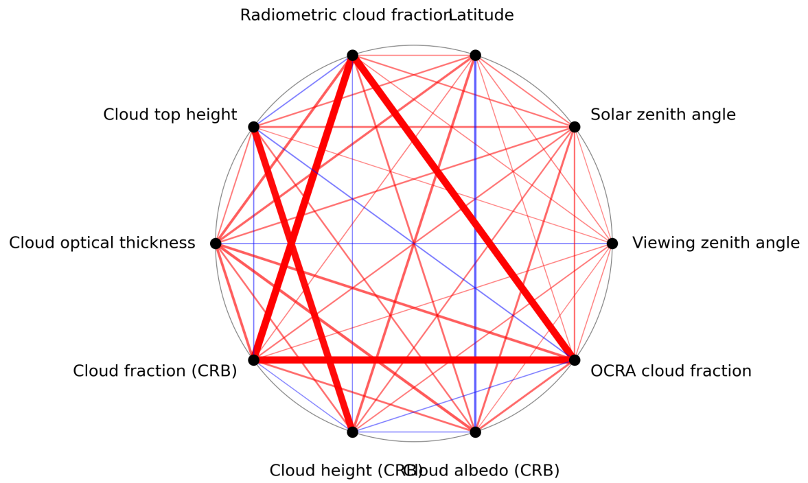
Figure 1: Map of correlation graph for 2023-11-21 to 2023-11-23.
