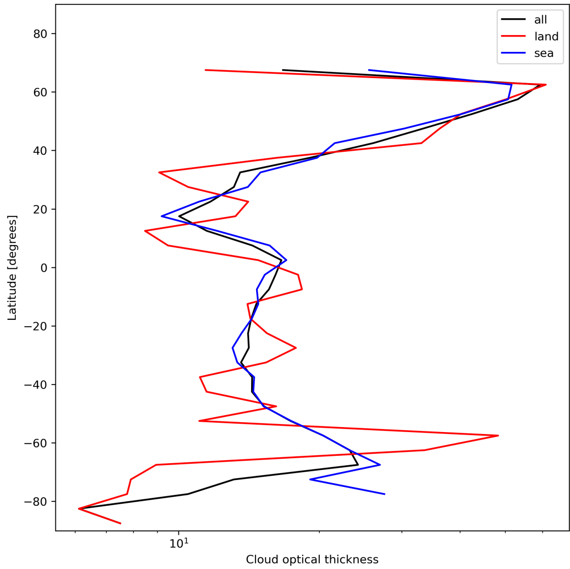
Figure 25: Zonal average of “Cloud optical thickness” for 2023-11-21 to 2023-11-23.
