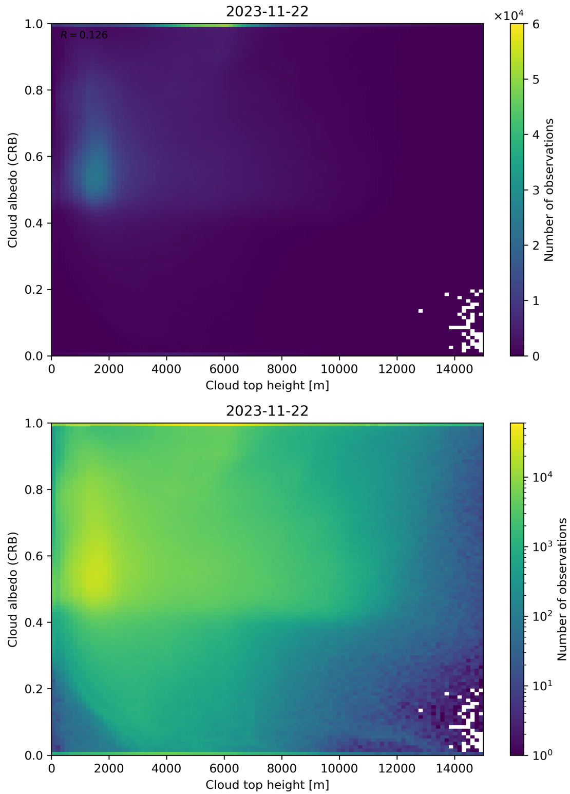
Figure 86: Scatter density plot of “Cloud top height” against “Cloud albedo (CRB)” for 2023-11-21 to 2023-11-23.
