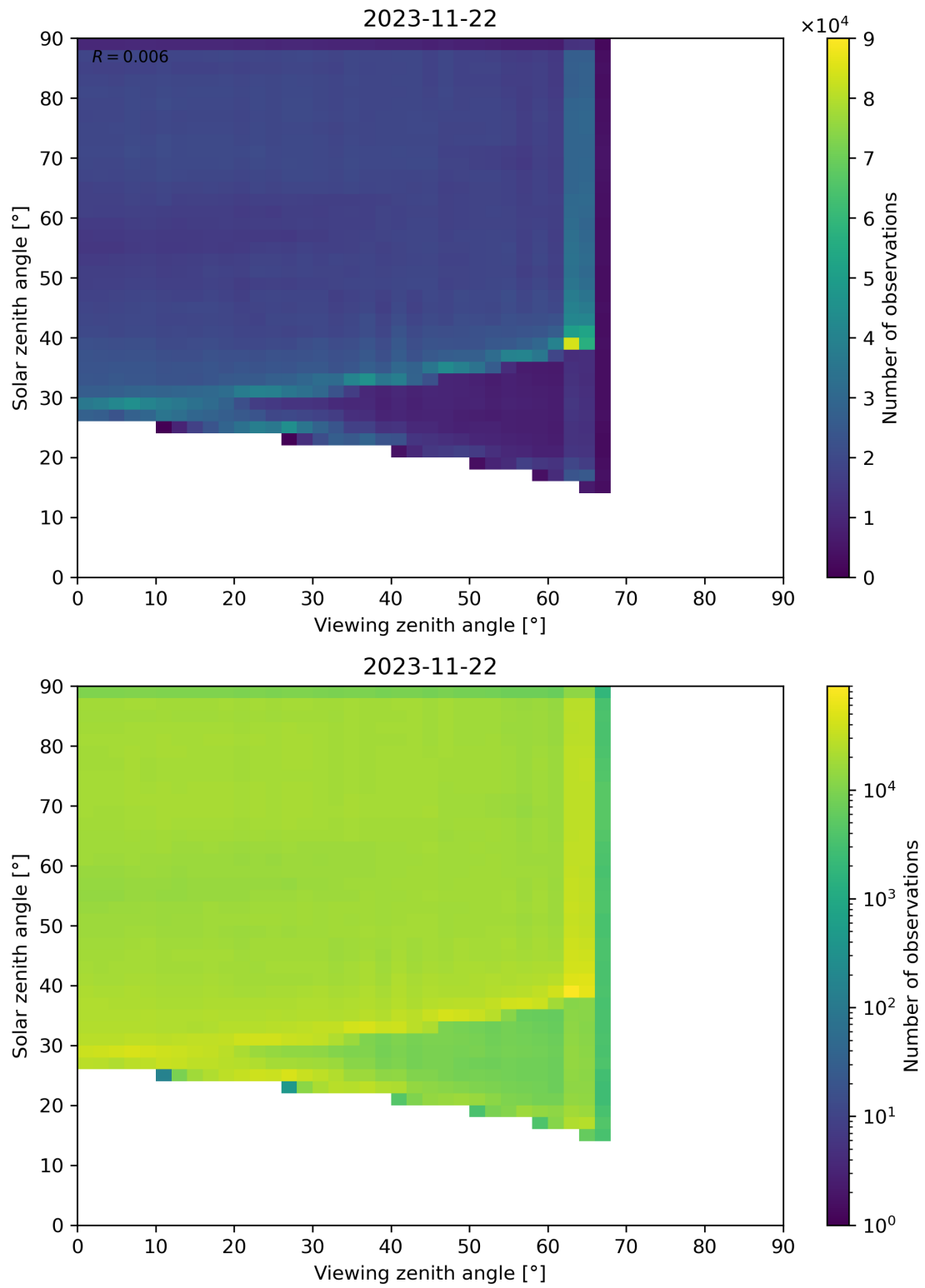
Figure 114: Scatter density plot of “Viewing zenith angle” against “Solar zenith angle” for 2023-11-21 to 2023-11-23.
