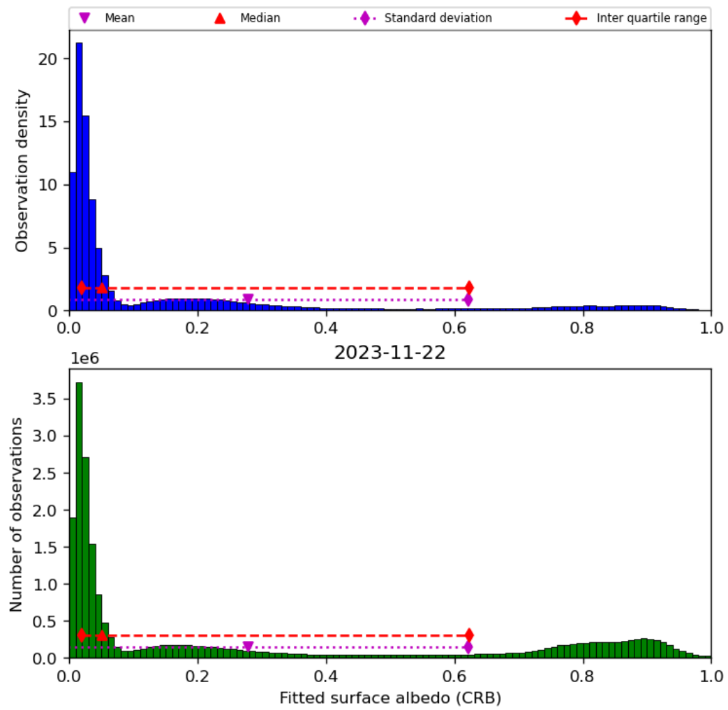
Figure 46: Histogram of “Fitted surface albedo (CRB)” for 2023-11-21 to 2023-11-23
