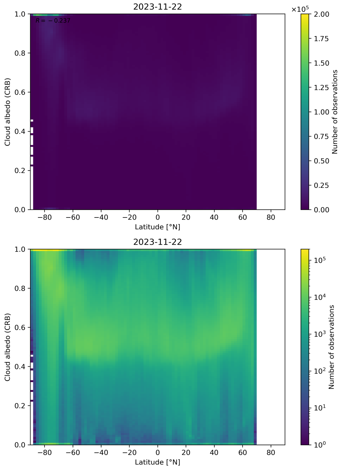
Figure 91: Scatter density plot of “Latitude” against “Cloud albedo (CRB)” for 2023-11-21 to 2023-11-23.
