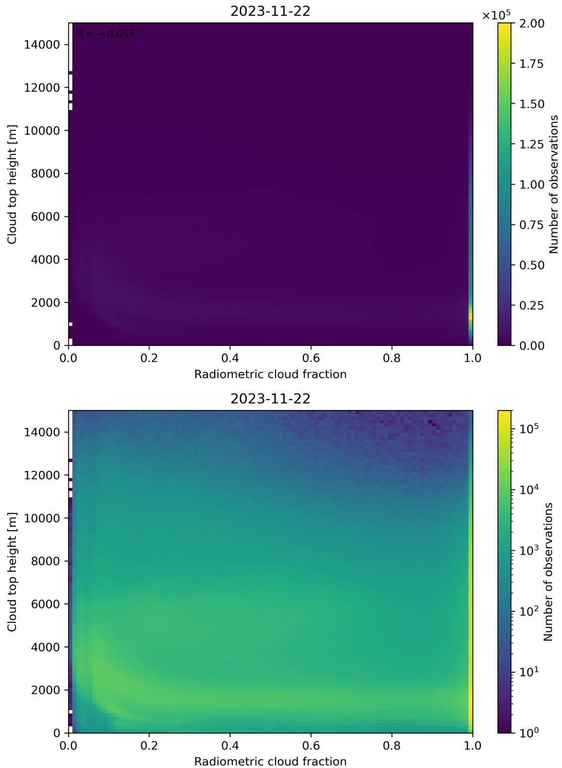
Figure 76: Scatter density plot of “Radiometric cloud fraction” against “Cloud top height” for 2023-11-21 to 2023-11-23.
