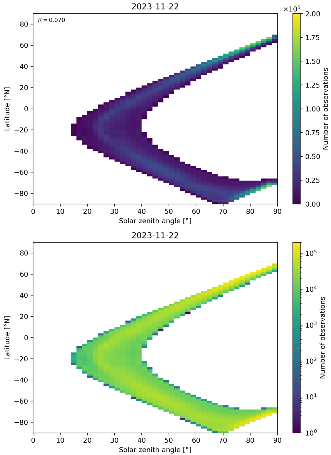
Figure 105: Scatter density plot of “Solar zenith angle” against “Latitude” for 2023-11-21 to 2023-11-23.
