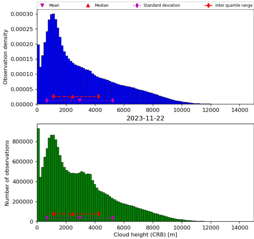
Figure 43: Histogram of “Cloud height (CRB)” for 2023-11-21 to 2023-11-23
