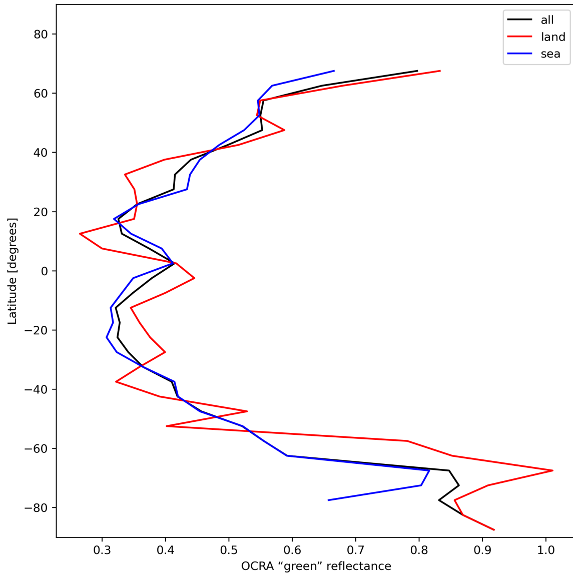
Figure 36: Zonal average of “OCRA “green” reflectance” for 2023-11-21 to 2023-11-23.
