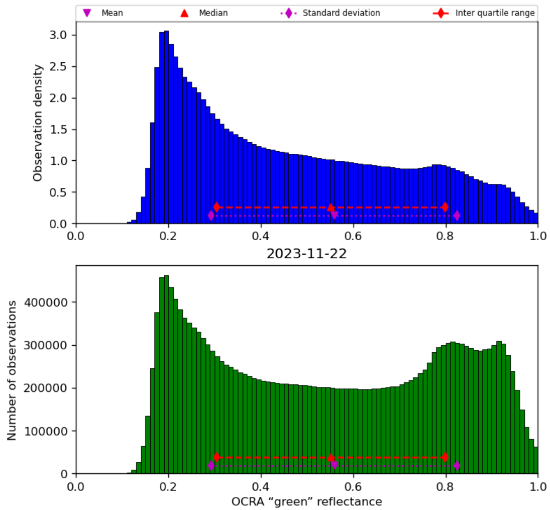
Figure 52: Histogram of “OCRA “green” reflectance” for 2023-11-21 to 2023-11-23
