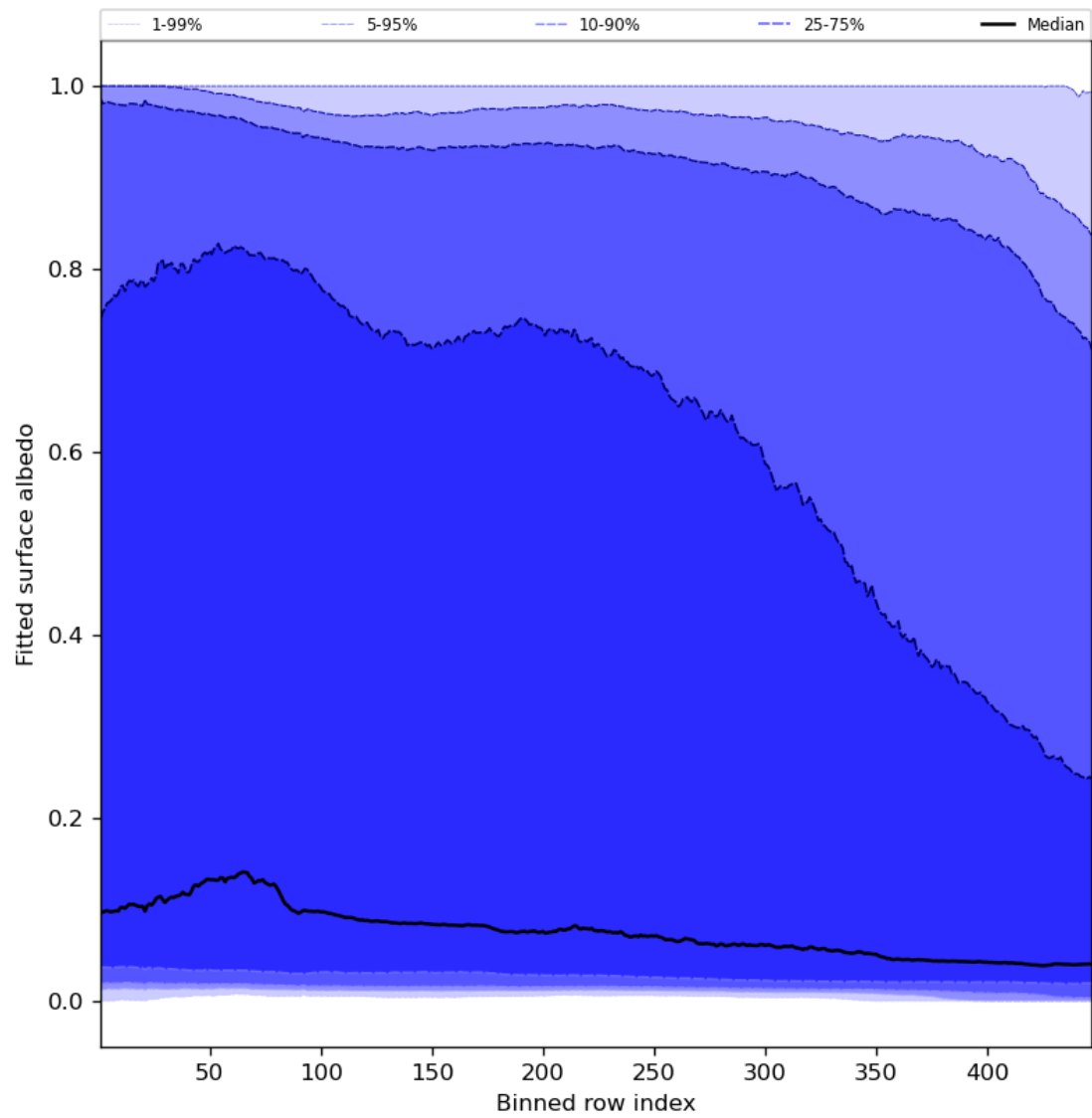
Figure 61: Along track statistics of “Fitted surface albedo” for 2023-11-21 to 2023-11-23
