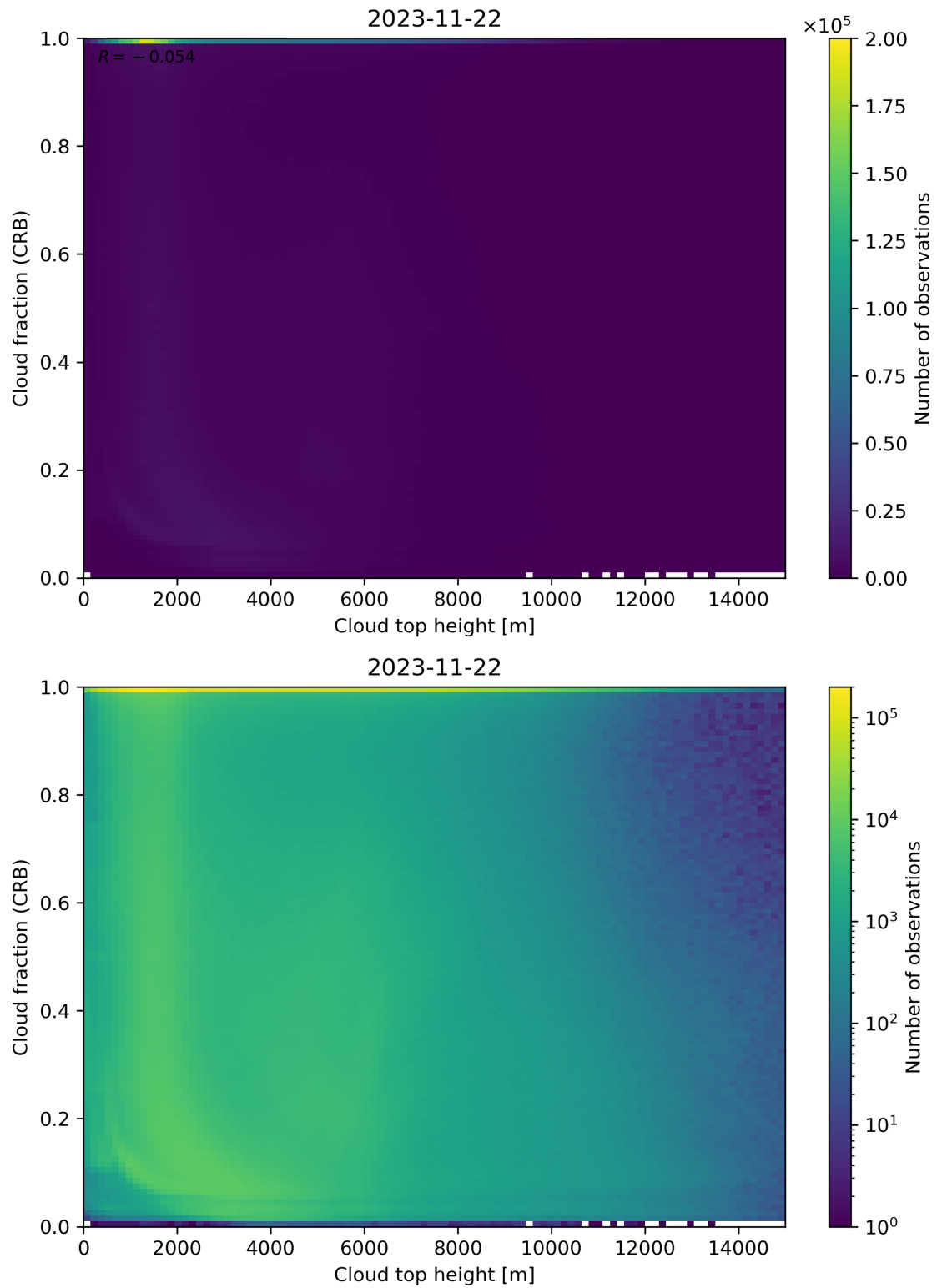
Figure 88: Scatter density plot of “Cloud top height” against “Cloud fraction (CRB)” for 2023-11-21 to 2023-11-23.
