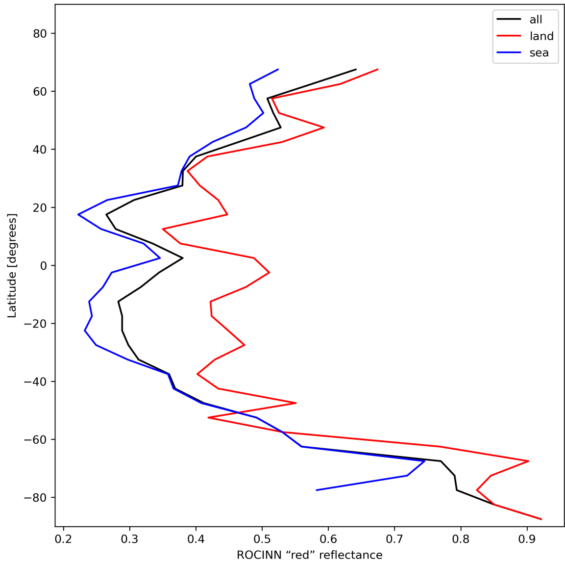
Figure 37: Zonal average of “ROCINN “red” reflectance” for 2023-11-21 to 2023-11-23.
