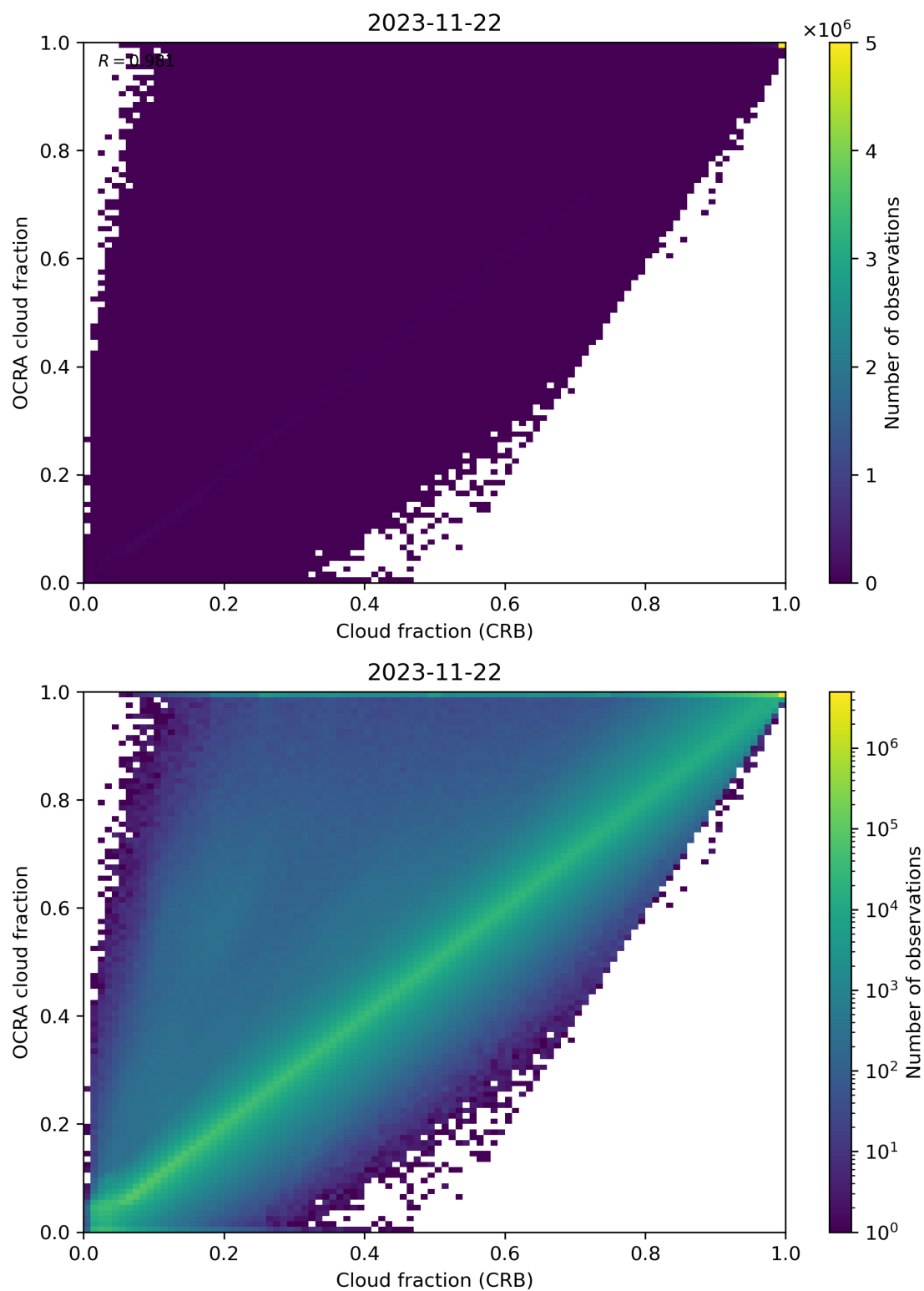
Figure 78: Scatter density plot of “Cloud fraction (CRB)” against “OCRA cloud fraction” for 2023-11-21 to 2023-11-23.
