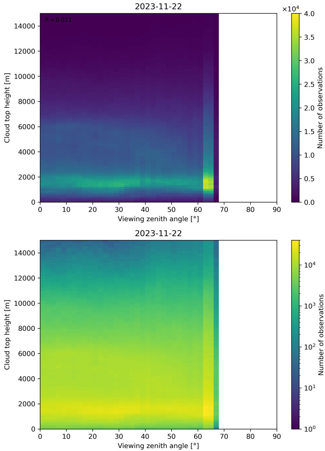
Figure 112: Scatter density plot of “Viewing zenith angle” against “Cloud top height” for 2023-11-21 to 2023-11-23.
