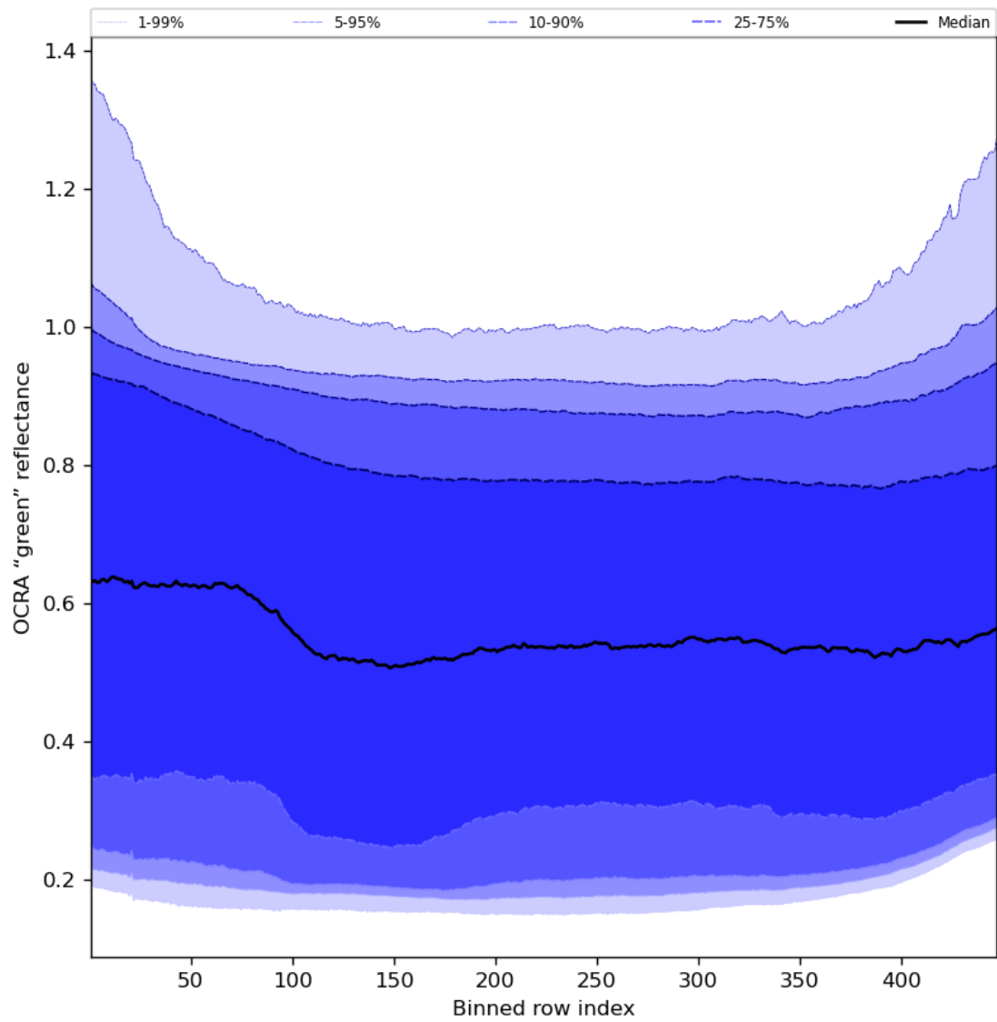
Figure 68: Along track statistics of "OCRA "green" reflectance" for 2023-11-21 to 2023-11-23
