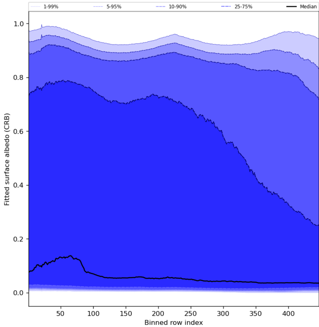
Figure 62: Along track statistics of “Fitted surface albedo (CRB)” for 2023-11-21 to 2023-11-23
