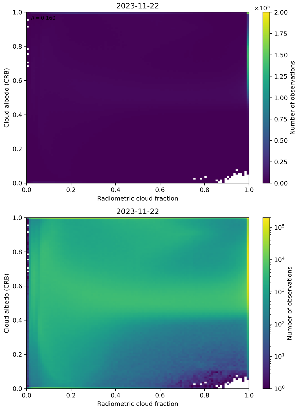
Figure 71: Scatter density plot of “Radiometric cloud fraction” against “Cloud albedo (CRB)” for 2023-11-21 to 2023-11-23.
