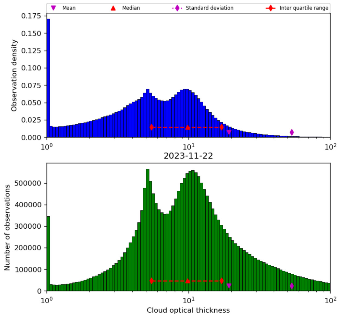
Figure 41: Histogram of “Cloud optical thickness” for 2023-11-21 to 2023-11-23
