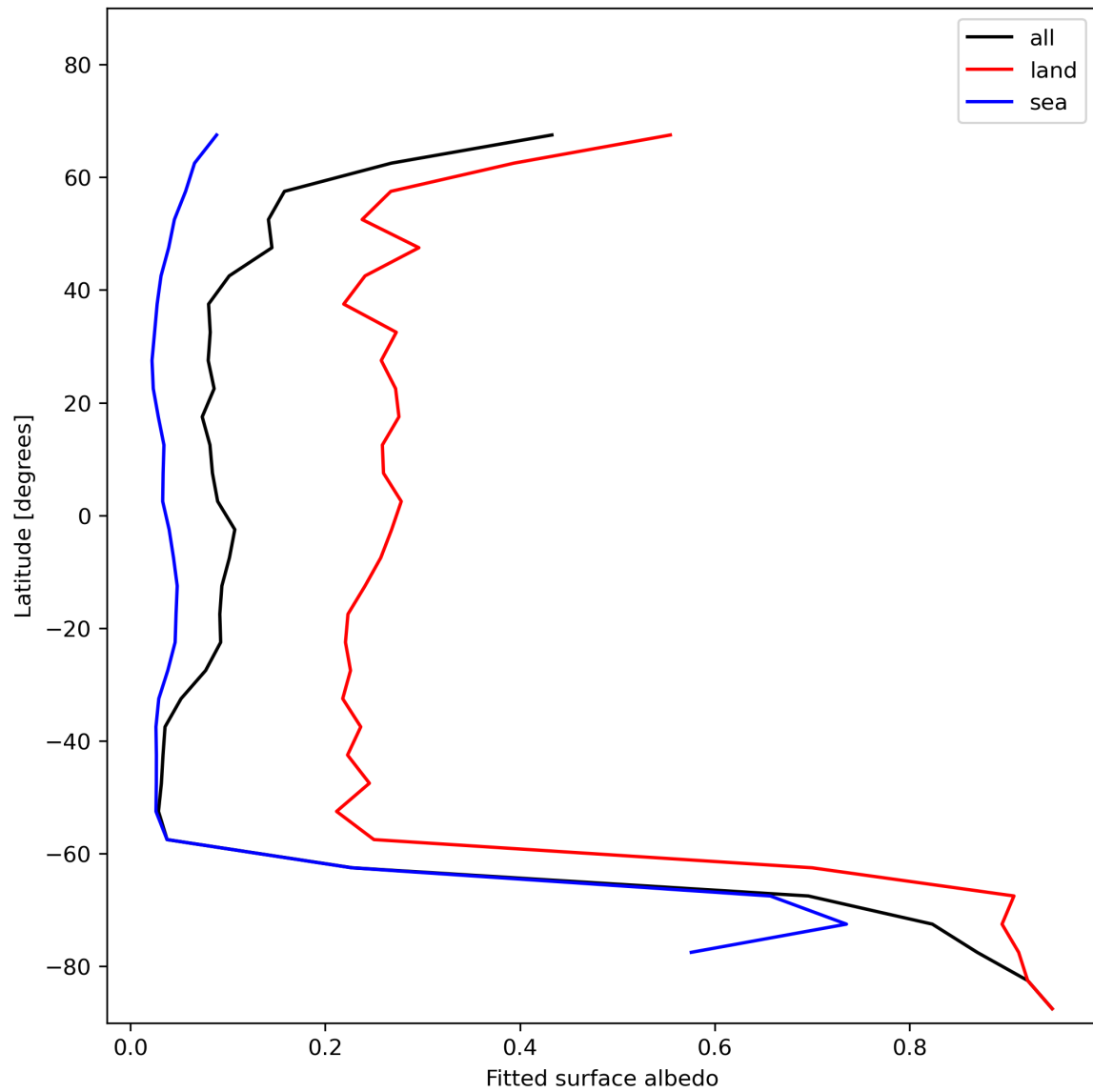
Figure 29: Zonal average of “Fitted surface albedo” for 2023-11-21 to 2023-11-23.
