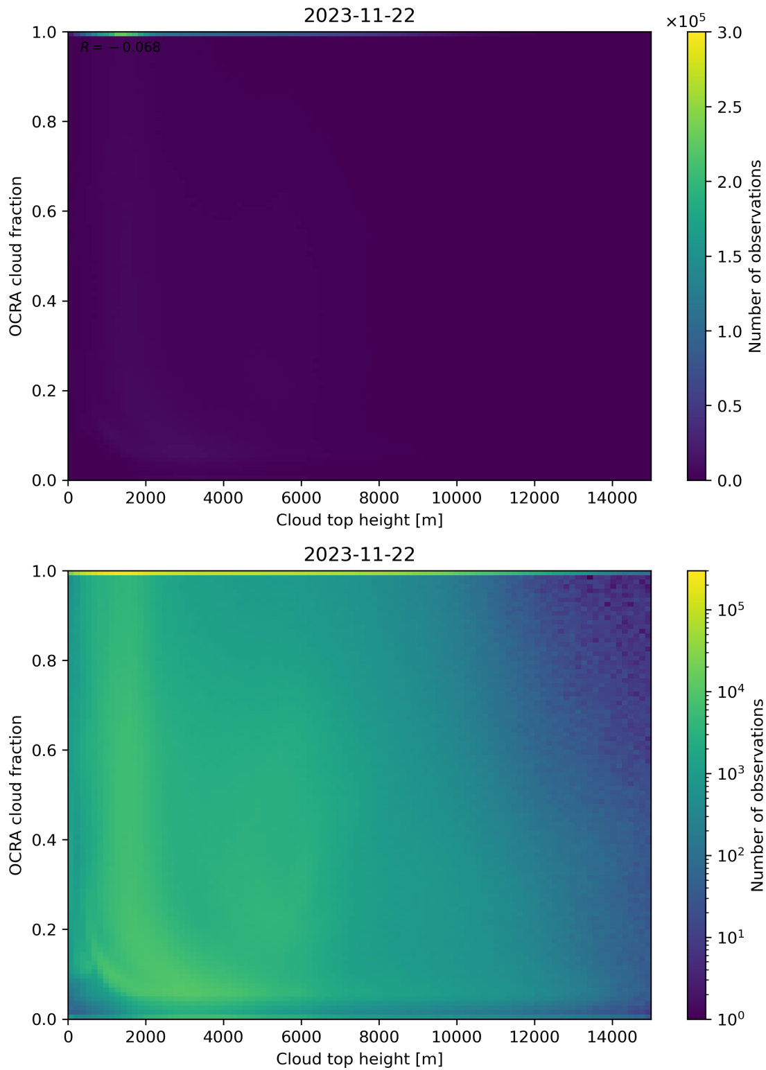
Figure 87: Scatter density plot of “Cloud top height” against “OCRA cloud fraction” for 2023-11-21 to 2023-11-23.
