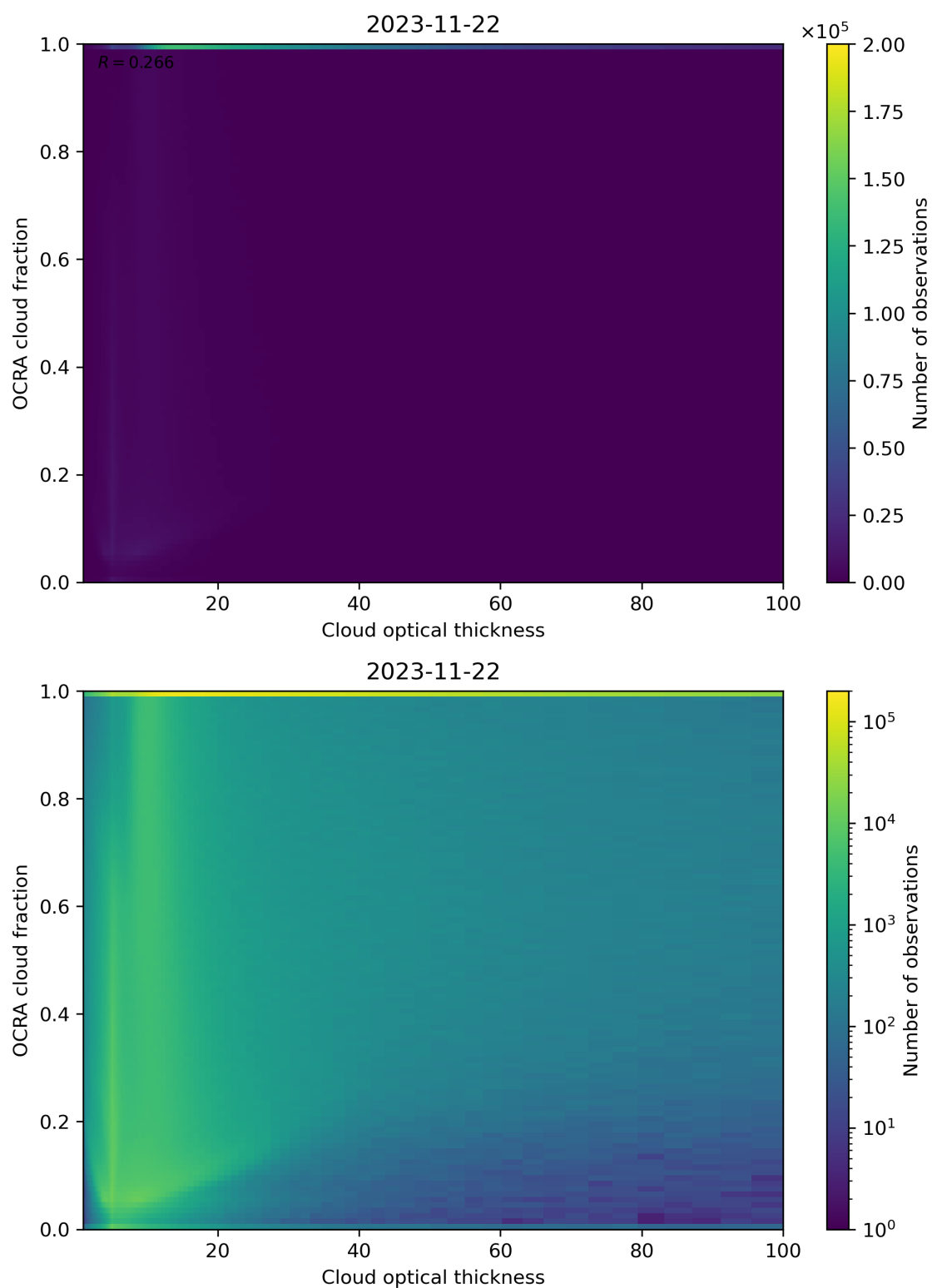
Figure 83: Scatter density plot of “Cloud optical thickness” against “OCRA cloud fraction” for 2023-11-21 to 2023-11-23.
