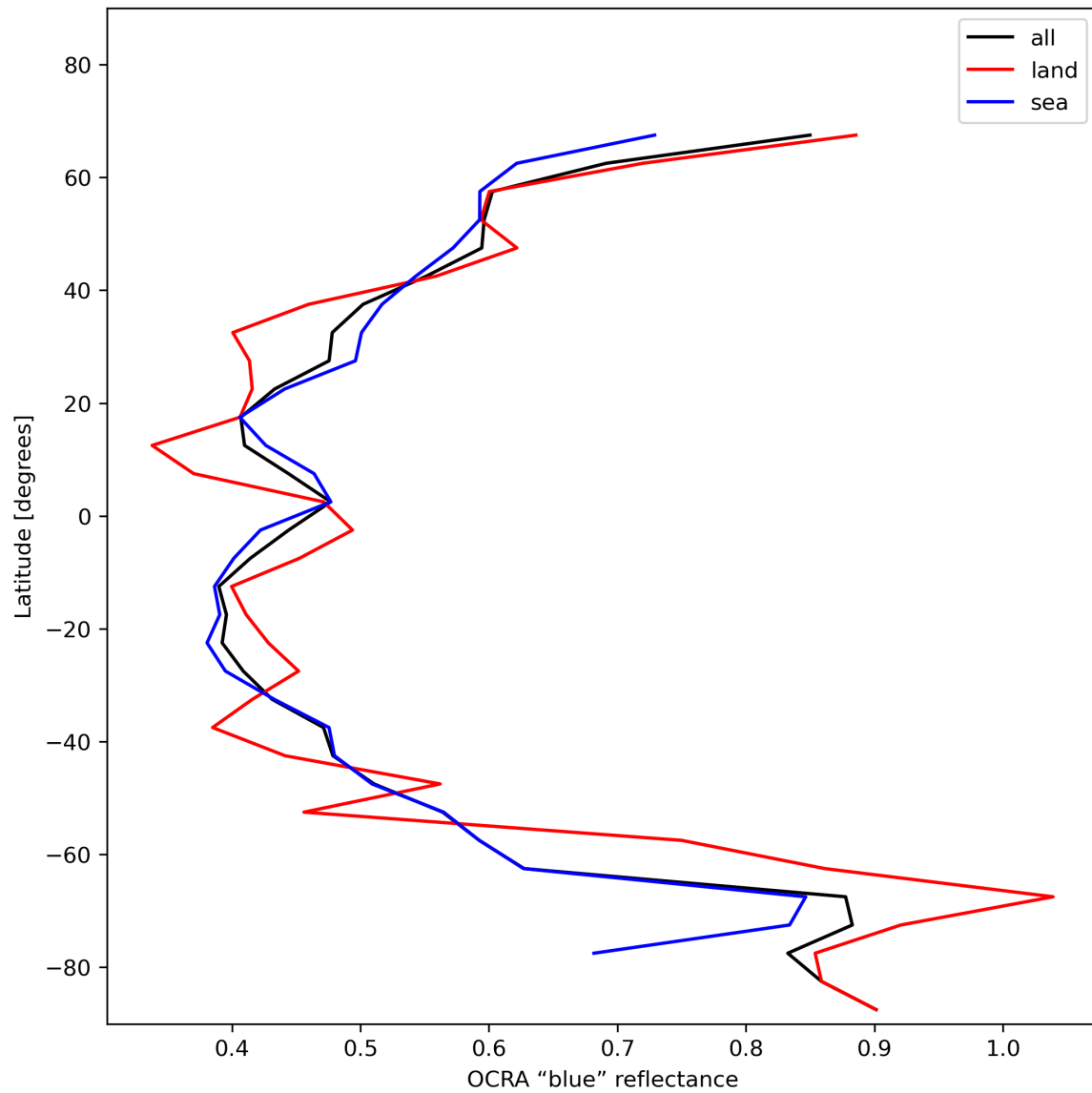
Figure 35: Zonal average of “OCRA “blue” reflectance” for 2023-11-21 to 2023-11-23.
