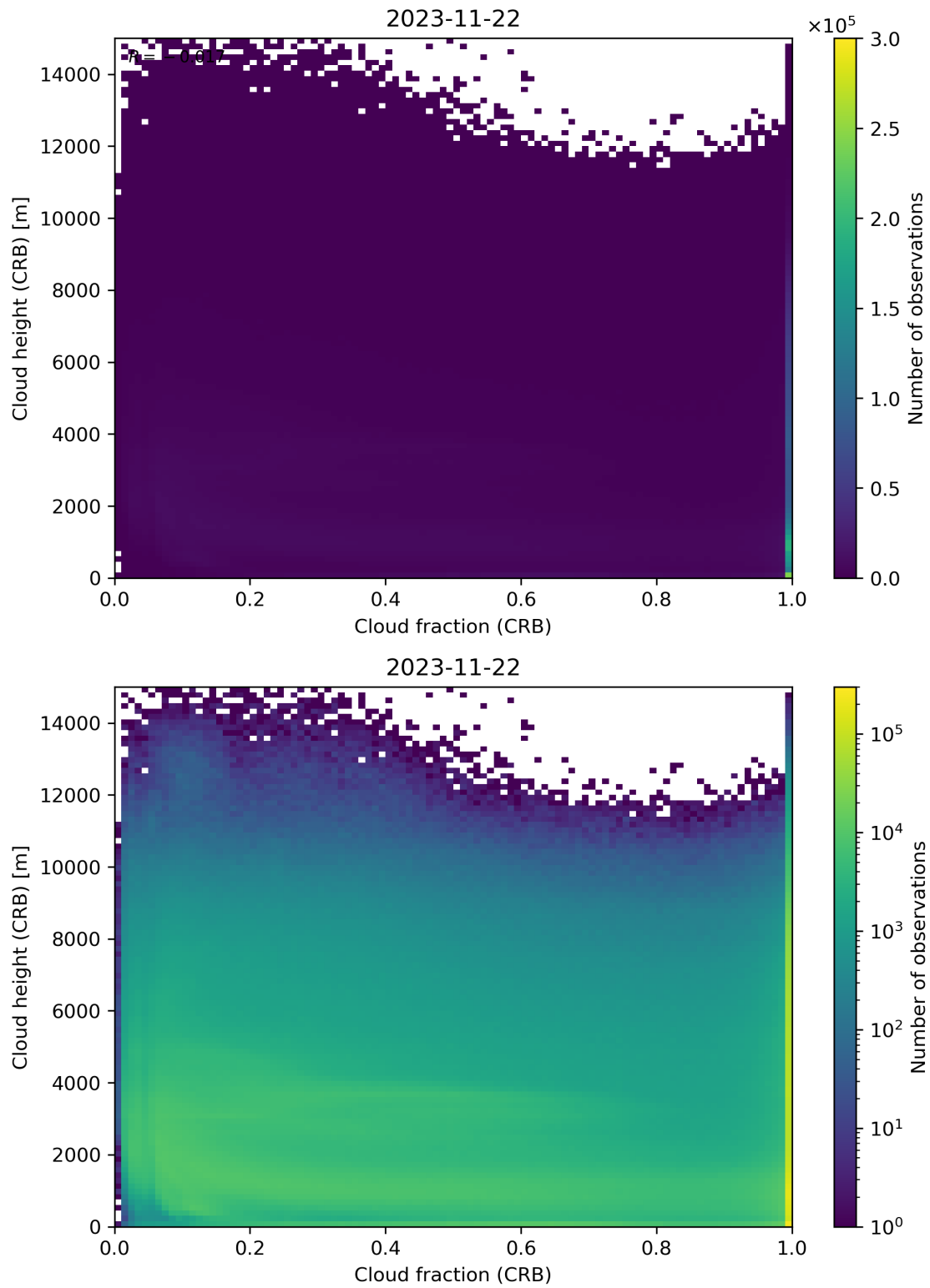
Figure 79: Scatter density plot of “Cloud fraction (CRB)” against “Cloud height (CRB)” for 2023-11-21 to 2023-11-23.
