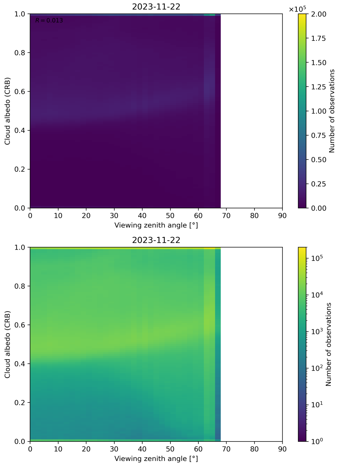
Figure 106: Scatter density plot of “Viewing zenith angle” against “Cloud albedo (CRB)” for 2023-11-21 to 2023-11-23.
