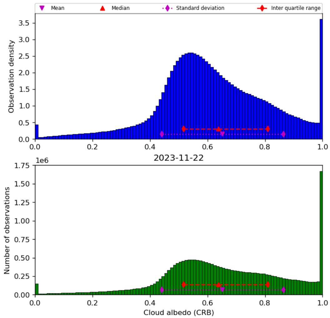
Figure 44: Histogram of “Cloud albedo (CRB)” for 2023-11-21 to 2023-11-23
