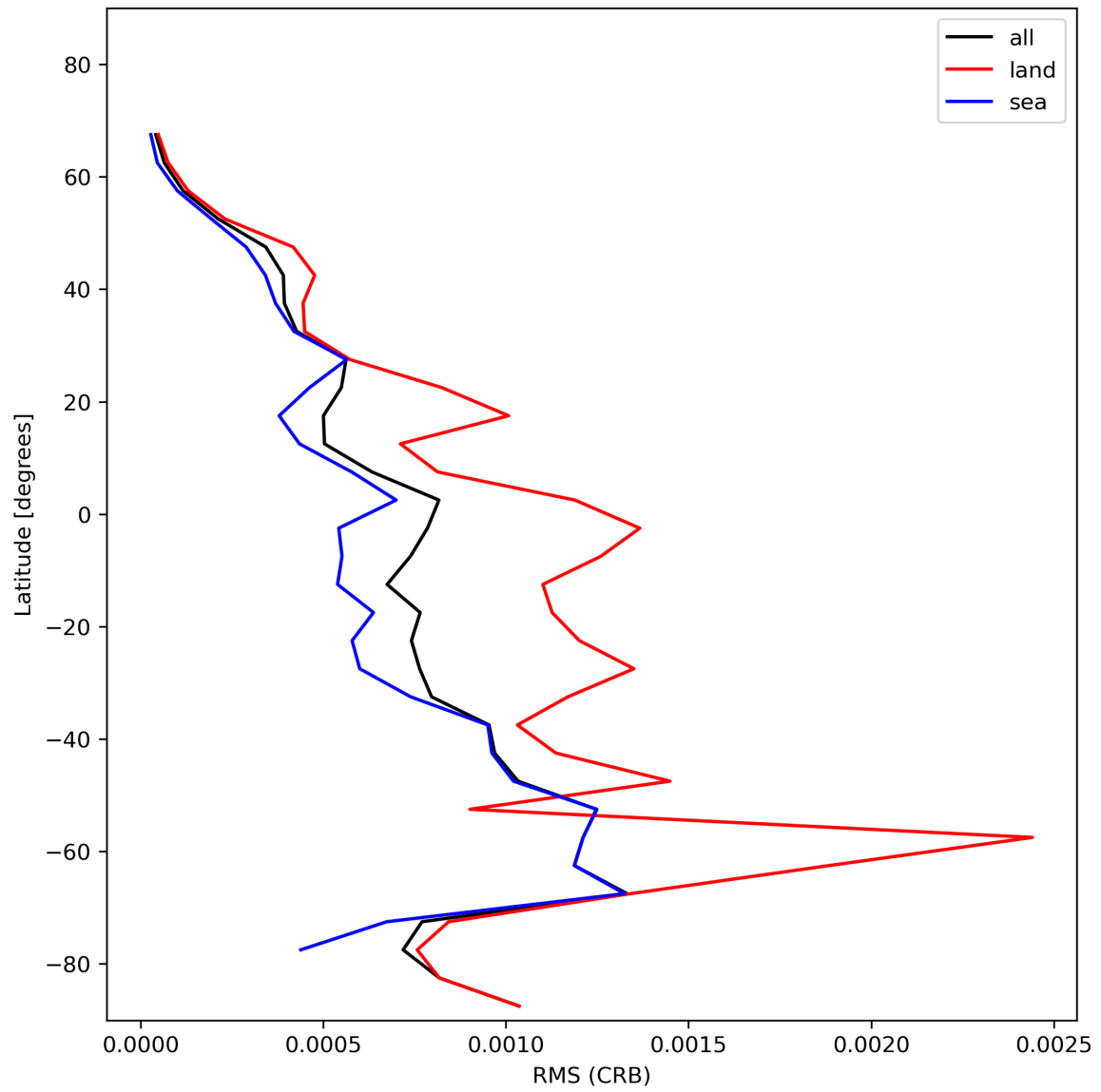
Figure 32: Zonal average of “RMS (CRB)” for 2023-11-21 to 2023-11-23.
