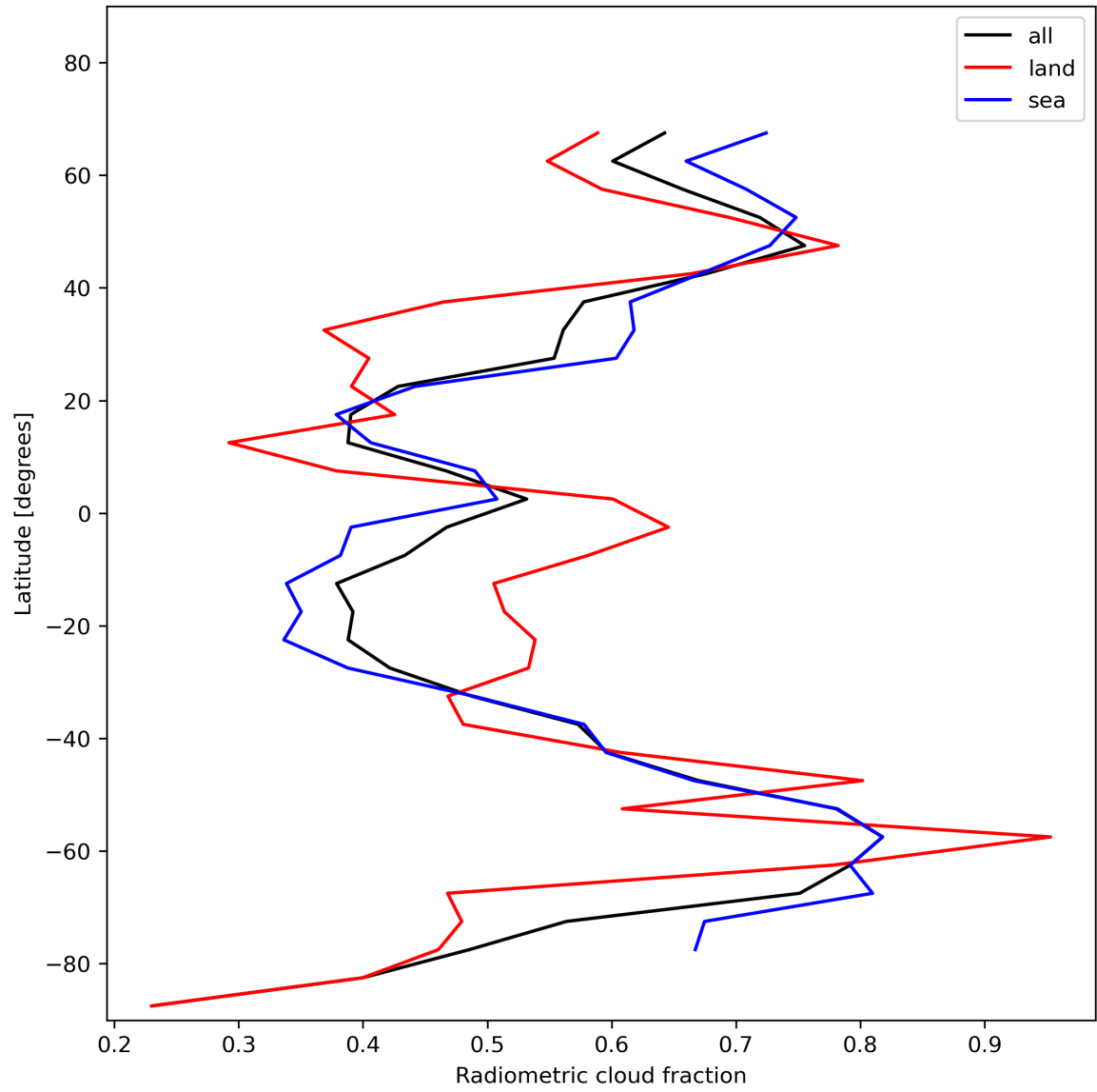
Figure 23: Zonal average of “Radiometric cloud fraction” for 2023-11-21 to 2023-11-23.
