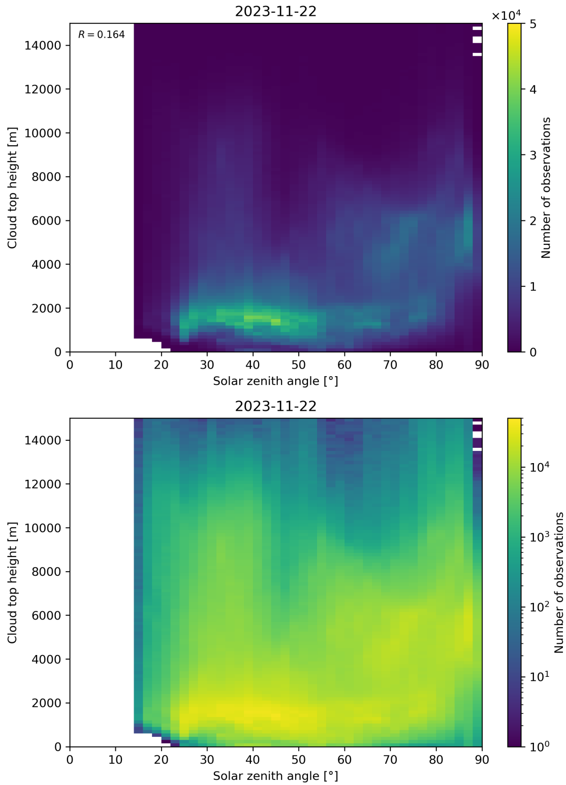
Figure 104: Scatter density plot of “Solar zenith angle” against “Cloud top height” for 2023-11-21 to 2023-11-23.
