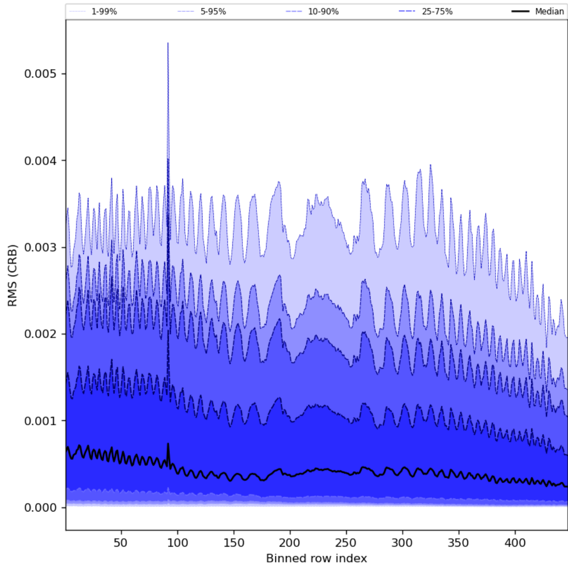
Figure 64: Along track statistics of “RMS (CRB)” for 2023-11-21 to 2023-11-23
