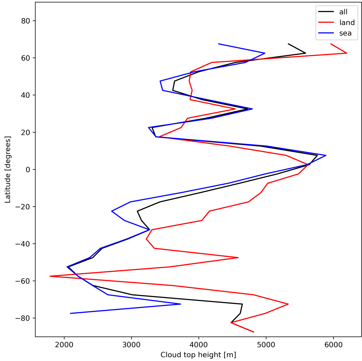
Figure 24: Zonal average of “Cloud top height” for 2023-11-21 to 2023-11-23.
