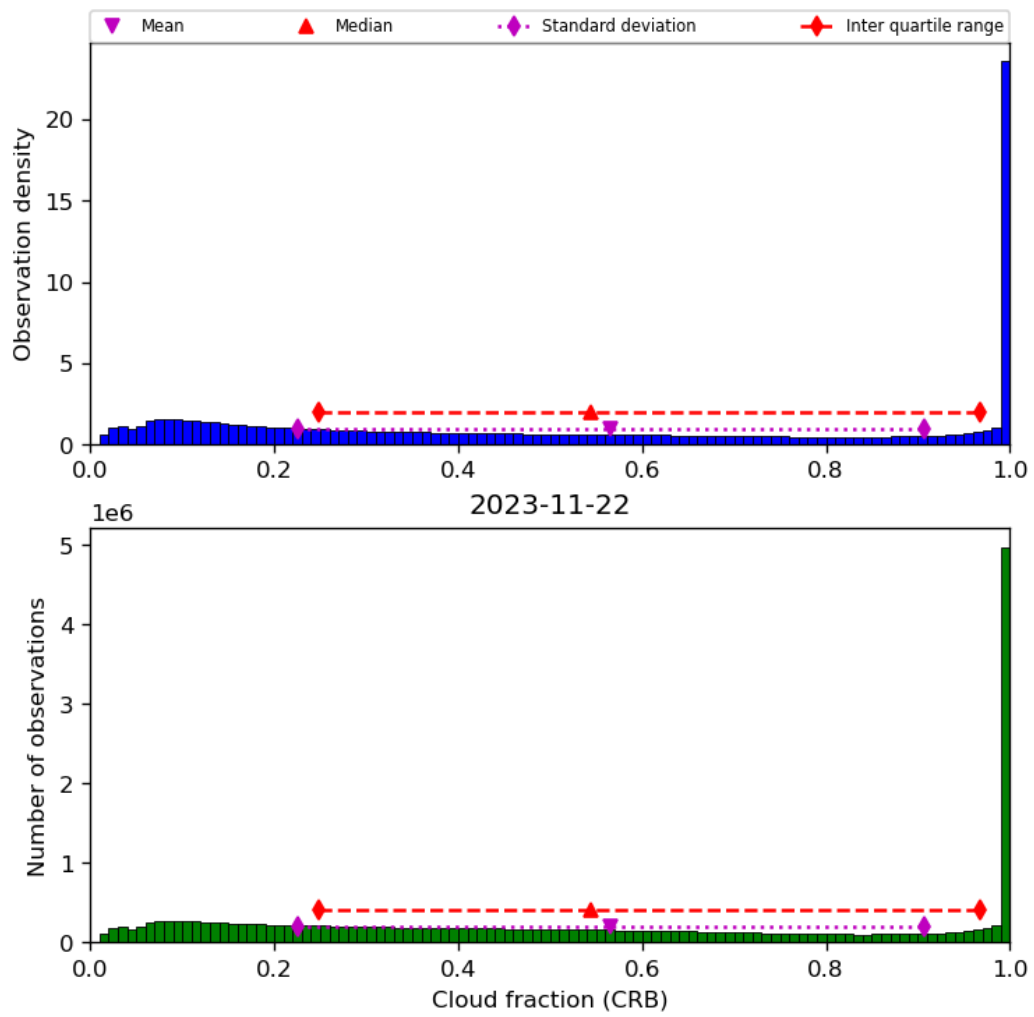
Figure 42: Histogram of “Cloud fraction (CRB)” for 2023-11-21 to 2023-11-23
