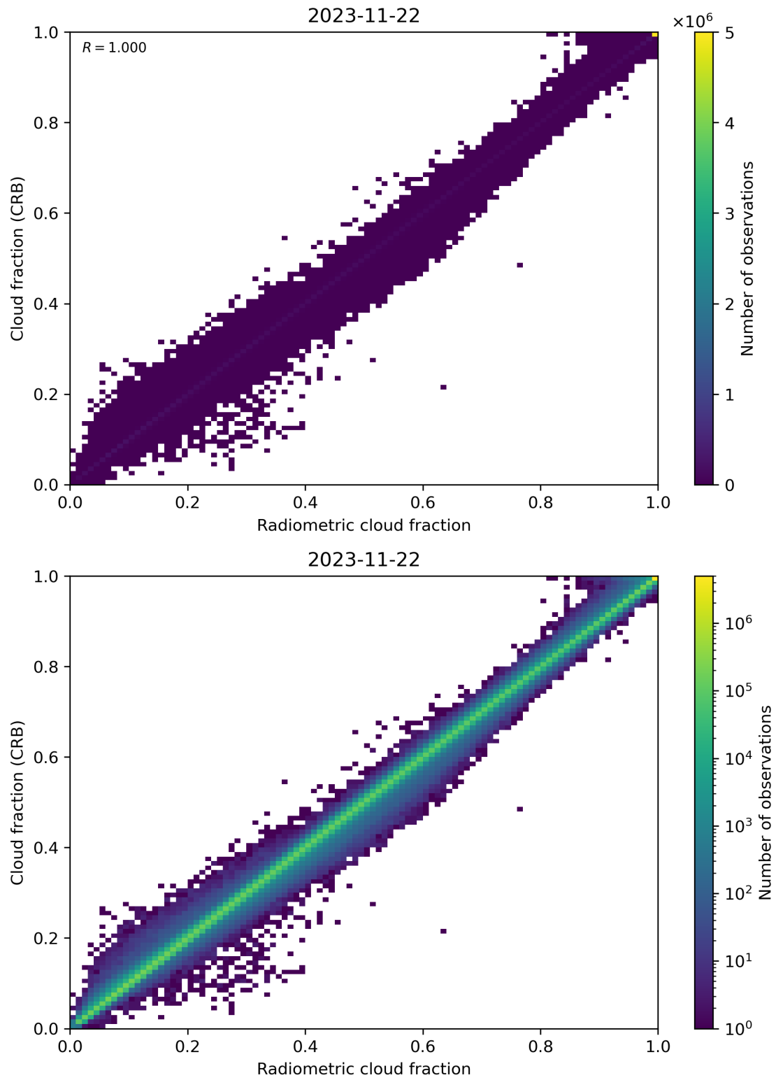
Figure 73: Scatter density plot of “Radiometric cloud fraction” against “Cloud fraction (CRB)” for 2023-11-21 to 2023-11-23.
