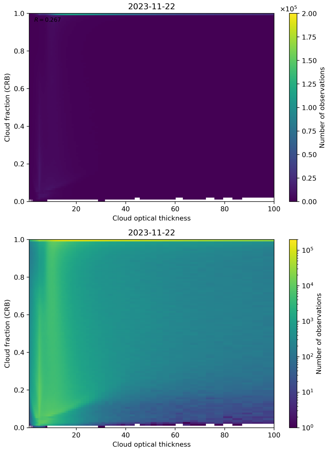
Figure 84: Scatter density plot of “Cloud optical thickness” against “Cloud fraction (CRB)” for 2023-11-21 to 2023-11-23.
