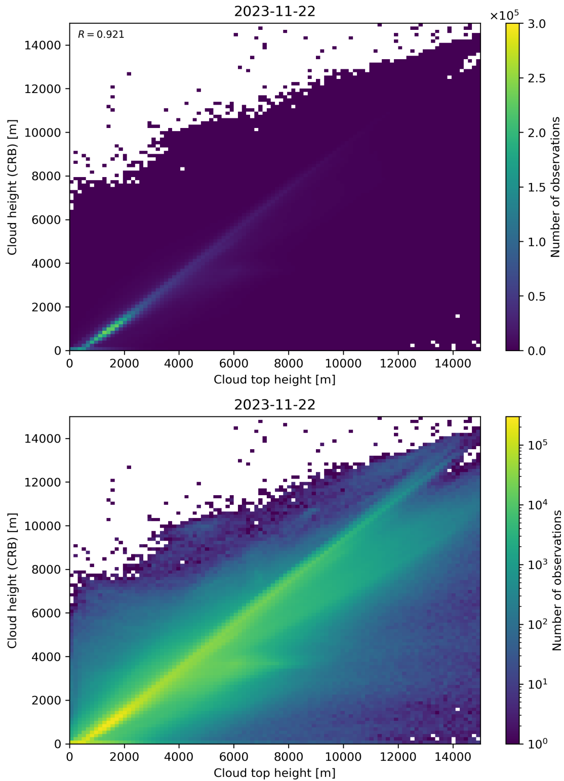
Figure 89: Scatter density plot of “Cloud top height” against “Cloud height (CRB)” for 2023-11-21 to 2023-11-23.
