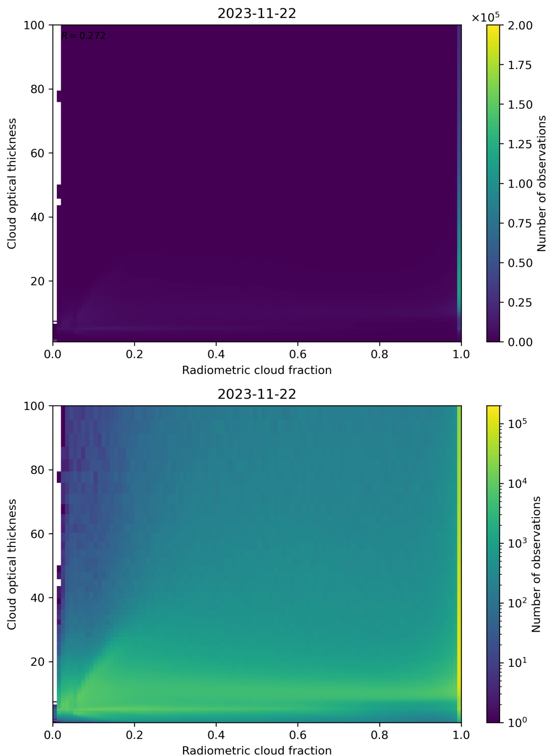
Figure 75: Scatter density plot of “Radiometric cloud fraction” against “Cloud optical thickness” for 2023-11-21 to 2023-11-23.
