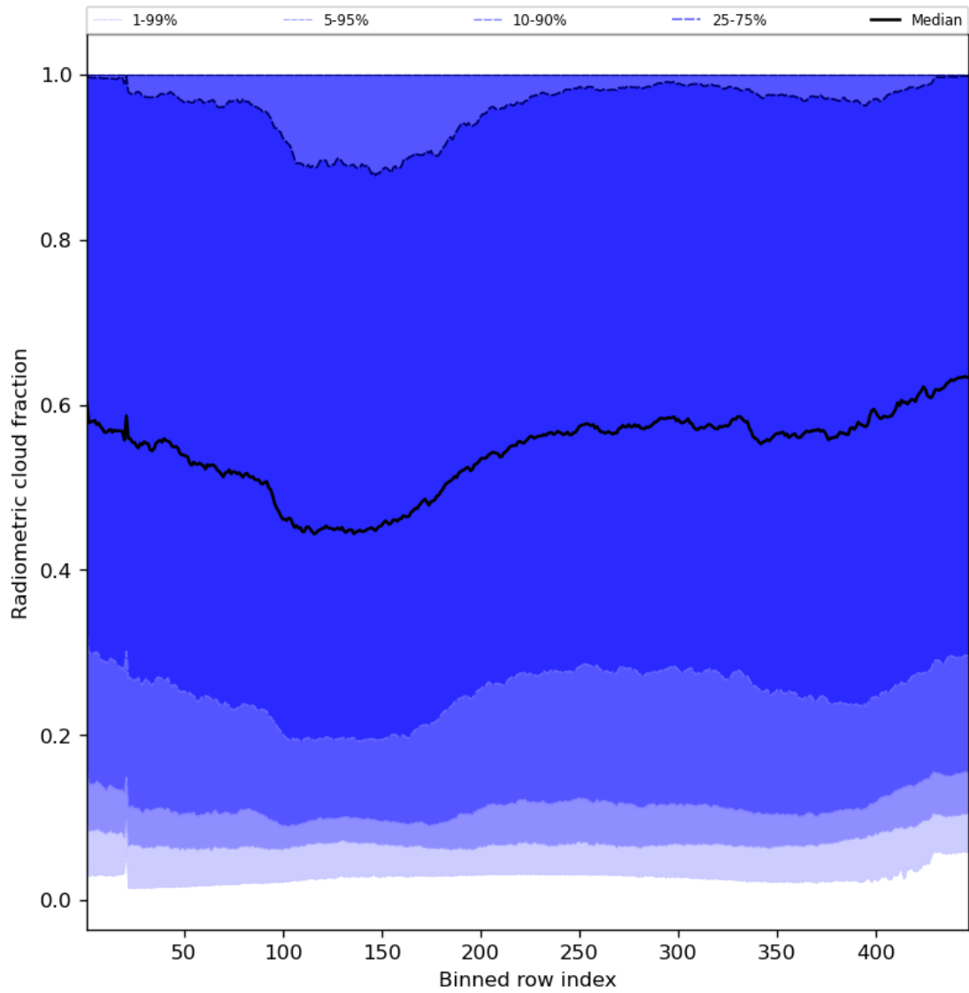
Figure 55: Along track statistics of “Radiometric cloud fraction” for 2023-11-21 to 2023-11-23
