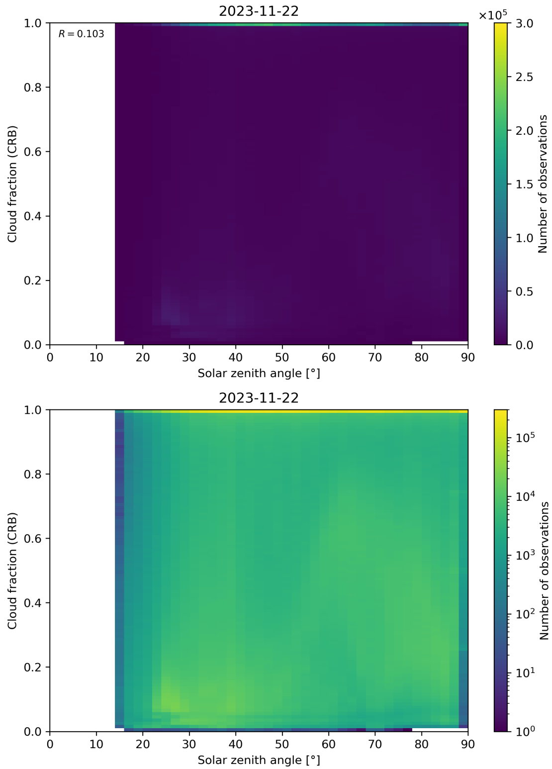
Figure 101: Scatter density plot of “Solar zenith angle” against “Cloud fraction (CRB)” for 2023-11-21 to 2023-11-23.
