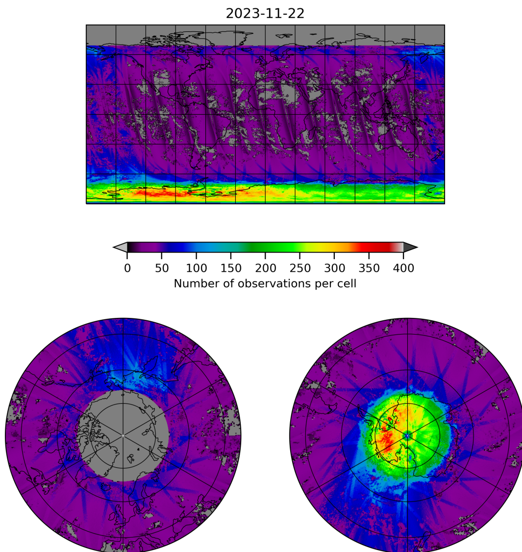
Figure 21: Map of the number of observations for 2023-11-21 to 2023-11-23
