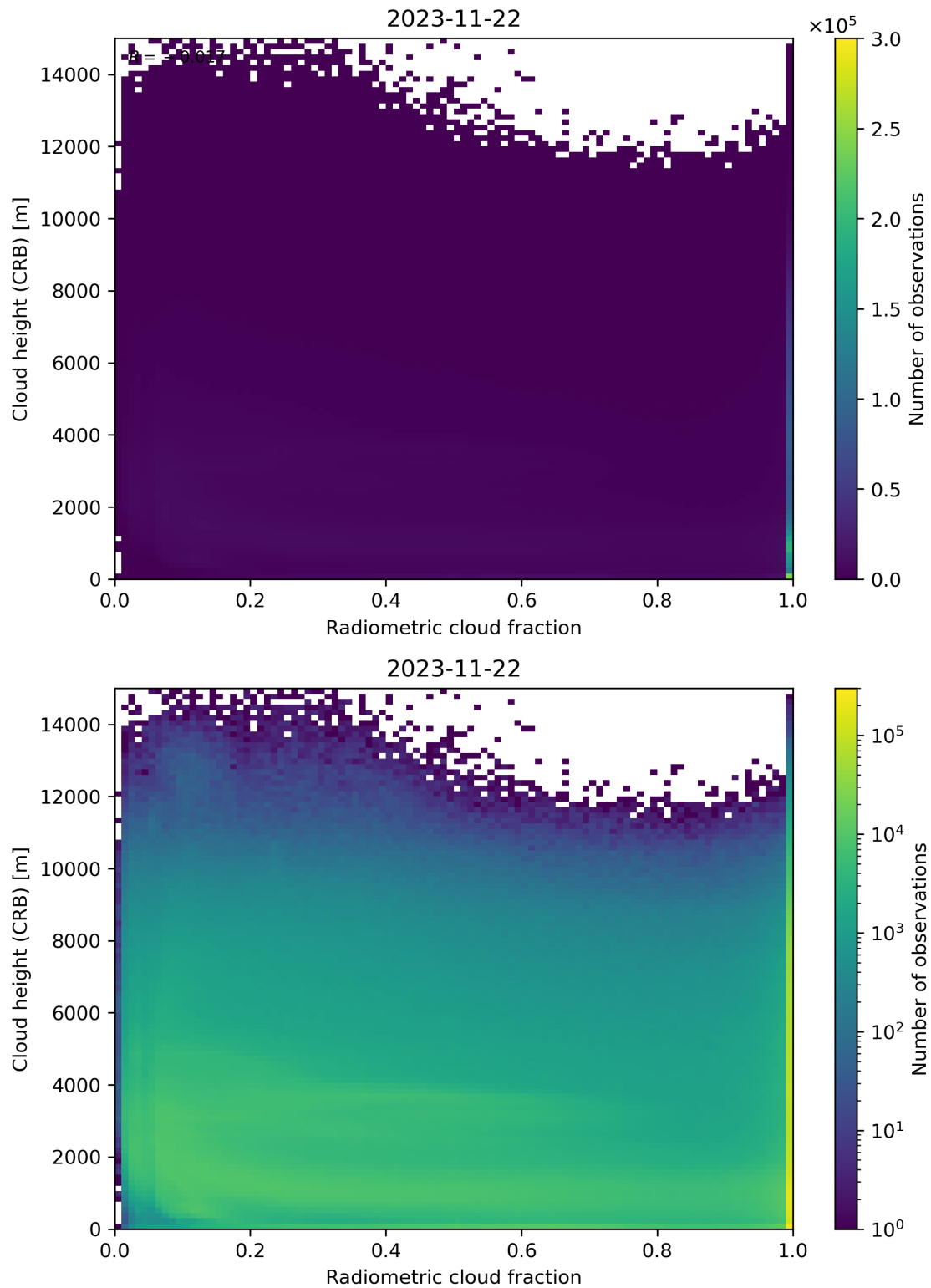
Figure 74: Scatter density plot of “Radiometric cloud fraction” against “Cloud height (CRB)” for 2023-11-21 to 2023-11-23.
