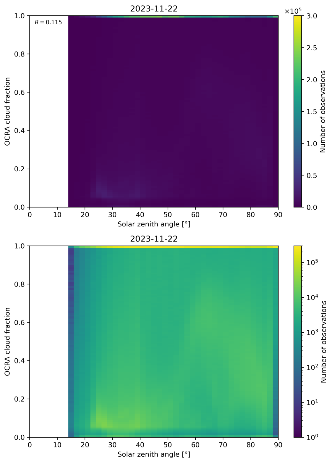
Figure 100: Scatter density plot of “Solar zenith angle” against “OCRA cloud fraction” for 2023-11-21 to 2023-11-23.
