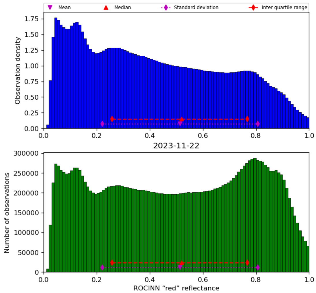
Figure 53: Histogram of “ROCINN “red” reflectance” for 2023-11-21 to 2023-11-23
