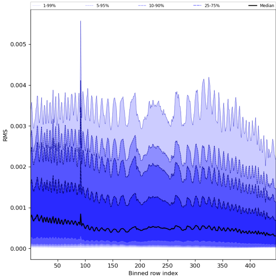
Figure 63: Along track statistics of “RMS” for 2023-11-21 to 2023-11-23
