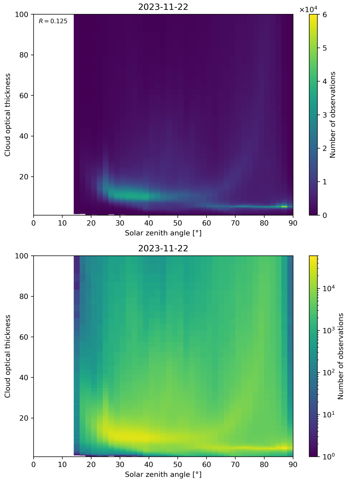
Figure 103: Scatter density plot of “Solar zenith angle” against “Cloud optical thickness” for 2023-11-21 to 2023-11-23.
