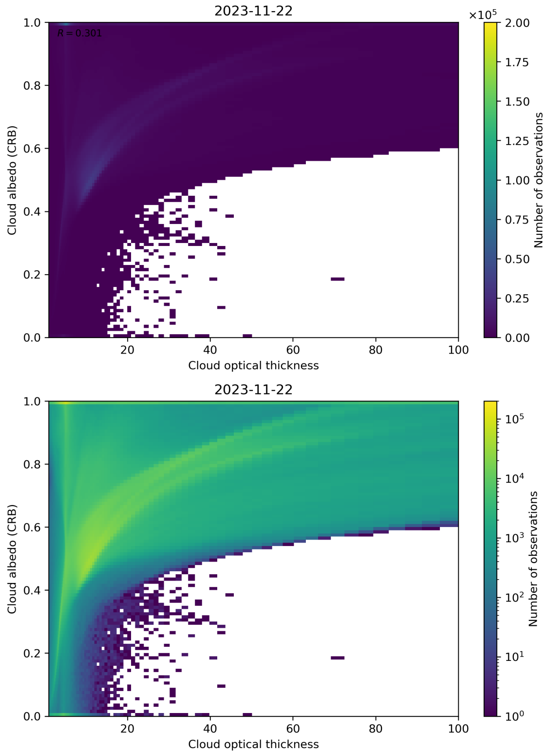
Figure 82: Scatter density plot of “Cloud optical thickness” against “Cloud albedo (CRB)” for 2023-11-21 to 2023-11-23.
