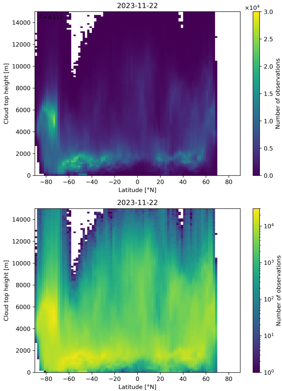
Figure 97: Scatter density plot of “Latitude” against “Cloud top height” for 2023-11-21 to 2023-11-23.
