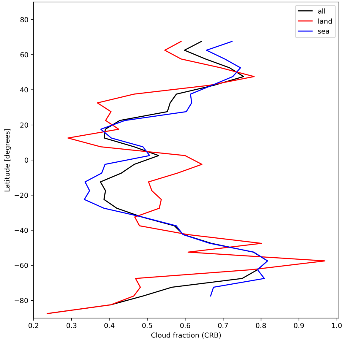
Figure 26: Zonal average of “Cloud fraction (CRB)” for 2023-11-21 to 2023-11-23.
