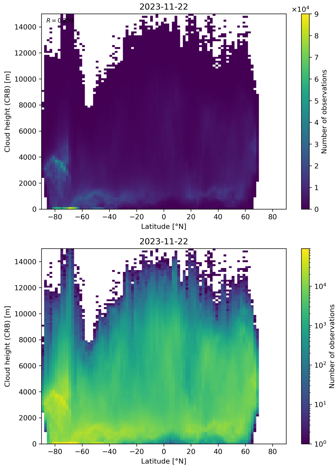
Figure 95: Scatter density plot of “Latitude” against “Cloud height (CRB)” for 2023-11-21 to 2023-11-23.
