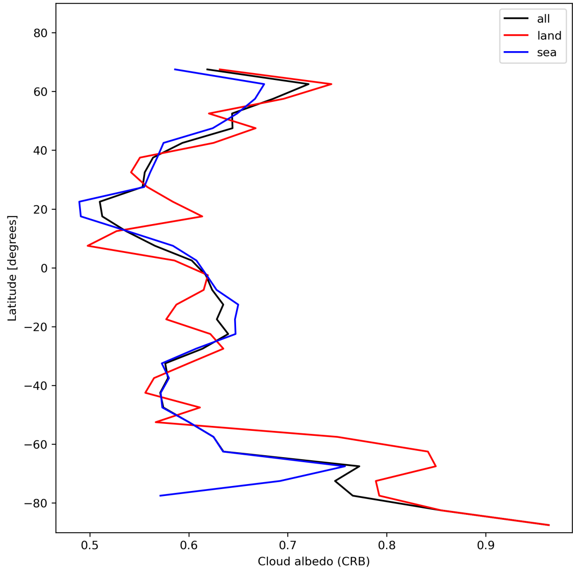
Figure 28: Zonal average of “Cloud albedo (CRB)” for 2023-11-21 to 2023-11-23.
