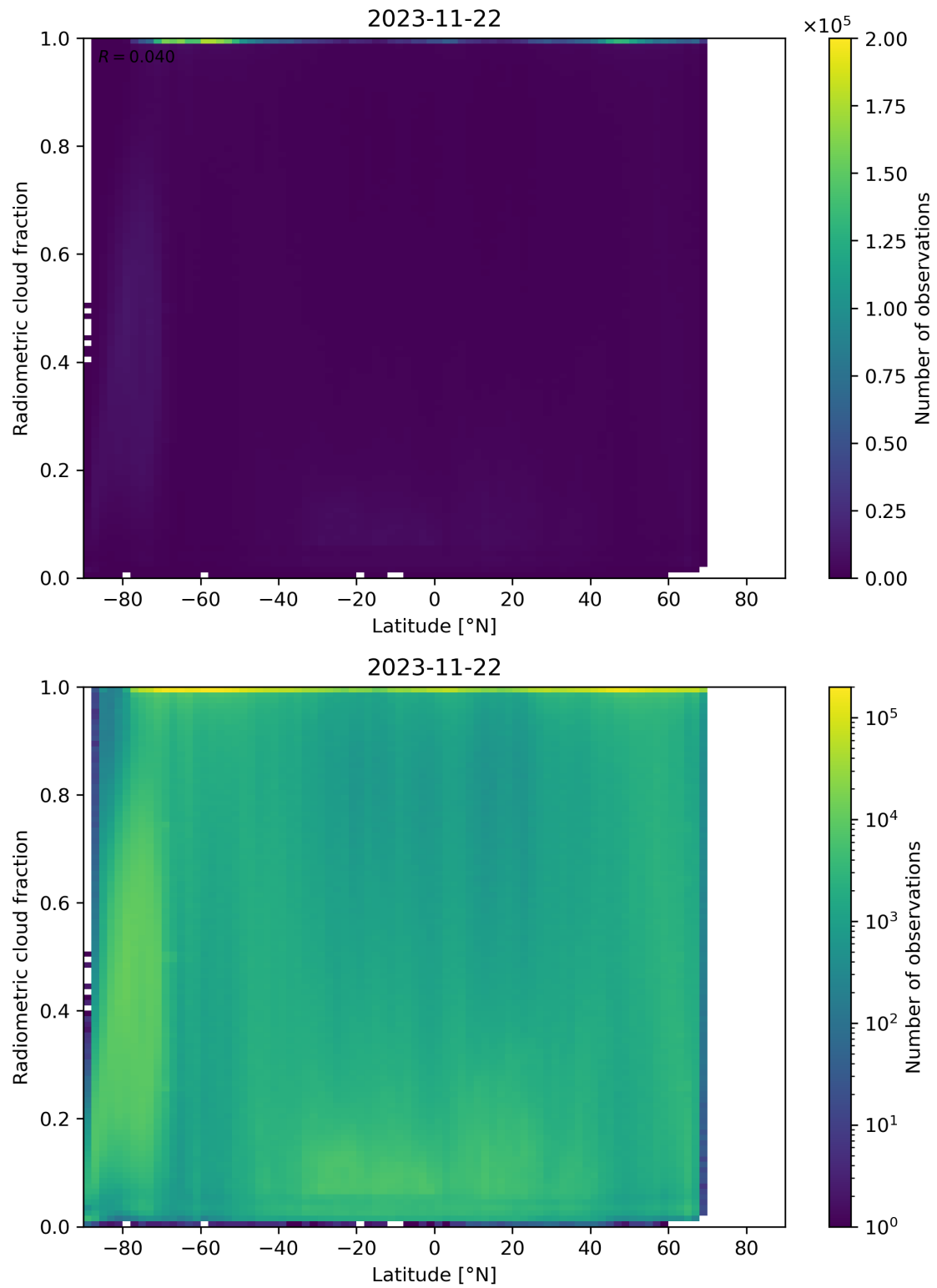
Figure 92: Scatter density plot of “Latitude” against “Radiometric cloud fraction” for 2023-11-21 to 2023-11-23.
