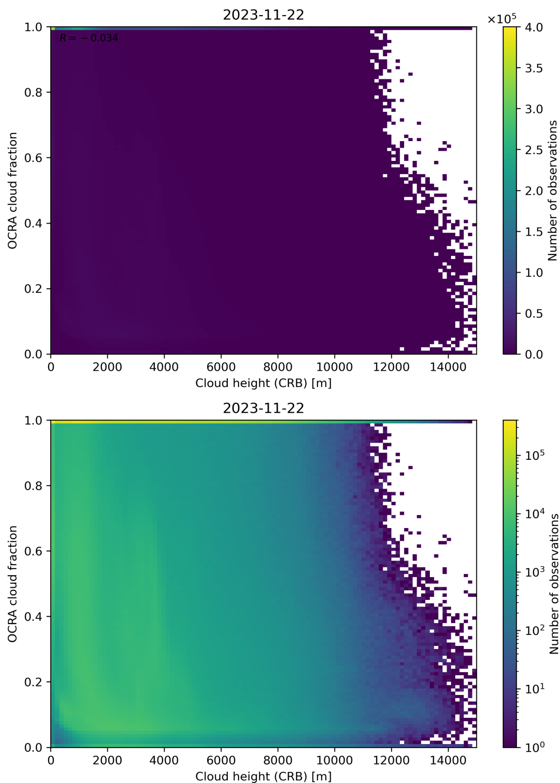
Figure 81: Scatter density plot of “Cloud height (CRB)” against “OCRA cloud fraction” for 2023-11-21 to 2023-11-23.
