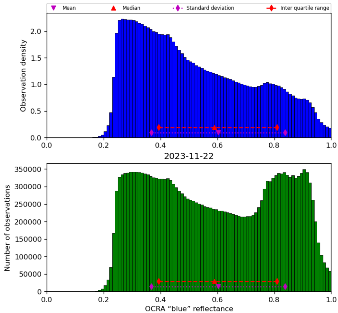
Figure 51: Histogram of “OCRA “blue” reflectance” for 2023-11-21 to 2023-11-23
