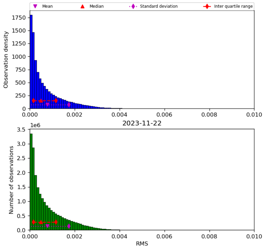
Figure 47: Histogram of “RMS” for 2023-11-21 to 2023-11-23
