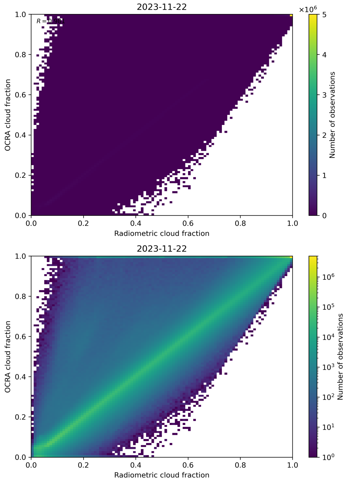
Figure 72: Scatter density plot of “Radiometric cloud fraction” against “OCRA cloud fraction” for 2023-11-21 to 2023-11-23.
