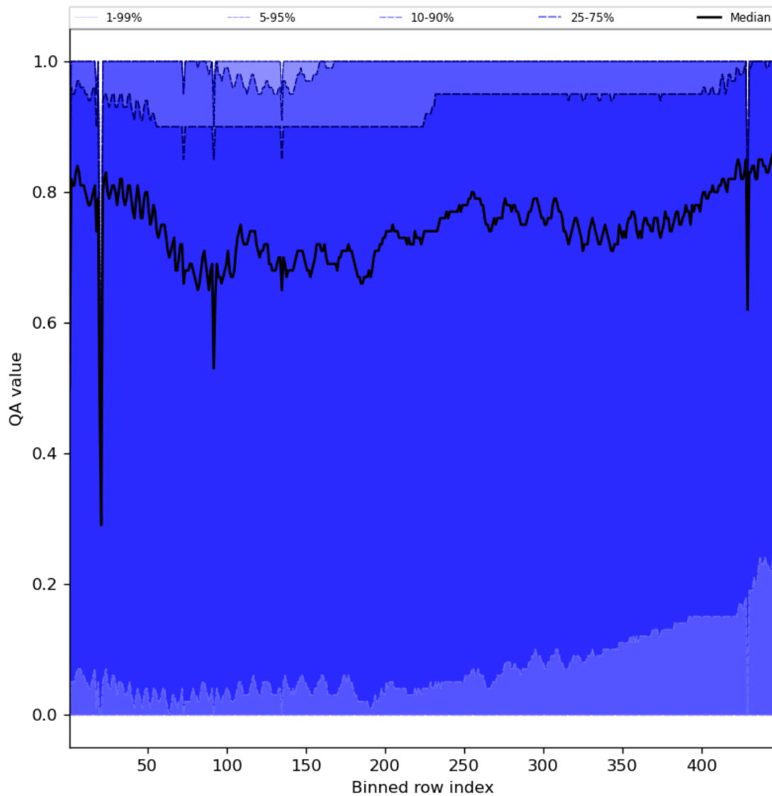
Figure 54: Along track statistics of “QA value” for 2023-11-21 to 2023-11-23
