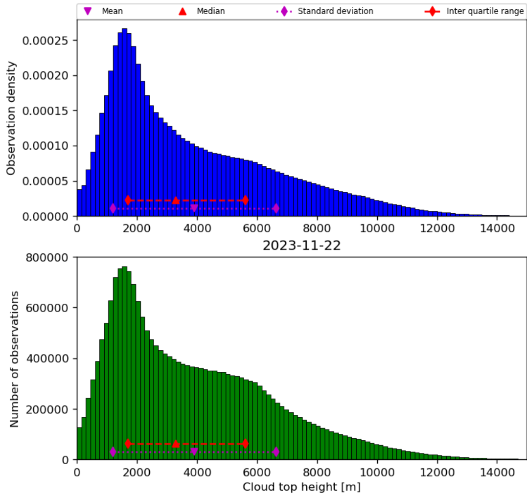
Figure 40: Histogram of “Cloud top height” for 2023-11-21 to 2023-11-23
