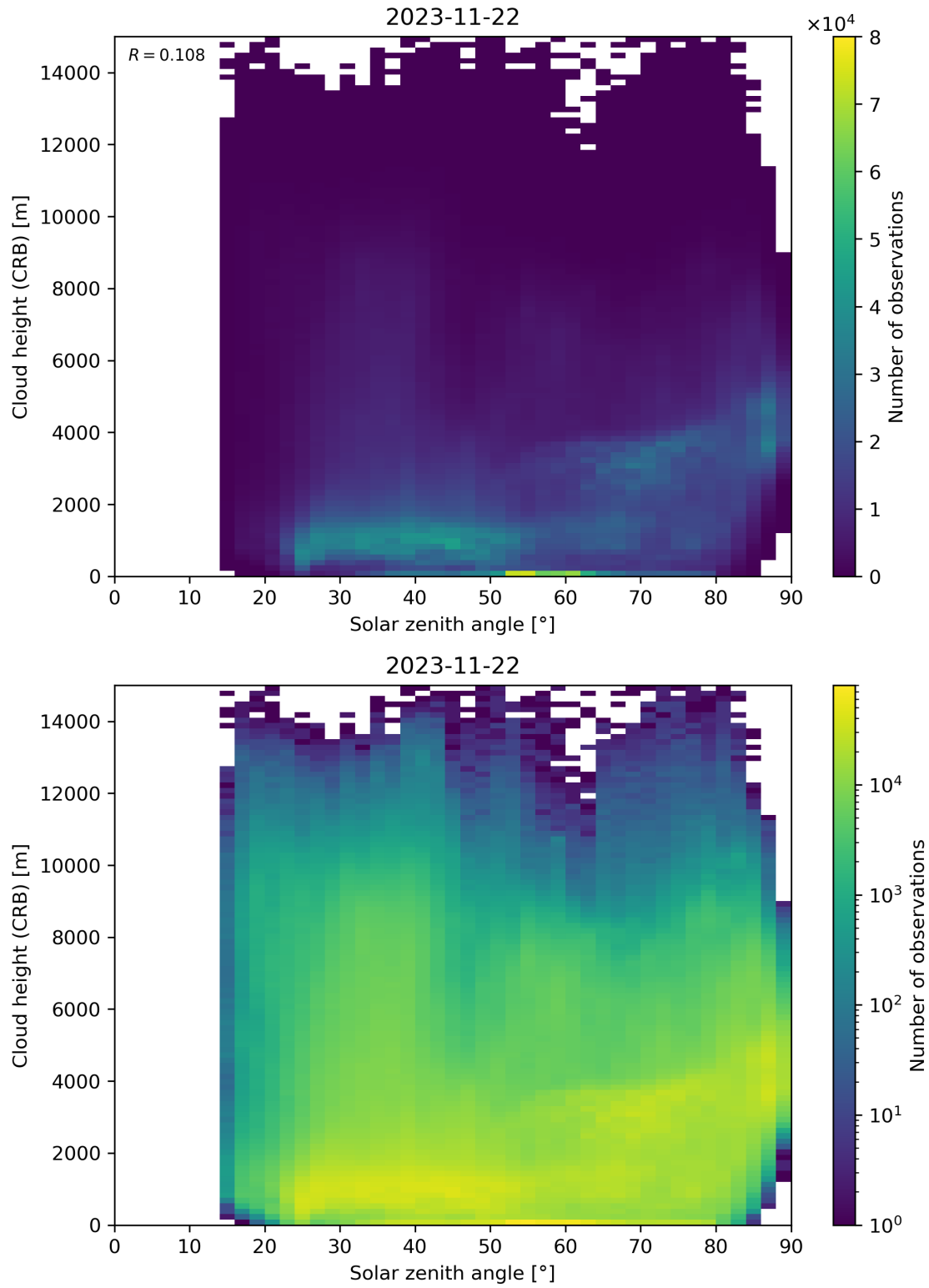
Figure 102: Scatter density plot of “Solar zenith angle” against “Cloud height (CRB)” for 2023-11-21 to 2023-11-23.
