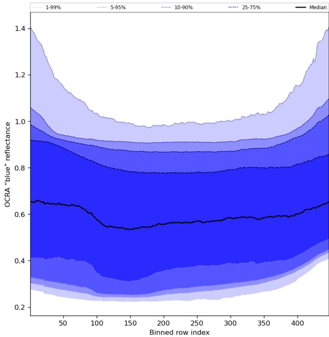
Figure 67: Along track statistics of “OCRA “blue” reflectance” for 2023-11-21 to 2023-11-23
