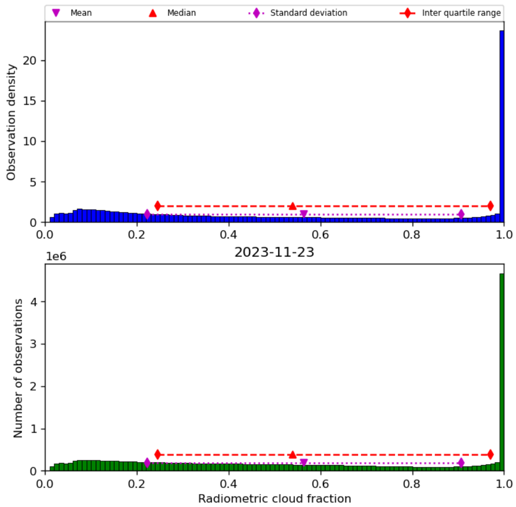
Figure 39: Histogram of “Radiometric cloud fraction” for 2023-11-23 to 2023-11-24
