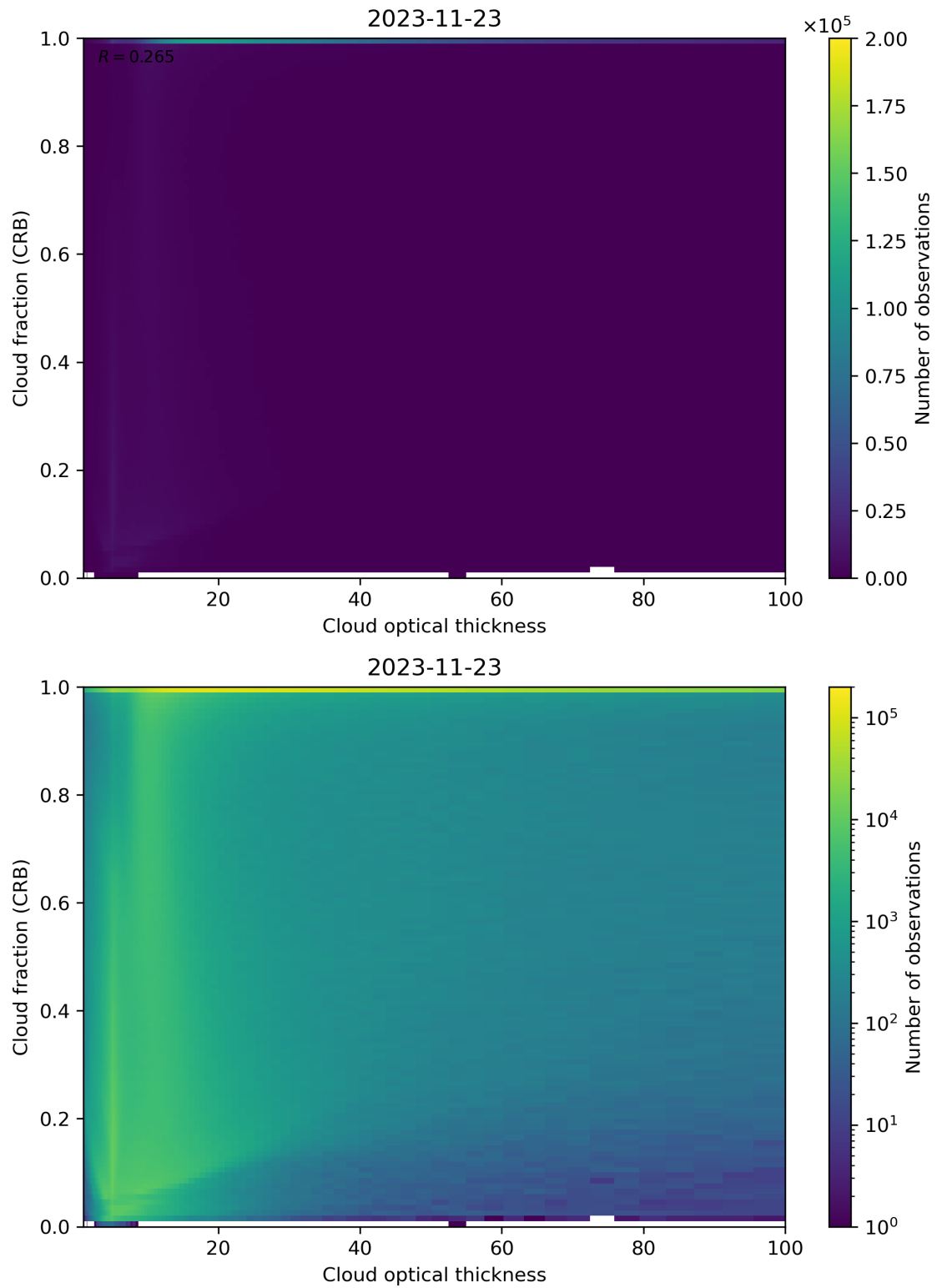
Figure 84: Scatter density plot of “Cloud optical thickness” against “Cloud fraction (CRB)” for 2023-11-23 to 2023-11-24.
