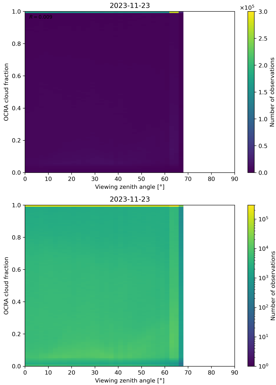
Figure 108: Scatter density plot of “Viewing zenith angle” against “OCRA cloud fraction” for 2023-11-23 to 2023-11-24.
