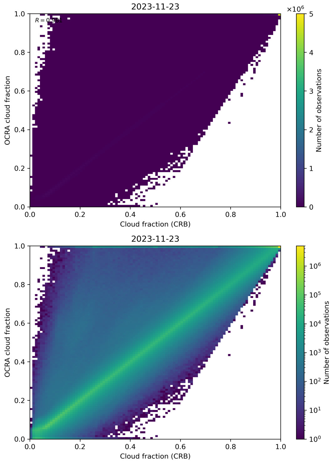
Figure 78: Scatter density plot of “Cloud fraction (CRB)” against “OCRA cloud fraction” for 2023-11-23 to 2023-11-24.
