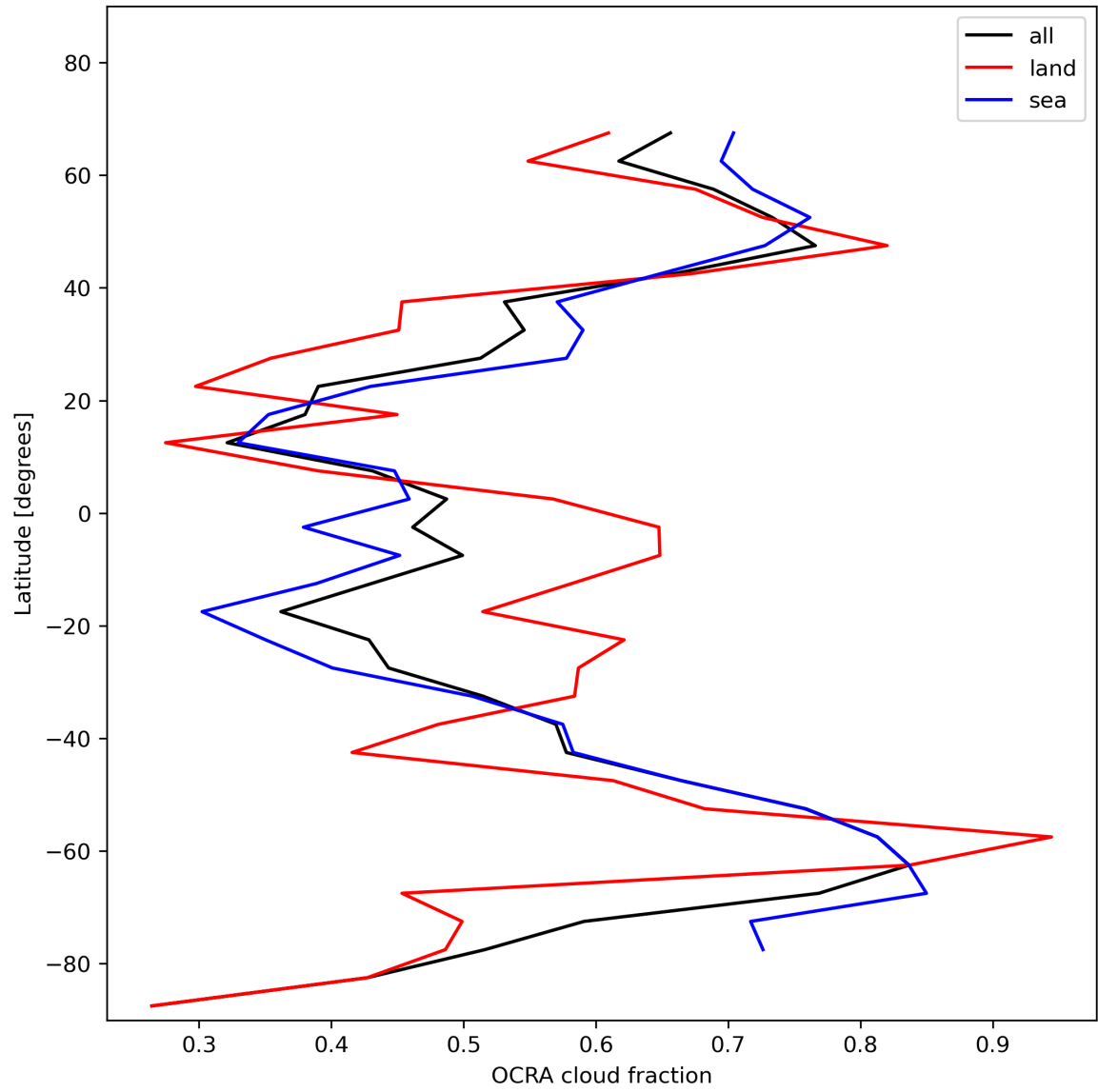
Figure 34: Zonal average of “OCRA cloud fraction” for 2023-11-23 to 2023-11-24.
