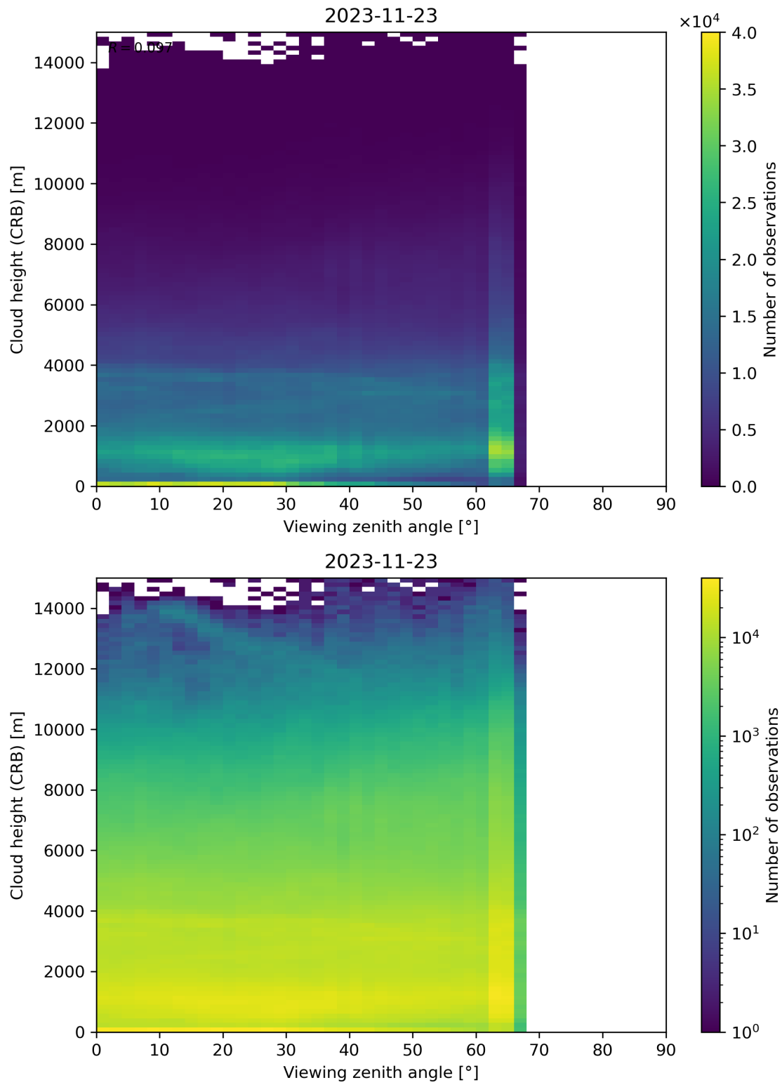
Figure 110: Scatter density plot of “Viewing zenith angle” against “Cloud height (CRB)” for 2023-11-23 to 2023-11-24.
