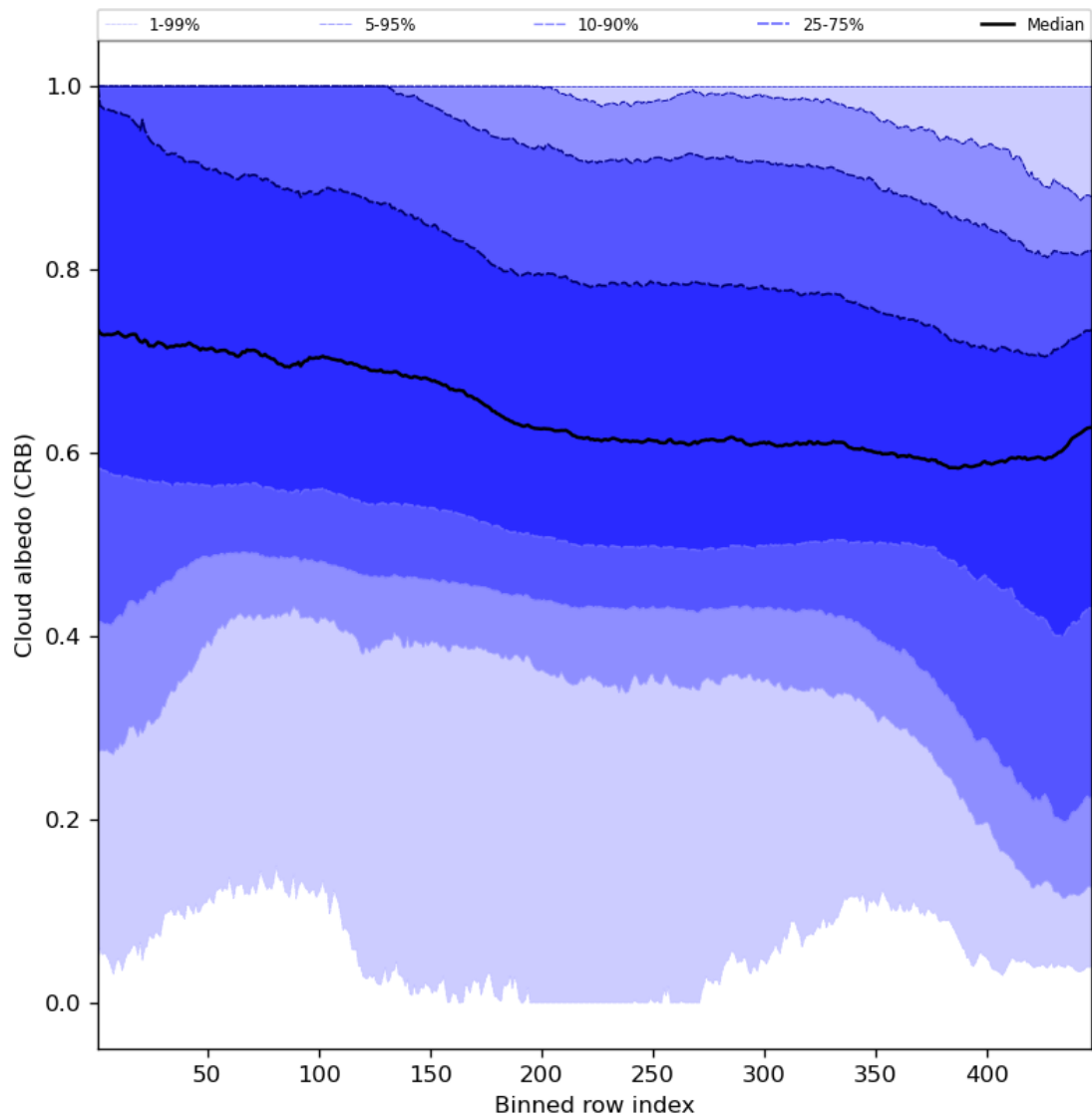
Figure 60: Along track statistics of “Cloud albedo (CRB)” for 2023-11-23 to 2023-11-24
