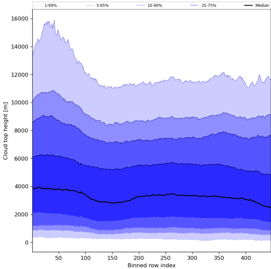
Figure 56: Along track statistics of “Cloud top height” for 2023-11-23 to 2023-11-24
