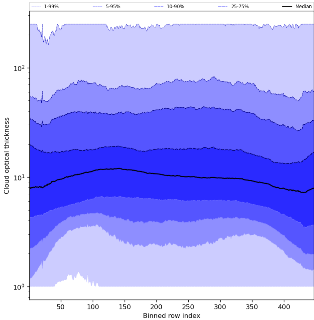
Figure 57: Along track statistics of “Cloud optical thickness” for 2023-11-23 to 2023-11-24
