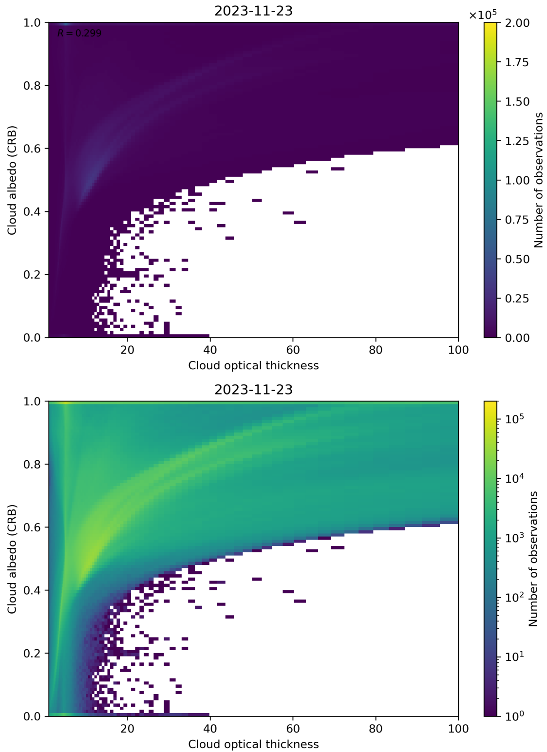
Figure 82: Scatter density plot of “Cloud optical thickness” against “Cloud albedo (CRB)” for 2023-11-23 to 2023-11-24.
