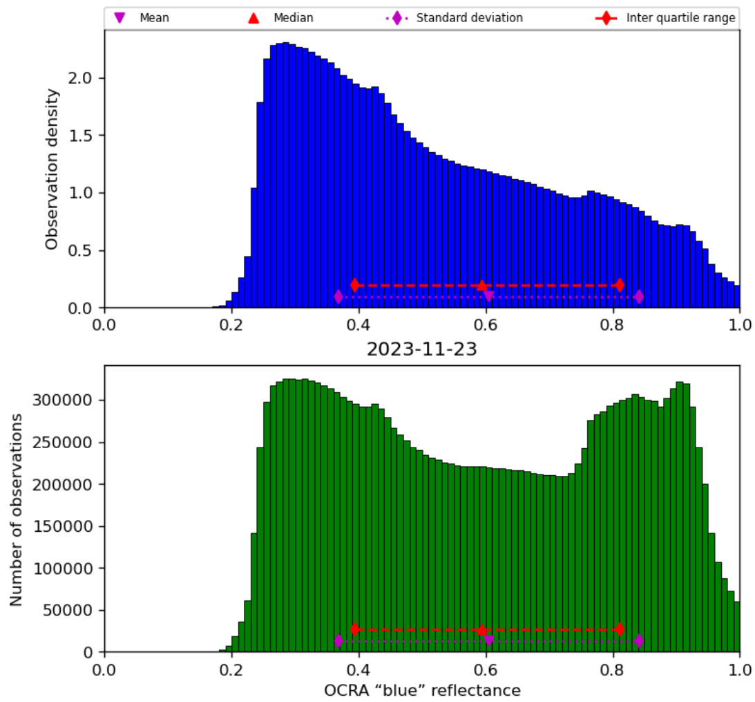
Figure 51: Histogram of “OCRA “blue” reflectance” for 2023-11-23 to 2023-11-24
