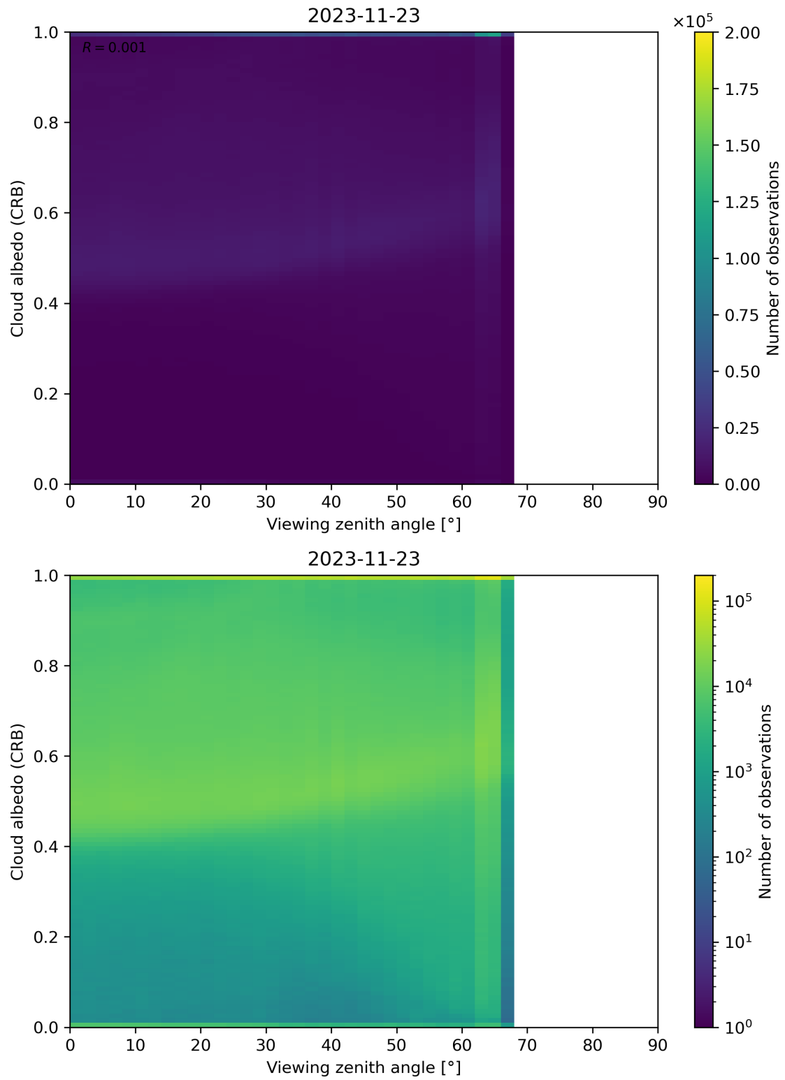
Figure 106: Scatter density plot of “Viewing zenith angle” against “Cloud albedo (CRB)” for 2023-11-23 to 2023-11-24.
