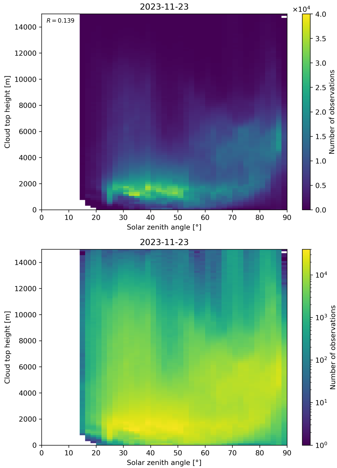
Figure 104: Scatter density plot of “Solar zenith angle” against “Cloud top height” for 2023-11-23 to 2023-11-24.
