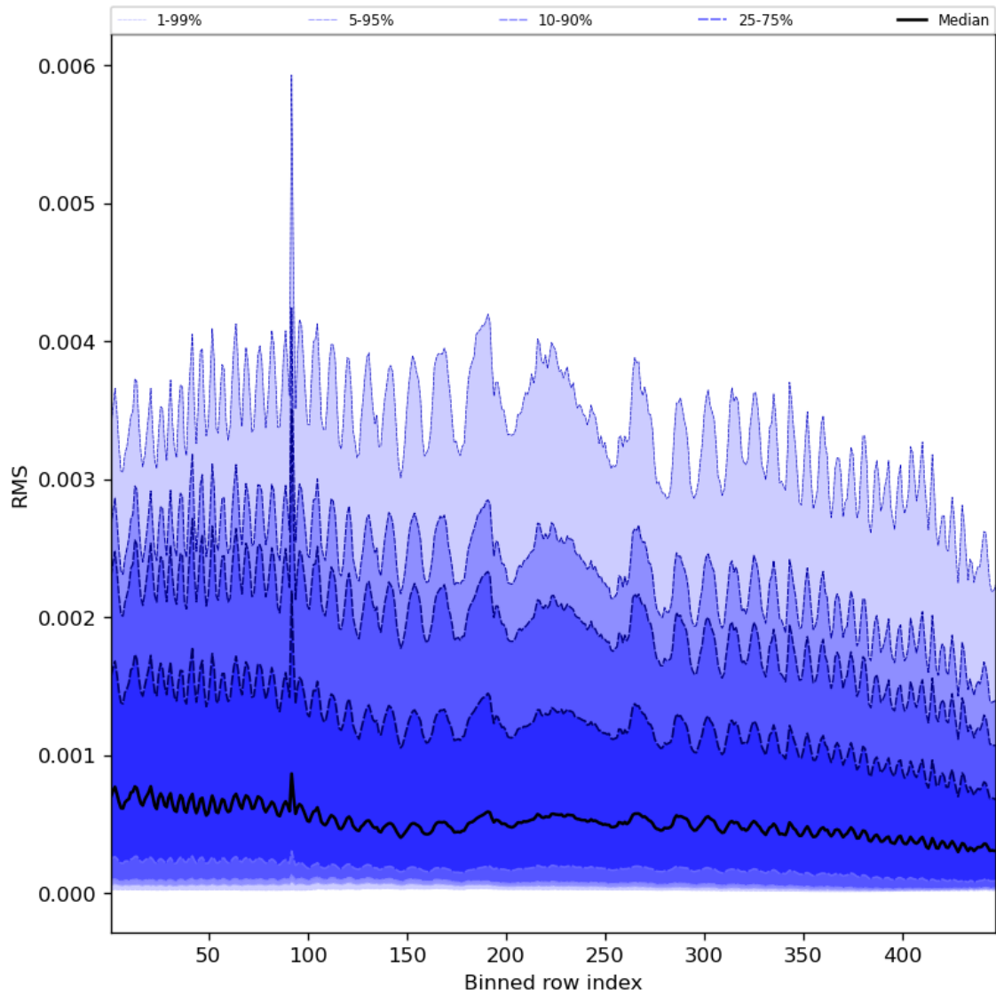
Figure 63: Along track statistics of “RMS” for 2023-11-23 to 2023-11-24
