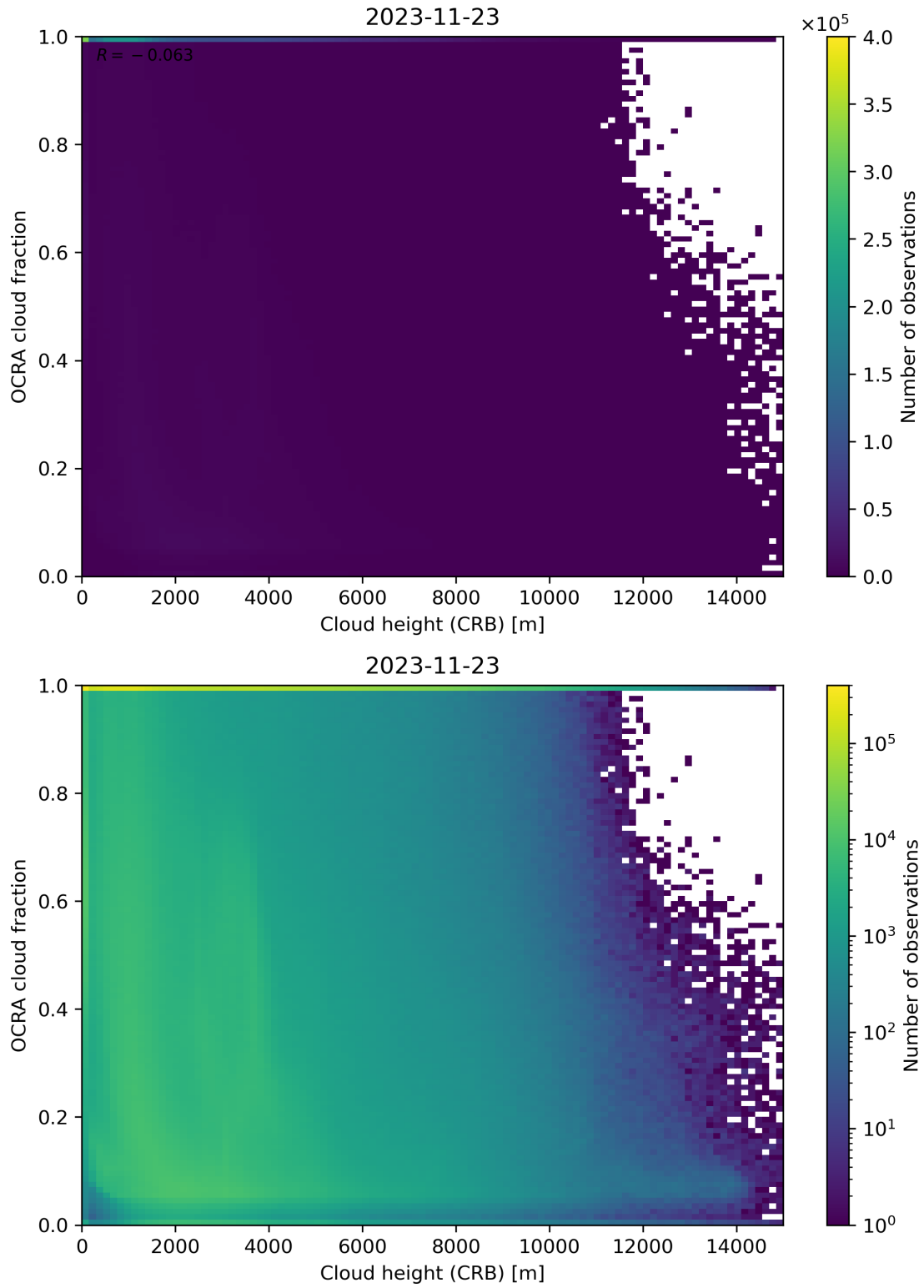
Figure 81: Scatter density plot of “Cloud height (CRB)” against “OCRA cloud fraction” for 2023-11-23 to 2023-11-24.
