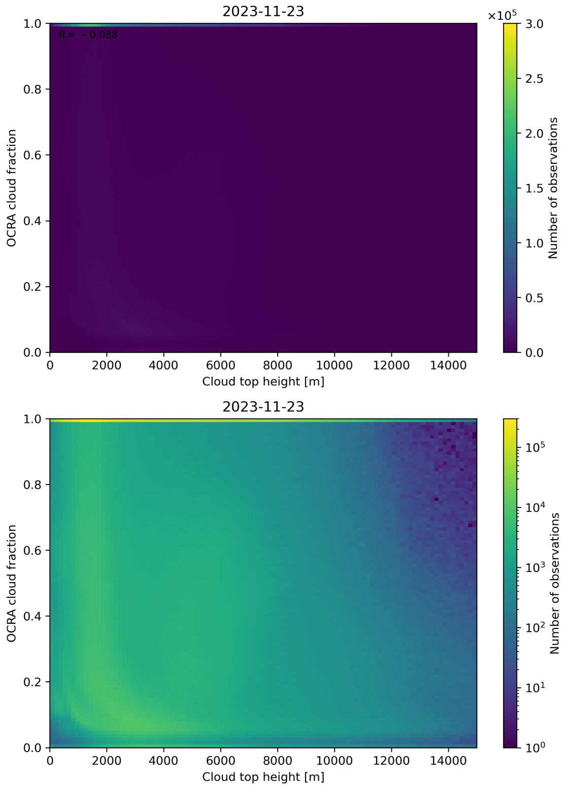
Figure 87: Scatter density plot of “Cloud top height” against “OCRA cloud fraction” for 2023-11-23 to 2023-11-24.
