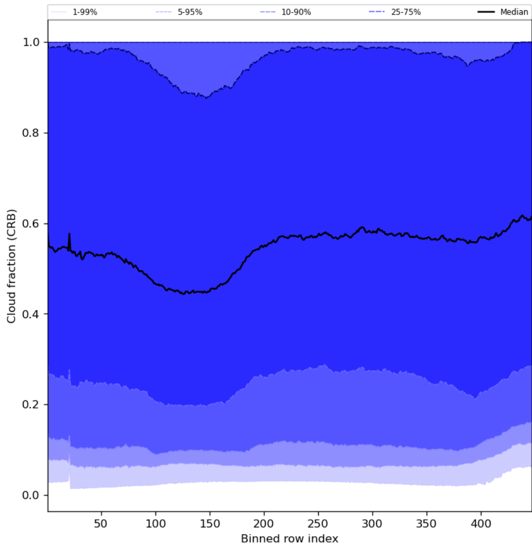
Figure 58: Along track statistics of “Cloud fraction (CRB)” for 2023-11-23 to 2023-11-24
