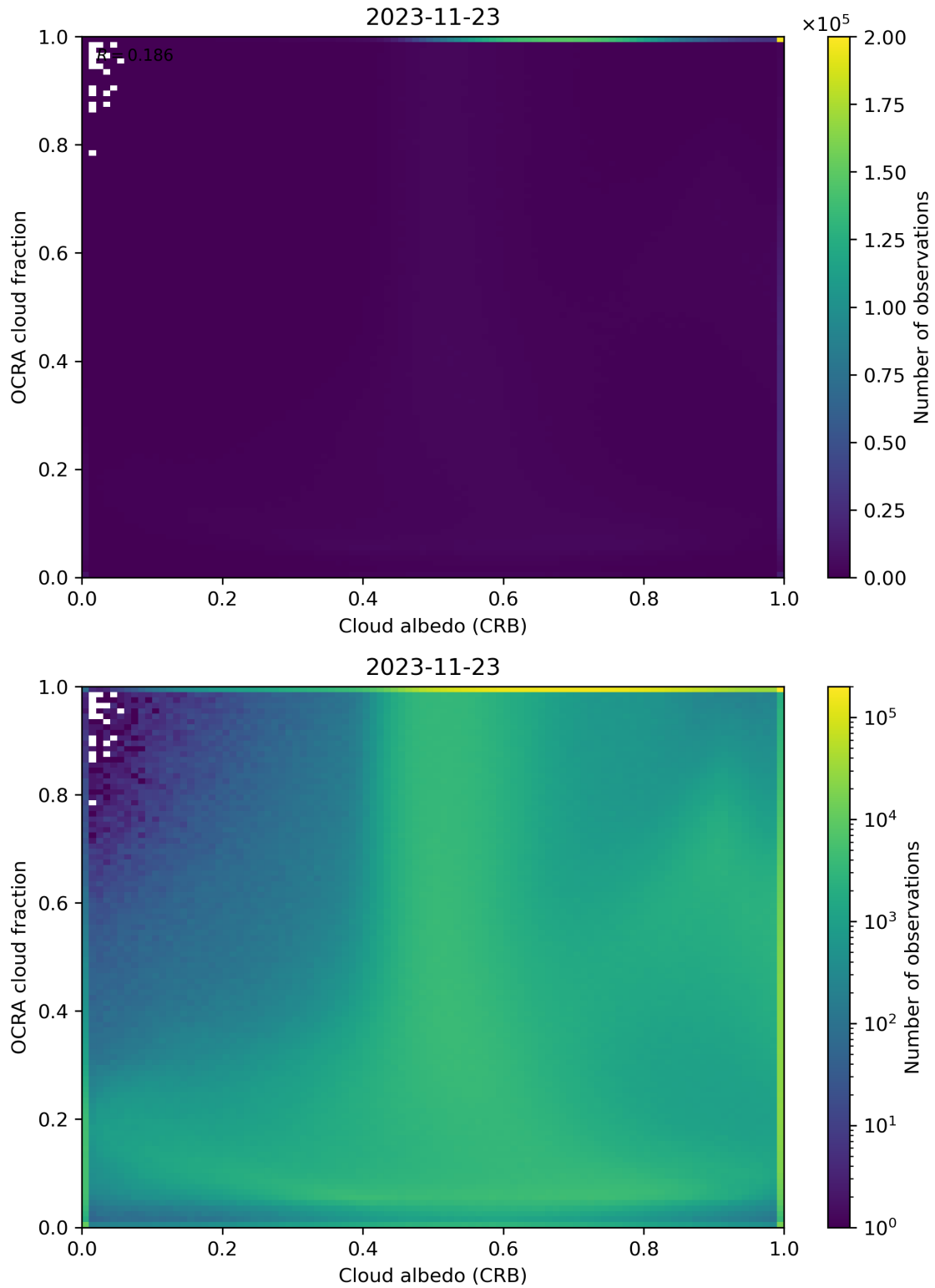
Figure 70: Scatter density plot of “Cloud albedo (CRB)” against “OCRA cloud fraction” for 2023-11-23 to 2023-11-24.
