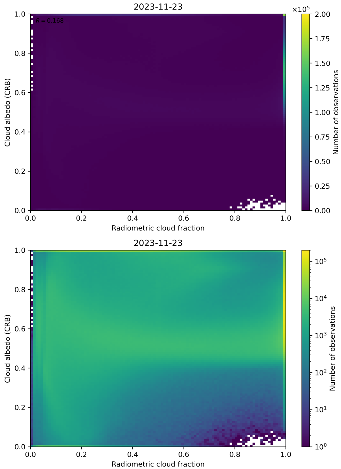
Figure 71: Scatter density plot of “Radiometric cloud fraction” against “Cloud albedo (CRB)” for 2023-11-23 to 2023-11-24.
