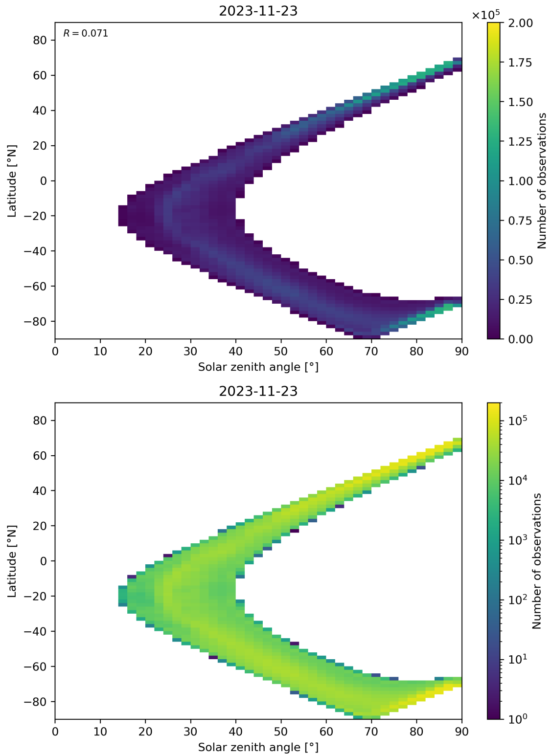
Figure 105: Scatter density plot of “Solar zenith angle” against “Latitude” for 2023-11-23 to 2023-11-24.
