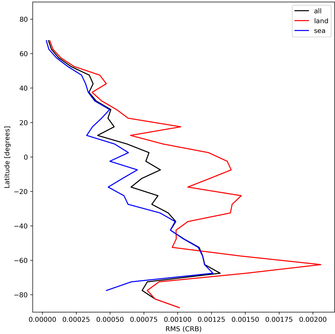
Figure 32: Zonal average of “RMS (CRB)” for 2023-11-23 to 2023-11-24.
