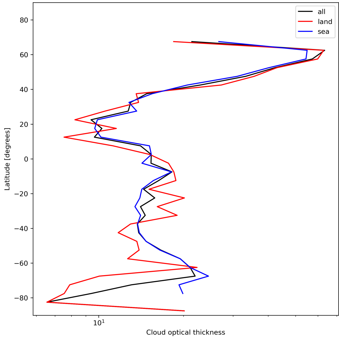
Figure 25: Zonal average of “Cloud optical thickness” for 2023-11-23 to 2023-11-24.
