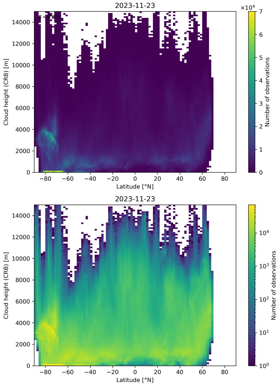
Figure 95: Scatter density plot of “Latitude” against “Cloud height (CRB)” for 2023-11-23 to 2023-11-24.
