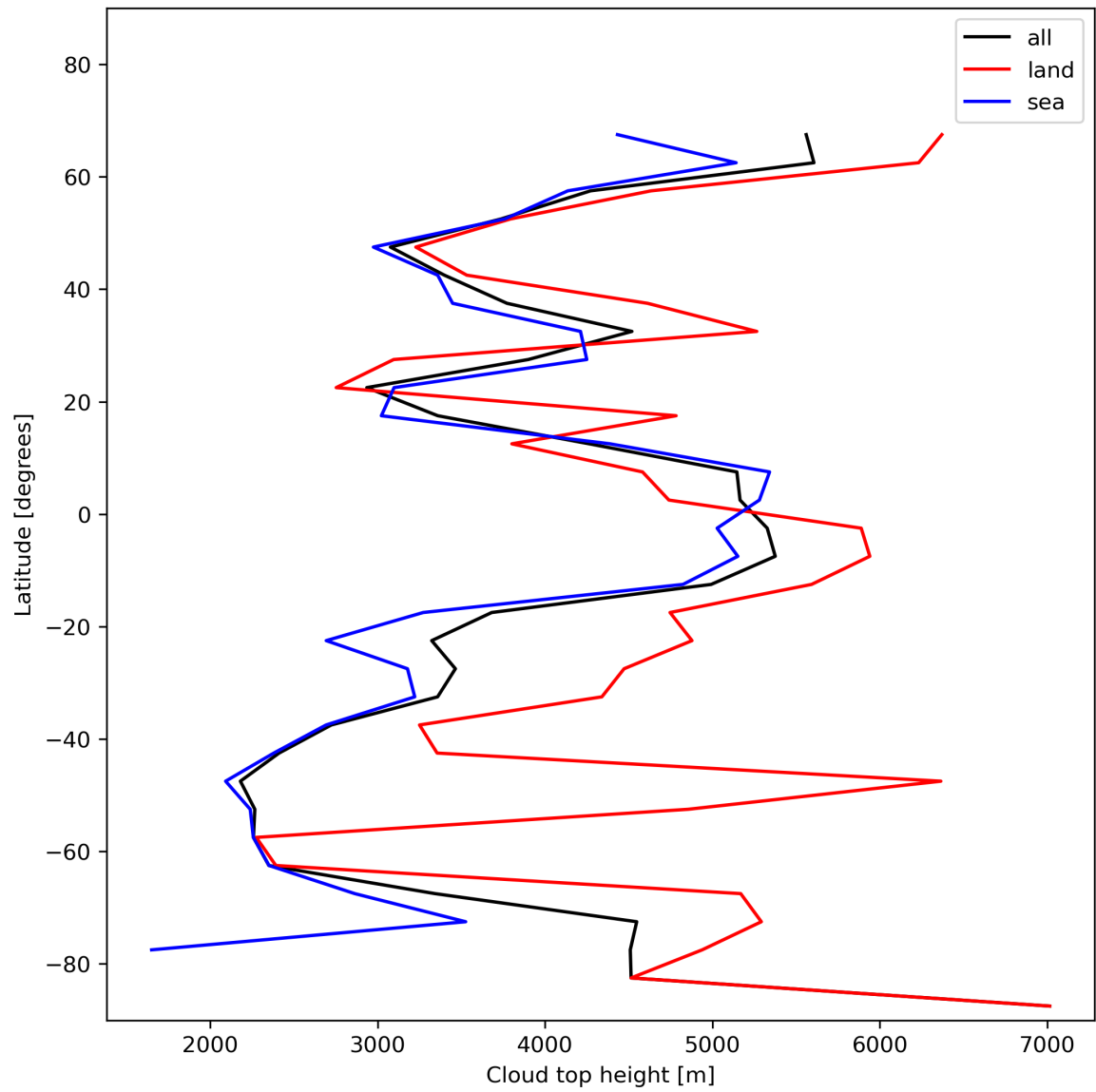
Figure 24: Zonal average of “Cloud top height” for 2023-11-23 to 2023-11-24.
