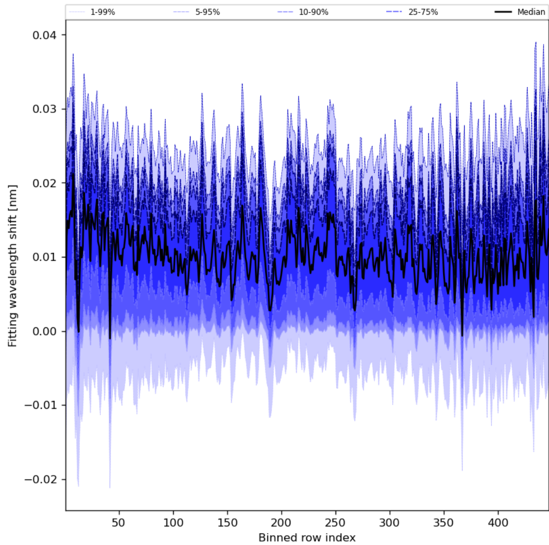
Figure 65: Along track statistics of “Fitting wavelength shift” for 2023-11-23 to 2023-11-24
