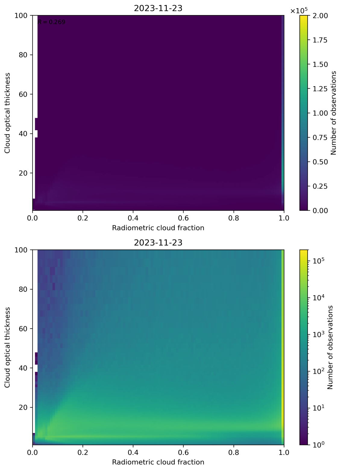
Figure 75: Scatter density plot of “Radiometric cloud fraction” against “Cloud optical thickness” for 2023-11-23 to 2023-11-24.
