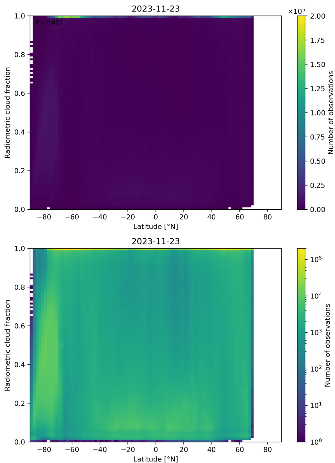
Figure 92: Scatter density plot of “Latitude” against “Radiometric cloud fraction” for 2023-11-23 to 2023-11-24.
