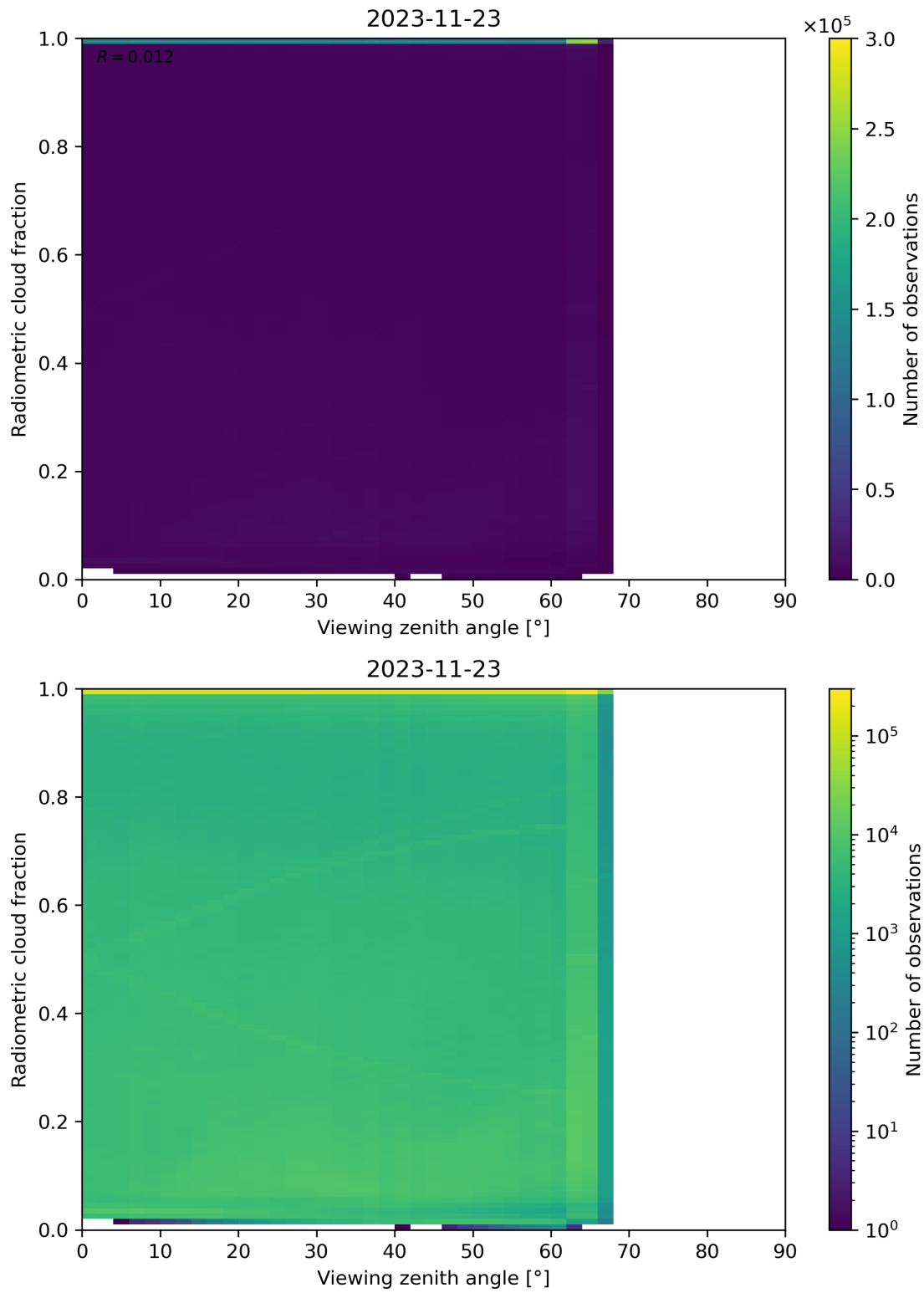
Figure 107: Scatter density plot of “Viewing zenith angle” against “Radiometric cloud fraction” for 2023-11-23 to 2023-11-24.
