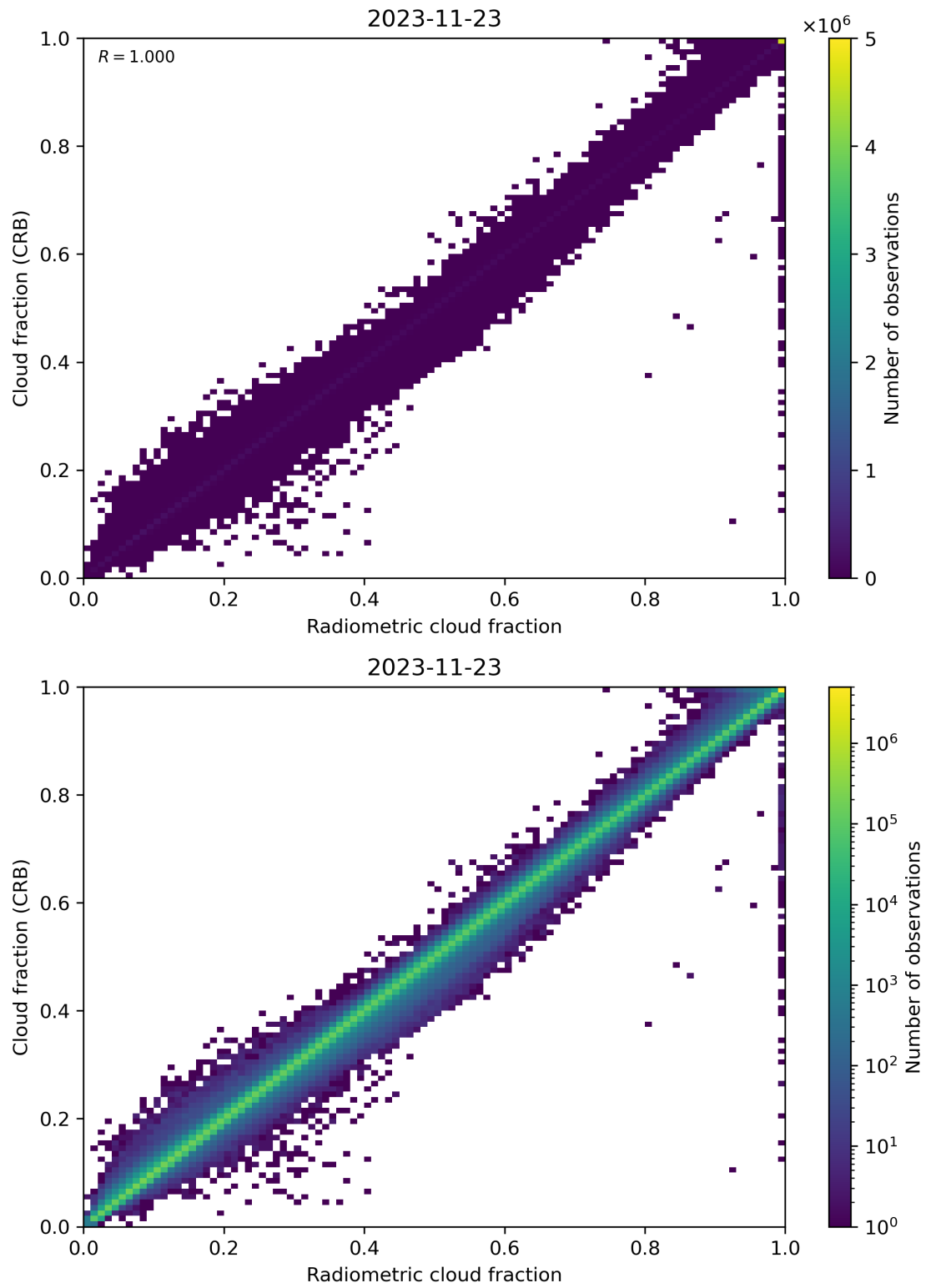
Figure 73: Scatter density plot of “Radiometric cloud fraction” against “Cloud fraction (CRB)” for 2023-11-23 to 2023-11-24.
