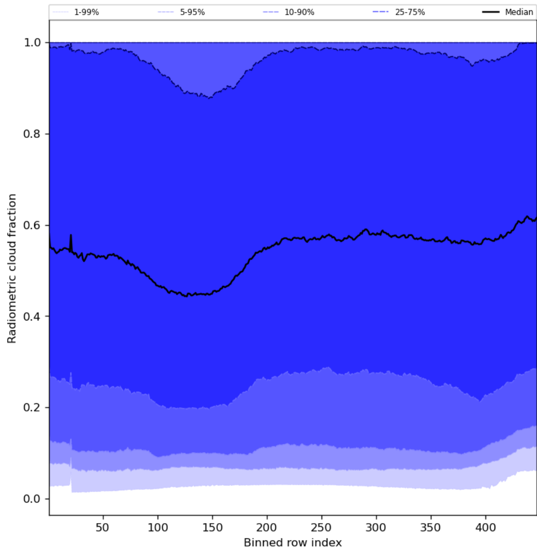
Figure 55: Along track statistics of “Radiometric cloud fraction” for 2023-11-23 to 2023-11-24
