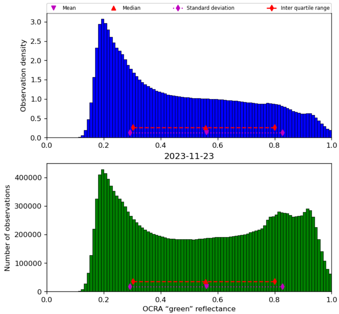
Figure 52: Histogram of “OCRA “green” reflectance” for 2023-11-23 to 2023-11-24
