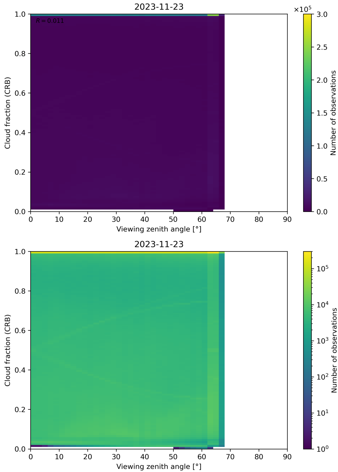
Figure 109: Scatter density plot of “Viewing zenith angle” against “Cloud fraction (CRB)” for 2023-11-23 to 2023-11-24.
