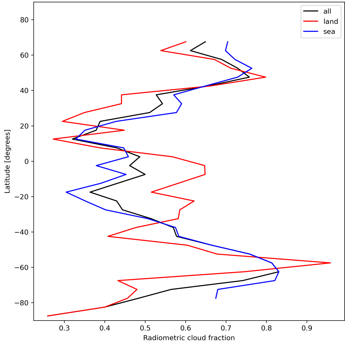
Figure 23: Zonal average of “Radiometric cloud fraction” for 2023-11-23 to 2023-11-24.
