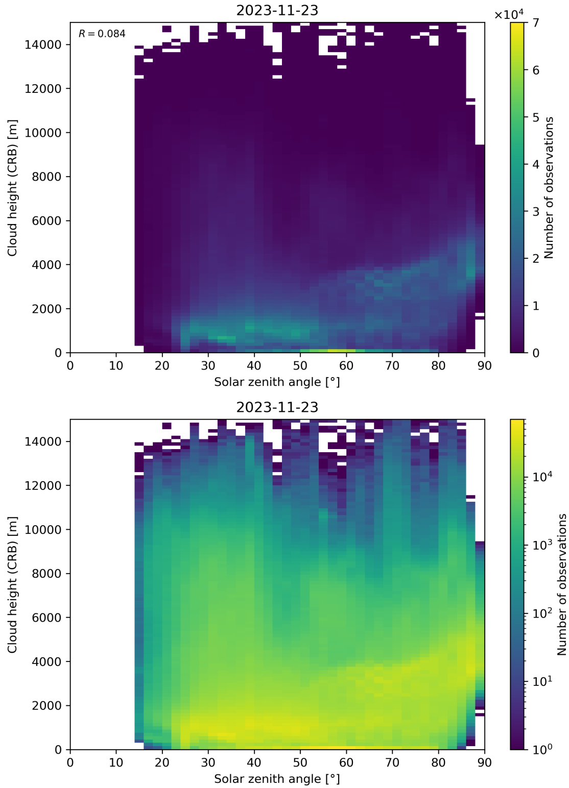
Figure 102: Scatter density plot of “Solar zenith angle” against “Cloud height (CRB)” for 2023-11-23 to 2023-11-24.
