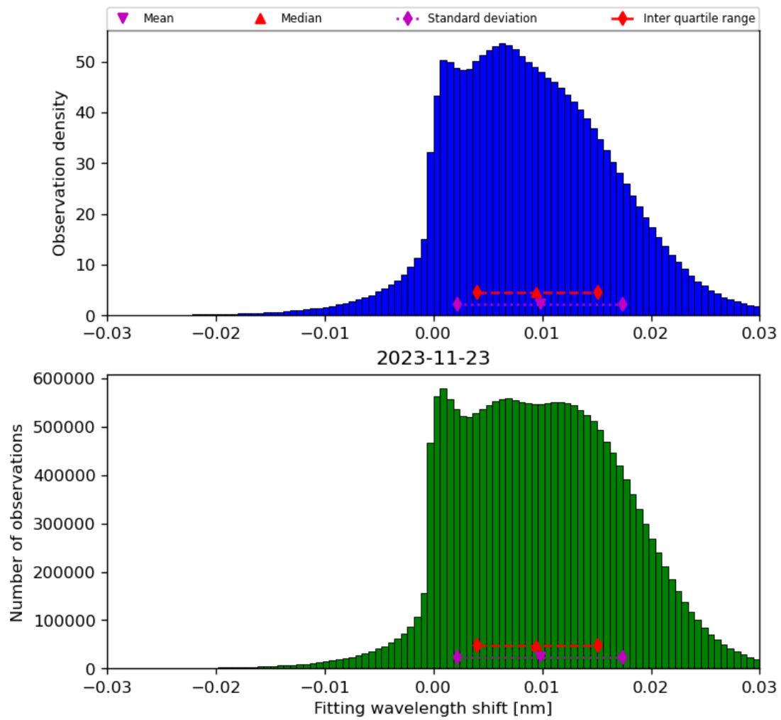
Figure 49: Histogram of “Fitting wavelength shift” for 2023-11-23 to 2023-11-24
