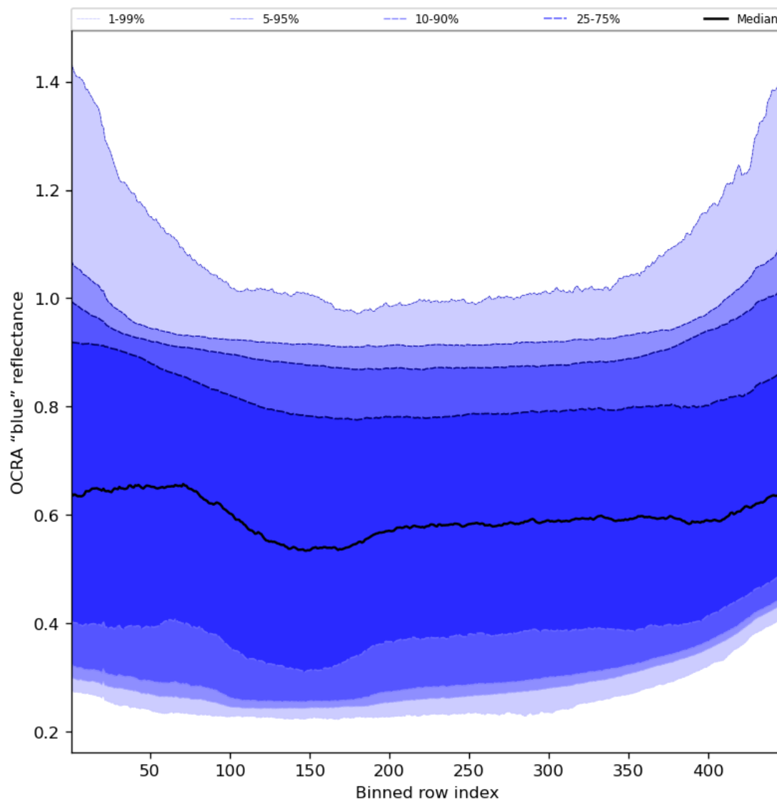
Figure 67: Along track statistics of “OCRA “blue” reflectance” for 2023-11-23 to 2023-11-24
