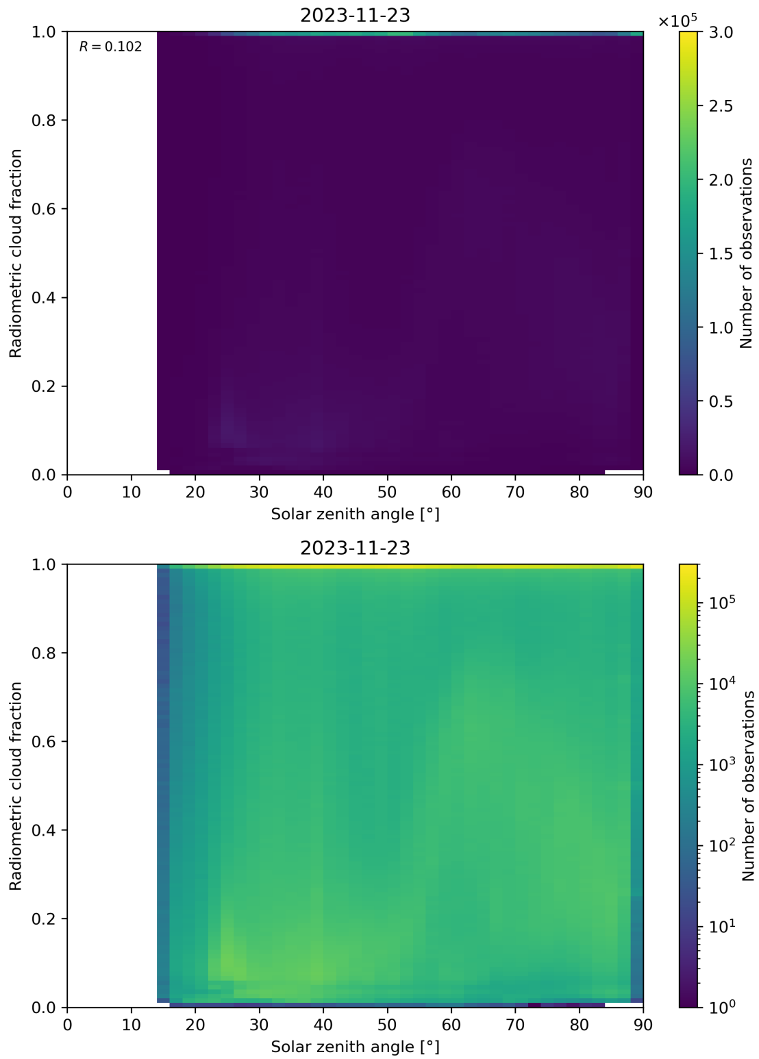
Figure 99: Scatter density plot of “Solar zenith angle” against “Radiometric cloud fraction” for 2023-11-23 to 2023-11-24.
