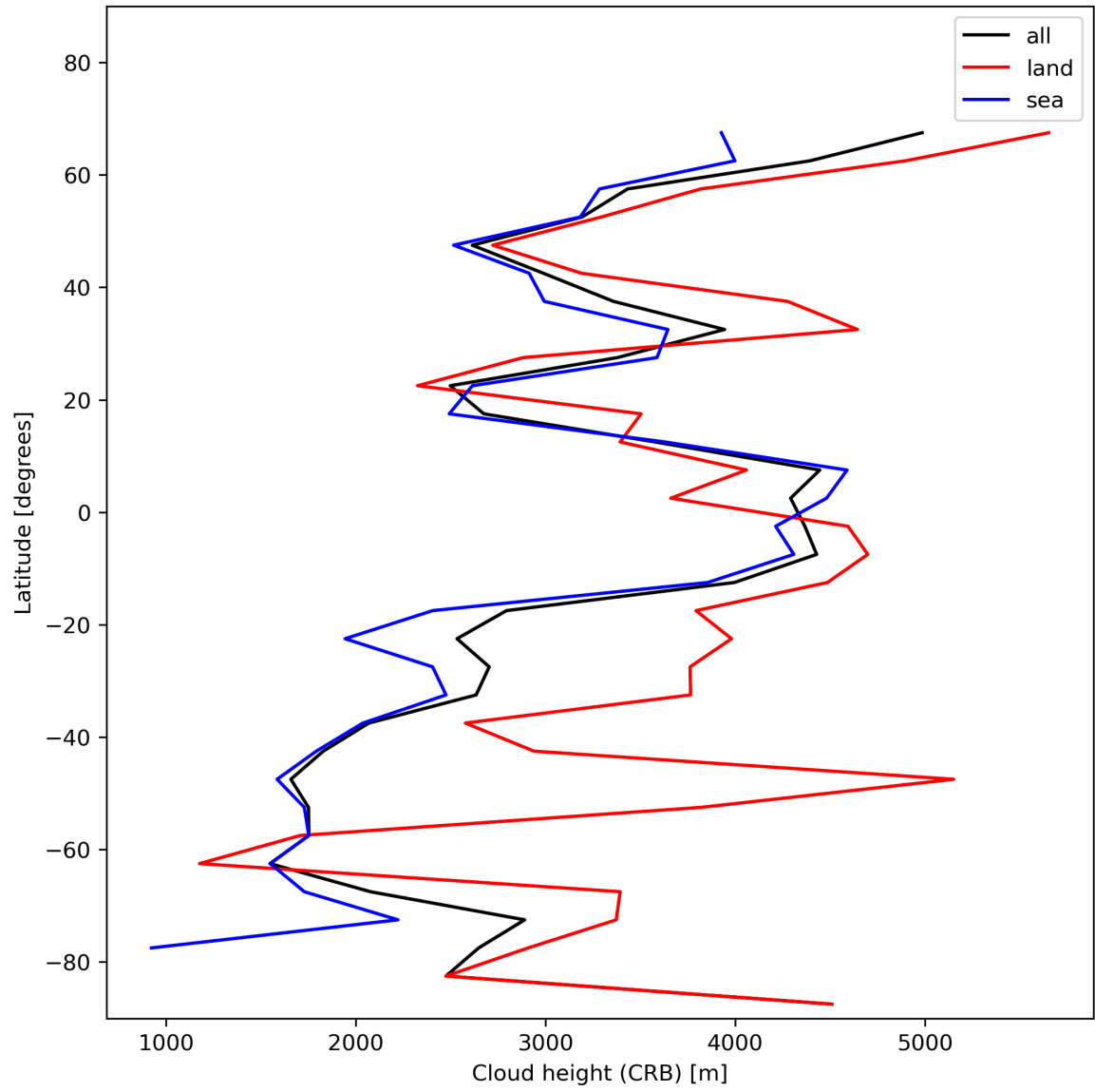
Figure 27: Zonal average of “Cloud height (CRB)” for 2023-11-23 to 2023-11-24.
