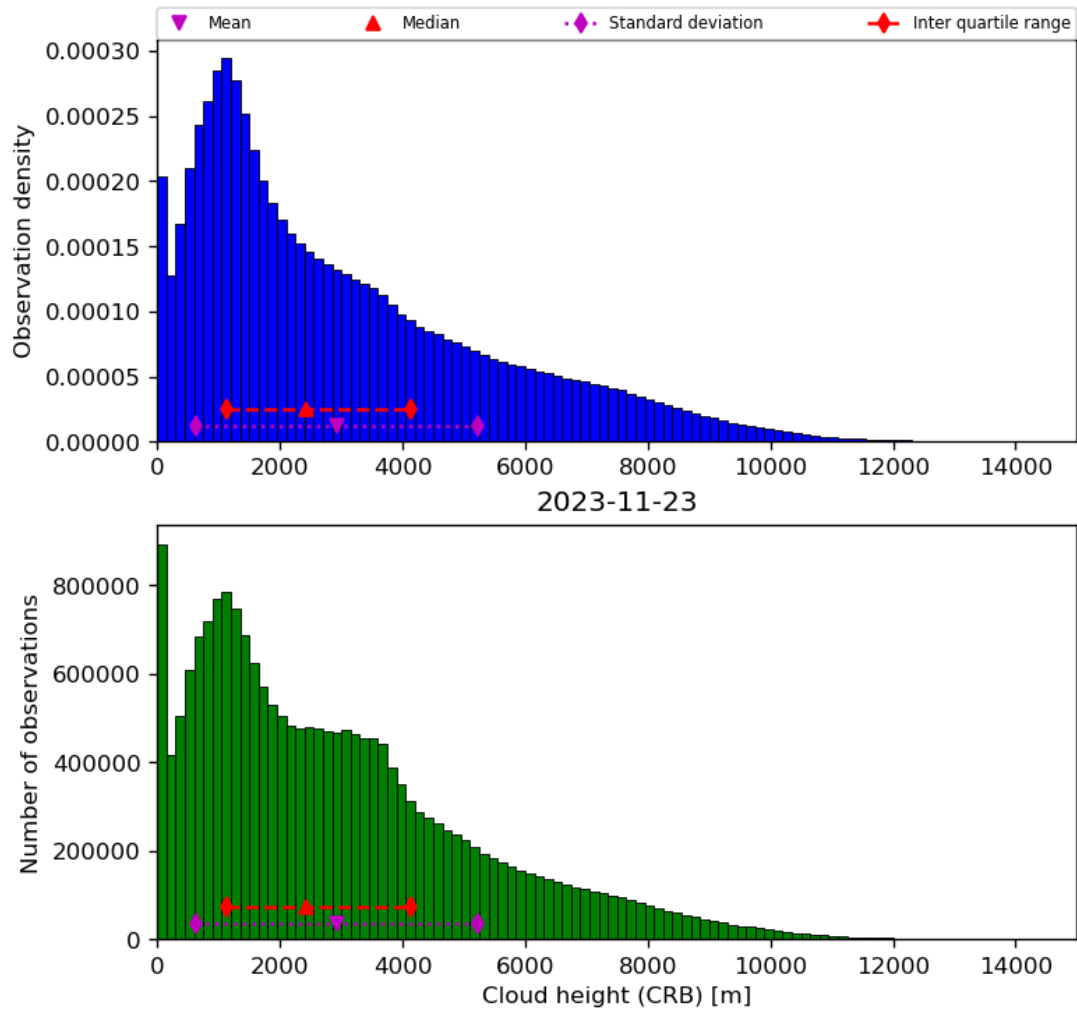
Figure 43: Histogram of “Cloud height (CRB)” for 2023-11-23 to 2023-11-24
