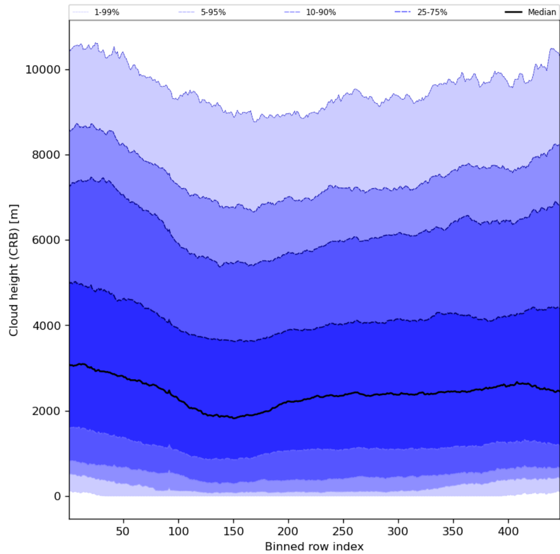
Figure 59: Along track statistics of “Cloud height (CRB)” for 2023-11-23 to 2023-11-24
