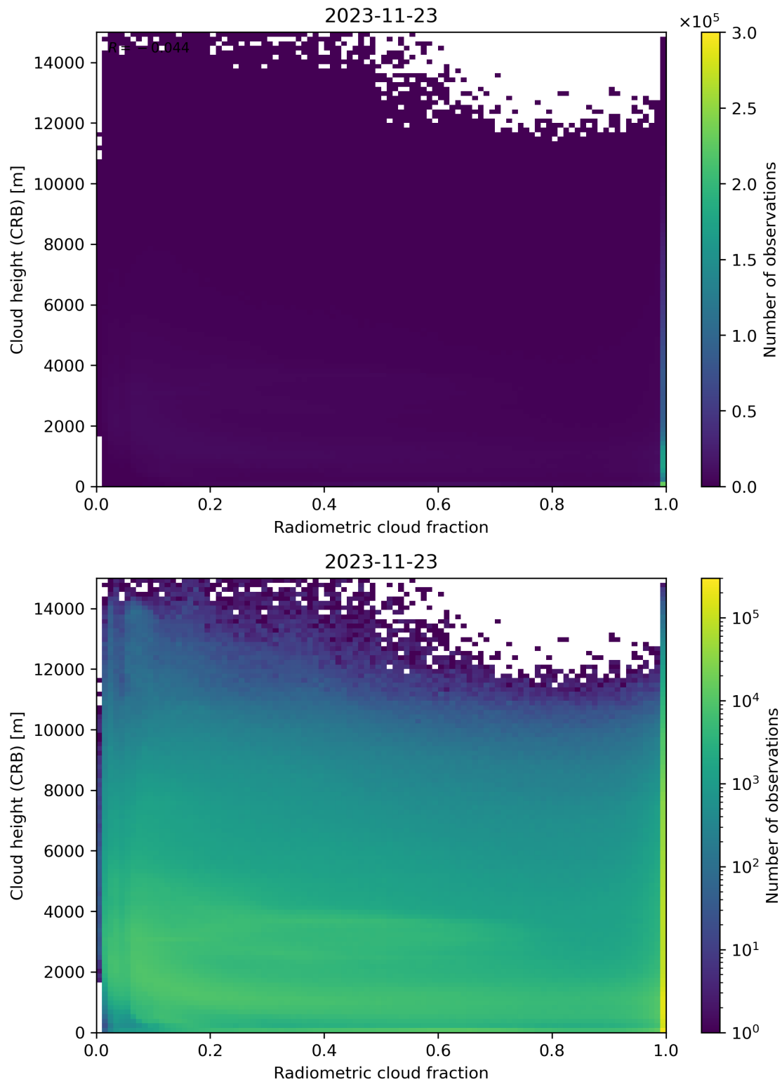
Figure 74: Scatter density plot of “Radiometric cloud fraction” against “Cloud height (CRB)” for 2023-11-23 to 2023-11-24.
