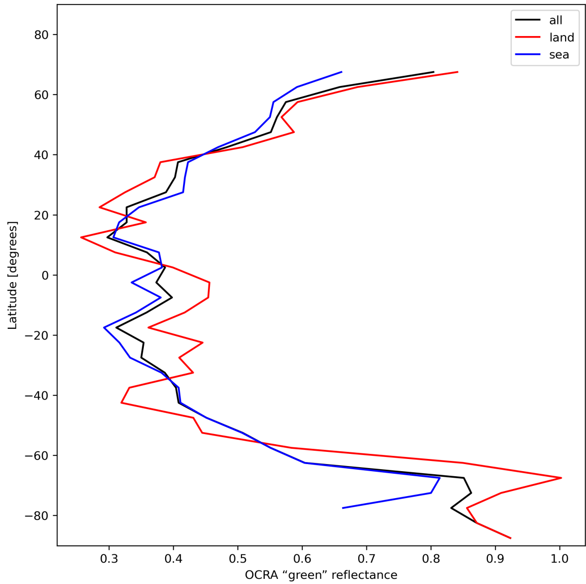
Figure 36: Zonal average of “OCRA “green” reflectance” for 2023-11-23 to 2023-11-24.
