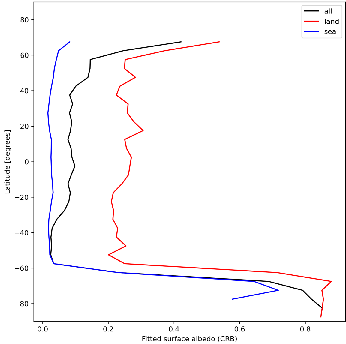
Figure 30: Zonal average of “Fitted surface albedo (CRB)” for 2023-11-23 to 2023-11-24.
