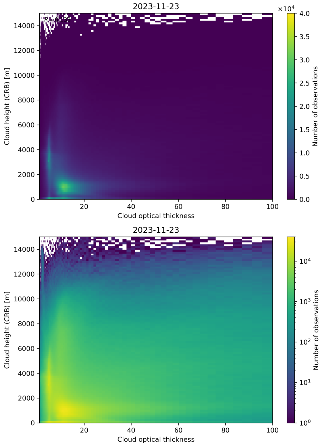
Figure 85: Scatter density plot of “Cloud optical thickness” against “Cloud height (CRB)” for 2023-11-23 to 2023-11-24.
