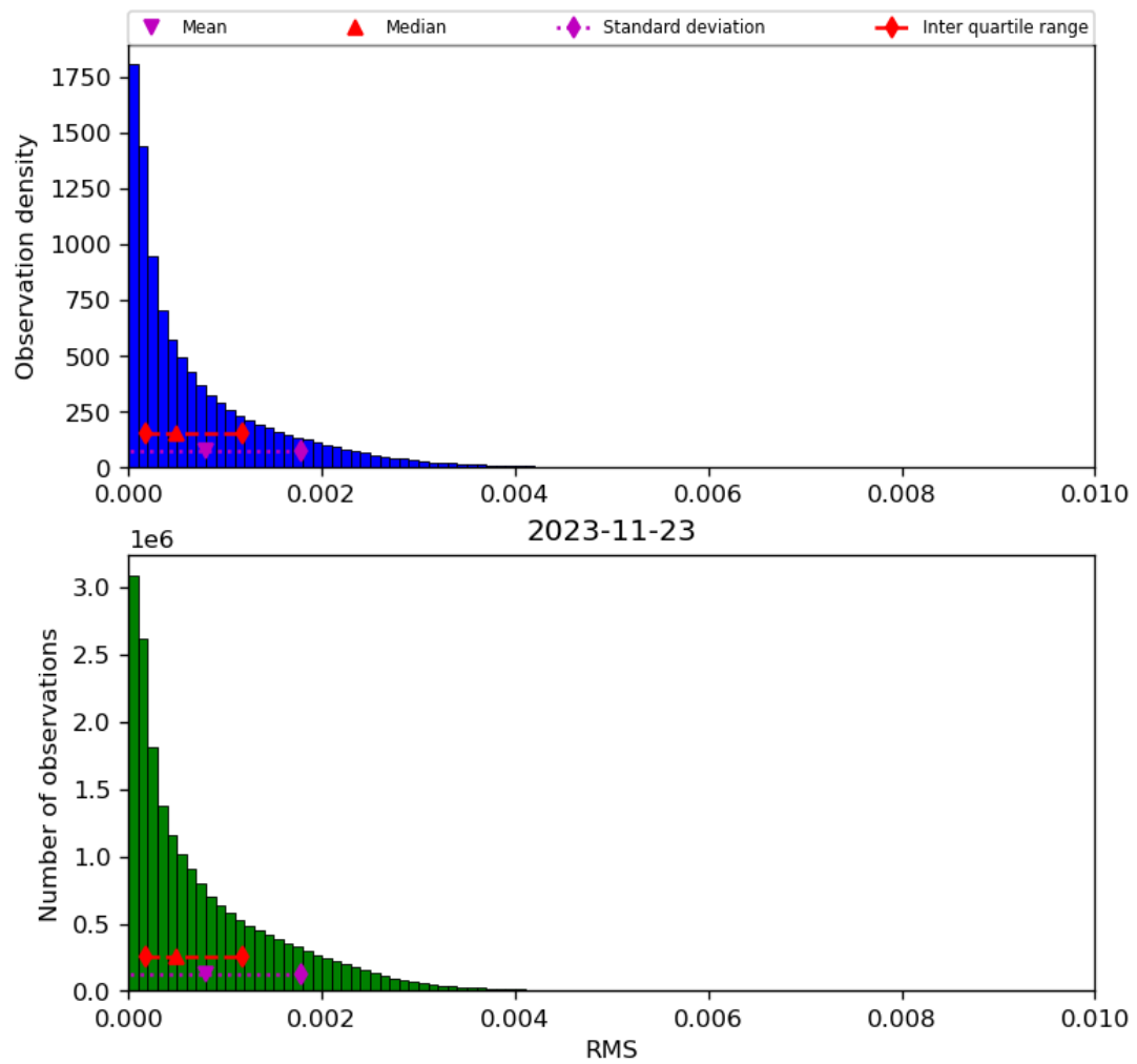
Figure 47: Histogram of “RMS” for 2023-11-23 to 2023-11-24
