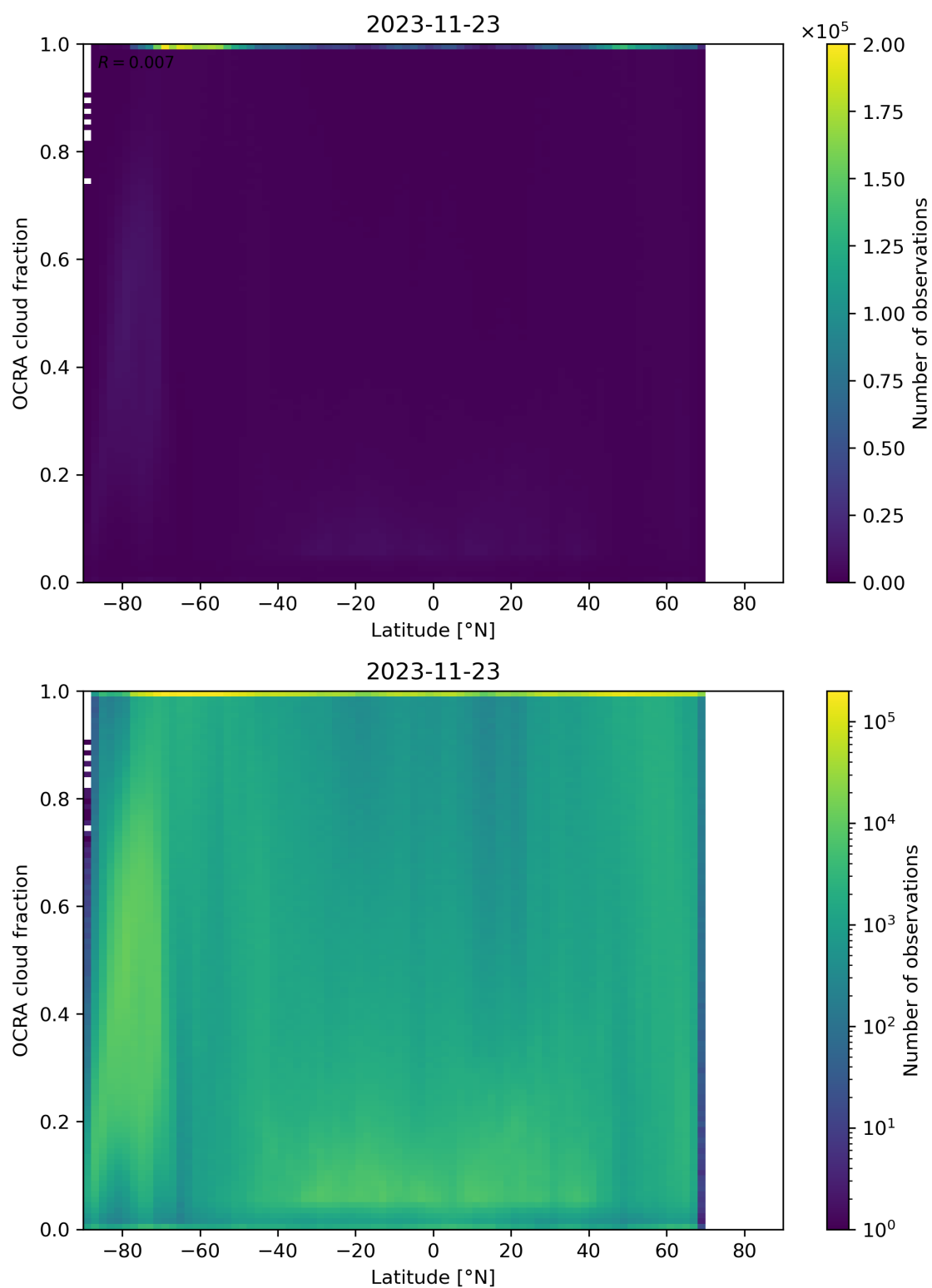
Figure 93: Scatter density plot of “Latitude” against “OCRA cloud fraction” for 2023-11-23 to 2023-11-24.
