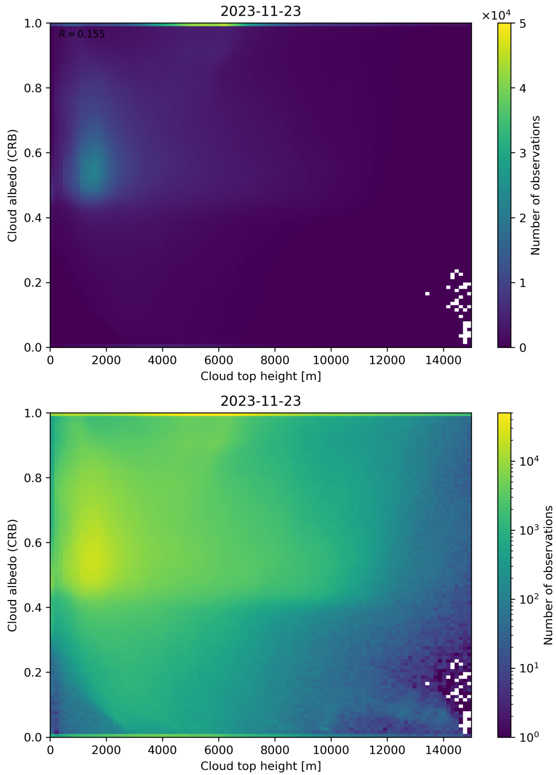
Figure 86: Scatter density plot of “Cloud top height” against “Cloud albedo (CRB)” for 2023-11-23 to 2023-11-24.
