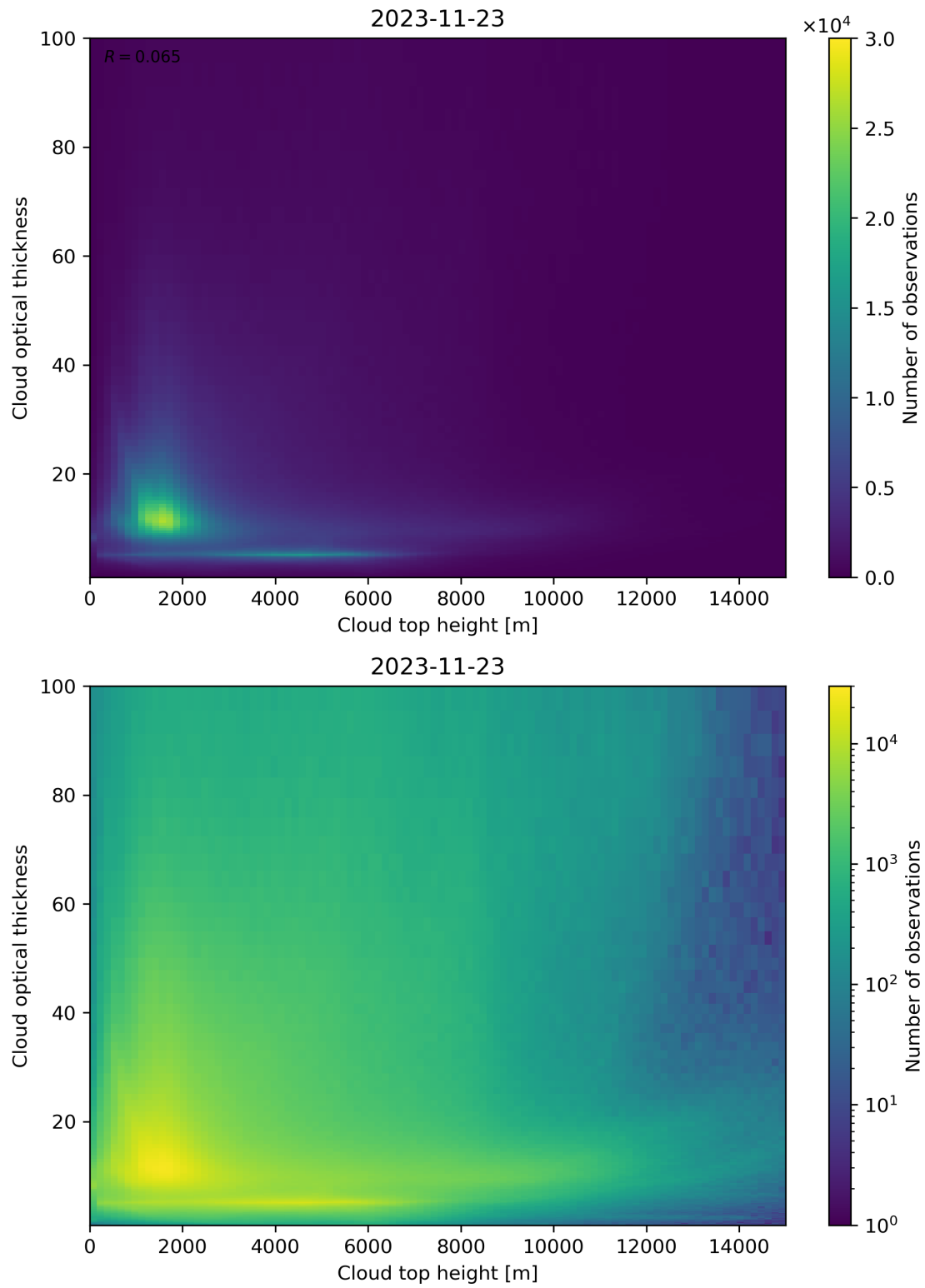
Figure 90: Scatter density plot of “Cloud top height” against “Cloud optical thickness” for 2023-11-23 to 2023-11-24.
