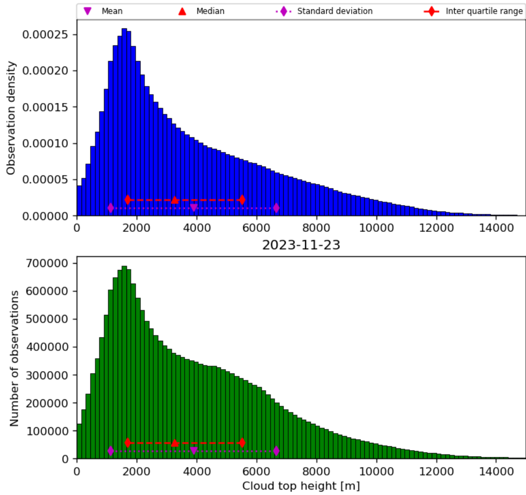
Figure 40: Histogram of “Cloud top height” for 2023-11-23 to 2023-11-24
