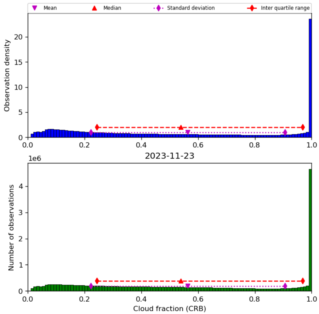
Figure 42: Histogram of “Cloud fraction (CRB)” for 2023-11-23 to 2023-11-24
