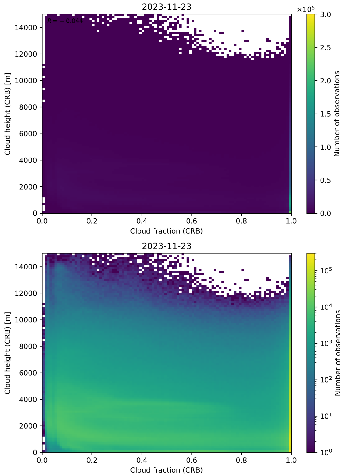
Figure 79: Scatter density plot of “Cloud fraction (CRB)” against “Cloud height (CRB)” for 2023-11-23 to 2023-11-24.
