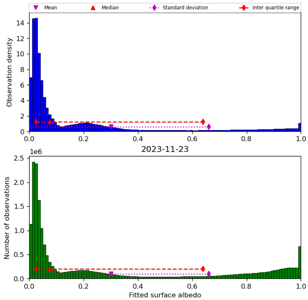
Figure 45: Histogram of “Fitted surface albedo” for 2023-11-23 to 2023-11-24
