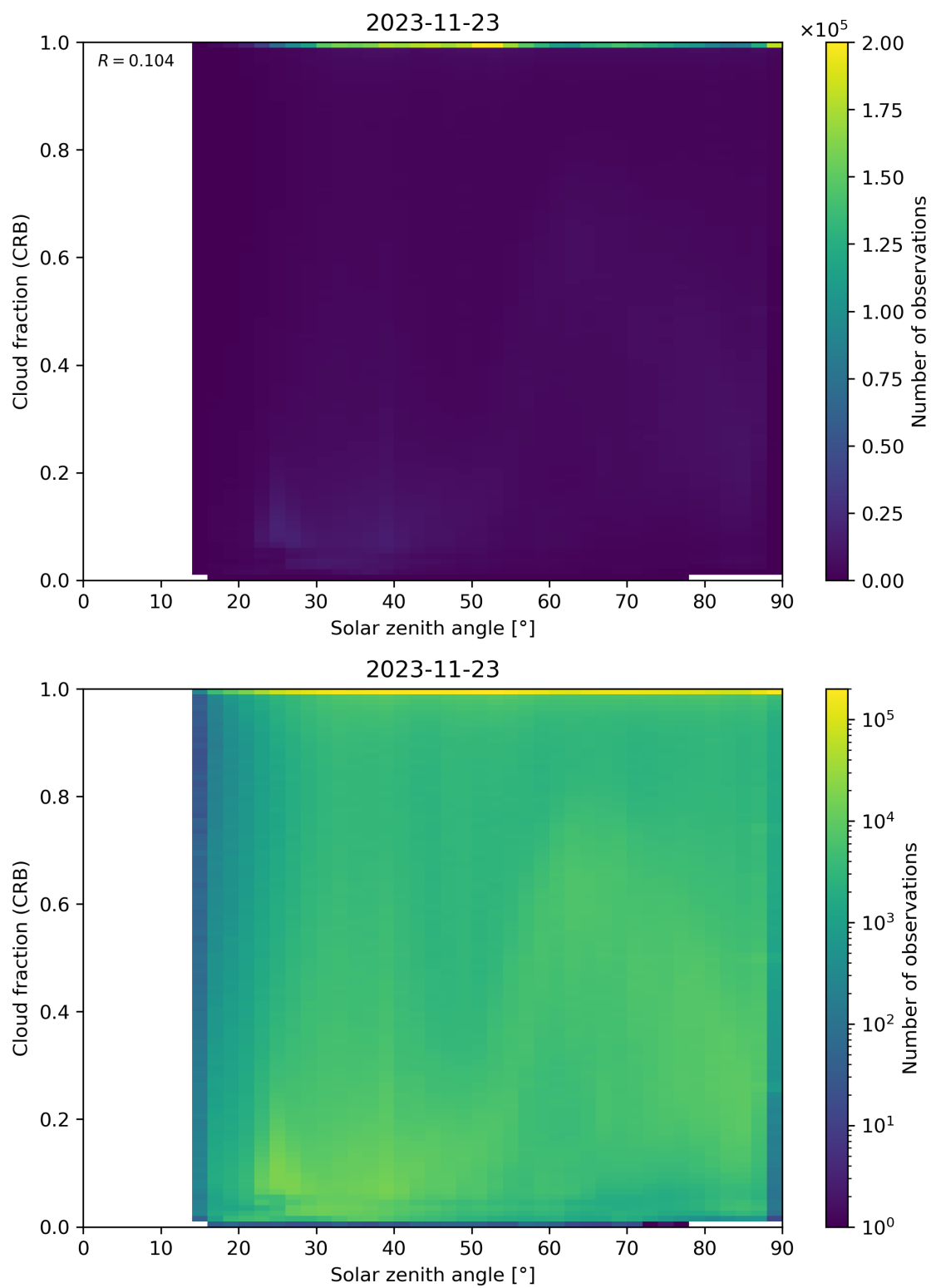
Figure 101: Scatter density plot of “Solar zenith angle” against “Cloud fraction (CRB)” for 2023-11-23 to 2023-11-24.
