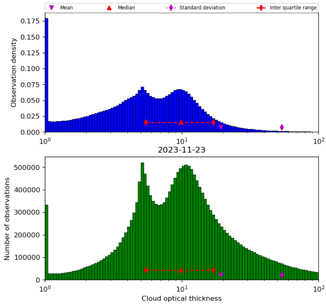
Figure 41: Histogram of “Cloud optical thickness” for 2023-11-23 to 2023-11-24
