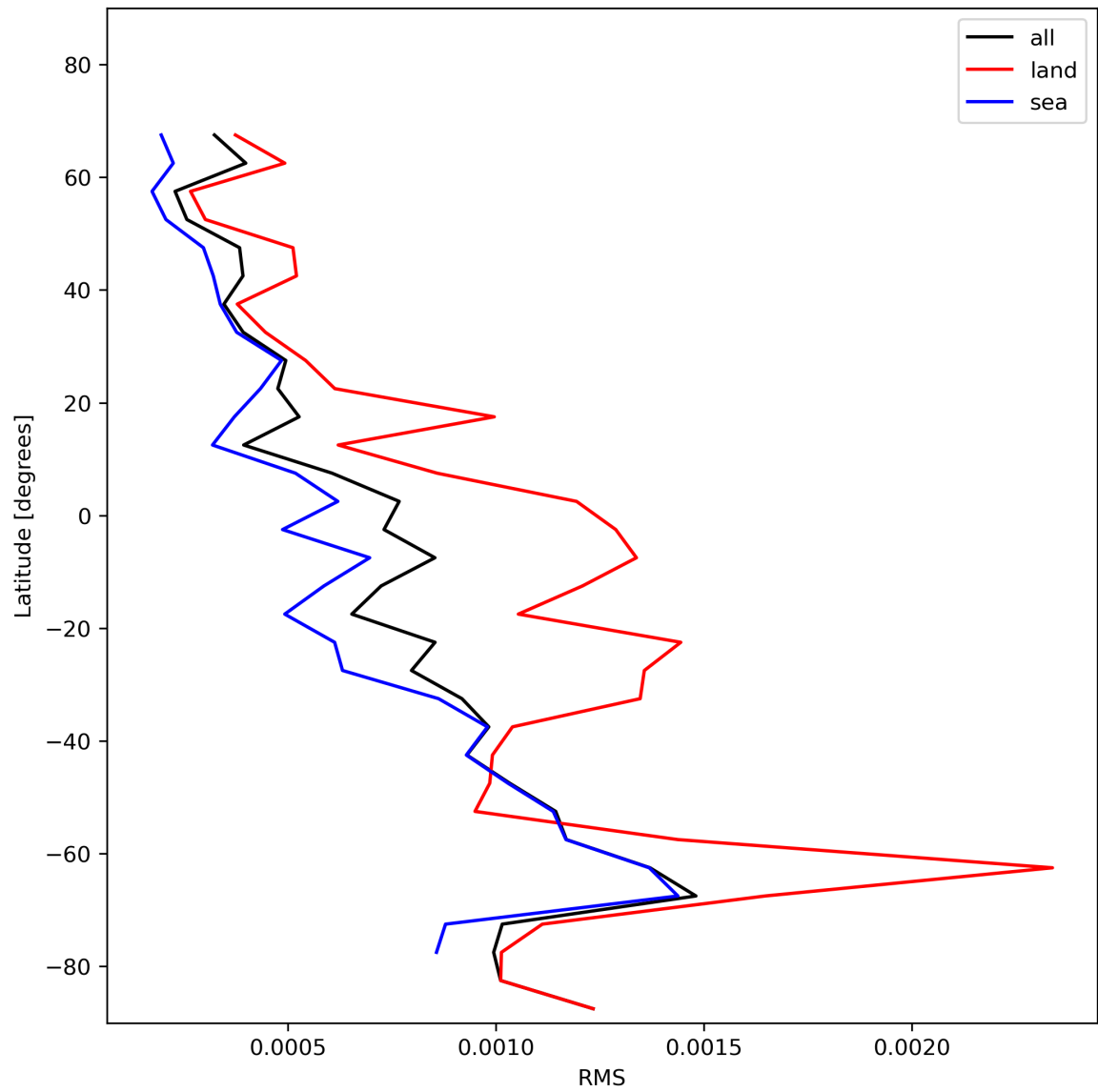
Figure 31: Zonal average of “RMS” for 2023-11-23 to 2023-11-24.
