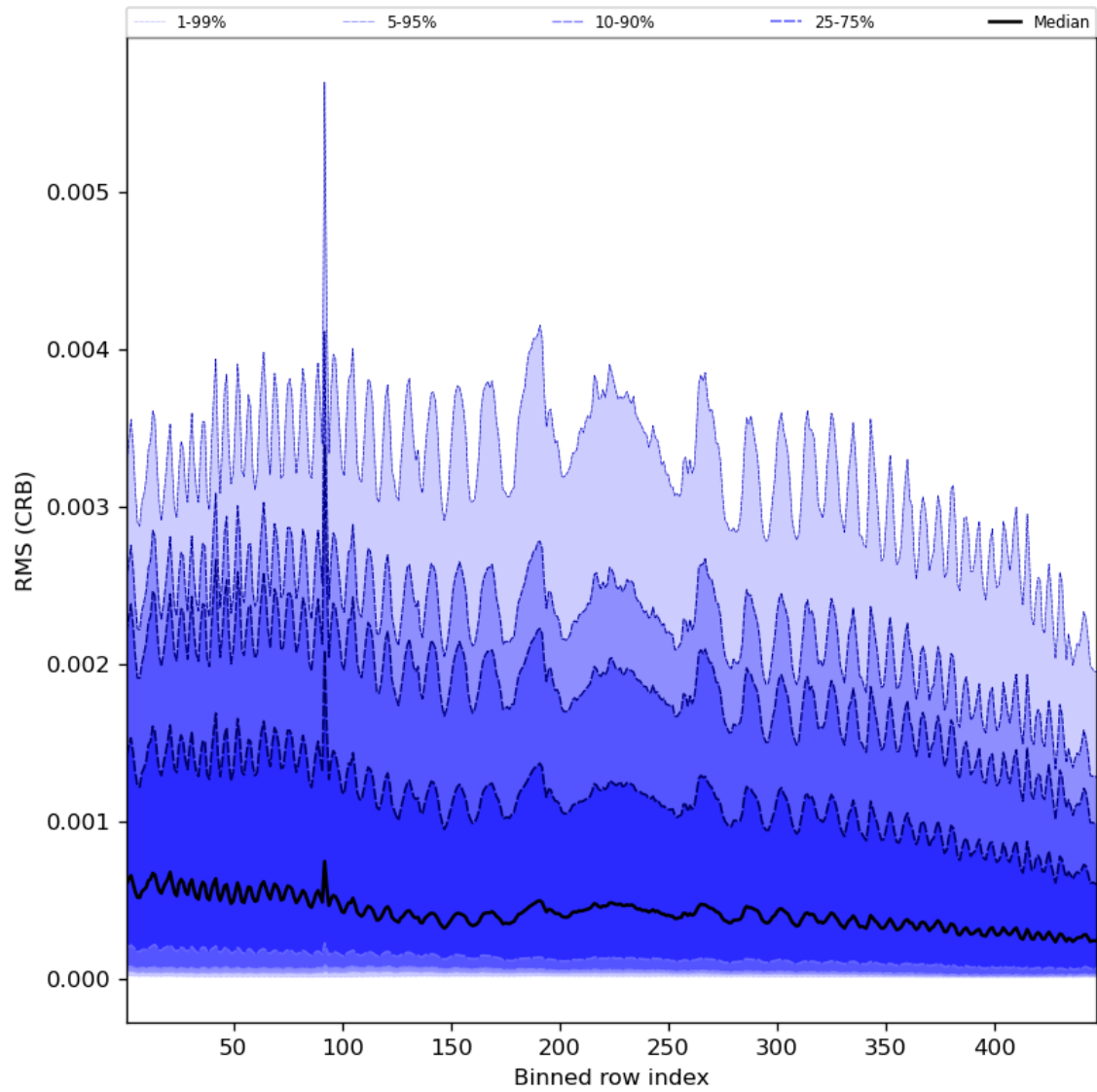
Figure 64: Along track statistics of “RMS (CRB)” for 2023-11-23 to 2023-11-24
