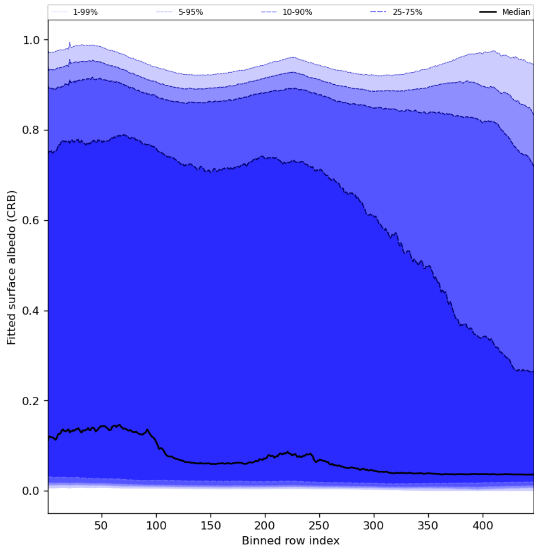
Figure 62: Along track statistics of “Fitted surface albedo (CRB)” for 2023-11-23 to 2023-11-24
