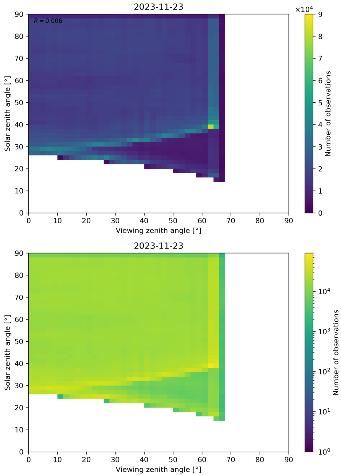
Figure 114: Scatter density plot of “Viewing zenith angle” against “Solar zenith angle” for 2023-11-23 to 2023-11-24.
