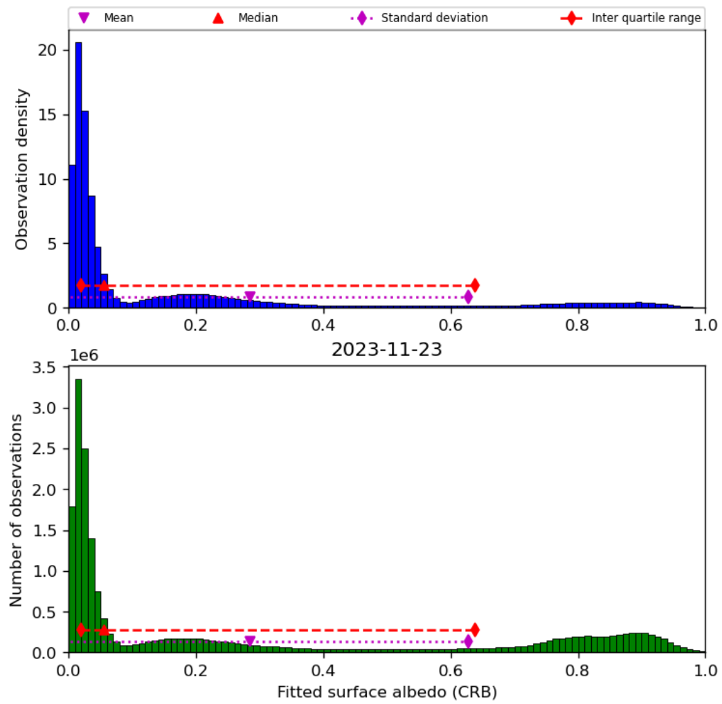
Figure 46: Histogram of “Fitted surface albedo (CRB)” for 2023-11-23 to 2023-11-24
