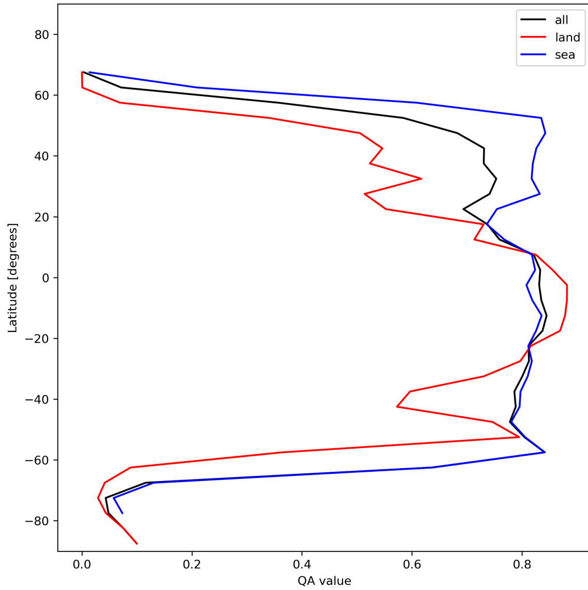
Figure 22: Zonal average of “QA value” for 2023-11-23 to 2023-11-24.
