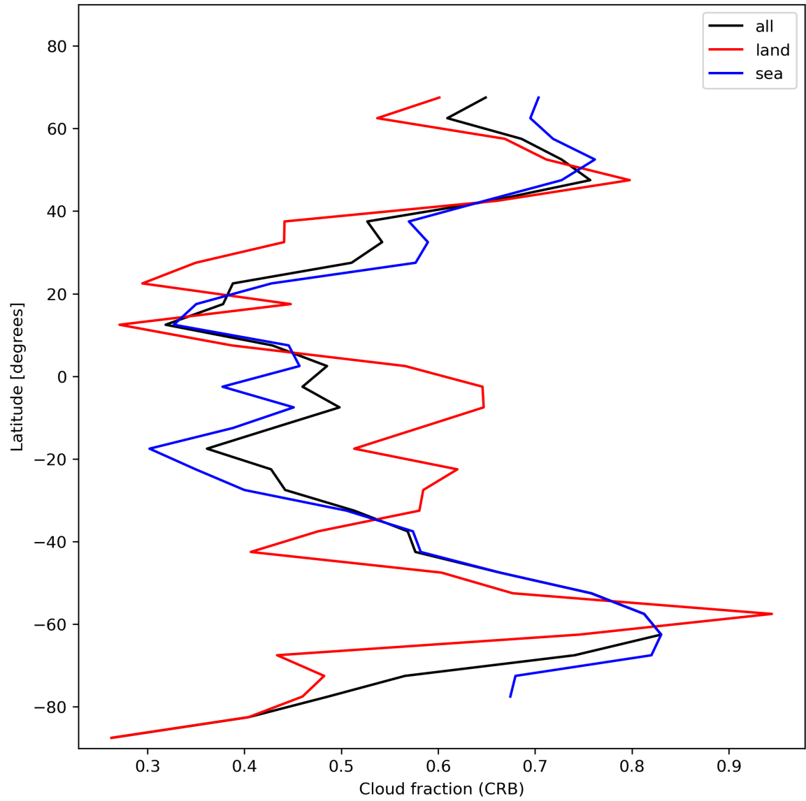
Figure 26: Zonal average of “Cloud fraction (CRB)” for 2023-11-23 to 2023-11-24.
