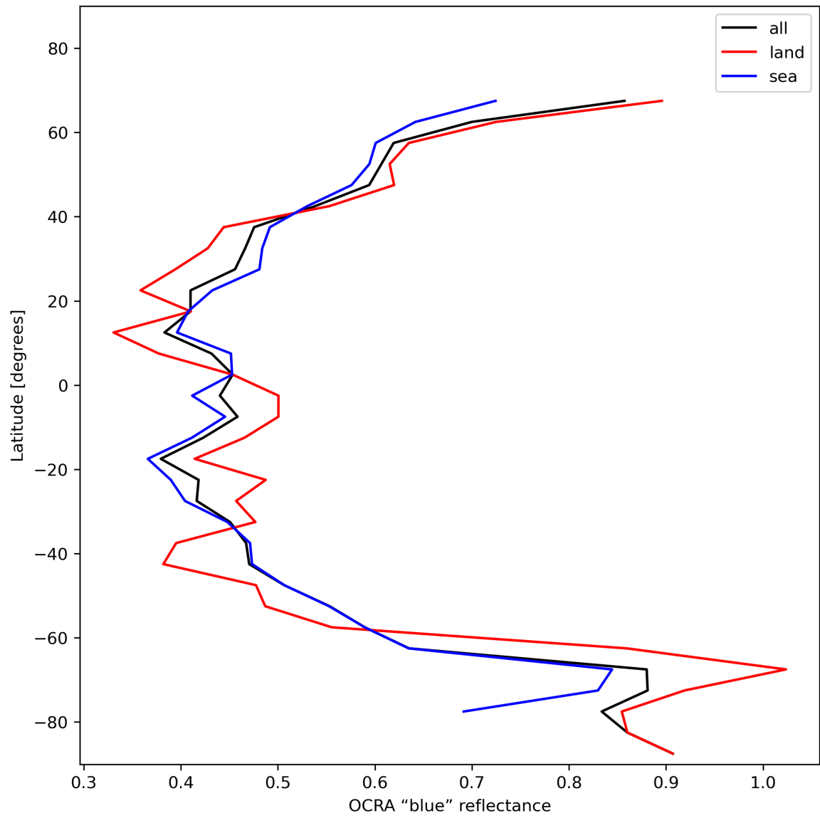
Figure 35: Zonal average of “OCRA “blue” reflectance” for 2023-11-23 to 2023-11-24.
