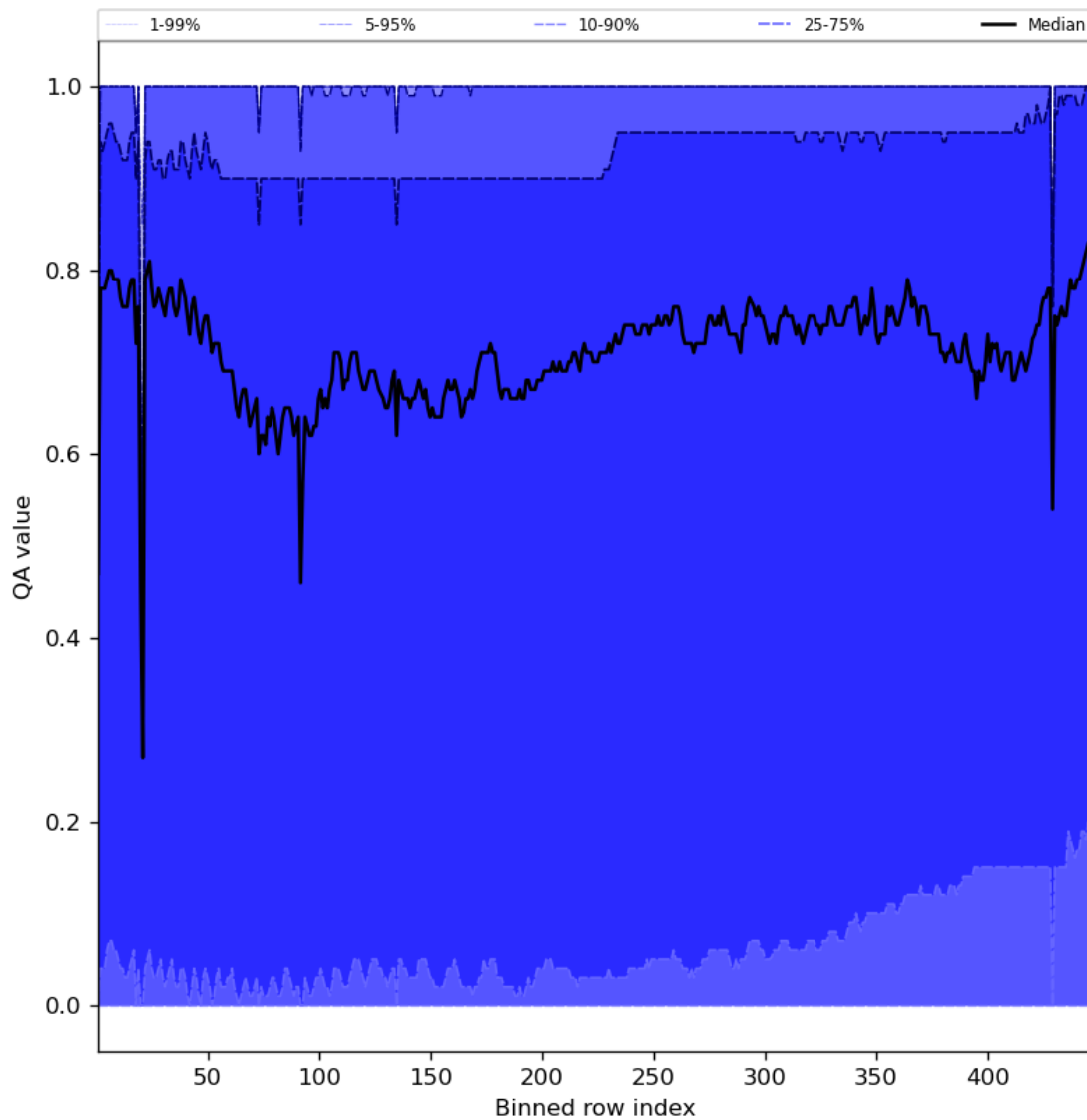
Figure 54: Along track statistics of “QA value” for 2023-11-23 to 2023-11-24
