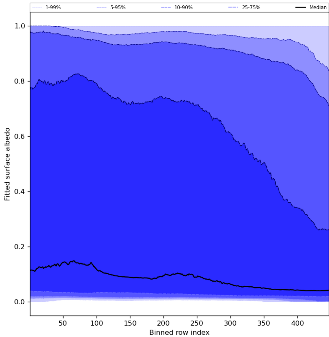
Figure 61: Along track statistics of “Fitted surface albedo” for 2023-11-23 to 2023-11-24
