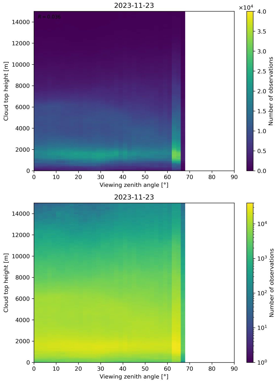
Figure 112: Scatter density plot of “Viewing zenith angle” against “Cloud top height” for 2023-11-23 to 2023-11-24.
