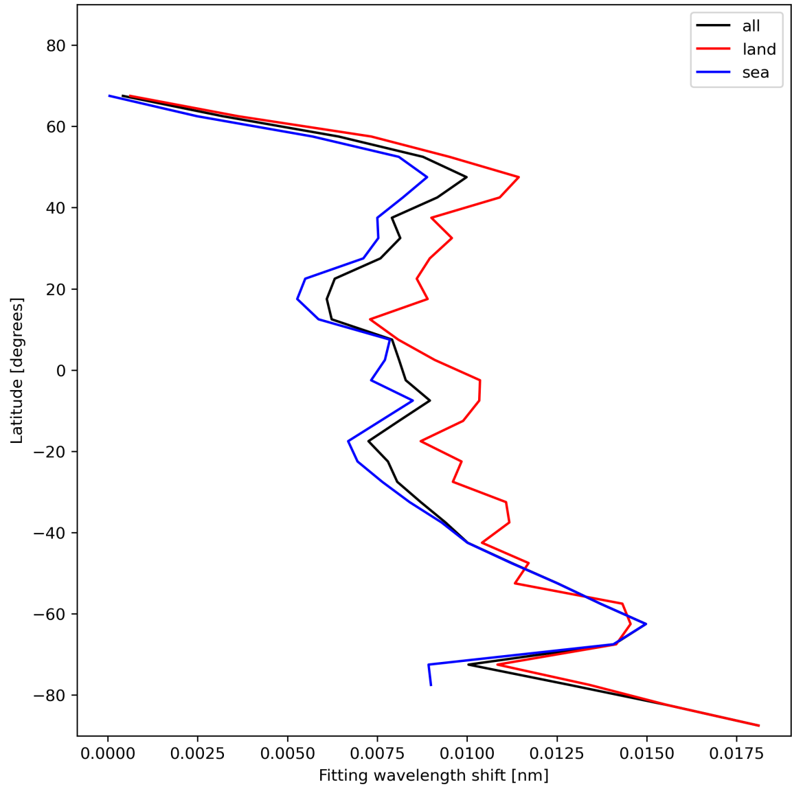
Figure 33: Zonal average of “Fitting wavelength shift” for 2023-11-23 to 2023-11-24.
