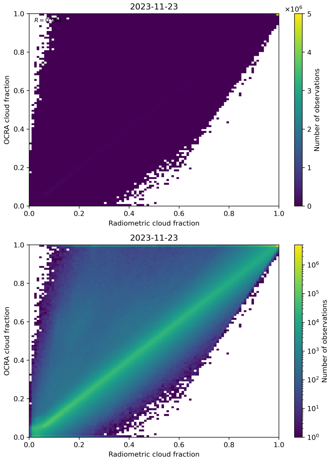
Figure 72: Scatter density plot of “Radiometric cloud fraction” against “OCRA cloud fraction” for 2023-11-23 to 2023-11-24.
