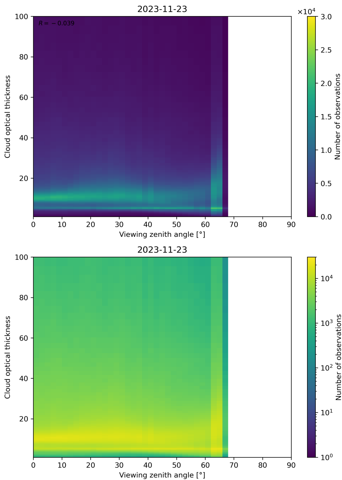
Figure 111: Scatter density plot of “Viewing zenith angle” against “Cloud optical thickness” for 2023-11-23 to 2023-11-24.
