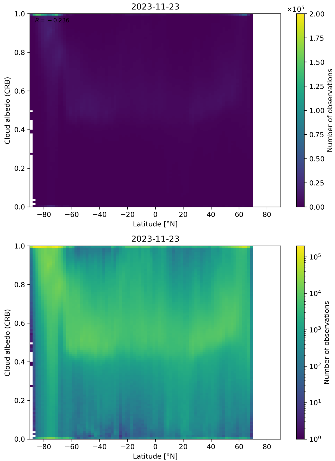
Figure 91: Scatter density plot of “Latitude” against “Cloud albedo (CRB)” for 2023-11-23 to 2023-11-24.
