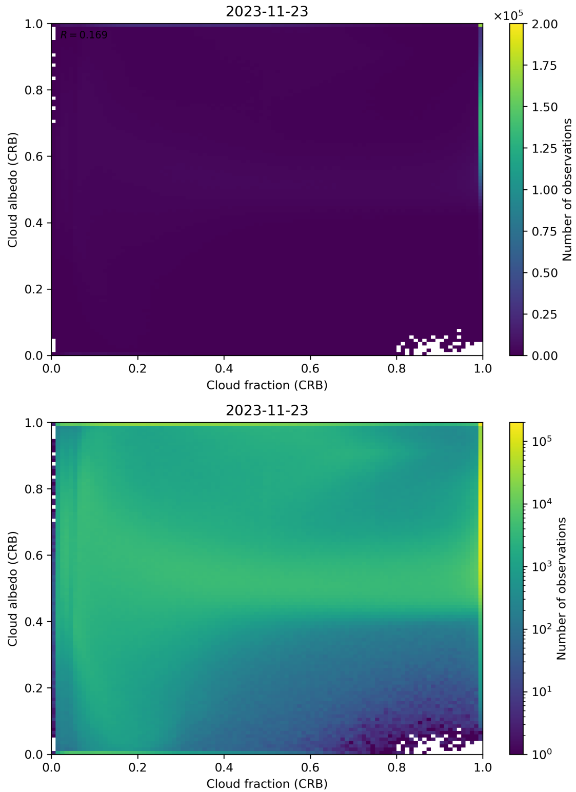
Figure 77: Scatter density plot of “Cloud fraction (CRB)” against “Cloud albedo (CRB)” for 2023-11-23 to 2023-11-24.
