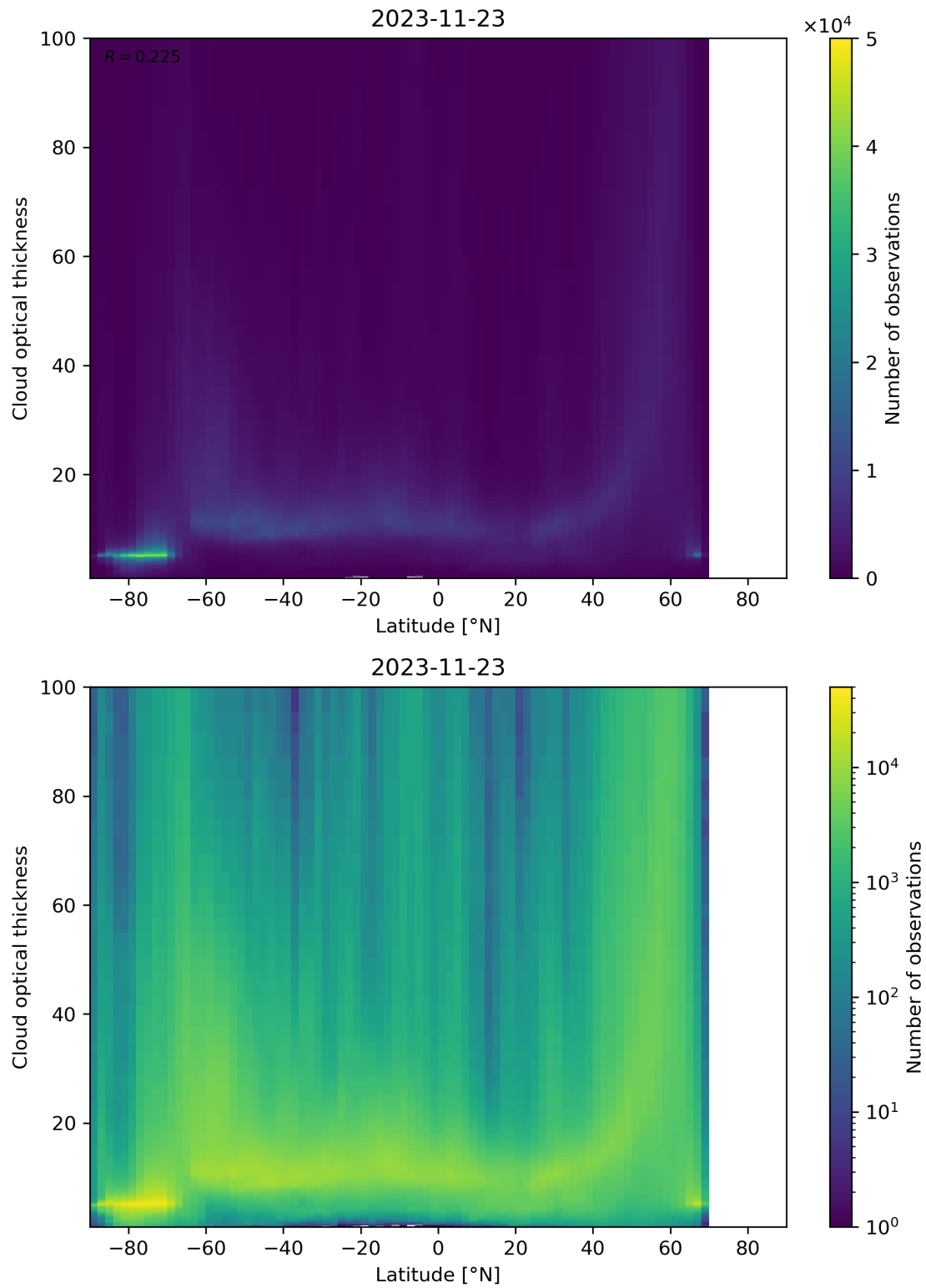
Figure 96: Scatter density plot of “Latitude” against “Cloud optical thickness” for 2023-11-23 to 2023-11-24.
