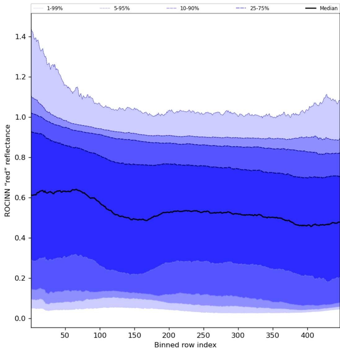
Figure 69: Along track statistics of “ROCINN “red” reflectance” for 2023-11-23 to 2023-11-24
