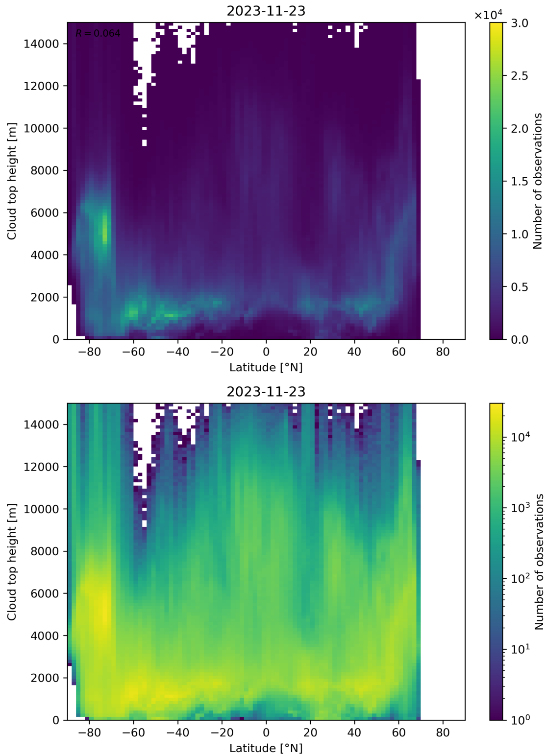
Figure 97: Scatter density plot of “Latitude” against “Cloud top height” for 2023-11-23 to 2023-11-24.
