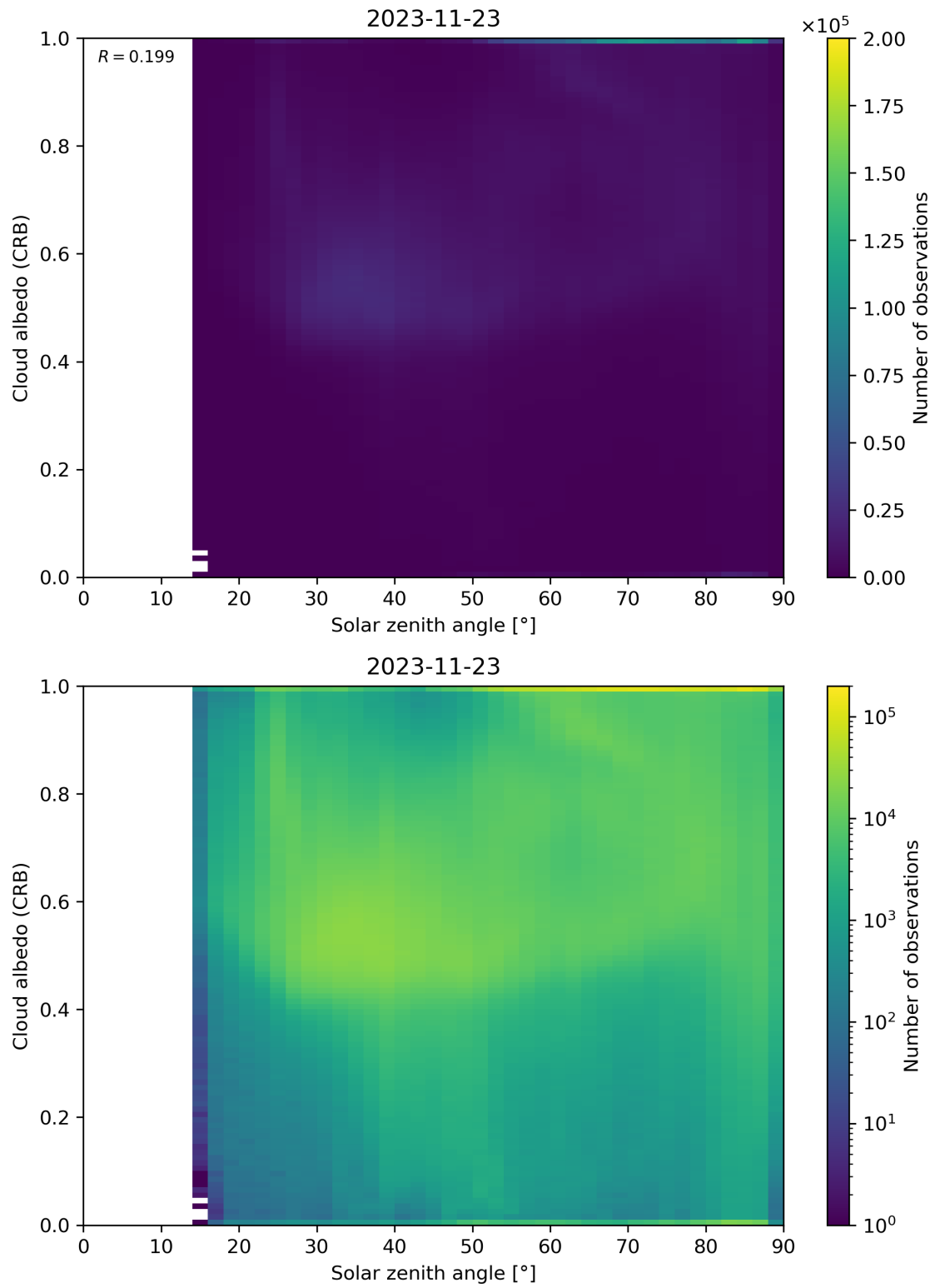
Figure 98: Scatter density plot of “Solar zenith angle” against “Cloud albedo (CRB)” for 2023-11-23 to 2023-11-24.
