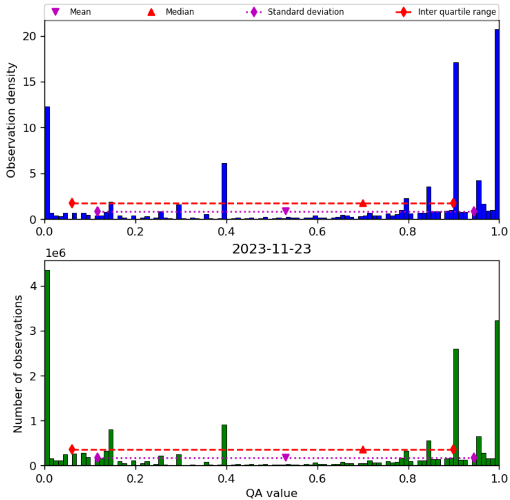
Figure 38: Histogram of “QA value” for 2023-11-23 to 2023-11-24
