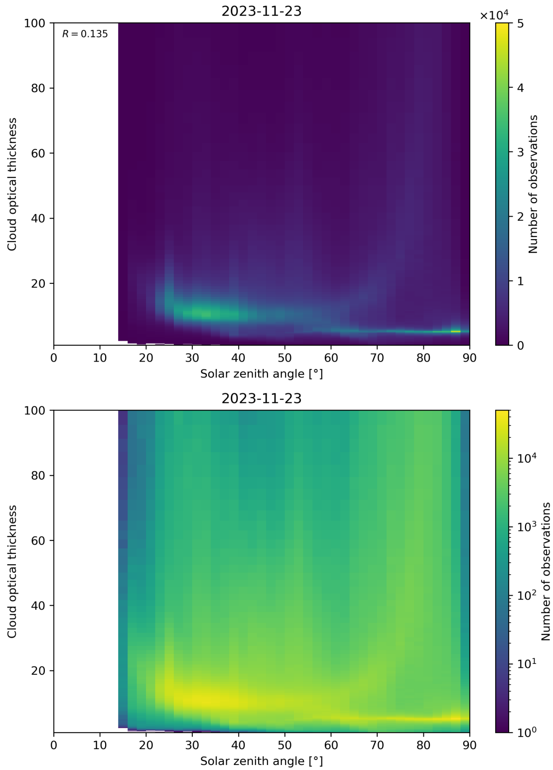
Figure 103: Scatter density plot of “Solar zenith angle” against “Cloud optical thickness” for 2023-11-23 to 2023-11-24.
