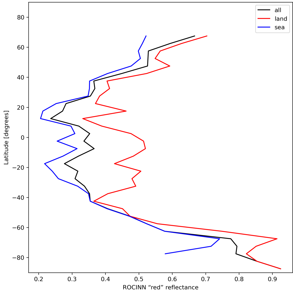
Figure 37: Zonal average of “ROCINN “red” reflectance” for 2023-11-23 to 2023-11-24.
