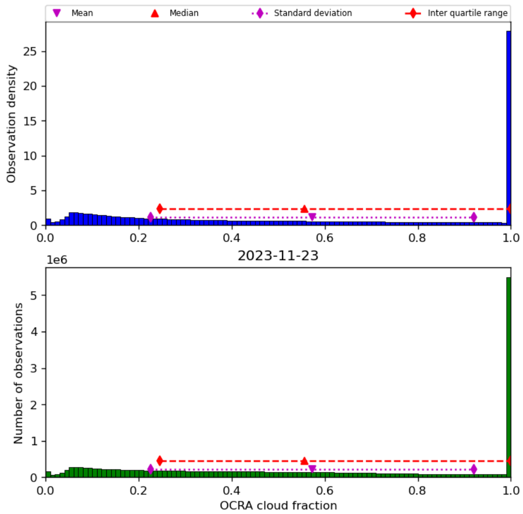
Figure 50: Histogram of “OCRA cloud fraction” for 2023-11-23 to 2023-11-24
