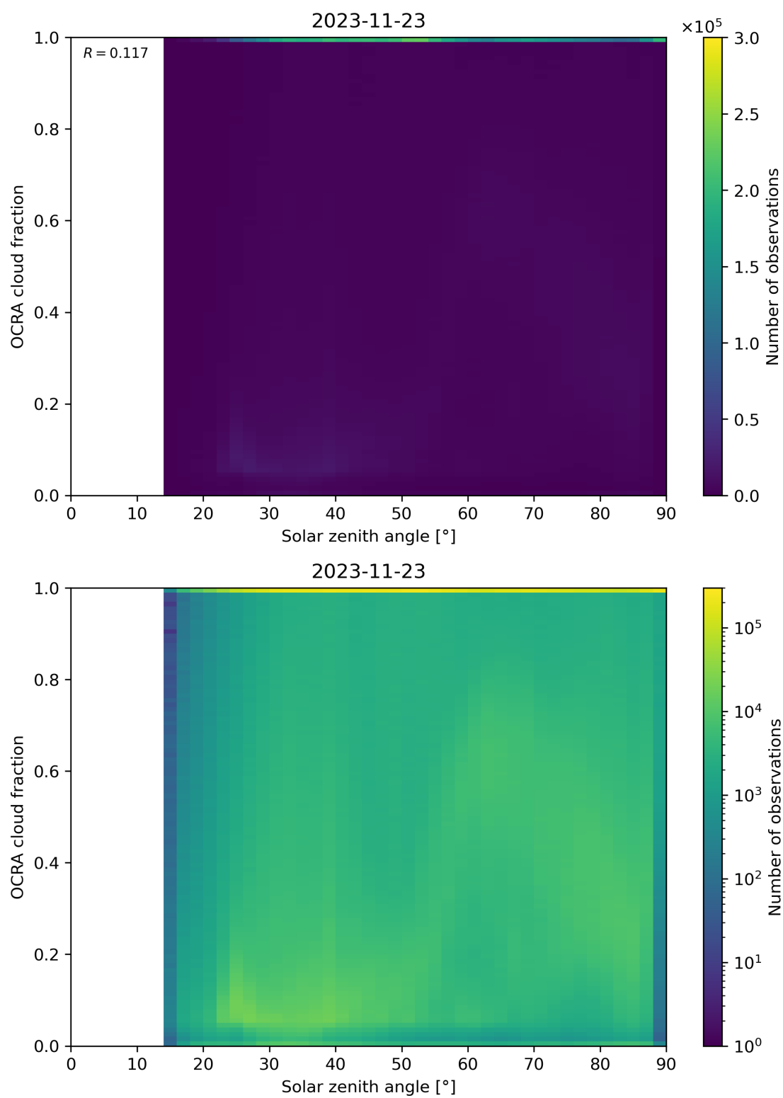
Figure 100: Scatter density plot of “Solar zenith angle” against “OCRA cloud fraction” for 2023-11-23 to 2023-11-24.
