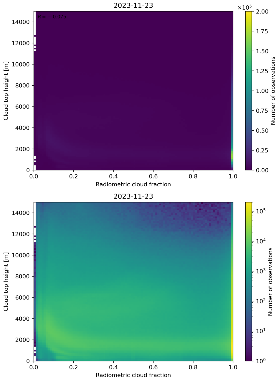
Figure 76: Scatter density plot of “Radiometric cloud fraction” against “Cloud top height” for 2023-11-23 to 2023-11-24.
