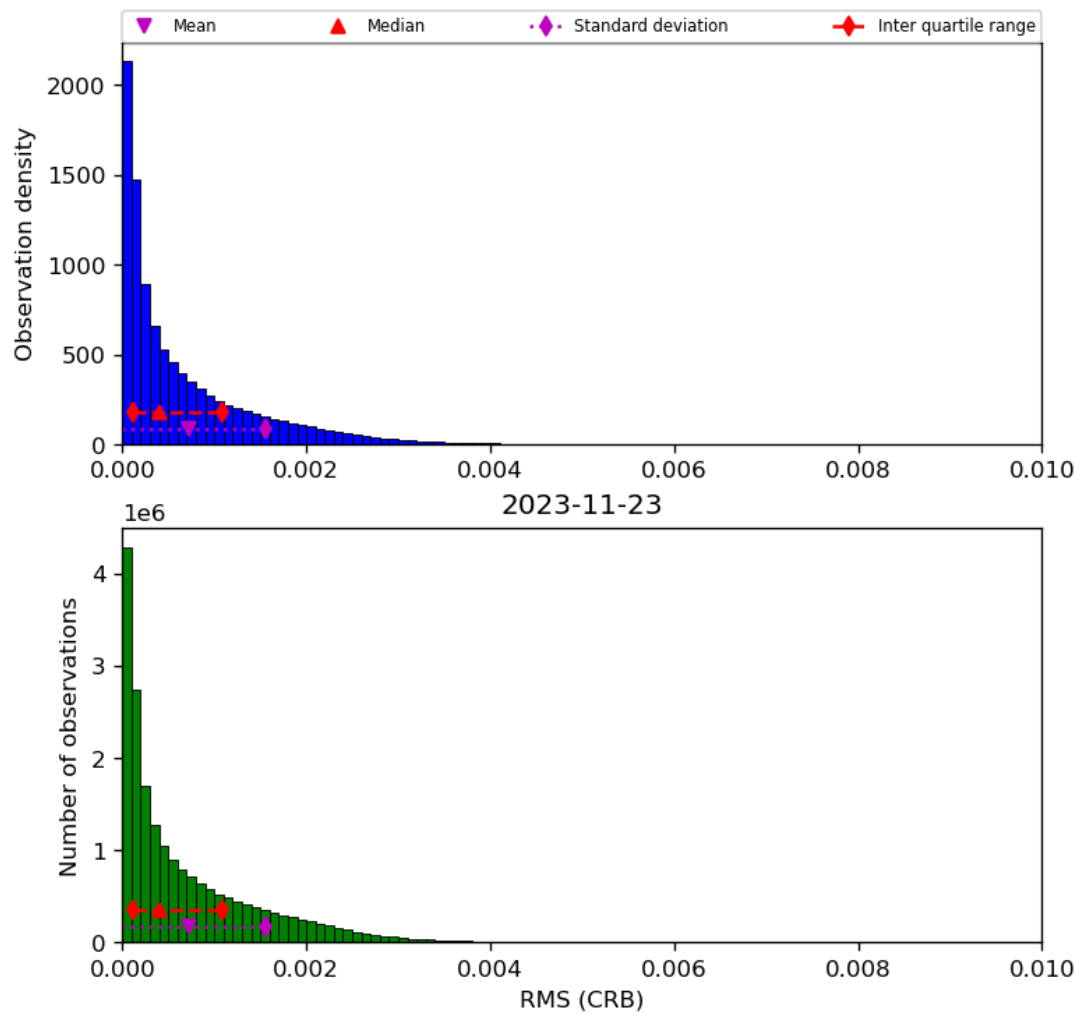
Figure 48: Histogram of “RMS (CRB)” for 2023-11-23 to 2023-11-24
