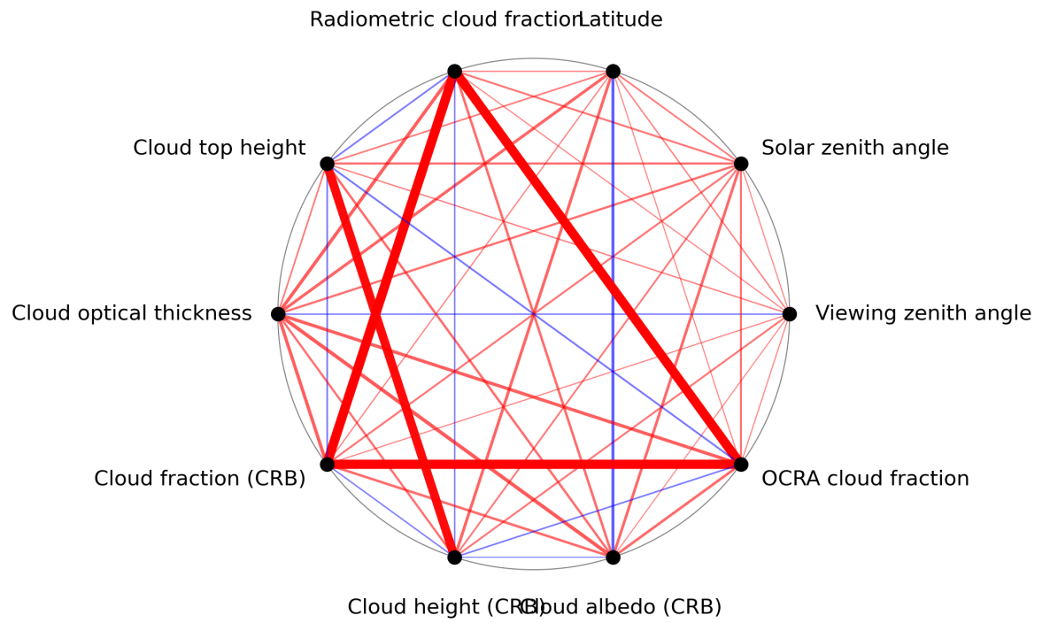
Figure 1: Map of correlation graph for 2023-11-23 to 2023-11-24.
