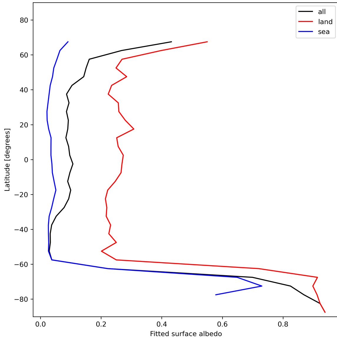
Figure 29: Zonal average of “Fitted surface albedo” for 2023-11-23 to 2023-11-24.
