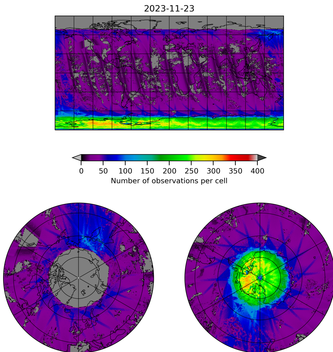
Figure 21: Map of the number of observations for 2023-11-23 to 2023-11-24
