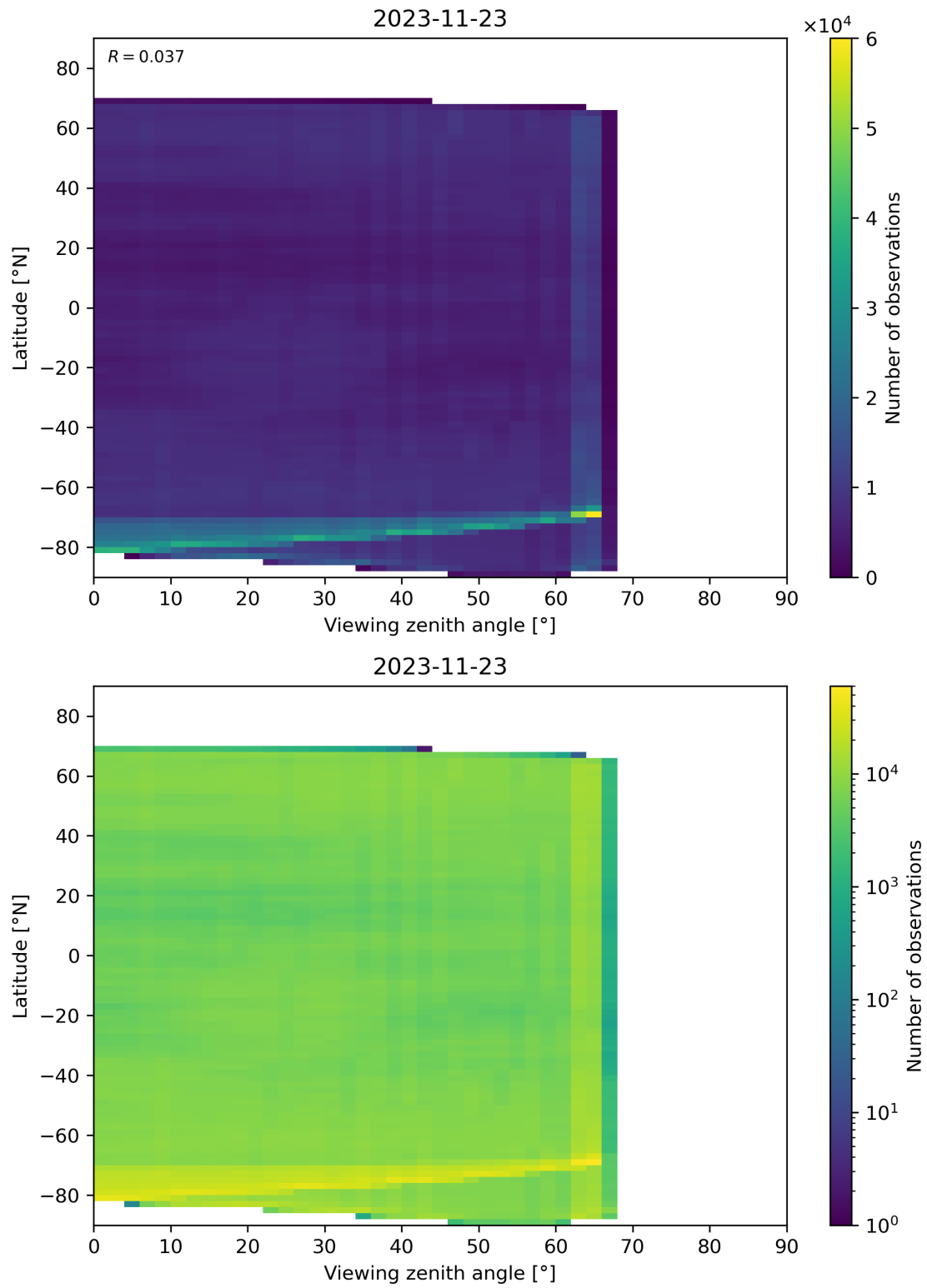
Figure 113: Scatter density plot of “Viewing zenith angle” against “Latitude” for 2023-11-23 to 2023-11-24.
