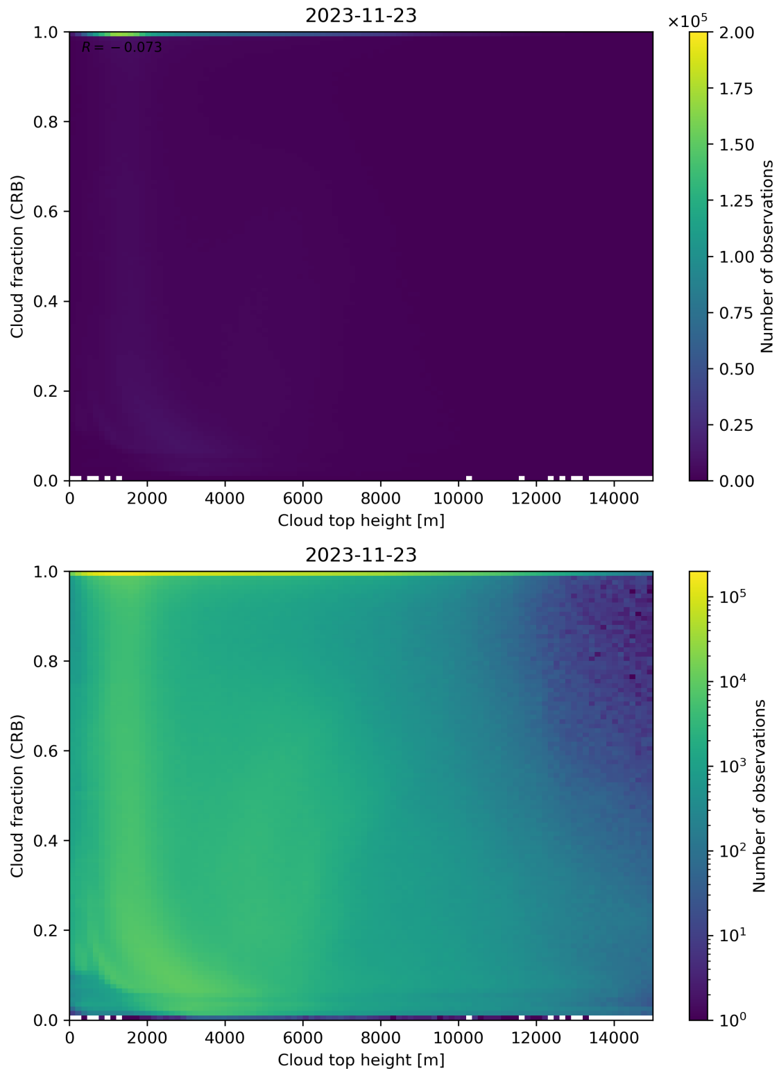
Figure 88: Scatter density plot of “Cloud top height” against “Cloud fraction (CRB)” for 2023-11-23 to 2023-11-24.
