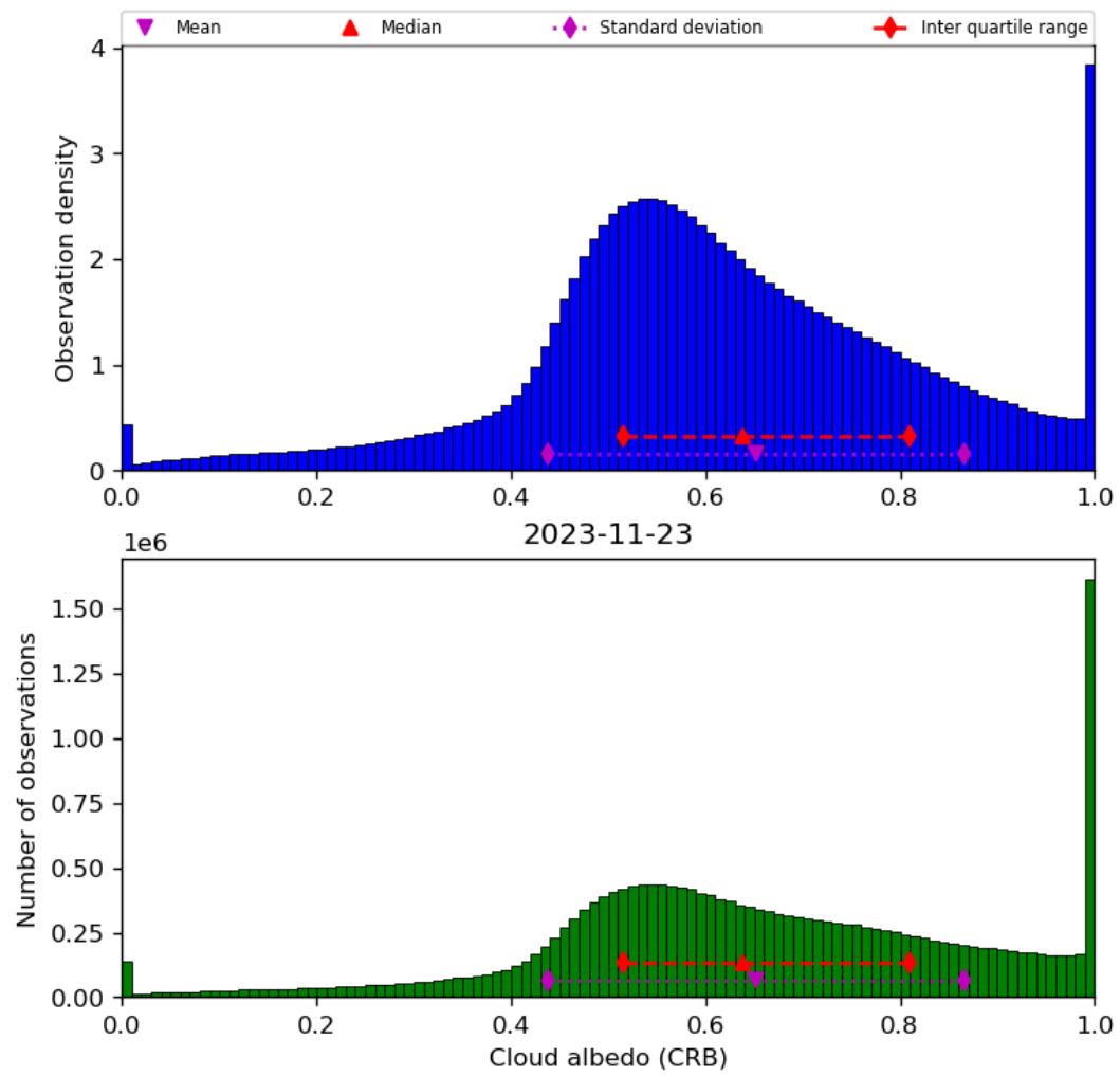
Figure 44: Histogram of “Cloud albedo (CRB)” for 2023-11-23 to 2023-11-24
