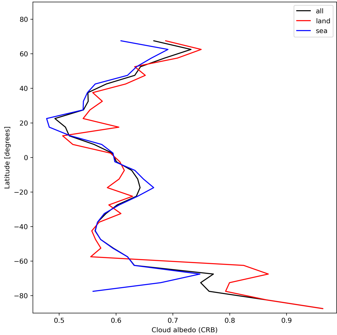
Figure 28: Zonal average of “Cloud albedo (CRB)” for 2023-11-23 to 2023-11-24.
