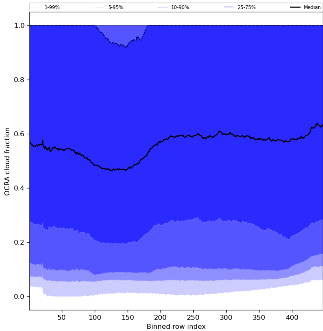
Figure 66: Along track statistics of “OCRA cloud fraction” for 2023-11-23 to 2023-11-24
