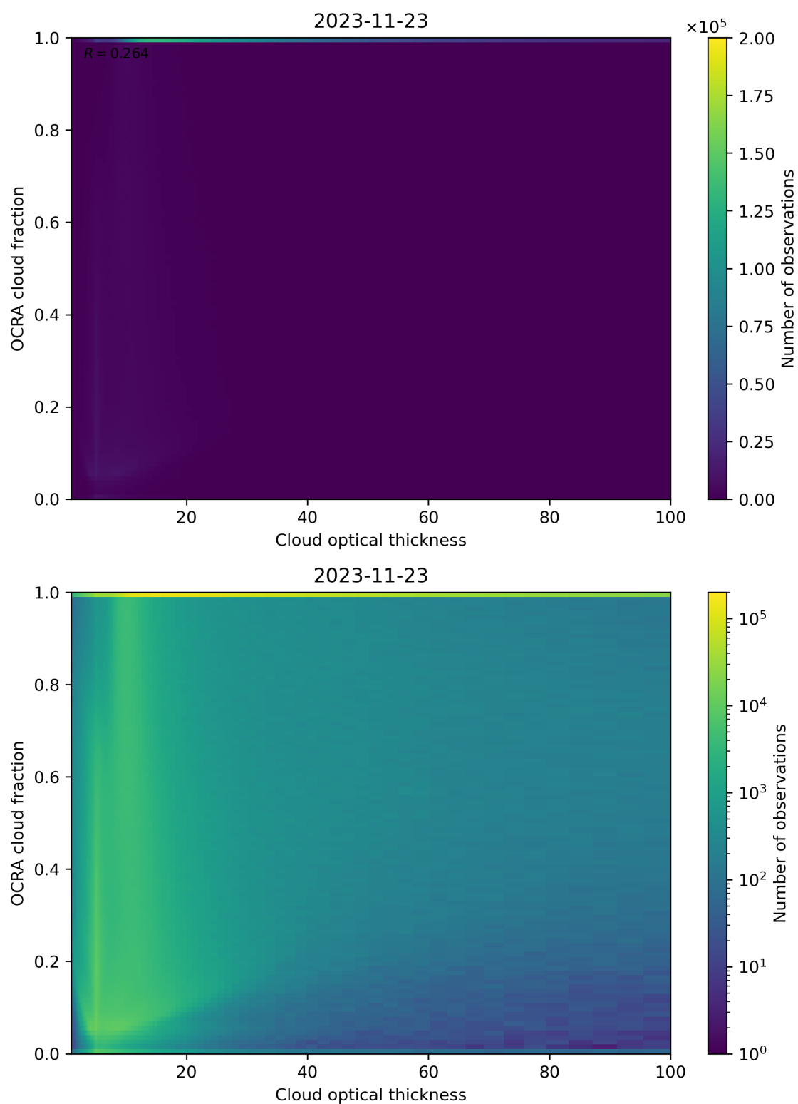
Figure 83: Scatter density plot of “Cloud optical thickness” against “OCRA cloud fraction” for 2023-11-23 to 2023-11-24.
