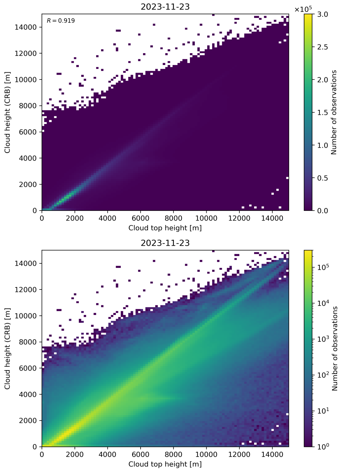
Figure 89: Scatter density plot of “Cloud top height” against “Cloud height (CRB)” for 2023-11-23 to 2023-11-24.
