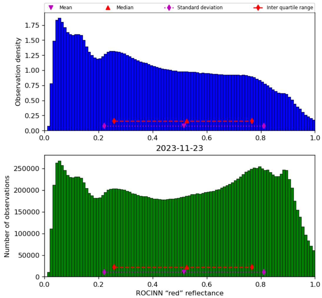
Figure 53: Histogram of “ROCINN “red” reflectance” for 2023-11-23 to 2023-11-24
