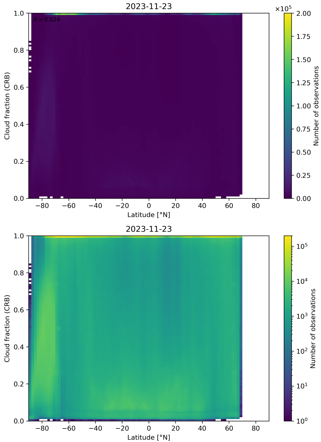
Figure 94: Scatter density plot of “Latitude” against “Cloud fraction (CRB)” for 2023-11-23 to 2023-11-24.
