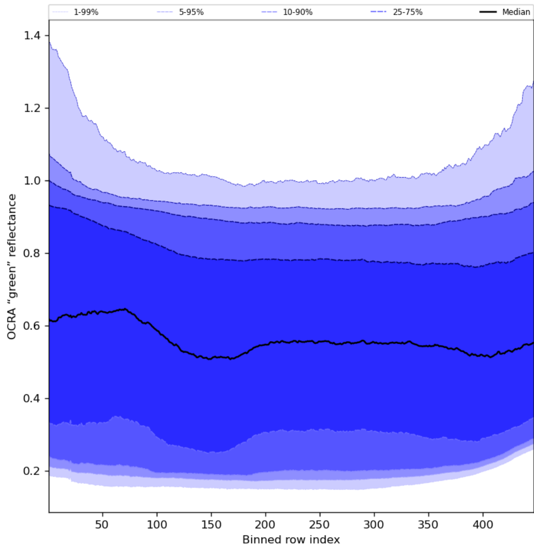
Figure 68: Along track statistics of "OCRA "green" reflectance" for 2023-11-23 to 2023-11-24
