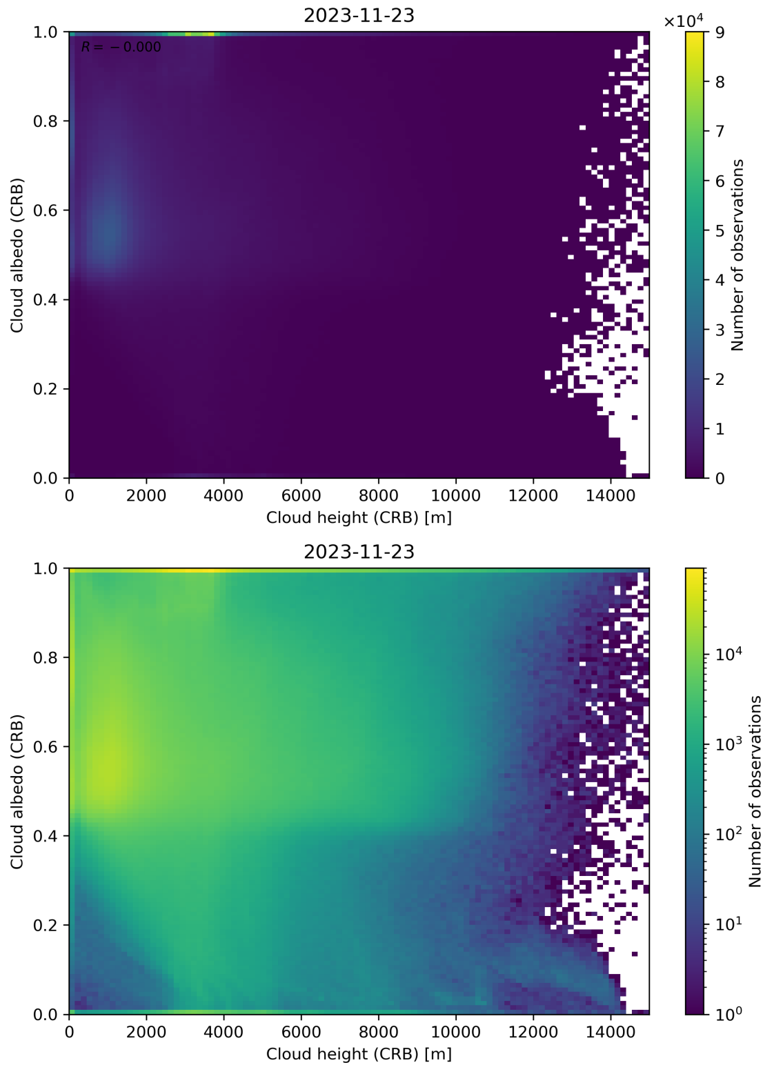
Figure 80: Scatter density plot of “Cloud height (CRB)” against “Cloud albedo (CRB)” for 2023-11-23 to 2023-11-24.
