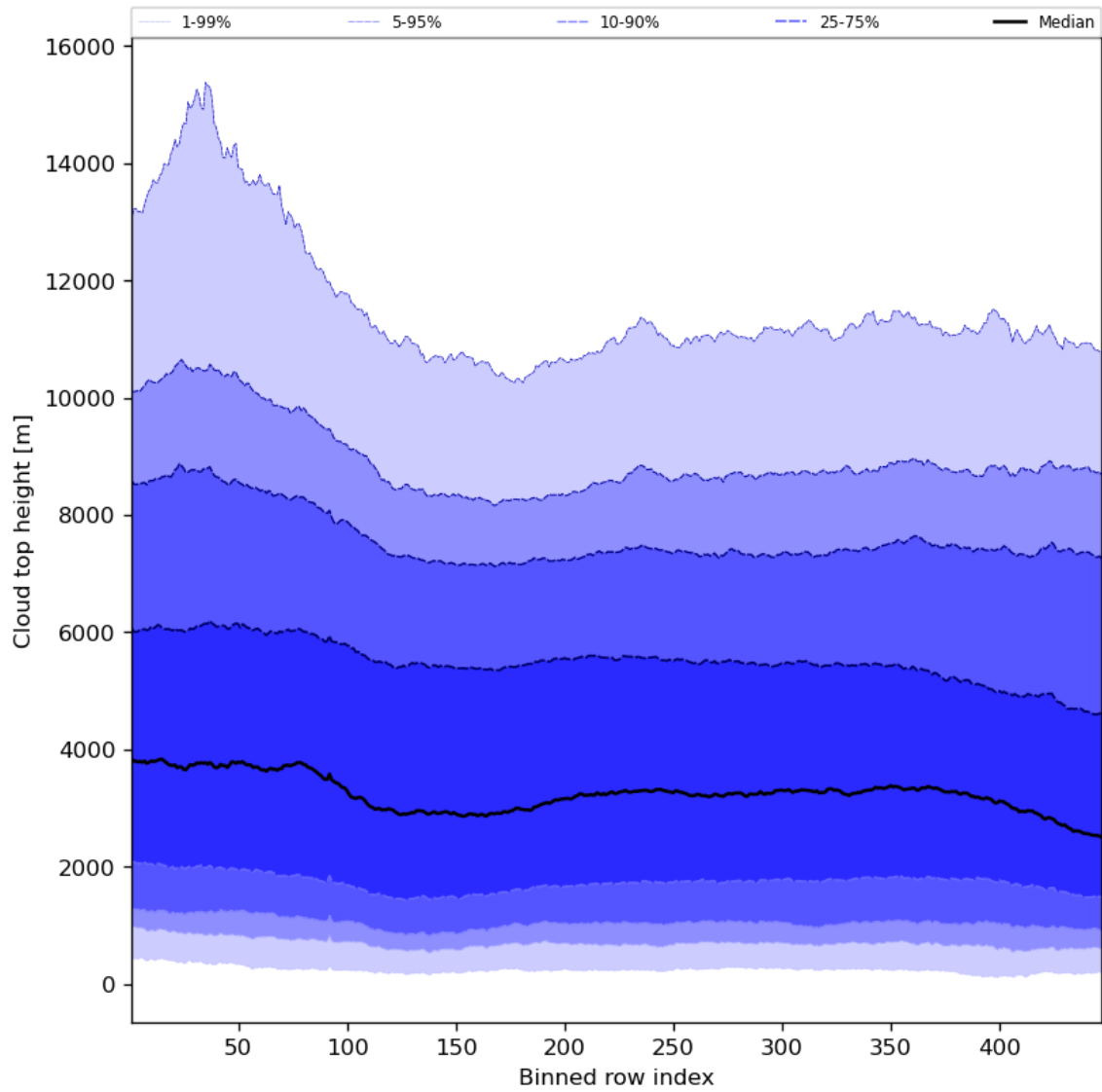
Figure 56: Along track statistics of “Cloud top height” for 2023-11-23 to 2023-11-25
