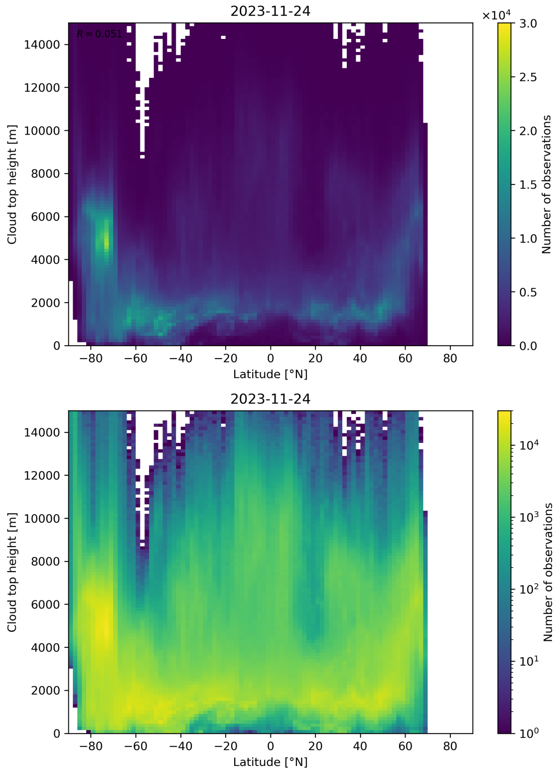
Figure 97: Scatter density plot of “Latitude” against “Cloud top height” for 2023-11-23 to 2023-11-25.
