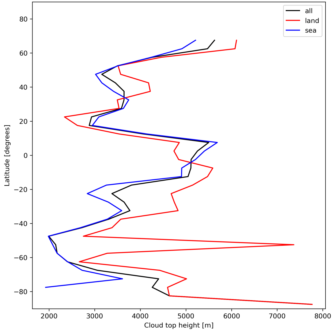
Figure 24: Zonal average of “Cloud top height” for 2023-11-23 to 2023-11-25.
