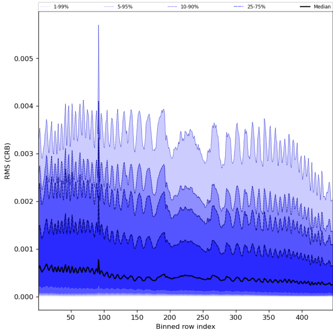
Figure 64: Along track statistics of “RMS (CRB)” for 2023-11-23 to 2023-11-25
