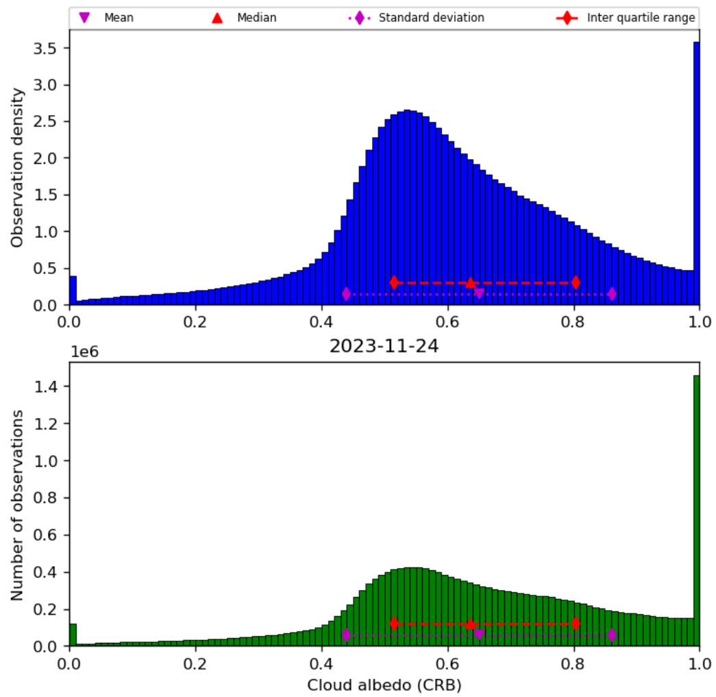
Figure 44: Histogram of “Cloud albedo (CRB)” for 2023-11-23 to 2023-11-25
