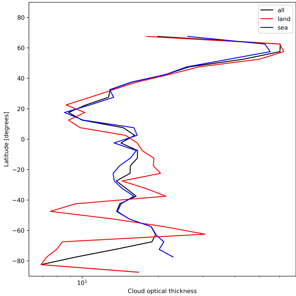
Figure 25: Zonal average of “Cloud optical thickness” for 2023-11-23 to 2023-11-25.
