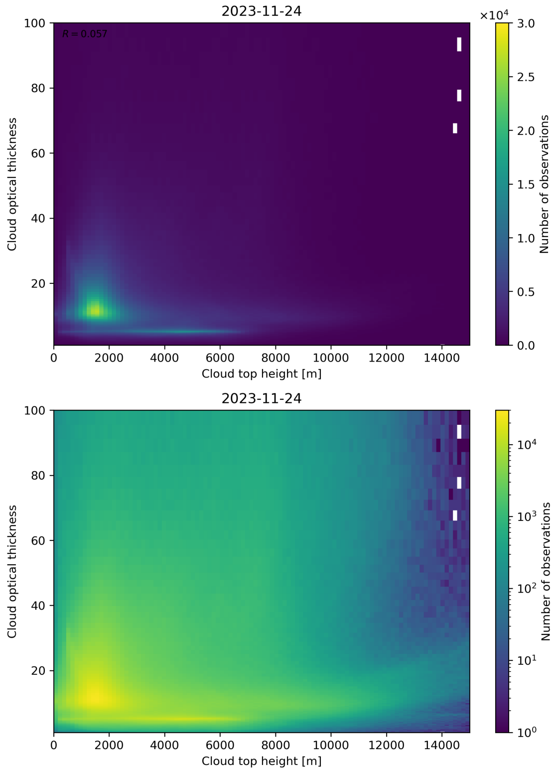
Figure 90: Scatter density plot of “Cloud top height” against “Cloud optical thickness” for 2023-11-23 to 2023-11-25.
