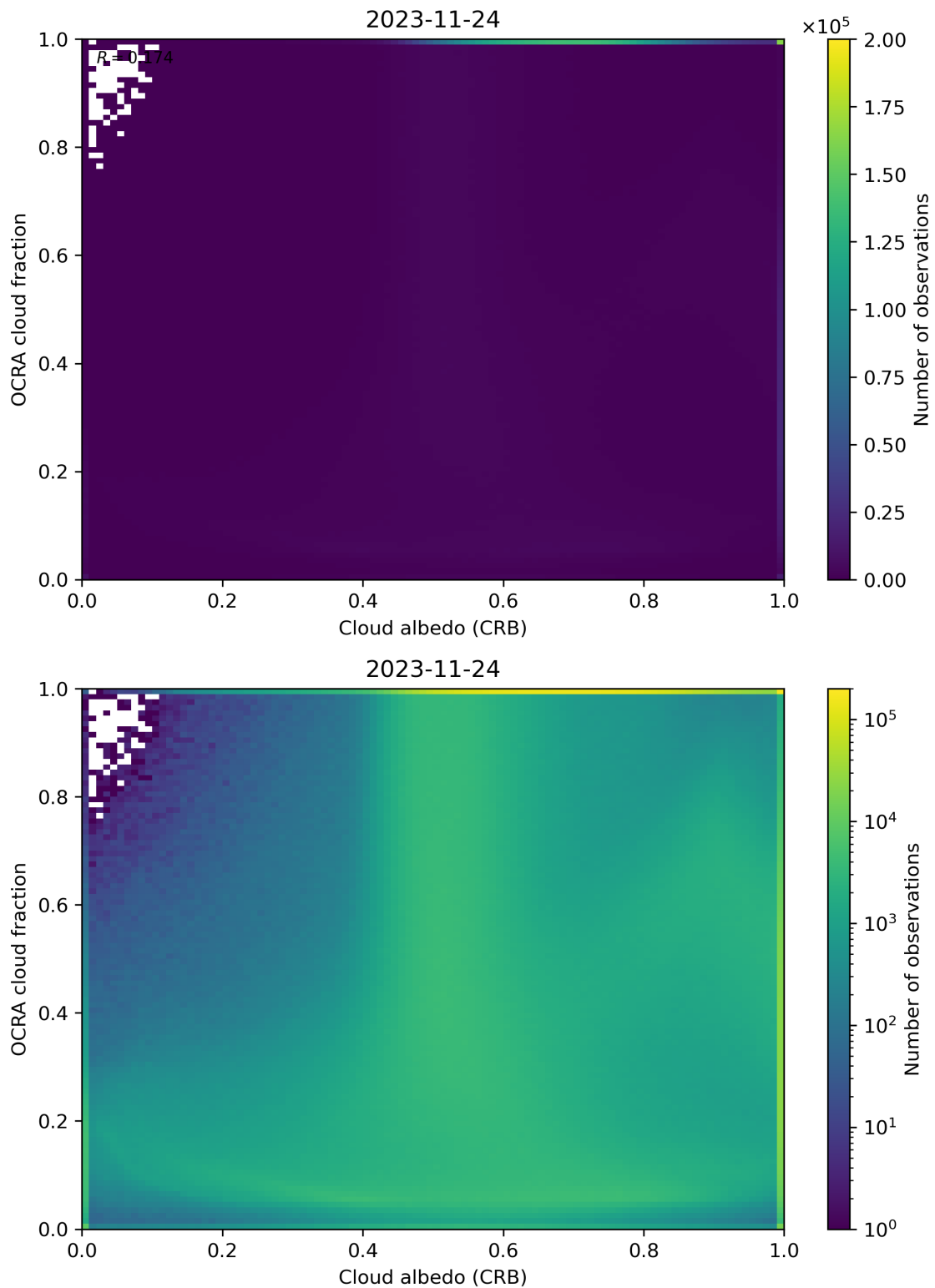
Figure 70: Scatter density plot of “Cloud albedo (CRB)” against “OCRA cloud fraction” for 2023-11-23 to 2023-11-25.
