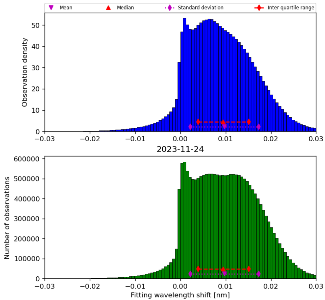
Figure 49: Histogram of “Fitting wavelength shift” for 2023-11-23 to 2023-11-25
