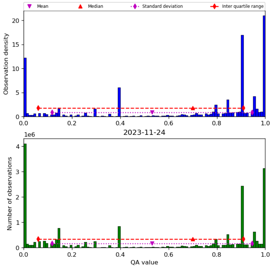
Figure 38: Histogram of “QA value” for 2023-11-23 to 2023-11-25
