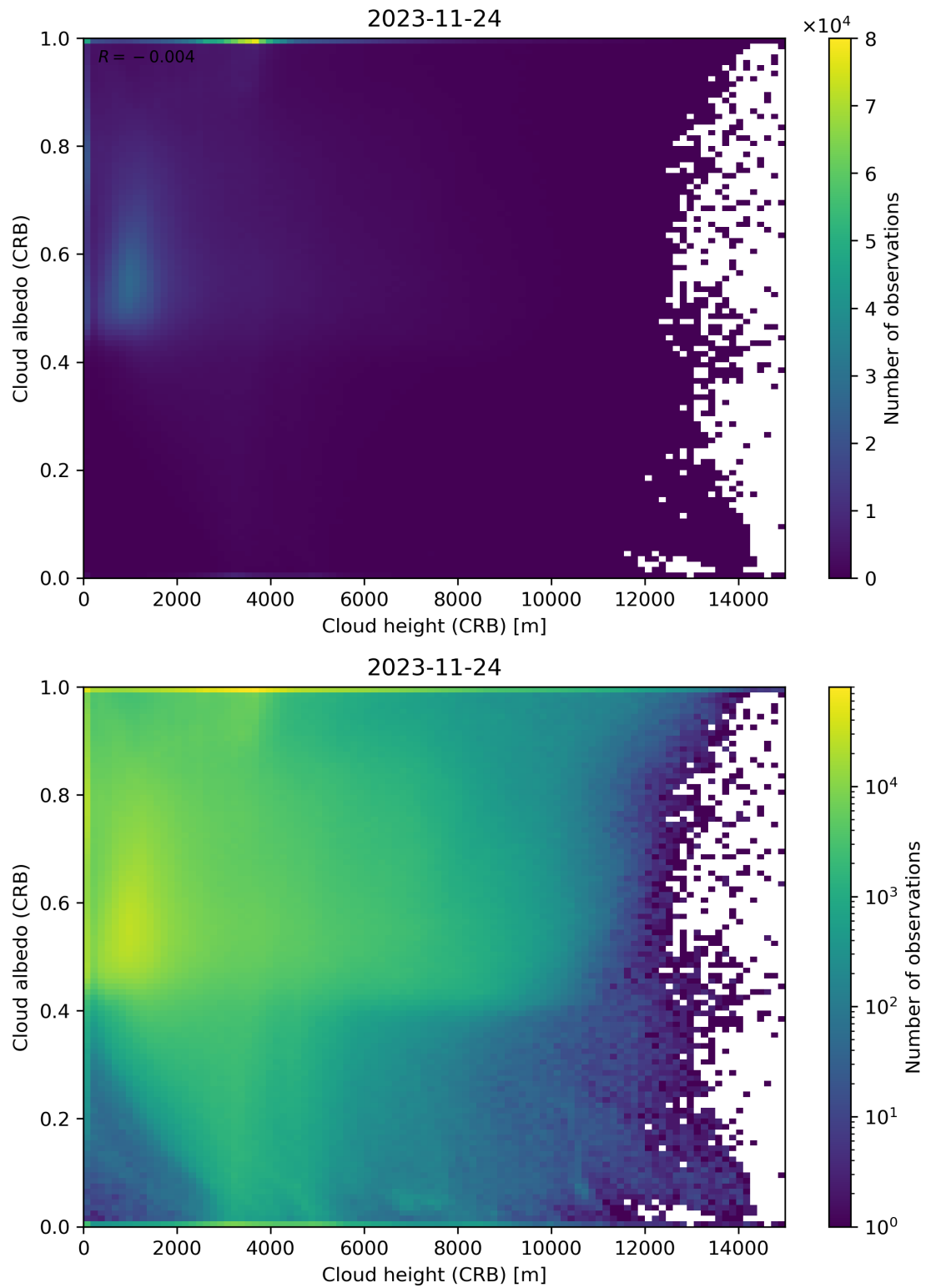
Figure 80: Scatter density plot of “Cloud height (CRB)” against “Cloud albedo (CRB)” for 2023-11-23 to 2023-11-25.
