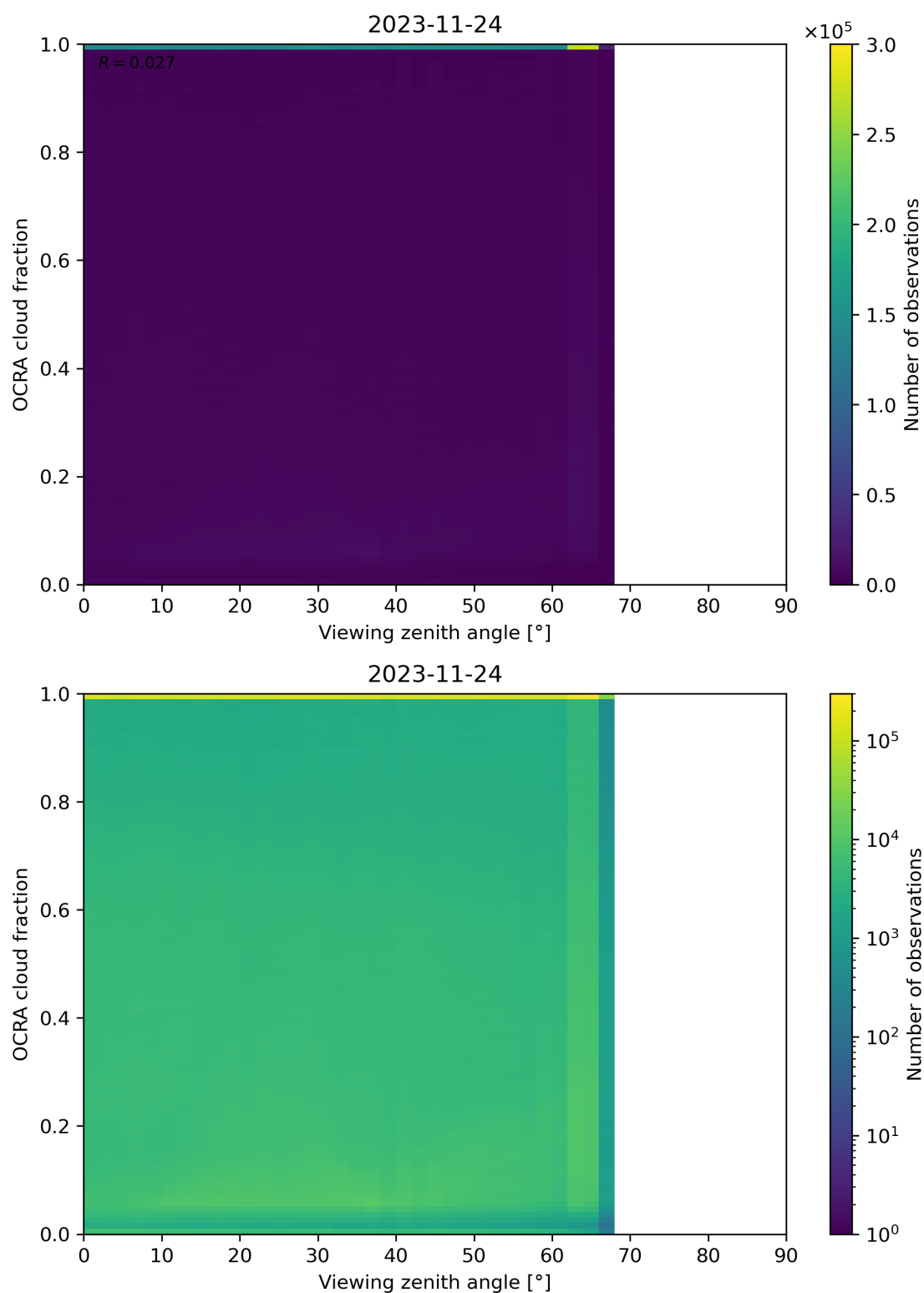
Figure 108: Scatter density plot of “Viewing zenith angle” against “OCRA cloud fraction” for 2023-11-23 to 2023-11-25.
