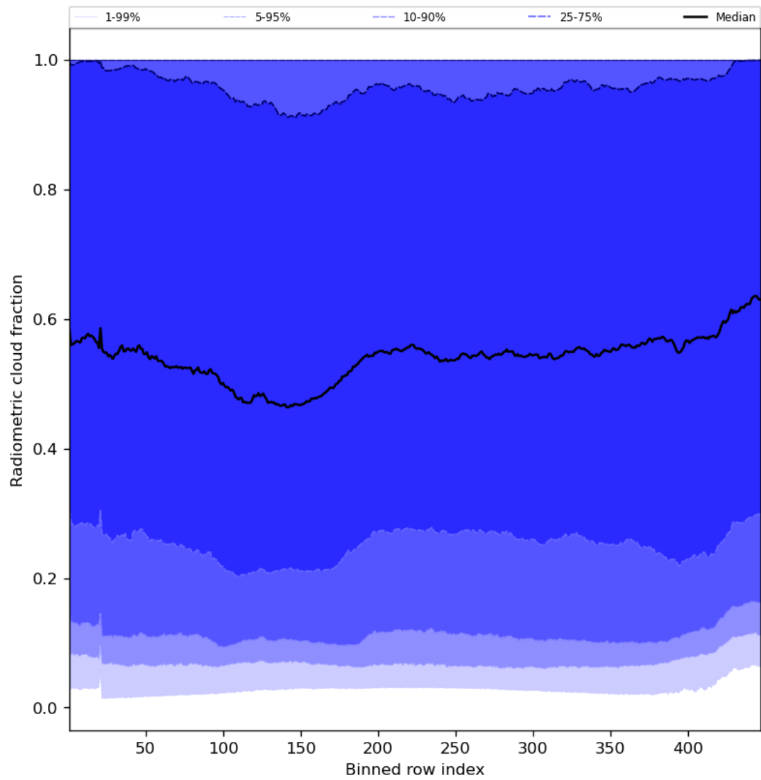
Figure 55: Along track statistics of “Radiometric cloud fraction” for 2023-11-23 to 2023-11-25
