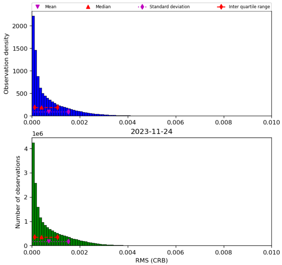
Figure 48: Histogram of “RMS (CRB)” for 2023-11-23 to 2023-11-25
