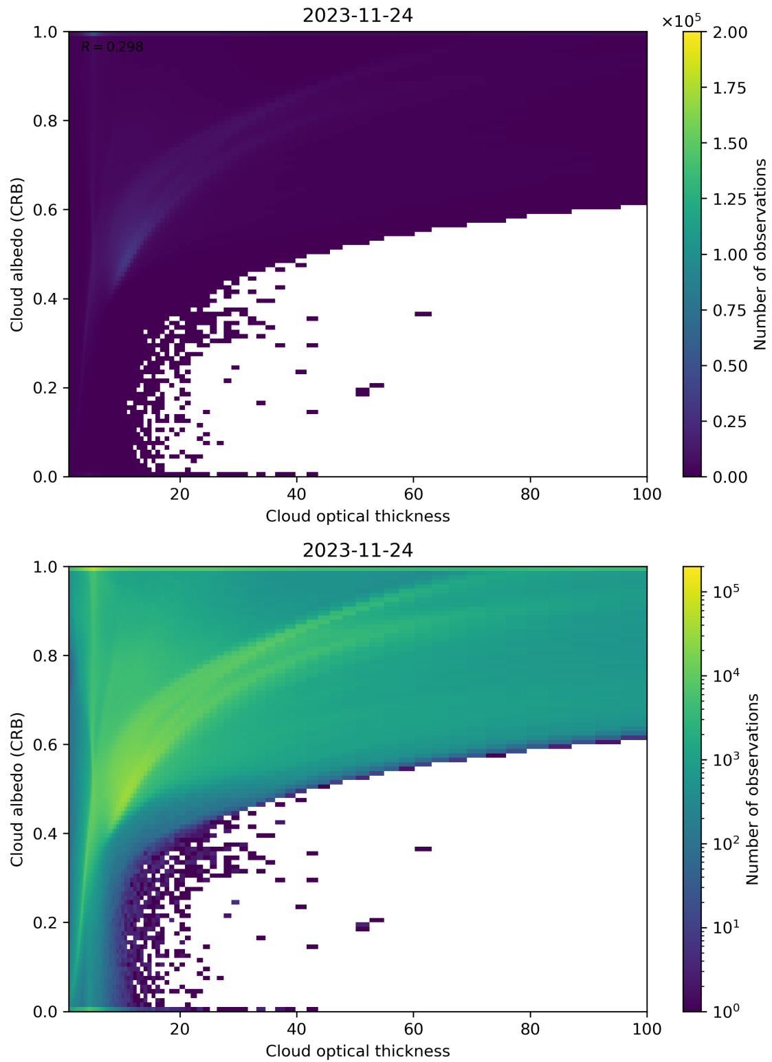
Figure 82: Scatter density plot of “Cloud optical thickness” against “Cloud albedo (CRB)” for 2023-11-23 to 2023-11-25.
