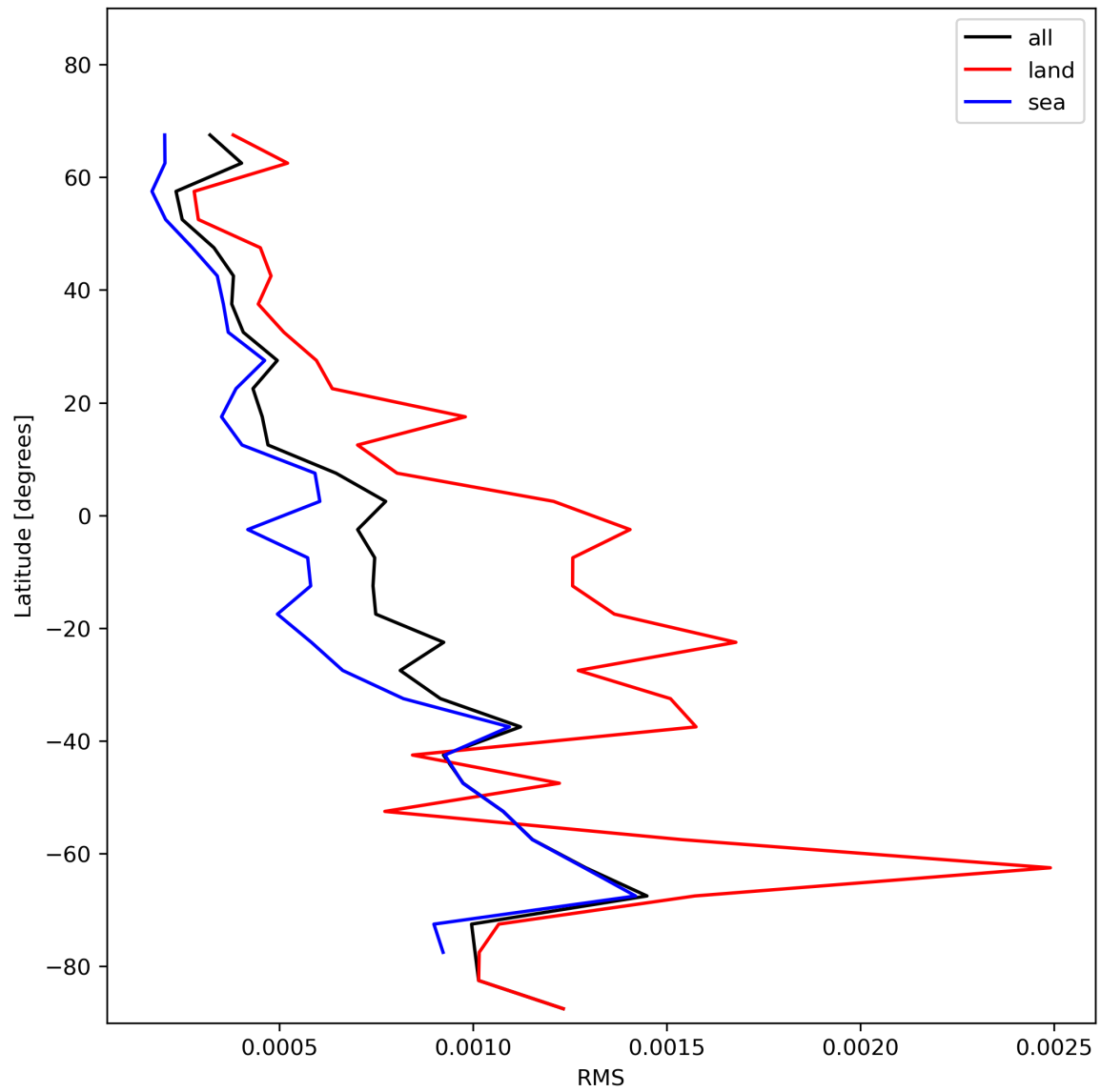
Figure 31: Zonal average of “RMS” for 2023-11-23 to 2023-11-25.
