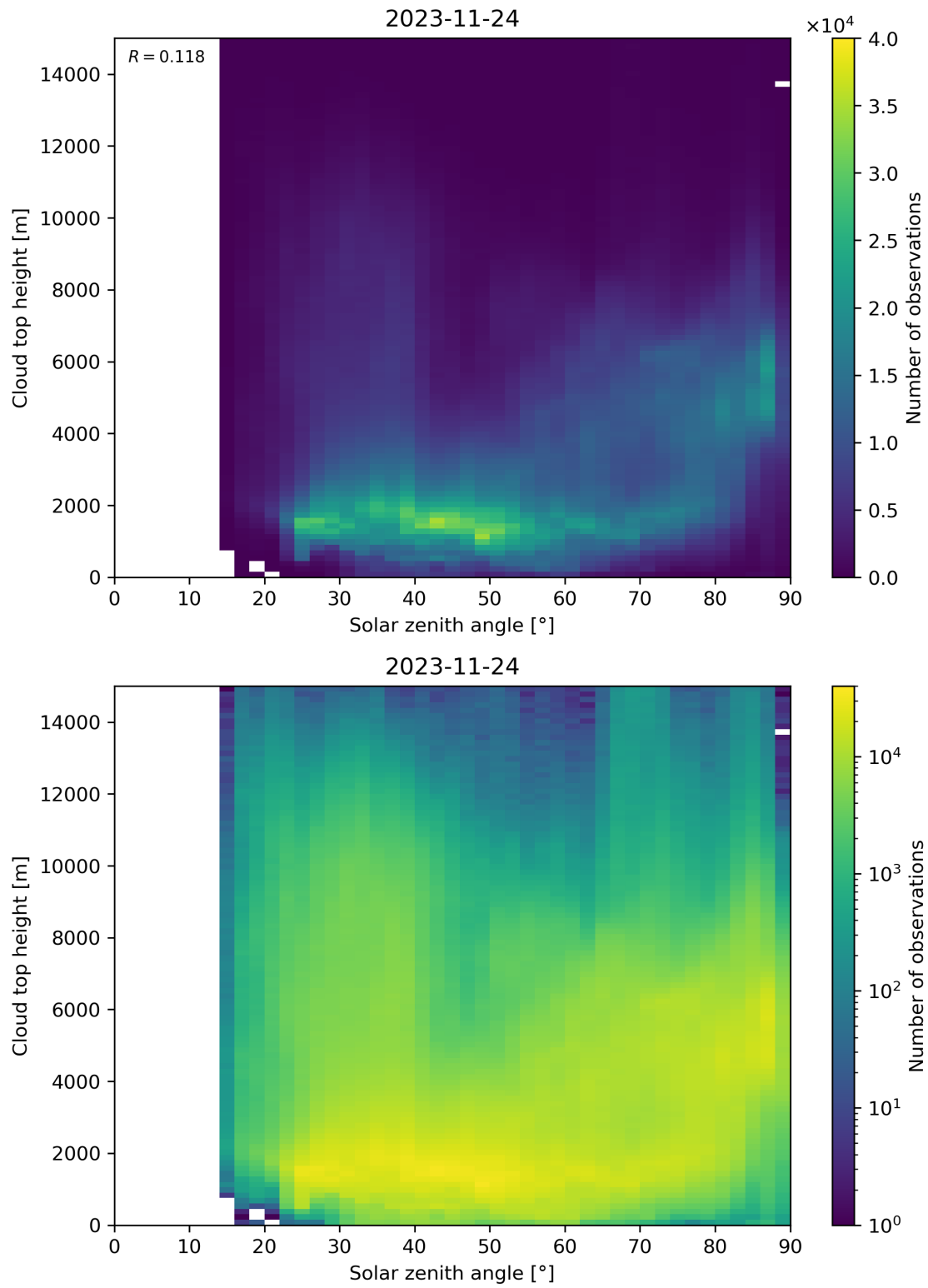
Figure 104: Scatter density plot of “Solar zenith angle” against “Cloud top height” for 2023-11-23 to 2023-11-25.
