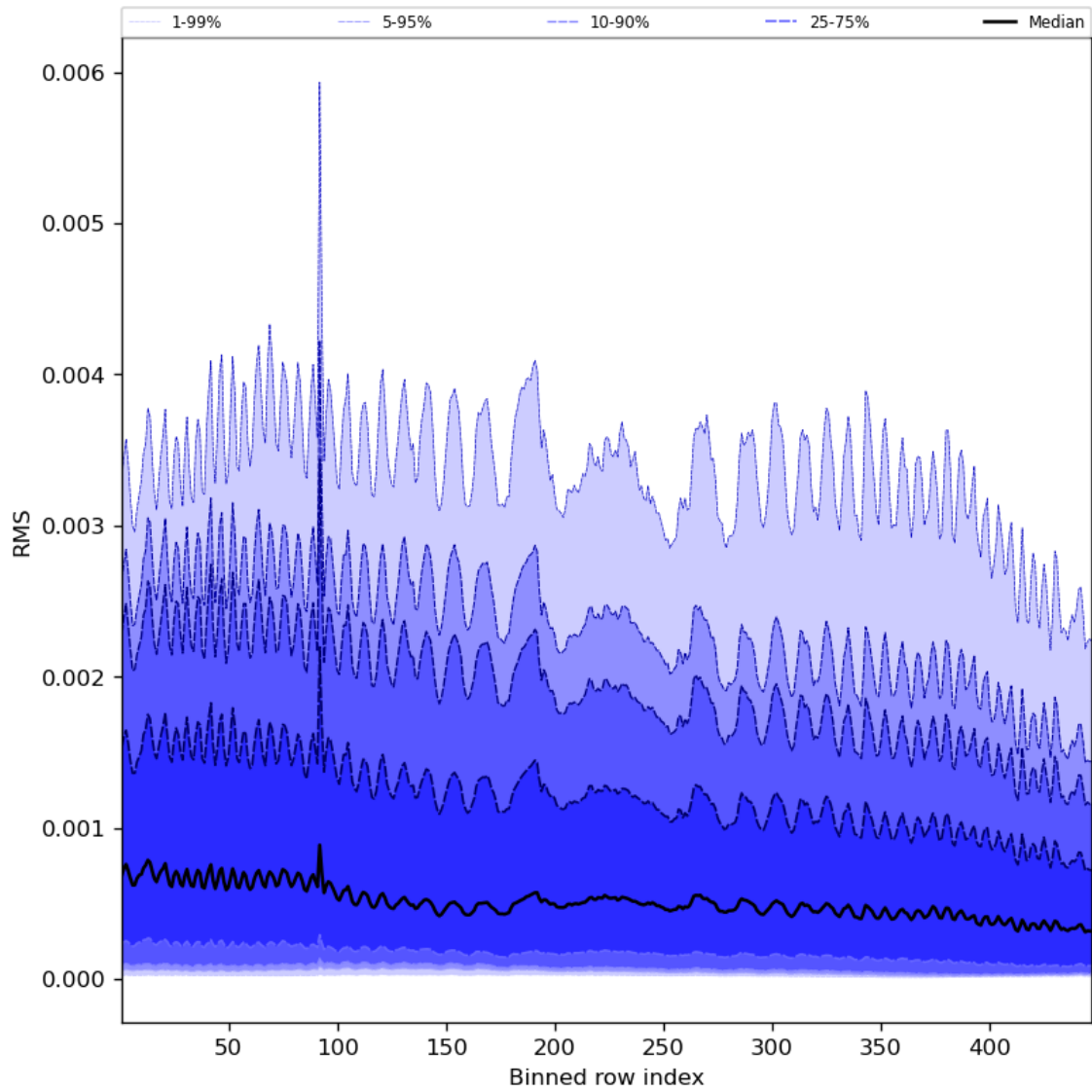
Figure 63: Along track statistics of “RMS” for 2023-11-23 to 2023-11-25
