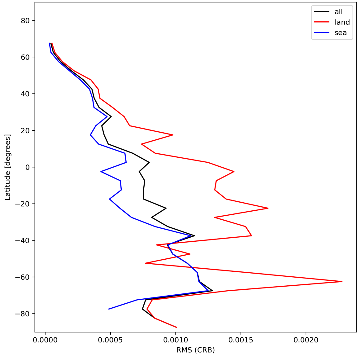
Figure 32: Zonal average of “RMS (CRB)” for 2023-11-23 to 2023-11-25.
