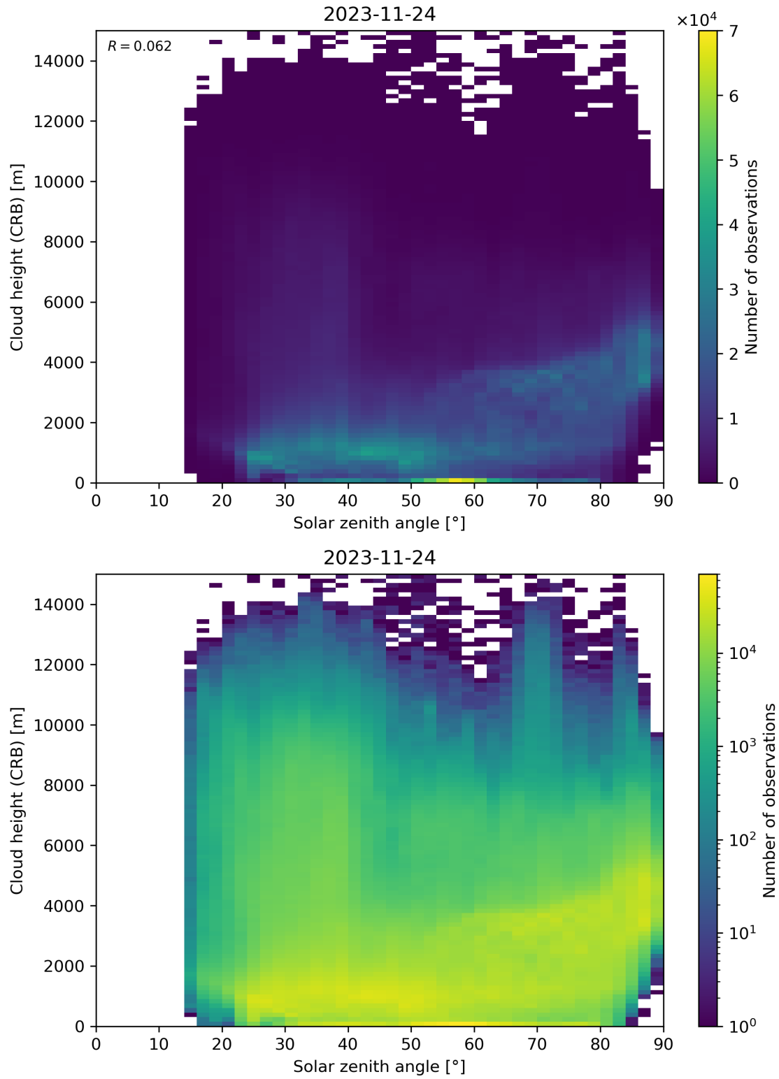
Figure 102: Scatter density plot of “Solar zenith angle” against “Cloud height (CRB)” for 2023-11-23 to 2023-11-25.
