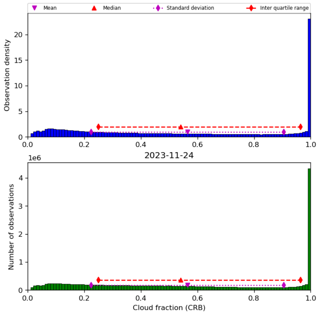
Figure 42: Histogram of “Cloud fraction (CRB)” for 2023-11-23 to 2023-11-25
