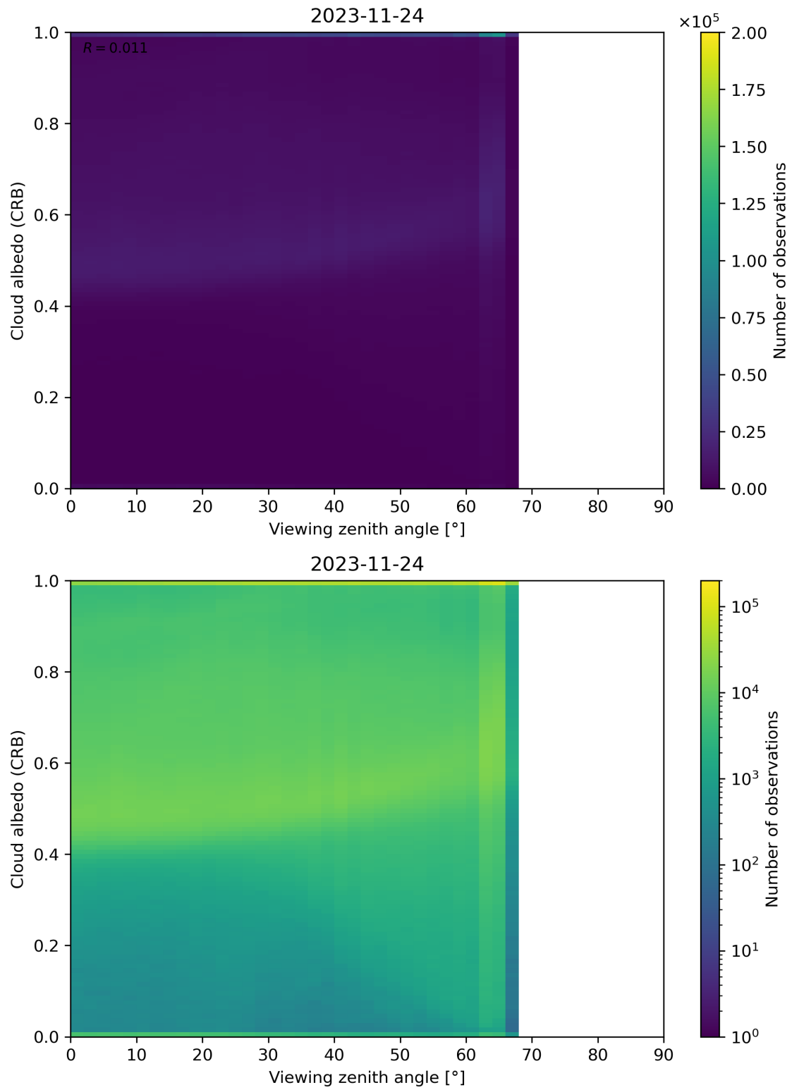
Figure 106: Scatter density plot of “Viewing zenith angle” against “Cloud albedo (CRB)” for 2023-11-23 to 2023-11-25.
