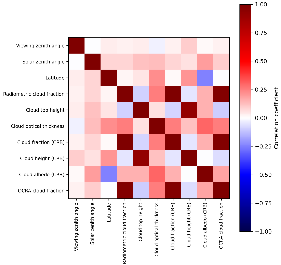
Figure 2: Map of correlation matrix for 2023-11-23 to 2023-11-25.
