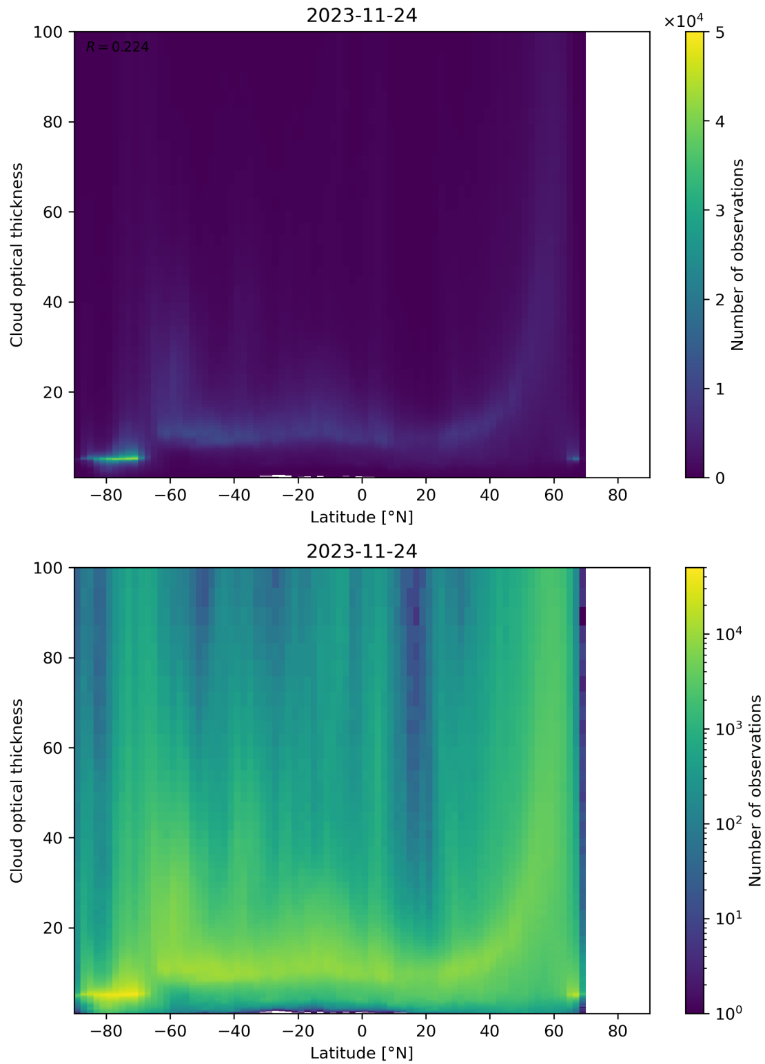
Figure 96: Scatter density plot of “Latitude” against “Cloud optical thickness” for 2023-11-23 to 2023-11-25.
