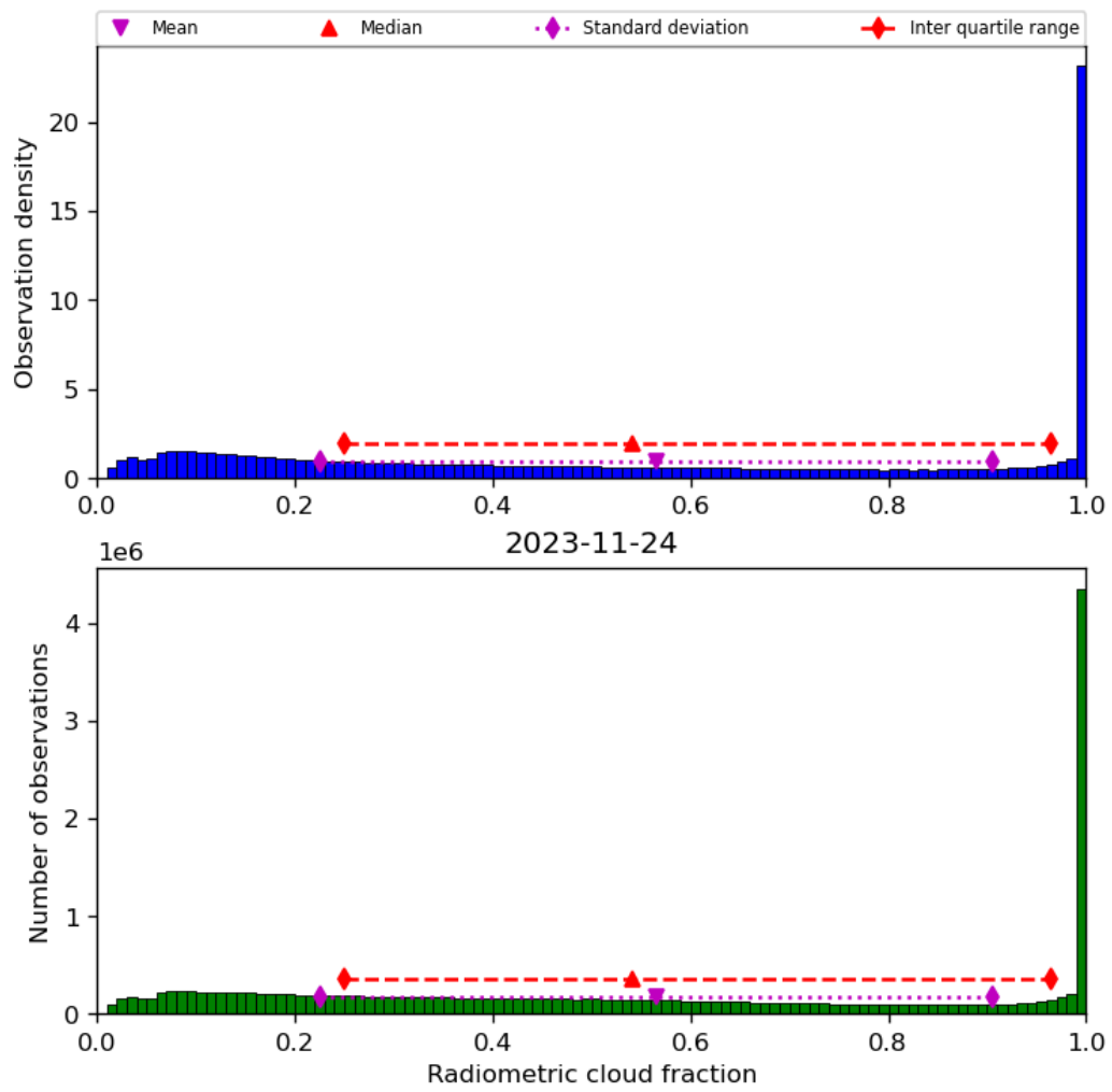
Figure 39: Histogram of “Radiometric cloud fraction” for 2023-11-23 to 2023-11-25
