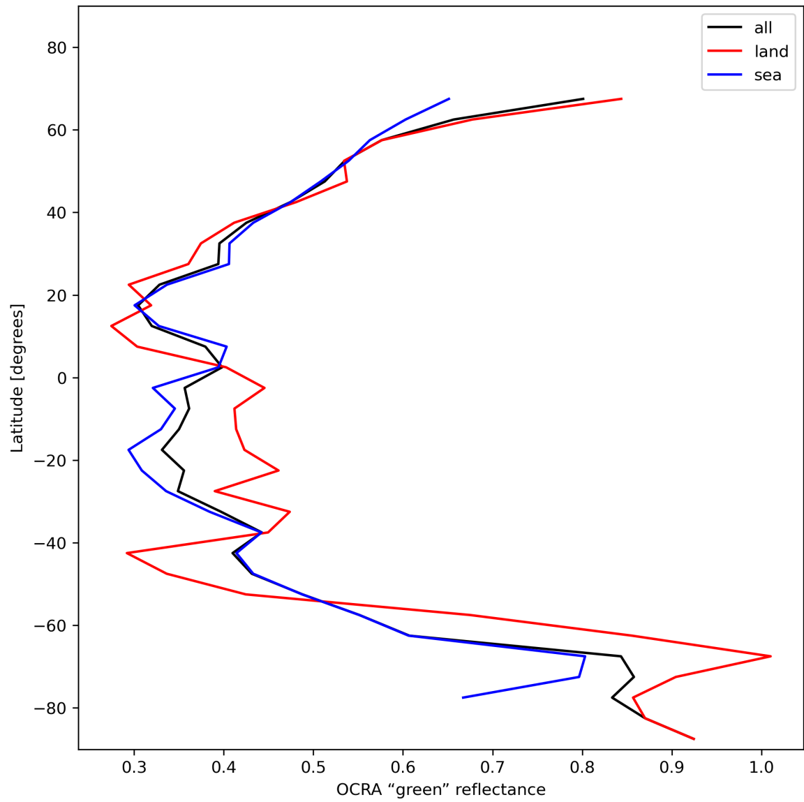
Figure 36: Zonal average of “OCRA “green” reflectance” for 2023-11-23 to 2023-11-25.
