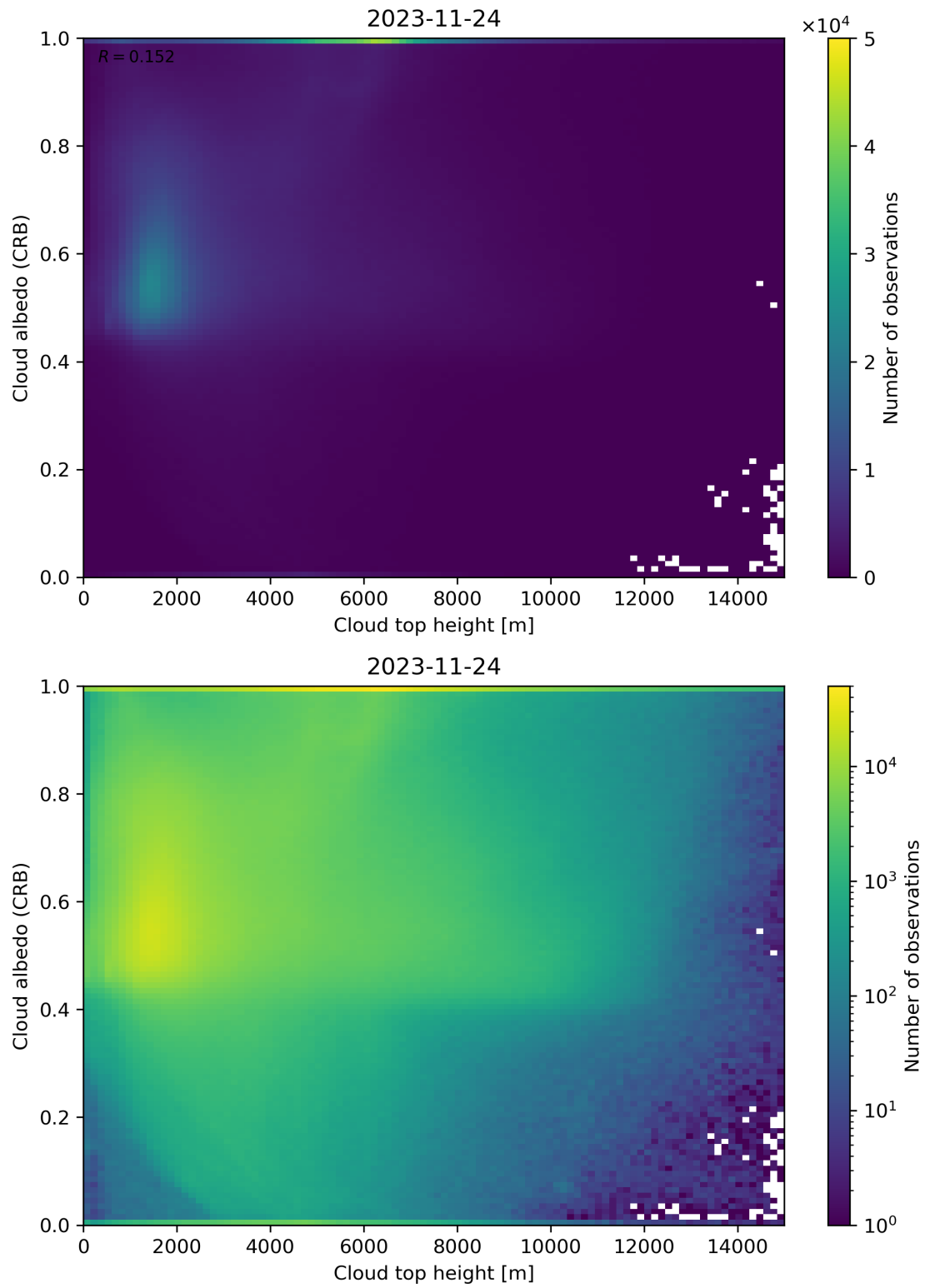
Figure 86: Scatter density plot of “Cloud top height” against “Cloud albedo (CRB)” for 2023-11-23 to 2023-11-25.
