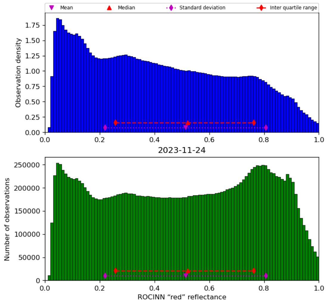
Figure 53: Histogram of “ROCINN “red” reflectance” for 2023-11-23 to 2023-11-25
