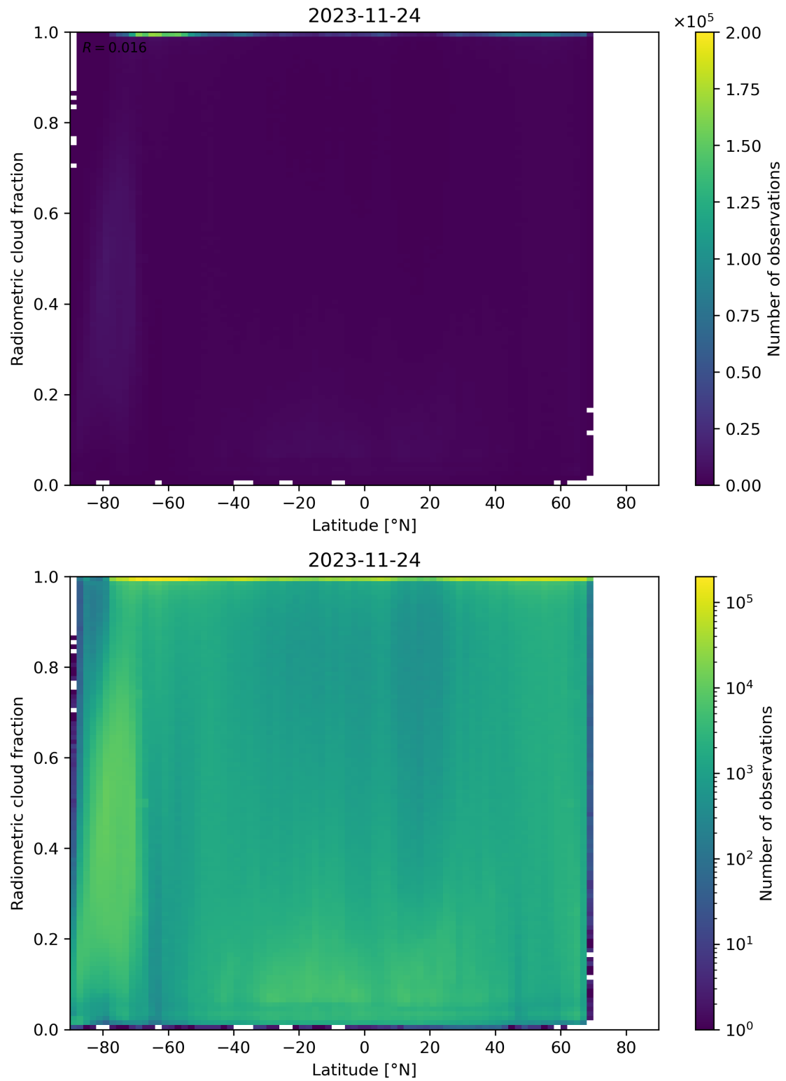
Figure 92: Scatter density plot of “Latitude” against “Radiometric cloud fraction” for 2023-11-23 to 2023-11-25.
