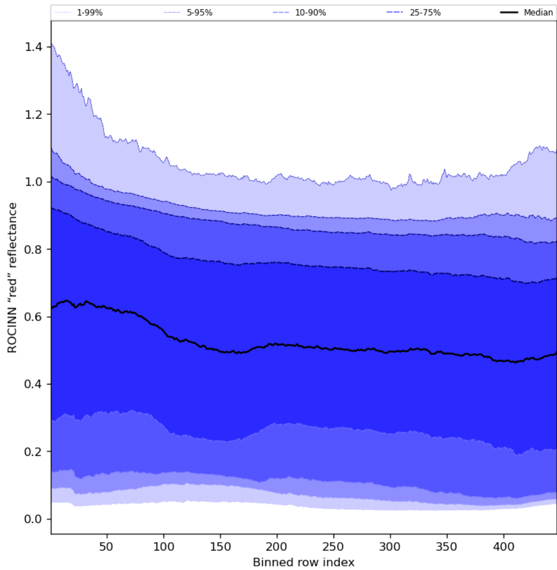
Figure 69: Along track statistics of “ROCINN “red” reflectance” for 2023-11-23 to 2023-11-25
