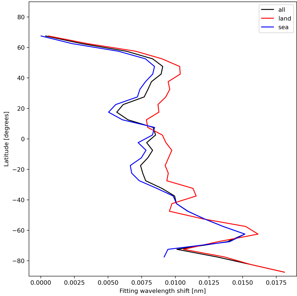
Figure 33: Zonal average of “Fitting wavelength shift” for 2023-11-23 to 2023-11-25.
