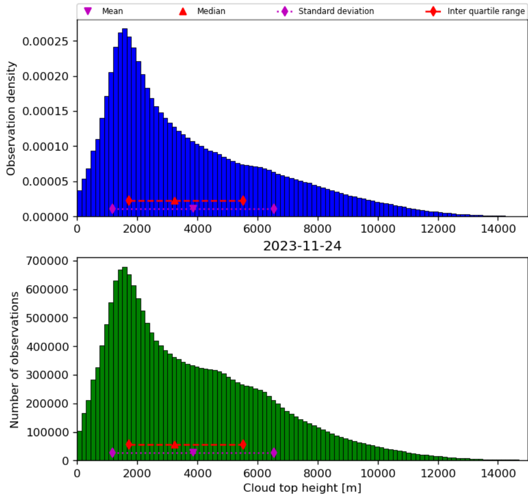
Figure 40: Histogram of “Cloud top height” for 2023-11-23 to 2023-11-25
