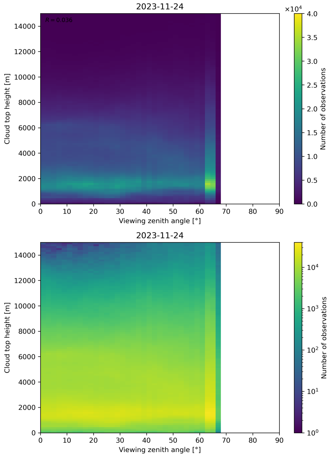
Figure 112: Scatter density plot of “Viewing zenith angle” against “Cloud top height” for 2023-11-23 to 2023-11-25.
