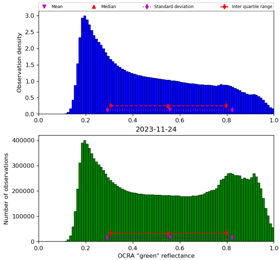
Figure 52: Histogram of “OCRA “green” reflectance” for 2023-11-23 to 2023-11-25
