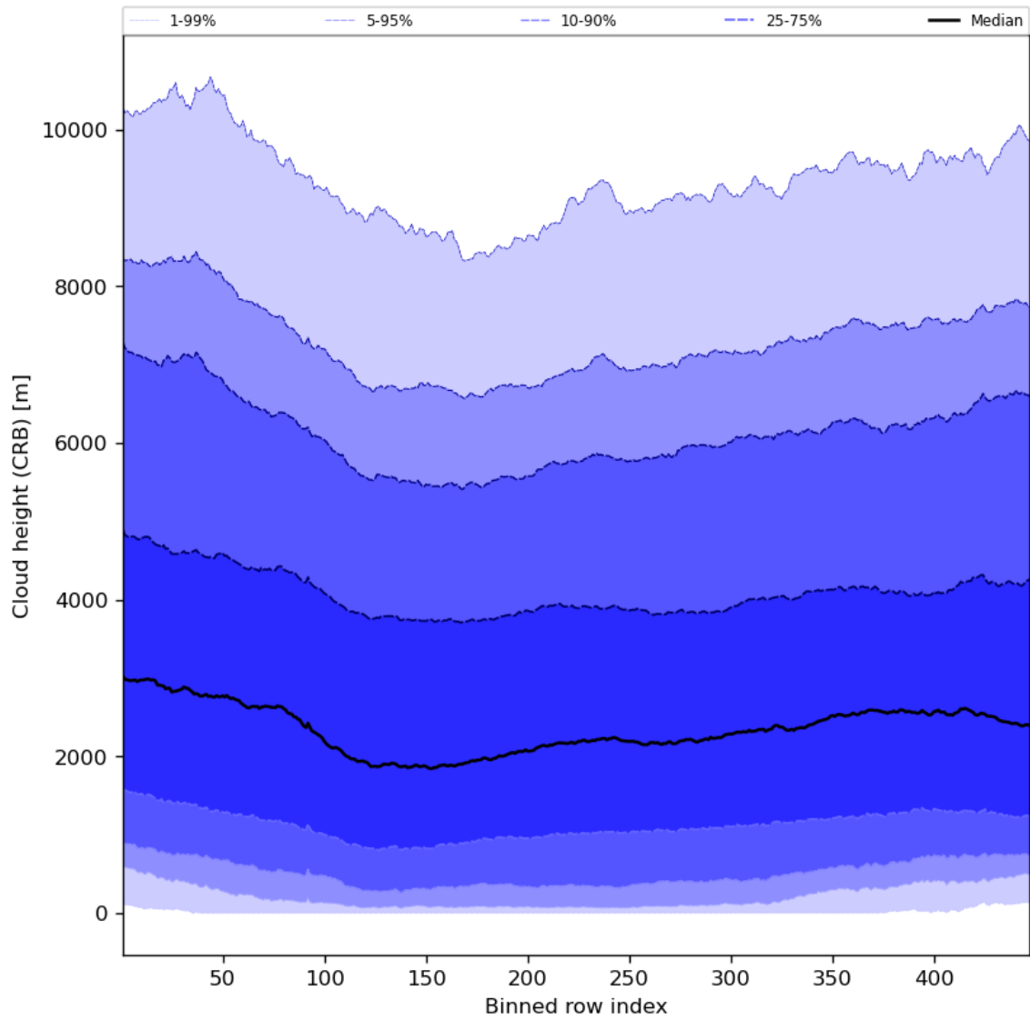
Figure 59: Along track statistics of “Cloud height (CRB)” for 2023-11-23 to 2023-11-25
