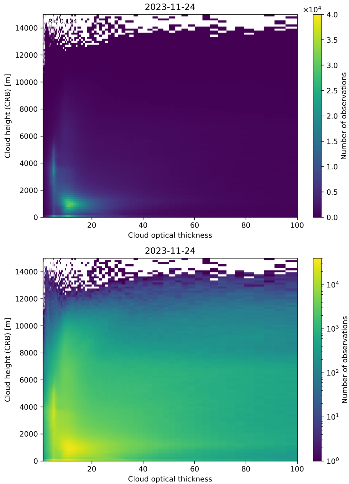
Figure 85: Scatter density plot of “Cloud optical thickness” against “Cloud height (CRB)” for 2023-11-23 to 2023-11-25.
