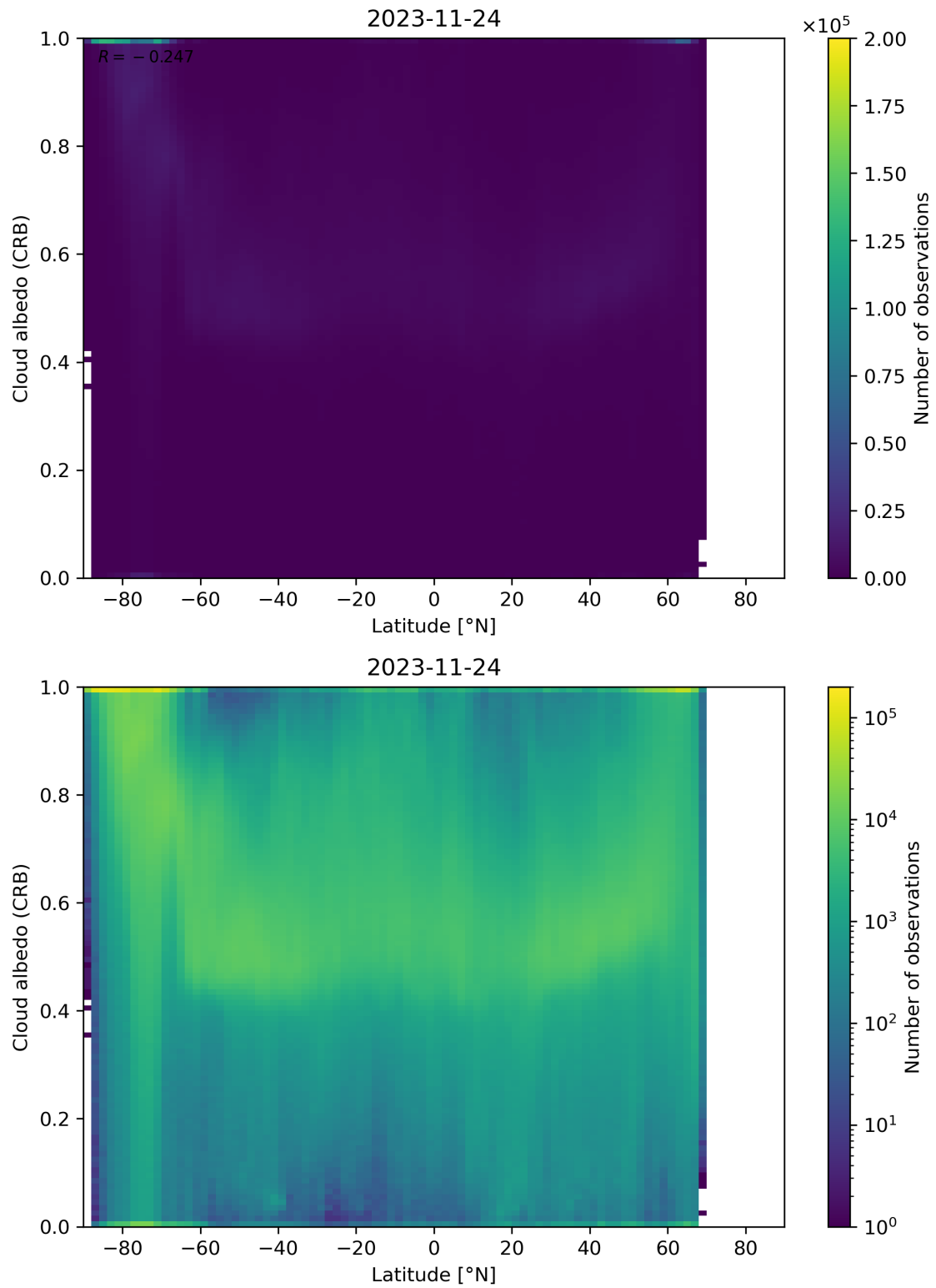
Figure 91: Scatter density plot of “Latitude” against “Cloud albedo (CRB)” for 2023-11-23 to 2023-11-25.
