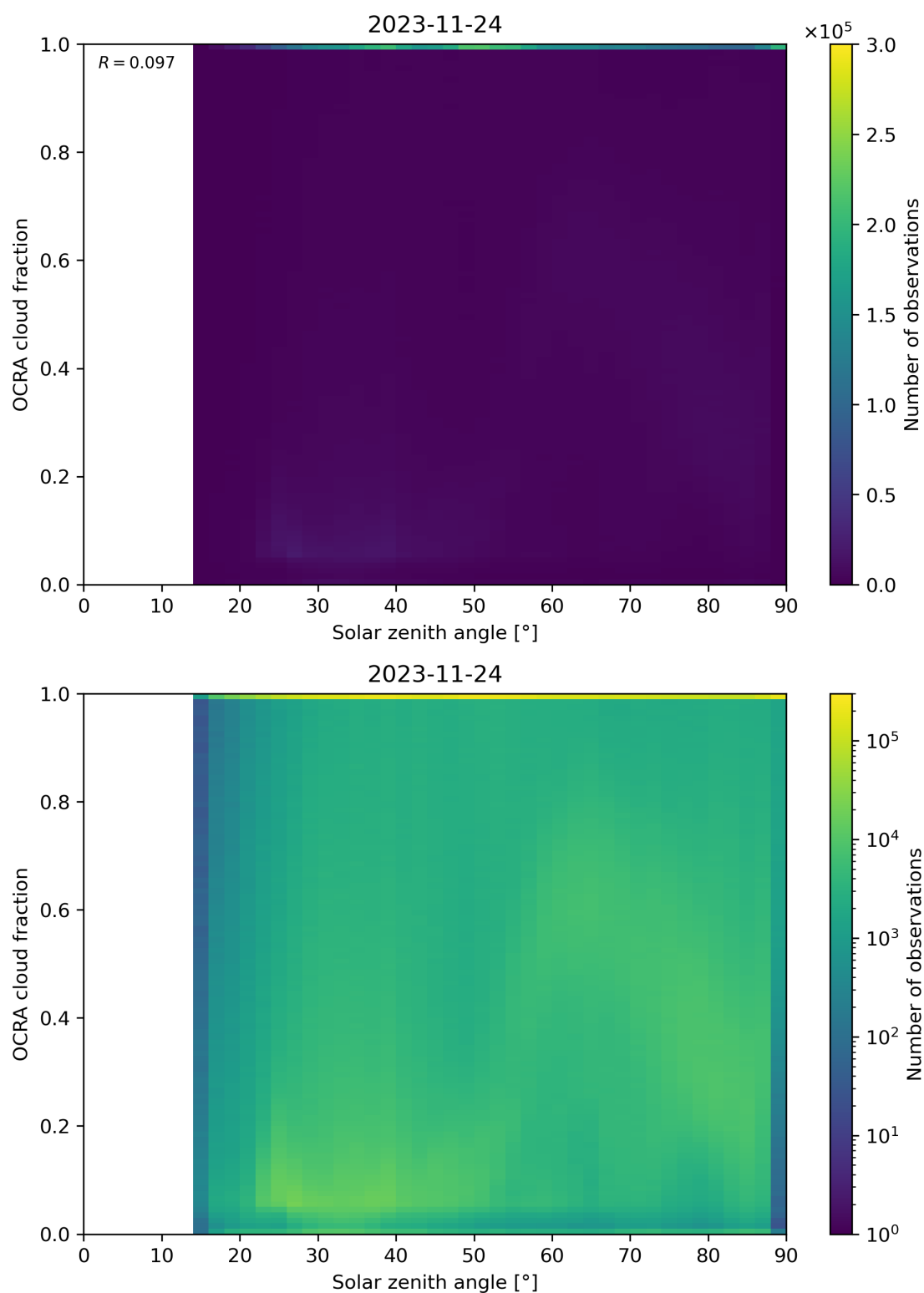
Figure 100: Scatter density plot of “Solar zenith angle” against “OCRA cloud fraction” for 2023-11-23 to 2023-11-25.
