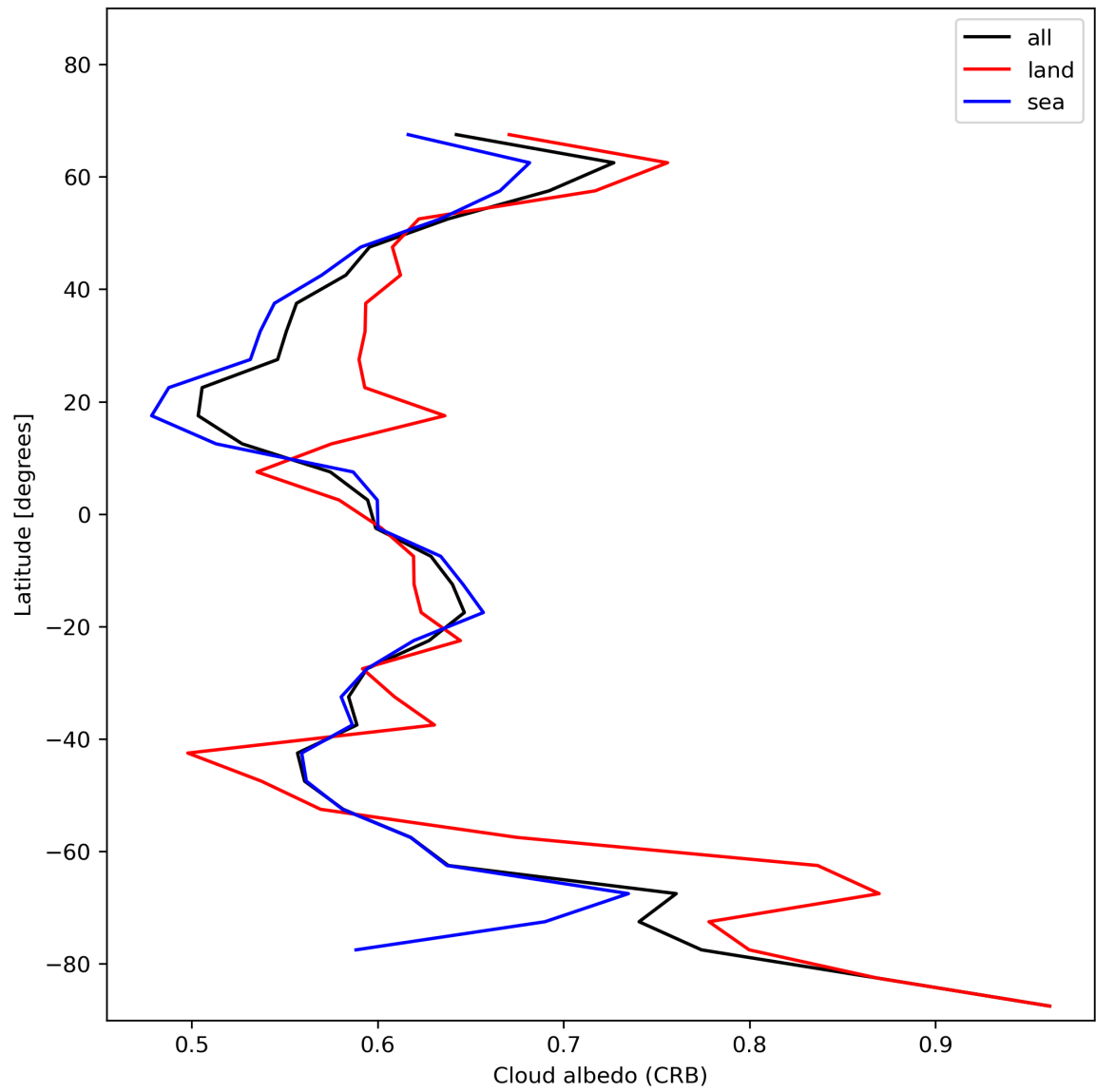
Figure 28: Zonal average of “Cloud albedo (CRB)” for 2023-11-23 to 2023-11-25.
