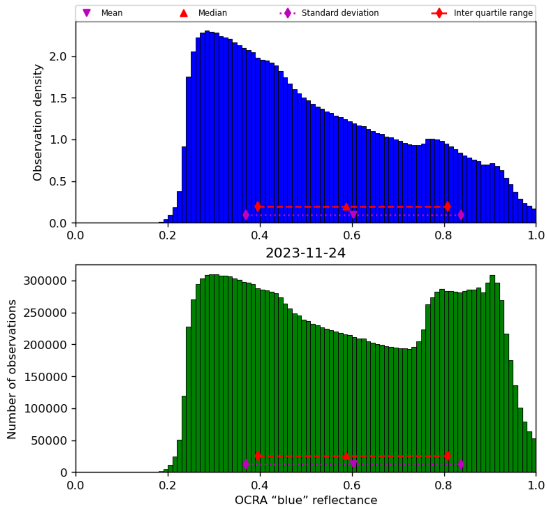
Figure 51: Histogram of “OCRA “blue” reflectance” for 2023-11-23 to 2023-11-25
