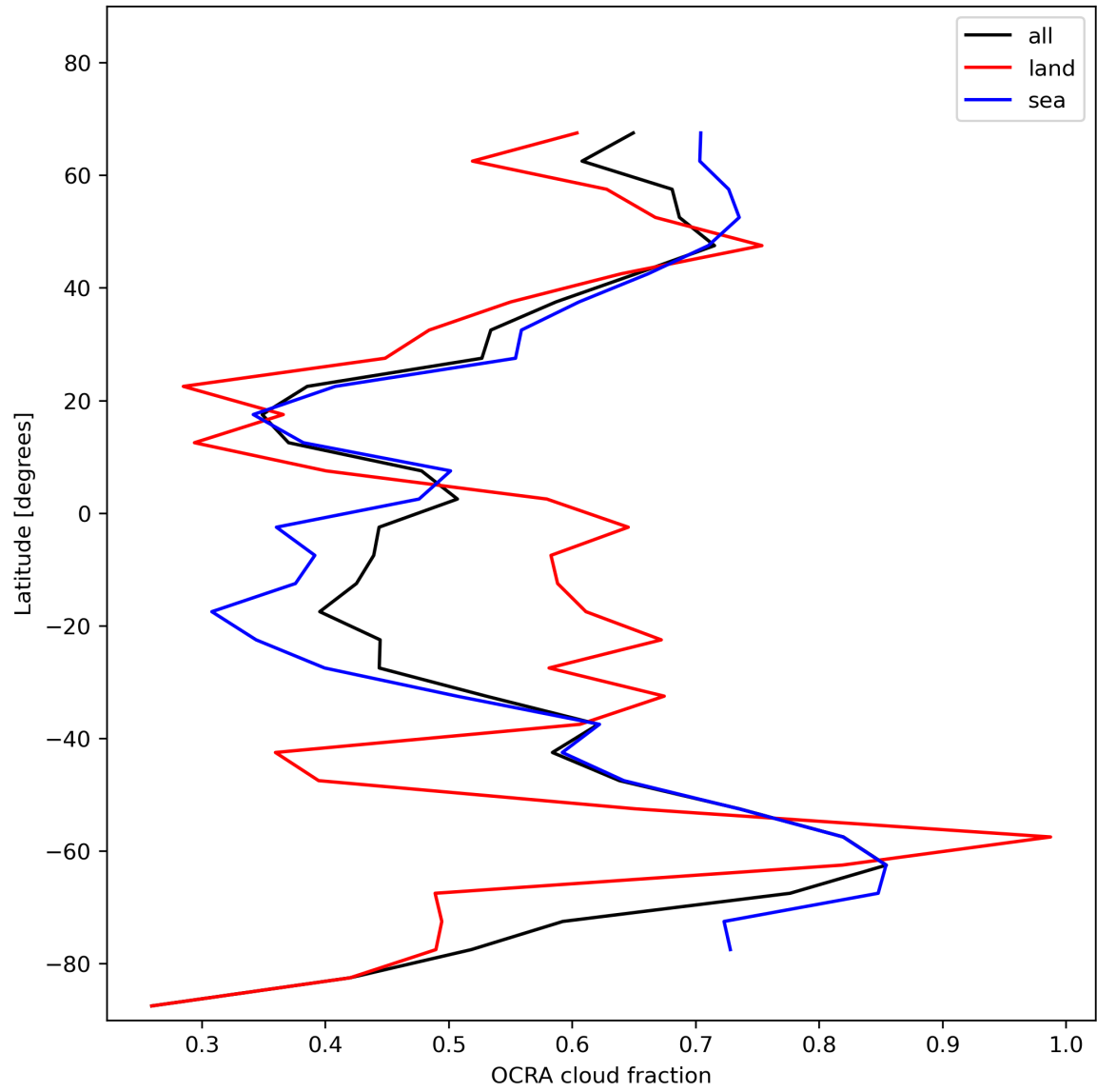
Figure 34: Zonal average of “OCRA cloud fraction” for 2023-11-23 to 2023-11-25.
