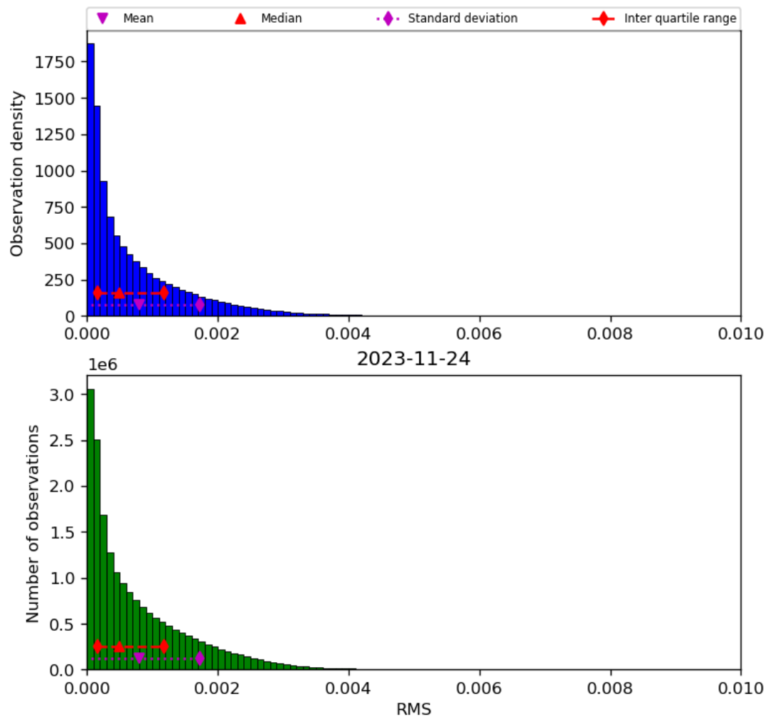
Figure 47: Histogram of “RMS” for 2023-11-23 to 2023-11-25
