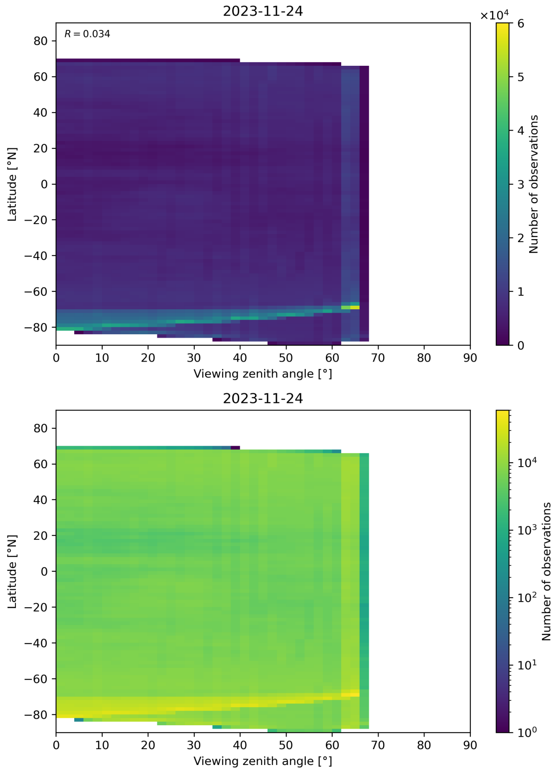
Figure 113: Scatter density plot of “Viewing zenith angle” against “Latitude” for 2023-11-23 to 2023-11-25.
