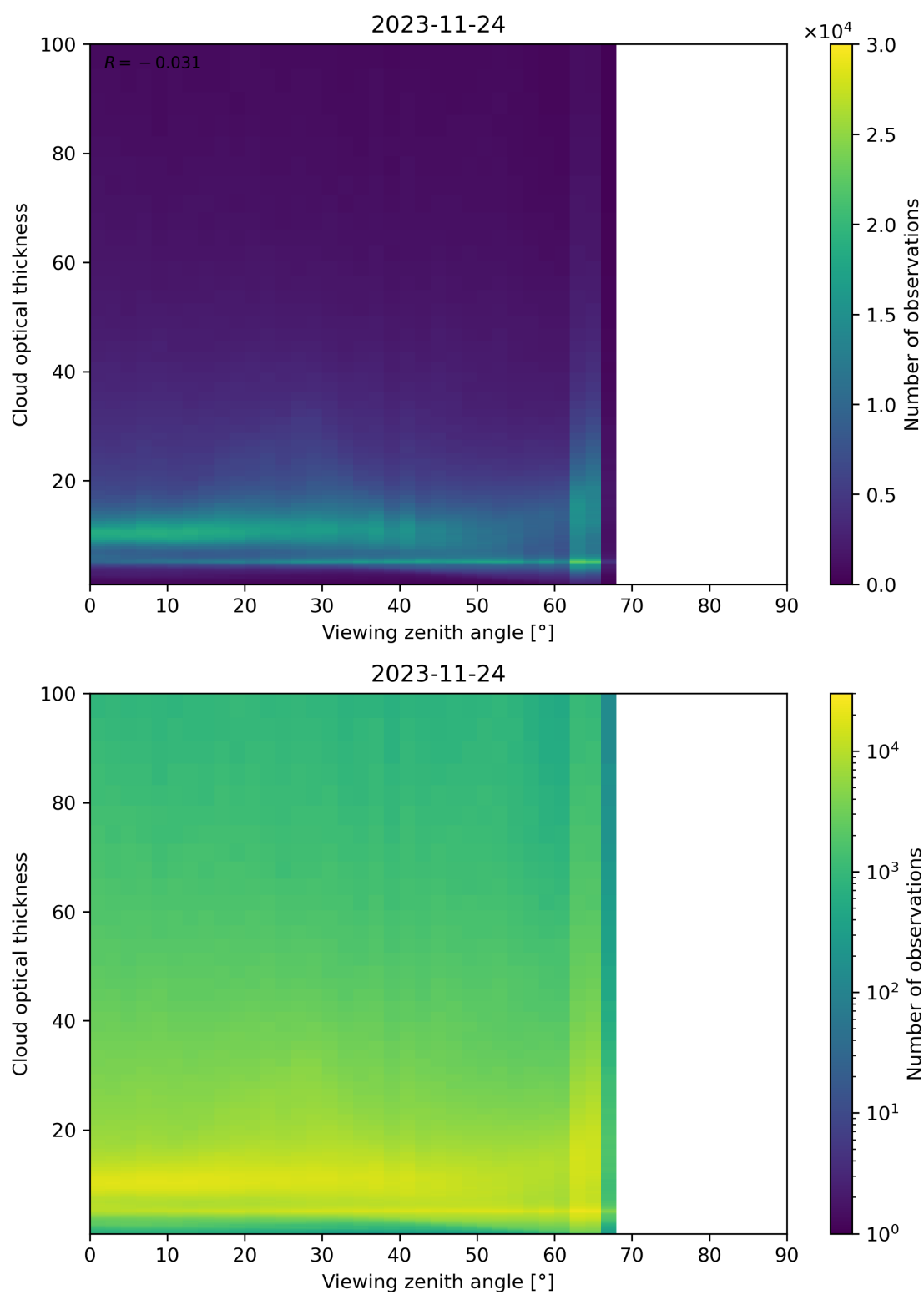
Figure 111: Scatter density plot of “Viewing zenith angle” against “Cloud optical thickness” for 2023-11-23 to 2023-11-25.
