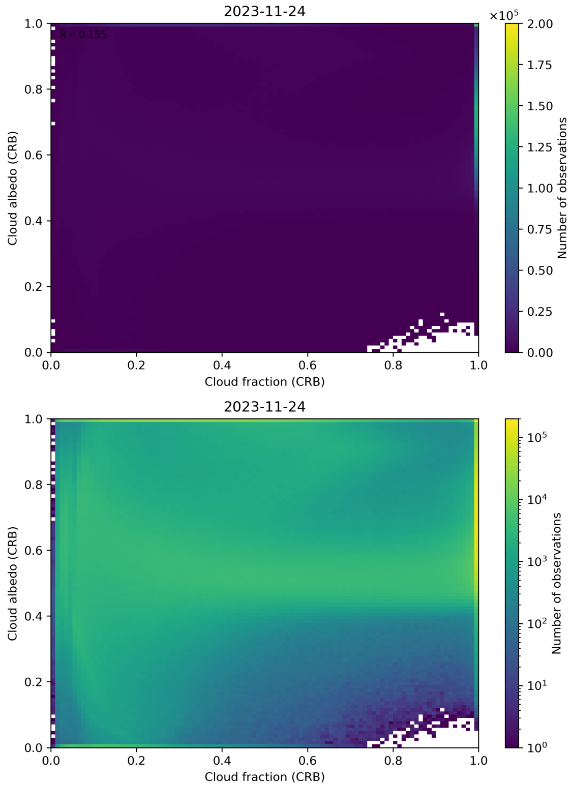
Figure 77: Scatter density plot of “Cloud fraction (CRB)” against “Cloud albedo (CRB)” for 2023-11-23 to 2023-11-25.
