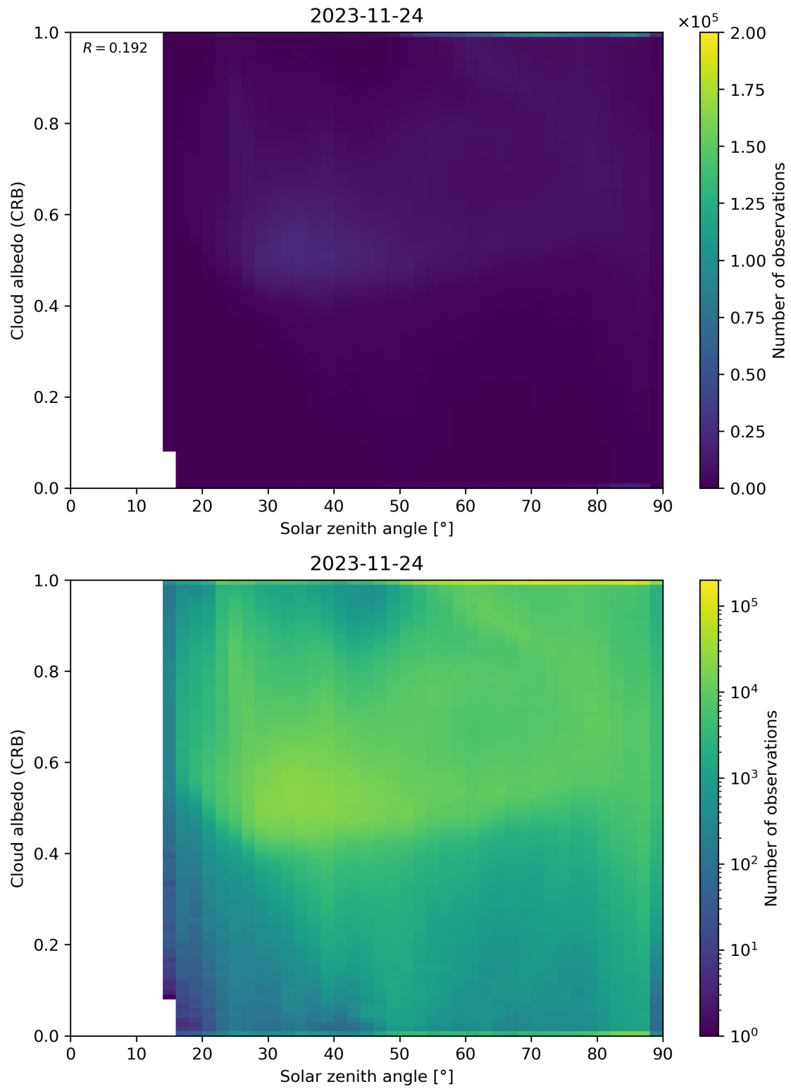
Figure 98: Scatter density plot of “Solar zenith angle” against “Cloud albedo (CRB)” for 2023-11-23 to 2023-11-25.
