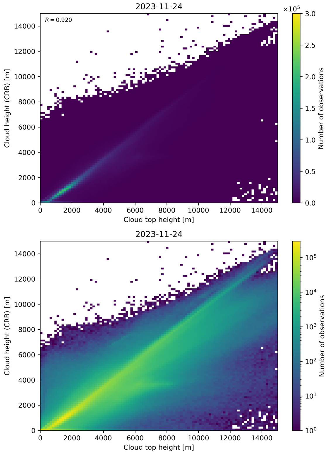
Figure 89: Scatter density plot of “Cloud top height” against “Cloud height (CRB)” for 2023-11-23 to 2023-11-25.
