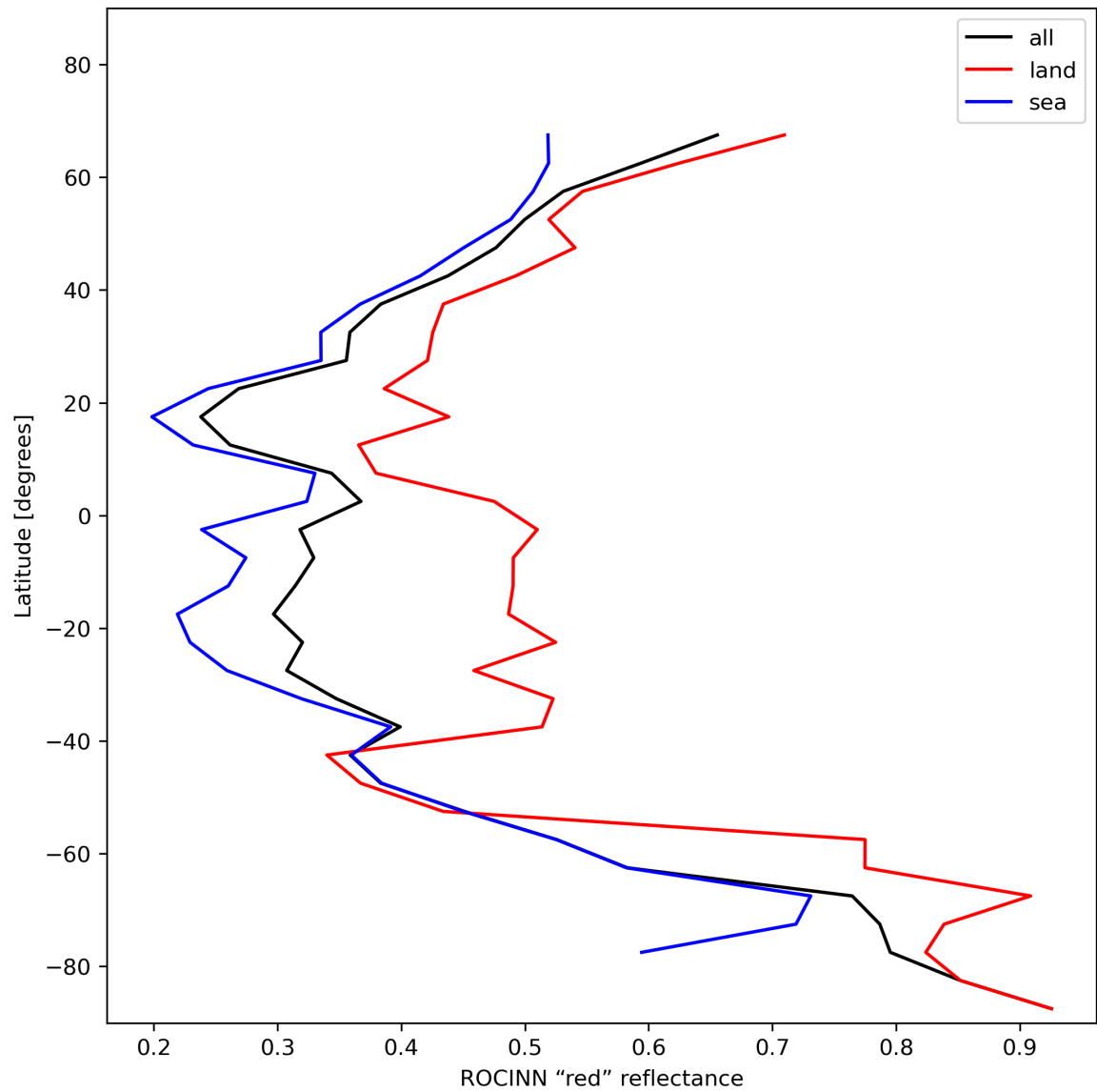
Figure 37: Zonal average of “ROCINN “red” reflectance” for 2023-11-23 to 2023-11-25.
