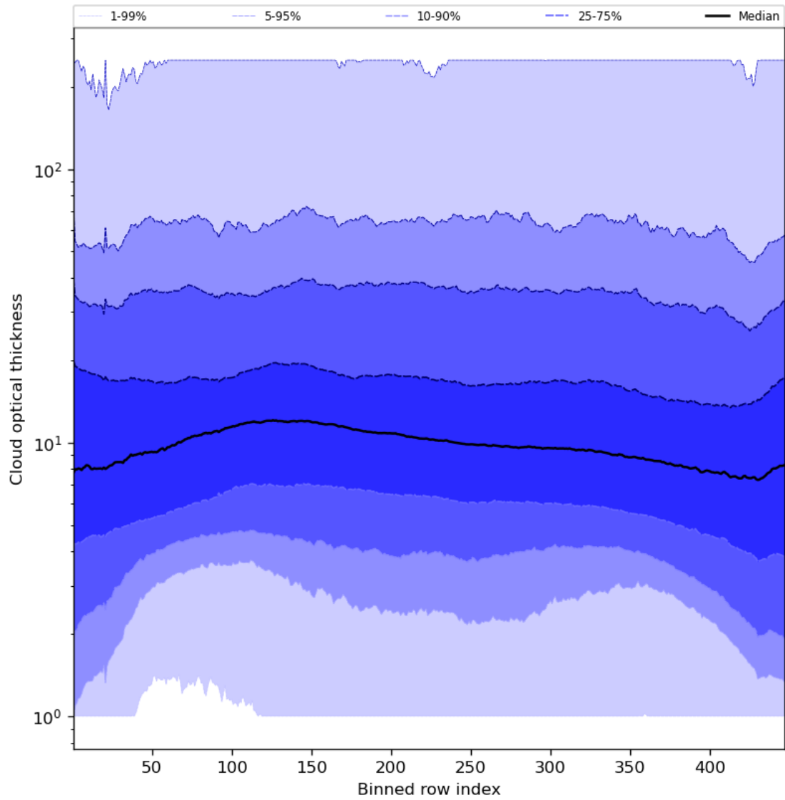
Figure 57: Along track statistics of “Cloud optical thickness” for 2023-11-23 to 2023-11-25
