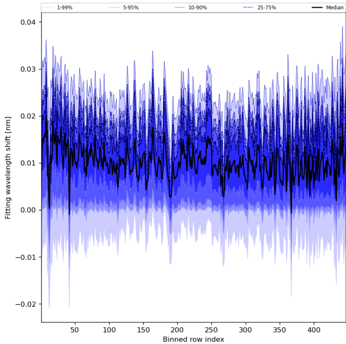
Figure 65: Along track statistics of “Fitting wavelength shift” for 2023-11-23 to 2023-11-25
