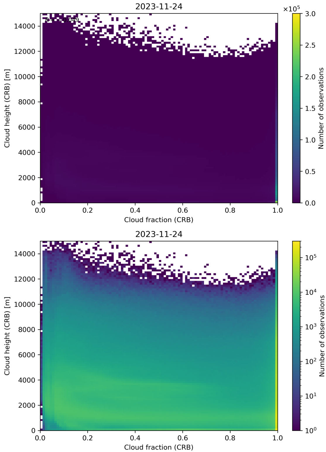
Figure 79: Scatter density plot of “Cloud fraction (CRB)” against “Cloud height (CRB)” for 2023-11-23 to 2023-11-25.
