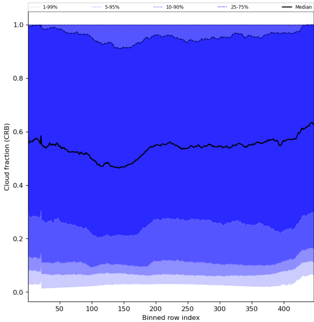
Figure 58: Along track statistics of “Cloud fraction (CRB)” for 2023-11-23 to 2023-11-25
