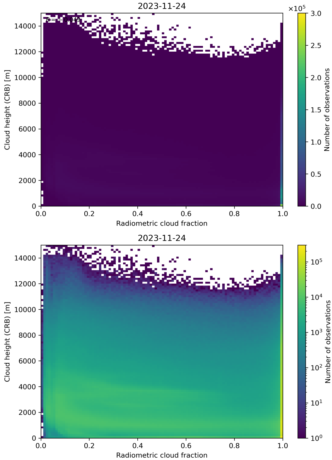
Figure 74: Scatter density plot of “Radiometric cloud fraction” against “Cloud height (CRB)” for 2023-11-23 to 2023-11-25.
