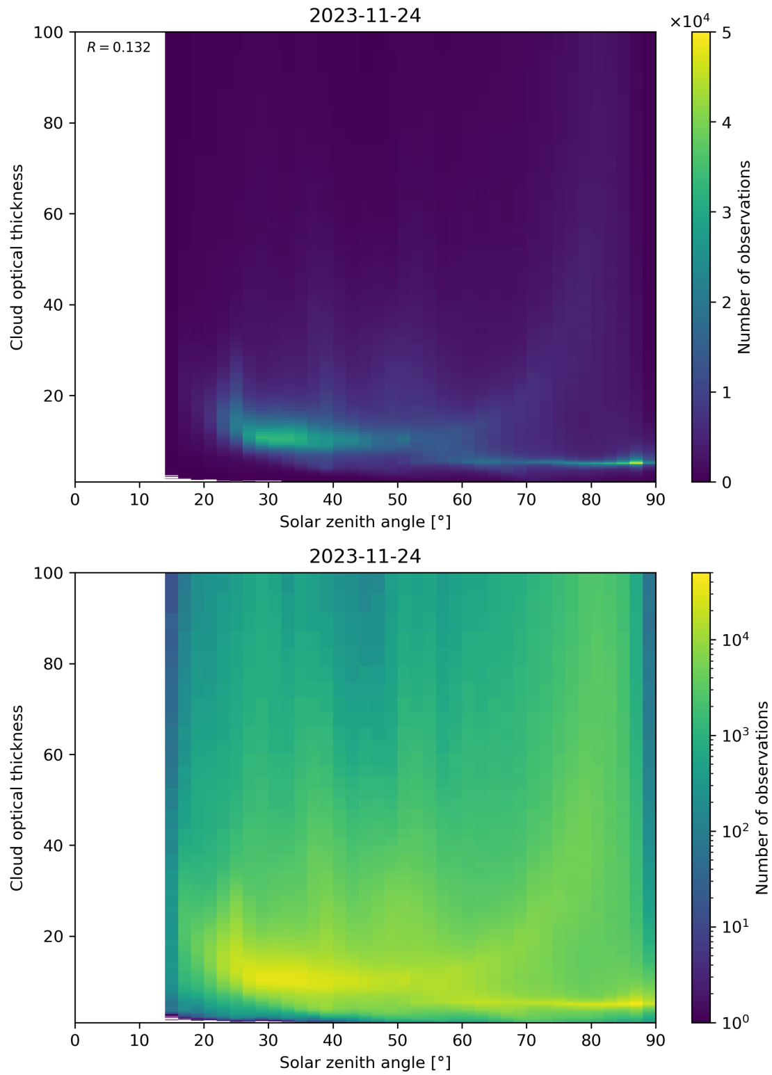
Figure 103: Scatter density plot of “Solar zenith angle” against “Cloud optical thickness” for 2023-11-23 to 2023-11-25.
