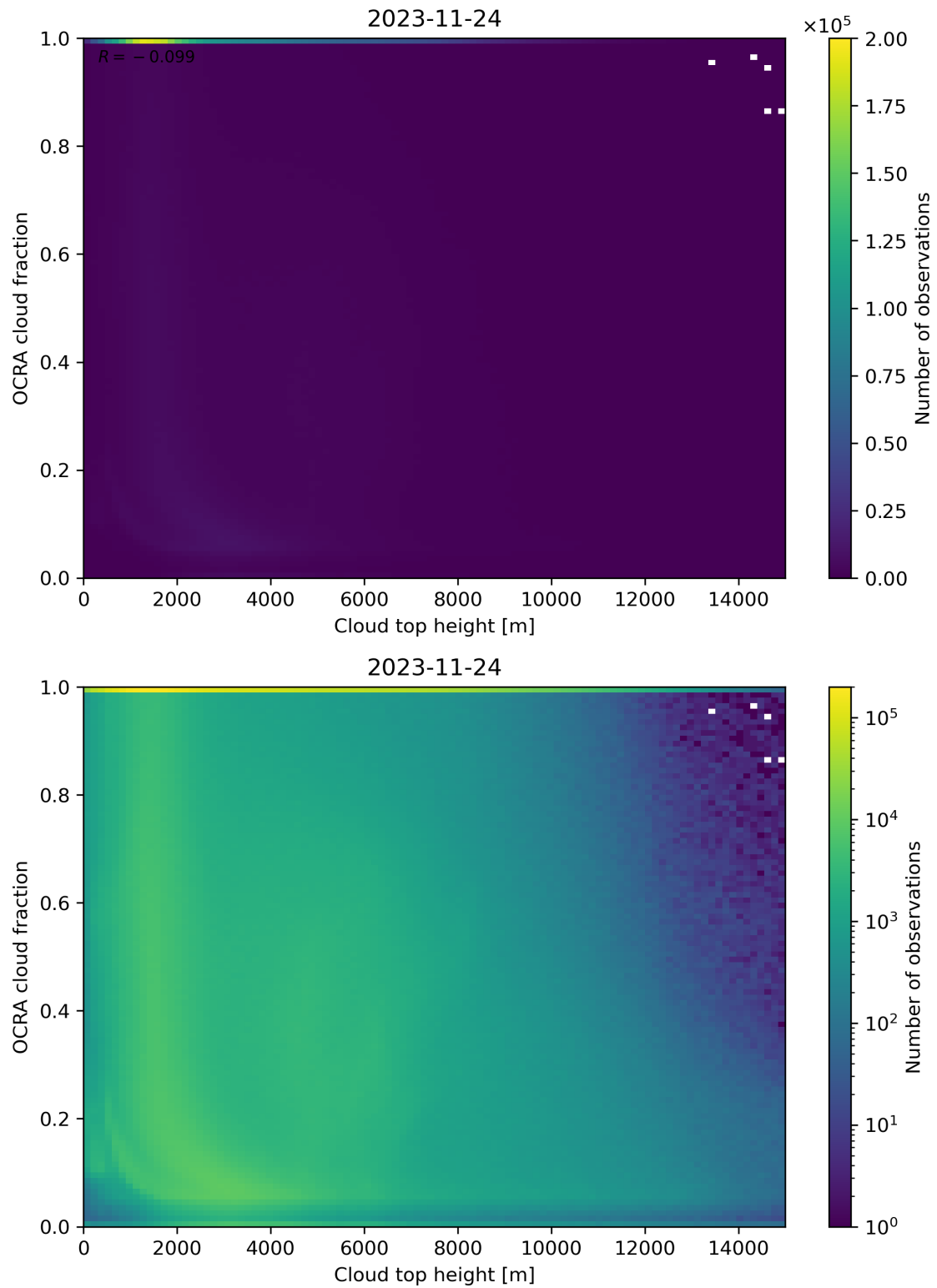
Figure 87: Scatter density plot of “Cloud top height” against “OCRA cloud fraction” for 2023-11-23 to 2023-11-25.
