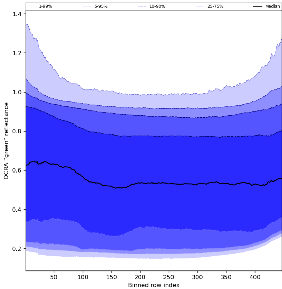
Figure 68: Along track statistics of "OCRA "green" reflectance" for 2023-11-23 to 2023-11-25
