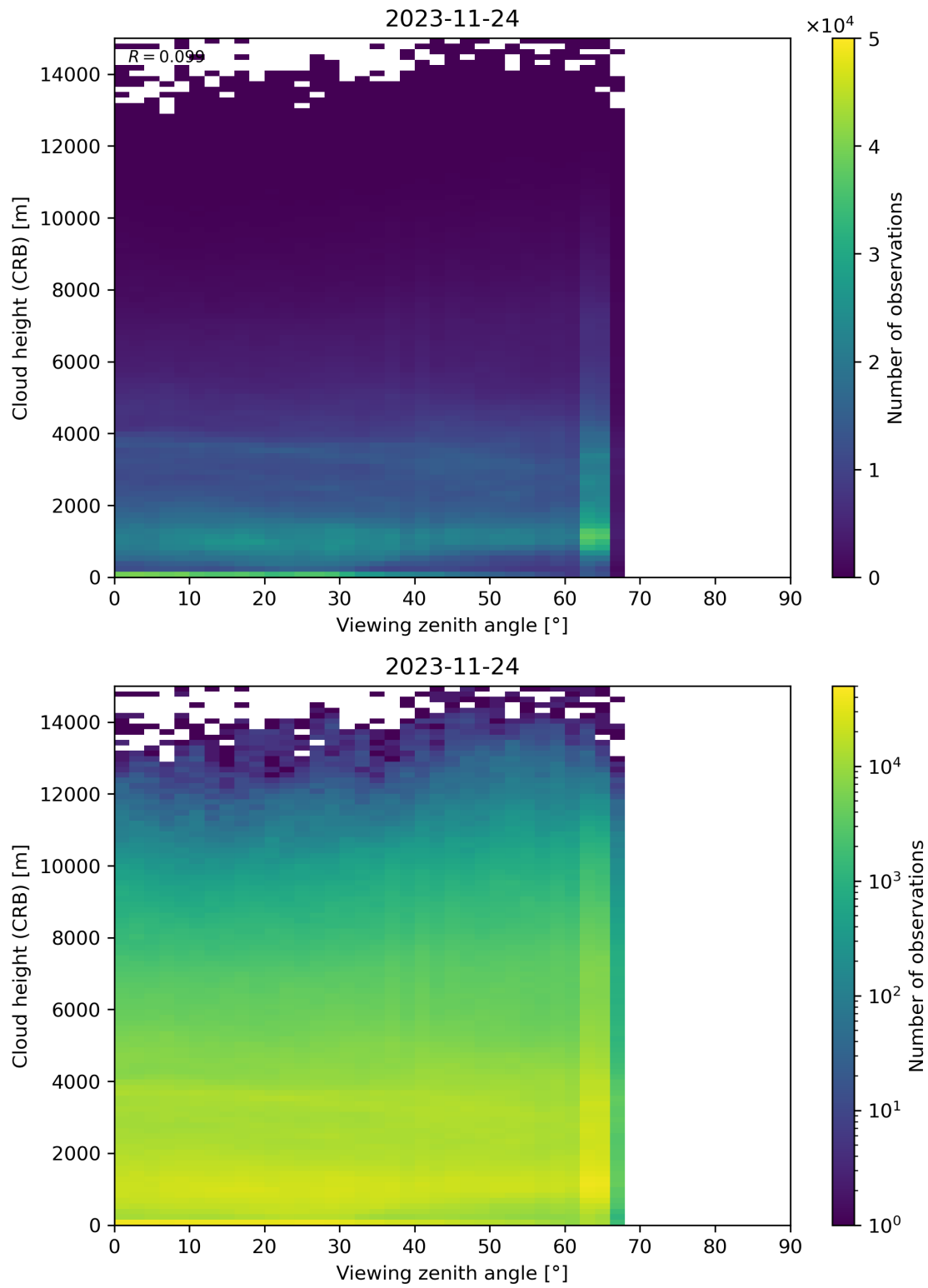
Figure 110: Scatter density plot of “Viewing zenith angle” against “Cloud height (CRB)” for 2023-11-23 to 2023-11-25.
