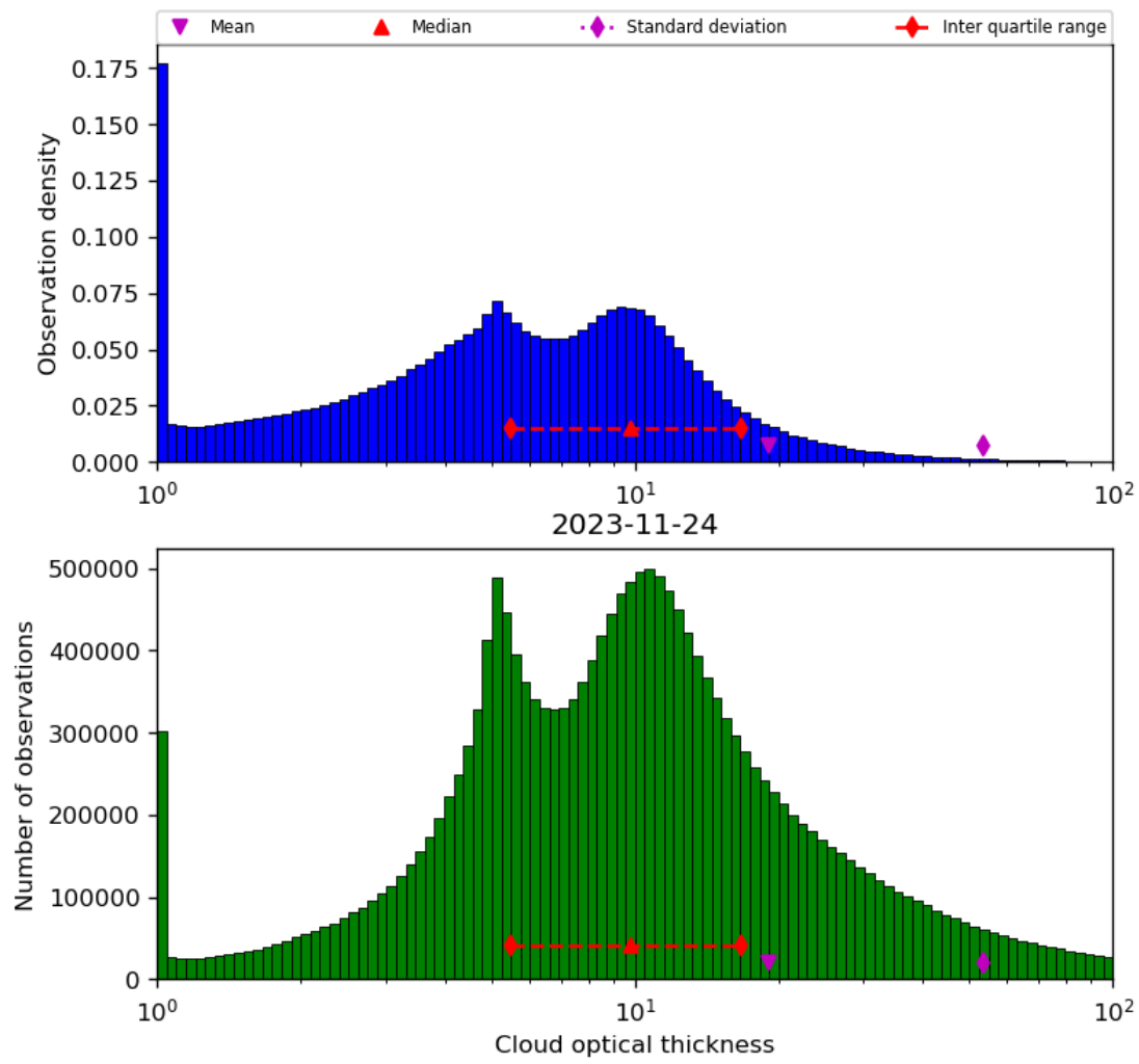
Figure 41: Histogram of “Cloud optical thickness” for 2023-11-23 to 2023-11-25
