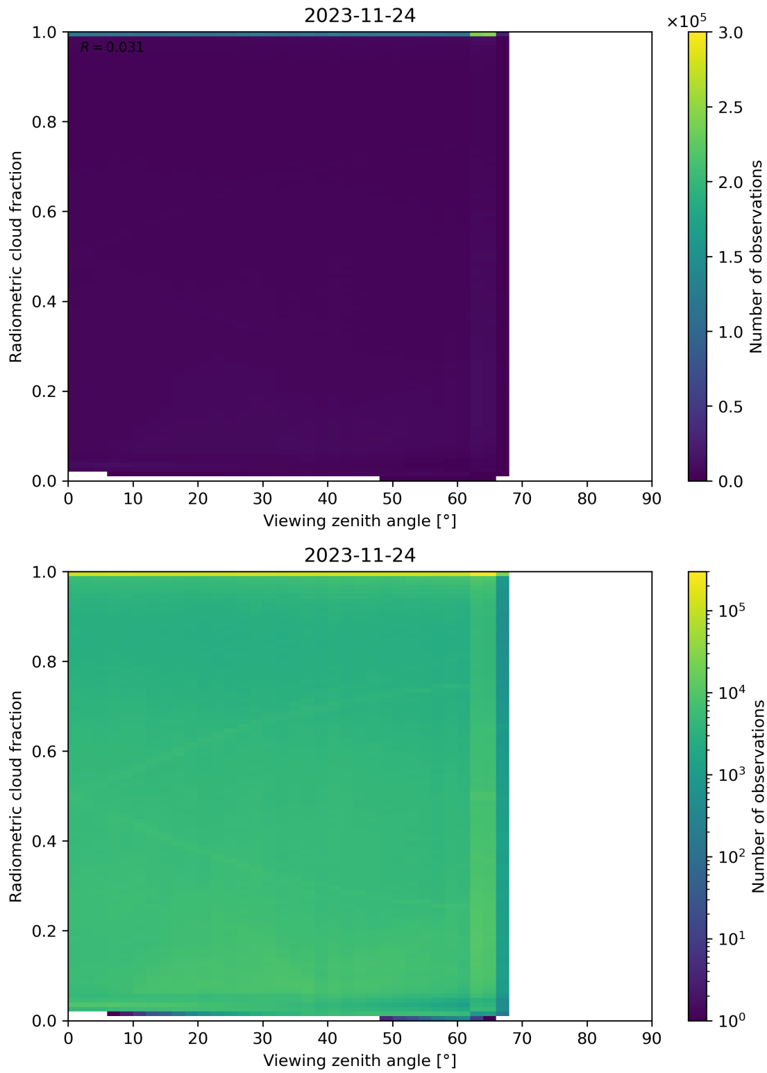
Figure 107: Scatter density plot of “Viewing zenith angle” against “Radiometric cloud fraction” for 2023-11-23 to 2023-11-25.
