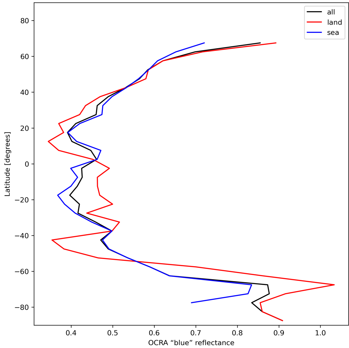
Figure 35: Zonal average of “OCRA “blue” reflectance” for 2023-11-23 to 2023-11-25.
