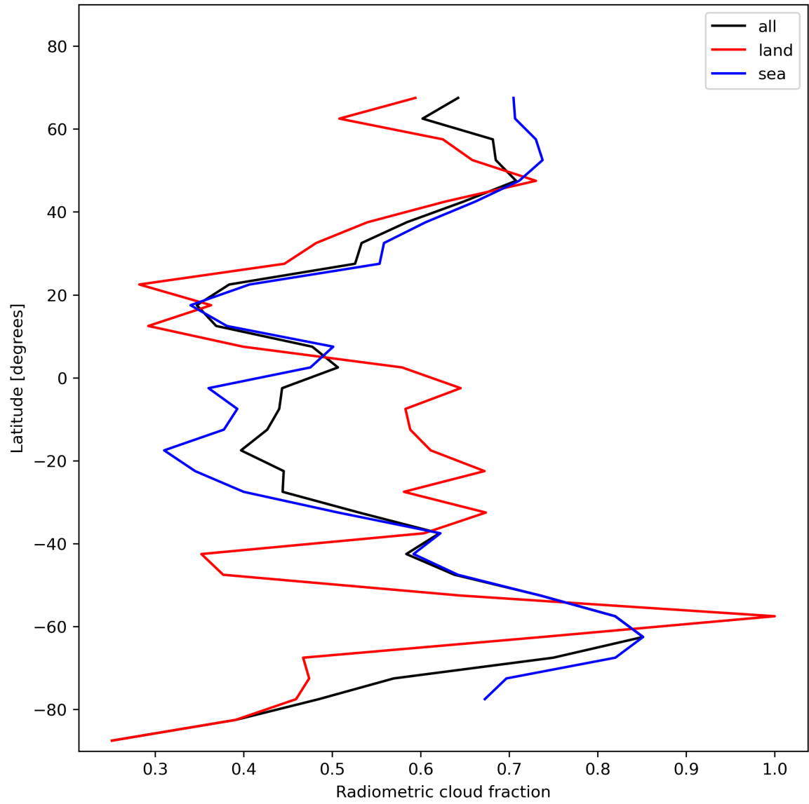
Figure 23: Zonal average of “Radiometric cloud fraction” for 2023-11-23 to 2023-11-25.
