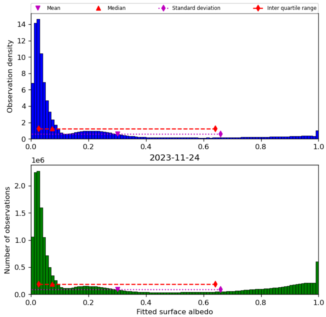
Figure 45: Histogram of “Fitted surface albedo” for 2023-11-23 to 2023-11-25
