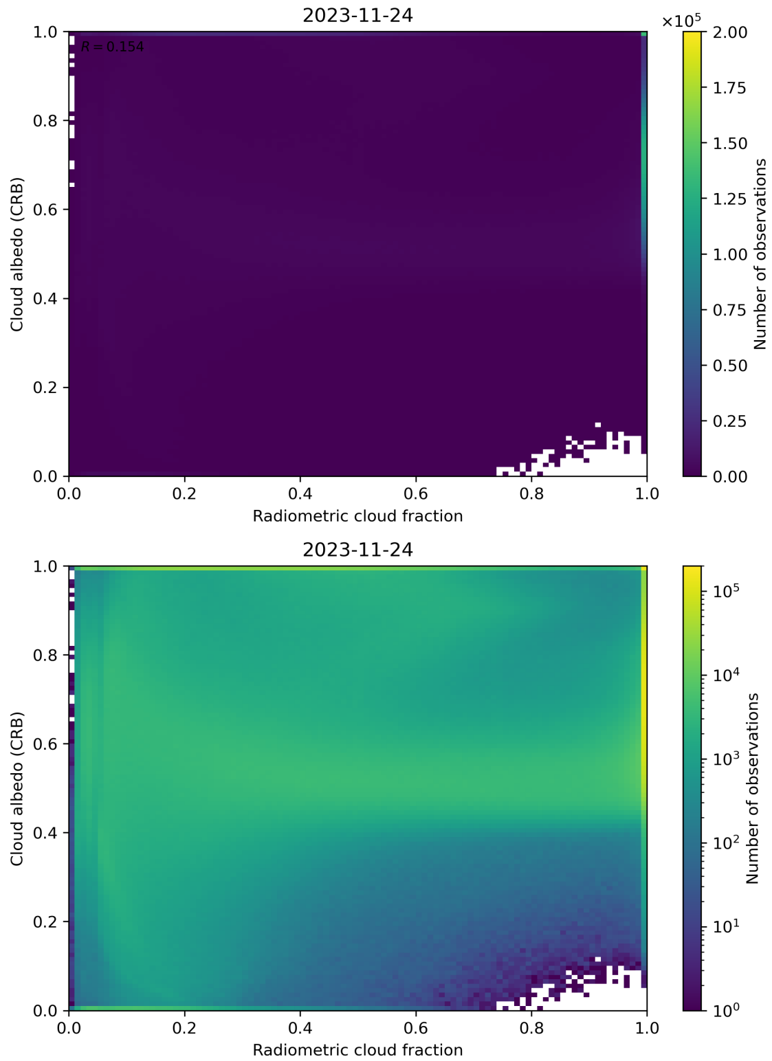
Figure 71: Scatter density plot of “Radiometric cloud fraction” against “Cloud albedo (CRB)” for 2023-11-23 to 2023-11-25.
