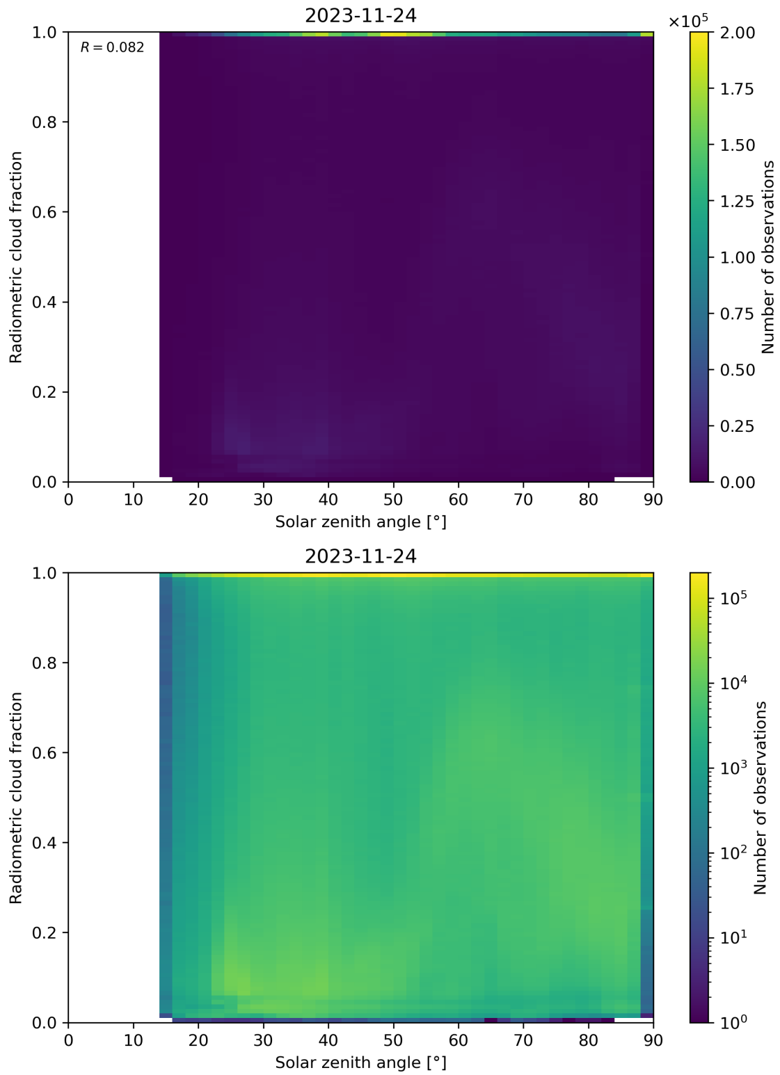
Figure 99: Scatter density plot of “Solar zenith angle” against “Radiometric cloud fraction” for 2023-11-23 to 2023-11-25.
