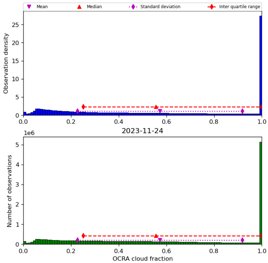
Figure 50: Histogram of “OCRA cloud fraction” for 2023-11-23 to 2023-11-25
