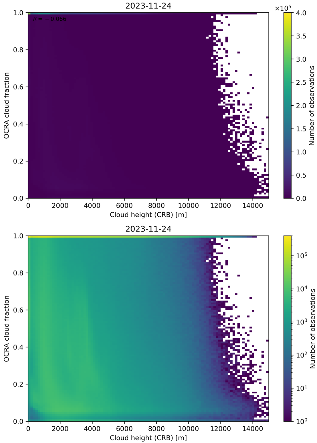
Figure 81: Scatter density plot of “Cloud height (CRB)” against “OCRA cloud fraction” for 2023-11-23 to 2023-11-25.
