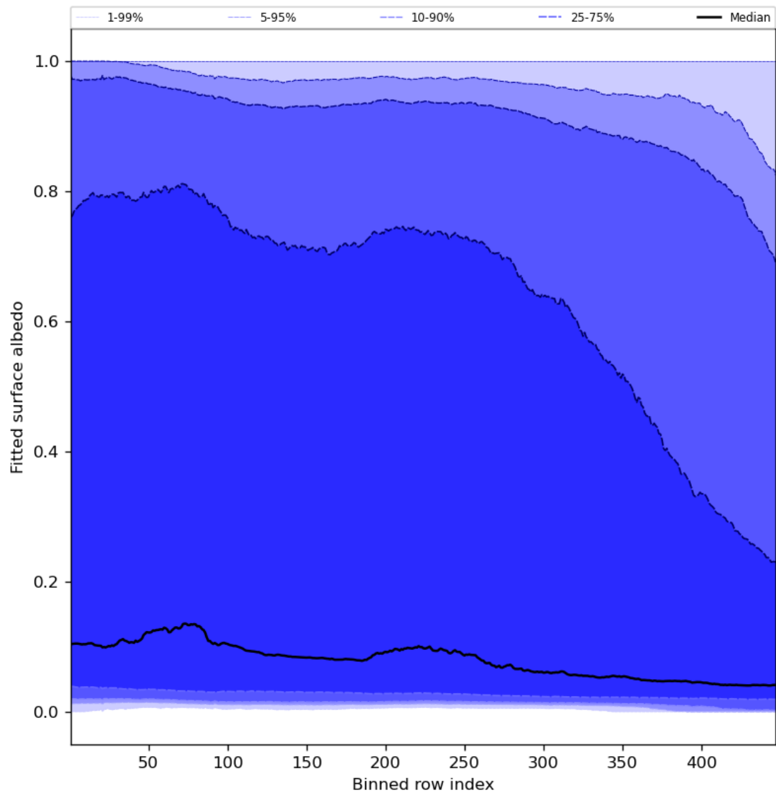
Figure 61: Along track statistics of “Fitted surface albedo” for 2023-11-23 to 2023-11-25
