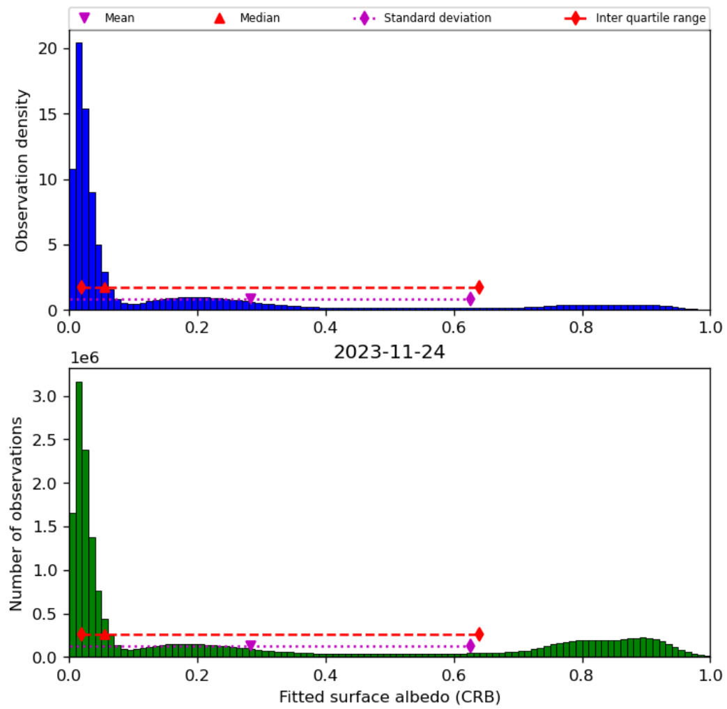
Figure 46: Histogram of “Fitted surface albedo (CRB)” for 2023-11-23 to 2023-11-25
