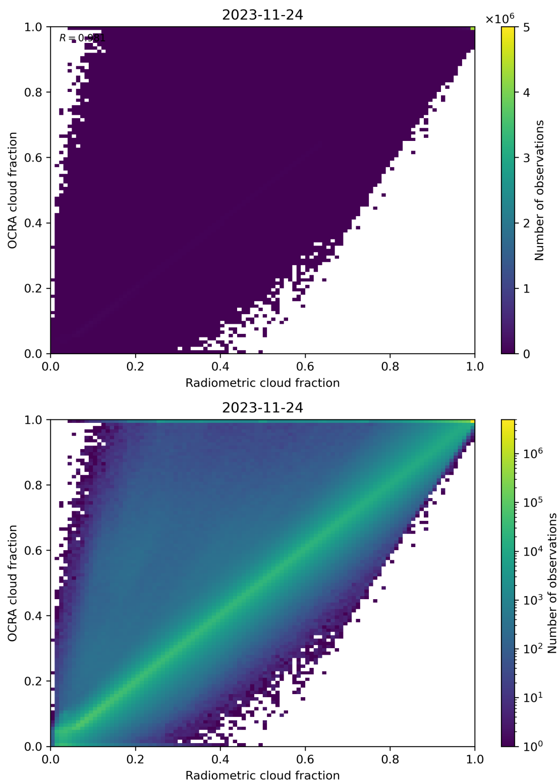
Figure 72: Scatter density plot of “Radiometric cloud fraction” against “OCRA cloud fraction” for 2023-11-23 to 2023-11-25.
