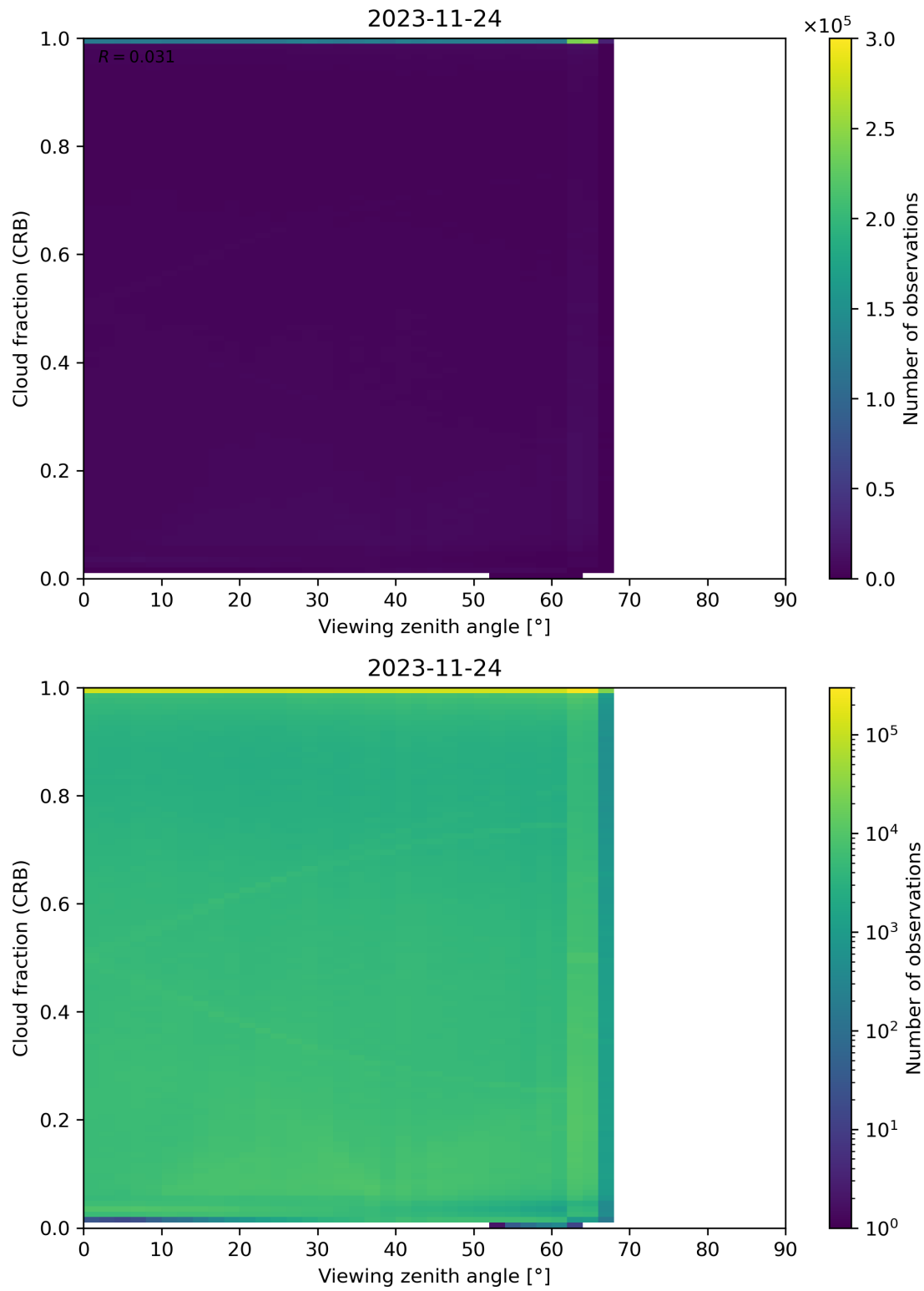
Figure 109: Scatter density plot of “Viewing zenith angle” against “Cloud fraction (CRB)” for 2023-11-23 to 2023-11-25.
