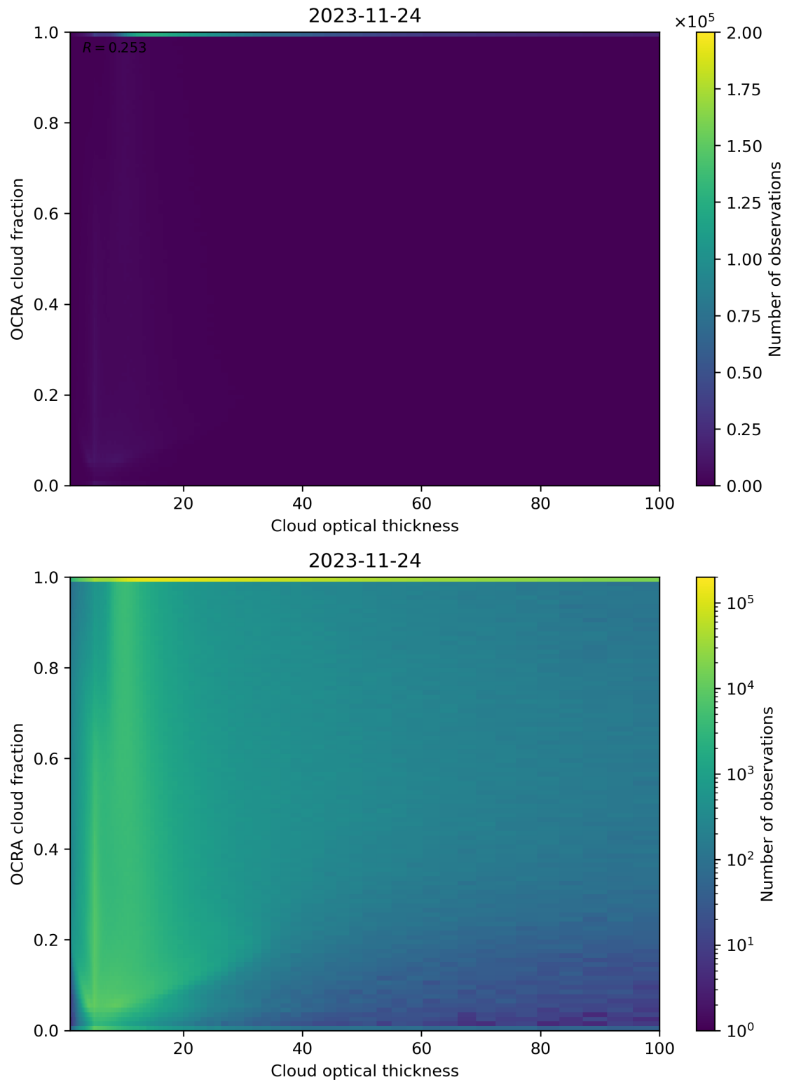
Figure 83: Scatter density plot of “Cloud optical thickness” against “OCRA cloud fraction” for 2023-11-23 to 2023-11-25.
