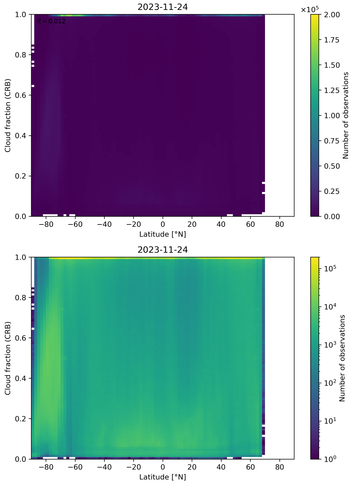
Figure 94: Scatter density plot of “Latitude” against “Cloud fraction (CRB)” for 2023-11-23 to 2023-11-25.
