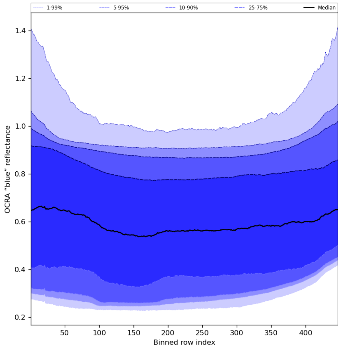
Figure 67: Along track statistics of "OCRA "blue" reflectance" for 2023-11-23 to 2023-11-25
