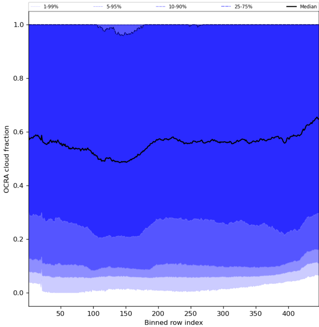
Figure 66: Along track statistics of “OCRA cloud fraction” for 2023-11-23 to 2023-11-25
