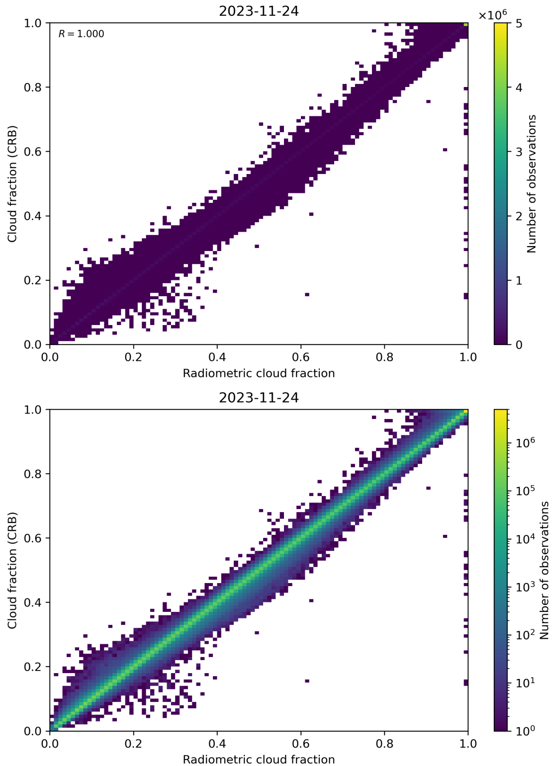
Figure 73: Scatter density plot of “Radiometric cloud fraction” against “Cloud fraction (CRB)” for 2023-11-23 to 2023-11-25.
