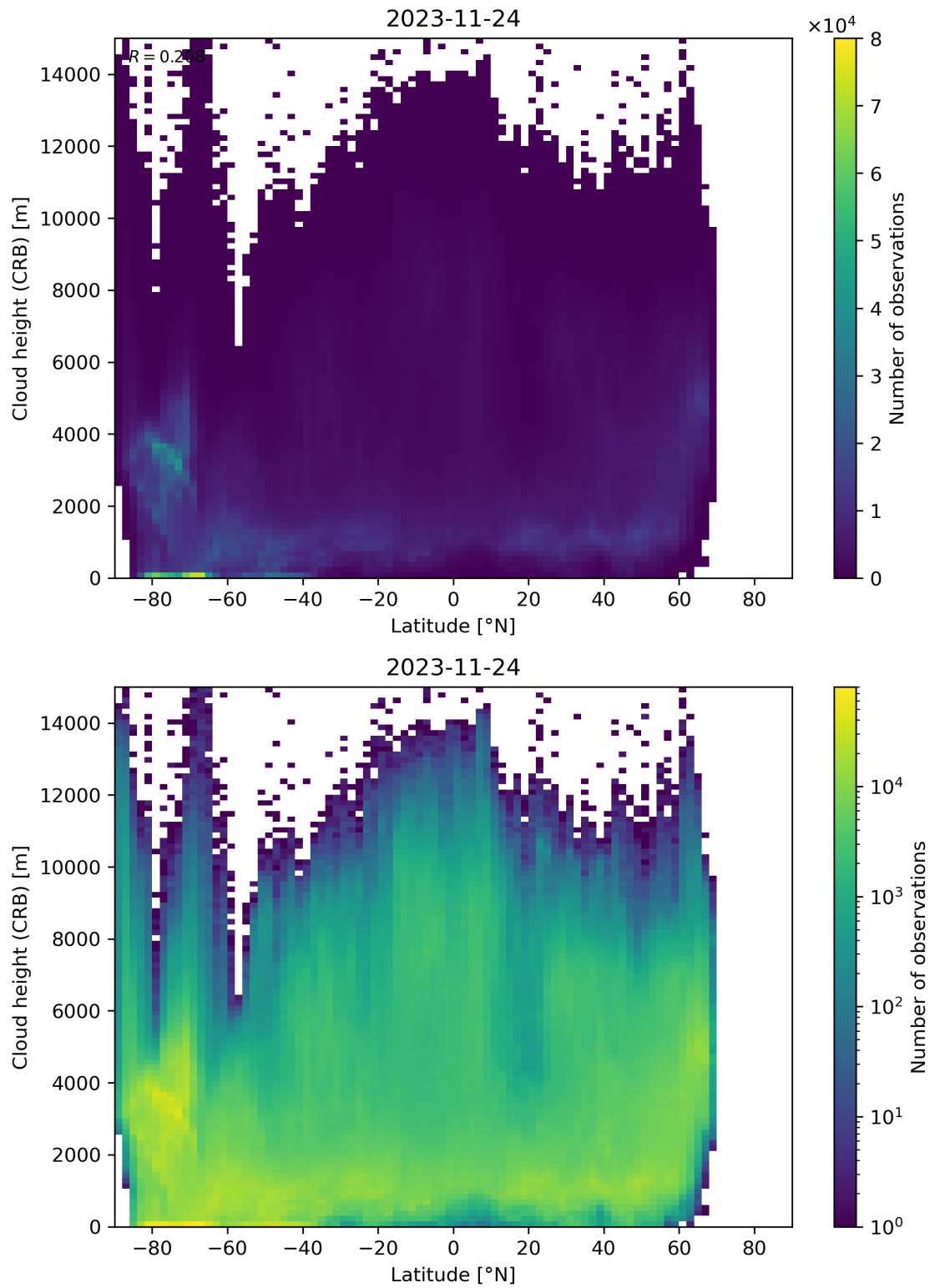
Figure 95: Scatter density plot of “Latitude” against “Cloud height (CRB)” for 2023-11-23 to 2023-11-25.
