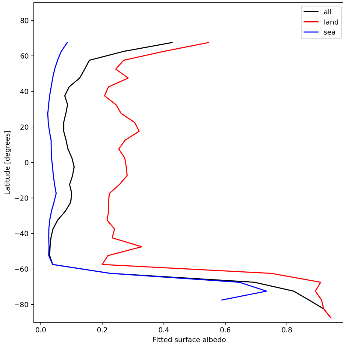
Figure 29: Zonal average of “Fitted surface albedo” for 2023-11-23 to 2023-11-25.
