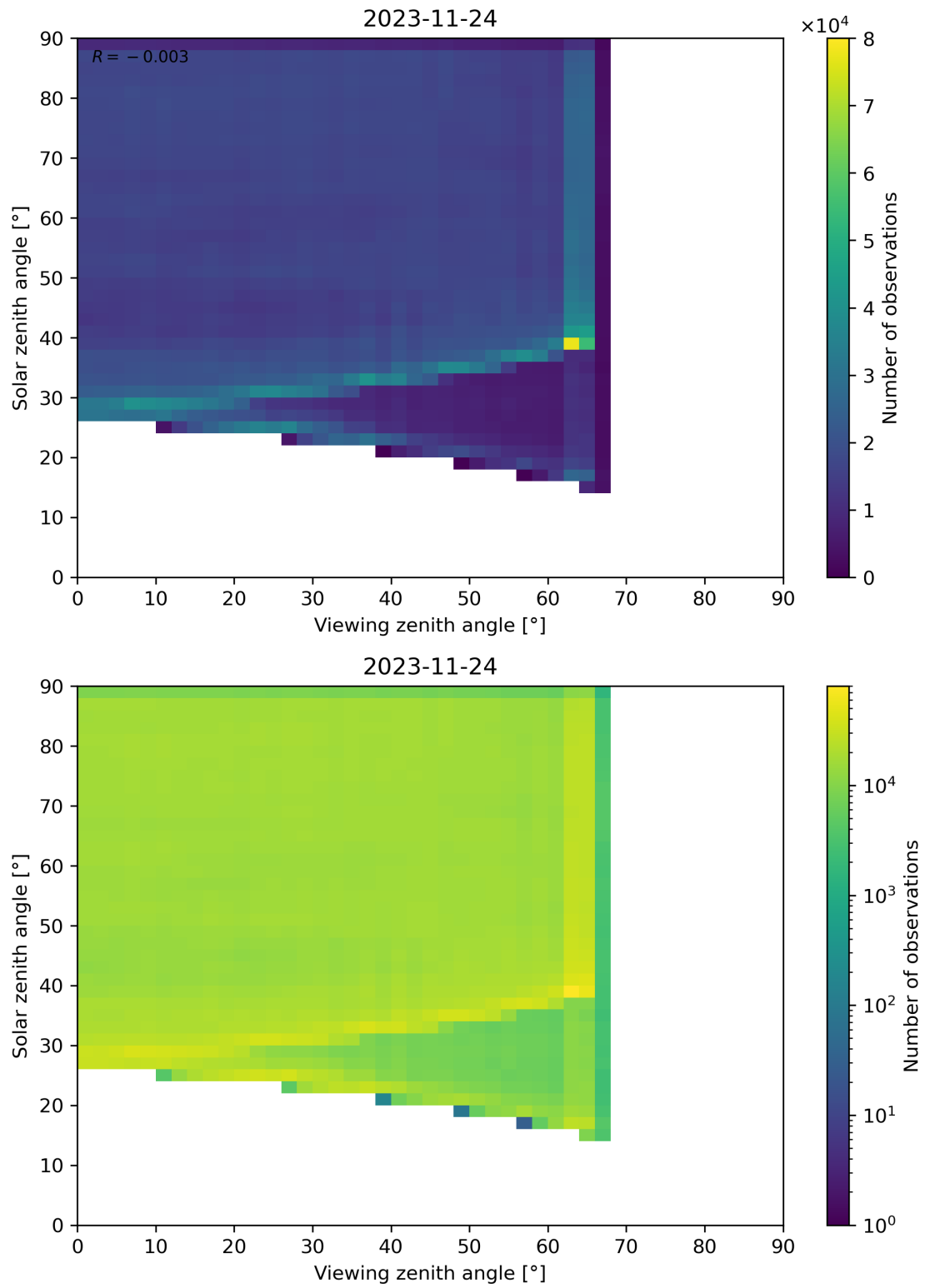
Figure 114: Scatter density plot of “Viewing zenith angle” against “Solar zenith angle” for 2023-11-23 to 2023-11-25.
