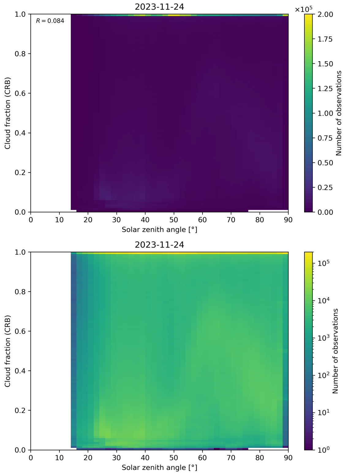
Figure 101: Scatter density plot of “Solar zenith angle” against “Cloud fraction (CRB)” for 2023-11-23 to 2023-11-25.
