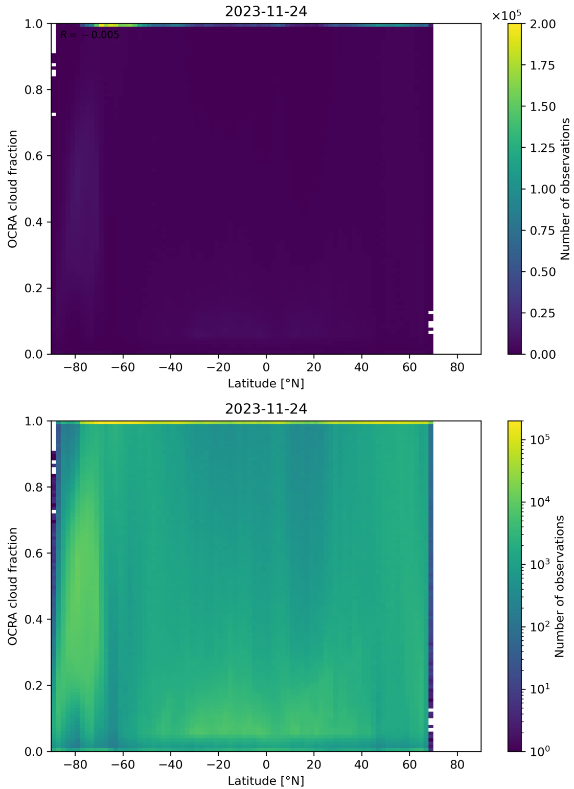
Figure 93: Scatter density plot of “Latitude” against “OCRA cloud fraction” for 2023-11-23 to 2023-11-25.
