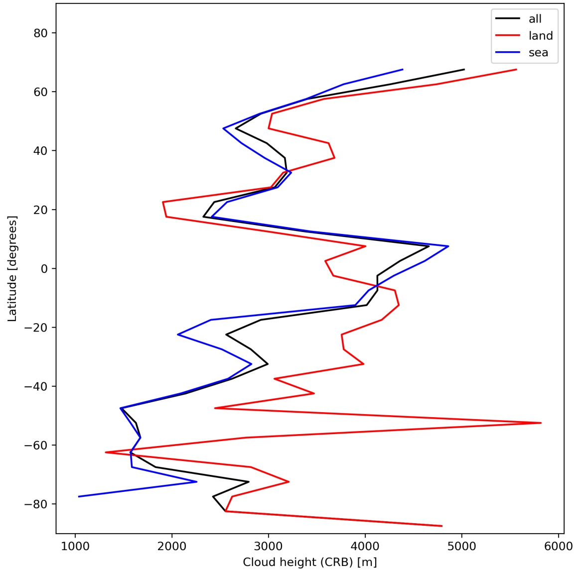
Figure 27: Zonal average of “Cloud height (CRB)” for 2023-11-23 to 2023-11-25.
