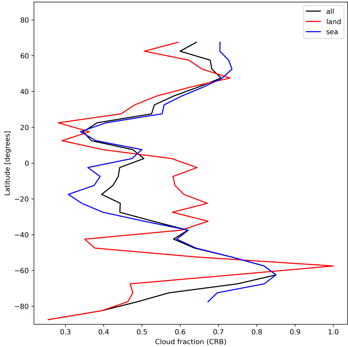
Figure 26: Zonal average of “Cloud fraction (CRB)” for 2023-11-23 to 2023-11-25.
