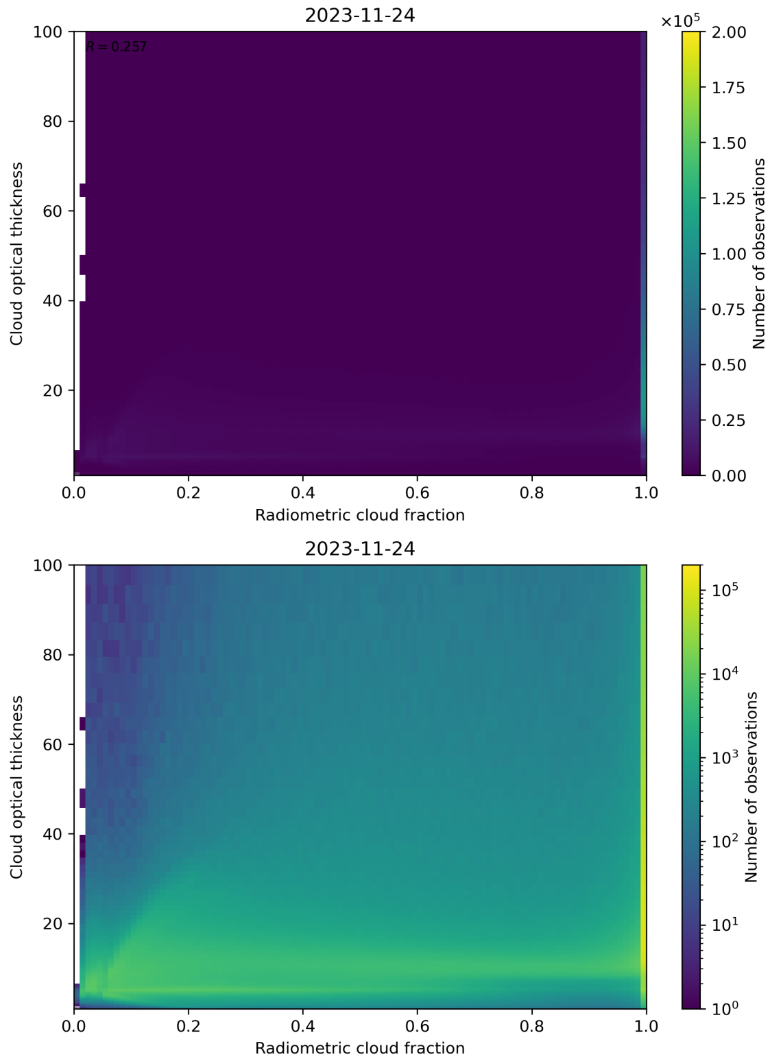
Figure 75: Scatter density plot of “Radiometric cloud fraction” against “Cloud optical thickness” for 2023-11-23 to 2023-11-25.
