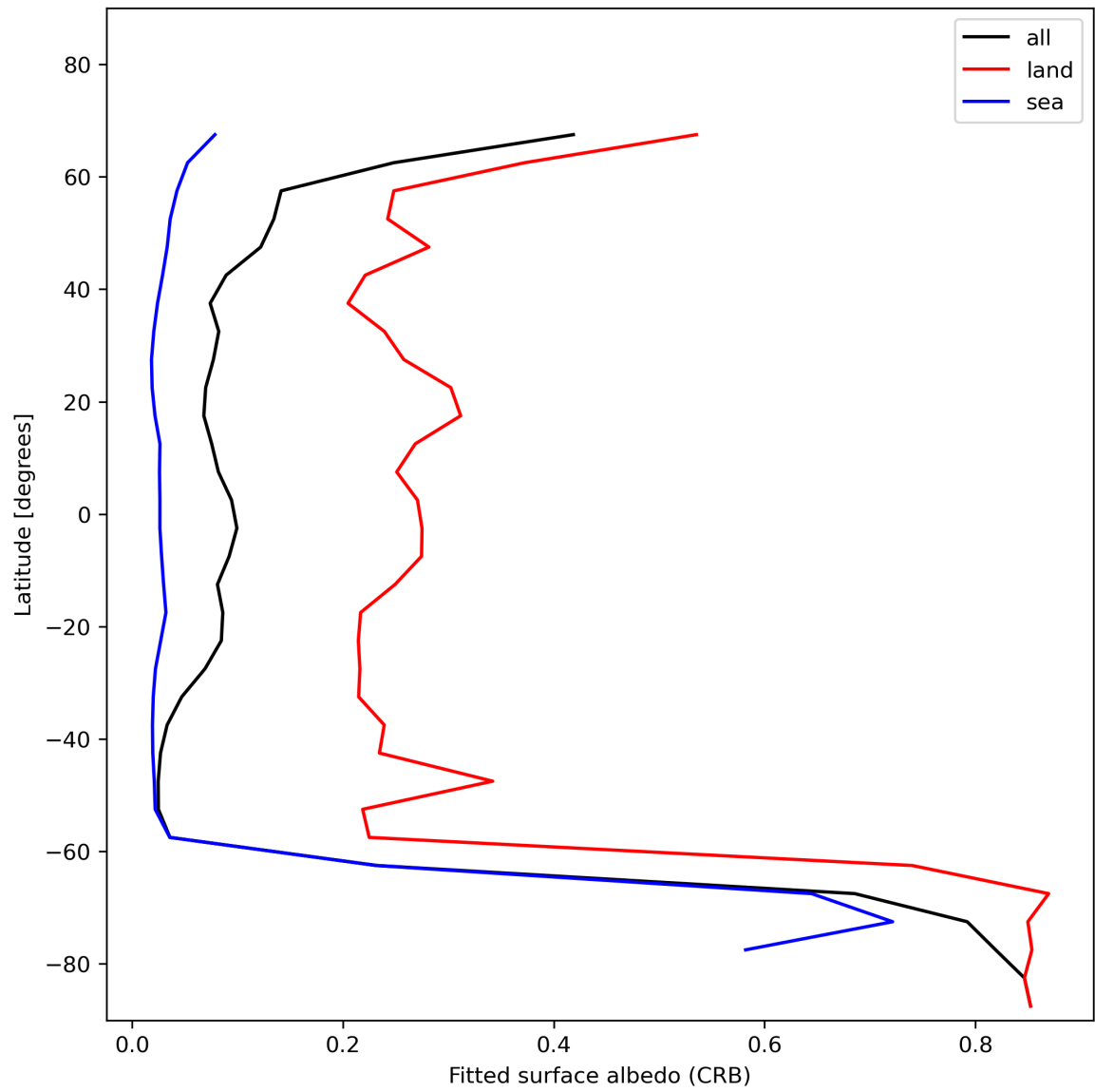
Figure 30: Zonal average of “Fitted surface albedo (CRB)” for 2023-11-23 to 2023-11-25.
