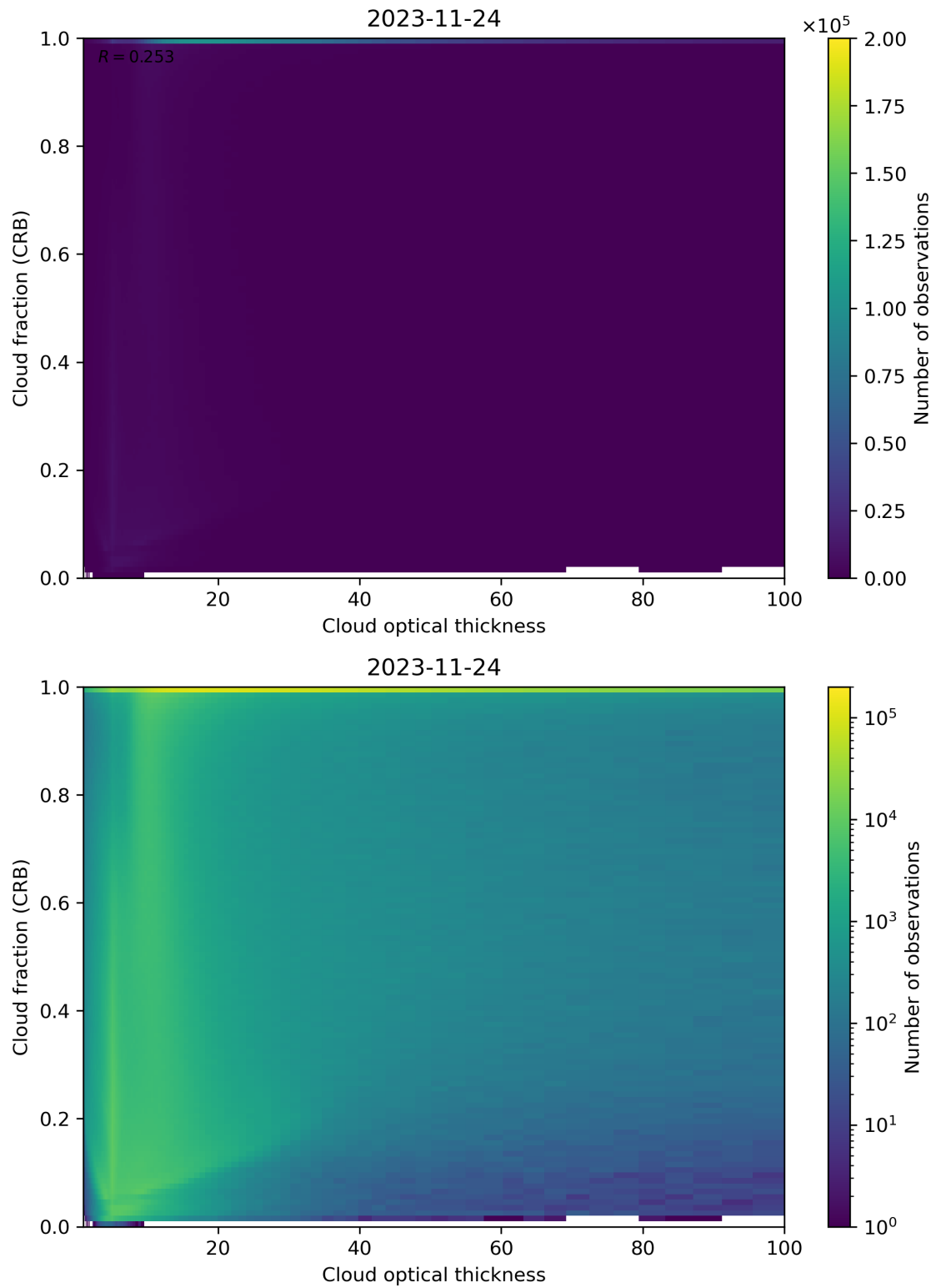
Figure 84: Scatter density plot of “Cloud optical thickness” against “Cloud fraction (CRB)” for 2023-11-23 to 2023-11-25.
