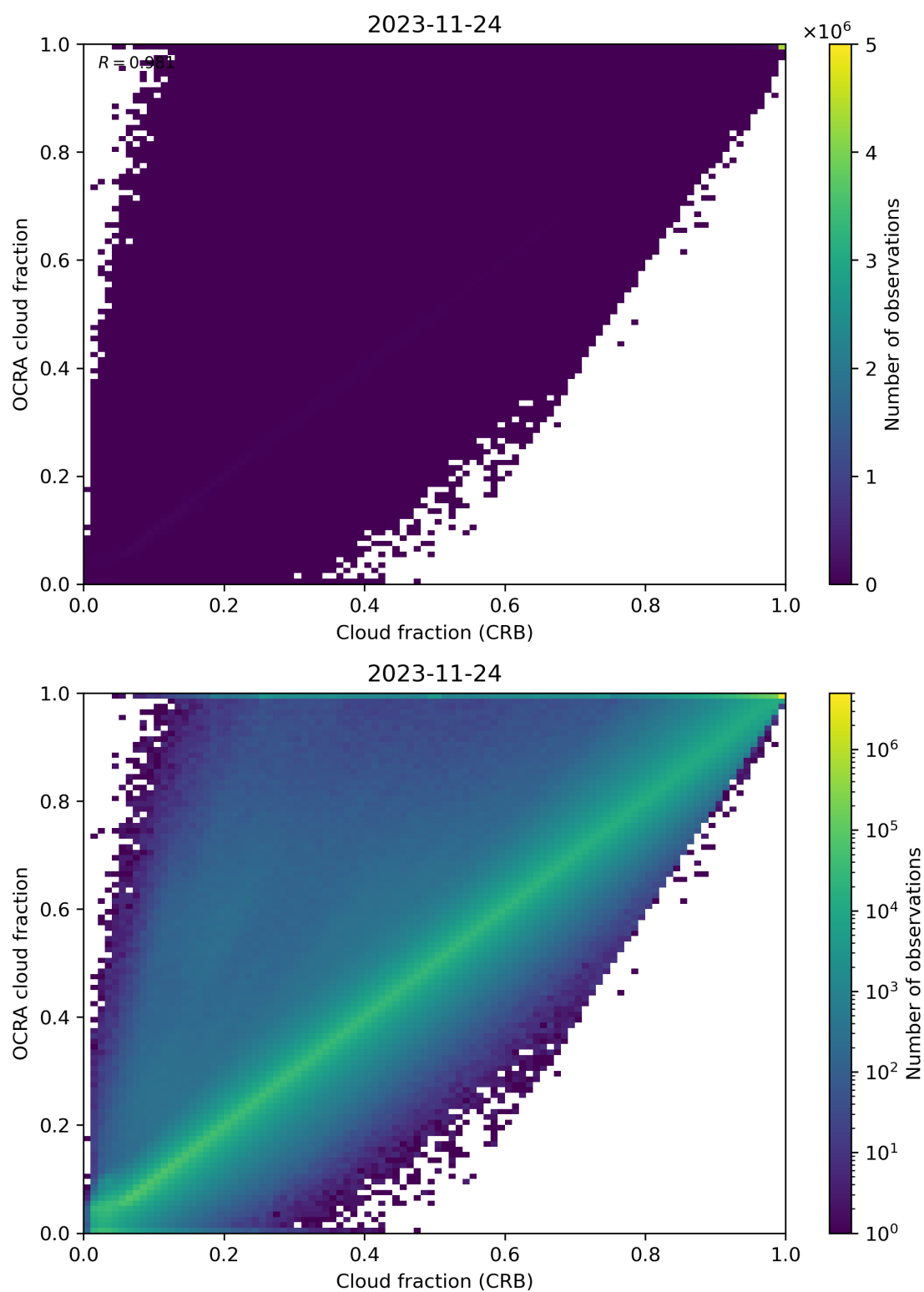
Figure 78: Scatter density plot of “Cloud fraction (CRB)” against “OCRA cloud fraction” for 2023-11-23 to 2023-11-25.
