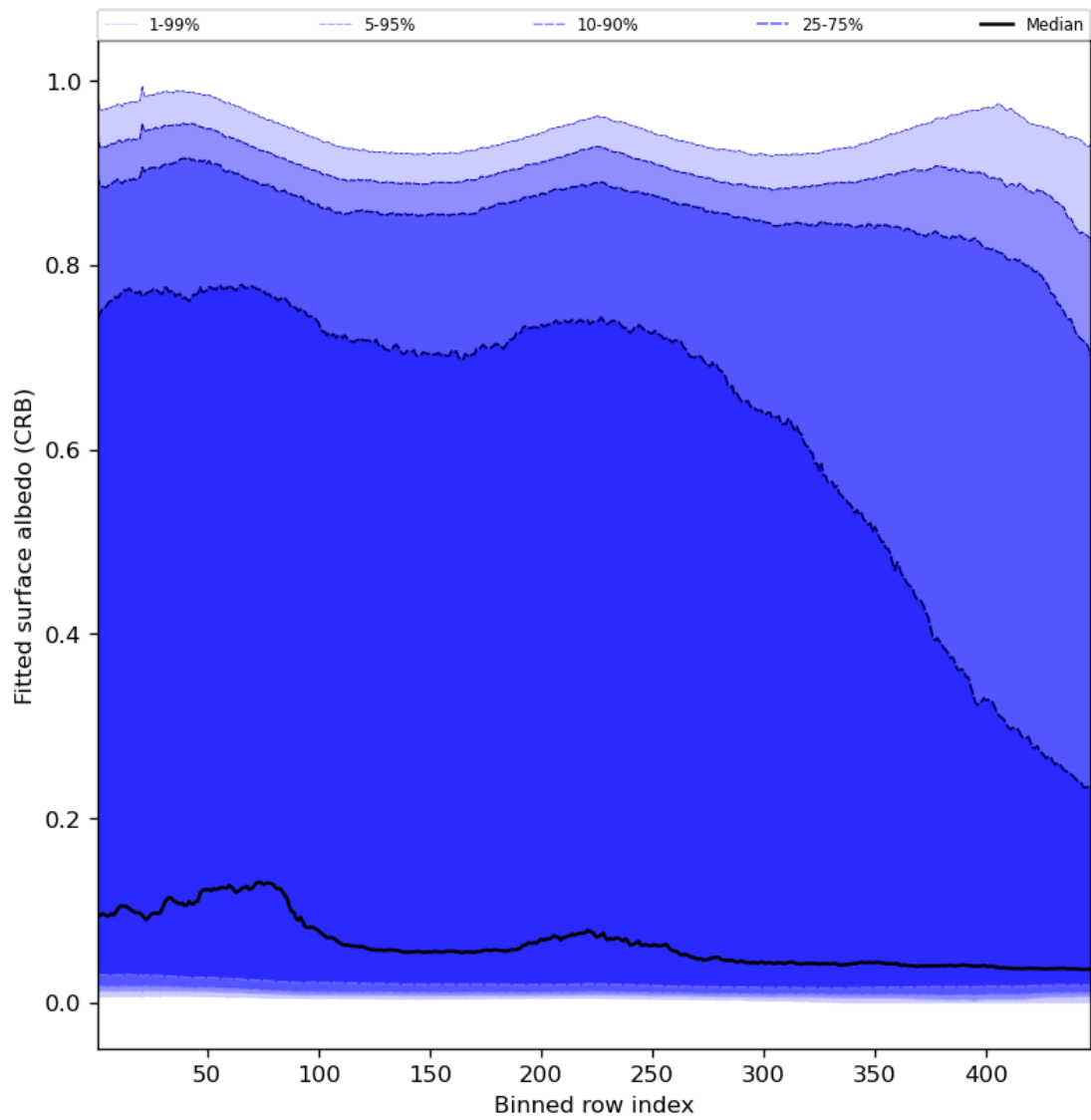
Figure 62: Along track statistics of “Fitted surface albedo (CRB)” for 2023-11-23 to 2023-11-25
