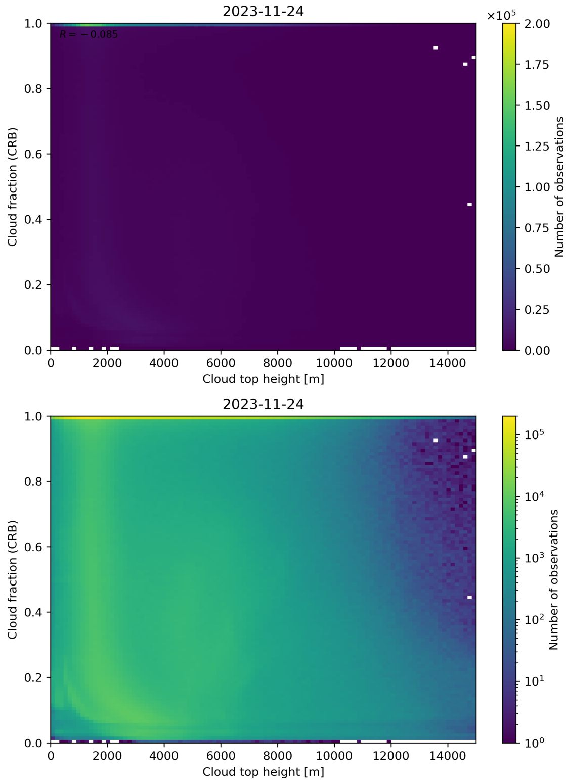
Figure 88: Scatter density plot of “Cloud top height” against “Cloud fraction (CRB)” for 2023-11-23 to 2023-11-25.
