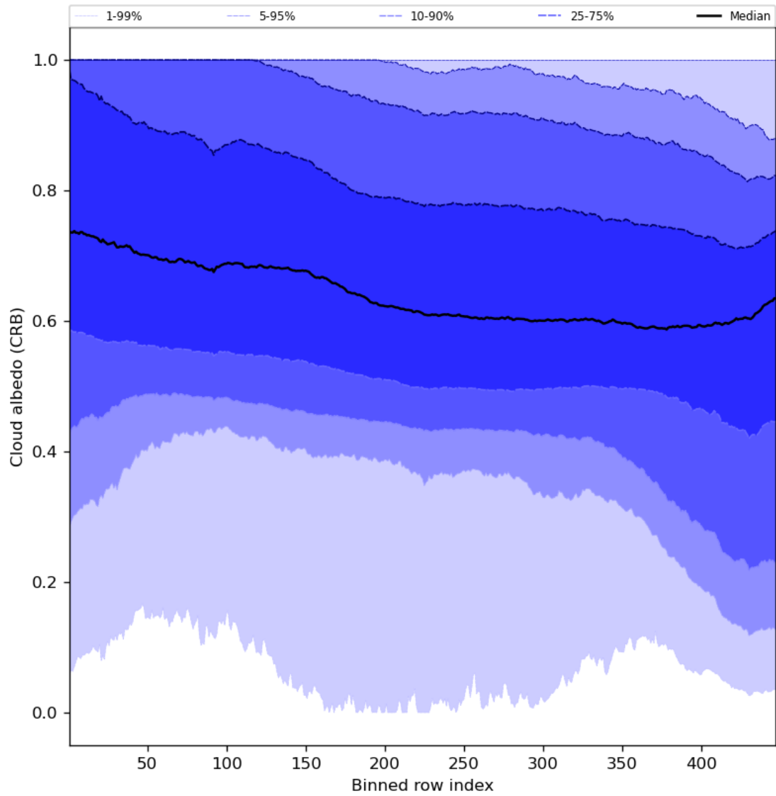
Figure 60: Along track statistics of “Cloud albedo (CRB)” for 2023-11-23 to 2023-11-25
