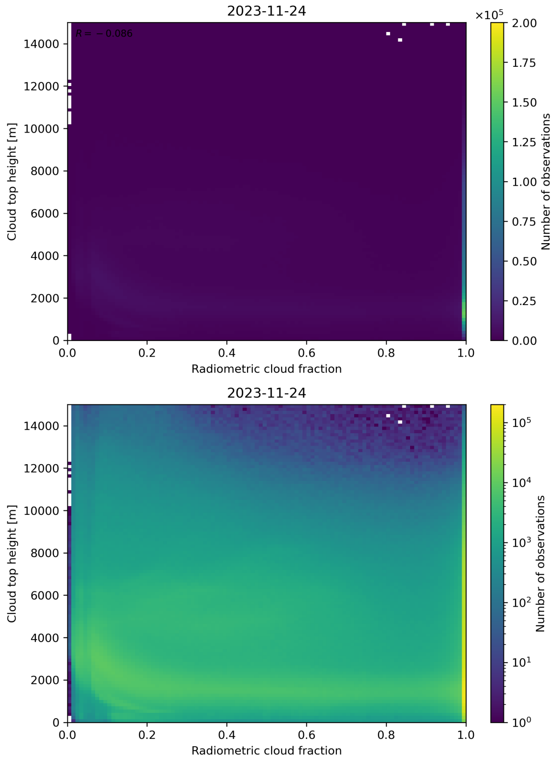
Figure 76: Scatter density plot of “Radiometric cloud fraction” against “Cloud top height” for 2023-11-23 to 2023-11-25.
