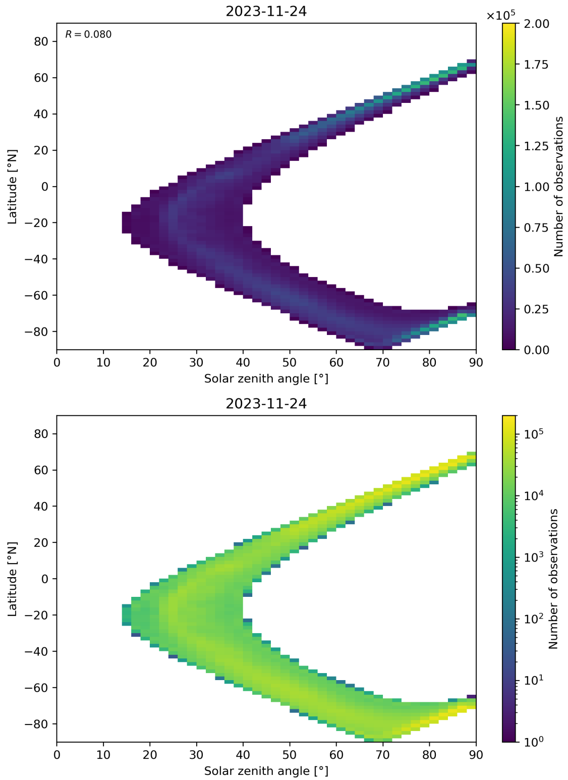
Figure 105: Scatter density plot of “Solar zenith angle” against “Latitude” for 2023-11-23 to 2023-11-25.
