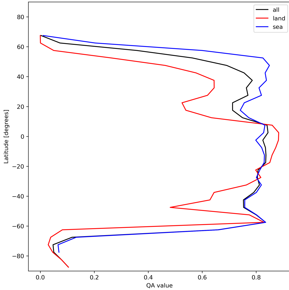
Figure 22: Zonal average of “QA value” for 2023-11-23 to 2023-11-25.
