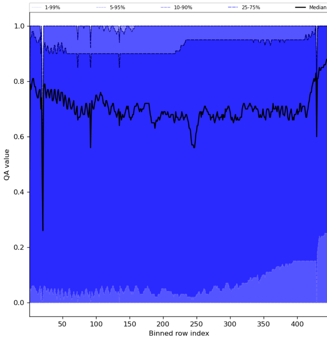
Figure 54: Along track statistics of “QA value” for 2023-11-23 to 2023-11-25
