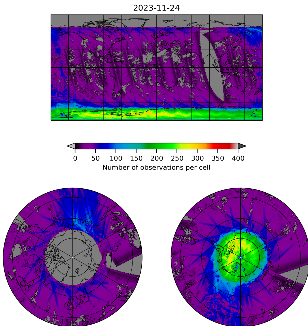
Figure 21: Map of the number of observations for 2023-11-23 to 2023-11-25
