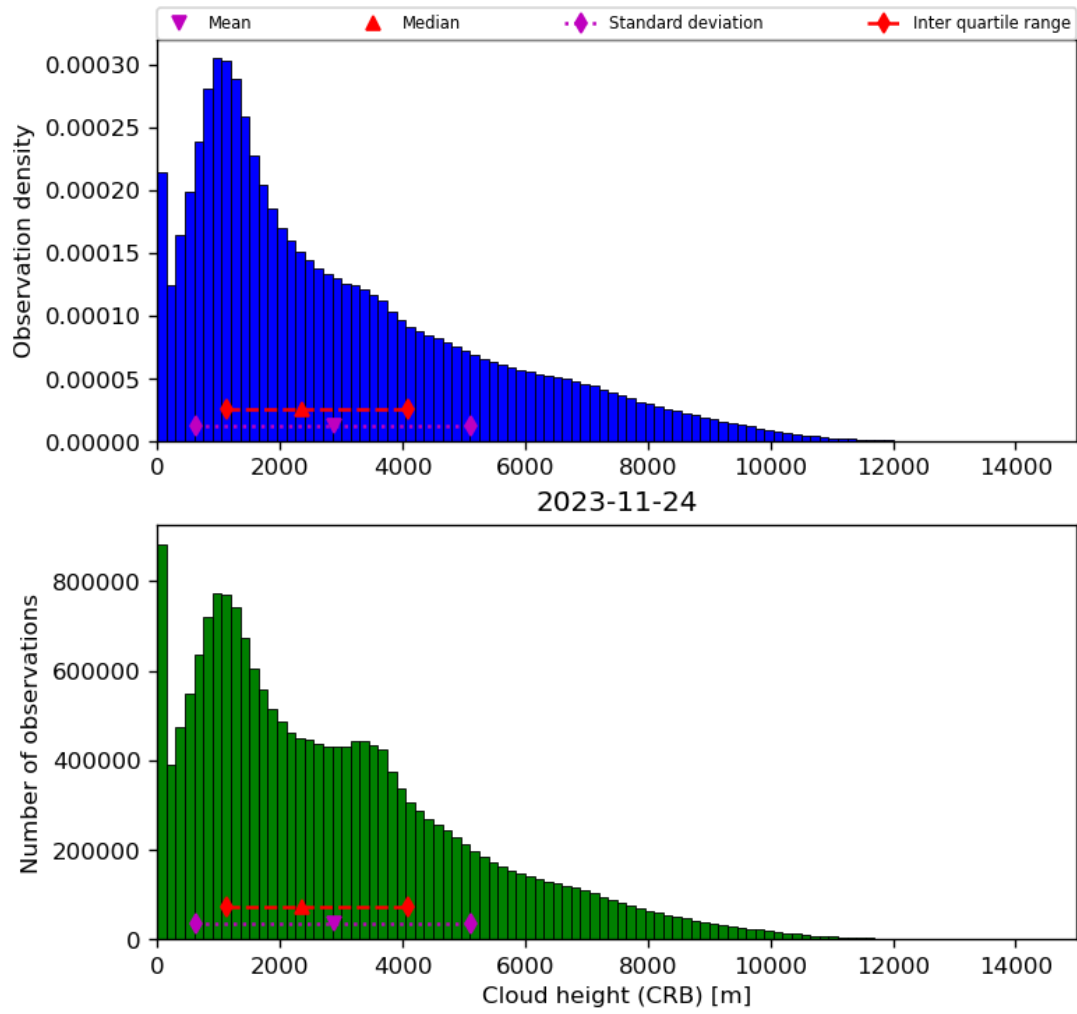
Figure 43: Histogram of “Cloud height (CRB)” for 2023-11-23 to 2023-11-25
