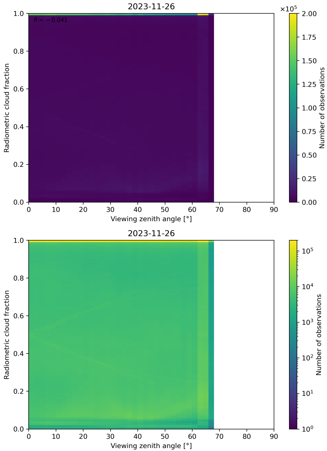
Figure 107: Scatter density plot of “Viewing zenith angle” against “Radiometric cloud fraction” for 2023-11-25 to 2023-11-27.
