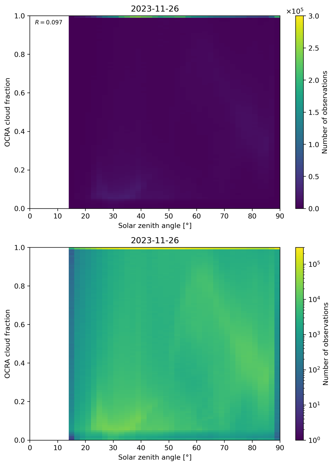
Figure 100: Scatter density plot of “Solar zenith angle” against “OCRA cloud fraction” for 2023-11-25 to 2023-11-27.
