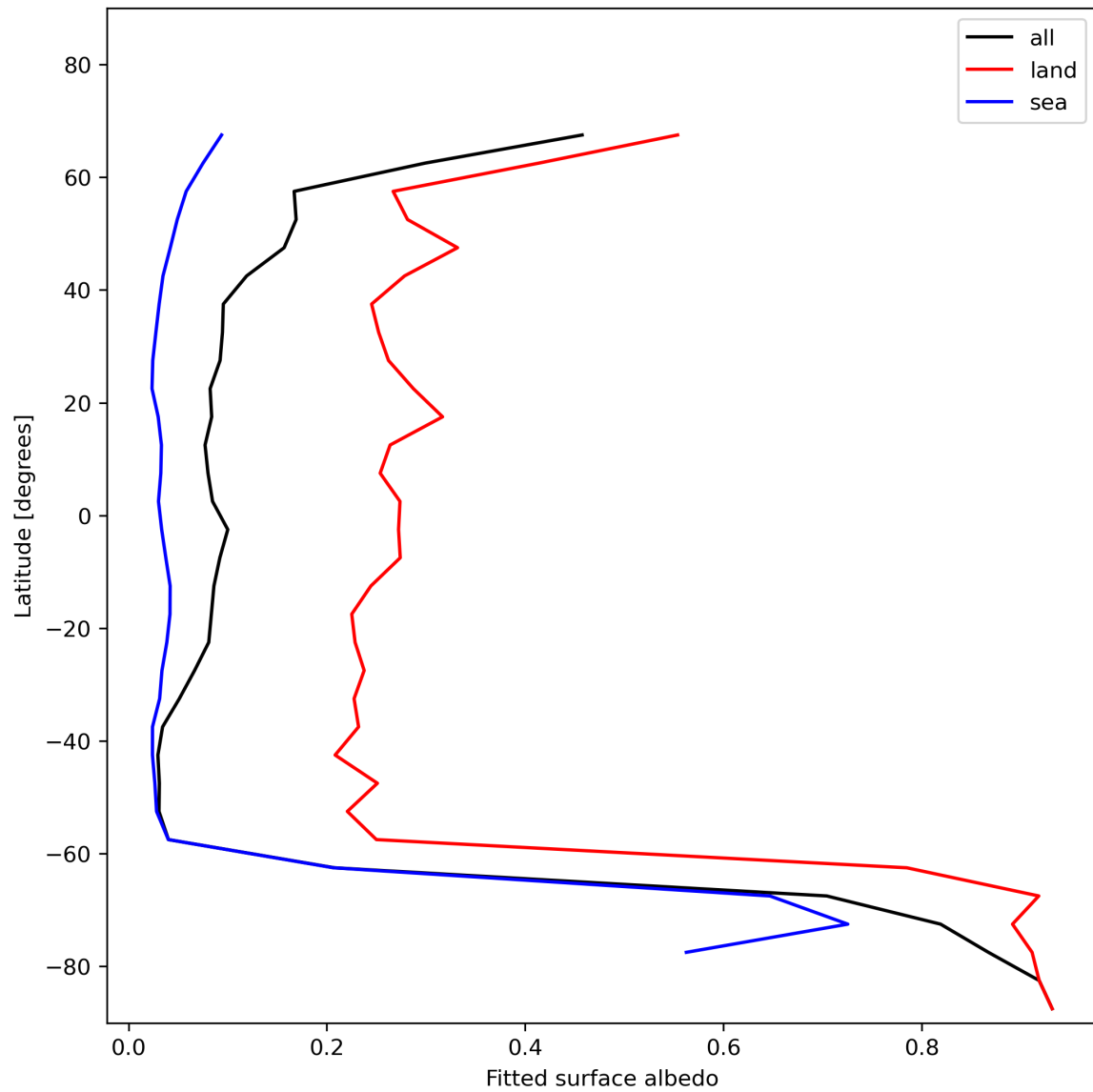
Figure 29: Zonal average of “Fitted surface albedo” for 2023-11-25 to 2023-11-27.
