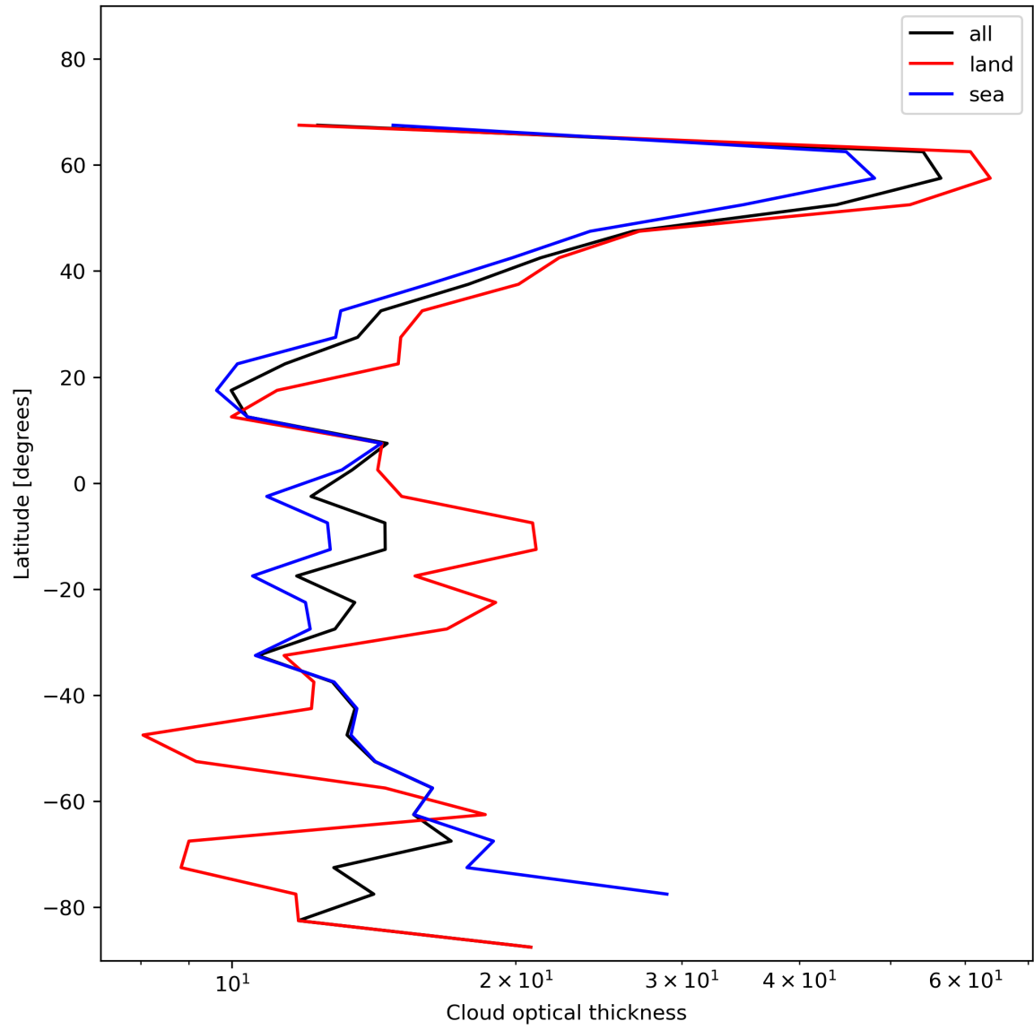
Figure 25: Zonal average of “Cloud optical thickness” for 2023-11-25 to 2023-11-27.
