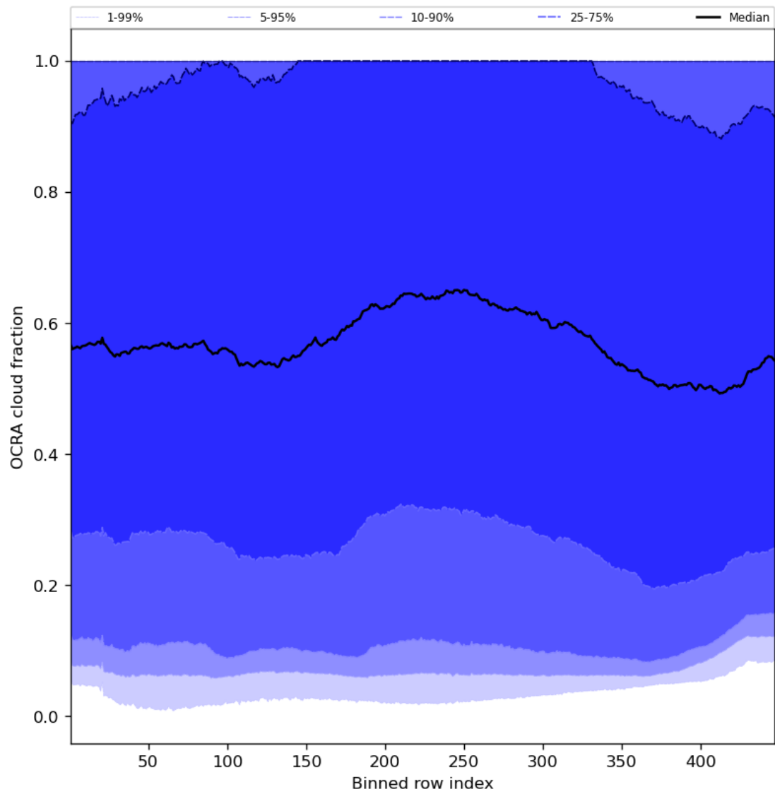
Figure 66: Along track statistics of “OCRA cloud fraction” for 2023-11-25 to 2023-11-27
