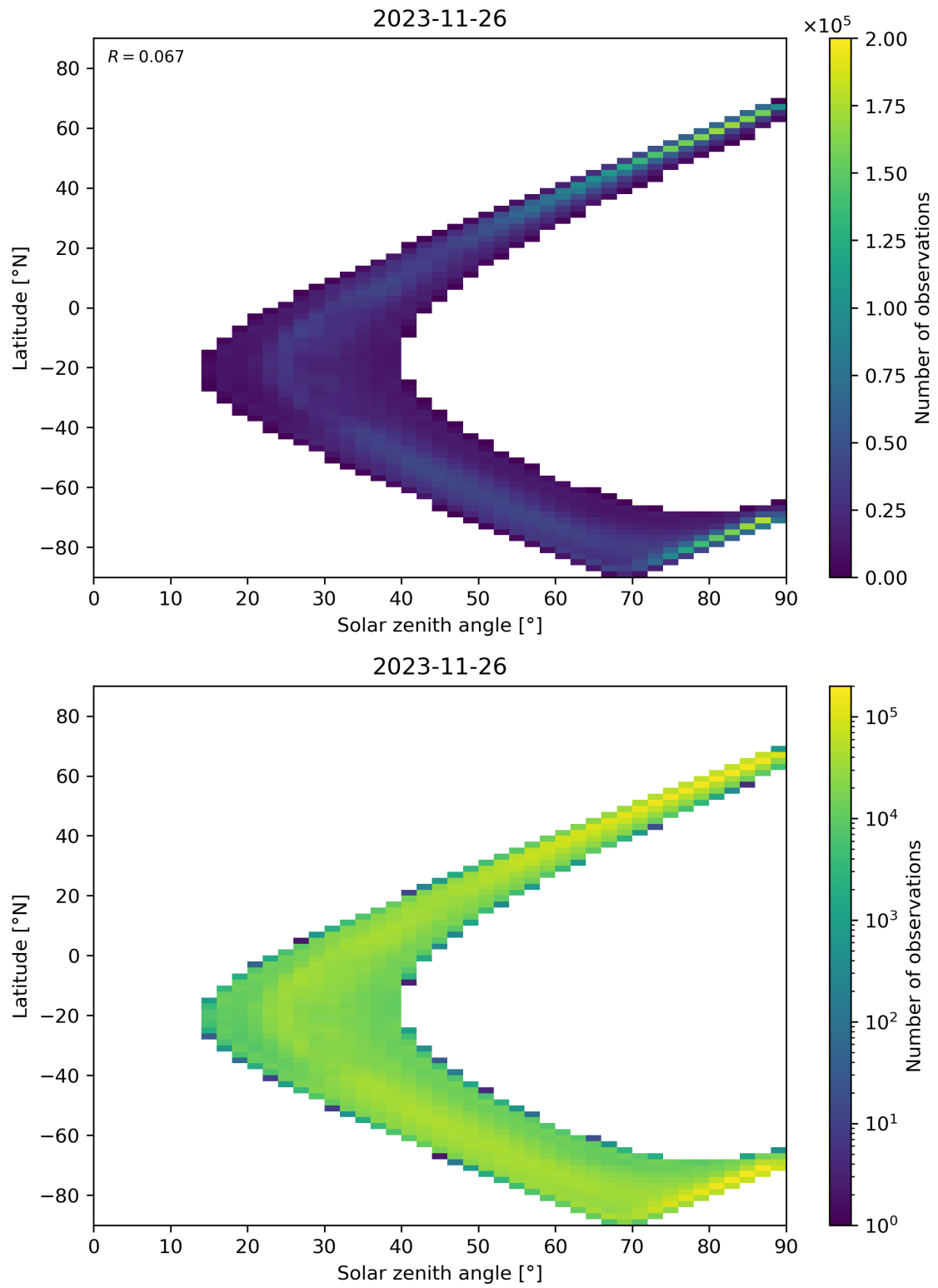
Figure 105: Scatter density plot of “Solar zenith angle” against “Latitude” for 2023-11-25 to 2023-11-27.
