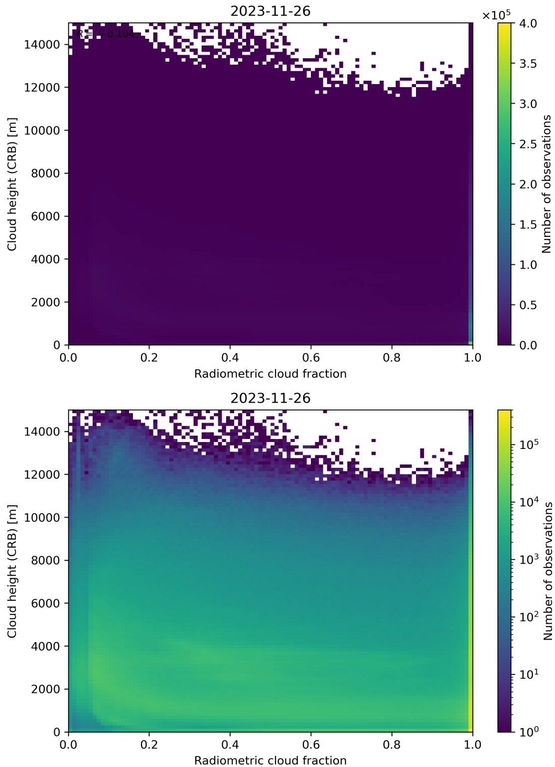
Figure 74: Scatter density plot of “Radiometric cloud fraction” against “Cloud height (CRB)” for 2023-11-25 to 2023-11-27.
