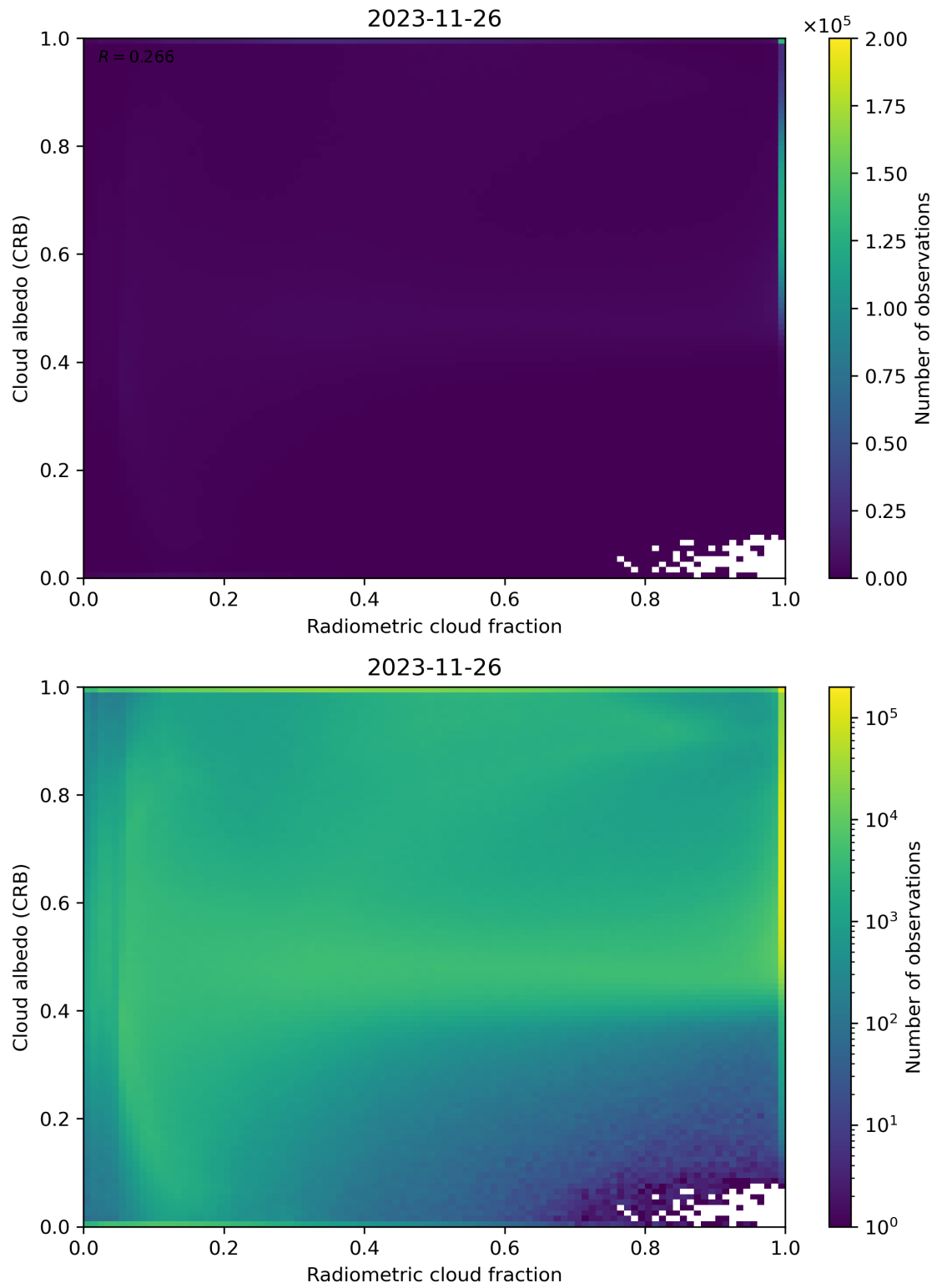
Figure 71: Scatter density plot of “Radiometric cloud fraction” against “Cloud albedo (CRB)” for 2023-11-25 to 2023-11-27.
