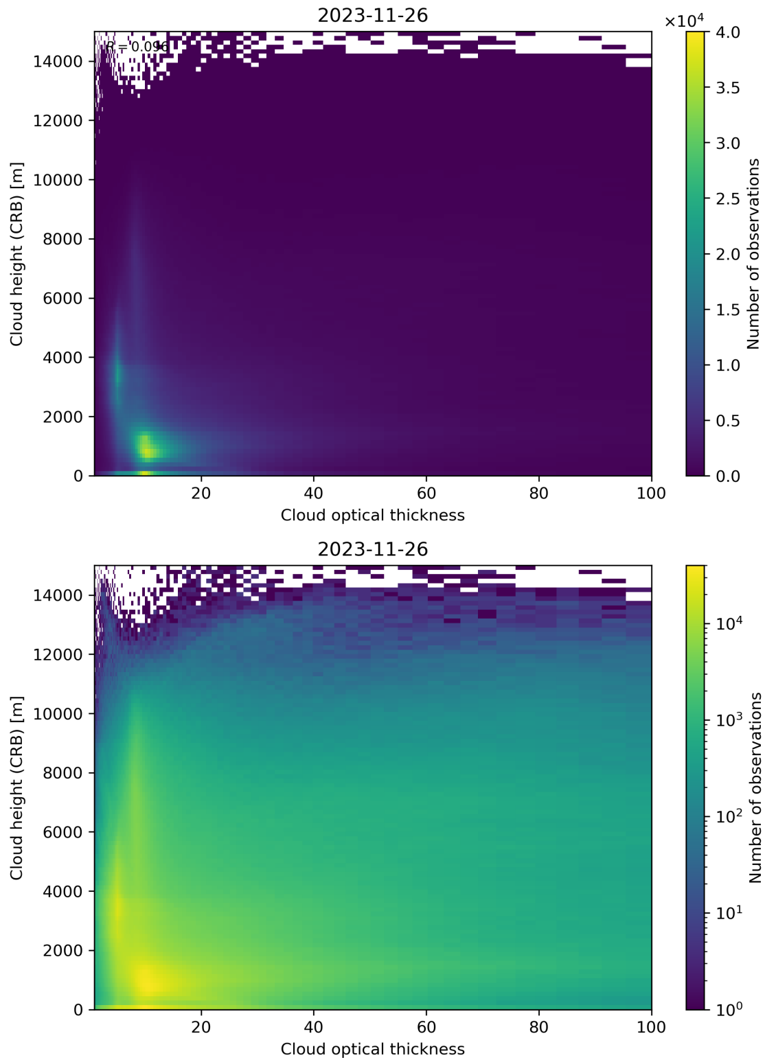
Figure 85: Scatter density plot of “Cloud optical thickness” against “Cloud height (CRB)” for 2023-11-25 to 2023-11-27.
