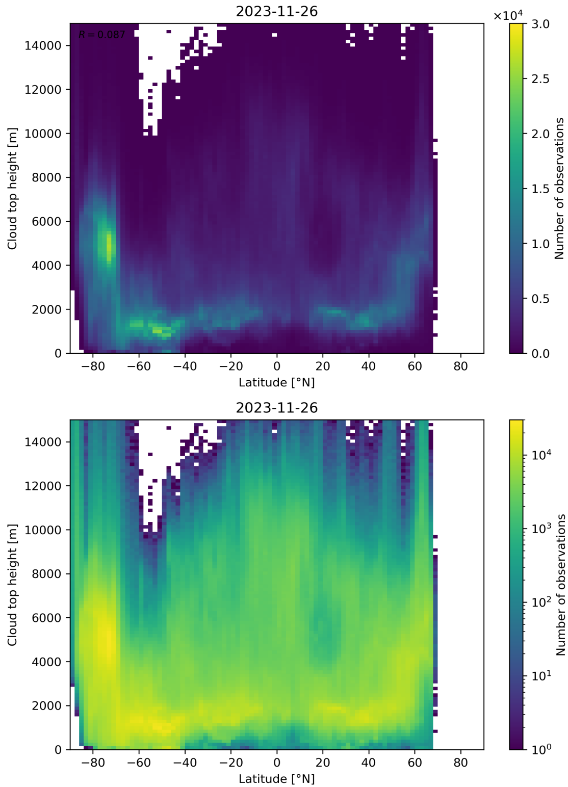
Figure 97: Scatter density plot of “Latitude” against “Cloud top height” for 2023-11-25 to 2023-11-27.
