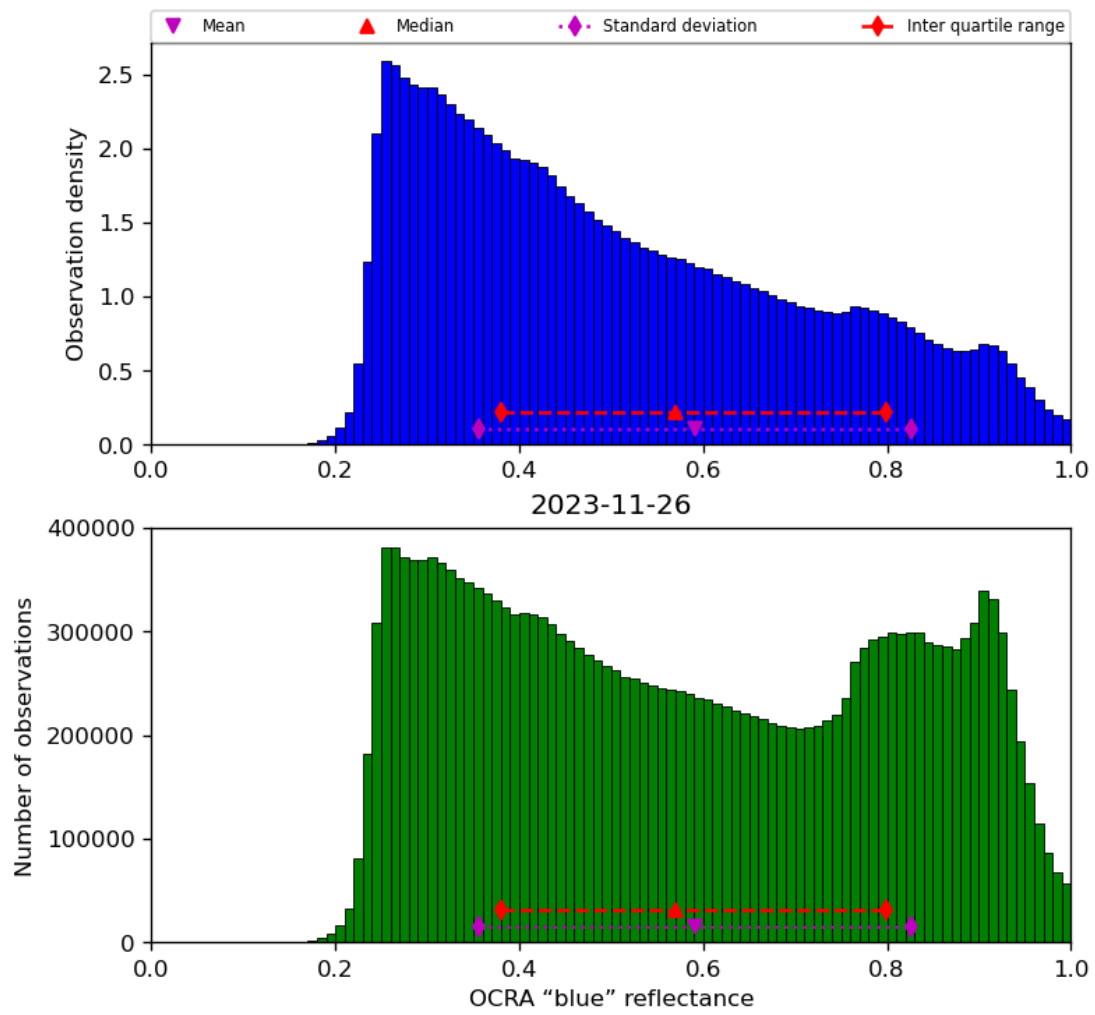
Figure 51: Histogram of “OCRA “blue” reflectance” for 2023-11-25 to 2023-11-27
