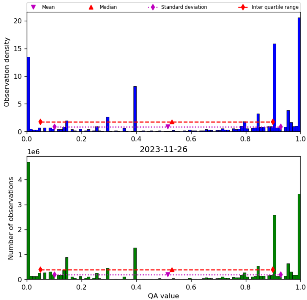
Figure 38: Histogram of “QA value” for 2023-11-25 to 2023-11-27
