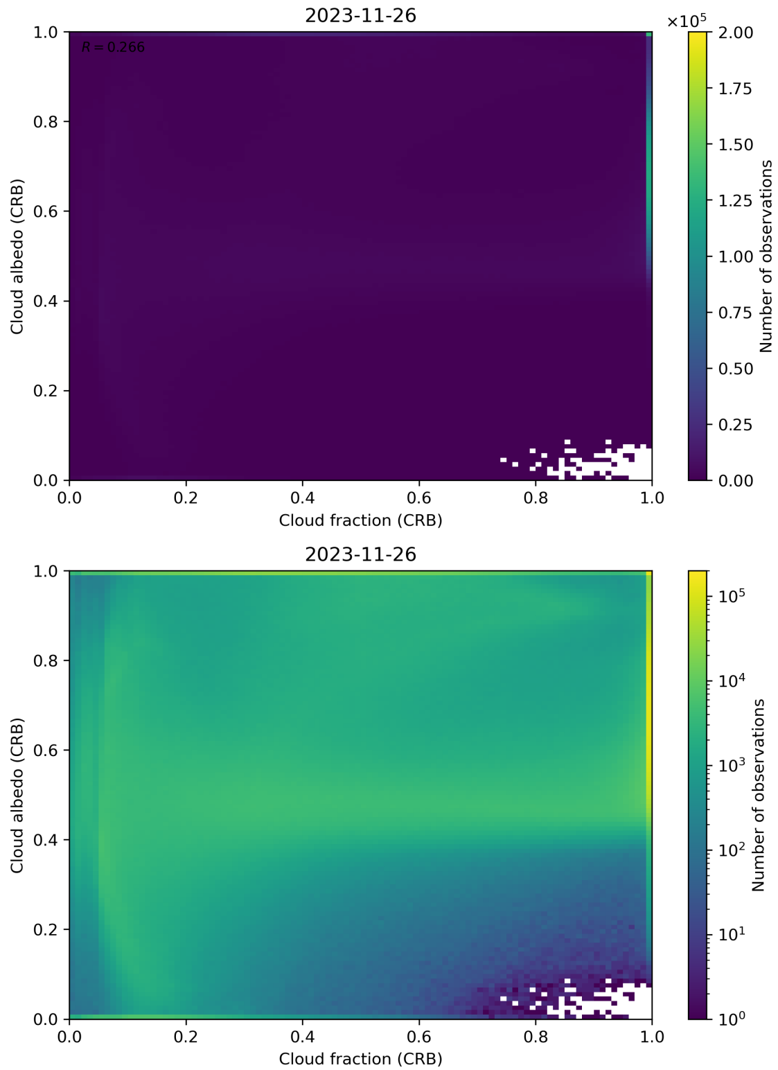
Figure 77: Scatter density plot of “Cloud fraction (CRB)” against “Cloud albedo (CRB)” for 2023-11-25 to 2023-11-27.
