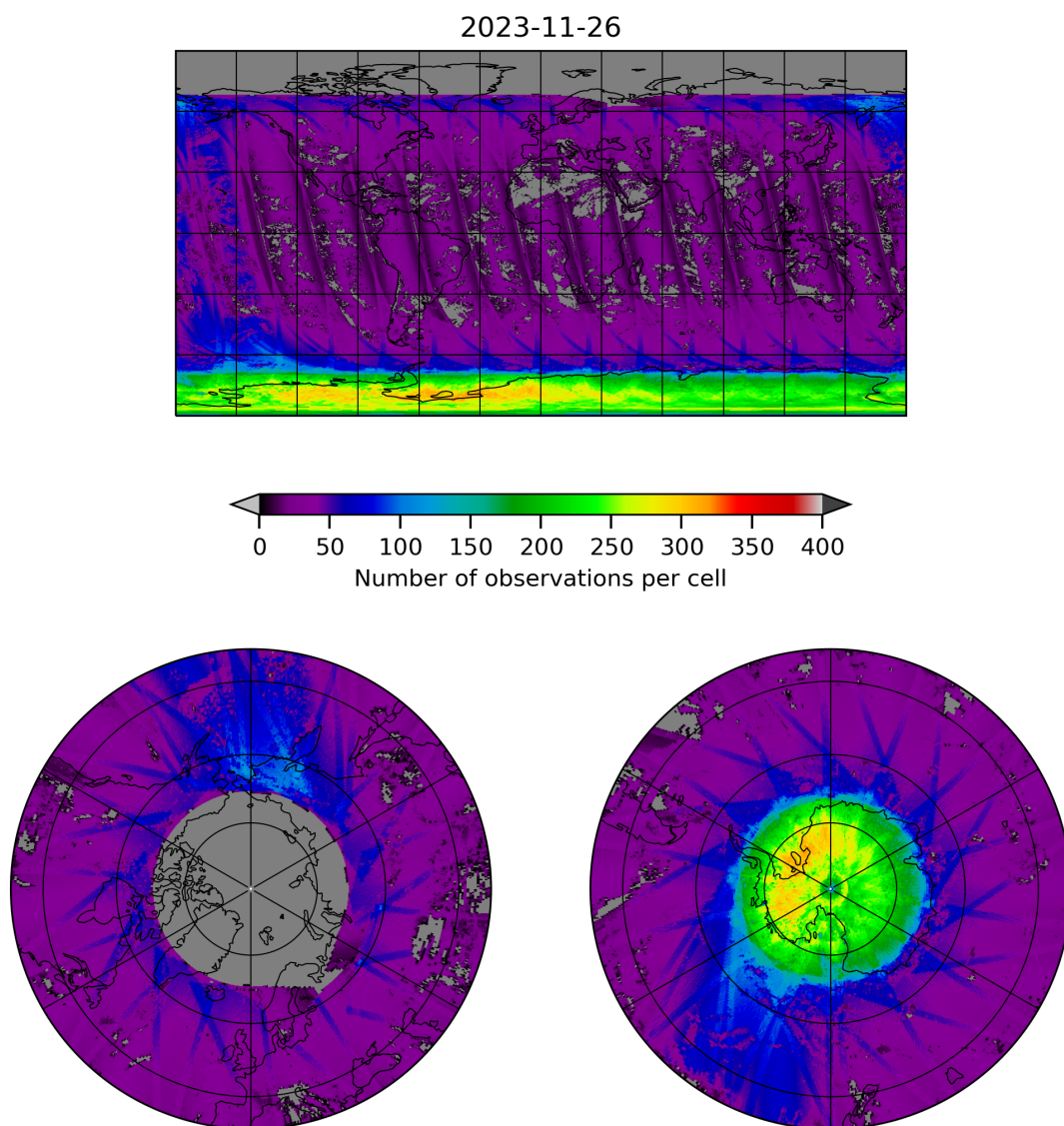
Figure 21: Map of the number of observations for 2023-11-25 to 2023-11-27
