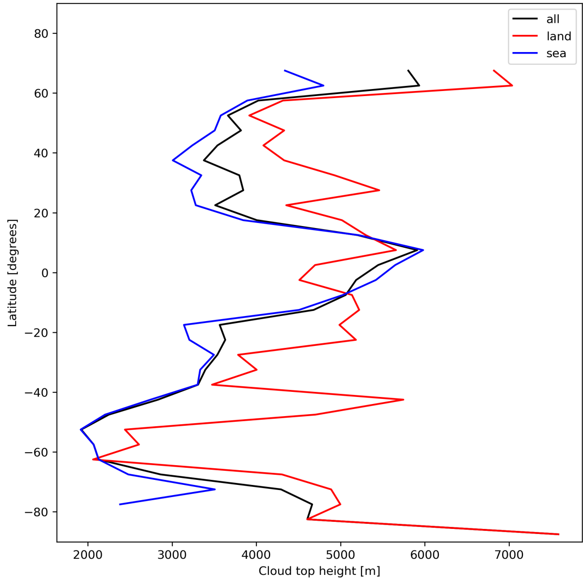
Figure 24: Zonal average of “Cloud top height” for 2023-11-25 to 2023-11-27.
