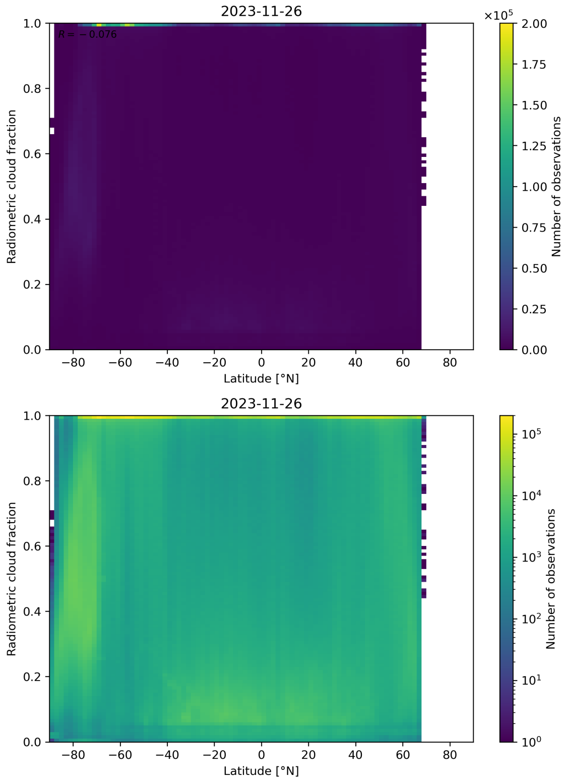
Figure 92: Scatter density plot of “Latitude” against “Radiometric cloud fraction” for 2023-11-25 to 2023-11-27.
