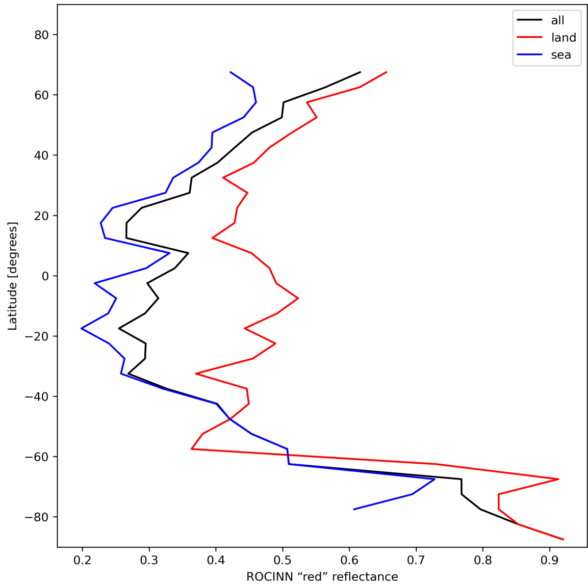
Figure 37: Zonal average of “ROCINN “red” reflectance” for 2023-11-25 to 2023-11-27.
