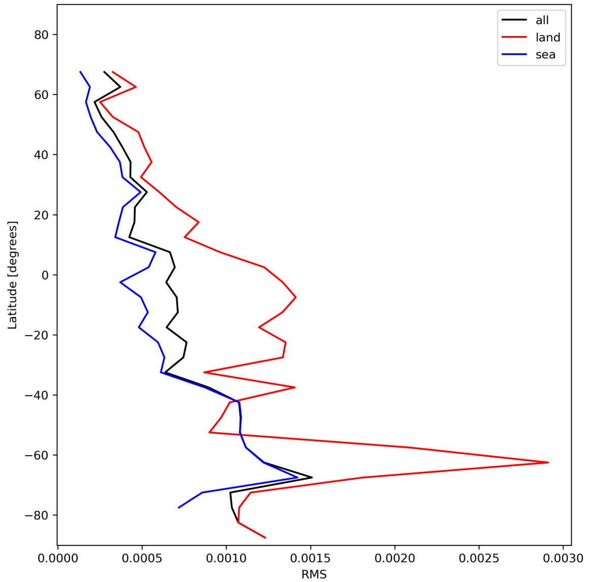
Figure 31: Zonal average of “RMS” for 2023-11-25 to 2023-11-27.
