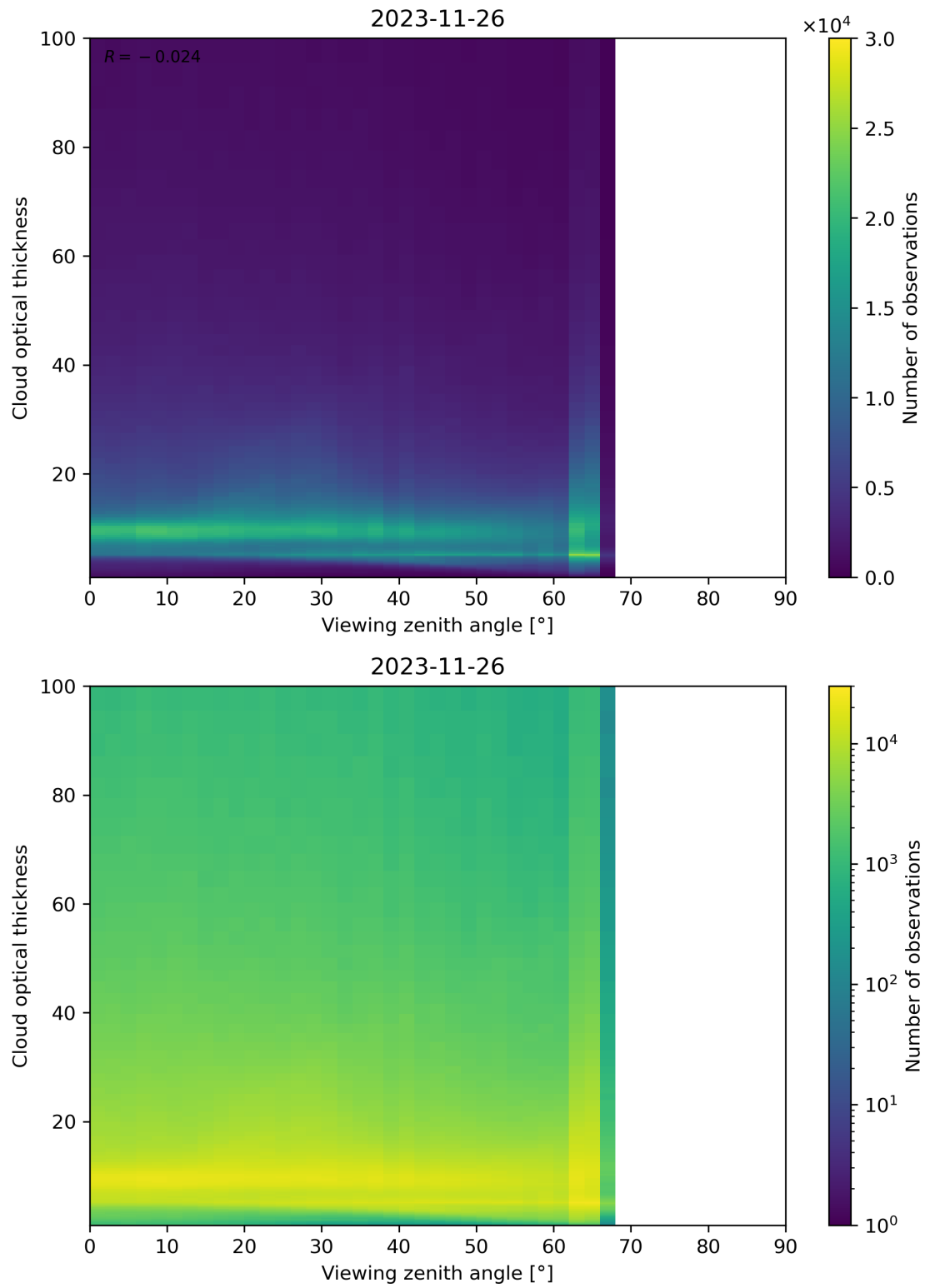
Figure 111: Scatter density plot of “Viewing zenith angle” against “Cloud optical thickness” for 2023-11-25 to 2023-11-27.
