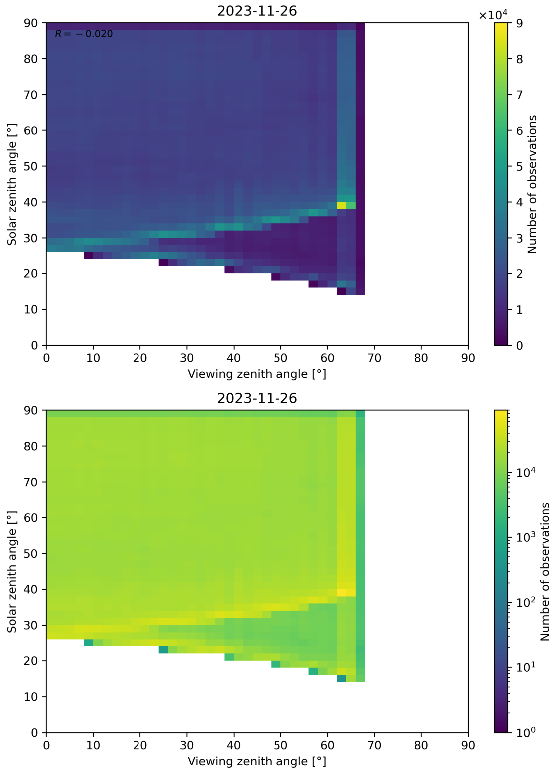
Figure 114: Scatter density plot of “Viewing zenith angle” against “Solar zenith angle” for 2023-11-25 to 2023-11-27.
