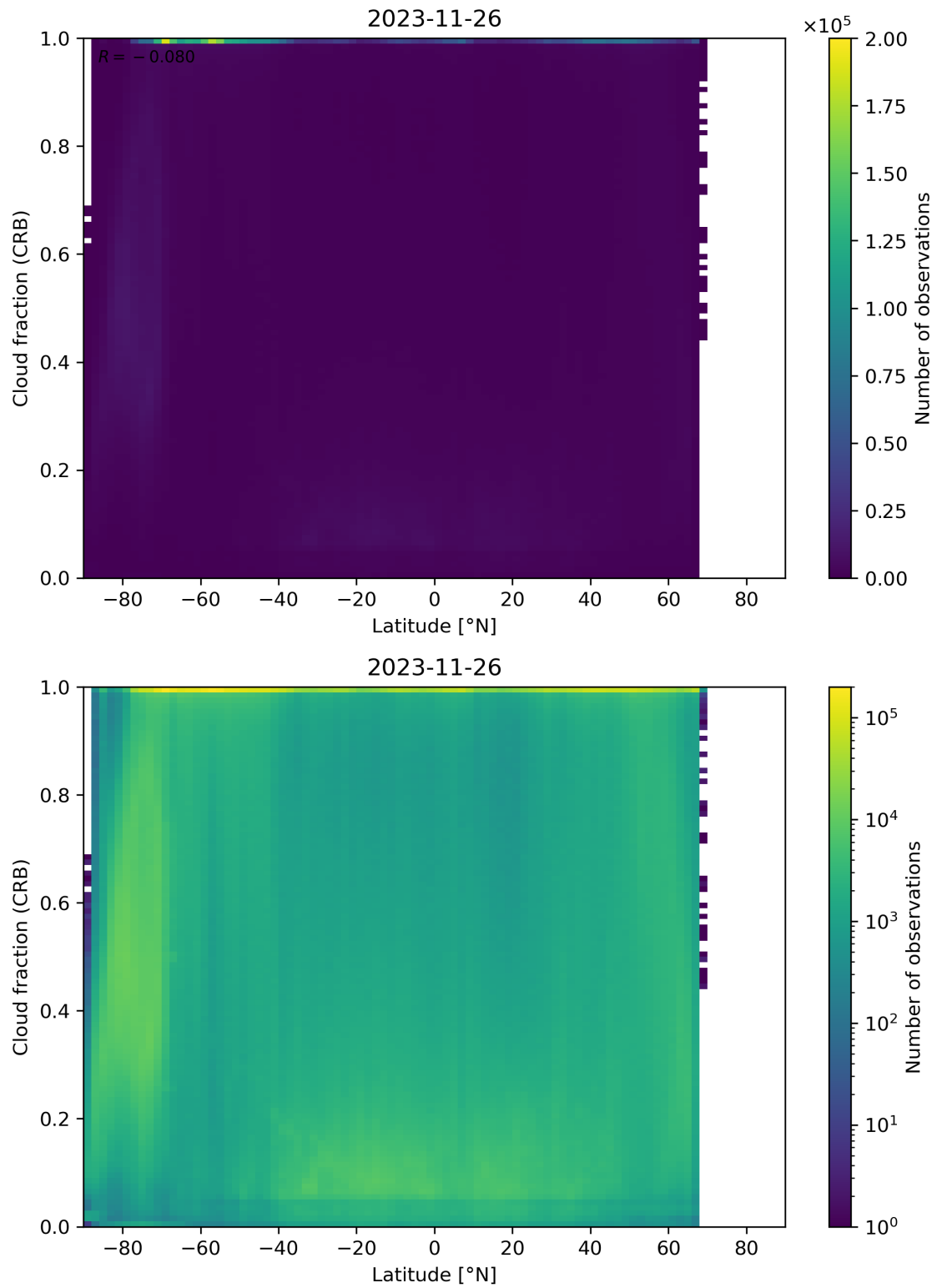
Figure 94: Scatter density plot of “Latitude” against “Cloud fraction (CRB)” for 2023-11-25 to 2023-11-27.
