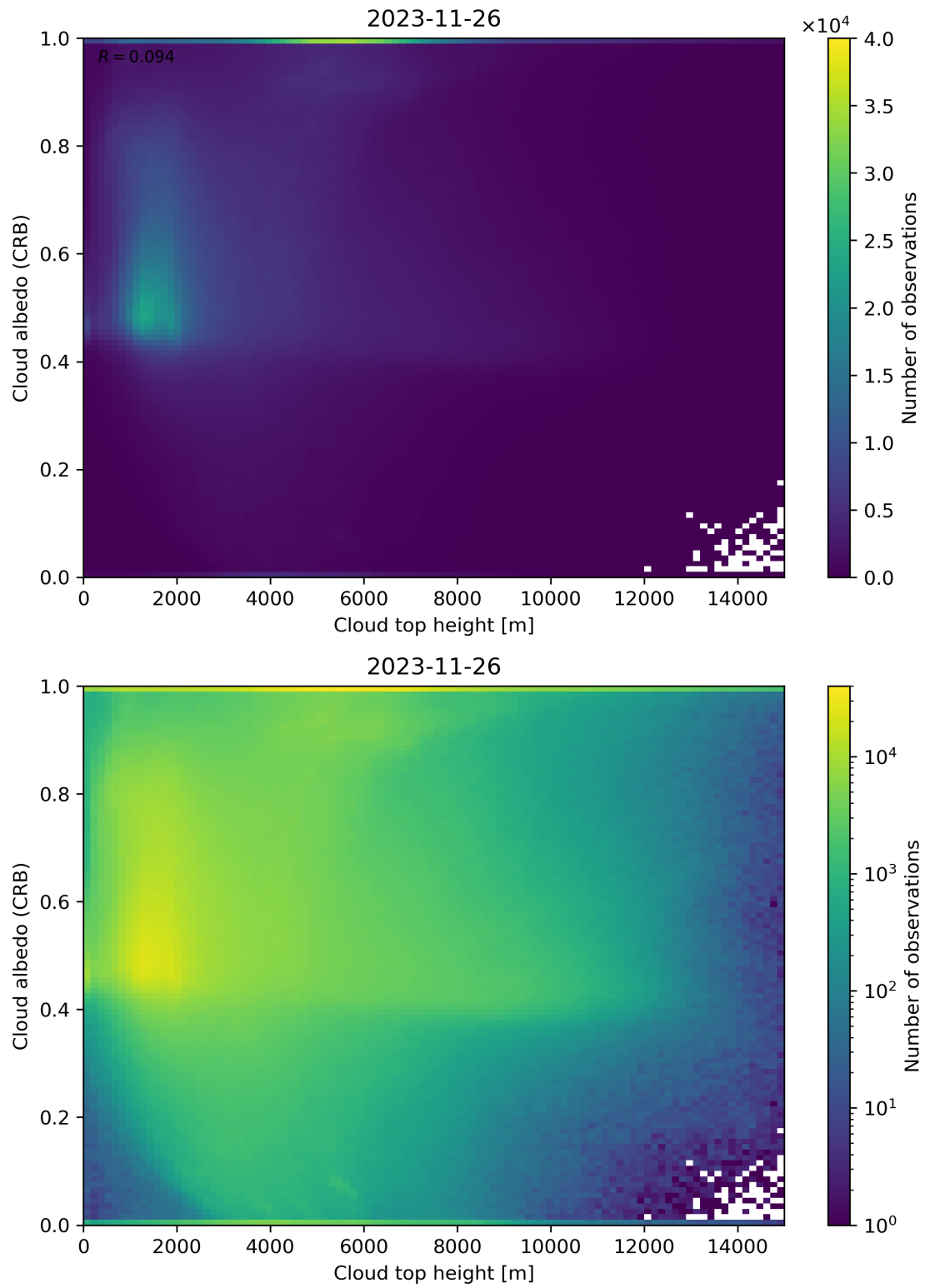
Figure 86: Scatter density plot of “Cloud top height” against “Cloud albedo (CRB)” for 2023-11-25 to 2023-11-27.
