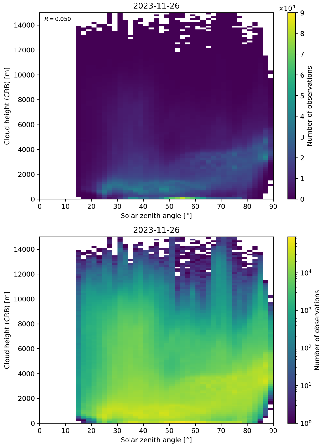
Figure 102: Scatter density plot of “Solar zenith angle” against “Cloud height (CRB)” for 2023-11-25 to 2023-11-27.
