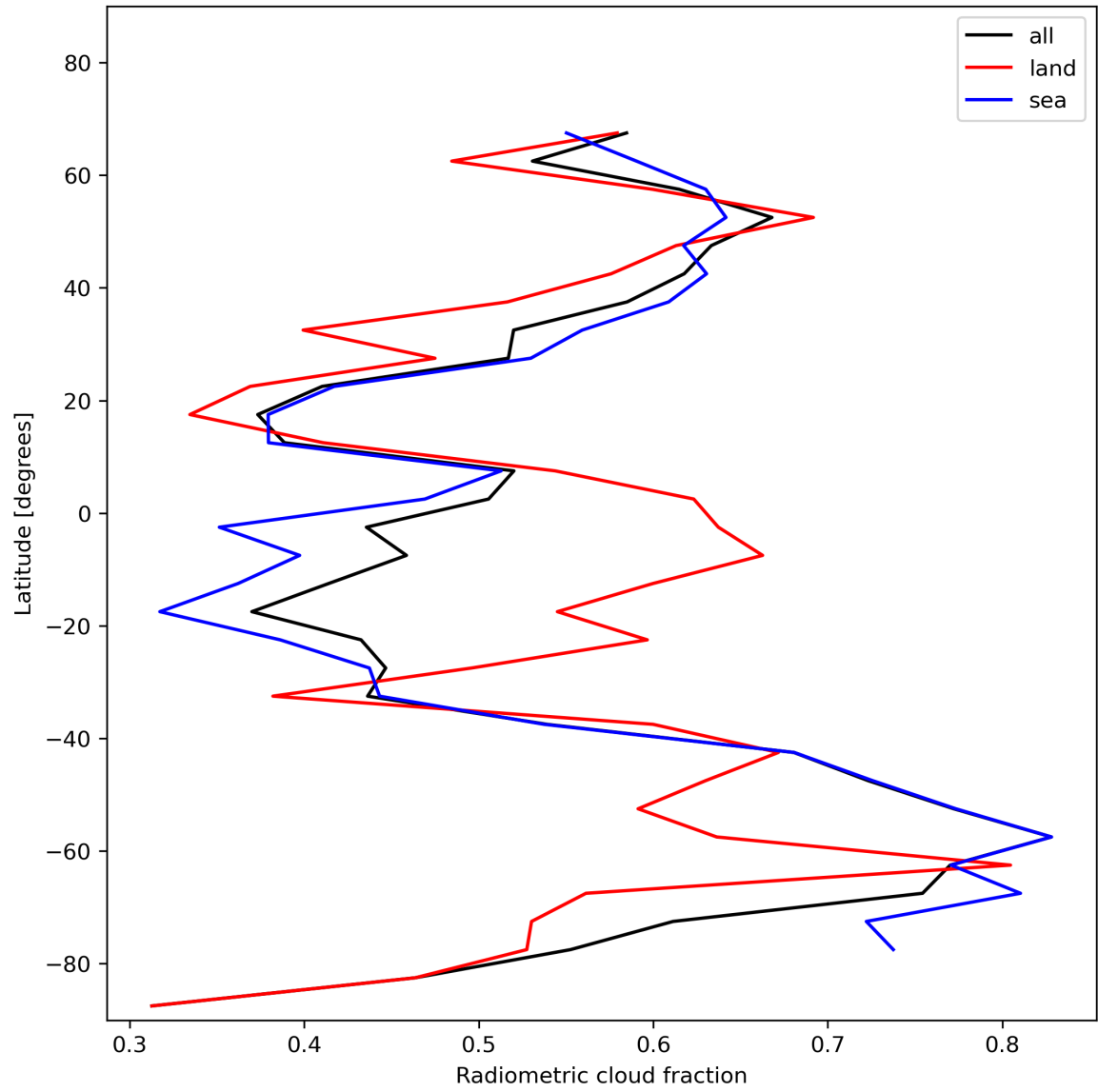
Figure 23: Zonal average of “Radiometric cloud fraction” for 2023-11-25 to 2023-11-27.
