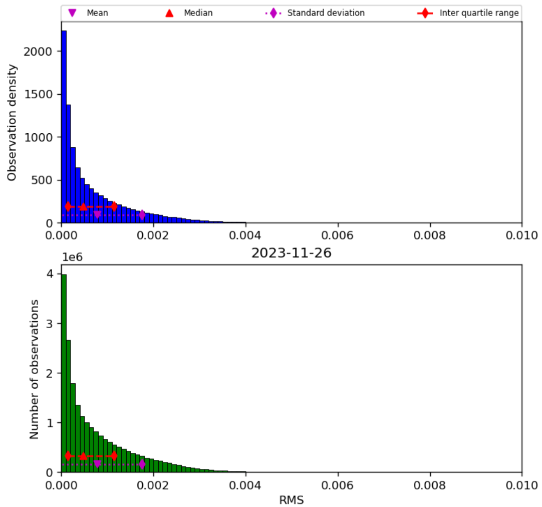
Figure 47: Histogram of “RMS” for 2023-11-25 to 2023-11-27
