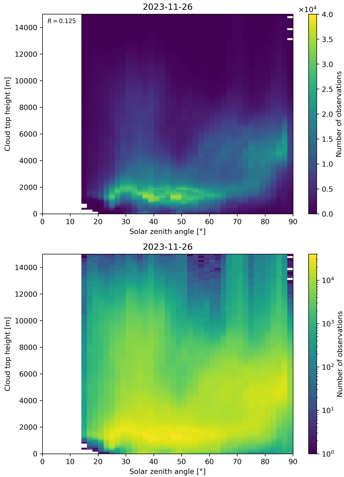
Figure 104: Scatter density plot of “Solar zenith angle” against “Cloud top height” for 2023-11-25 to 2023-11-27.
