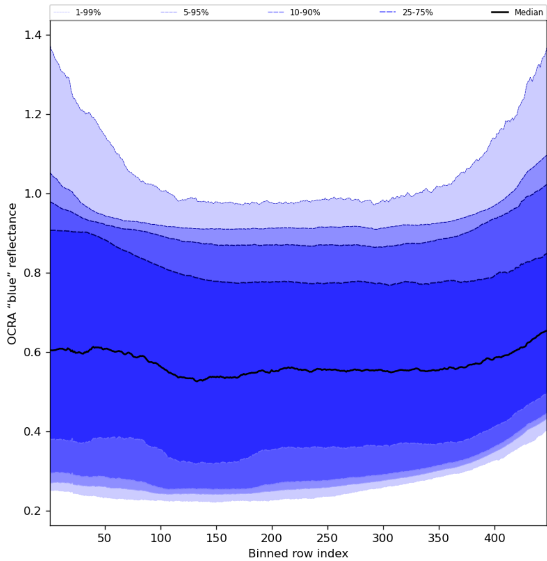
Figure 67: Along track statistics of “OCRA “blue” reflectance” for 2023-11-25 to 2023-11-27
