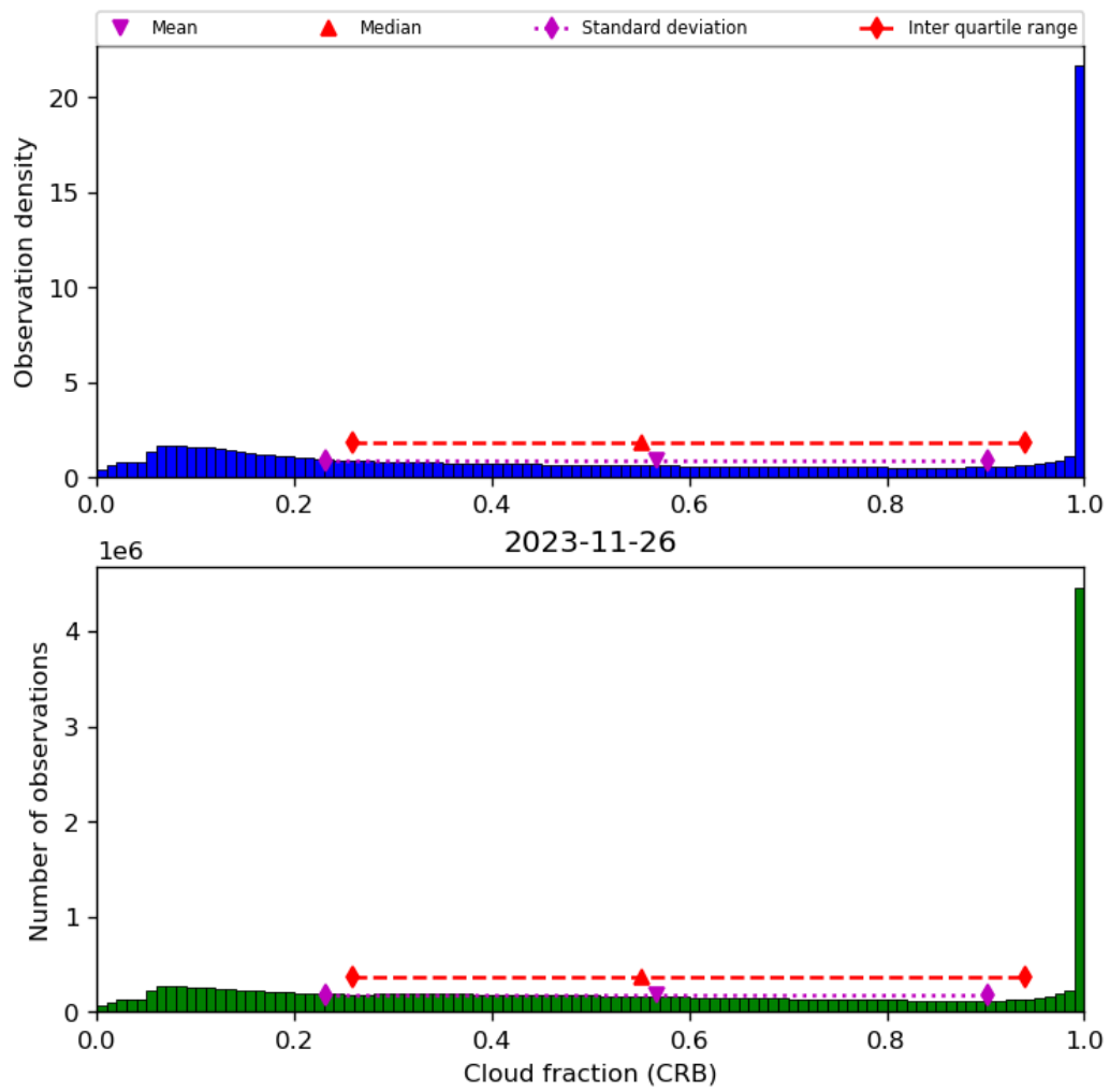
Figure 42: Histogram of “Cloud fraction (CRB)” for 2023-11-25 to 2023-11-27
