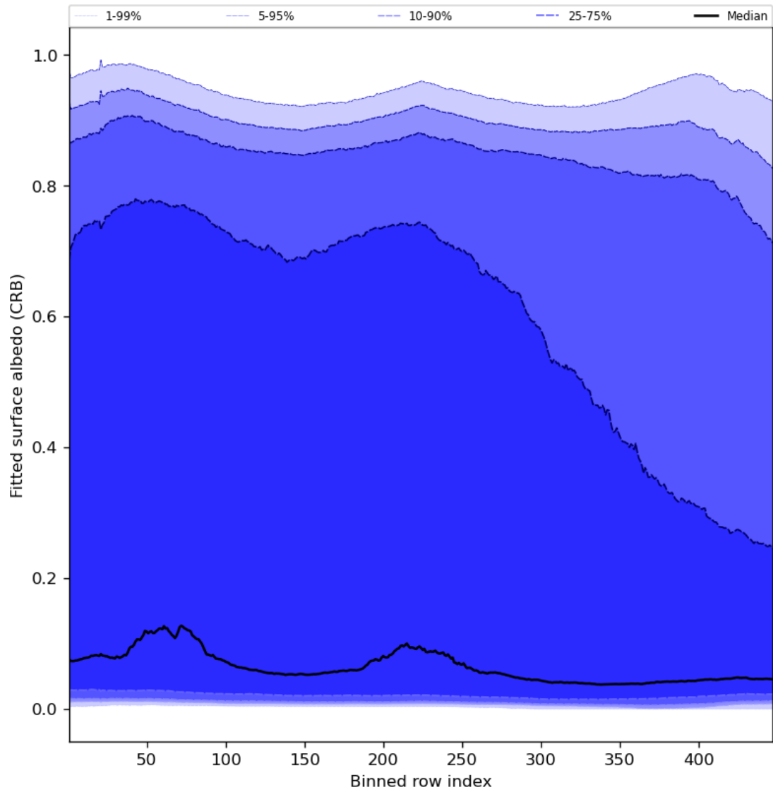
Figure 62: Along track statistics of “Fitted surface albedo (CRB)” for 2023-11-25 to 2023-11-27
