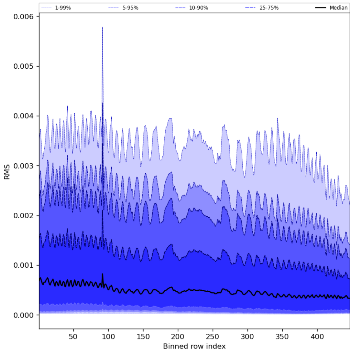
Figure 63: Along track statistics of “RMS” for 2023-11-25 to 2023-11-27
