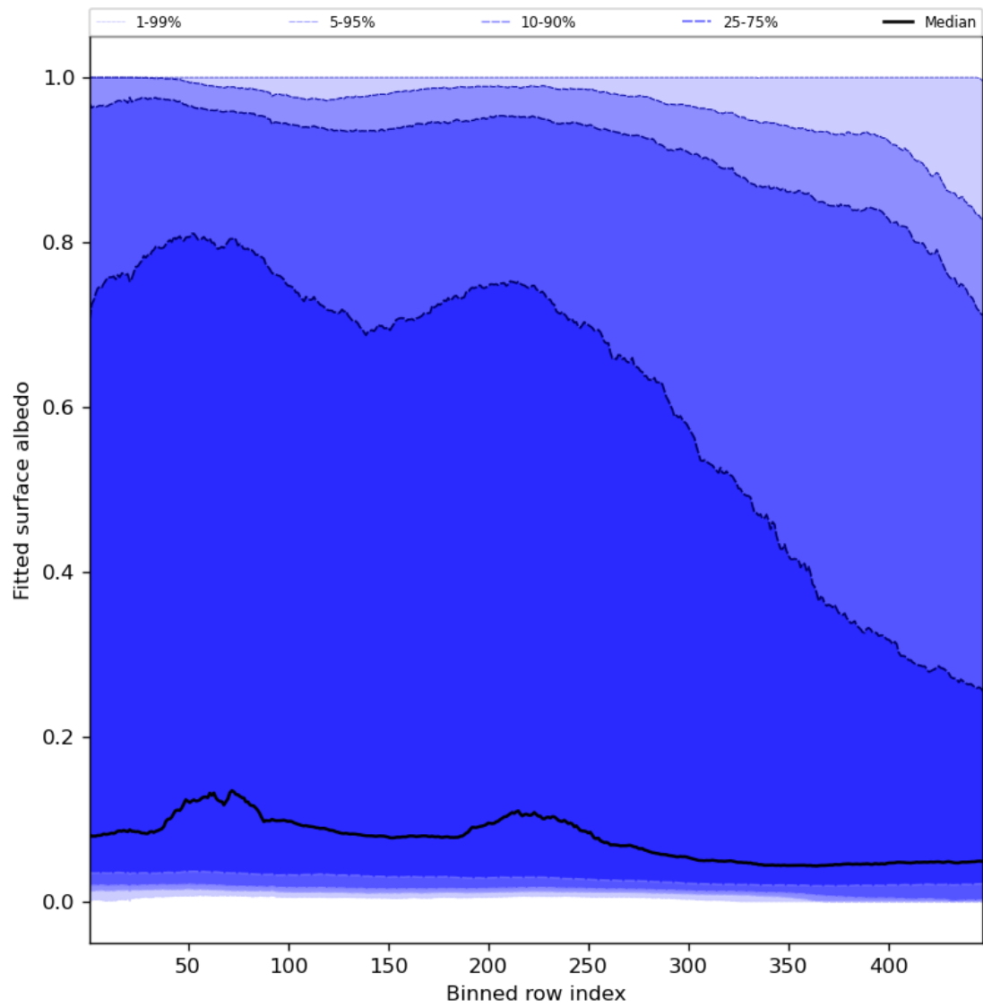
Figure 61: Along track statistics of “Fitted surface albedo” for 2023-11-25 to 2023-11-27
