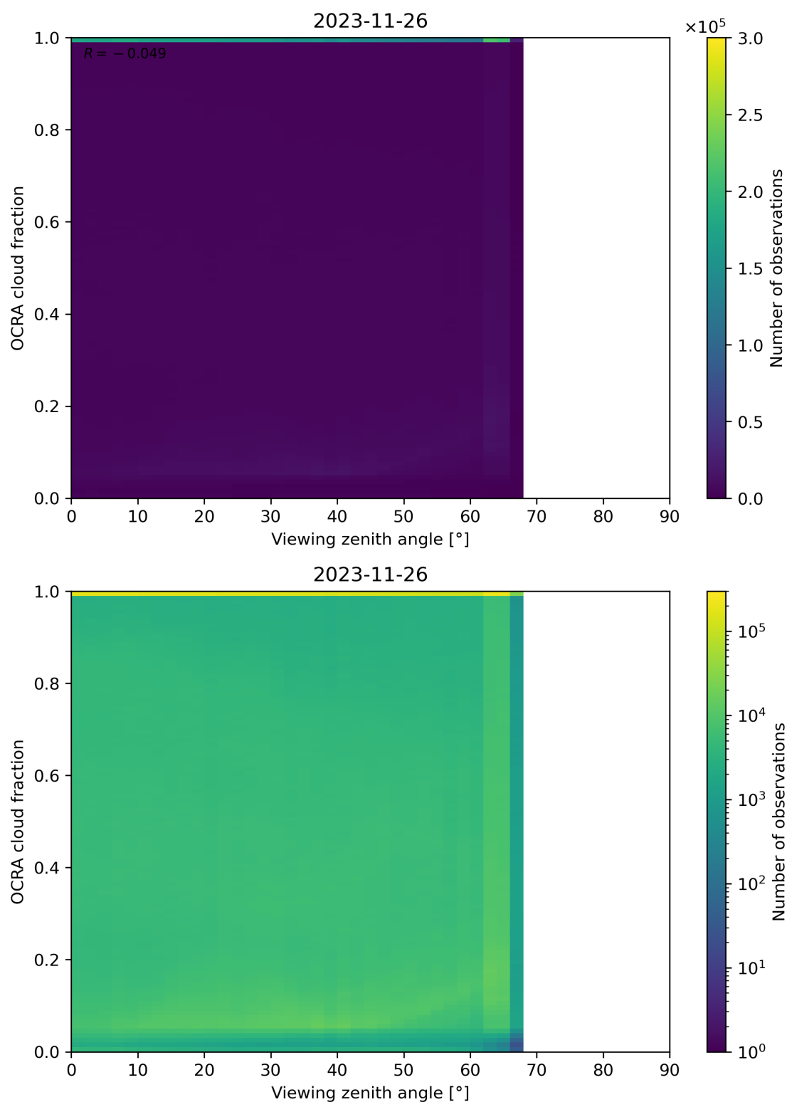
Figure 108: Scatter density plot of “Viewing zenith angle” against “OCRA cloud fraction” for 2023-11-25 to 2023-11-27.
