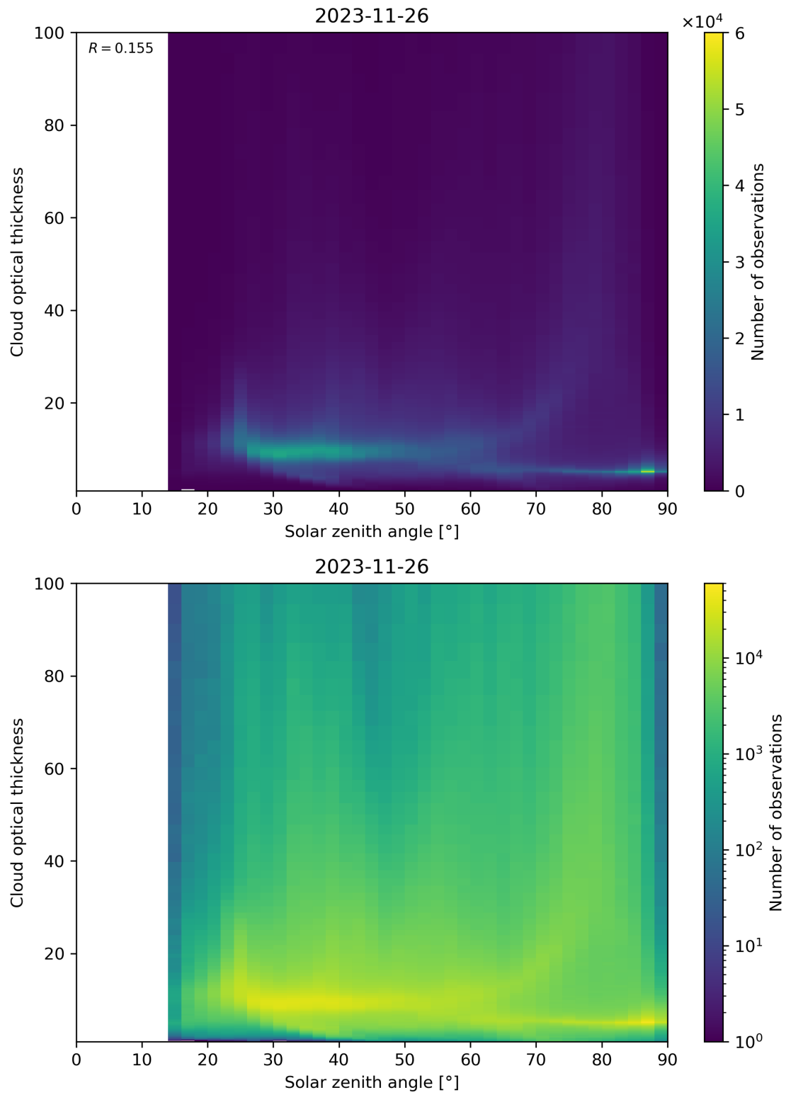
Figure 103: Scatter density plot of “Solar zenith angle” against “Cloud optical thickness” for 2023-11-25 to 2023-11-27.
