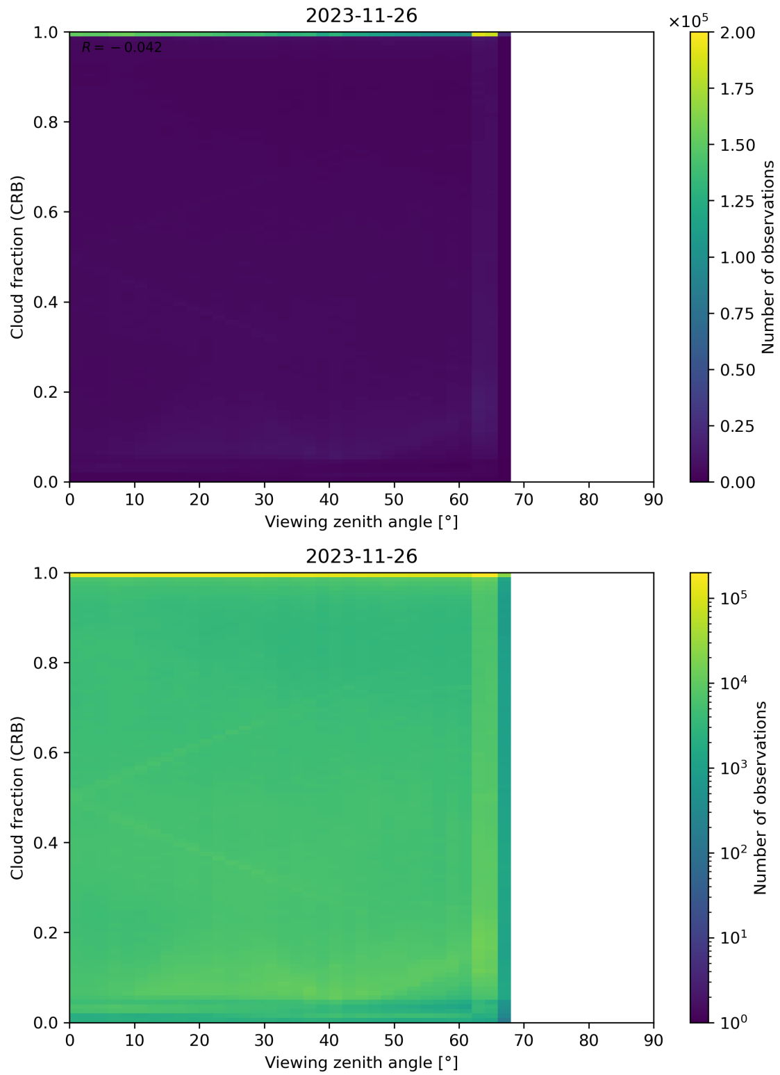
Figure 109: Scatter density plot of “Viewing zenith angle” against “Cloud fraction (CRB)” for 2023-11-25 to 2023-11-27.
