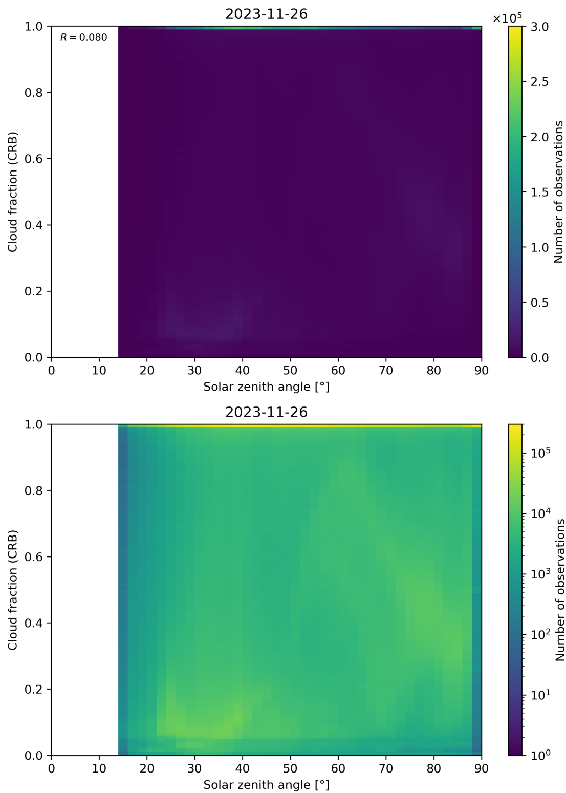
Figure 101: Scatter density plot of “Solar zenith angle” against “Cloud fraction (CRB)” for 2023-11-25 to 2023-11-27.
