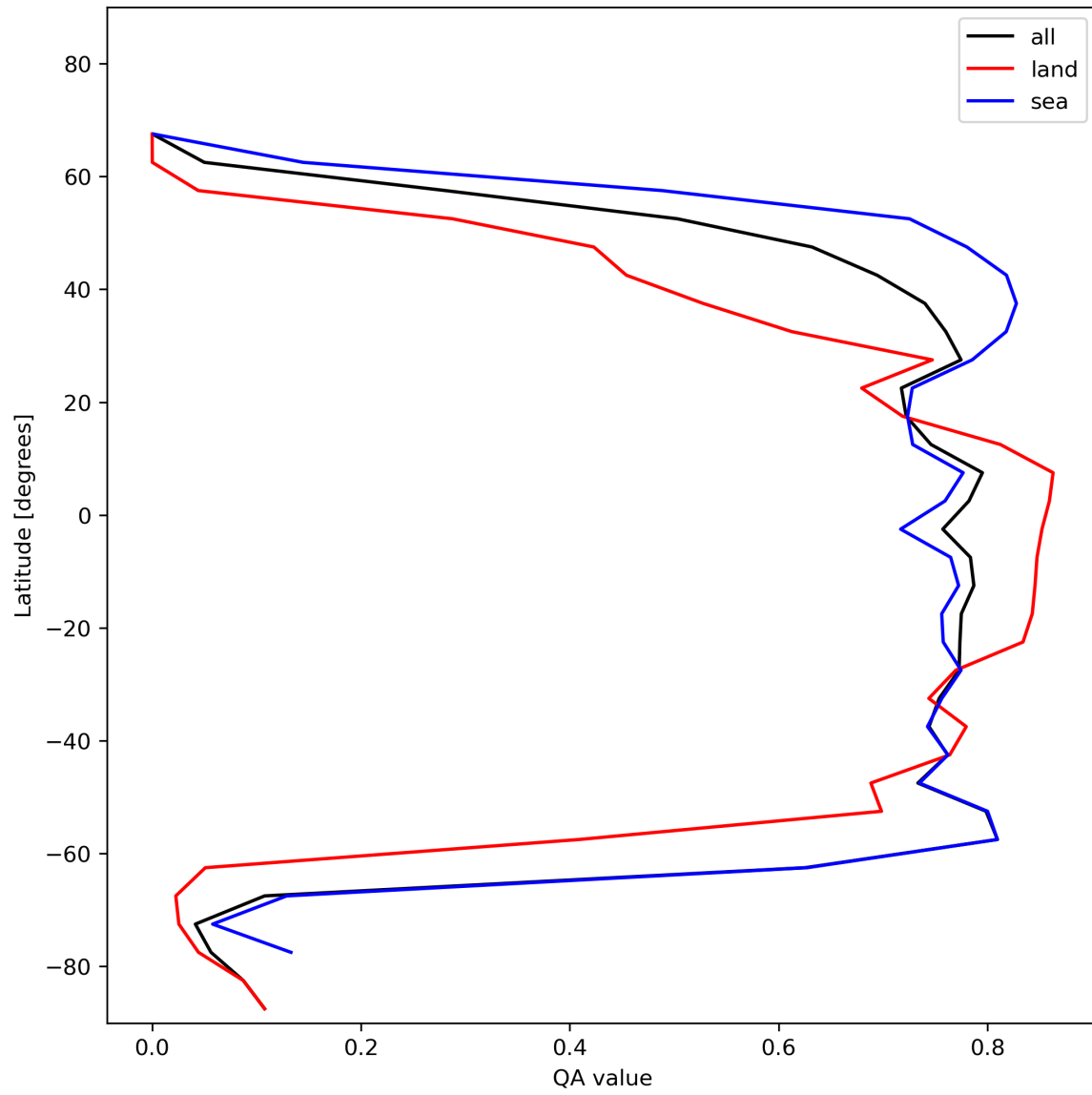
Figure 22: Zonal average of “QA value” for 2023-11-25 to 2023-11-27.
