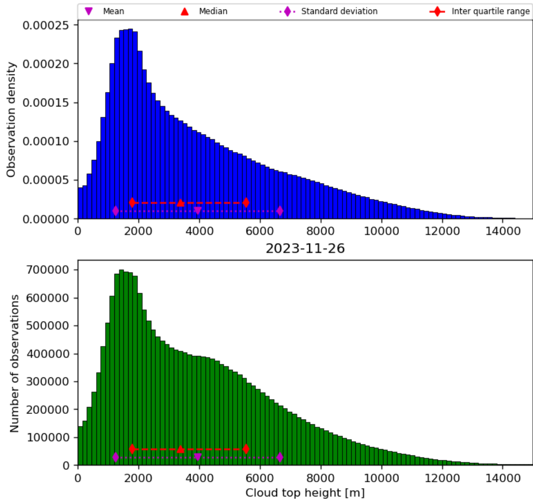
Figure 40: Histogram of “Cloud top height” for 2023-11-25 to 2023-11-27
