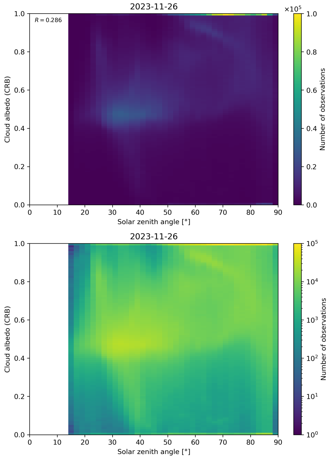
Figure 98: Scatter density plot of “Solar zenith angle” against “Cloud albedo (CRB)” for 2023-11-25 to 2023-11-27.
