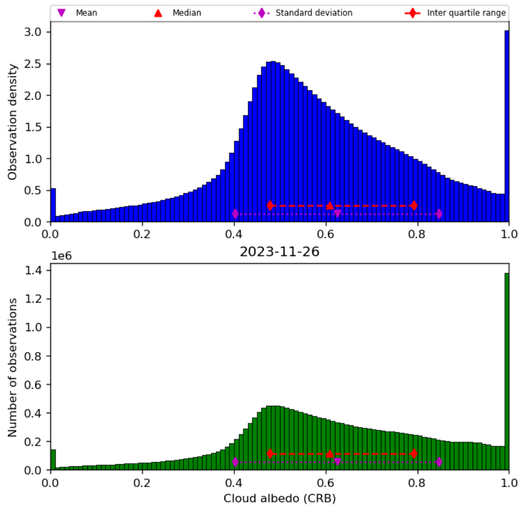
Figure 44: Histogram of “Cloud albedo (CRB)” for 2023-11-25 to 2023-11-27
