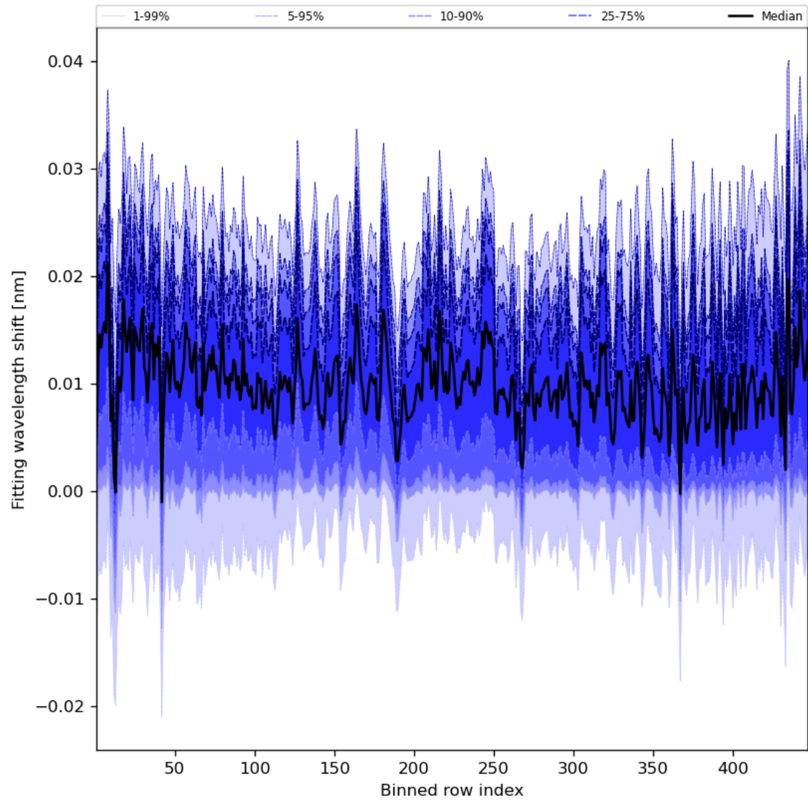
Figure 65: Along track statistics of “Fitting wavelength shift” for 2023-11-25 to 2023-11-27
