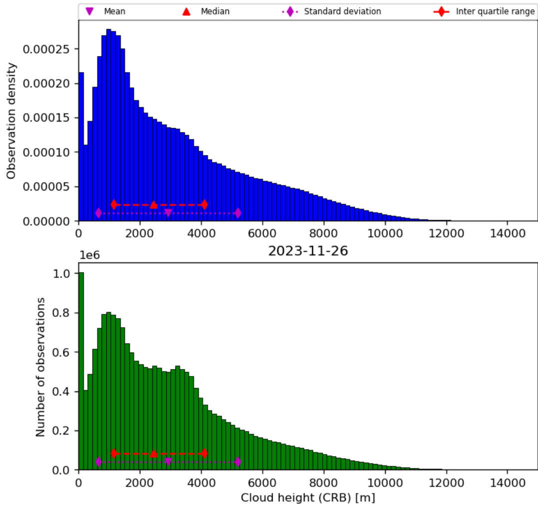
Figure 43: Histogram of “Cloud height (CRB)” for 2023-11-25 to 2023-11-27
