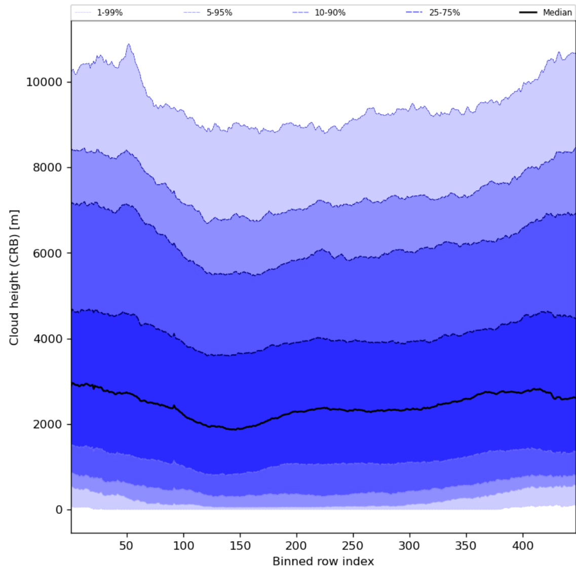
Figure 59: Along track statistics of “Cloud height (CRB)” for 2023-11-25 to 2023-11-27
