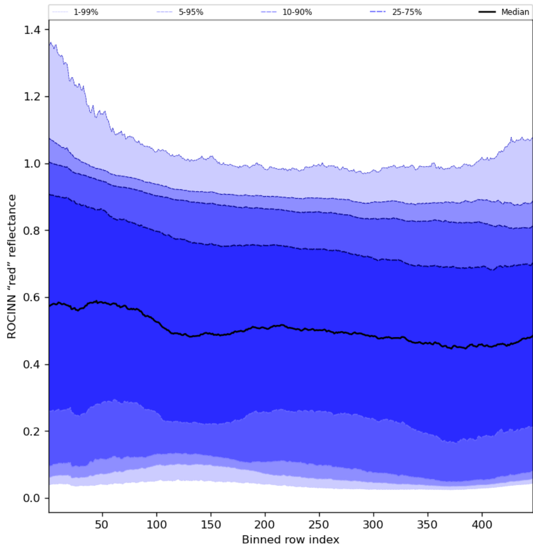
Figure 69: Along track statistics of "ROCINN "red" reflectance" for 2023-11-25 to 2023-11-27
