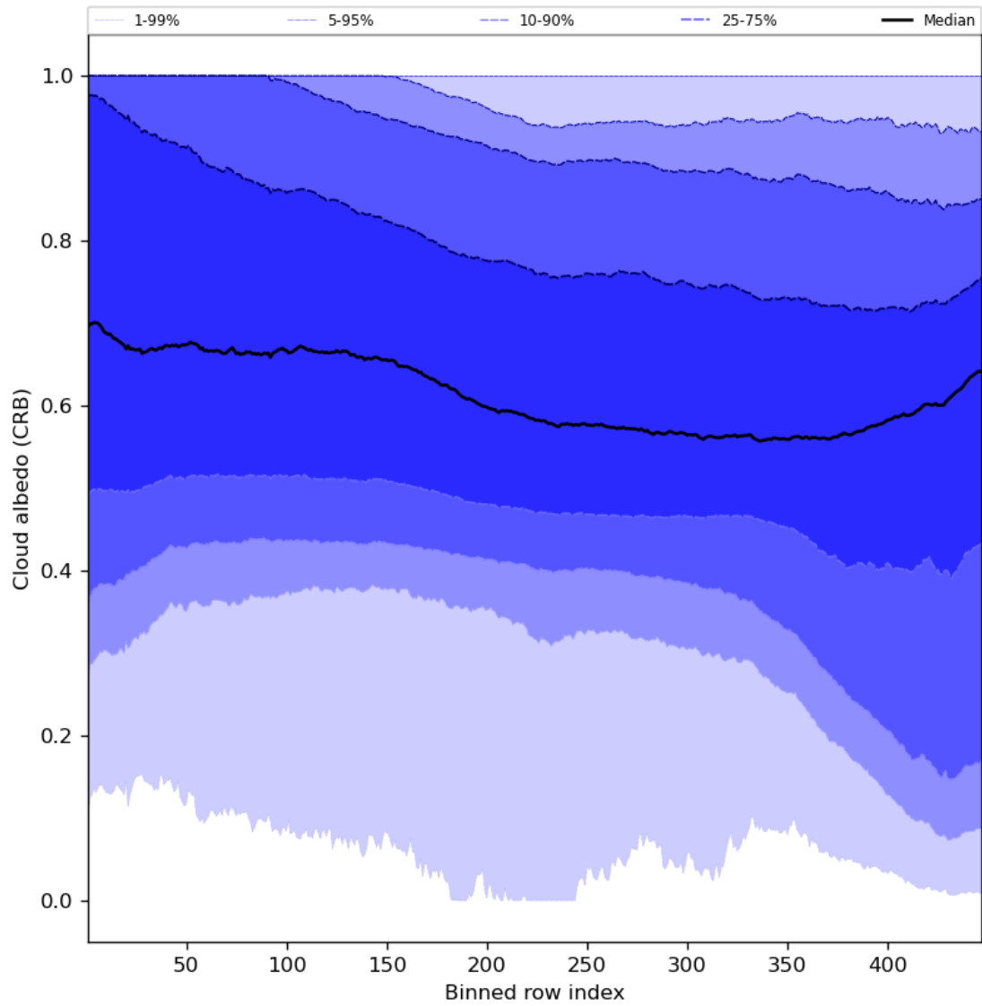
Figure 60: Along track statistics of “Cloud albedo (CRB)” for 2023-11-25 to 2023-11-27
