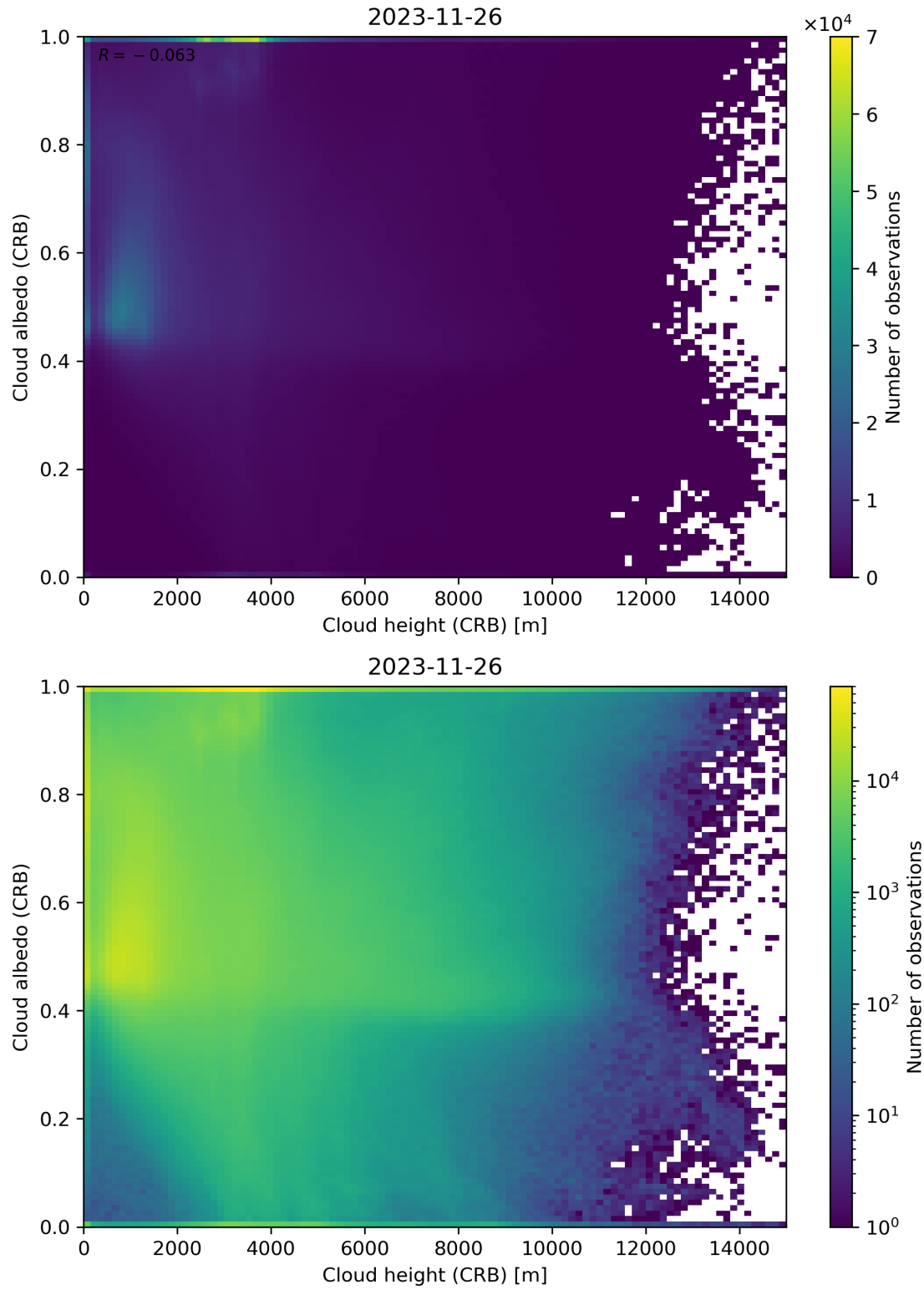
Figure 80: Scatter density plot of “Cloud height (CRB)” against “Cloud albedo (CRB)” for 2023-11-25 to 2023-11-27.
