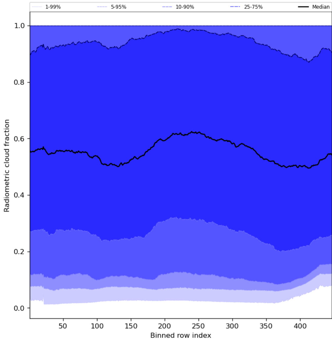
Figure 55: Along track statistics of “Radiometric cloud fraction” for 2023-11-25 to 2023-11-27
