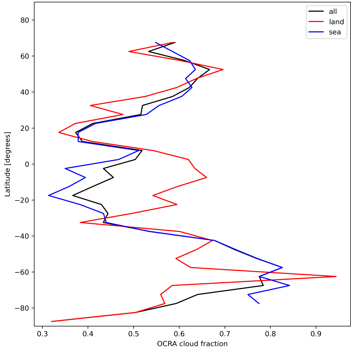
Figure 34: Zonal average of “OCRA cloud fraction” for 2023-11-25 to 2023-11-27.
