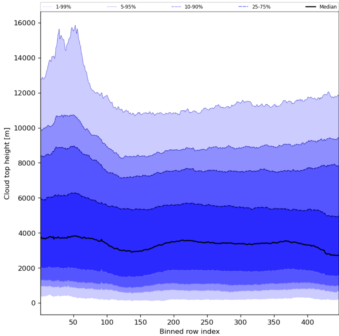
Figure 56: Along track statistics of “Cloud top height” for 2023-11-25 to 2023-11-27
