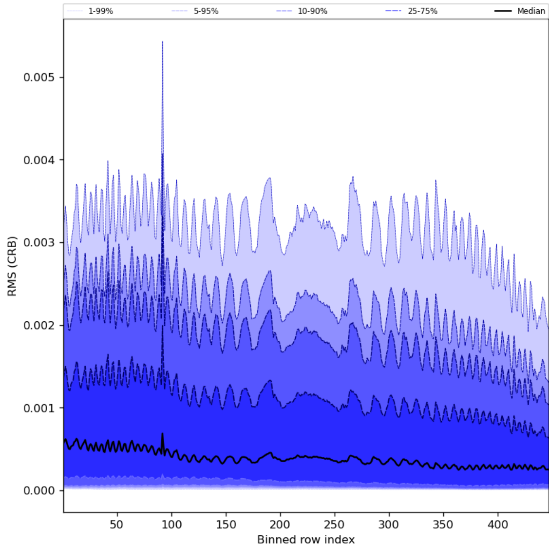
Figure 64: Along track statistics of “RMS (CRB)” for 2023-11-25 to 2023-11-27
