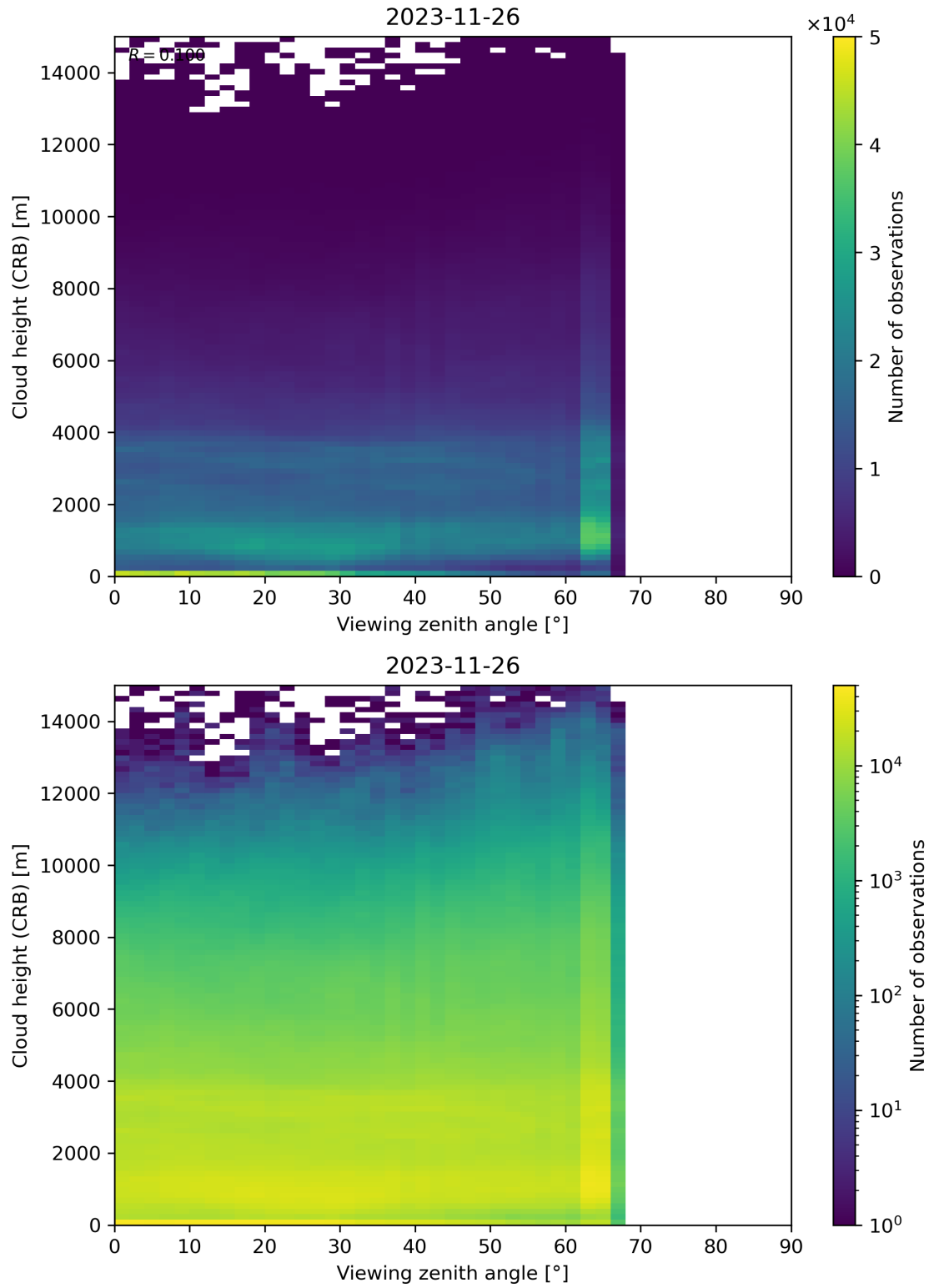
Figure 110: Scatter density plot of “Viewing zenith angle” against “Cloud height (CRB)” for 2023-11-25 to 2023-11-27.
