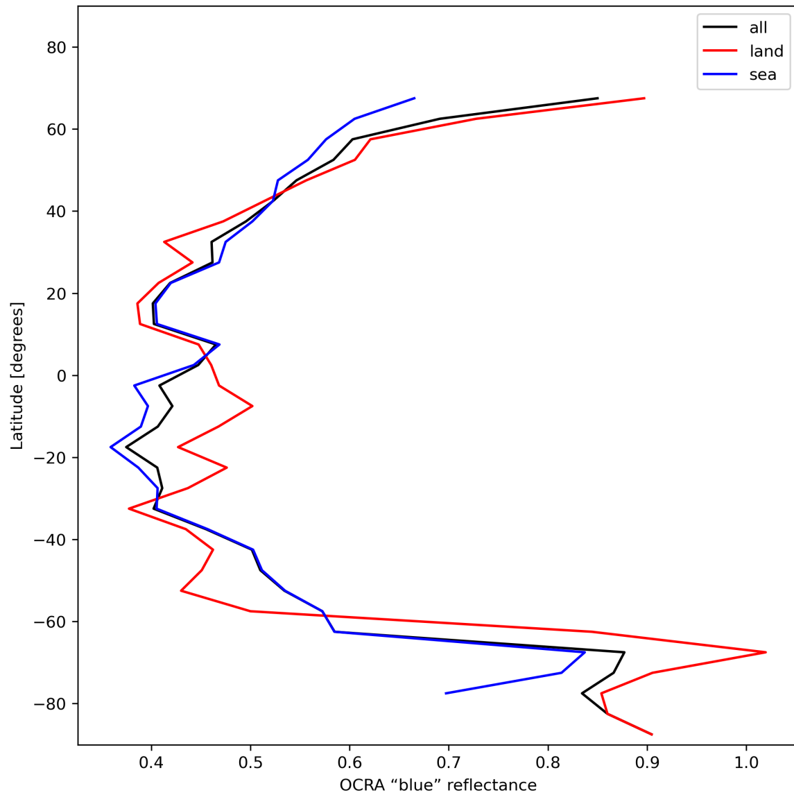
Figure 35: Zonal average of “OCRA “blue” reflectance” for 2023-11-25 to 2023-11-27.
