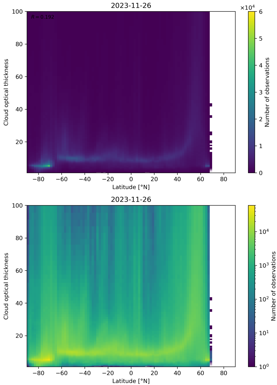
Figure 96: Scatter density plot of “Latitude” against “Cloud optical thickness” for 2023-11-25 to 2023-11-27.
