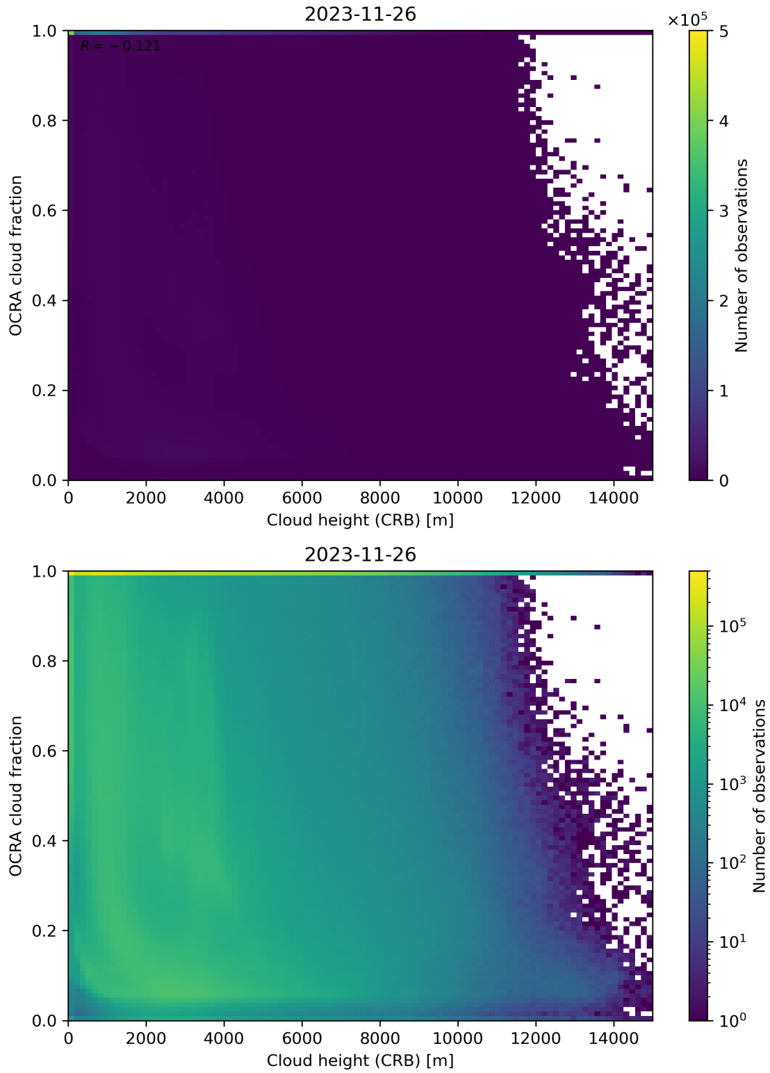
Figure 81: Scatter density plot of “Cloud height (CRB)” against “OCRA cloud fraction” for 2023-11-25 to 2023-11-27.
