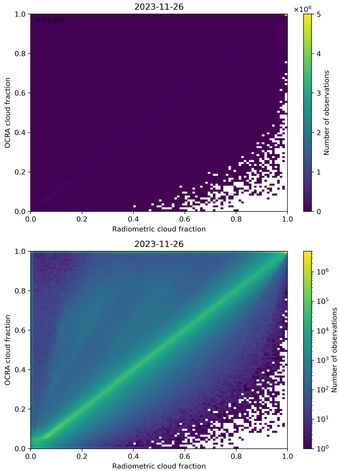
Figure 72: Scatter density plot of “Radiometric cloud fraction” against “OCRA cloud fraction” for 2023-11-25 to 2023-11-27.
