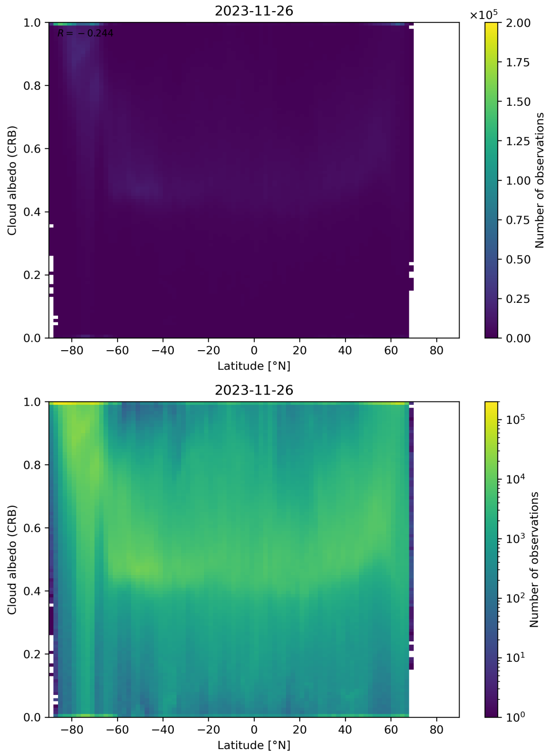
Figure 91: Scatter density plot of “Latitude” against “Cloud albedo (CRB)” for 2023-11-25 to 2023-11-27.
