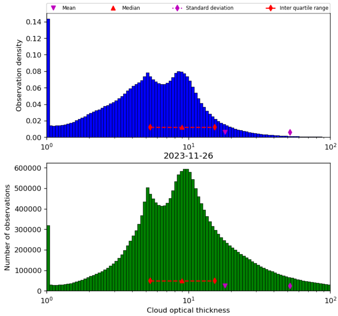
Figure 41: Histogram of “Cloud optical thickness” for 2023-11-25 to 2023-11-27
