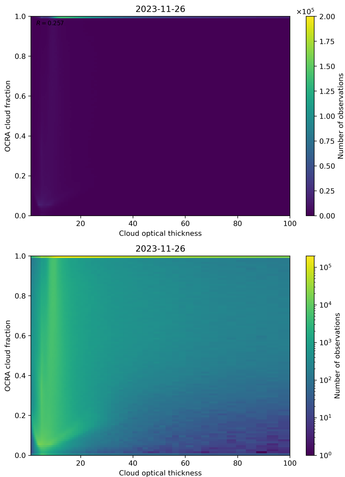
Figure 83: Scatter density plot of “Cloud optical thickness” against “OCRA cloud fraction” for 2023-11-25 to 2023-11-27.
