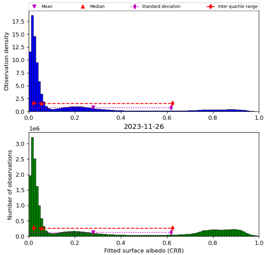
Figure 46: Histogram of “Fitted surface albedo (CRB)” for 2023-11-25 to 2023-11-27
