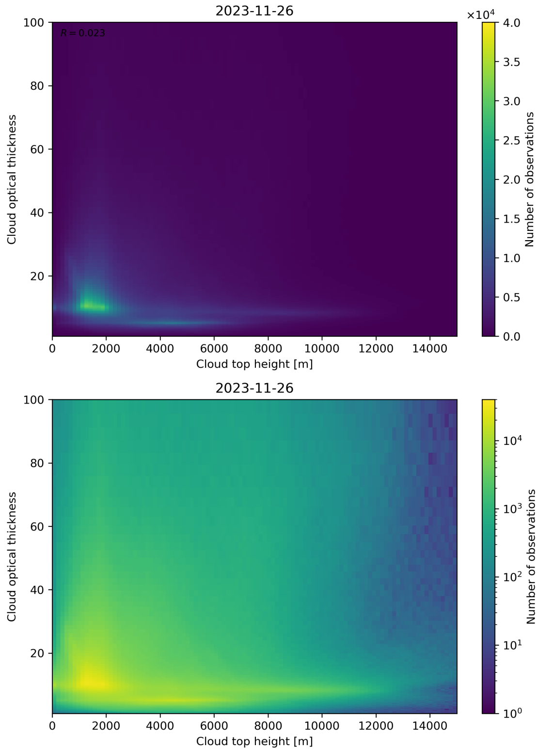
Figure 90: Scatter density plot of “Cloud top height” against “Cloud optical thickness” for 2023-11-25 to 2023-11-27.
