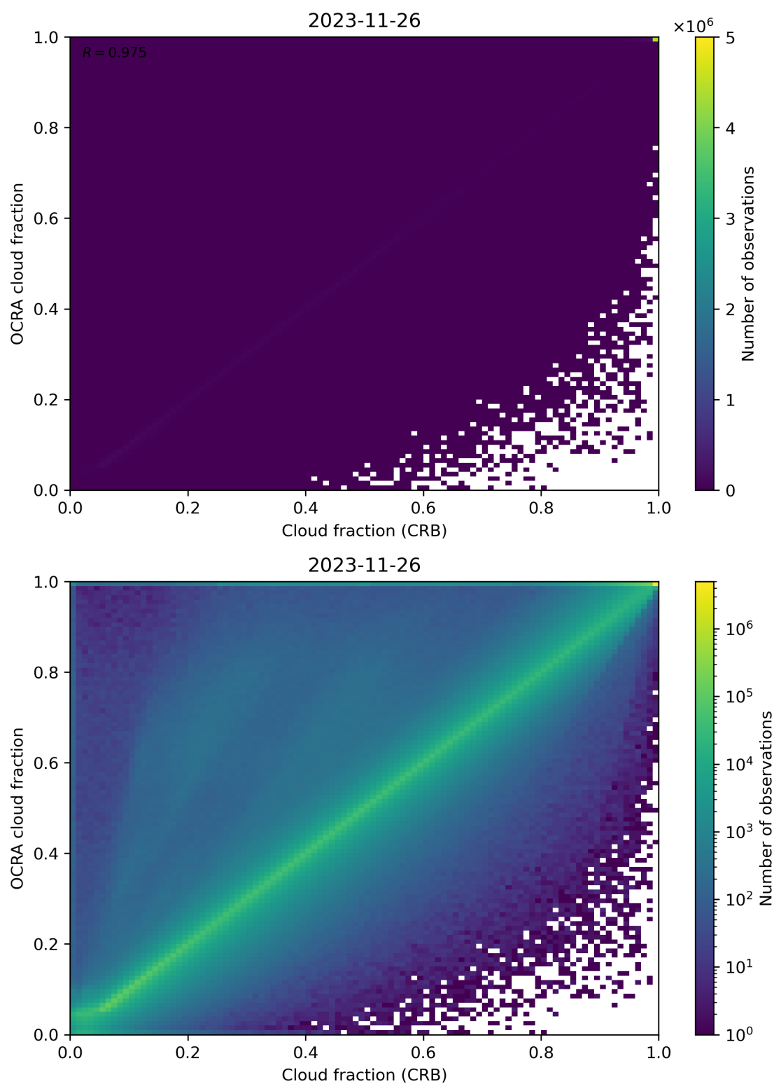
Figure 78: Scatter density plot of “Cloud fraction (CRB)” against “OCRA cloud fraction” for 2023-11-25 to 2023-11-27.
