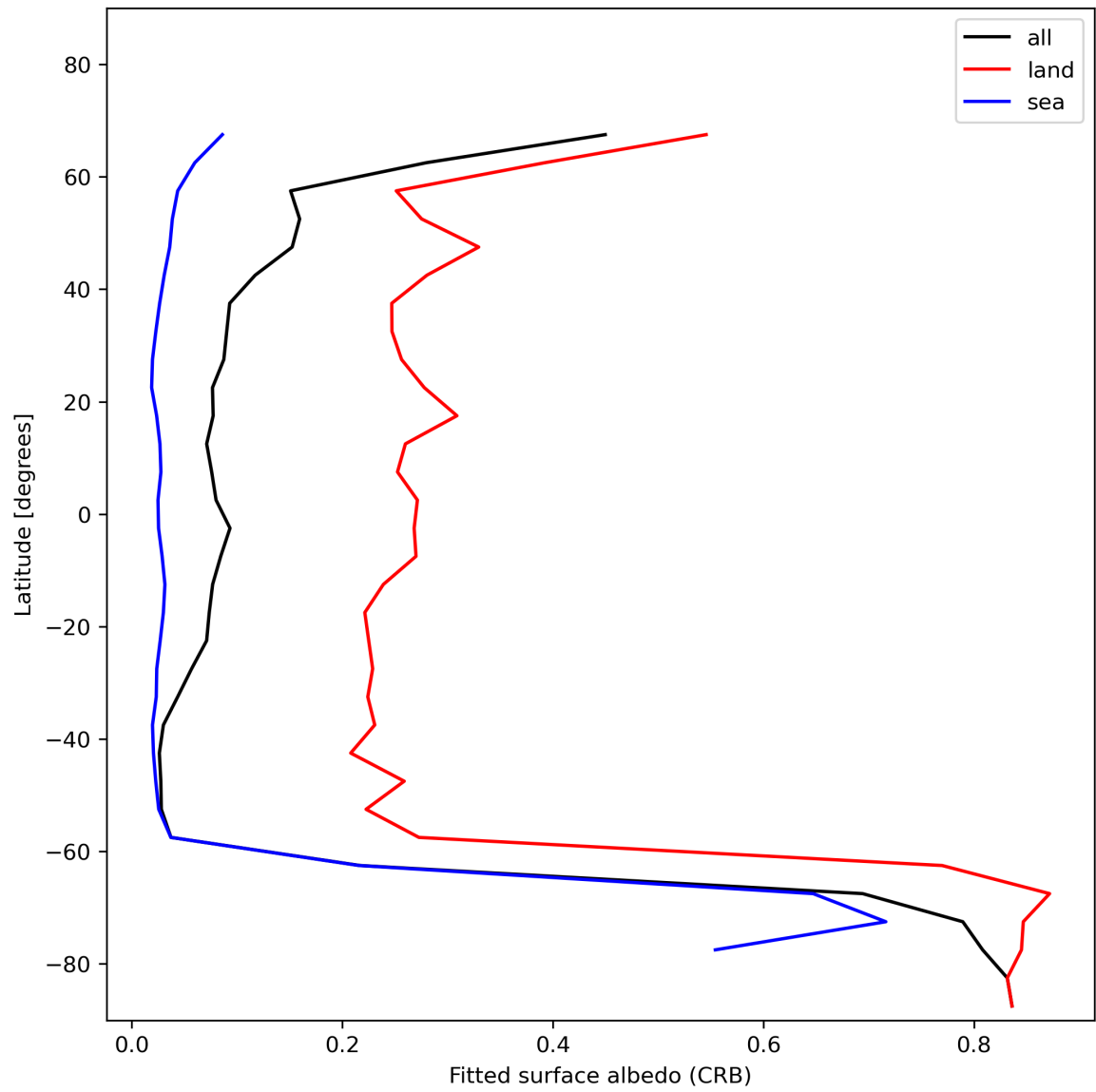
Figure 30: Zonal average of “Fitted surface albedo (CRB)” for 2023-11-25 to 2023-11-27.
