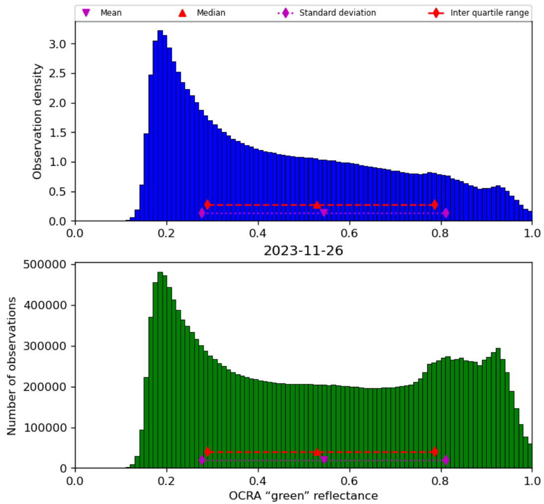
Figure 52: Histogram of “OCRA “green” reflectance” for 2023-11-25 to 2023-11-27
