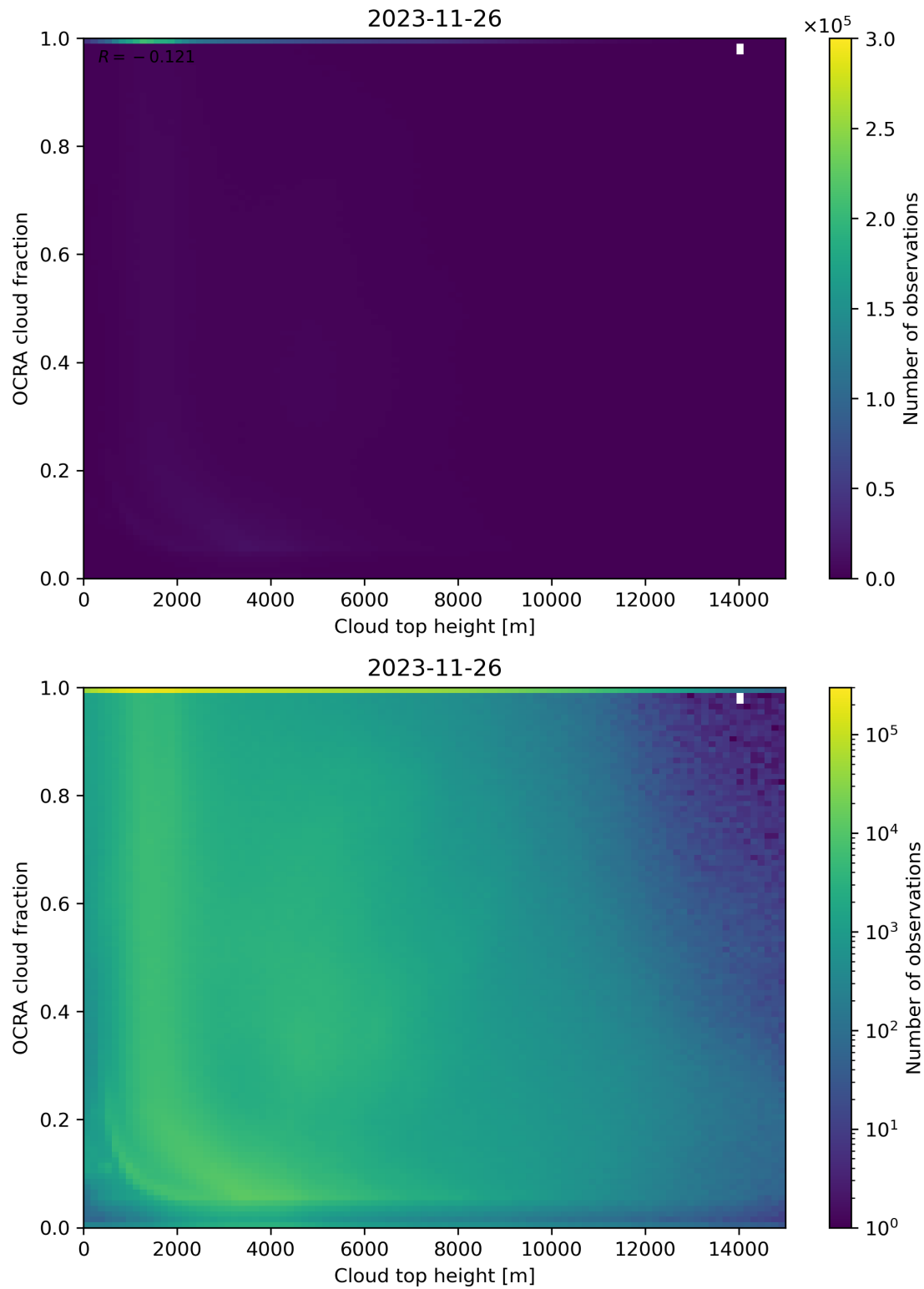
Figure 87: Scatter density plot of “Cloud top height” against “OCRA cloud fraction” for 2023-11-25 to 2023-11-27.
