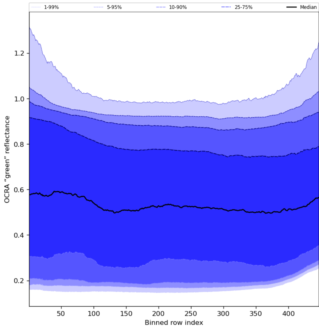
Figure 68: Along track statistics of "OCRA "green" reflectance" for 2023-11-25 to 2023-11-27
