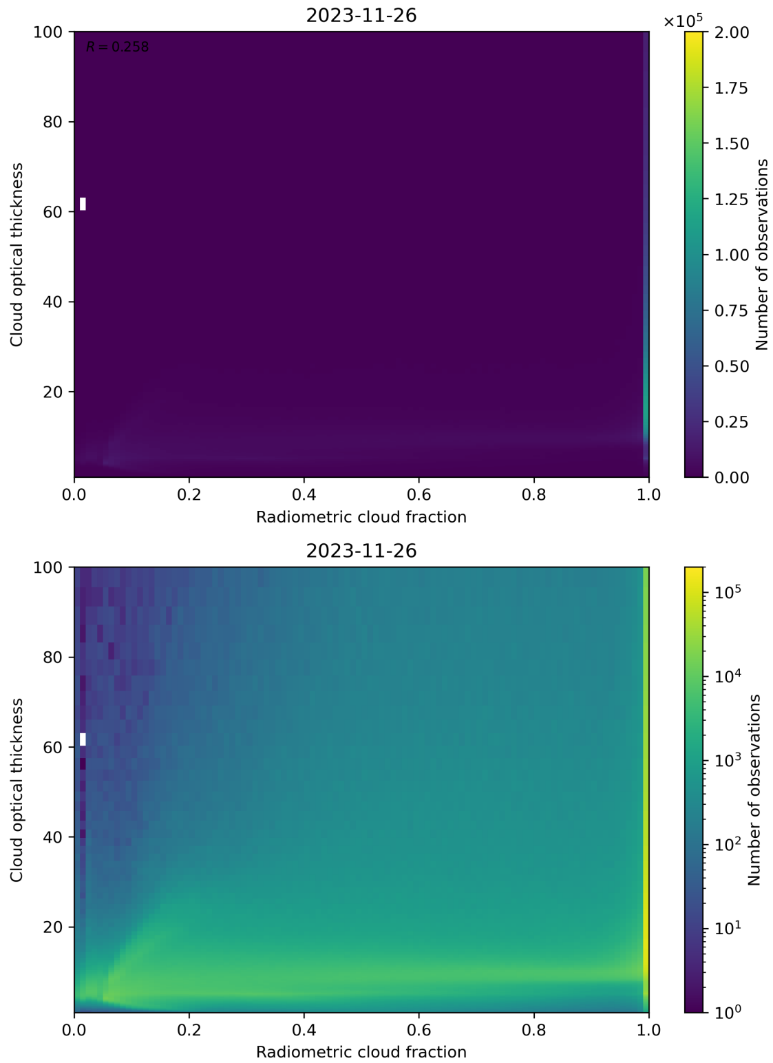
Figure 75: Scatter density plot of “Radiometric cloud fraction” against “Cloud optical thickness” for 2023-11-25 to 2023-11-27.
