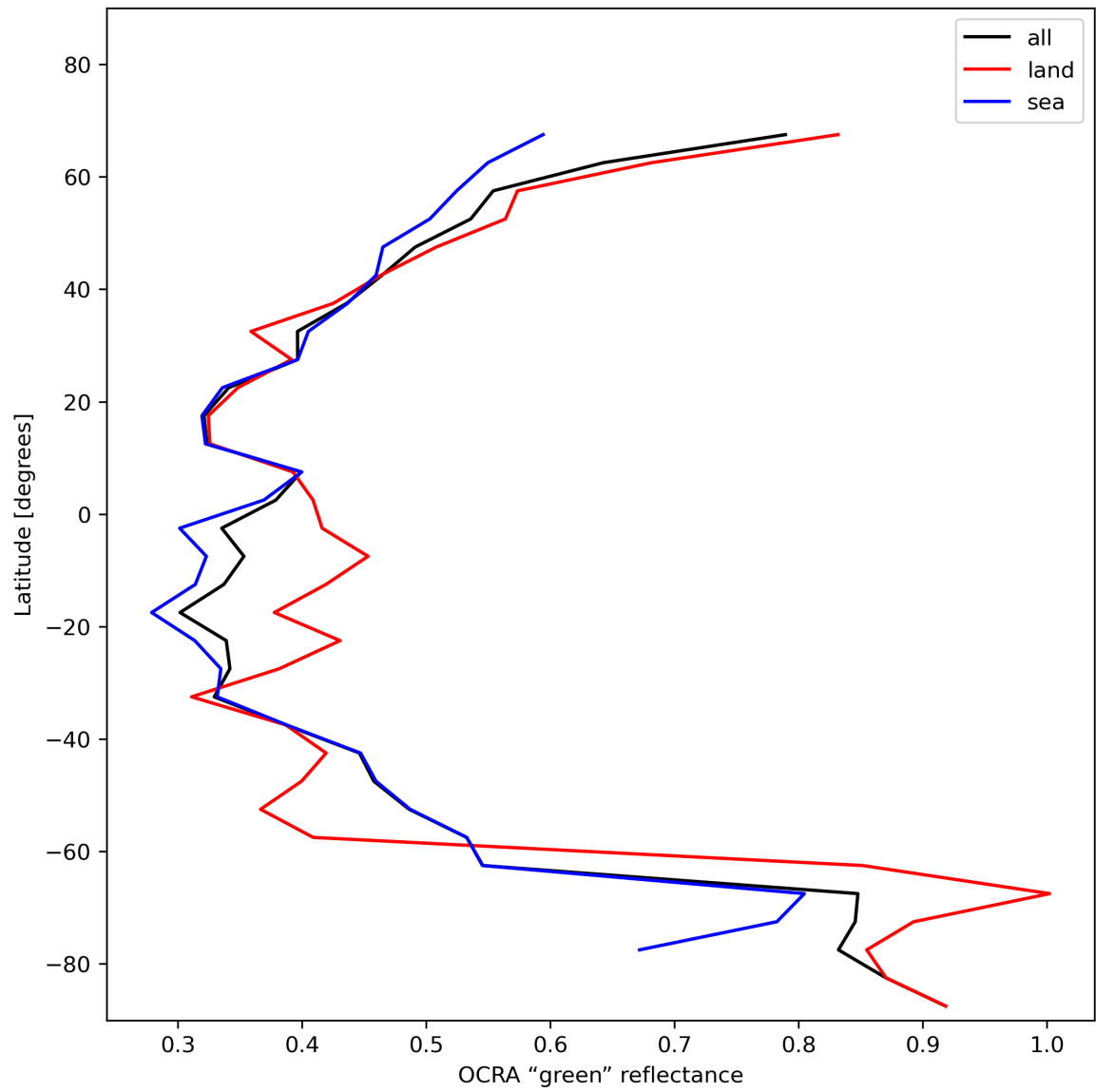
Figure 36: Zonal average of “OCRA “green” reflectance” for 2023-11-25 to 2023-11-27.
