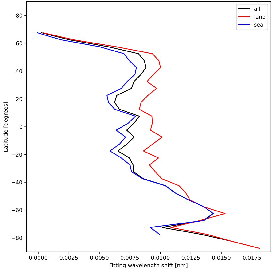
Figure 33: Zonal average of “Fitting wavelength shift” for 2023-11-25 to 2023-11-27.
