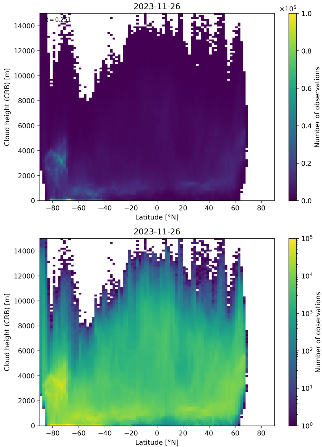
Figure 95: Scatter density plot of “Latitude” against “Cloud height (CRB)” for 2023-11-25 to 2023-11-27.
