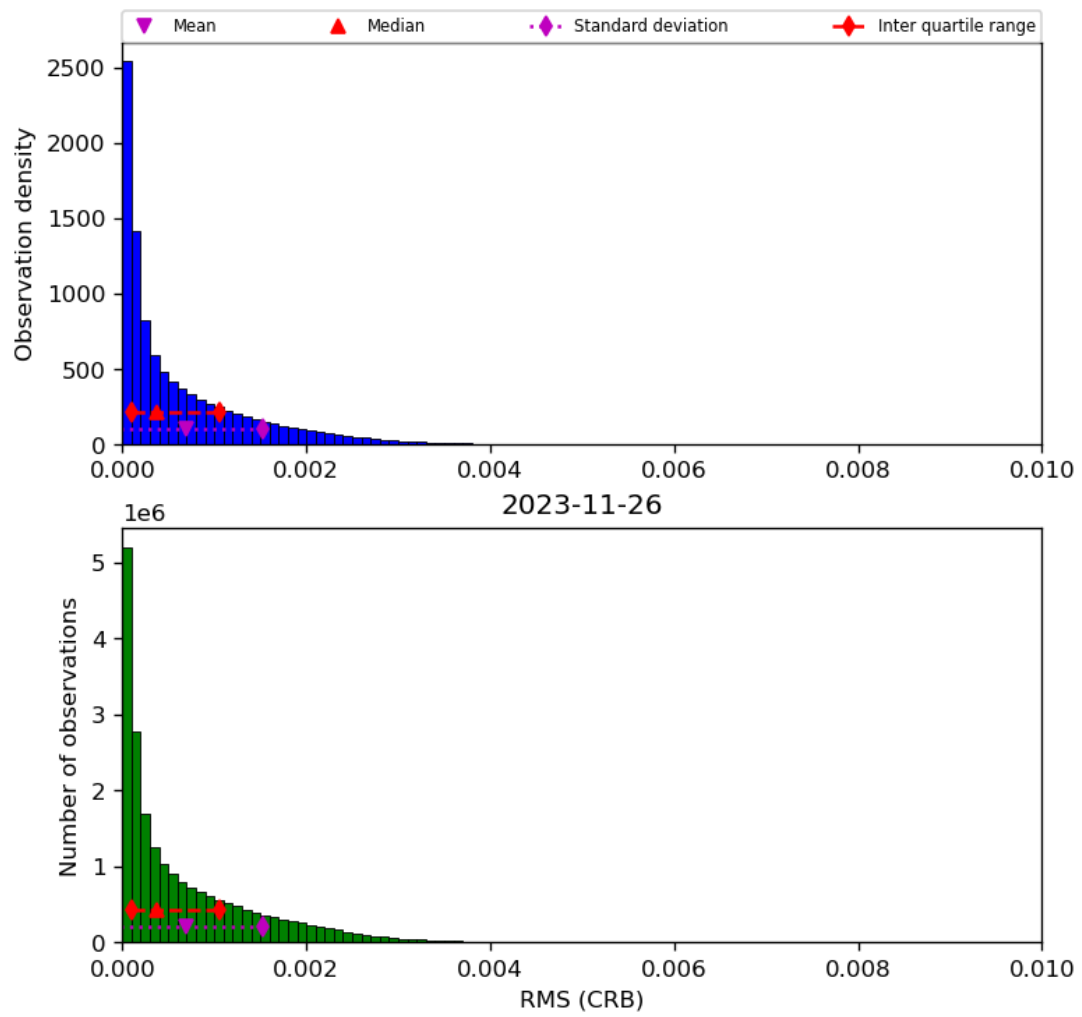
Figure 48: Histogram of “RMS (CRB)” for 2023-11-25 to 2023-11-27
