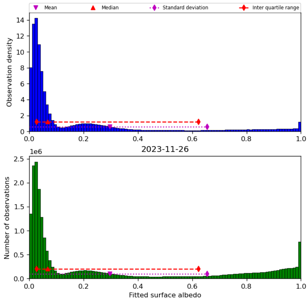
Figure 45: Histogram of “Fitted surface albedo” for 2023-11-25 to 2023-11-27
