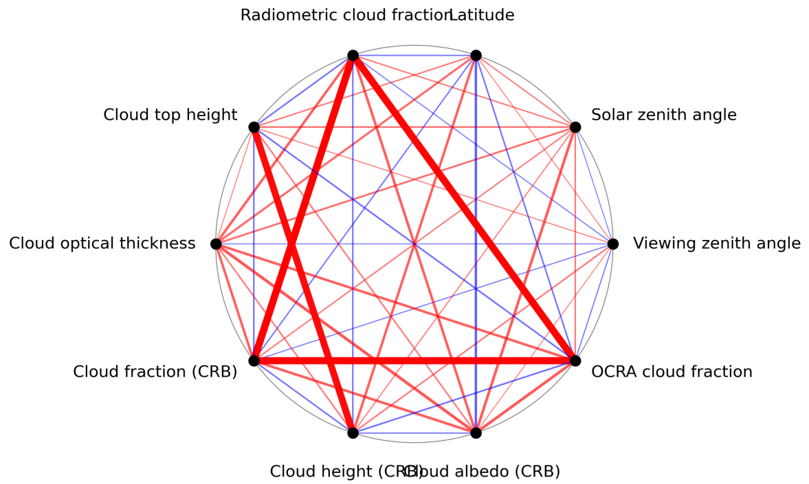
Figure 1: Map of correlation graph for 2023-11-25 to 2023-11-27.
