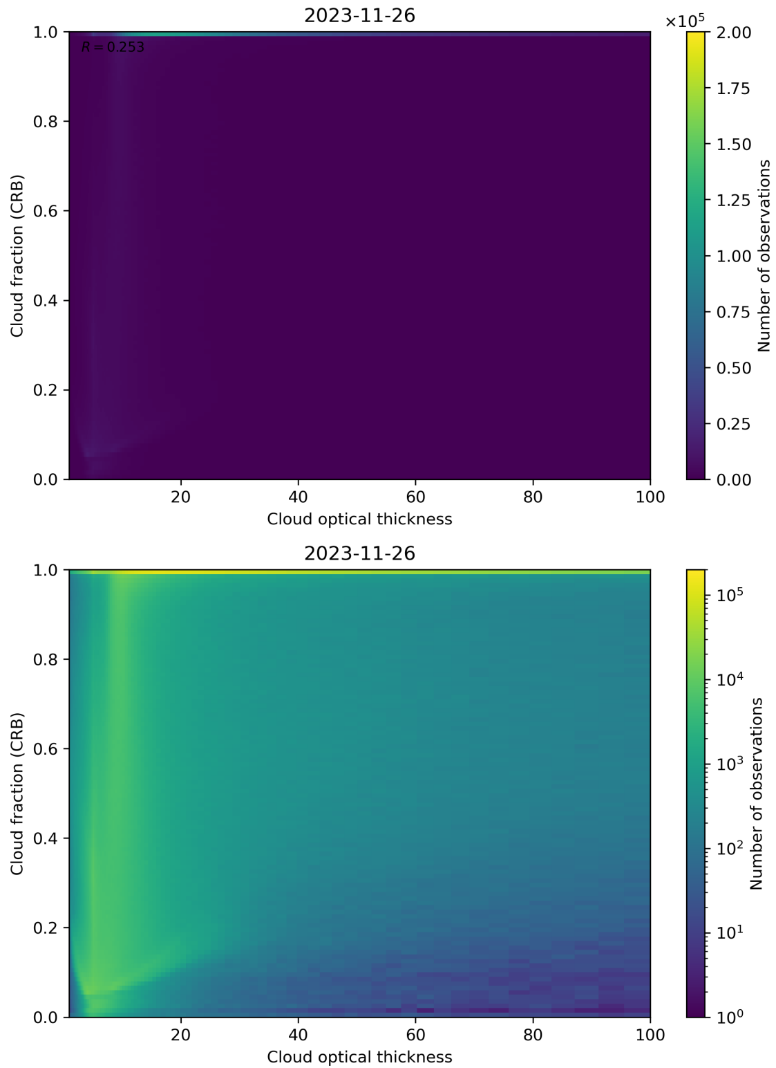
Figure 84: Scatter density plot of “Cloud optical thickness” against “Cloud fraction (CRB)” for 2023-11-25 to 2023-11-27.
