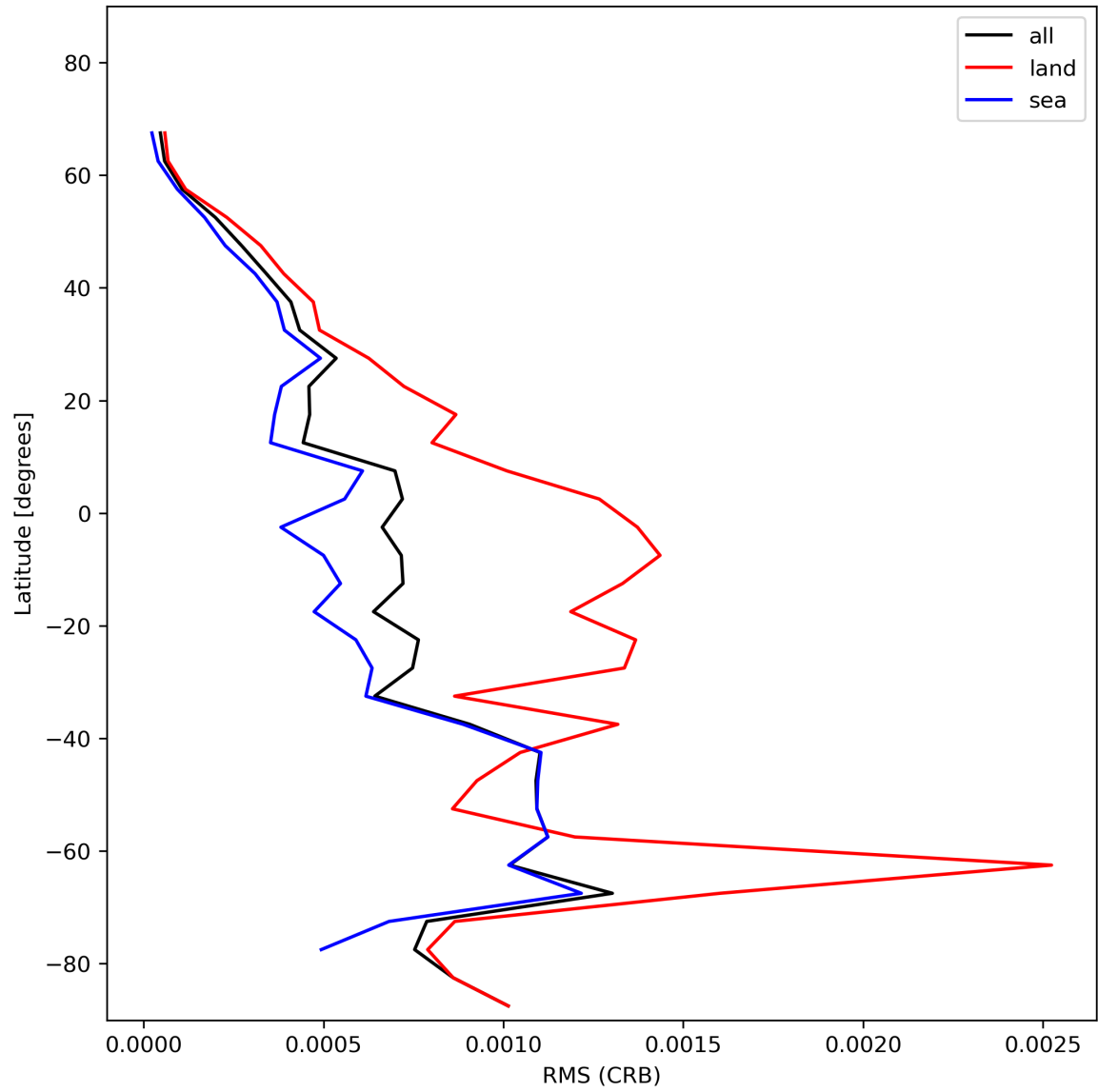
Figure 32: Zonal average of “RMS (CRB)” for 2023-11-25 to 2023-11-27.
