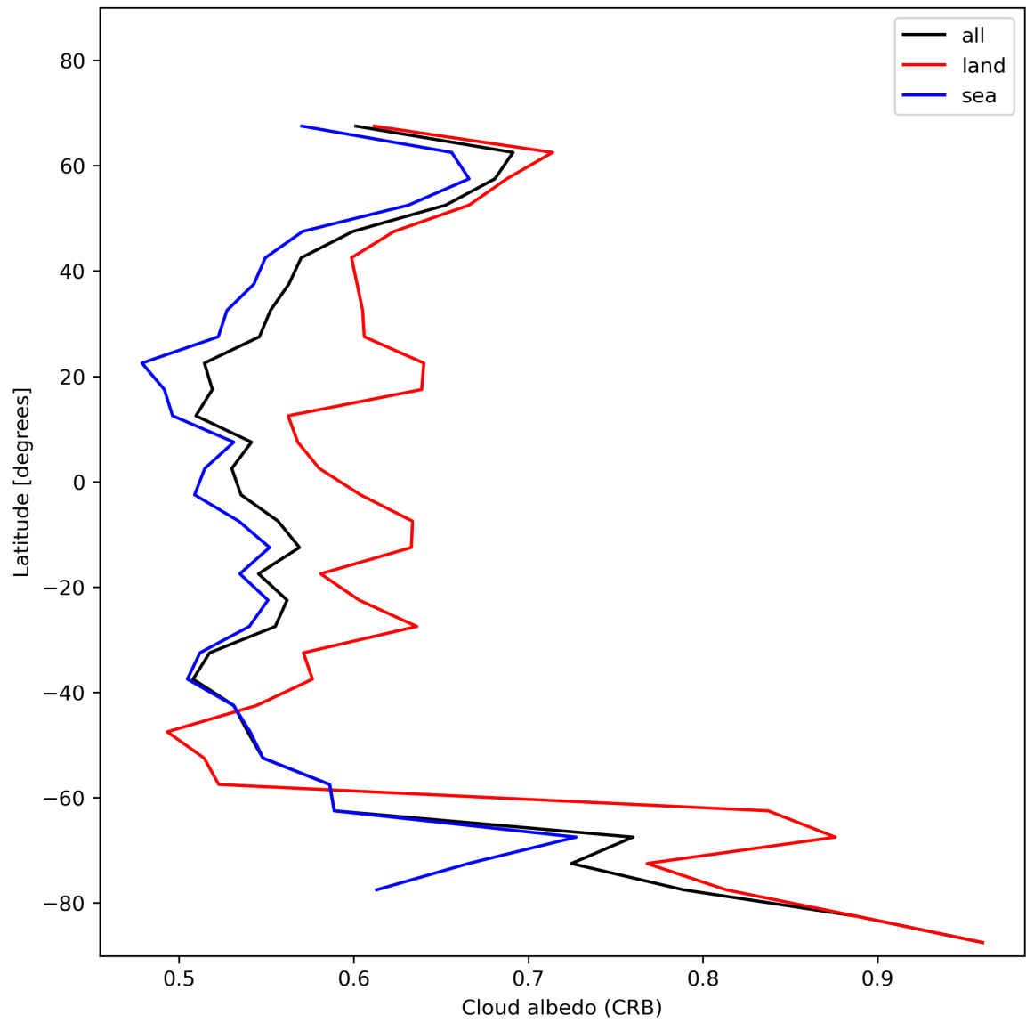
Figure 28: Zonal average of “Cloud albedo (CRB)” for 2023-11-25 to 2023-11-27.
