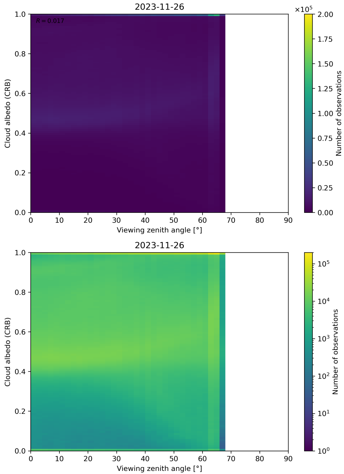
Figure 106: Scatter density plot of “Viewing zenith angle” against “Cloud albedo (CRB)” for 2023-11-25 to 2023-11-27.
