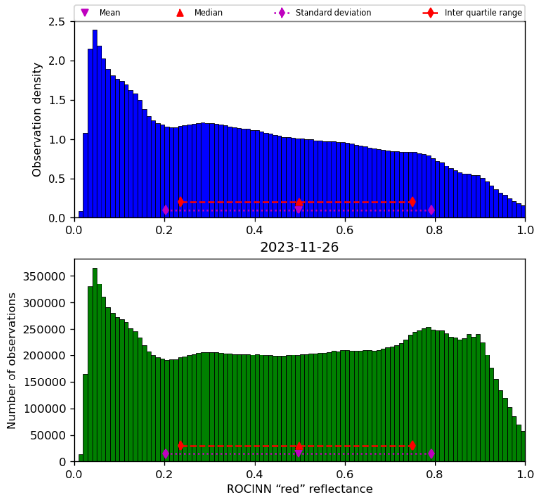
Figure 53: Histogram of “ROCINN “red” reflectance” for 2023-11-25 to 2023-11-27
