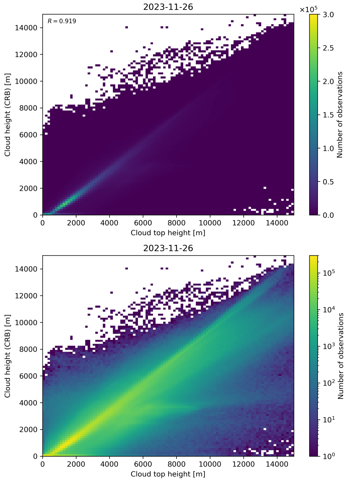
Figure 89: Scatter density plot of “Cloud top height” against “Cloud height (CRB)” for 2023-11-25 to 2023-11-27.
