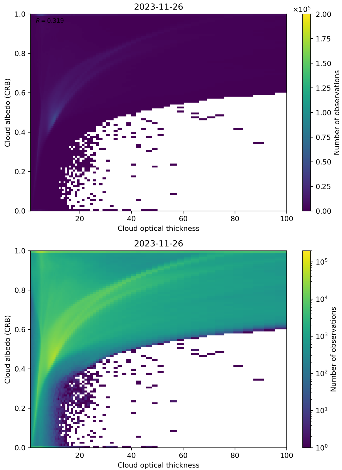
Figure 82: Scatter density plot of “Cloud optical thickness” against “Cloud albedo (CRB)” for 2023-11-25 to 2023-11-27.
