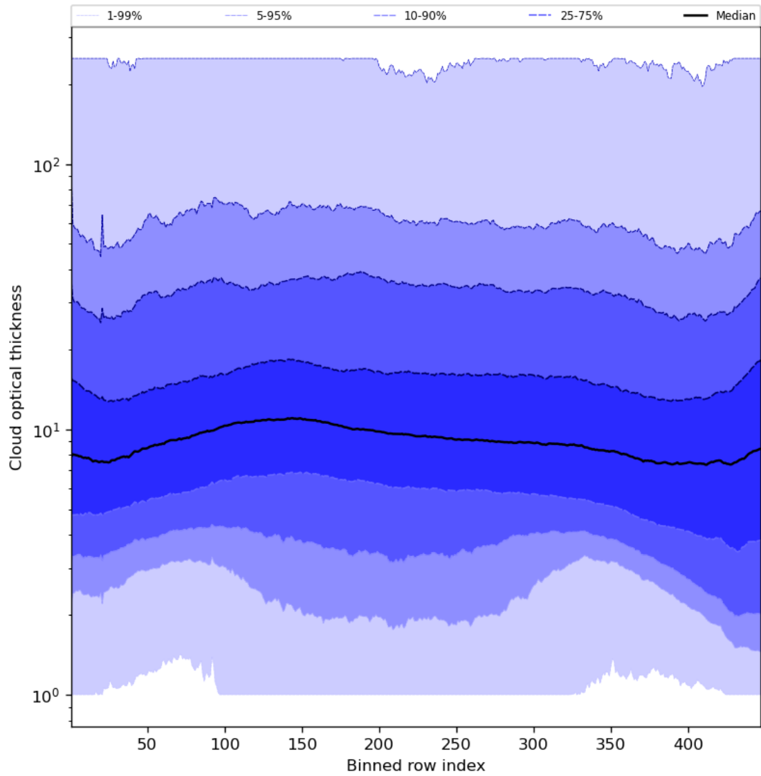
Figure 57: Along track statistics of “Cloud optical thickness” for 2023-11-25 to 2023-11-27
