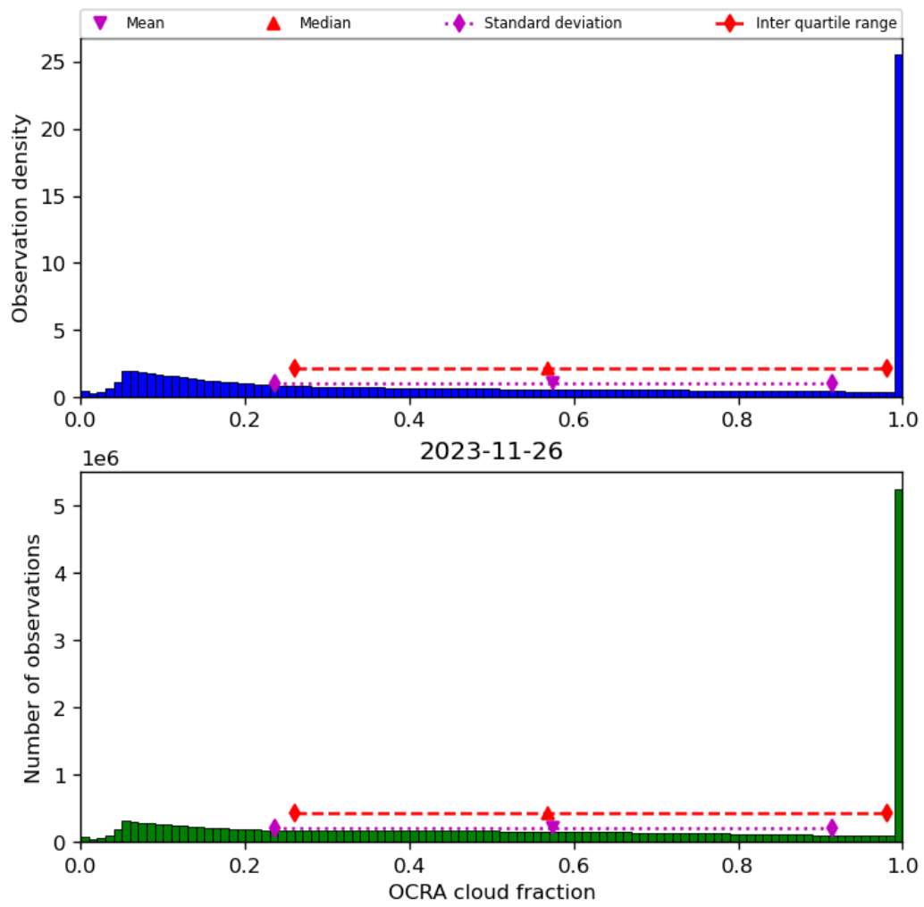
Figure 50: Histogram of “OCRA cloud fraction” for 2023-11-25 to 2023-11-27
