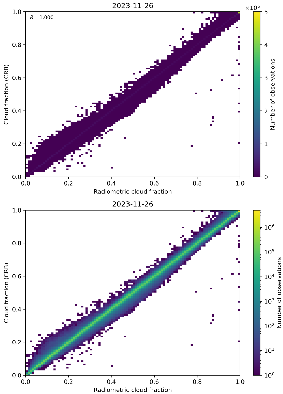
Figure 73: Scatter density plot of “Radiometric cloud fraction” against “Cloud fraction (CRB)” for 2023-11-25 to 2023-11-27.
