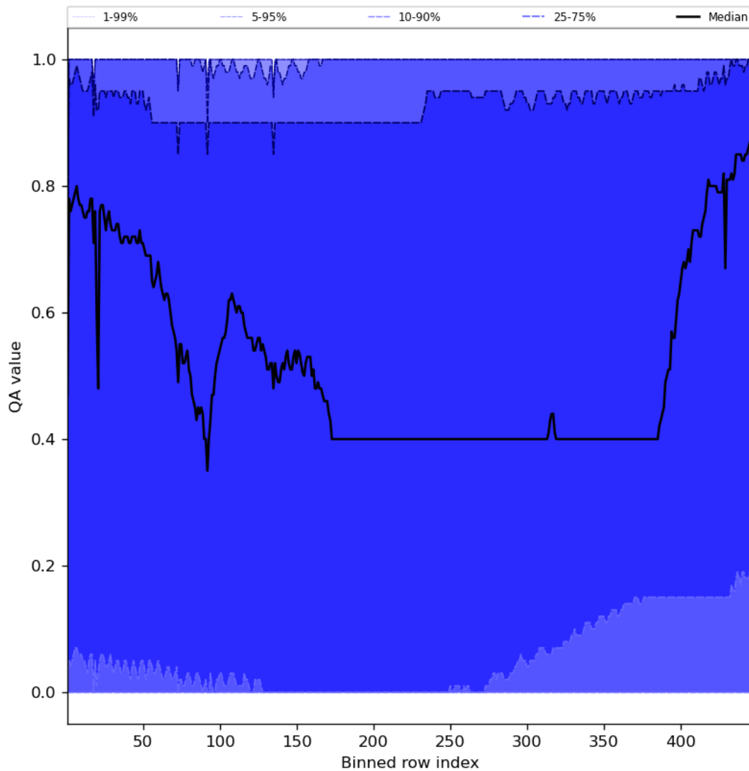
Figure 54: Along track statistics of “QA value” for 2023-11-25 to 2023-11-27
