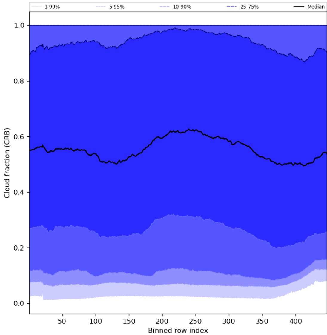
Figure 58: Along track statistics of “Cloud fraction (CRB)” for 2023-11-25 to 2023-11-27
