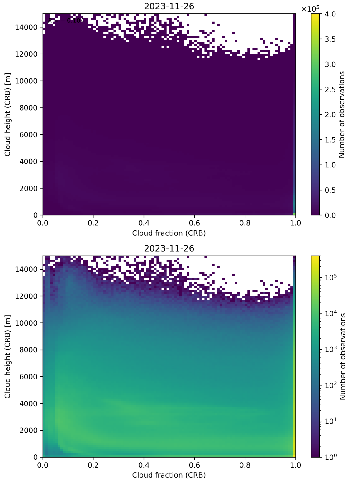
Figure 79: Scatter density plot of “Cloud fraction (CRB)” against “Cloud height (CRB)” for 2023-11-25 to 2023-11-27.
