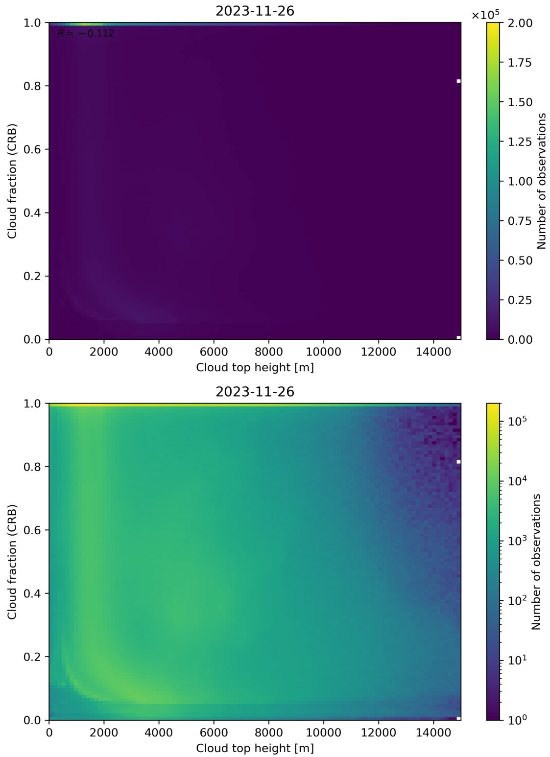
Figure 88: Scatter density plot of “Cloud top height” against “Cloud fraction (CRB)” for 2023-11-25 to 2023-11-27.
