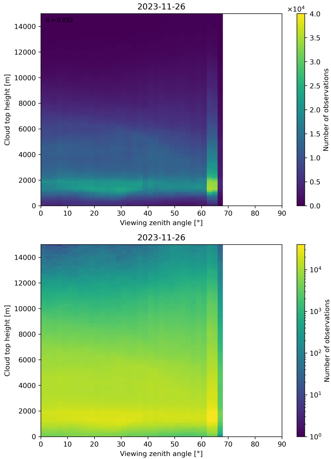
Figure 112: Scatter density plot of “Viewing zenith angle” against “Cloud top height” for 2023-11-25 to 2023-11-27.
