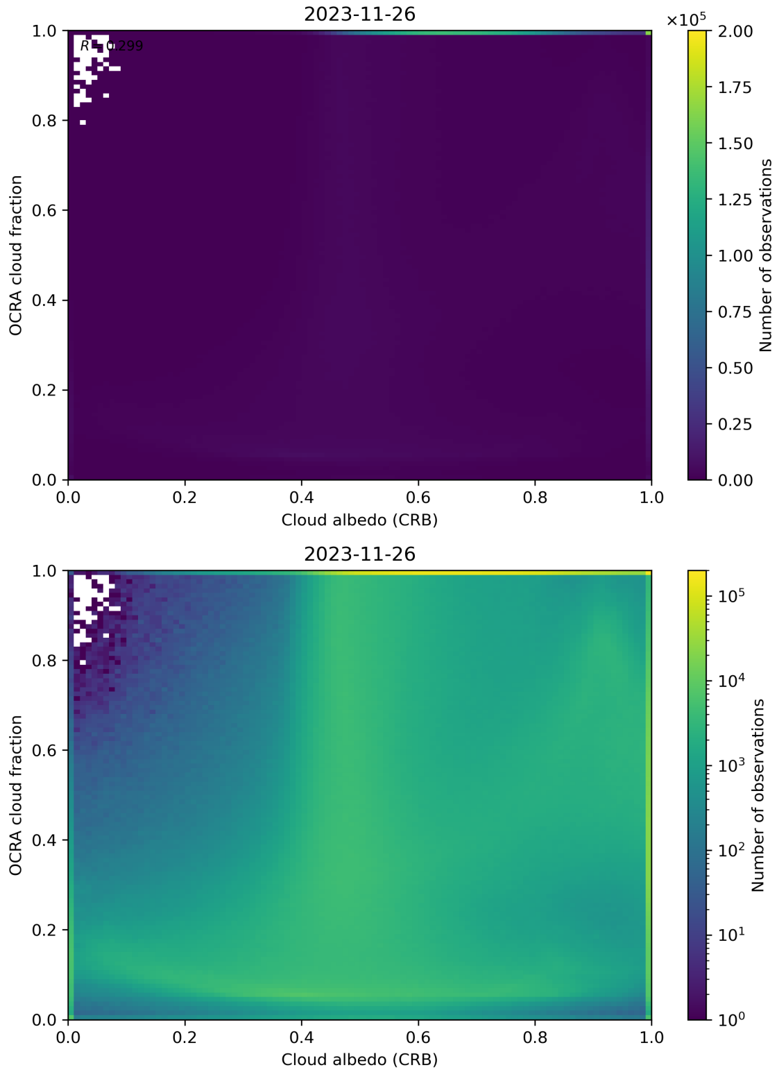
Figure 70: Scatter density plot of “Cloud albedo (CRB)” against “OCRA cloud fraction” for 2023-11-25 to 2023-11-27.
