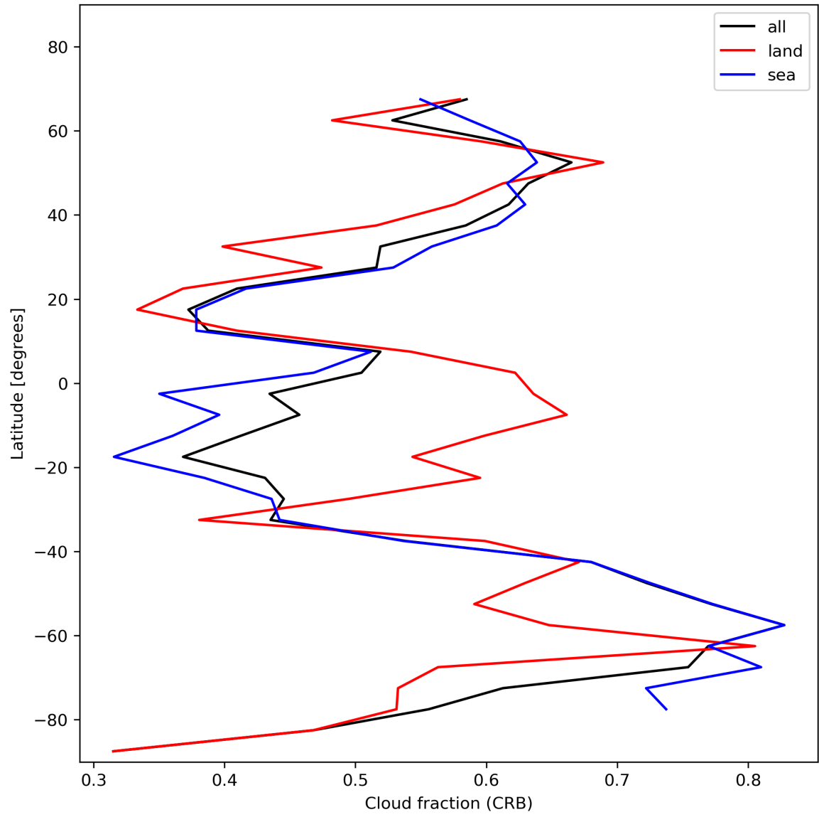
Figure 26: Zonal average of “Cloud fraction (CRB)” for 2023-11-25 to 2023-11-27.
