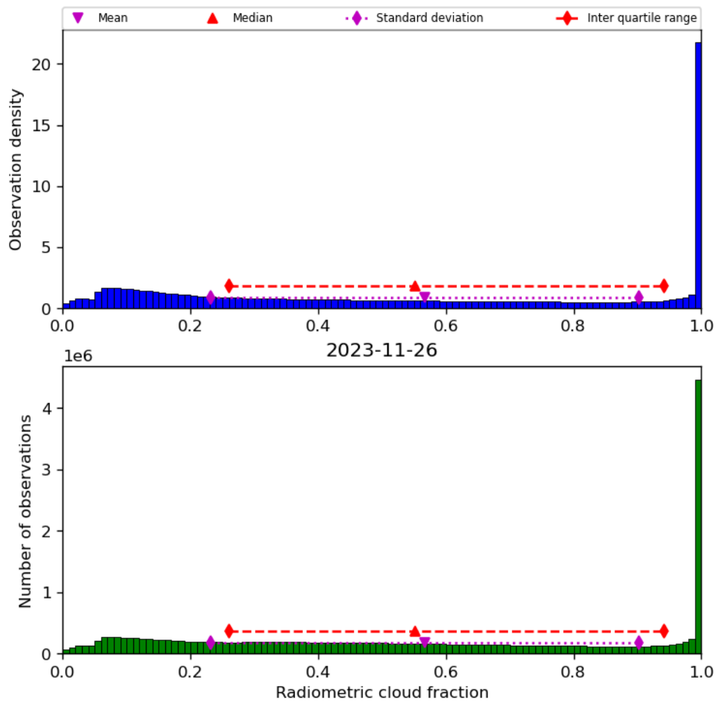
Figure 39: Histogram of “Radiometric cloud fraction” for 2023-11-25 to 2023-11-27
