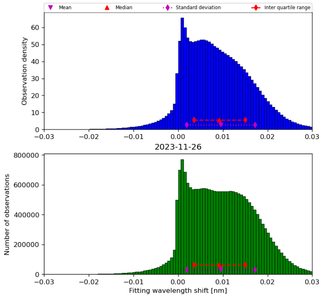
Figure 49: Histogram of “Fitting wavelength shift” for 2023-11-25 to 2023-11-27
