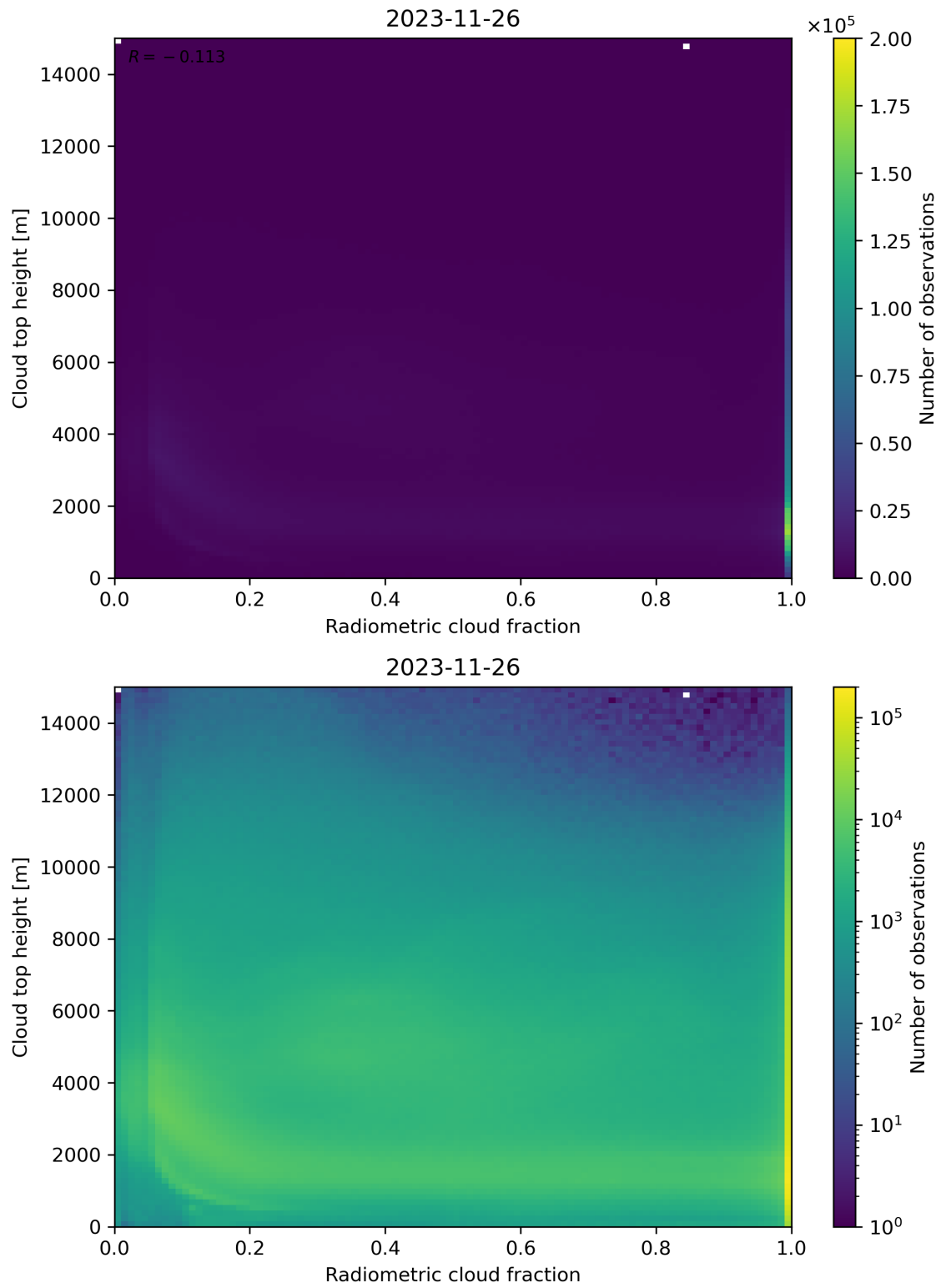
Figure 76: Scatter density plot of “Radiometric cloud fraction” against “Cloud top height” for 2023-11-25 to 2023-11-27.
