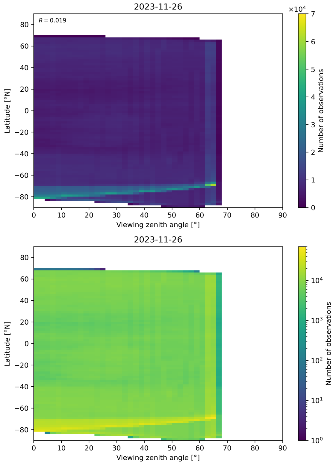
Figure 113: Scatter density plot of “Viewing zenith angle” against “Latitude” for 2023-11-25 to 2023-11-27.
