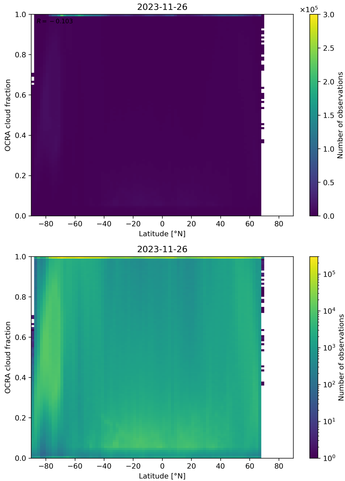
Figure 93: Scatter density plot of “Latitude” against “OCRA cloud fraction” for 2023-11-25 to 2023-11-27.
