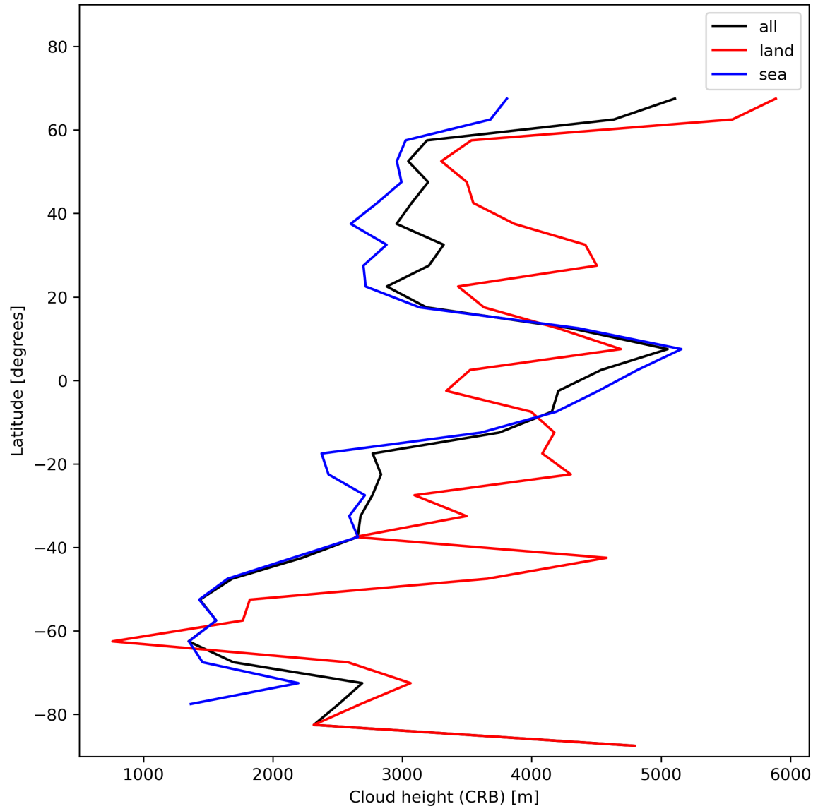
Figure 27: Zonal average of “Cloud height (CRB)” for 2023-11-25 to 2023-11-27.
