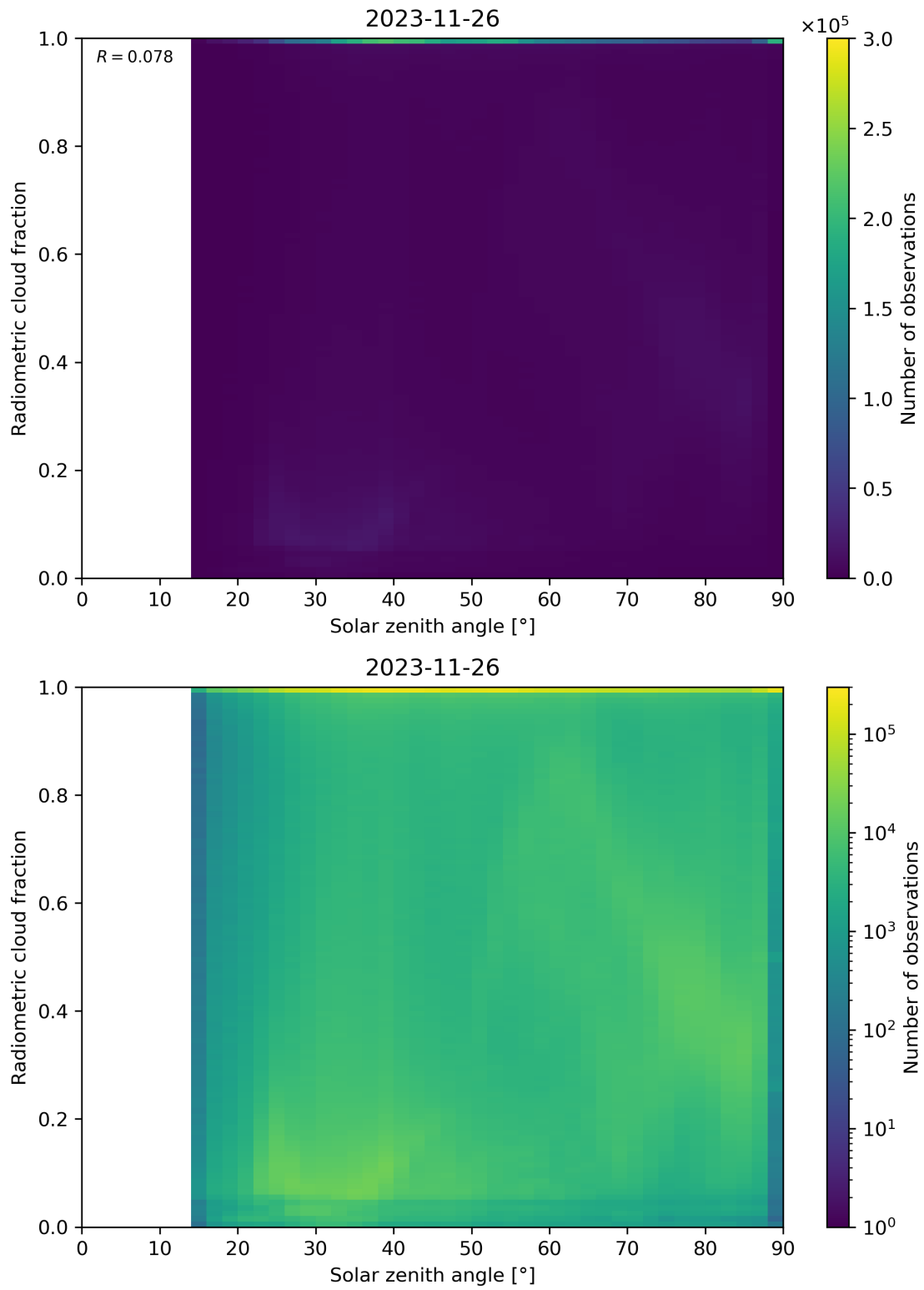
Figure 99: Scatter density plot of “Solar zenith angle” against “Radiometric cloud fraction” for 2023-11-25 to 2023-11-27.
