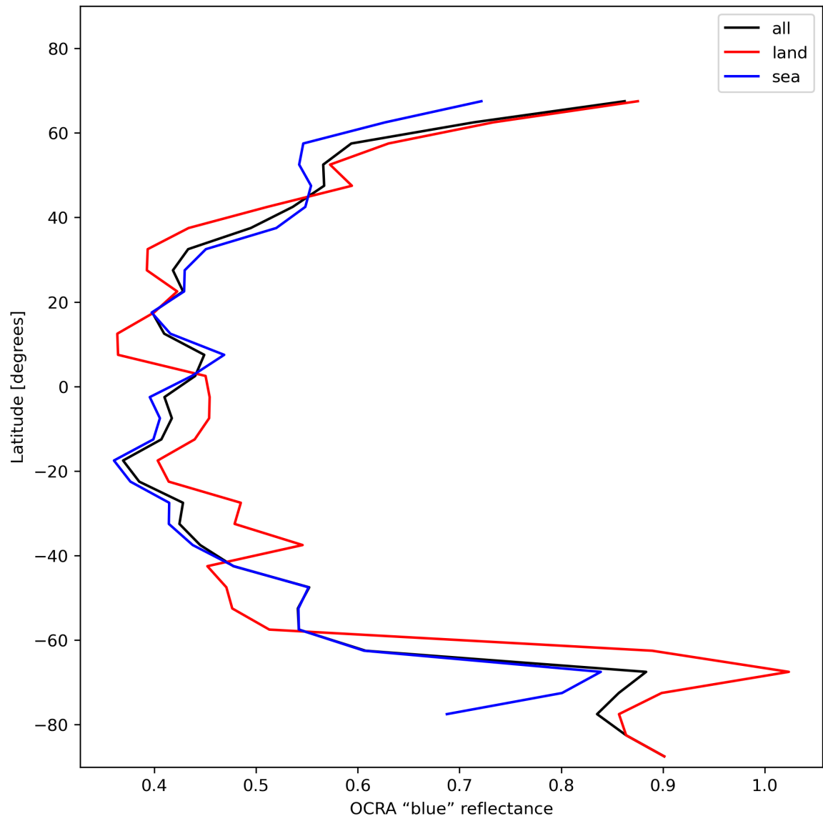
Figure 35: Zonal average of “OCRA “blue” reflectance” for 2023-11-28 to 2023-11-29.
