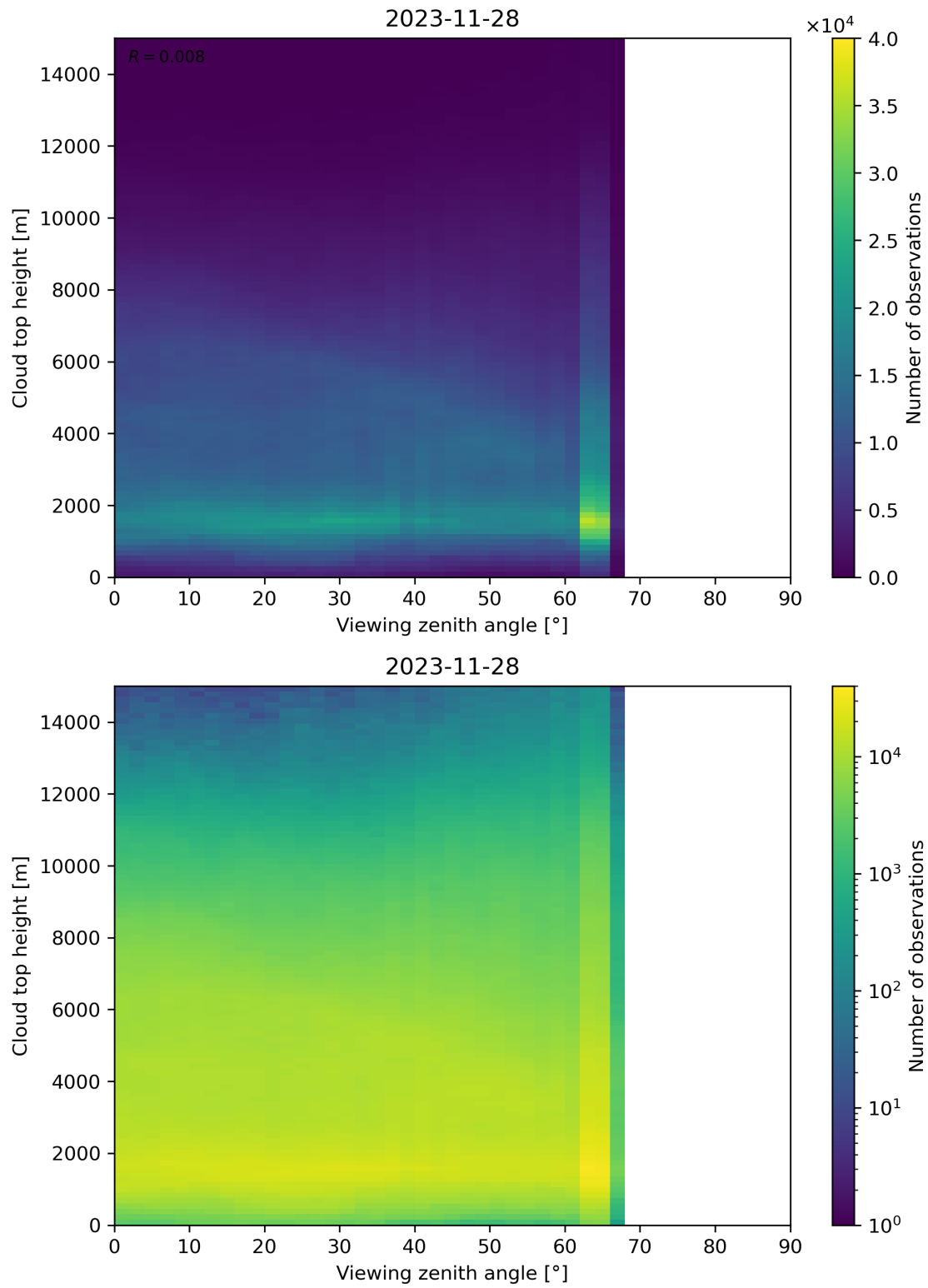
Figure 112: Scatter density plot of “Viewing zenith angle” against “Cloud top height” for 2023-11-28 to 2023-11-29.
