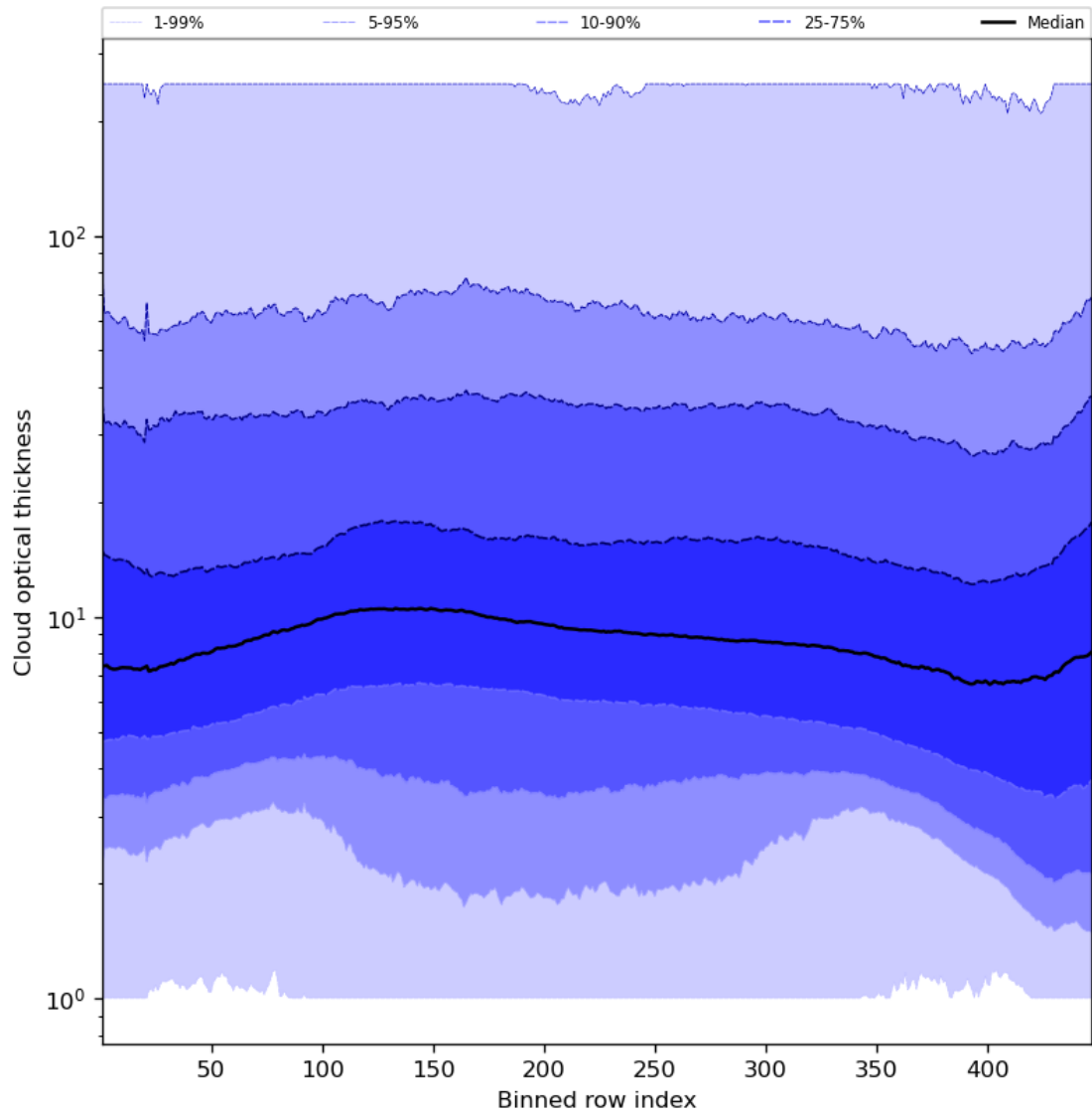
Figure 57: Along track statistics of “Cloud optical thickness” for 2023-11-28 to 2023-11-29
