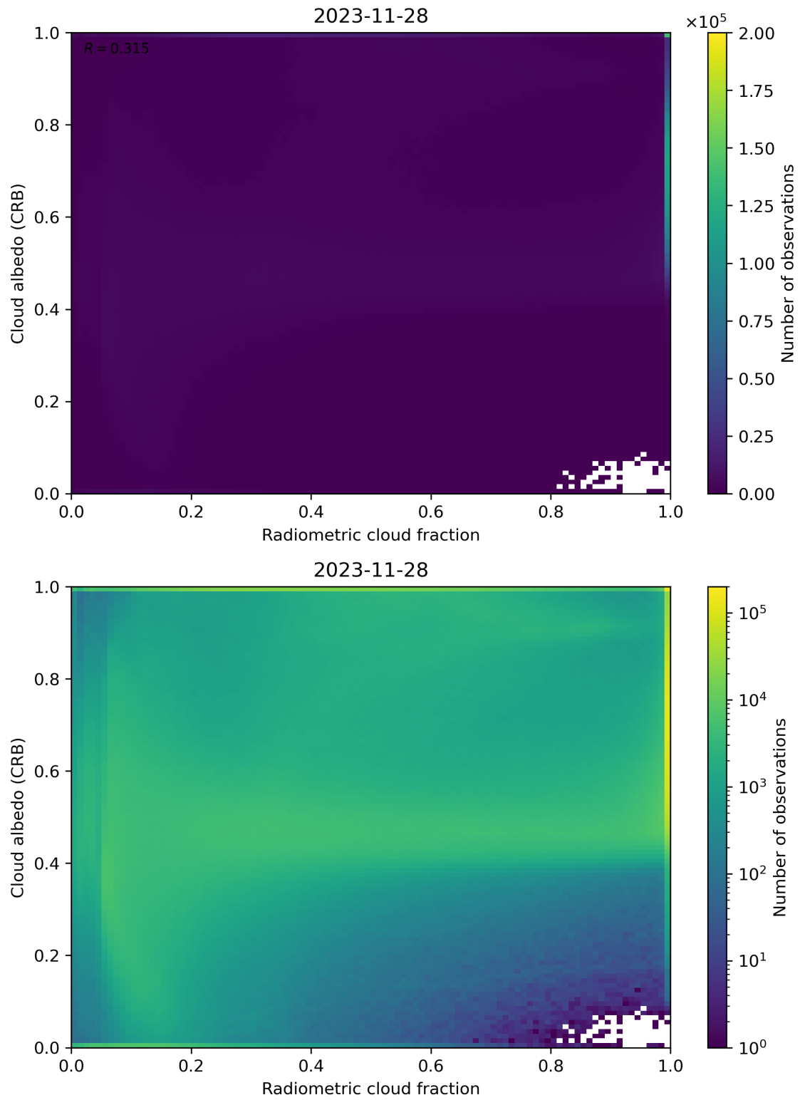
Figure 71: Scatter density plot of “Radiometric cloud fraction” against “Cloud albedo (CRB)” for 2023-11-28 to 2023-11-29.
