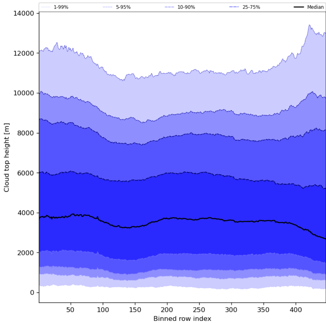
Figure 56: Along track statistics of “Cloud top height” for 2023-11-28 to 2023-11-29
