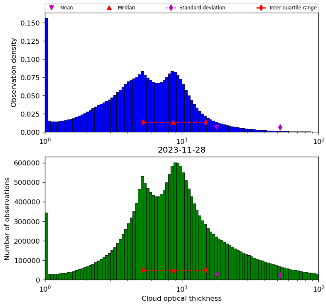
Figure 41: Histogram of “Cloud optical thickness” for 2023-11-28 to 2023-11-29
