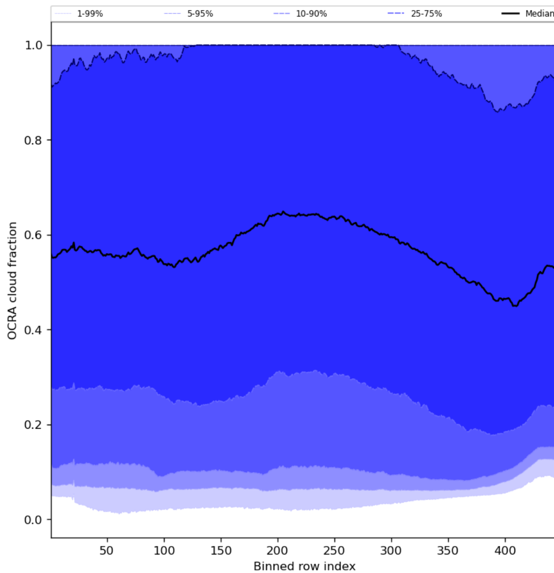
Figure 66: Along track statistics of “OCRA cloud fraction” for 2023-11-28 to 2023-11-29
