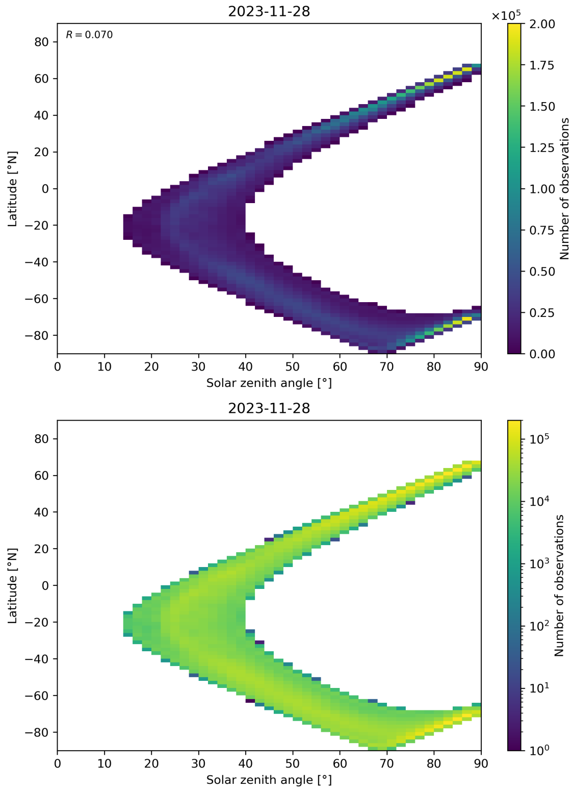
Figure 105: Scatter density plot of “Solar zenith angle” against “Latitude” for 2023-11-28 to 2023-11-29.
