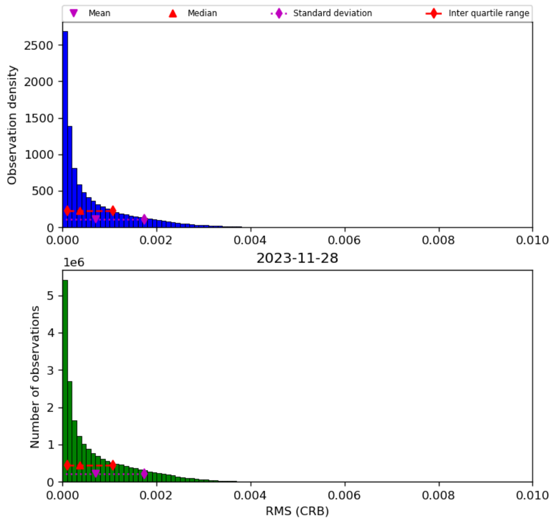
Figure 48: Histogram of "RMS (CRB)" for 2023-11-28 to 2023-11-29
