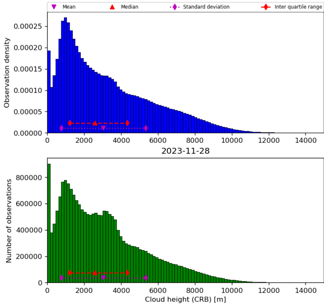
Figure 43: Histogram of “Cloud height (CRB)” for 2023-11-28 to 2023-11-29
