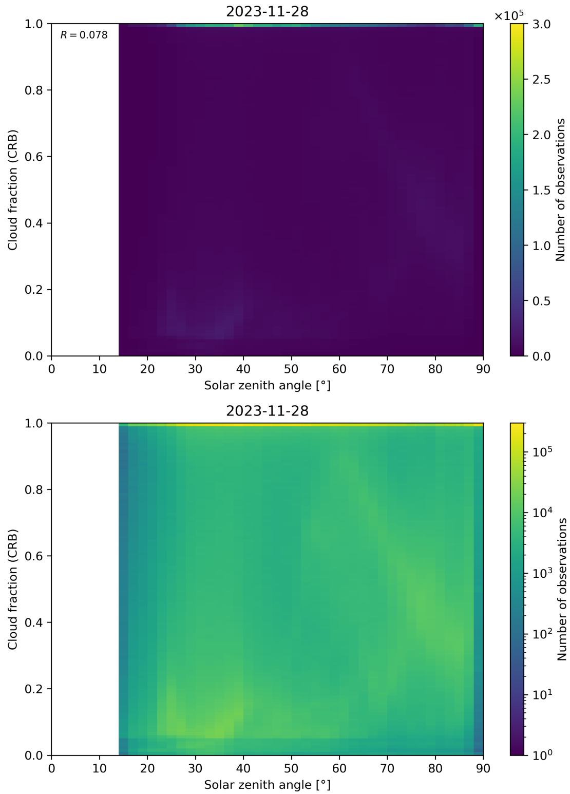
Figure 101: Scatter density plot of “Solar zenith angle” against “Cloud fraction (CRB)” for 2023-11-28 to 2023-11-29.
