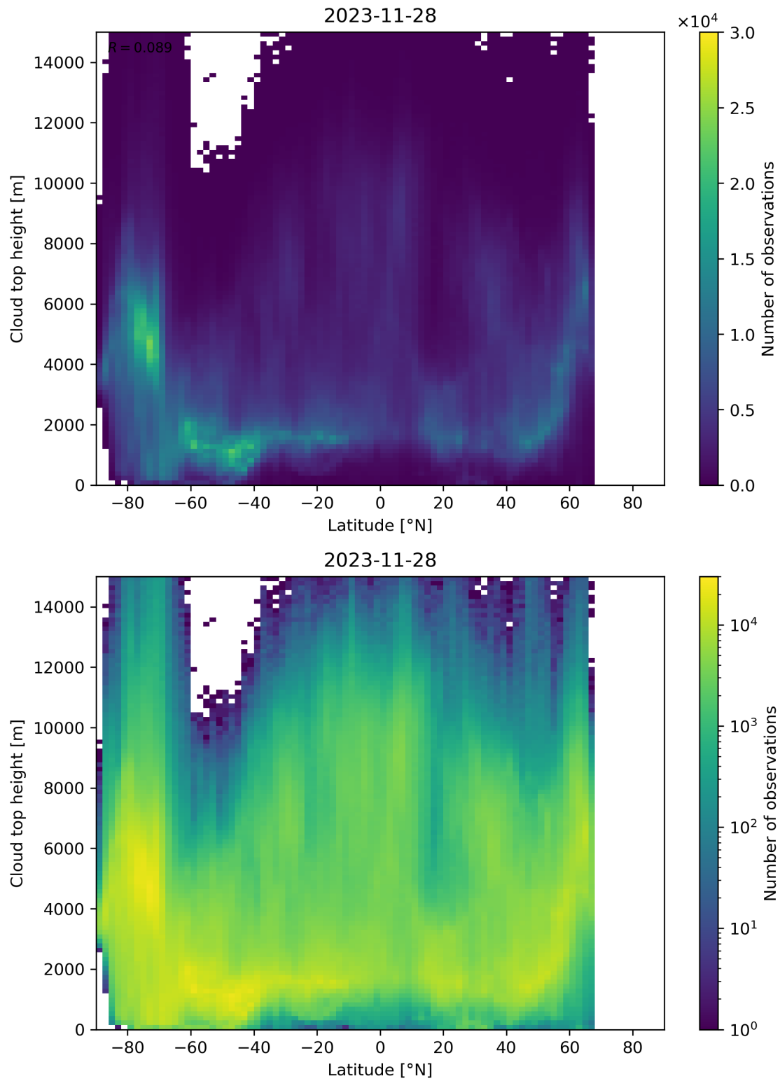
Figure 97: Scatter density plot of “Latitude” against “Cloud top height” for 2023-11-28 to 2023-11-29.
