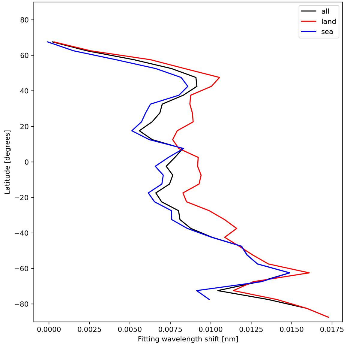
Figure 33: Zonal average of “Fitting wavelength shift” for 2023-11-28 to 2023-11-29.
