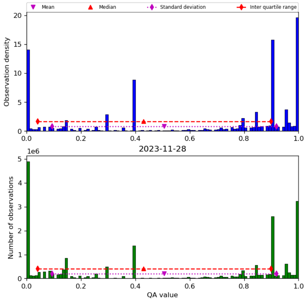
Figure 38: Histogram of “QA value” for 2023-11-28 to 2023-11-29
