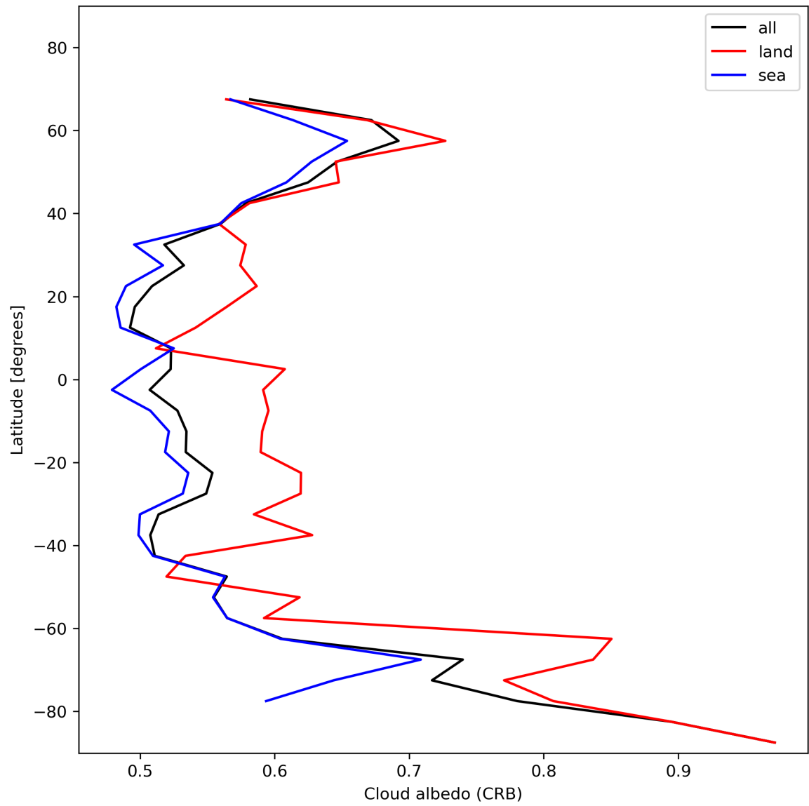
Figure 28: Zonal average of “Cloud albedo (CRB)” for 2023-11-28 to 2023-11-29.
