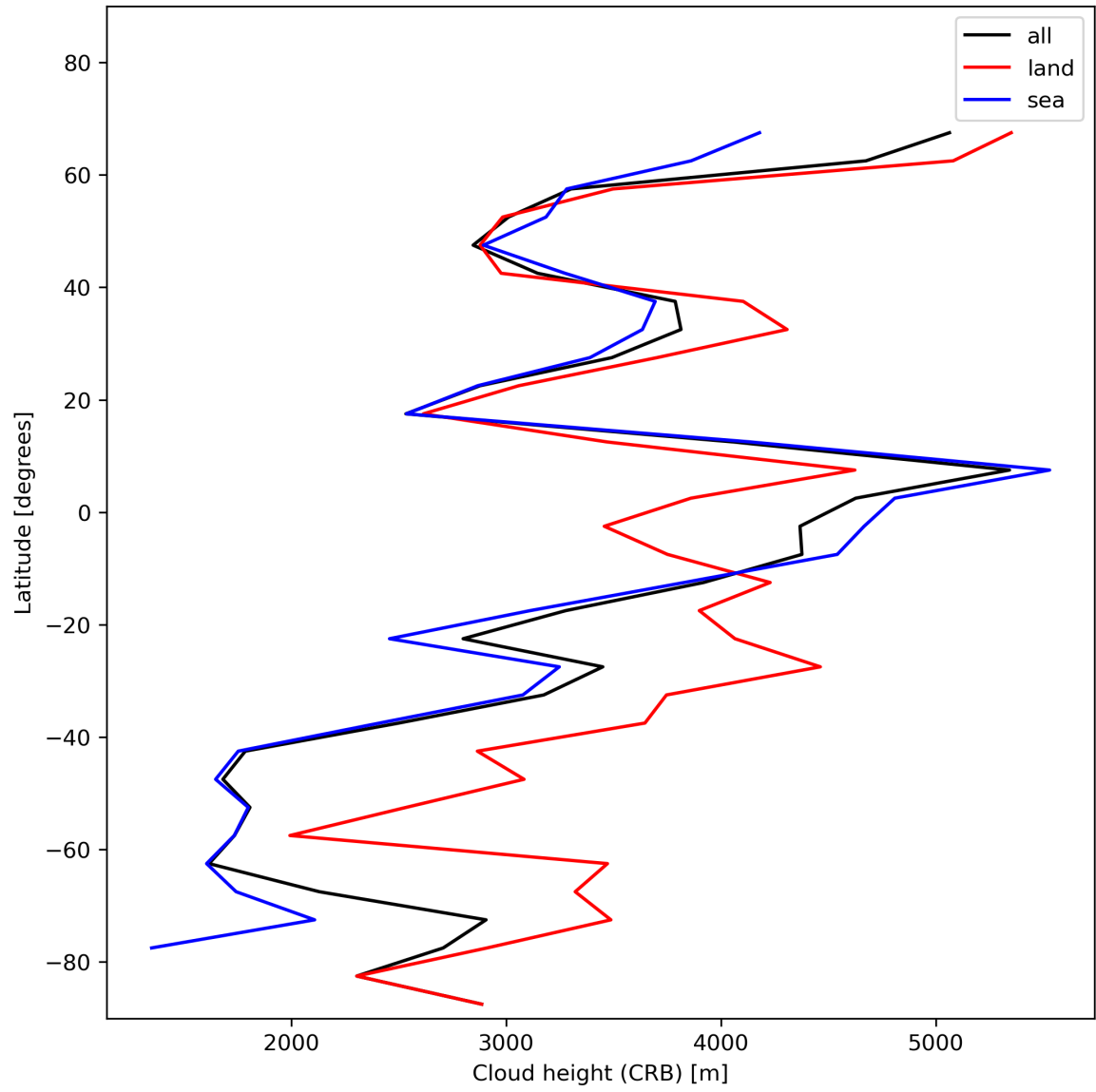
Figure 27: Zonal average of “Cloud height (CRB)” for 2023-11-28 to 2023-11-29.
