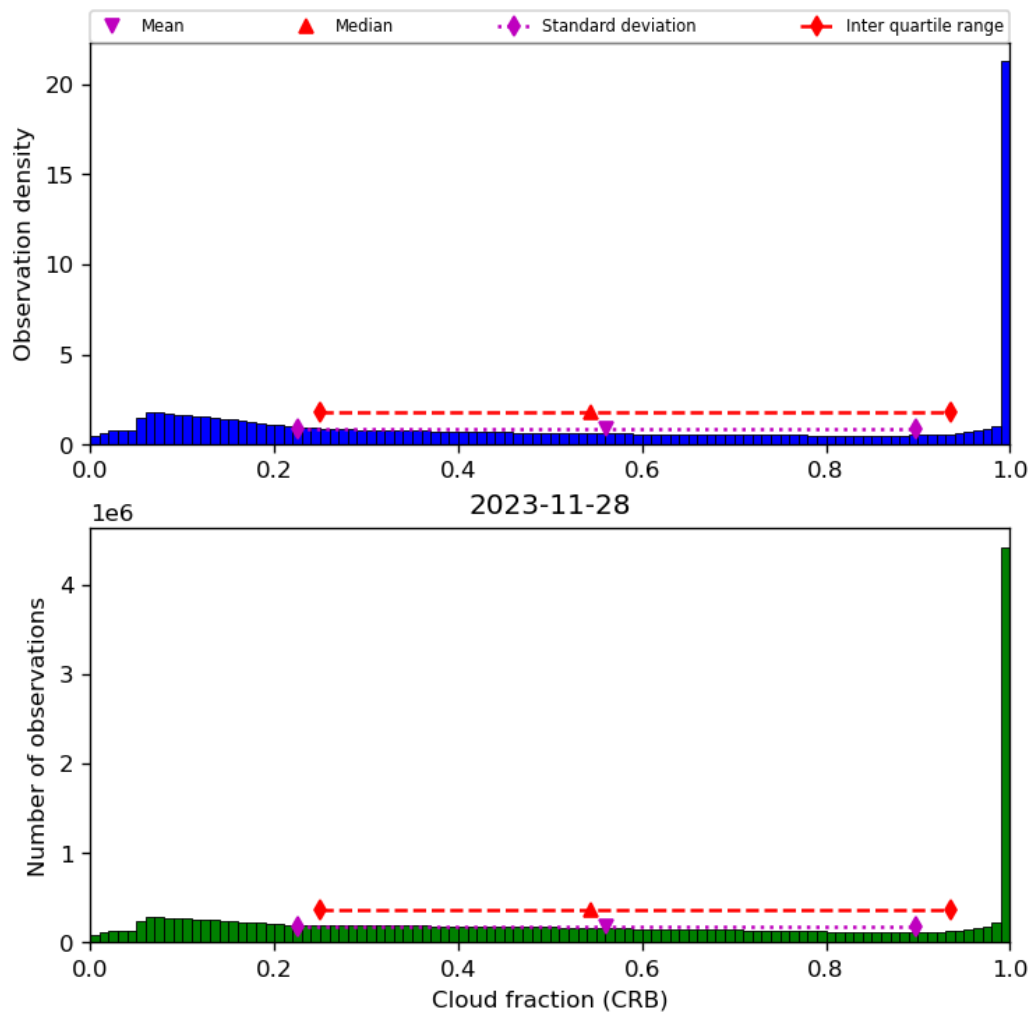
Figure 42: Histogram of “Cloud fraction (CRB)” for 2023-11-28 to 2023-11-29
