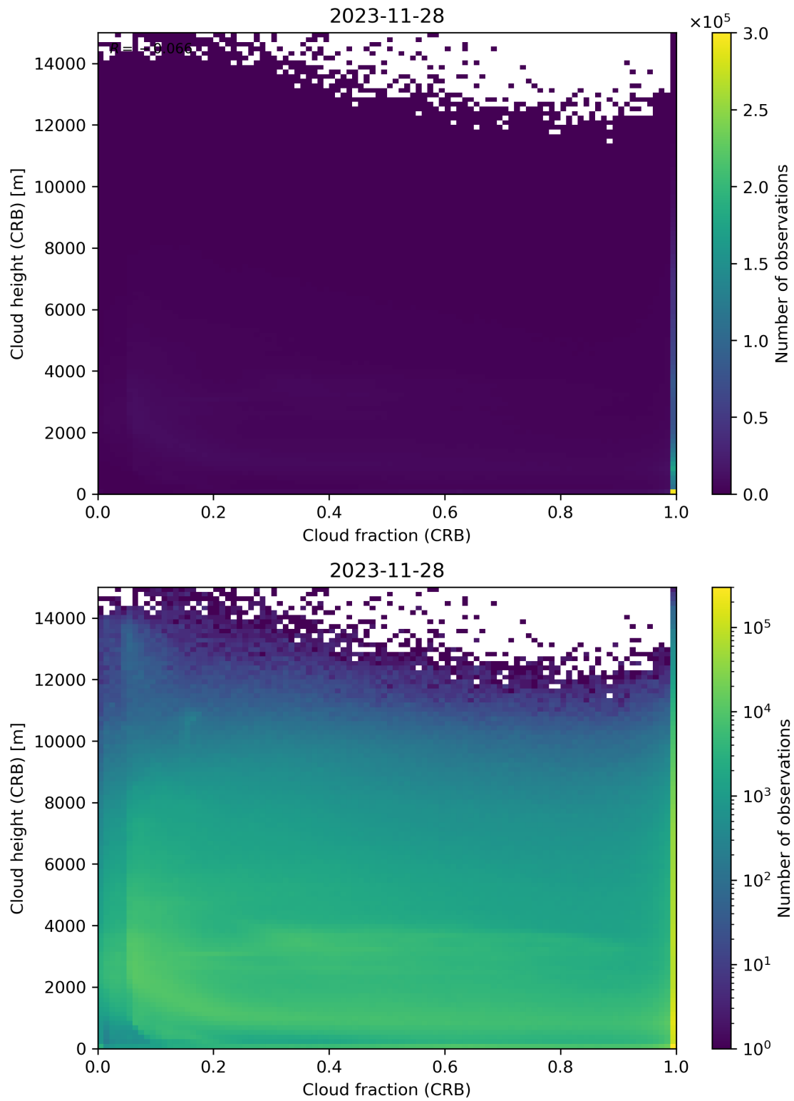
Figure 79: Scatter density plot of “Cloud fraction (CRB)” against “Cloud height (CRB)” for 2023-11-28 to 2023-11-29.
