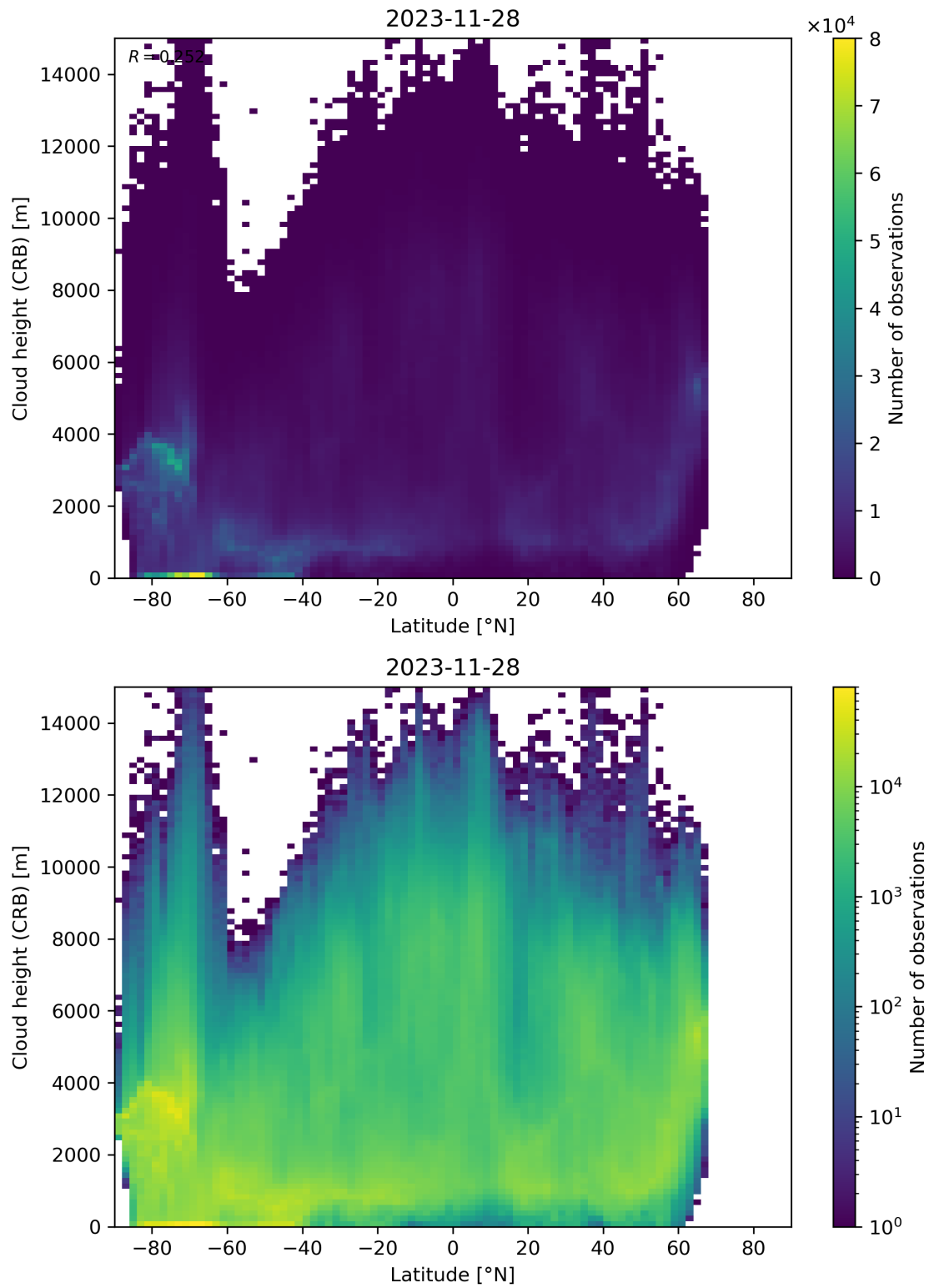
Figure 95: Scatter density plot of “Latitude” against “Cloud height (CRB)” for 2023-11-28 to 2023-11-29.
