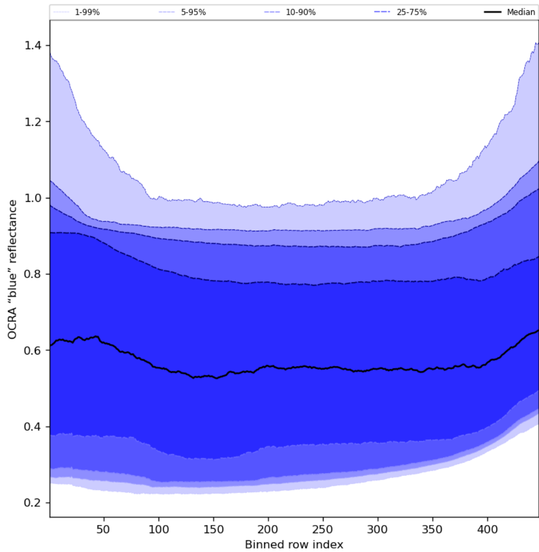
Figure 67: Along track statistics of “OCRA “blue” reflectance” for 2023-11-28 to 2023-11-29
