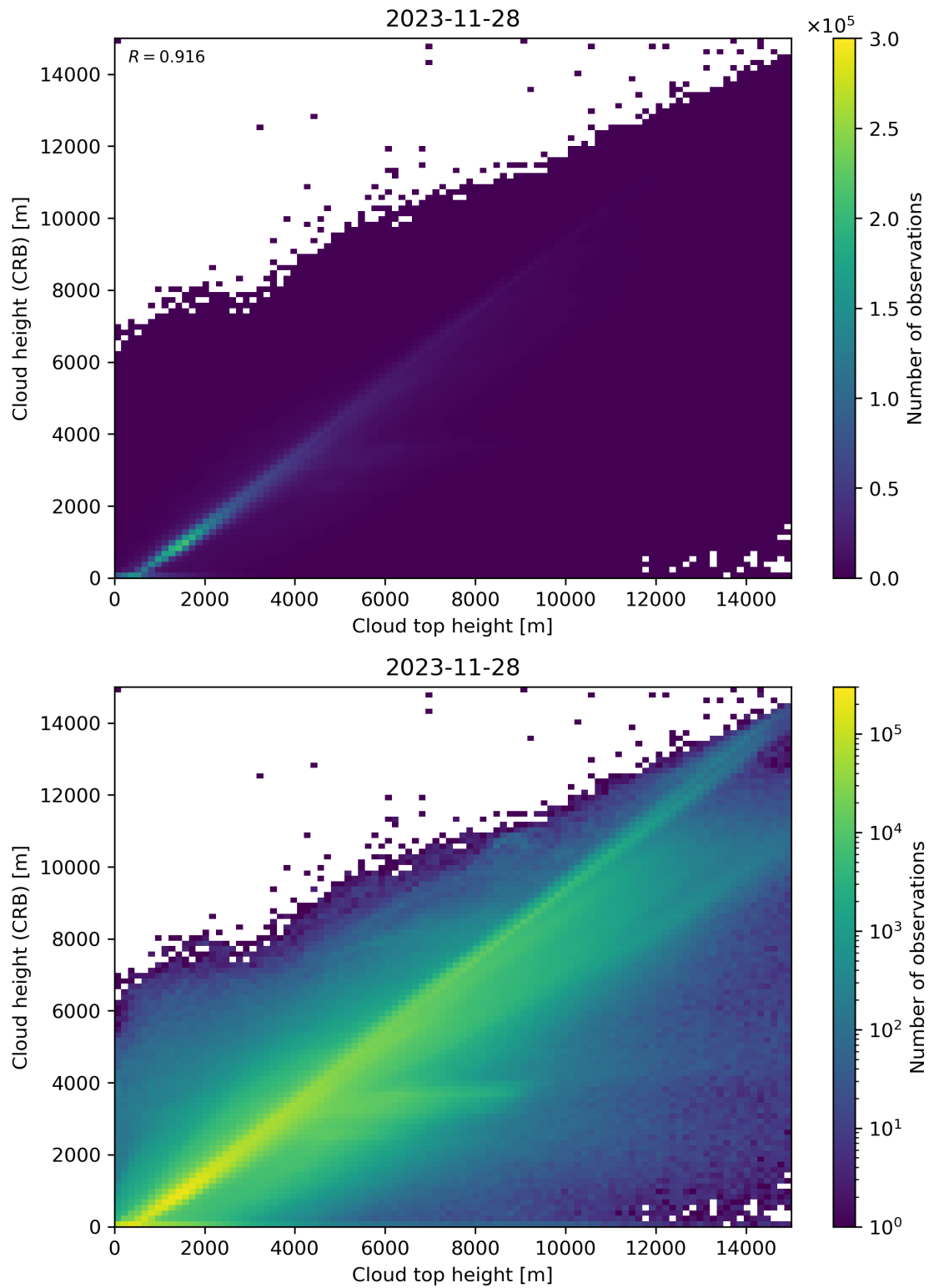
Figure 89: Scatter density plot of “Cloud top height” against “Cloud height (CRB)” for 2023-11-28 to 2023-11-29.
