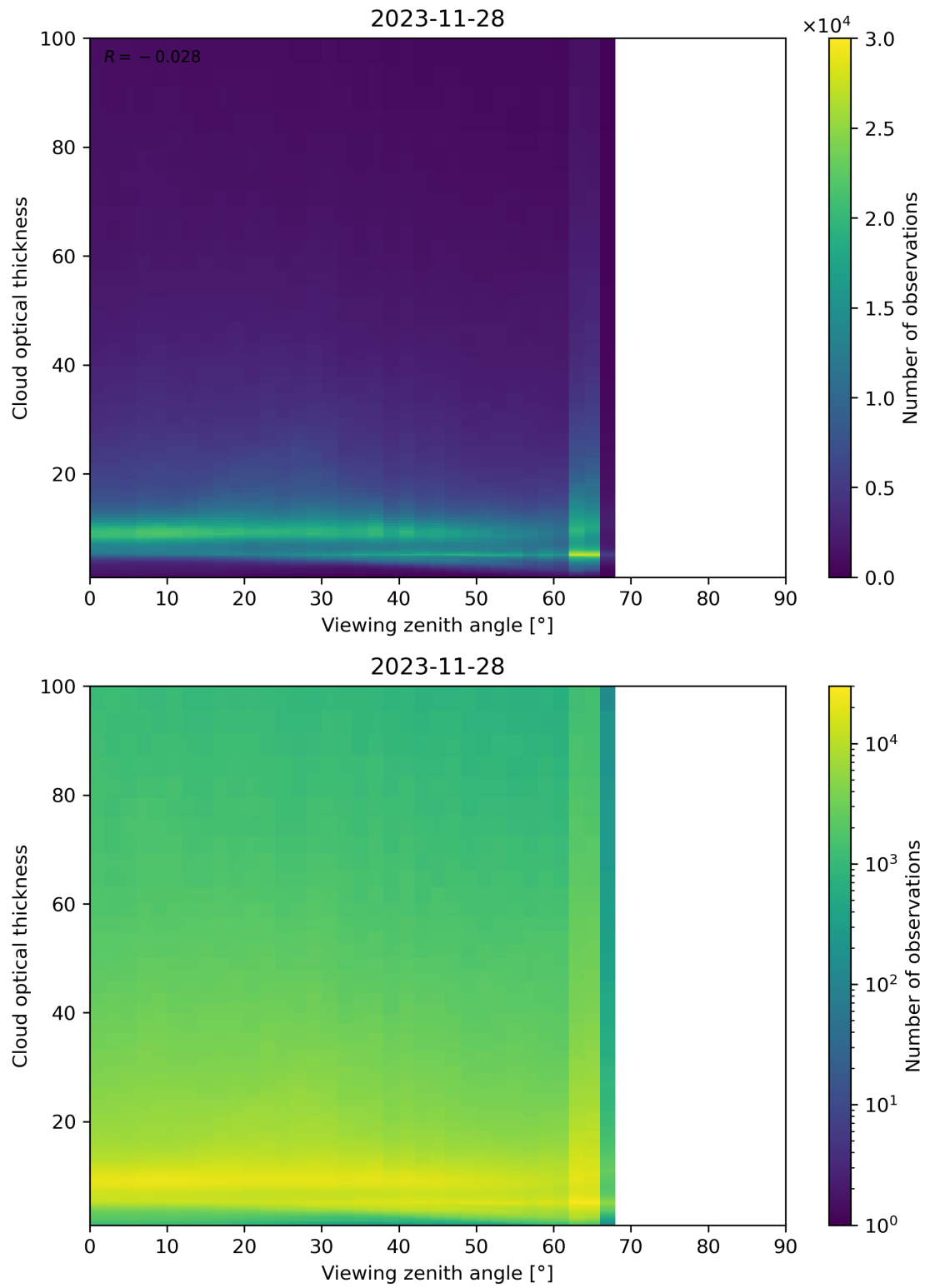
Figure 111: Scatter density plot of “Viewing zenith angle” against “Cloud optical thickness” for 2023-11-28 to 2023-11-29.
