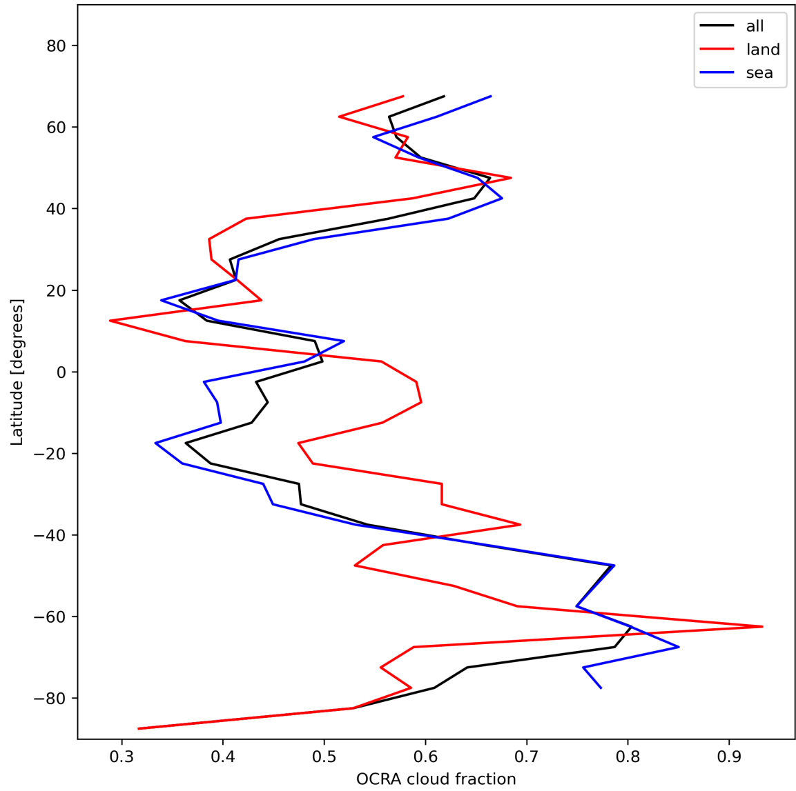
Figure 34: Zonal average of “OCRA cloud fraction” for 2023-11-28 to 2023-11-29.
