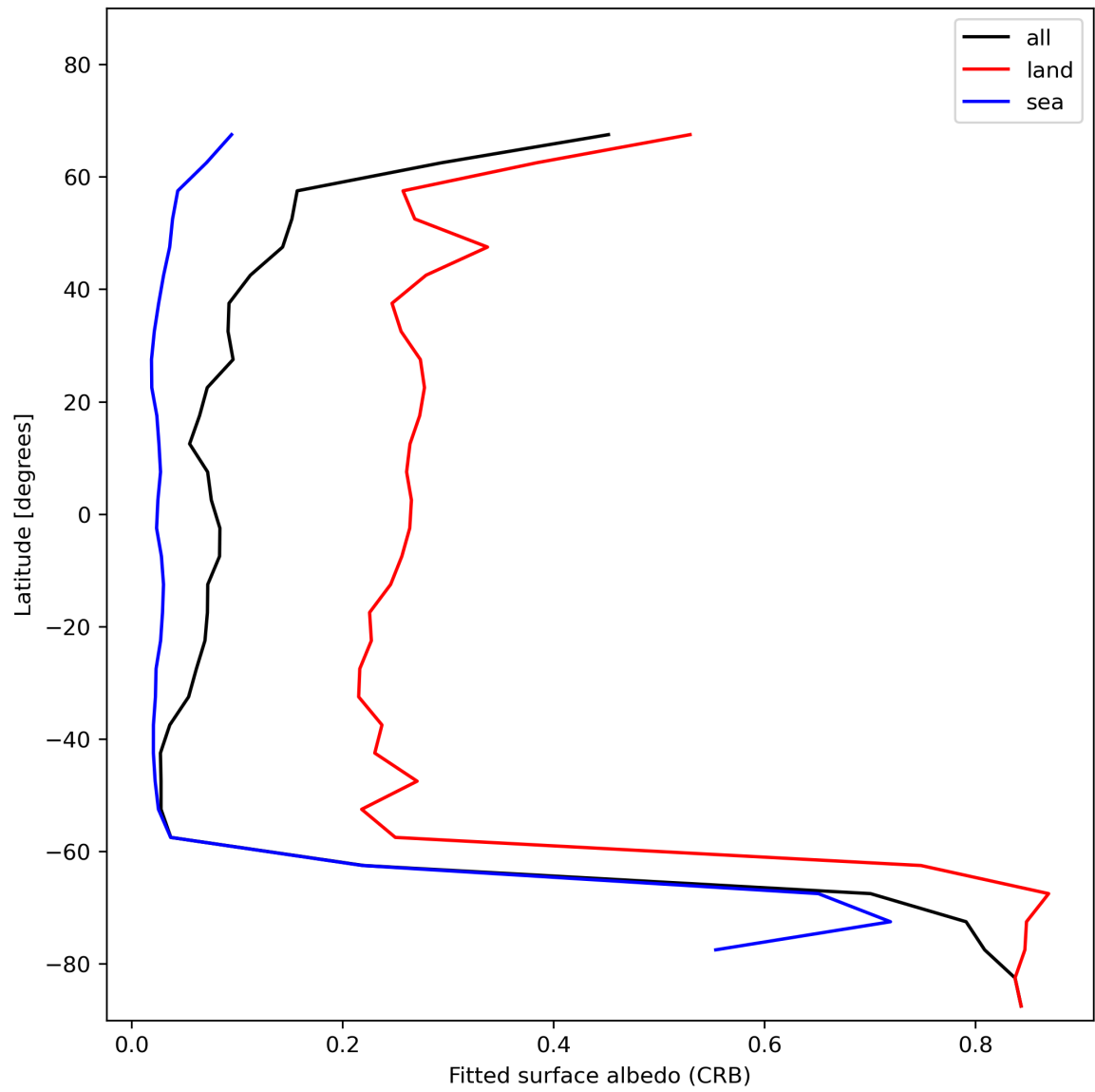
Figure 30: Zonal average of “Fitted surface albedo (CRB)” for 2023-11-28 to 2023-11-29.
