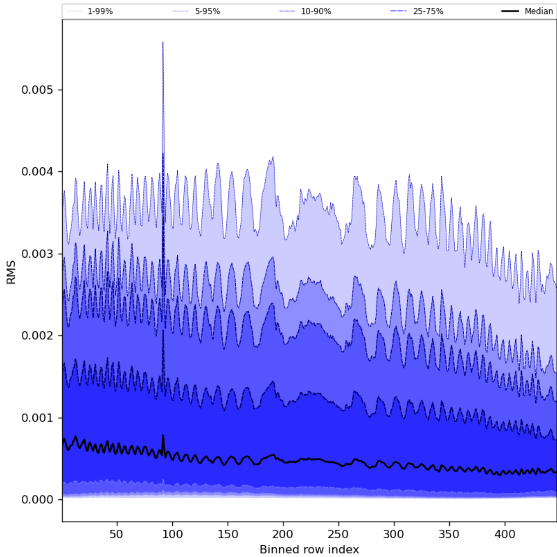
Figure 63: Along track statistics of “RMS” for 2023-11-28 to 2023-11-29
