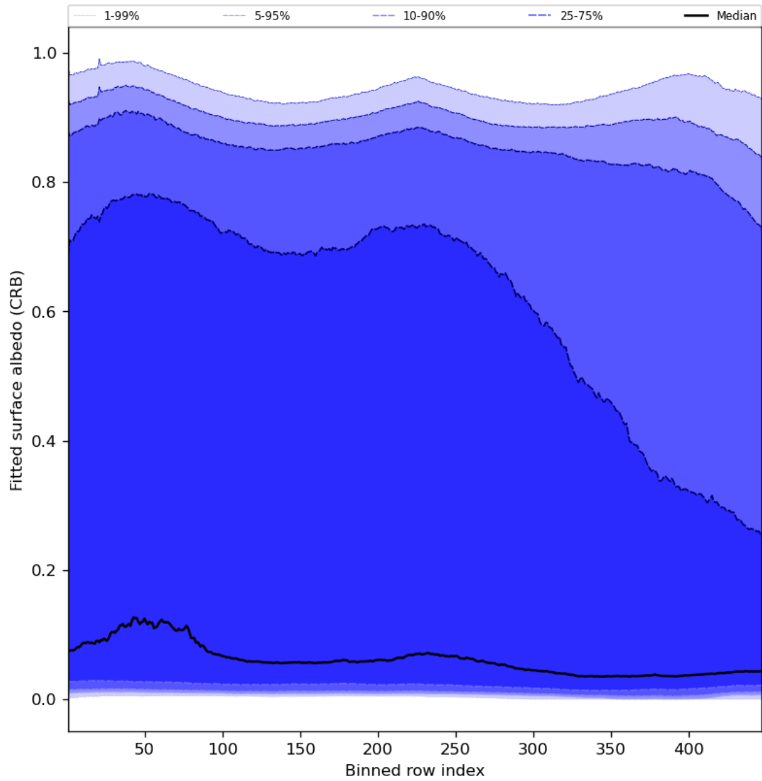
Figure 62: Along track statistics of “Fitted surface albedo (CRB)” for 2023-11-28 to 2023-11-29
