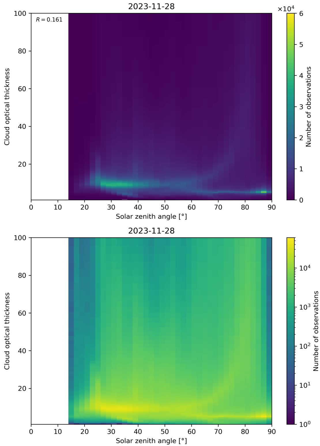
Figure 103: Scatter density plot of “Solar zenith angle” against “Cloud optical thickness” for 2023-11-28 to 2023-11-29.
