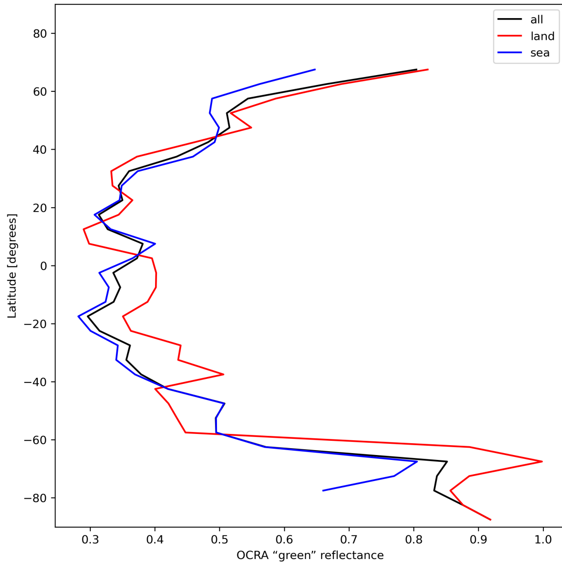
Figure 36: Zonal average of “OCRA “green” reflectance” for 2023-11-28 to 2023-11-29.
