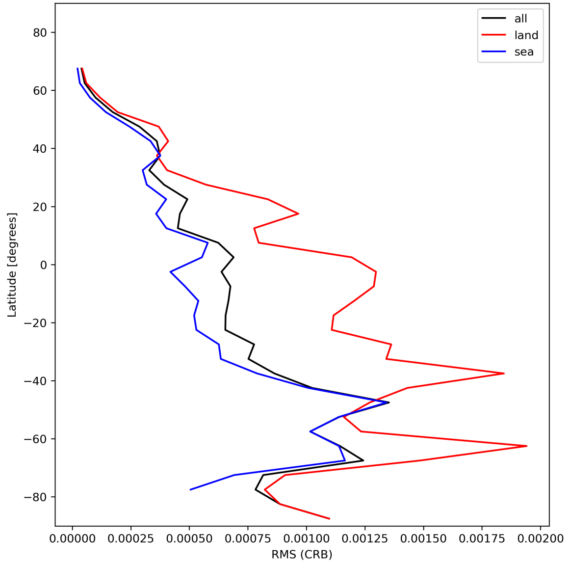
Figure 32: Zonal average of “RMS (CRB)” for 2023-11-28 to 2023-11-29.
