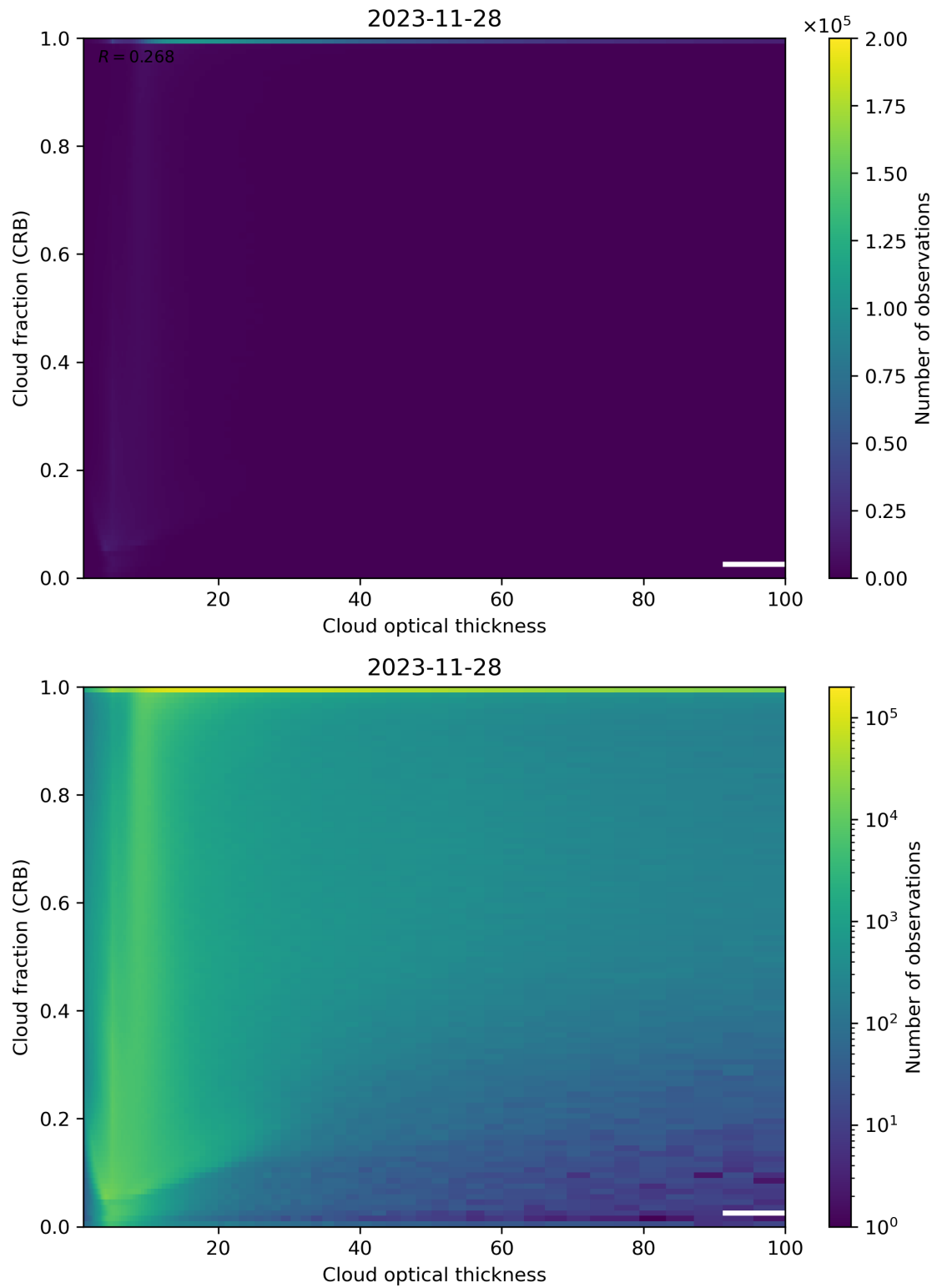
Figure 84: Scatter density plot of “Cloud optical thickness” against “Cloud fraction (CRB)” for 2023-11-28 to 2023-11-29.
