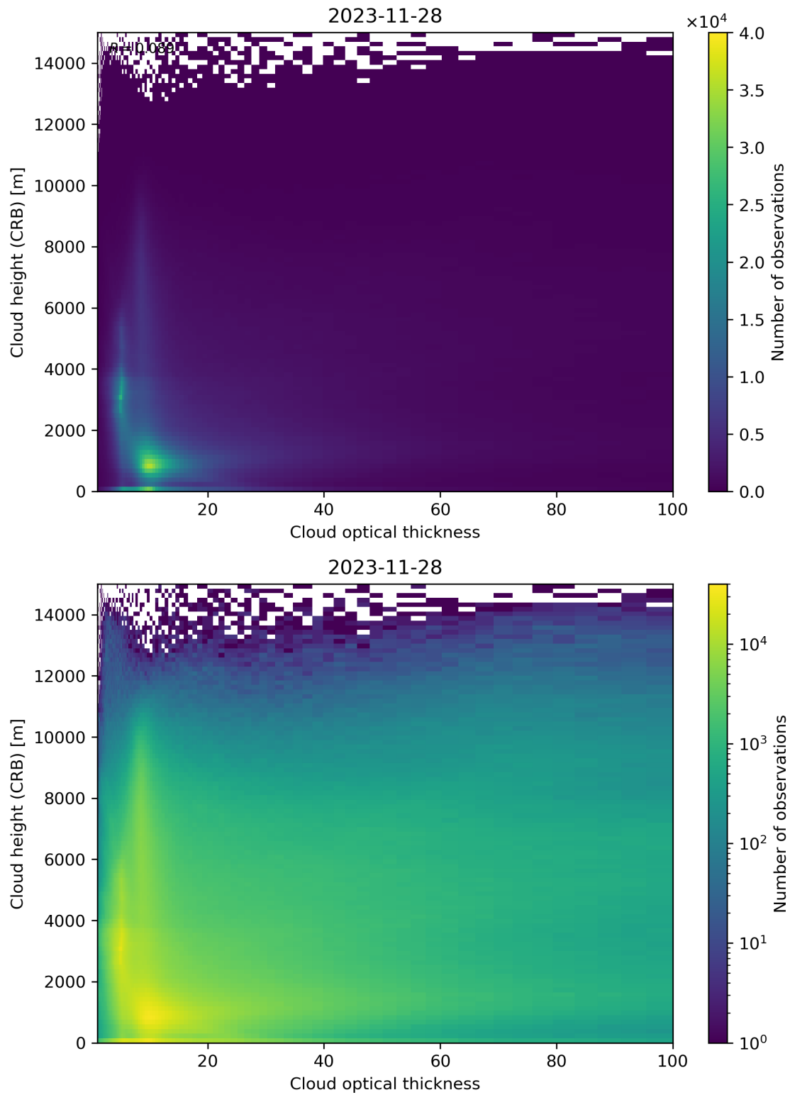
Figure 85: Scatter density plot of “Cloud optical thickness” against “Cloud height (CRB)” for 2023-11-28 to 2023-11-29.
