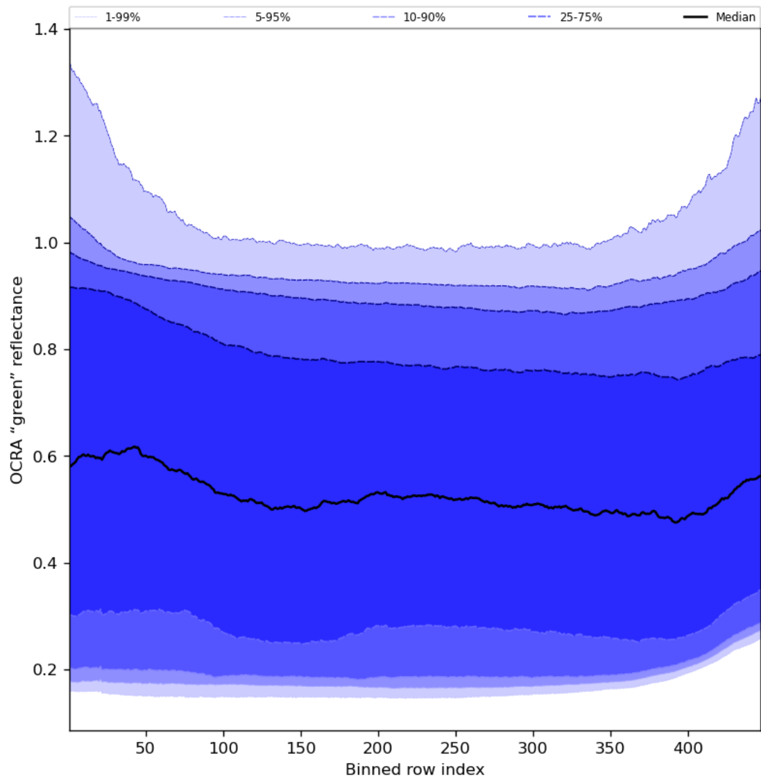
Figure 68: Along track statistics of “OCRA “green” reflectance” for 2023-11-28 to 2023-11-29
