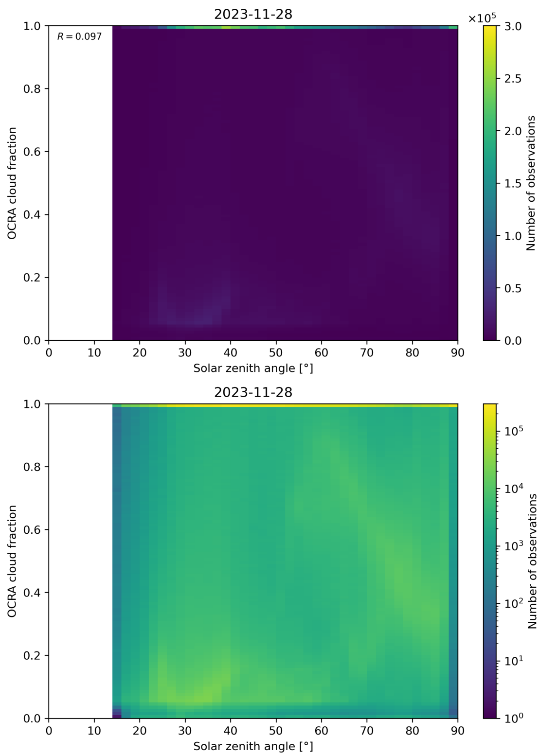
Figure 100: Scatter density plot of “Solar zenith angle” against “OCRA cloud fraction” for 2023-11-28 to 2023-11-29.
