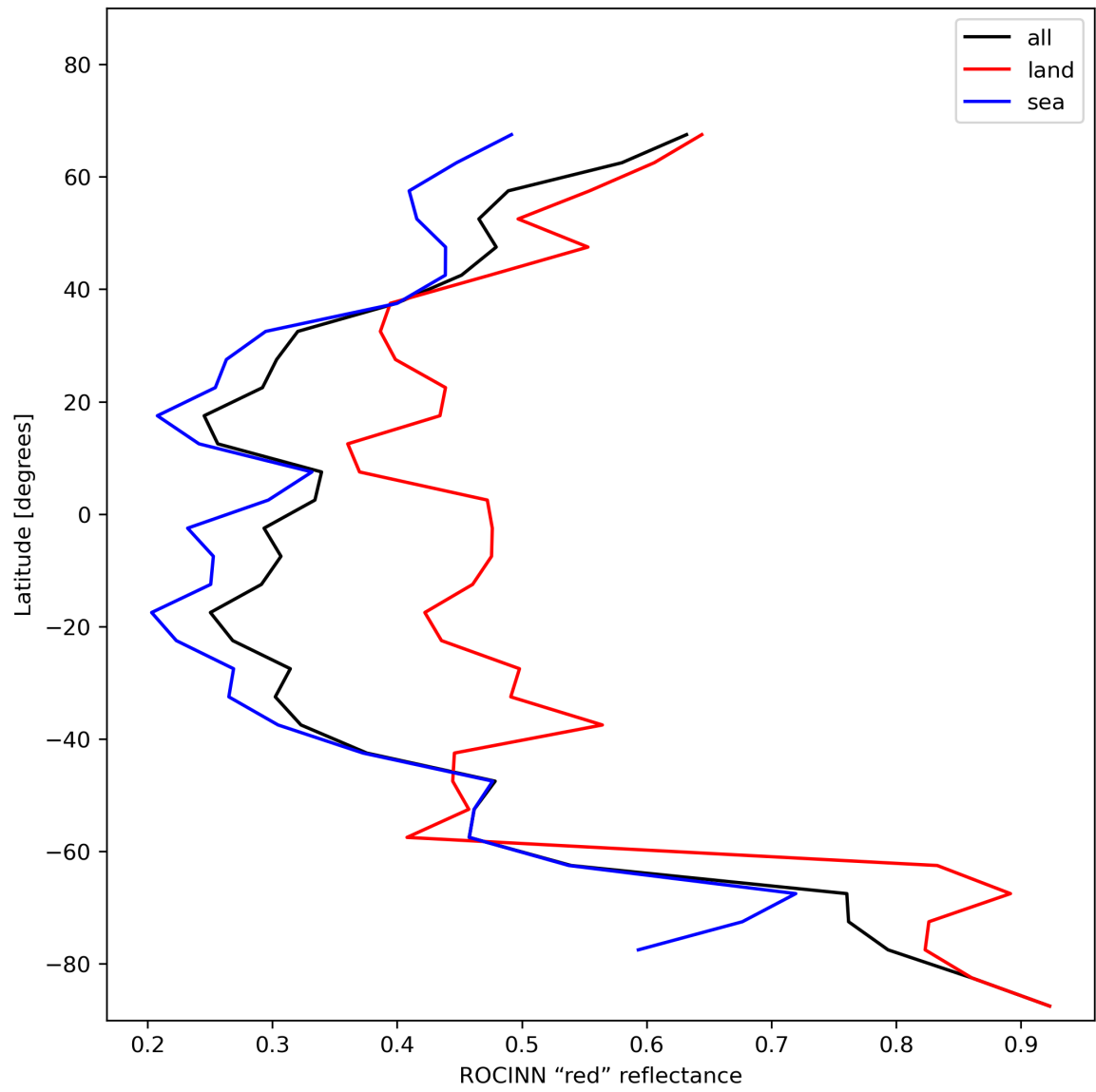
Figure 37: Zonal average of “ROCINN “red” reflectance” for 2023-11-28 to 2023-11-29.
