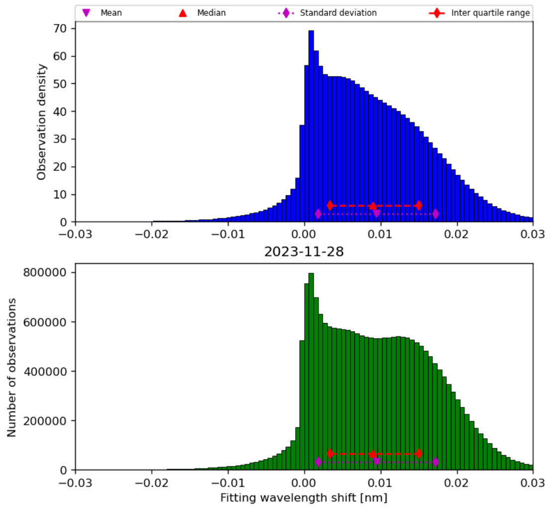
Figure 49: Histogram of “Fitting wavelength shift” for 2023-11-28 to 2023-11-29
