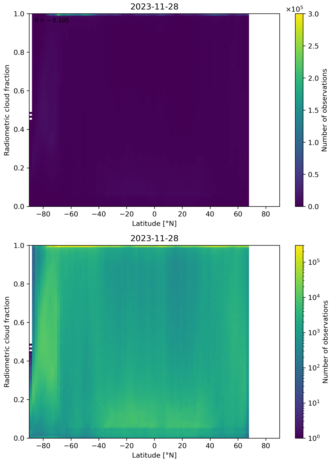
Figure 92: Scatter density plot of “Latitude” against “Radiometric cloud fraction” for 2023-11-28 to 2023-11-29.
