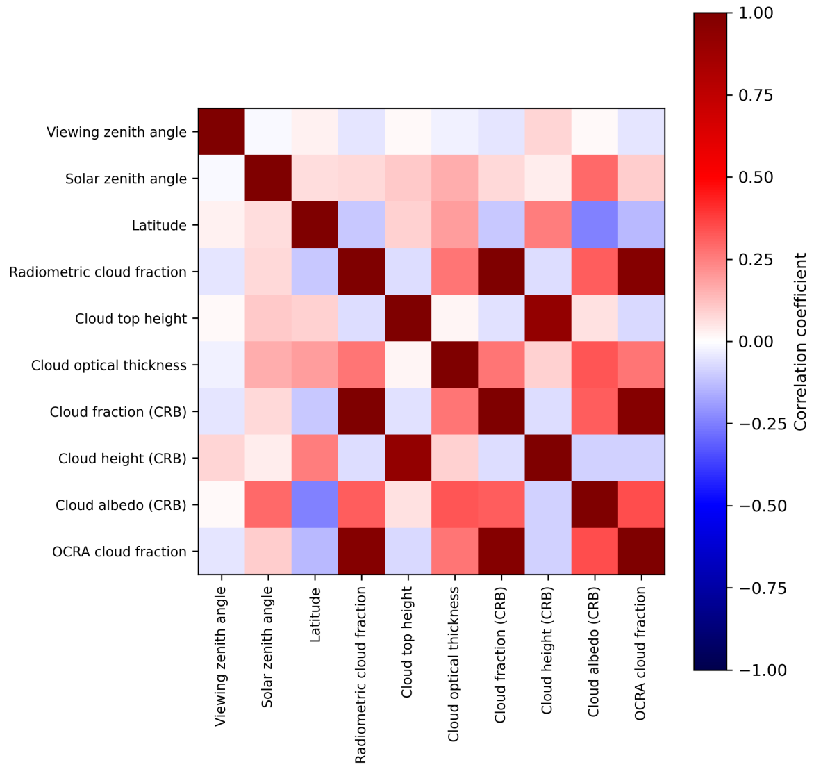
Figure 2: Map of correlation matrix for 2023-11-28 to 2023-11-29.
