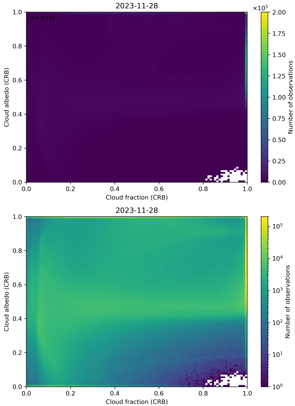
Figure 77: Scatter density plot of “Cloud fraction (CRB)” against “Cloud albedo (CRB)” for 2023-11-28 to 2023-11-29.
