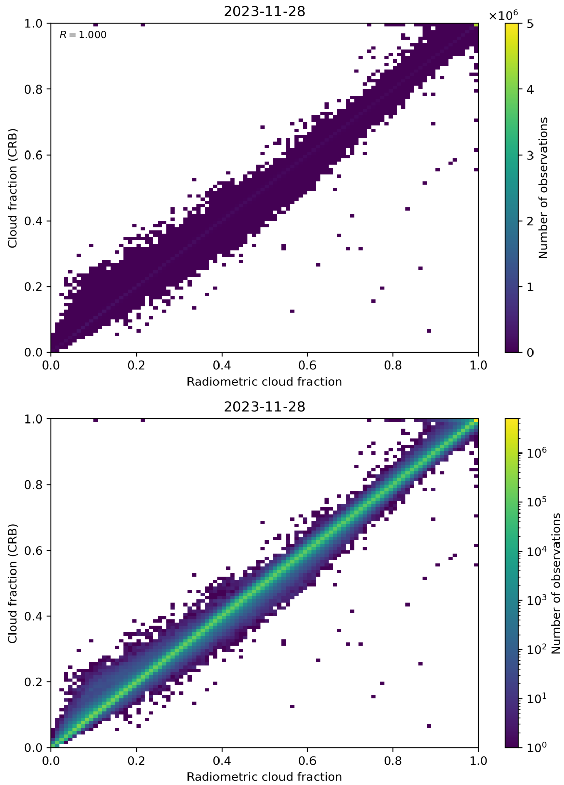
Figure 73: Scatter density plot of “Radiometric cloud fraction” against “Cloud fraction (CRB)” for 2023-11-28 to 2023-11-29.
