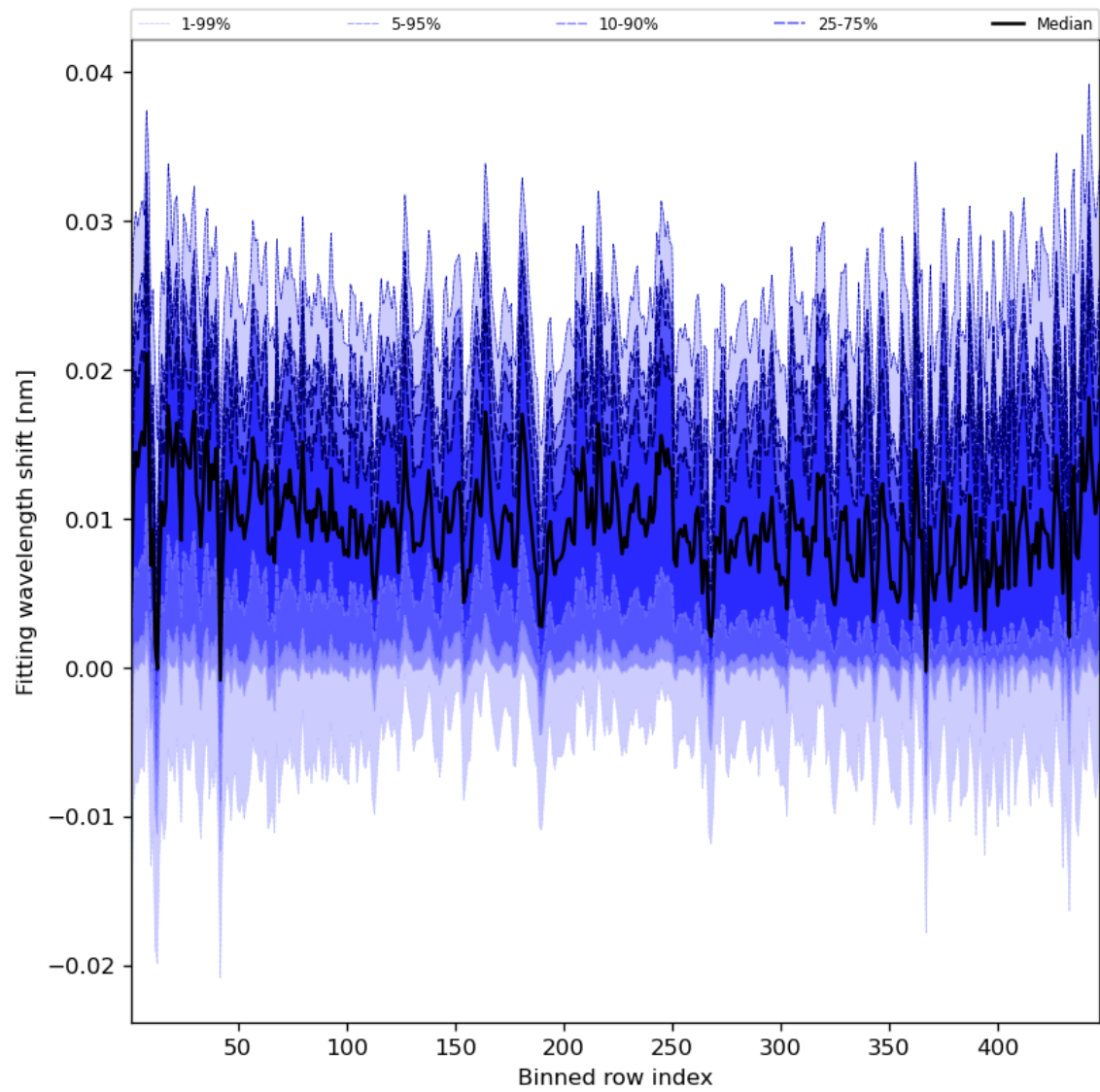
Figure 65: Along track statistics of “Fitting wavelength shift” for 2023-11-28 to 2023-11-29
