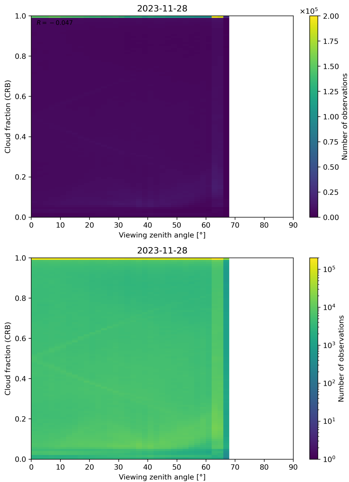
Figure 109: Scatter density plot of “Viewing zenith angle” against “Cloud fraction (CRB)” for 2023-11-28 to 2023-11-29.
