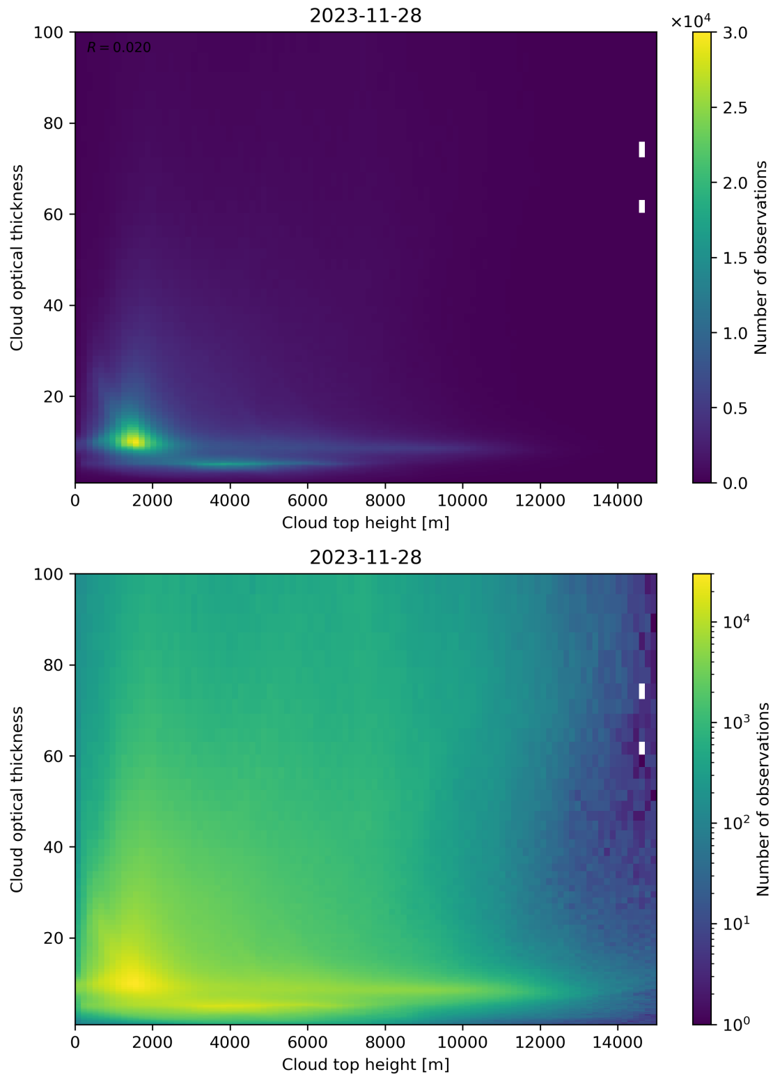
Figure 90: Scatter density plot of “Cloud top height” against “Cloud optical thickness” for 2023-11-28 to 2023-11-29.
