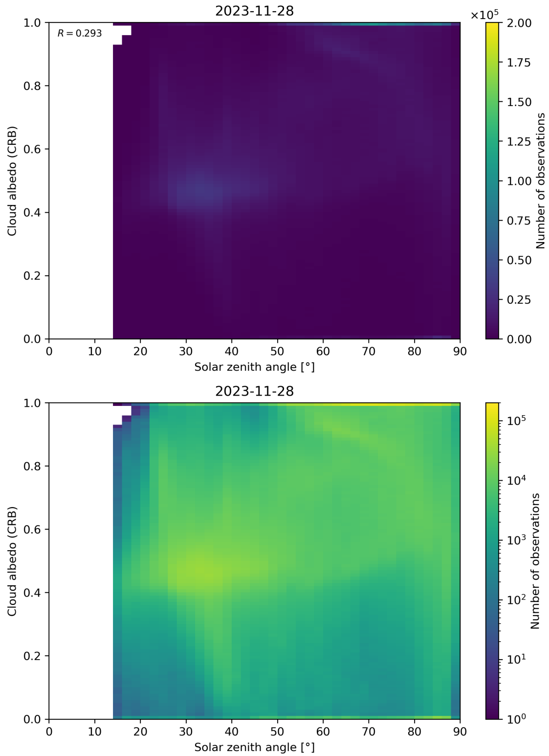
Figure 98: Scatter density plot of “Solar zenith angle” against “Cloud albedo (CRB)” for 2023-11-28 to 2023-11-29.
