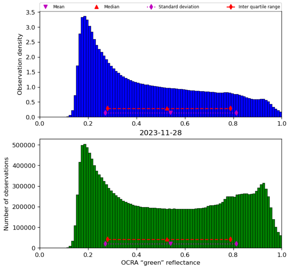
Figure 52: Histogram of “OCRA “green” reflectance” for 2023-11-28 to 2023-11-29
