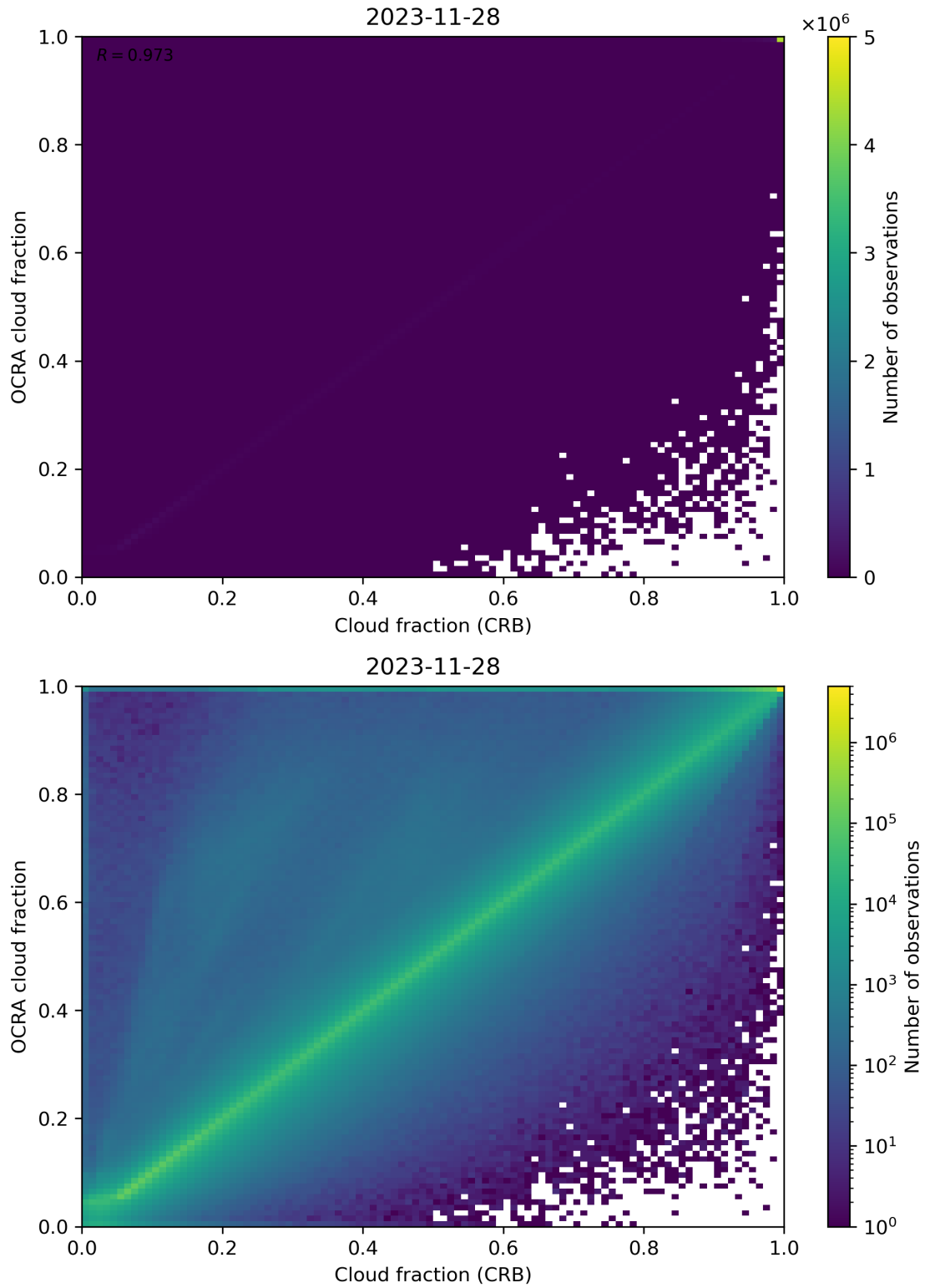
Figure 78: Scatter density plot of “Cloud fraction (CRB)” against “OCRA cloud fraction” for 2023-11-28 to 2023-11-29.
