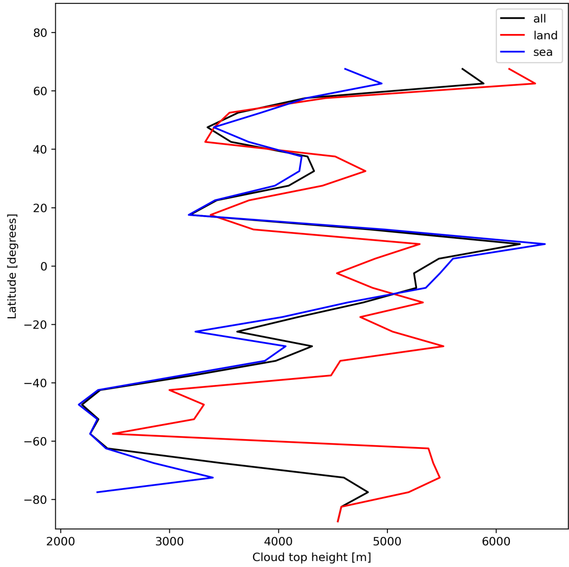
Figure 24: Zonal average of “Cloud top height” for 2023-11-28 to 2023-11-29.
