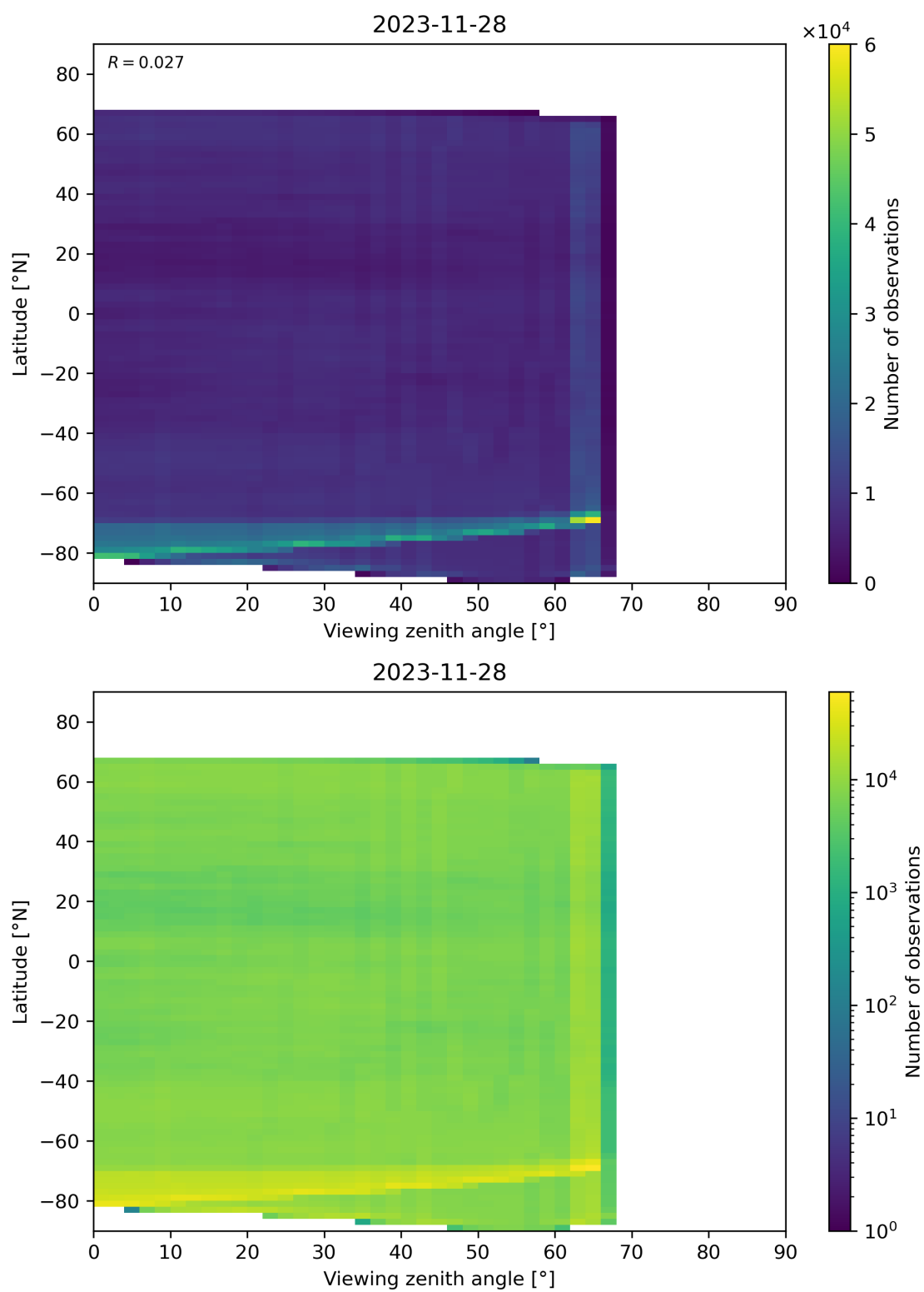
Figure 113: Scatter density plot of “Viewing zenith angle” against “Latitude” for 2023-11-28 to 2023-11-29.
