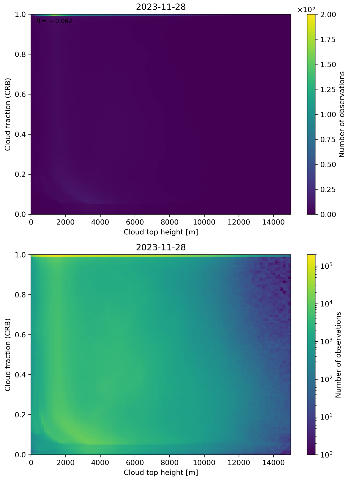
Figure 88: Scatter density plot of “Cloud top height” against “Cloud fraction (CRB)” for 2023-11-28 to 2023-11-29.
