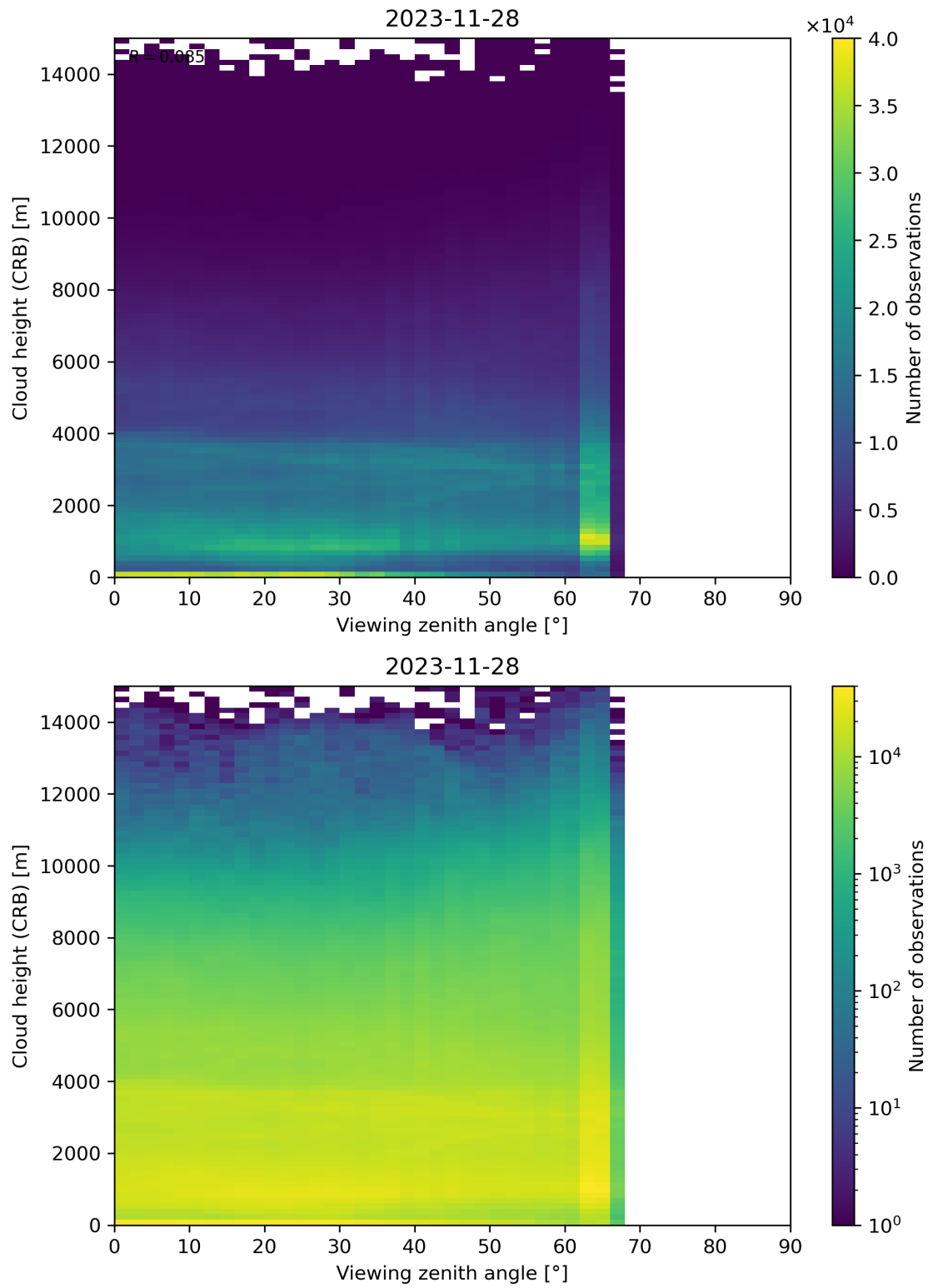
Figure 110: Scatter density plot of “Viewing zenith angle” against “Cloud height (CRB)” for 2023-11-28 to 2023-11-29.
