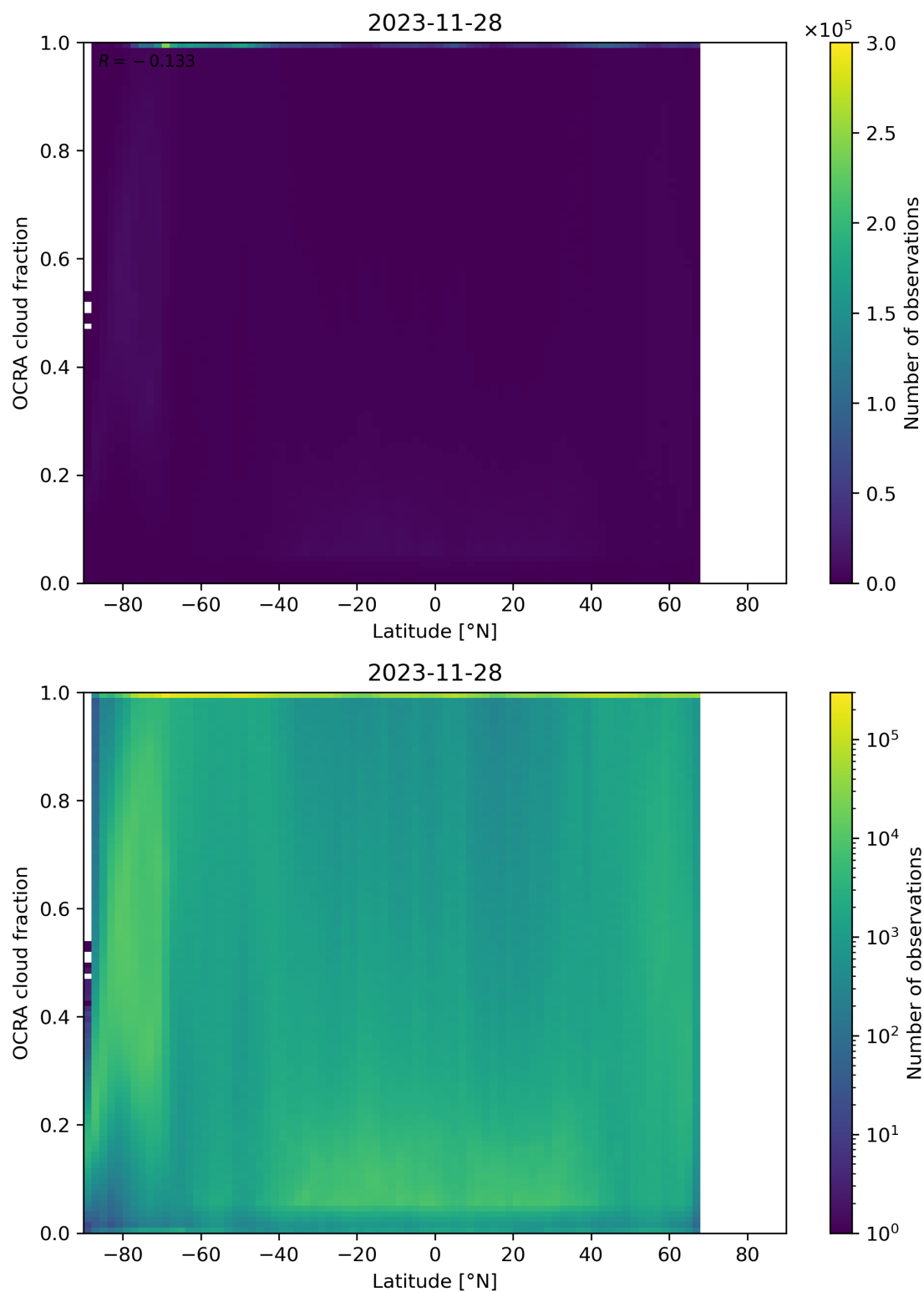
Figure 93: Scatter density plot of “Latitude” against “OCRA cloud fraction” for 2023-11-28 to 2023-11-29.
