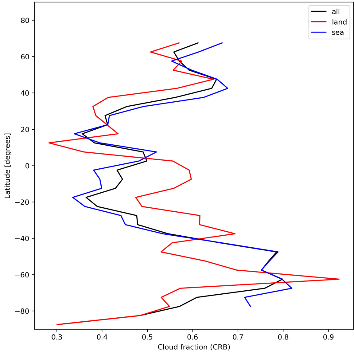
Figure 26: Zonal average of “Cloud fraction (CRB)” for 2023-11-28 to 2023-11-29.
