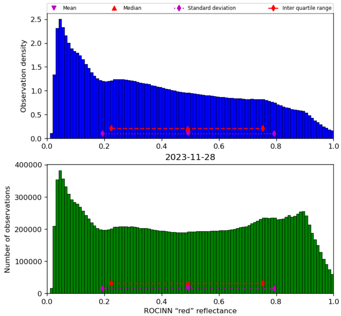
Figure 53: Histogram of “ROCINN “red” reflectance” for 2023-11-28 to 2023-11-29
