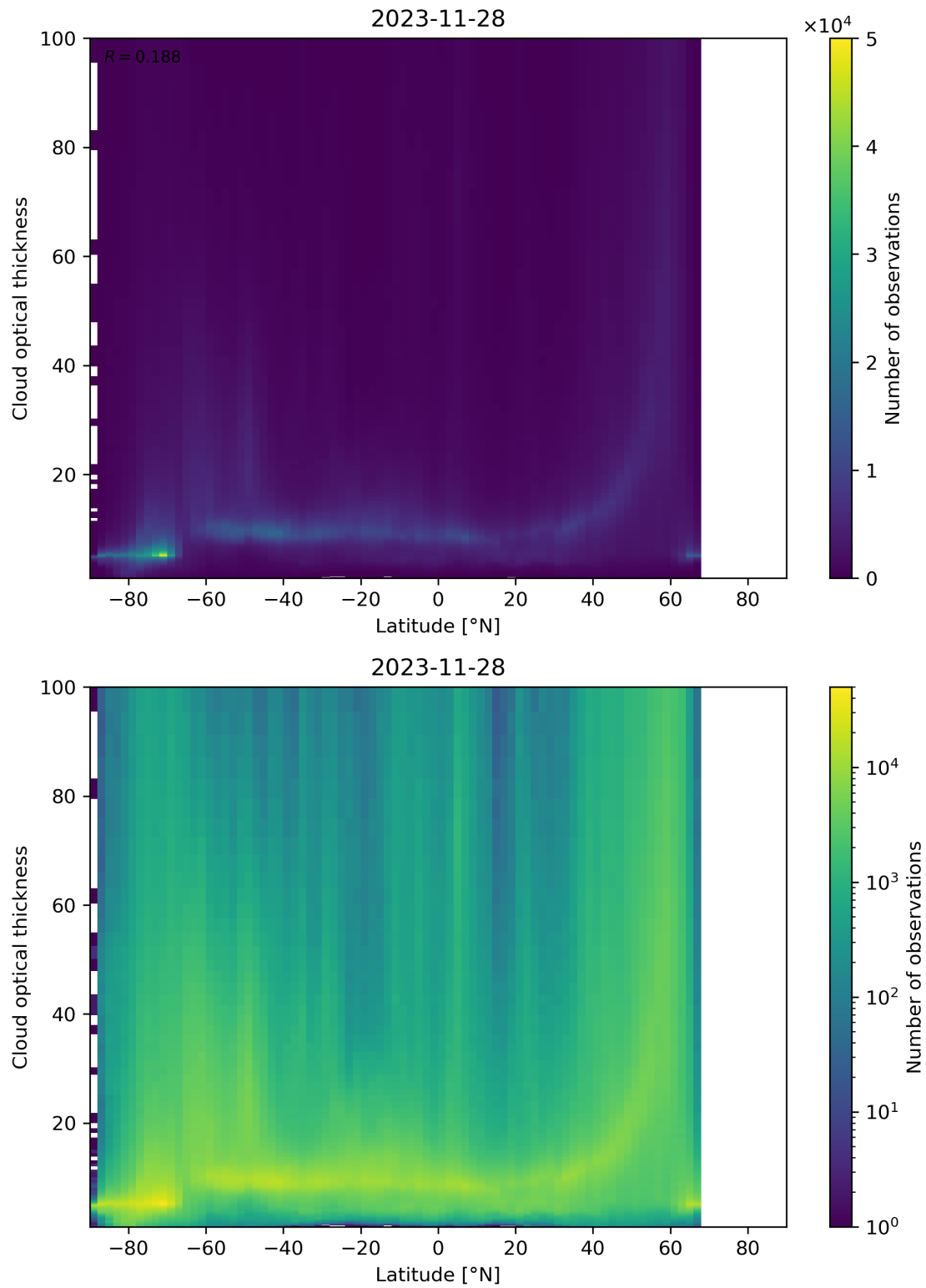
Figure 96: Scatter density plot of “Latitude” against “Cloud optical thickness” for 2023-11-28 to 2023-11-29.
