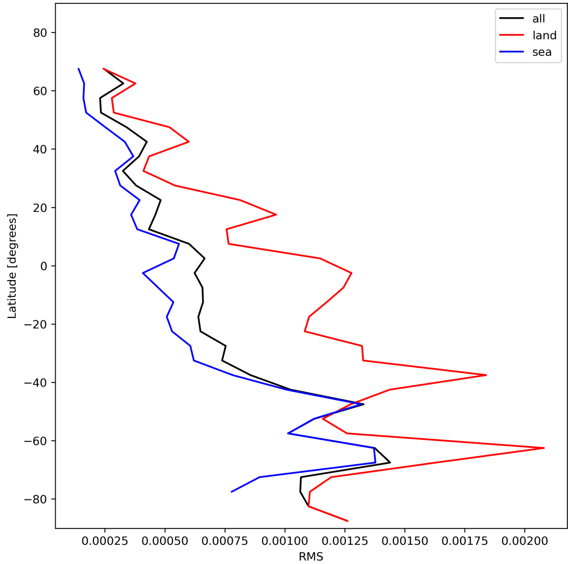
Figure 31: Zonal average of “RMS” for 2023-11-28 to 2023-11-29.
