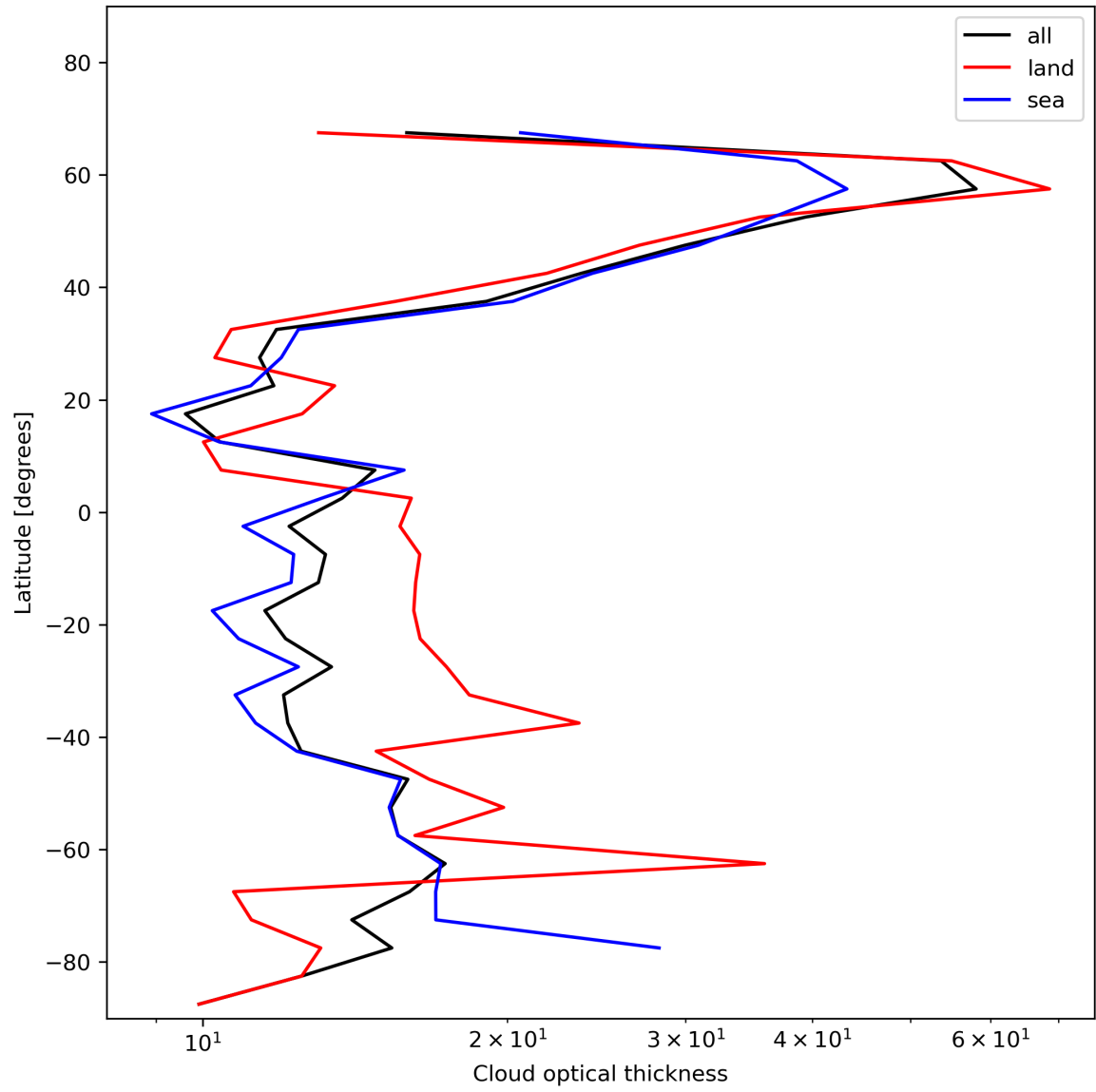
Figure 25: Zonal average of “Cloud optical thickness” for 2023-11-28 to 2023-11-29.
