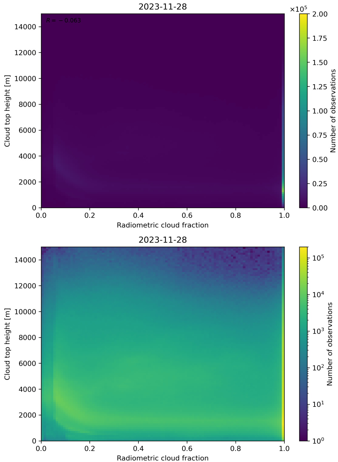
Figure 76: Scatter density plot of “Radiometric cloud fraction” against “Cloud top height” for 2023-11-28 to 2023-11-29.
