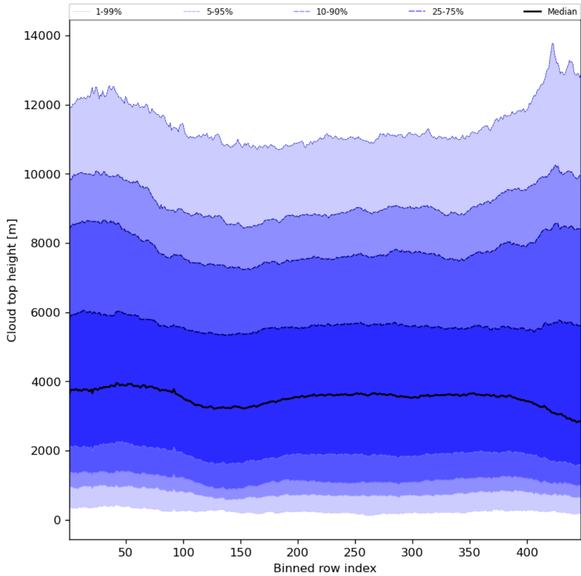
Figure 56: Along track statistics of “Cloud top height” for 2023-11-28 to 2023-11-30
