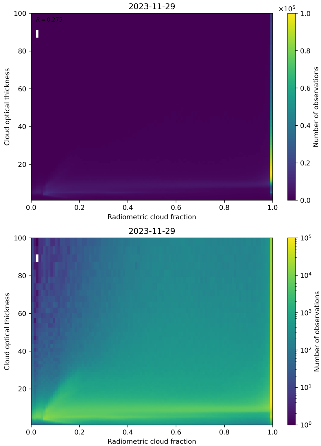
Figure 75: Scatter density plot of “Radiometric cloud fraction” against “Cloud optical thickness” for 2023-11-28 to 2023-11-30.
