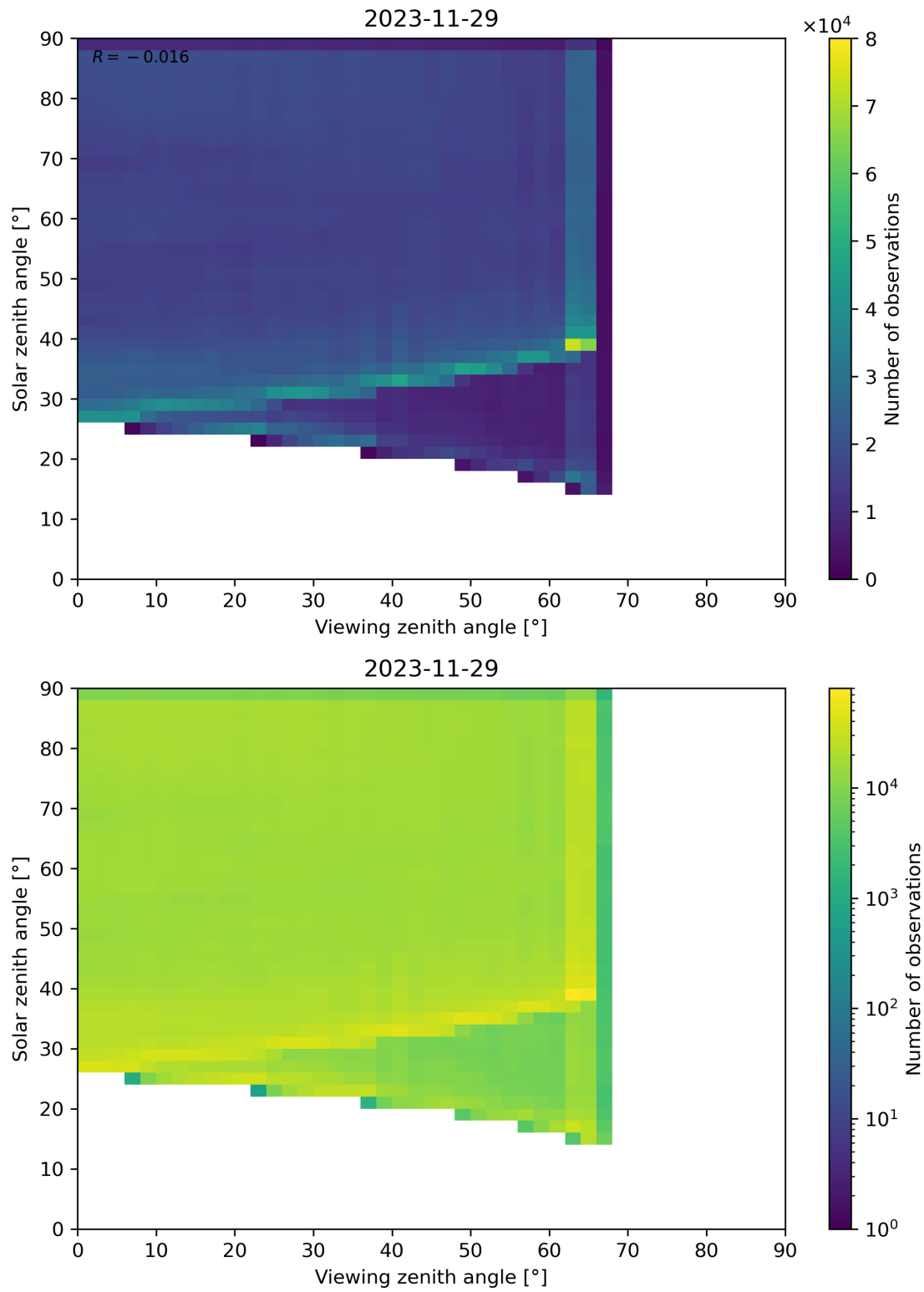
Figure 114: Scatter density plot of “Viewing zenith angle” against “Solar zenith angle” for 2023-11-28 to 2023-11-30.
