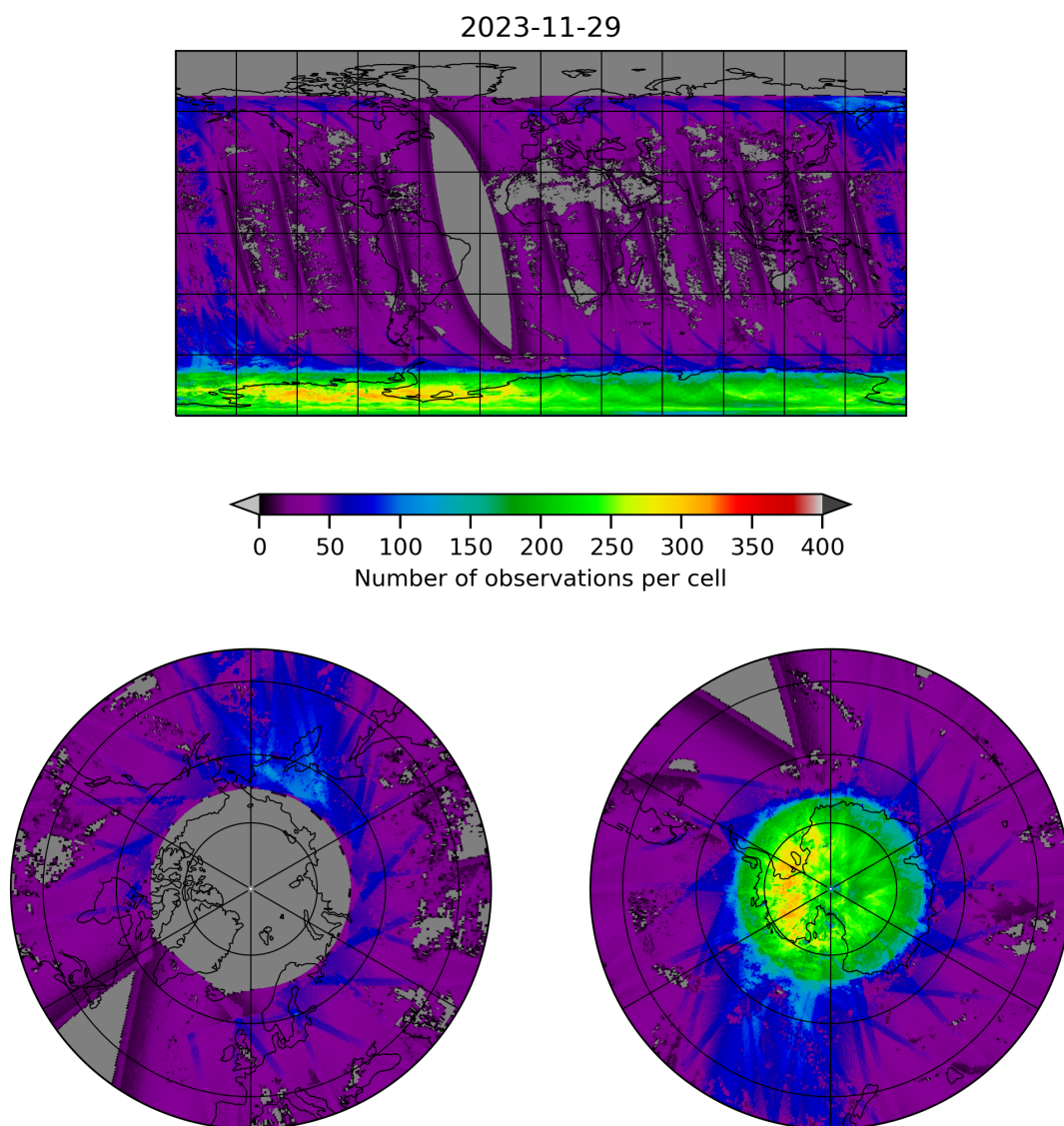
Figure 21: Map of the number of observations for 2023-11-28 to 2023-11-30
