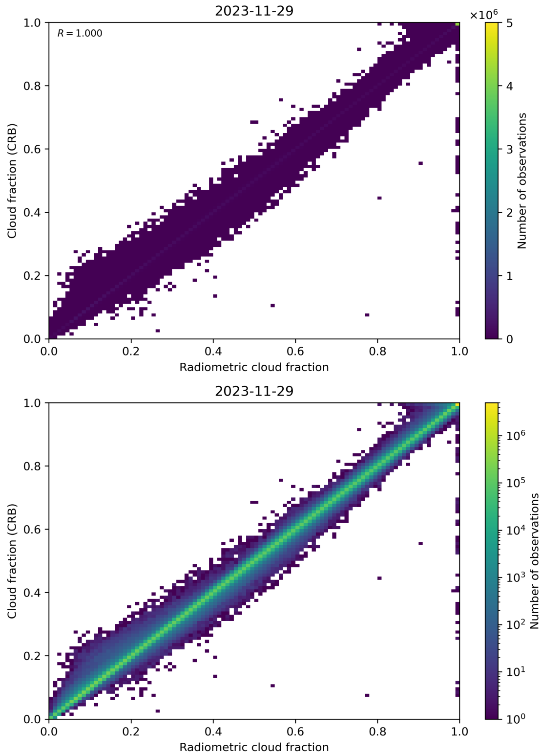
Figure 73: Scatter density plot of “Radiometric cloud fraction” against “Cloud fraction (CRB)” for 2023-11-28 to 2023-11-30.
