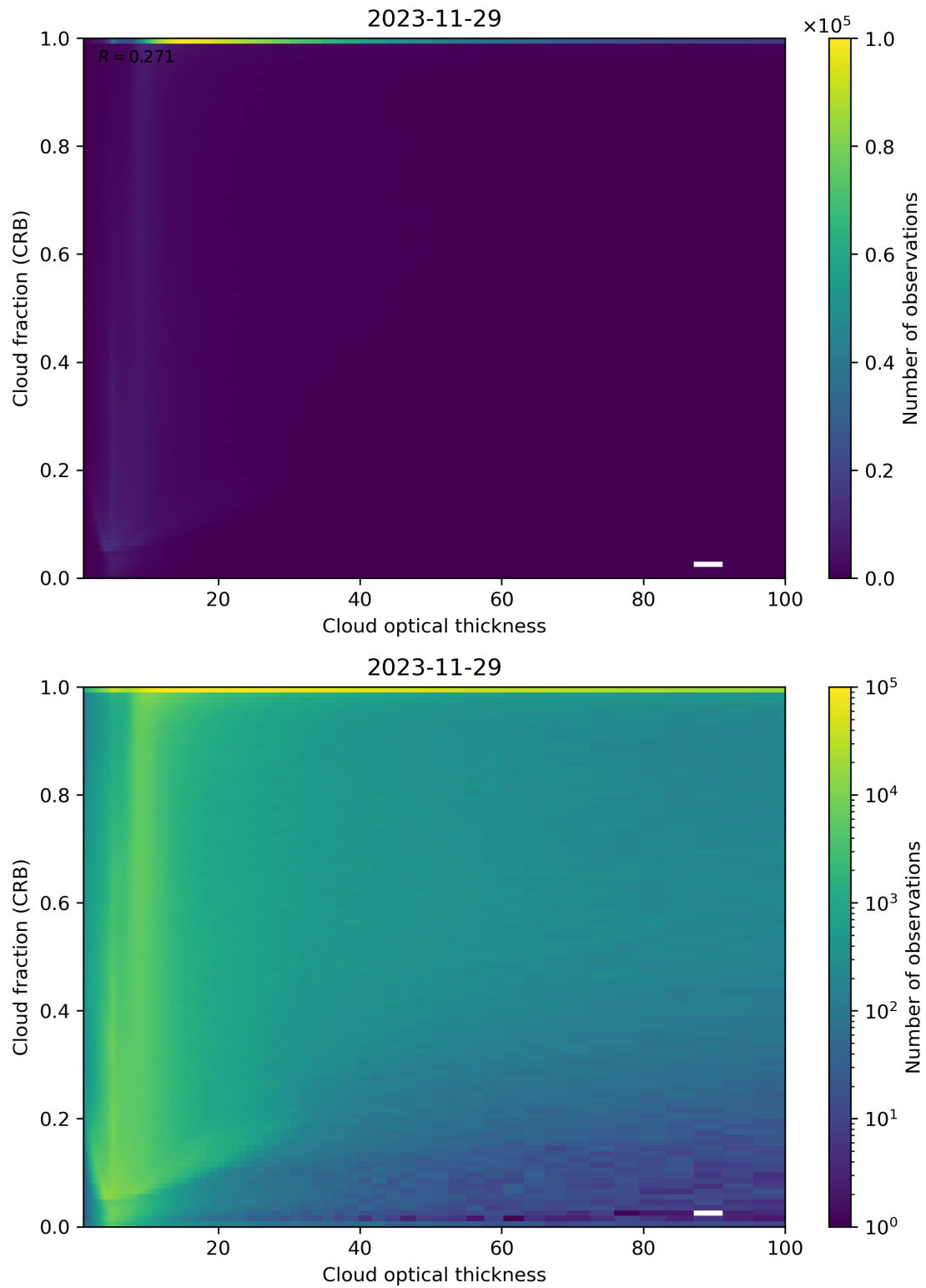
Figure 84: Scatter density plot of “Cloud optical thickness” against “Cloud fraction (CRB)” for 2023-11-28 to 2023-11-30.
