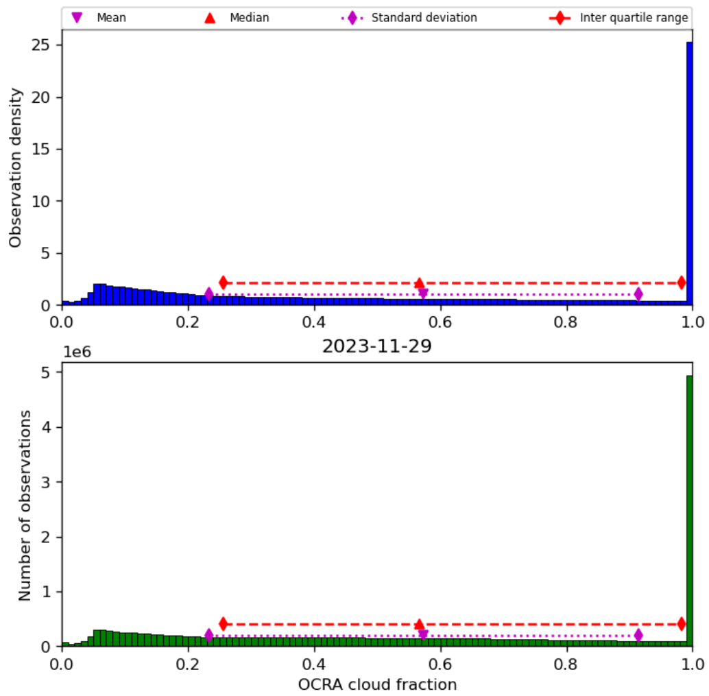
Figure 50: Histogram of “OCRA cloud fraction” for 2023-11-28 to 2023-11-30
