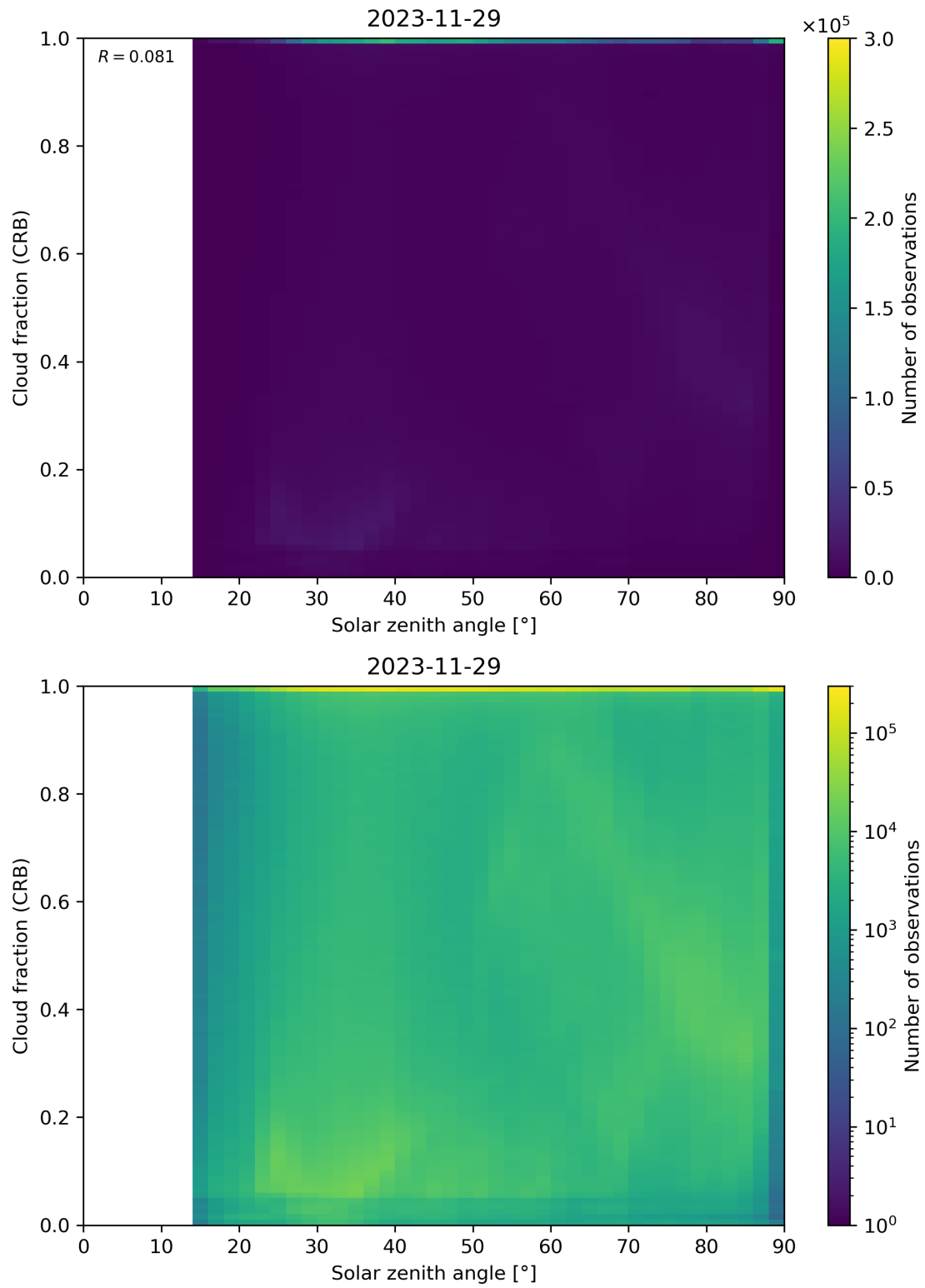
Figure 101: Scatter density plot of “Solar zenith angle” against “Cloud fraction (CRB)” for 2023-11-28 to 2023-11-30.
