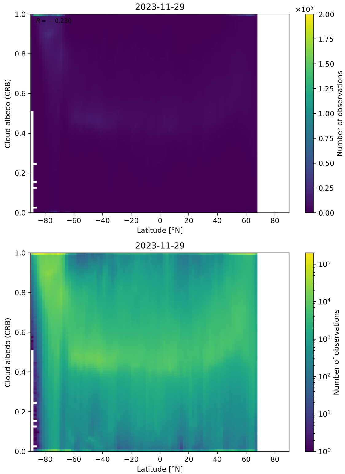
Figure 91: Scatter density plot of “Latitude” against “Cloud albedo (CRB)” for 2023-11-28 to 2023-11-30.
