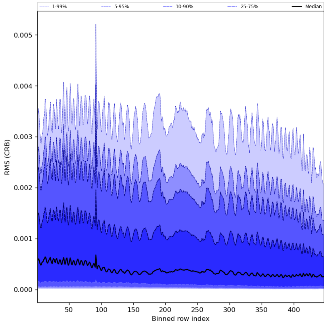
Figure 64: Along track statistics of “RMS (CRB)” for 2023-11-28 to 2023-11-30
