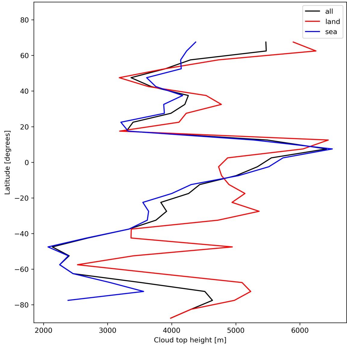
Figure 24: Zonal average of “Cloud top height” for 2023-11-28 to 2023-11-30.
