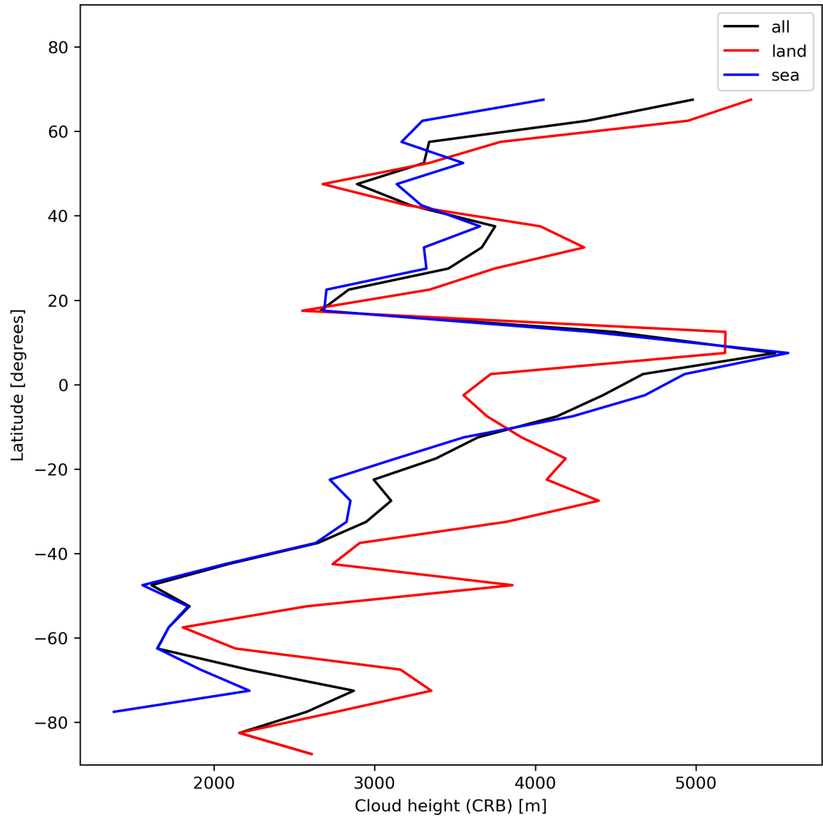
Figure 27: Zonal average of “Cloud height (CRB)” for 2023-11-28 to 2023-11-30.
