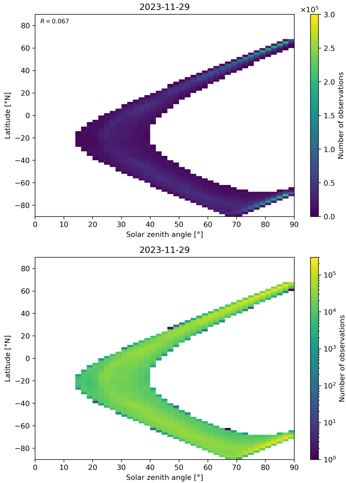
Figure 105: Scatter density plot of “Solar zenith angle” against “Latitude” for 2023-11-28 to 2023-11-30.
