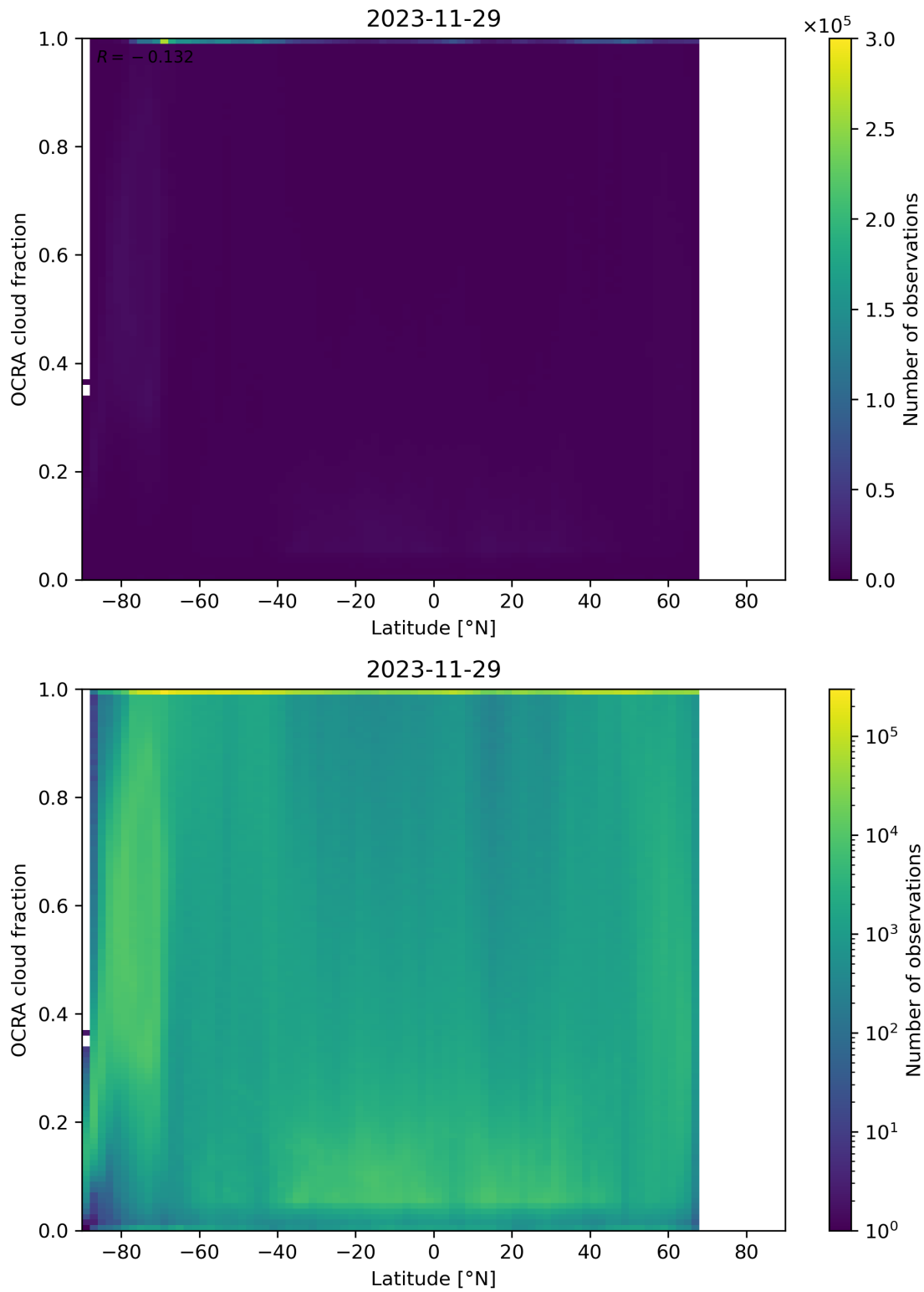
Figure 93: Scatter density plot of “Latitude” against “OCRA cloud fraction” for 2023-11-28 to 2023-11-30.
