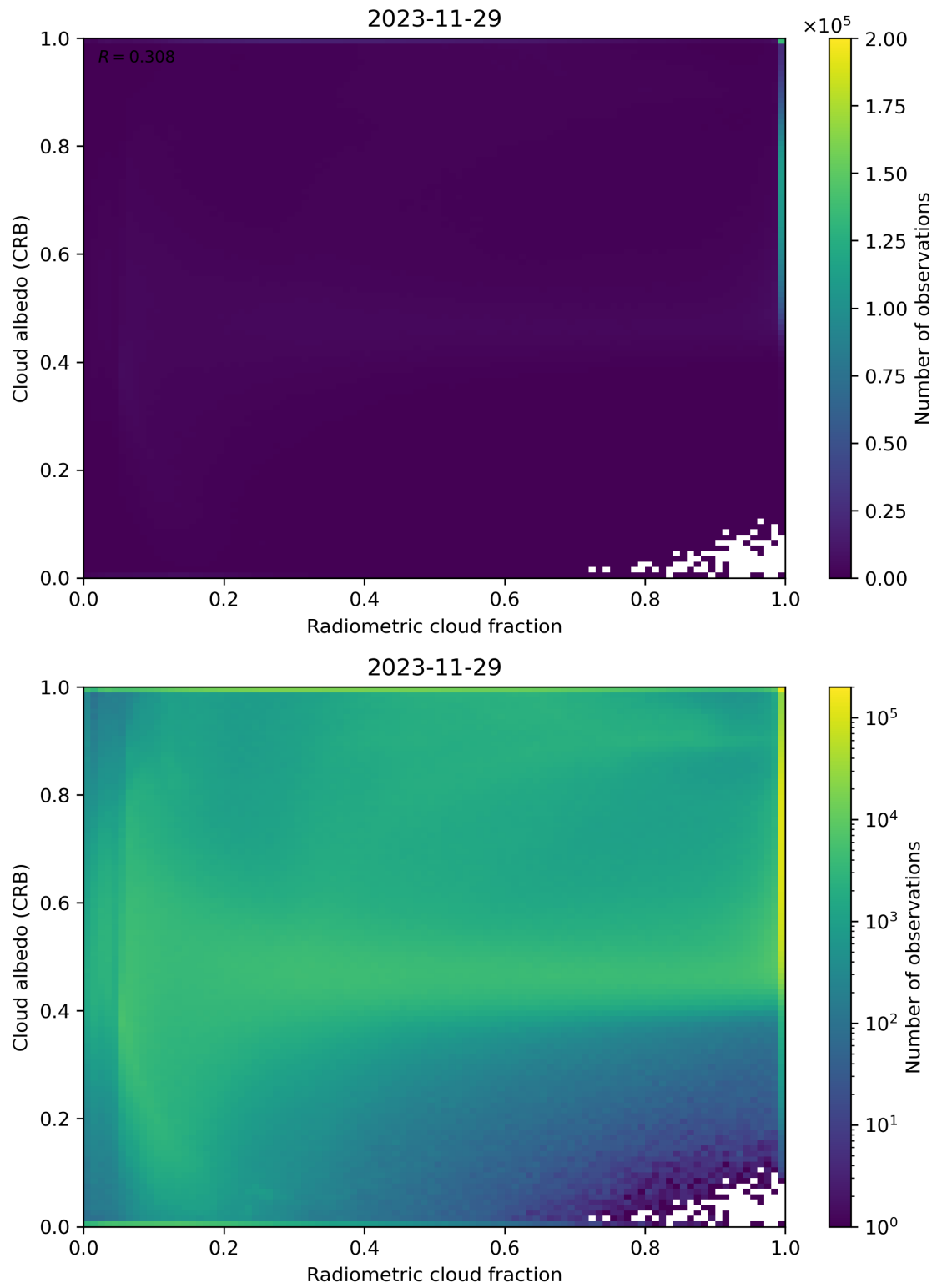
Figure 71: Scatter density plot of “Radiometric cloud fraction” against “Cloud albedo (CRB)” for 2023-11-28 to 2023-11-30.
