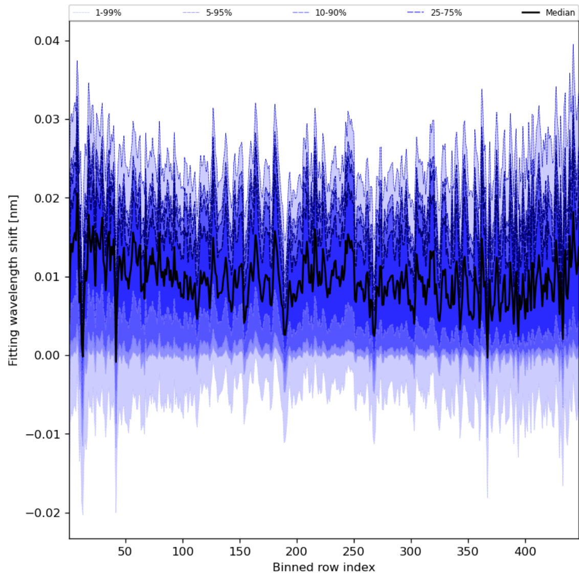
Figure 65: Along track statistics of “Fitting wavelength shift” for 2023-11-28 to 2023-11-30
