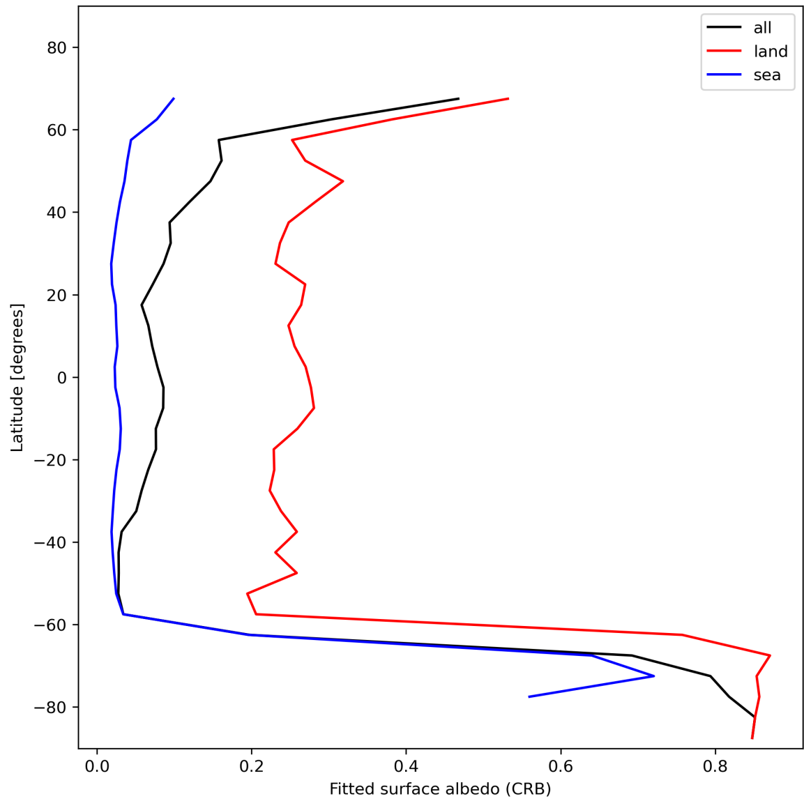
Figure 30: Zonal average of “Fitted surface albedo (CRB)” for 2023-11-28 to 2023-11-30.
