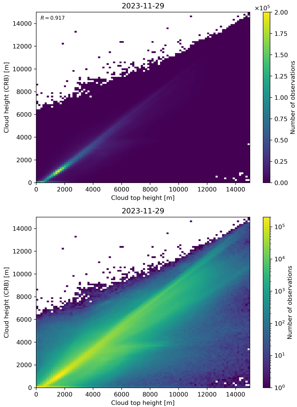
Figure 89: Scatter density plot of “Cloud top height” against “Cloud height (CRB)” for 2023-11-28 to 2023-11-30.
