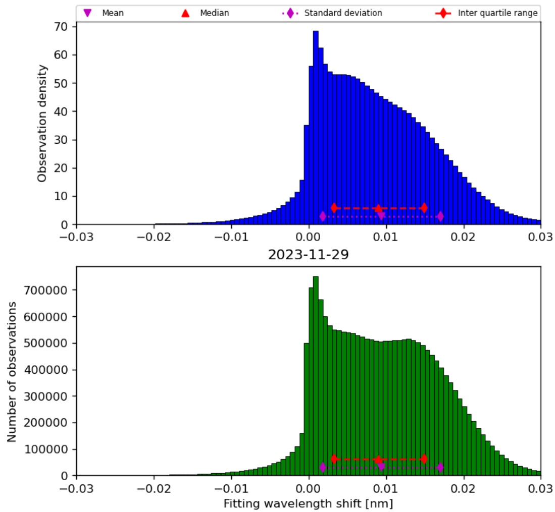
Figure 49: Histogram of “Fitting wavelength shift” for 2023-11-28 to 2023-11-30
