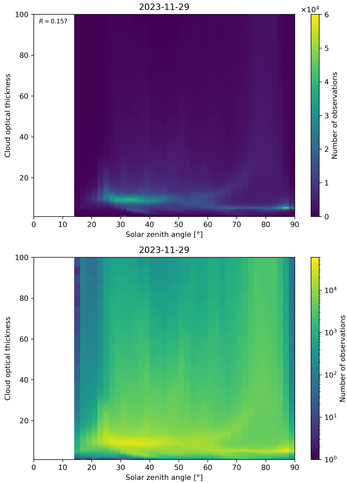
Figure 103: Scatter density plot of “Solar zenith angle” against “Cloud optical thickness” for 2023-11-28 to 2023-11-30.
