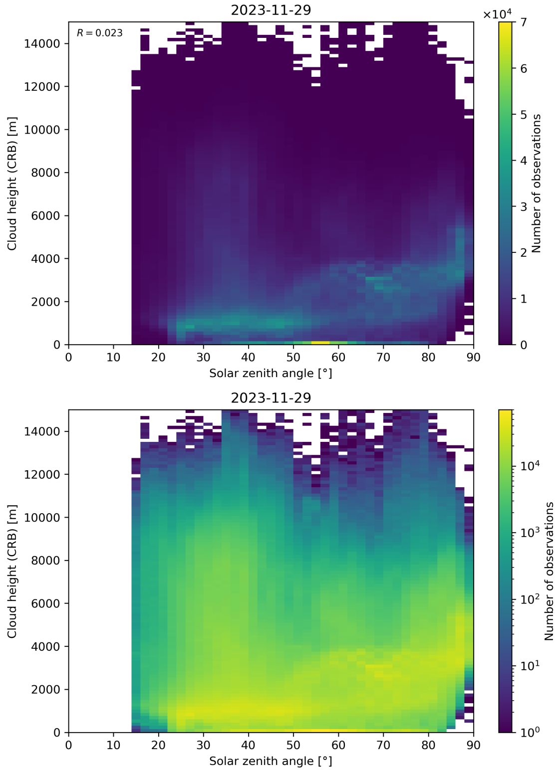
Figure 102: Scatter density plot of “Solar zenith angle” against “Cloud height (CRB)” for 2023-11-28 to 2023-11-30.
