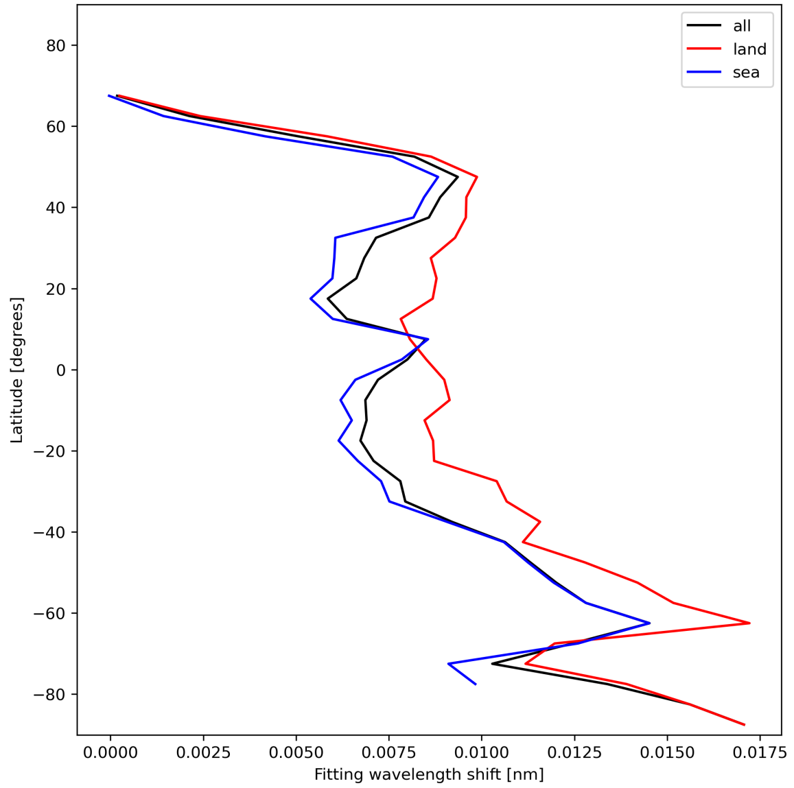
Figure 33: Zonal average of “Fitting wavelength shift” for 2023-11-28 to 2023-11-30.
