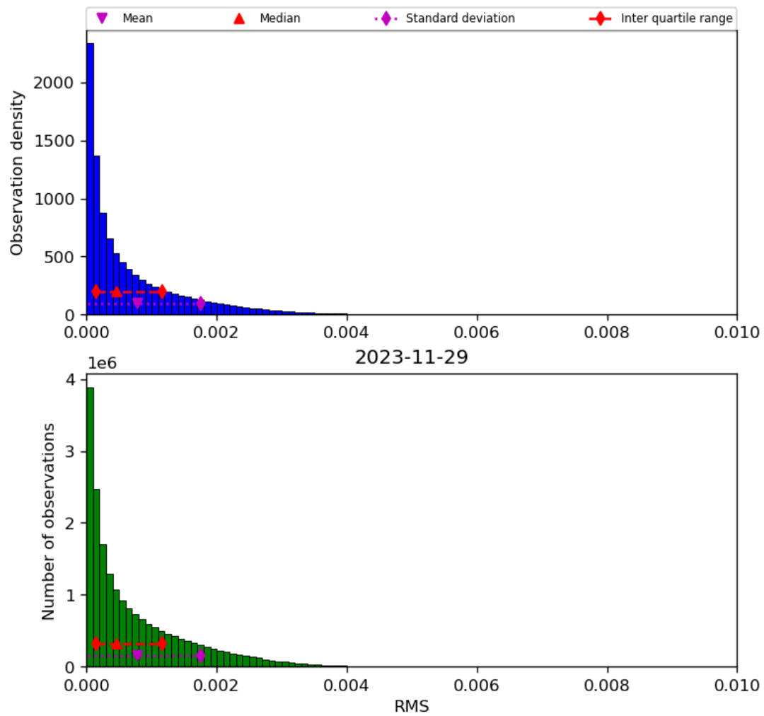
Figure 47: Histogram of “RMS” for 2023-11-28 to 2023-11-30
