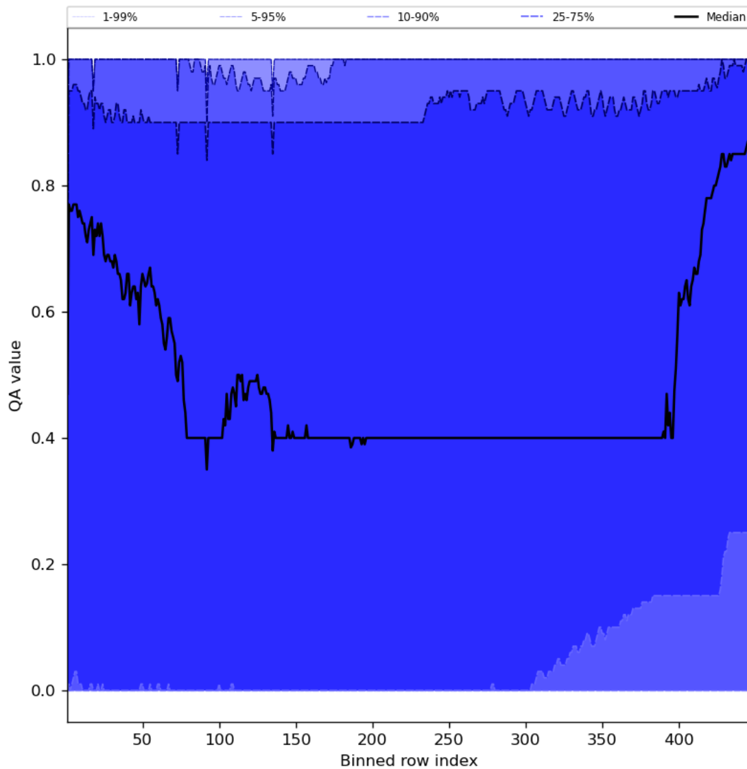
Figure 54: Along track statistics of “QA value” for 2023-11-28 to 2023-11-30
