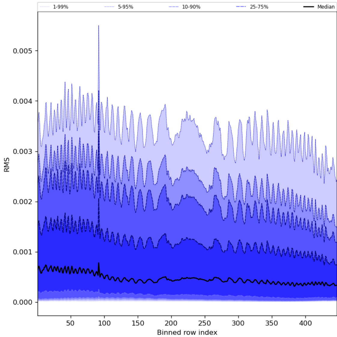
Figure 63: Along track statistics of “RMS” for 2023-11-28 to 2023-11-30
