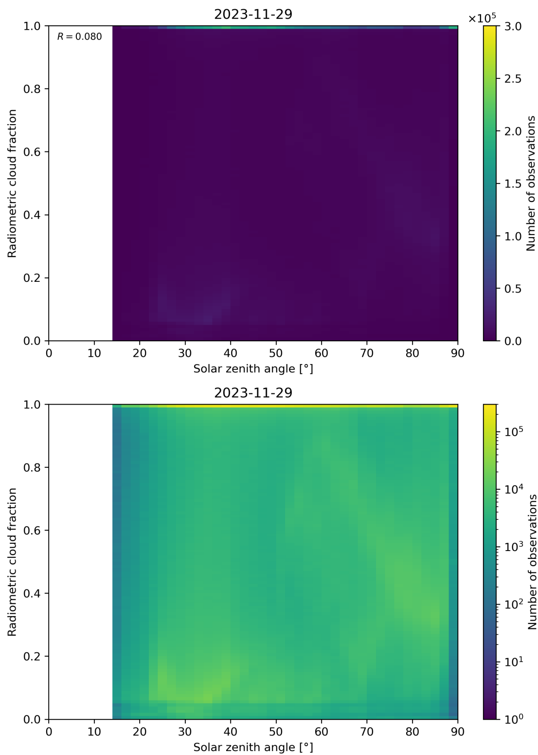
Figure 99: Scatter density plot of “Solar zenith angle” against “Radiometric cloud fraction” for 2023-11-28 to 2023-11-30.
