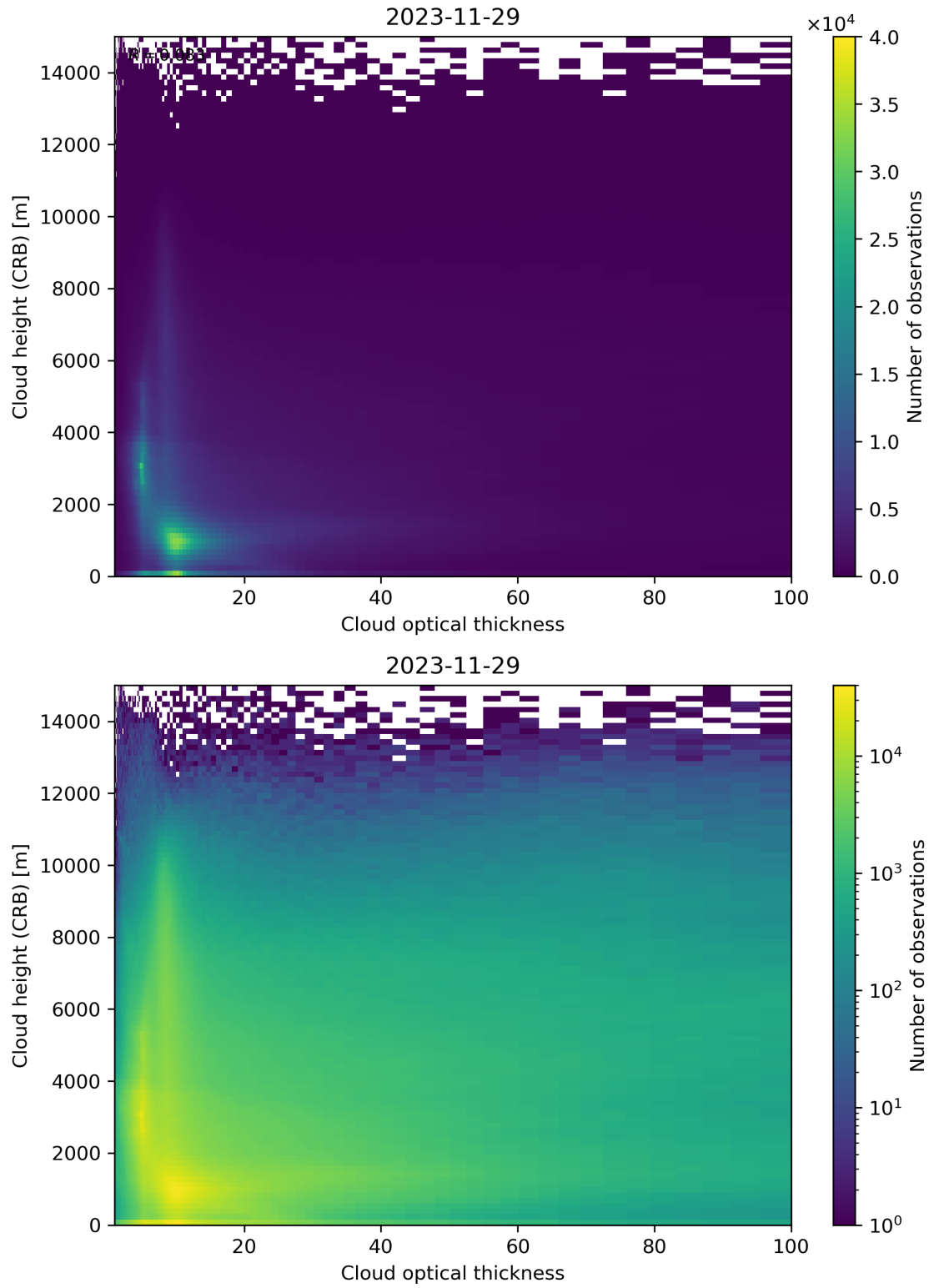
Figure 85: Scatter density plot of “Cloud optical thickness” against “Cloud height (CRB)” for 2023-11-28 to 2023-11-30.
