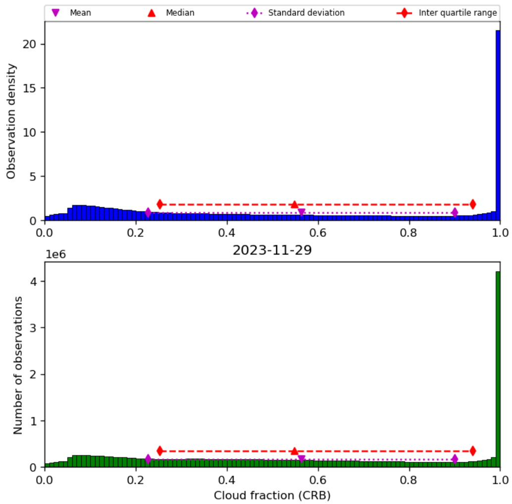
Figure 42: Histogram of “Cloud fraction (CRB)” for 2023-11-28 to 2023-11-30
