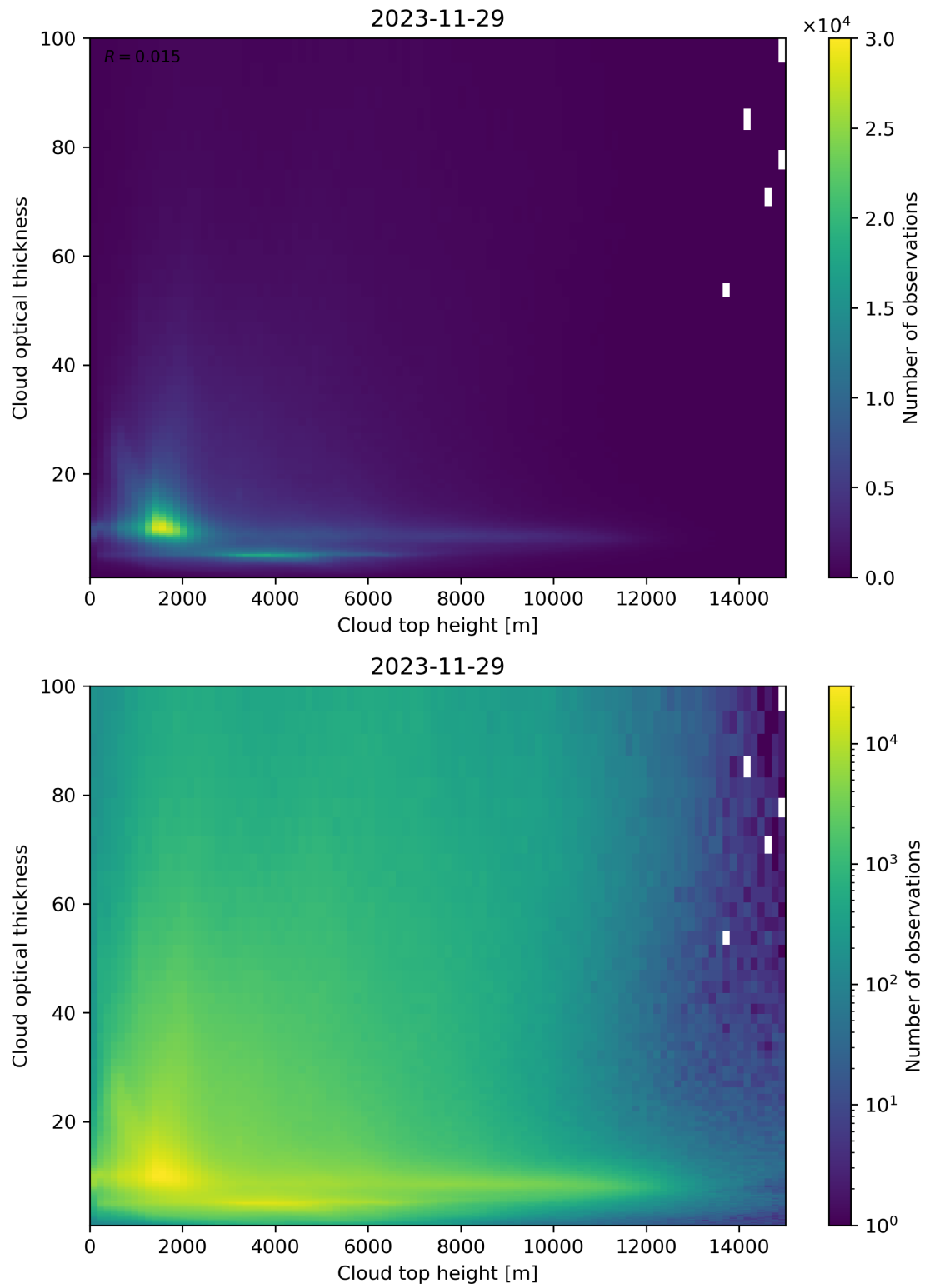
Figure 90: Scatter density plot of “Cloud top height” against “Cloud optical thickness” for 2023-11-28 to 2023-11-30.
