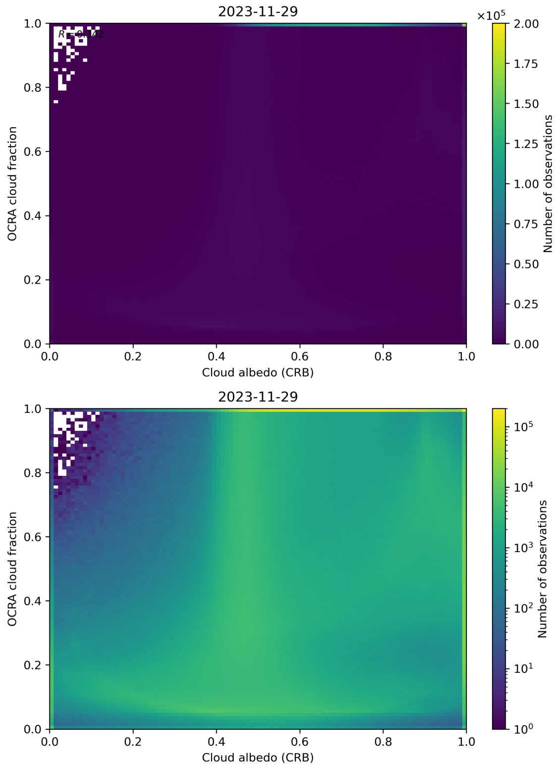
Figure 70: Scatter density plot of “Cloud albedo (CRB)” against “OCRA cloud fraction” for 2023-11-28 to 2023-11-30.
