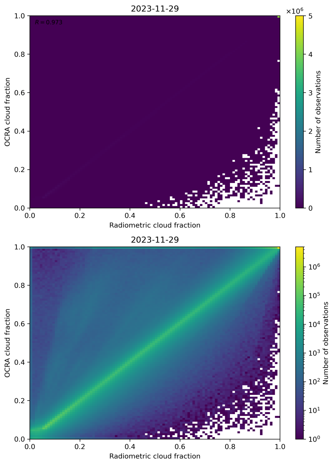
Figure 72: Scatter density plot of “Radiometric cloud fraction” against “OCRA cloud fraction” for 2023-11-28 to 2023-11-30.
