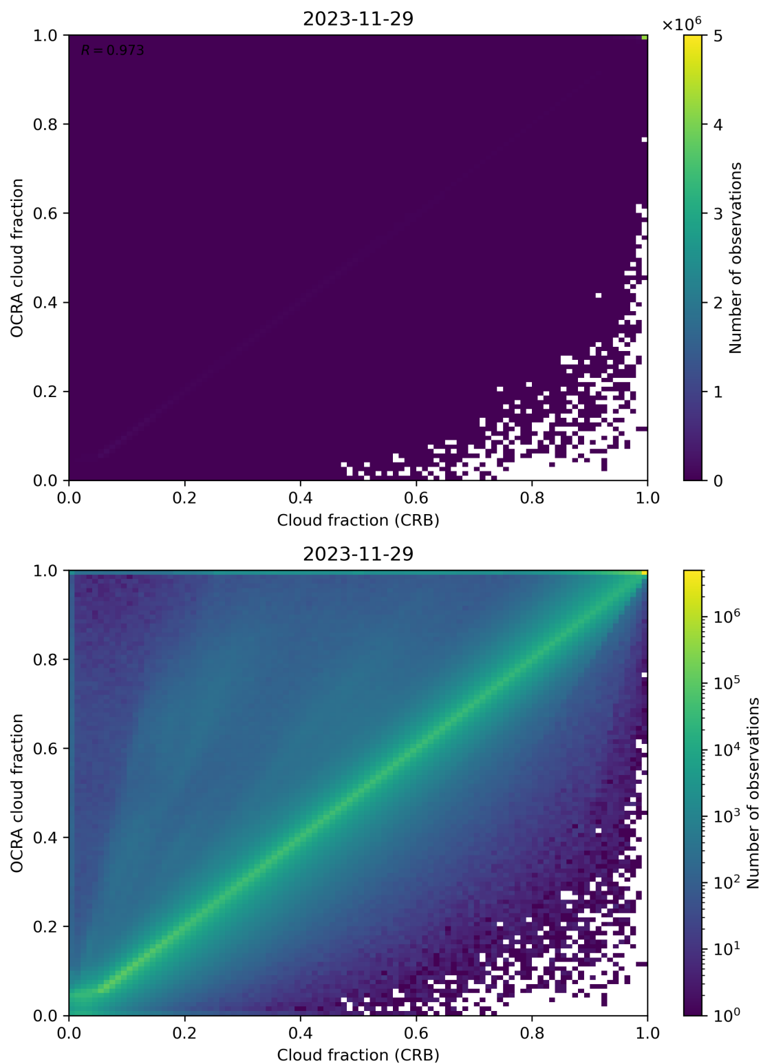
Figure 78: Scatter density plot of “Cloud fraction (CRB)” against “OCRA cloud fraction” for 2023-11-28 to 2023-11-30.
