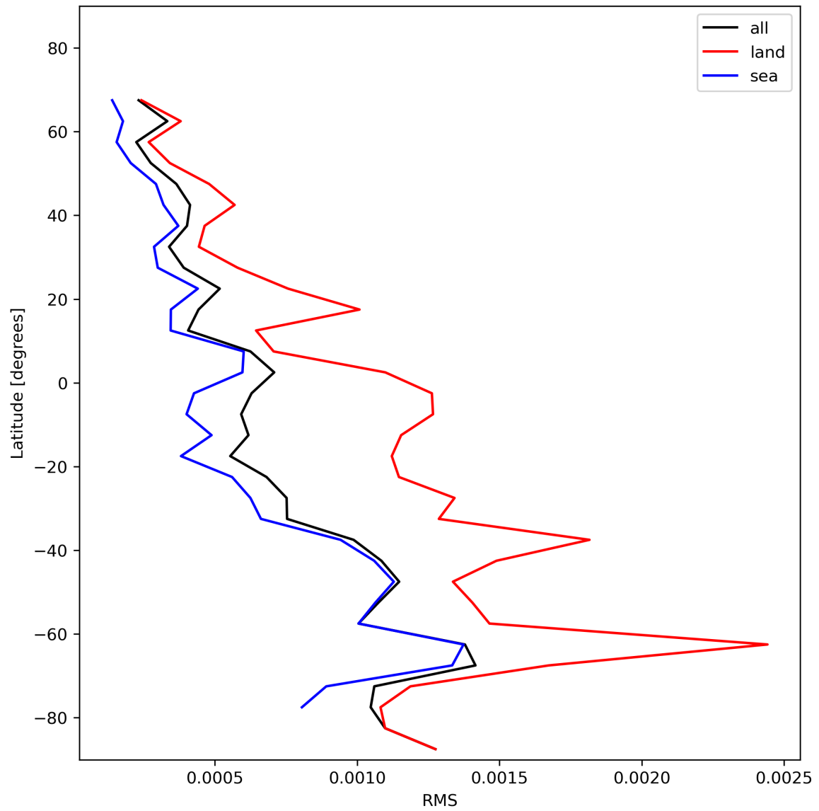
Figure 31: Zonal average of “RMS” for 2023-11-28 to 2023-11-30.
