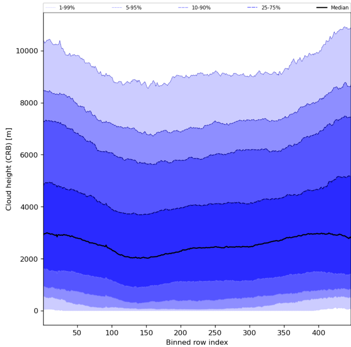
Figure 59: Along track statistics of “Cloud height (CRB)” for 2023-11-28 to 2023-11-30
