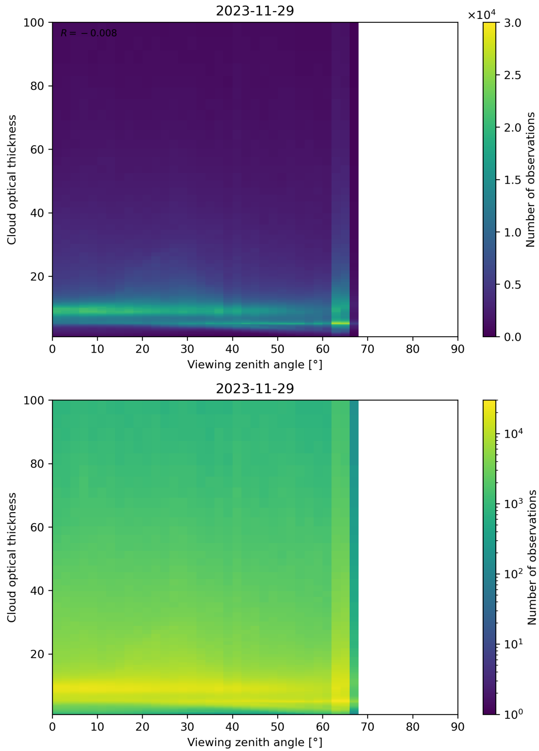
Figure 111: Scatter density plot of “Viewing zenith angle” against “Cloud optical thickness” for 2023-11-28 to 2023-11-30.
