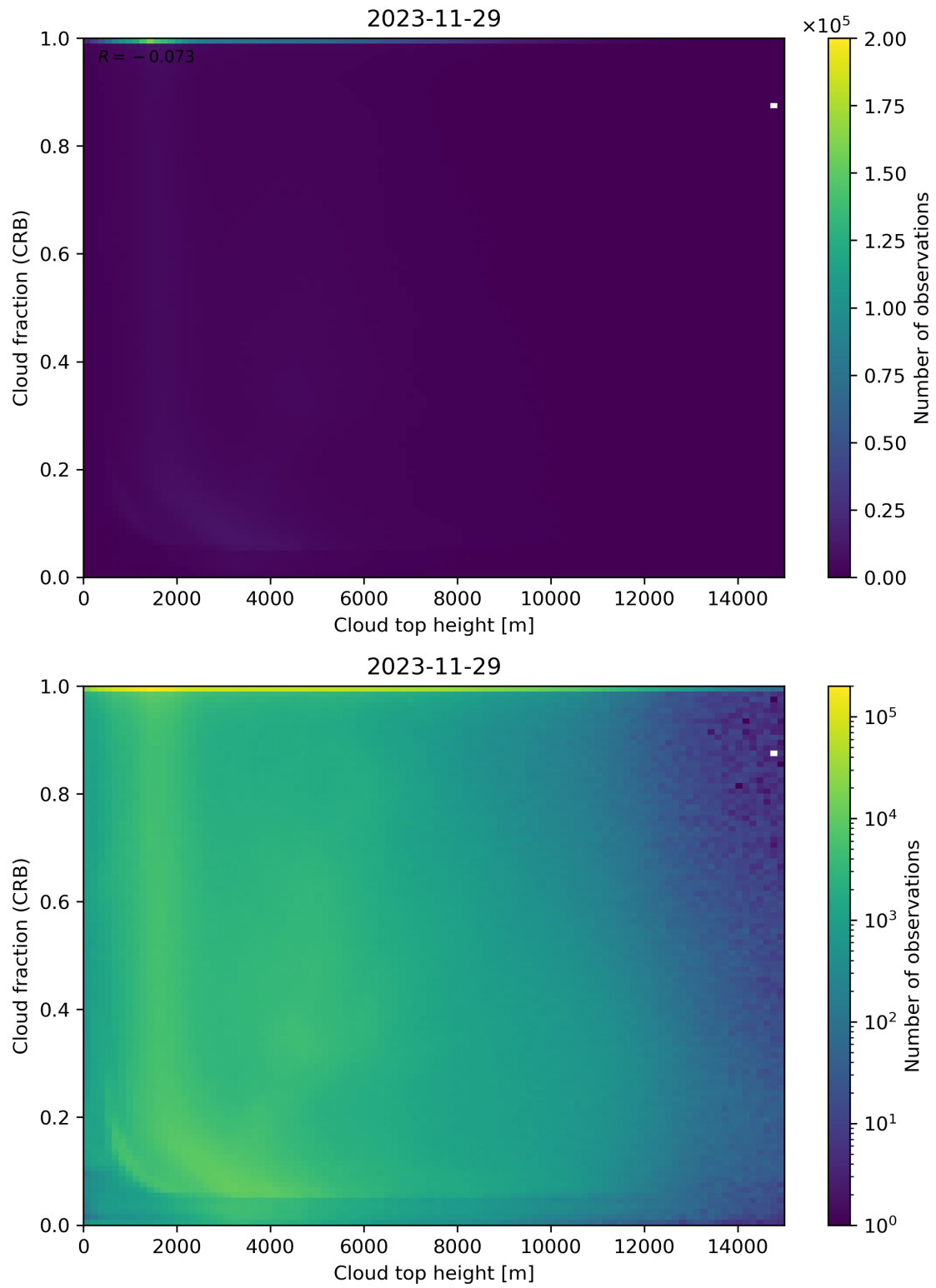
Figure 88: Scatter density plot of “Cloud top height” against “Cloud fraction (CRB)” for 2023-11-28 to 2023-11-30.
