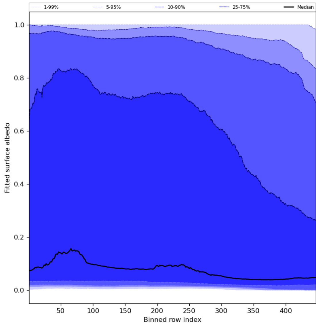
Figure 61: Along track statistics of “Fitted surface albedo” for 2023-11-28 to 2023-11-30
