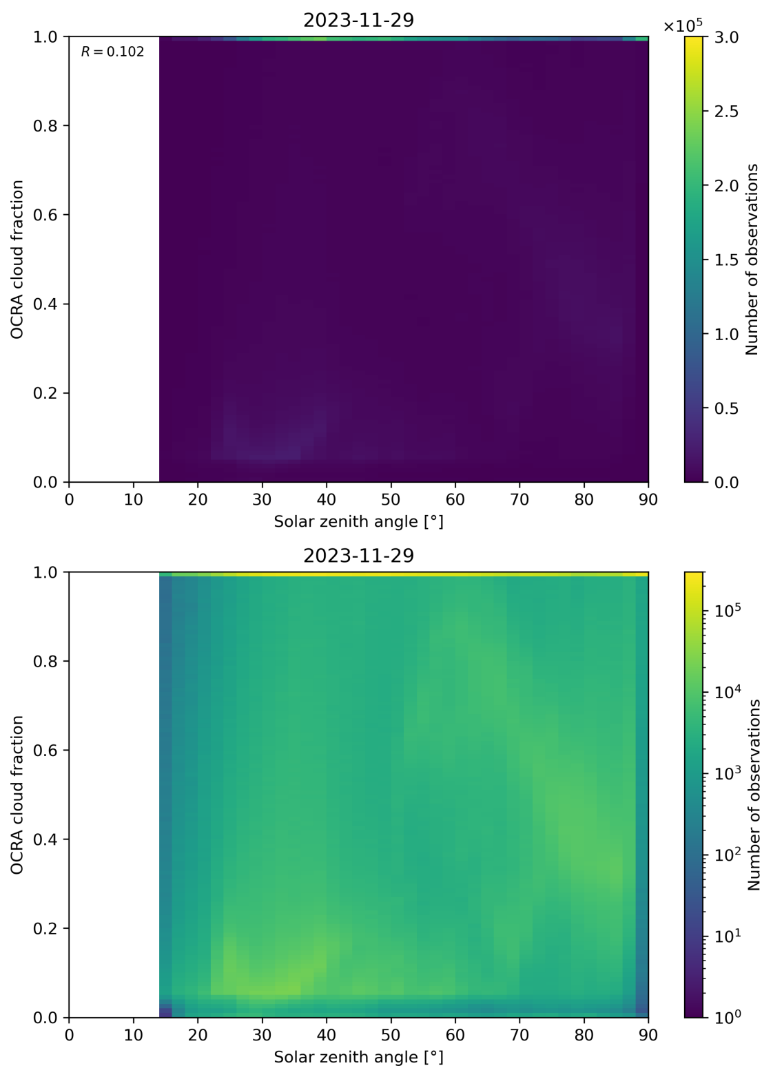
Figure 100: Scatter density plot of “Solar zenith angle” against “OCRA cloud fraction” for 2023-11-28 to 2023-11-30.
