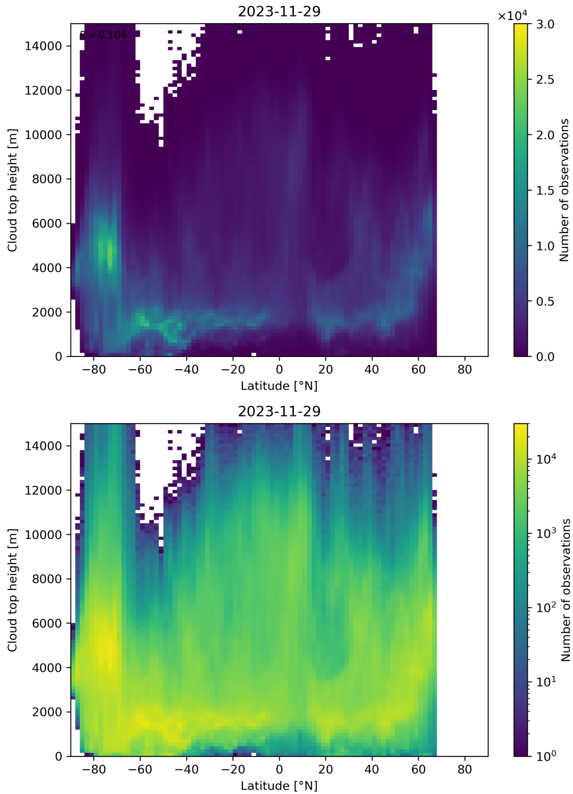
Figure 97: Scatter density plot of “Latitude” against “Cloud top height” for 2023-11-28 to 2023-11-30.
