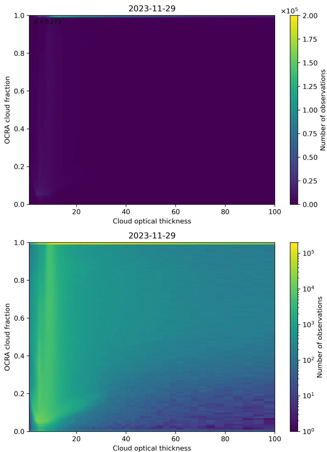
Figure 83: Scatter density plot of “Cloud optical thickness” against “OCRA cloud fraction” for 2023-11-28 to 2023-11-30.
