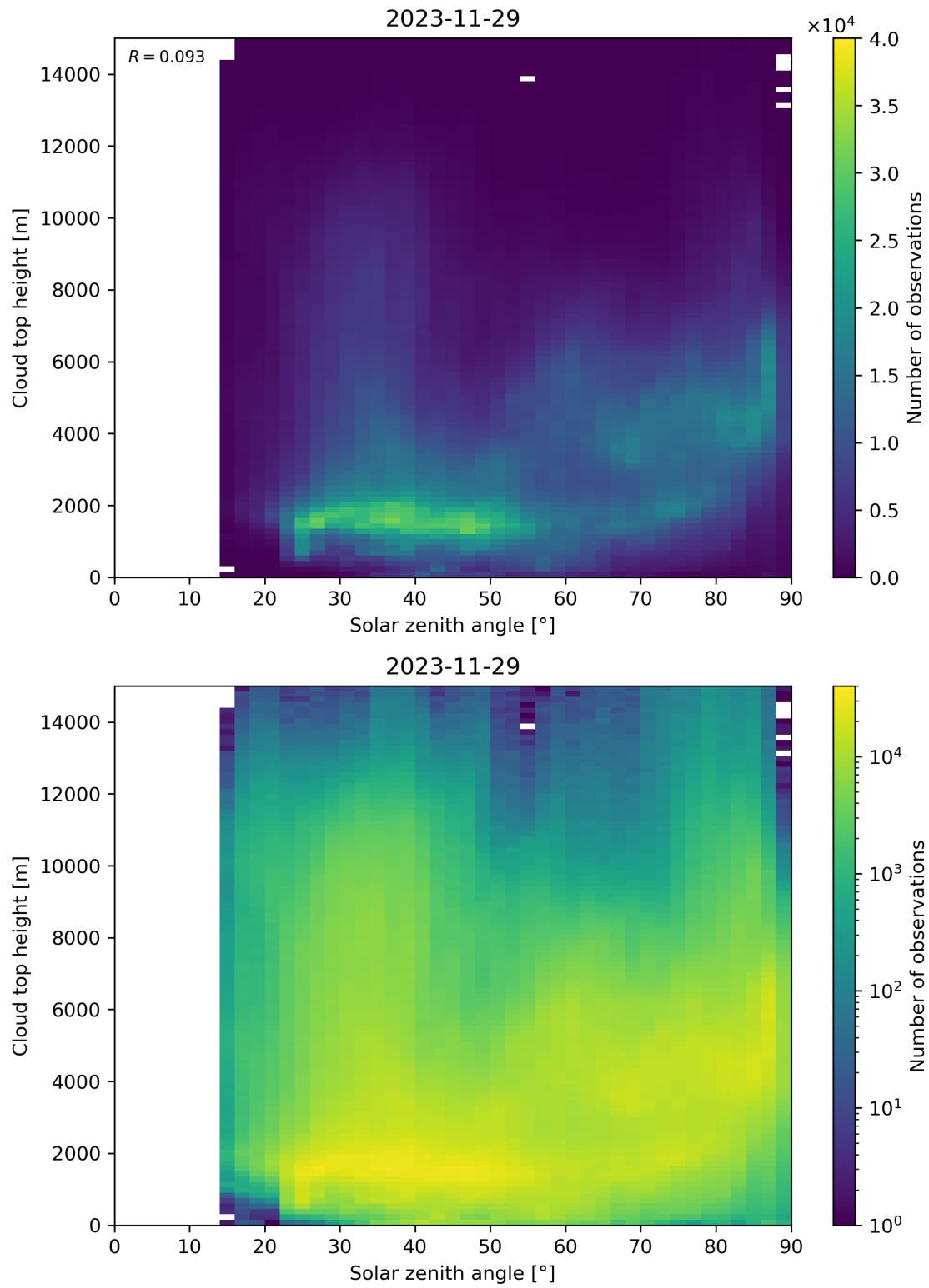
Figure 104: Scatter density plot of “Solar zenith angle” against “Cloud top height” for 2023-11-28 to 2023-11-30.
