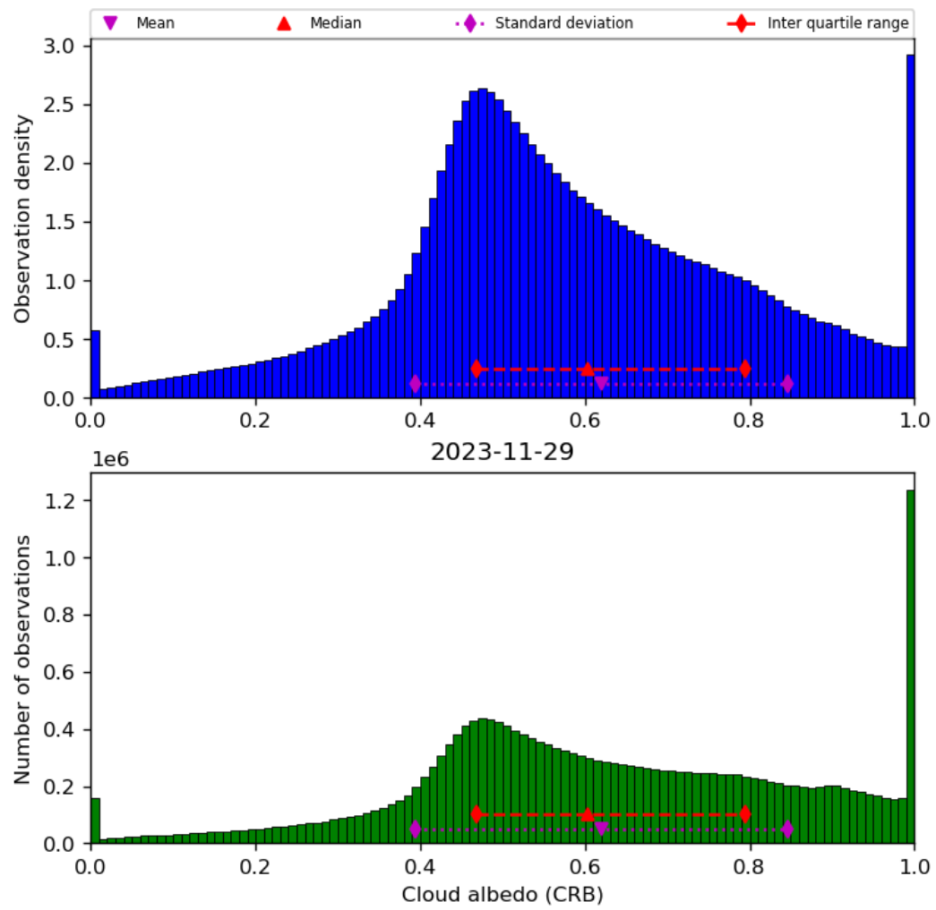
Figure 44: Histogram of “Cloud albedo (CRB)” for 2023-11-28 to 2023-11-30
