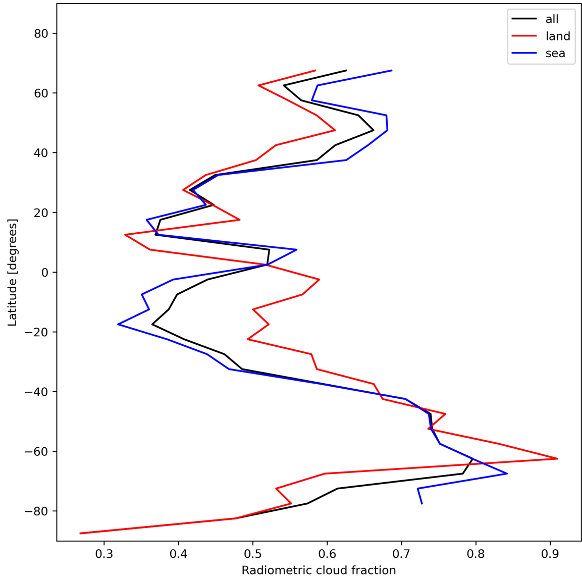
Figure 23: Zonal average of “Radiometric cloud fraction” for 2023-11-28 to 2023-11-30.
