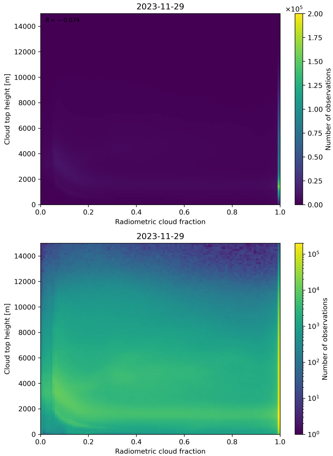
Figure 76: Scatter density plot of “Radiometric cloud fraction” against “Cloud top height” for 2023-11-28 to 2023-11-30.
