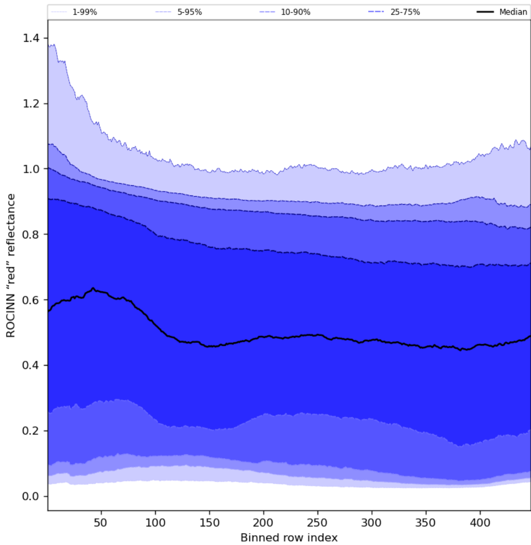
Figure 69: Along track statistics of “ROCINN “red” reflectance” for 2023-11-28 to 2023-11-30
