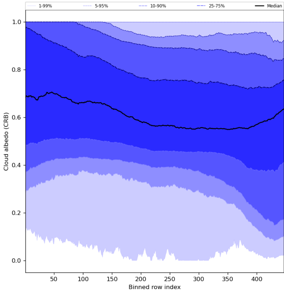
Figure 60: Along track statistics of “Cloud albedo (CRB)” for 2023-11-28 to 2023-11-30
