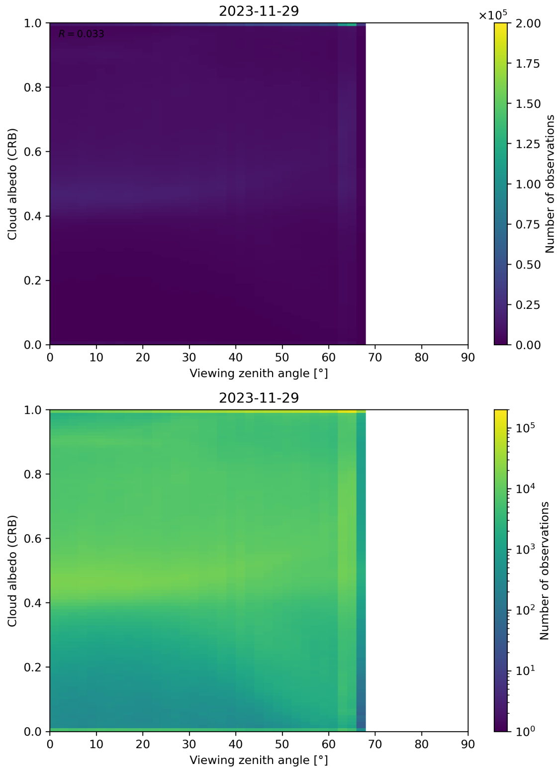
Figure 106: Scatter density plot of “Viewing zenith angle” against “Cloud albedo (CRB)” for 2023-11-28 to 2023-11-30.
