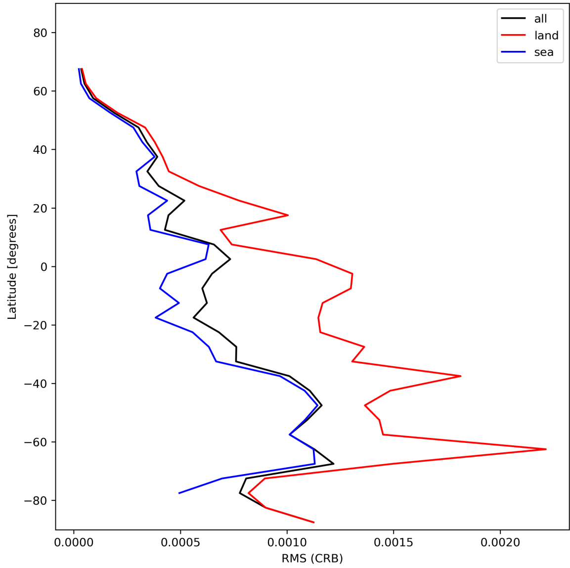
Figure 32: Zonal average of “RMS (CRB)” for 2023-11-28 to 2023-11-30.
