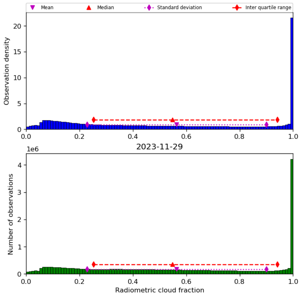
Figure 39: Histogram of “Radiometric cloud fraction” for 2023-11-28 to 2023-11-30
