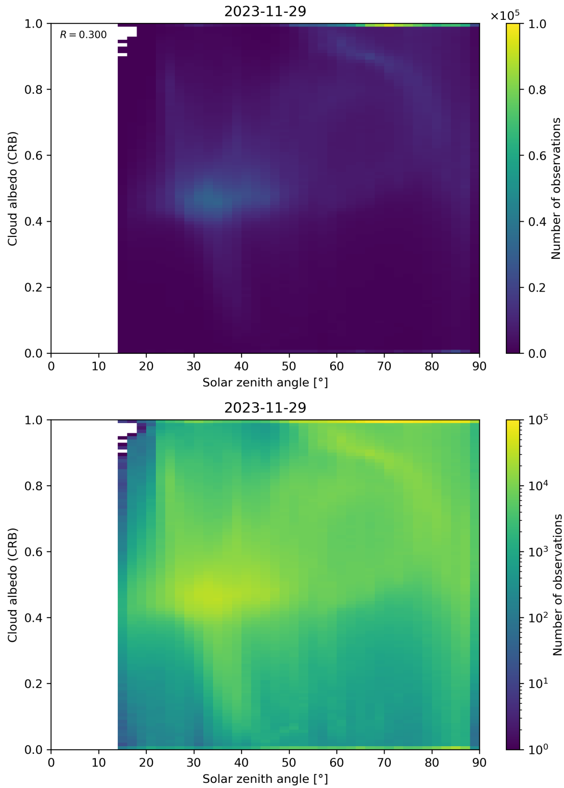
Figure 98: Scatter density plot of “Solar zenith angle” against “Cloud albedo (CRB)” for 2023-11-28 to 2023-11-30.
