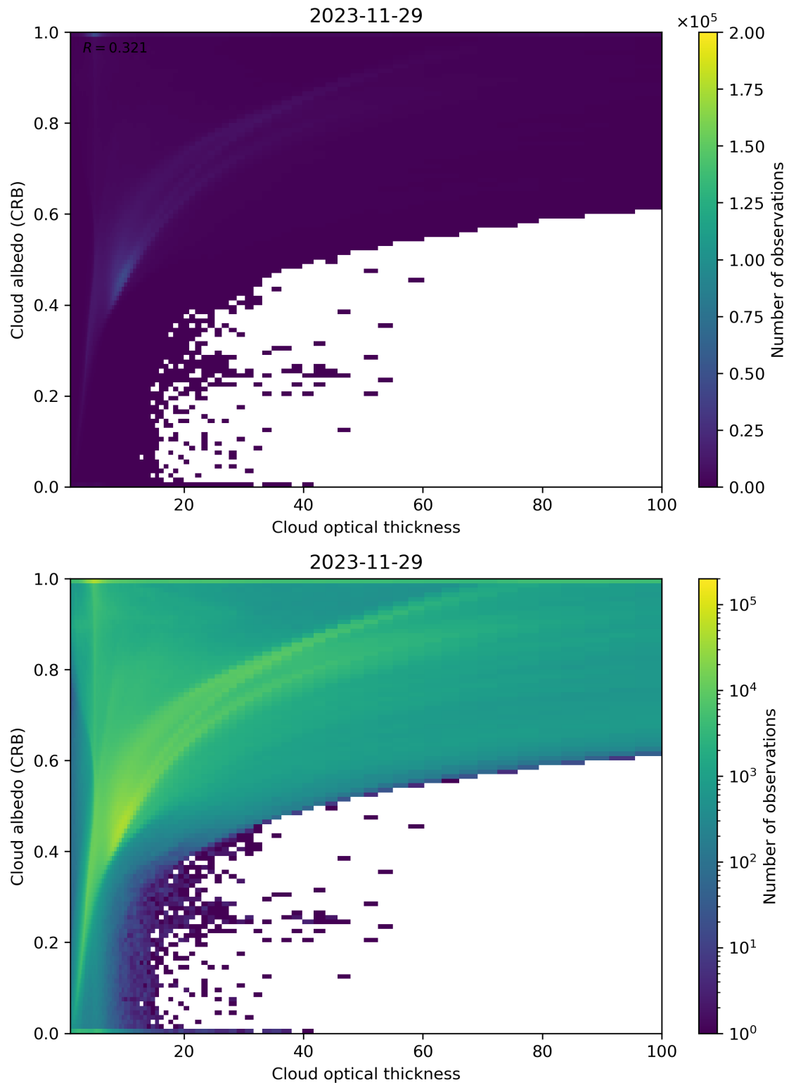
Figure 82: Scatter density plot of “Cloud optical thickness” against “Cloud albedo (CRB)” for 2023-11-28 to 2023-11-30.
