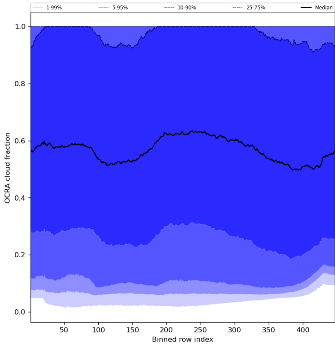
Figure 66: Along track statistics of “OCRA cloud fraction” for 2023-11-28 to 2023-11-30
