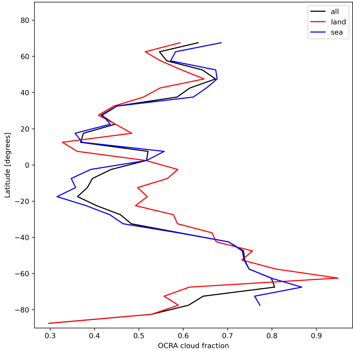
Figure 34: Zonal average of “OCRA cloud fraction” for 2023-11-28 to 2023-11-30.
