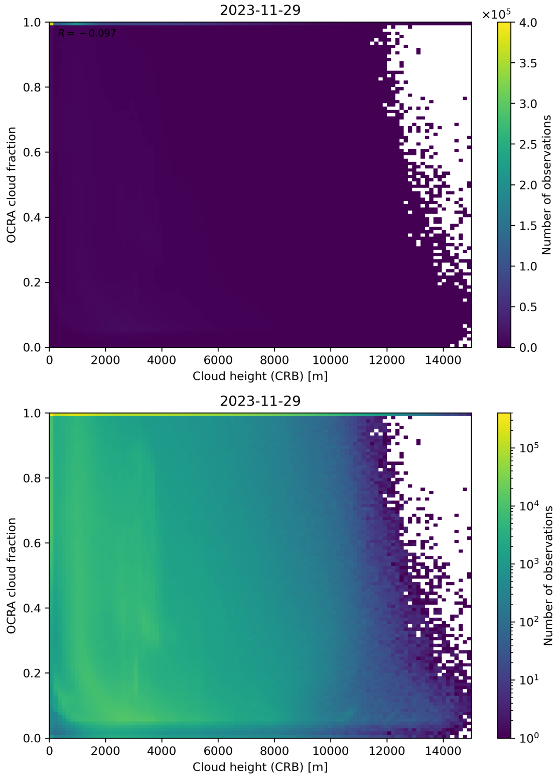
Figure 81: Scatter density plot of “Cloud height (CRB)” against “OCRA cloud fraction” for 2023-11-28 to 2023-11-30.
