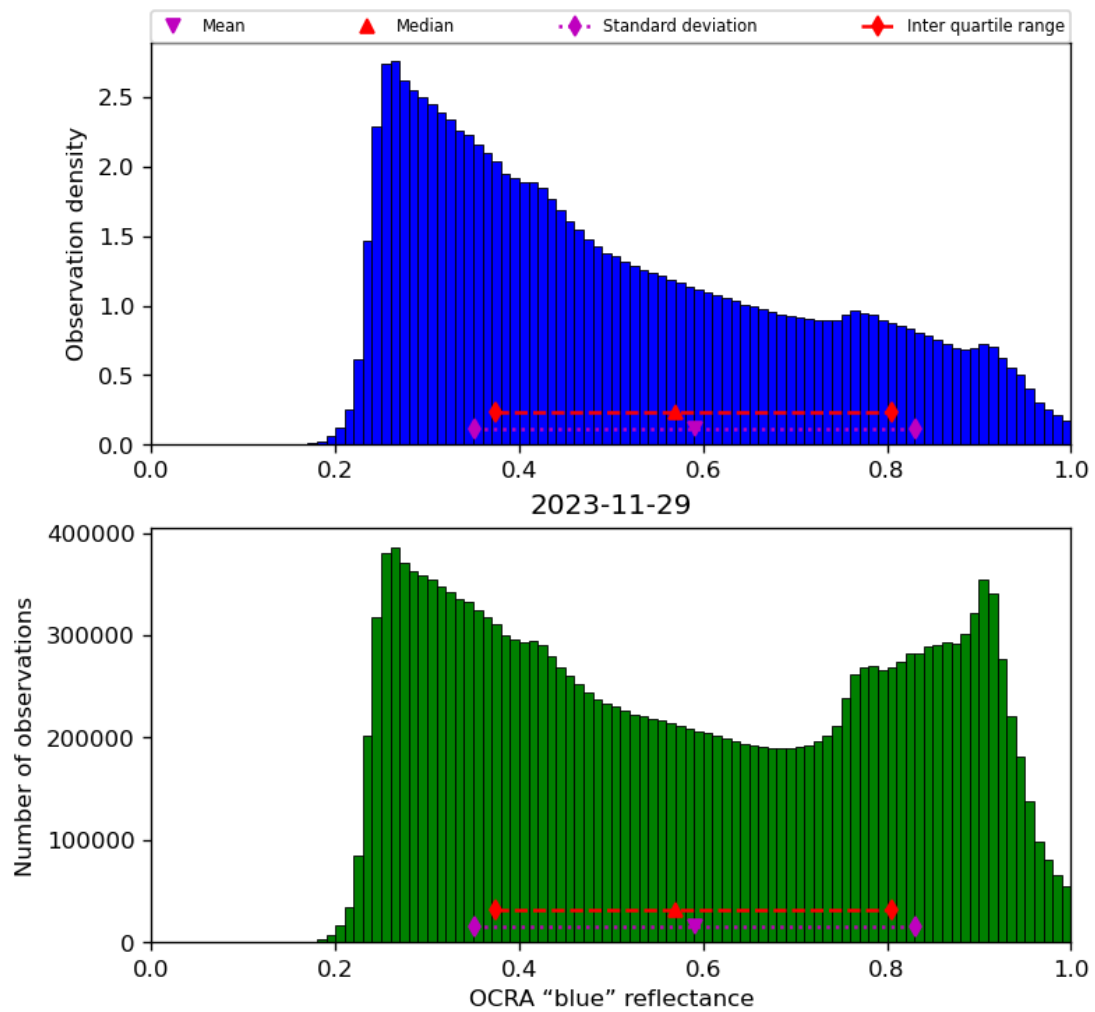
Figure 51: Histogram of “OCRA “blue” reflectance” for 2023-11-28 to 2023-11-30
