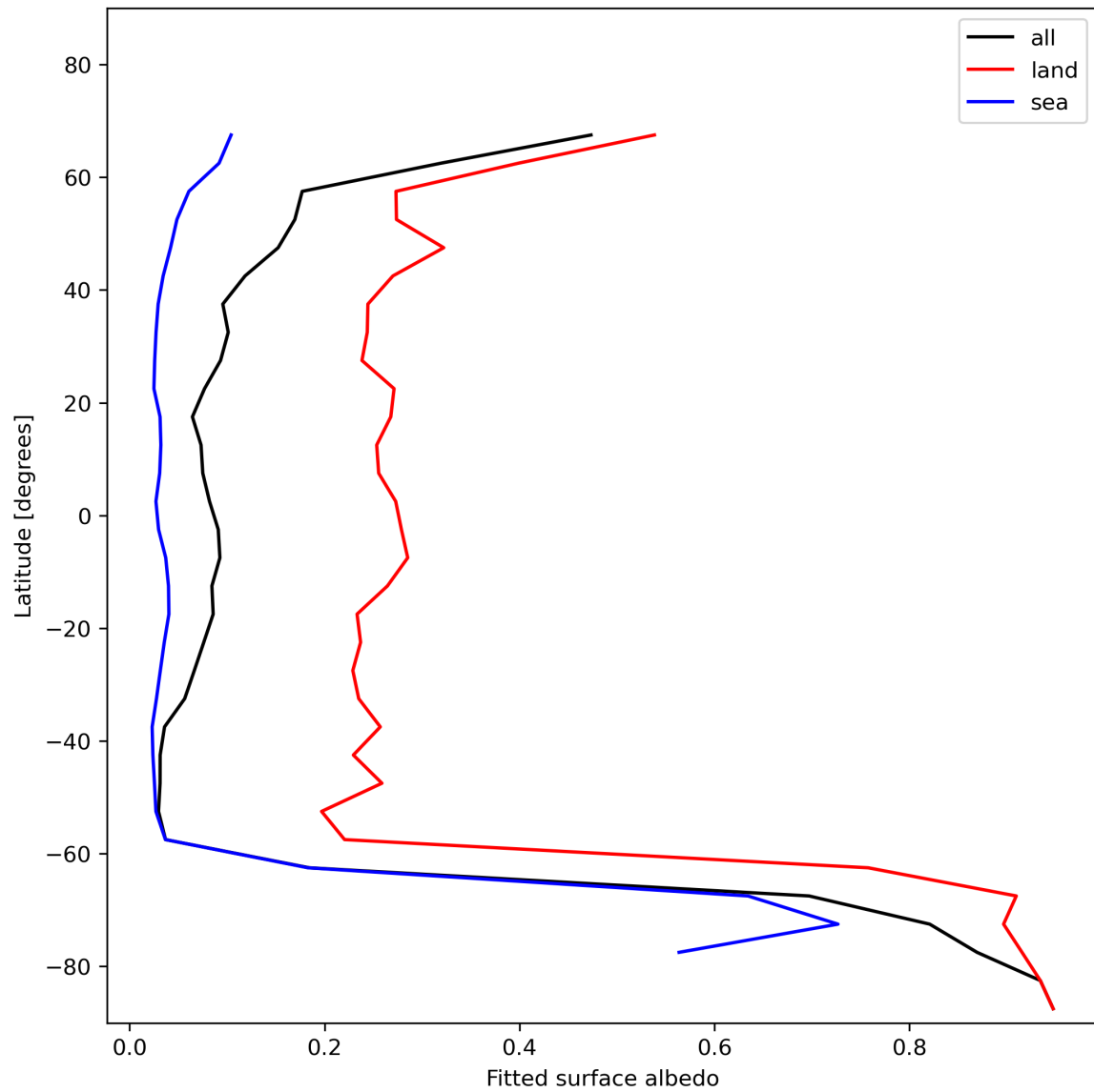
Figure 29: Zonal average of “Fitted surface albedo” for 2023-11-28 to 2023-11-30.
