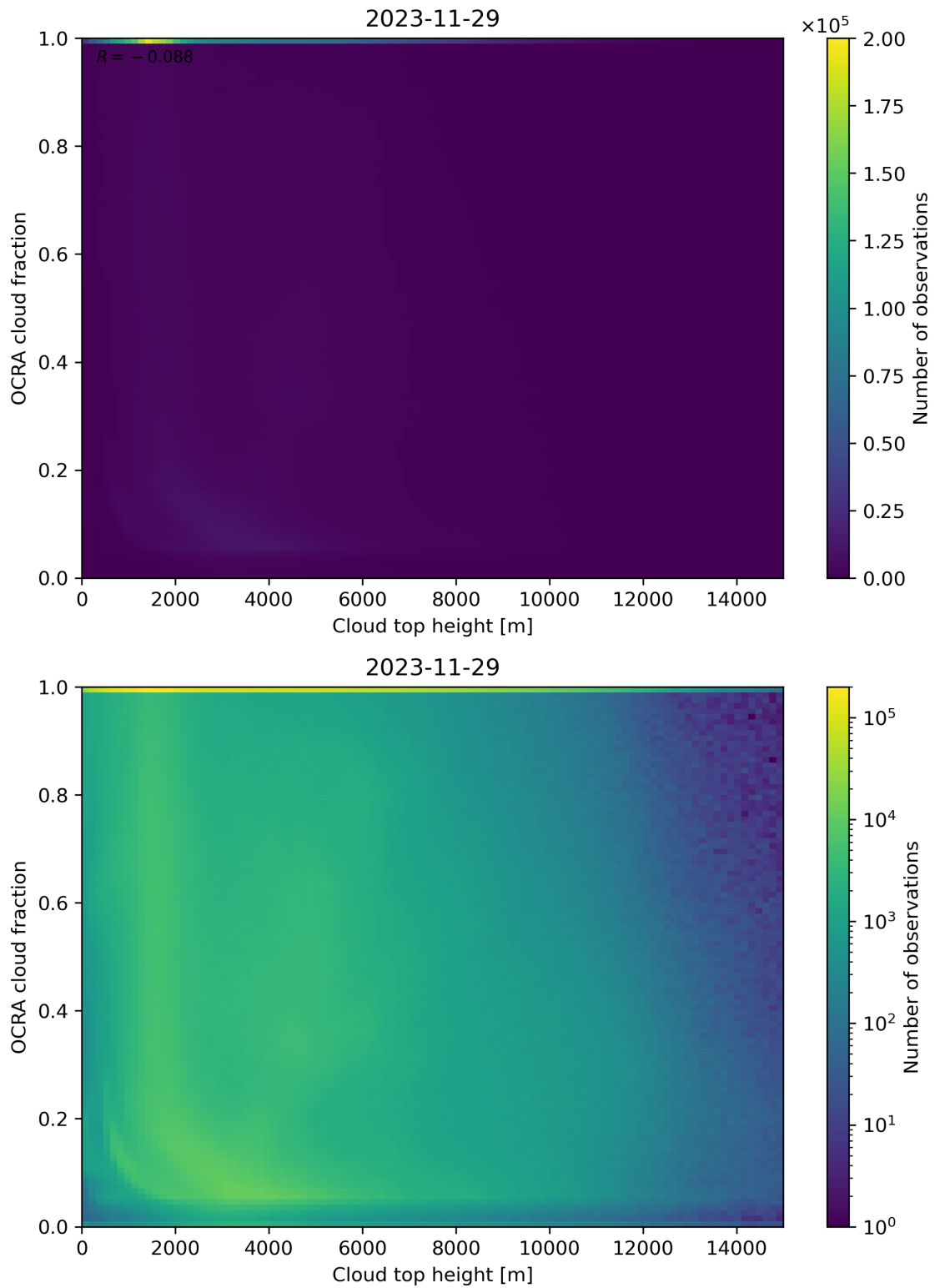
Figure 87: Scatter density plot of “Cloud top height” against “OCRA cloud fraction” for 2023-11-28 to 2023-11-30.
