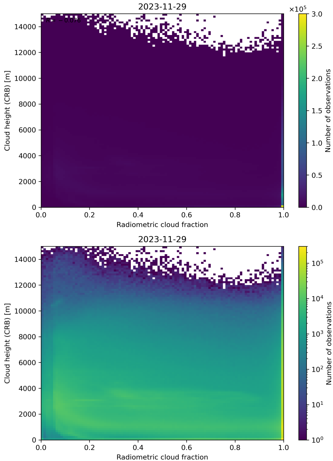
Figure 74: Scatter density plot of “Radiometric cloud fraction” against “Cloud height (CRB)” for 2023-11-28 to 2023-11-30.
