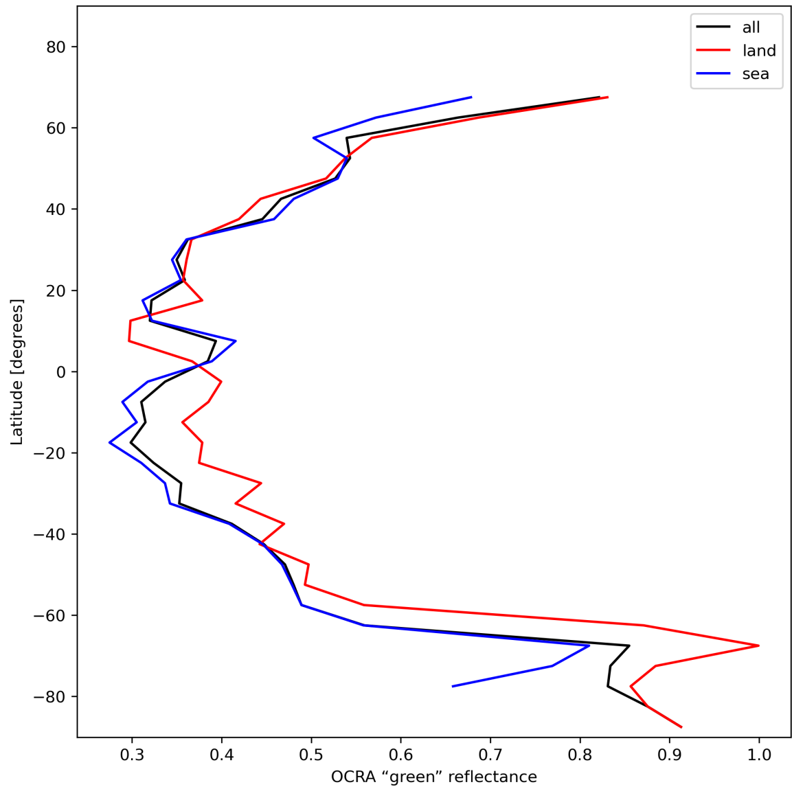
Figure 36: Zonal average of “OCRA “green” reflectance” for 2023-11-28 to 2023-11-30.
