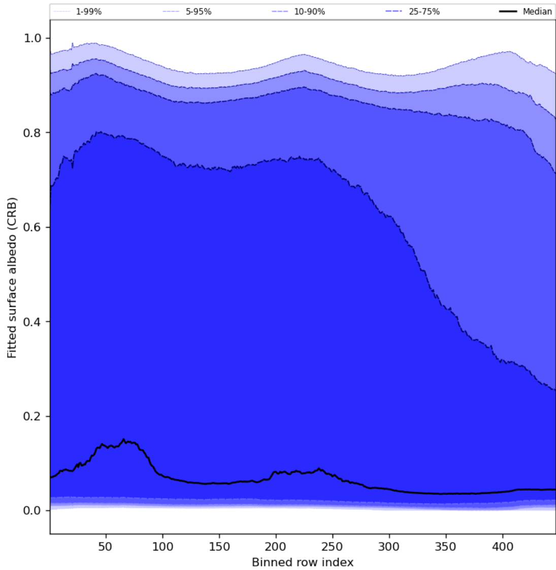
Figure 62: Along track statistics of “Fitted surface albedo (CRB)” for 2023-11-28 to 2023-11-30
