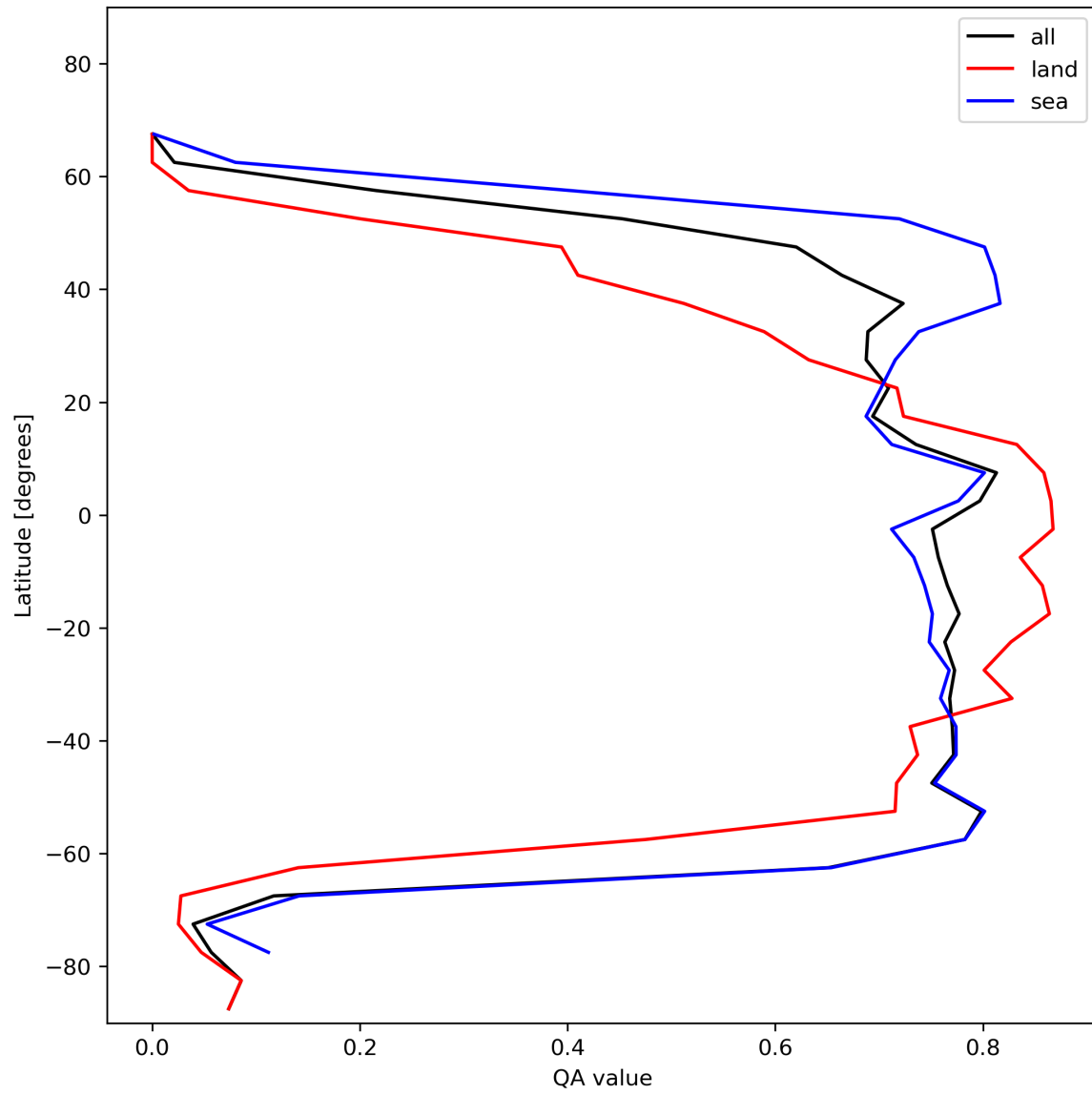
Figure 22: Zonal average of “QA value” for 2023-11-28 to 2023-11-30.
