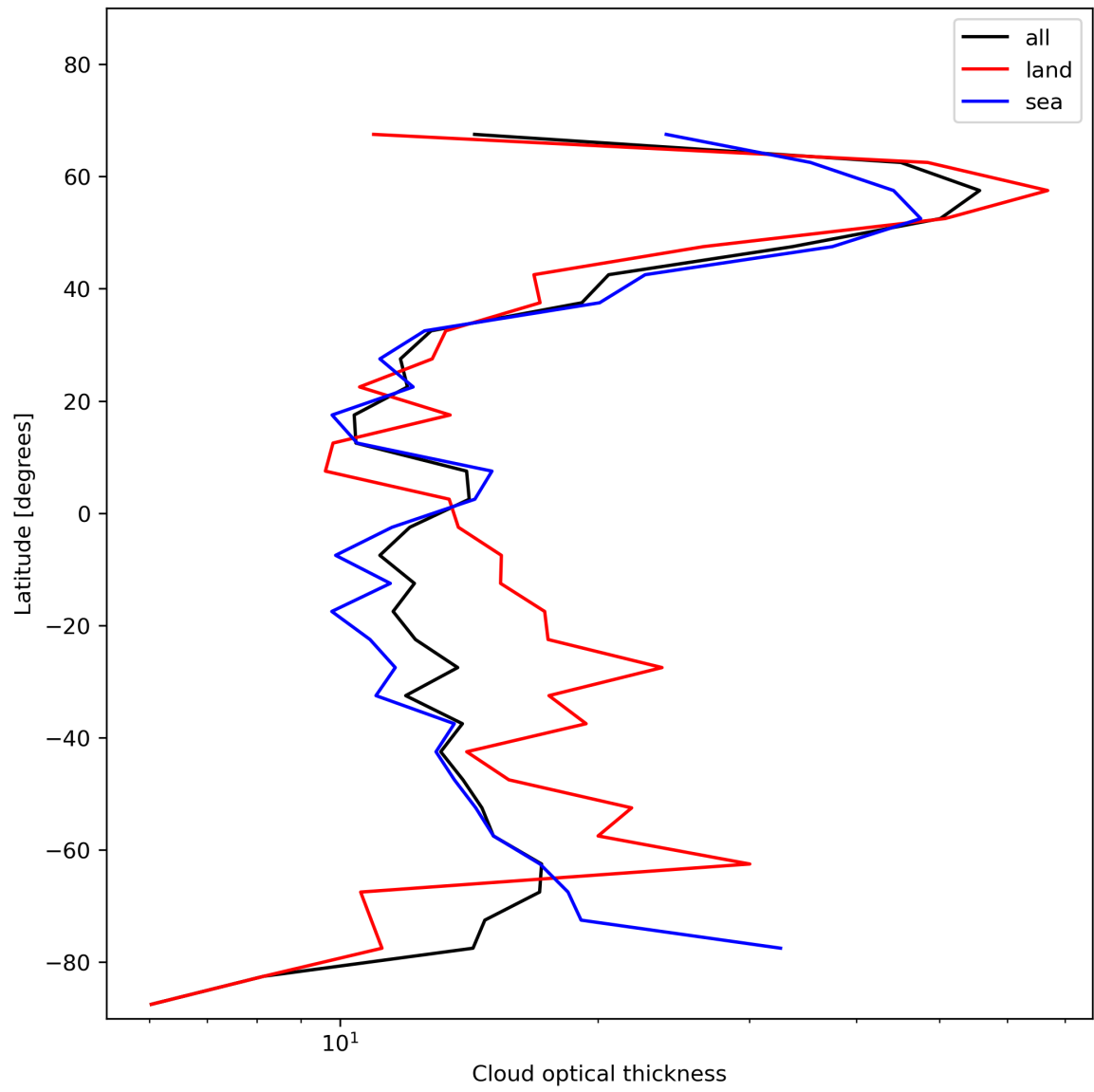
Figure 25: Zonal average of “Cloud optical thickness” for 2023-11-28 to 2023-11-30.
