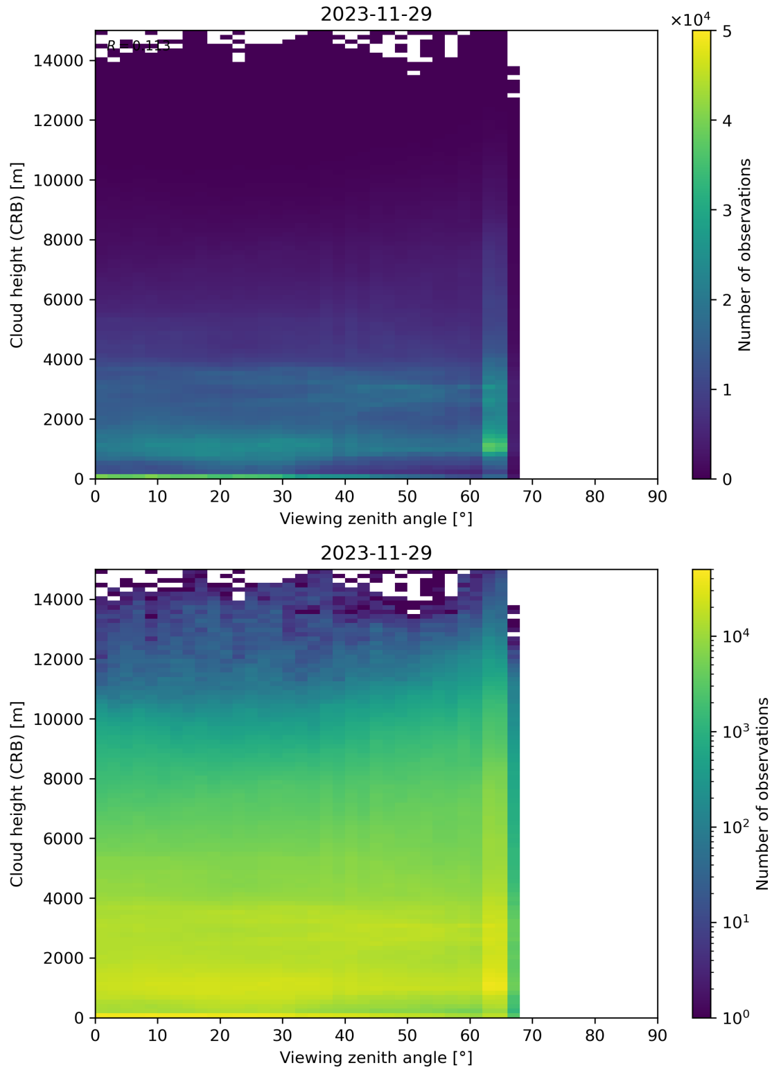
Figure 110: Scatter density plot of “Viewing zenith angle” against “Cloud height (CRB)” for 2023-11-28 to 2023-11-30.
