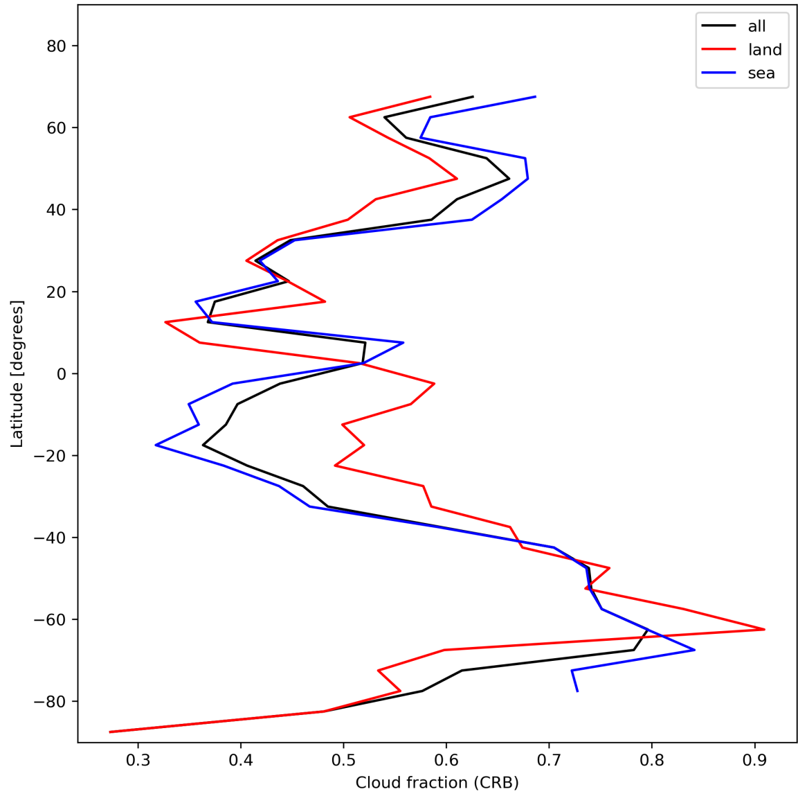
Figure 26: Zonal average of “Cloud fraction (CRB)” for 2023-11-28 to 2023-11-30.
