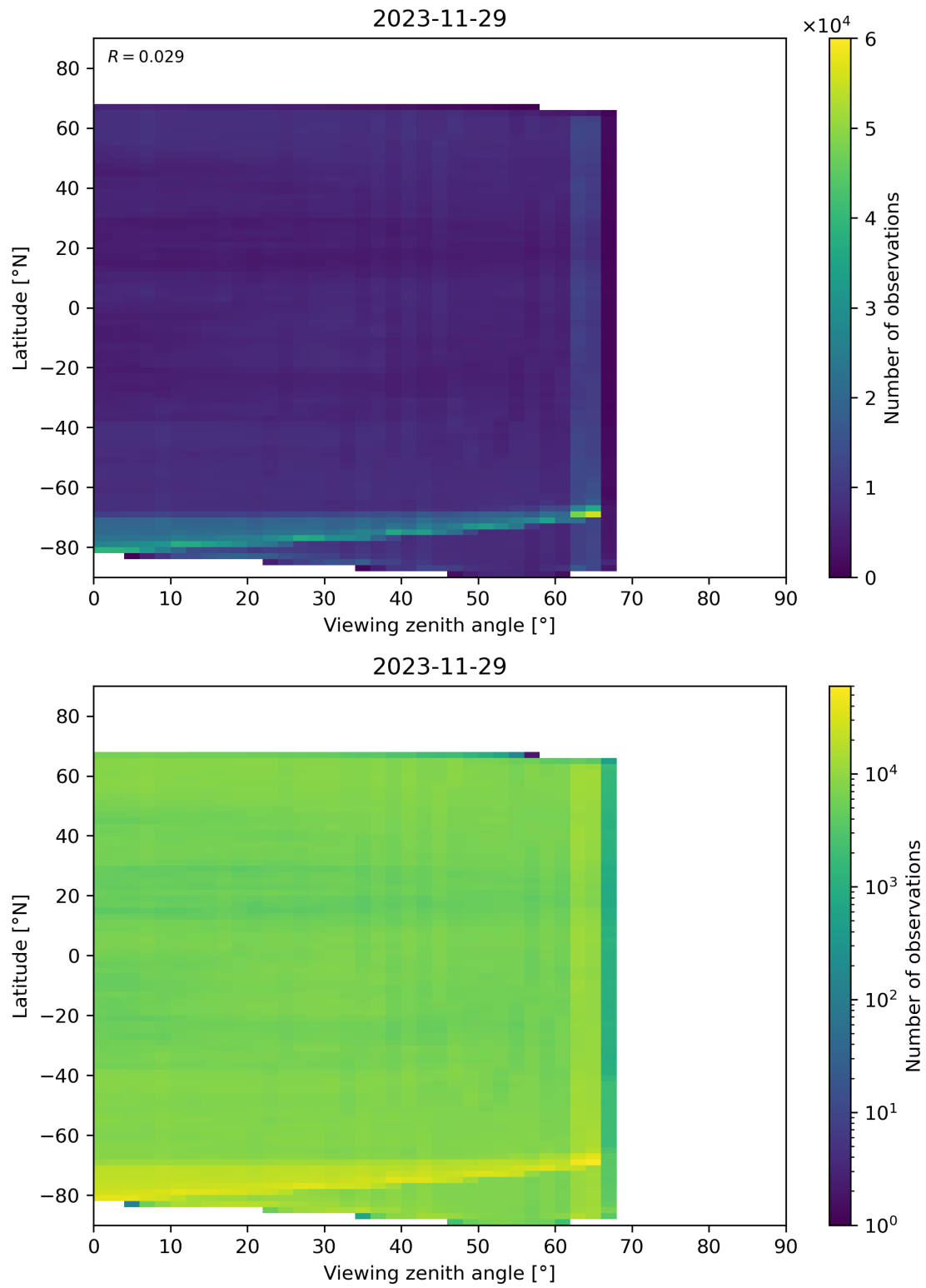
Figure 113: Scatter density plot of “Viewing zenith angle” against “Latitude” for 2023-11-28 to 2023-11-30.
