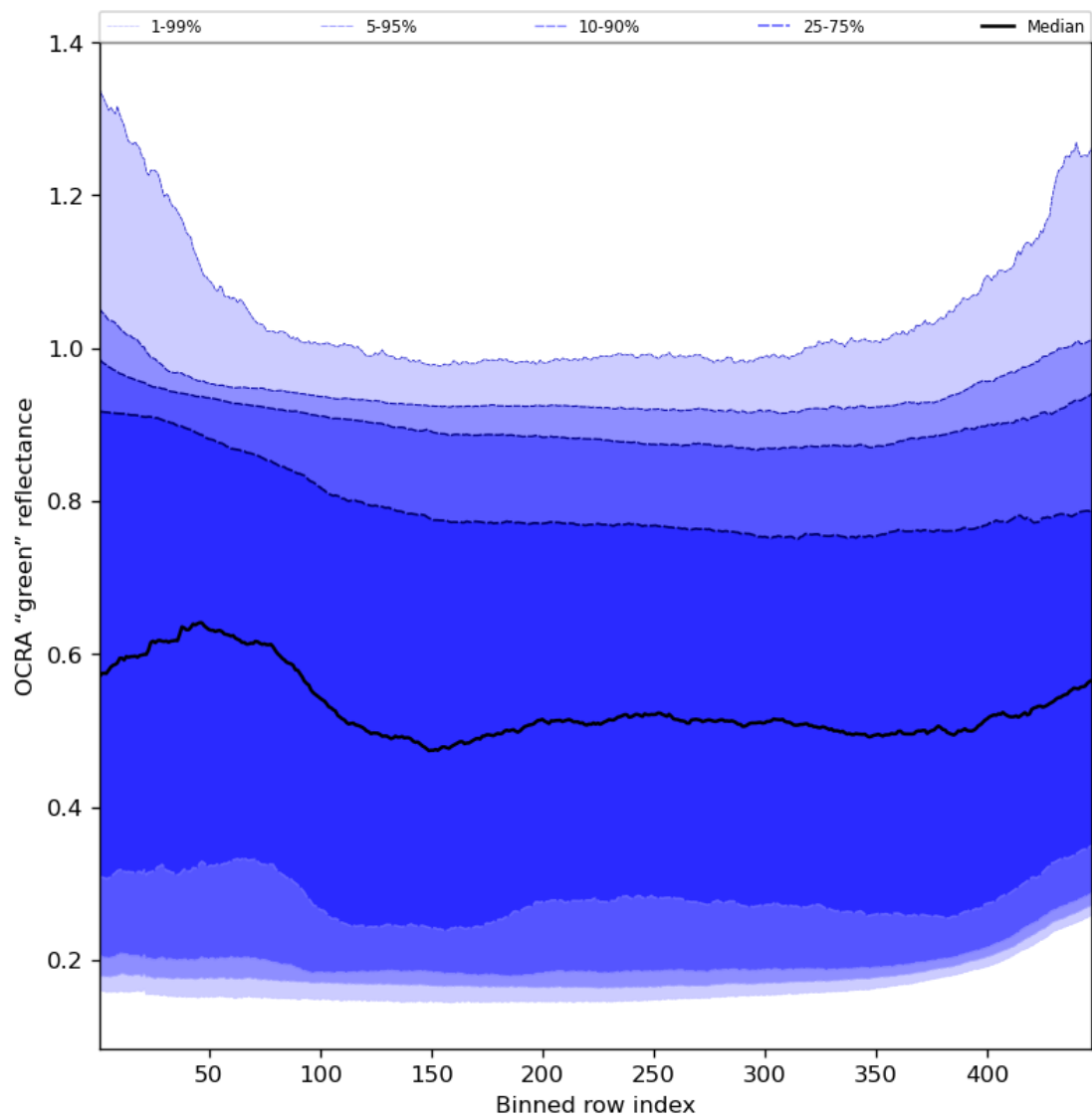
Figure 68: Along track statistics of “OCRA “green” reflectance” for 2023-11-28 to 2023-11-30
