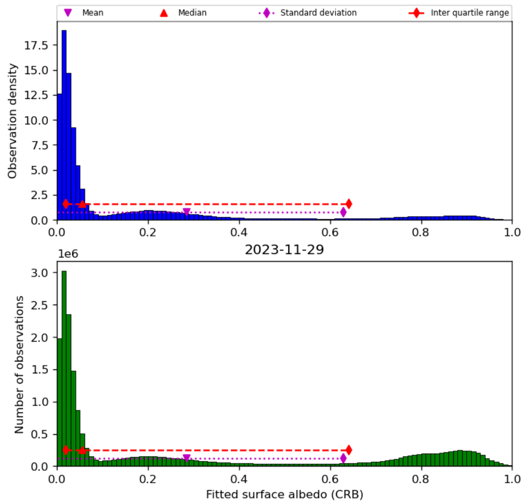
Figure 46: Histogram of “Fitted surface albedo (CRB)” for 2023-11-28 to 2023-11-30
