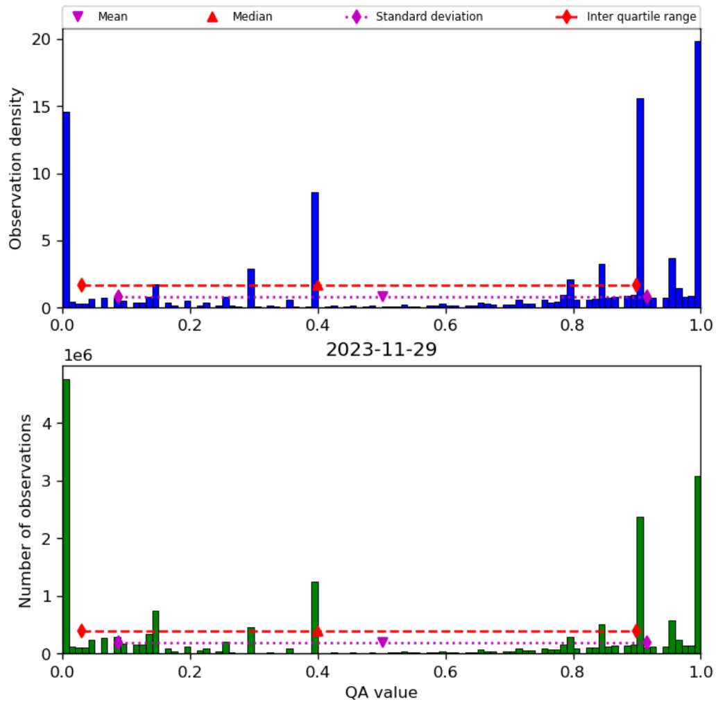
Figure 38: Histogram of “QA value” for 2023-11-28 to 2023-11-30
