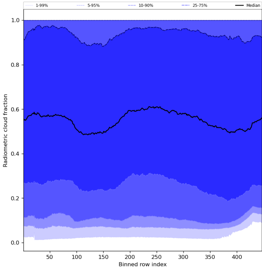
Figure 55: Along track statistics of “Radiometric cloud fraction” for 2023-11-28 to 2023-11-30
