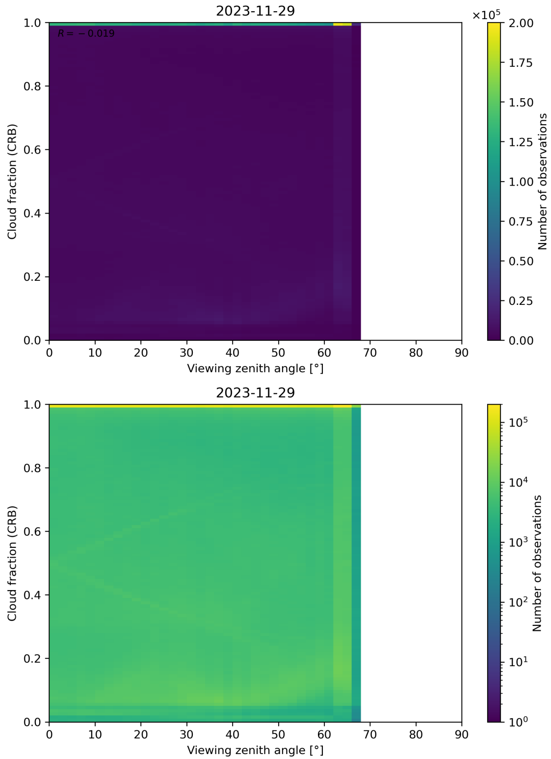
Figure 109: Scatter density plot of “Viewing zenith angle” against “Cloud fraction (CRB)” for 2023-11-28 to 2023-11-30.
