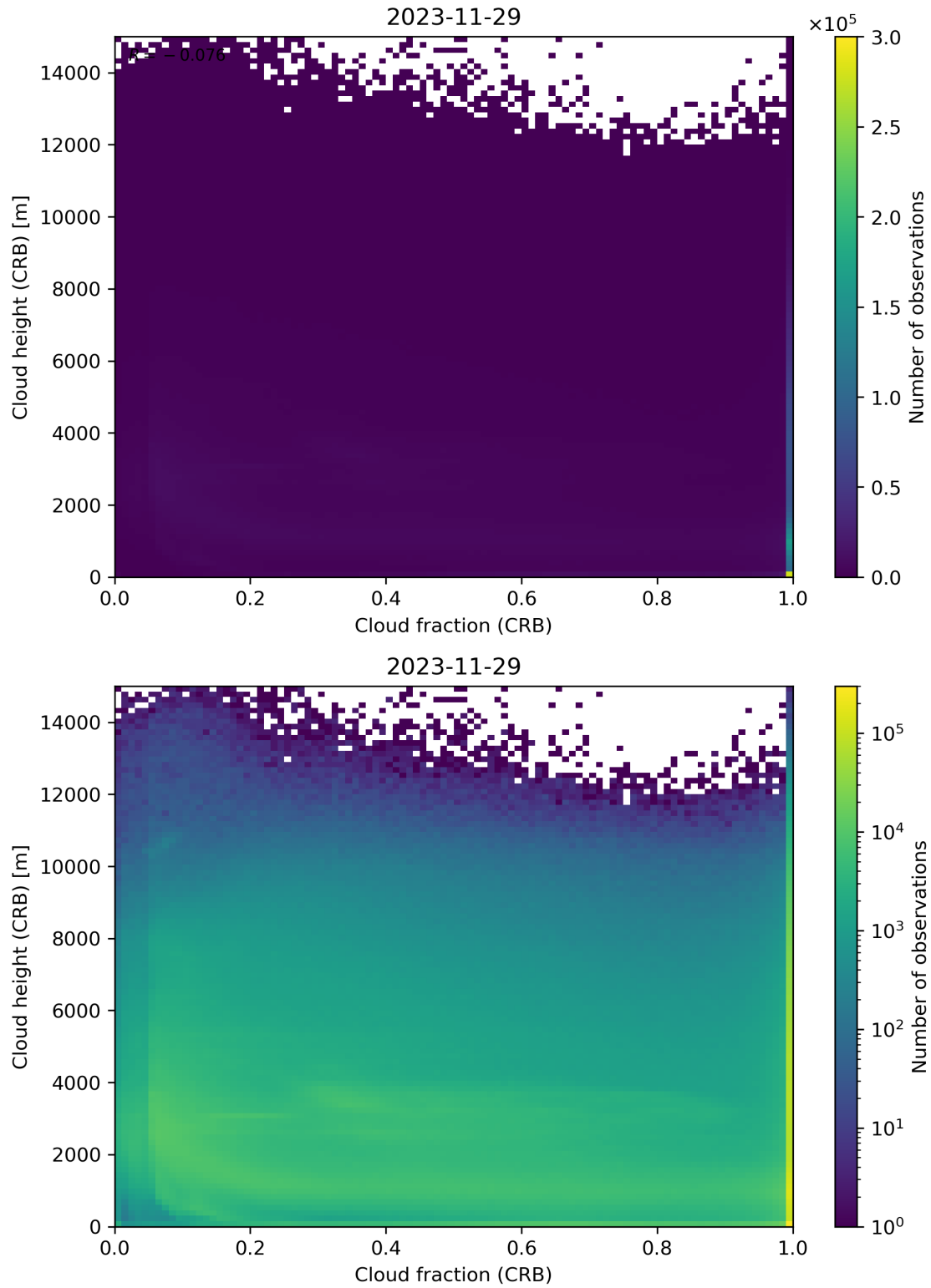
Figure 79: Scatter density plot of “Cloud fraction (CRB)” against “Cloud height (CRB)” for 2023-11-28 to 2023-11-30.
