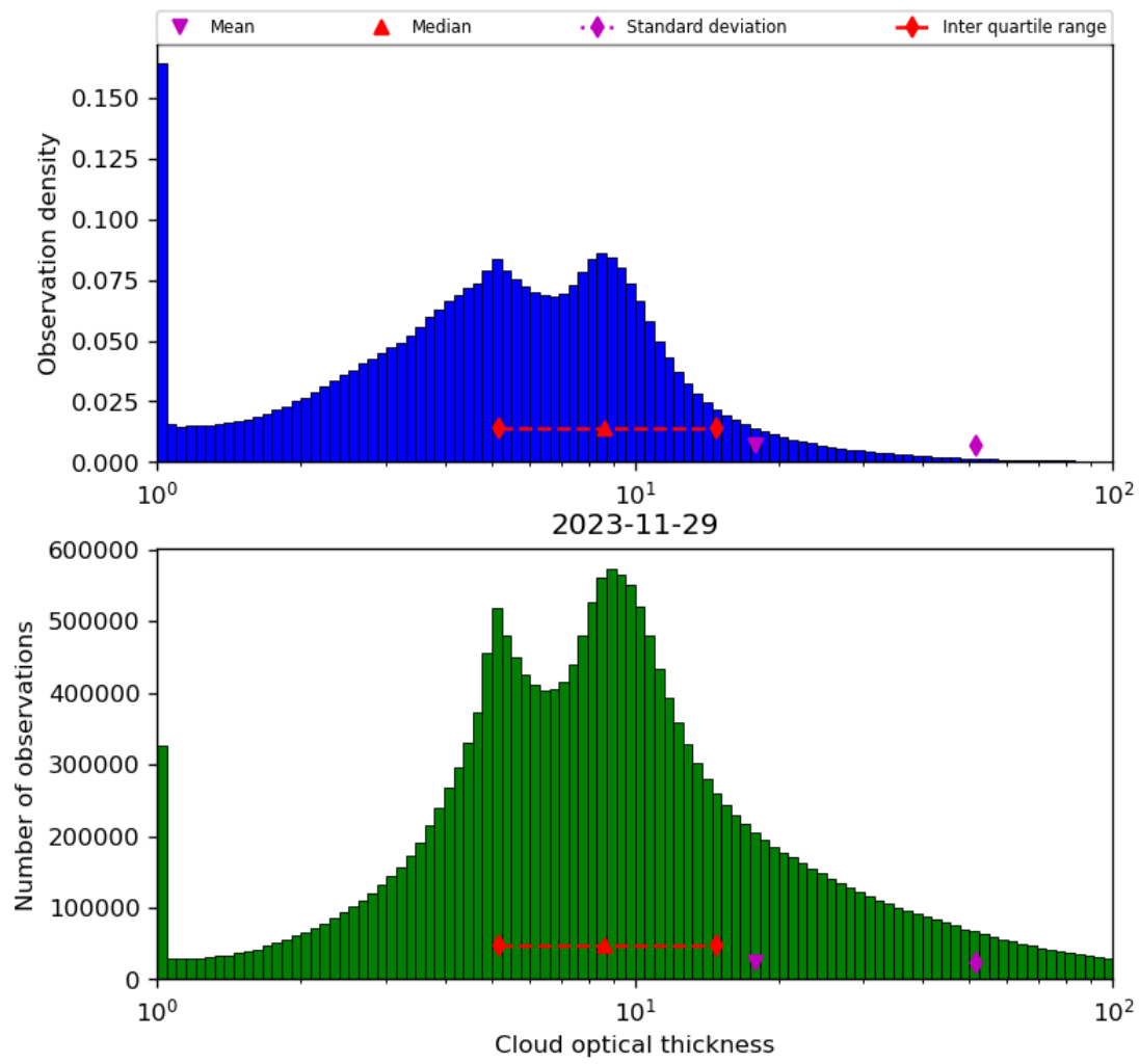
Figure 41: Histogram of “Cloud optical thickness” for 2023-11-28 to 2023-11-30
