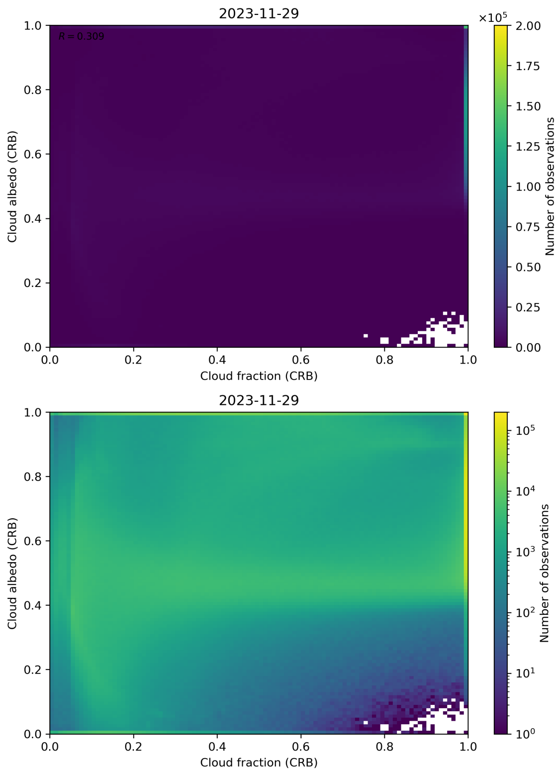
Figure 77: Scatter density plot of “Cloud fraction (CRB)” against “Cloud albedo (CRB)” for 2023-11-28 to 2023-11-30.
