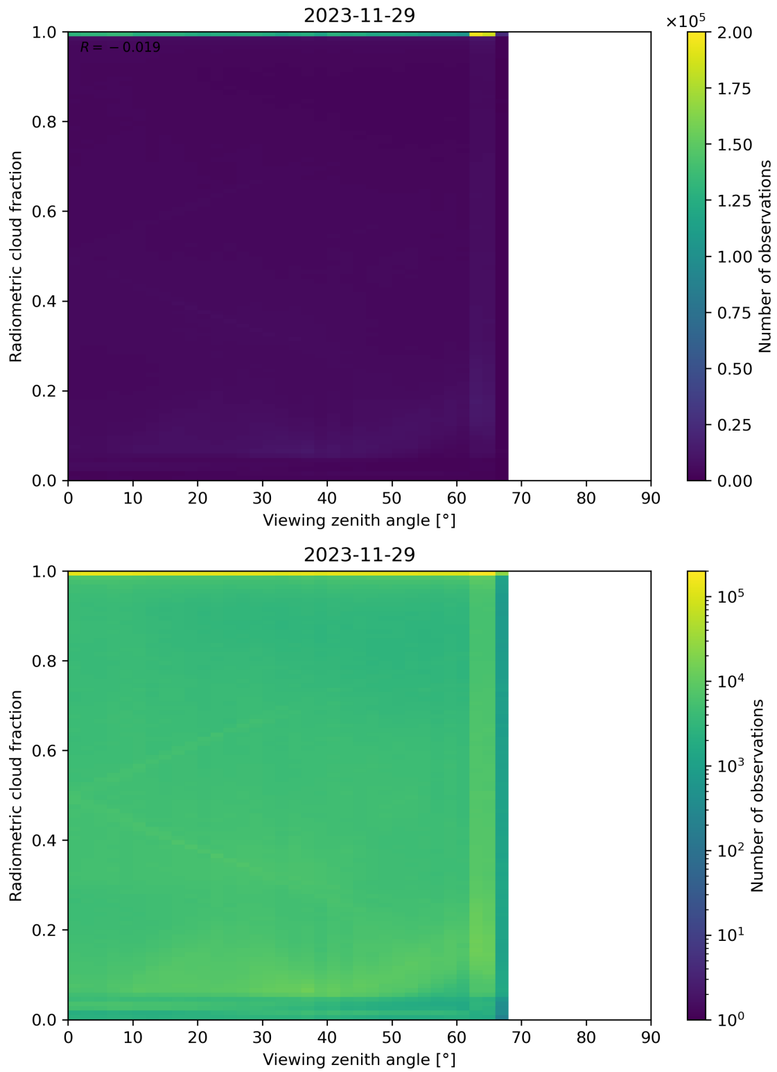
Figure 107: Scatter density plot of “Viewing zenith angle” against “Radiometric cloud fraction” for 2023-11-28 to 2023-11-30.
