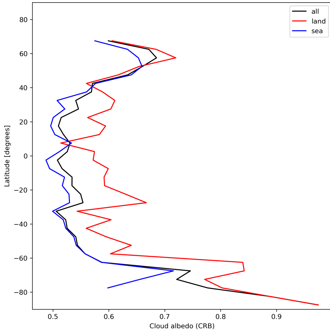
Figure 28: Zonal average of “Cloud albedo (CRB)” for 2023-11-28 to 2023-11-30.
