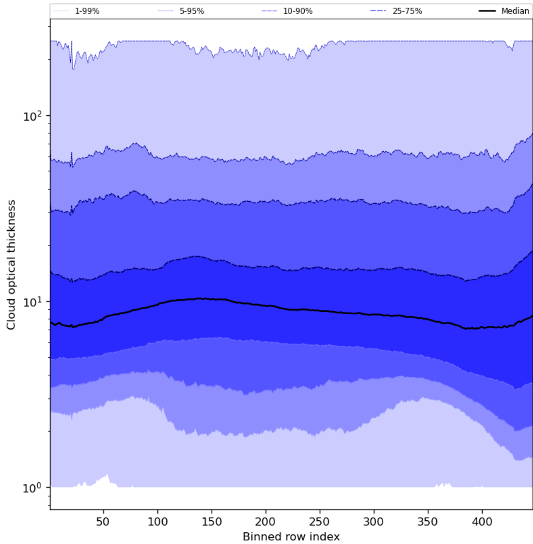
Figure 57: Along track statistics of “Cloud optical thickness” for 2023-11-28 to 2023-11-30
