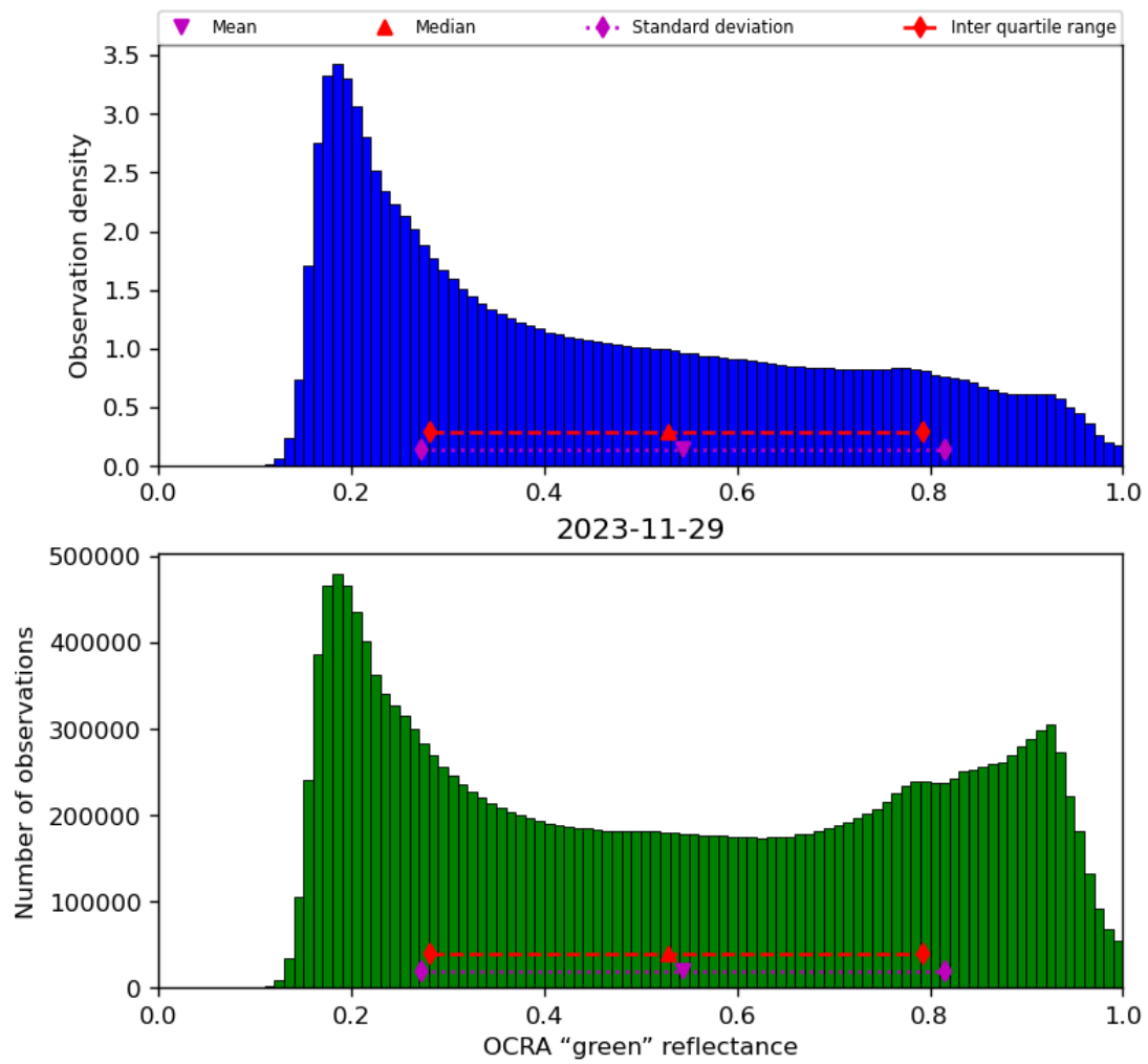
Figure 52: Histogram of “OCRA “green” reflectance” for 2023-11-28 to 2023-11-30
