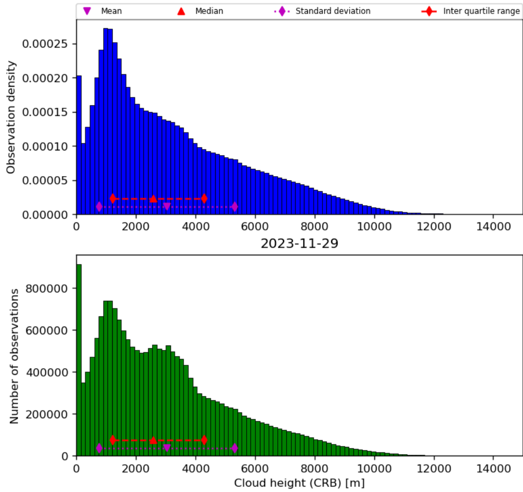
Figure 43: Histogram of “Cloud height (CRB)” for 2023-11-28 to 2023-11-30
