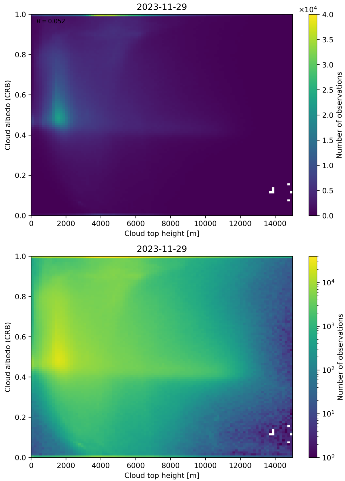
Figure 86: Scatter density plot of “Cloud top height” against “Cloud albedo (CRB)” for 2023-11-28 to 2023-11-30.
