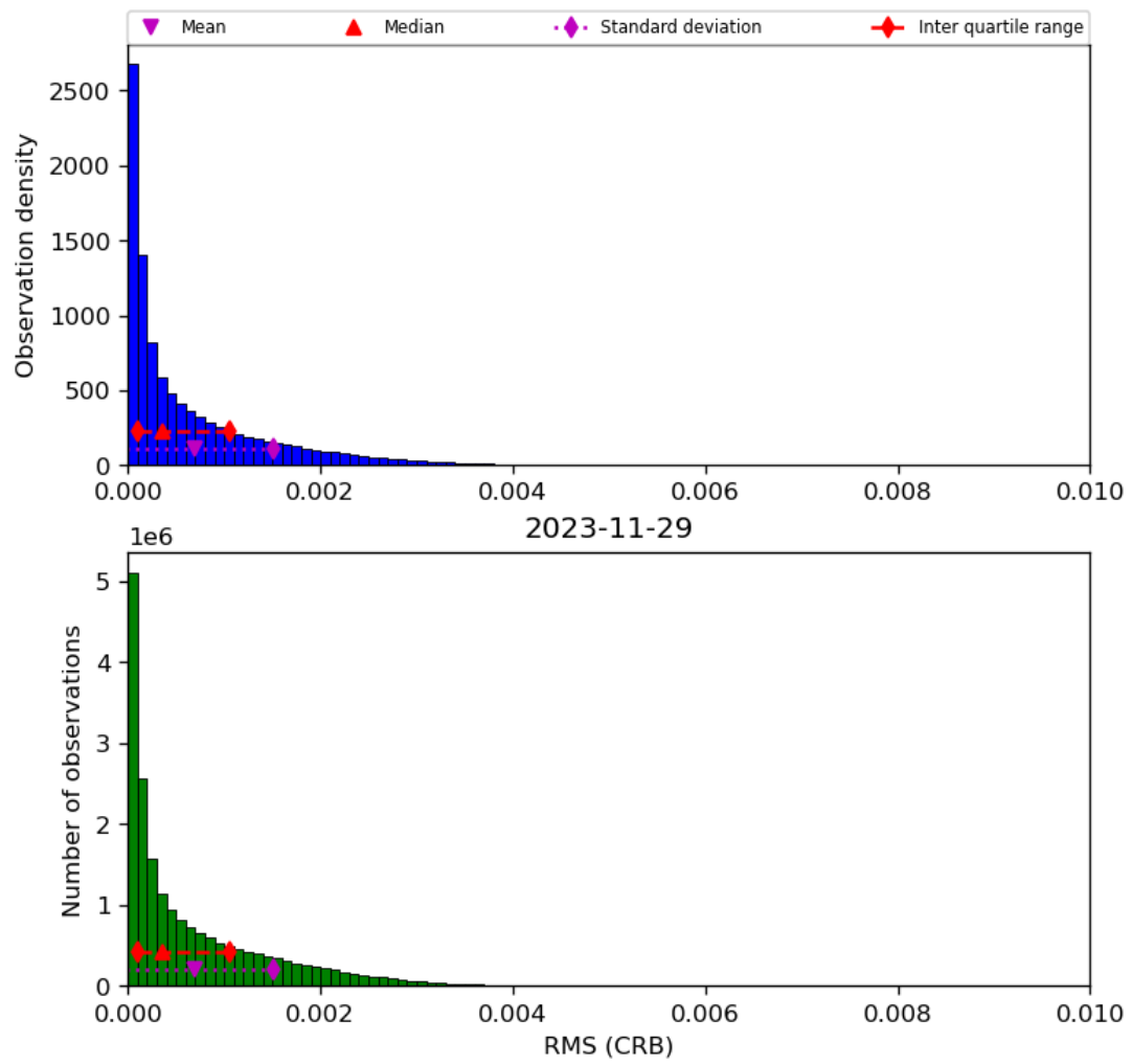
Figure 48: Histogram of “RMS (CRB)” for 2023-11-28 to 2023-11-30
