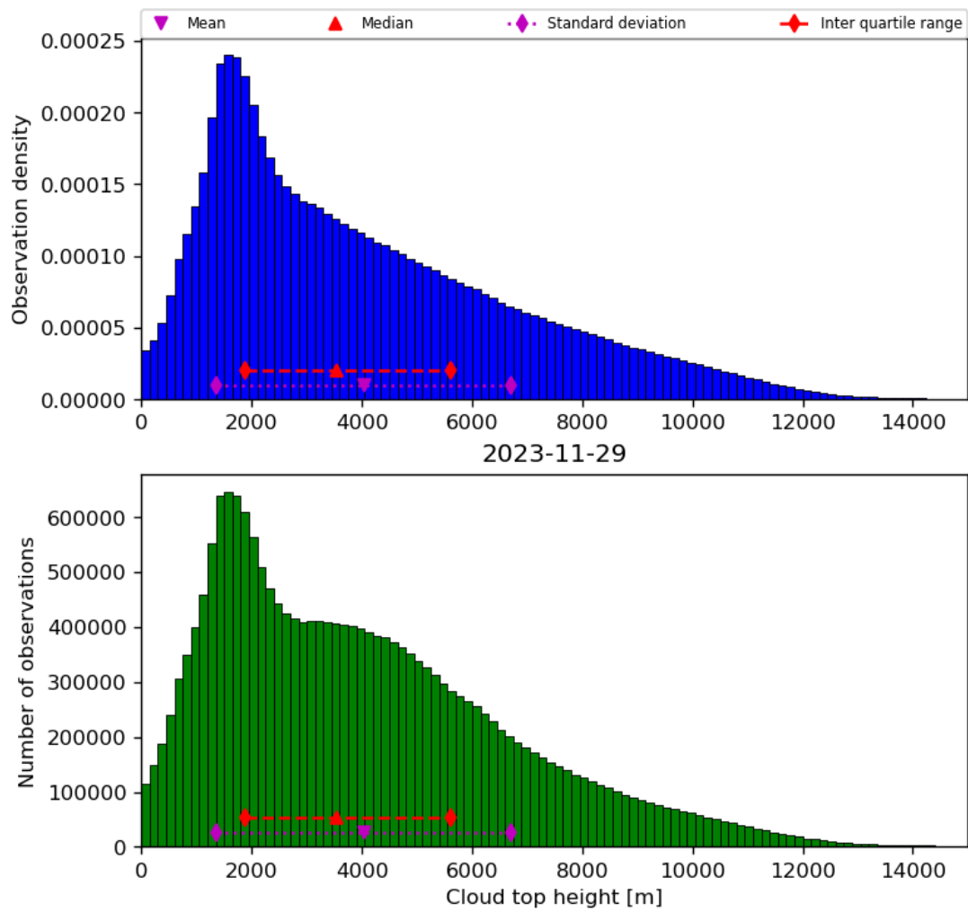
Figure 40: Histogram of “Cloud top height” for 2023-11-28 to 2023-11-30
