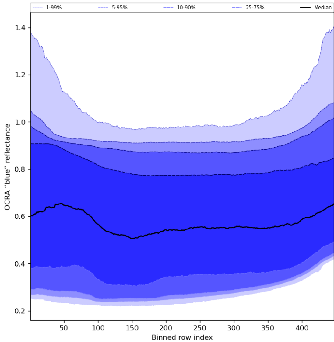
Figure 67: Along track statistics of “OCRA “blue” reflectance” for 2023-11-28 to 2023-11-30
