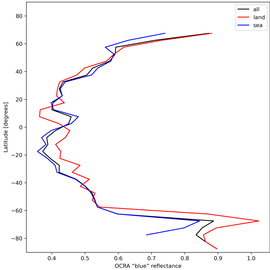
Figure 35: Zonal average of “OCRA “blue” reflectance” for 2023-11-28 to 2023-11-30.
