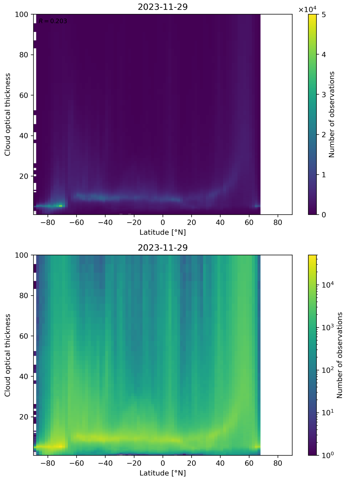
Figure 96: Scatter density plot of “Latitude” against “Cloud optical thickness” for 2023-11-28 to 2023-11-30.
