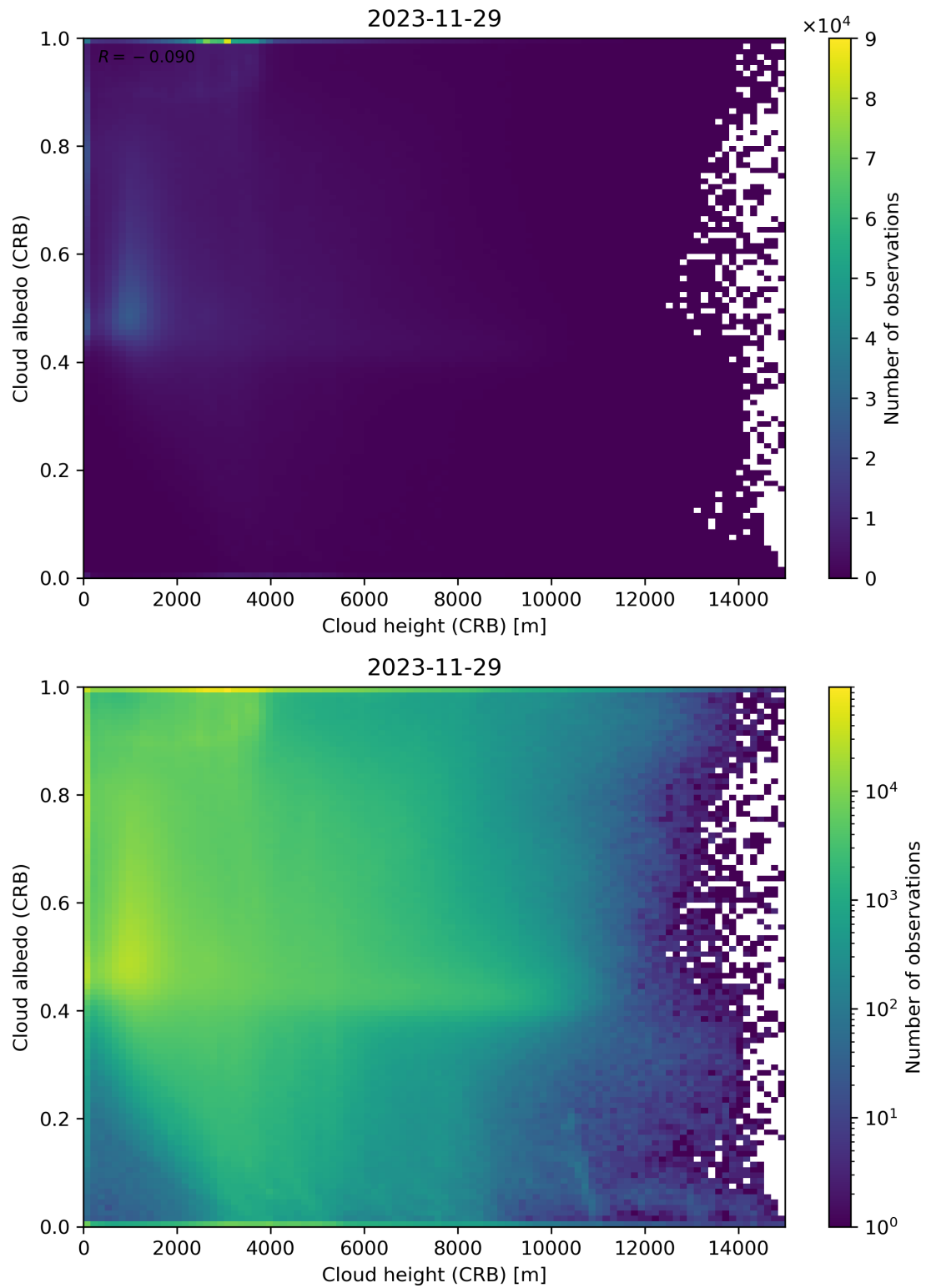
Figure 80: Scatter density plot of “Cloud height (CRB)” against “Cloud albedo (CRB)” for 2023-11-28 to 2023-11-30.
