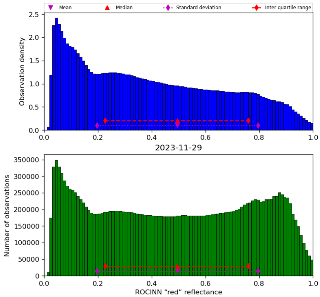
Figure 53: Histogram of “ROCINN “red” reflectance” for 2023-11-28 to 2023-11-30
