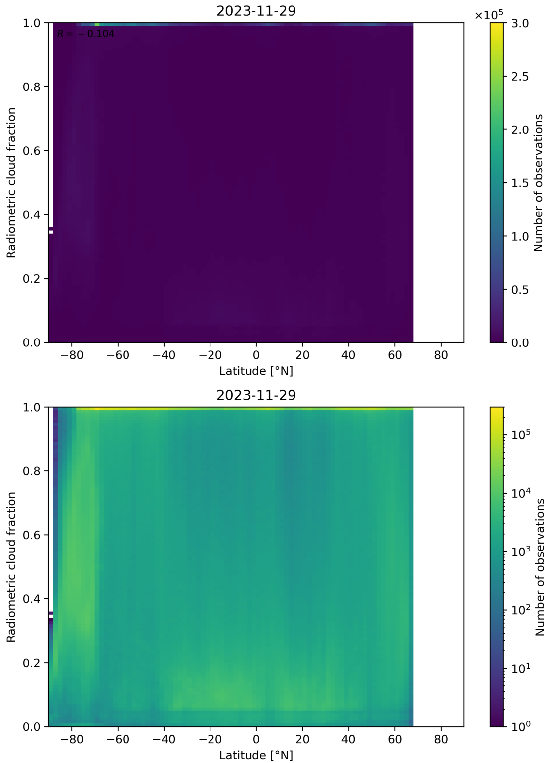
Figure 92: Scatter density plot of “Latitude” against “Radiometric cloud fraction” for 2023-11-28 to 2023-11-30.
