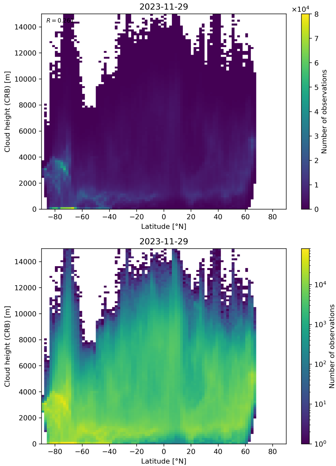
Figure 95: Scatter density plot of “Latitude” against “Cloud height (CRB)” for 2023-11-28 to 2023-11-30.
