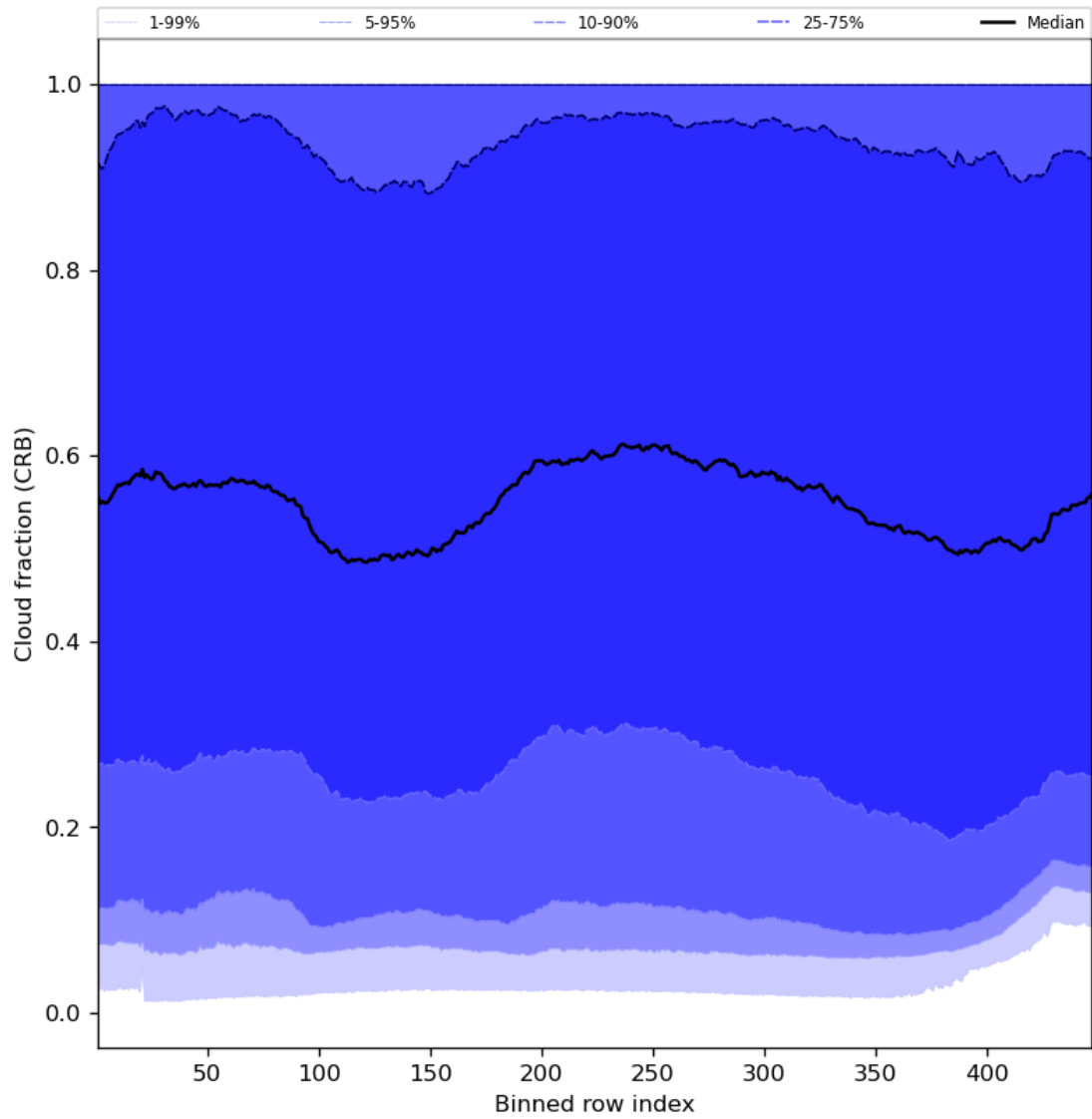
Figure 58: Along track statistics of “Cloud fraction (CRB)” for 2023-11-28 to 2023-11-30
