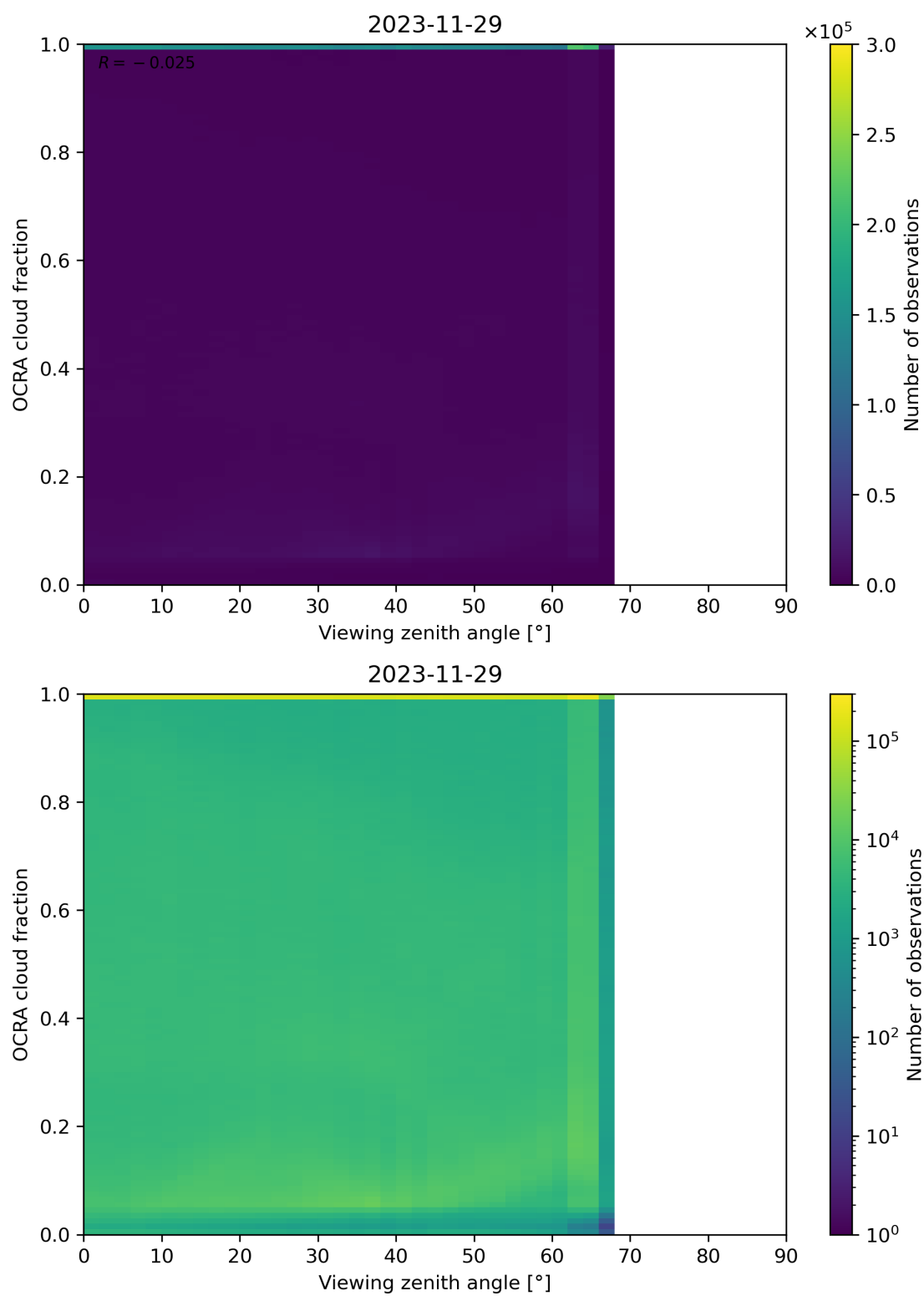
Figure 108: Scatter density plot of “Viewing zenith angle” against “OCRA cloud fraction” for 2023-11-28 to 2023-11-30.
