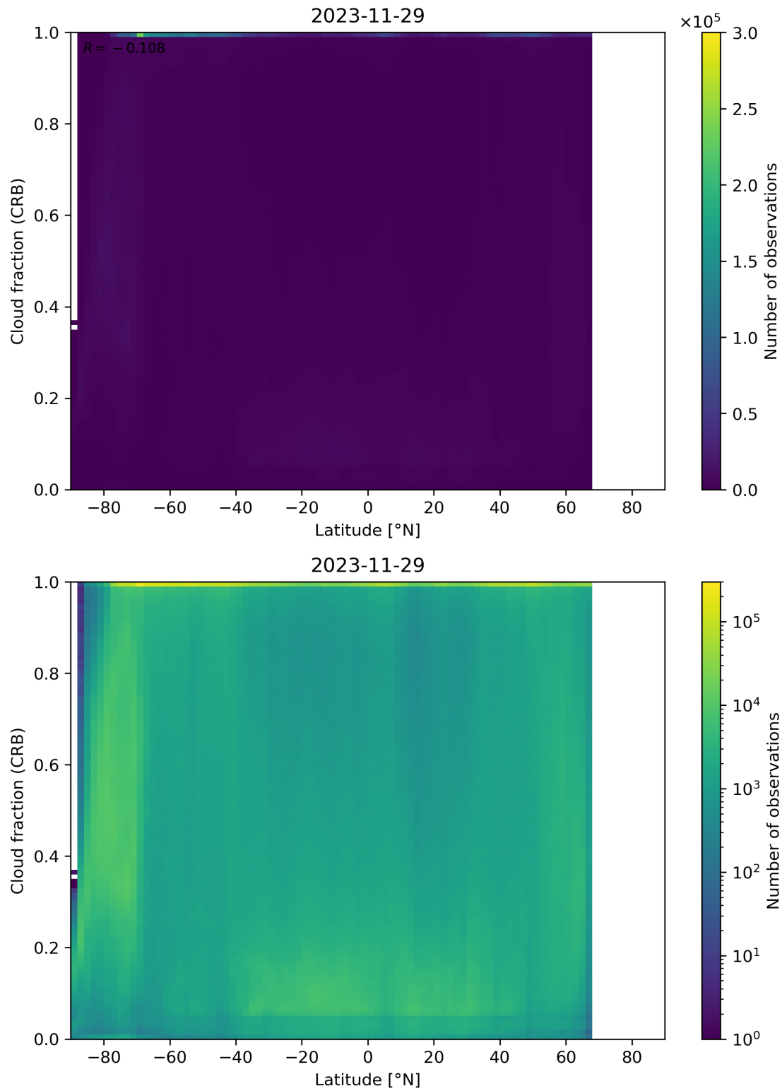
Figure 94: Scatter density plot of “Latitude” against “Cloud fraction (CRB)” for 2023-11-28 to 2023-11-30.
