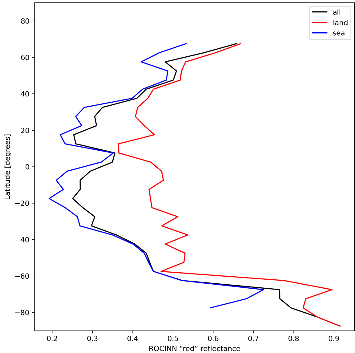
Figure 37: Zonal average of "ROCINN "red" reflectance" for 2023-11-28 to 2023-11-30.
