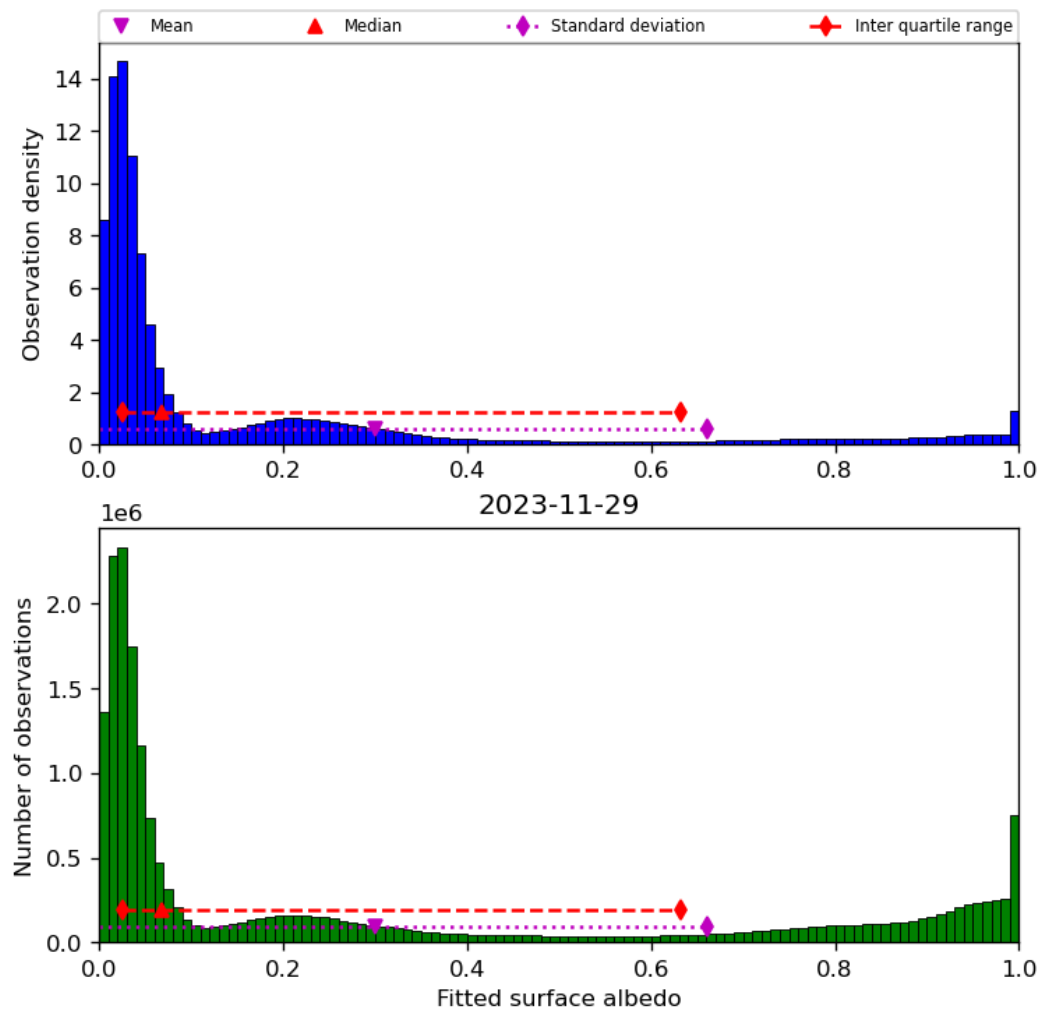
Figure 45: Histogram of “Fitted surface albedo” for 2023-11-28 to 2023-11-30
