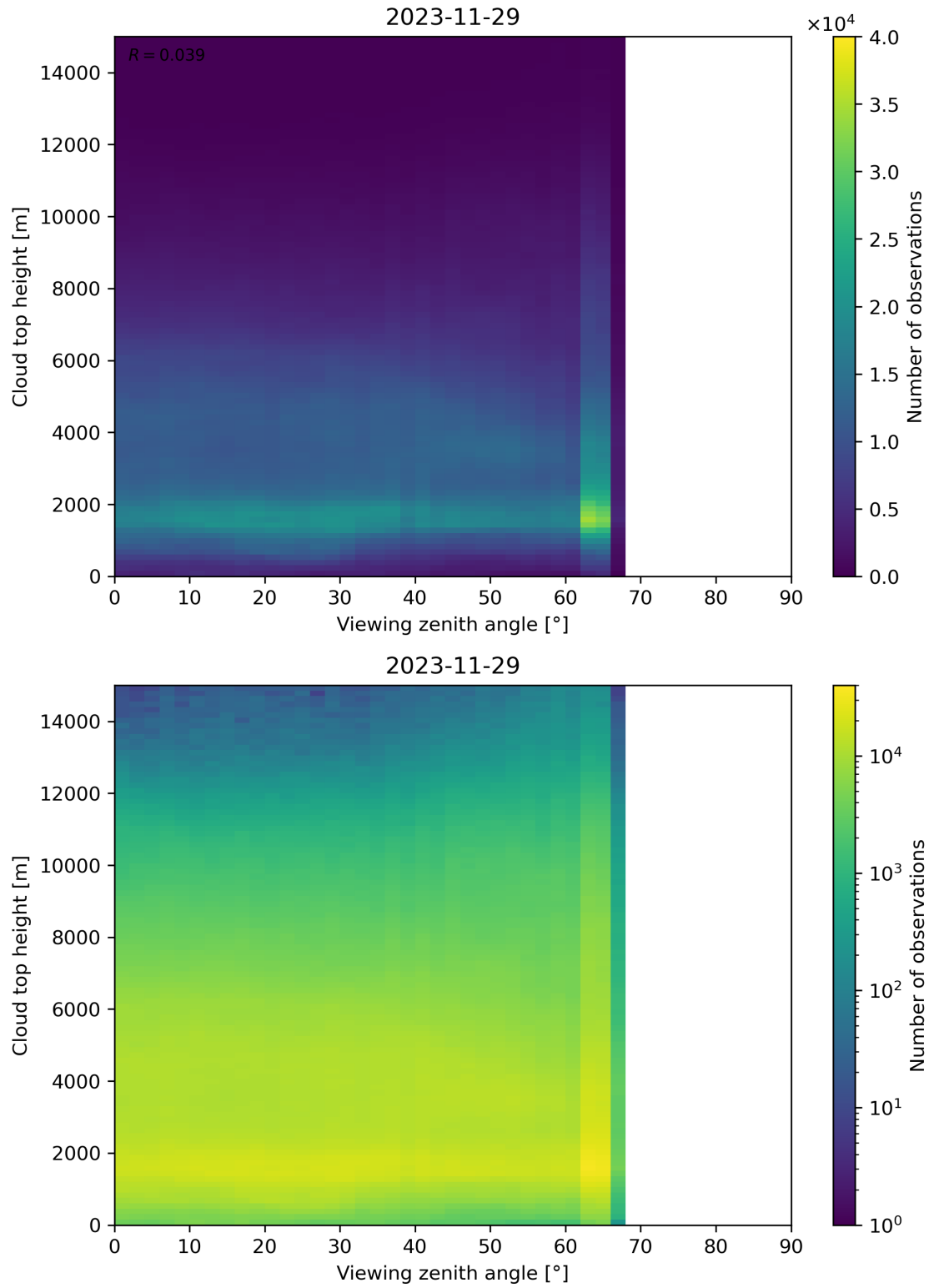
Figure 112: Scatter density plot of “Viewing zenith angle” against “Cloud top height” for 2023-11-28 to 2023-11-30.
