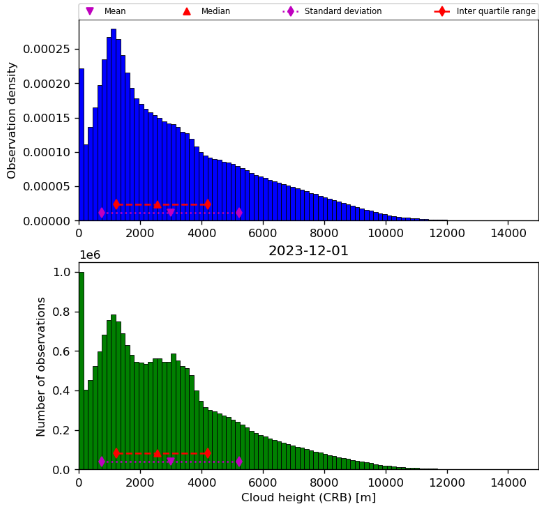
Figure 43: Histogram of “Cloud height (CRB)” for 2023-11-30 to 2023-12-02
