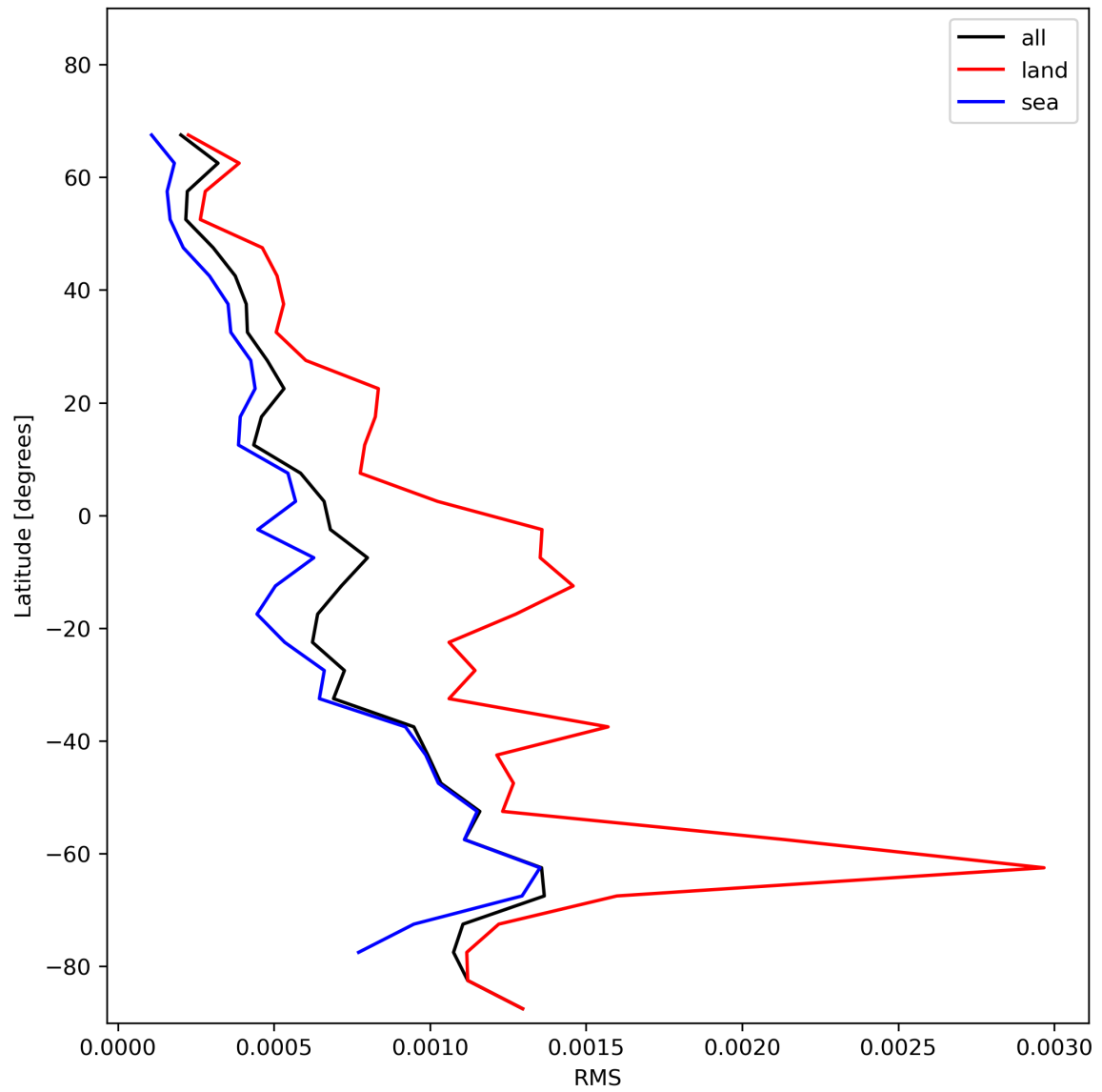
Figure 31: Zonal average of “RMS” for 2023-11-30 to 2023-12-02.
