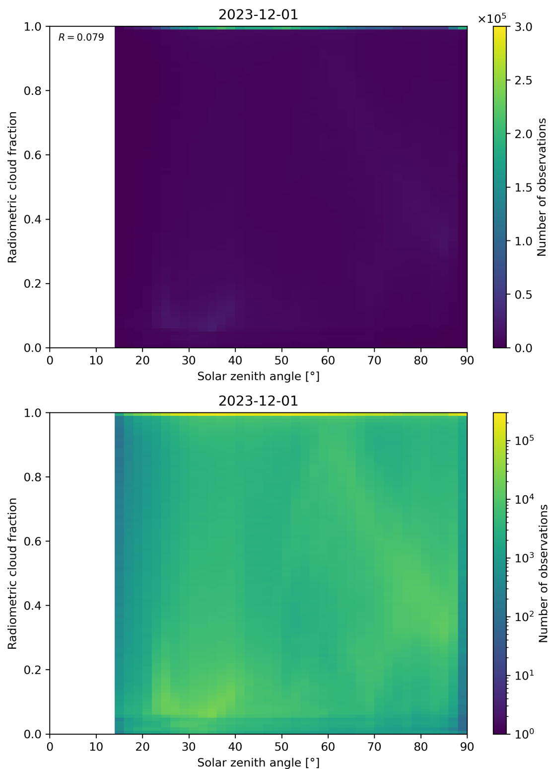
Figure 99: Scatter density plot of “Solar zenith angle” against “Radiometric cloud fraction” for 2023-11-30 to 2023-12-02.
