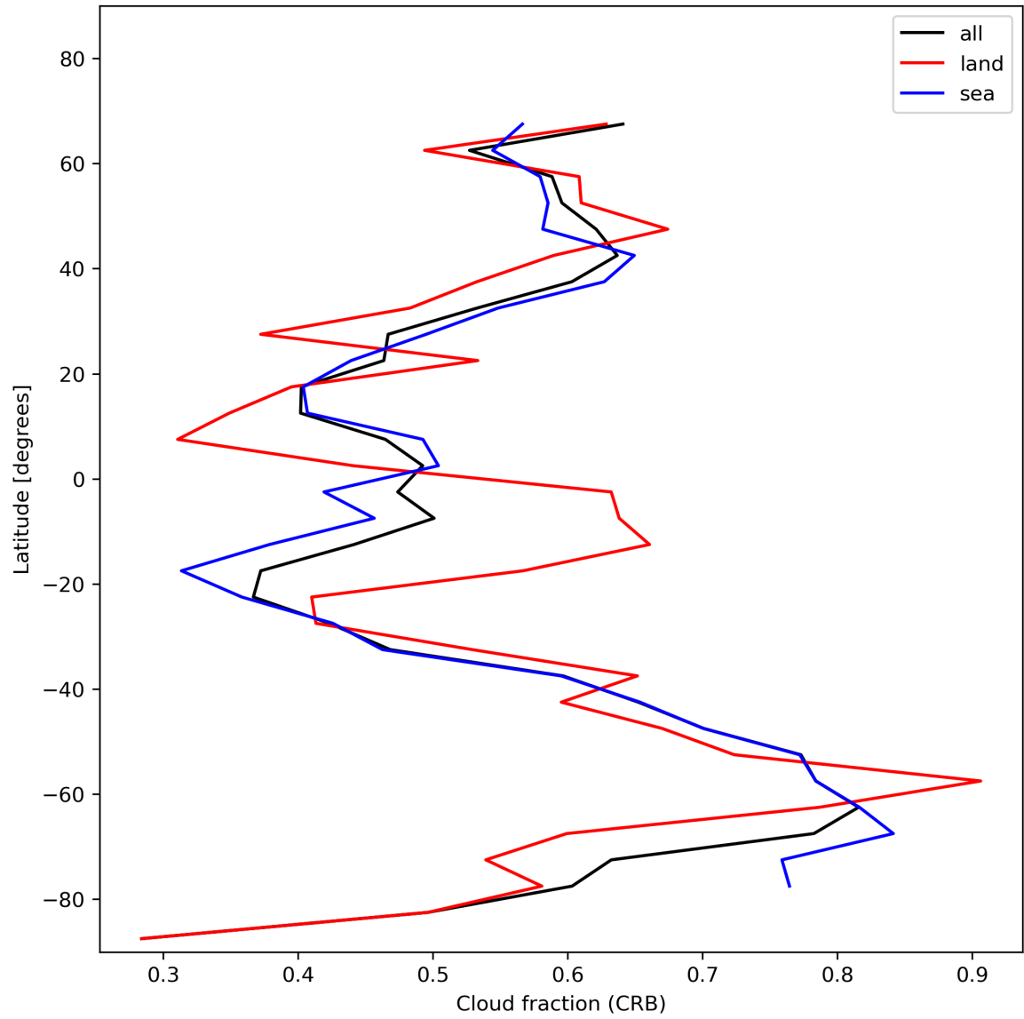
Figure 26: Zonal average of “Cloud fraction (CRB)” for 2023-11-30 to 2023-12-02.
