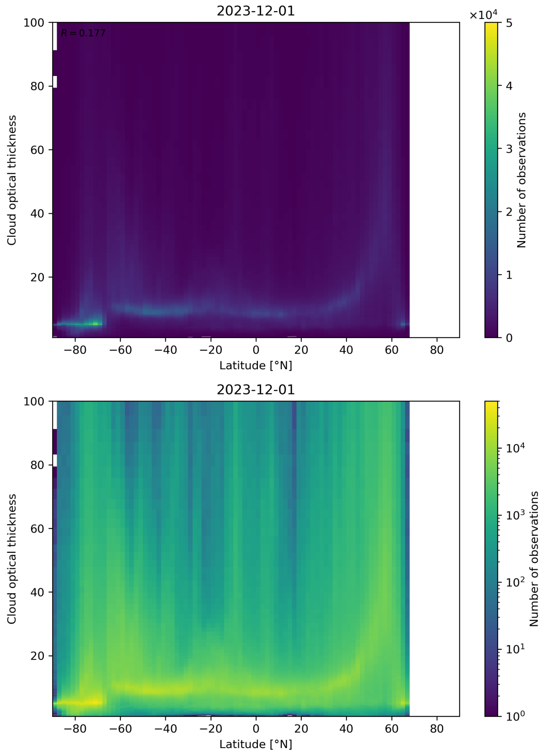
Figure 96: Scatter density plot of “Latitude” against “Cloud optical thickness” for 2023-11-30 to 2023-12-02.
