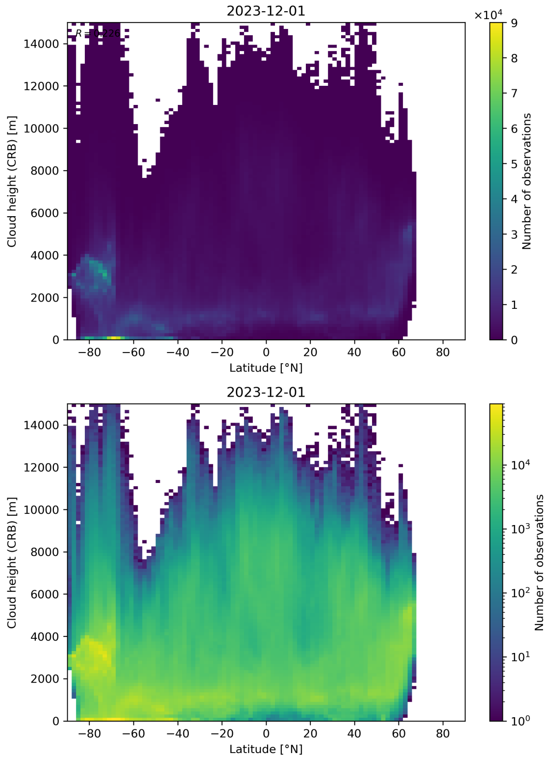
Figure 95: Scatter density plot of “Latitude” against “Cloud height (CRB)” for 2023-11-30 to 2023-12-02.
