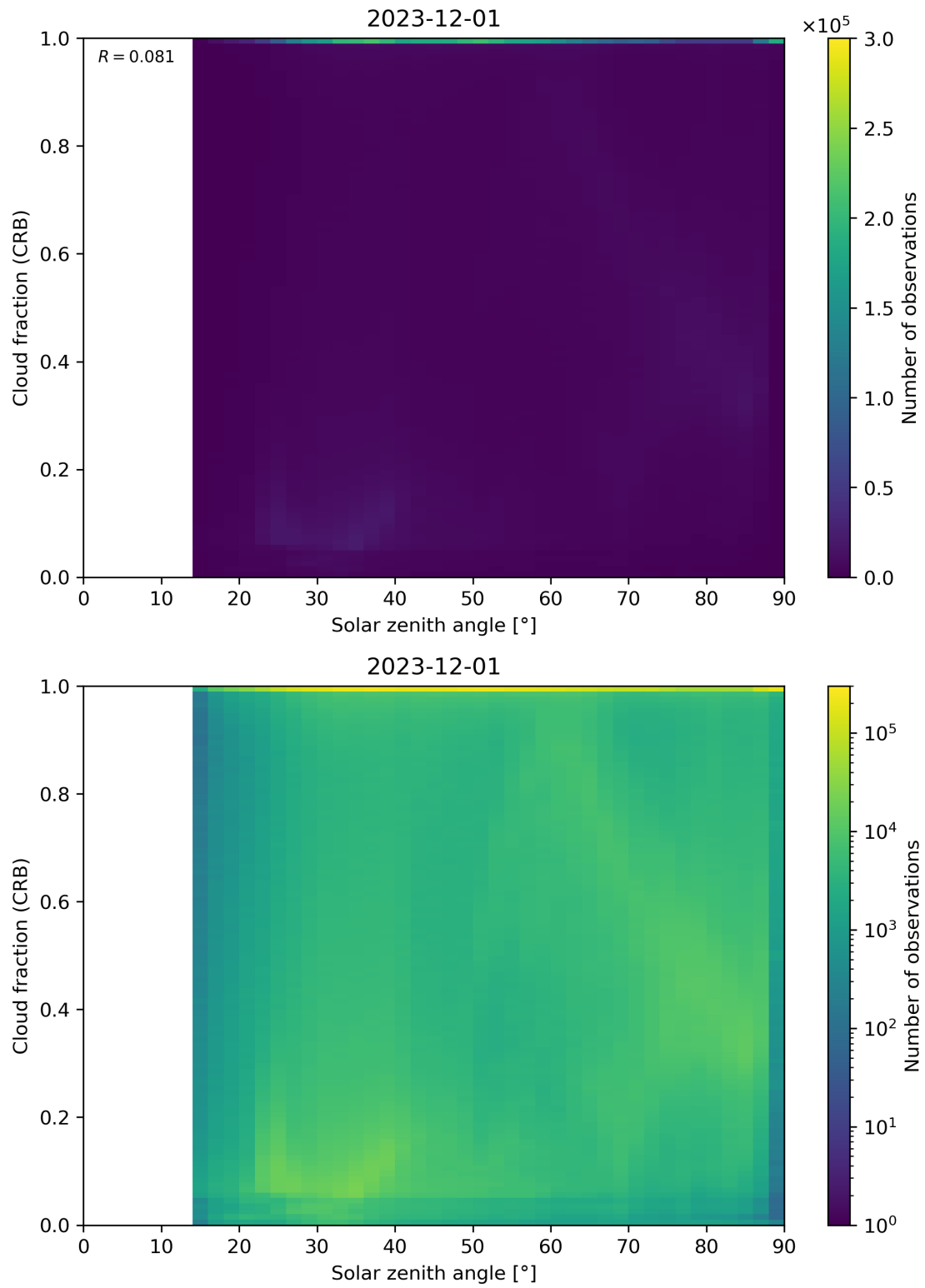
Figure 101: Scatter density plot of “Solar zenith angle” against “Cloud fraction (CRB)” for 2023-11-30 to 2023-12-02.
