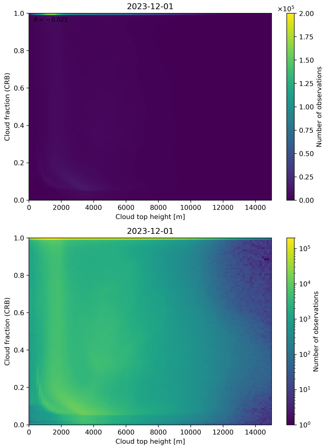
Figure 88: Scatter density plot of “Cloud top height” against “Cloud fraction (CRB)” for 2023-11-30 to 2023-12-02.
