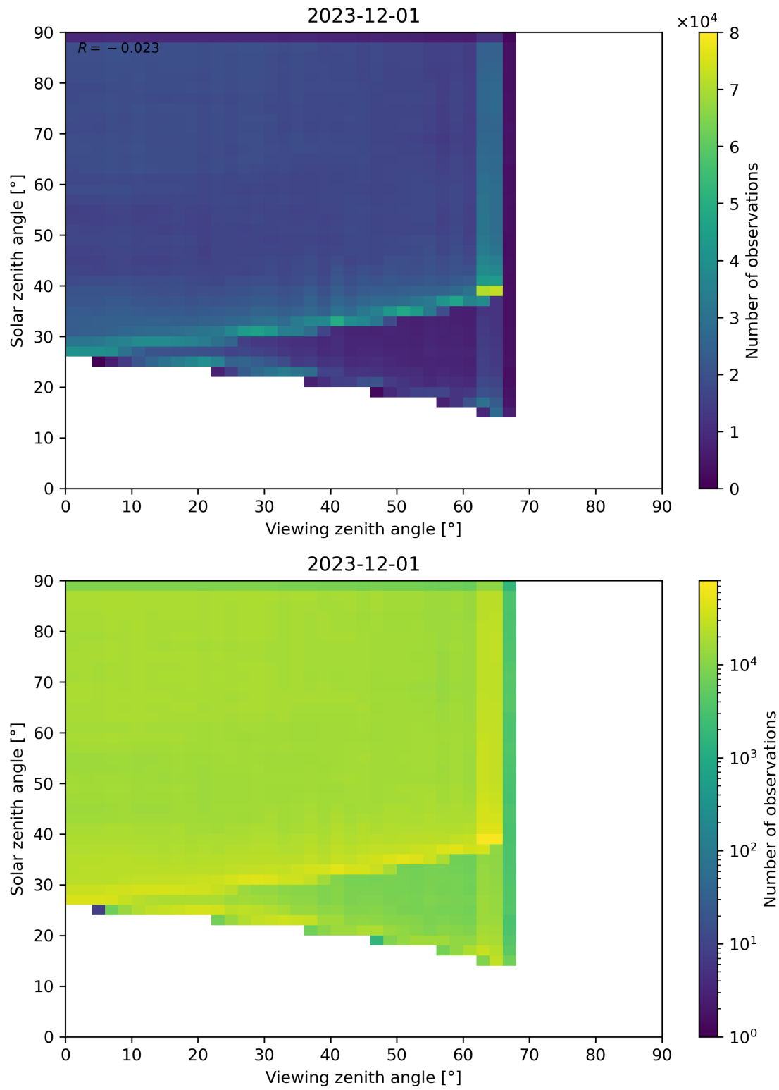
Figure 114: Scatter density plot of “Viewing zenith angle” against “Solar zenith angle” for 2023-11-30 to 2023-12-02.
