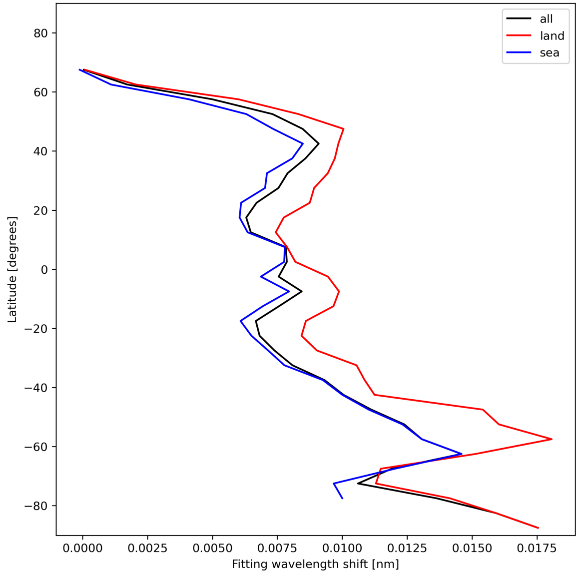
Figure 33: Zonal average of “Fitting wavelength shift” for 2023-11-30 to 2023-12-02.
