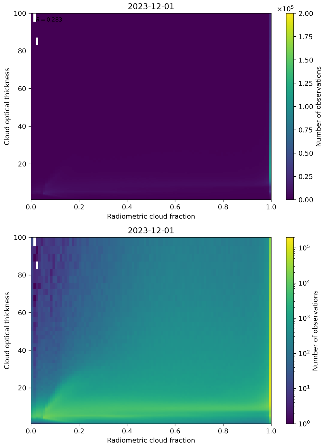
Figure 75: Scatter density plot of “Radiometric cloud fraction” against “Cloud optical thickness” for 2023-11-30 to 2023-12-02.
