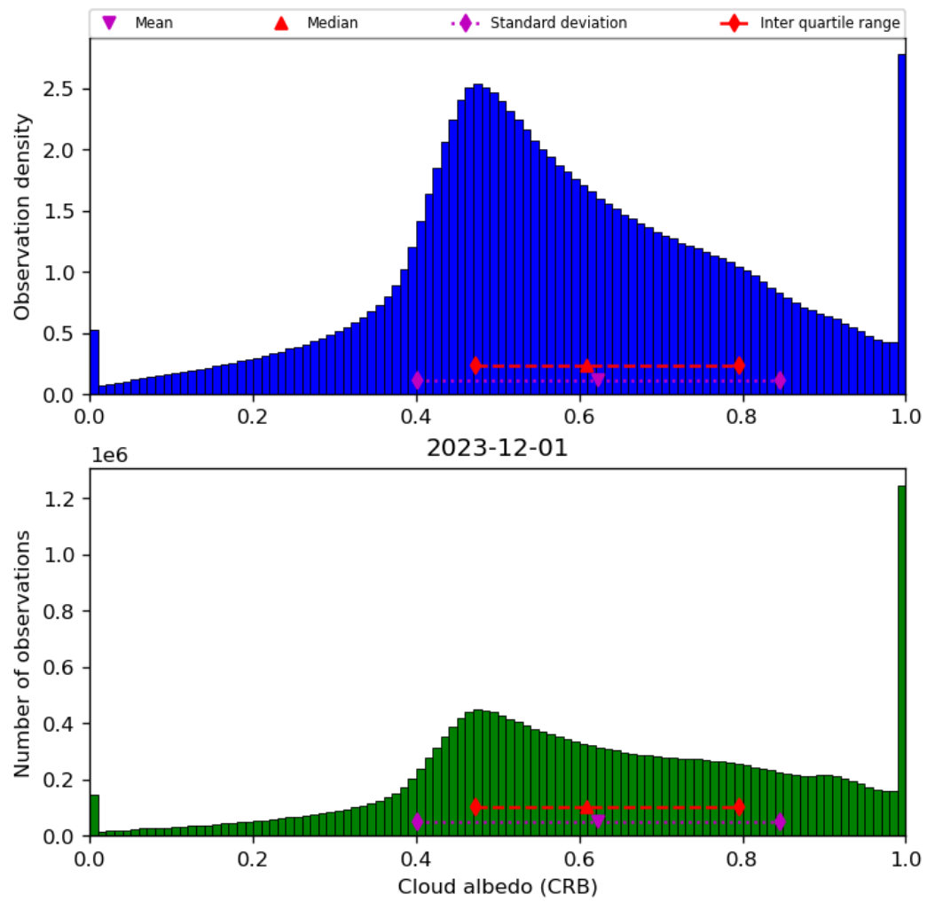
Figure 44: Histogram of “Cloud albedo (CRB)” for 2023-11-30 to 2023-12-02
