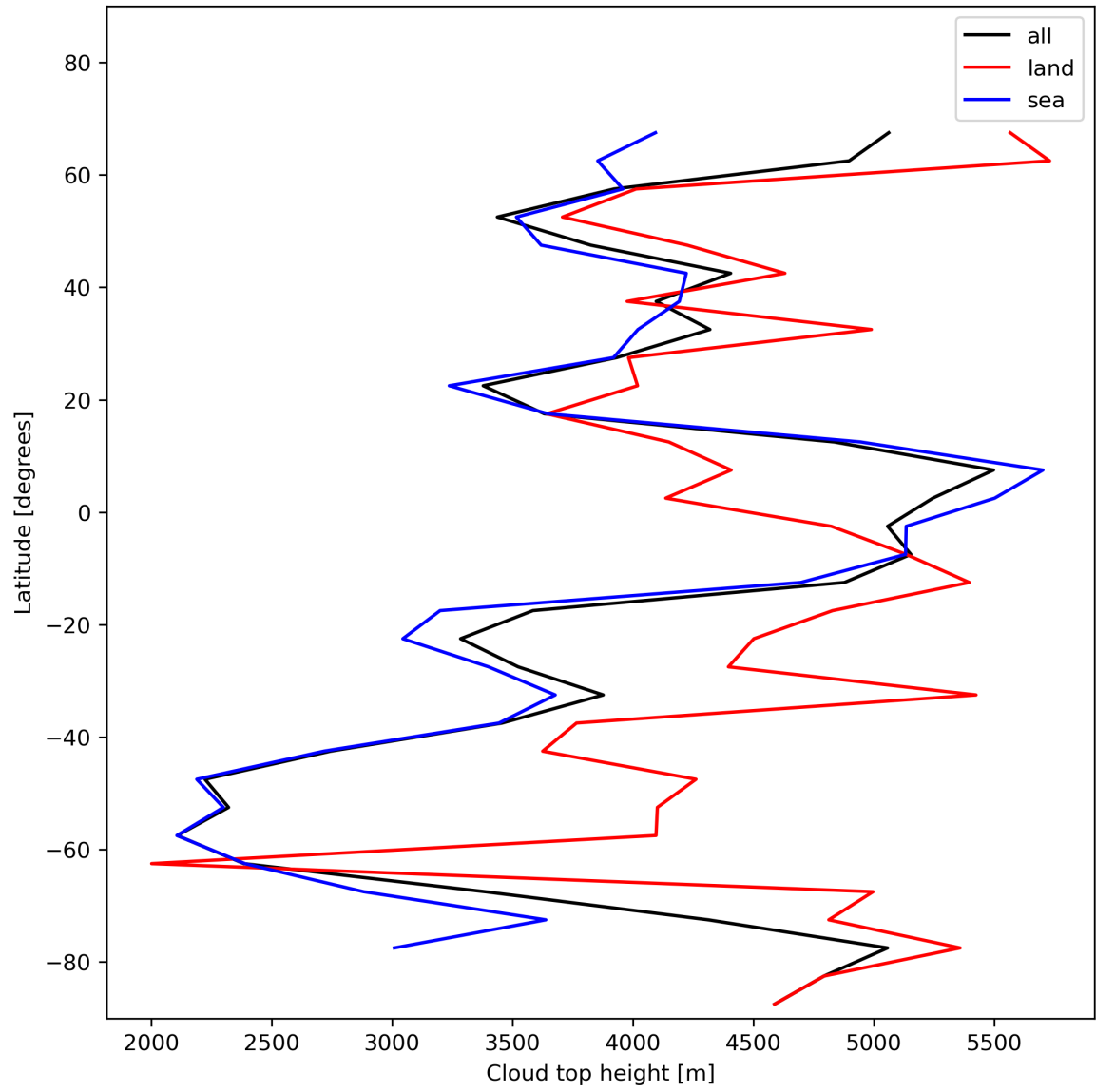
Figure 24: Zonal average of “Cloud top height” for 2023-11-30 to 2023-12-02.
