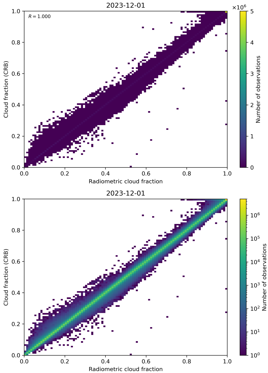
Figure 73: Scatter density plot of “Radiometric cloud fraction” against “Cloud fraction (CRB)” for 2023-11-30 to 2023-12-02.
