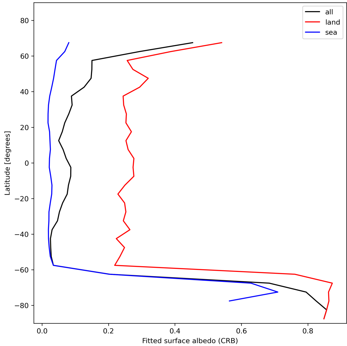
Figure 30: Zonal average of “Fitted surface albedo (CRB)” for 2023-11-30 to 2023-12-02.
