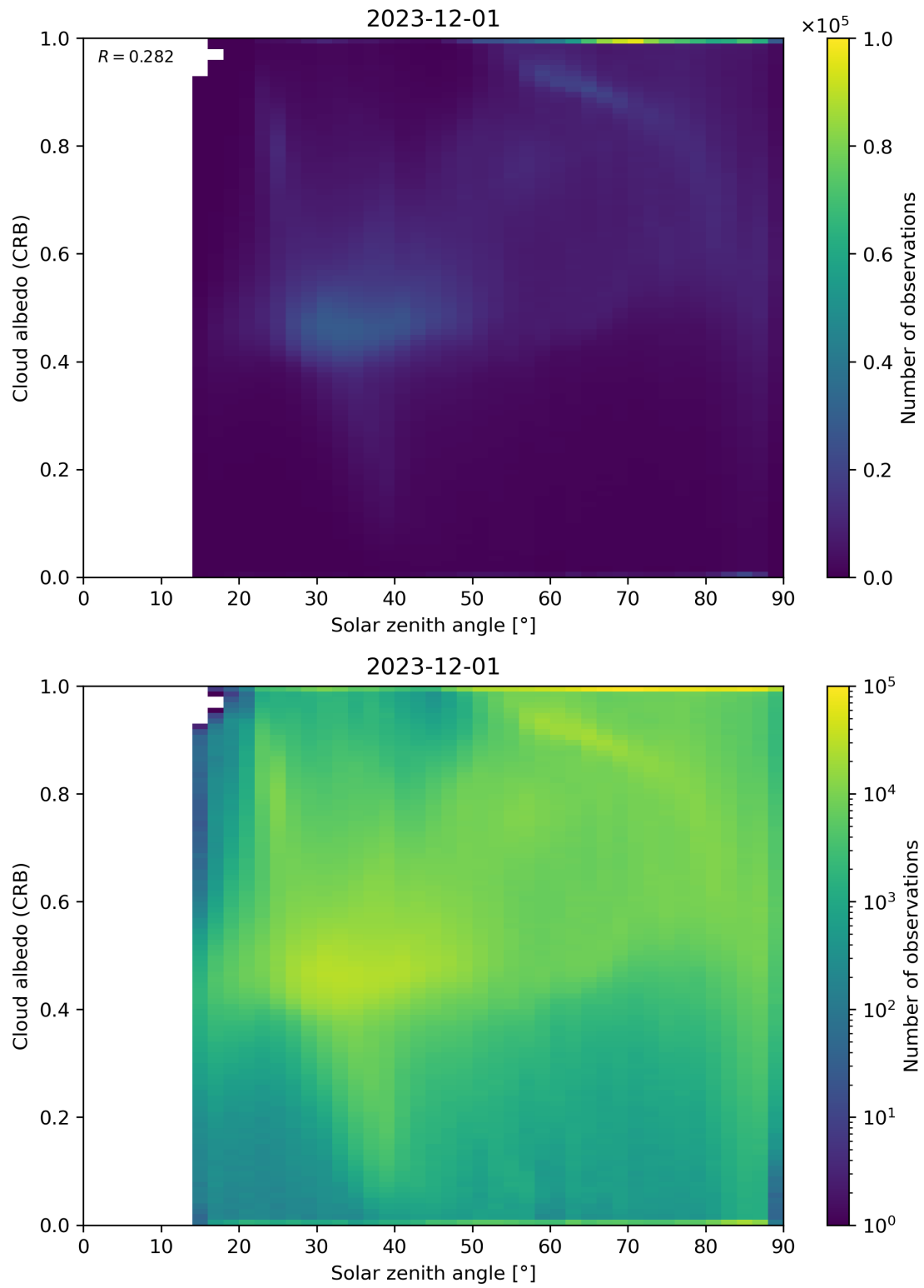
Figure 98: Scatter density plot of “Solar zenith angle” against “Cloud albedo (CRB)” for 2023-11-30 to 2023-12-02.
