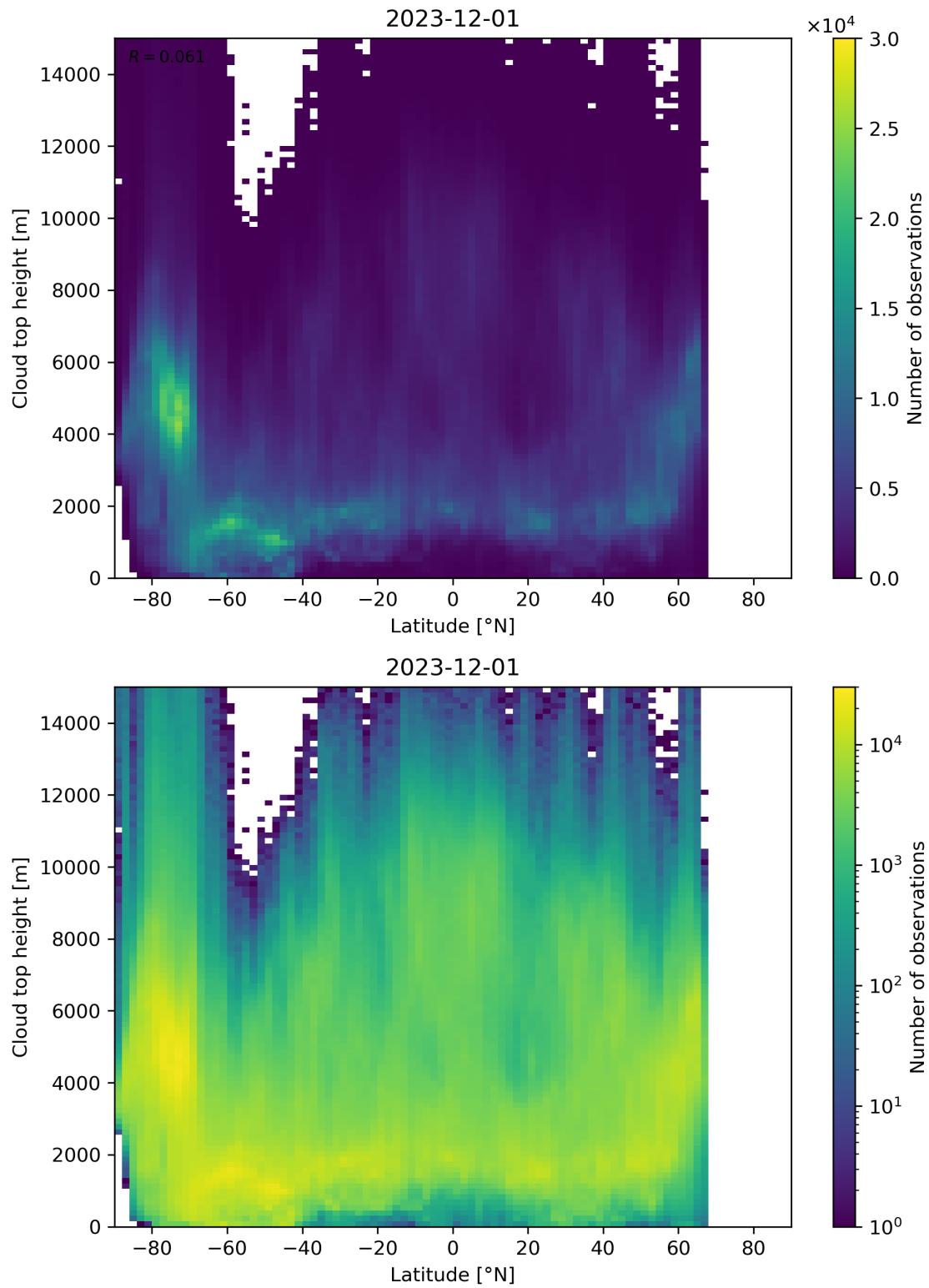
Figure 97: Scatter density plot of “Latitude” against “Cloud top height” for 2023-11-30 to 2023-12-02.
