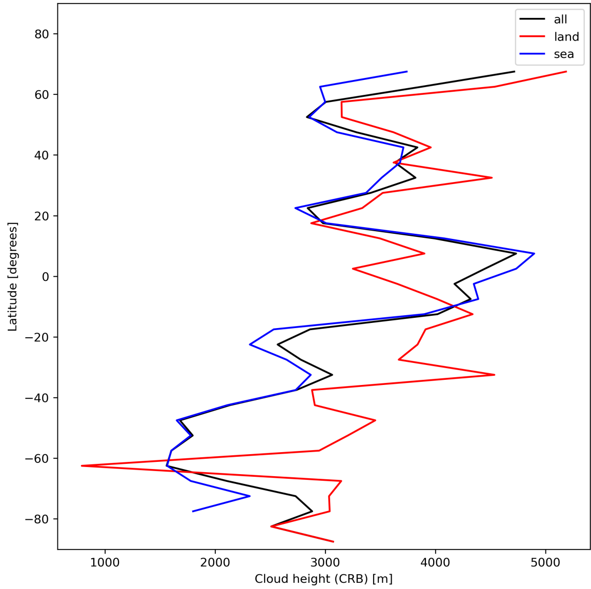
Figure 27: Zonal average of “Cloud height (CRB)” for 2023-11-30 to 2023-12-02.
