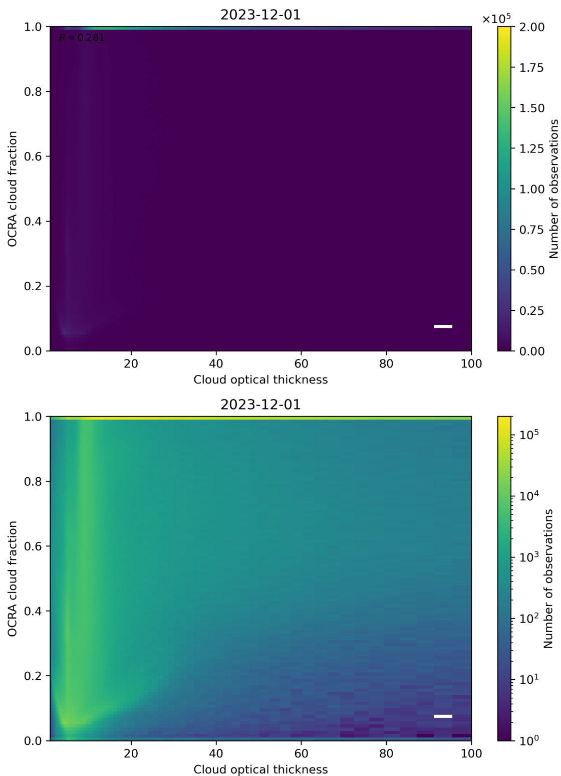
Figure 83: Scatter density plot of “Cloud optical thickness” against “OCRA cloud fraction” for 2023-11-30 to 2023-12-02.
