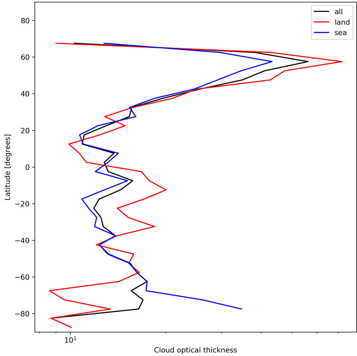
Figure 25: Zonal average of “Cloud optical thickness” for 2023-11-30 to 2023-12-02.
