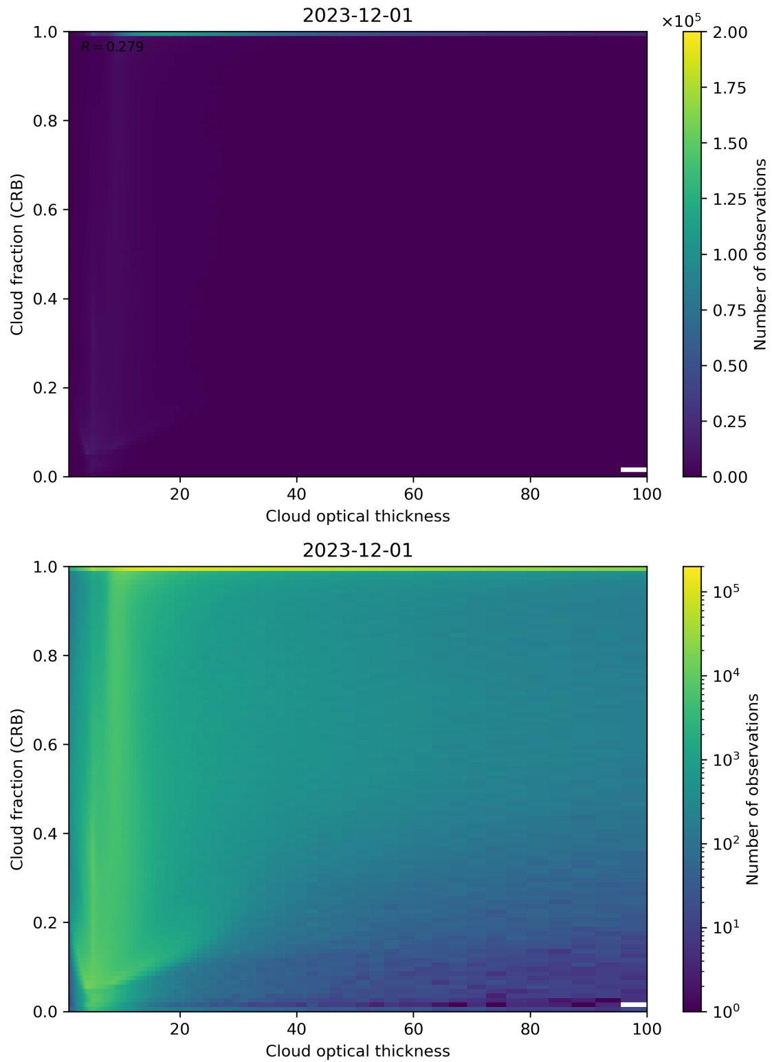
Figure 84: Scatter density plot of “Cloud optical thickness” against “Cloud fraction (CRB)” for 2023-11-30 to 2023-12-02.
