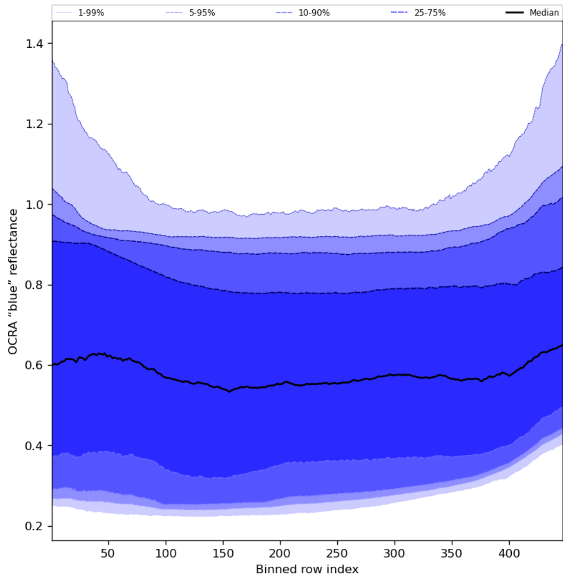
Figure 67: Along track statistics of "OCRA "blue" reflectance" for 2023-11-30 to 2023-12-02
