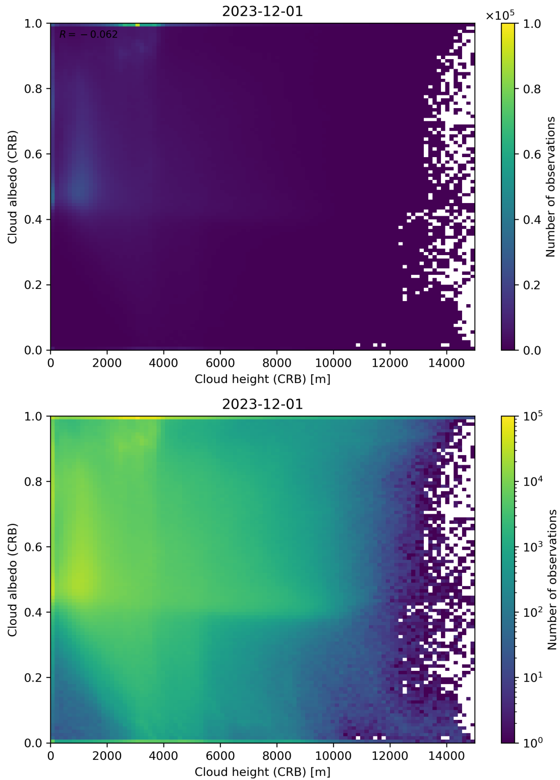
Figure 80: Scatter density plot of “Cloud height (CRB)” against “Cloud albedo (CRB)” for 2023-11-30 to 2023-12-02.
