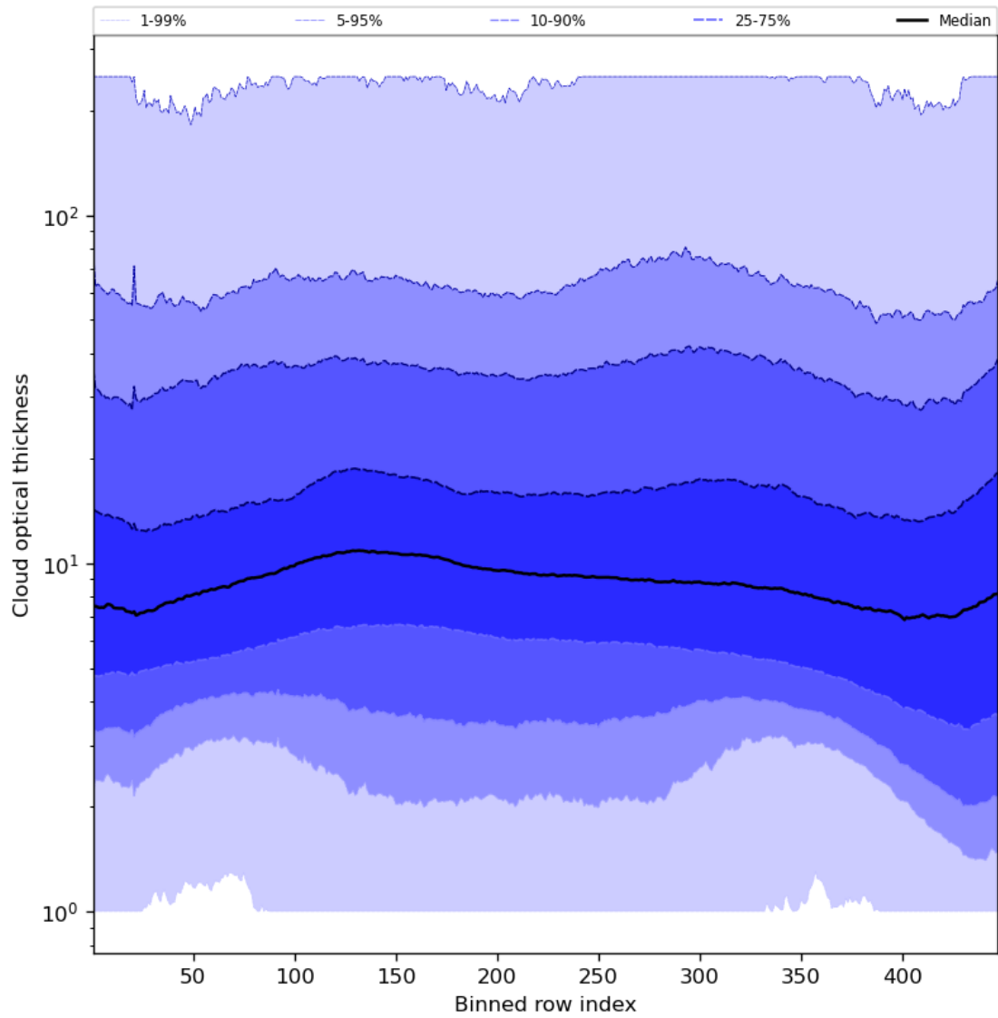
Figure 57: Along track statistics of “Cloud optical thickness” for 2023-11-30 to 2023-12-02
