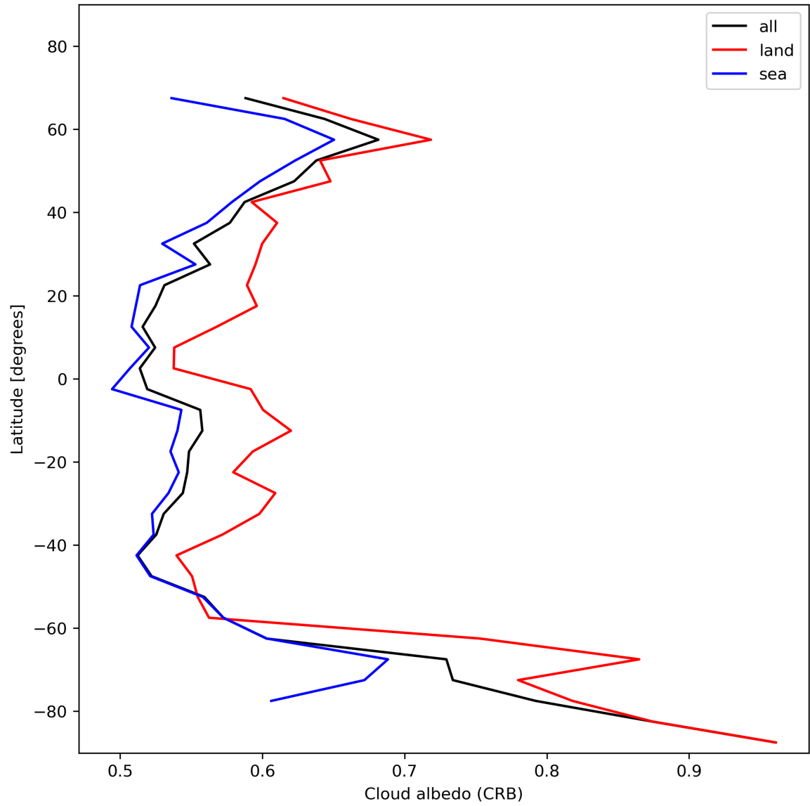
Figure 28: Zonal average of “Cloud albedo (CRB)” for 2023-11-30 to 2023-12-02.
