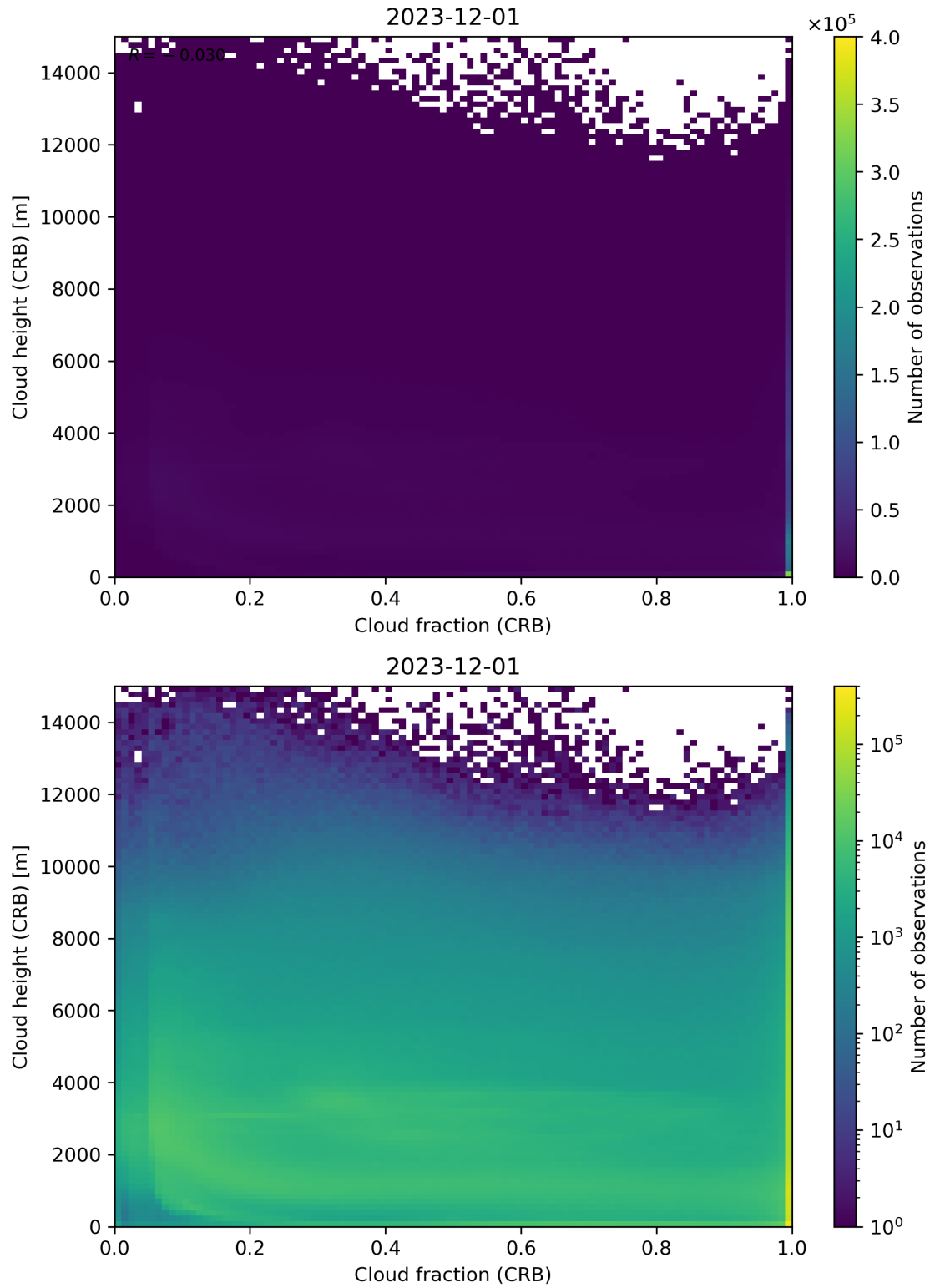
Figure 79: Scatter density plot of “Cloud fraction (CRB)” against “Cloud height (CRB)” for 2023-11-30 to 2023-12-02.
