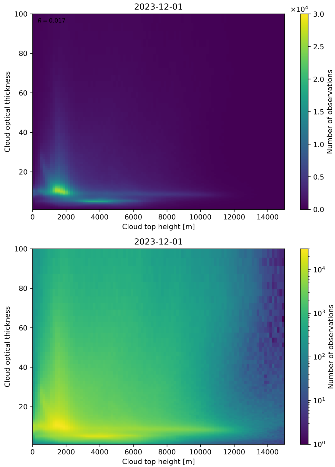
Figure 90: Scatter density plot of “Cloud top height” against “Cloud optical thickness” for 2023-11-30 to 2023-12-02.
