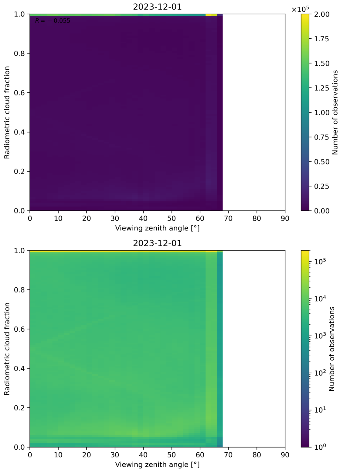
Figure 107: Scatter density plot of “Viewing zenith angle” against “Radiometric cloud fraction” for 2023-11-30 to 2023-12-02.
