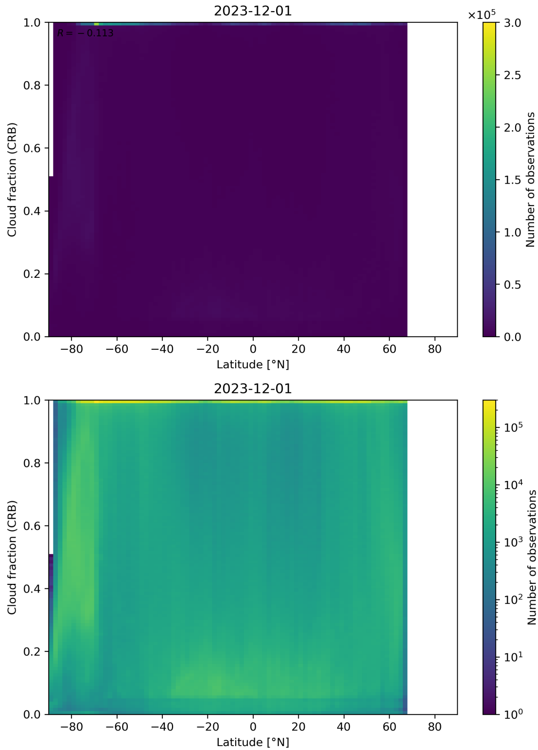
Figure 94: Scatter density plot of “Latitude” against “Cloud fraction (CRB)” for 2023-11-30 to 2023-12-02.
