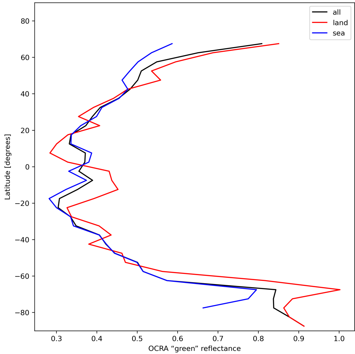
Figure 36: Zonal average of “OCRA “green” reflectance” for 2023-11-30 to 2023-12-02.
