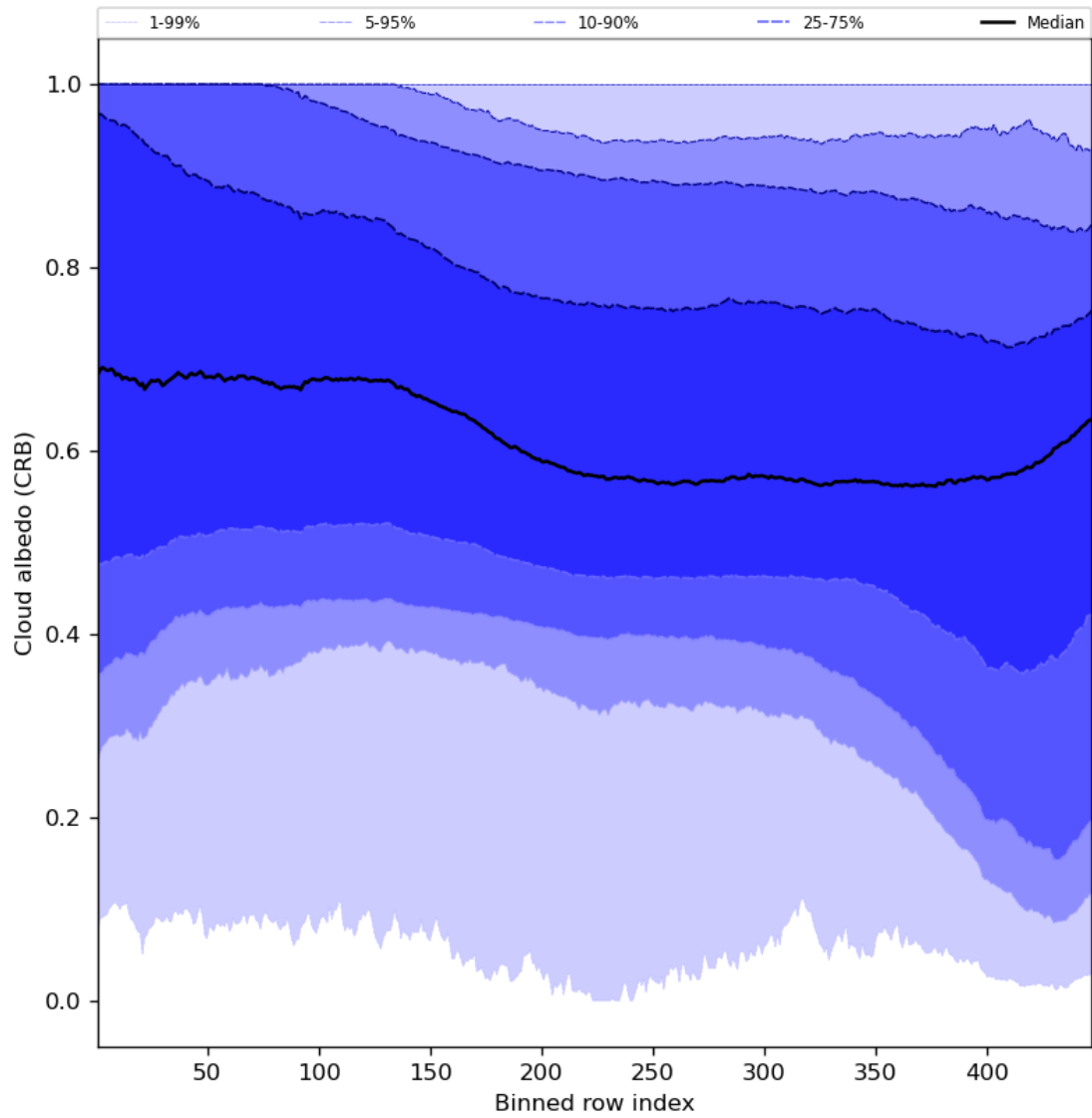
Figure 60: Along track statistics of “Cloud albedo (CRB)” for 2023-11-30 to 2023-12-02
