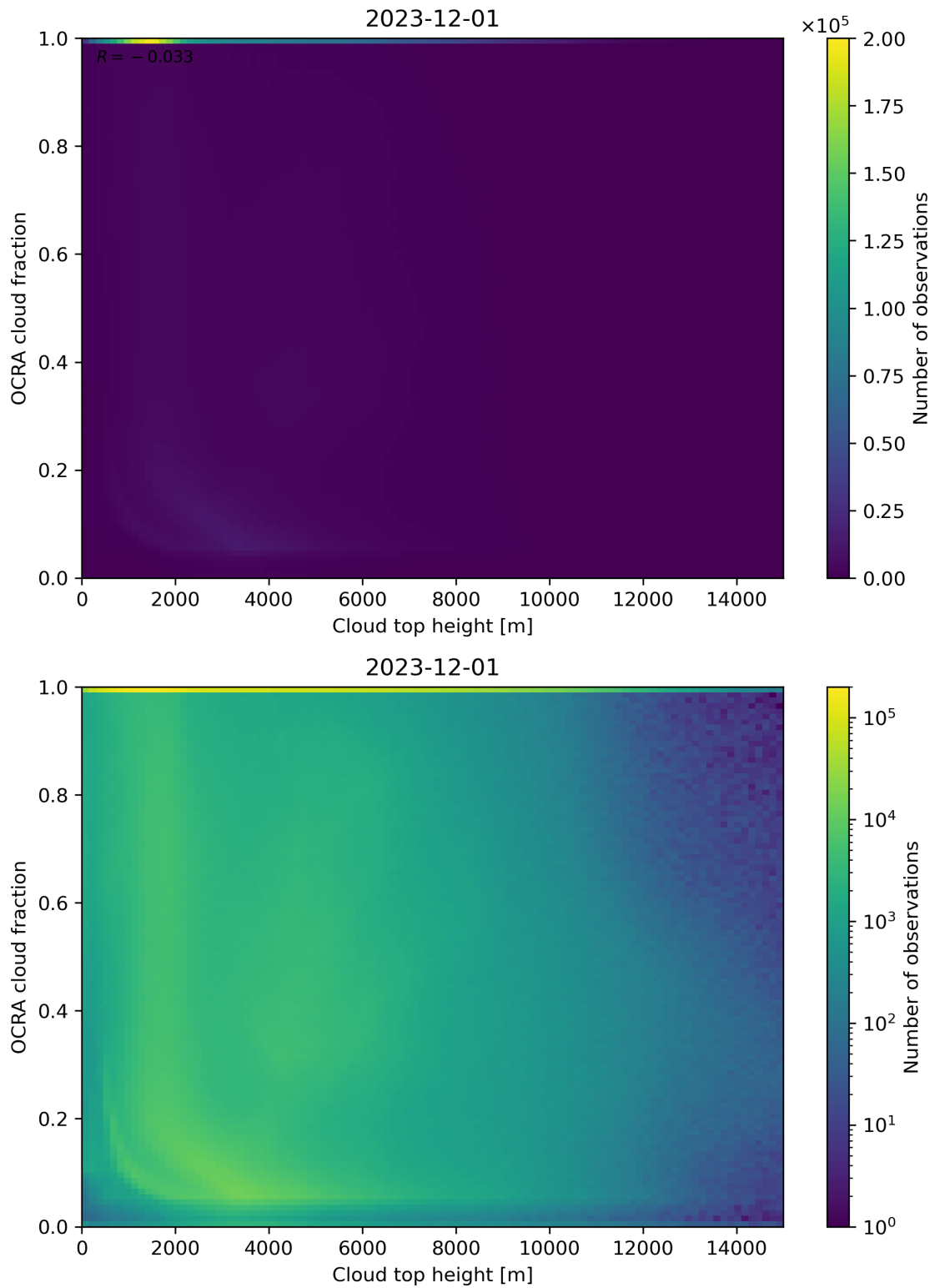
Figure 87: Scatter density plot of “Cloud top height” against “OCRA cloud fraction” for 2023-11-30 to 2023-12-02.
