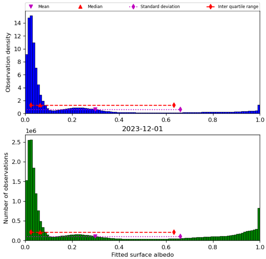
Figure 45: Histogram of “Fitted surface albedo” for 2023-11-30 to 2023-12-02
