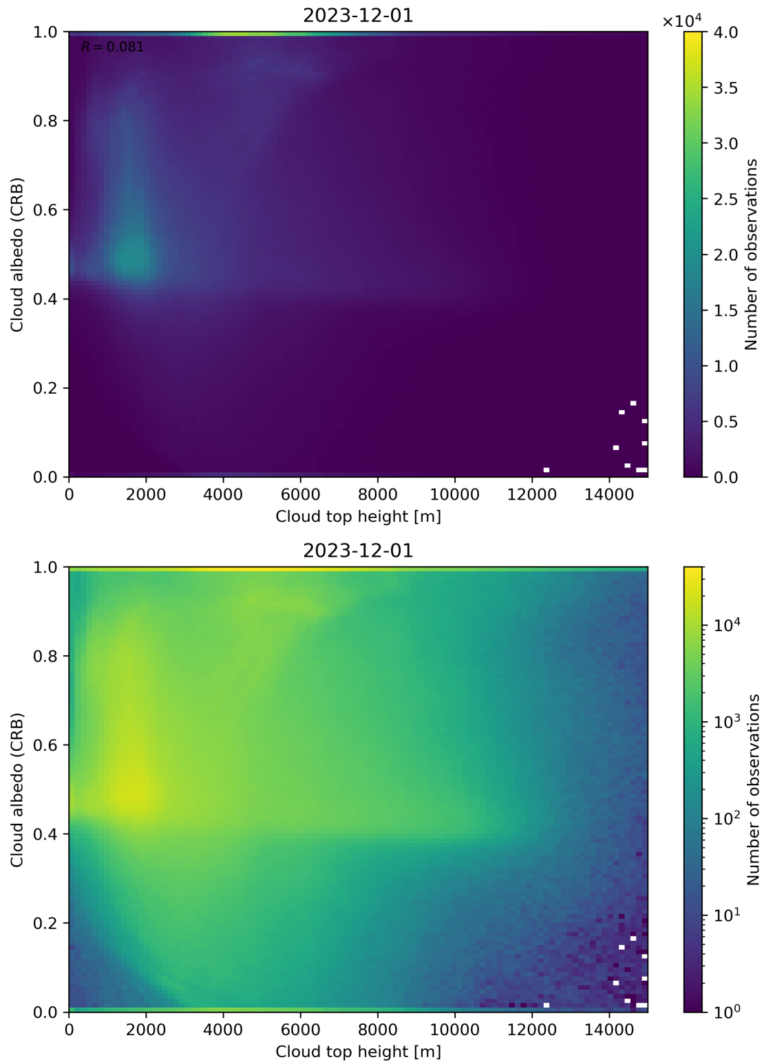
Figure 86: Scatter density plot of “Cloud top height” against “Cloud albedo (CRB)” for 2023-11-30 to 2023-12-02.
