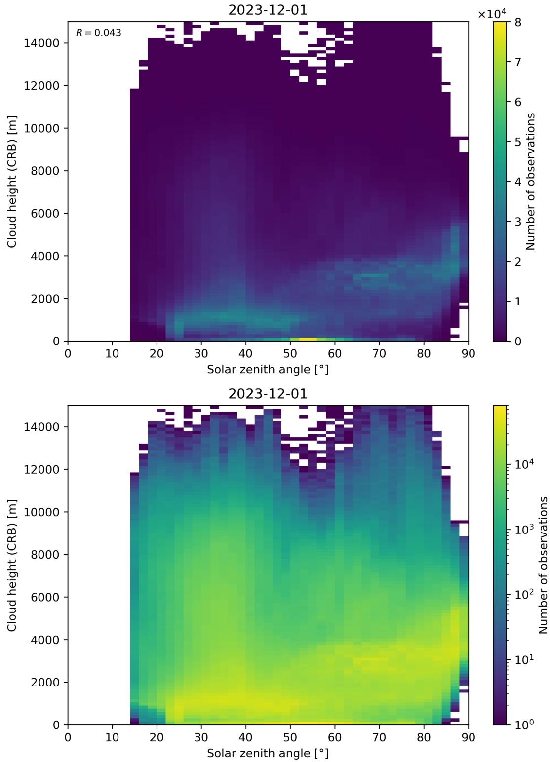
Figure 102: Scatter density plot of “Solar zenith angle” against “Cloud height (CRB)” for 2023-11-30 to 2023-12-02.
