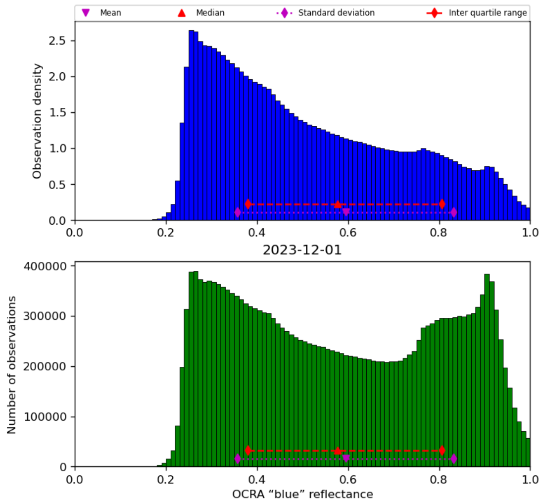
Figure 51: Histogram of “OCRA “blue” reflectance” for 2023-11-30 to 2023-12-02
