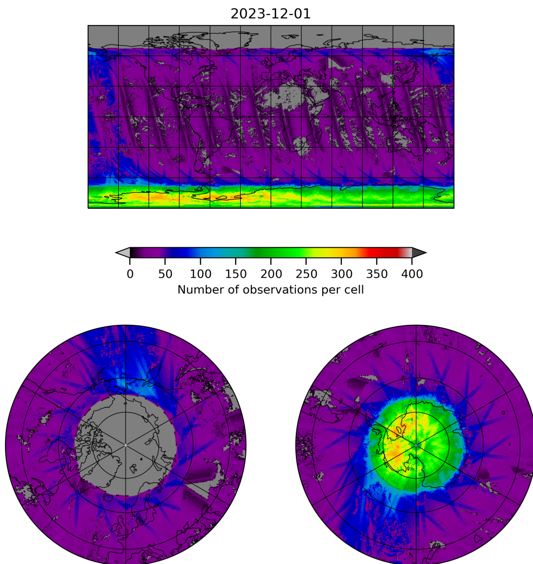
Figure 21: Map of the number of observations for 2023-11-30 to 2023-12-02
