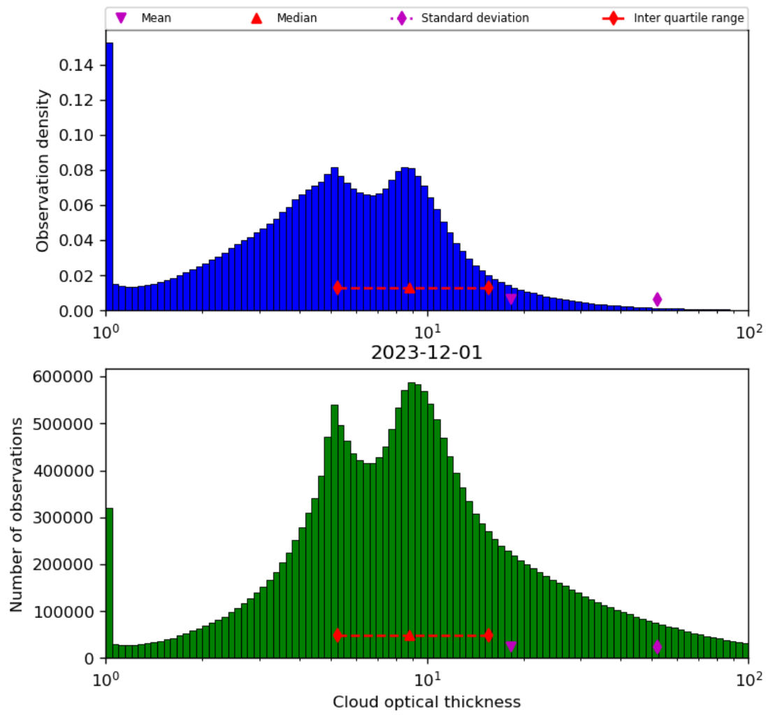
Figure 41: Histogram of “Cloud optical thickness” for 2023-11-30 to 2023-12-02
