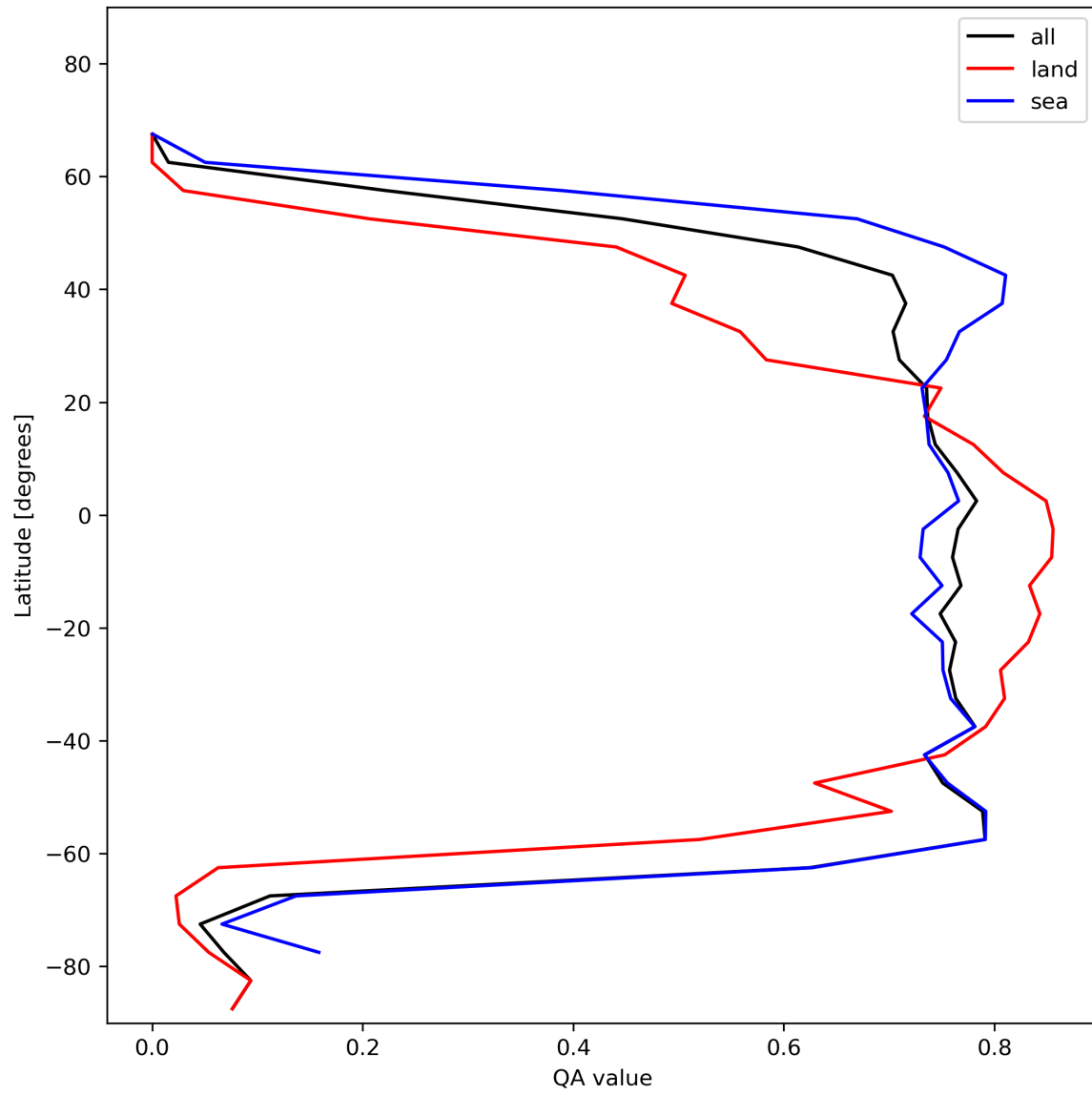
Figure 22: Zonal average of “QA value” for 2023-11-30 to 2023-12-02.
