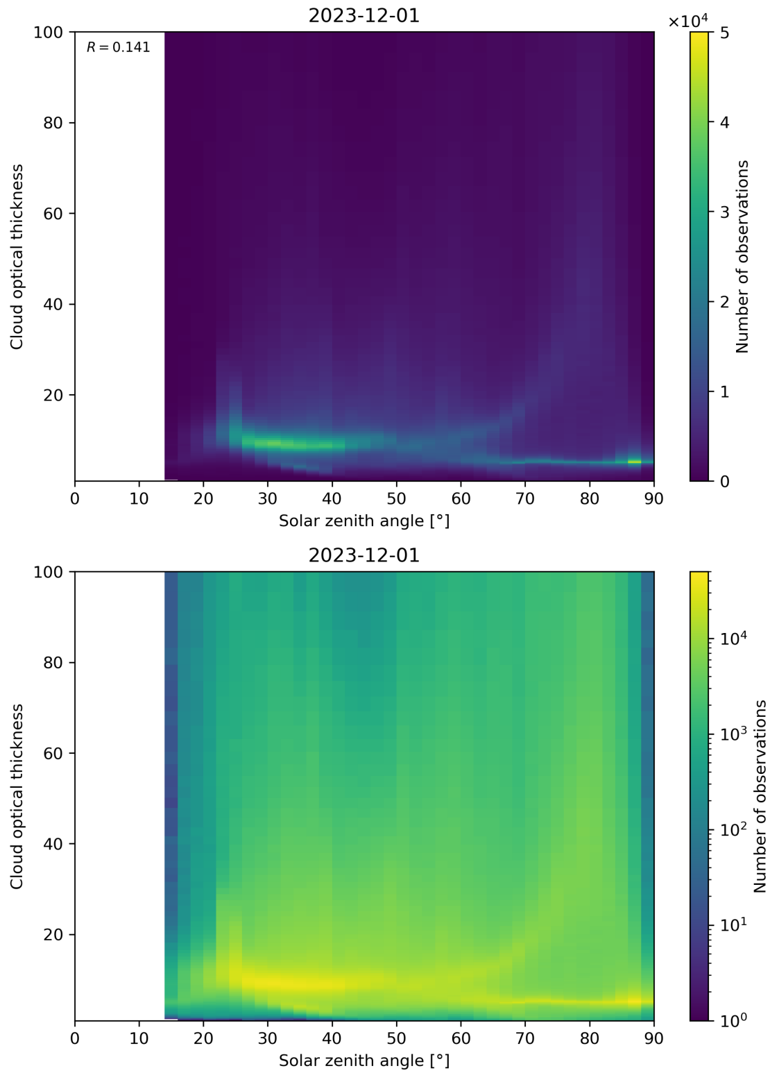
Figure 103: Scatter density plot of “Solar zenith angle” against “Cloud optical thickness” for 2023-11-30 to 2023-12-02.
