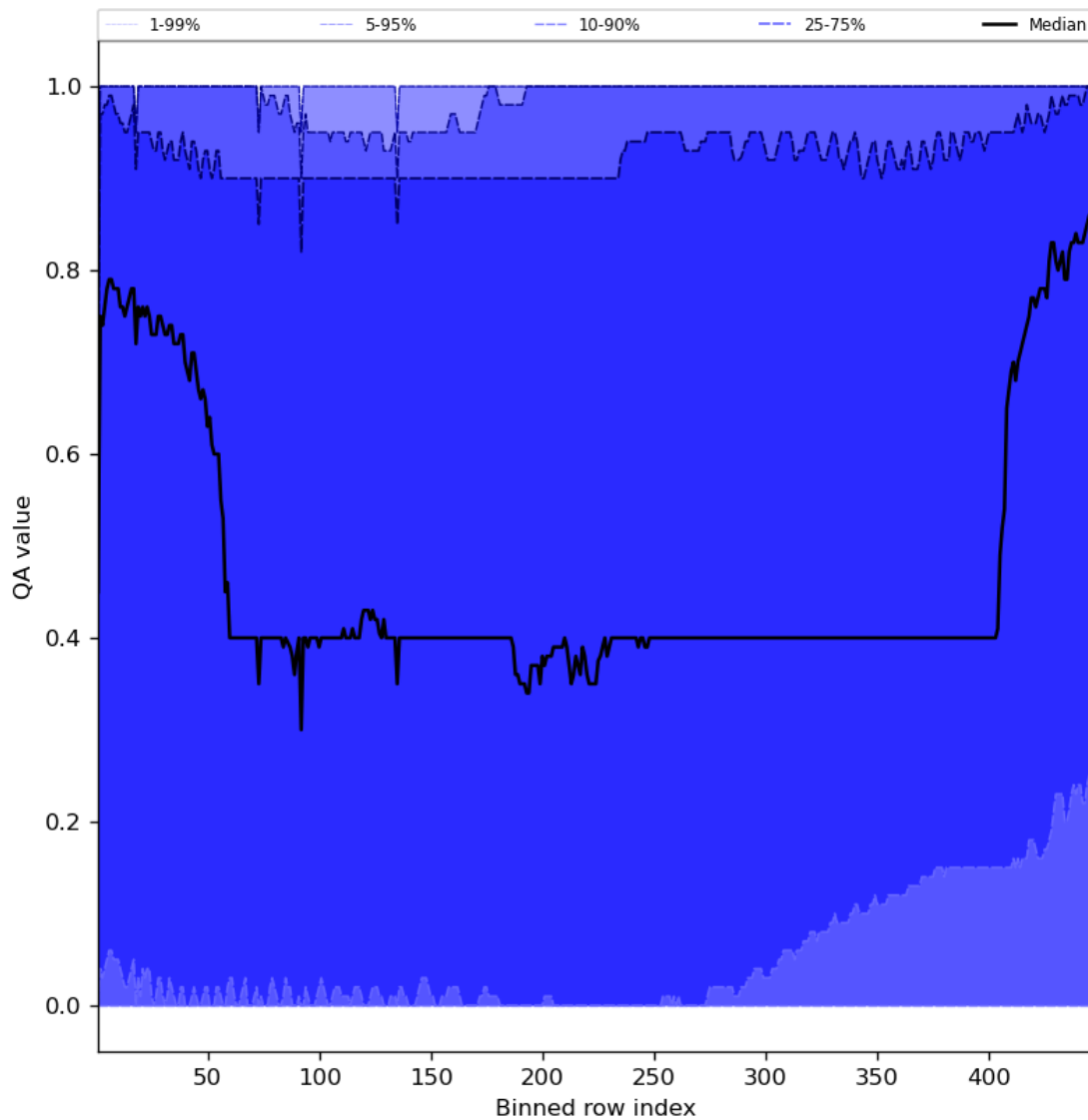
Figure 54: Along track statistics of “QA value” for 2023-11-30 to 2023-12-02
