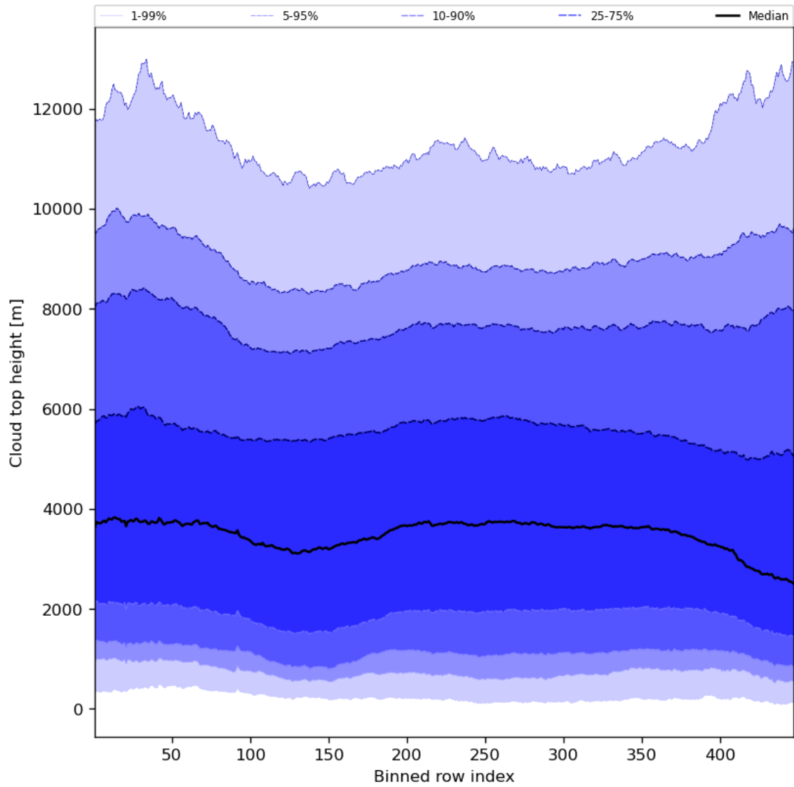
Figure 56: Along track statistics of “Cloud top height” for 2023-11-30 to 2023-12-02
