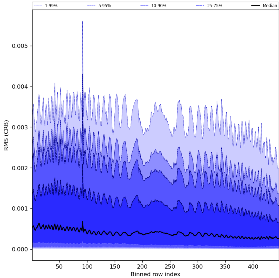
Figure 64: Along track statistics of “RMS (CRB)” for 2023-11-30 to 2023-12-02
