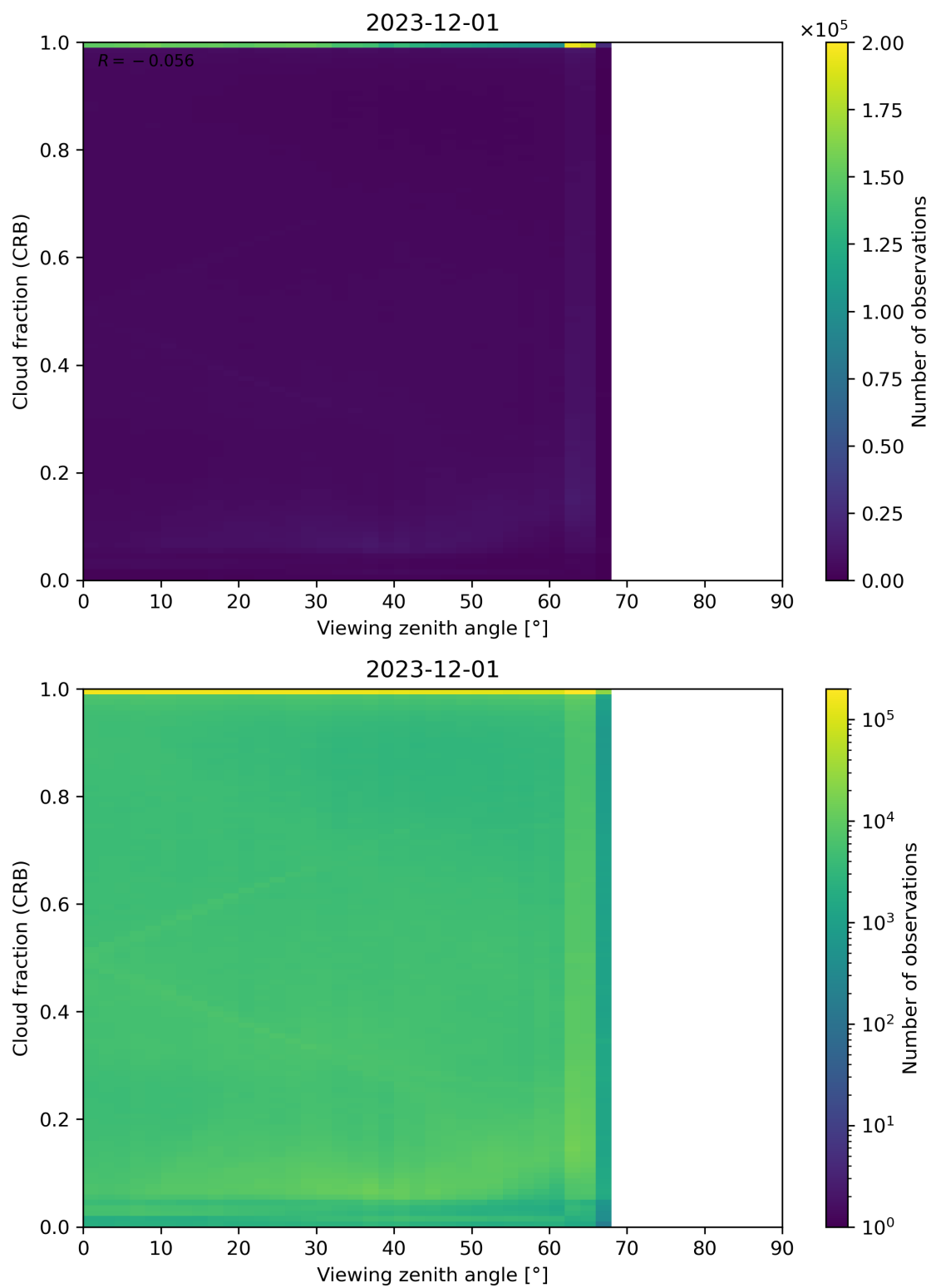
Figure 109: Scatter density plot of “Viewing zenith angle” against “Cloud fraction (CRB)” for 2023-11-30 to 2023-12-02.
