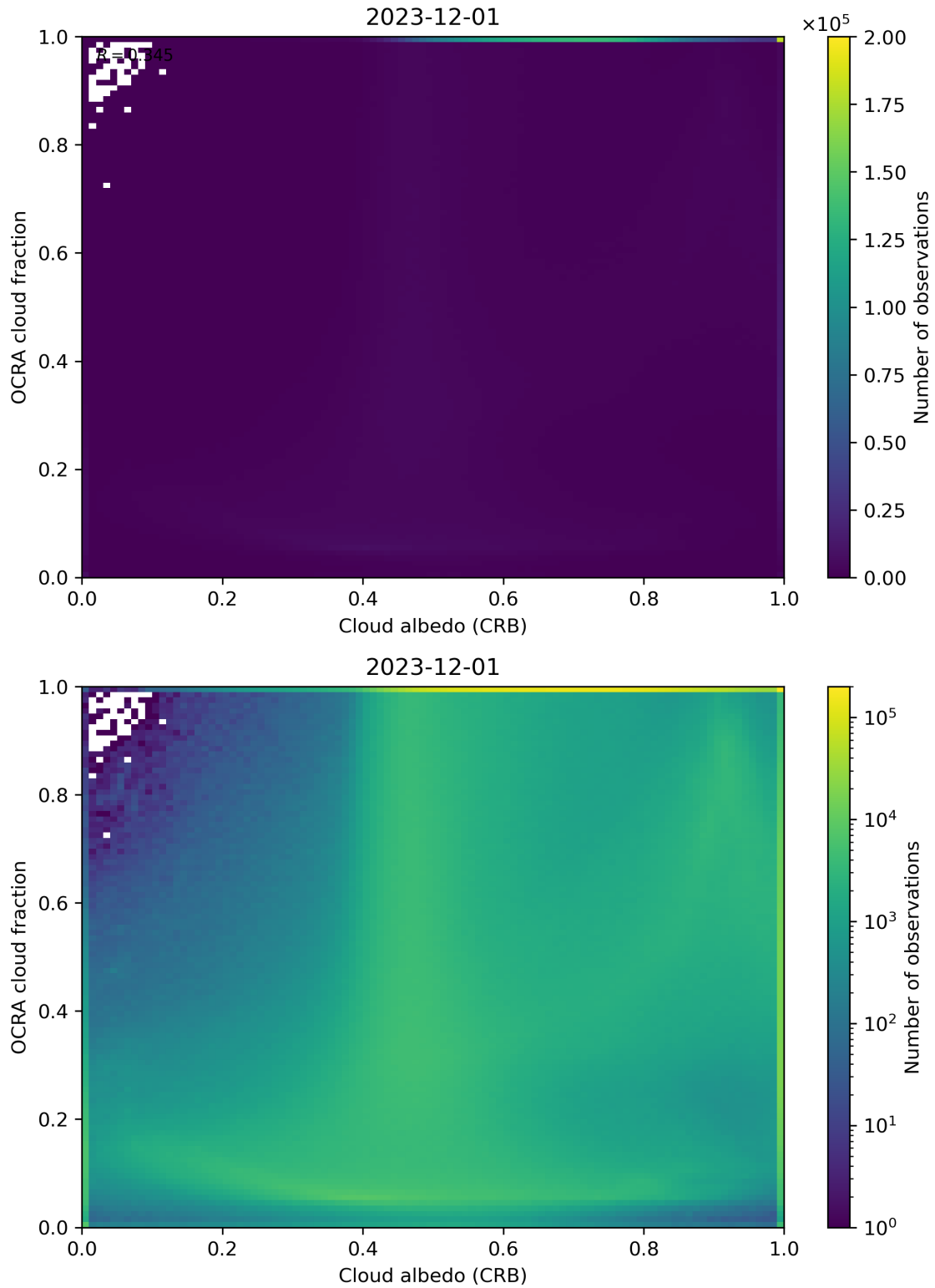
Figure 70: Scatter density plot of “Cloud albedo (CRB)” against “OCRA cloud fraction” for 2023-11-30 to 2023-12-02.
