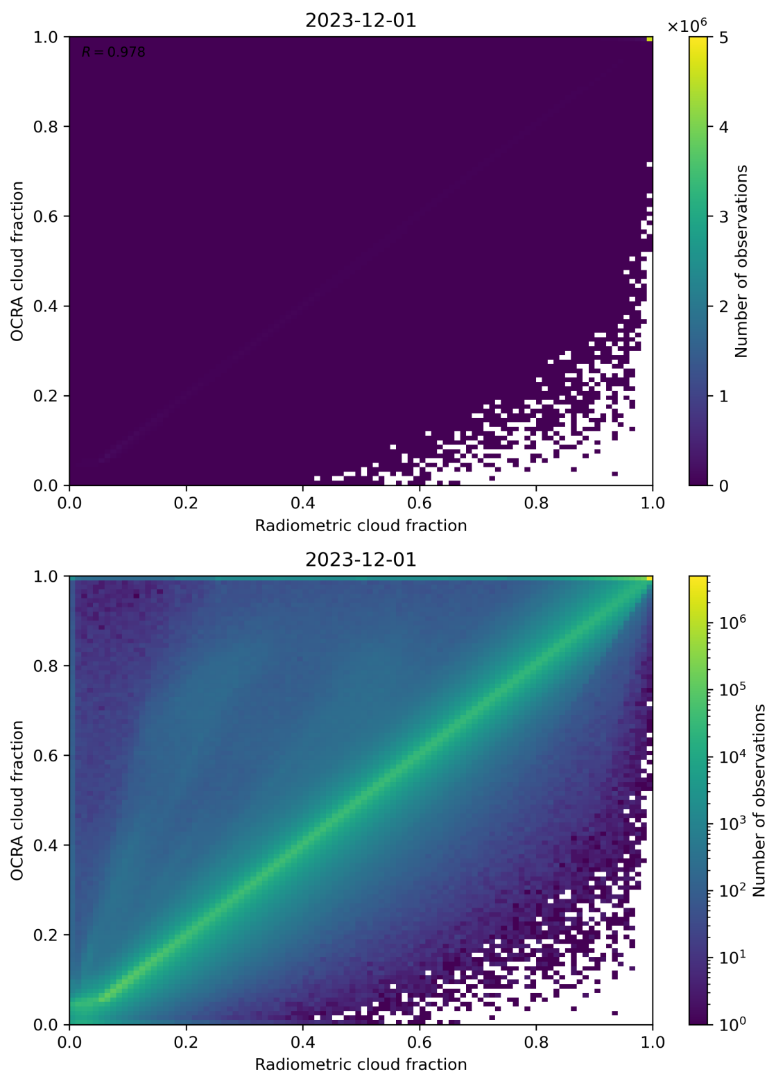
Figure 72: Scatter density plot of “Radiometric cloud fraction” against “OCRA cloud fraction” for 2023-11-30 to 2023-12-02.
