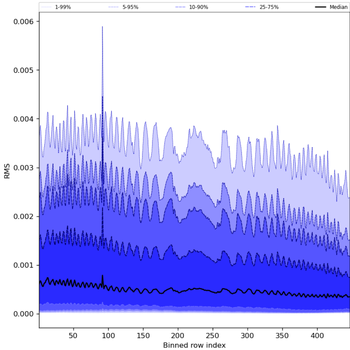
Figure 63: Along track statistics of “RMS” for 2023-11-30 to 2023-12-02
