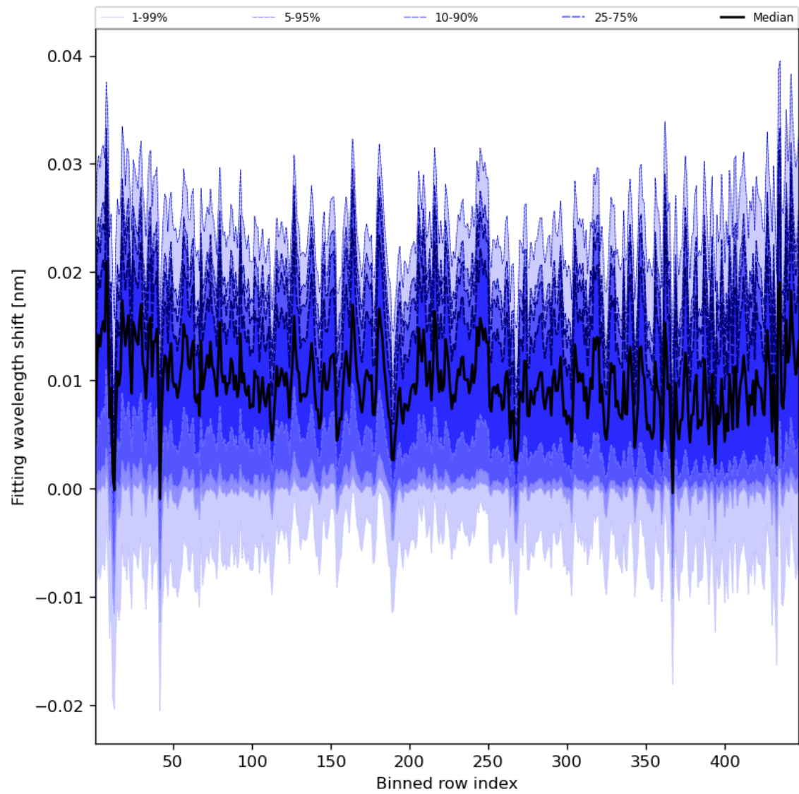
Figure 65: Along track statistics of “Fitting wavelength shift” for 2023-11-30 to 2023-12-02
