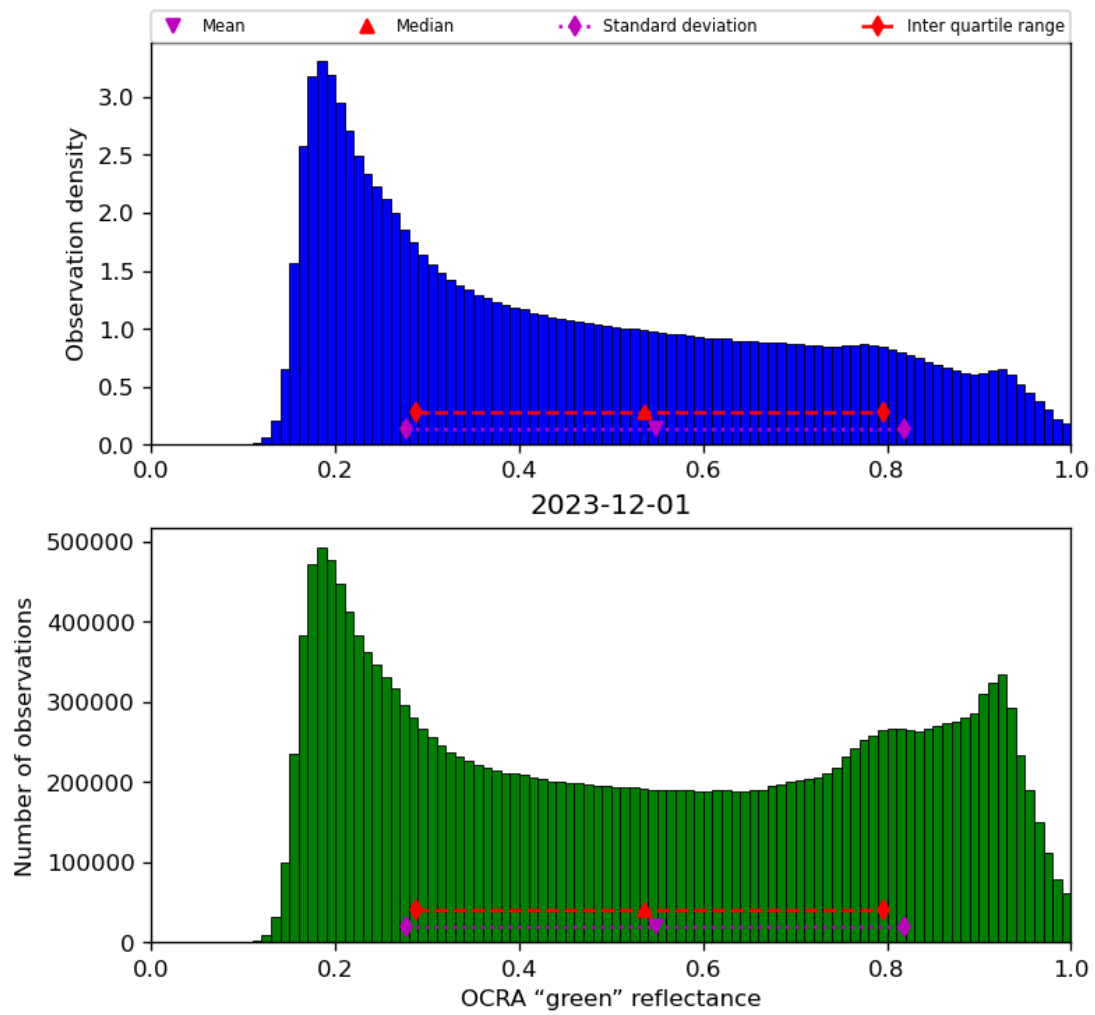
Figure 52: Histogram of “OCRA “green” reflectance” for 2023-11-30 to 2023-12-02
