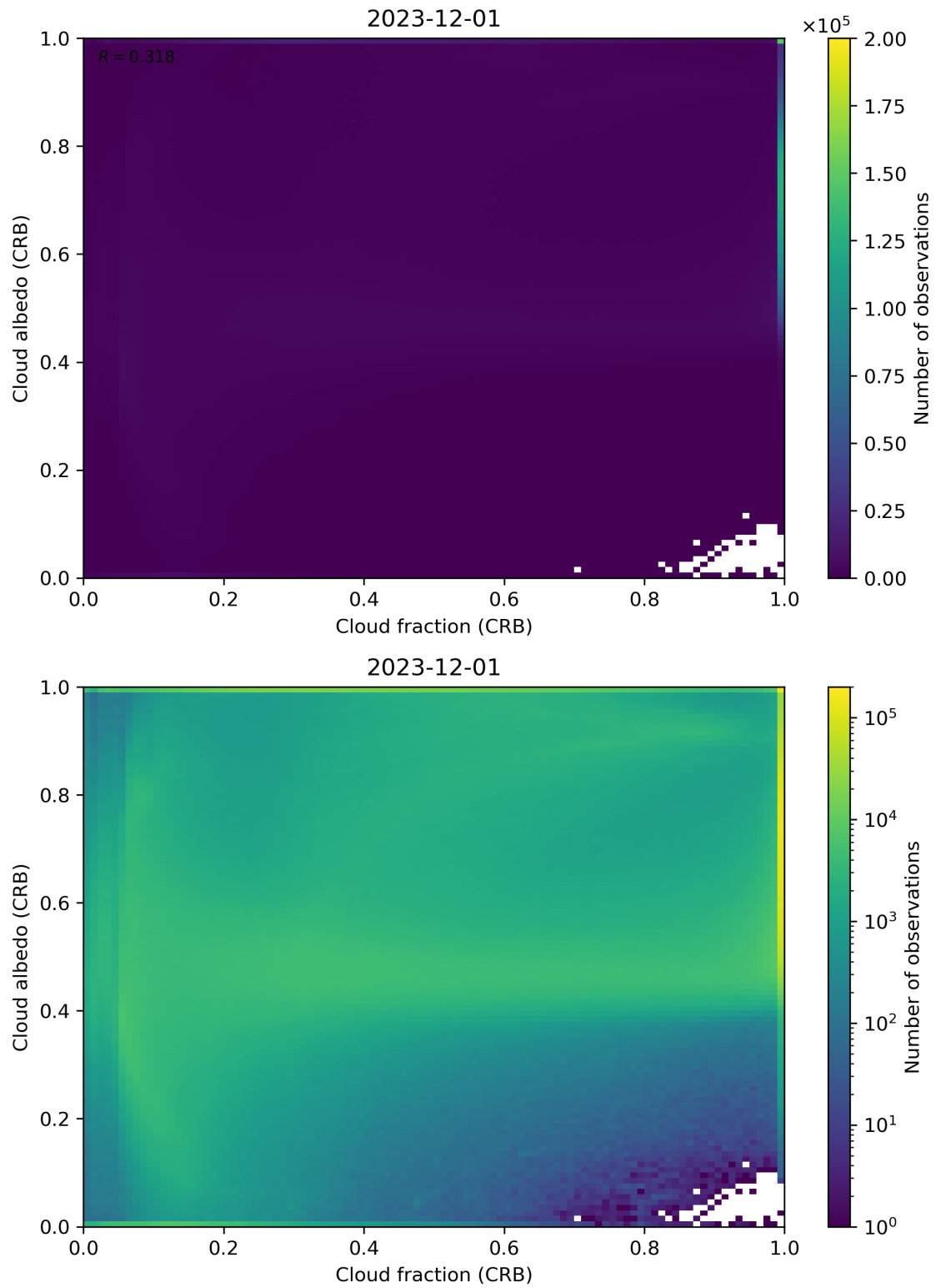
Figure 77: Scatter density plot of “Cloud fraction (CRB)” against “Cloud albedo (CRB)” for 2023-11-30 to 2023-12-02.
