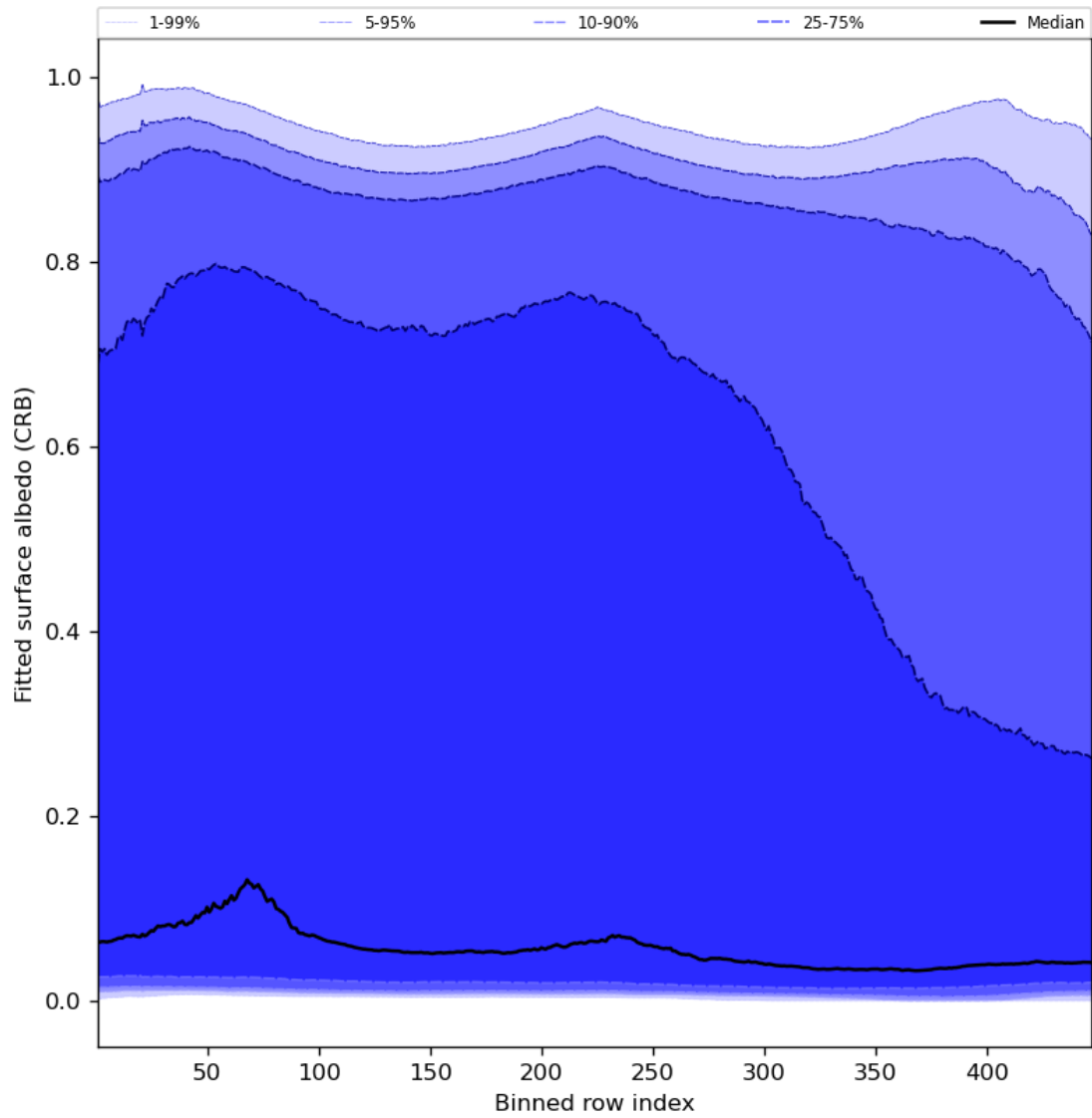
Figure 62: Along track statistics of “Fitted surface albedo (CRB)” for 2023-11-30 to 2023-12-02
