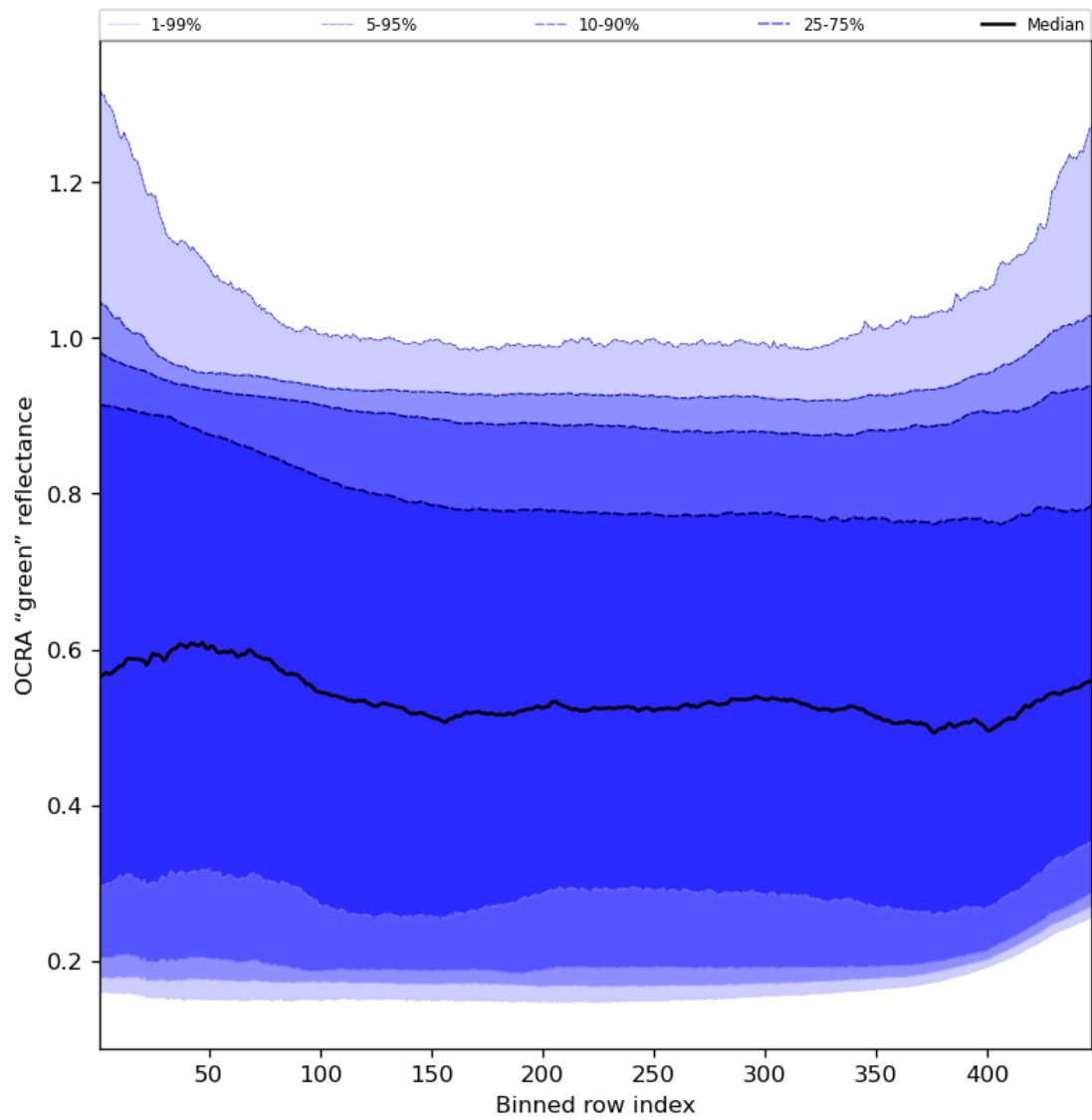
Figure 68: Along track statistics of "OCRA "green" reflectance" for 2023-11-30 to 2023-12-02
