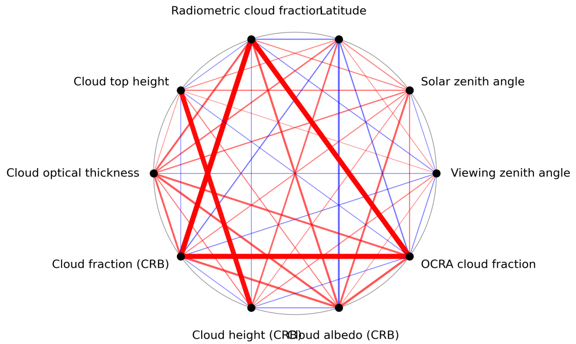
Figure 1: Map of correlation graph for 2023-11-30 to 2023-12-02.
