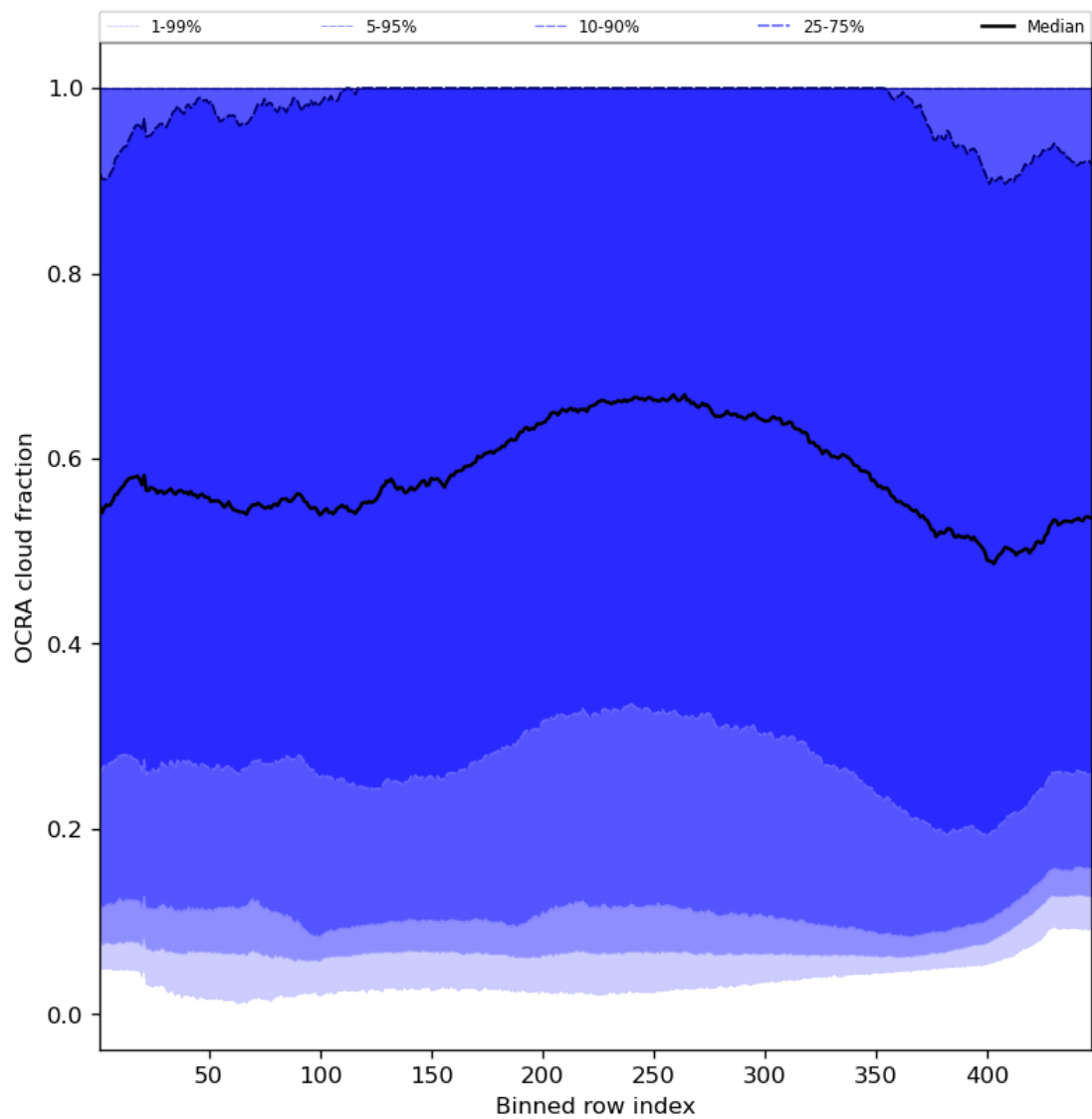
Figure 66: Along track statistics of “OCRA cloud fraction” for 2023-11-30 to 2023-12-02
