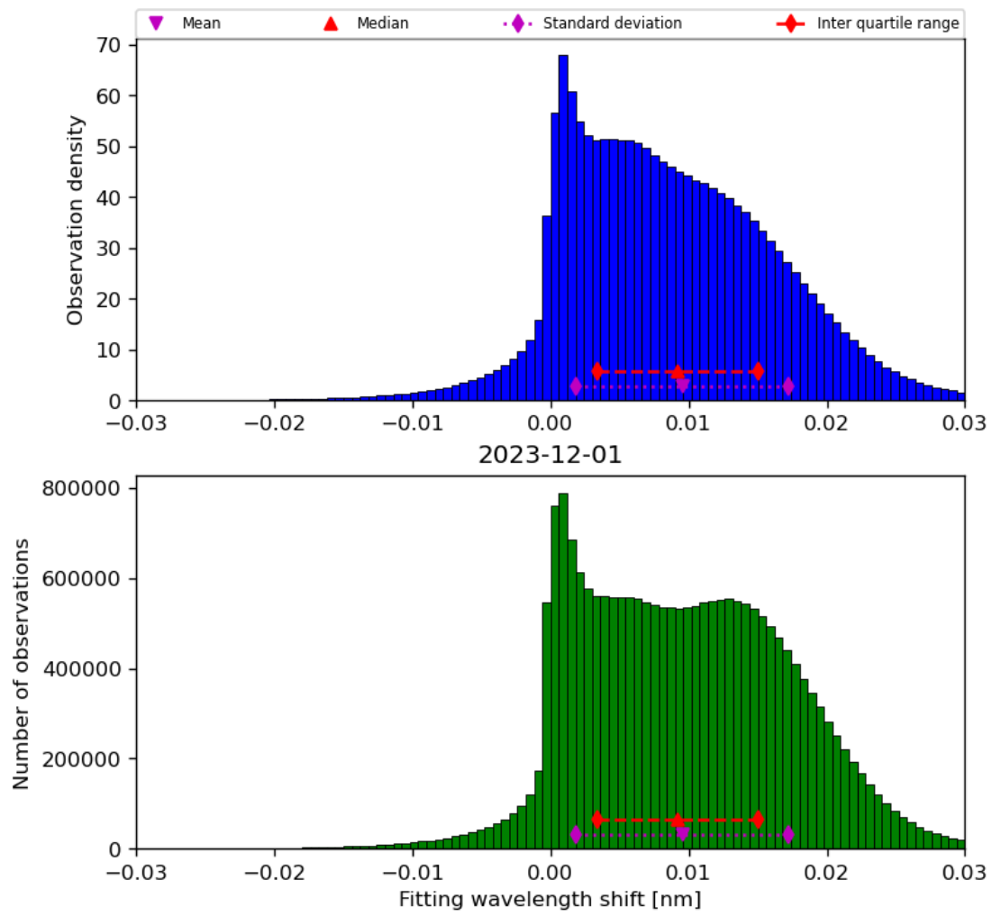
Figure 49: Histogram of “Fitting wavelength shift” for 2023-11-30 to 2023-12-02
