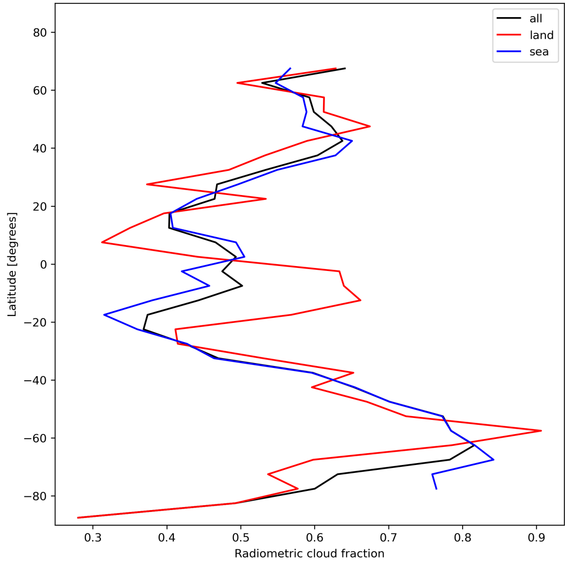
Figure 23: Zonal average of “Radiometric cloud fraction” for 2023-11-30 to 2023-12-02.
