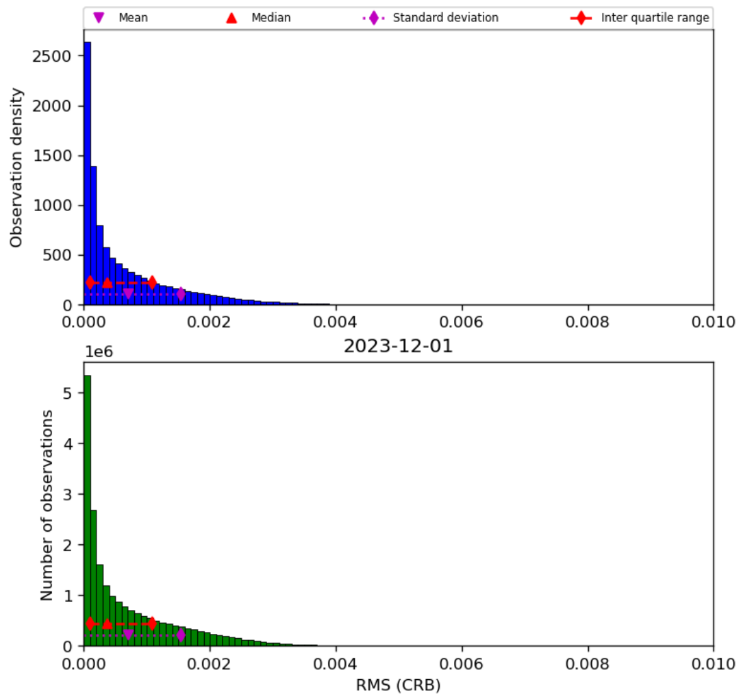
Figure 48: Histogram of “RMS (CRB)” for 2023-11-30 to 2023-12-02
