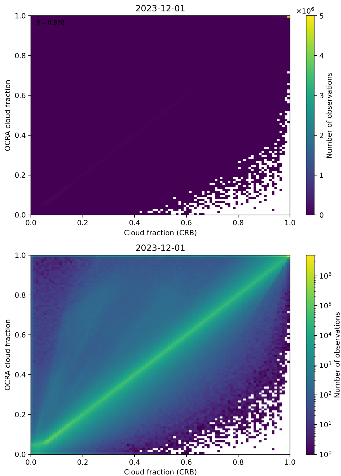
Figure 78: Scatter density plot of “Cloud fraction (CRB)” against “OCRA cloud fraction” for 2023-11-30 to 2023-12-02.
