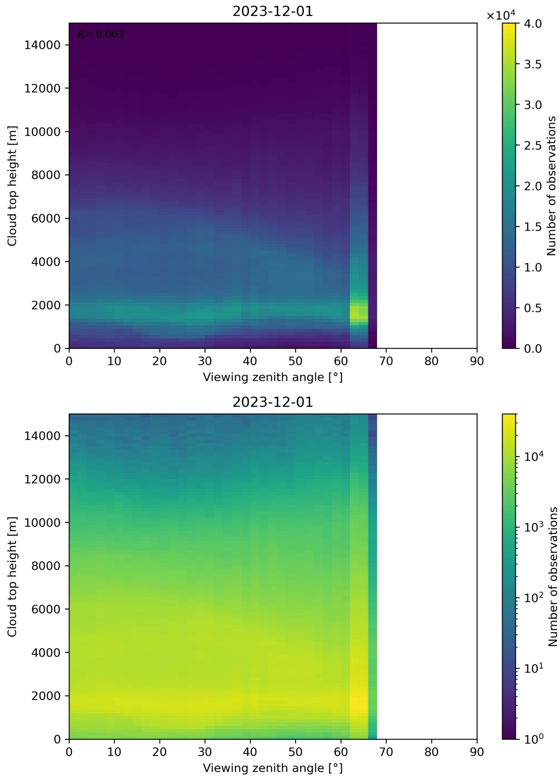
Figure 112: Scatter density plot of “Viewing zenith angle” against “Cloud top height” for 2023-11-30 to 2023-12-02.
