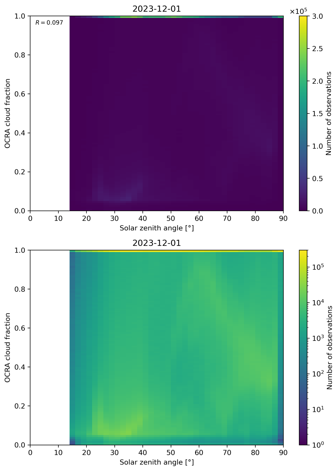
Figure 100: Scatter density plot of “Solar zenith angle” against “OCRA cloud fraction” for 2023-11-30 to 2023-12-02.
