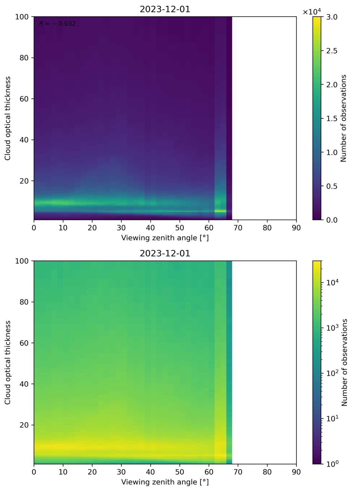
Figure 111: Scatter density plot of “Viewing zenith angle” against “Cloud optical thickness” for 2023-11-30 to 2023-12-02.
