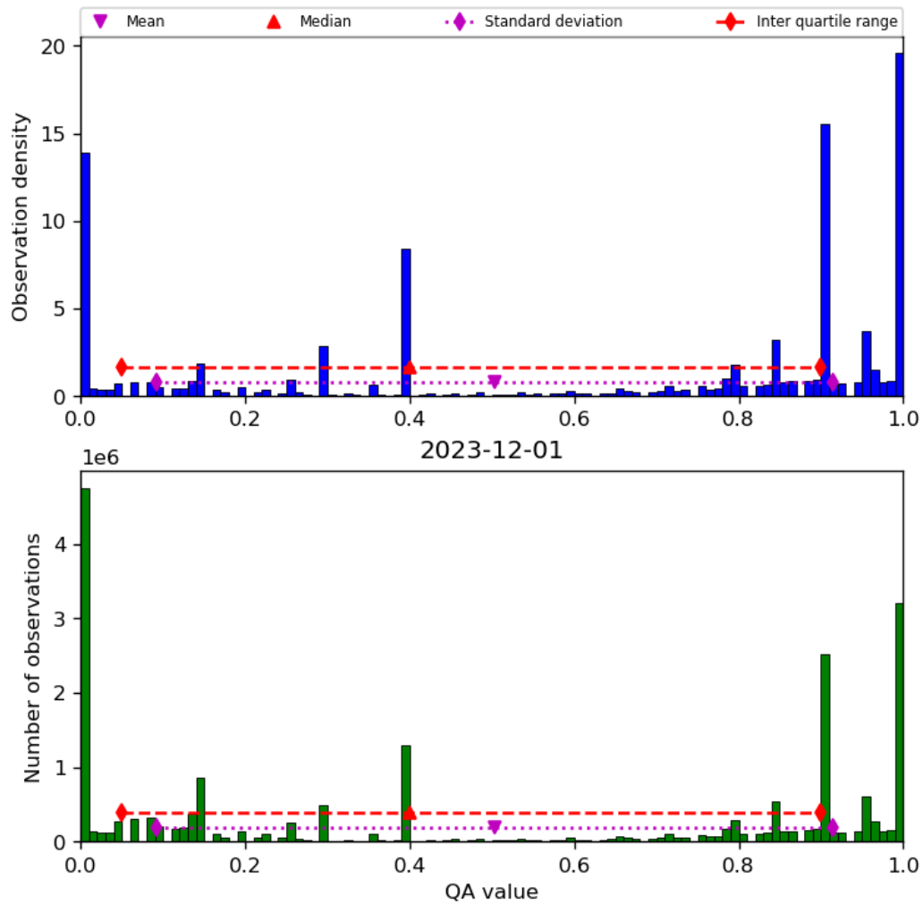
Figure 38: Histogram of “QA value” for 2023-11-30 to 2023-12-02
