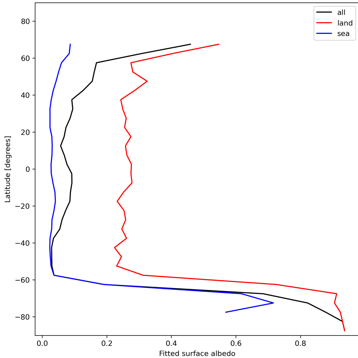
Figure 29: Zonal average of “Fitted surface albedo” for 2023-11-30 to 2023-12-02.
