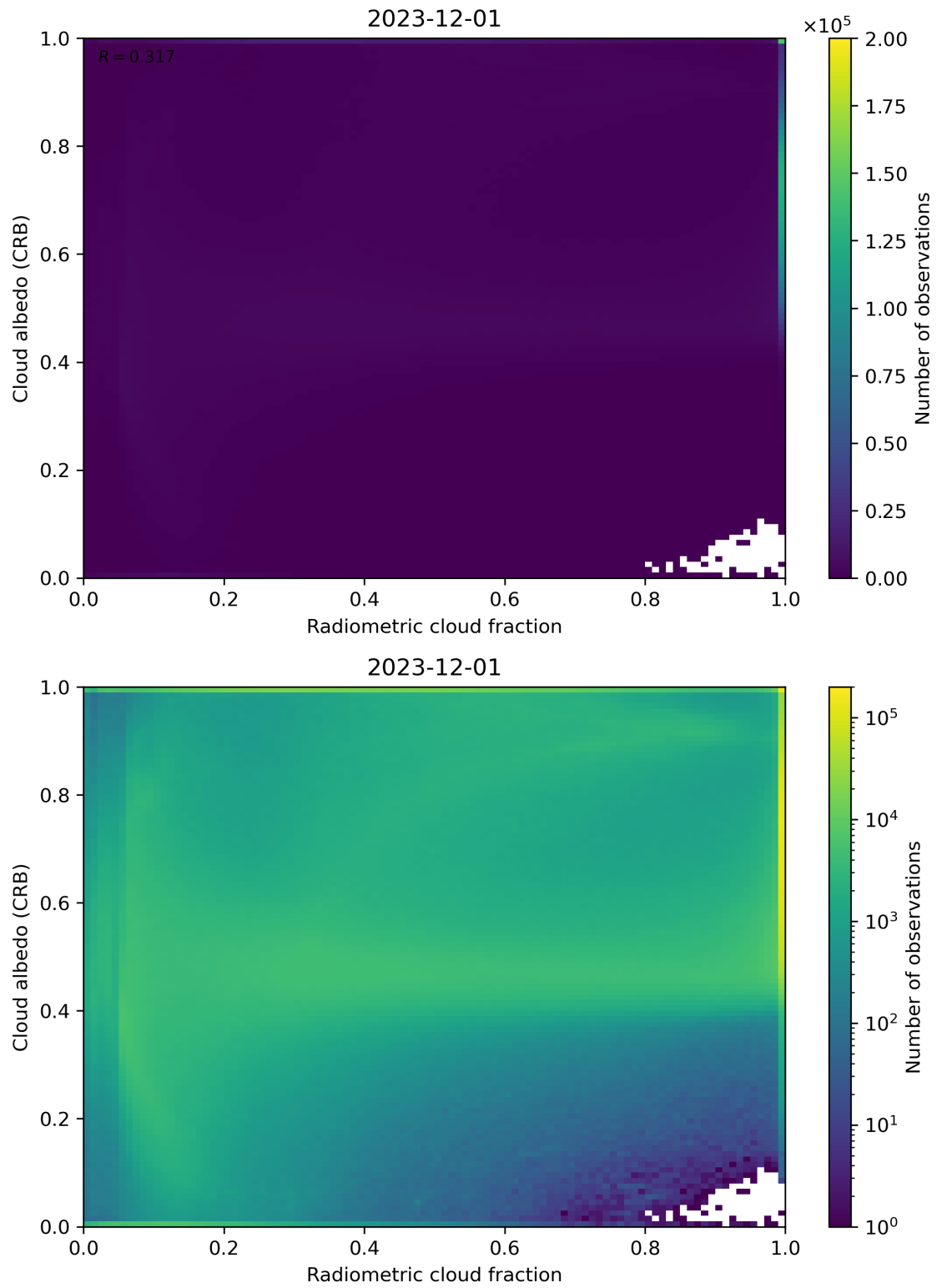
Figure 71: Scatter density plot of “Radiometric cloud fraction” against “Cloud albedo (CRB)” for 2023-11-30 to 2023-12-02.
