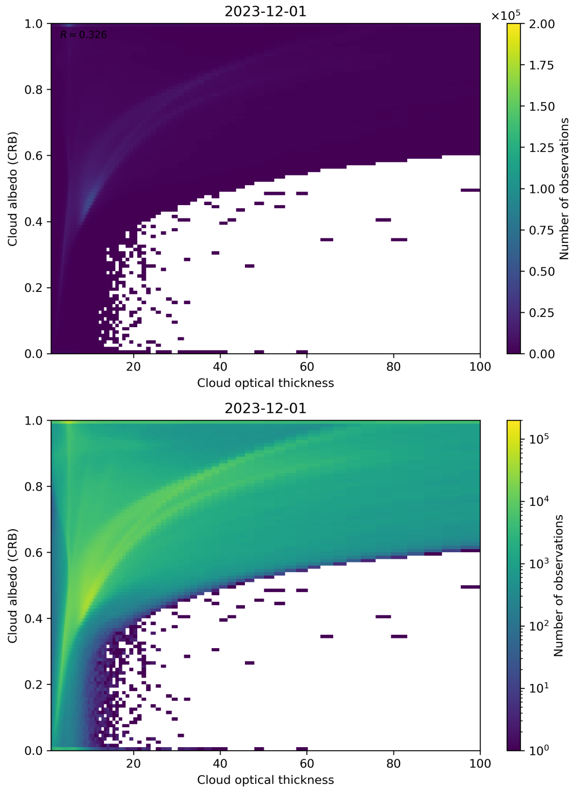
Figure 82: Scatter density plot of “Cloud optical thickness” against “Cloud albedo (CRB)” for 2023-11-30 to 2023-12-02.
