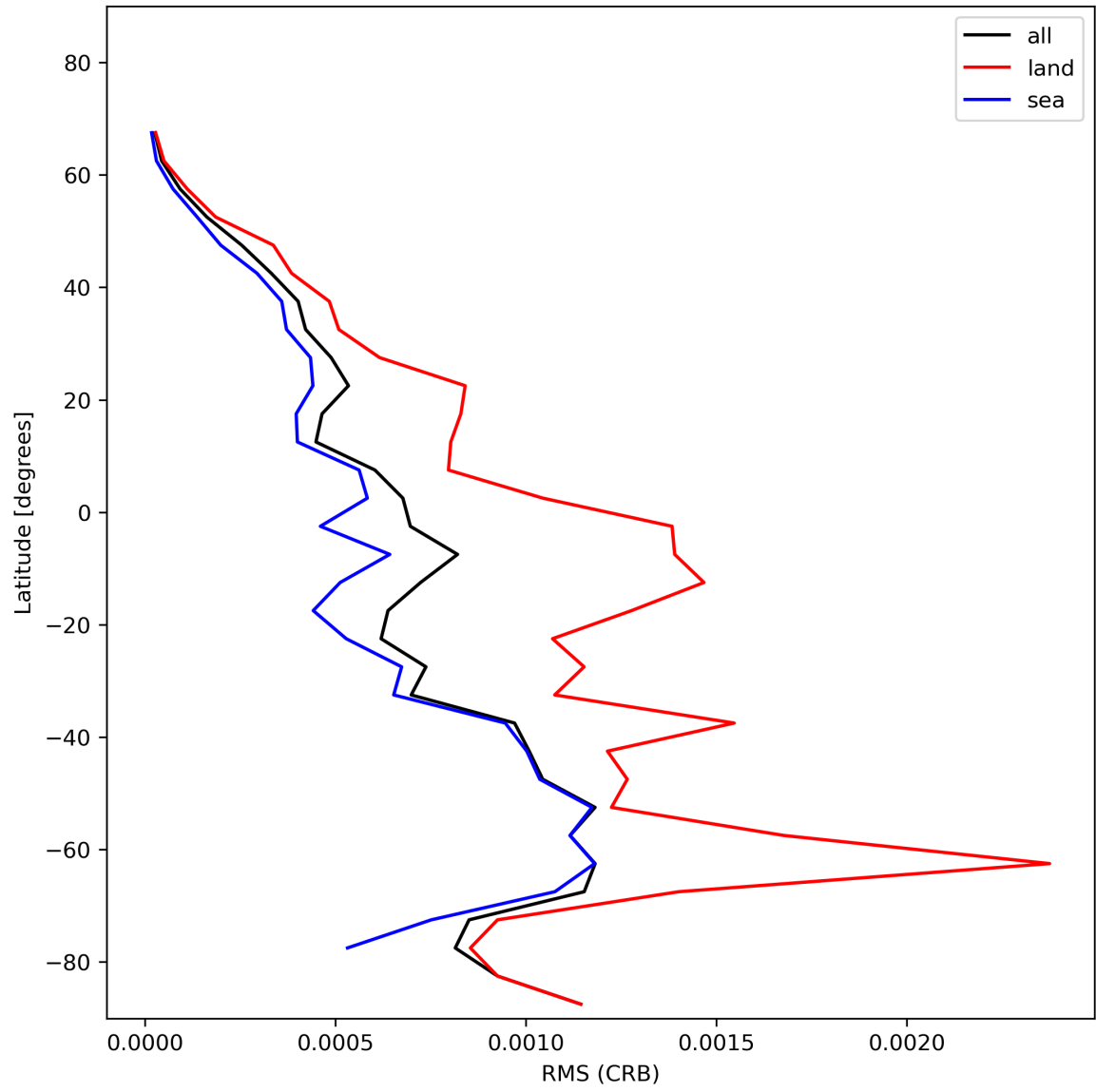
Figure 32: Zonal average of “RMS (CRB)” for 2023-11-30 to 2023-12-02.
