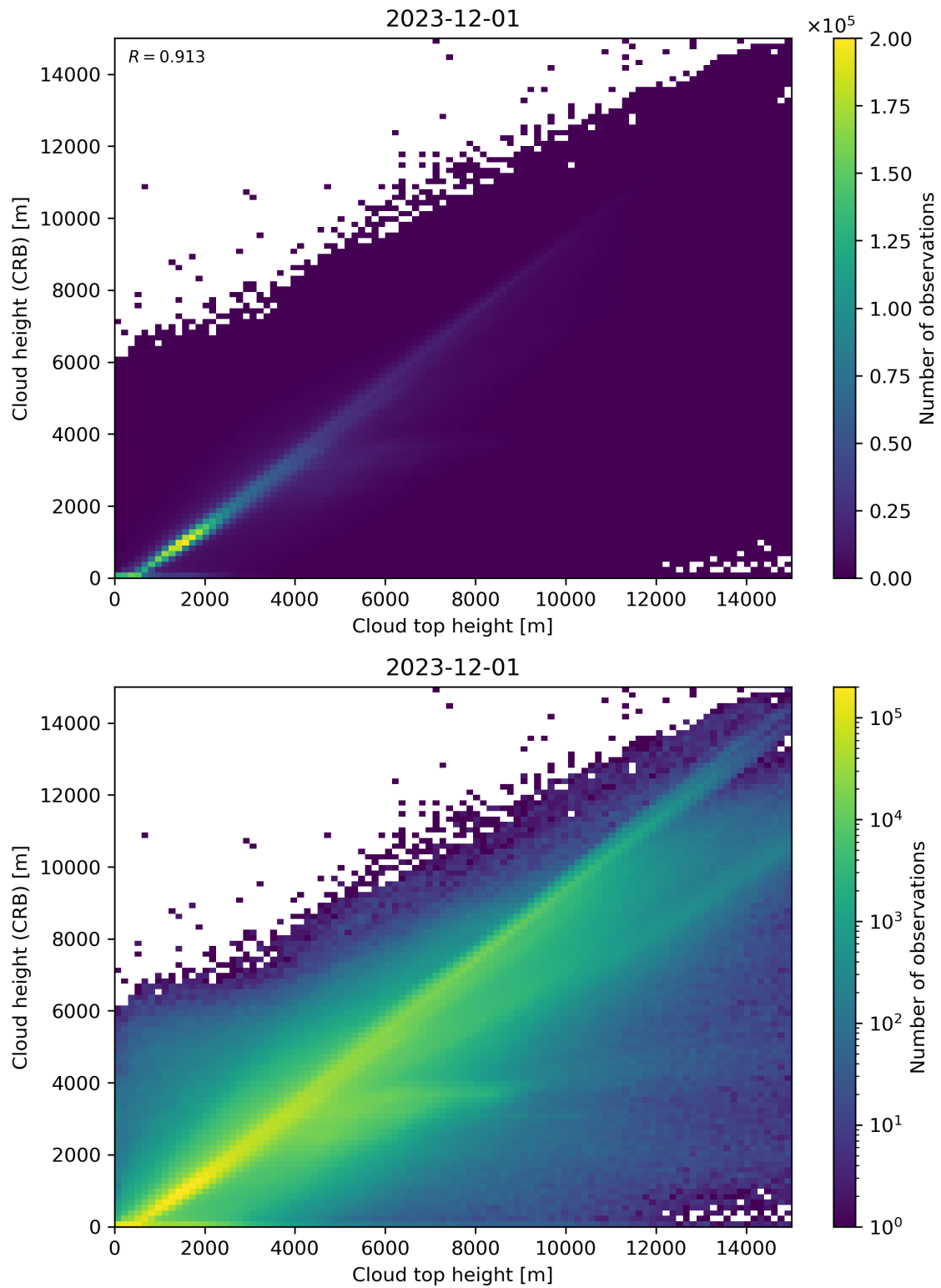
Figure 89: Scatter density plot of “Cloud top height” against “Cloud height (CRB)” for 2023-11-30 to 2023-12-02.
