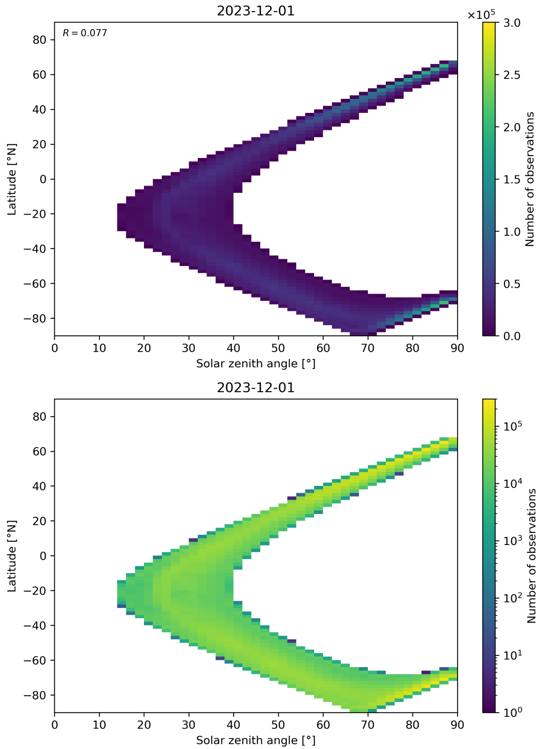
Figure 105: Scatter density plot of “Solar zenith angle” against “Latitude” for 2023-11-30 to 2023-12-02.
