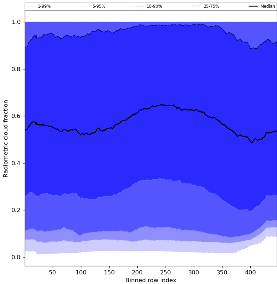
Figure 55: Along track statistics of “Radiometric cloud fraction” for 2023-11-30 to 2023-12-02
