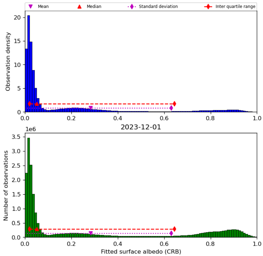
Figure 46: Histogram of “Fitted surface albedo (CRB)” for 2023-11-30 to 2023-12-02
