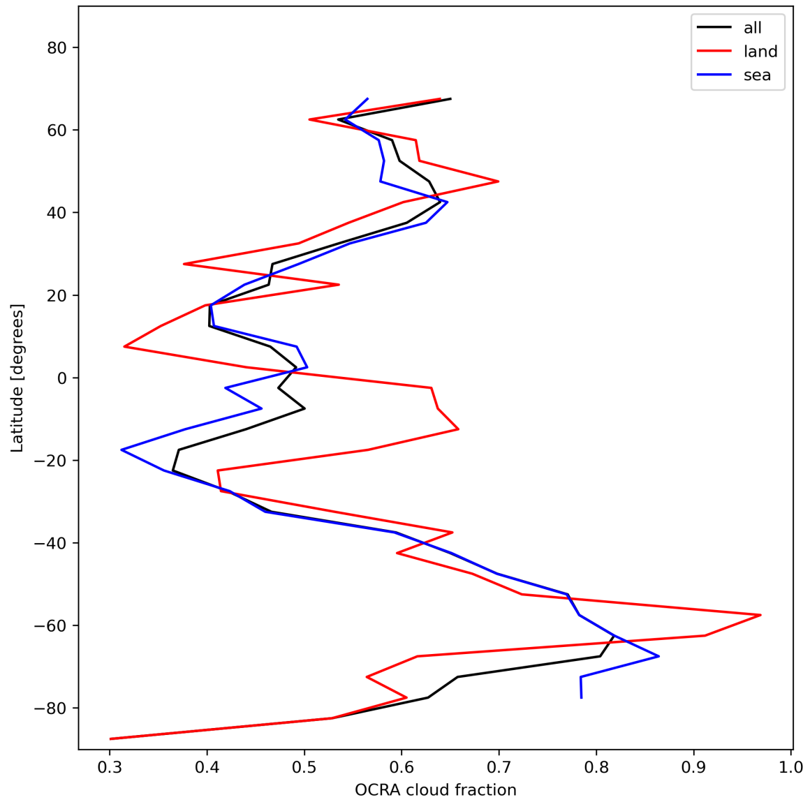
Figure 34: Zonal average of “OCRA cloud fraction” for 2023-11-30 to 2023-12-02.
