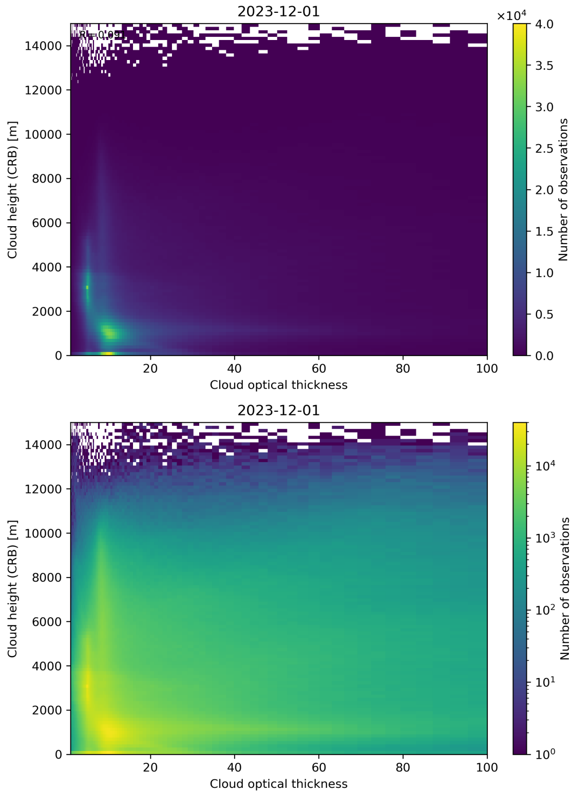
Figure 85: Scatter density plot of “Cloud optical thickness” against “Cloud height (CRB)” for 2023-11-30 to 2023-12-02.
