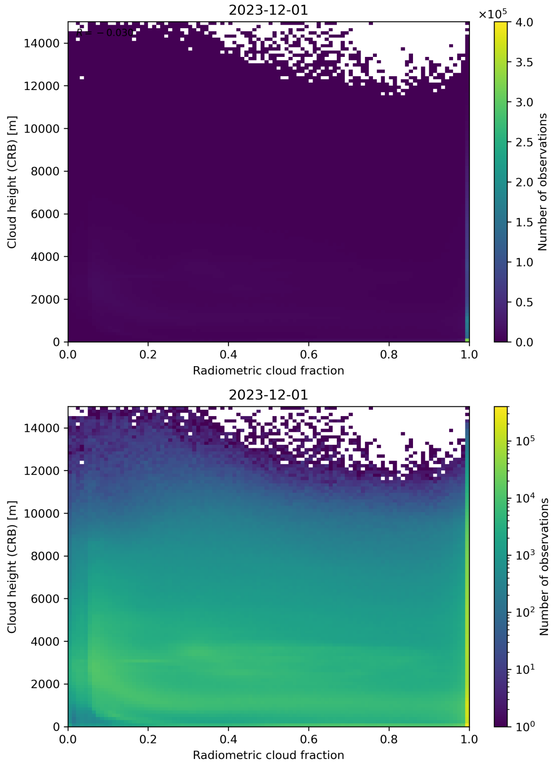
Figure 74: Scatter density plot of “Radiometric cloud fraction” against “Cloud height (CRB)” for 2023-11-30 to 2023-12-02.
