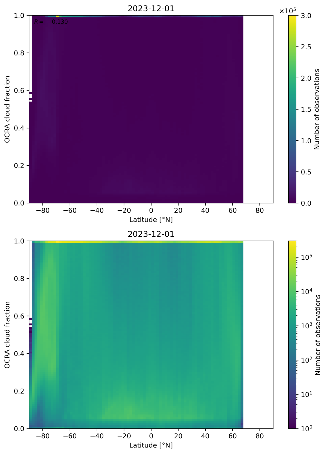
Figure 93: Scatter density plot of “Latitude” against “OCRA cloud fraction” for 2023-11-30 to 2023-12-02.
