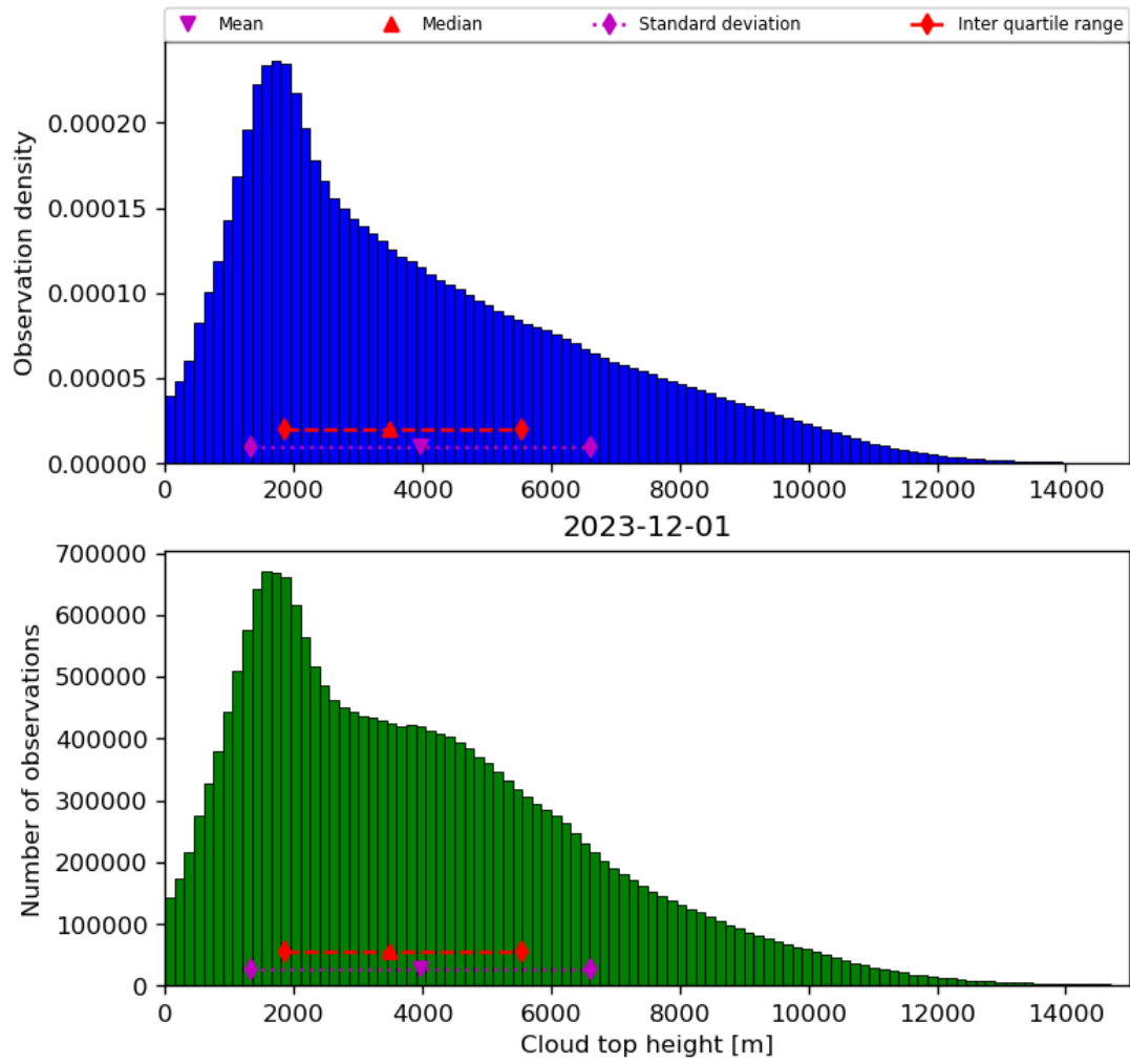
Figure 40: Histogram of “Cloud top height” for 2023-11-30 to 2023-12-02
