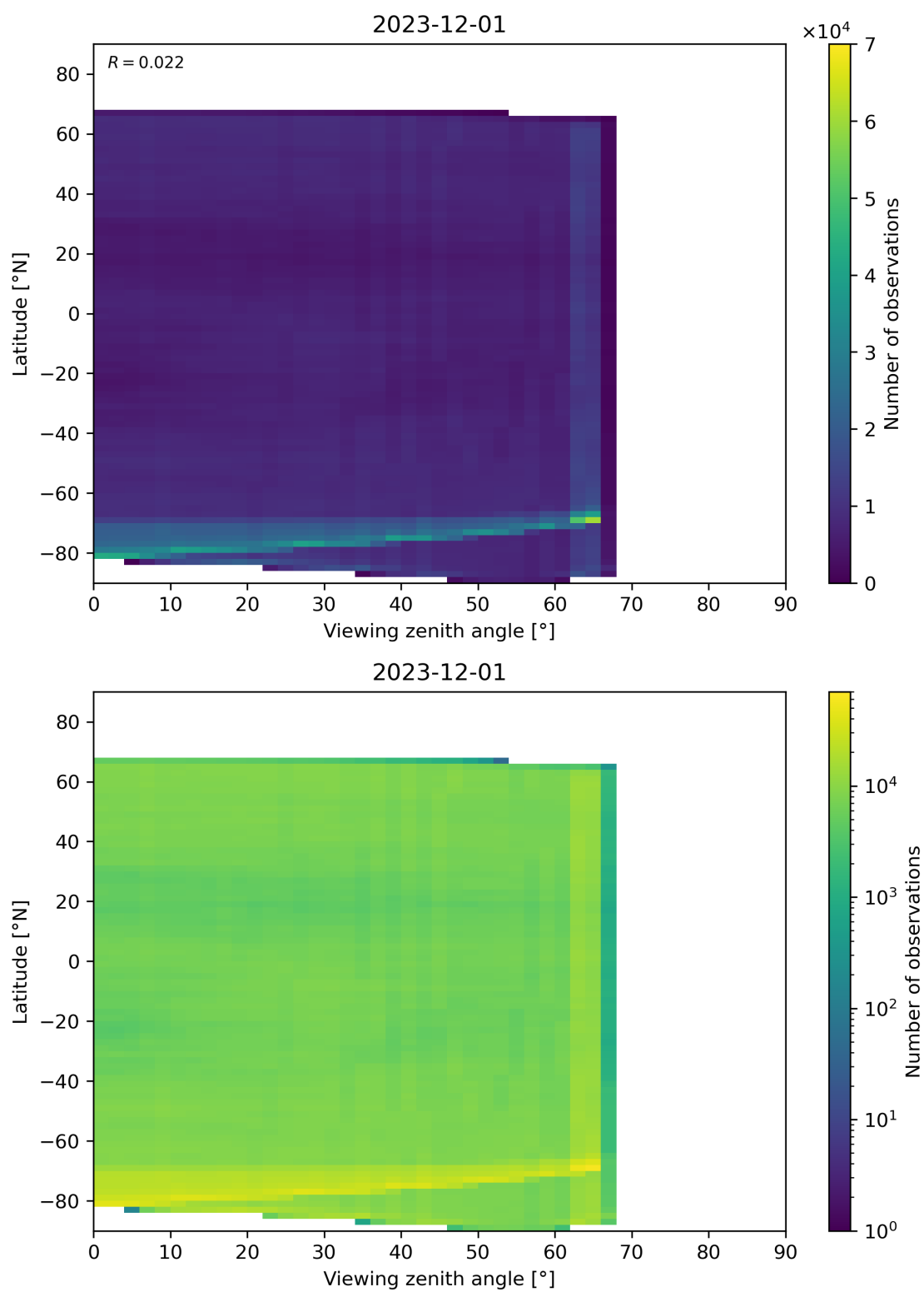
Figure 113: Scatter density plot of “Viewing zenith angle” against “Latitude” for 2023-11-30 to 2023-12-02.
