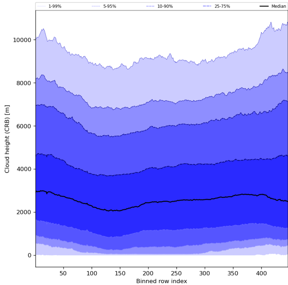
Figure 59: Along track statistics of “Cloud height (CRB)” for 2023-11-30 to 2023-12-02
