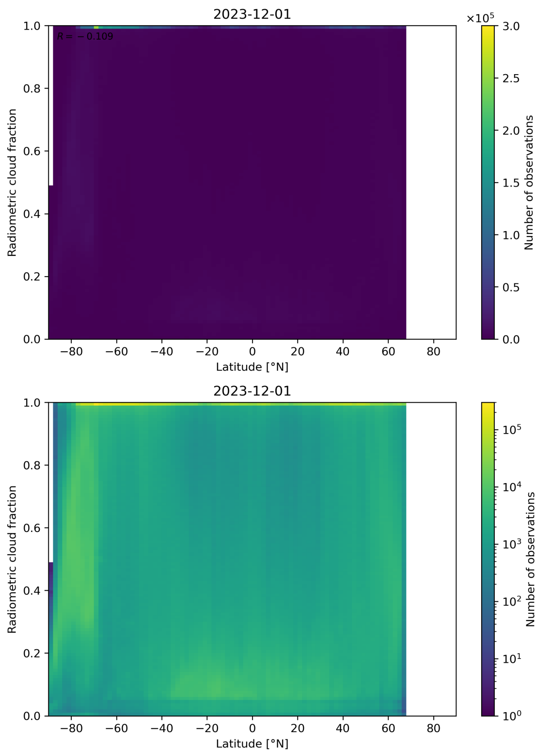
Figure 92: Scatter density plot of “Latitude” against “Radiometric cloud fraction” for 2023-11-30 to 2023-12-02.
