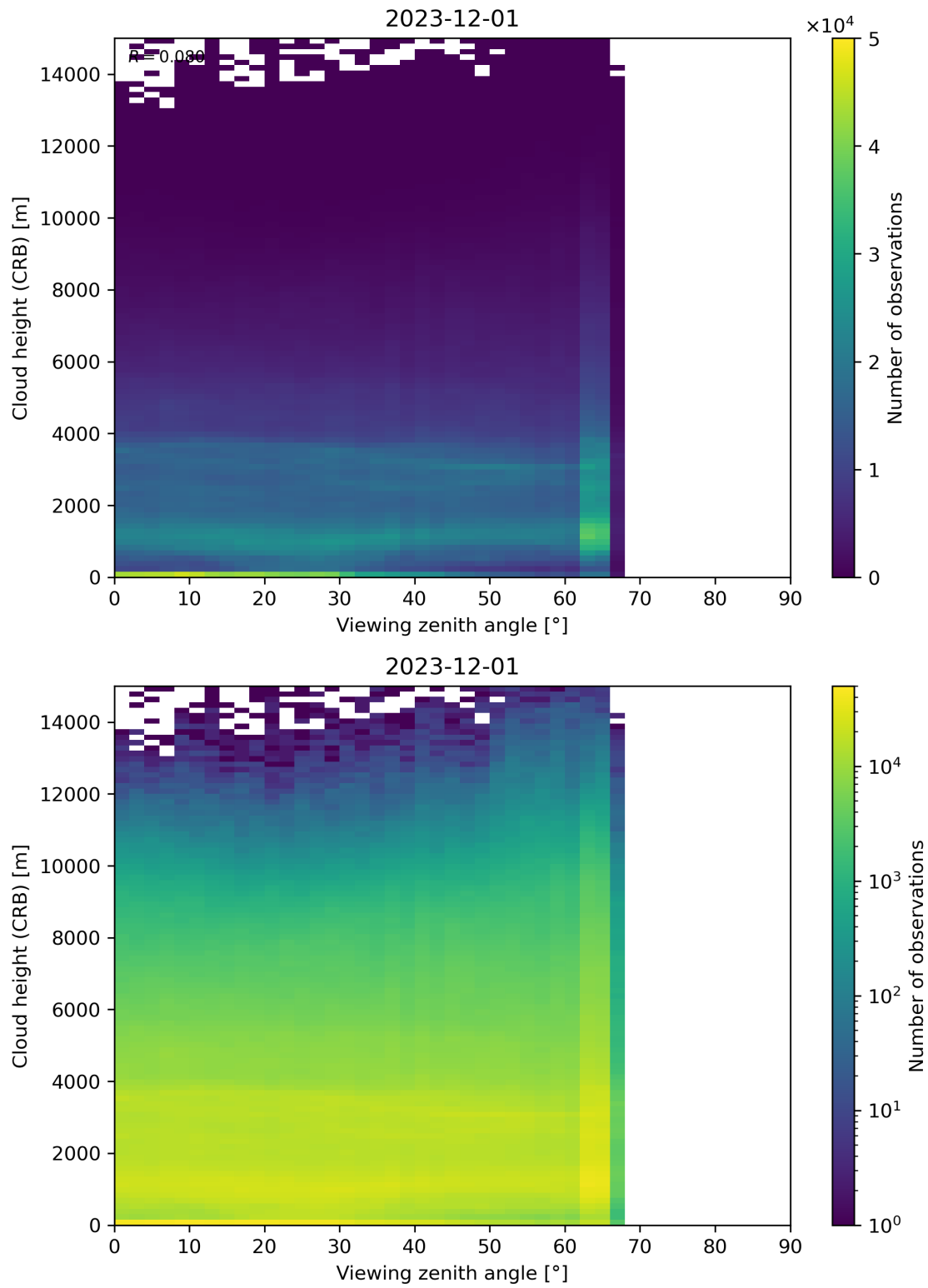
Figure 110: Scatter density plot of “Viewing zenith angle” against “Cloud height (CRB)” for 2023-11-30 to 2023-12-02.
