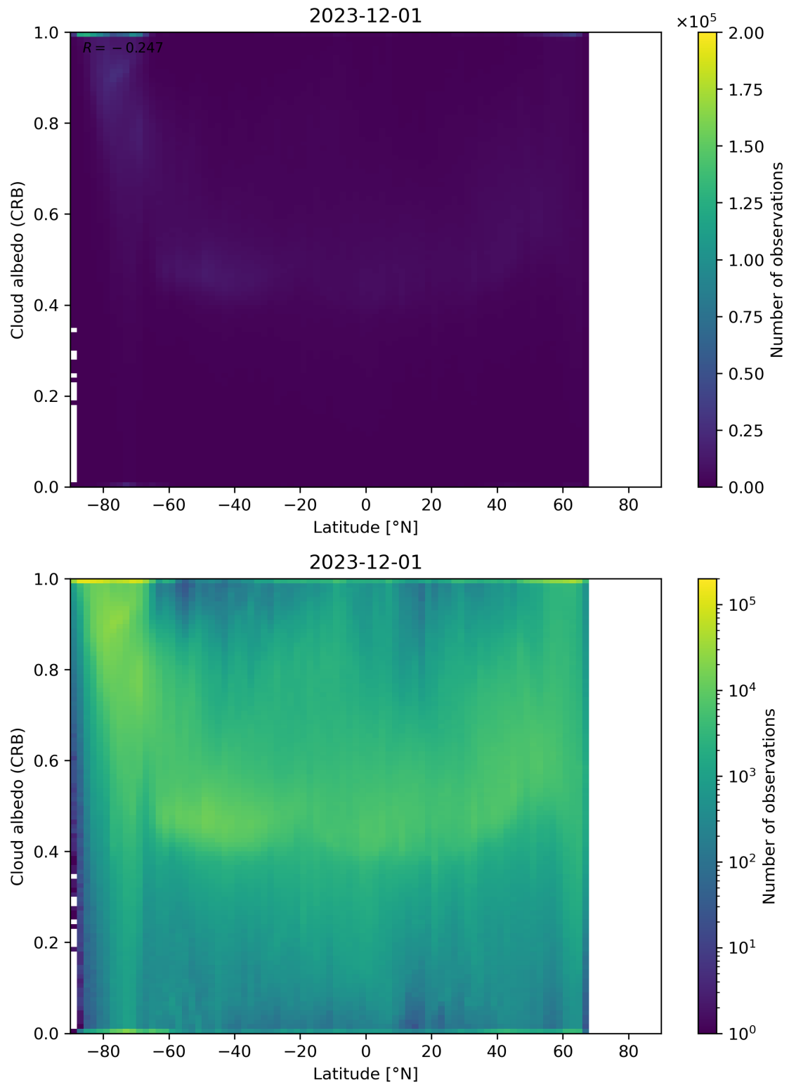
Figure 91: Scatter density plot of “Latitude” against “Cloud albedo (CRB)” for 2023-11-30 to 2023-12-02.
