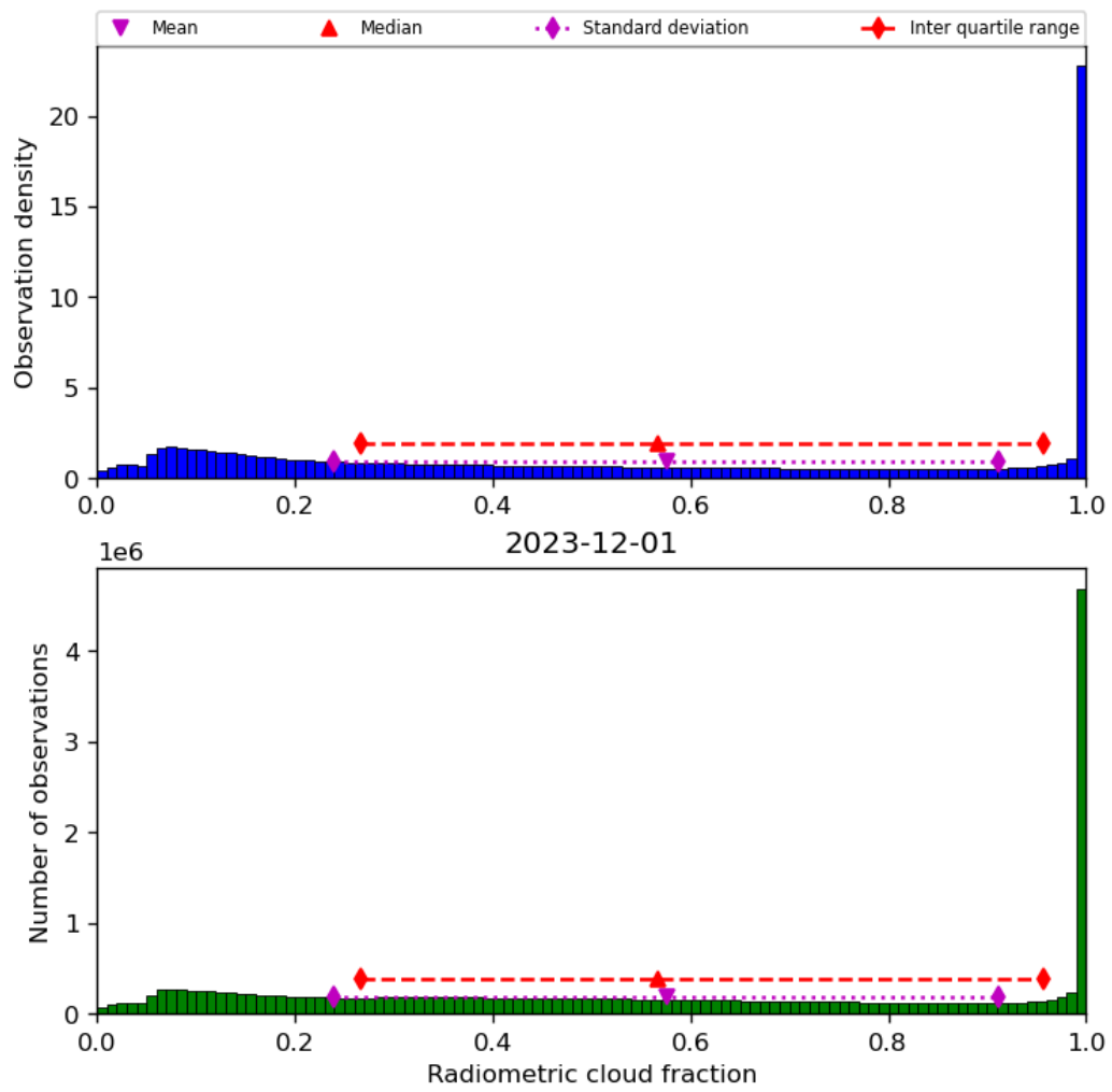
Figure 39: Histogram of “Radiometric cloud fraction” for 2023-11-30 to 2023-12-02
