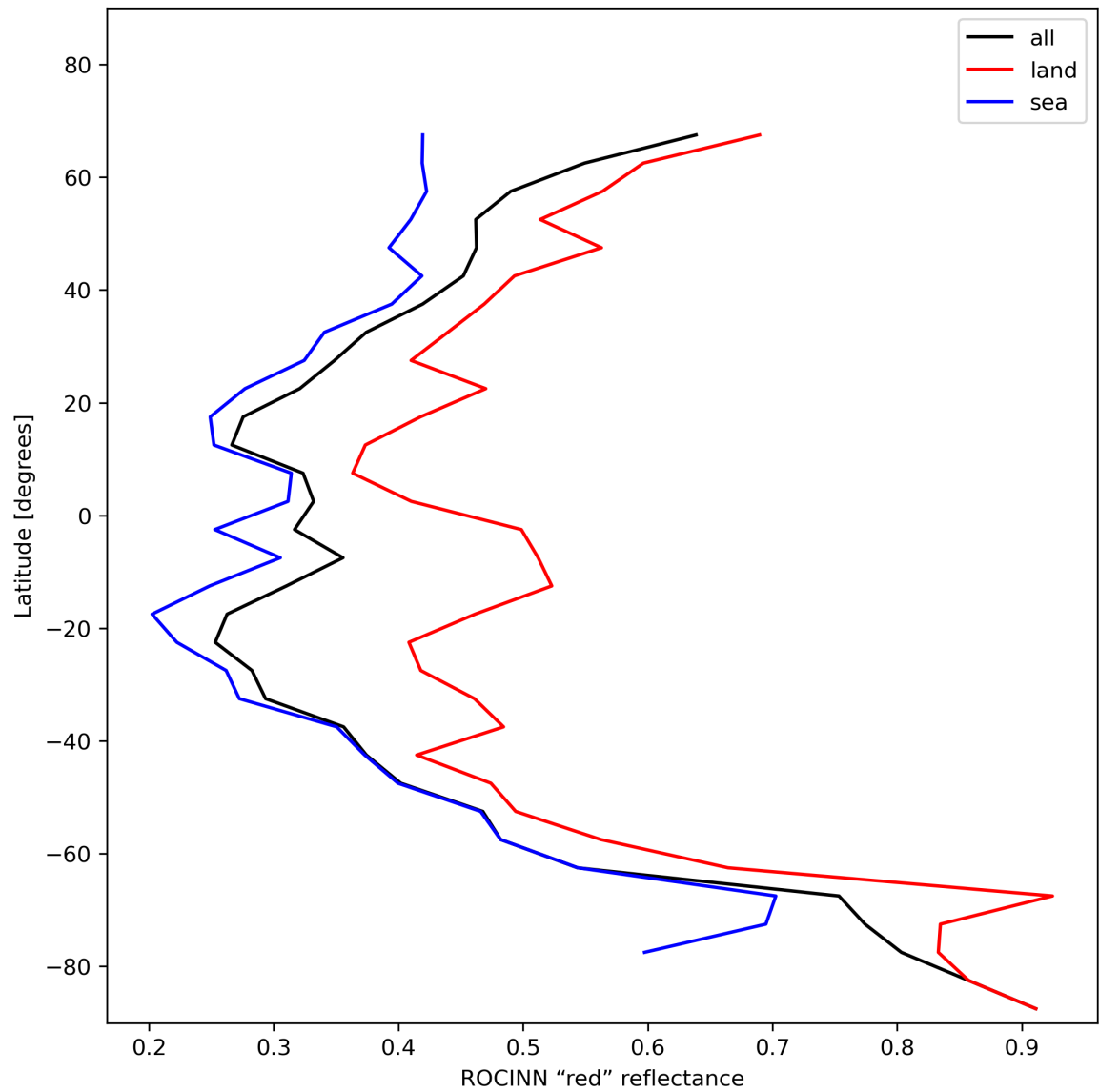
Figure 37: Zonal average of "ROCINN "red" reflectance" for 2023-11-30 to 2023-12-02.
