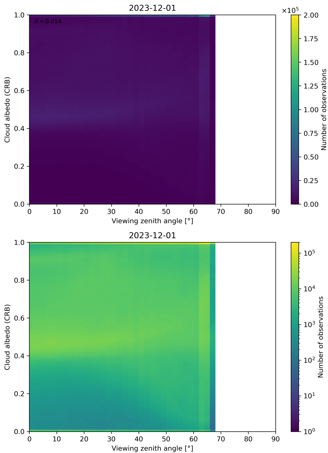
Figure 106: Scatter density plot of “Viewing zenith angle” against “Cloud albedo (CRB)” for 2023-11-30 to 2023-12-02.
