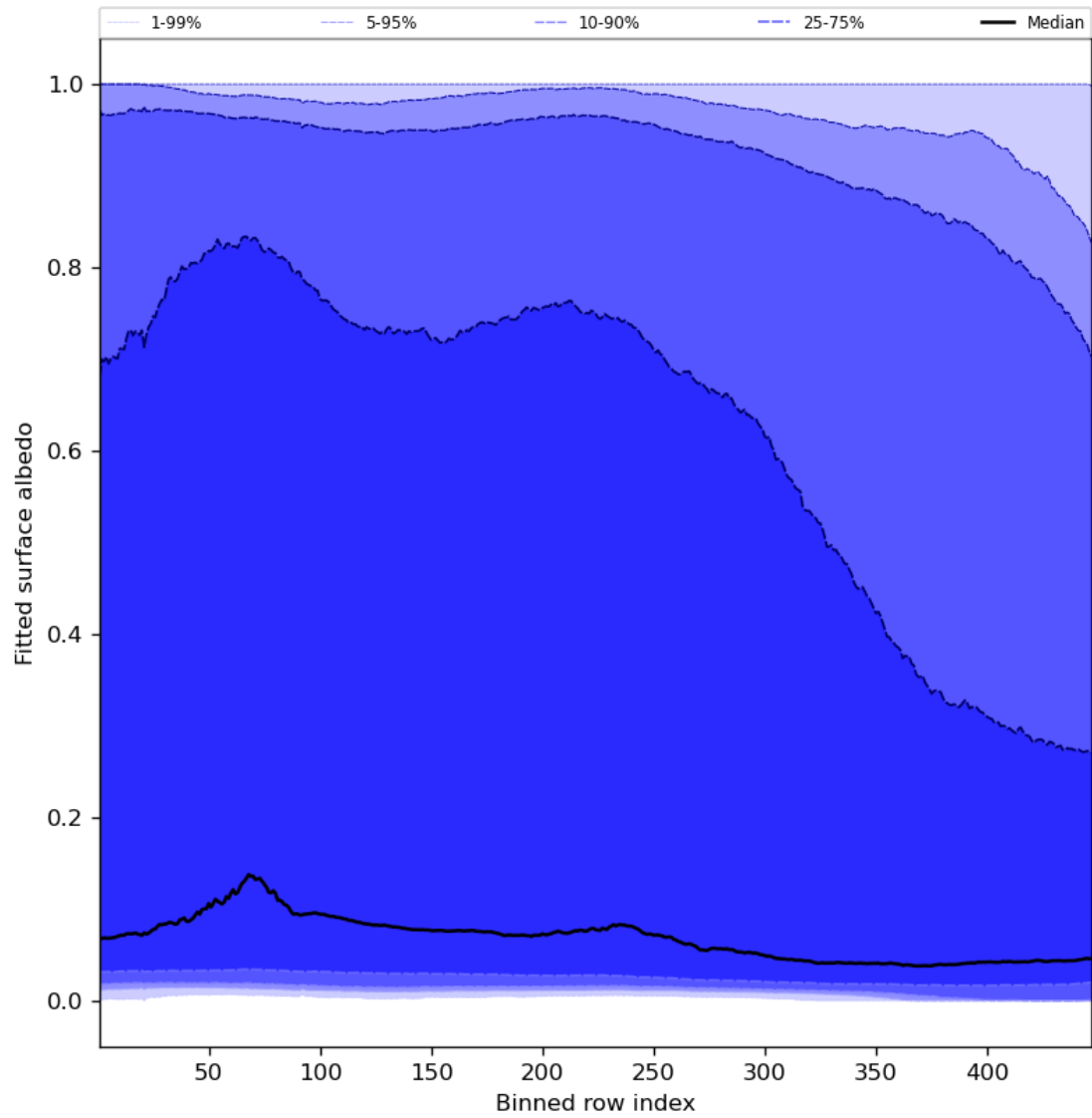
Figure 61: Along track statistics of “Fitted surface albedo” for 2023-11-30 to 2023-12-02
