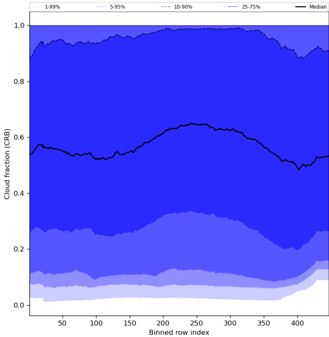
Figure 58: Along track statistics of “Cloud fraction (CRB)” for 2023-11-30 to 2023-12-02
