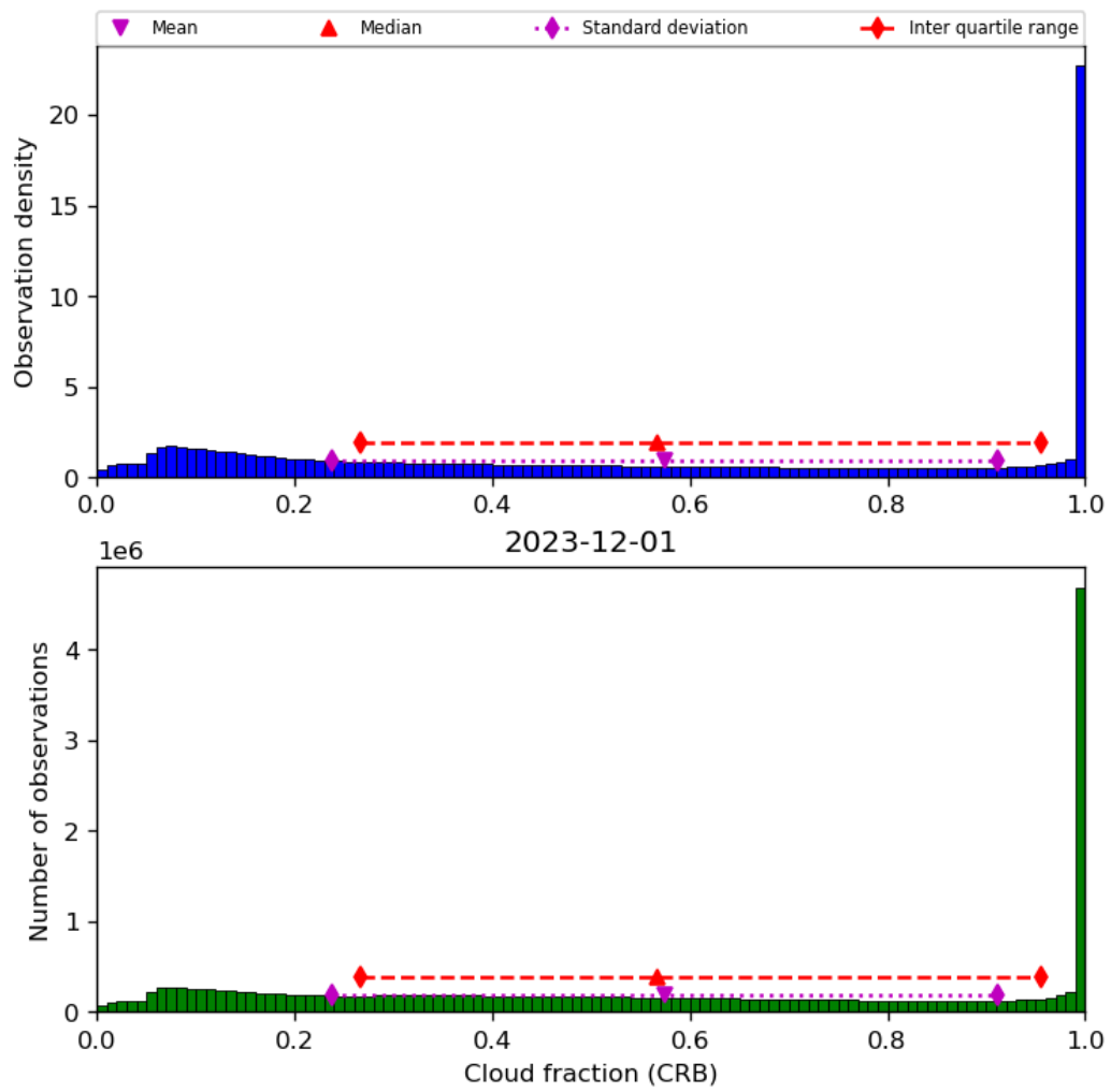
Figure 42: Histogram of “Cloud fraction (CRB)” for 2023-11-30 to 2023-12-02
