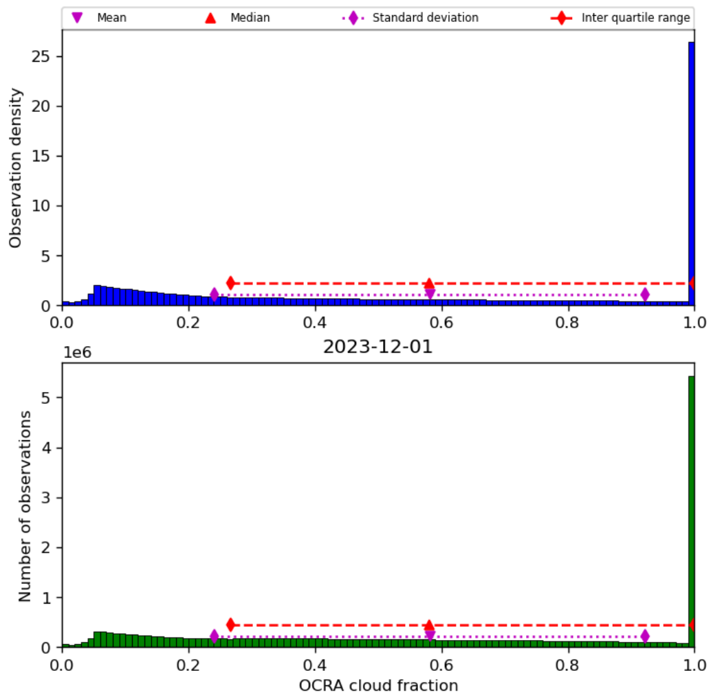
Figure 50: Histogram of “OCRA cloud fraction” for 2023-11-30 to 2023-12-02
