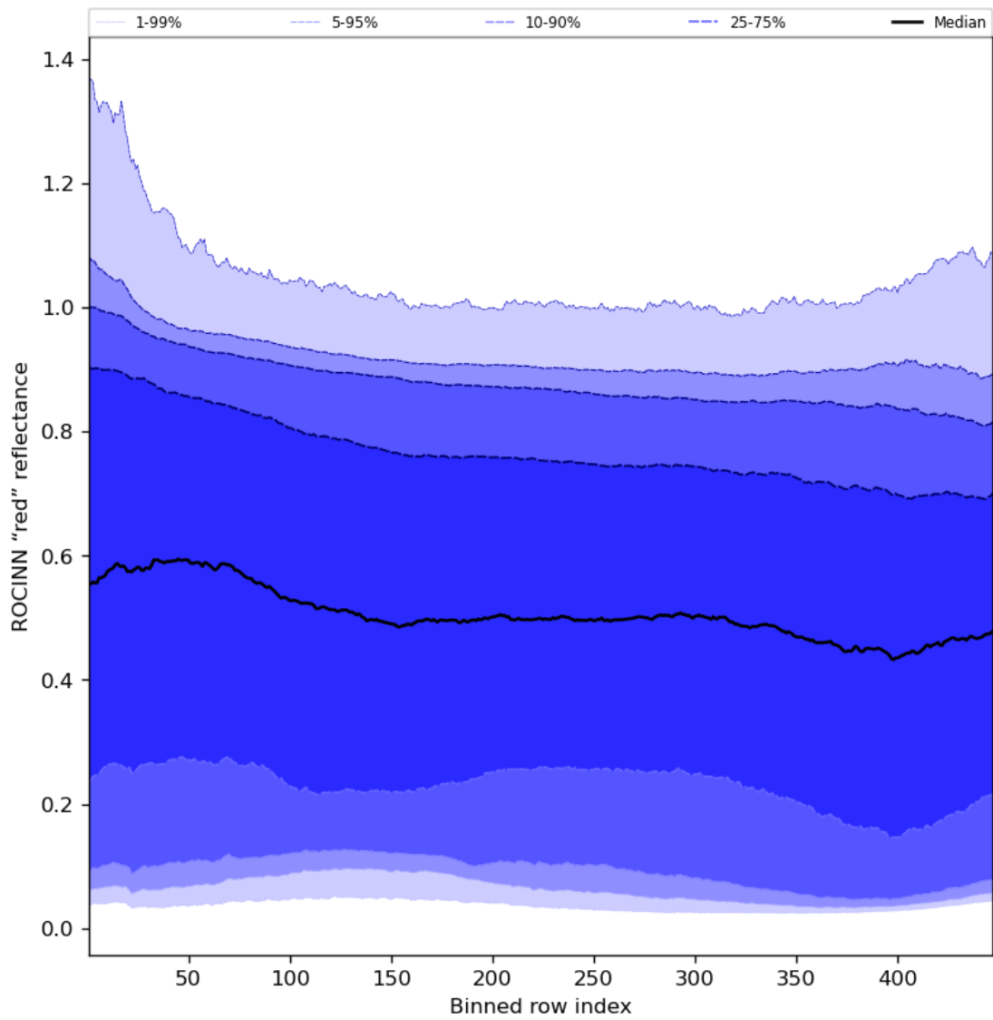
Figure 69: Along track statistics of "ROCINN "red" reflectance" for 2023-11-30 to 2023-12-02
