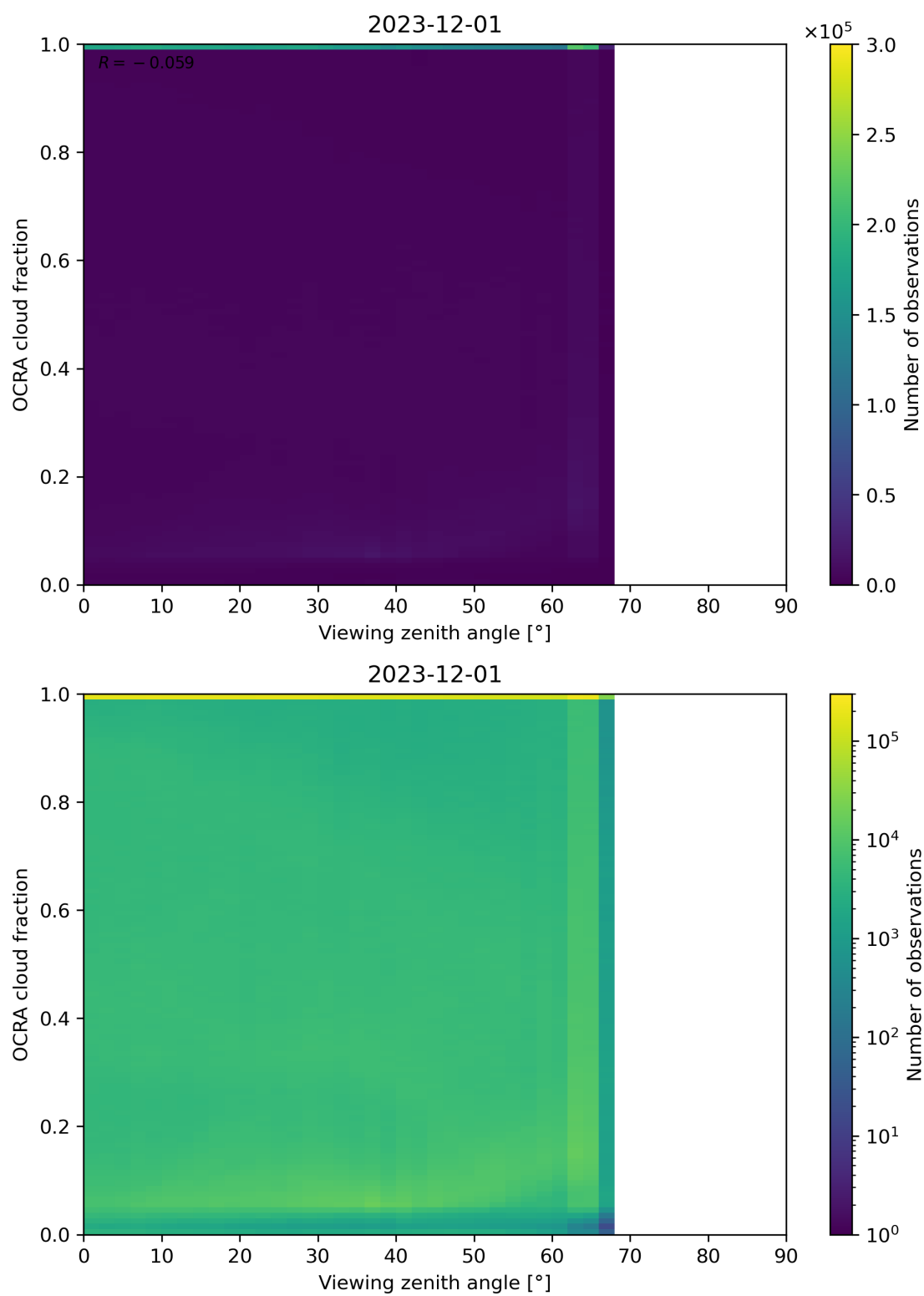
Figure 108: Scatter density plot of “Viewing zenith angle” against “OCRA cloud fraction” for 2023-11-30 to 2023-12-02.
