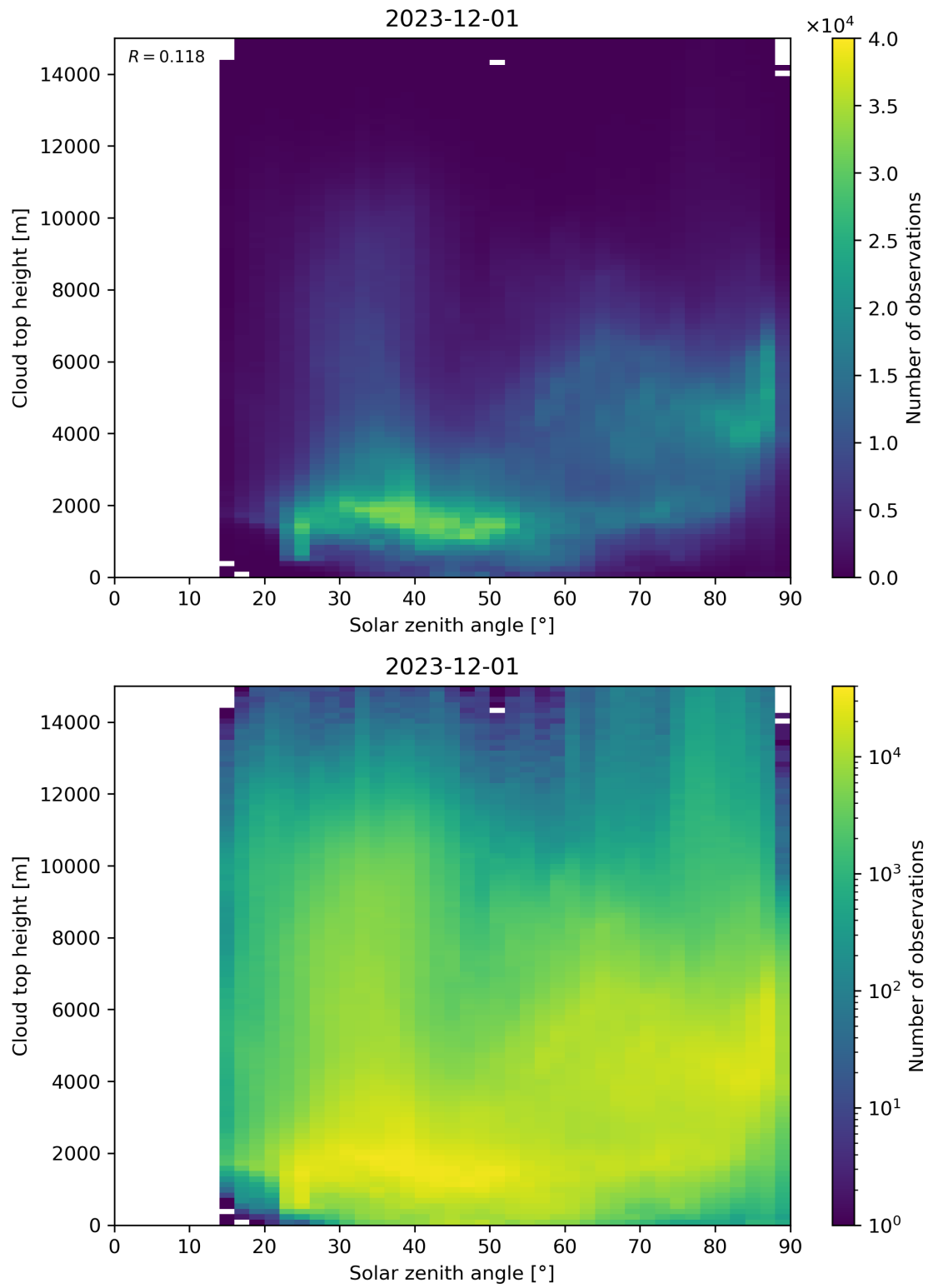
Figure 104: Scatter density plot of “Solar zenith angle” against “Cloud top height” for 2023-11-30 to 2023-12-02.
