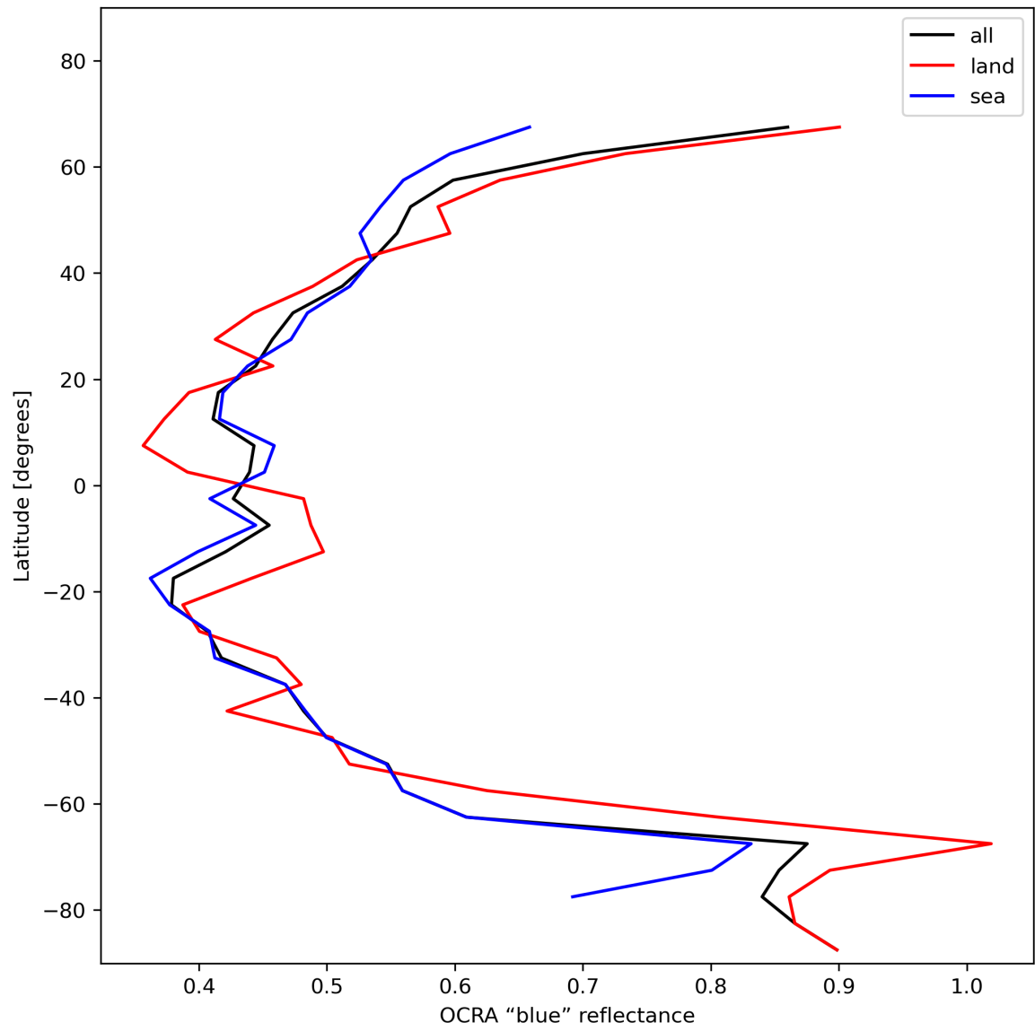
Figure 35: Zonal average of “OCRA “blue” reflectance” for 2023-11-30 to 2023-12-02.
