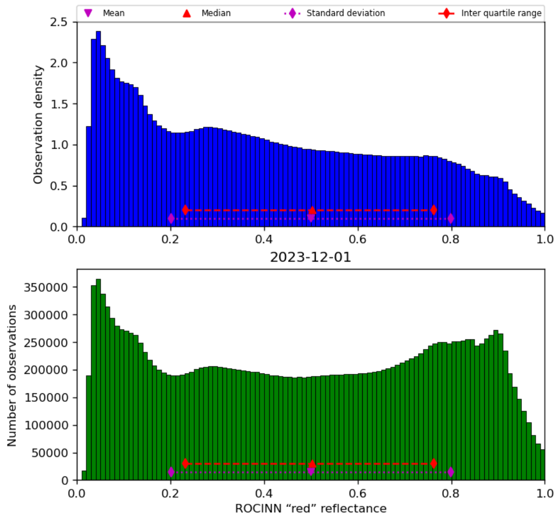
Figure 53: Histogram of “ROCINN “red” reflectance” for 2023-11-30 to 2023-12-02
