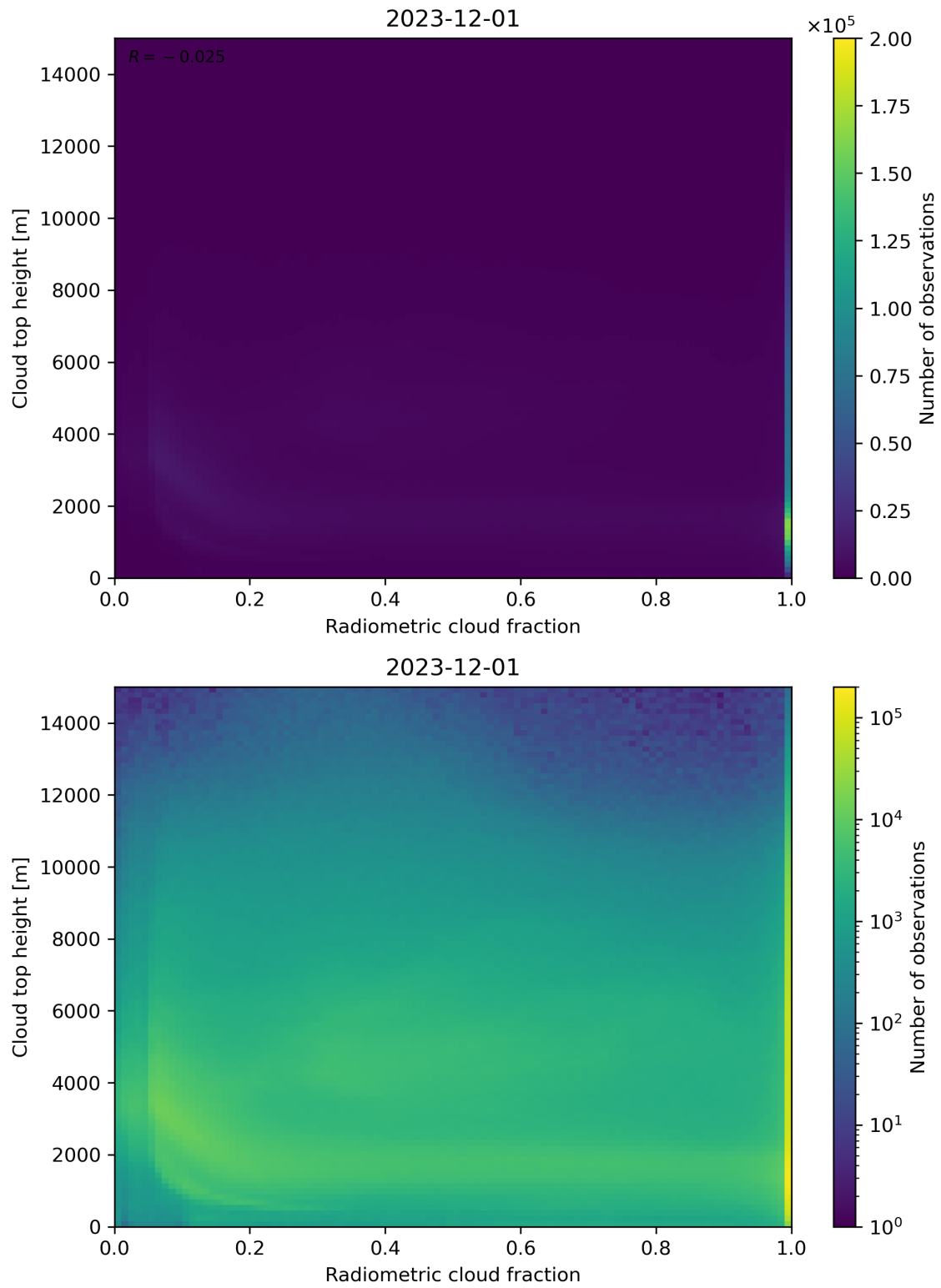
Figure 76: Scatter density plot of “Radiometric cloud fraction” against “Cloud top height” for 2023-11-30 to 2023-12-02.
