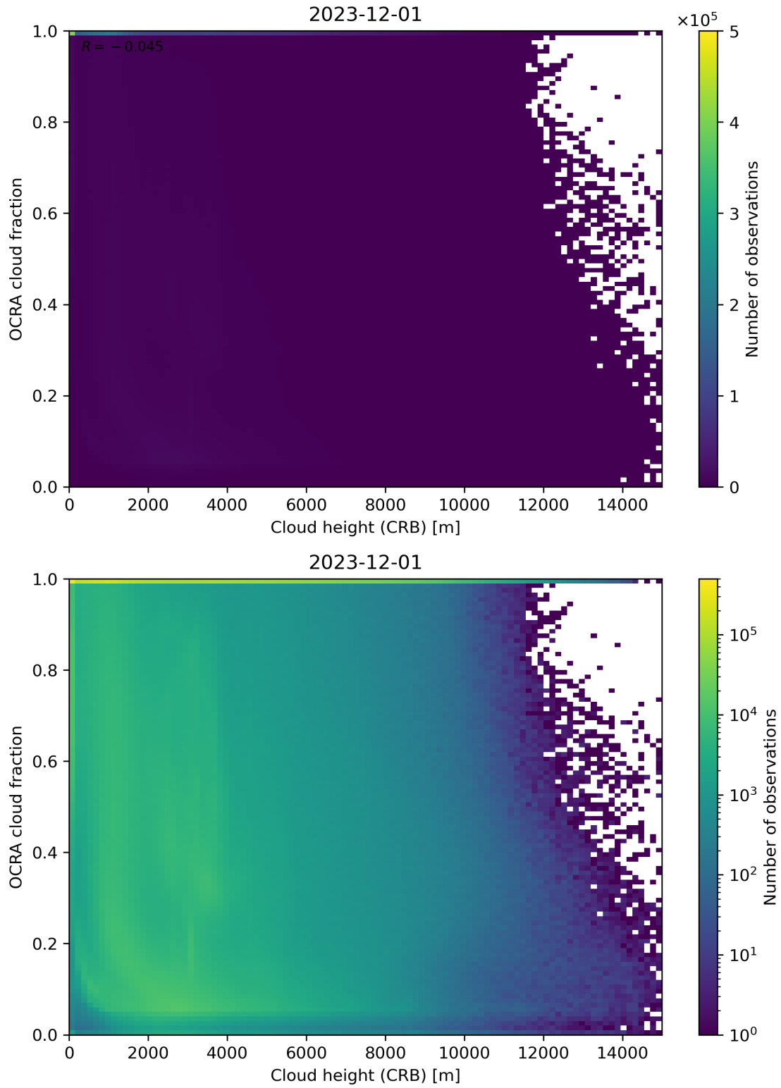
Figure 81: Scatter density plot of “Cloud height (CRB)” against “OCRA cloud fraction” for 2023-11-30 to 2023-12-02.
