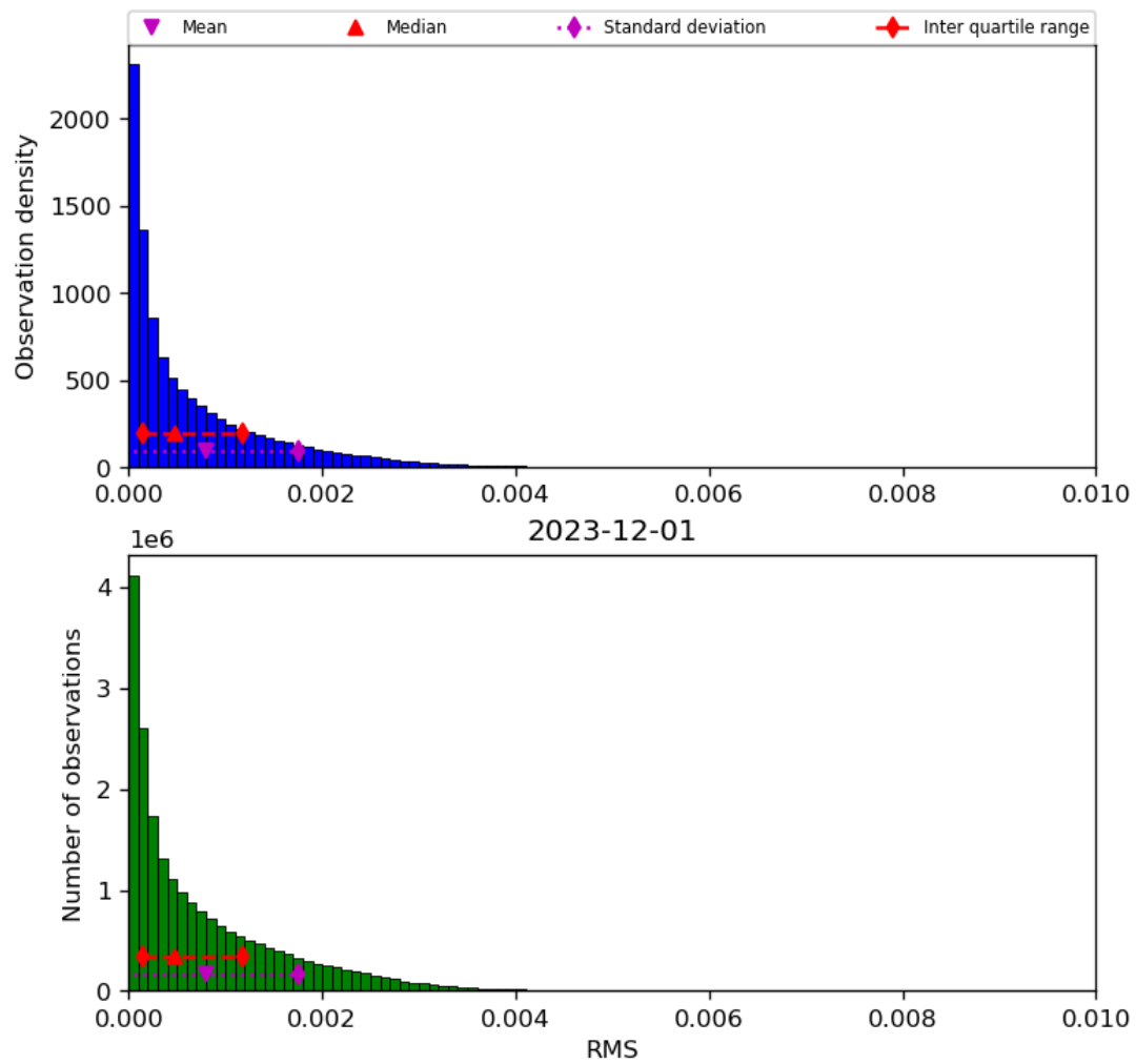
Figure 47: Histogram of “RMS” for 2023-11-30 to 2023-12-02
