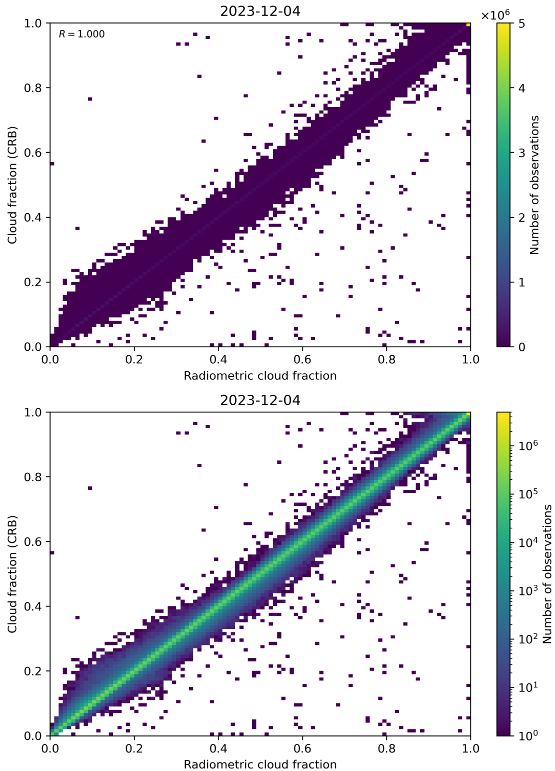
Figure 73: Scatter density plot of “Radiometric cloud fraction” against “Cloud fraction (CRB)” for 2023-12-04 to 2023-12-05.
