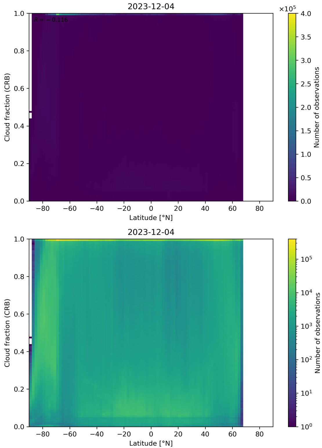
Figure 94: Scatter density plot of “Latitude” against “Cloud fraction (CRB)” for 2023-12-04 to 2023-12-05.
