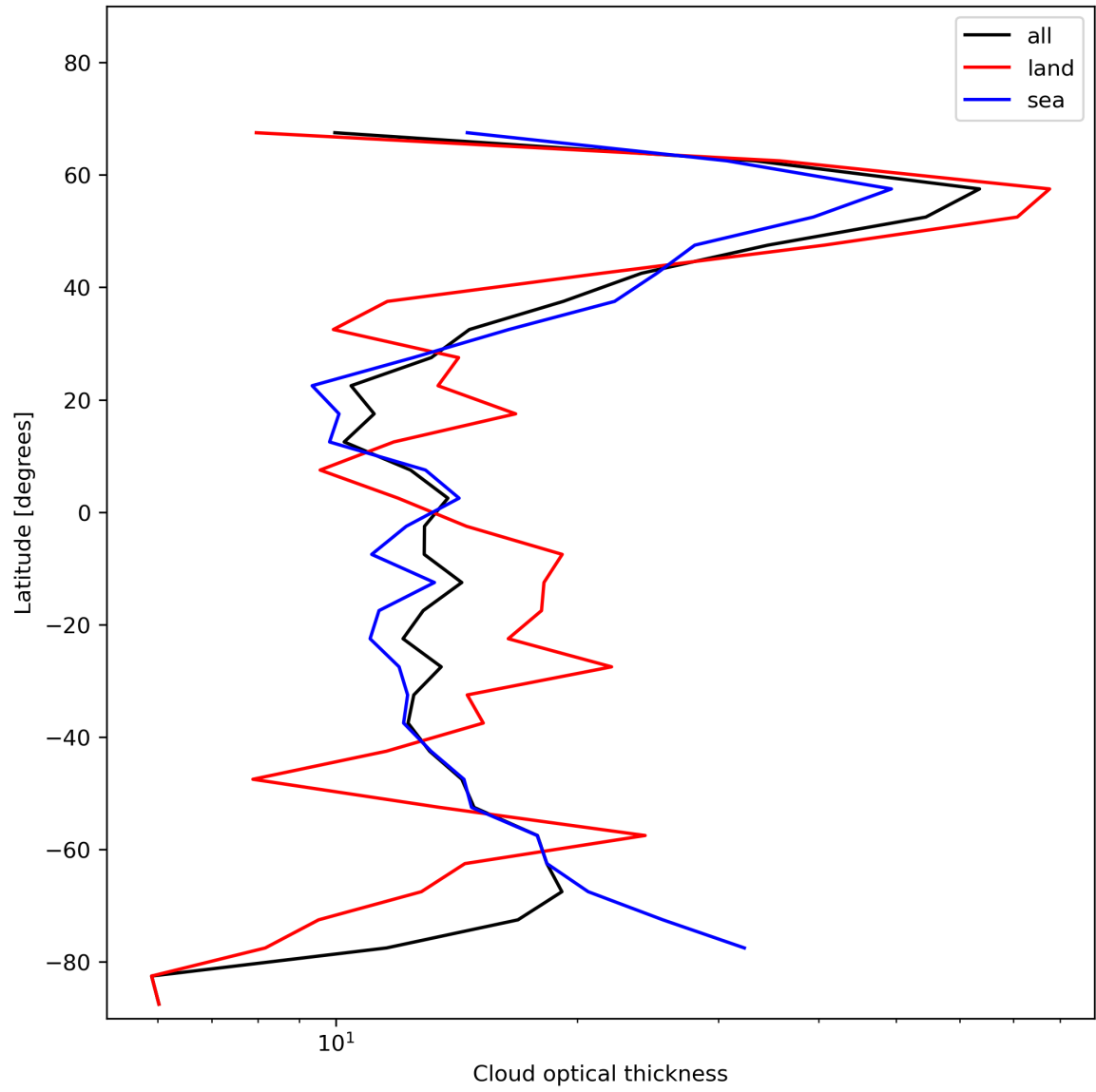
Figure 25: Zonal average of “Cloud optical thickness” for 2023-12-04 to 2023-12-05.
