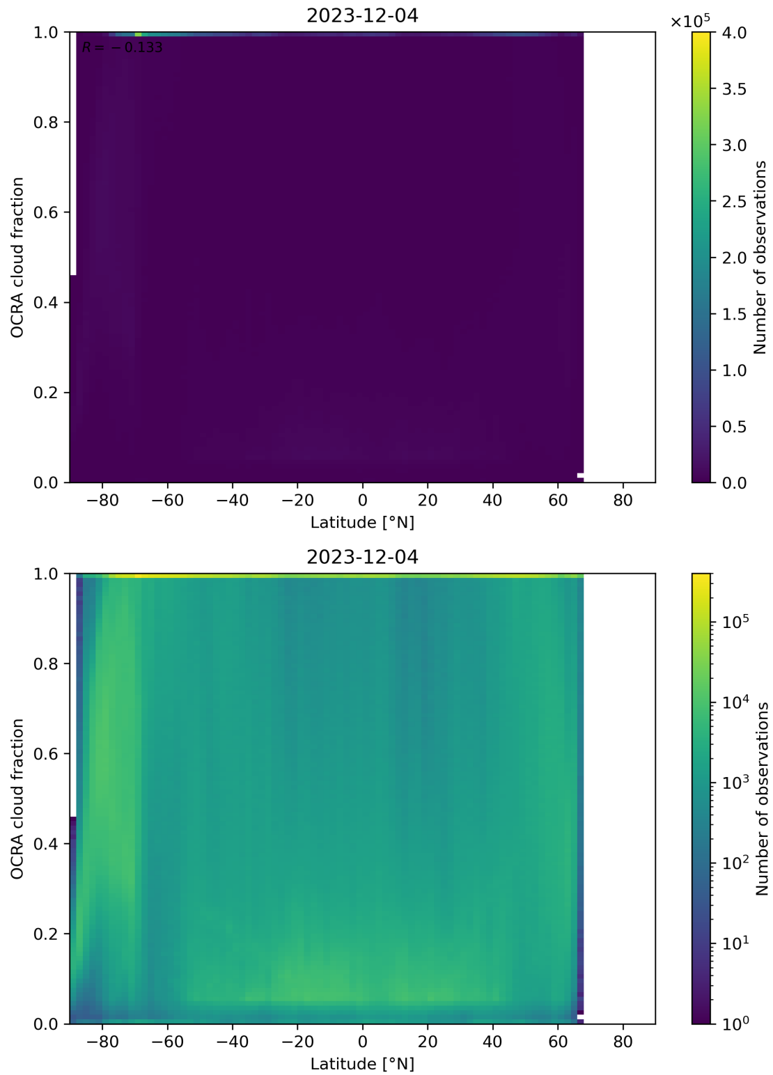
Figure 93: Scatter density plot of “Latitude” against “OCRA cloud fraction” for 2023-12-04 to 2023-12-05.
