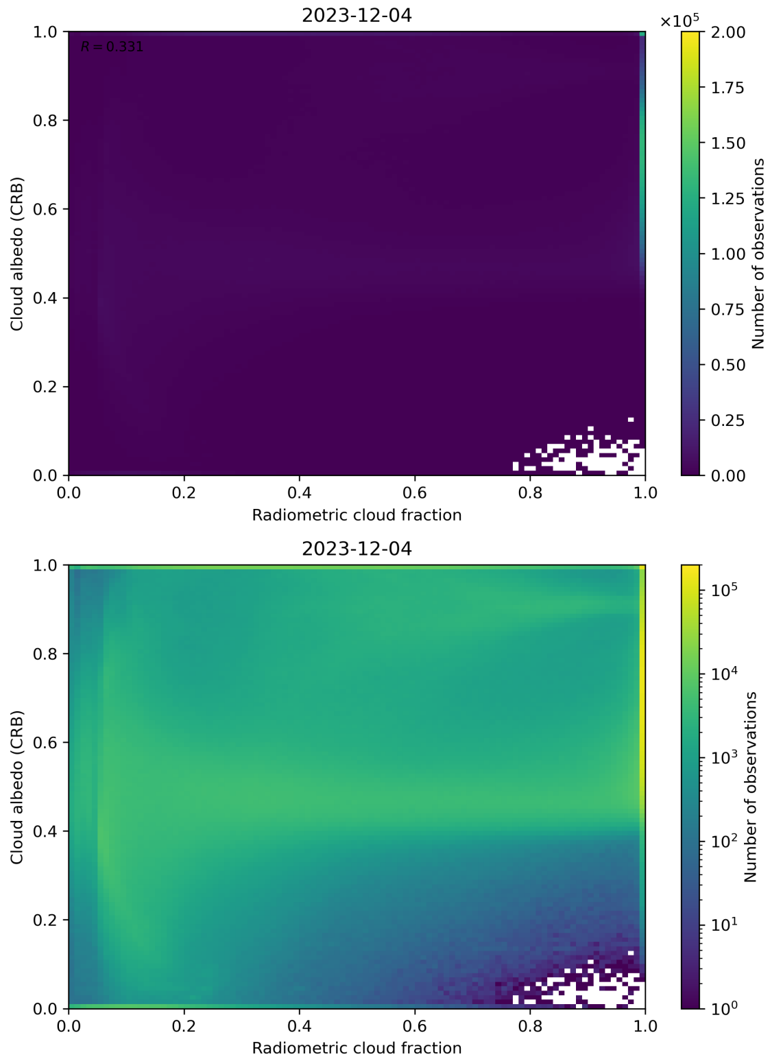
Figure 71: Scatter density plot of “Radiometric cloud fraction” against “Cloud albedo (CRB)” for 2023-12-04 to 2023-12-05.
