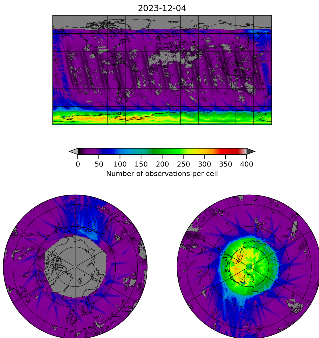
Figure 21: Map of the number of observations for 2023-12-04 to 2023-12-05
