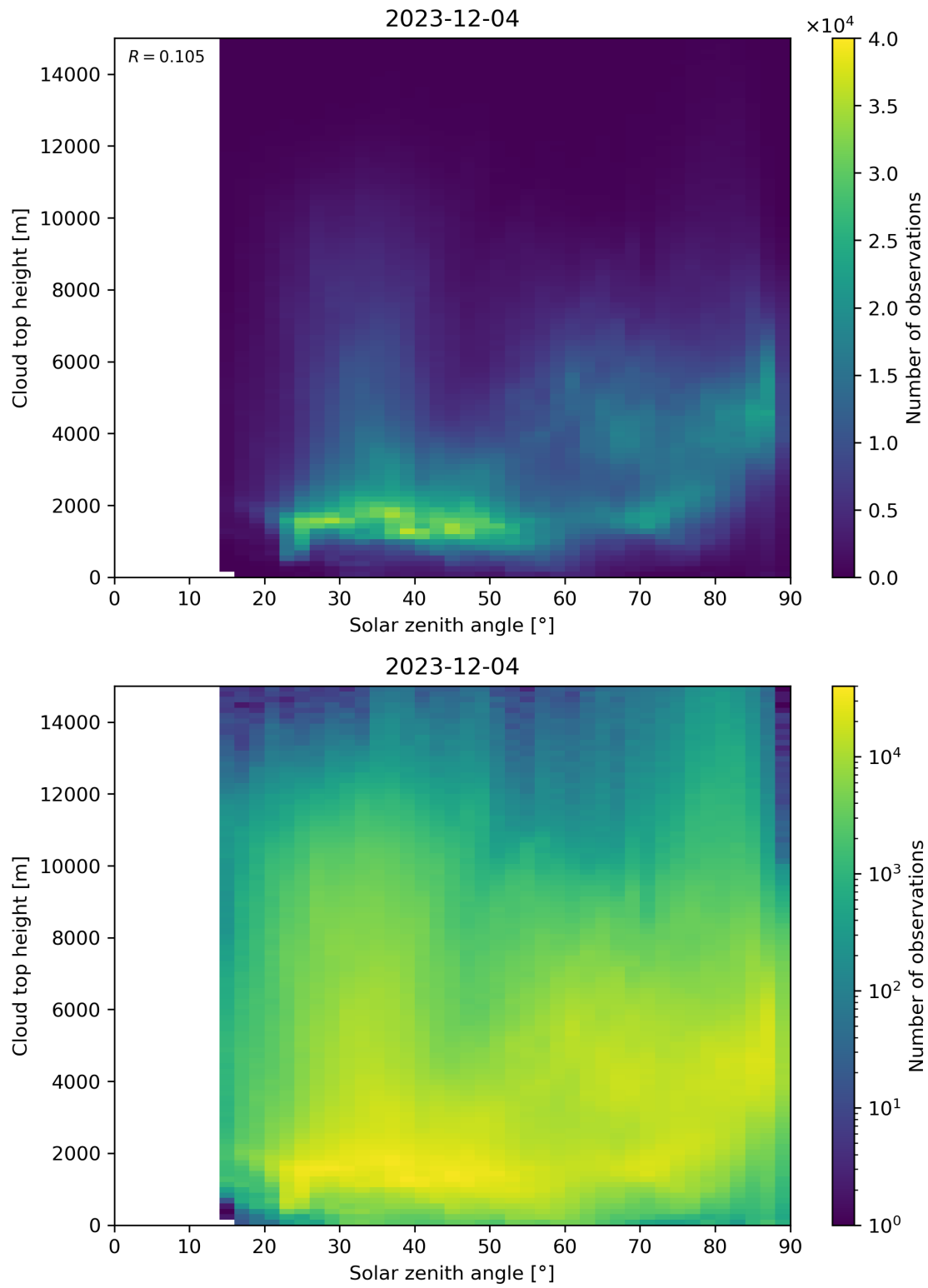
Figure 104: Scatter density plot of “Solar zenith angle” against “Cloud top height” for 2023-12-04 to 2023-12-05.
