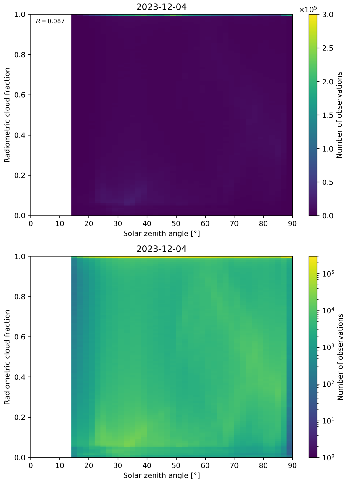
Figure 99: Scatter density plot of “Solar zenith angle” against “Radiometric cloud fraction” for 2023-12-04 to 2023-12-05.
