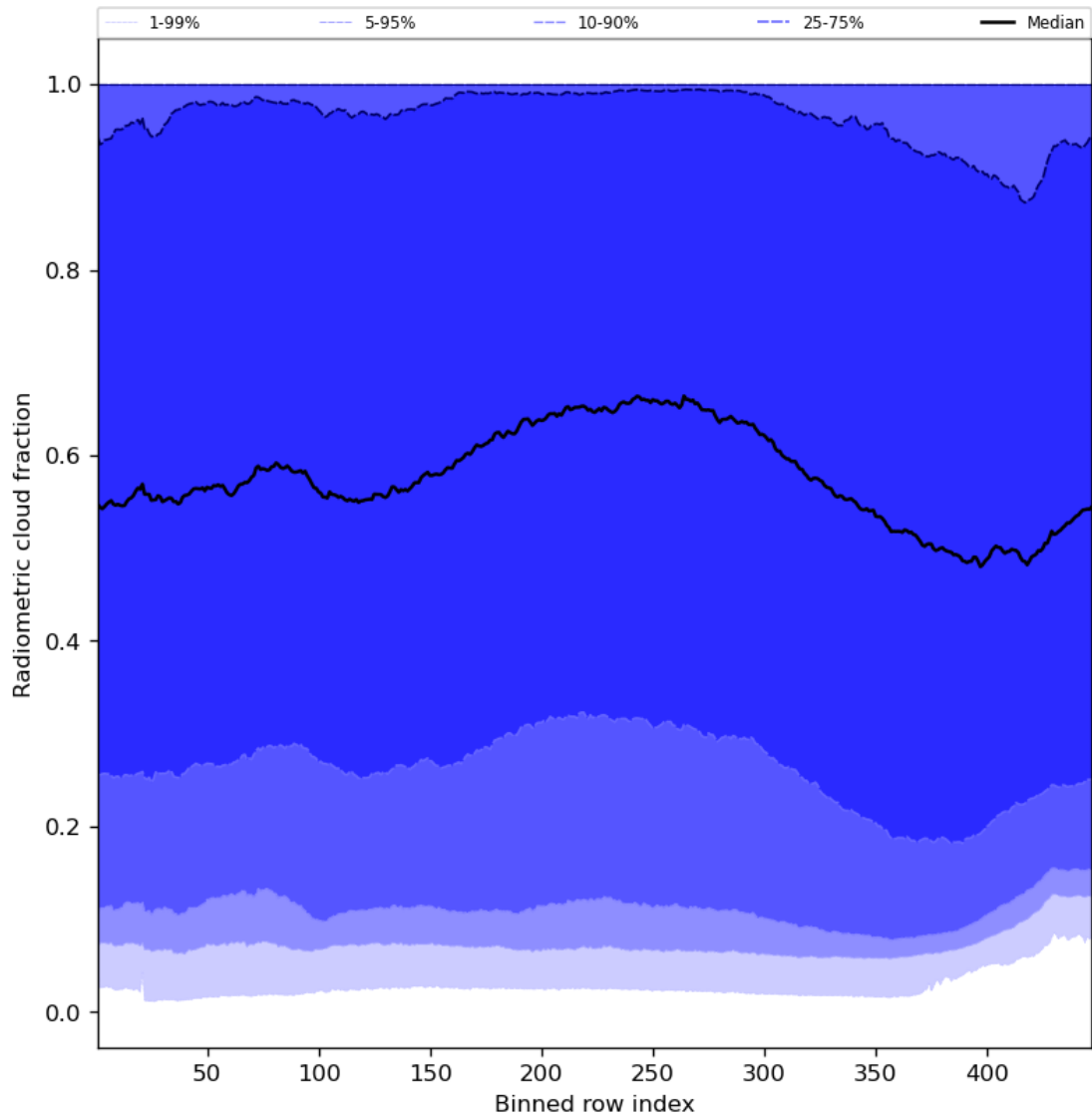
Figure 55: Along track statistics of “Radiometric cloud fraction” for 2023-12-04 to 2023-12-05
