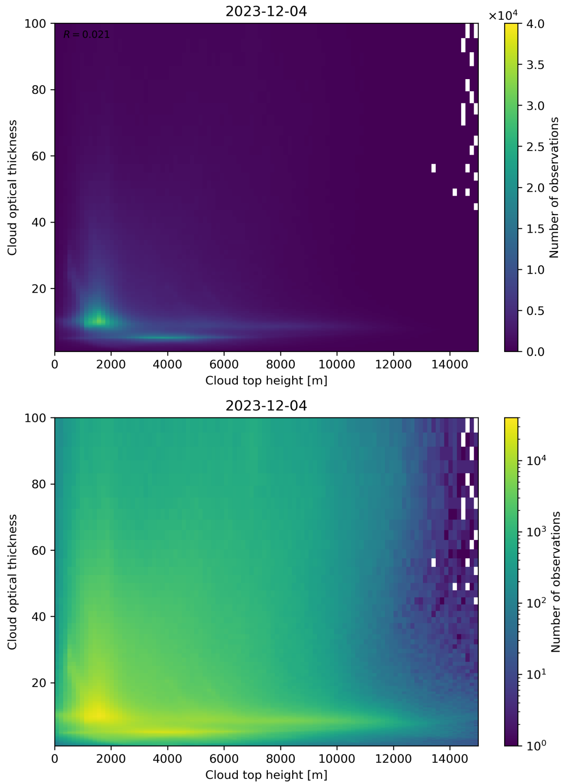
Figure 90: Scatter density plot of “Cloud top height” against “Cloud optical thickness” for 2023-12-04 to 2023-12-05.
