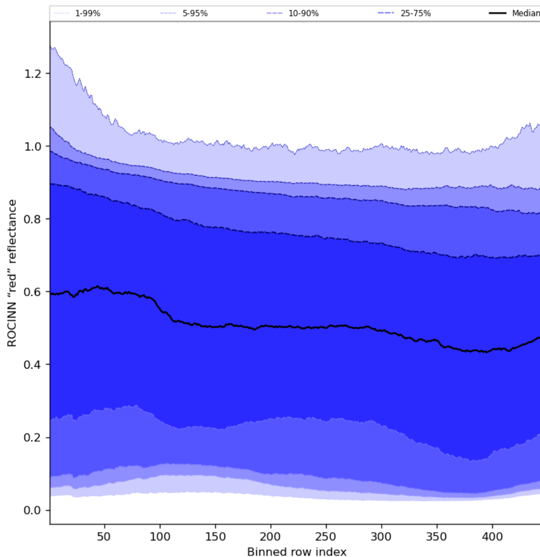
Figure 69: Along track statistics of “ROCINN “red” reflectance” for 2023-12-04 to 2023-12-05
