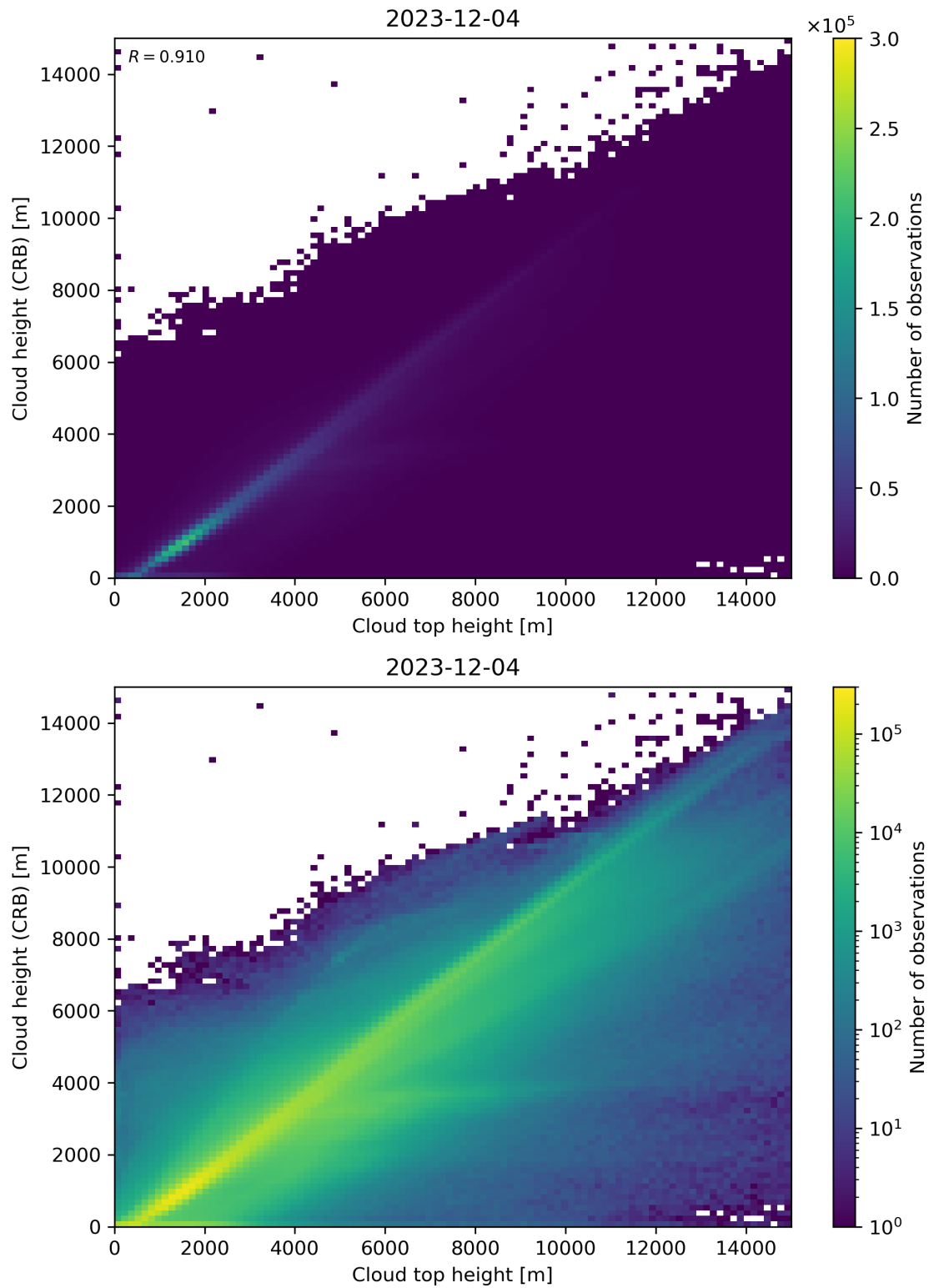
Figure 89: Scatter density plot of “Cloud top height” against “Cloud height (CRB)” for 2023-12-04 to 2023-12-05.
