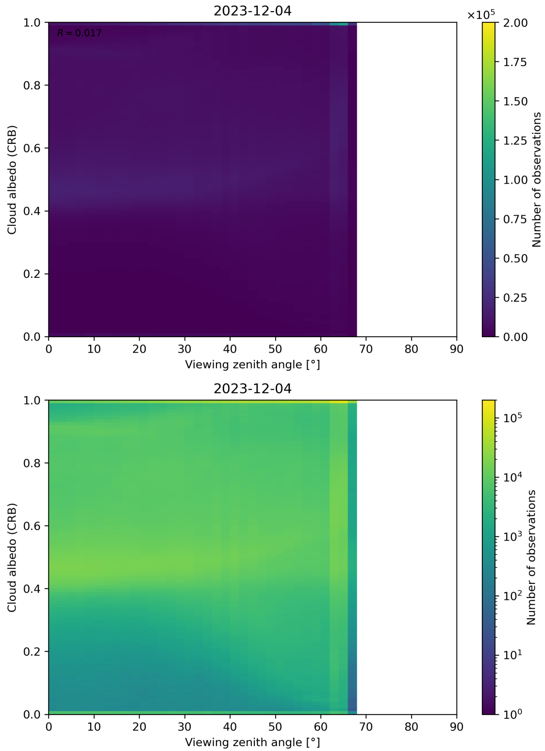
Figure 106: Scatter density plot of “Viewing zenith angle” against “Cloud albedo (CRB)” for 2023-12-04 to 2023-12-05.
