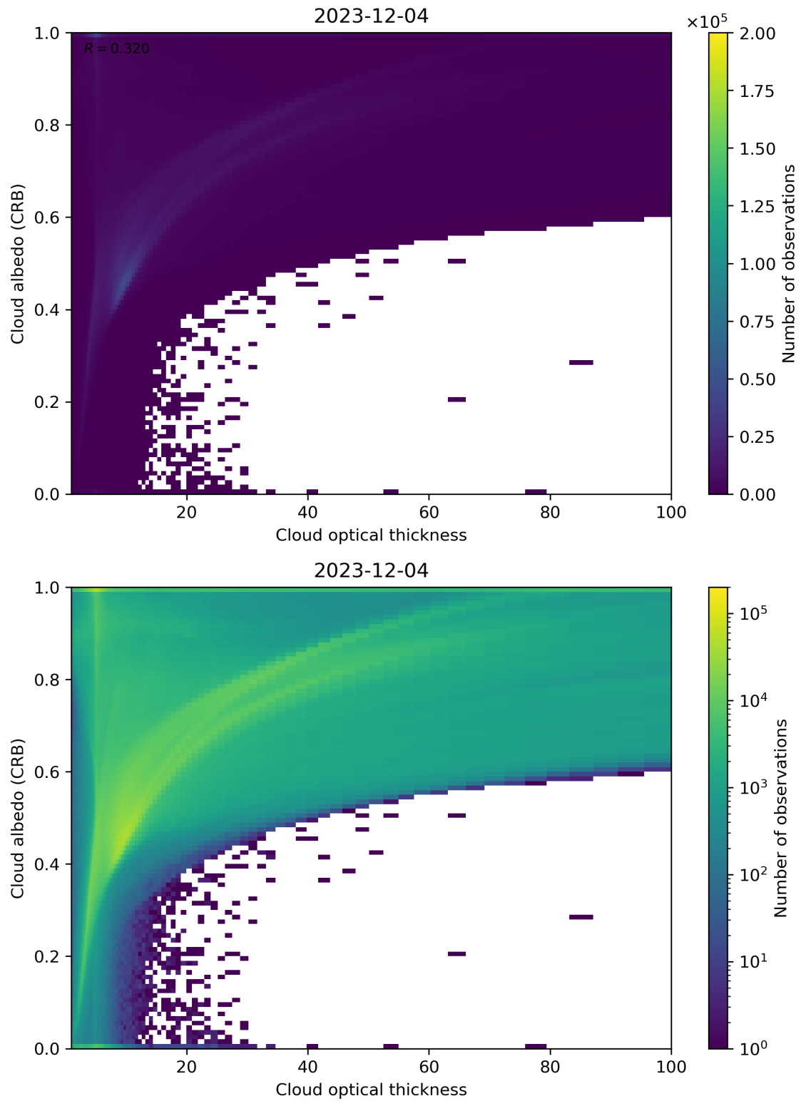
Figure 82: Scatter density plot of “Cloud optical thickness” against “Cloud albedo (CRB)” for 2023-12-04 to 2023-12-05.
