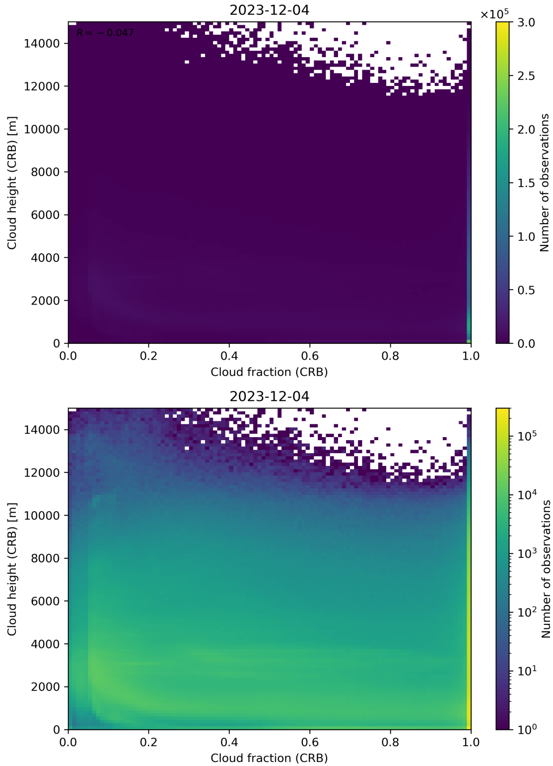
Figure 79: Scatter density plot of “Cloud fraction (CRB)” against “Cloud height (CRB)” for 2023-12-04 to 2023-12-05.
