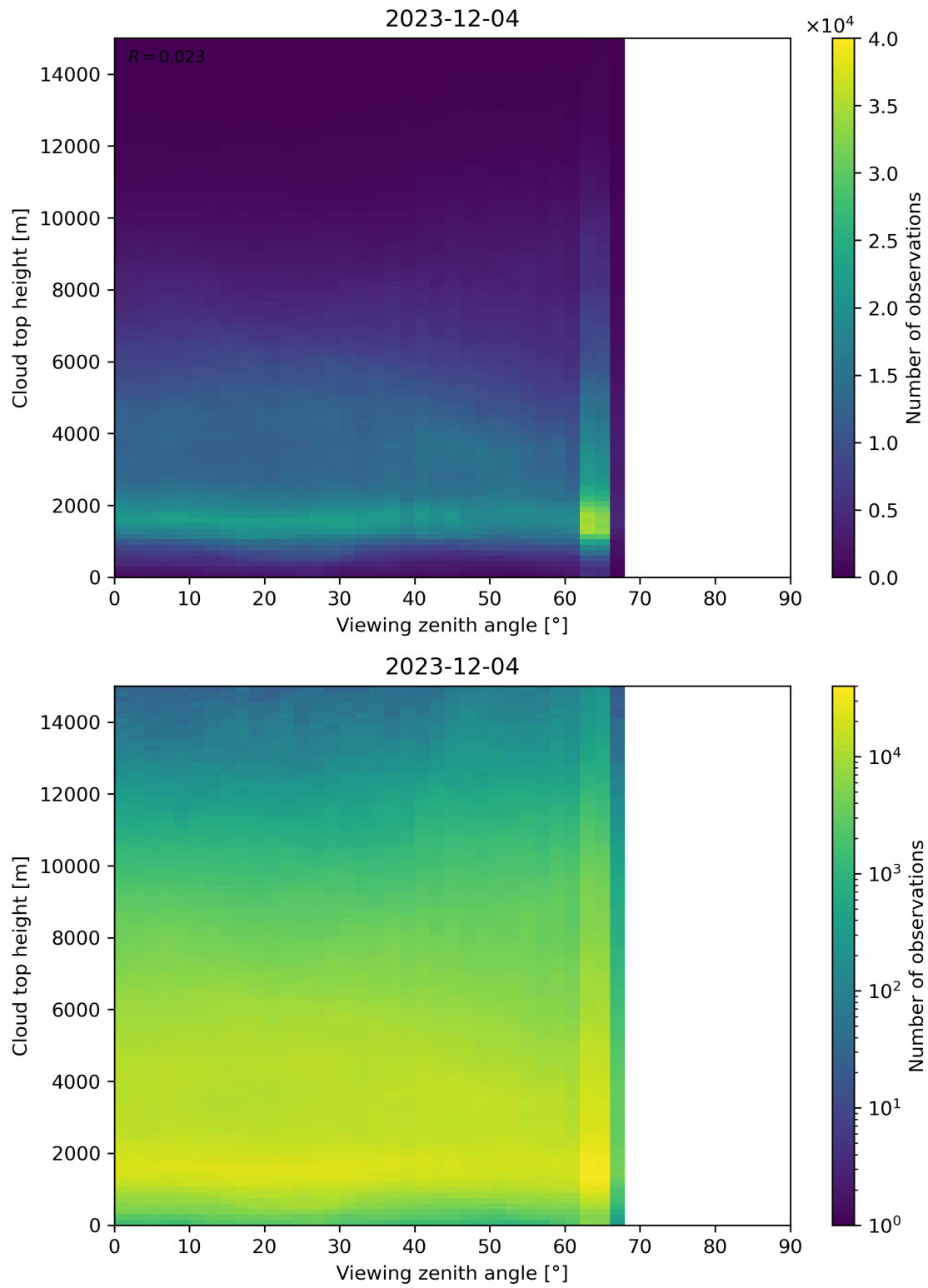
Figure 112: Scatter density plot of “Viewing zenith angle” against “Cloud top height” for 2023-12-04 to 2023-12-05.
