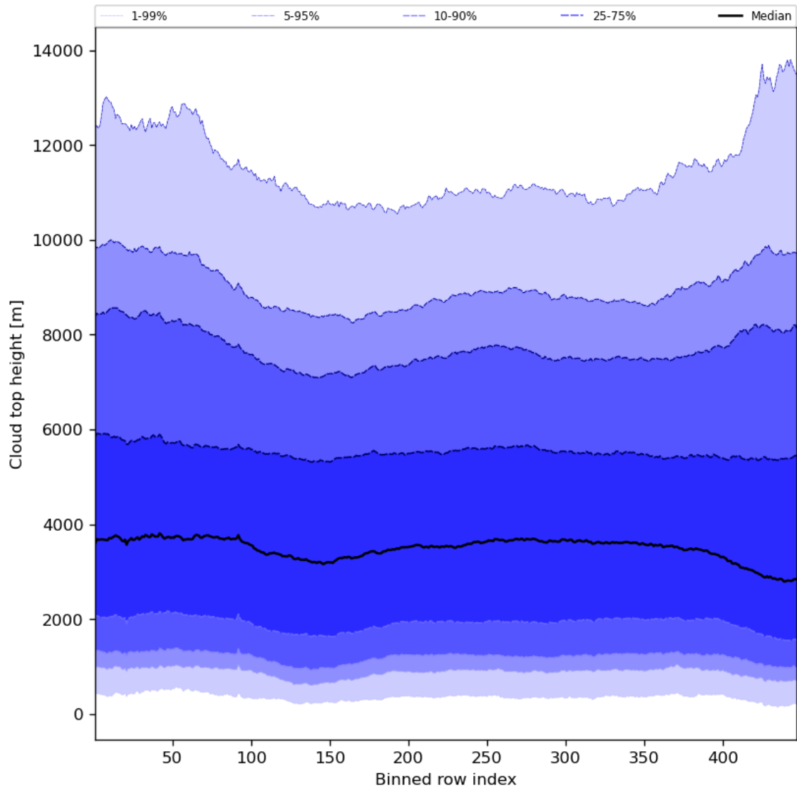
Figure 56: Along track statistics of “Cloud top height” for 2023-12-04 to 2023-12-05
