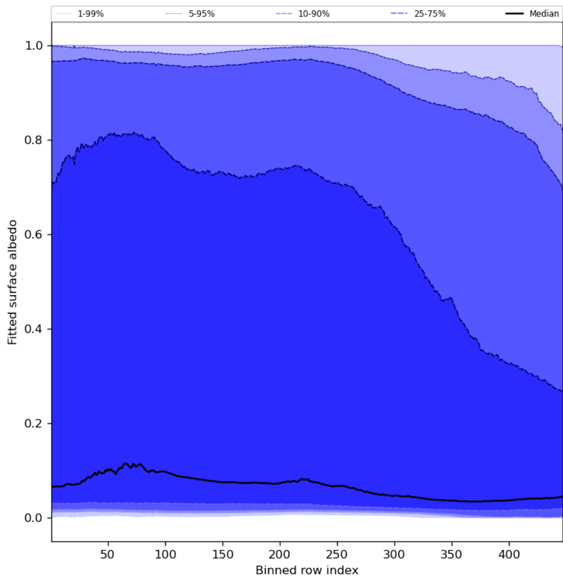
Figure 61: Along track statistics of “Fitted surface albedo” for 2023-12-04 to 2023-12-05
