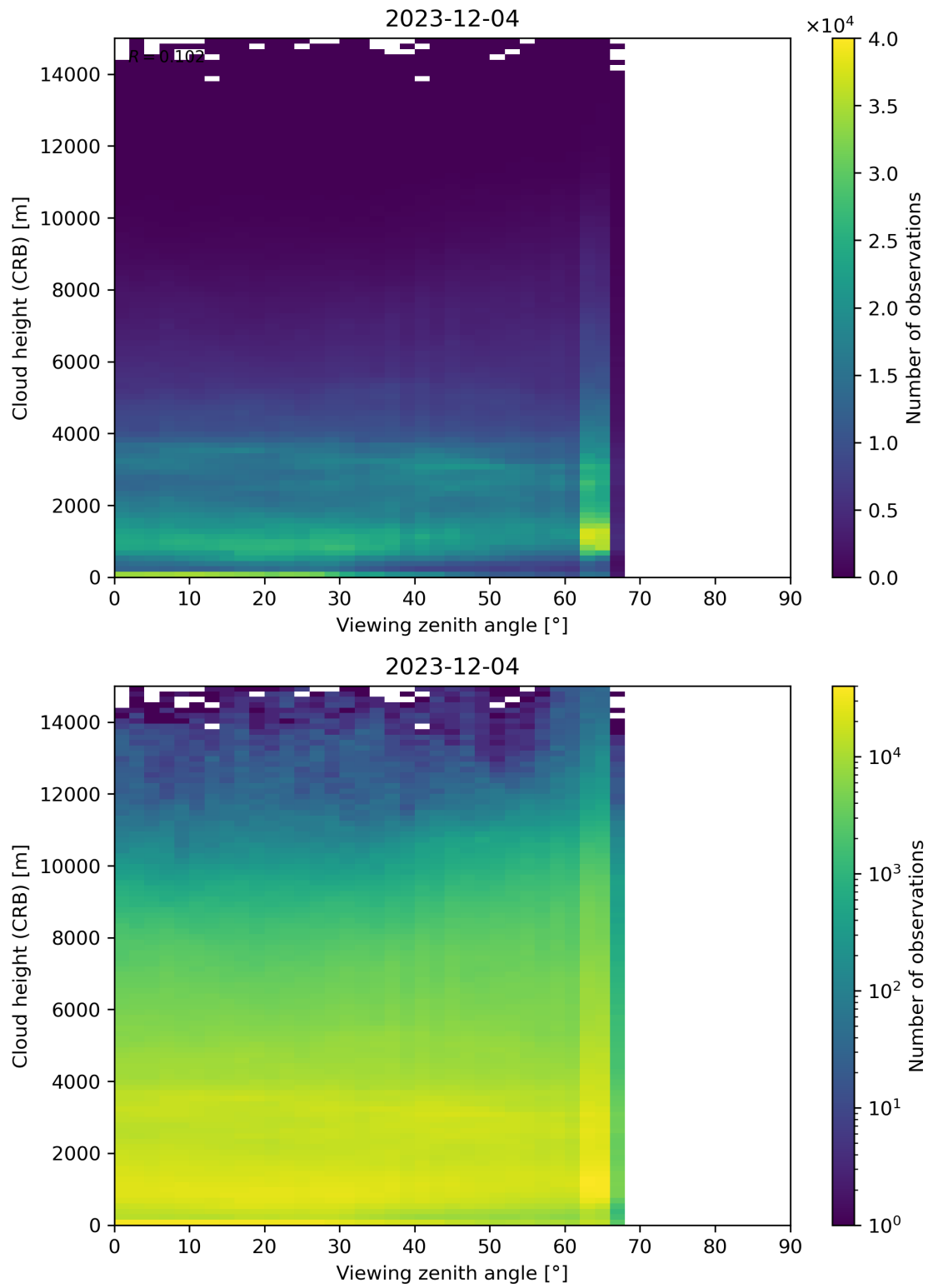
Figure 110: Scatter density plot of “Viewing zenith angle” against “Cloud height (CRB)” for 2023-12-04 to 2023-12-05.
