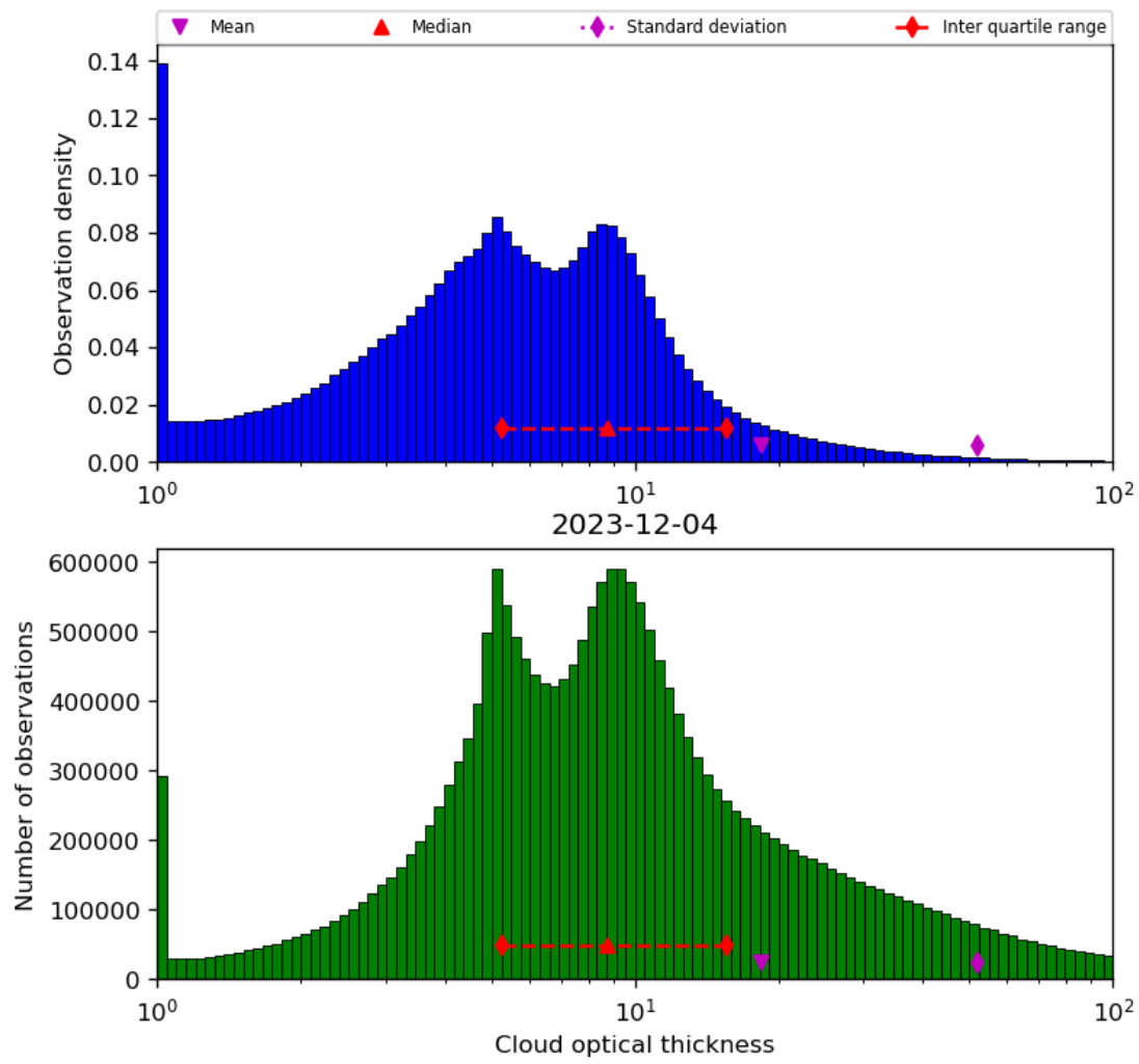
Figure 41: Histogram of “Cloud optical thickness” for 2023-12-04 to 2023-12-05
