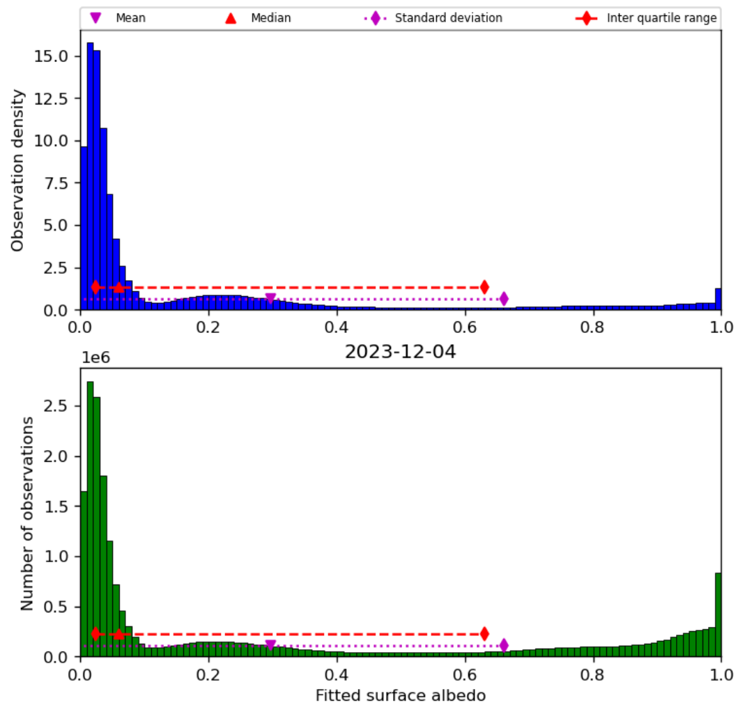
Figure 45: Histogram of “Fitted surface albedo” for 2023-12-04 to 2023-12-05
