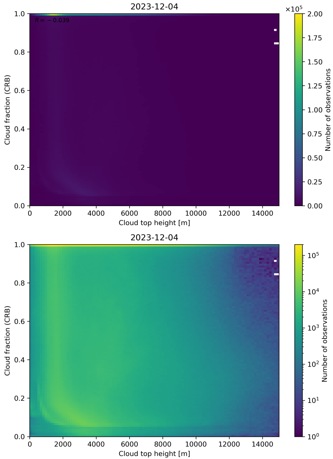
Figure 88: Scatter density plot of “Cloud top height” against “Cloud fraction (CRB)” for 2023-12-04 to 2023-12-05.
