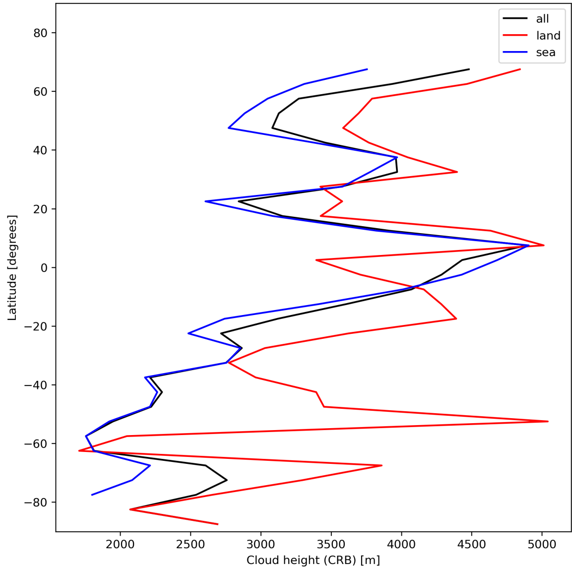
Figure 27: Zonal average of “Cloud height (CRB)” for 2023-12-04 to 2023-12-05.
