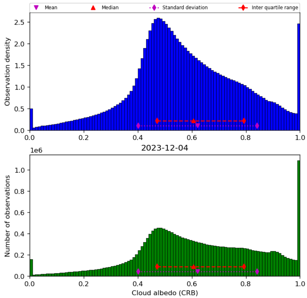
Figure 44: Histogram of “Cloud albedo (CRB)” for 2023-12-04 to 2023-12-05
