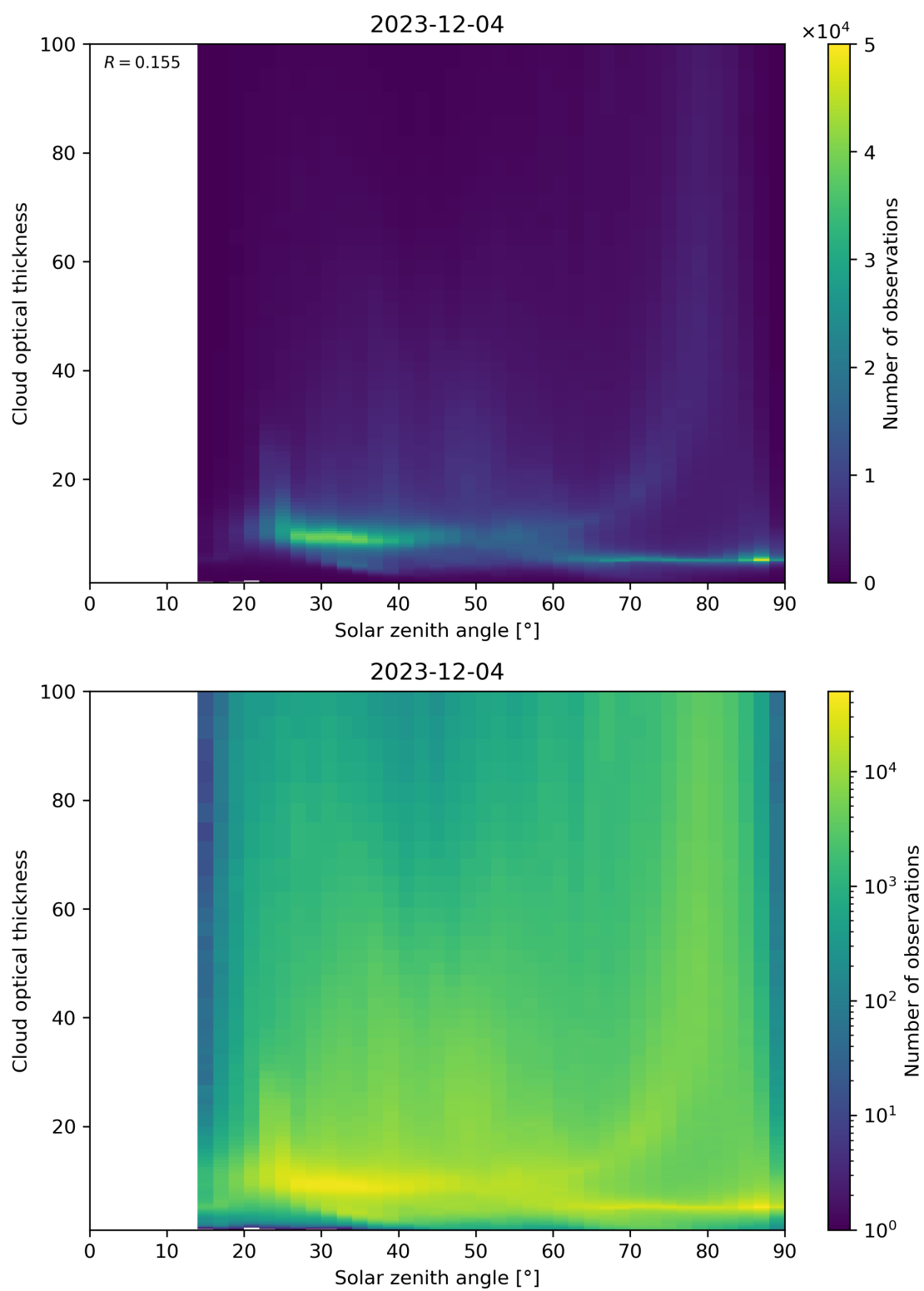
Figure 103: Scatter density plot of “Solar zenith angle” against “Cloud optical thickness” for 2023-12-04 to 2023-12-05.
