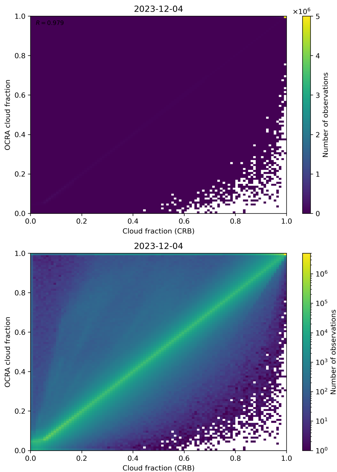
Figure 78: Scatter density plot of “Cloud fraction (CRB)” against “OCRA cloud fraction” for 2023-12-04 to 2023-12-05.
