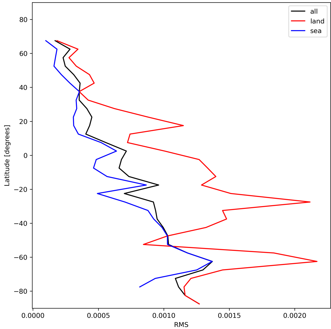
Figure 31: Zonal average of “RMS” for 2023-12-04 to 2023-12-05.
