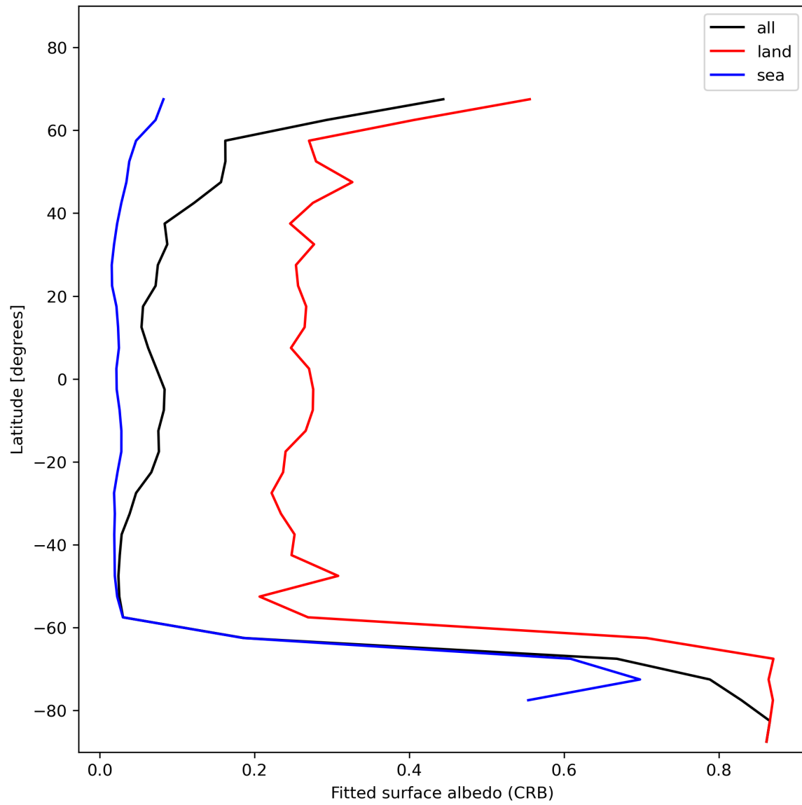
Figure 30: Zonal average of “Fitted surface albedo (CRB)” for 2023-12-04 to 2023-12-05.
