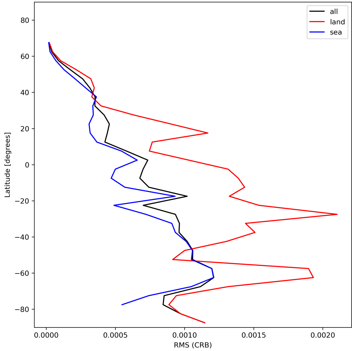
Figure 32: Zonal average of “RMS (CRB)” for 2023-12-04 to 2023-12-05.
