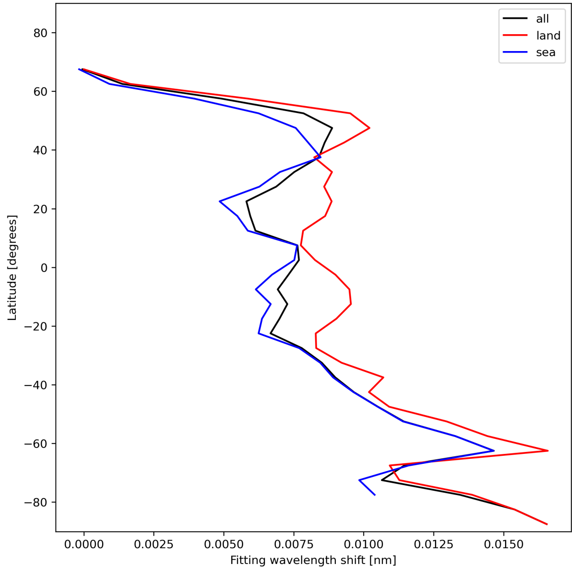
Figure 33: Zonal average of “Fitting wavelength shift” for 2023-12-04 to 2023-12-05.
