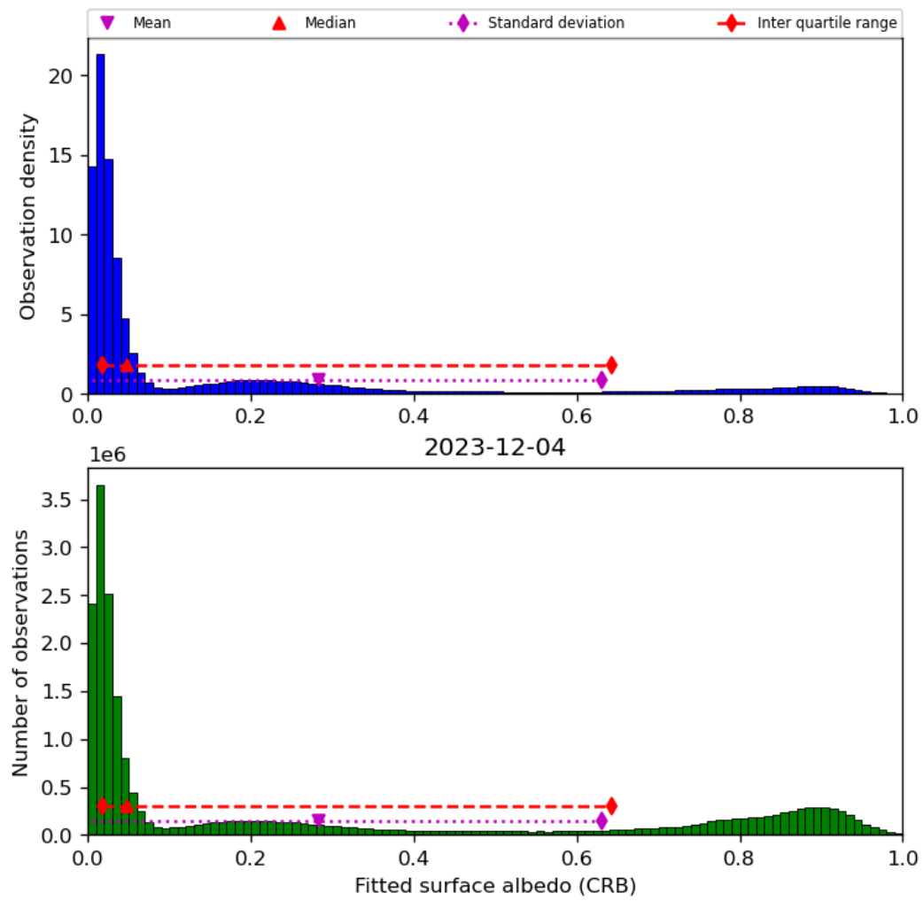
Figure 46: Histogram of “Fitted surface albedo (CRB)” for 2023-12-04 to 2023-12-05
