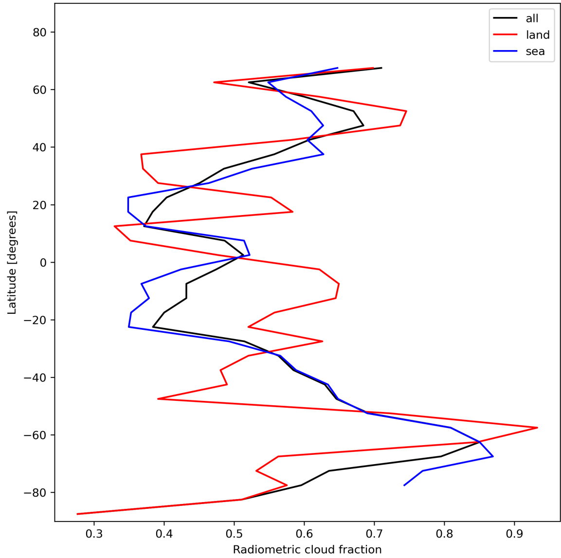
Figure 23: Zonal average of “Radiometric cloud fraction” for 2023-12-04 to 2023-12-05.
