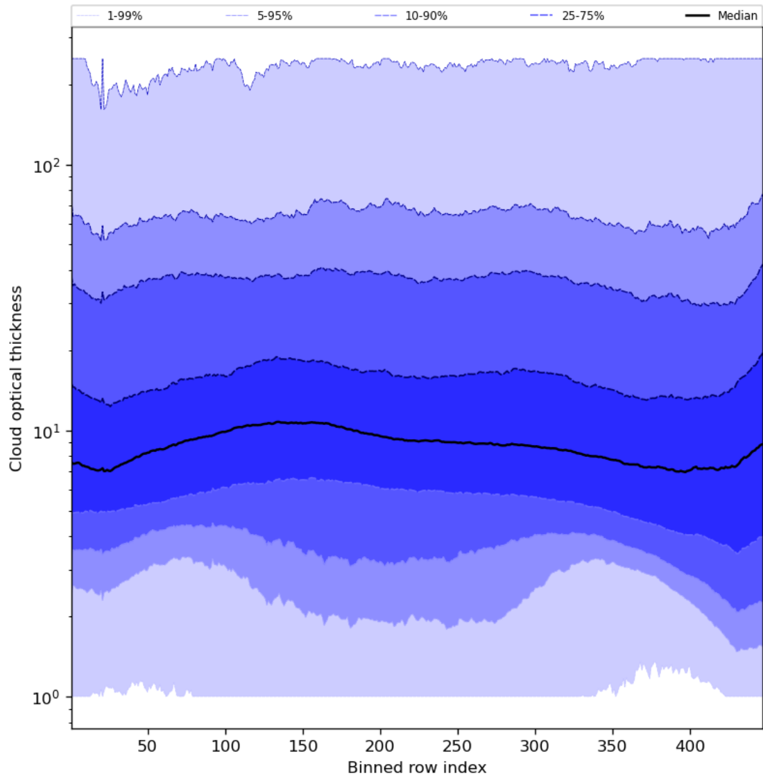
Figure 57: Along track statistics of “Cloud optical thickness” for 2023-12-04 to 2023-12-05
