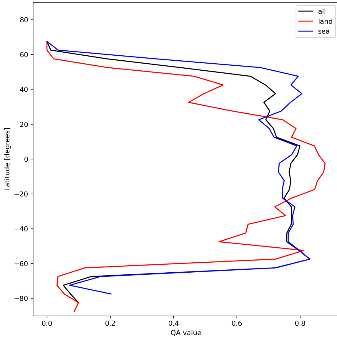
Figure 22: Zonal average of “QA value” for 2023-12-04 to 2023-12-05.
