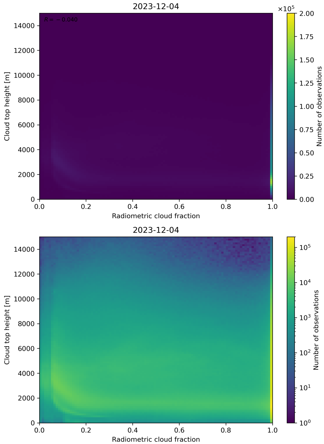
Figure 76: Scatter density plot of “Radiometric cloud fraction” against “Cloud top height” for 2023-12-04 to 2023-12-05.
