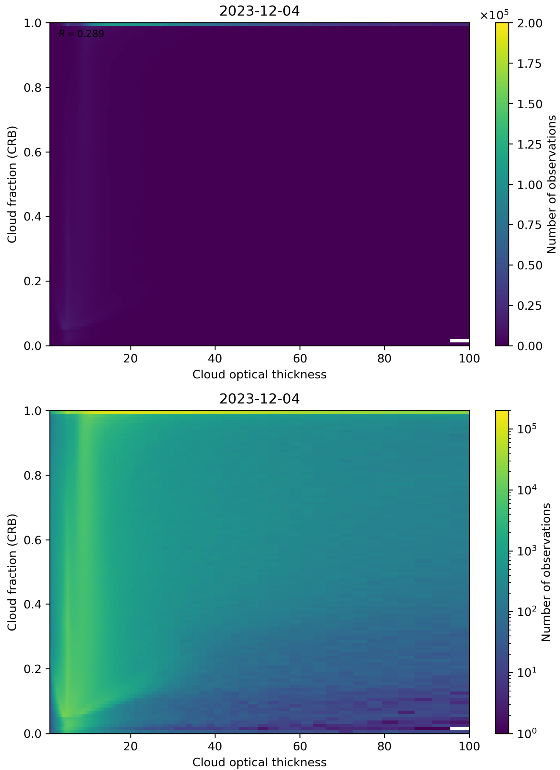
Figure 84: Scatter density plot of “Cloud optical thickness” against “Cloud fraction (CRB)” for 2023-12-04 to 2023-12-05.
