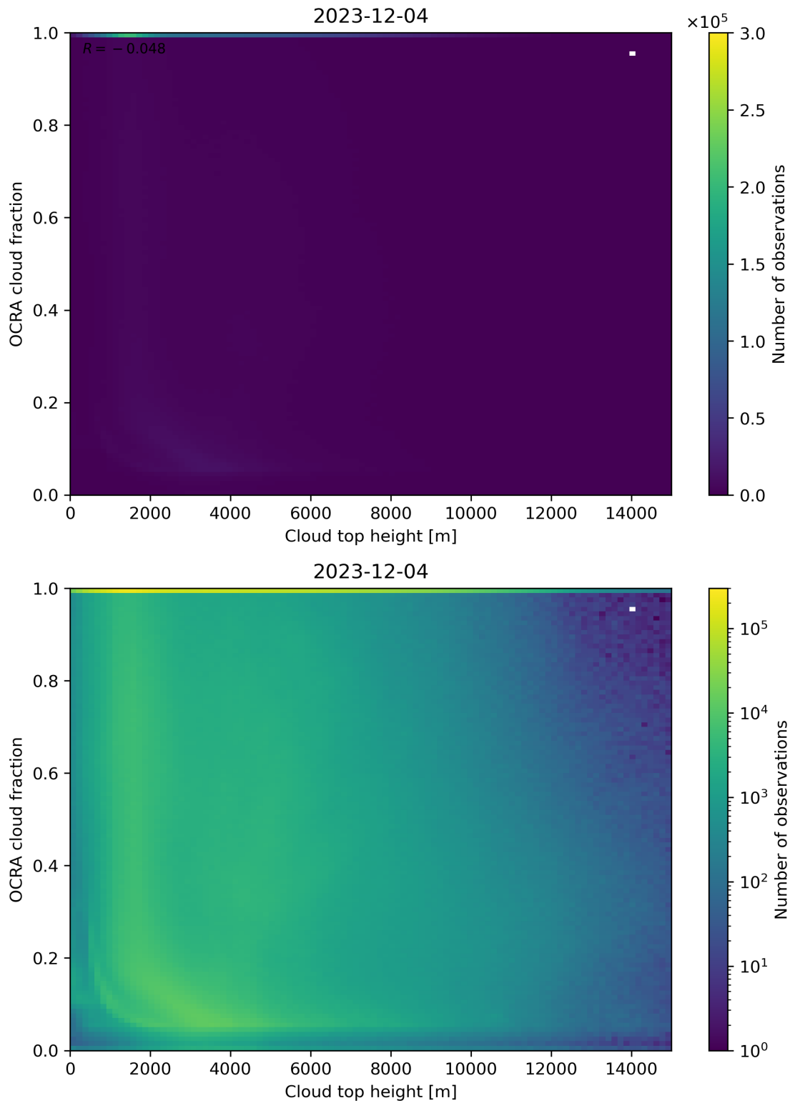
Figure 87: Scatter density plot of “Cloud top height” against “OCRA cloud fraction” for 2023-12-04 to 2023-12-05.
