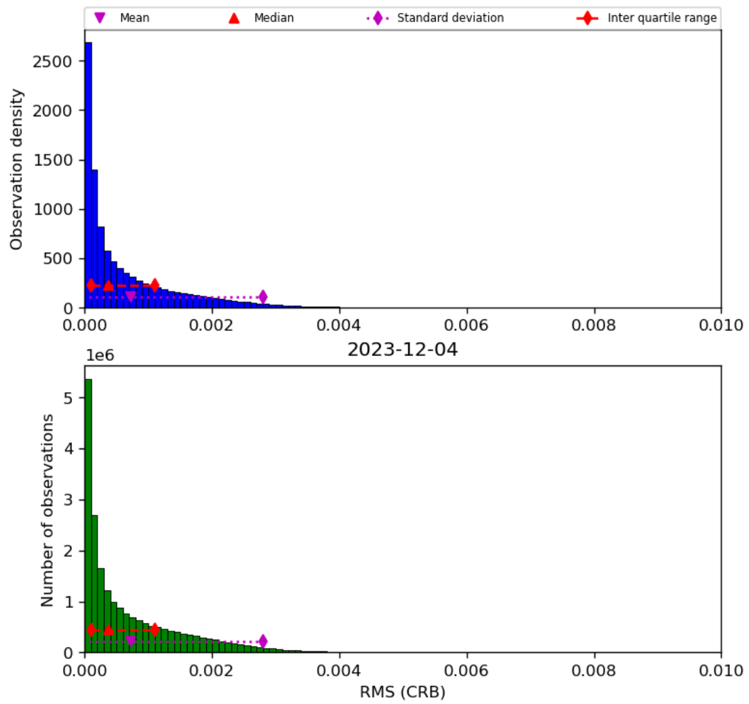
Figure 48: Histogram of “RMS (CRB)” for 2023-12-04 to 2023-12-05
