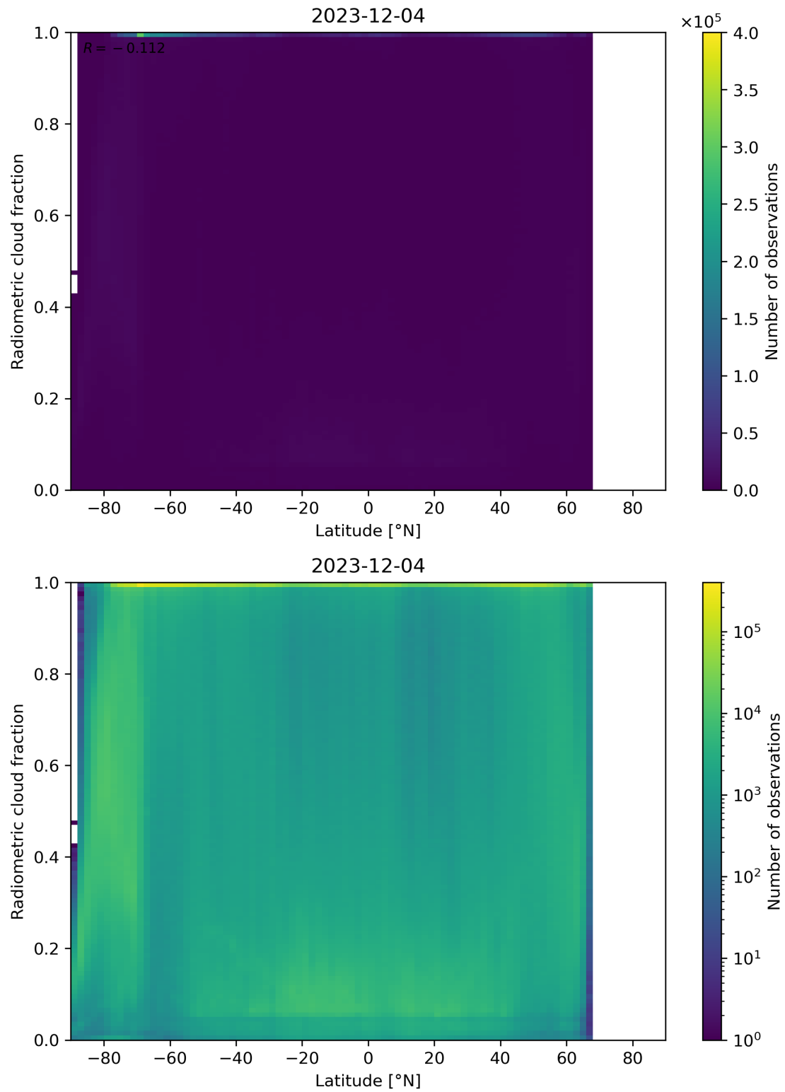
Figure 92: Scatter density plot of “Latitude” against “Radiometric cloud fraction” for 2023-12-04 to 2023-12-05.
