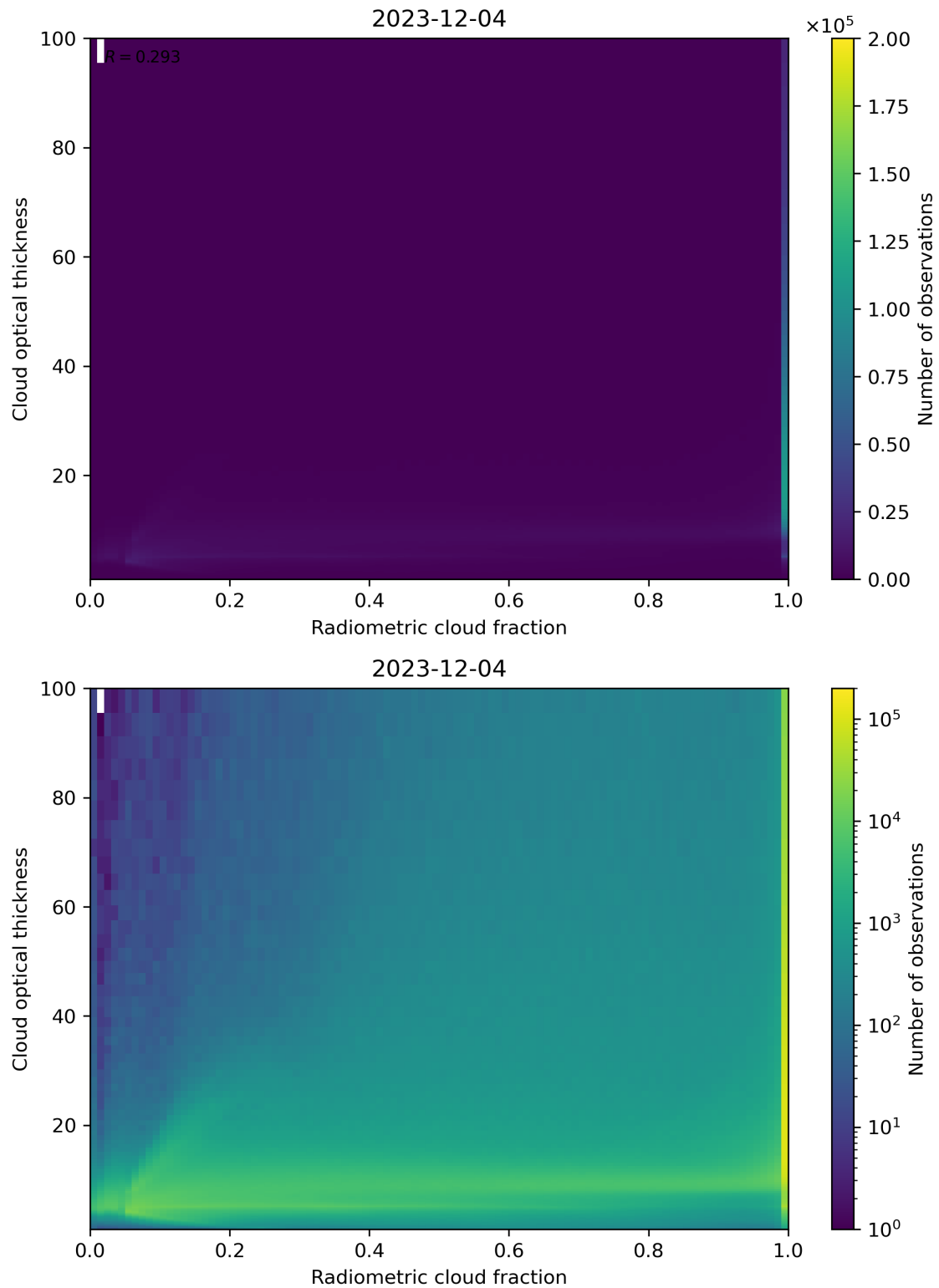
Figure 75: Scatter density plot of “Radiometric cloud fraction” against “Cloud optical thickness” for 2023-12-04 to 2023-12-05.
