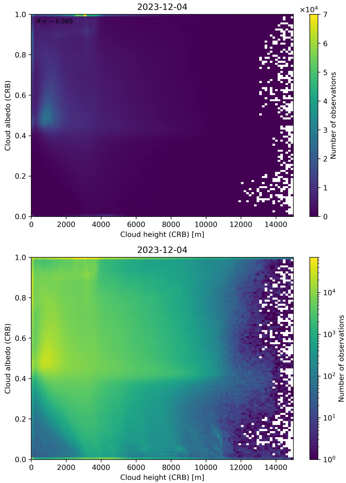
Figure 80: Scatter density plot of “Cloud height (CRB)” against “Cloud albedo (CRB)” for 2023-12-04 to 2023-12-05.
