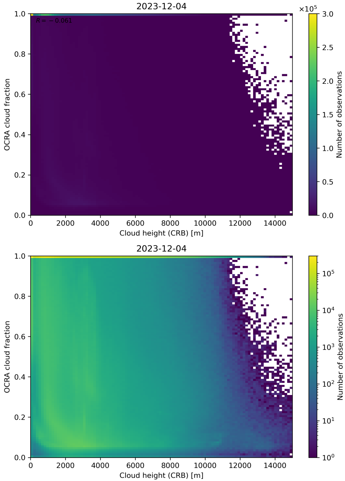
Figure 81: Scatter density plot of “Cloud height (CRB)” against “OCRA cloud fraction” for 2023-12-04 to 2023-12-05.
