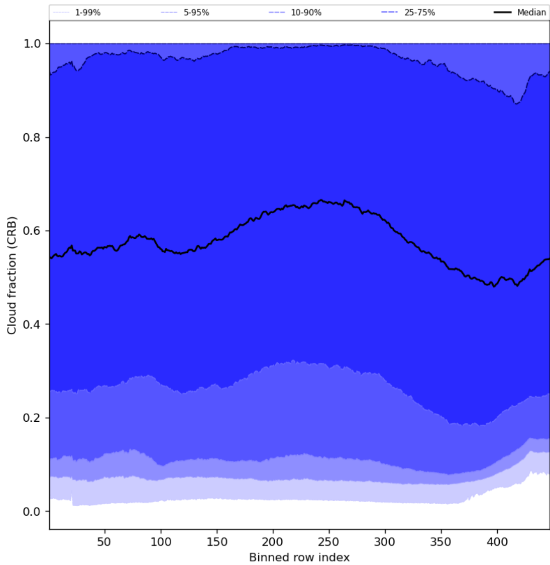
Figure 58: Along track statistics of “Cloud fraction (CRB)” for 2023-12-04 to 2023-12-05
