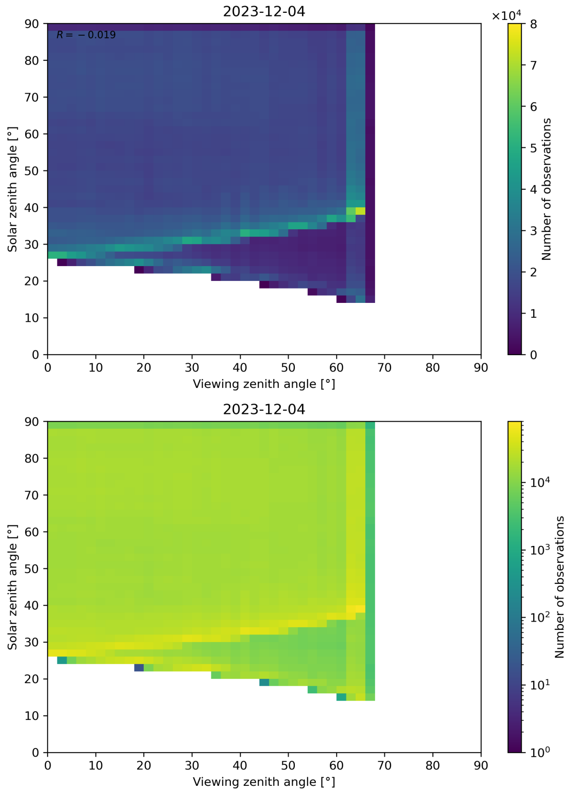
Figure 114: Scatter density plot of “Viewing zenith angle” against “Solar zenith angle” for 2023-12-04 to 2023-12-05.
