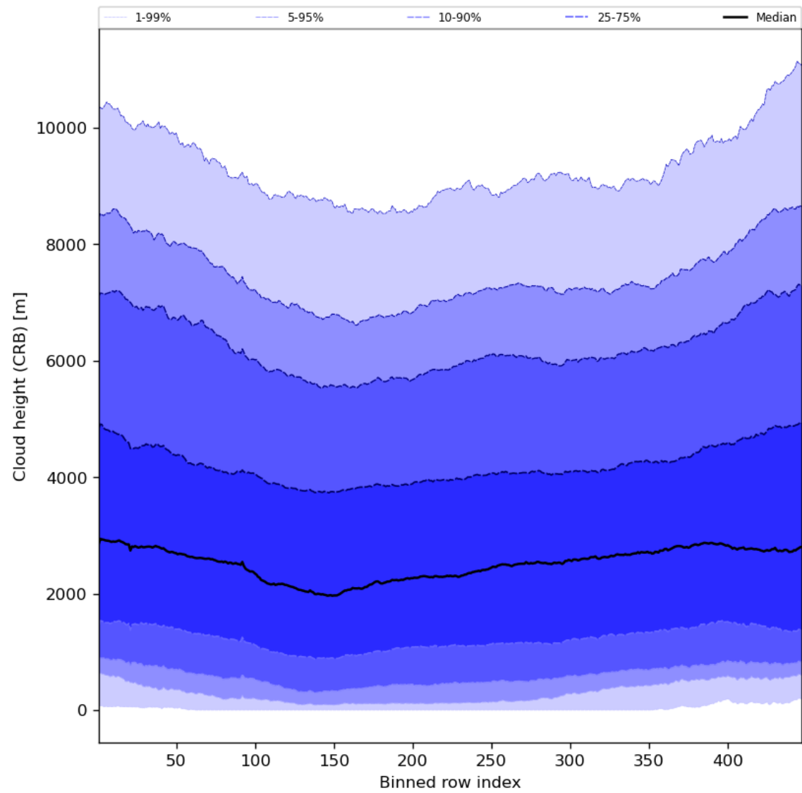
Figure 59: Along track statistics of “Cloud height (CRB)” for 2023-12-04 to 2023-12-05
