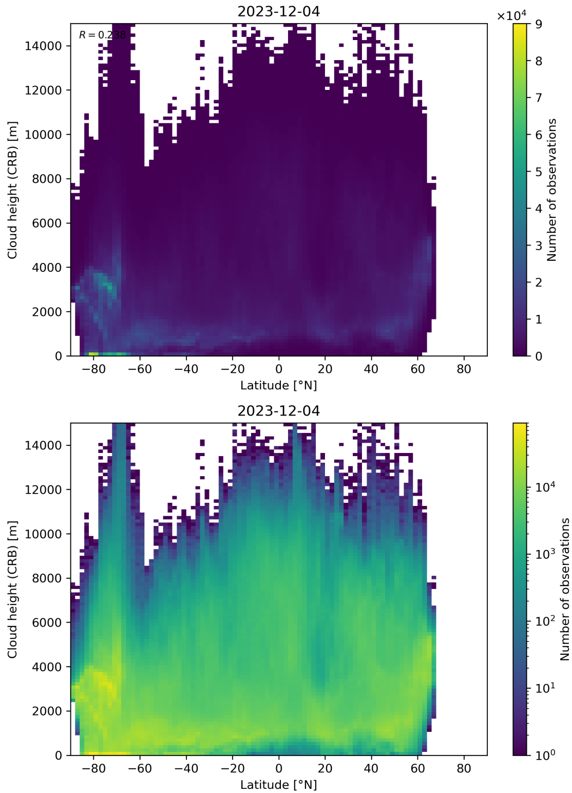
Figure 95: Scatter density plot of “Latitude” against “Cloud height (CRB)” for 2023-12-04 to 2023-12-05.
