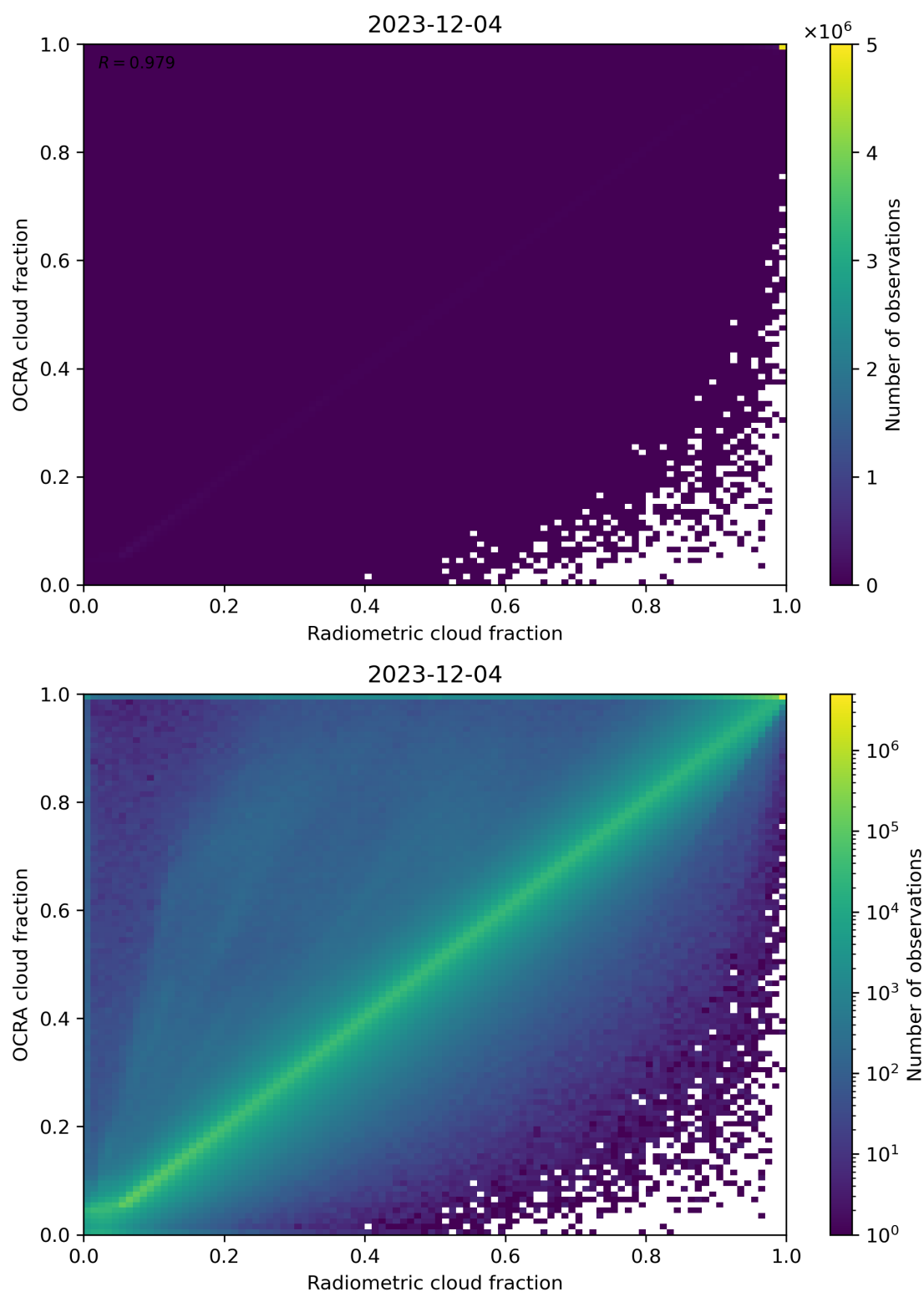
Figure 72: Scatter density plot of “Radiometric cloud fraction” against “OCRA cloud fraction” for 2023-12-04 to 2023-12-05.
