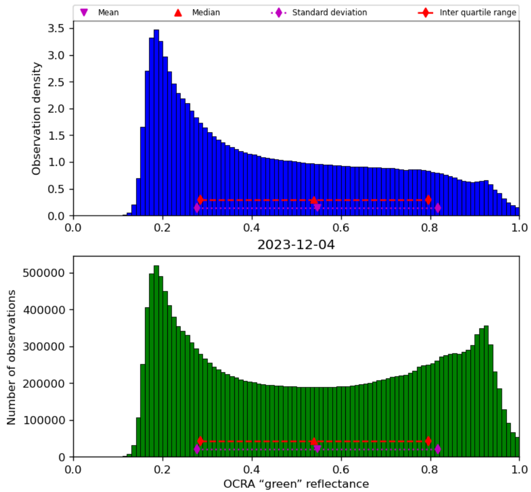
Figure 52: Histogram of “OCRA “green” reflectance” for 2023-12-04 to 2023-12-05
