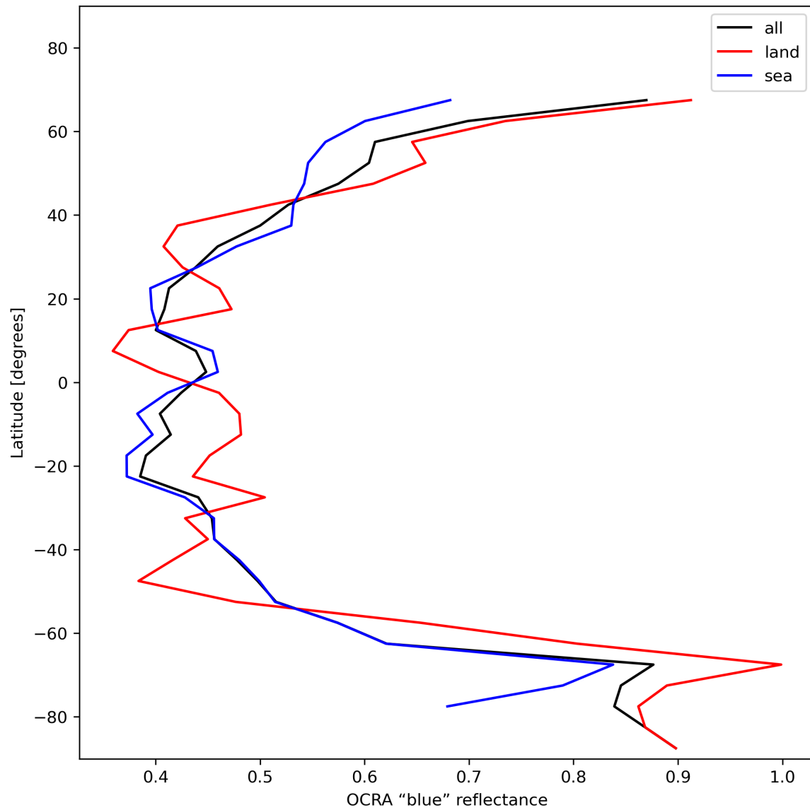
Figure 35: Zonal average of “OCRA “blue” reflectance” for 2023-12-04 to 2023-12-05.
