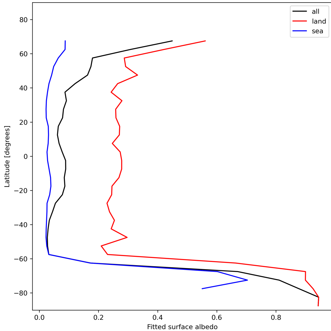
Figure 29: Zonal average of “Fitted surface albedo” for 2023-12-04 to 2023-12-05.
