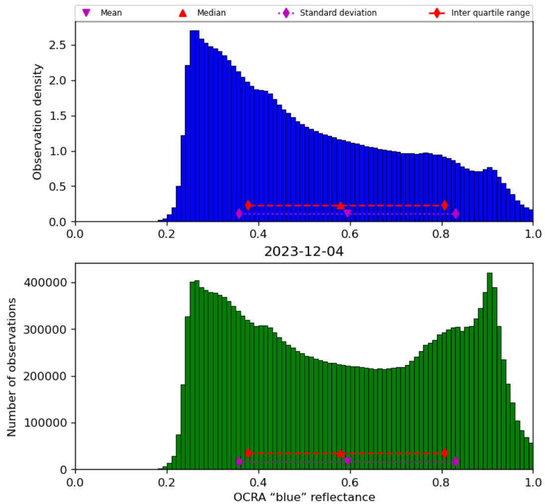
Figure 51: Histogram of “OCRA “blue” reflectance” for 2023-12-04 to 2023-12-05
