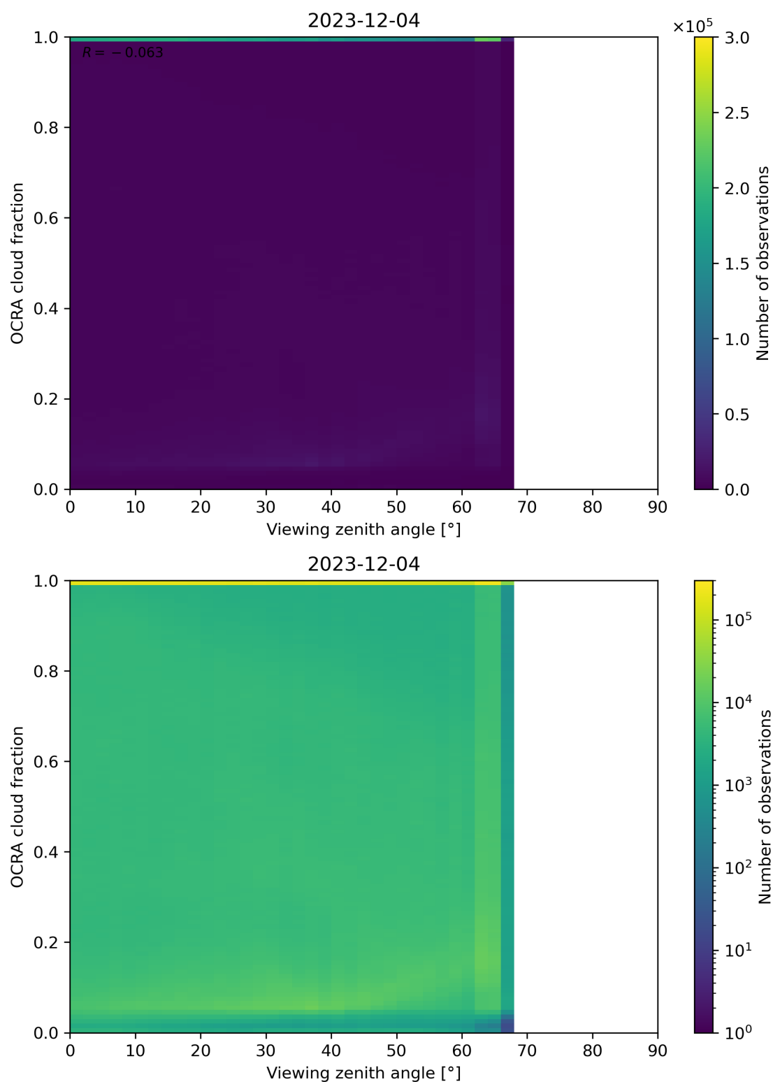
Figure 108: Scatter density plot of “Viewing zenith angle” against “OCRA cloud fraction” for 2023-12-04 to 2023-12-05.
