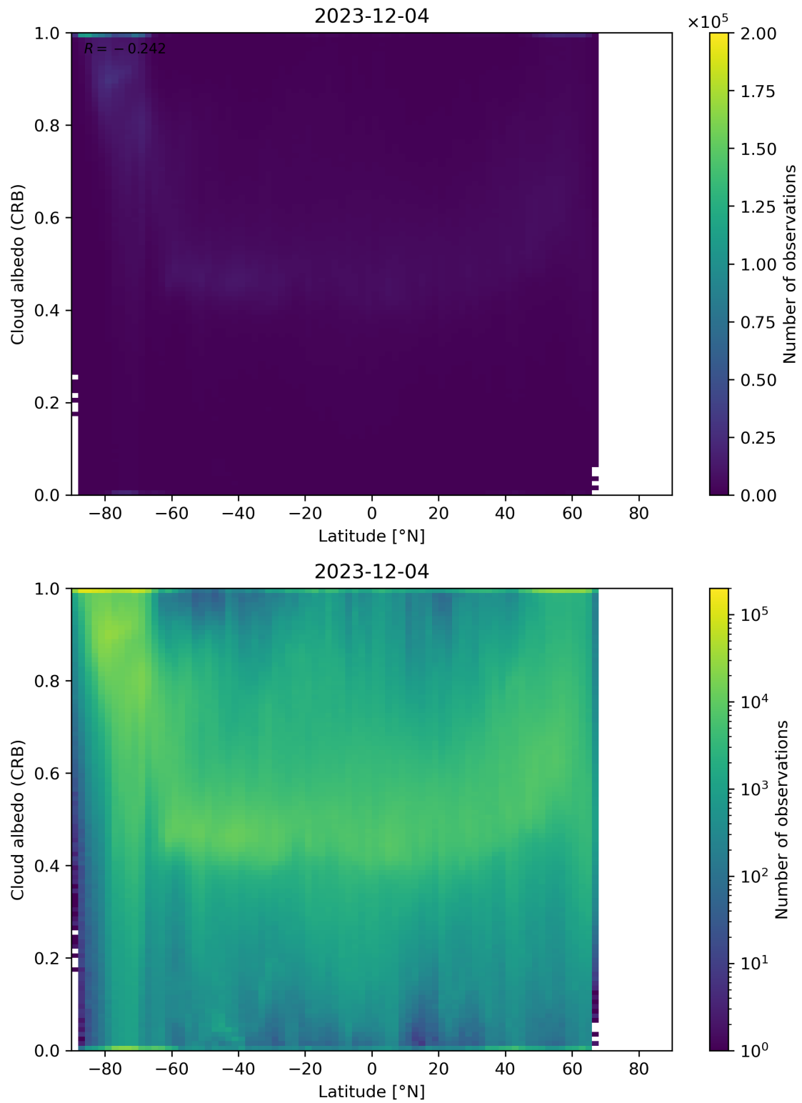
Figure 91: Scatter density plot of “Latitude” against “Cloud albedo (CRB)” for 2023-12-04 to 2023-12-05.
