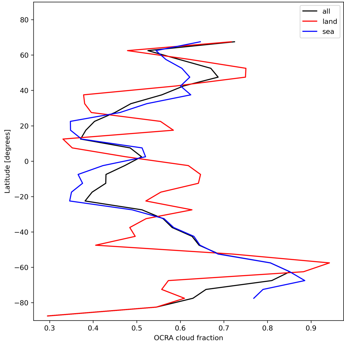
Figure 34: Zonal average of “OCRA cloud fraction” for 2023-12-04 to 2023-12-05.
