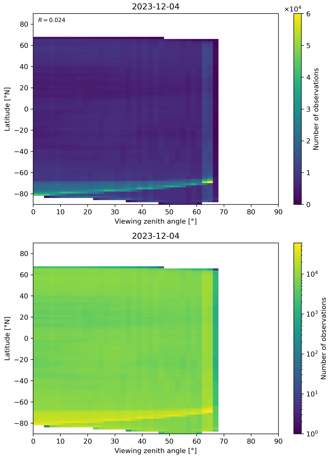
Figure 113: Scatter density plot of “Viewing zenith angle” against “Latitude” for 2023-12-04 to 2023-12-05.
