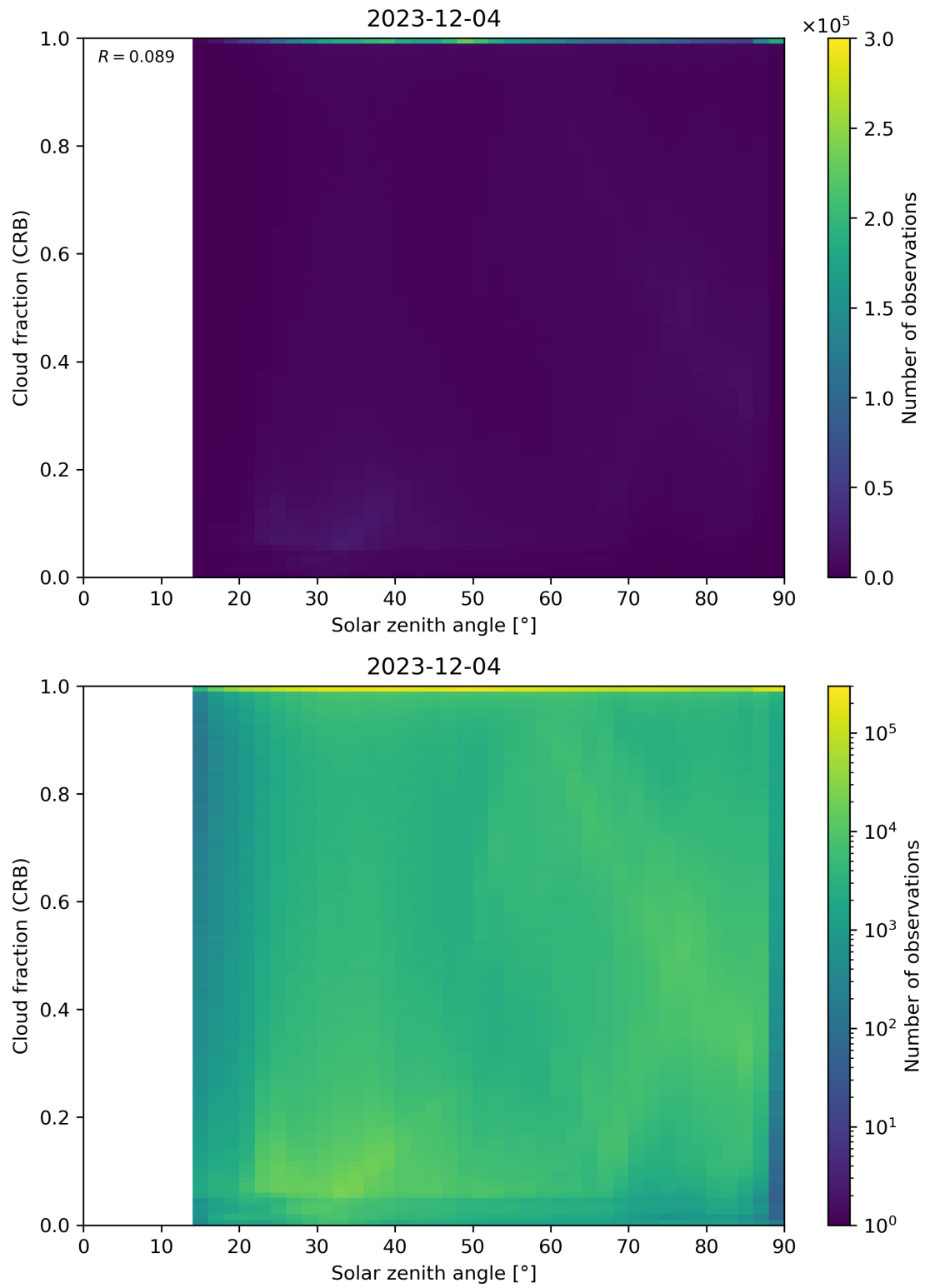
Figure 101: Scatter density plot of “Solar zenith angle” against “Cloud fraction (CRB)” for 2023-12-04 to 2023-12-05.
