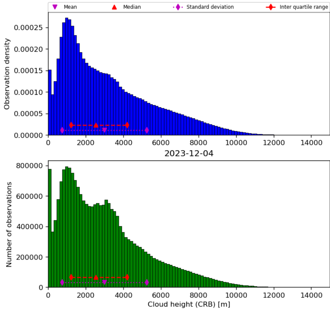
Figure 43: Histogram of “Cloud height (CRB)” for 2023-12-04 to 2023-12-05
