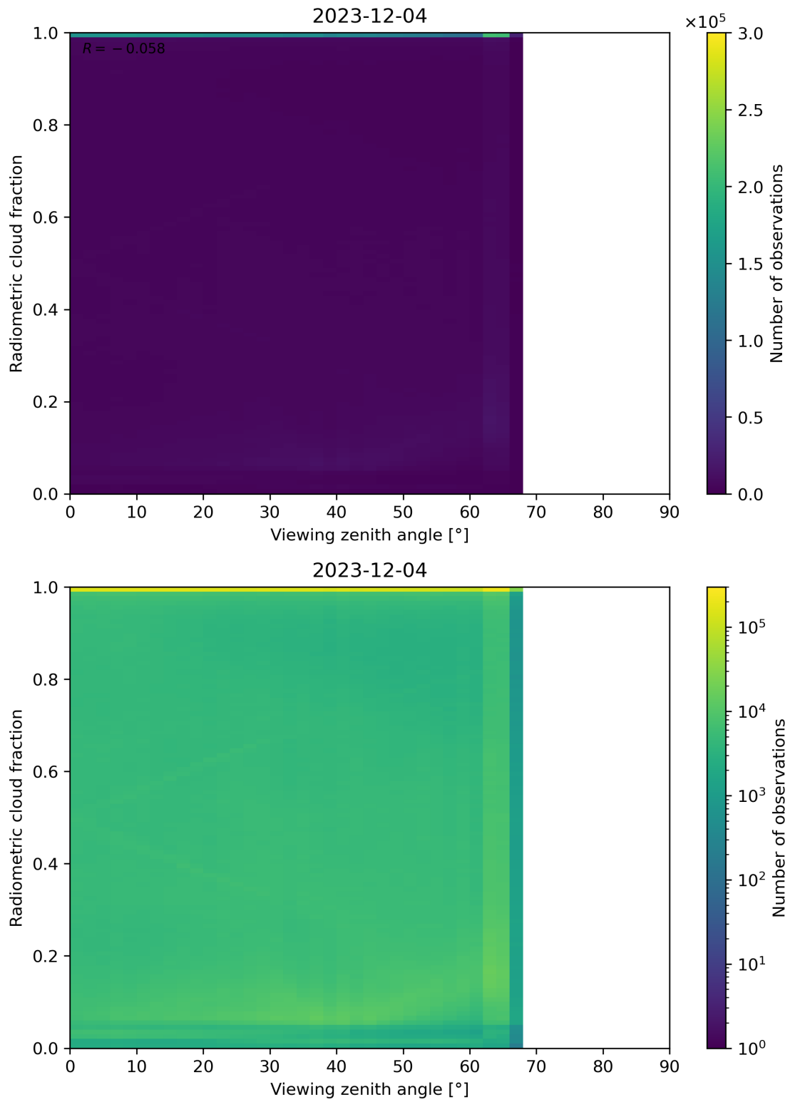
Figure 107: Scatter density plot of “Viewing zenith angle” against “Radiometric cloud fraction” for 2023-12-04 to 2023-12-05.
