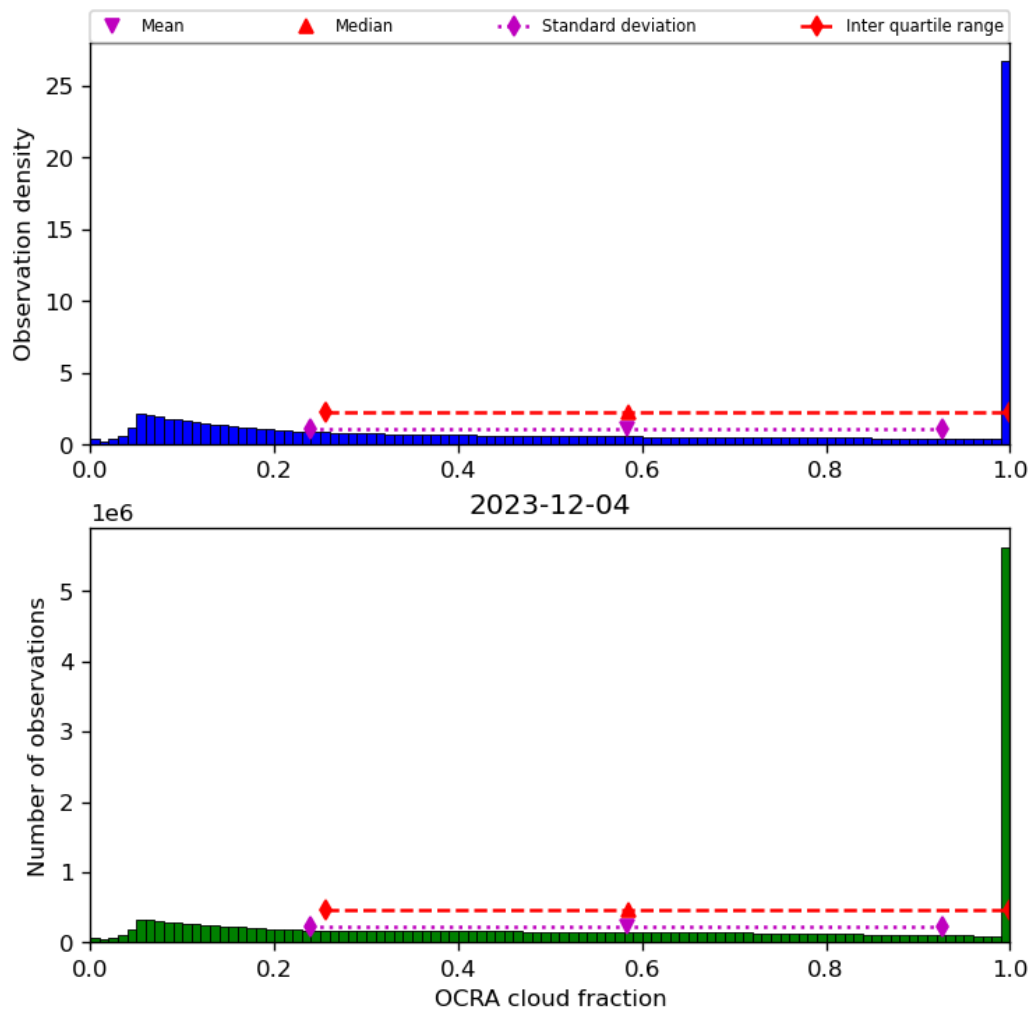
Figure 50: Histogram of “OCRA cloud fraction” for 2023-12-04 to 2023-12-05
