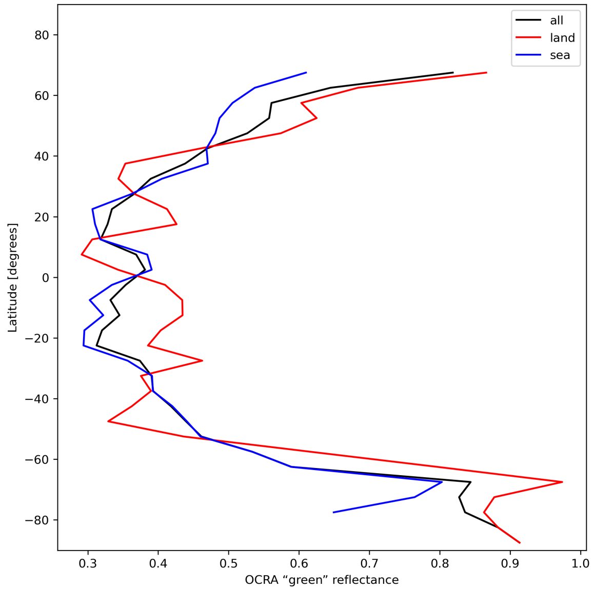
Figure 36: Zonal average of “OCRA “green” reflectance” for 2023-12-04 to 2023-12-05.
