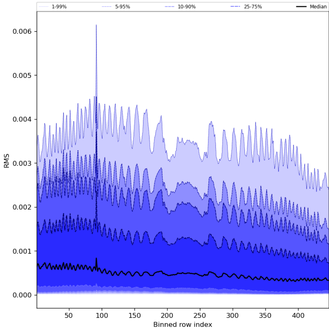
Figure 63: Along track statistics of “RMS” for 2023-12-04 to 2023-12-05
