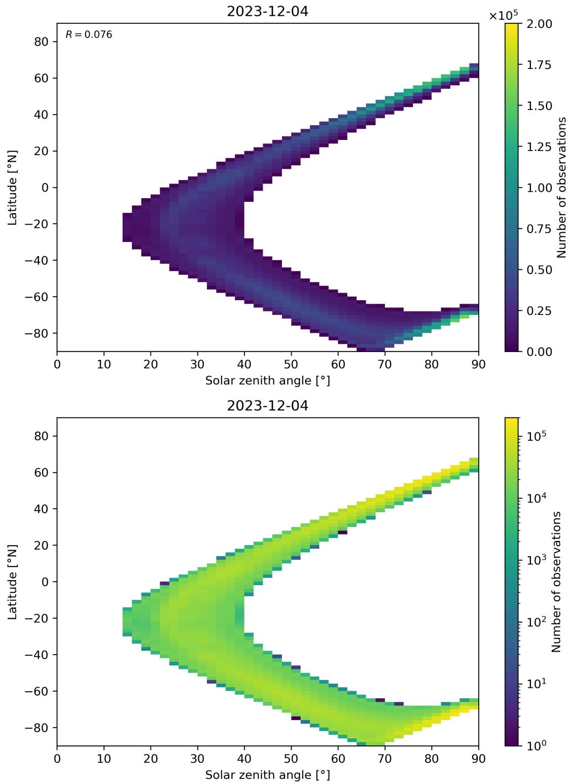
Figure 105: Scatter density plot of “Solar zenith angle” against “Latitude” for 2023-12-04 to 2023-12-05.
