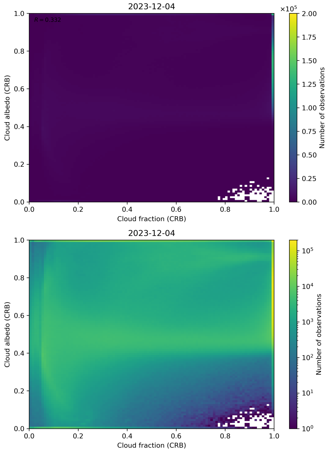
Figure 77: Scatter density plot of “Cloud fraction (CRB)” against “Cloud albedo (CRB)” for 2023-12-04 to 2023-12-05.
