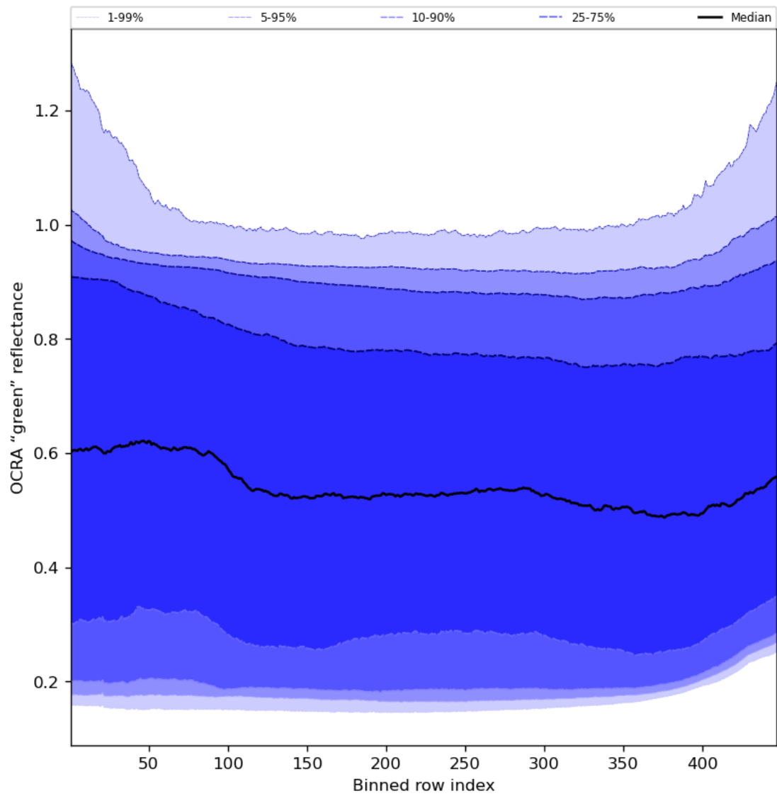
Figure 68: Along track statistics of “OCRA “green” reflectance” for 2023-12-04 to 2023-12-05
