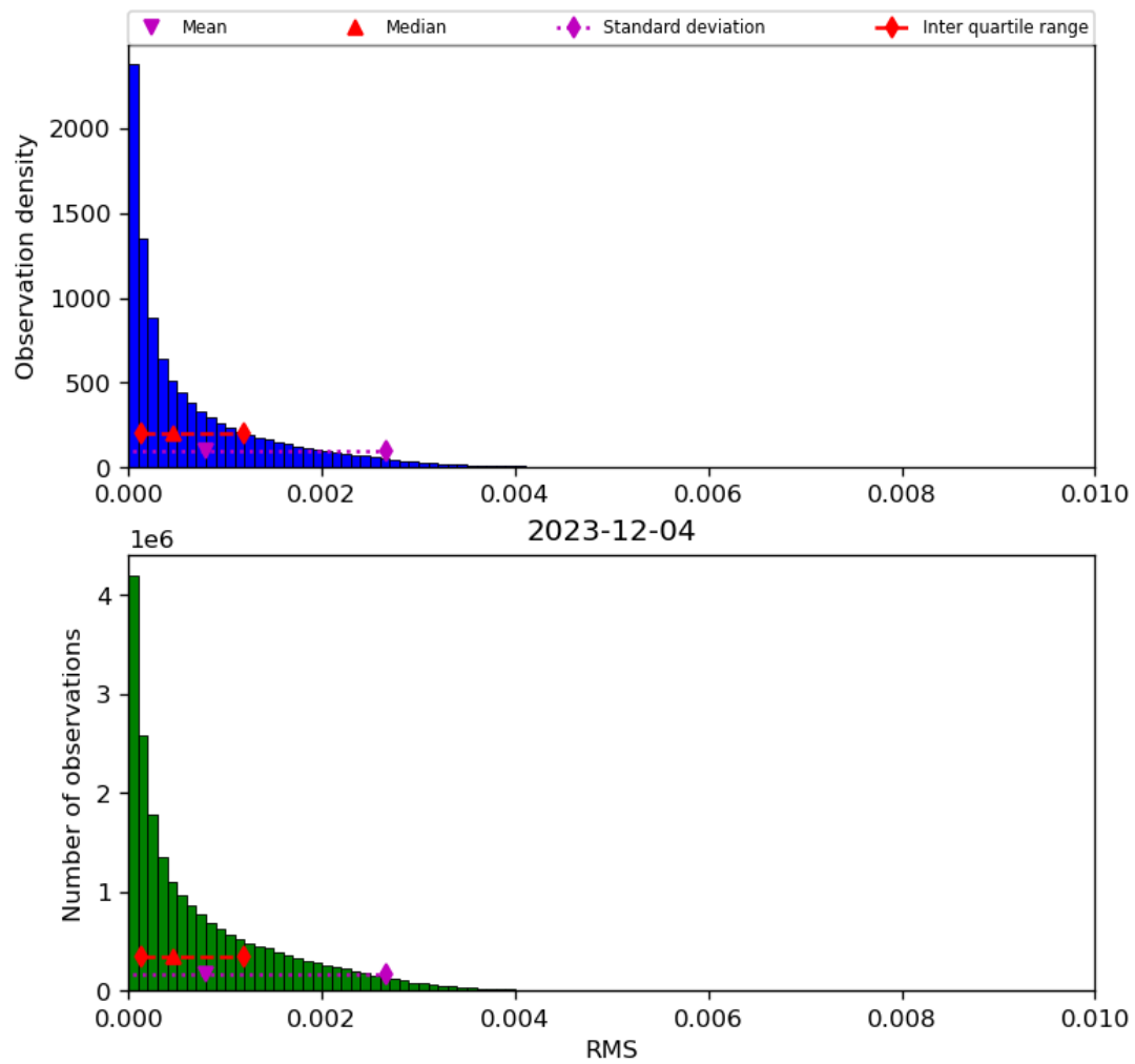
Figure 47: Histogram of “RMS” for 2023-12-04 to 2023-12-05
