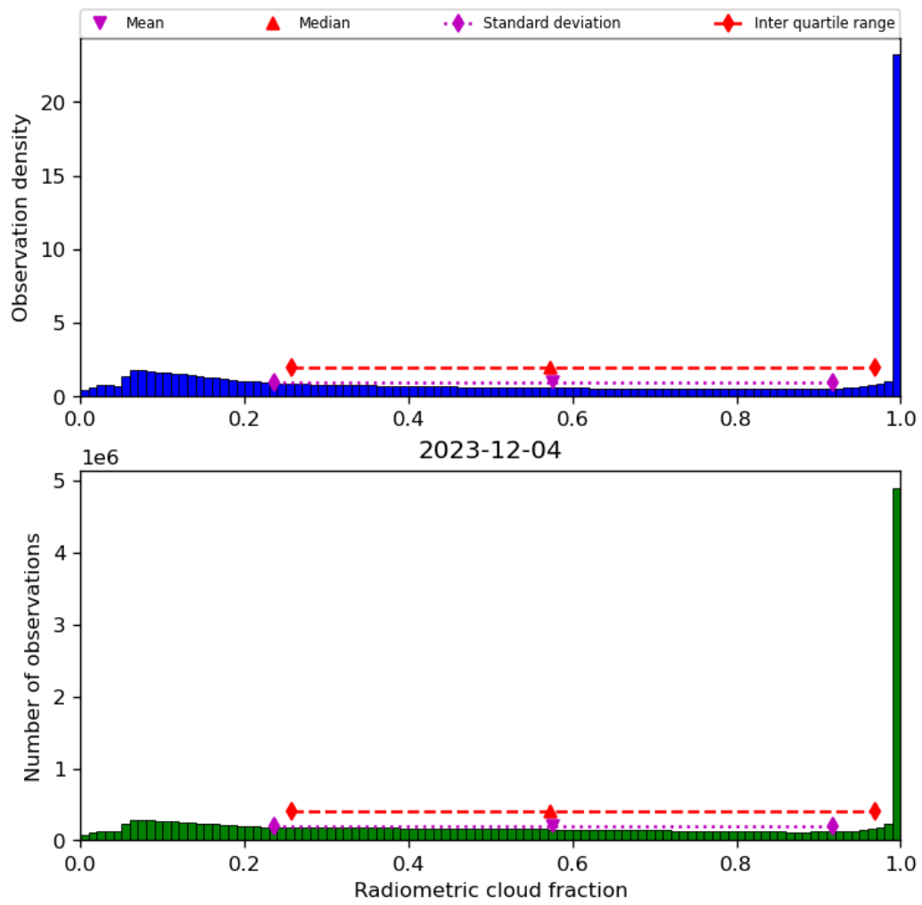
Figure 39: Histogram of “Radiometric cloud fraction” for 2023-12-04 to 2023-12-05
