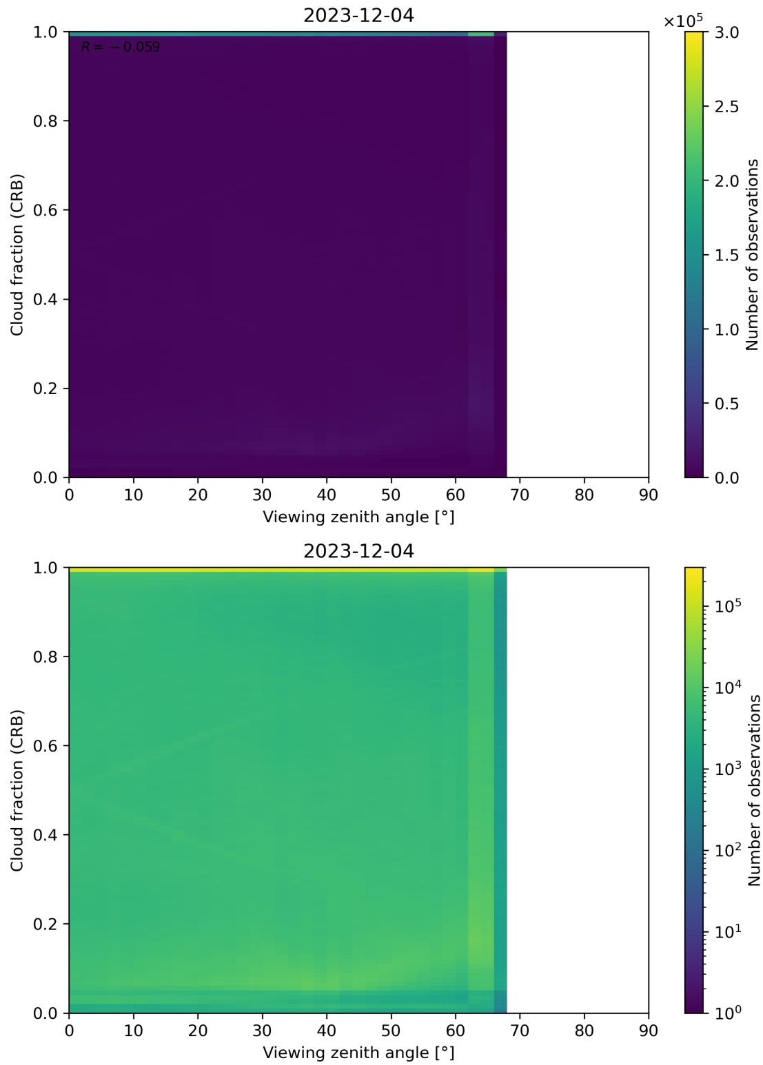
Figure 109: Scatter density plot of “Viewing zenith angle” against “Cloud fraction (CRB)” for 2023-12-04 to 2023-12-05.
