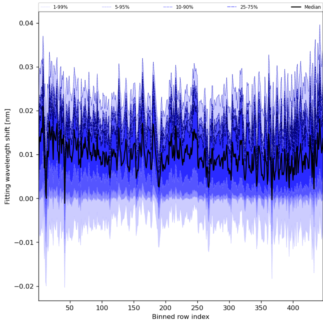
Figure 65: Along track statistics of “Fitting wavelength shift” for 2023-12-04 to 2023-12-05
