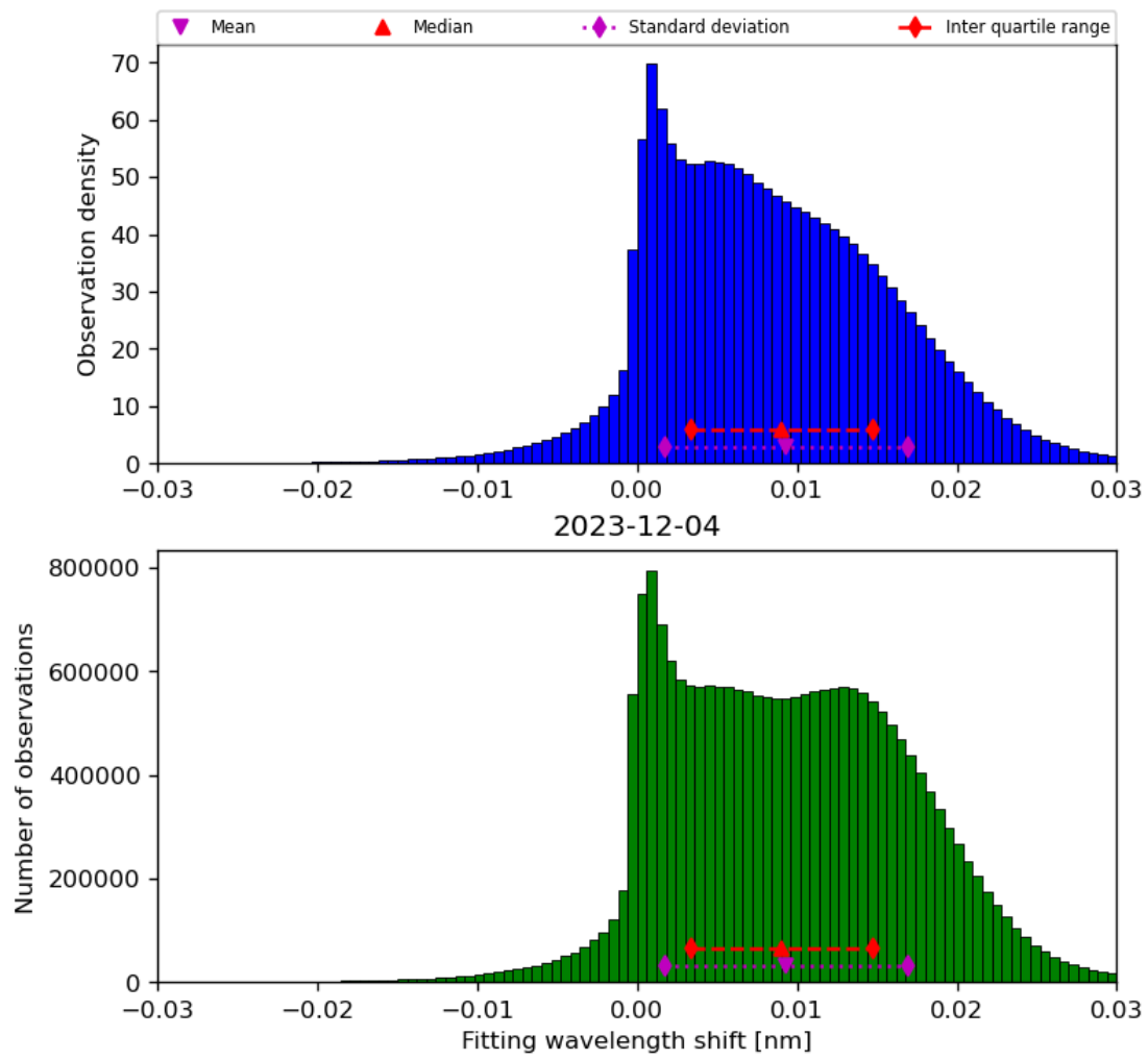
Figure 49: Histogram of “Fitting wavelength shift” for 2023-12-04 to 2023-12-05
