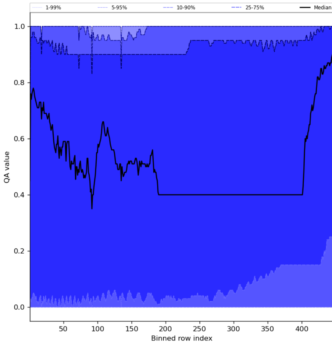
Figure 54: Along track statistics of “QA value” for 2023-12-04 to 2023-12-05
