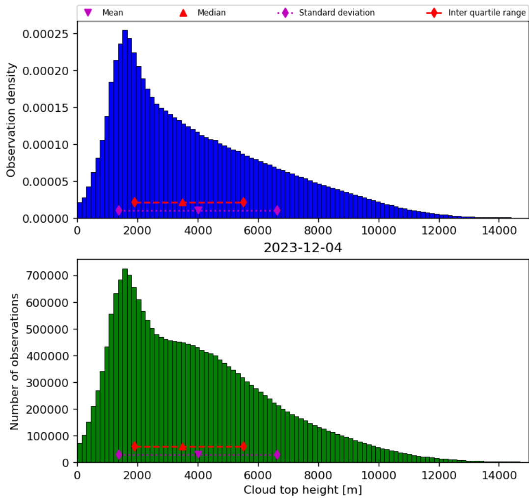
Figure 40: Histogram of “Cloud top height” for 2023-12-04 to 2023-12-05
