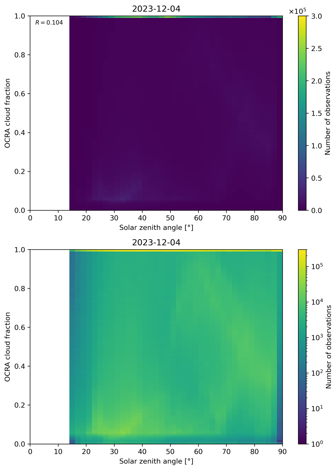
Figure 100: Scatter density plot of “Solar zenith angle” against “OCRA cloud fraction” for 2023-12-04 to 2023-12-05.
