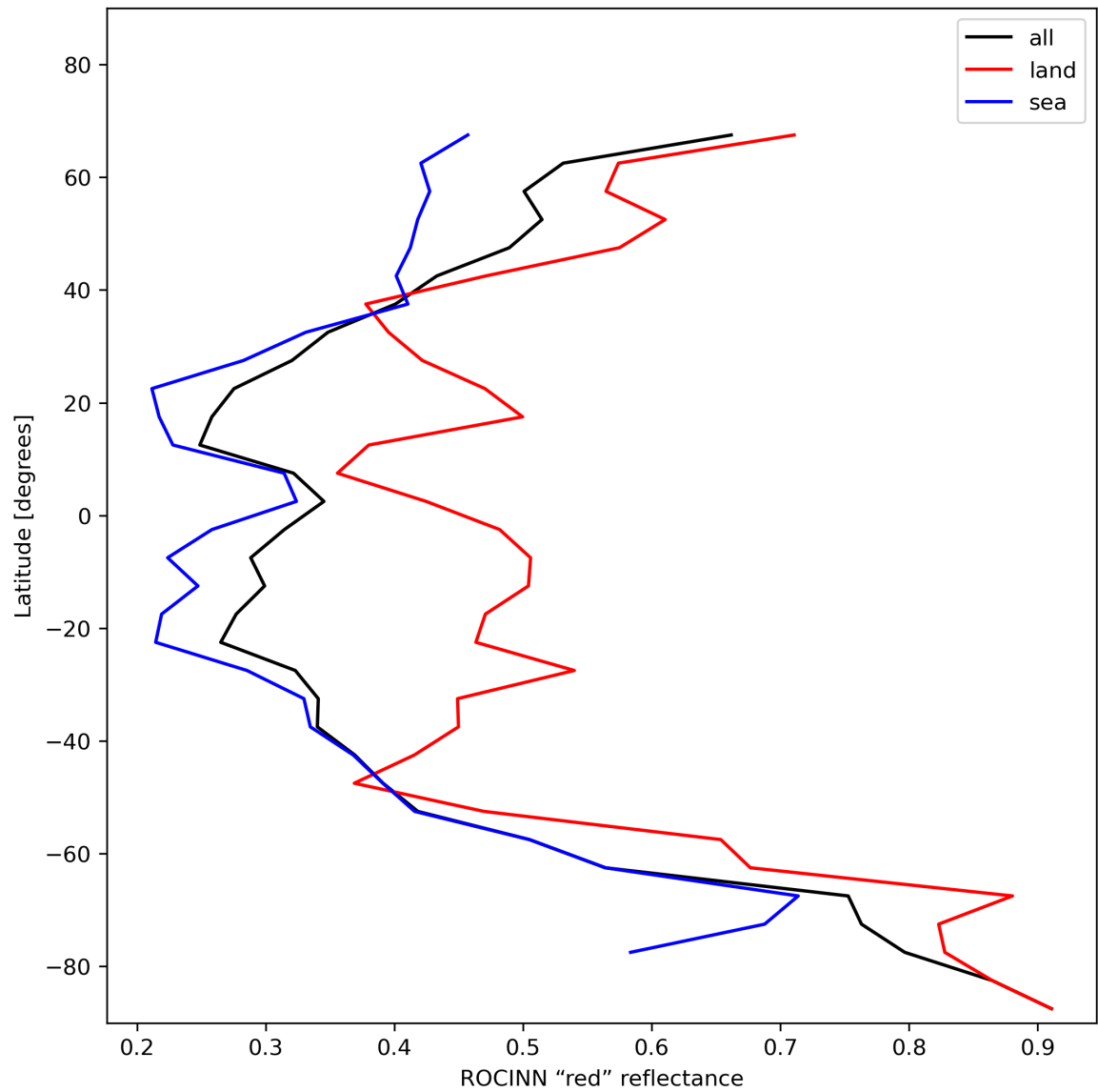
Figure 37: Zonal average of "ROCINN "red" reflectance" for 2023-12-04 to 2023-12-05.
