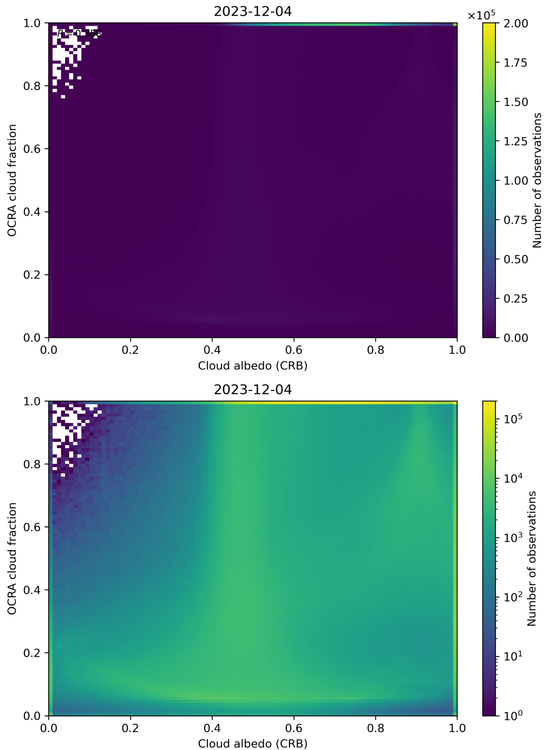
Figure 70: Scatter density plot of “Cloud albedo (CRB)” against “OCRA cloud fraction” for 2023-12-04 to 2023-12-05.
