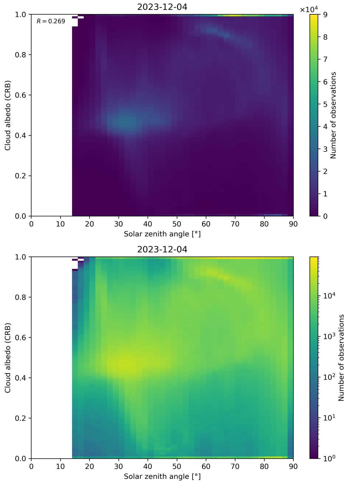
Figure 98: Scatter density plot of “Solar zenith angle” against “Cloud albedo (CRB)” for 2023-12-04 to 2023-12-05.
