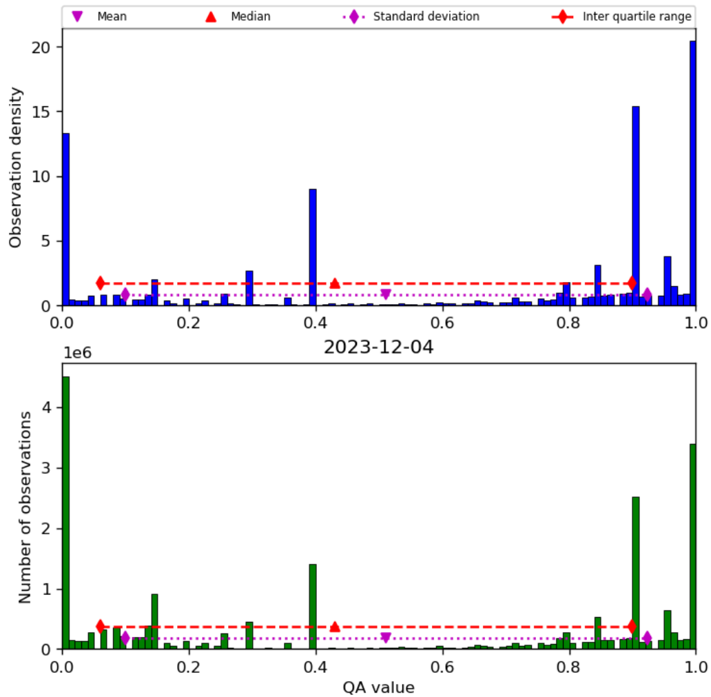
Figure 38: Histogram of “QA value” for 2023-12-04 to 2023-12-05
