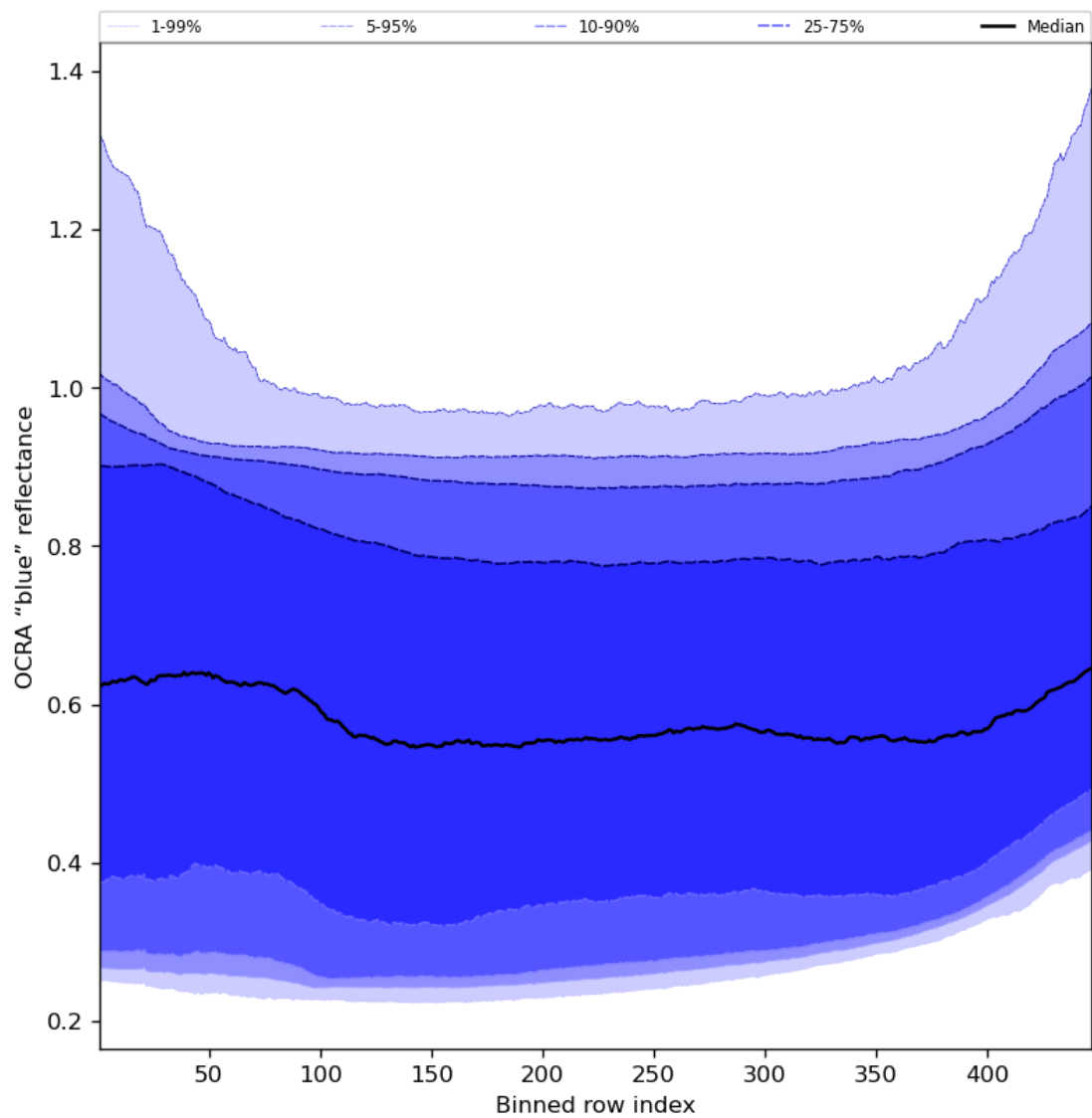
Figure 67: Along track statistics of “OCRA “blue” reflectance” for 2023-12-04 to 2023-12-05
