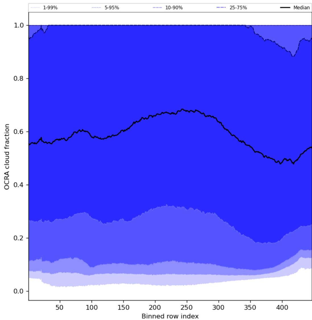
Figure 66: Along track statistics of “OCRA cloud fraction” for 2023-12-04 to 2023-12-05
