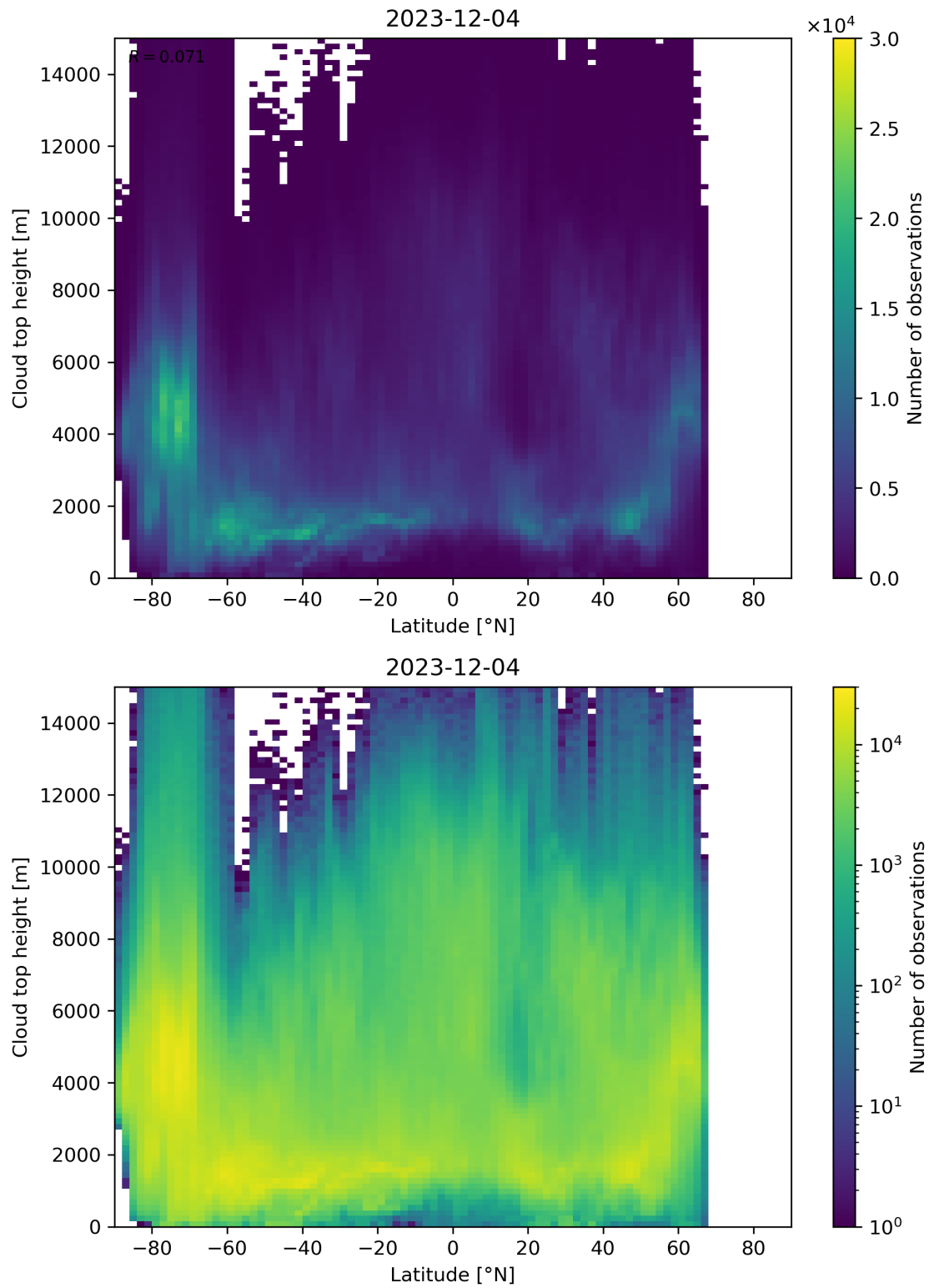
Figure 97: Scatter density plot of “Latitude” against “Cloud top height” for 2023-12-04 to 2023-12-05.
