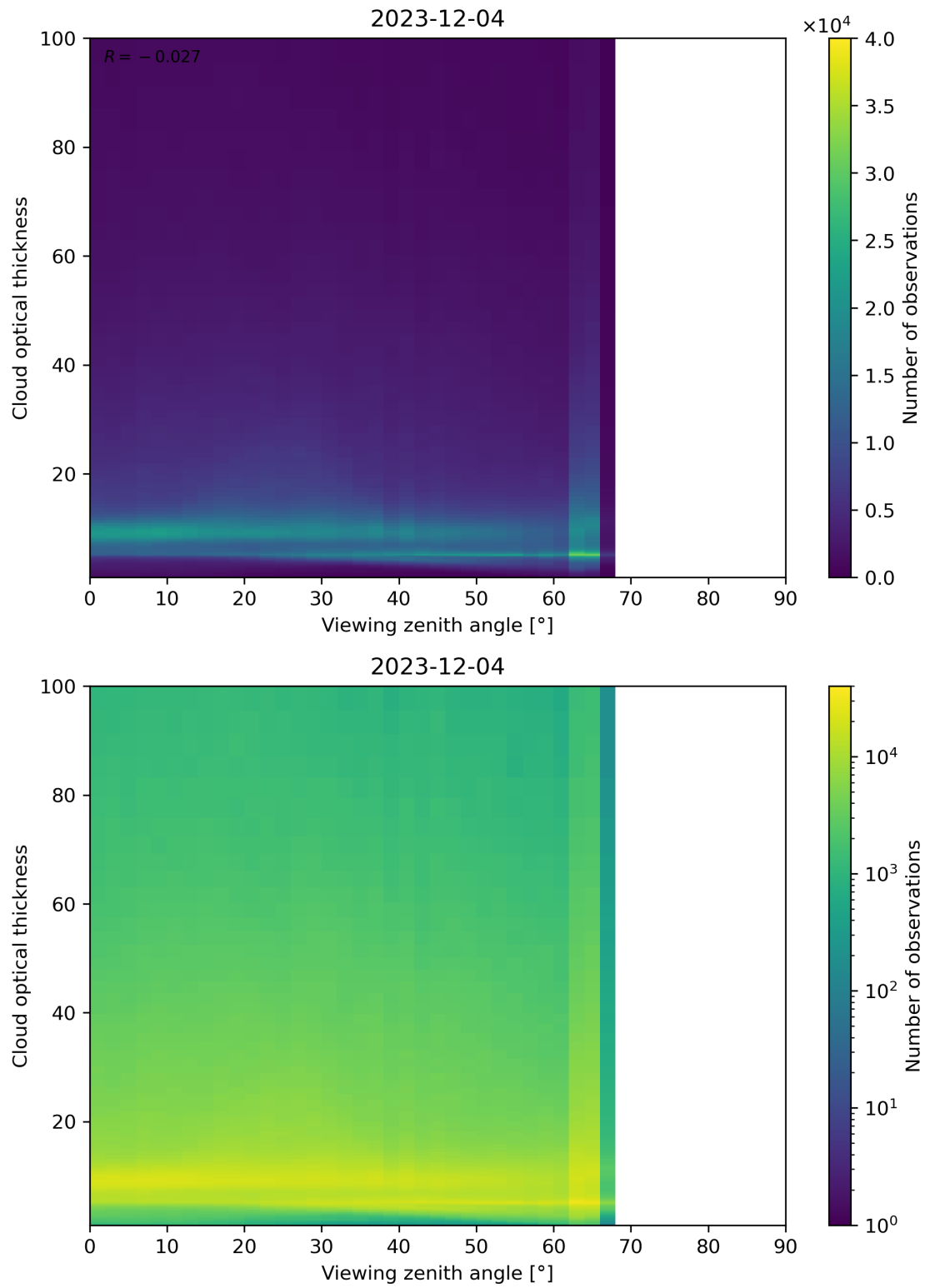
Figure 111: Scatter density plot of “Viewing zenith angle” against “Cloud optical thickness” for 2023-12-04 to 2023-12-05.
