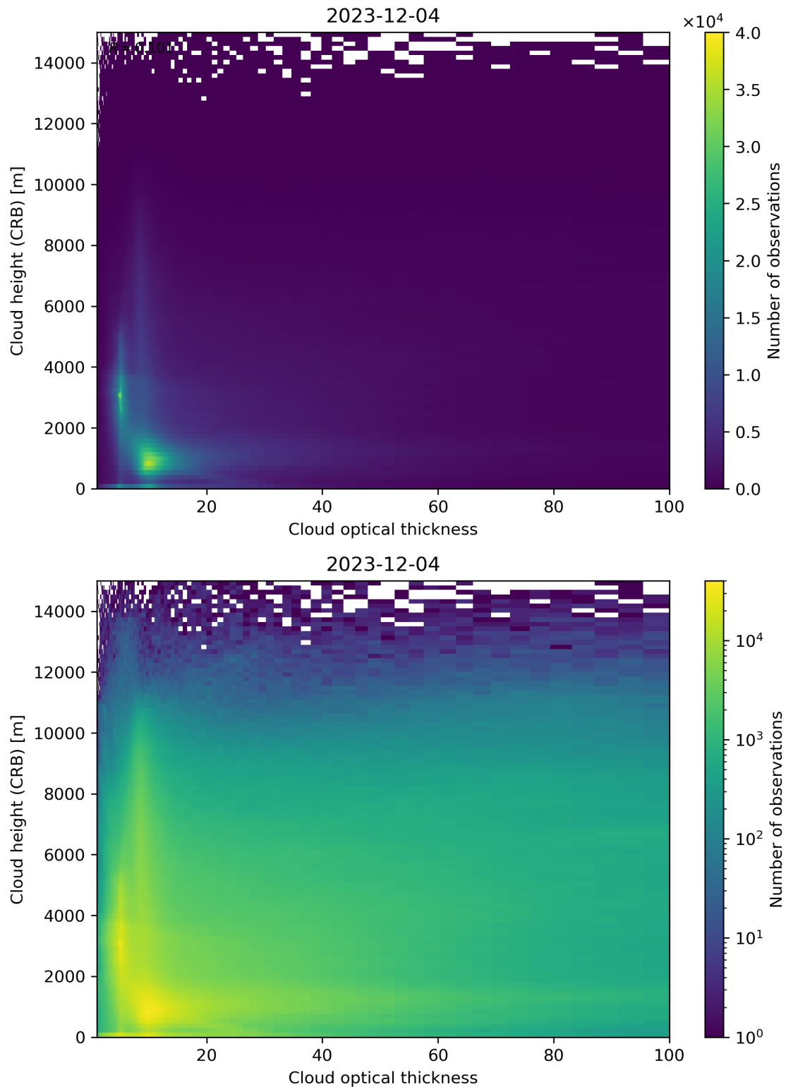
Figure 85: Scatter density plot of “Cloud optical thickness” against “Cloud height (CRB)” for 2023-12-04 to 2023-12-05.
