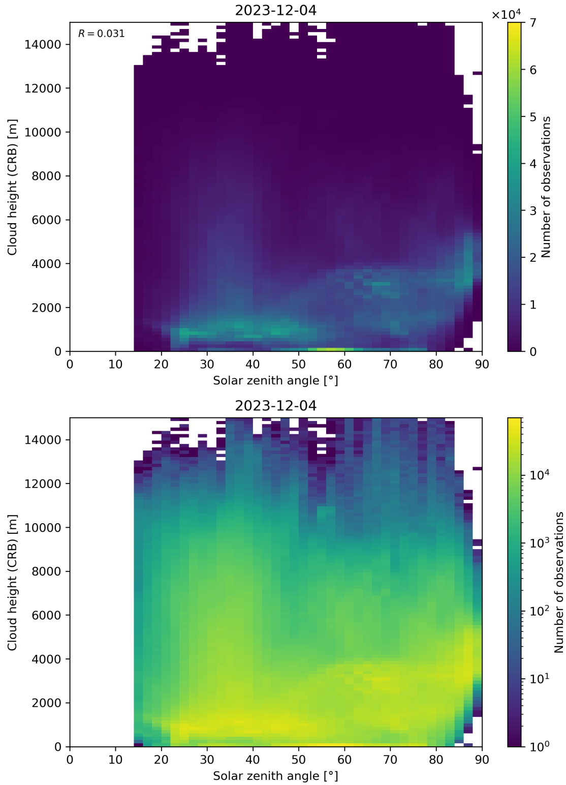
Figure 102: Scatter density plot of “Solar zenith angle” against “Cloud height (CRB)” for 2023-12-04 to 2023-12-05.
