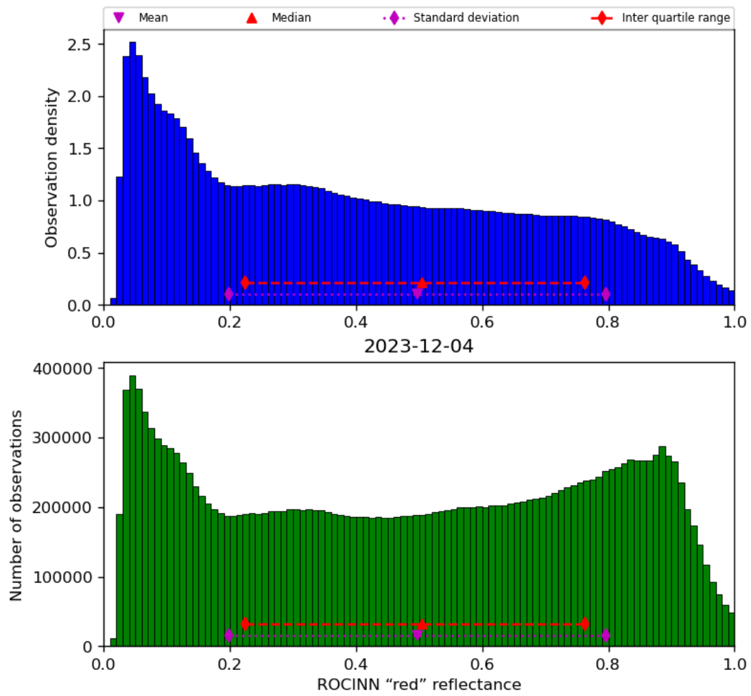
Figure 53: Histogram of “ROCINN “red” reflectance” for 2023-12-04 to 2023-12-05
