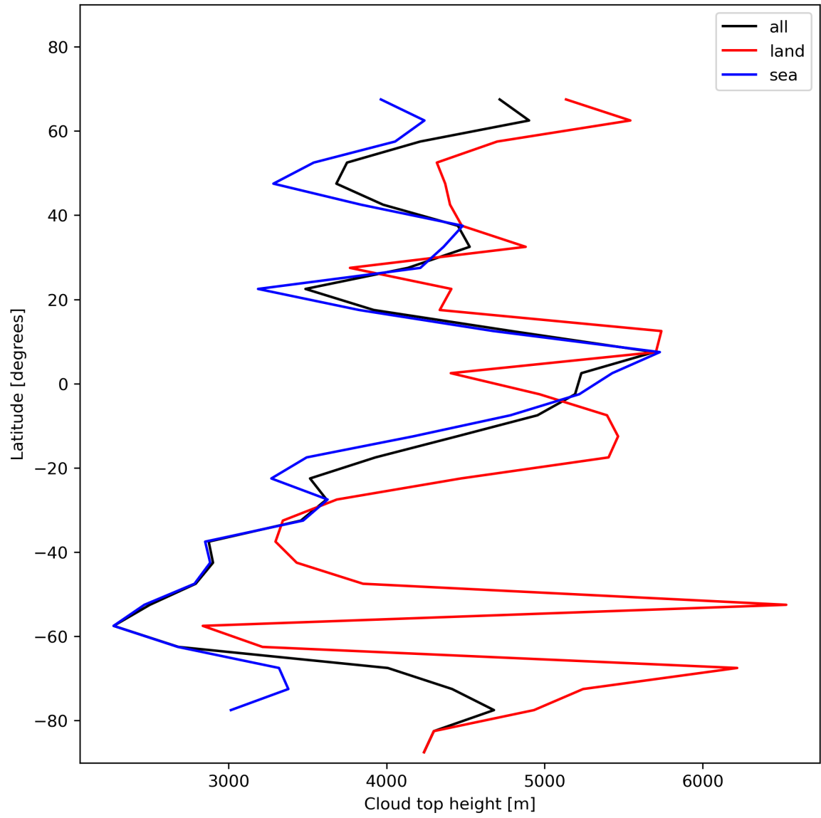
Figure 24: Zonal average of “Cloud top height” for 2023-12-04 to 2023-12-05.
