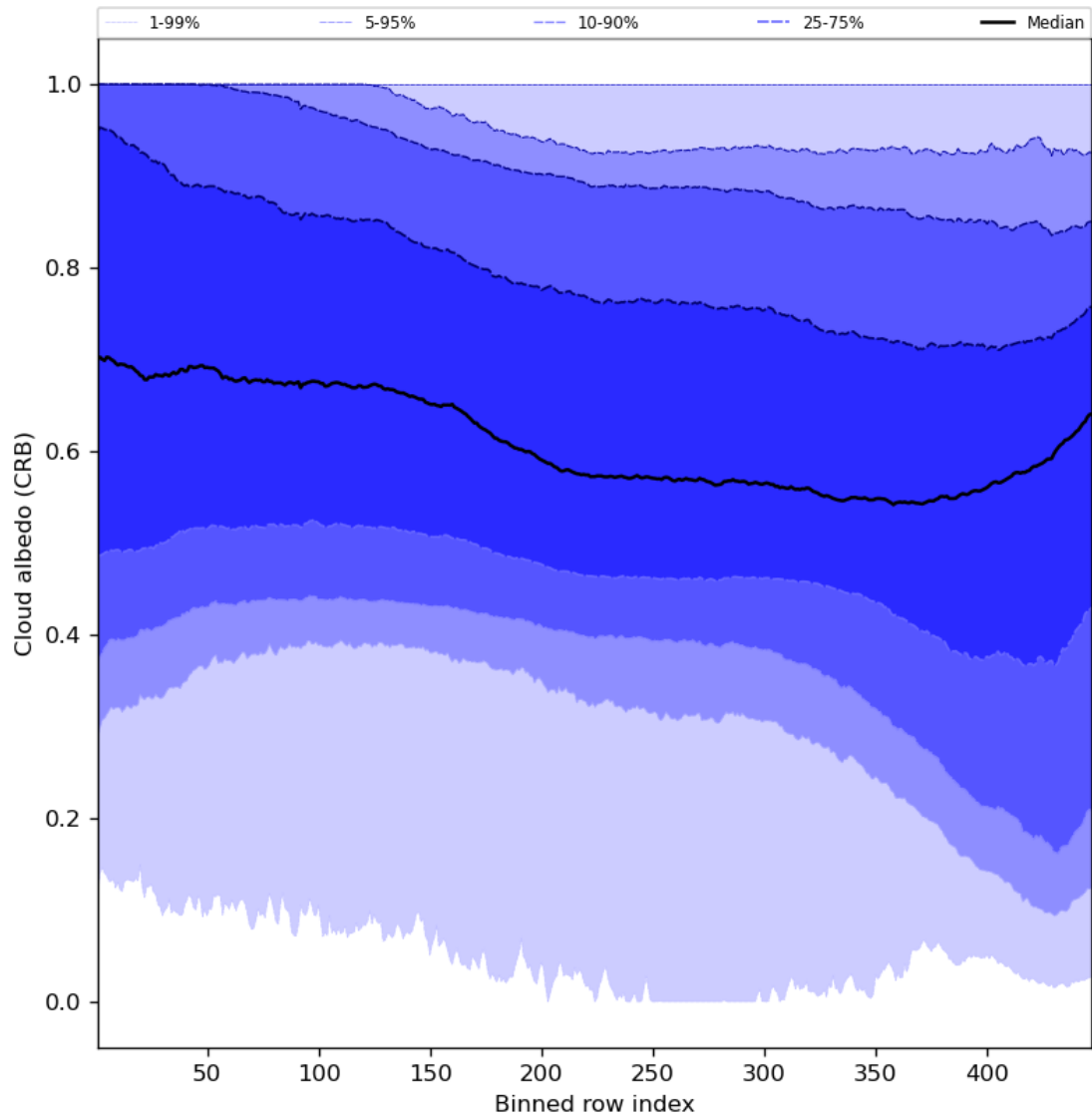
Figure 60: Along track statistics of “Cloud albedo (CRB)” for 2023-12-04 to 2023-12-05
