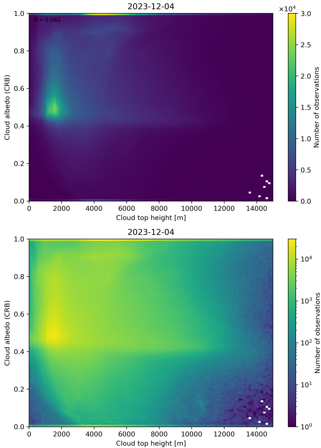
Figure 86: Scatter density plot of “Cloud top height” against “Cloud albedo (CRB)” for 2023-12-04 to 2023-12-05.
