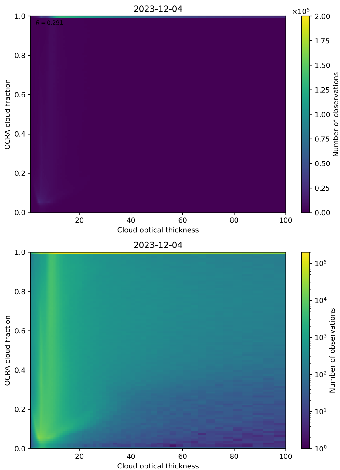
Figure 83: Scatter density plot of “Cloud optical thickness” against “OCRA cloud fraction” for 2023-12-04 to 2023-12-05.
