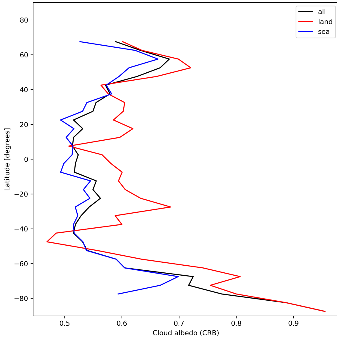
Figure 28: Zonal average of “Cloud albedo (CRB)” for 2023-12-04 to 2023-12-05.
