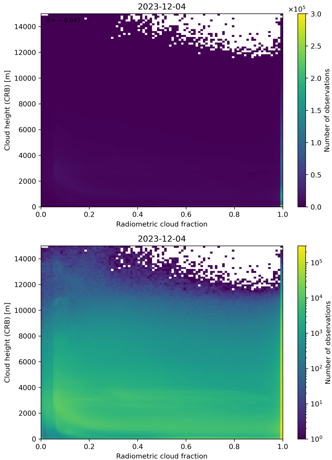
Figure 74: Scatter density plot of “Radiometric cloud fraction” against “Cloud height (CRB)” for 2023-12-04 to 2023-12-05.
