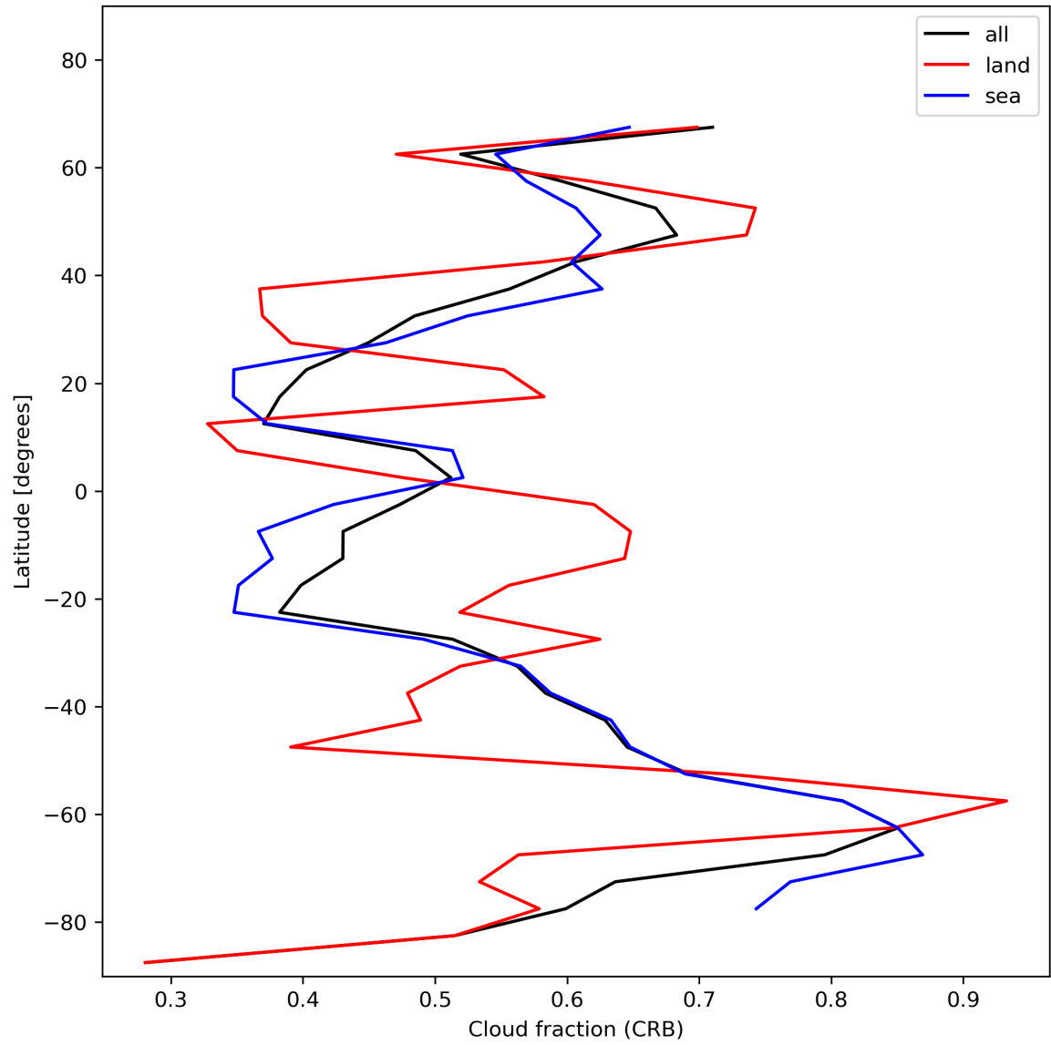
Figure 26: Zonal average of “Cloud fraction (CRB)” for 2023-12-04 to 2023-12-05.
