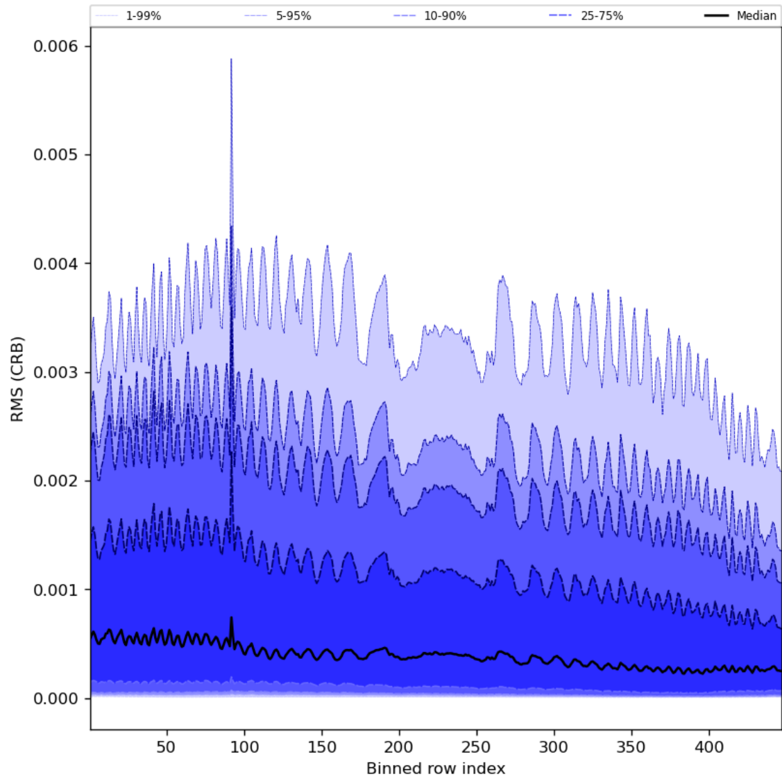
Figure 64: Along track statistics of “RMS (CRB)” for 2023-12-04 to 2023-12-05
