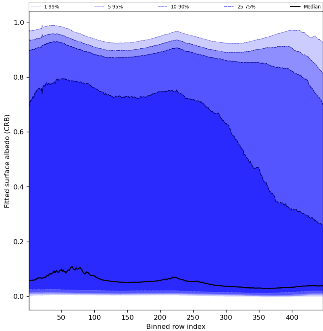
Figure 62: Along track statistics of “Fitted surface albedo (CRB)” for 2023-12-04 to 2023-12-05
