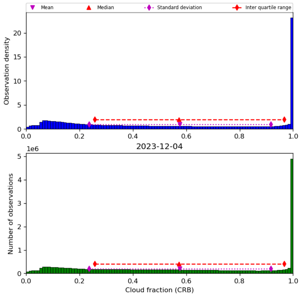
Figure 42: Histogram of “Cloud fraction (CRB)” for 2023-12-04 to 2023-12-05
