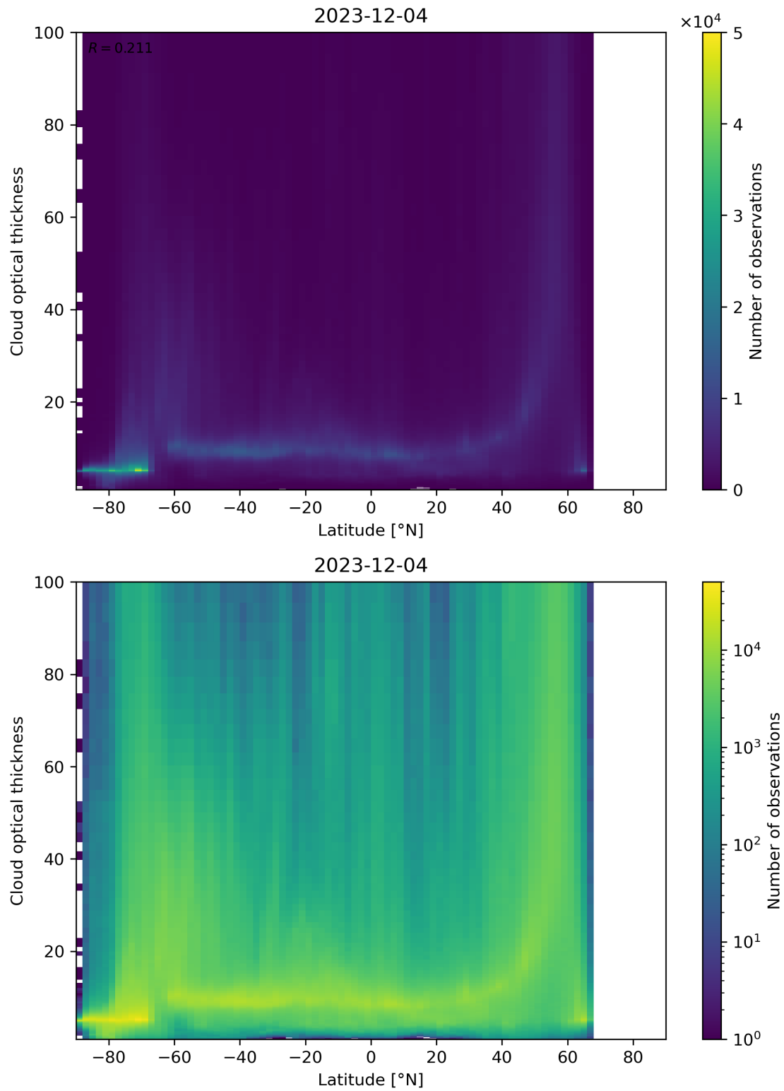
Figure 96: Scatter density plot of “Latitude” against “Cloud optical thickness” for 2023-12-04 to 2023-12-05.
