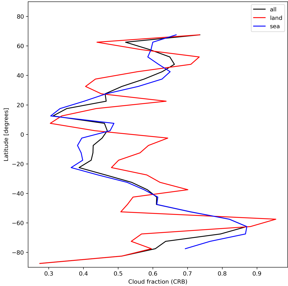
Figure 26: Zonal average of “Cloud fraction (CRB)” for 2023-12-04 to 2023-12-06.
