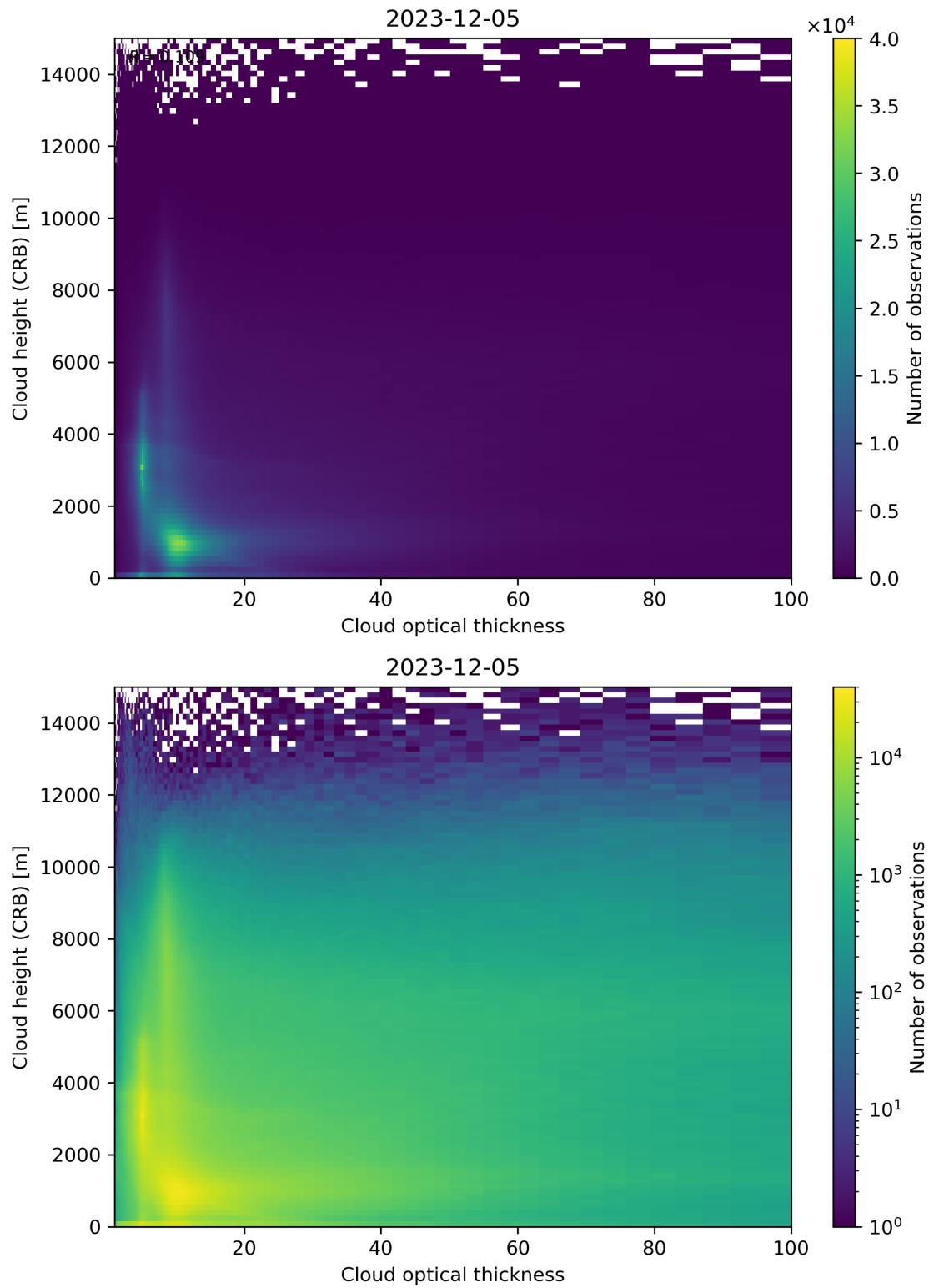
Figure 85: Scatter density plot of “Cloud optical thickness” against “Cloud height (CRB)” for 2023-12-04 to 2023-12-06.
