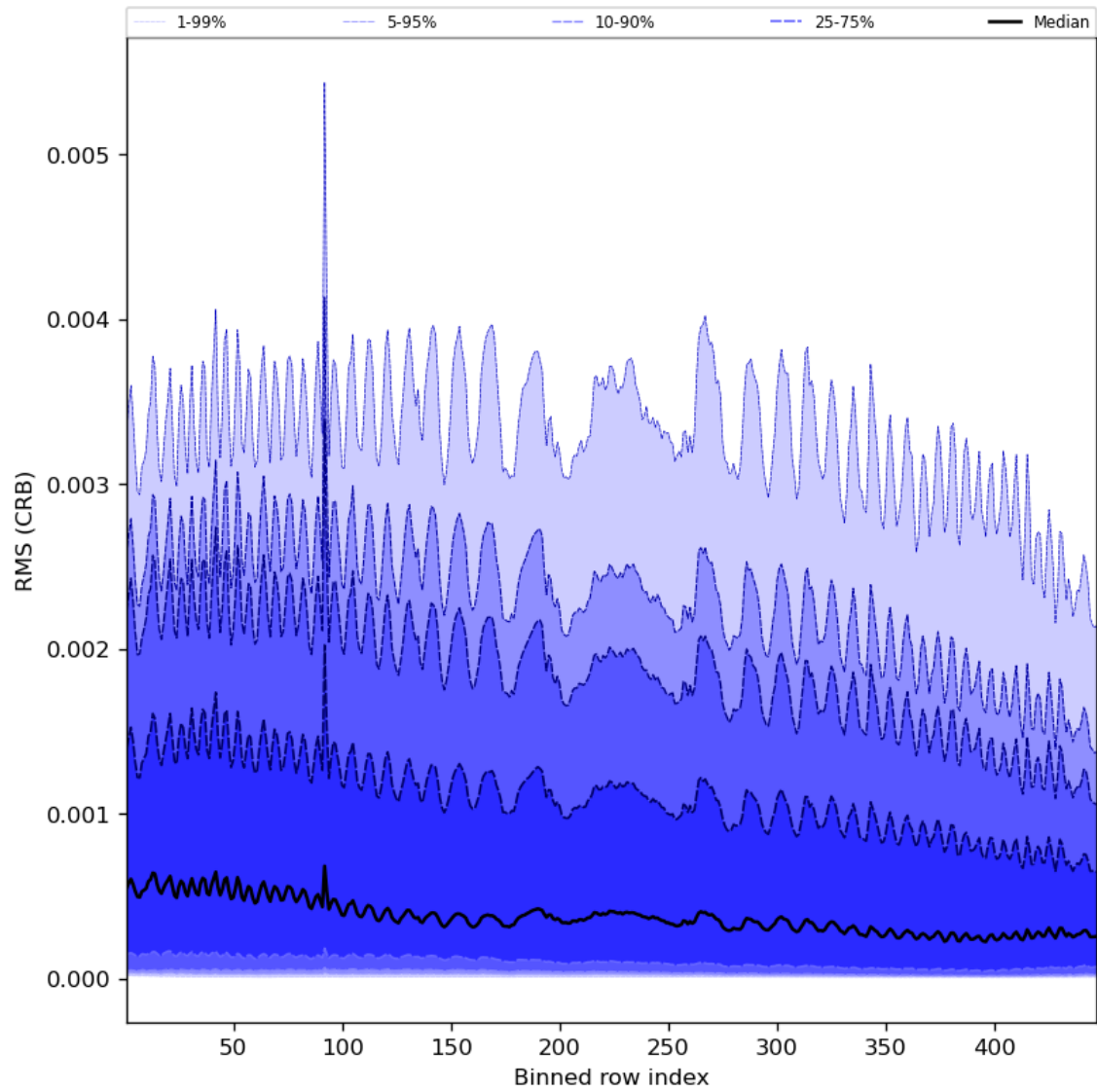
Figure 64: Along track statistics of “RMS (CRB)” for 2023-12-04 to 2023-12-06
