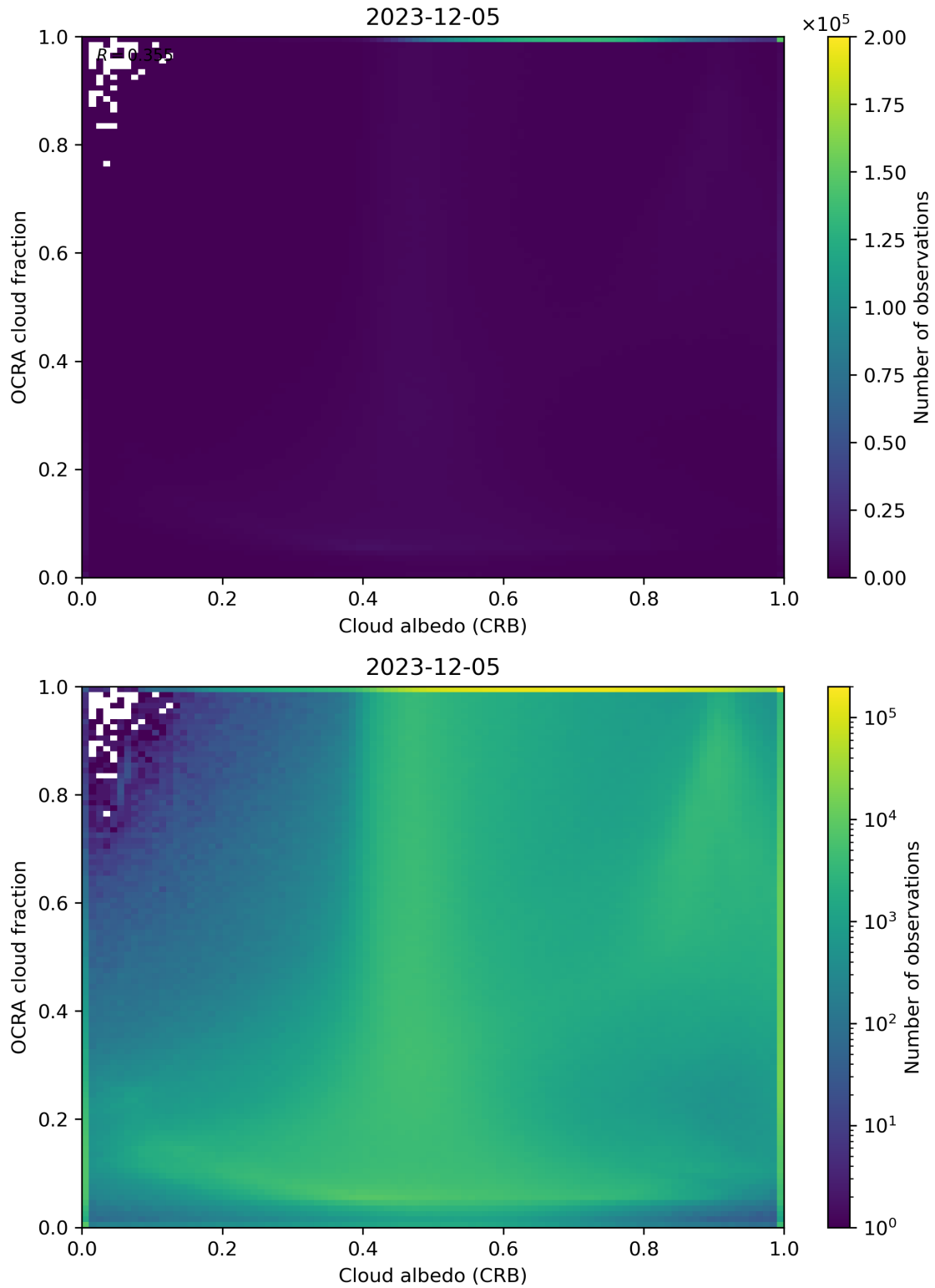
Figure 70: Scatter density plot of “Cloud albedo (CRB)” against “OCRA cloud fraction” for 2023-12-04 to 2023-12-06.
