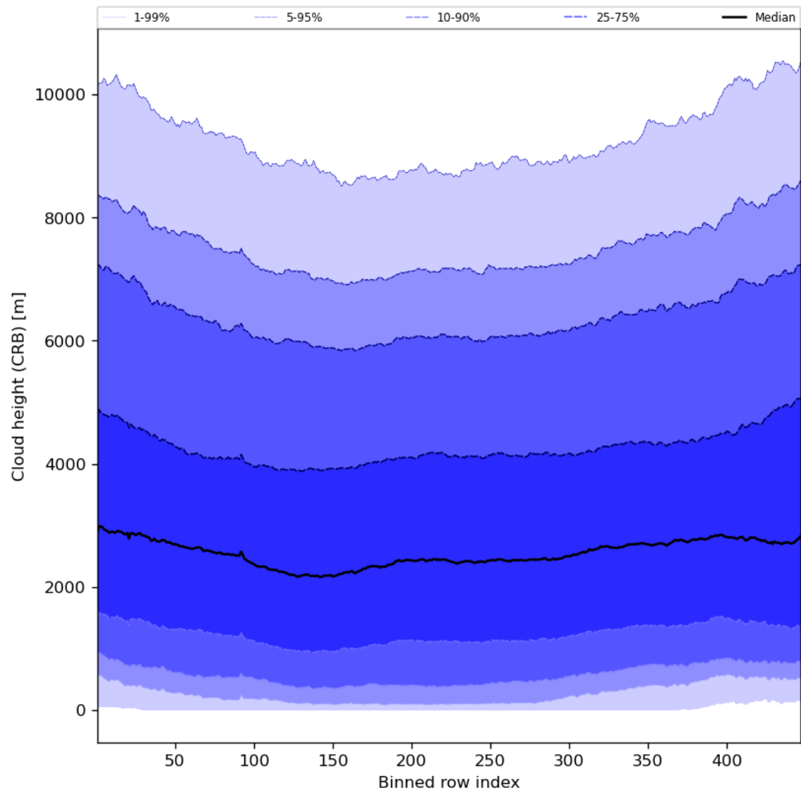
Figure 59: Along track statistics of “Cloud height (CRB)” for 2023-12-04 to 2023-12-06
