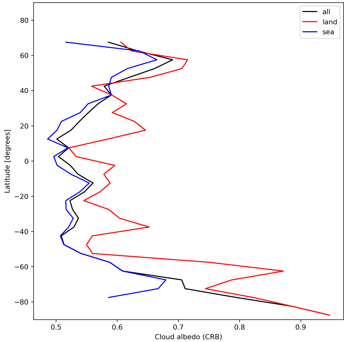
Figure 28: Zonal average of “Cloud albedo (CRB)” for 2023-12-04 to 2023-12-06.
