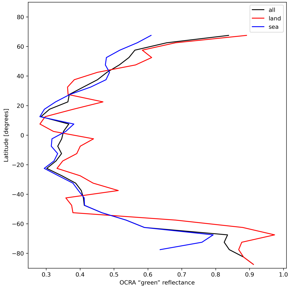
Figure 36: Zonal average of “OCRA “green” reflectance” for 2023-12-04 to 2023-12-06.
