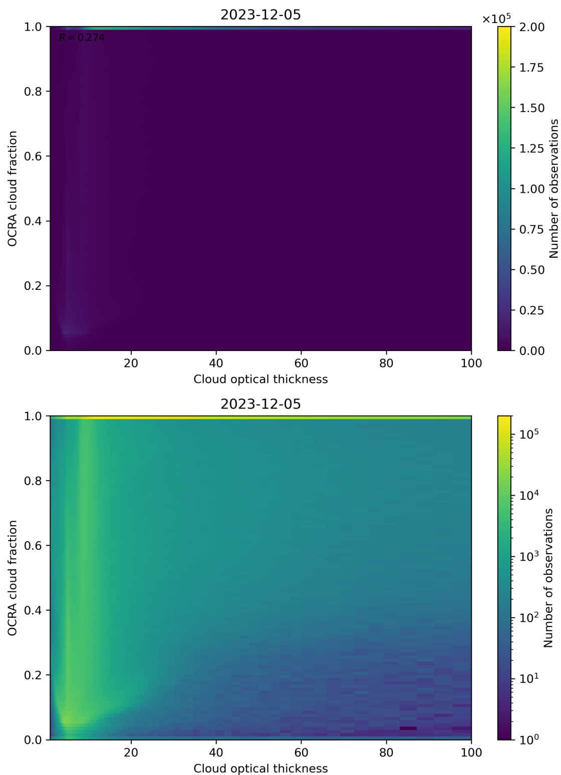
Figure 83: Scatter density plot of “Cloud optical thickness” against “OCRA cloud fraction” for 2023-12-04 to 2023-12-06.
