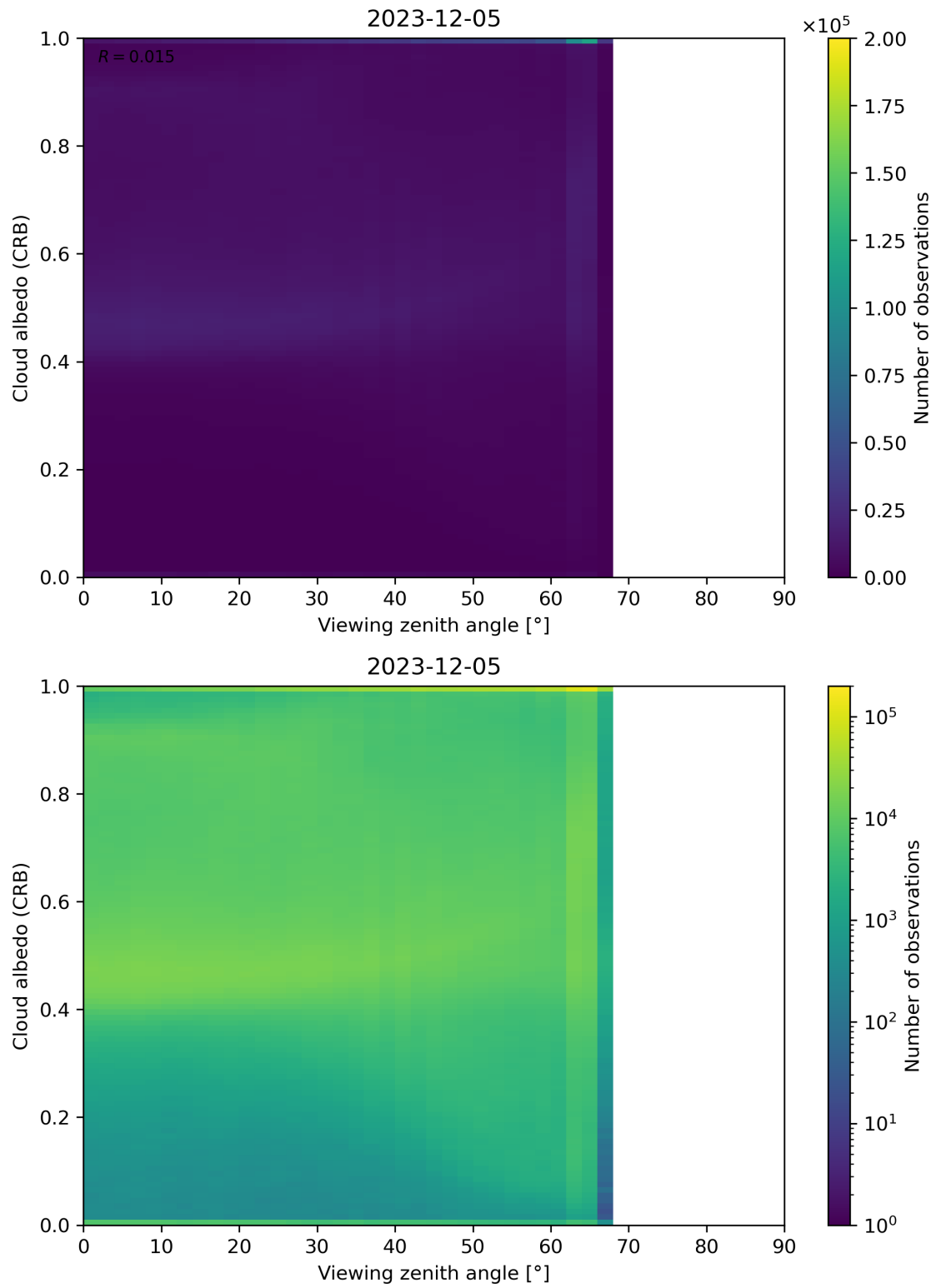
Figure 106: Scatter density plot of “Viewing zenith angle” against “Cloud albedo (CRB)” for 2023-12-04 to 2023-12-06.
