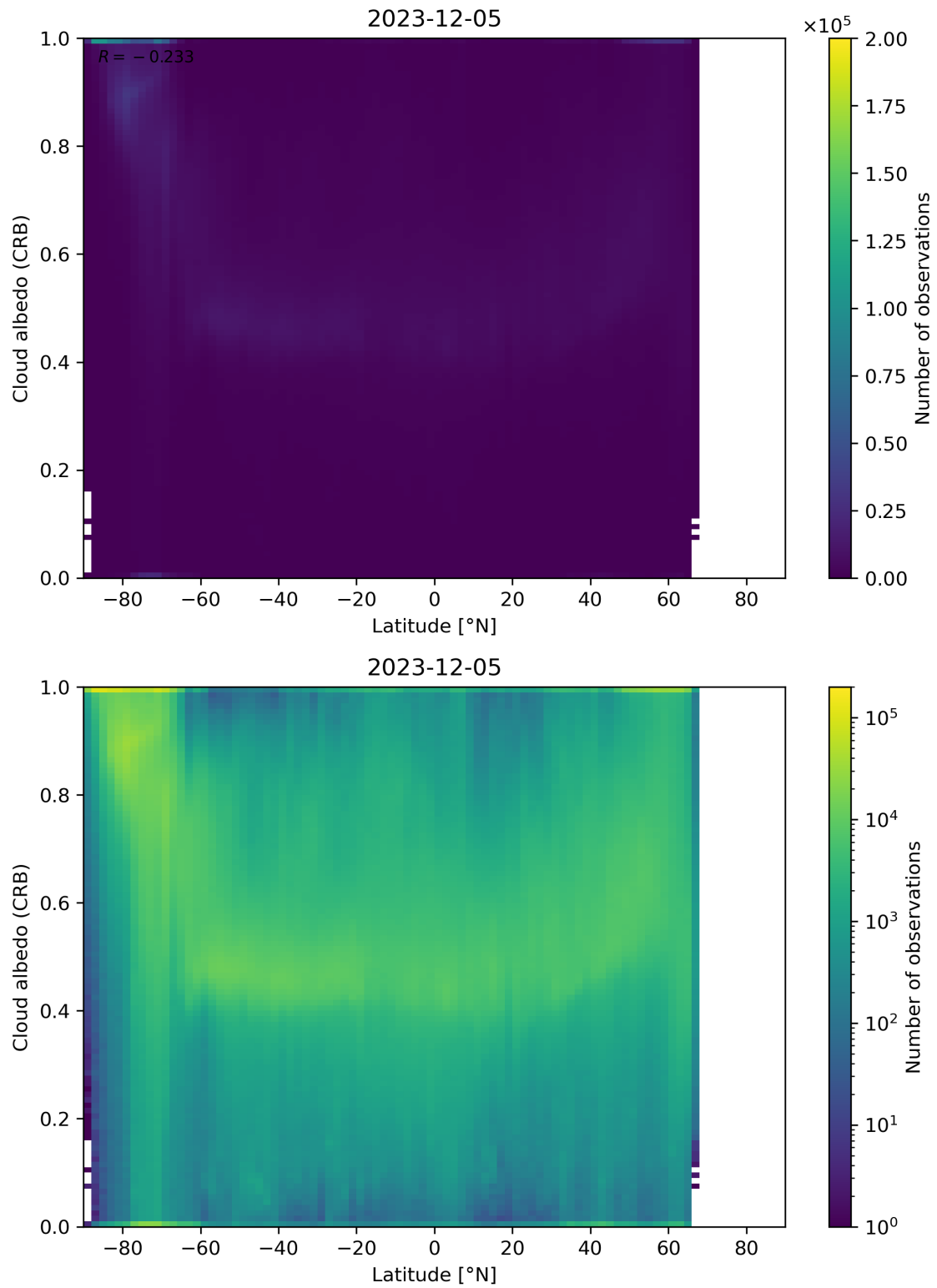
Figure 91: Scatter density plot of “Latitude” against “Cloud albedo (CRB)” for 2023-12-04 to 2023-12-06.
