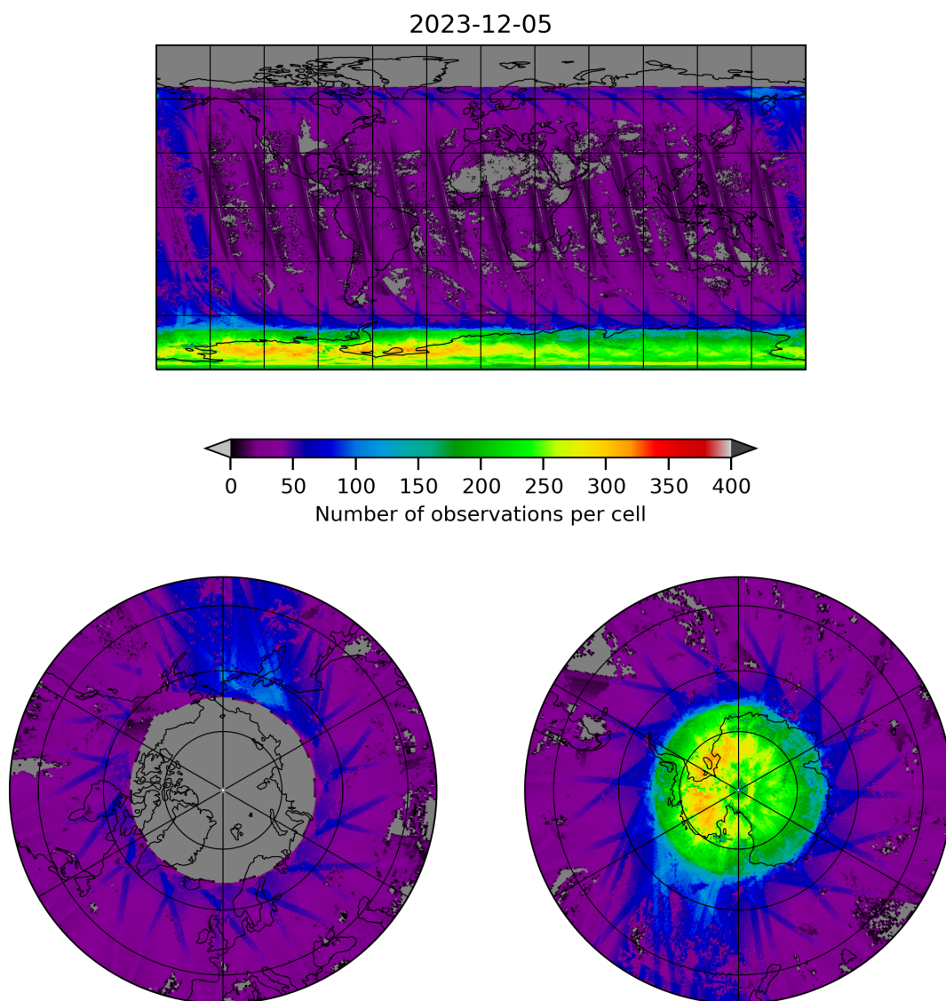
Figure 21: Map of the number of observations for 2023-12-04 to 2023-12-06
