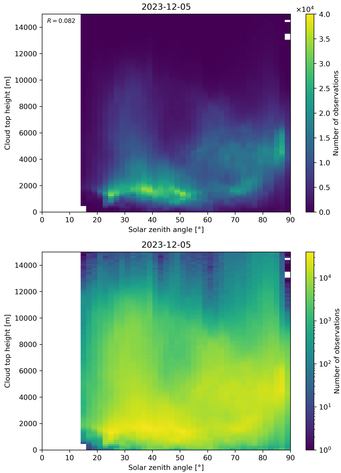
Figure 104: Scatter density plot of “Solar zenith angle” against “Cloud top height” for 2023-12-04 to 2023-12-06.
