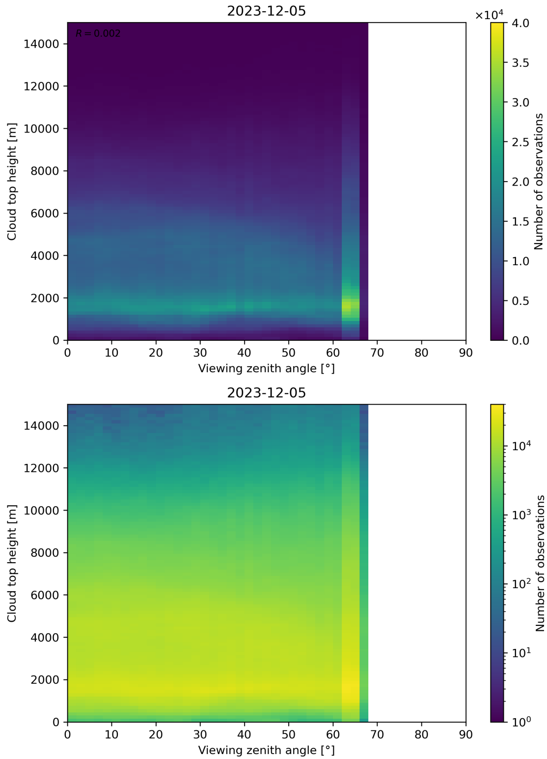
Figure 112: Scatter density plot of “Viewing zenith angle” against “Cloud top height” for 2023-12-04 to 2023-12-06.
