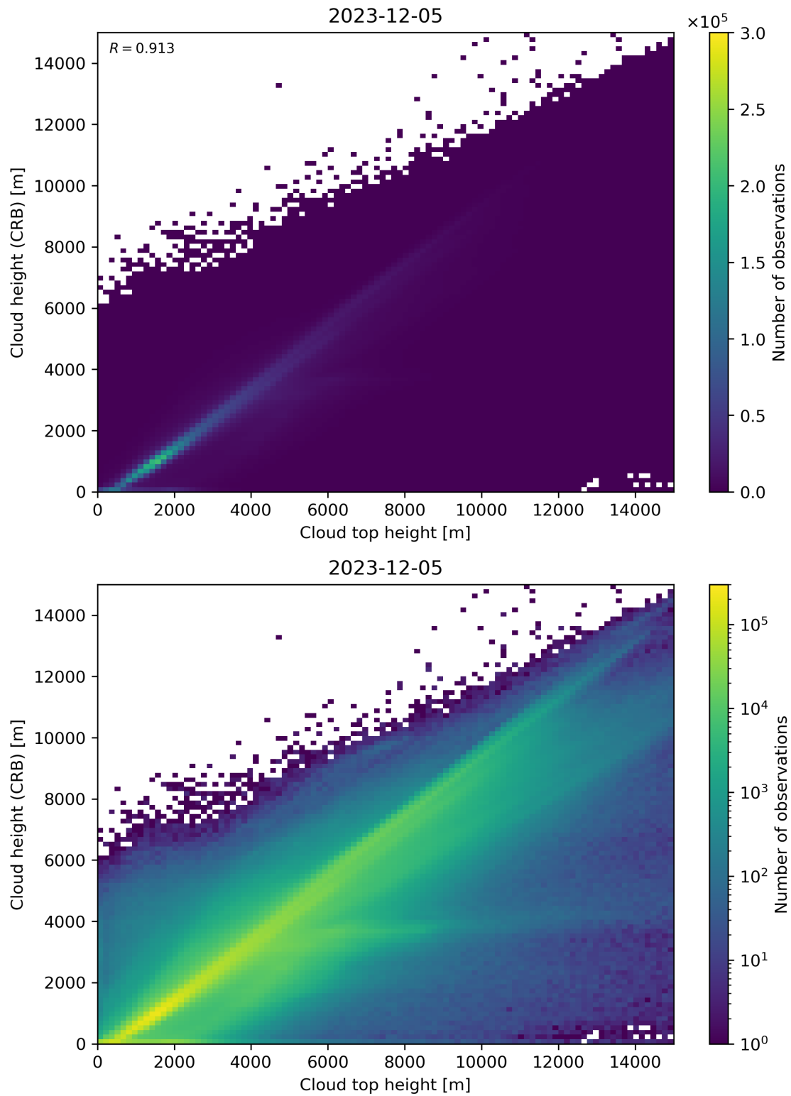
Figure 89: Scatter density plot of “Cloud top height” against “Cloud height (CRB)” for 2023-12-04 to 2023-12-06.
