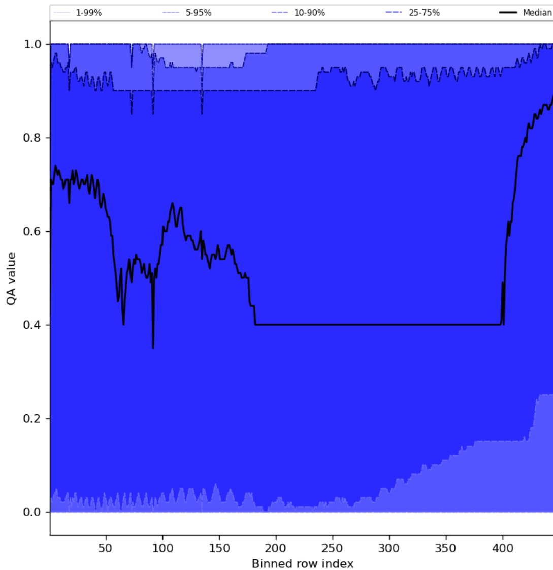
Figure 54: Along track statistics of “QA value” for 2023-12-04 to 2023-12-06
