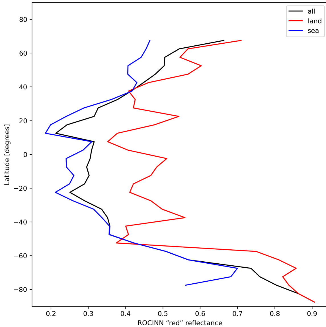
Figure 37: Zonal average of “ROCINN “red” reflectance” for 2023-12-04 to 2023-12-06.
