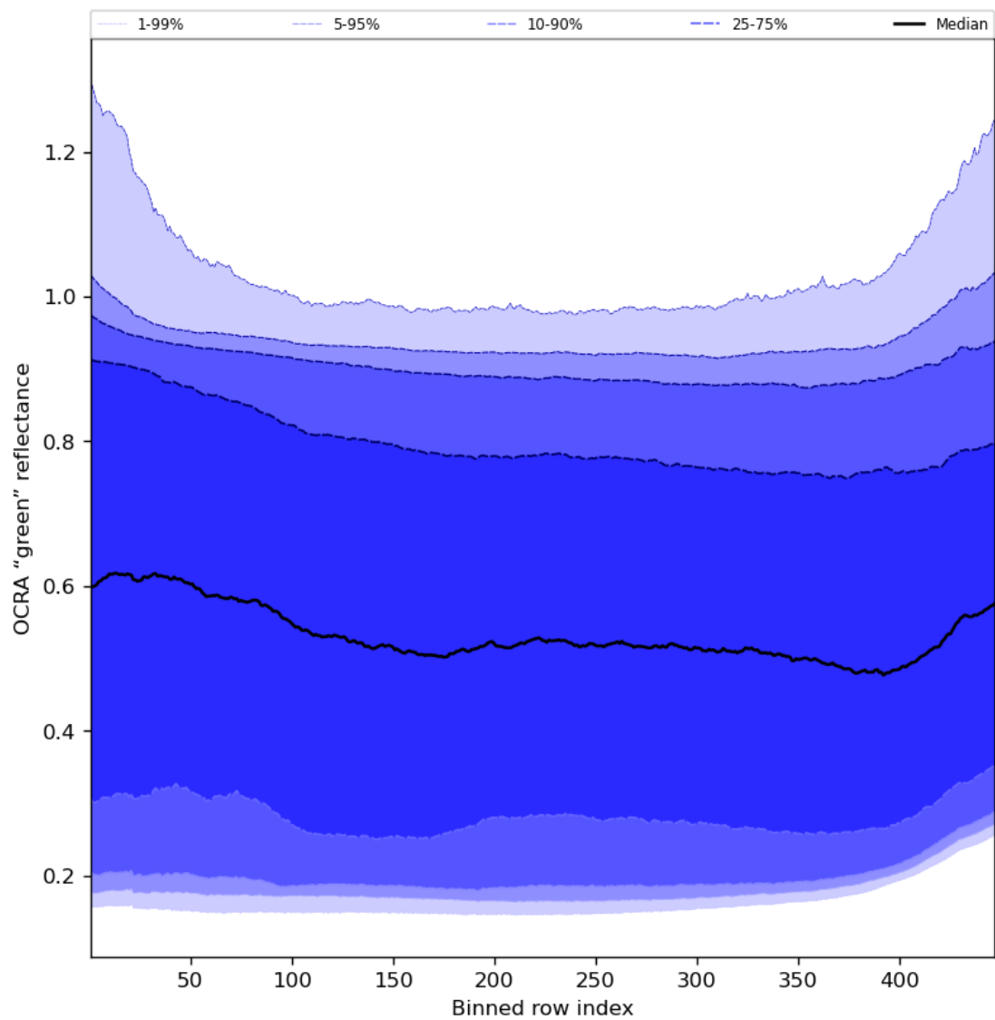
Figure 68: Along track statistics of “OCRA “green” reflectance” for 2023-12-04 to 2023-12-06
