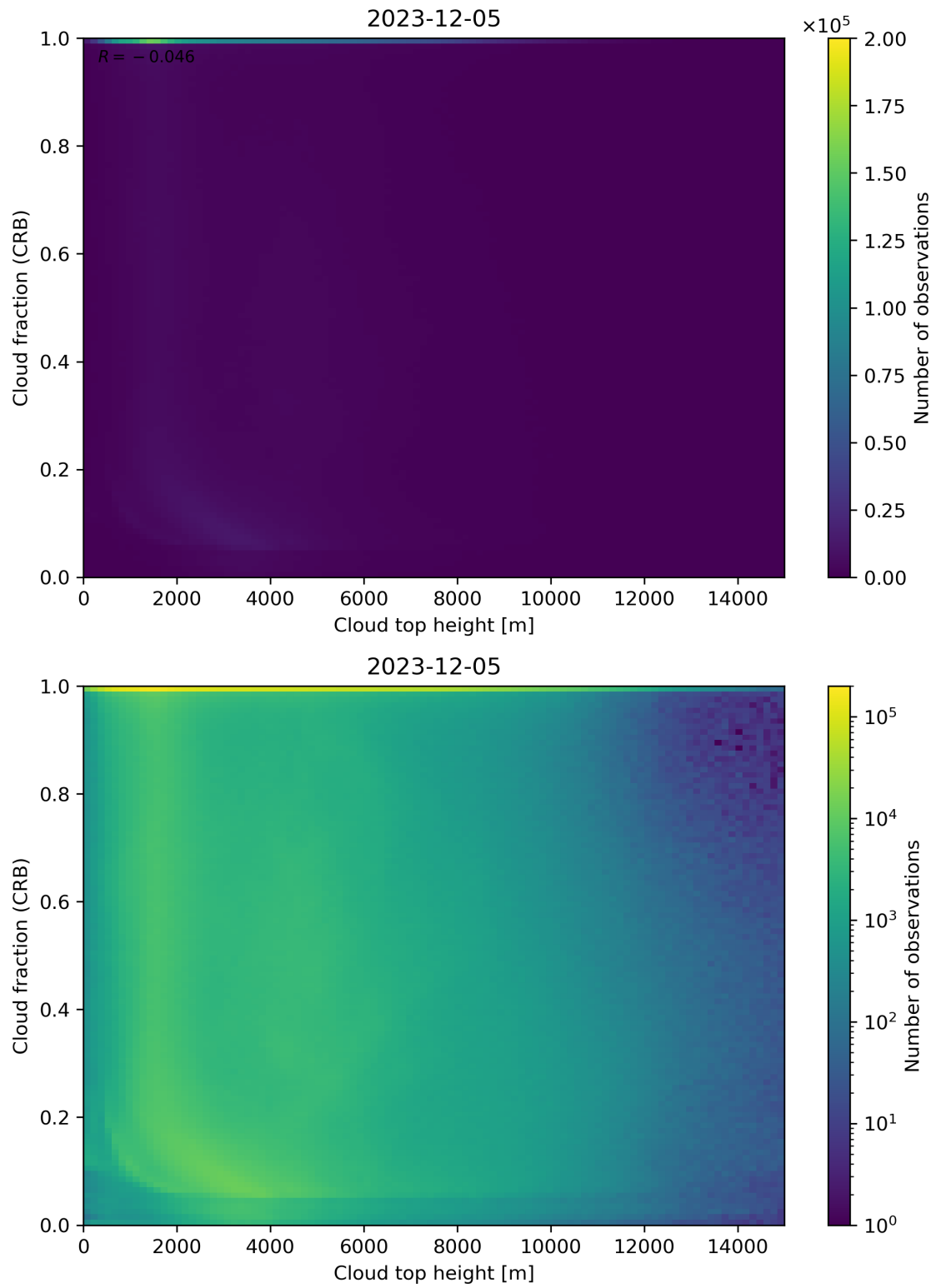
Figure 88: Scatter density plot of “Cloud top height” against “Cloud fraction (CRB)” for 2023-12-04 to 2023-12-06.
