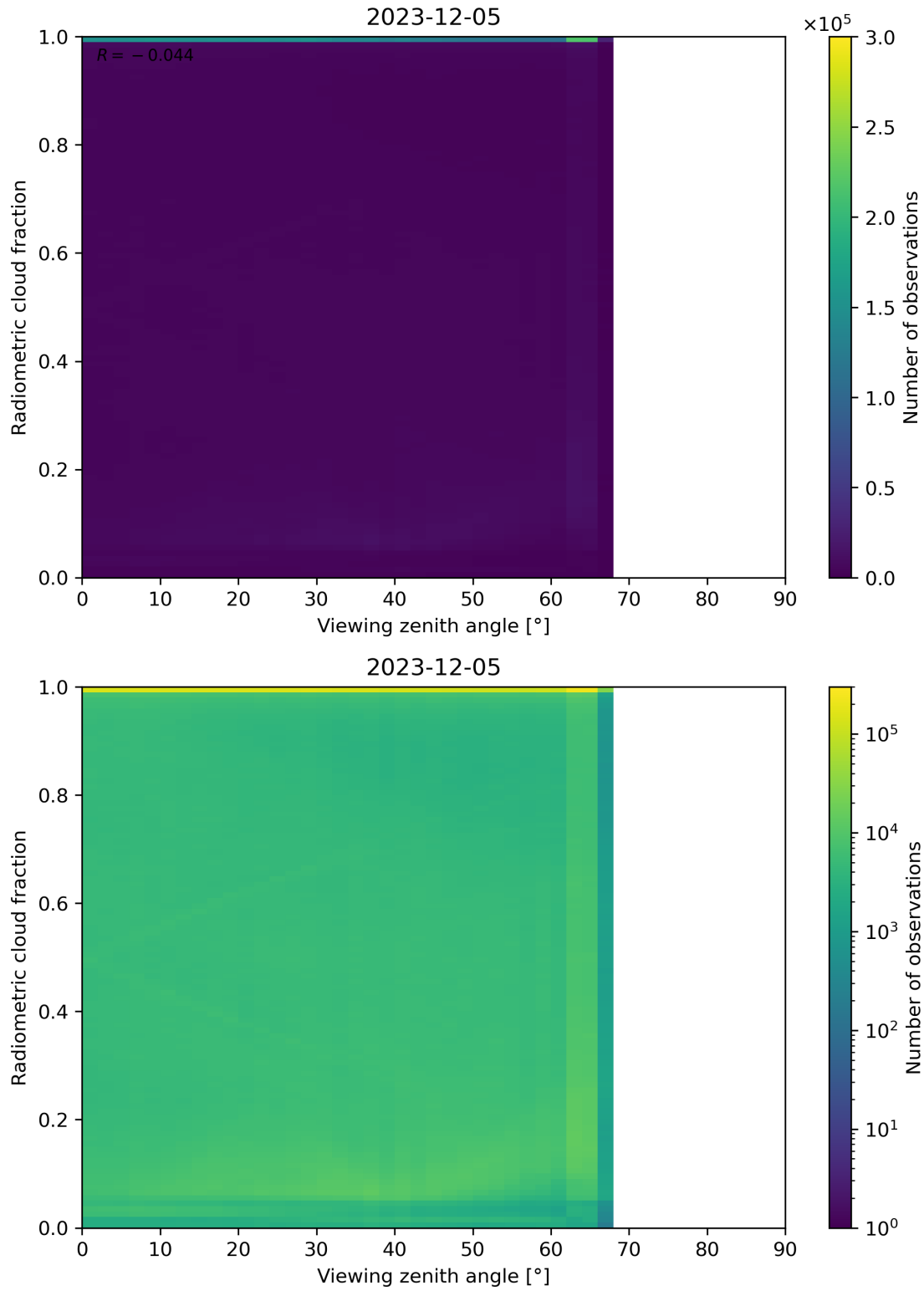
Figure 107: Scatter density plot of “Viewing zenith angle” against “Radiometric cloud fraction” for 2023-12-04 to 2023-12-06.
