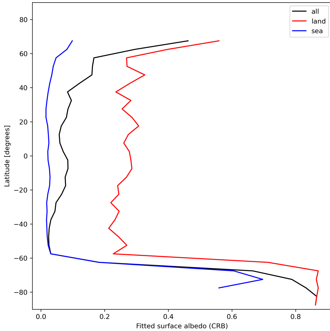
Figure 30: Zonal average of “Fitted surface albedo (CRB)” for 2023-12-04 to 2023-12-06.
