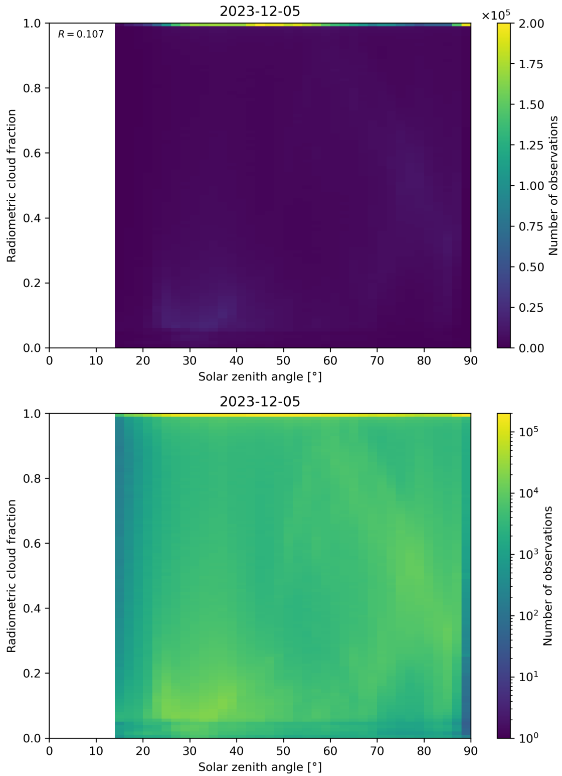
Figure 99: Scatter density plot of “Solar zenith angle” against “Radiometric cloud fraction” for 2023-12-04 to 2023-12-06.
