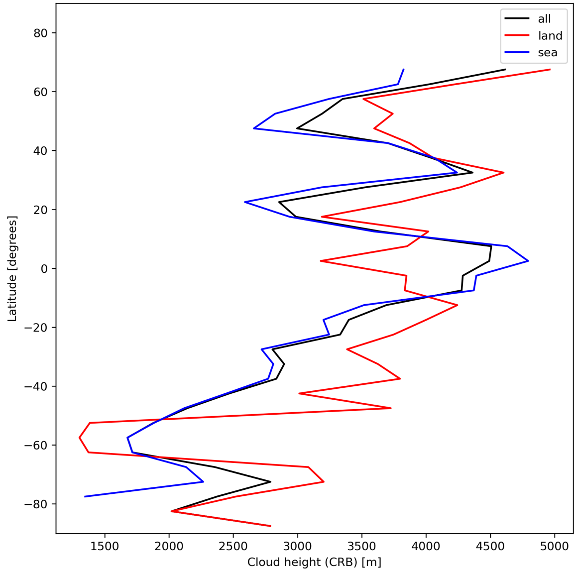
Figure 27: Zonal average of “Cloud height (CRB)” for 2023-12-04 to 2023-12-06.
