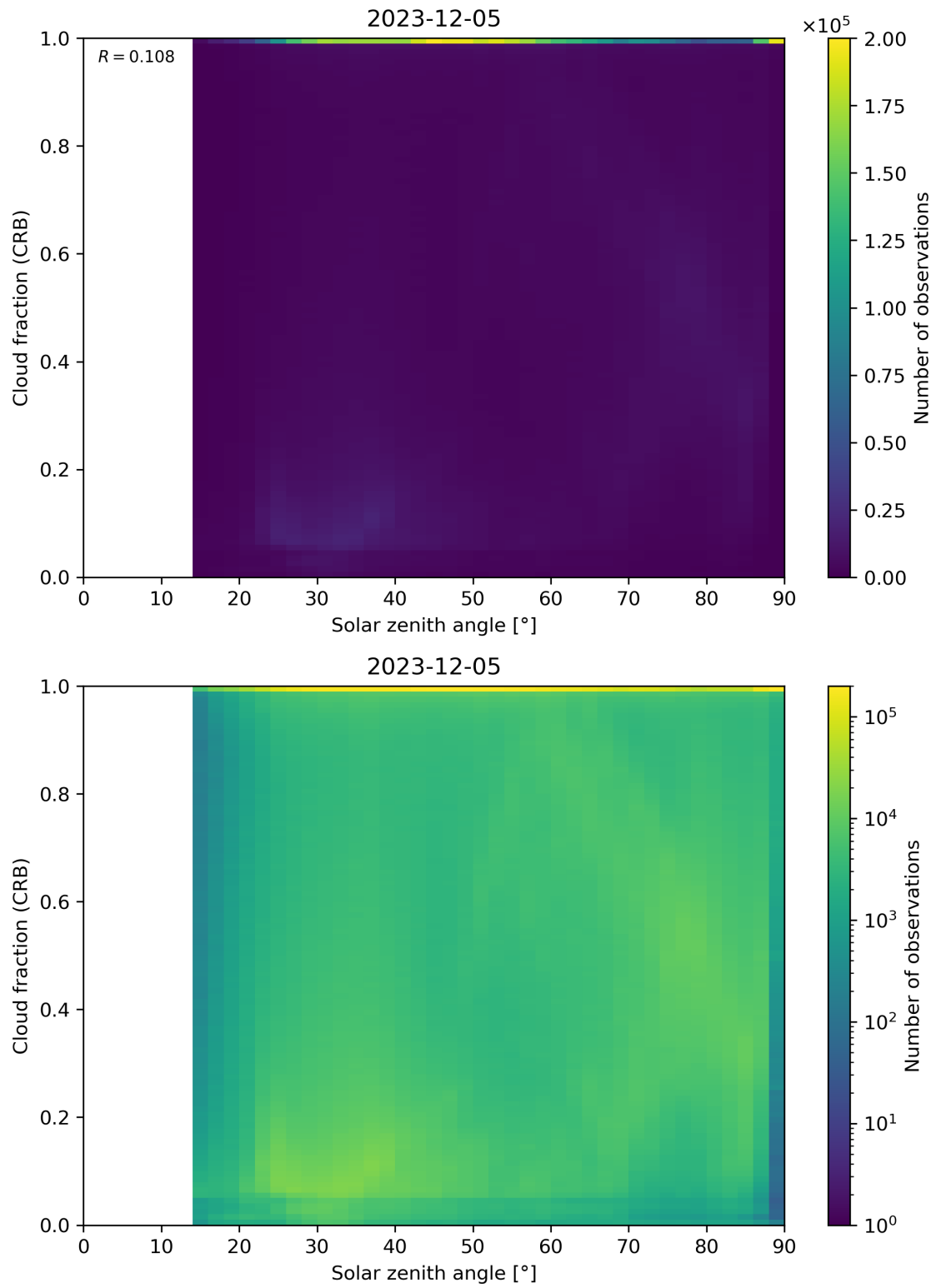
Figure 101: Scatter density plot of “Solar zenith angle” against “Cloud fraction (CRB)” for 2023-12-04 to 2023-12-06.
