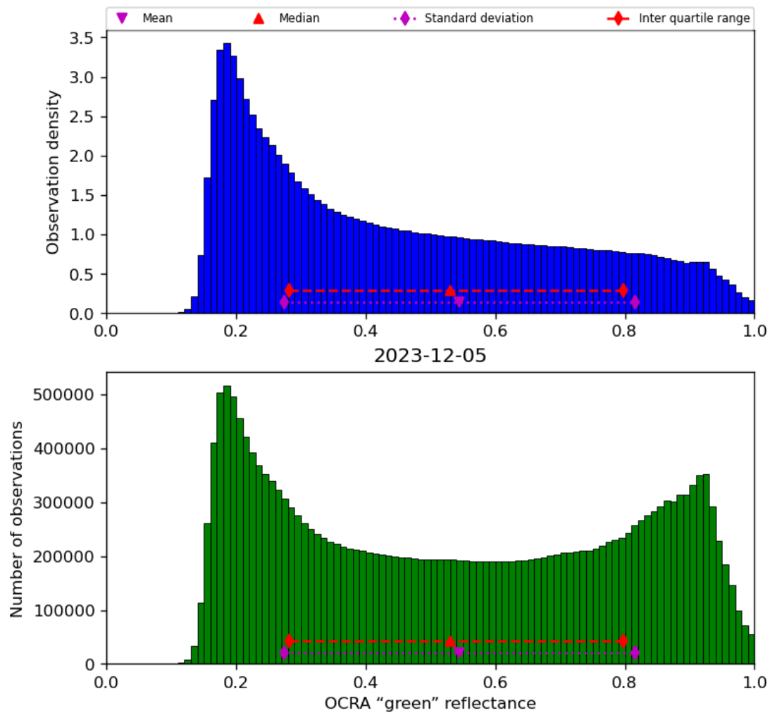
Figure 52: Histogram of “OCRA “green” reflectance” for 2023-12-04 to 2023-12-06
