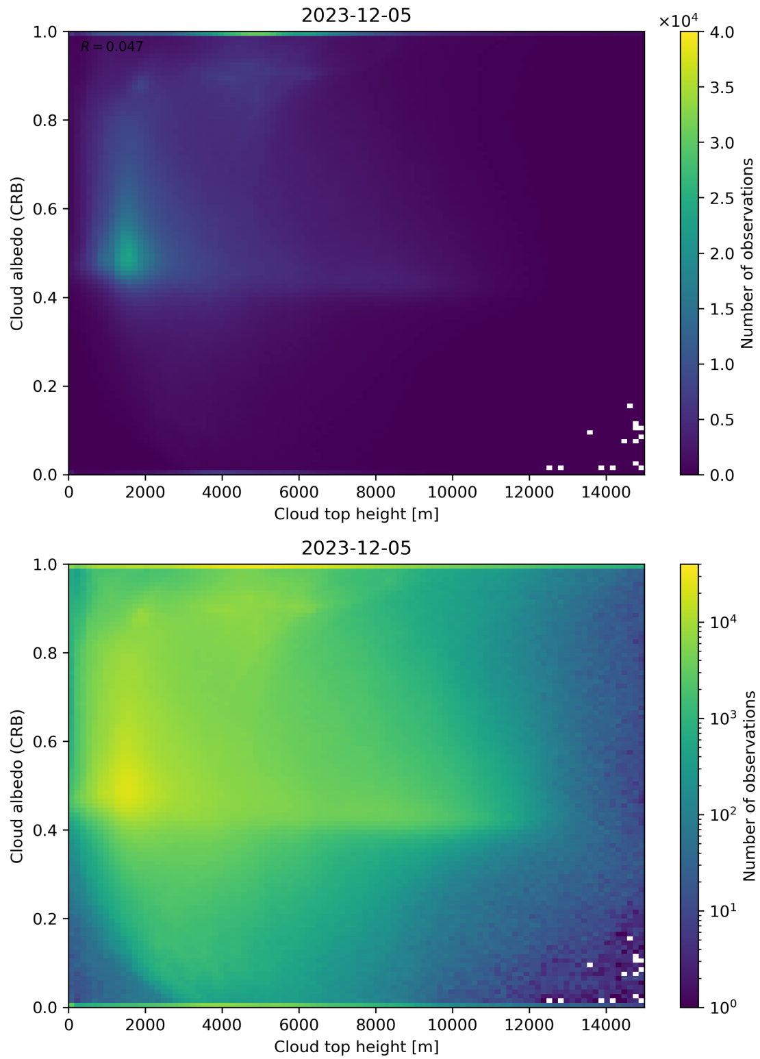
Figure 86: Scatter density plot of “Cloud top height” against “Cloud albedo (CRB)” for 2023-12-04 to 2023-12-06.
