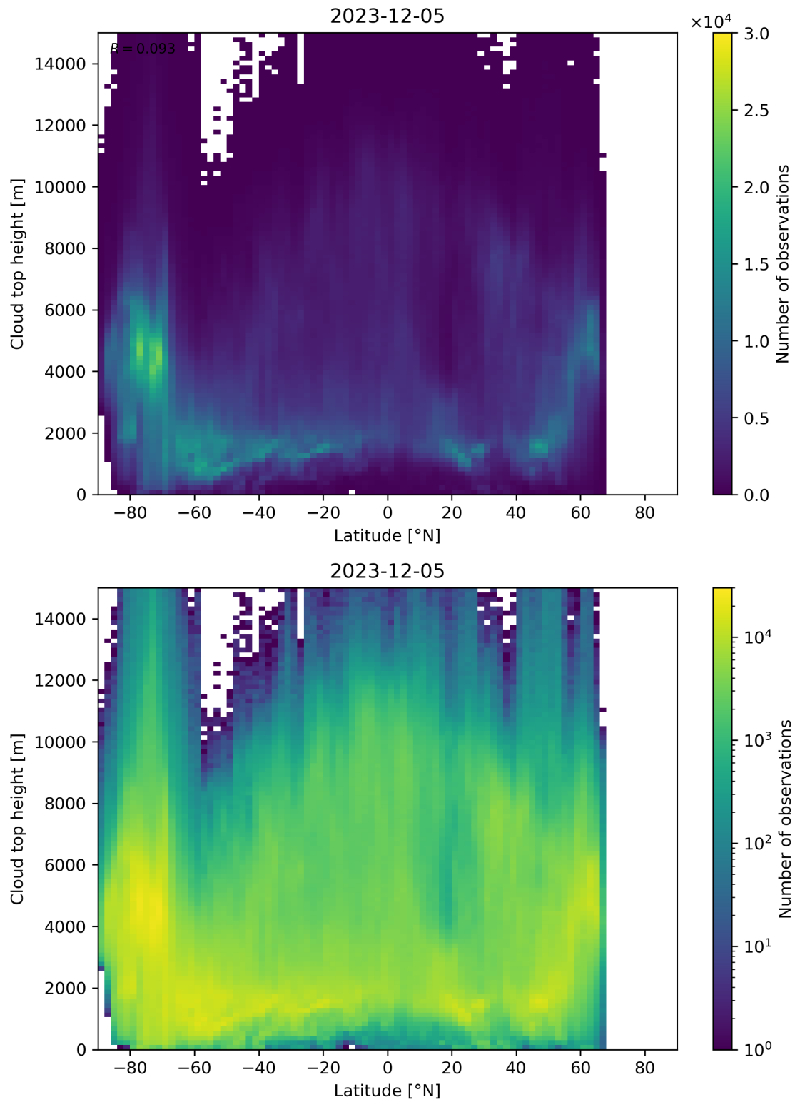
Figure 97: Scatter density plot of “Latitude” against “Cloud top height” for 2023-12-04 to 2023-12-06.
