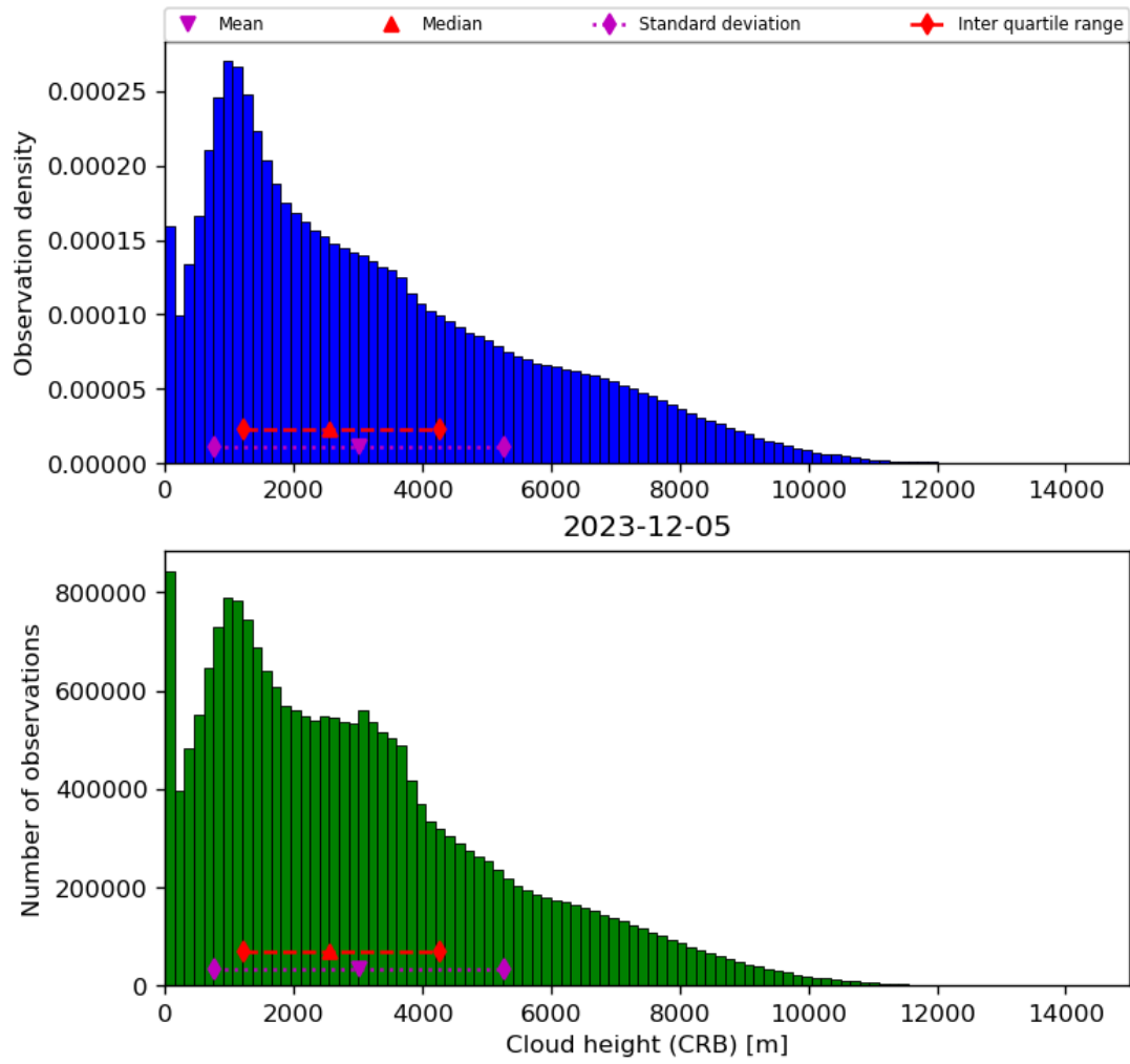
Figure 43: Histogram of “Cloud height (CRB)” for 2023-12-04 to 2023-12-06
