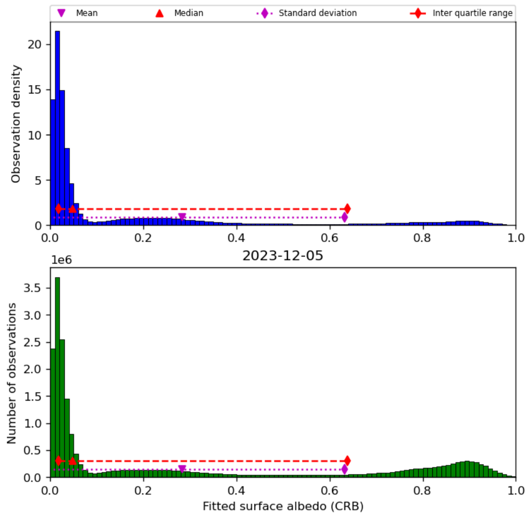
Figure 46: Histogram of “Fitted surface albedo (CRB)” for 2023-12-04 to 2023-12-06
