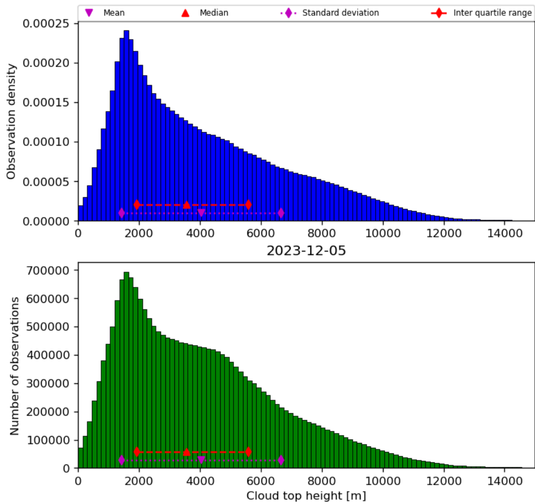
Figure 40: Histogram of “Cloud top height” for 2023-12-04 to 2023-12-06
