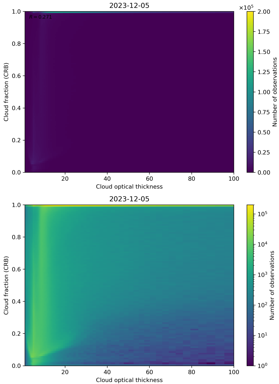
Figure 84: Scatter density plot of “Cloud optical thickness” against “Cloud fraction (CRB)” for 2023-12-04 to 2023-12-06.
