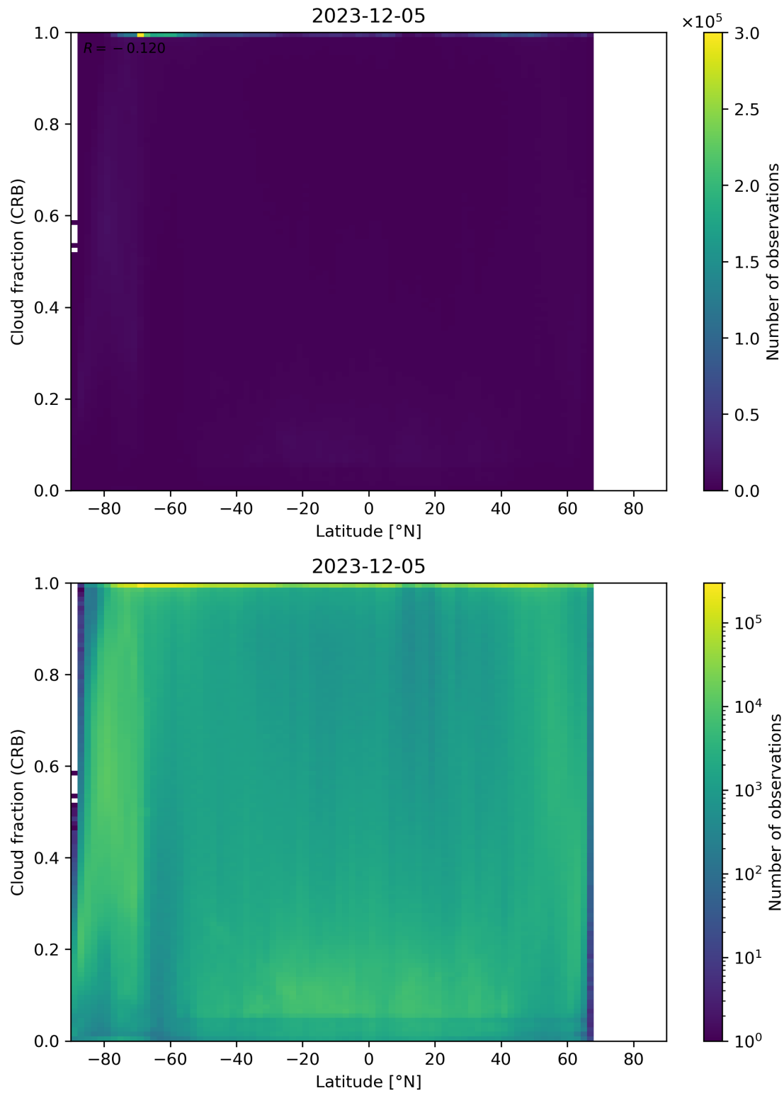
Figure 94: Scatter density plot of “Latitude” against “Cloud fraction (CRB)” for 2023-12-04 to 2023-12-06.
