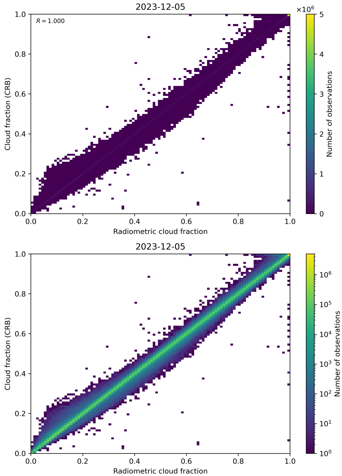
Figure 73: Scatter density plot of “Radiometric cloud fraction” against “Cloud fraction (CRB)” for 2023-12-04 to 2023-12-06.
