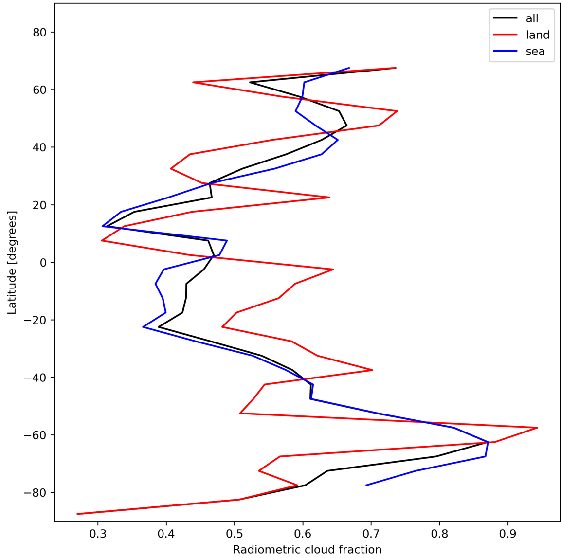
Figure 23: Zonal average of “Radiometric cloud fraction” for 2023-12-04 to 2023-12-06.
