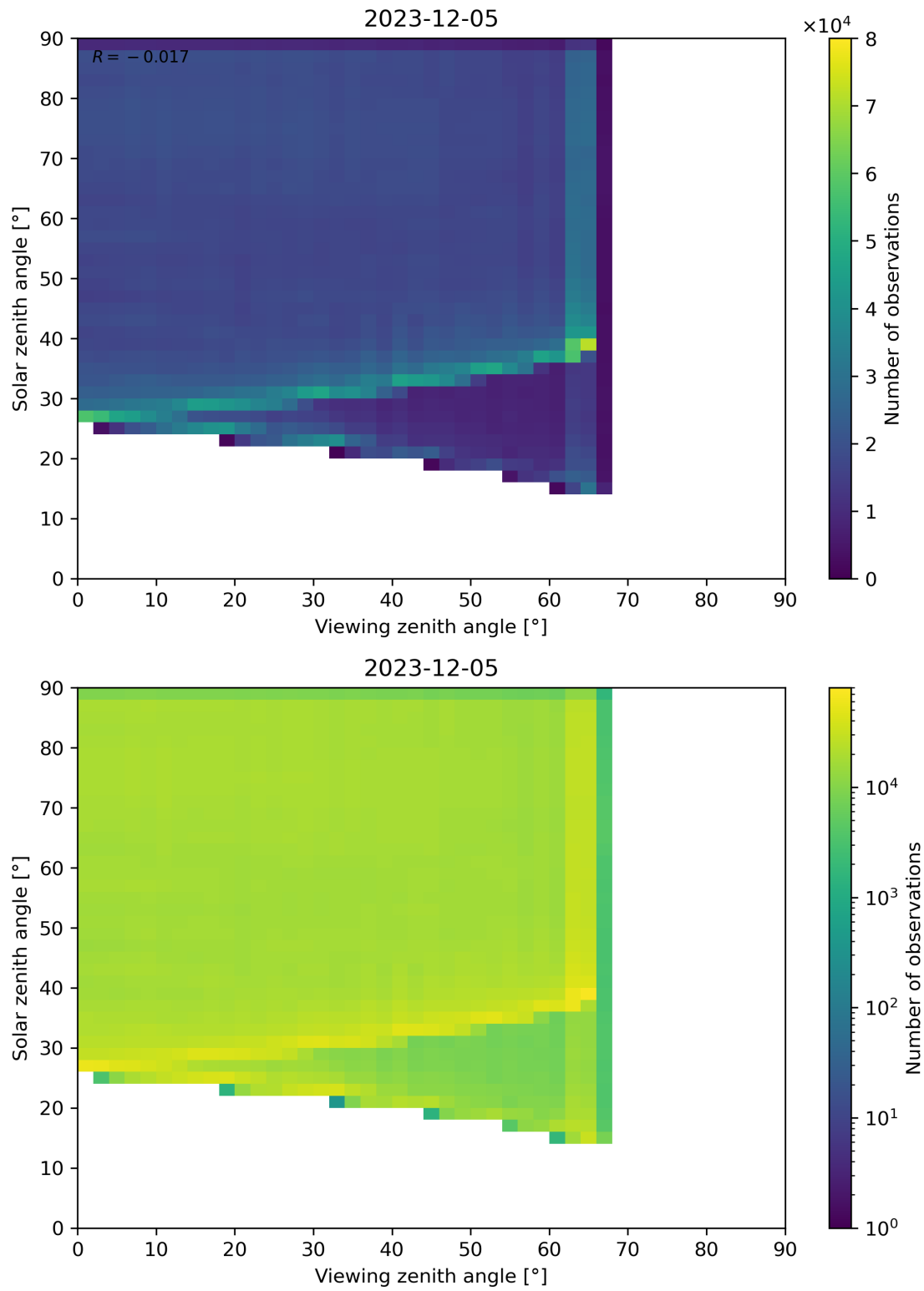
Figure 114: Scatter density plot of “Viewing zenith angle” against “Solar zenith angle” for 2023-12-04 to 2023-12-06.
