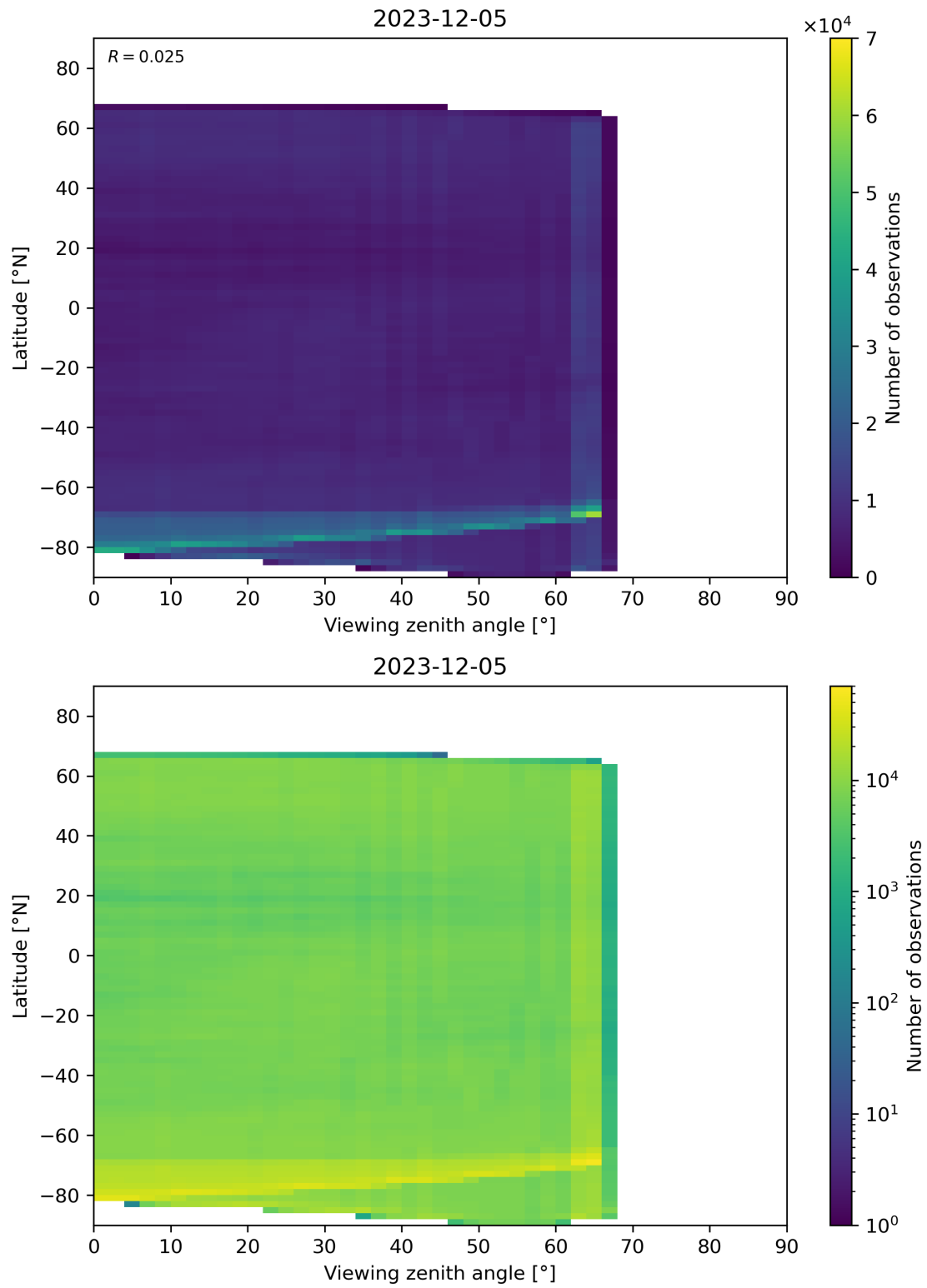
Figure 113: Scatter density plot of “Viewing zenith angle” against “Latitude” for 2023-12-04 to 2023-12-06.
