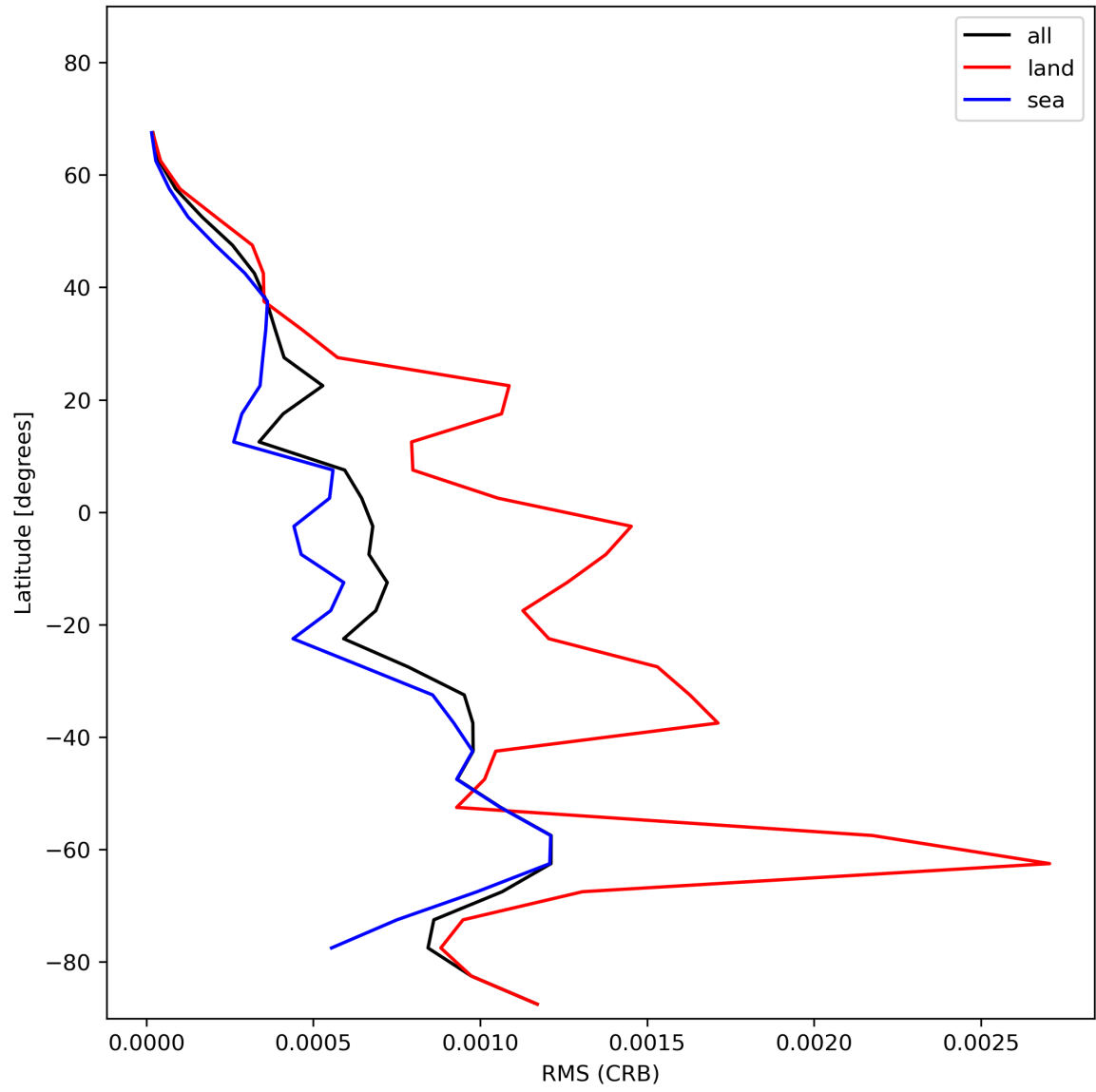
Figure 32: Zonal average of “RMS (CRB)” for 2023-12-04 to 2023-12-06.
