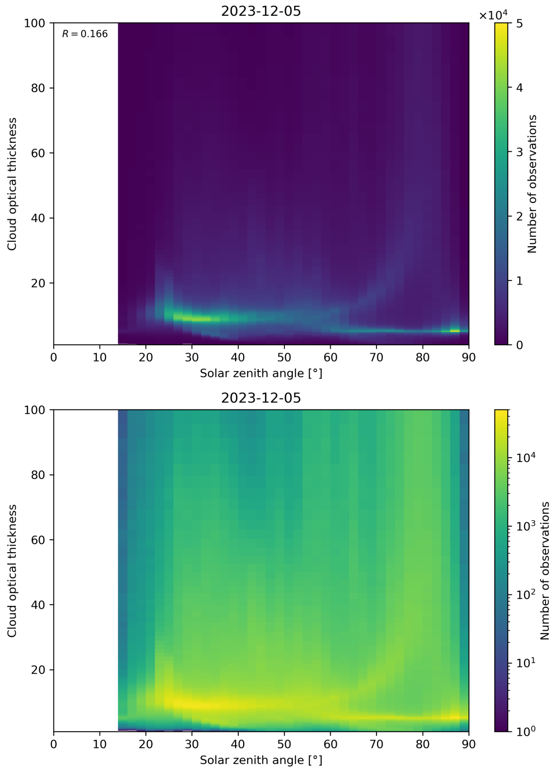
Figure 103: Scatter density plot of “Solar zenith angle” against “Cloud optical thickness” for 2023-12-04 to 2023-12-06.
