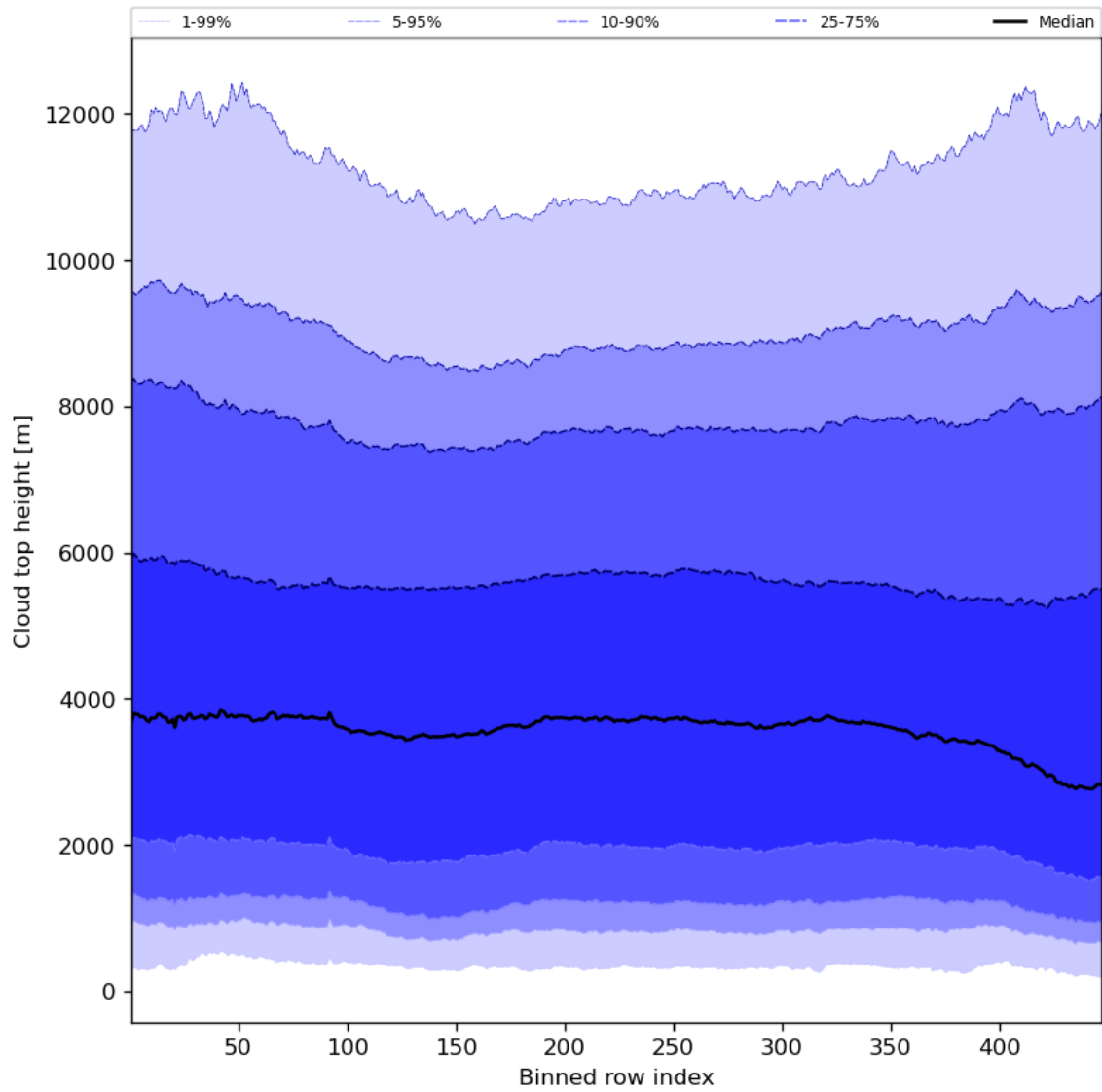
Figure 56: Along track statistics of “Cloud top height” for 2023-12-04 to 2023-12-06
