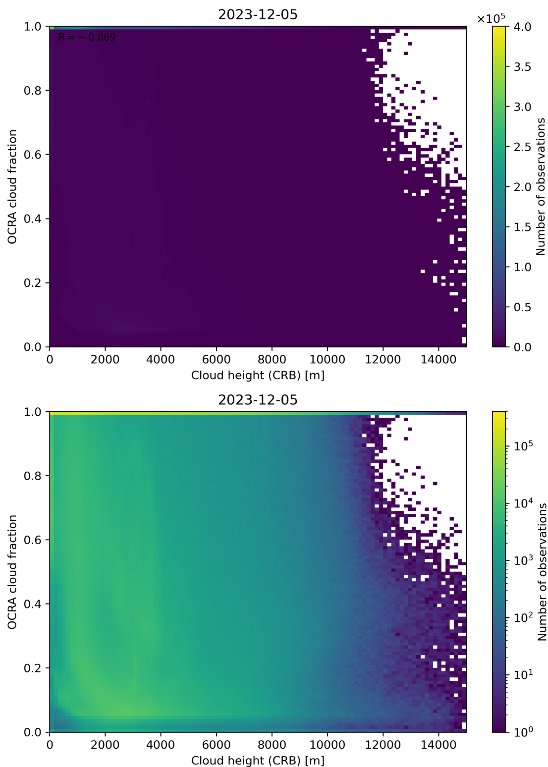
Figure 81: Scatter density plot of “Cloud height (CRB)” against “OCRA cloud fraction” for 2023-12-04 to 2023-12-06.
