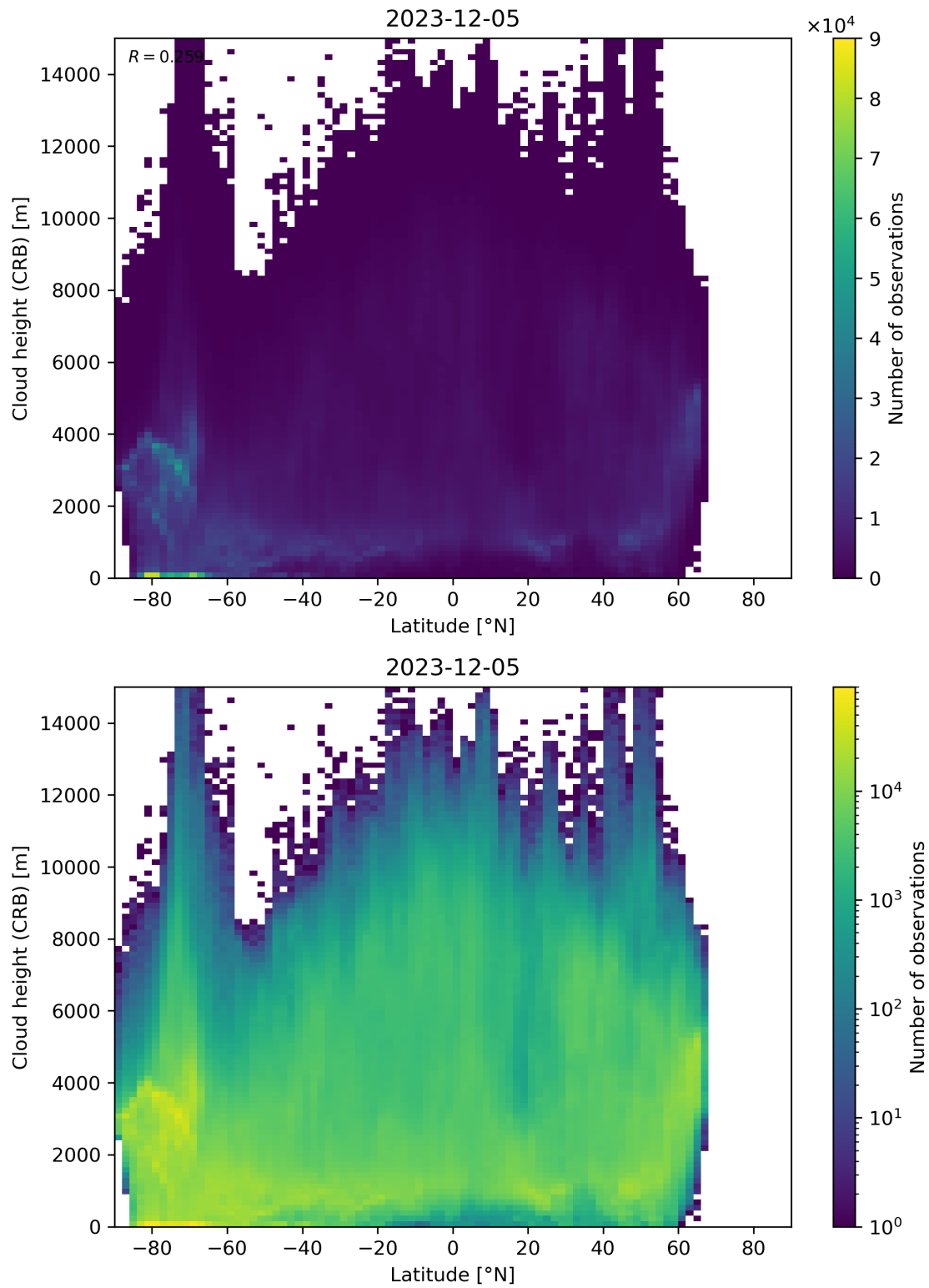
Figure 95: Scatter density plot of “Latitude” against “Cloud height (CRB)” for 2023-12-04 to 2023-12-06.
