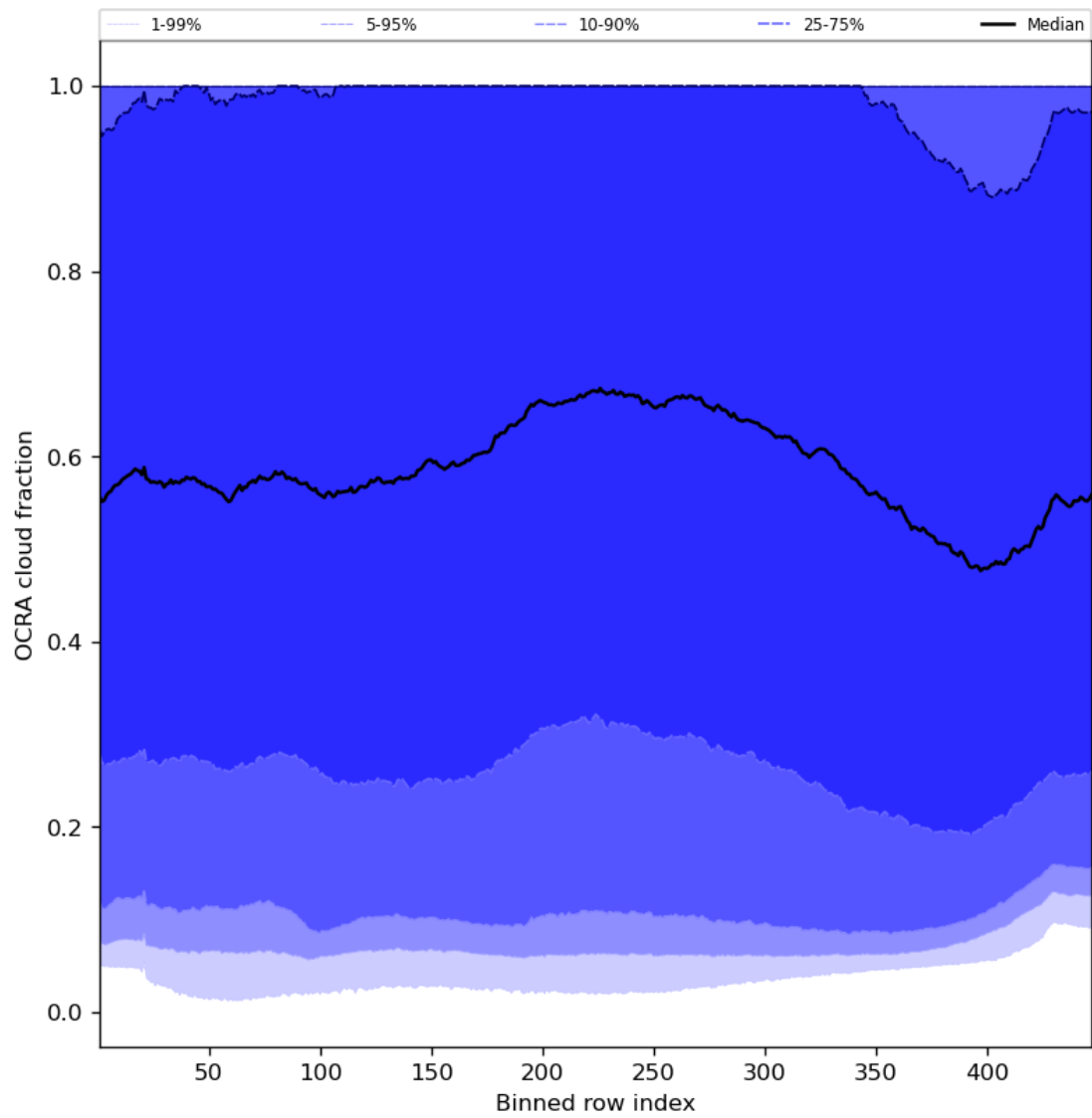
Figure 66: Along track statistics of “OCRA cloud fraction” for 2023-12-04 to 2023-12-06
