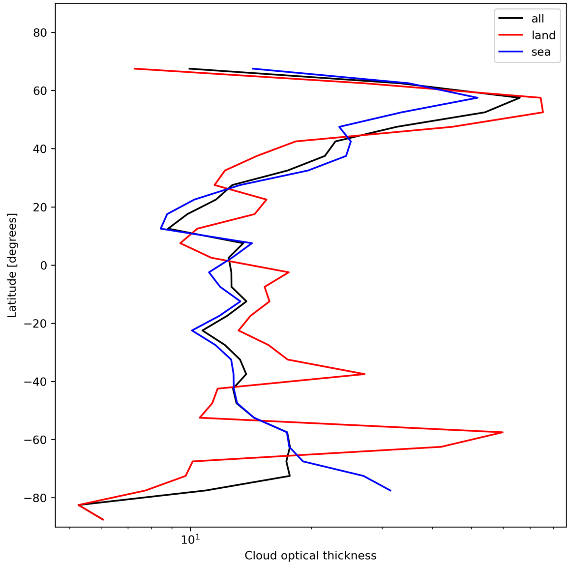
Figure 25: Zonal average of “Cloud optical thickness” for 2023-12-04 to 2023-12-06.
