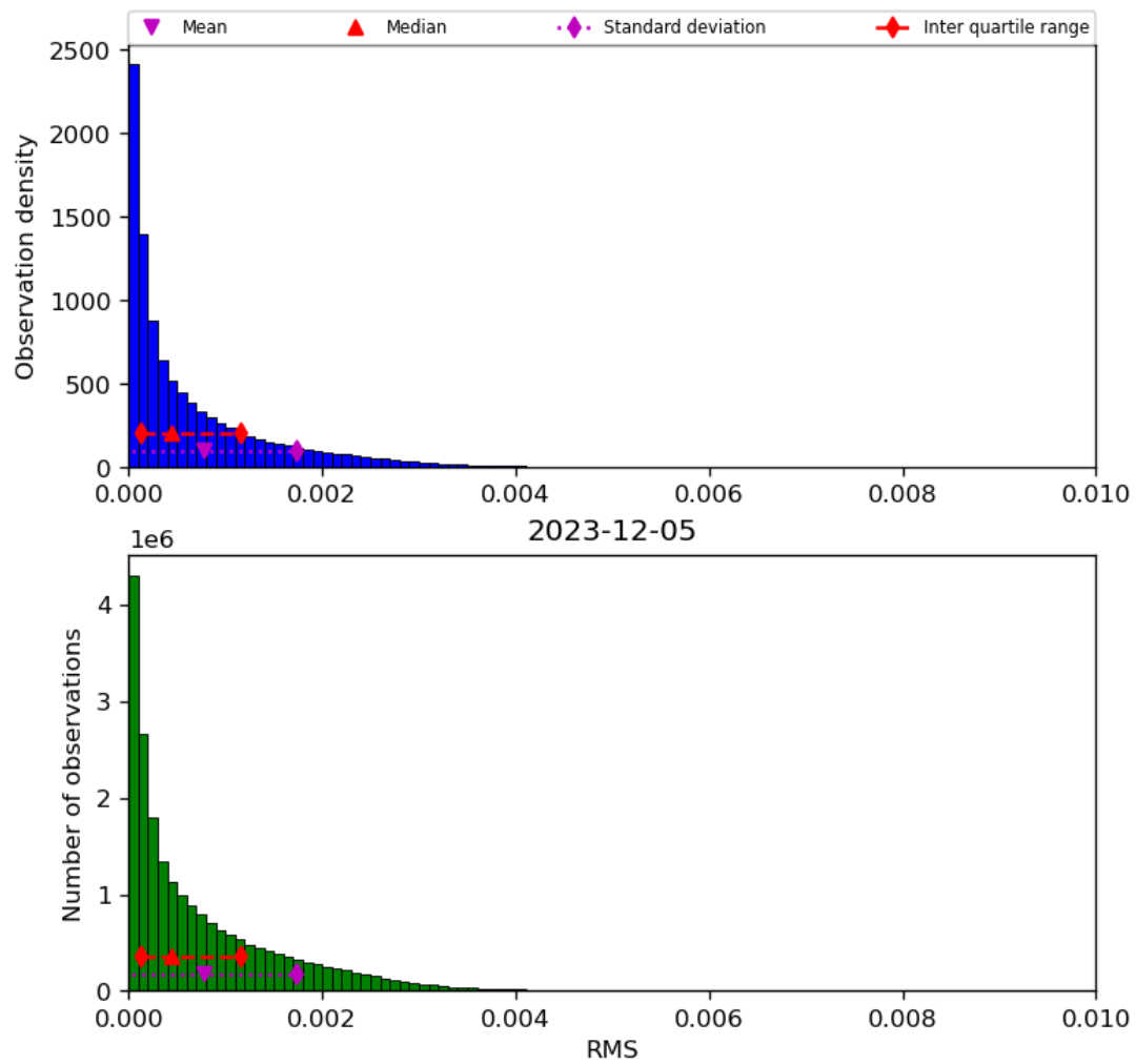
Figure 47: Histogram of “RMS” for 2023-12-04 to 2023-12-06
