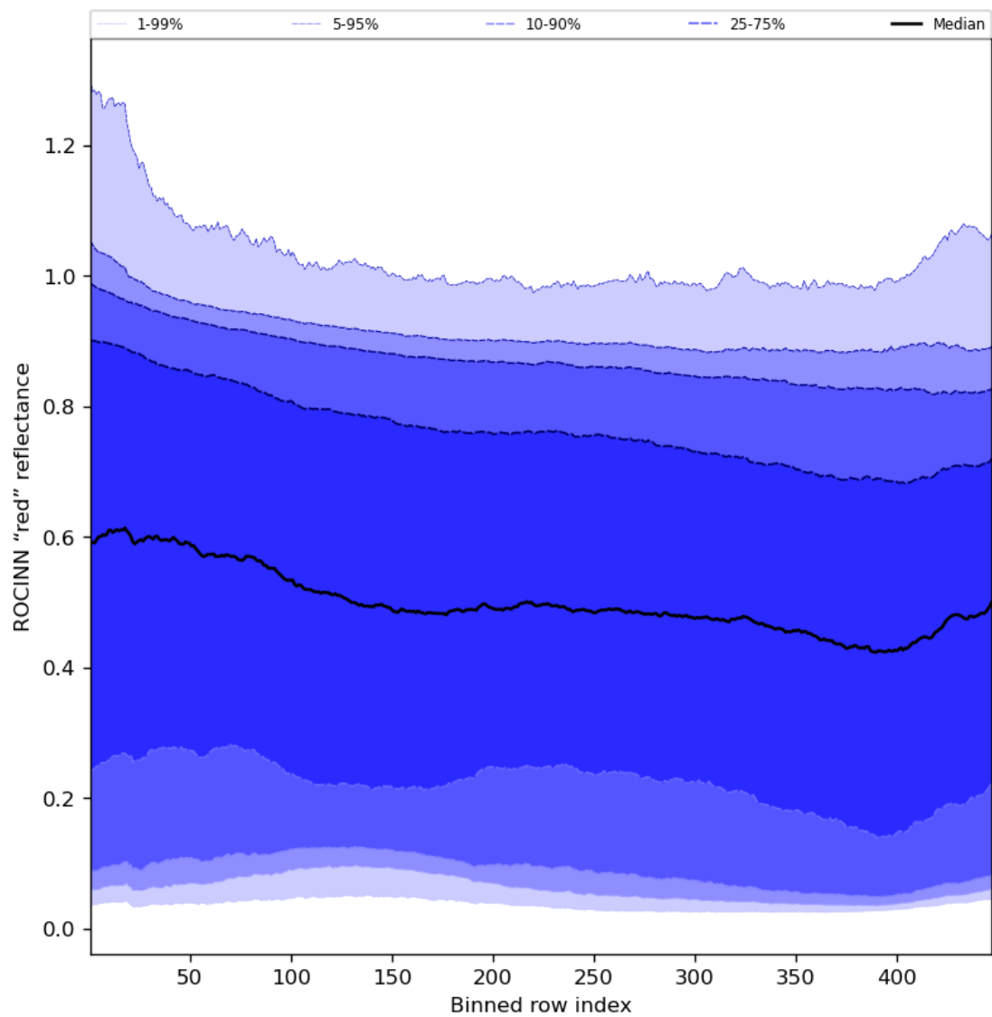
Figure 69: Along track statistics of "ROCINN "red" reflectance" for 2023-12-04 to 2023-12-06
