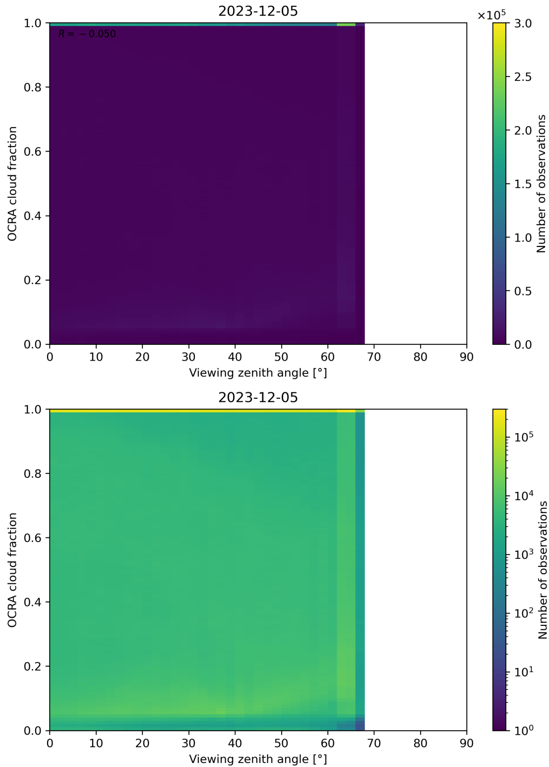
Figure 108: Scatter density plot of “Viewing zenith angle” against “OCRA cloud fraction” for 2023-12-04 to 2023-12-06.
