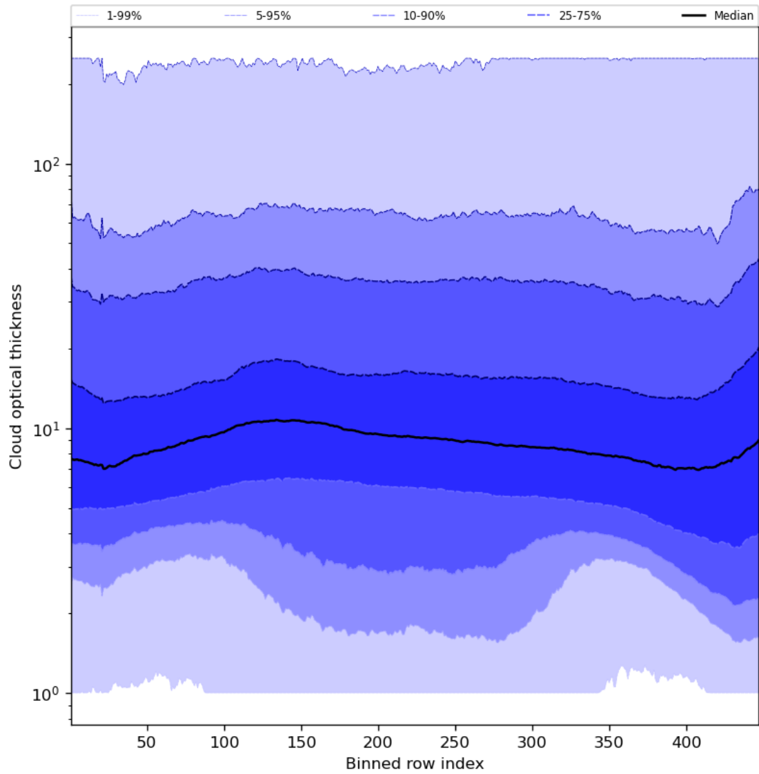
Figure 57: Along track statistics of “Cloud optical thickness” for 2023-12-04 to 2023-12-06
