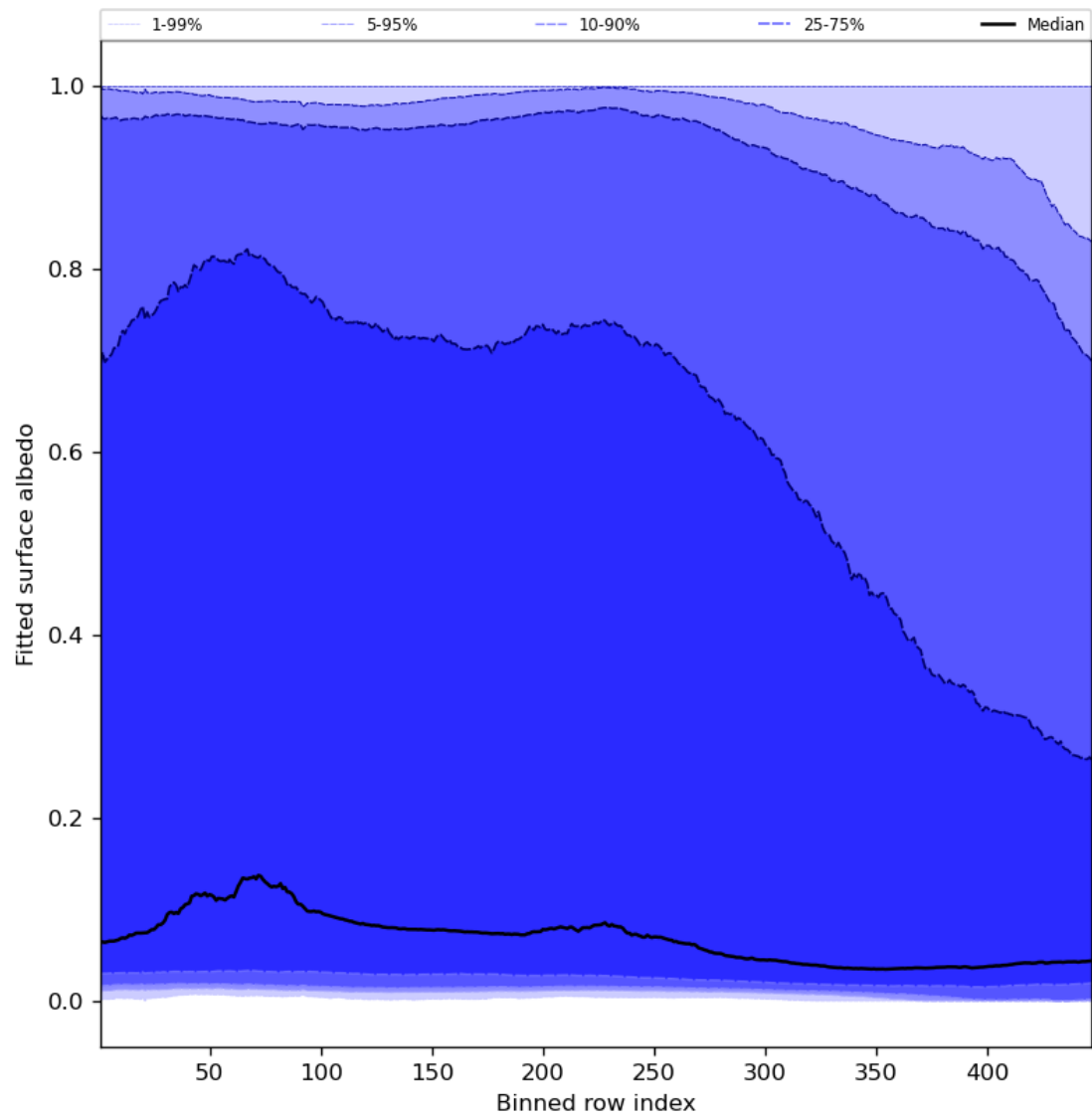
Figure 61: Along track statistics of “Fitted surface albedo” for 2023-12-04 to 2023-12-06
