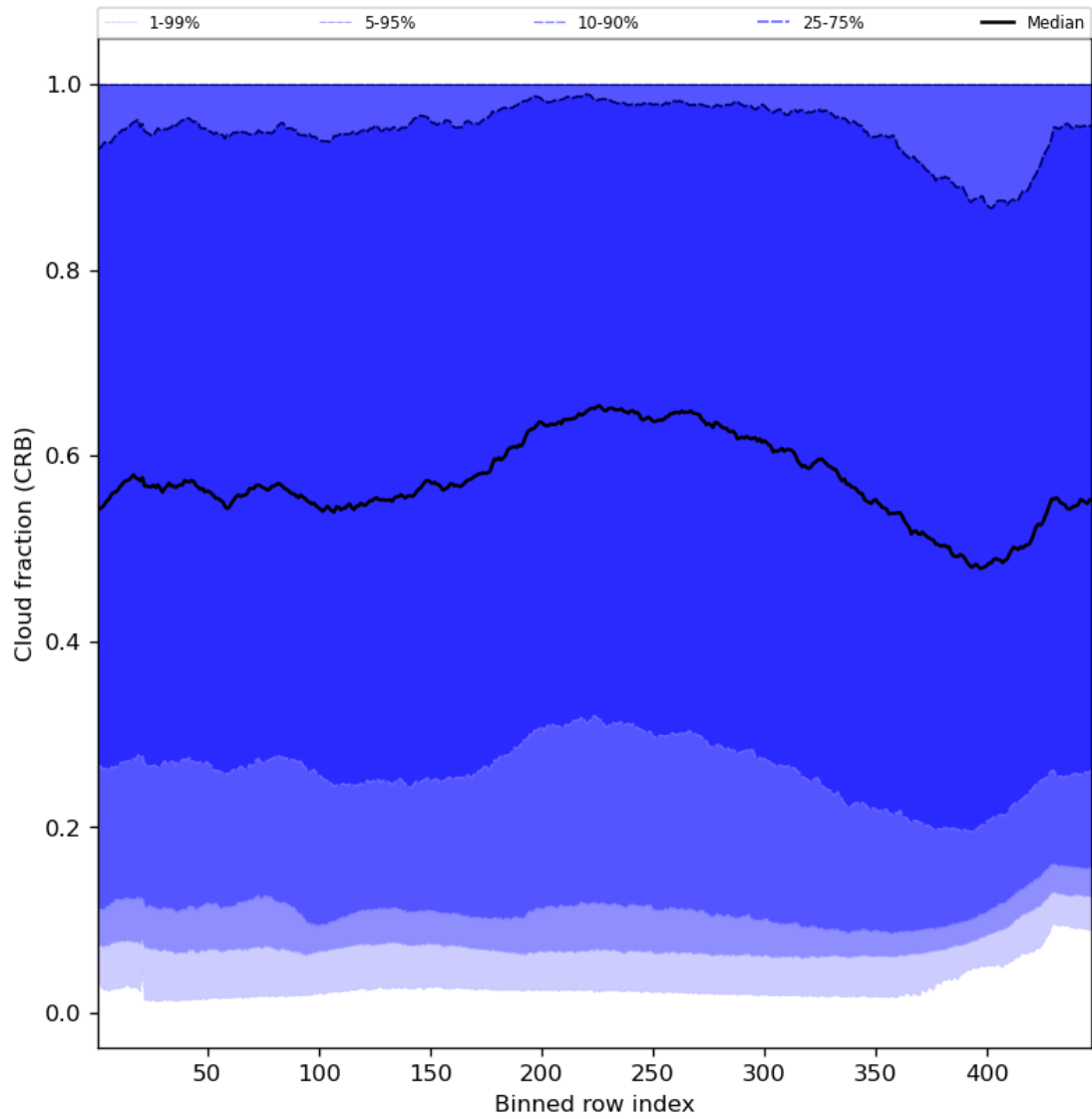
Figure 58: Along track statistics of “Cloud fraction (CRB)” for 2023-12-04 to 2023-12-06
