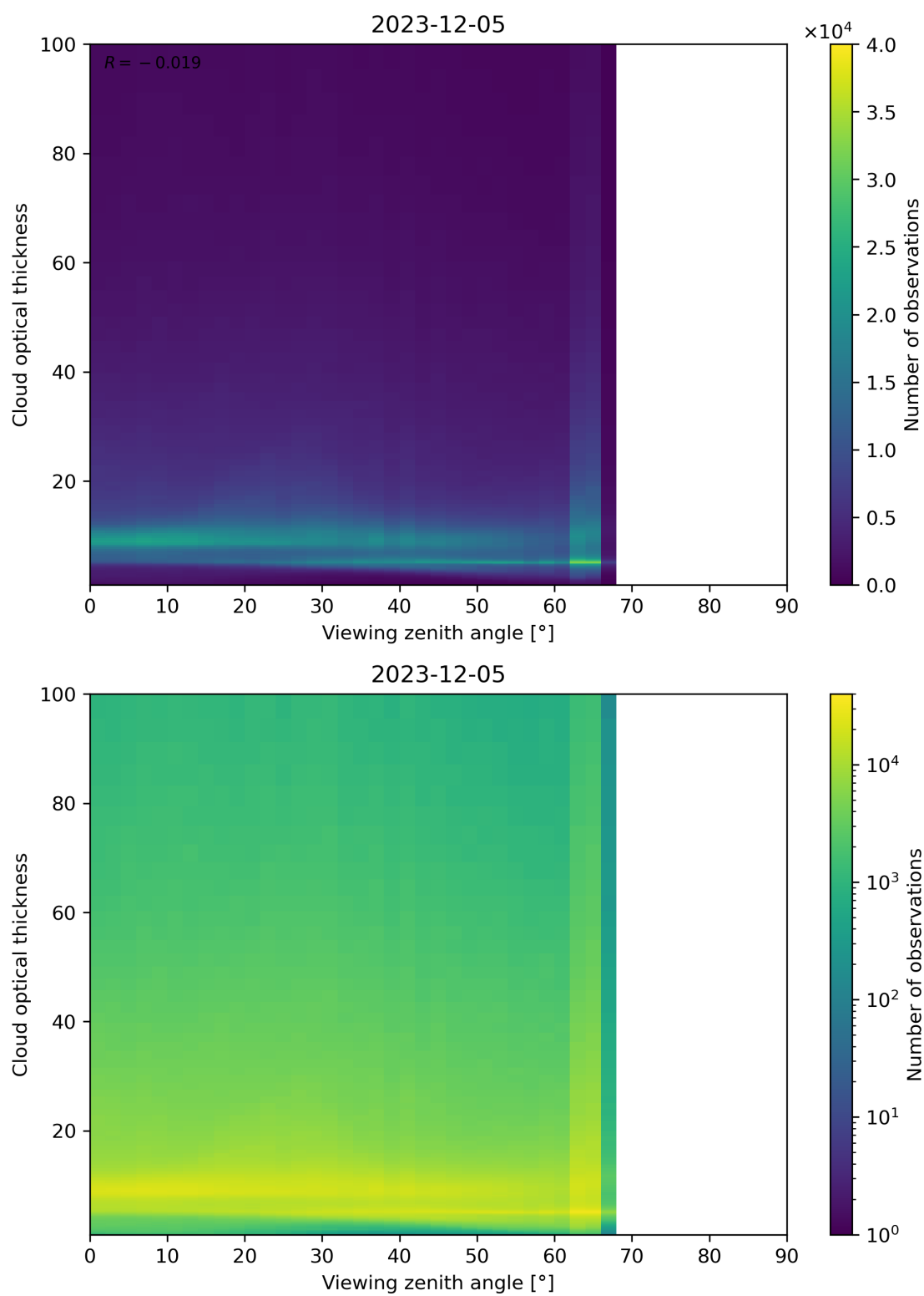
Figure 111: Scatter density plot of “Viewing zenith angle” against “Cloud optical thickness” for 2023-12-04 to 2023-12-06.
