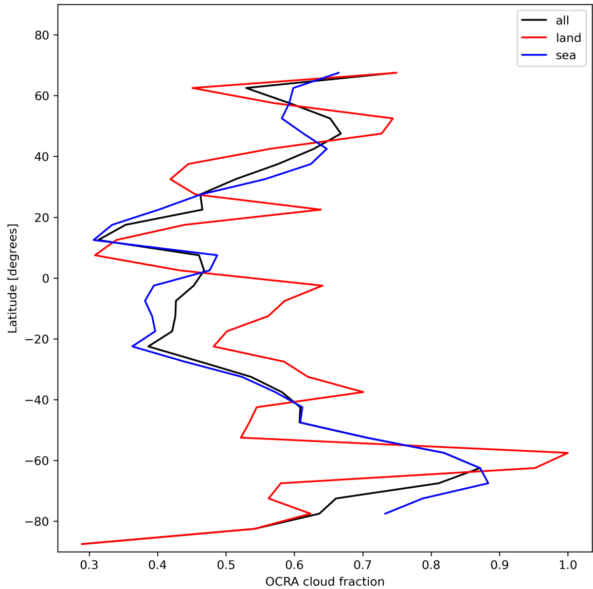
Figure 34: Zonal average of “OCRA cloud fraction” for 2023-12-04 to 2023-12-06.
