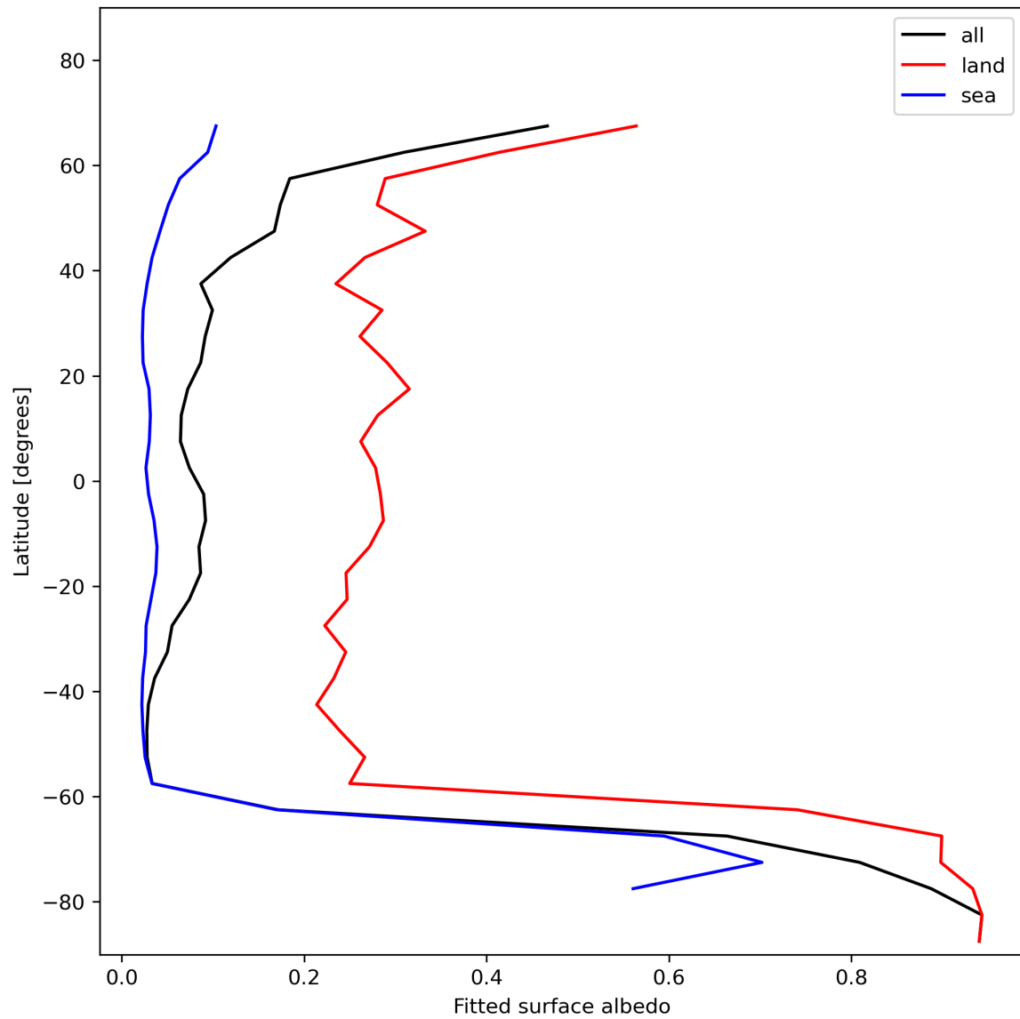
Figure 29: Zonal average of “Fitted surface albedo” for 2023-12-04 to 2023-12-06.
