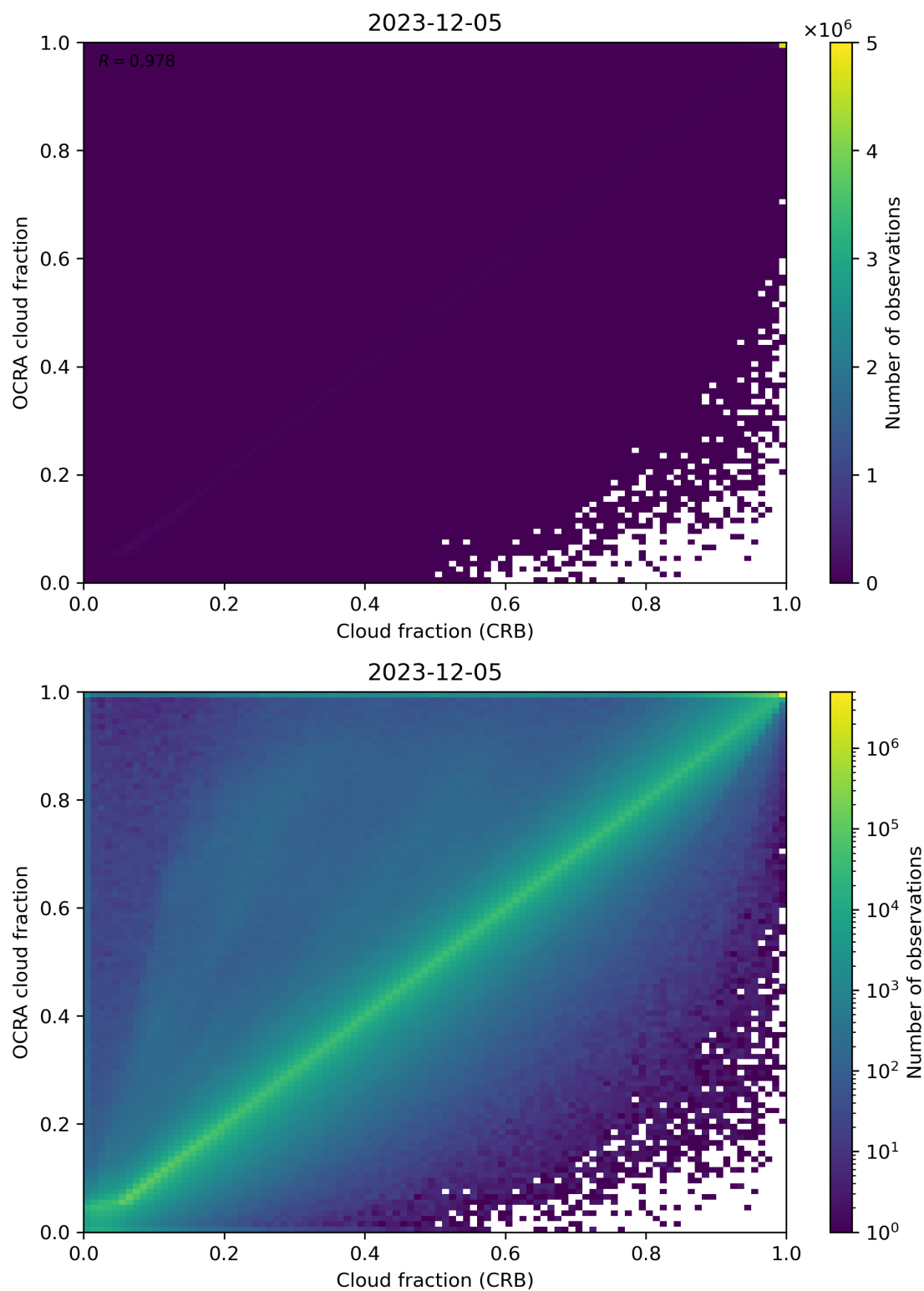
Figure 78: Scatter density plot of “Cloud fraction (CRB)” against “OCRA cloud fraction” for 2023-12-04 to 2023-12-06.
