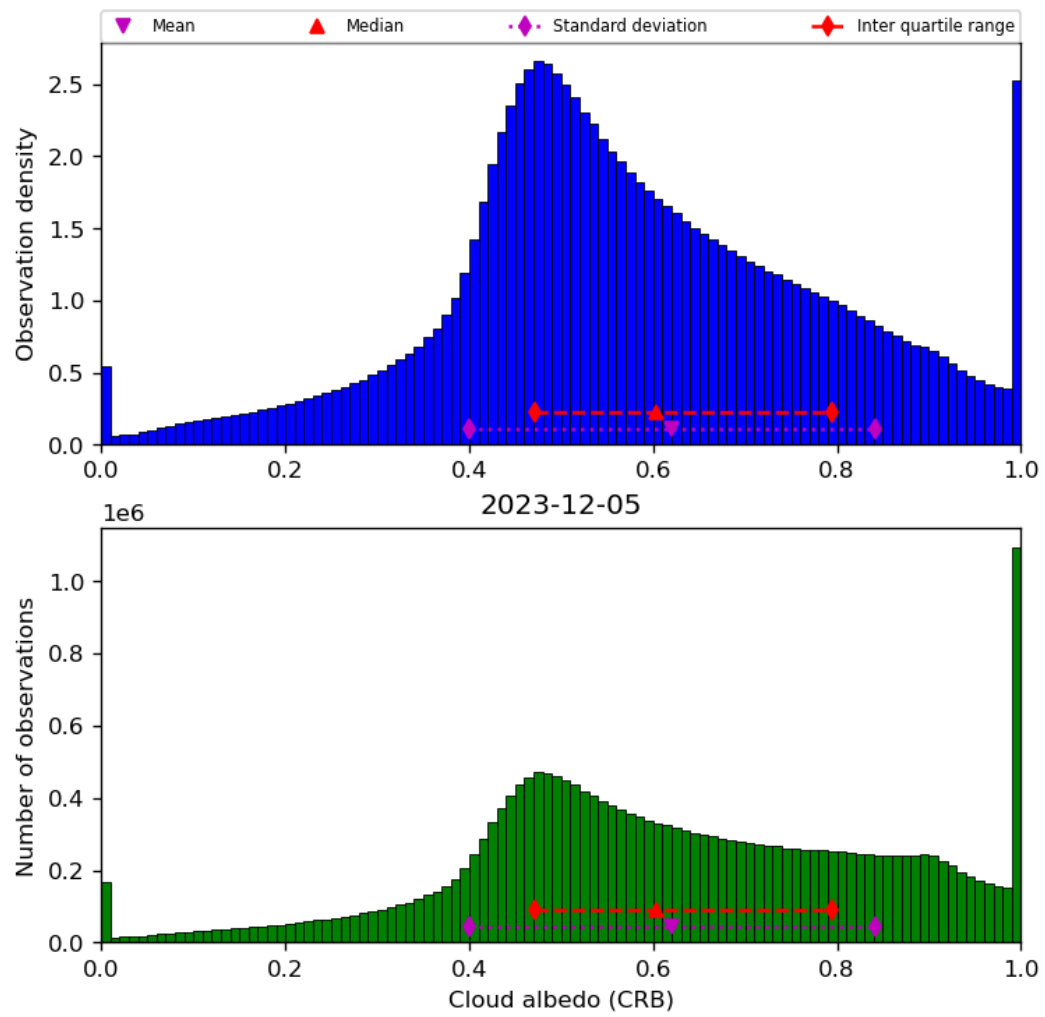
Figure 44: Histogram of “Cloud albedo (CRB)” for 2023-12-04 to 2023-12-06
