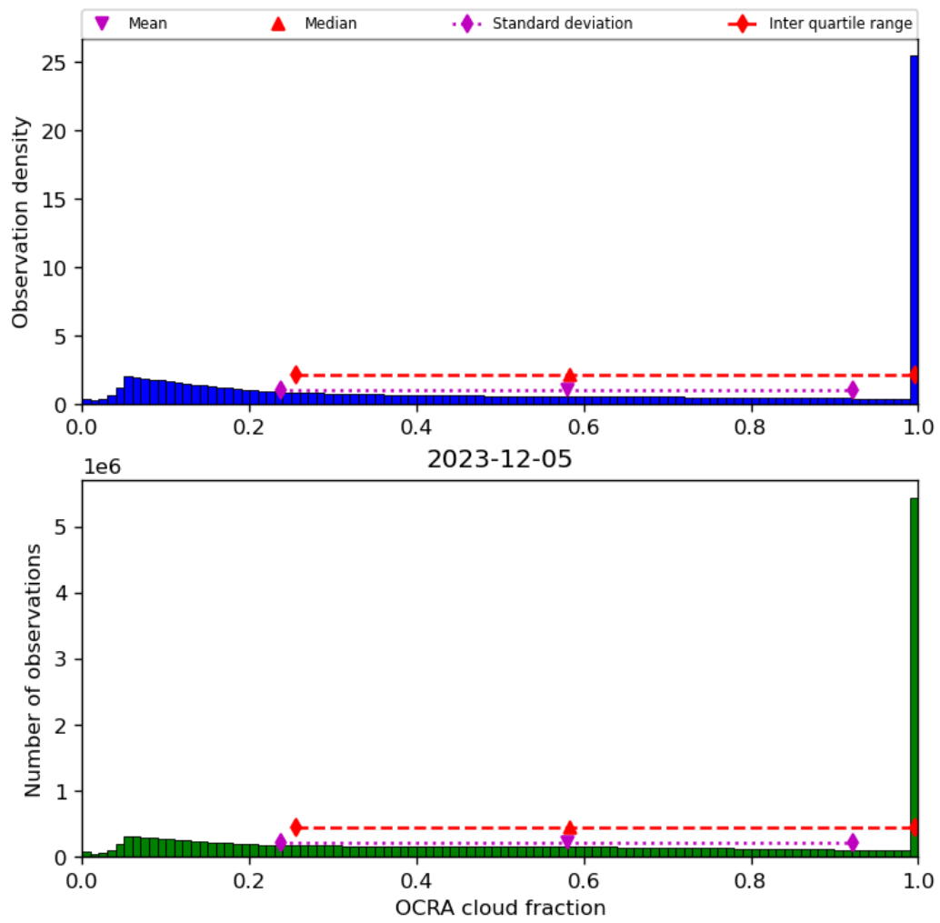
Figure 50: Histogram of “OCRA cloud fraction” for 2023-12-04 to 2023-12-06
