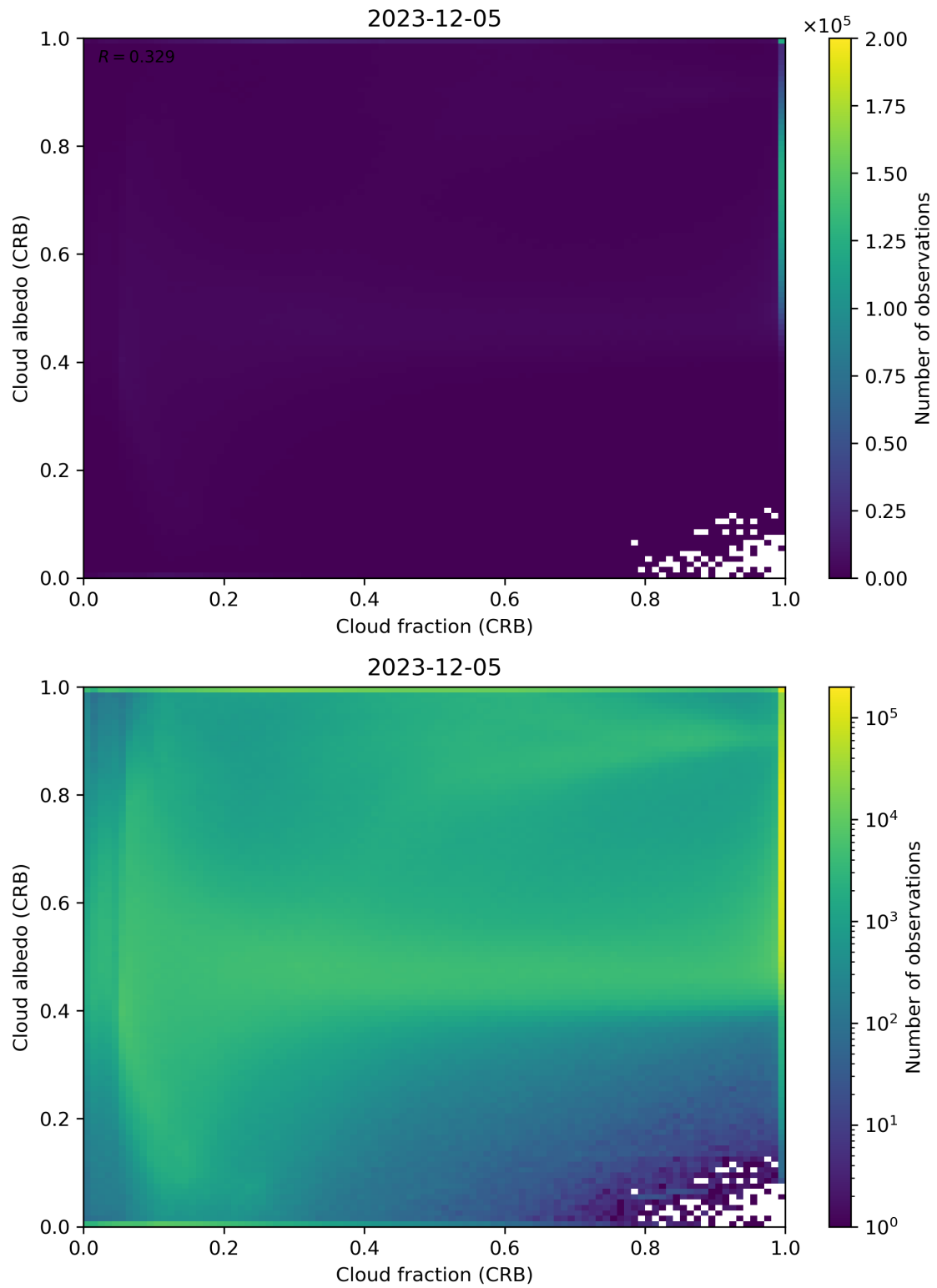
Figure 77: Scatter density plot of “Cloud fraction (CRB)” against “Cloud albedo (CRB)” for 2023-12-04 to 2023-12-06.
