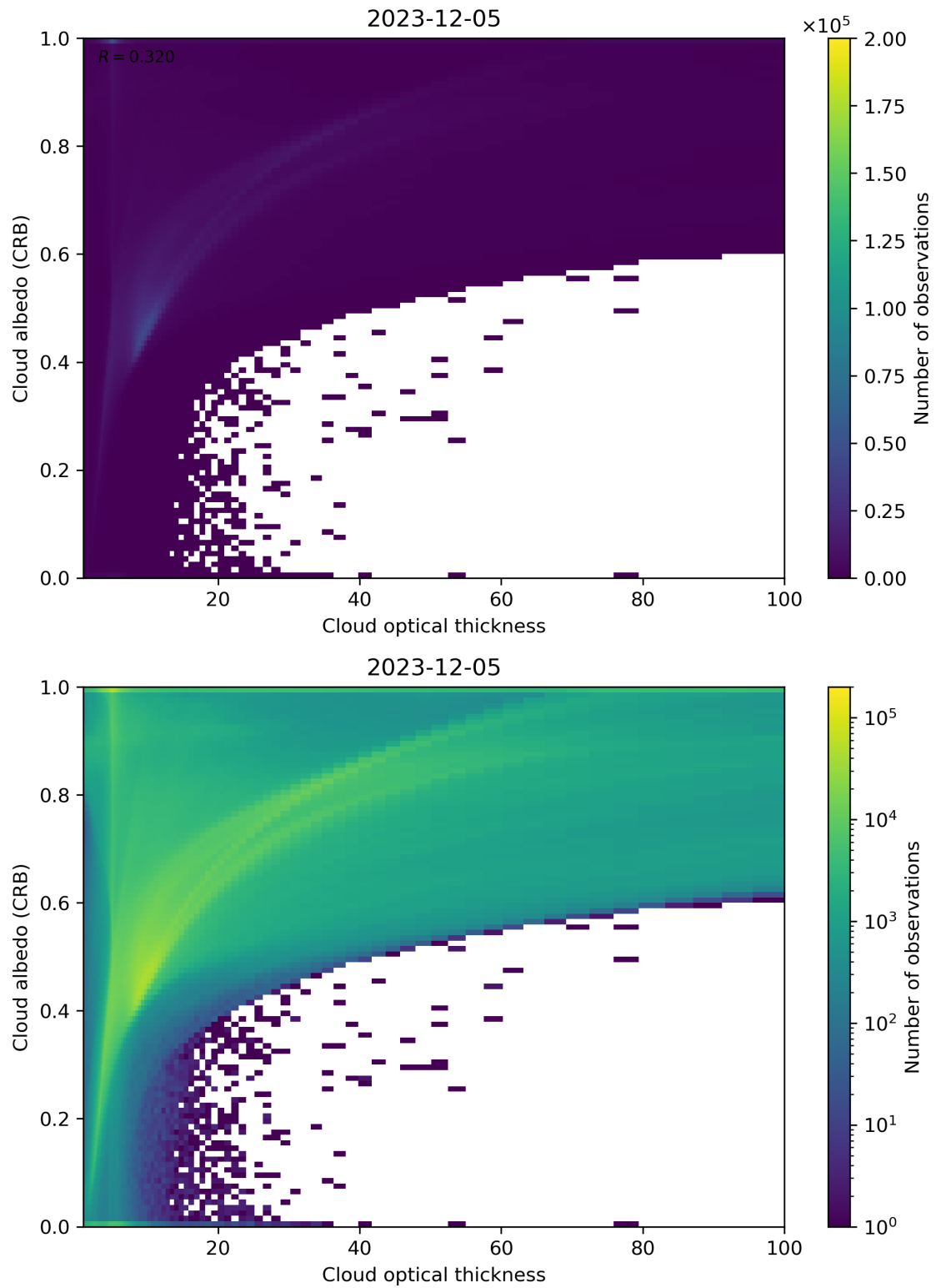
Figure 82: Scatter density plot of “Cloud optical thickness” against “Cloud albedo (CRB)” for 2023-12-04 to 2023-12-06.
