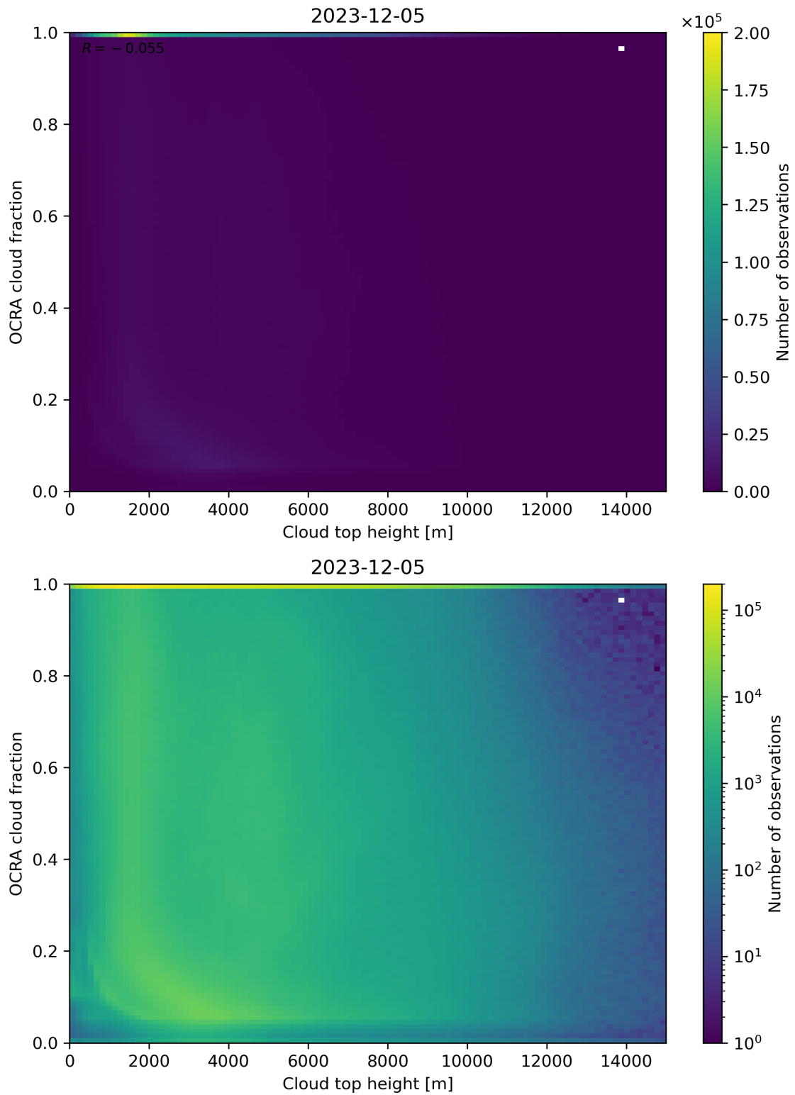
Figure 87: Scatter density plot of “Cloud top height” against “OCRA cloud fraction” for 2023-12-04 to 2023-12-06.
