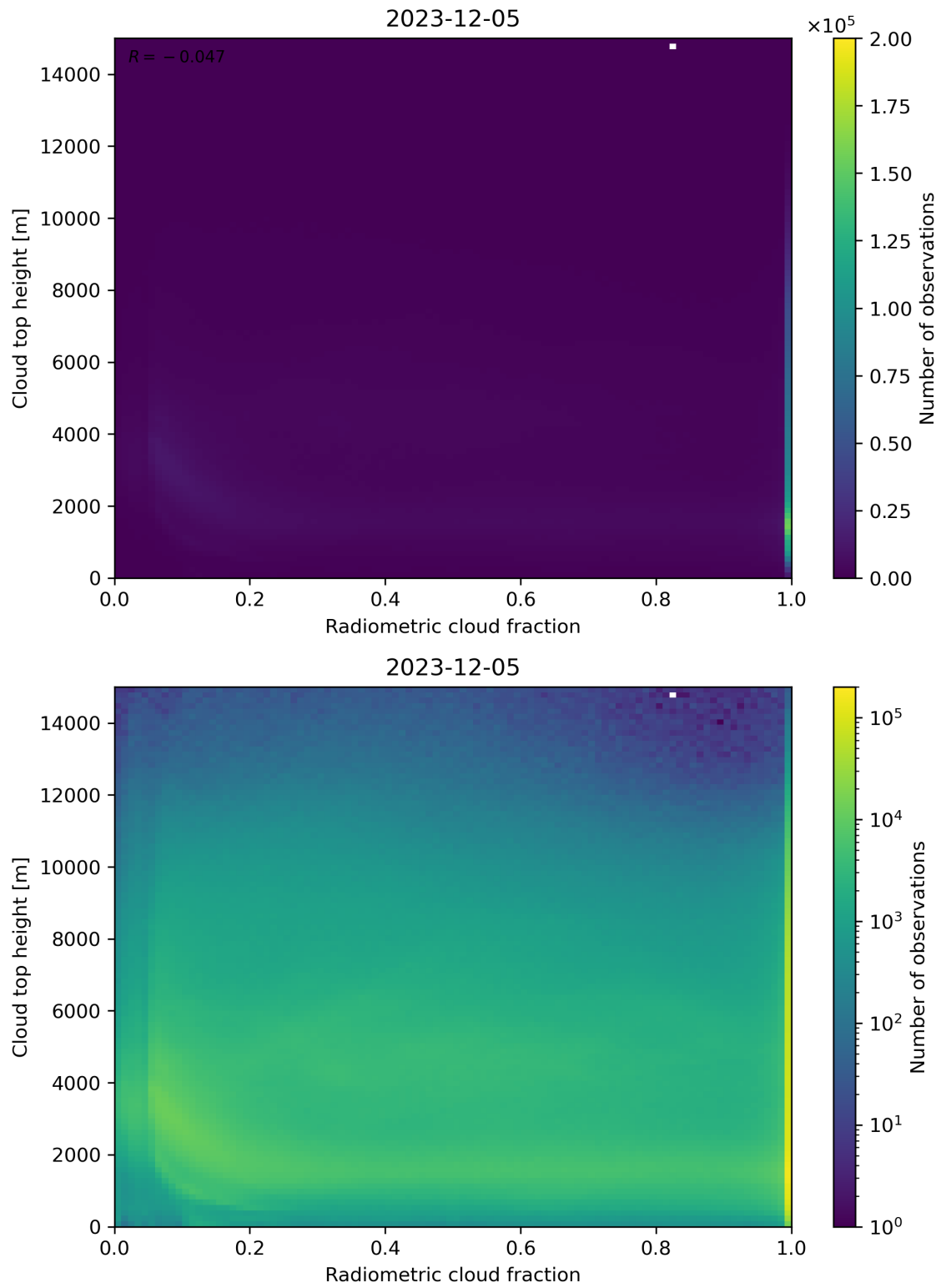
Figure 76: Scatter density plot of “Radiometric cloud fraction” against “Cloud top height” for 2023-12-04 to 2023-12-06.
