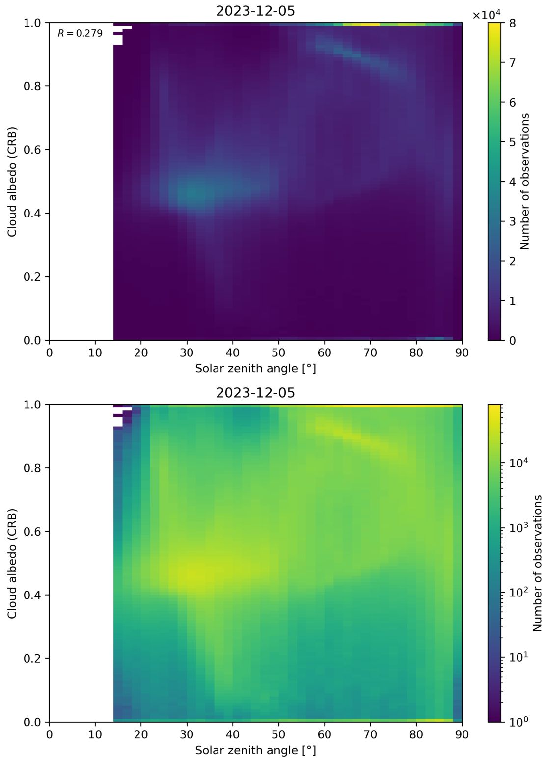
Figure 98: Scatter density plot of “Solar zenith angle” against “Cloud albedo (CRB)” for 2023-12-04 to 2023-12-06.
