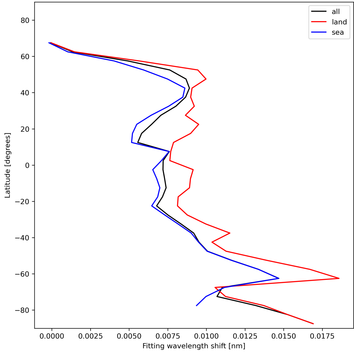
Figure 33: Zonal average of “Fitting wavelength shift” for 2023-12-04 to 2023-12-06.
