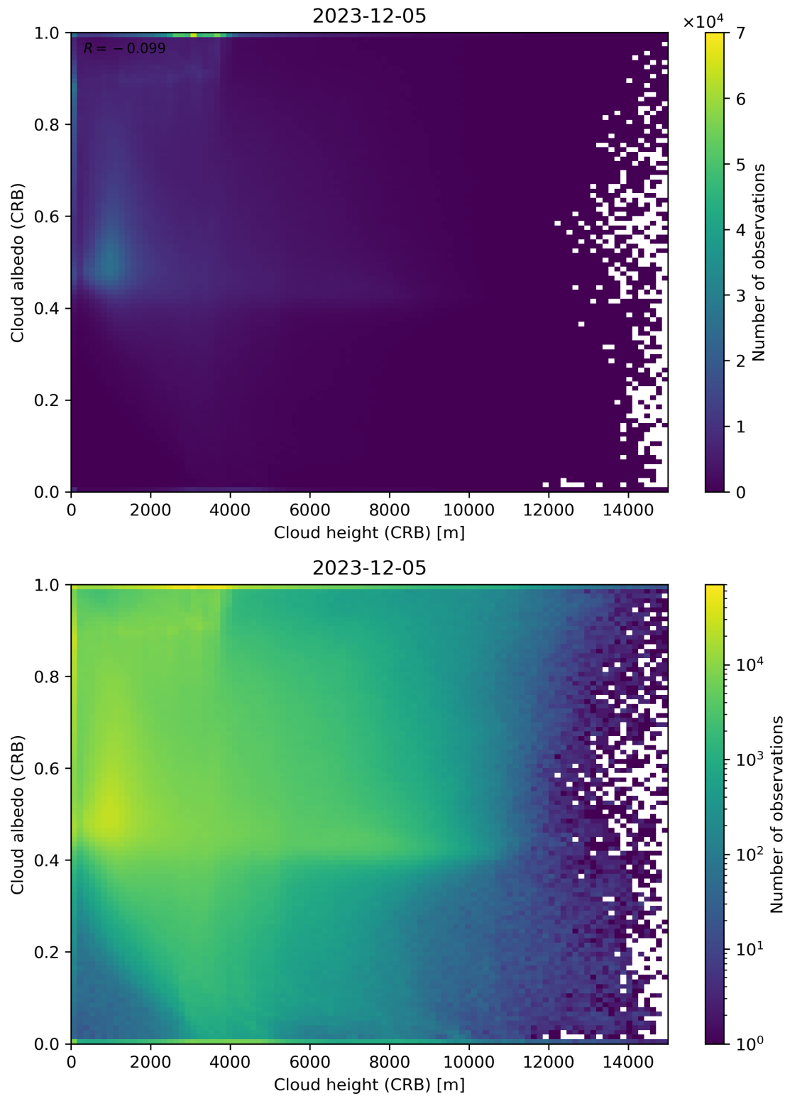
Figure 80: Scatter density plot of “Cloud height (CRB)” against “Cloud albedo (CRB)” for 2023-12-04 to 2023-12-06.
