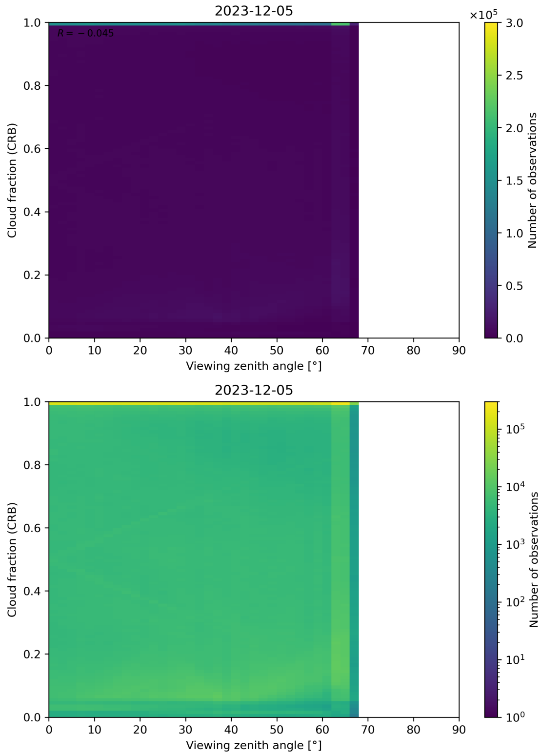
Figure 109: Scatter density plot of “Viewing zenith angle” against “Cloud fraction (CRB)” for 2023-12-04 to 2023-12-06.
