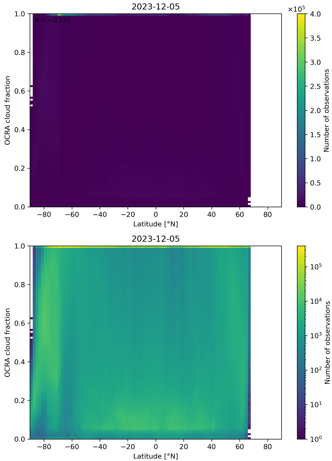
Figure 93: Scatter density plot of “Latitude” against “OCRA cloud fraction” for 2023-12-04 to 2023-12-06.
