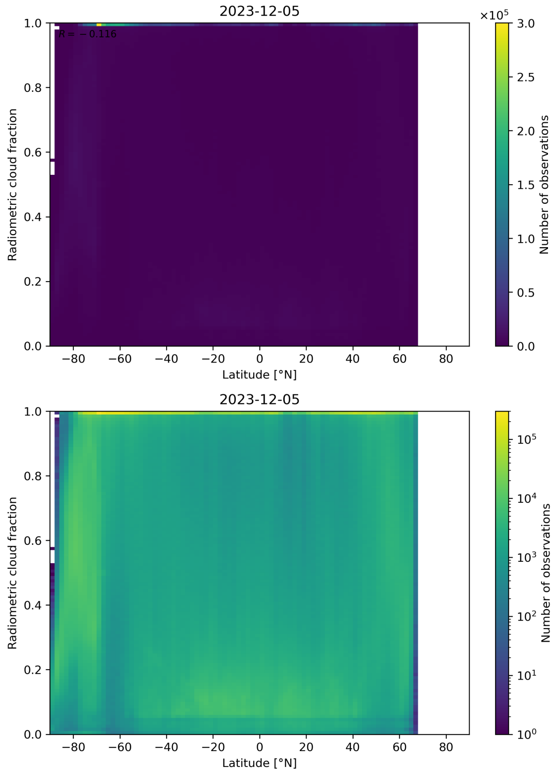
Figure 92: Scatter density plot of “Latitude” against “Radiometric cloud fraction” for 2023-12-04 to 2023-12-06.
