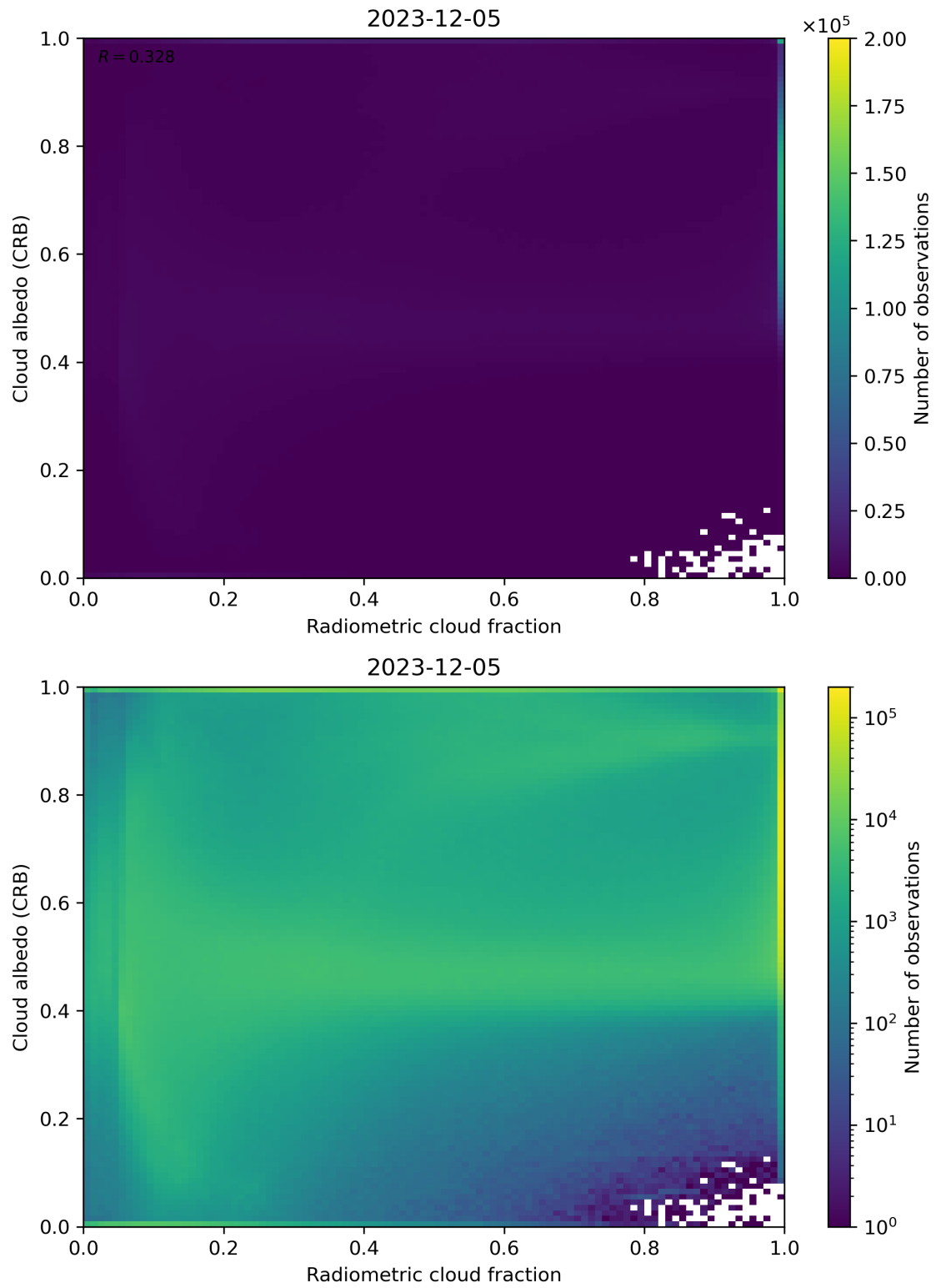
Figure 71: Scatter density plot of “Radiometric cloud fraction” against “Cloud albedo (CRB)” for 2023-12-04 to 2023-12-06.
