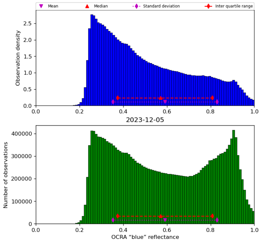
Figure 51: Histogram of “OCRA “blue” reflectance” for 2023-12-04 to 2023-12-06
