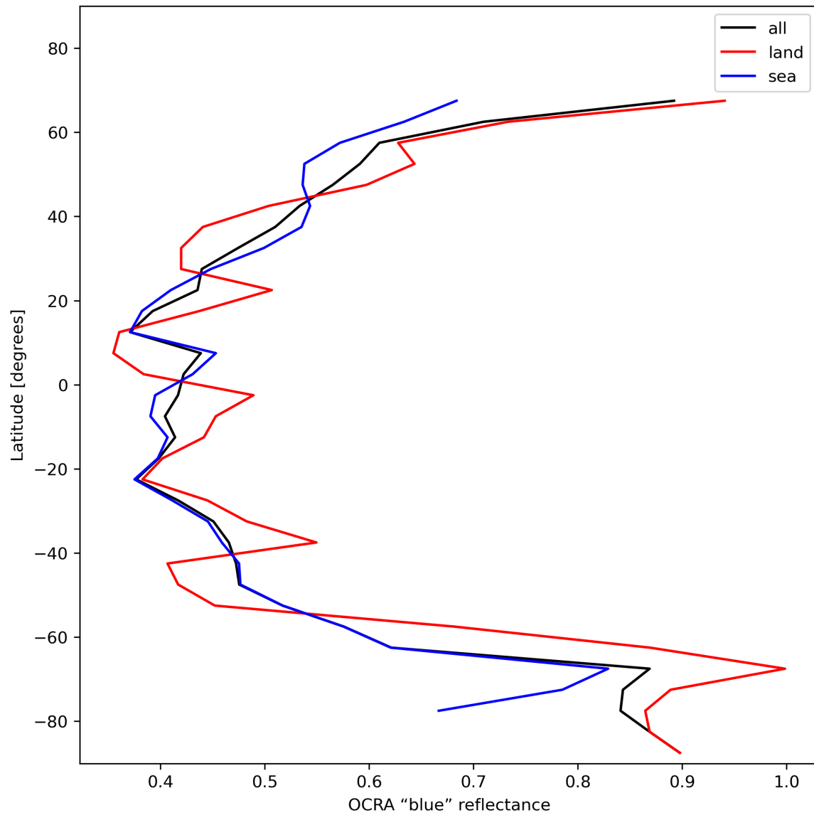
Figure 35: Zonal average of “OCRA “blue” reflectance” for 2023-12-04 to 2023-12-06.
