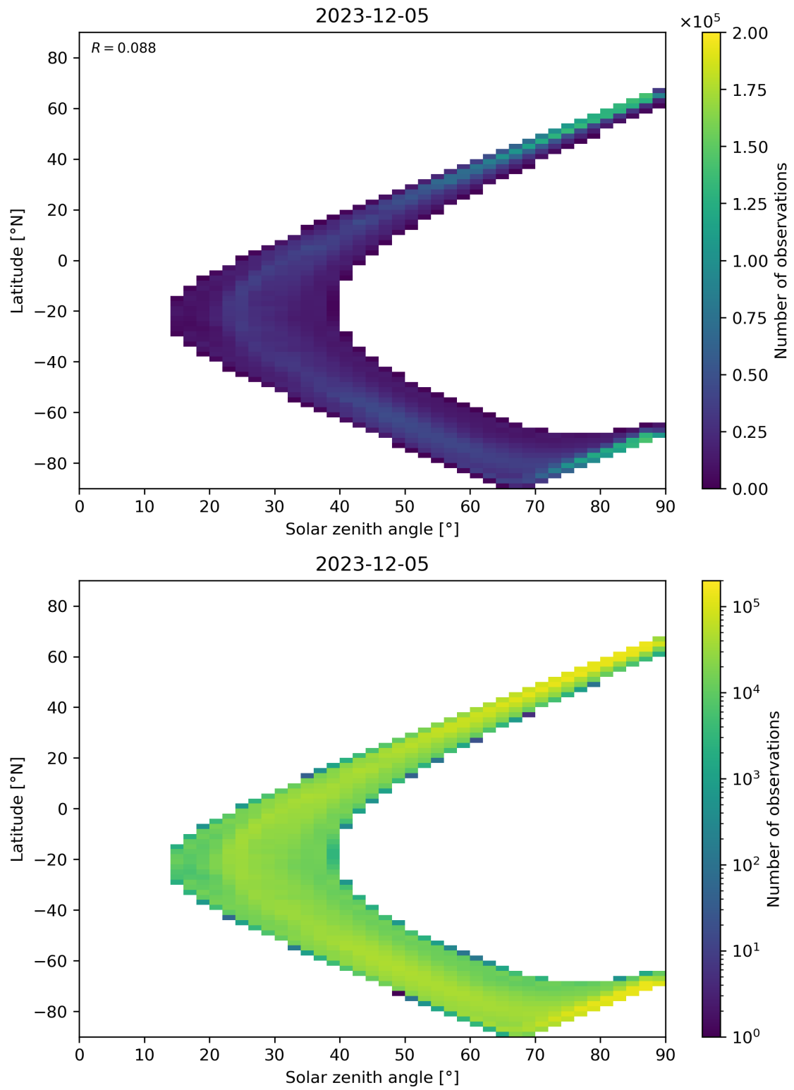
Figure 105: Scatter density plot of “Solar zenith angle” against “Latitude” for 2023-12-04 to 2023-12-06.
