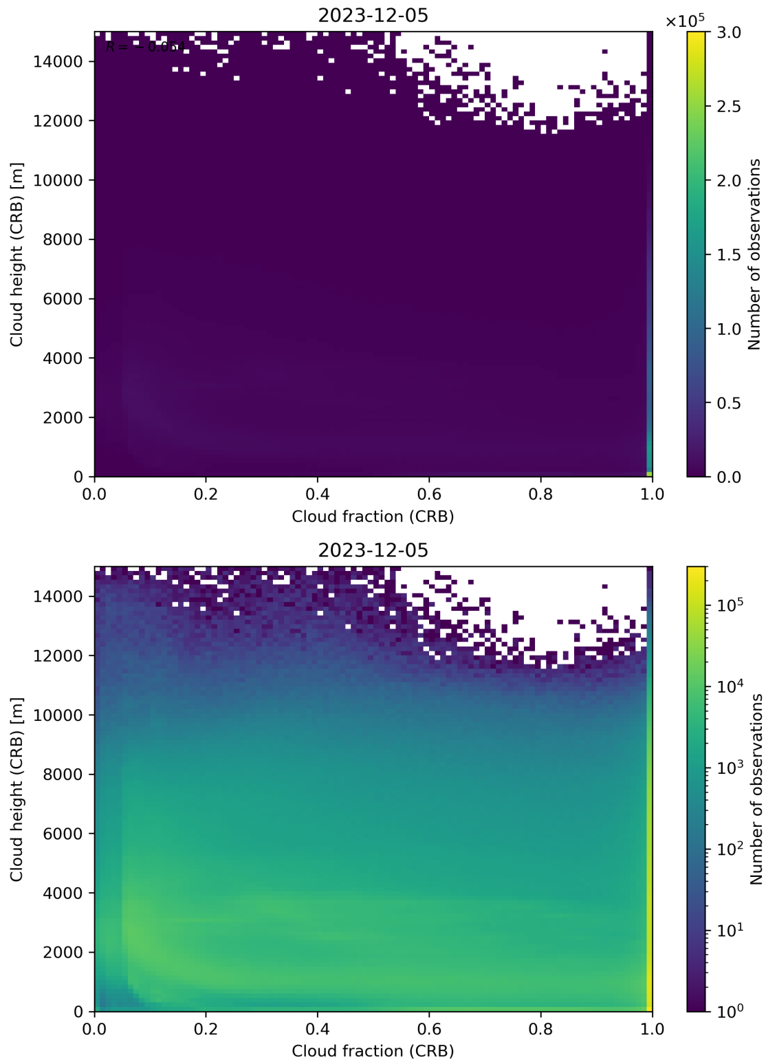
Figure 79: Scatter density plot of “Cloud fraction (CRB)” against “Cloud height (CRB)” for 2023-12-04 to 2023-12-06.
