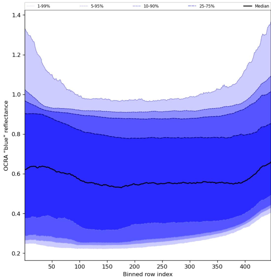
Figure 67: Along track statistics of “OCRA “blue” reflectance” for 2023-12-04 to 2023-12-06
