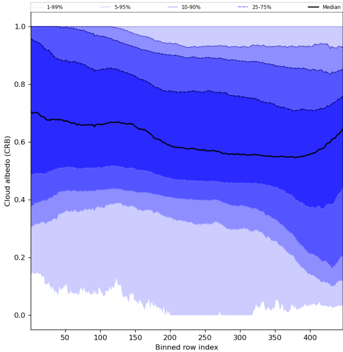
Figure 60: Along track statistics of “Cloud albedo (CRB)” for 2023-12-04 to 2023-12-06
