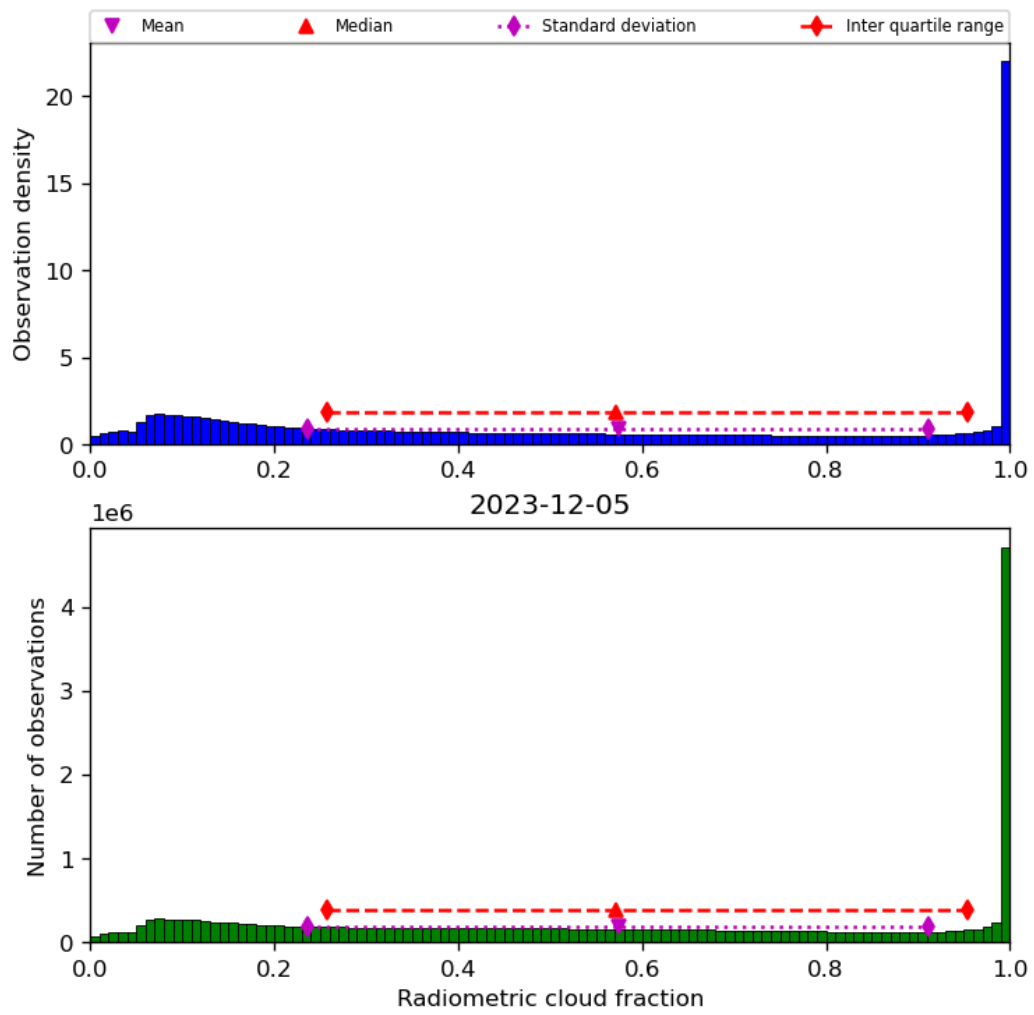
Figure 39: Histogram of “Radiometric cloud fraction” for 2023-12-04 to 2023-12-06
