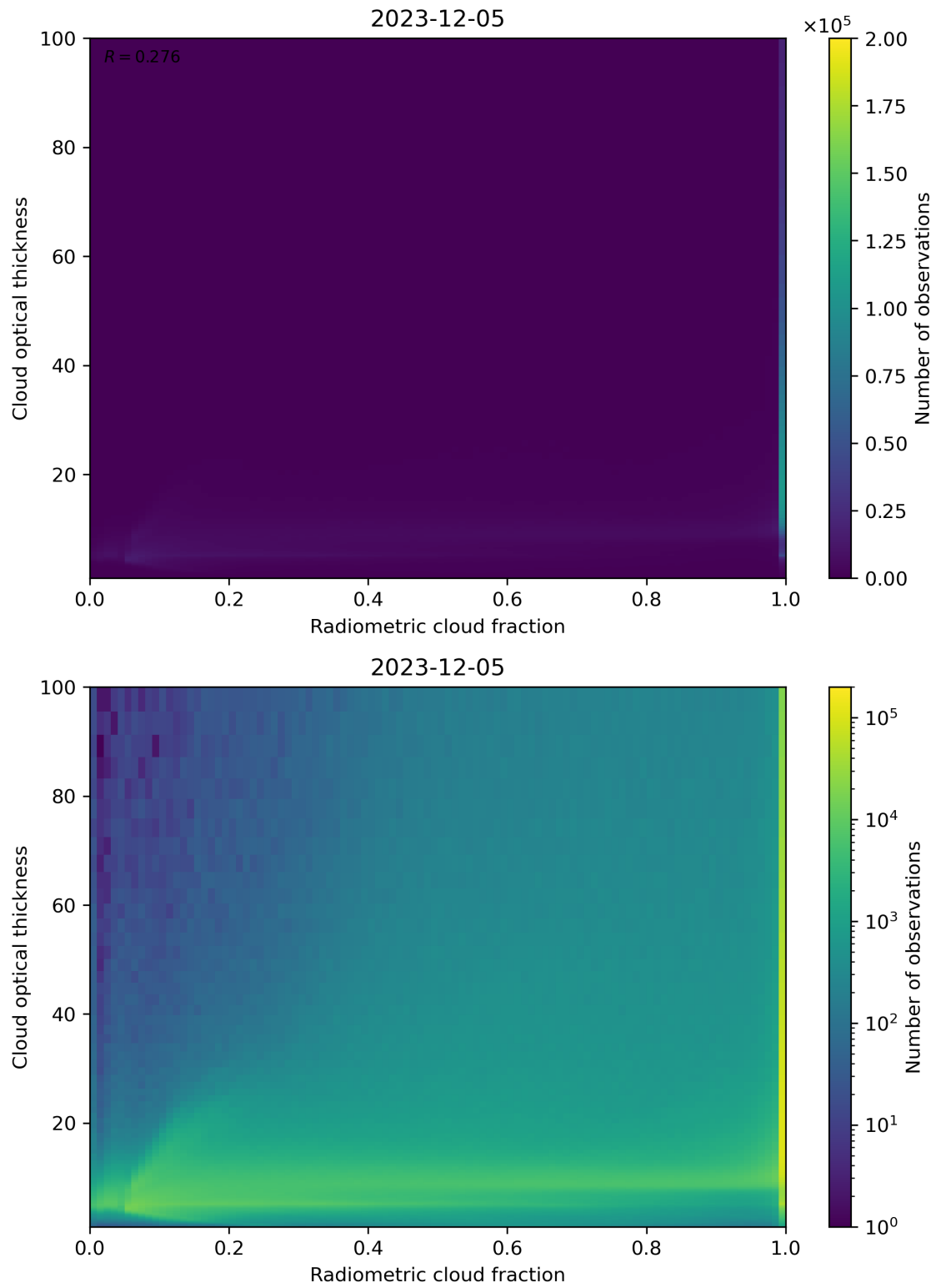
Figure 75: Scatter density plot of “Radiometric cloud fraction” against “Cloud optical thickness” for 2023-12-04 to 2023-12-06.
