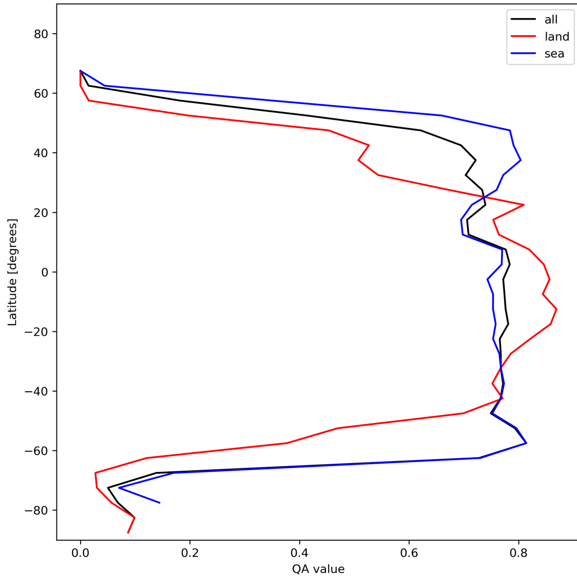
Figure 22: Zonal average of “QA value” for 2023-12-04 to 2023-12-06.
