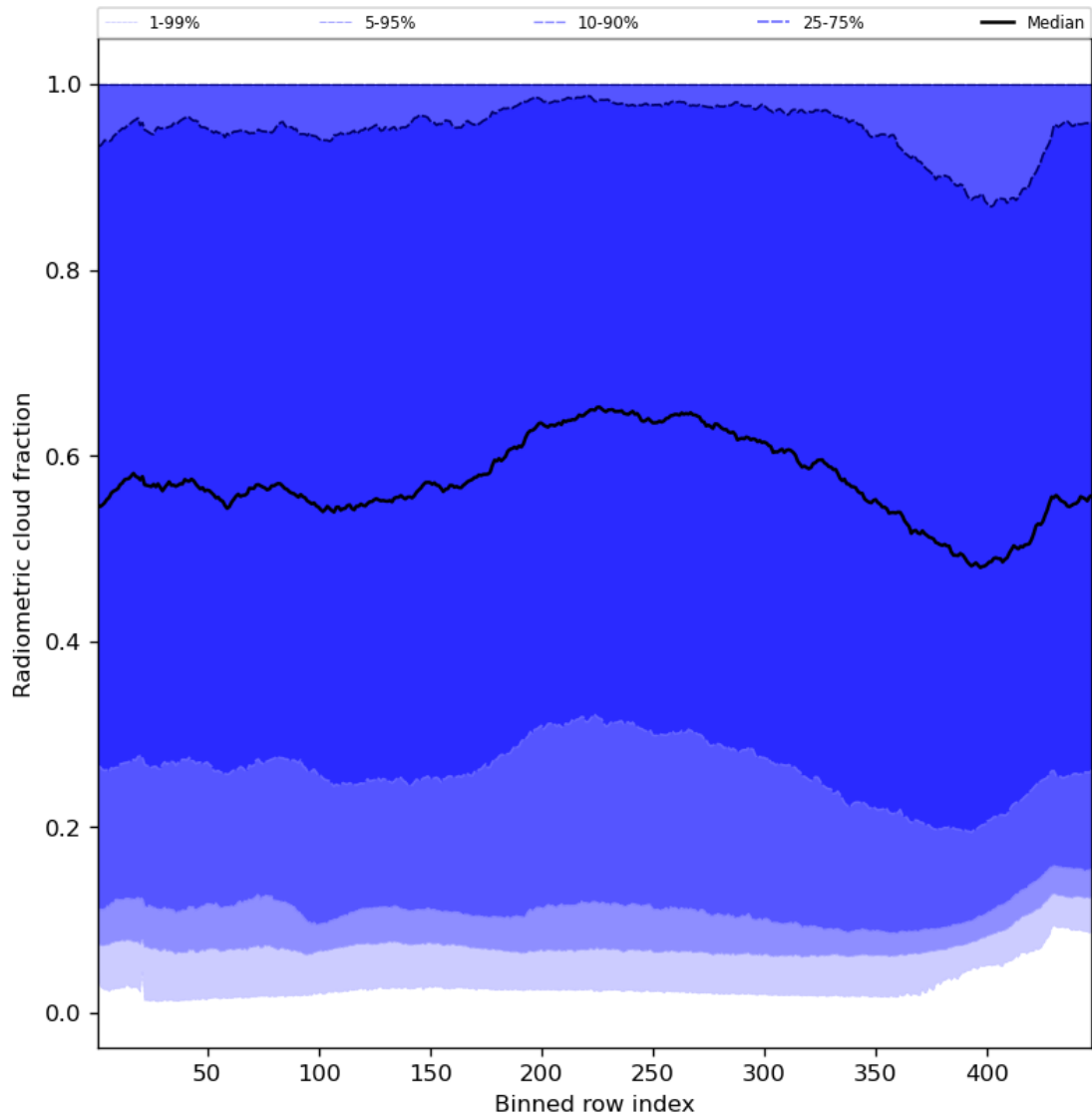
Figure 55: Along track statistics of “Radiometric cloud fraction” for 2023-12-04 to 2023-12-06
