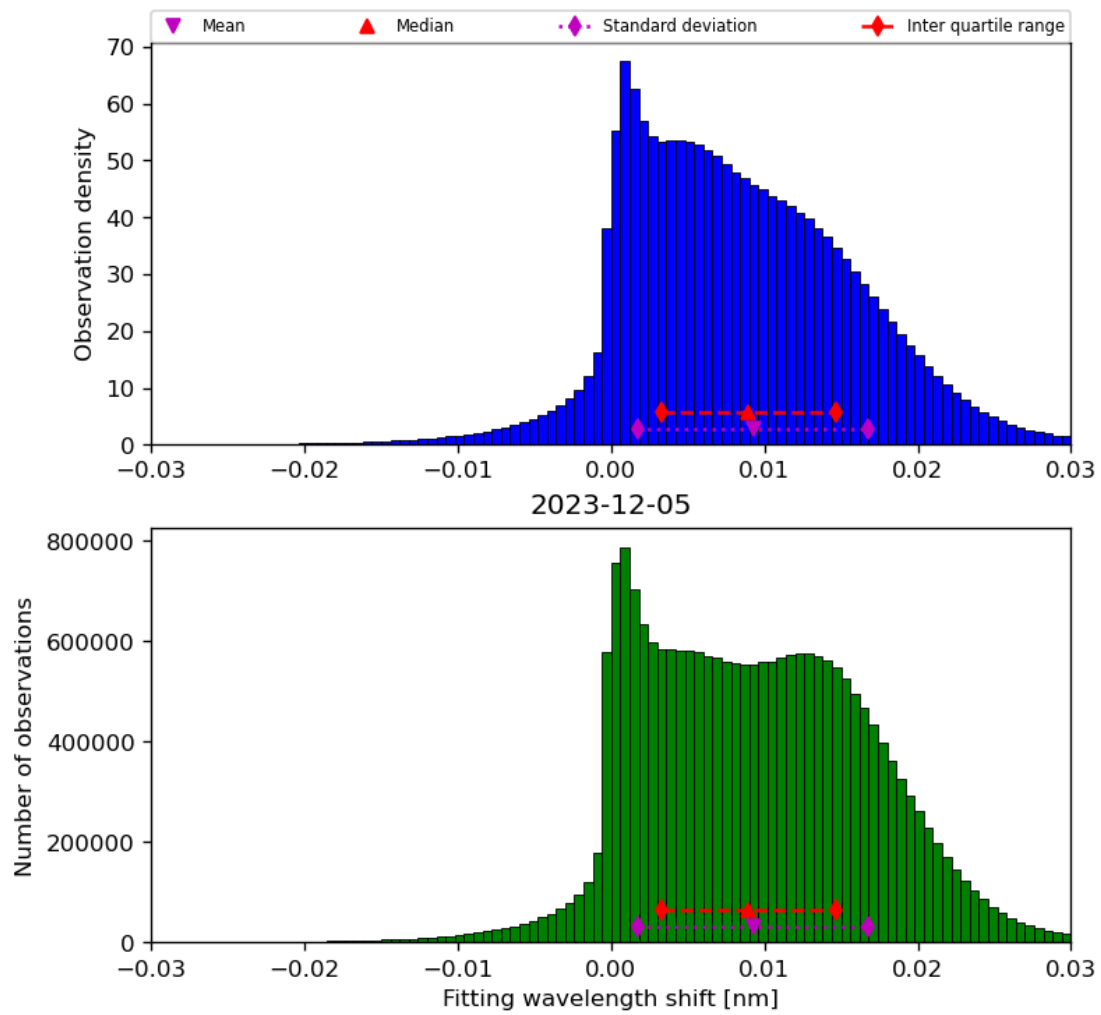
Figure 49: Histogram of “Fitting wavelength shift” for 2023-12-04 to 2023-12-06
