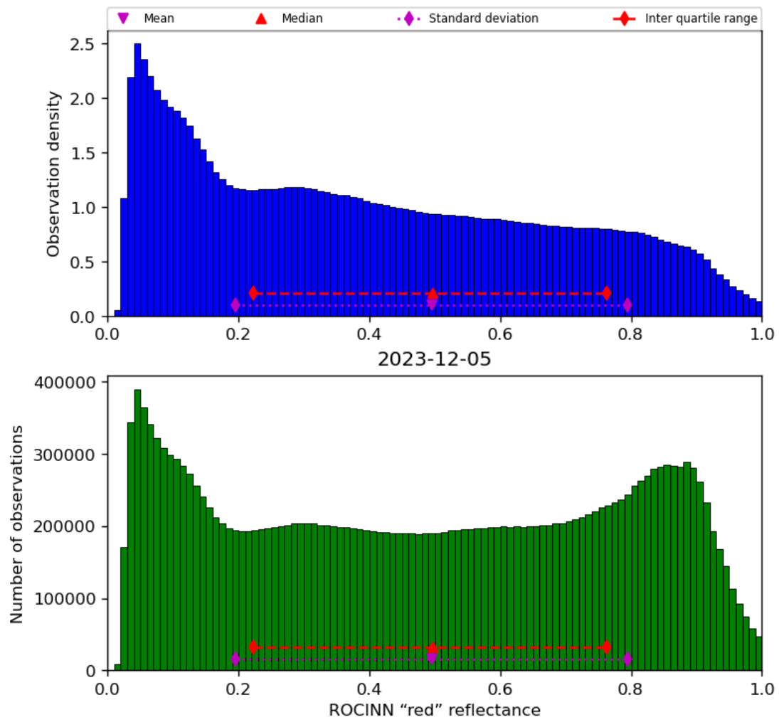
Figure 53: Histogram of “ROCINN “red” reflectance” for 2023-12-04 to 2023-12-06
