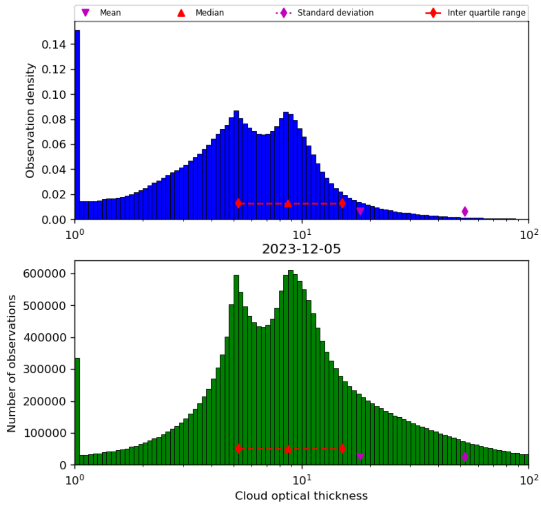
Figure 41: Histogram of “Cloud optical thickness” for 2023-12-04 to 2023-12-06
