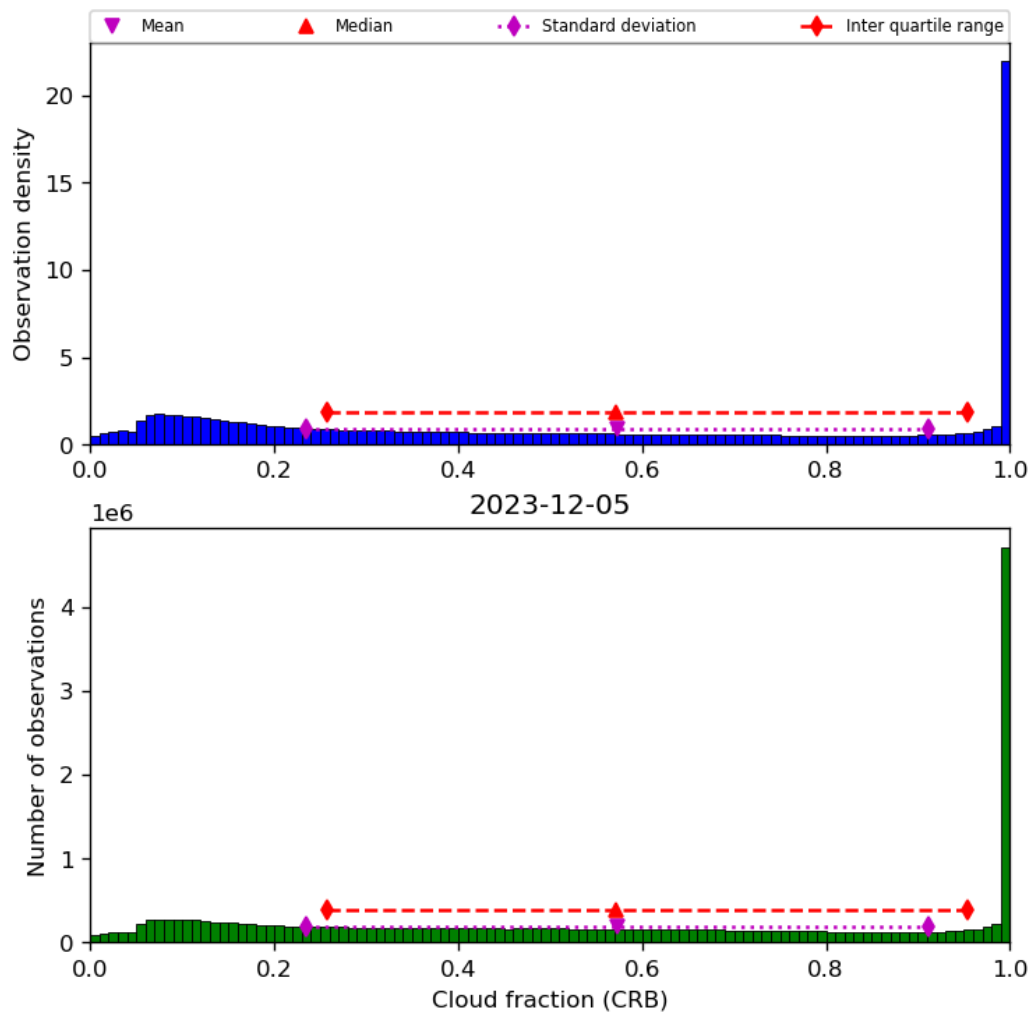
Figure 42: Histogram of “Cloud fraction (CRB)” for 2023-12-04 to 2023-12-06
