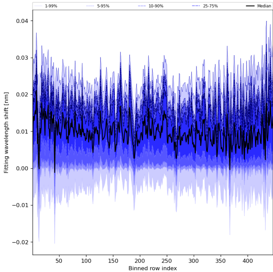
Figure 65: Along track statistics of “Fitting wavelength shift” for 2023-12-04 to 2023-12-06
