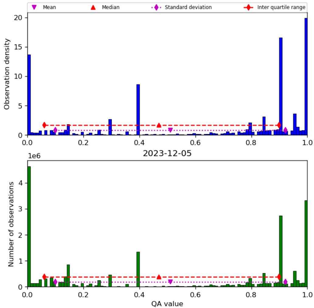
Figure 38: Histogram of “QA value” for 2023-12-04 to 2023-12-06
