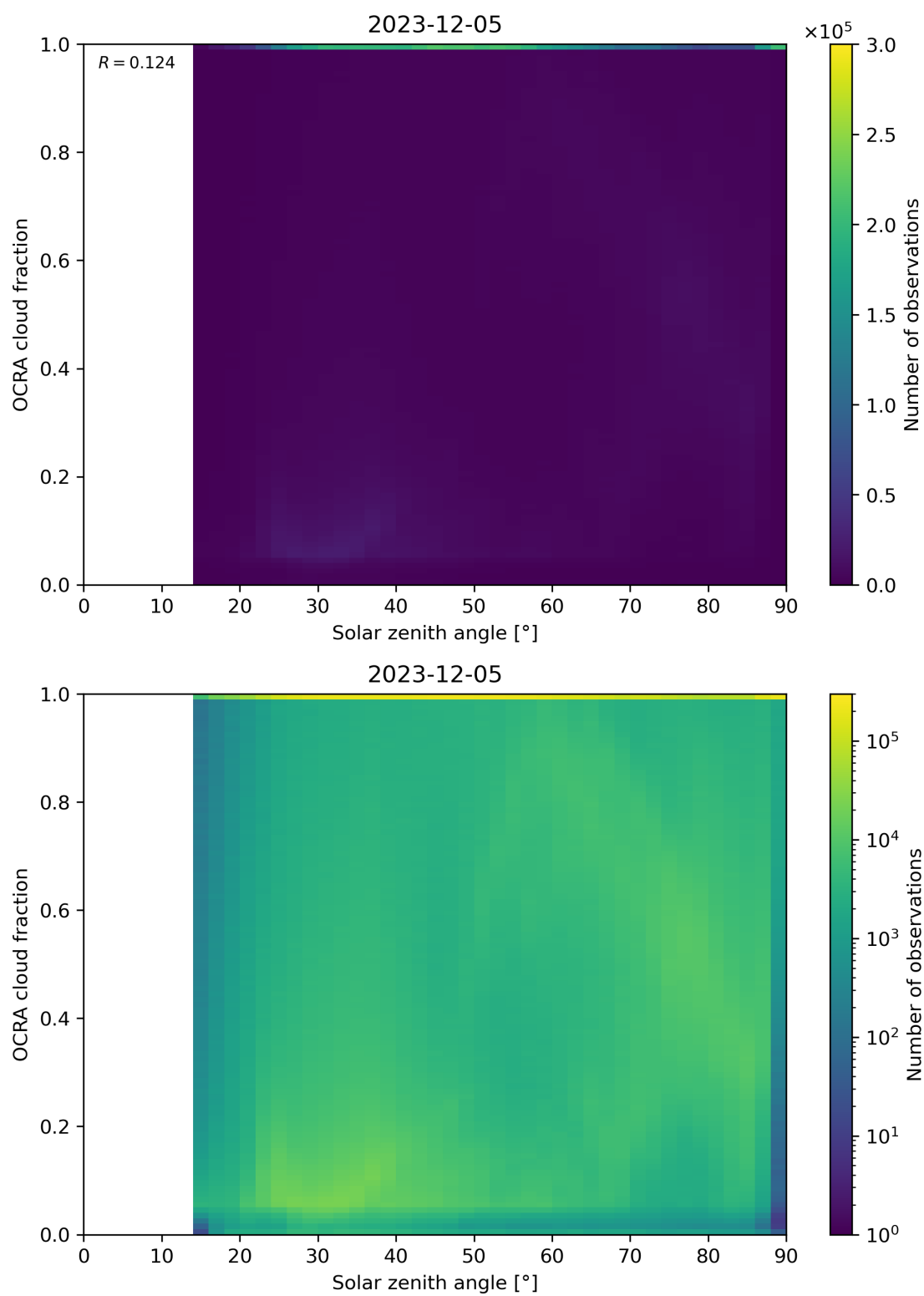
Figure 100: Scatter density plot of “Solar zenith angle” against “OCRA cloud fraction” for 2023-12-04 to 2023-12-06.
