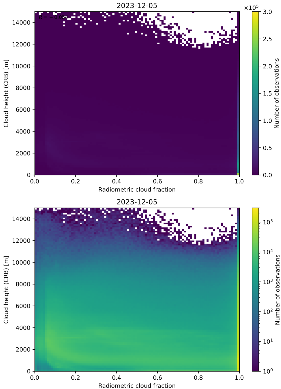
Figure 74: Scatter density plot of “Radiometric cloud fraction” against “Cloud height (CRB)” for 2023-12-04 to 2023-12-06.
