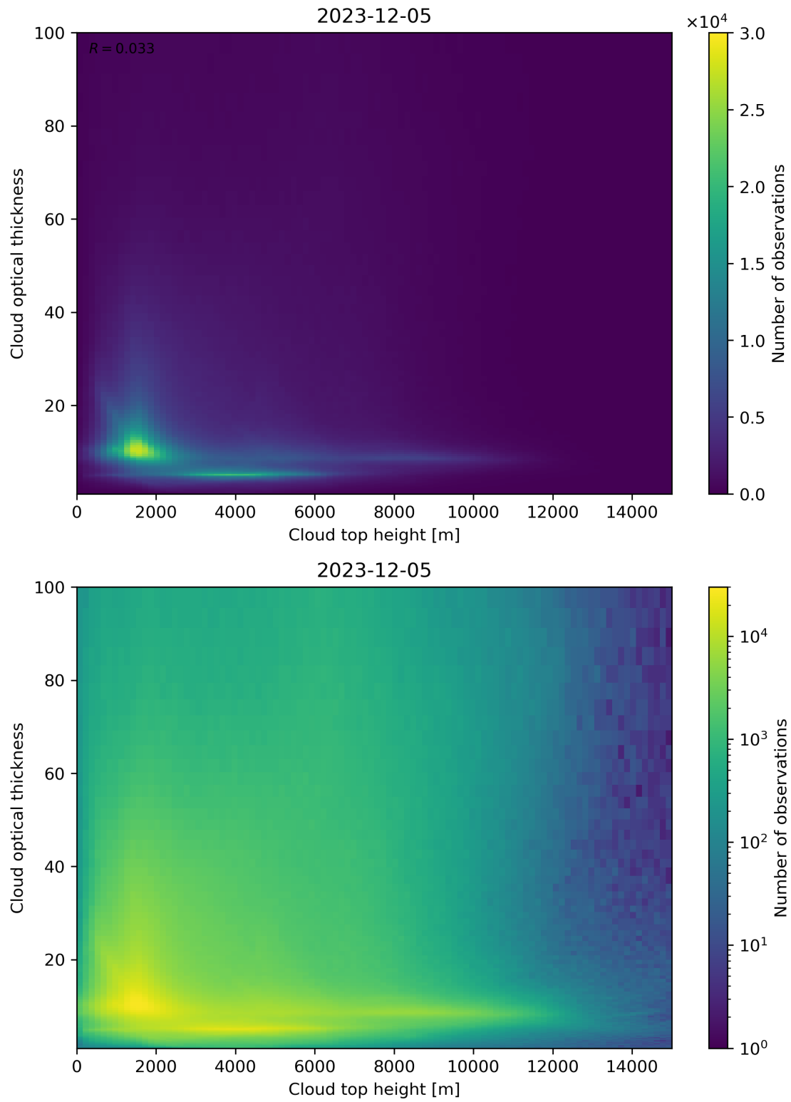
Figure 90: Scatter density plot of “Cloud top height” against “Cloud optical thickness” for 2023-12-04 to 2023-12-06.
