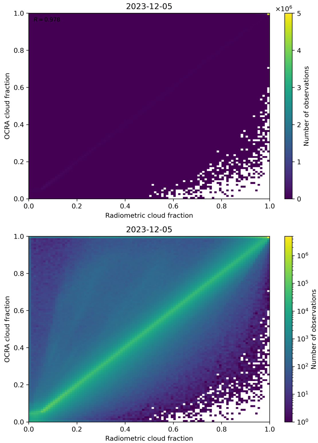
Figure 72: Scatter density plot of “Radiometric cloud fraction” against “OCRA cloud fraction” for 2023-12-04 to 2023-12-06.
