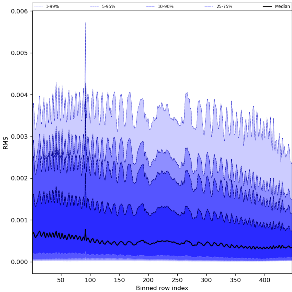
Figure 63: Along track statistics of “RMS” for 2023-12-04 to 2023-12-06
