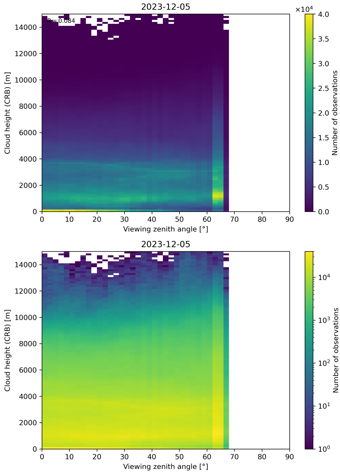
Figure 110: Scatter density plot of “Viewing zenith angle” against “Cloud height (CRB)” for 2023-12-04 to 2023-12-06.
