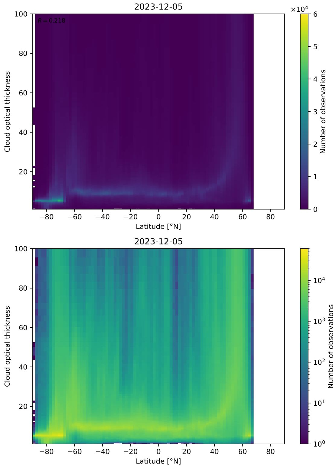
Figure 96: Scatter density plot of “Latitude” against “Cloud optical thickness” for 2023-12-04 to 2023-12-06.
