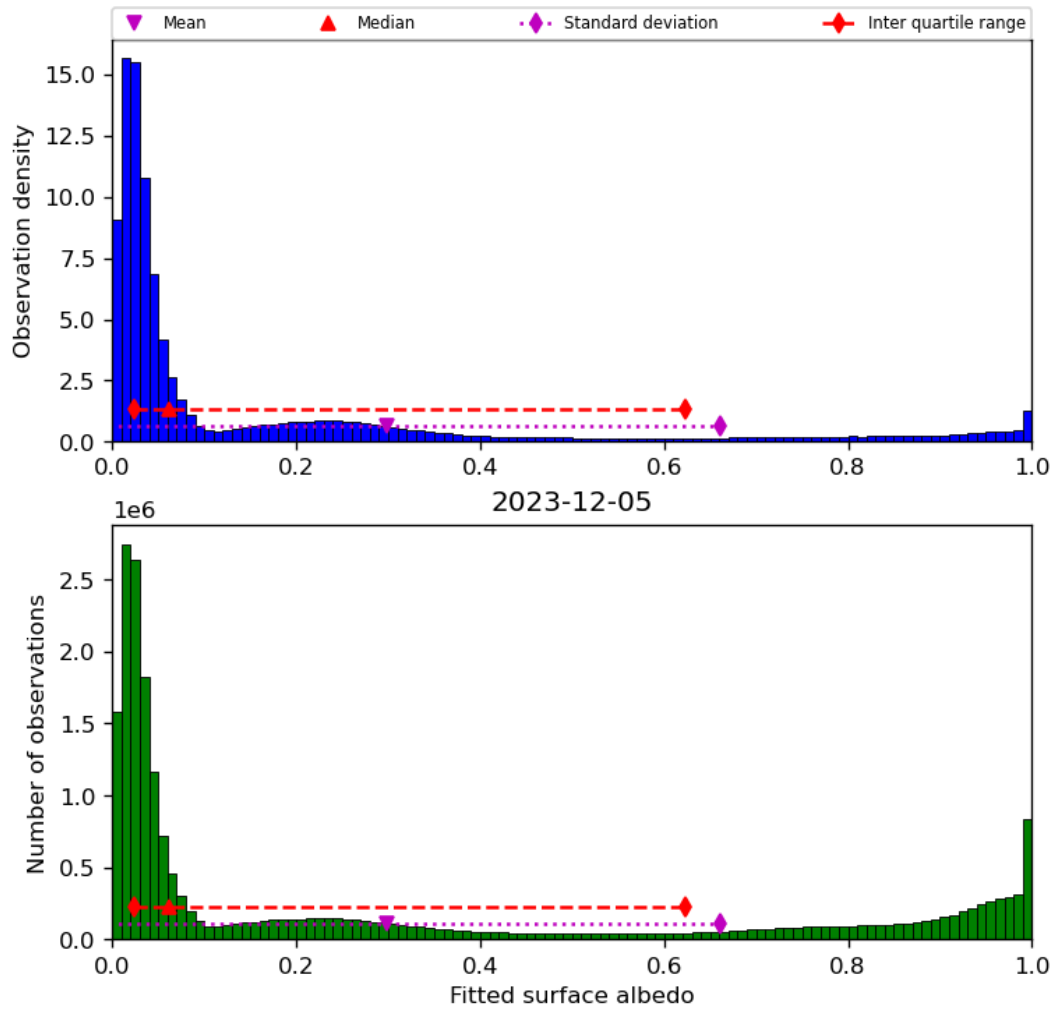
Figure 45: Histogram of “Fitted surface albedo” for 2023-12-04 to 2023-12-06
