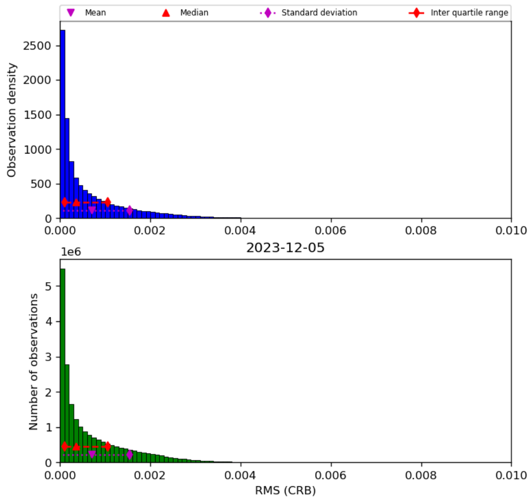
Figure 48: Histogram of “RMS (CRB)” for 2023-12-04 to 2023-12-06
