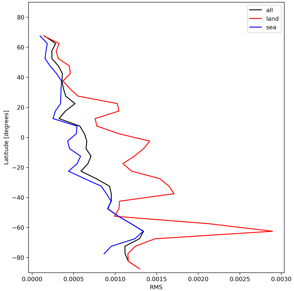
Figure 31: Zonal average of “RMS” for 2023-12-04 to 2023-12-06.
