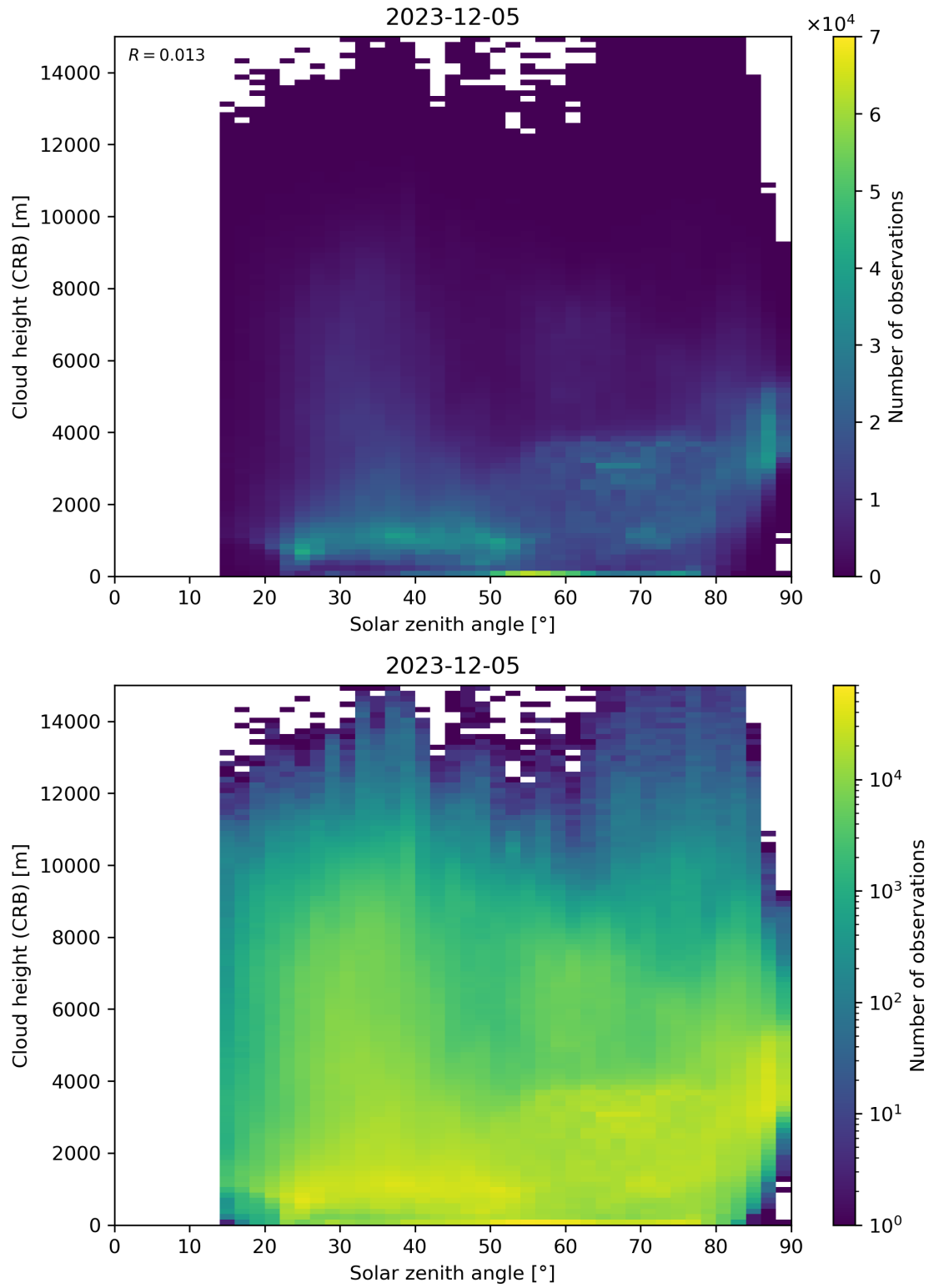
Figure 102: Scatter density plot of “Solar zenith angle” against “Cloud height (CRB)” for 2023-12-04 to 2023-12-06.
