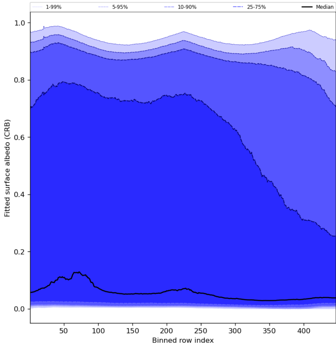
Figure 62: Along track statistics of “Fitted surface albedo (CRB)” for 2023-12-04 to 2023-12-06
