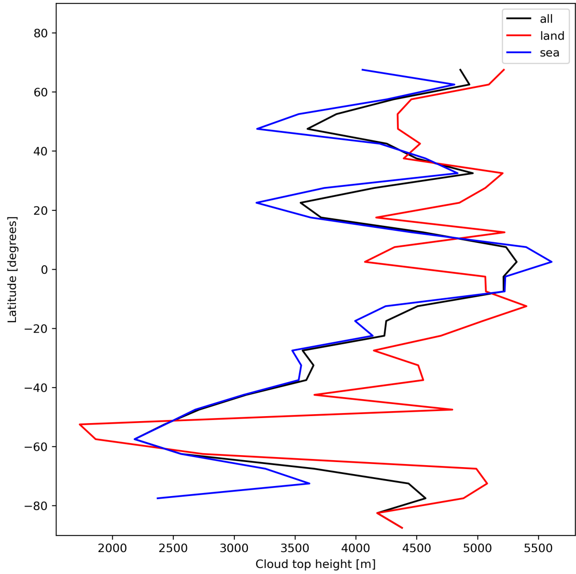
Figure 24: Zonal average of “Cloud top height” for 2023-12-04 to 2023-12-06.
