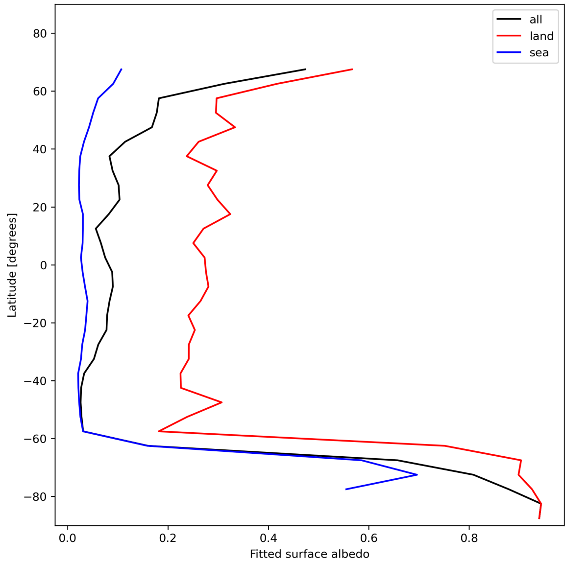
Figure 29: Zonal average of “Fitted surface albedo” for 2023-12-05 to 2023-12-07.
