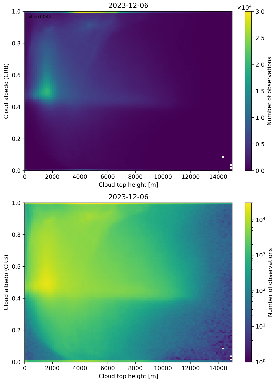
Figure 86: Scatter density plot of “Cloud top height” against “Cloud albedo (CRB)” for 2023-12-05 to 2023-12-07.
