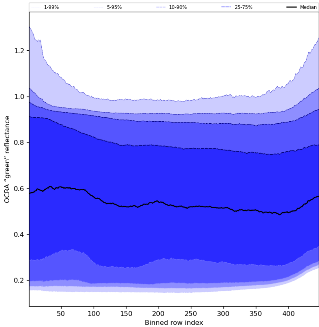
Figure 68: Along track statistics of “OCRA “green” reflectance” for 2023-12-05 to 2023-12-07
