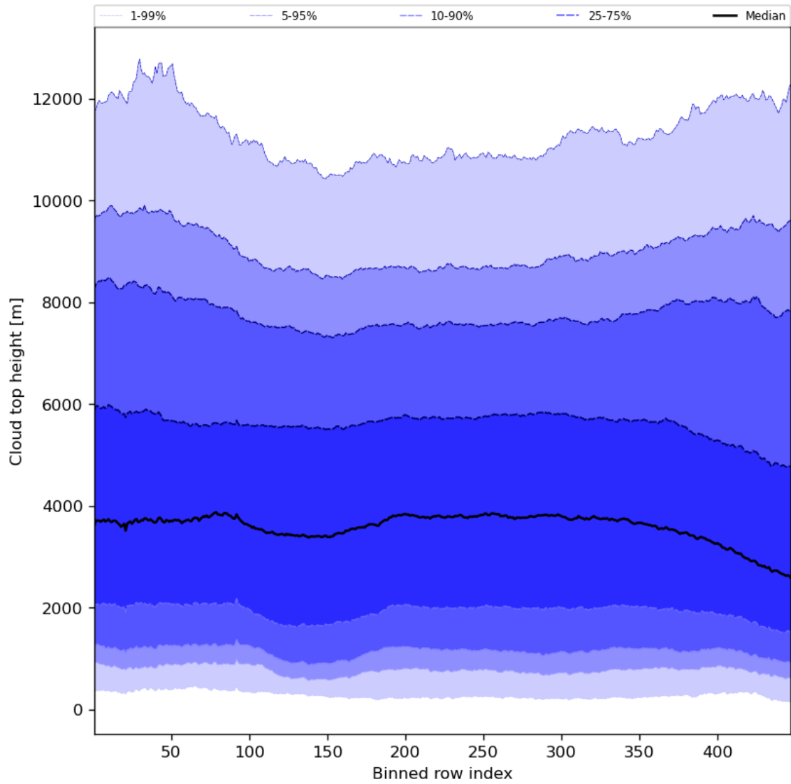
Figure 56: Along track statistics of “Cloud top height” for 2023-12-05 to 2023-12-07
