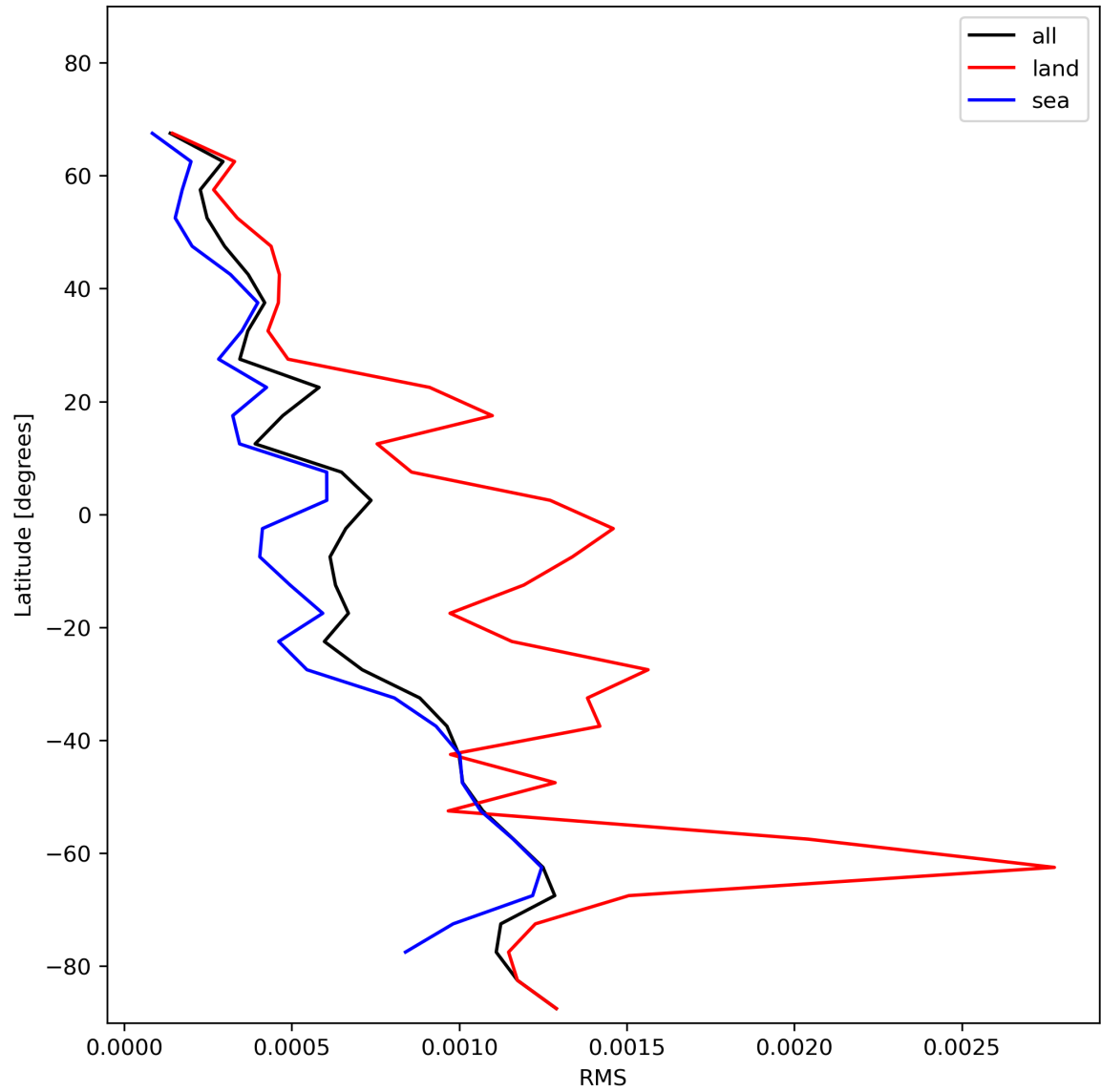
Figure 31: Zonal average of “RMS” for 2023-12-05 to 2023-12-07.
