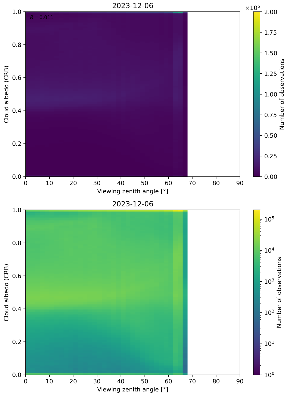
Figure 106: Scatter density plot of “Viewing zenith angle” against “Cloud albedo (CRB)” for 2023-12-05 to 2023-12-07.
