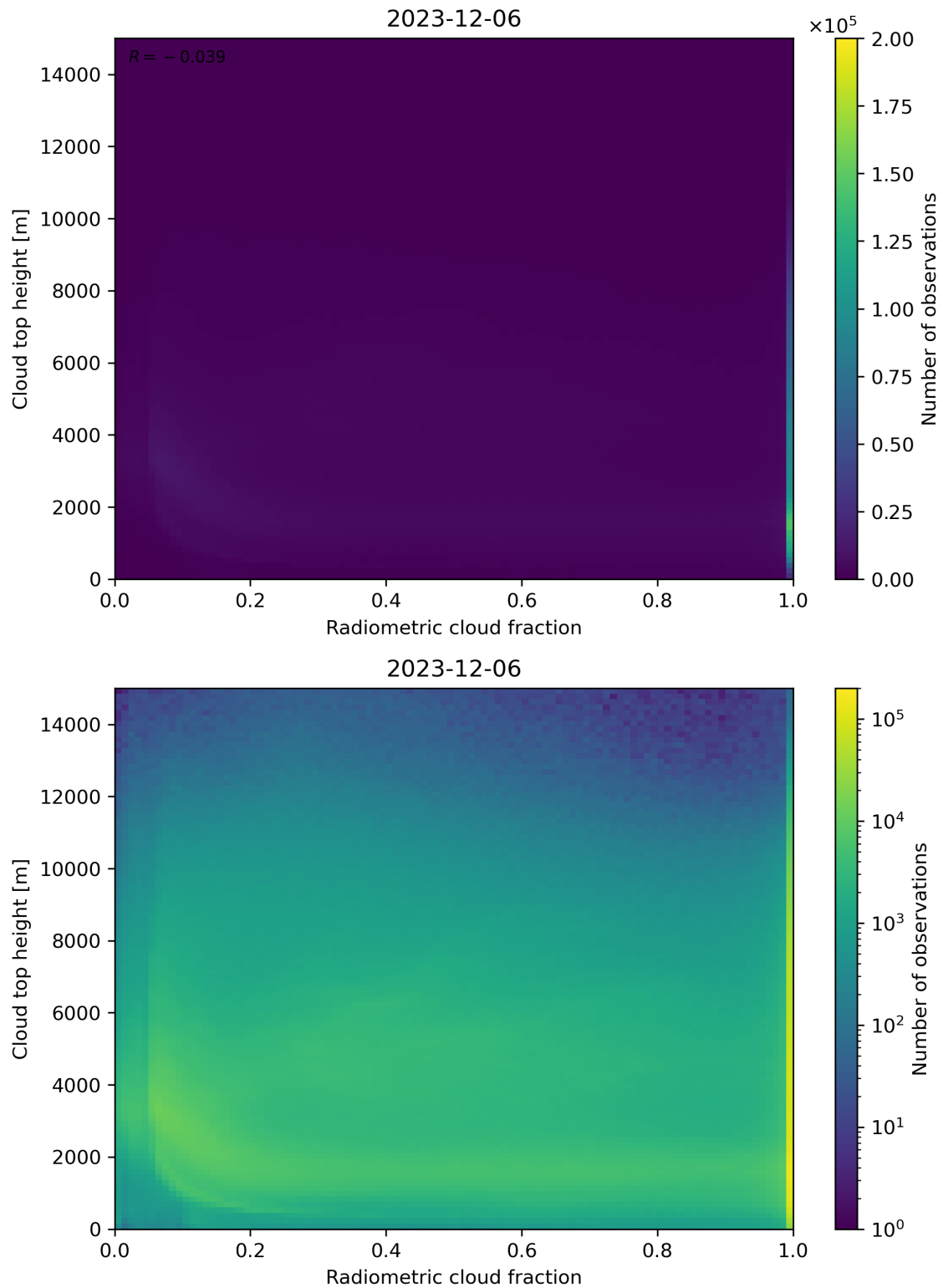
Figure 76: Scatter density plot of “Radiometric cloud fraction” against “Cloud top height” for 2023-12-05 to 2023-12-07.
