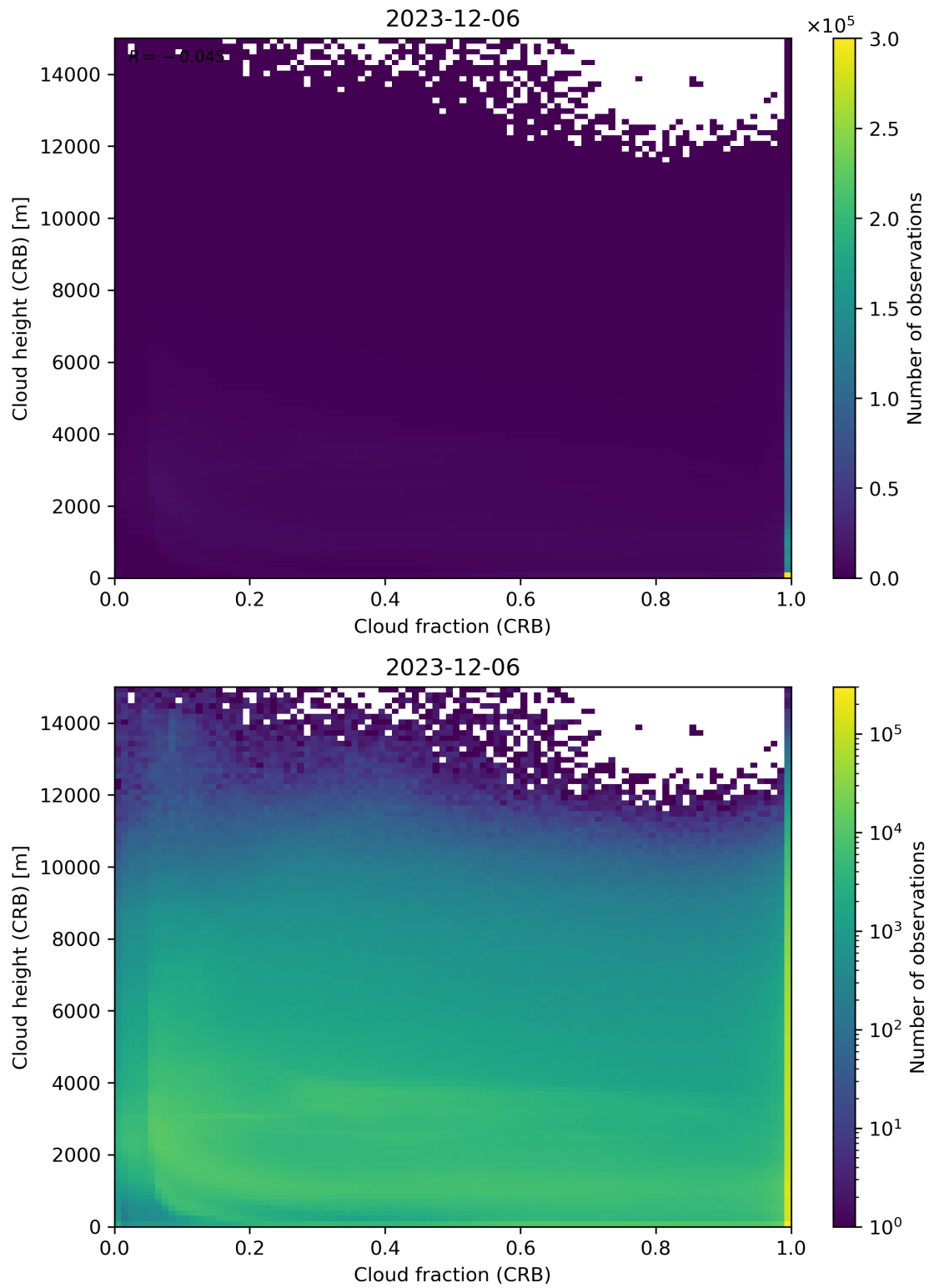
Figure 79: Scatter density plot of “Cloud fraction (CRB)” against “Cloud height (CRB)” for 2023-12-05 to 2023-12-07.
