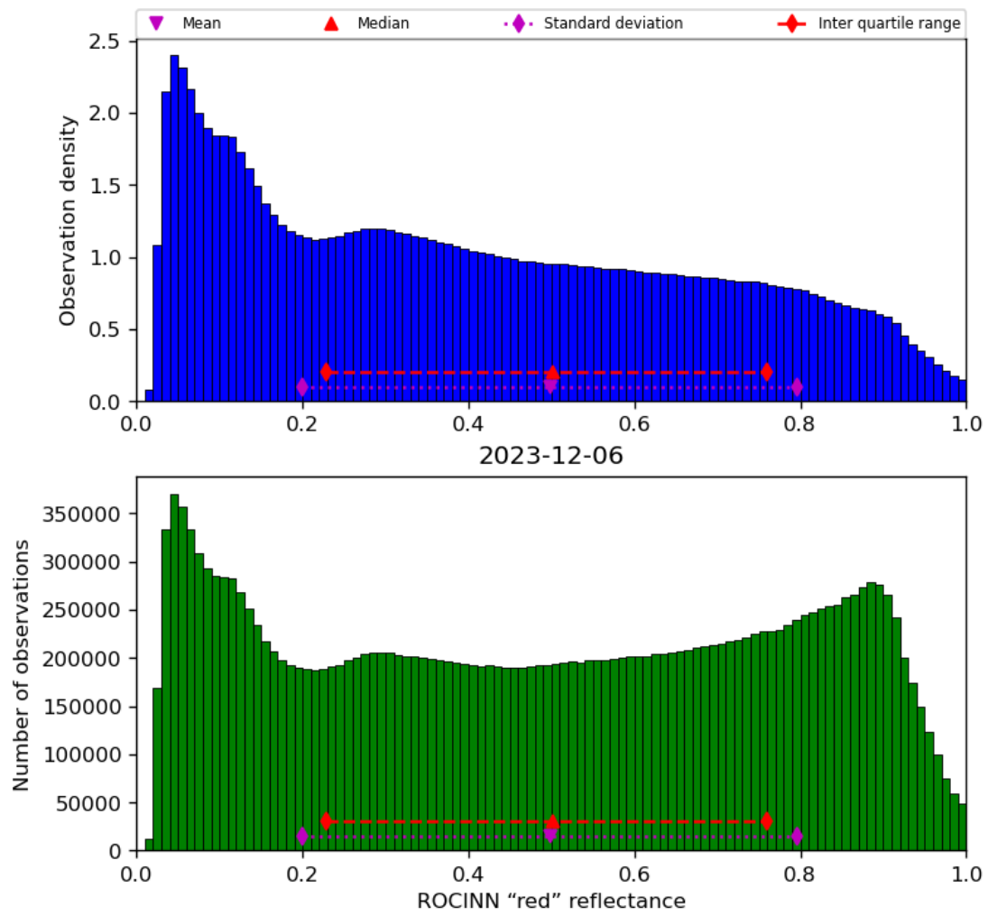
Figure 53: Histogram of “ROCINN “red” reflectance” for 2023-12-05 to 2023-12-07
