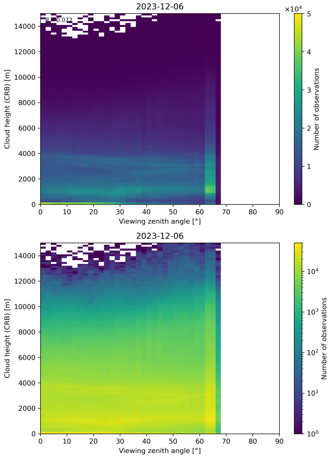
Figure 110: Scatter density plot of “Viewing zenith angle” against “Cloud height (CRB)” for 2023-12-05 to 2023-12-07.
