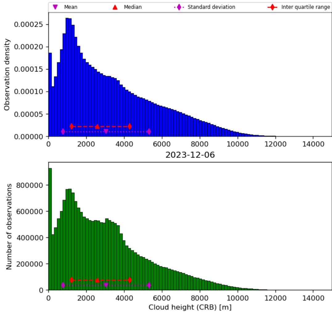
Figure 43: Histogram of “Cloud height (CRB)” for 2023-12-05 to 2023-12-07
