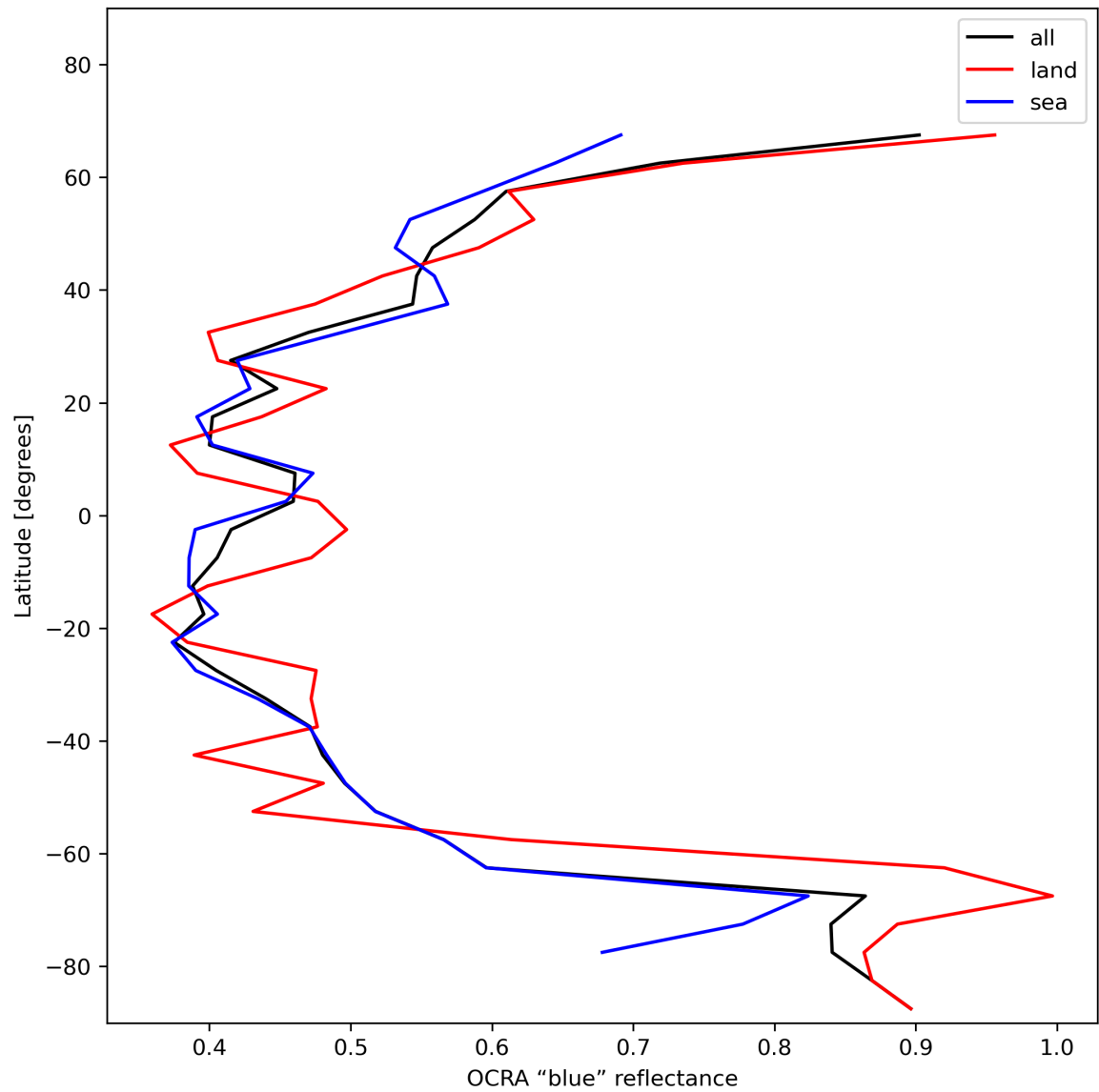
Figure 35: Zonal average of “OCRA “blue” reflectance” for 2023-12-05 to 2023-12-07.
