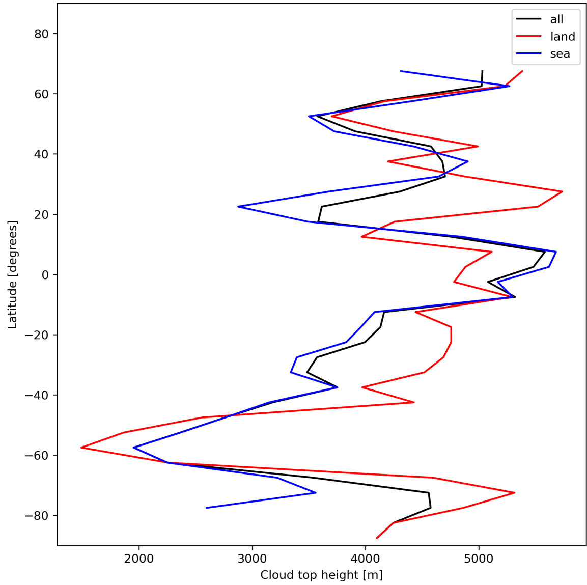
Figure 24: Zonal average of “Cloud top height” for 2023-12-05 to 2023-12-07.
