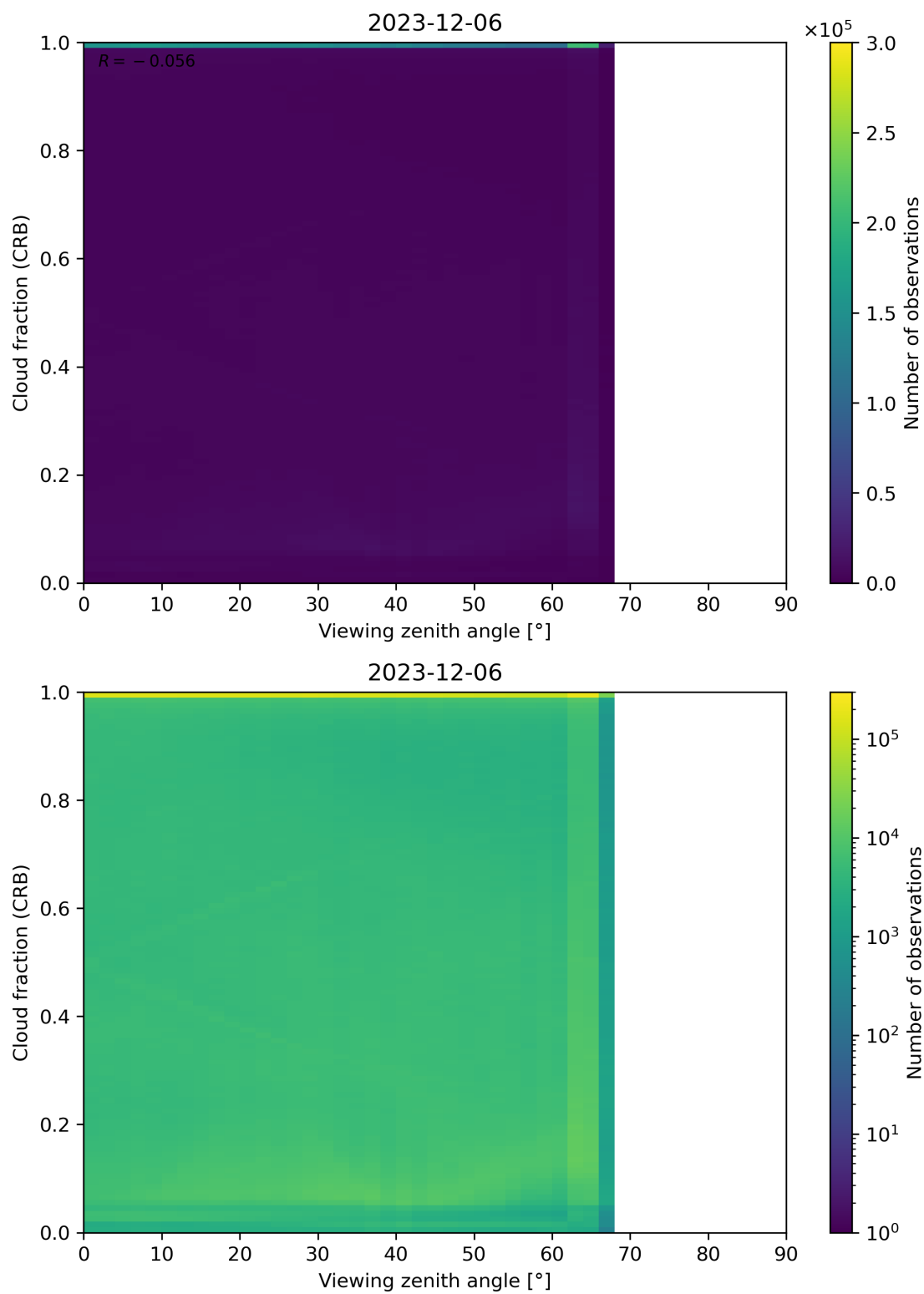
Figure 109: Scatter density plot of “Viewing zenith angle” against “Cloud fraction (CRB)” for 2023-12-05 to 2023-12-07.
