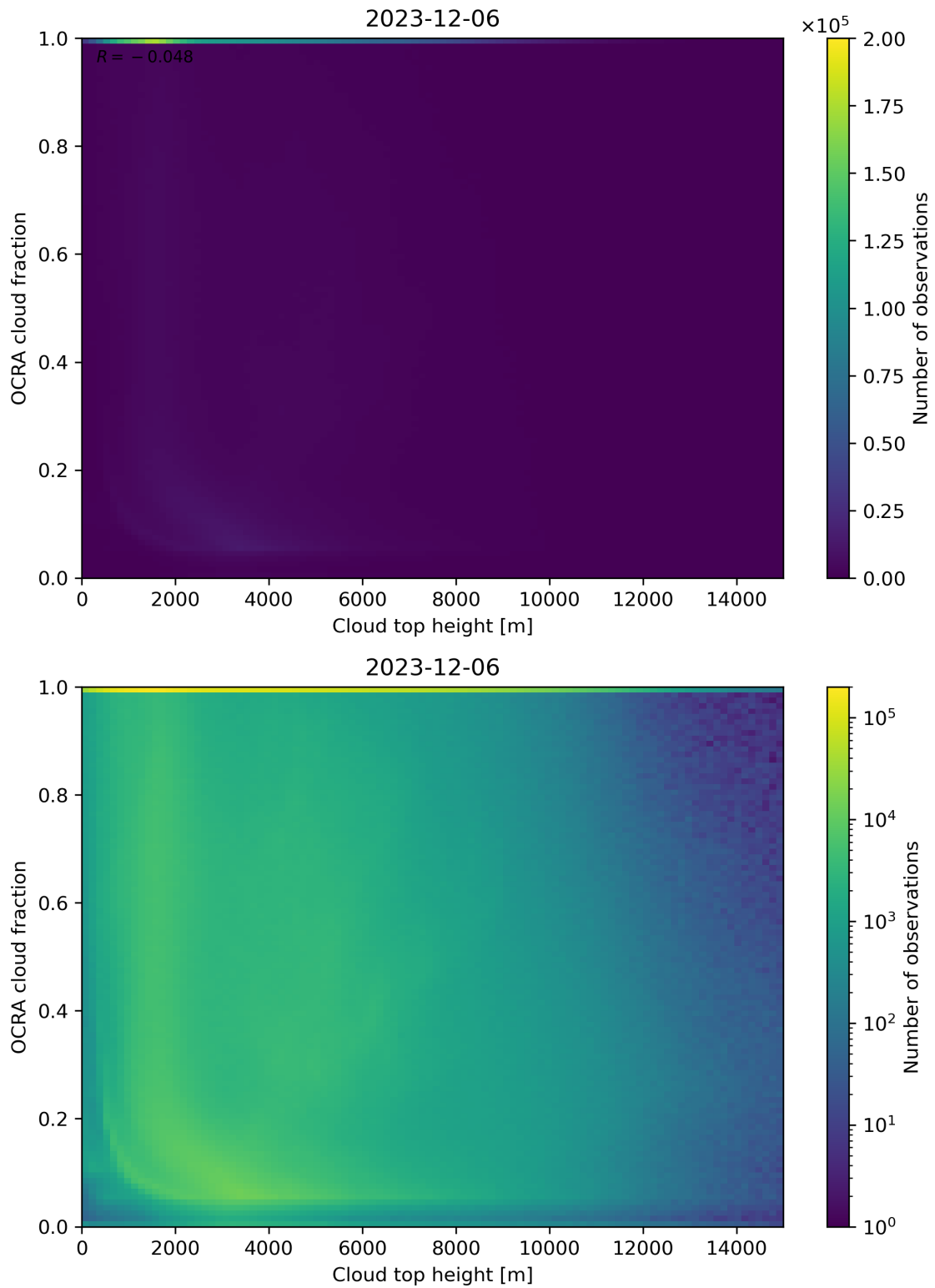
Figure 87: Scatter density plot of “Cloud top height” against “OCRA cloud fraction” for 2023-12-05 to 2023-12-07.
