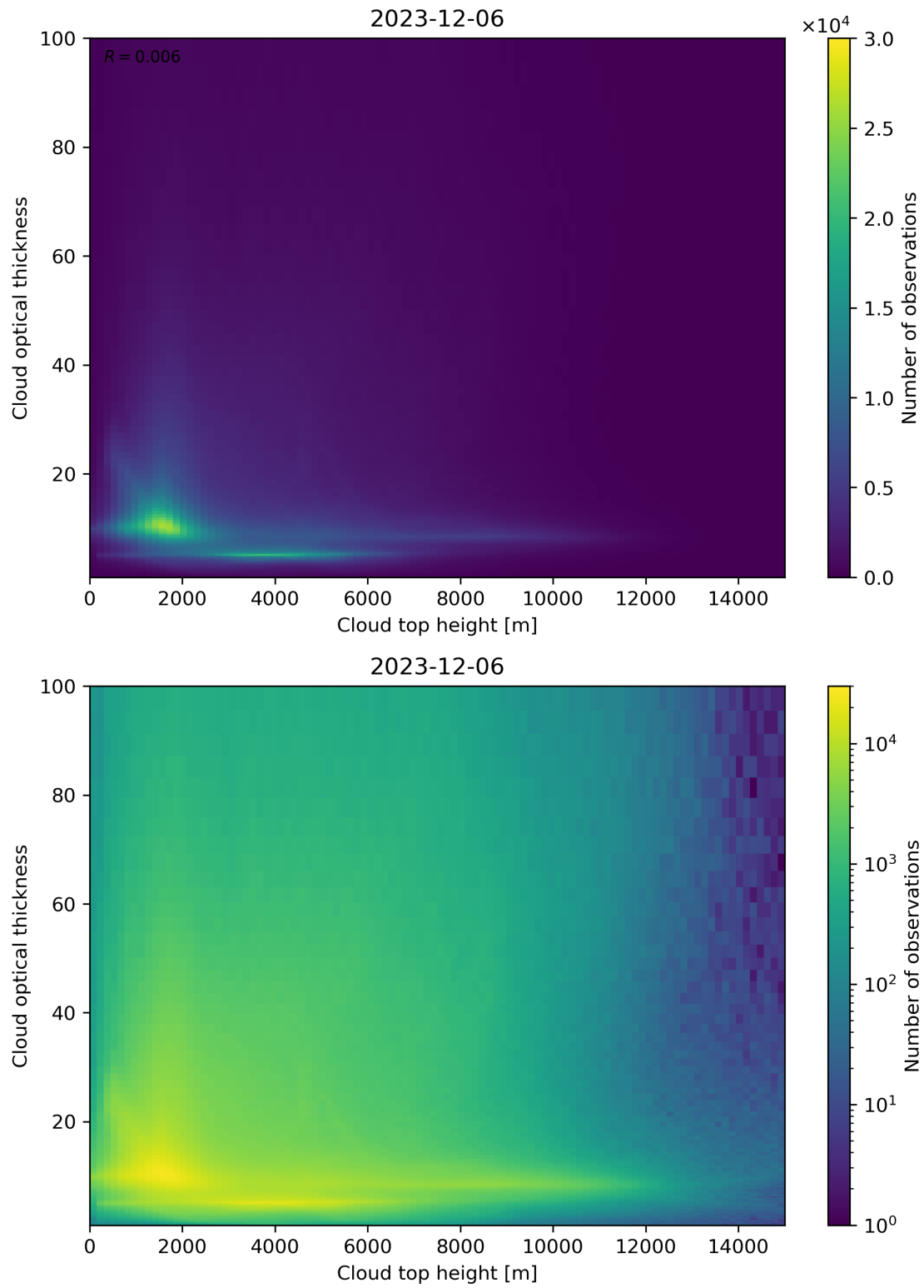
Figure 90: Scatter density plot of “Cloud top height” against “Cloud optical thickness” for 2023-12-05 to 2023-12-07.
