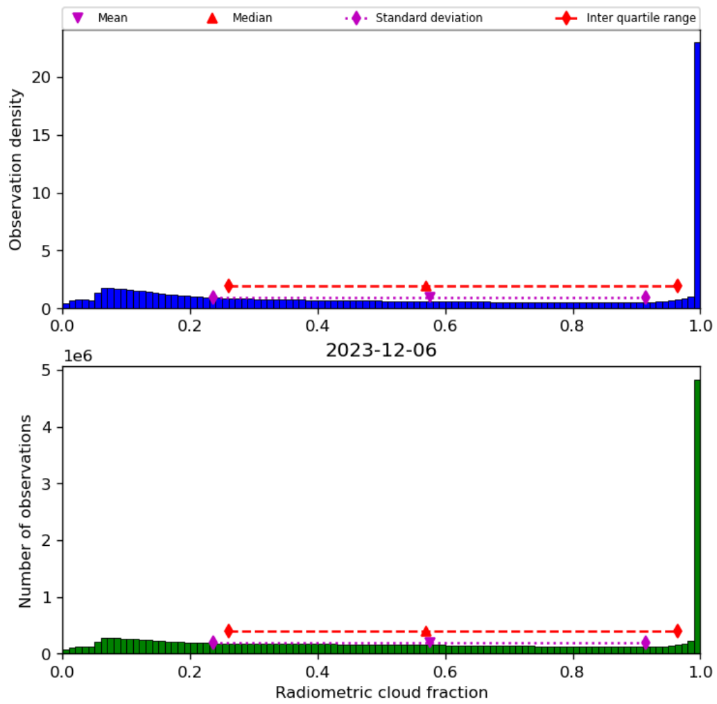
Figure 39: Histogram of “Radiometric cloud fraction” for 2023-12-05 to 2023-12-07
