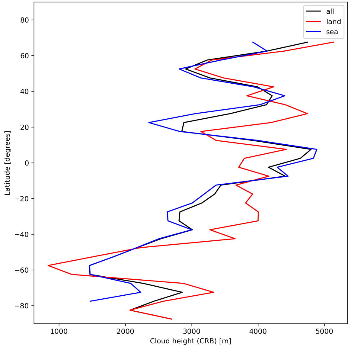
Figure 27: Zonal average of “Cloud height (CRB)” for 2023-12-05 to 2023-12-07.
