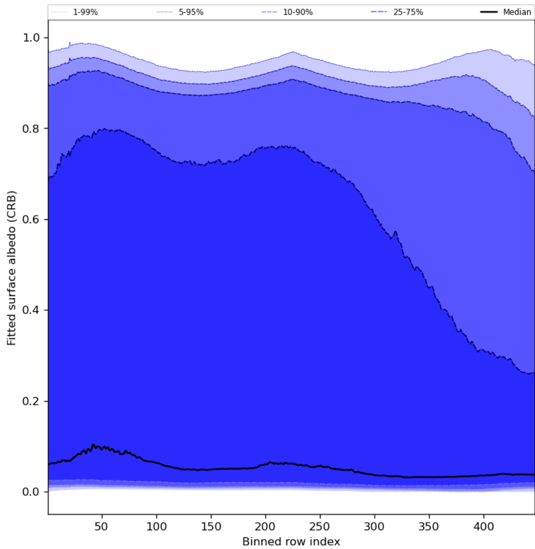
Figure 62: Along track statistics of “Fitted surface albedo (CRB)” for 2023-12-05 to 2023-12-07
