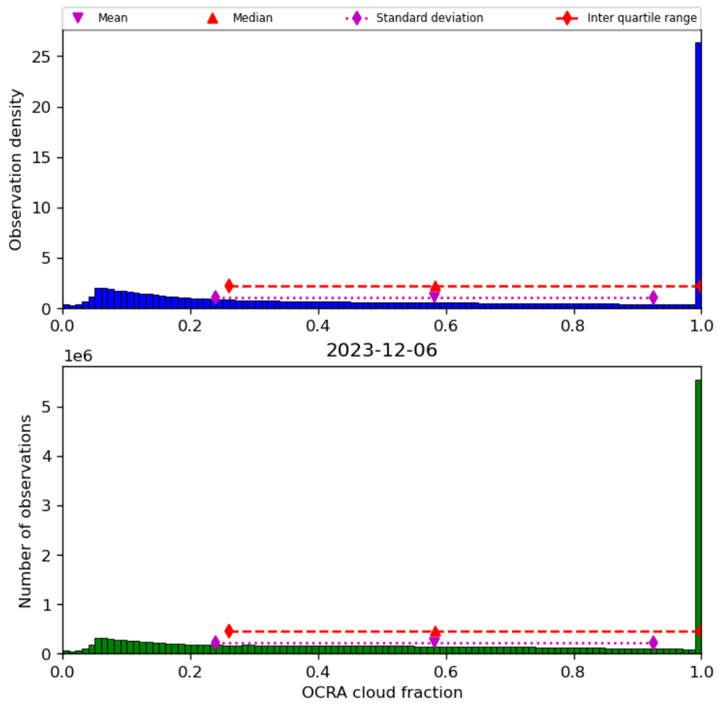
Figure 50: Histogram of “OCRA cloud fraction” for 2023-12-05 to 2023-12-07
