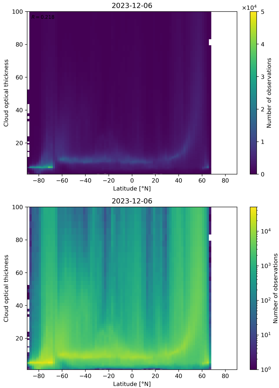
Figure 96: Scatter density plot of “Latitude” against “Cloud optical thickness” for 2023-12-05 to 2023-12-07.
