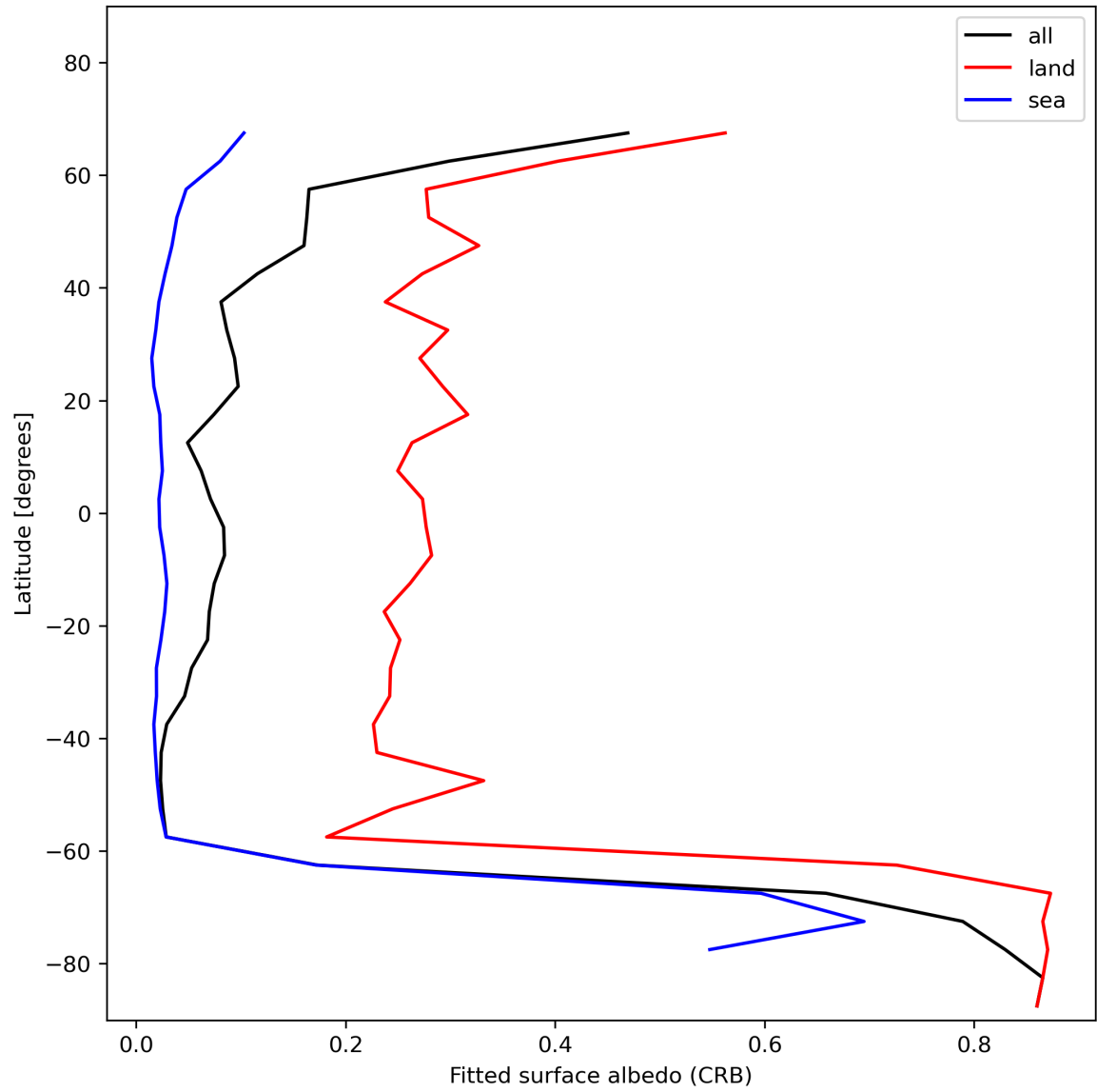
Figure 30: Zonal average of “Fitted surface albedo (CRB)” for 2023-12-05 to 2023-12-07.
