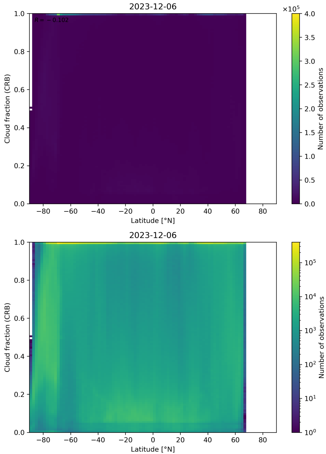
Figure 94: Scatter density plot of “Latitude” against “Cloud fraction (CRB)” for 2023-12-05 to 2023-12-07.
