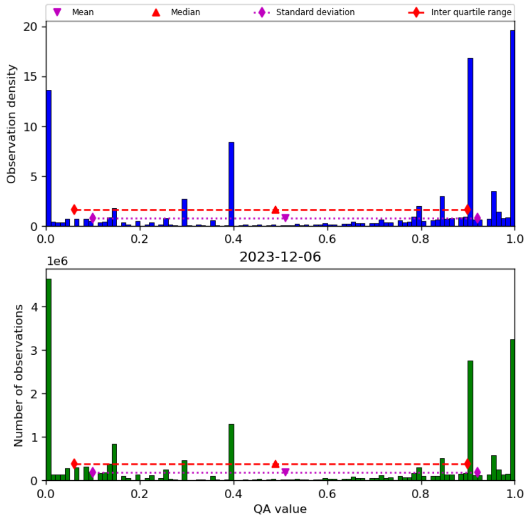
Figure 38: Histogram of “QA value” for 2023-12-05 to 2023-12-07
