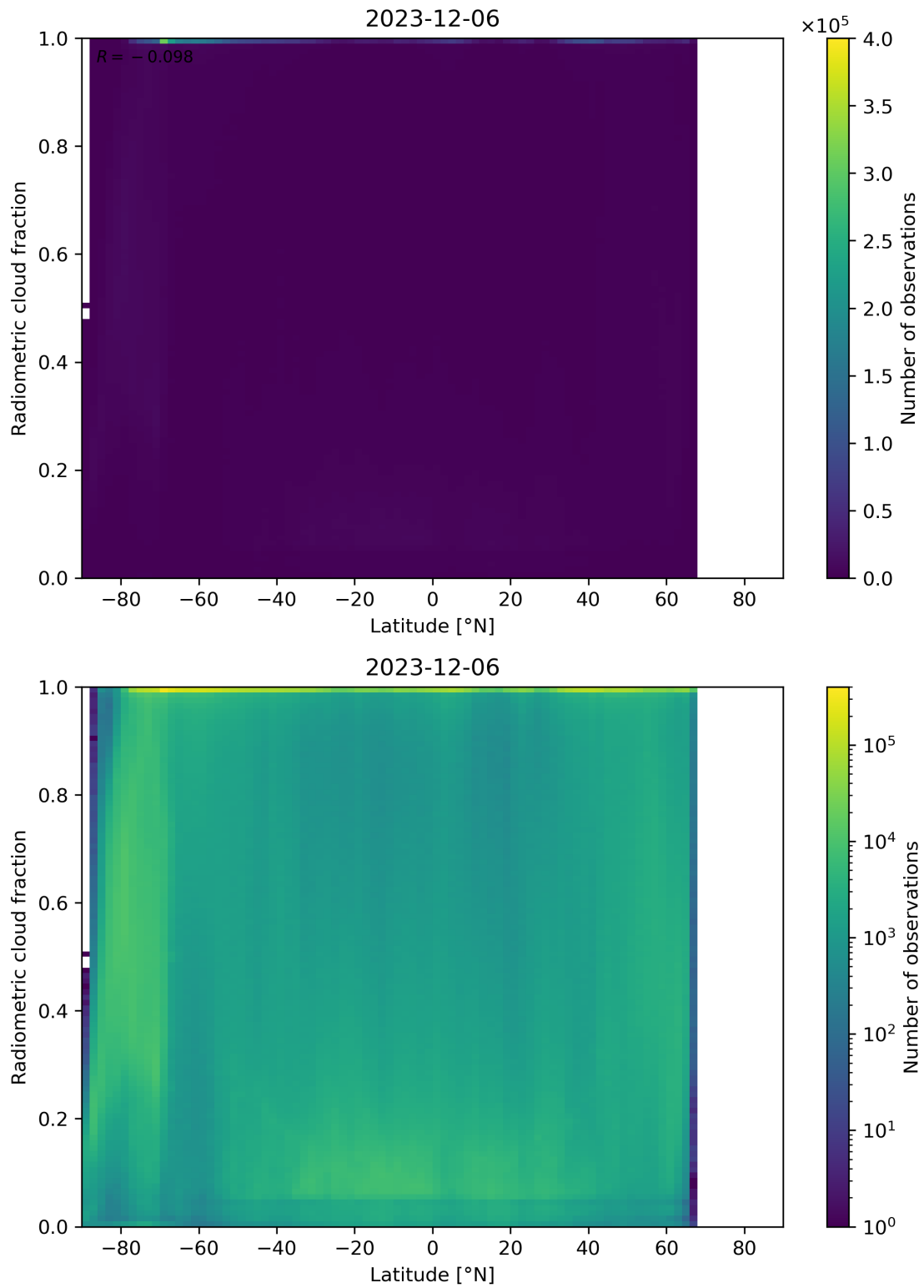
Figure 92: Scatter density plot of “Latitude” against “Radiometric cloud fraction” for 2023-12-05 to 2023-12-07.
