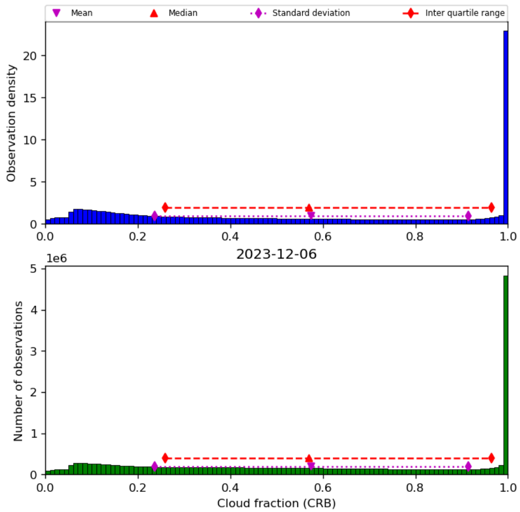
Figure 42: Histogram of “Cloud fraction (CRB)” for 2023-12-05 to 2023-12-07
