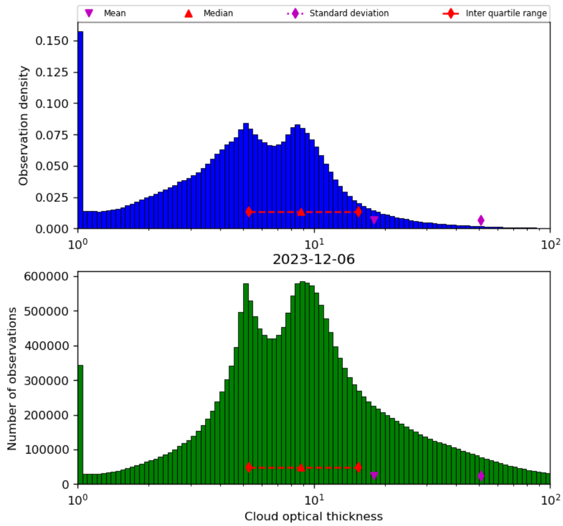
Figure 41: Histogram of “Cloud optical thickness” for 2023-12-05 to 2023-12-07
