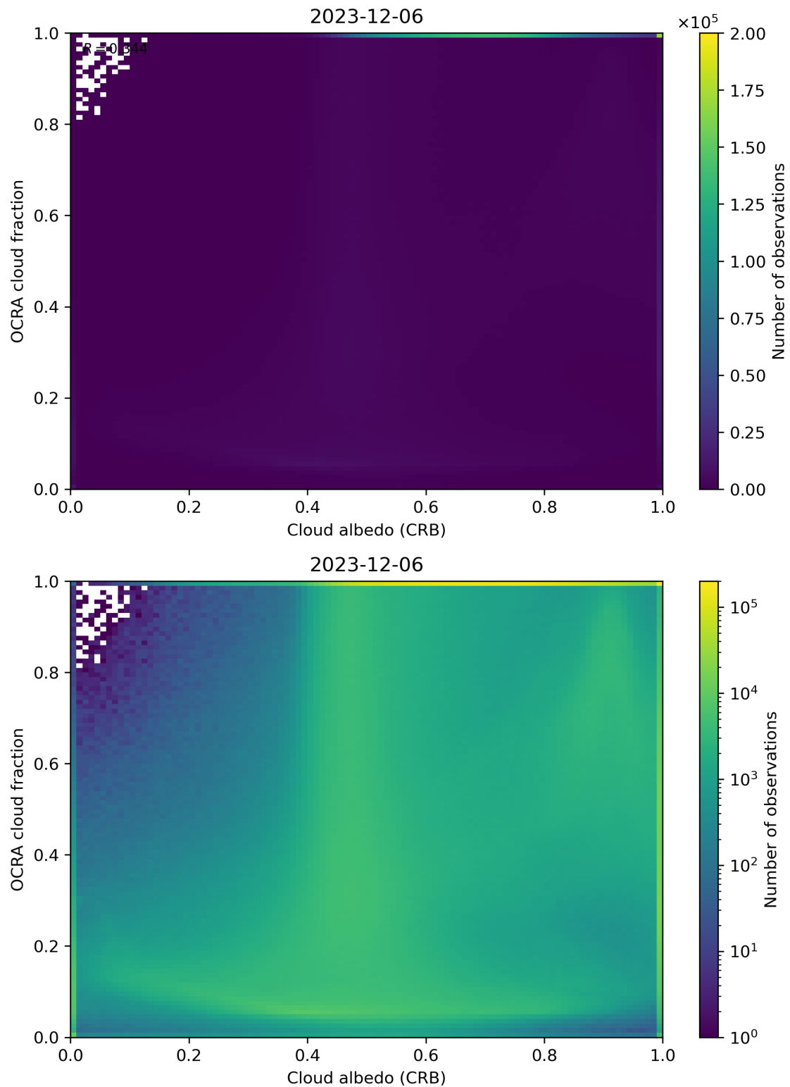
Figure 70: Scatter density plot of “Cloud albedo (CRB)” against “OCRA cloud fraction” for 2023-12-05 to 2023-12-07.
