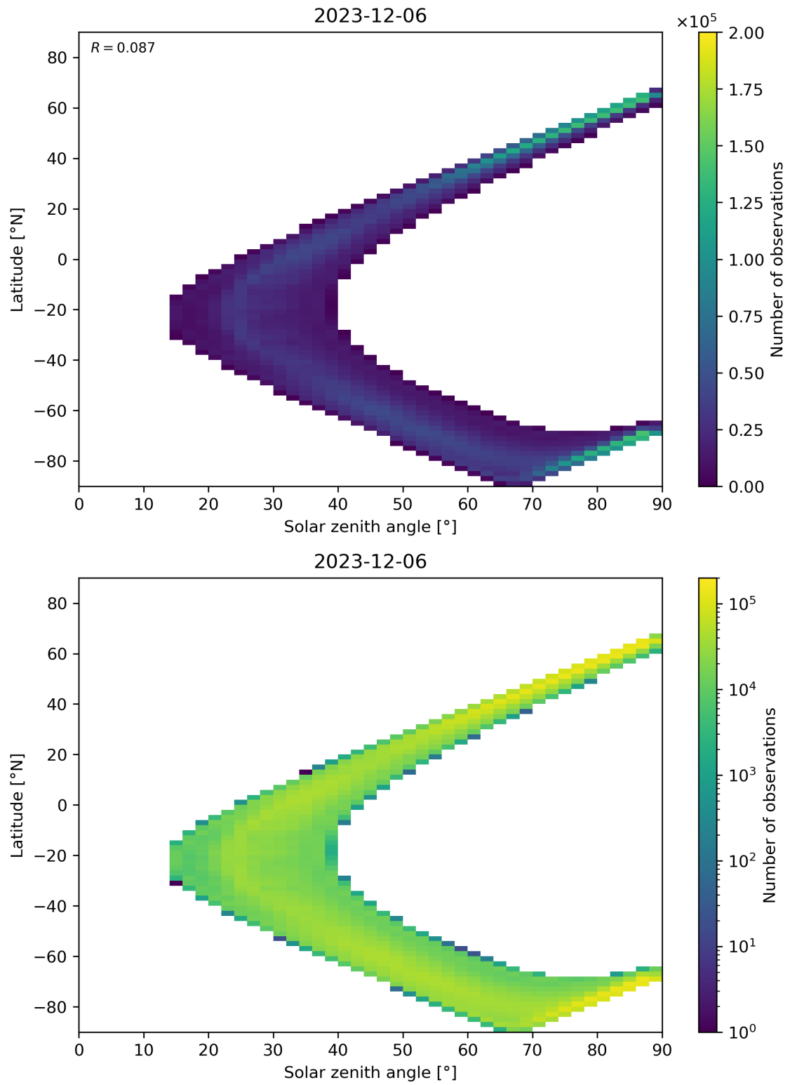
Figure 105: Scatter density plot of “Solar zenith angle” against “Latitude” for 2023-12-05 to 2023-12-07.
