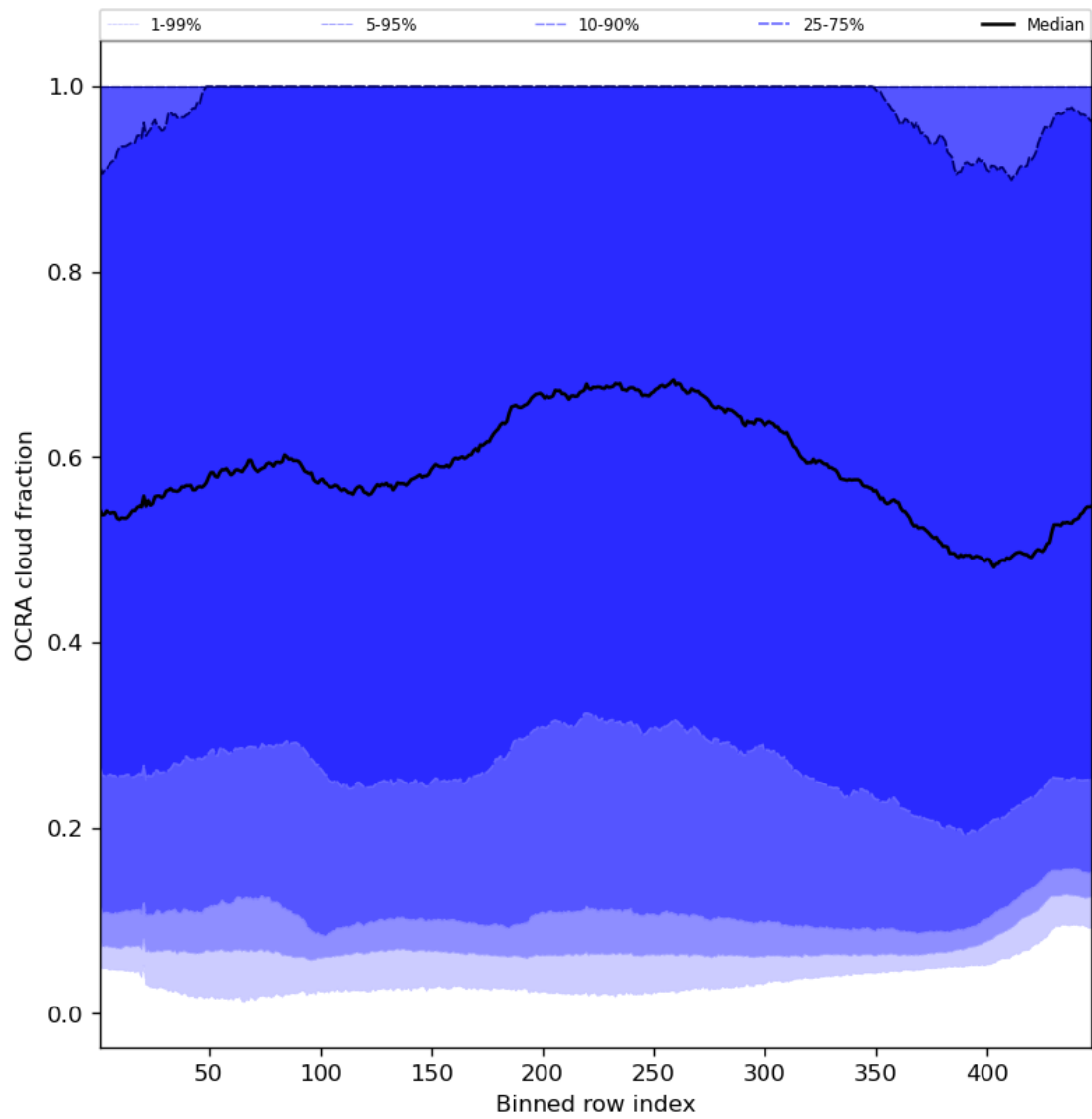
Figure 66: Along track statistics of “OCRA cloud fraction” for 2023-12-05 to 2023-12-07
