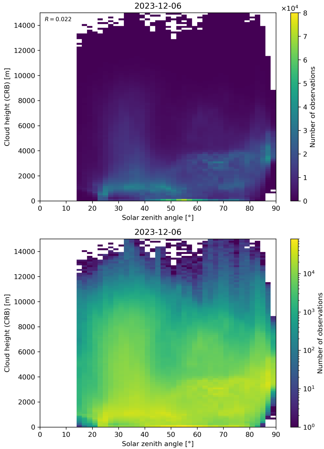
Figure 102: Scatter density plot of “Solar zenith angle” against “Cloud height (CRB)” for 2023-12-05 to 2023-12-07.
