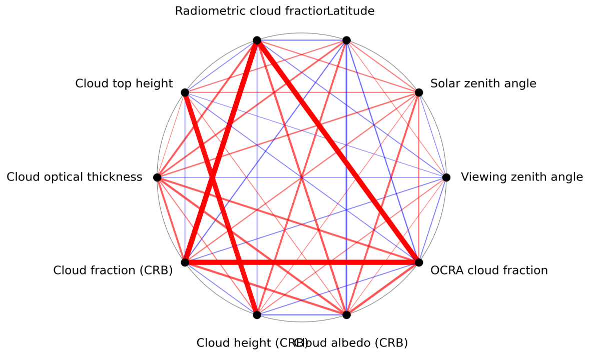
Figure 1: Map of correlation graph for 2023-12-05 to 2023-12-07.
