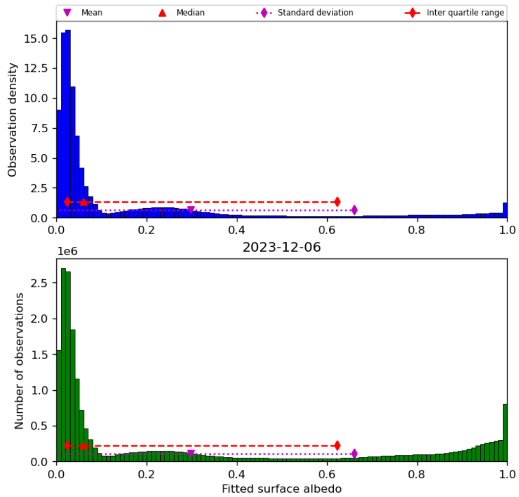
Figure 45: Histogram of “Fitted surface albedo” for 2023-12-05 to 2023-12-07
