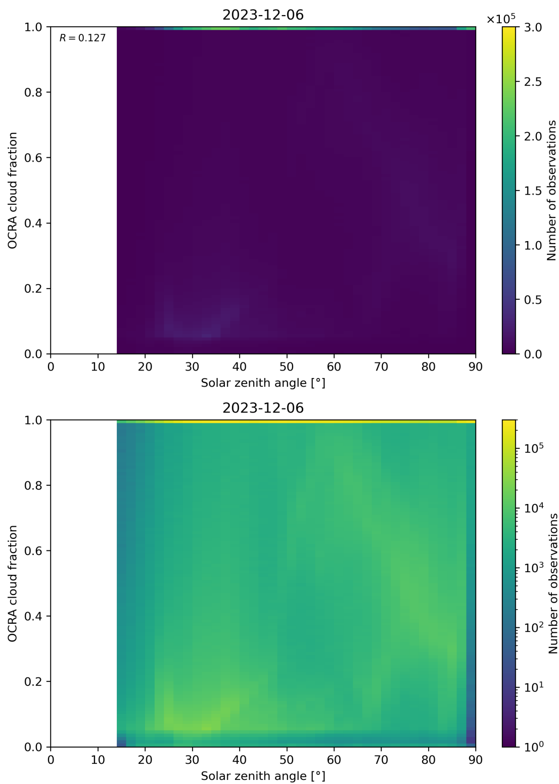
Figure 100: Scatter density plot of “Solar zenith angle” against “OCRA cloud fraction” for 2023-12-05 to 2023-12-07.
