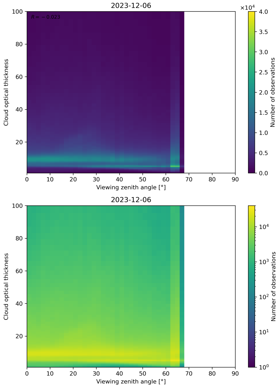
Figure 111: Scatter density plot of “Viewing zenith angle” against “Cloud optical thickness” for 2023-12-05 to 2023-12-07.
