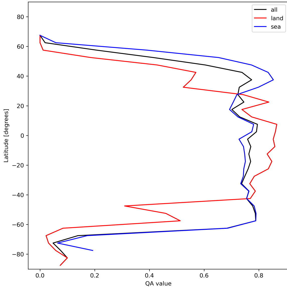
Figure 22: Zonal average of “QA value” for 2023-12-05 to 2023-12-07.
