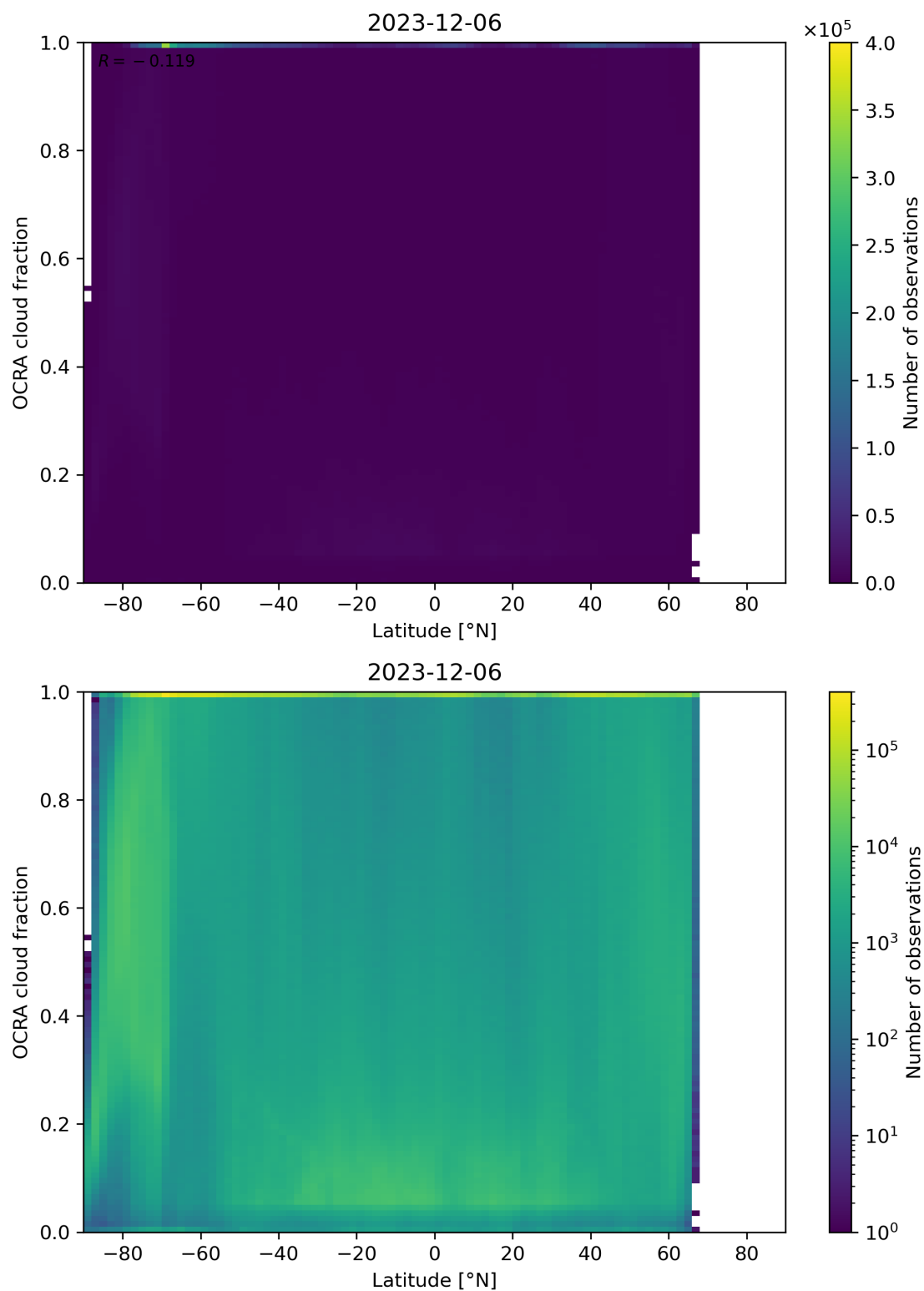
Figure 93: Scatter density plot of “Latitude” against “OCRA cloud fraction” for 2023-12-05 to 2023-12-07.
