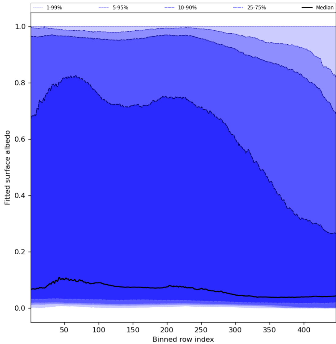
Figure 61: Along track statistics of “Fitted surface albedo” for 2023-12-05 to 2023-12-07
