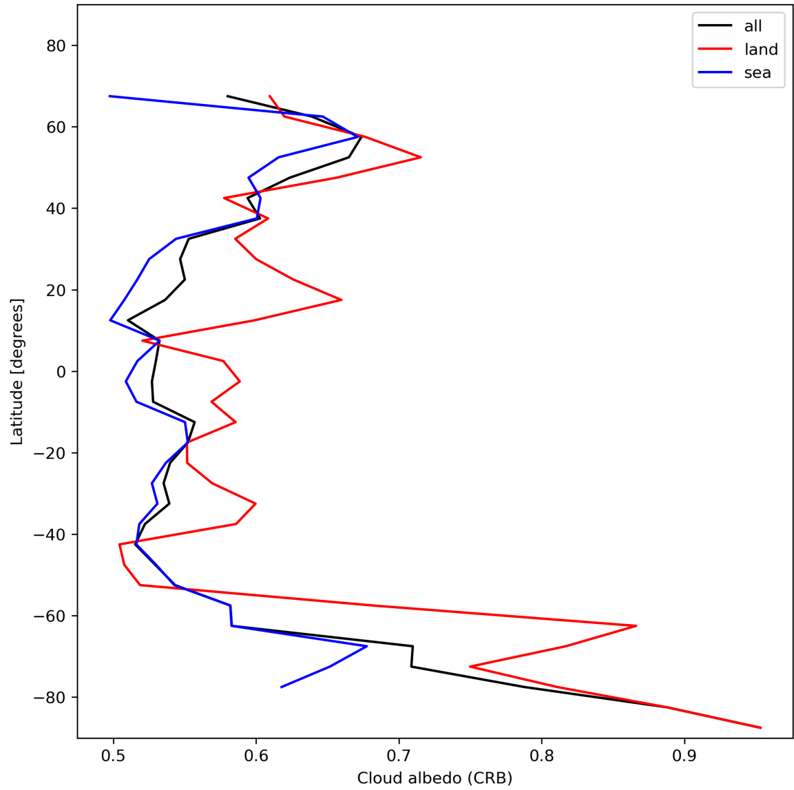
Figure 28: Zonal average of “Cloud albedo (CRB)” for 2023-12-05 to 2023-12-07.
