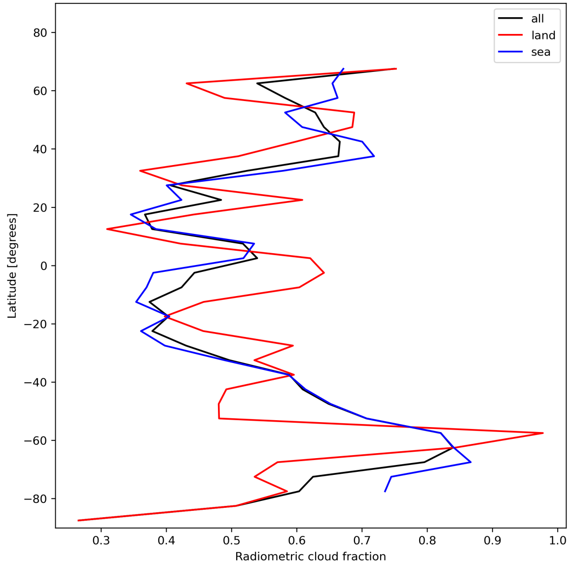
Figure 23: Zonal average of “Radiometric cloud fraction” for 2023-12-05 to 2023-12-07.
