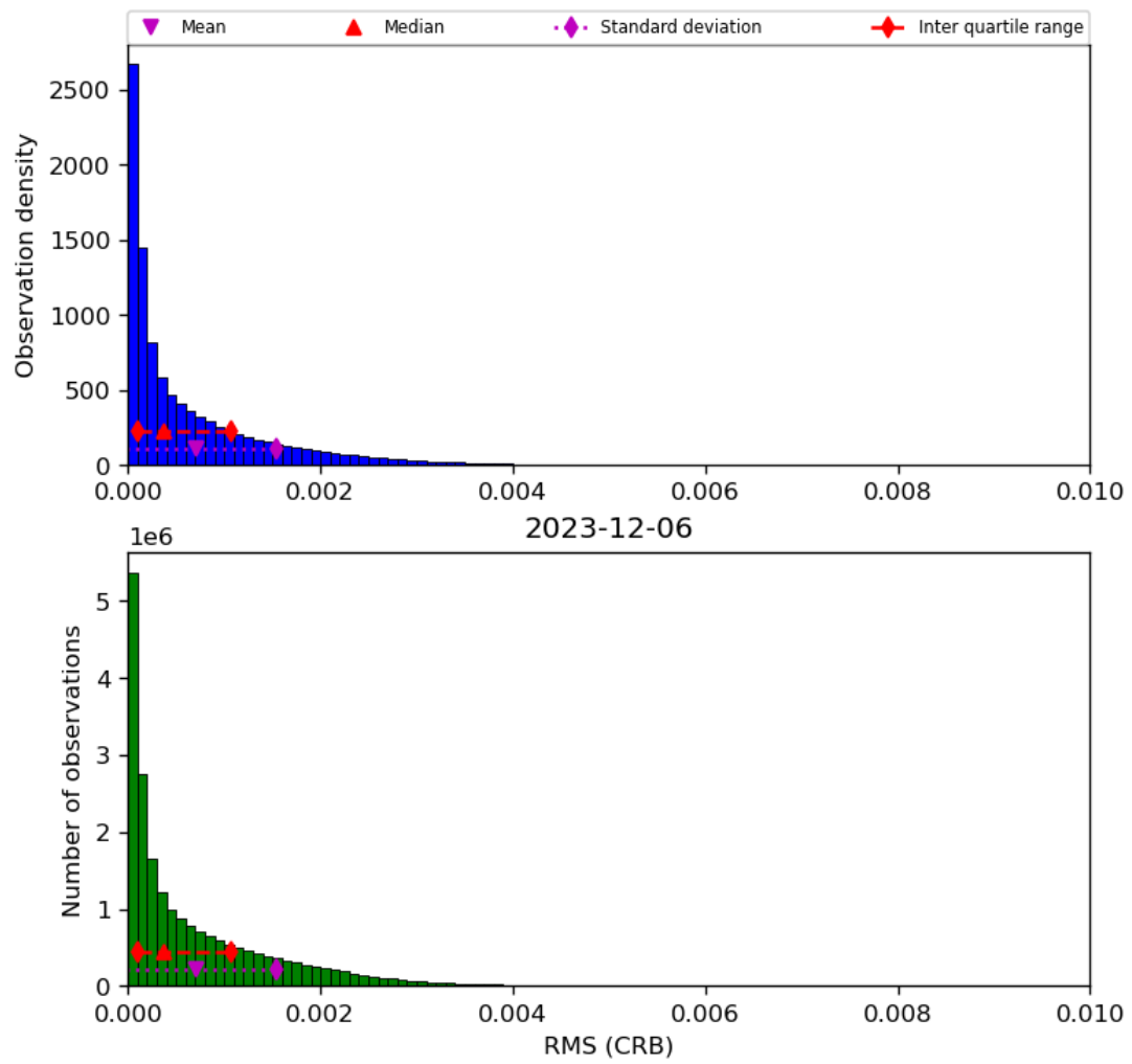
Figure 48: Histogram of “RMS (CRB)” for 2023-12-05 to 2023-12-07
