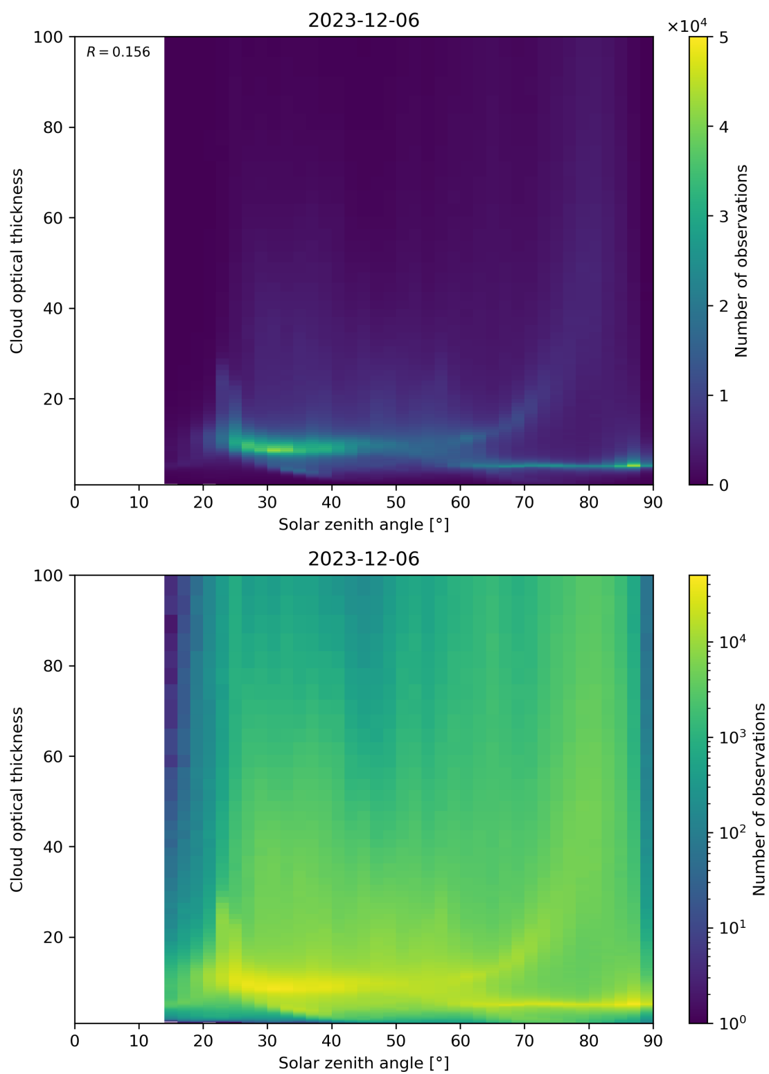
Figure 103: Scatter density plot of “Solar zenith angle” against “Cloud optical thickness” for 2023-12-05 to 2023-12-07.
