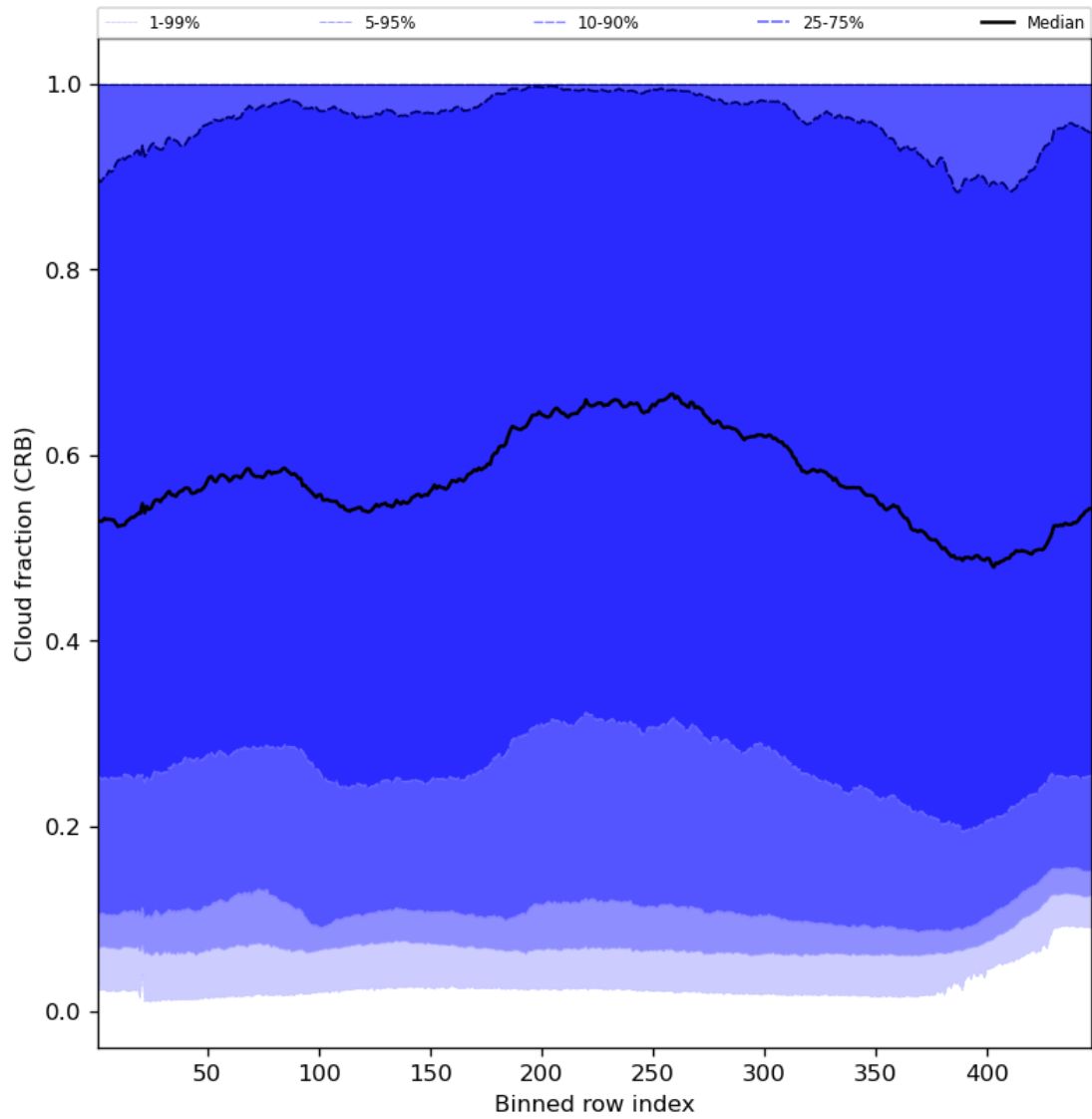
Figure 58: Along track statistics of “Cloud fraction (CRB)” for 2023-12-05 to 2023-12-07
