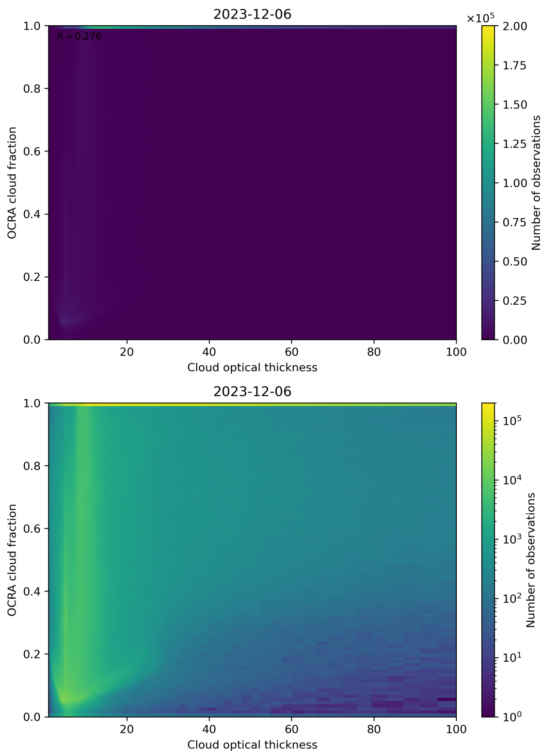
Figure 83: Scatter density plot of “Cloud optical thickness” against “OCRA cloud fraction” for 2023-12-05 to 2023-12-07.
