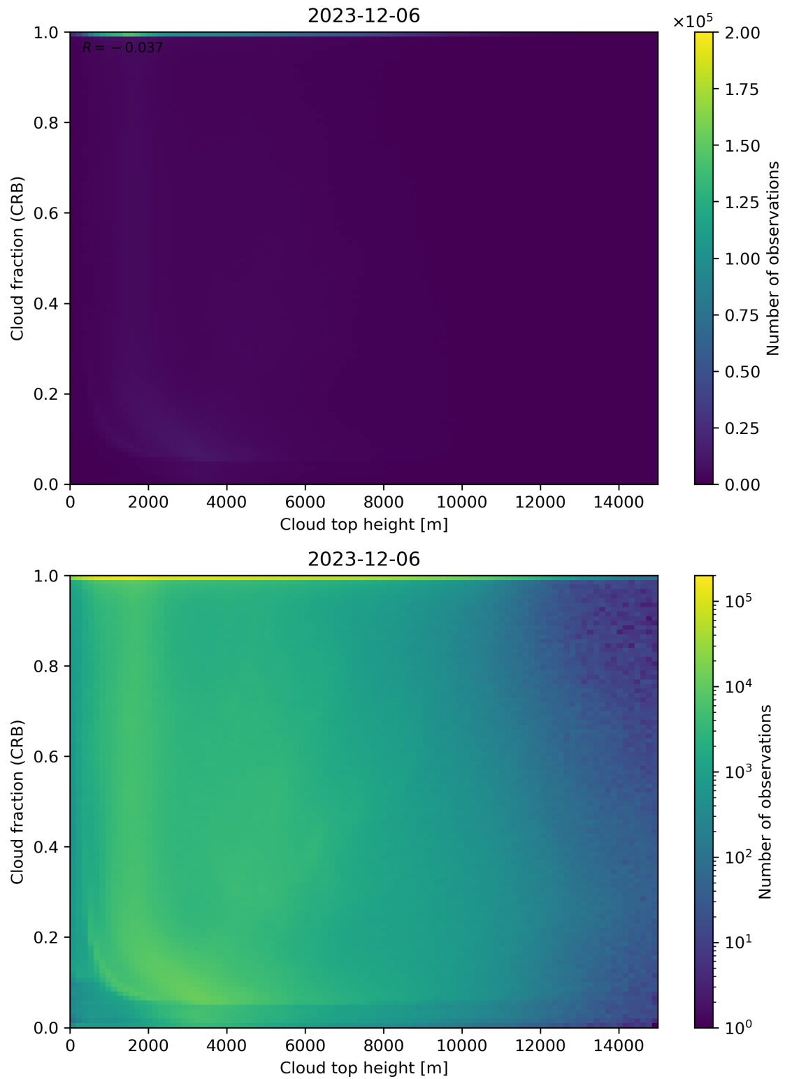
Figure 88: Scatter density plot of “Cloud top height” against “Cloud fraction (CRB)” for 2023-12-05 to 2023-12-07.
