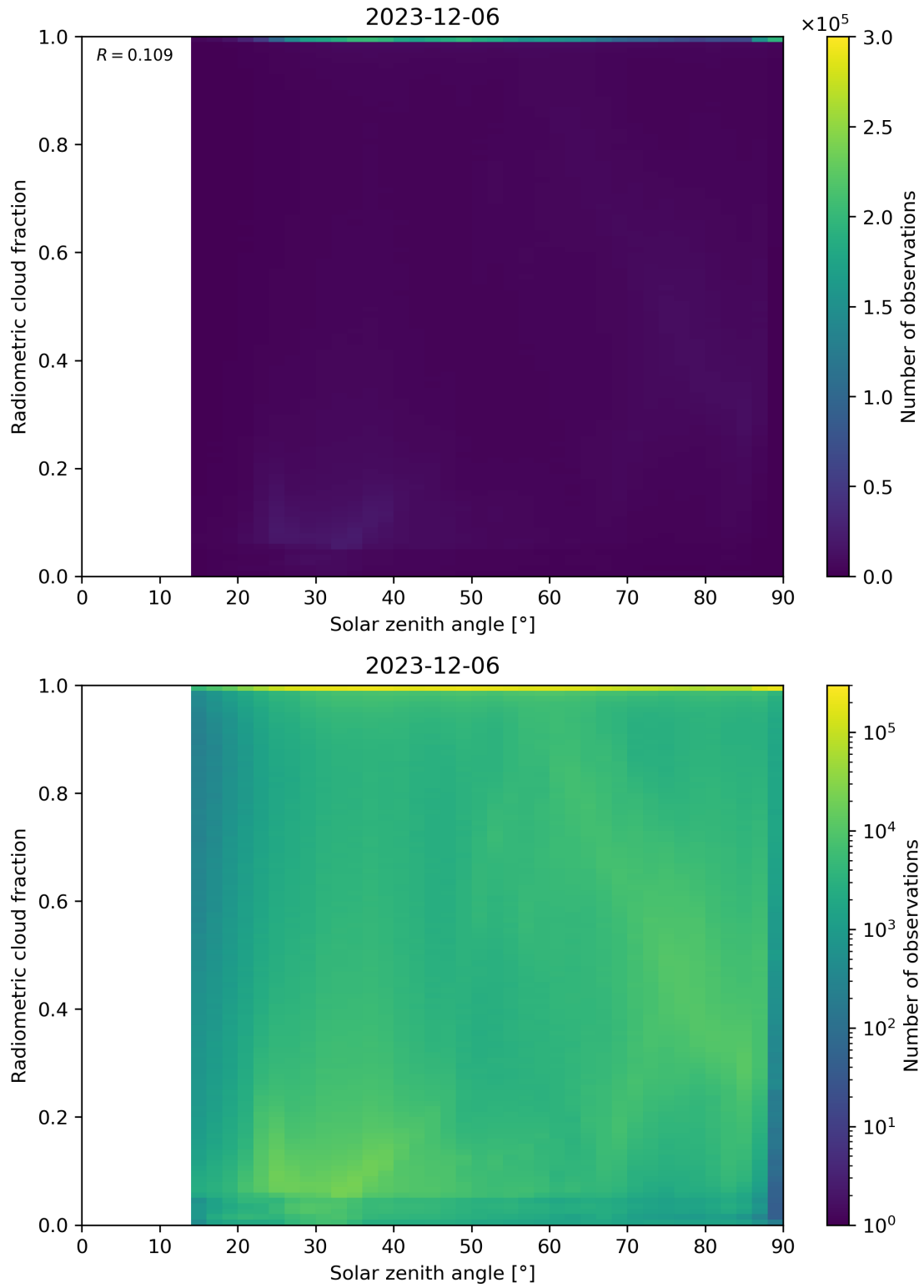
Figure 99: Scatter density plot of “Solar zenith angle” against “Radiometric cloud fraction” for 2023-12-05 to 2023-12-07.
