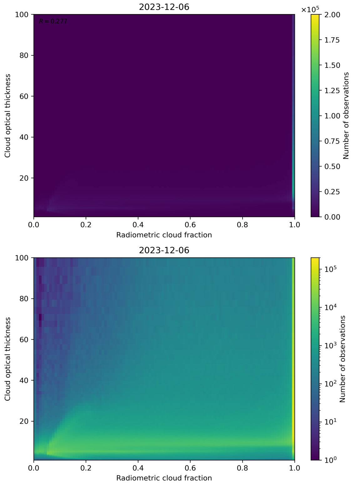
Figure 75: Scatter density plot of “Radiometric cloud fraction” against “Cloud optical thickness” for 2023-12-05 to 2023-12-07.
