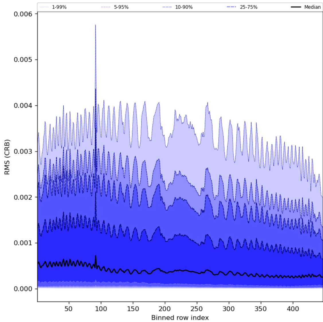
Figure 64: Along track statistics of “RMS (CRB)” for 2023-12-05 to 2023-12-07
