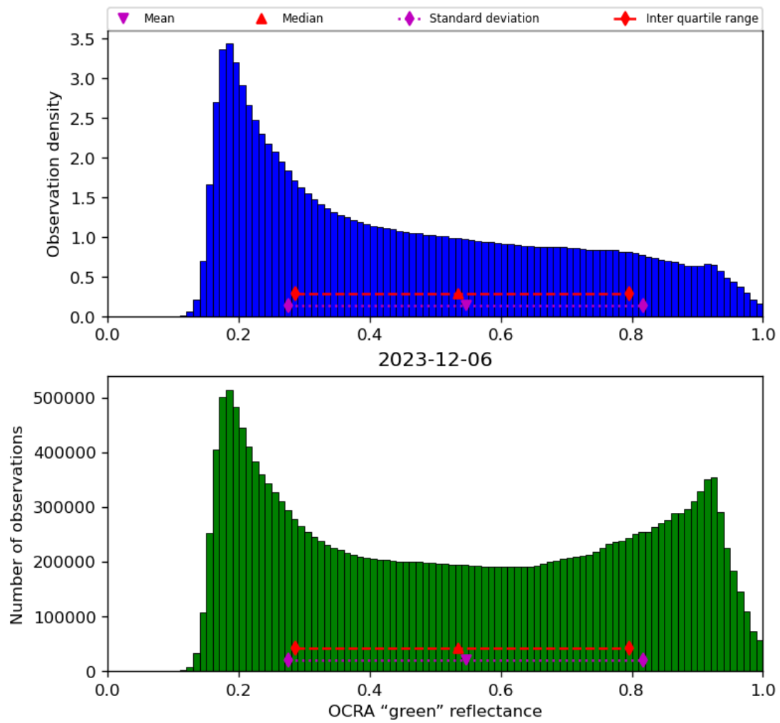
Figure 52: Histogram of “OCRA “green” reflectance” for 2023-12-05 to 2023-12-07
