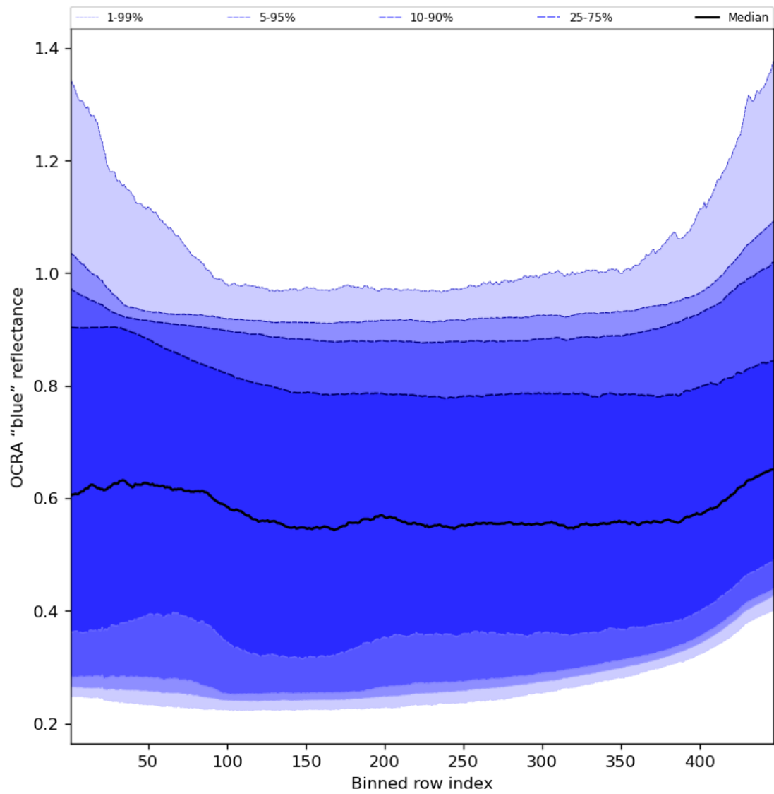
Figure 67: Along track statistics of “OCRA “blue” reflectance” for 2023-12-05 to 2023-12-07
