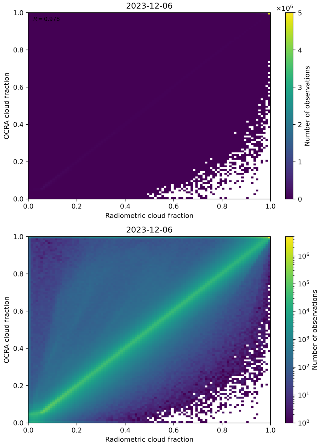
Figure 72: Scatter density plot of “Radiometric cloud fraction” against “OCRA cloud fraction” for 2023-12-05 to 2023-12-07.
