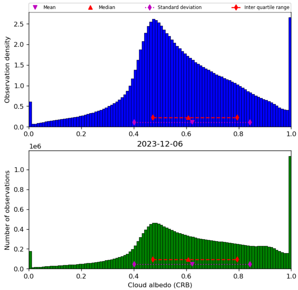
Figure 44: Histogram of “Cloud albedo (CRB)” for 2023-12-05 to 2023-12-07
