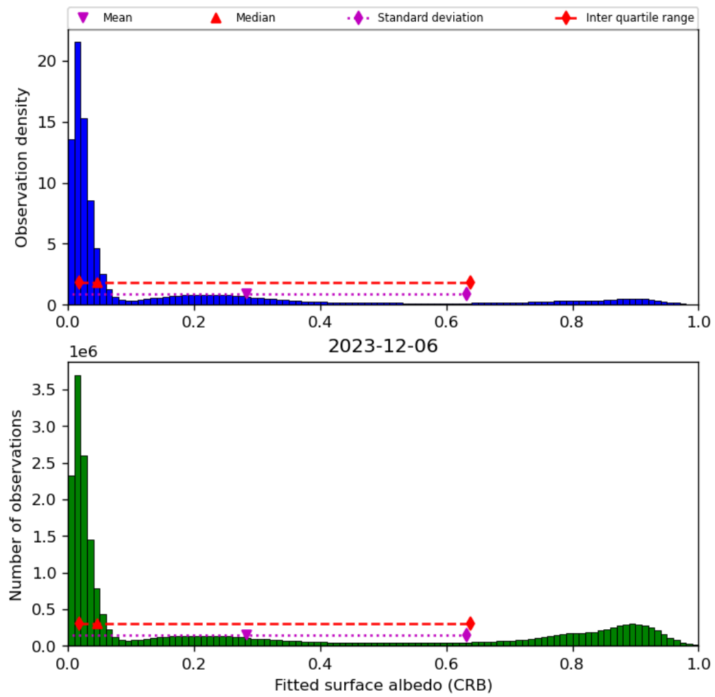
Figure 46: Histogram of “Fitted surface albedo (CRB)” for 2023-12-05 to 2023-12-07
