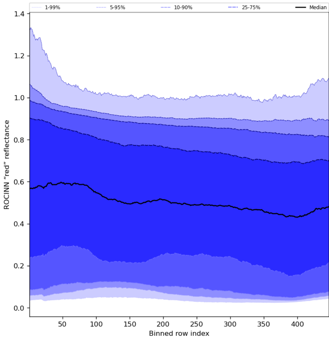
Figure 69: Along track statistics of “ROCINN “red” reflectance” for 2023-12-05 to 2023-12-07
