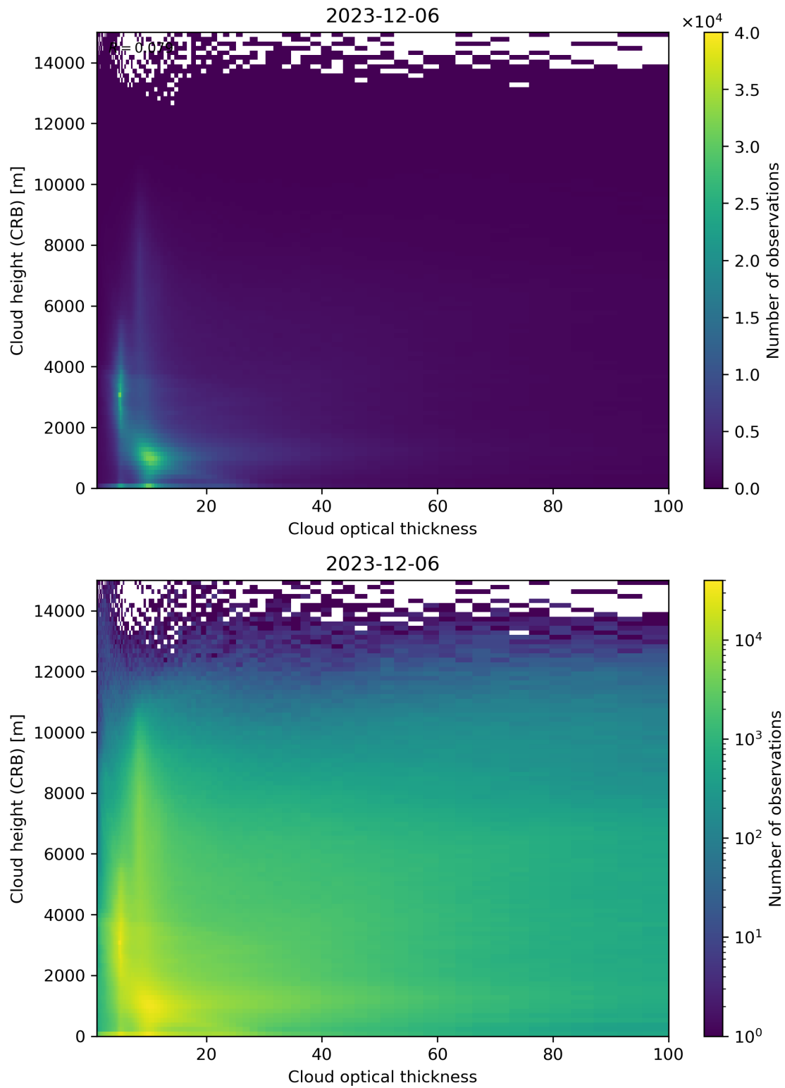
Figure 85: Scatter density plot of “Cloud optical thickness” against “Cloud height (CRB)” for 2023-12-05 to 2023-12-07.
