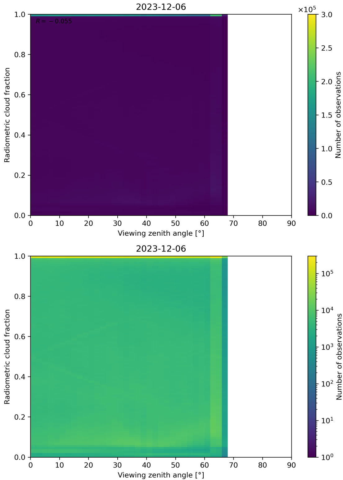
Figure 107: Scatter density plot of “Viewing zenith angle” against “Radiometric cloud fraction” for 2023-12-05 to 2023-12-07.
