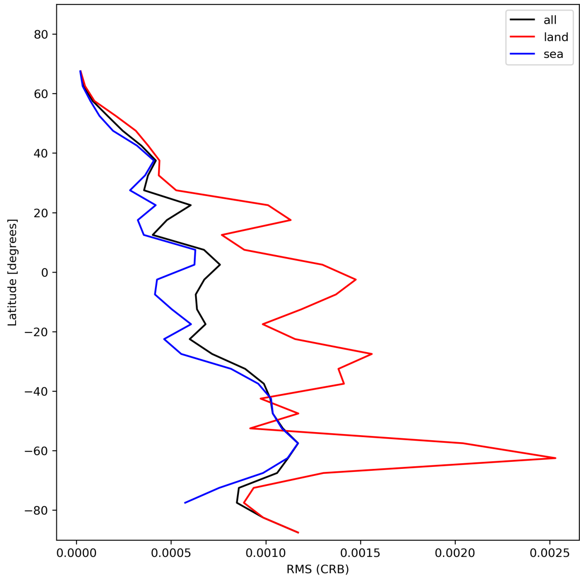
Figure 32: Zonal average of “RMS (CRB)” for 2023-12-05 to 2023-12-07.
