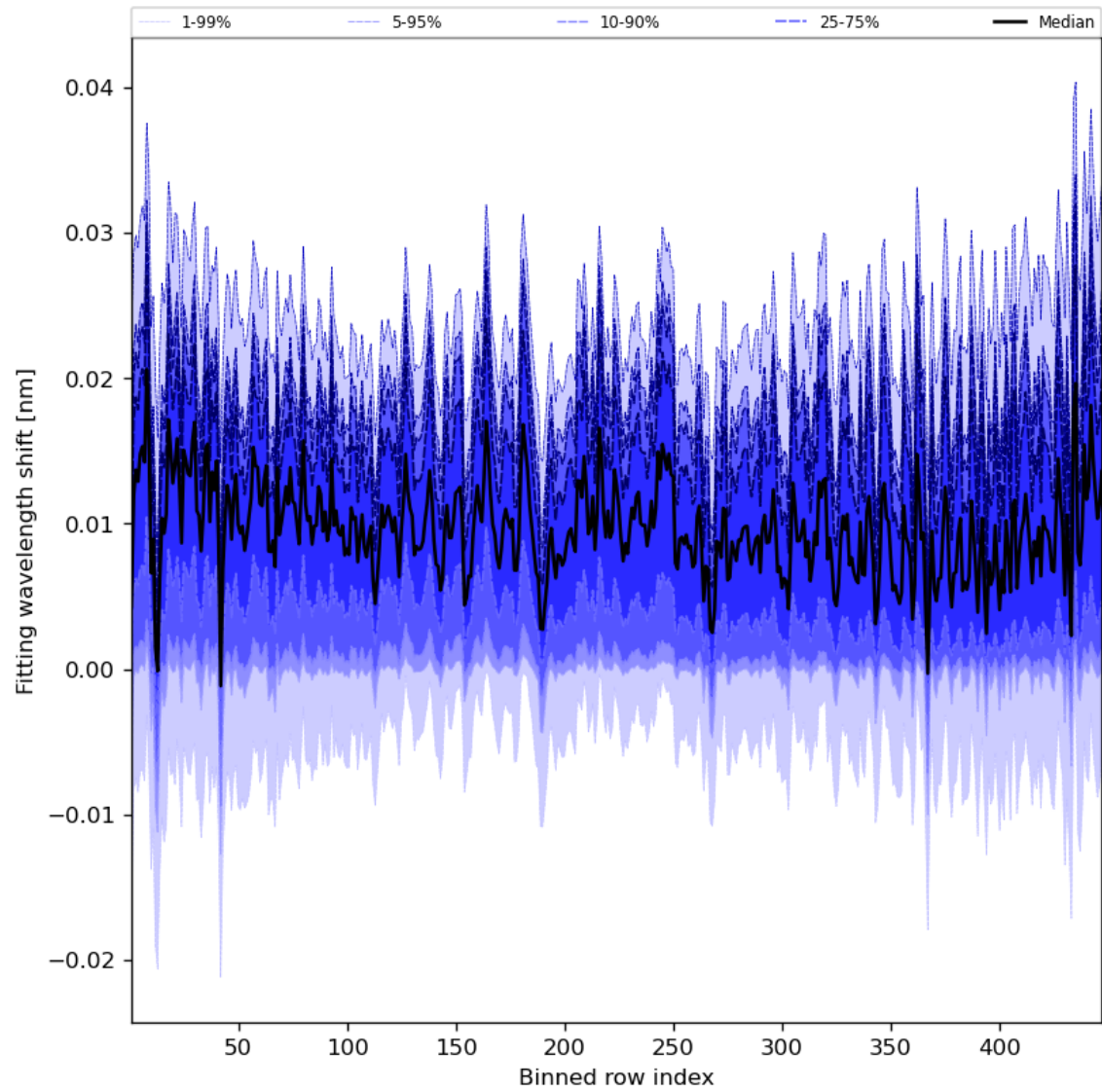
Figure 65: Along track statistics of “Fitting wavelength shift” for 2023-12-05 to 2023-12-07
