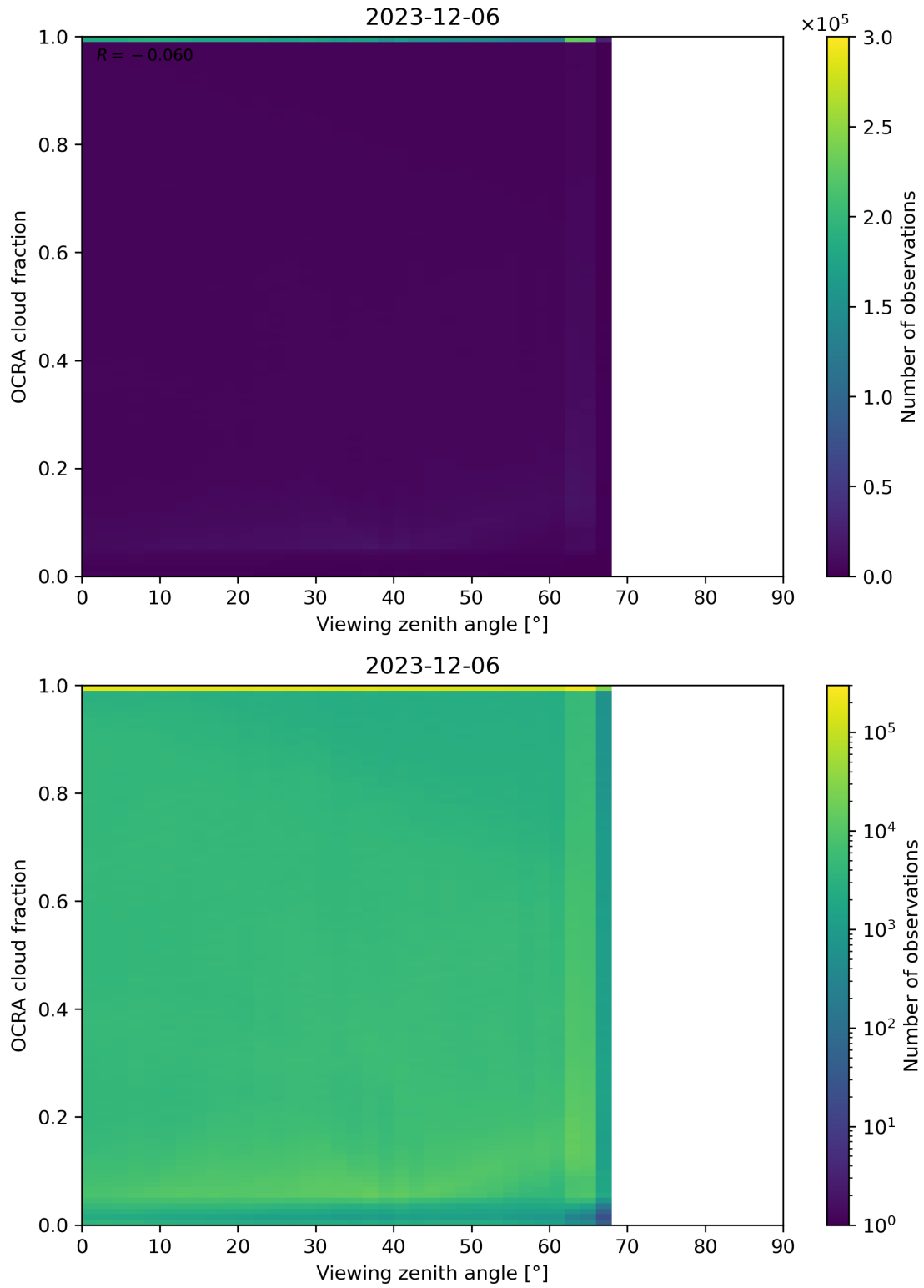
Figure 108: Scatter density plot of “Viewing zenith angle” against “OCRA cloud fraction” for 2023-12-05 to 2023-12-07.
