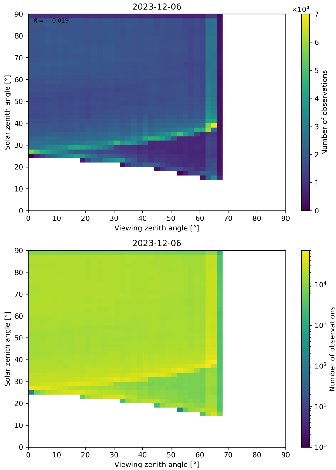
Figure 114: Scatter density plot of “Viewing zenith angle” against “Solar zenith angle” for 2023-12-05 to 2023-12-07.
