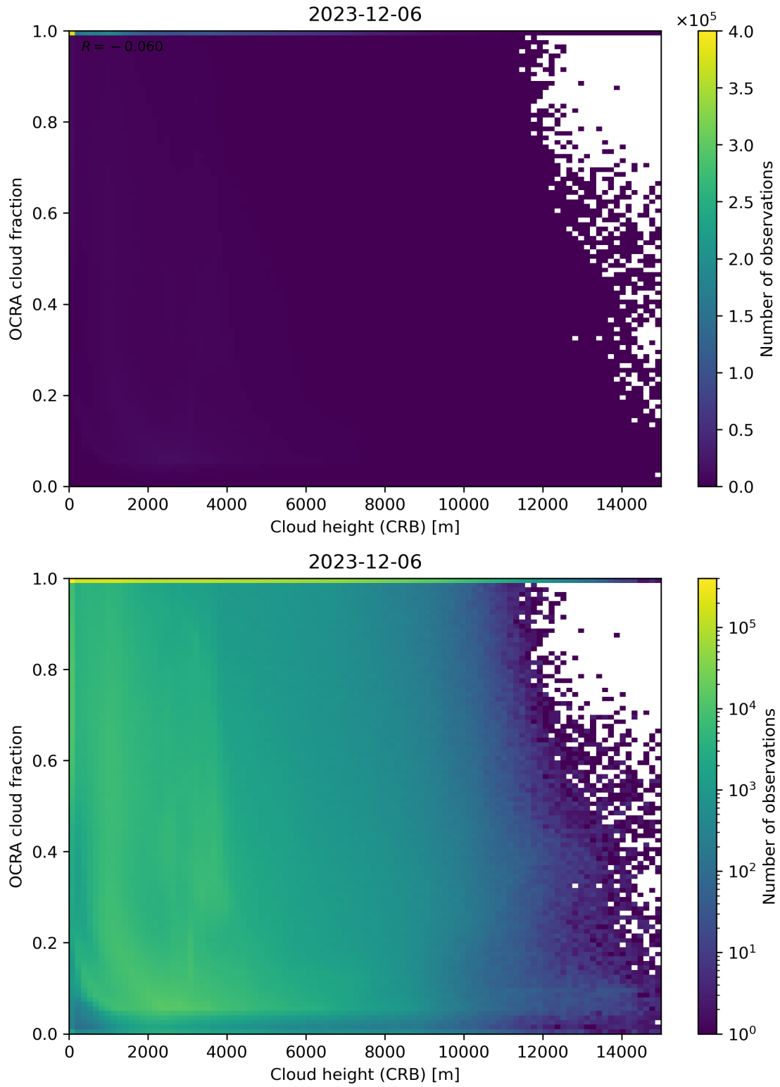
Figure 81: Scatter density plot of “Cloud height (CRB)” against “OCRA cloud fraction” for 2023-12-05 to 2023-12-07.
