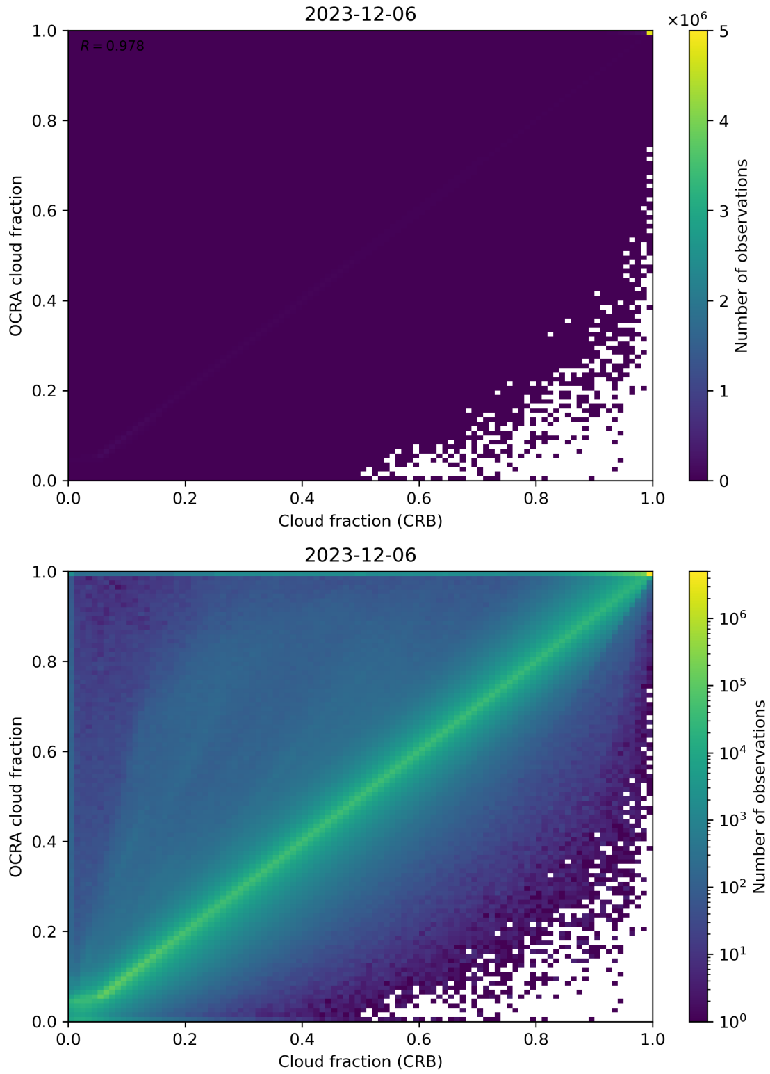
Figure 78: Scatter density plot of “Cloud fraction (CRB)” against “OCRA cloud fraction” for 2023-12-05 to 2023-12-07.
