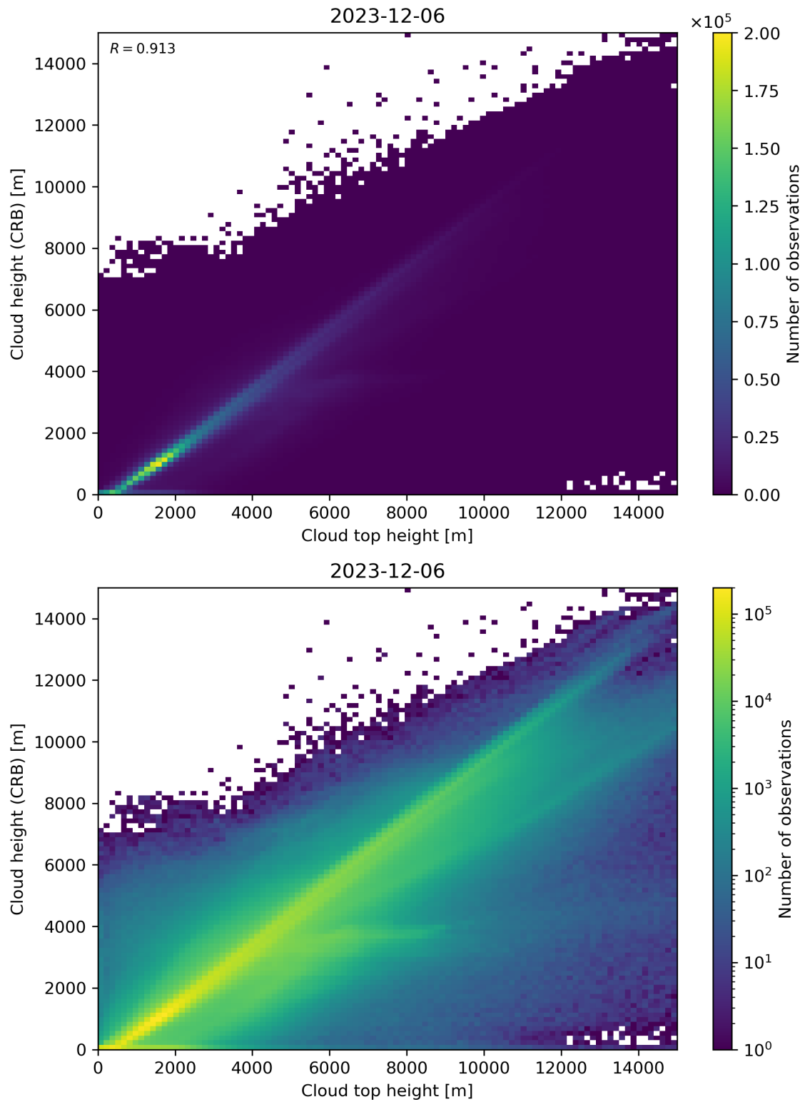
Figure 89: Scatter density plot of “Cloud top height” against “Cloud height (CRB)” for 2023-12-05 to 2023-12-07.
