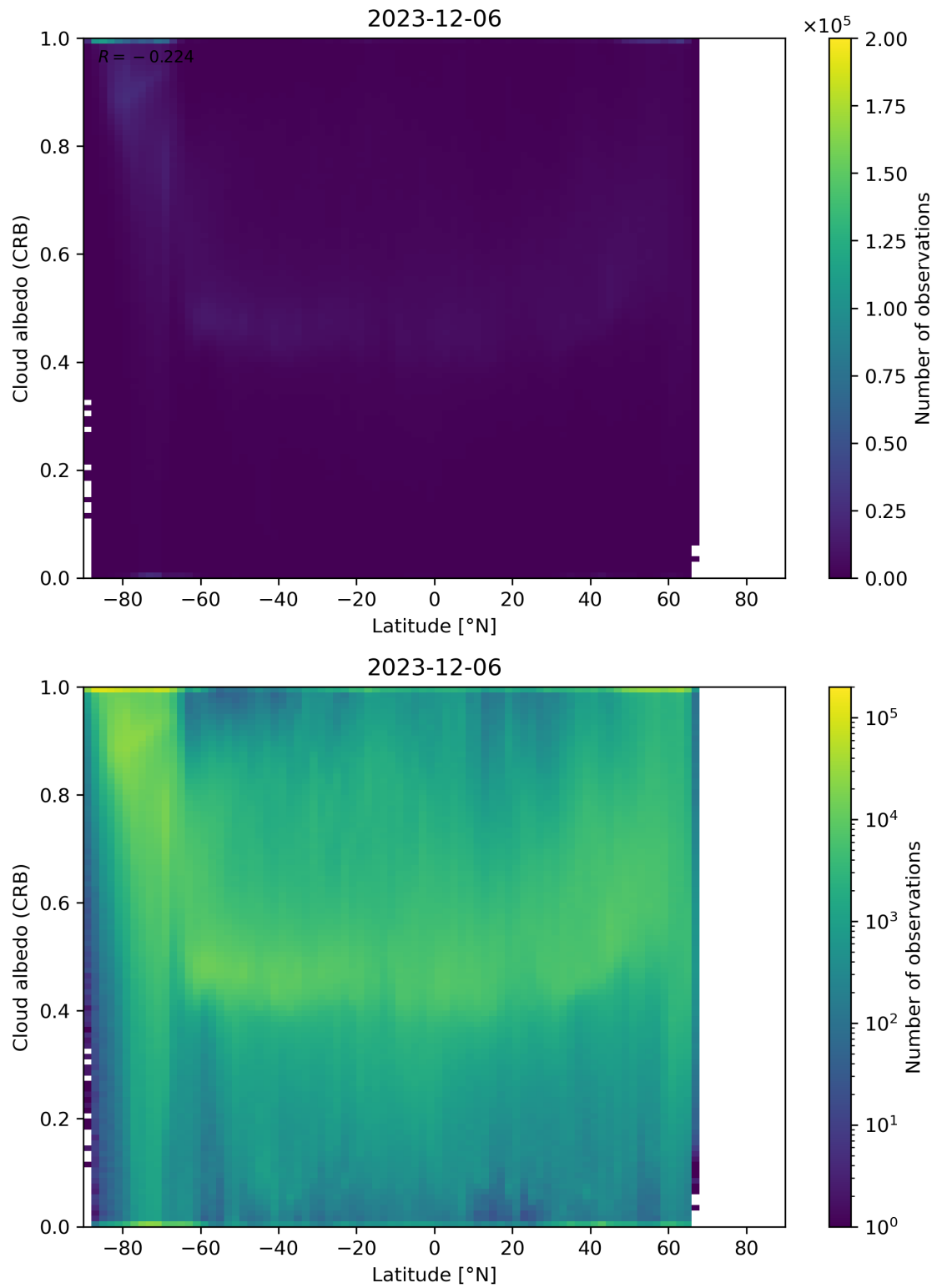
Figure 91: Scatter density plot of “Latitude” against “Cloud albedo (CRB)” for 2023-12-05 to 2023-12-07.
