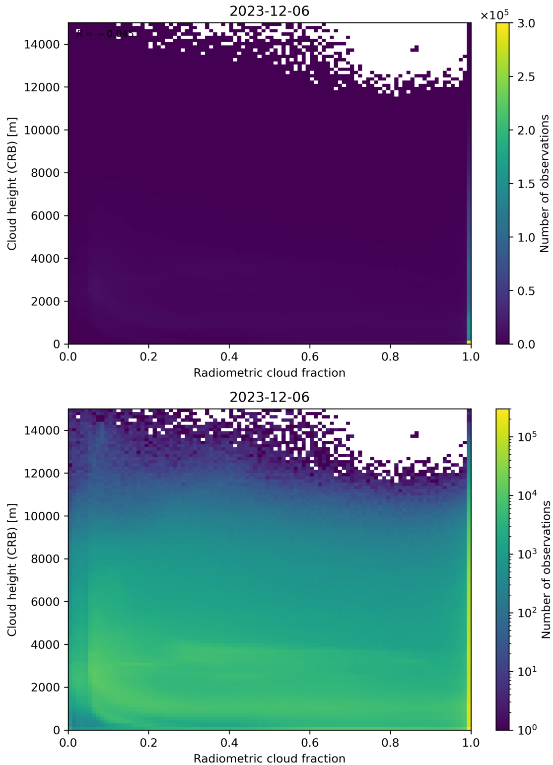
Figure 74: Scatter density plot of “Radiometric cloud fraction” against “Cloud height (CRB)” for 2023-12-05 to 2023-12-07.
