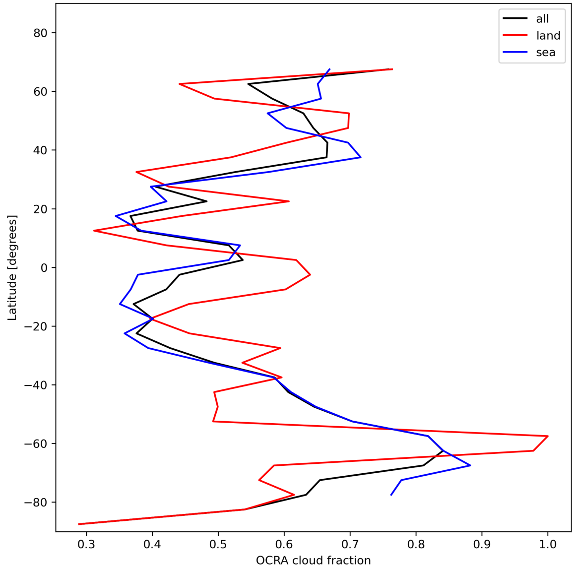
Figure 34: Zonal average of “OCRA cloud fraction” for 2023-12-05 to 2023-12-07.
