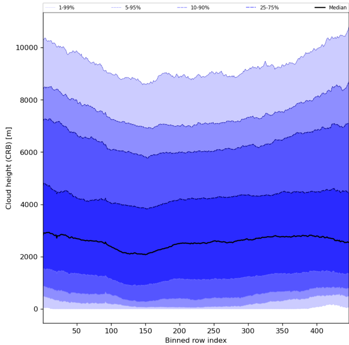
Figure 59: Along track statistics of “Cloud height (CRB)” for 2023-12-05 to 2023-12-07
