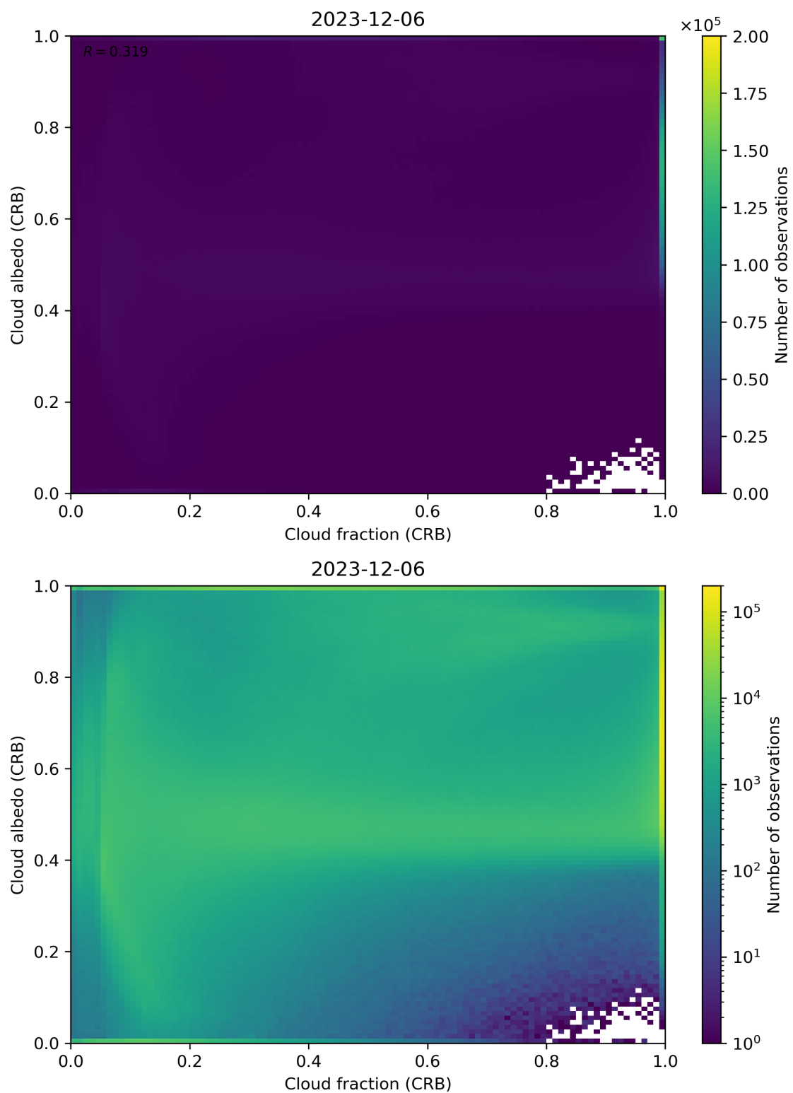
Figure 77: Scatter density plot of “Cloud fraction (CRB)” against “Cloud albedo (CRB)” for 2023-12-05 to 2023-12-07.
