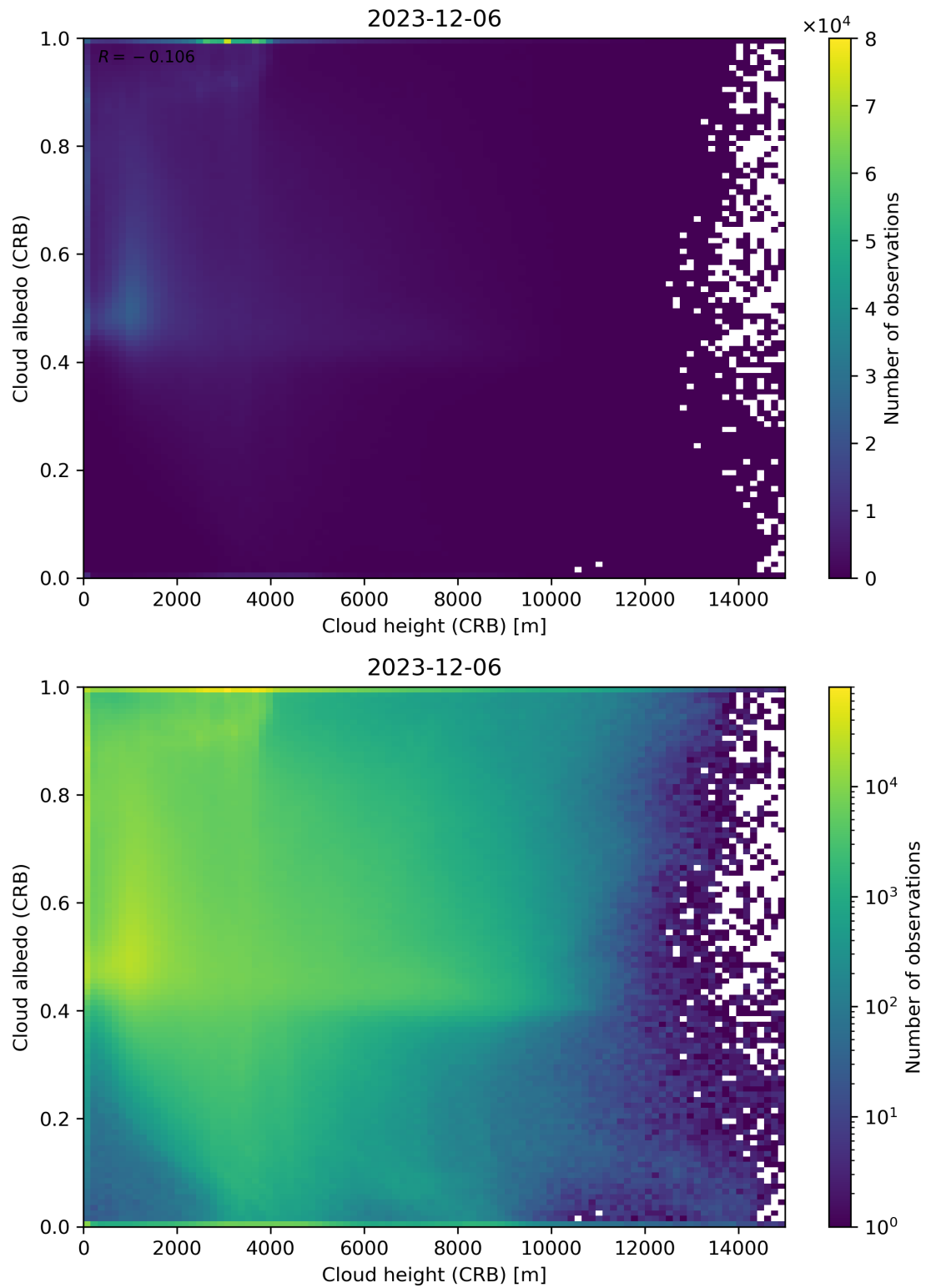
Figure 80: Scatter density plot of “Cloud height (CRB)” against “Cloud albedo (CRB)” for 2023-12-05 to 2023-12-07.
