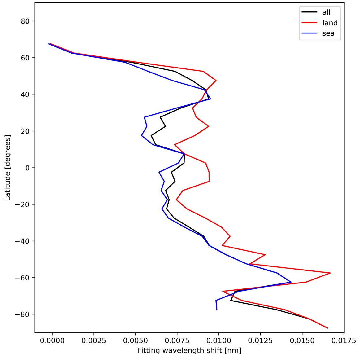
Figure 33: Zonal average of “Fitting wavelength shift” for 2023-12-05 to 2023-12-07.
