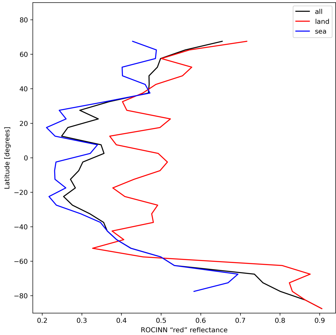
Figure 37: Zonal average of “ROCINN “red” reflectance” for 2023-12-05 to 2023-12-07.
