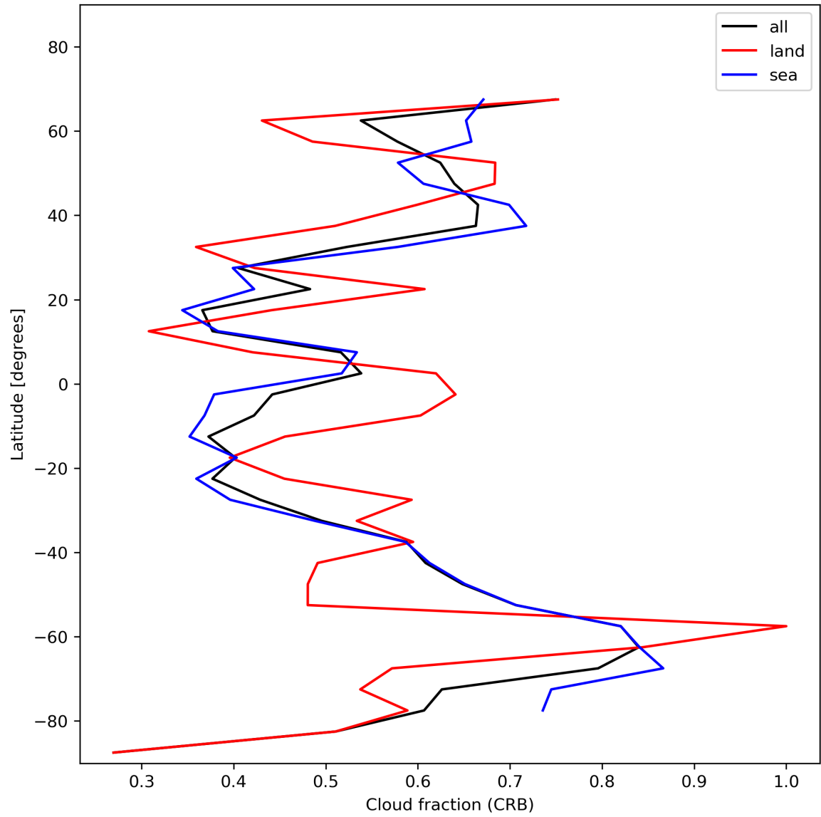
Figure 26: Zonal average of “Cloud fraction (CRB)” for 2023-12-05 to 2023-12-07.
