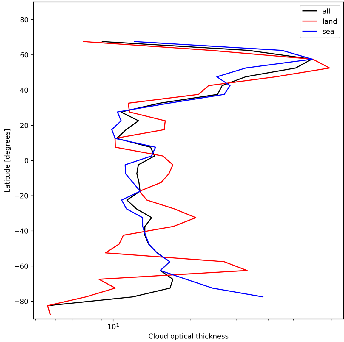
Figure 25: Zonal average of “Cloud optical thickness” for 2023-12-05 to 2023-12-07.
