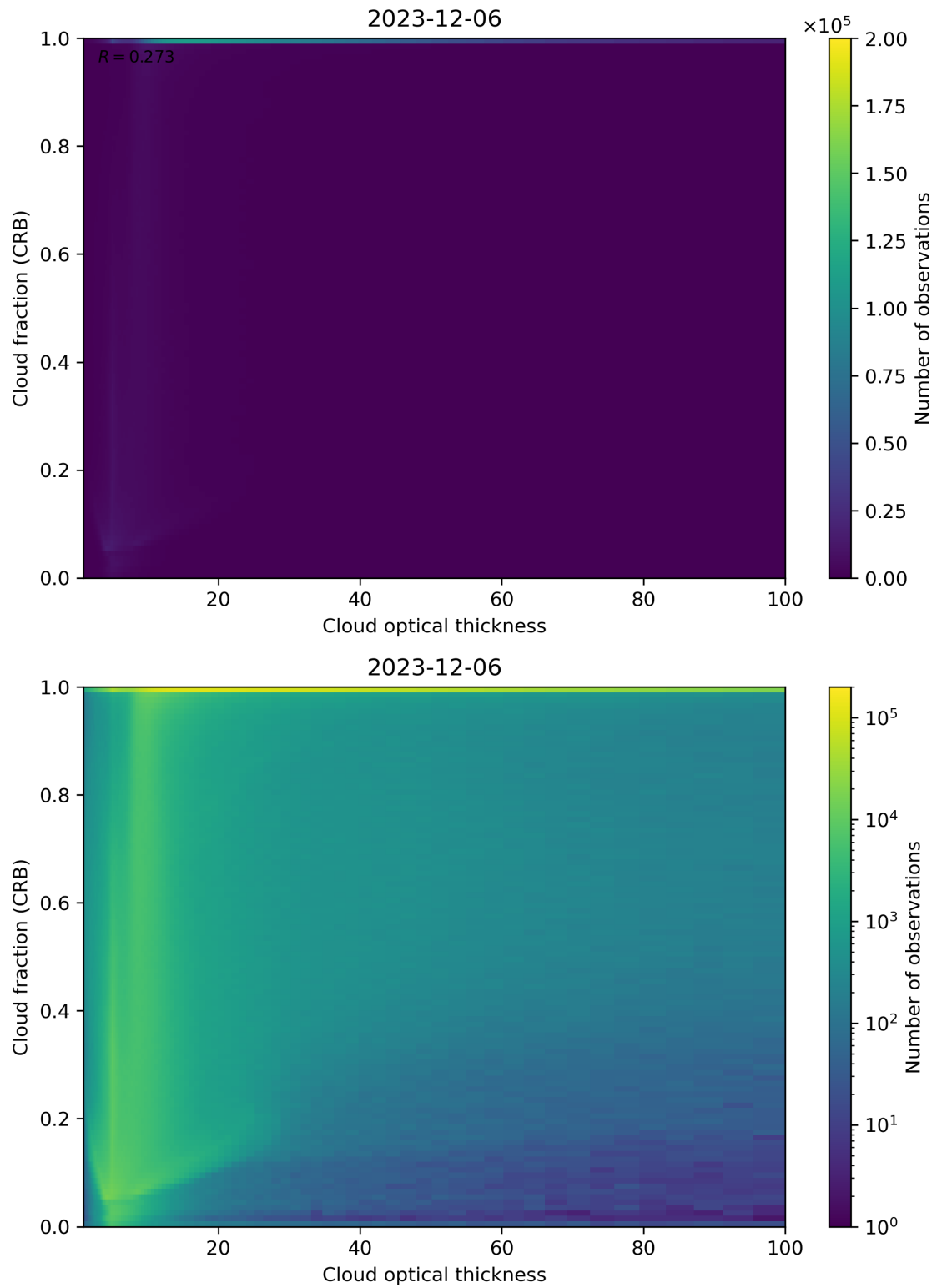
Figure 84: Scatter density plot of “Cloud optical thickness” against “Cloud fraction (CRB)” for 2023-12-05 to 2023-12-07.
