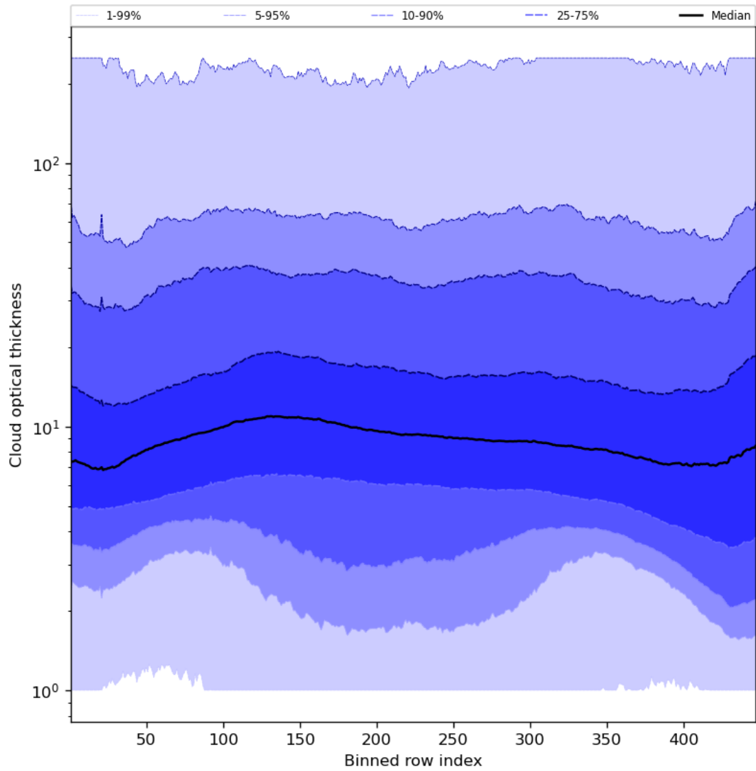
Figure 57: Along track statistics of “Cloud optical thickness” for 2023-12-05 to 2023-12-07
