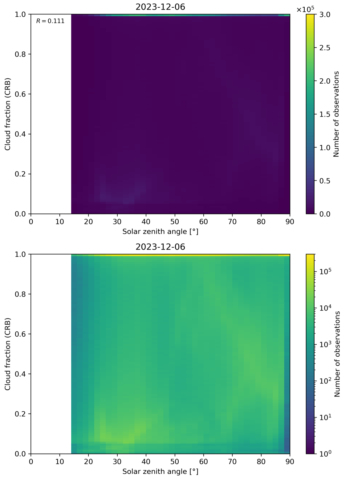
Figure 101: Scatter density plot of “Solar zenith angle” against “Cloud fraction (CRB)” for 2023-12-05 to 2023-12-07.
