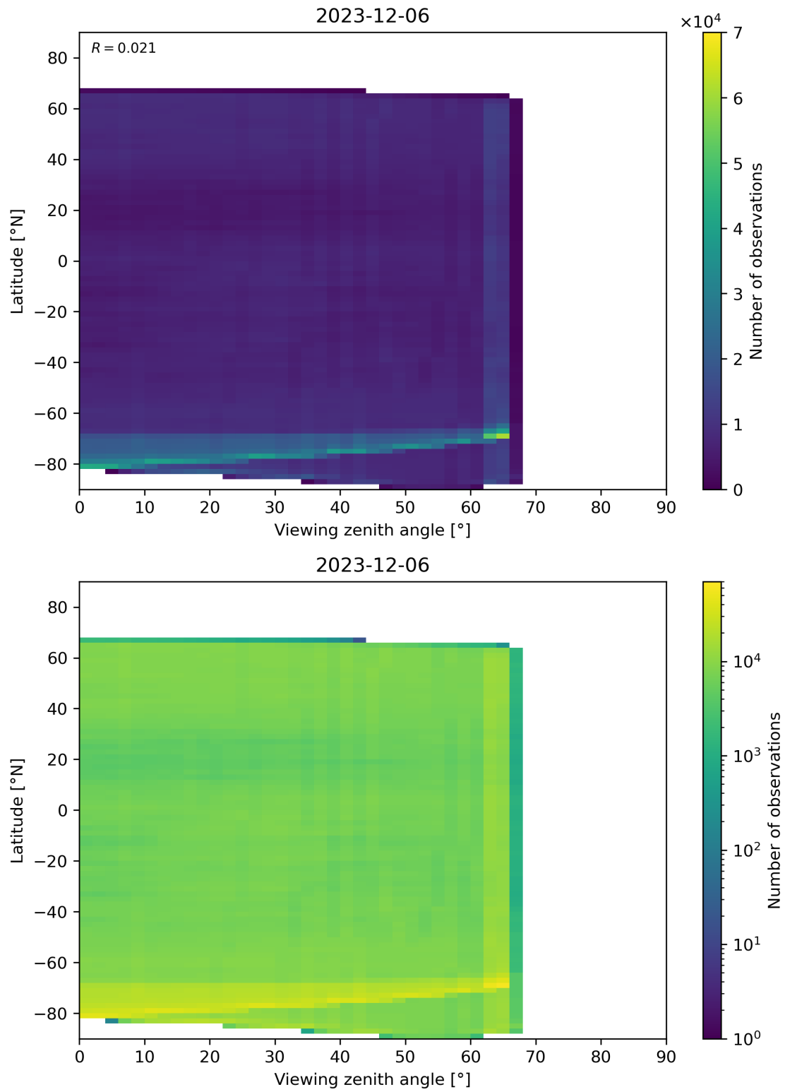
Figure 113: Scatter density plot of “Viewing zenith angle” against “Latitude” for 2023-12-05 to 2023-12-07.
