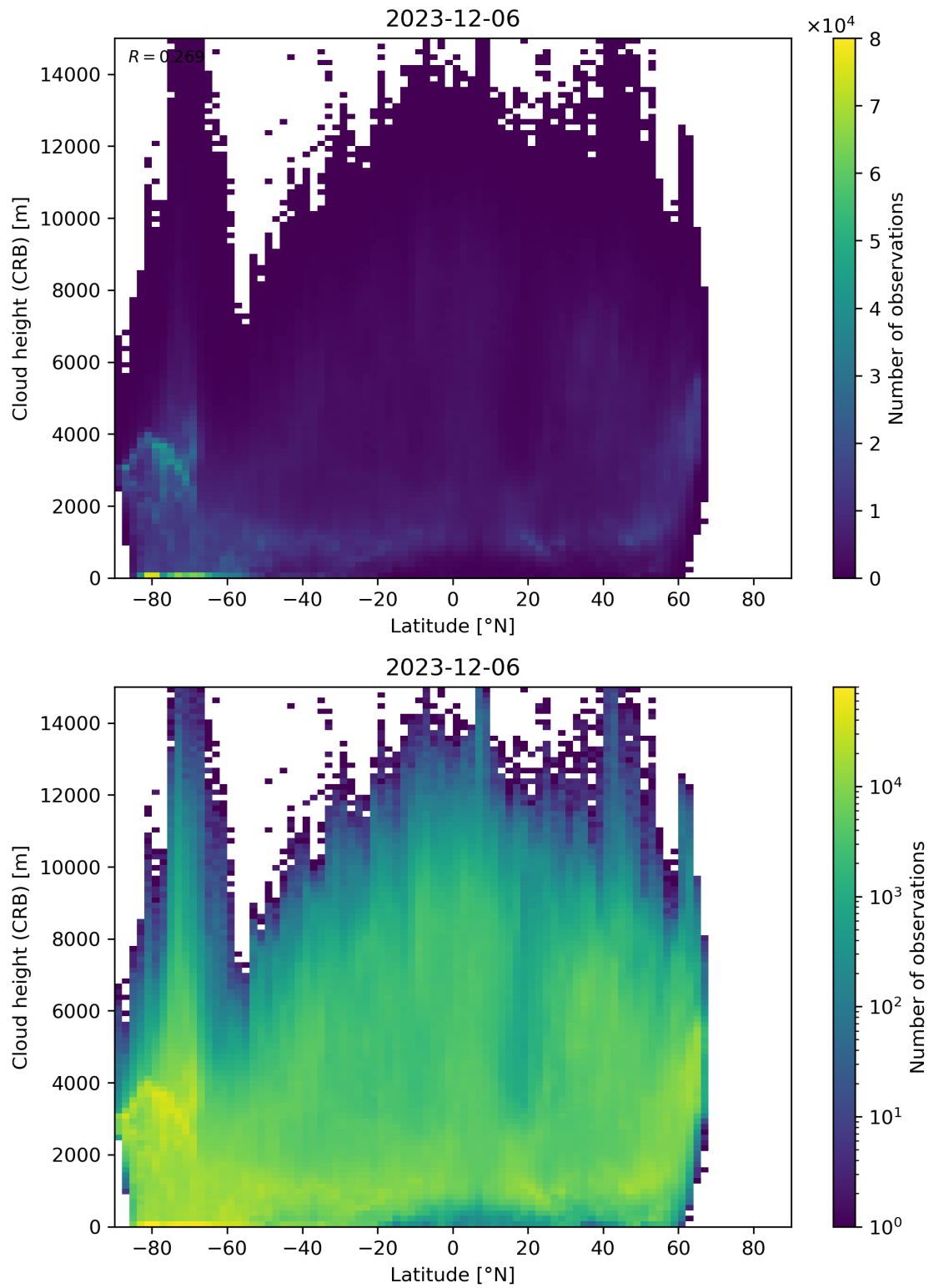
Figure 95: Scatter density plot of “Latitude” against “Cloud height (CRB)” for 2023-12-05 to 2023-12-07.
