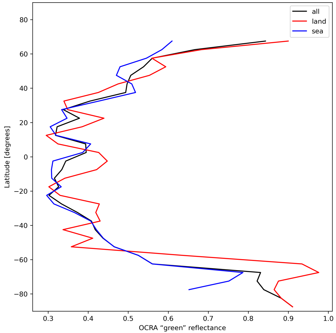
Figure 36: Zonal average of “OCRA “green” reflectance” for 2023-12-05 to 2023-12-07.
