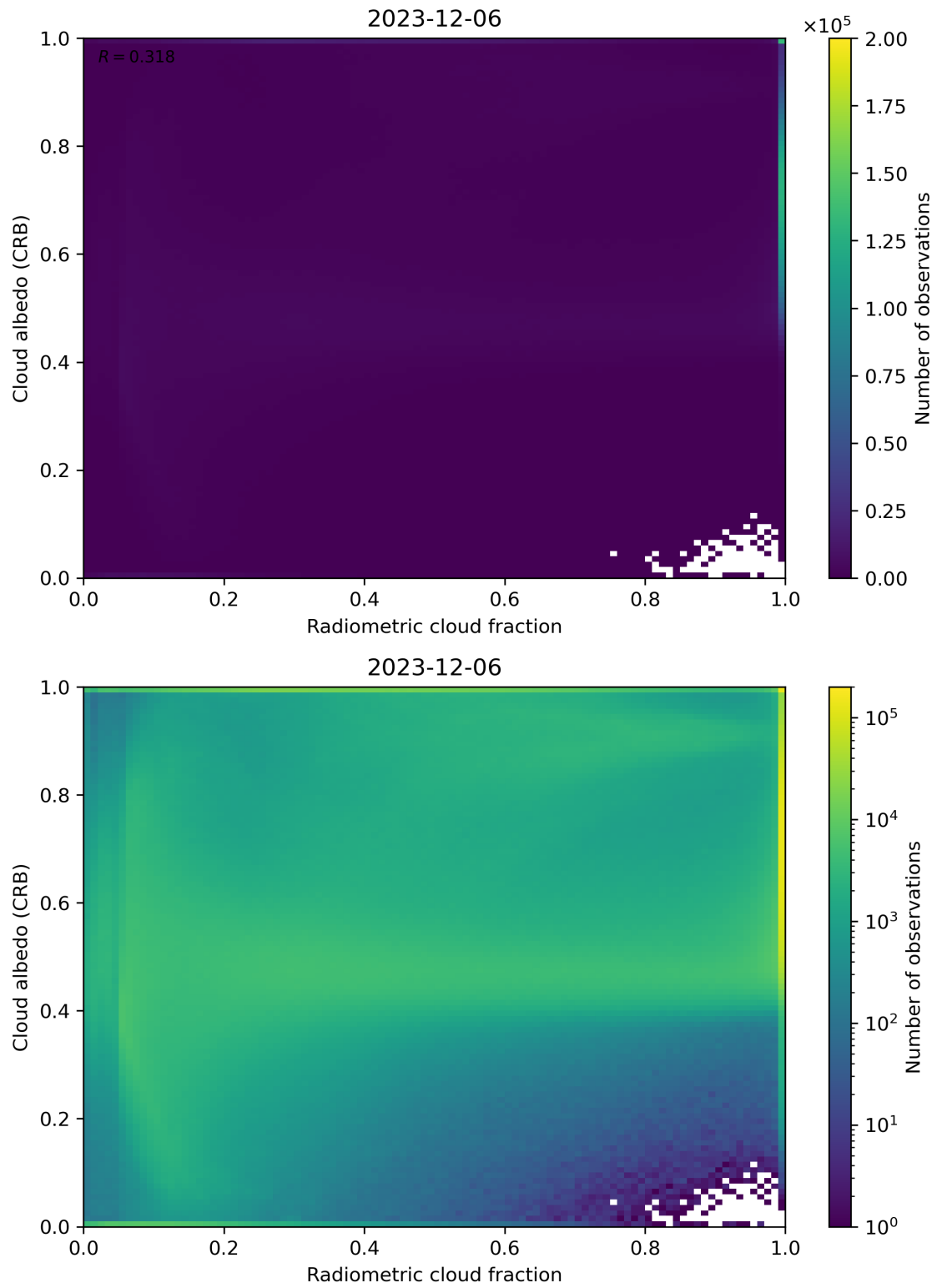
Figure 71: Scatter density plot of “Radiometric cloud fraction” against “Cloud albedo (CRB)” for 2023-12-05 to 2023-12-07.
