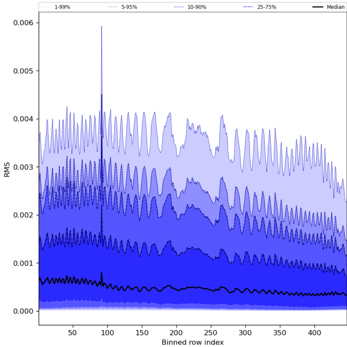
Figure 63: Along track statistics of “RMS” for 2023-12-05 to 2023-12-07
