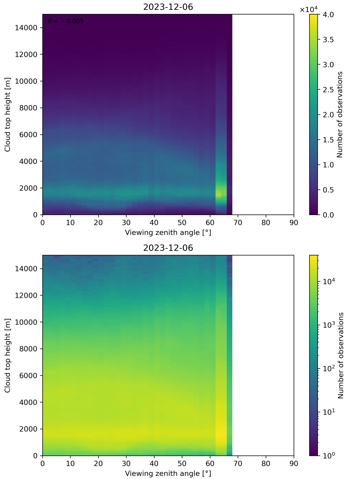
Figure 112: Scatter density plot of “Viewing zenith angle” against “Cloud top height” for 2023-12-05 to 2023-12-07.
