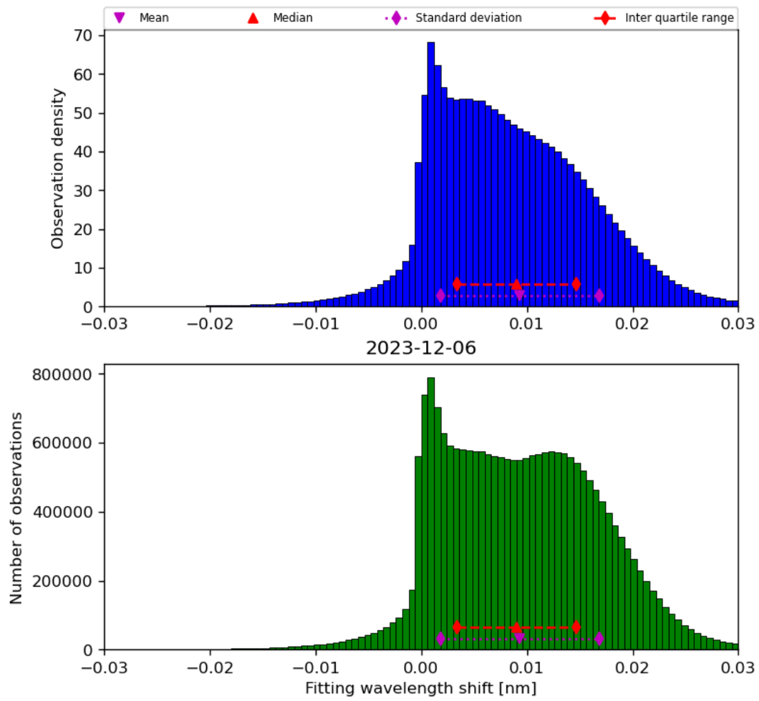
Figure 49: Histogram of “Fitting wavelength shift” for 2023-12-05 to 2023-12-07
