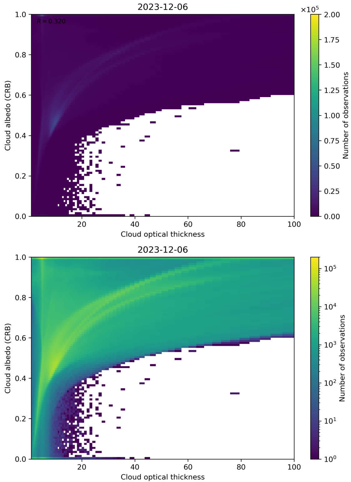
Figure 82: Scatter density plot of “Cloud optical thickness” against “Cloud albedo (CRB)” for 2023-12-05 to 2023-12-07.
