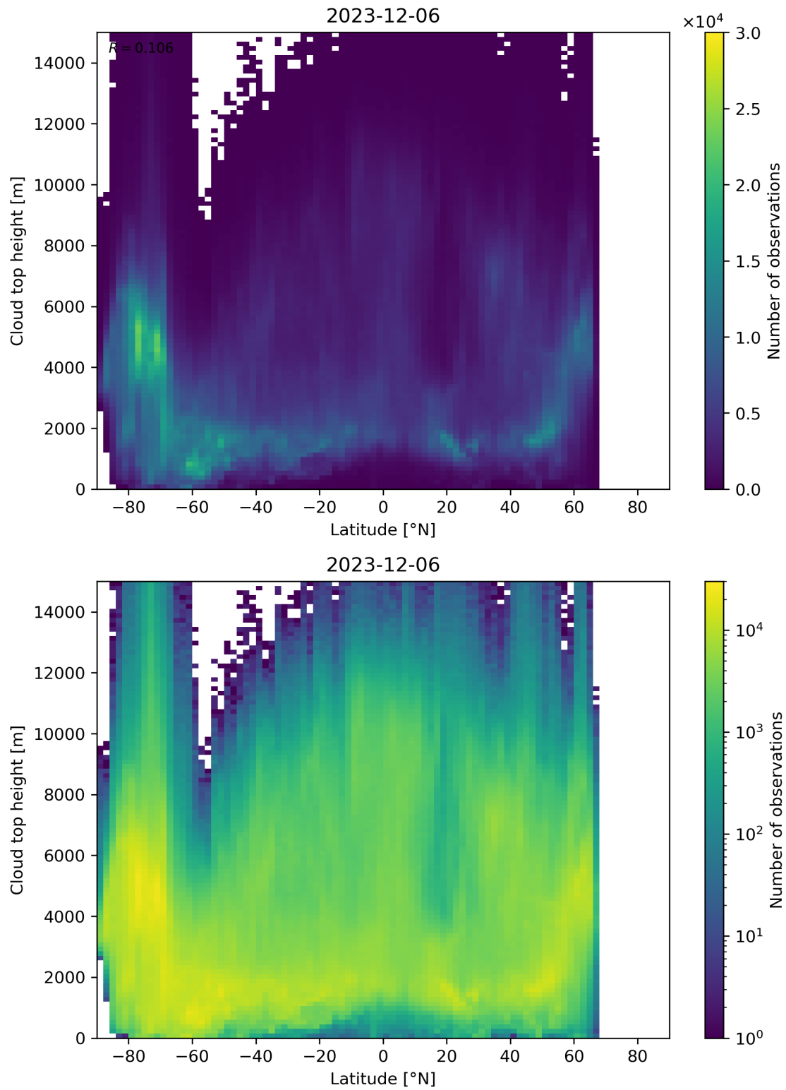
Figure 97: Scatter density plot of “Latitude” against “Cloud top height” for 2023-12-05 to 2023-12-07.
