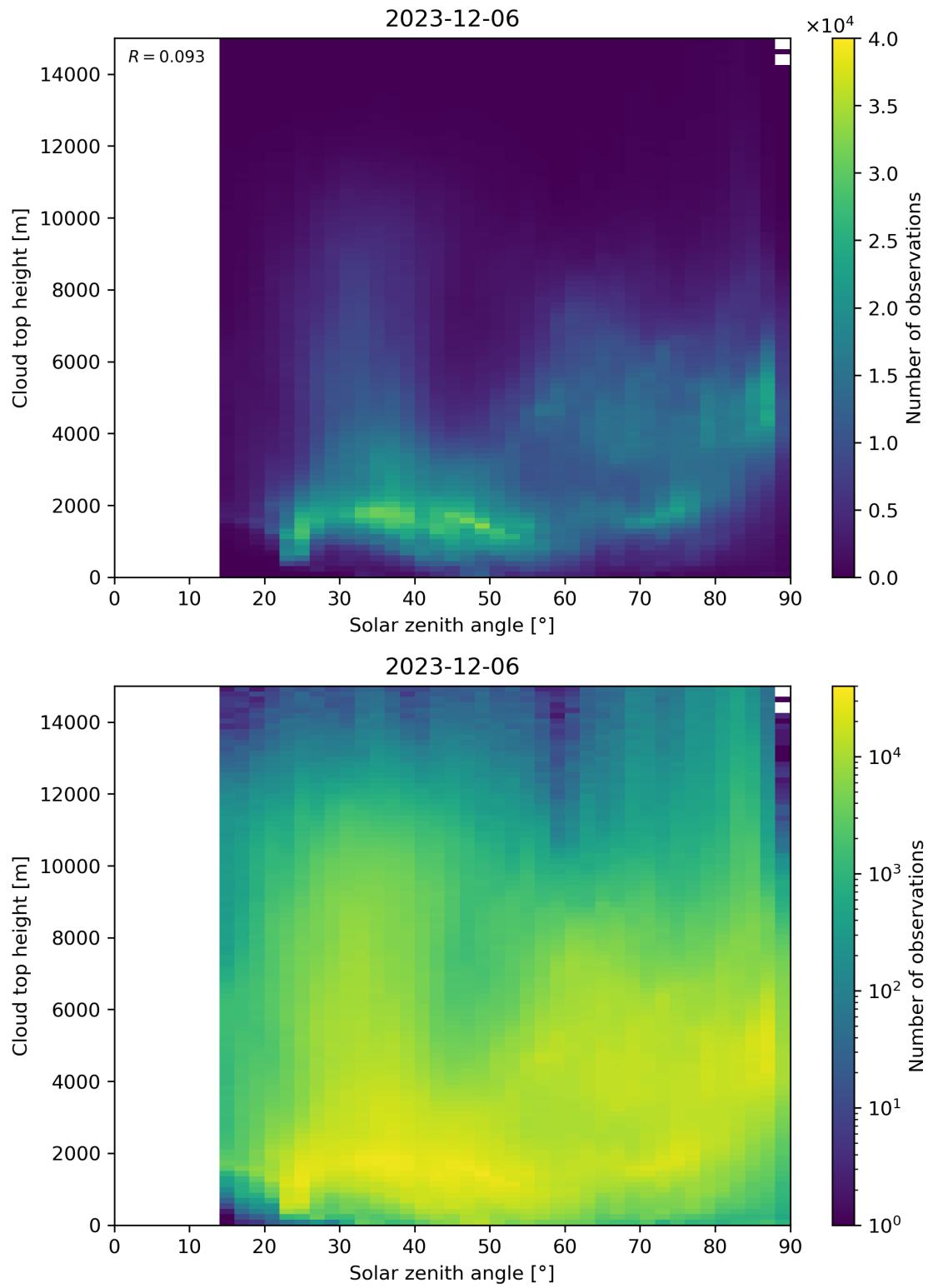
Figure 104: Scatter density plot of “Solar zenith angle” against “Cloud top height” for 2023-12-05 to 2023-12-07.
