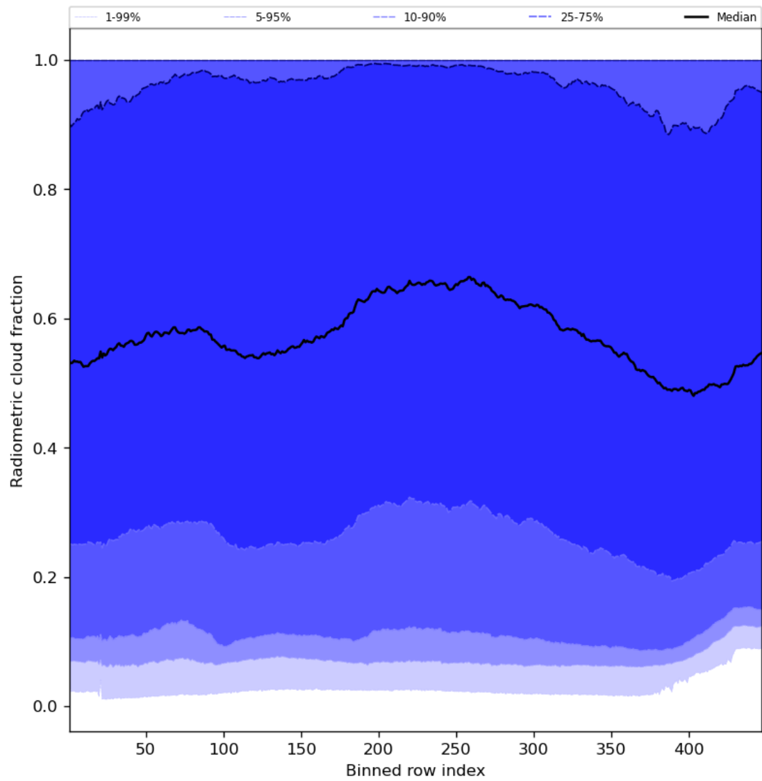
Figure 55: Along track statistics of “Radiometric cloud fraction” for 2023-12-05 to 2023-12-07
