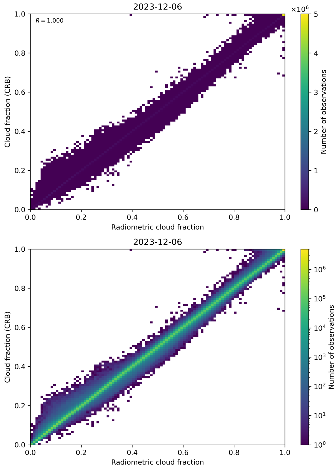
Figure 73: Scatter density plot of “Radiometric cloud fraction” against “Cloud fraction (CRB)” for 2023-12-05 to 2023-12-07.
