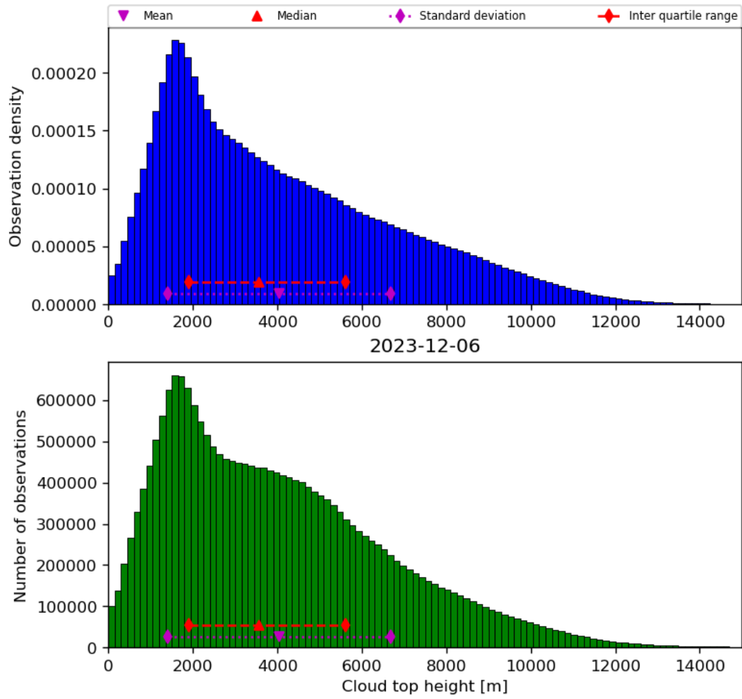
Figure 40: Histogram of “Cloud top height” for 2023-12-05 to 2023-12-07
