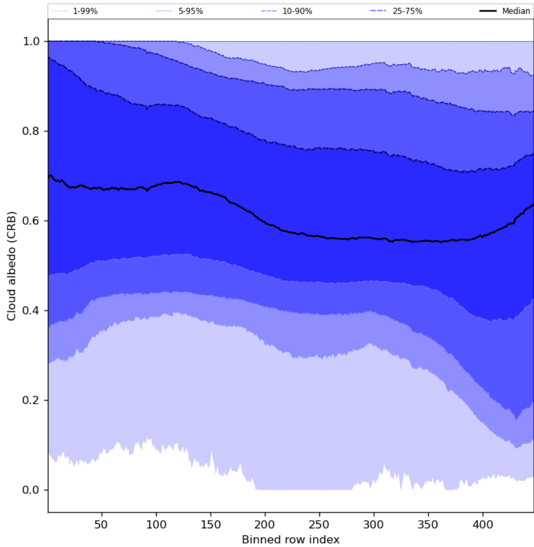
Figure 60: Along track statistics of “Cloud albedo (CRB)” for 2023-12-05 to 2023-12-07
