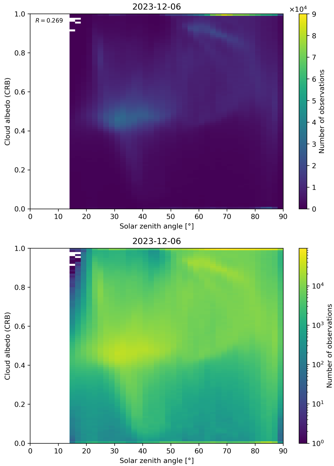
Figure 98: Scatter density plot of “Solar zenith angle” against “Cloud albedo (CRB)” for 2023-12-05 to 2023-12-07.
