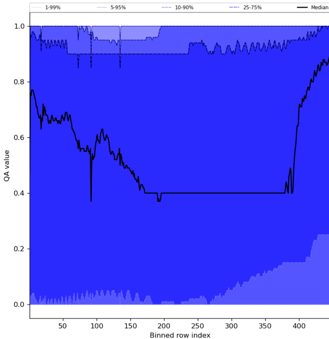
Figure 54: Along track statistics of “QA value” for 2023-12-05 to 2023-12-07
