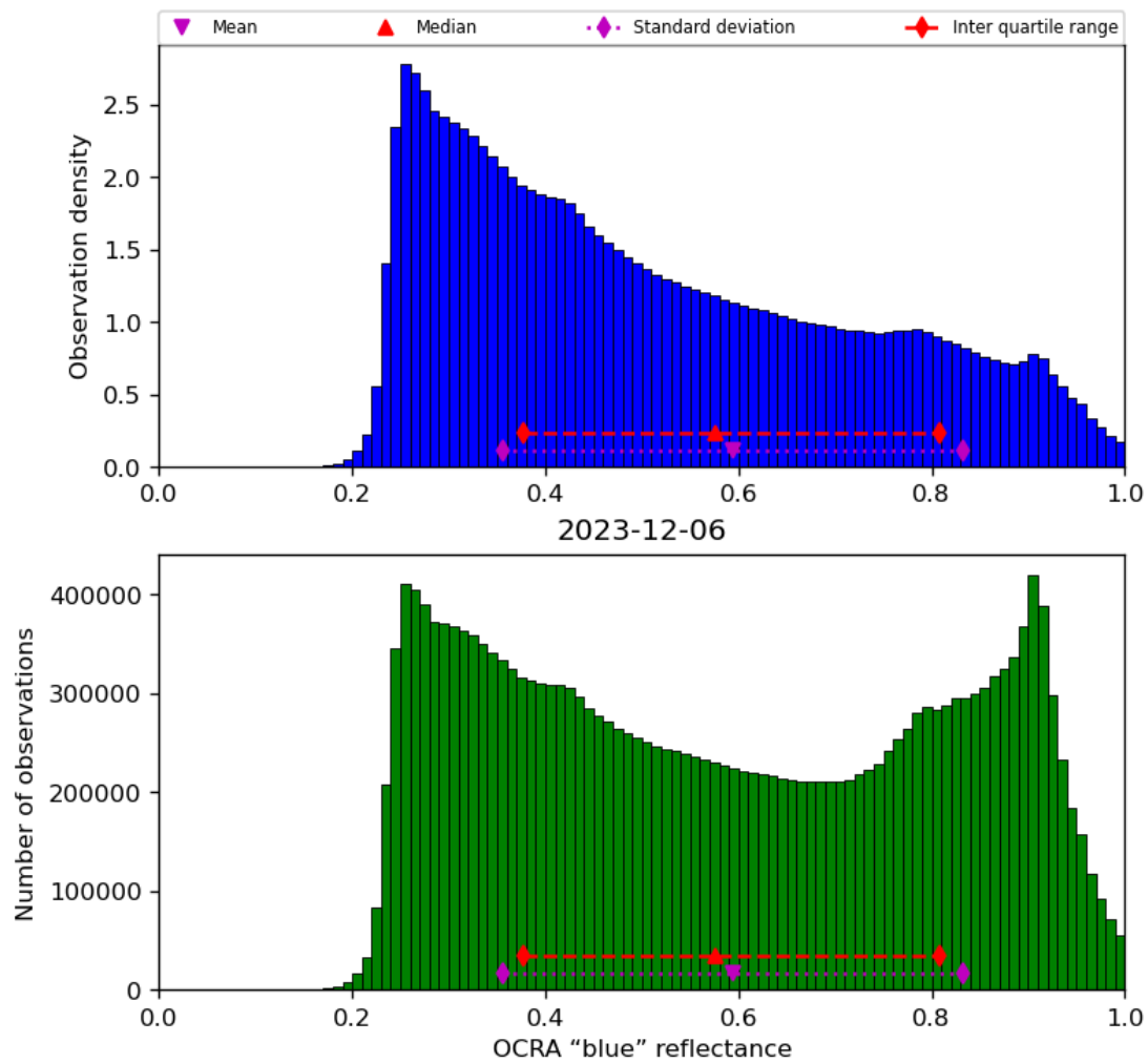
Figure 51: Histogram of "OCRA "blue" reflectance" for 2023-12-05 to 2023-12-07
