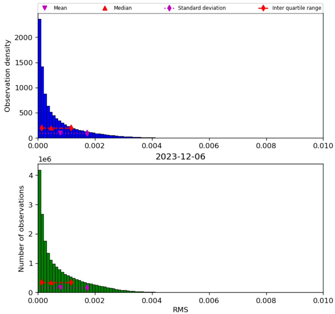
Figure 47: Histogram of “RMS” for 2023-12-05 to 2023-12-07
