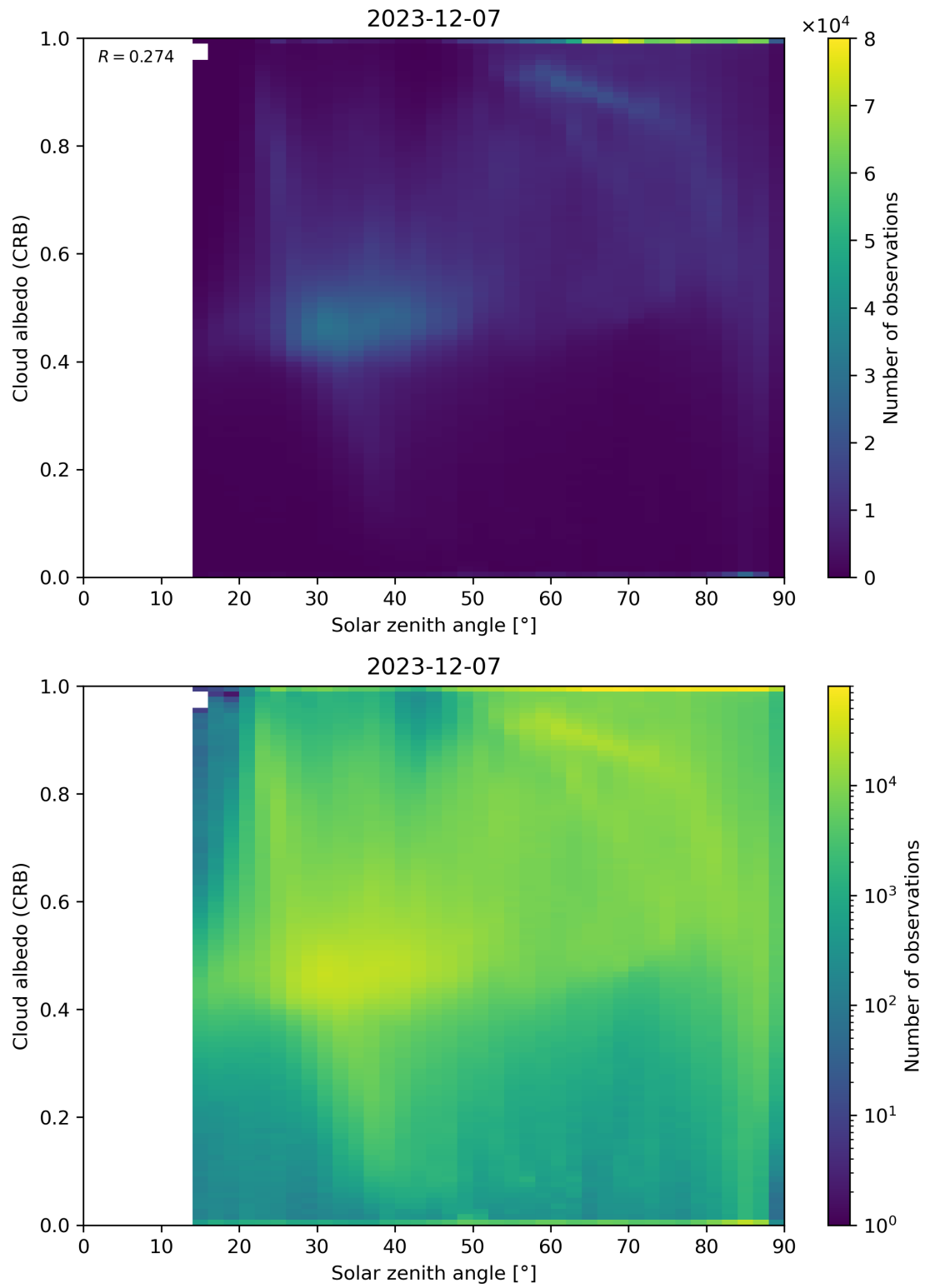
Figure 98: Scatter density plot of “Solar zenith angle” against “Cloud albedo (CRB)” for 2023-12-06 to 2023-12-08.
