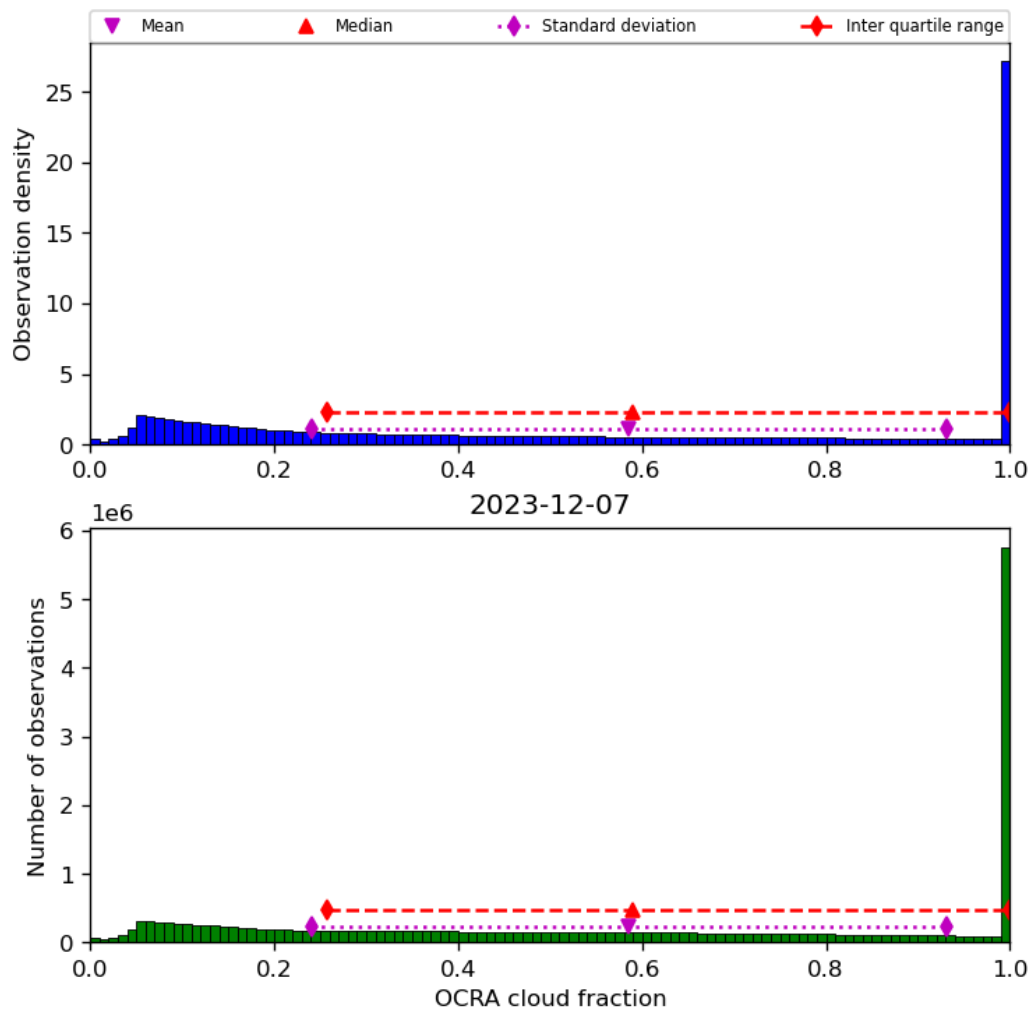
Figure 50: Histogram of "OCRA cloud fraction" for 2023-12-06 to 2023-12-08
