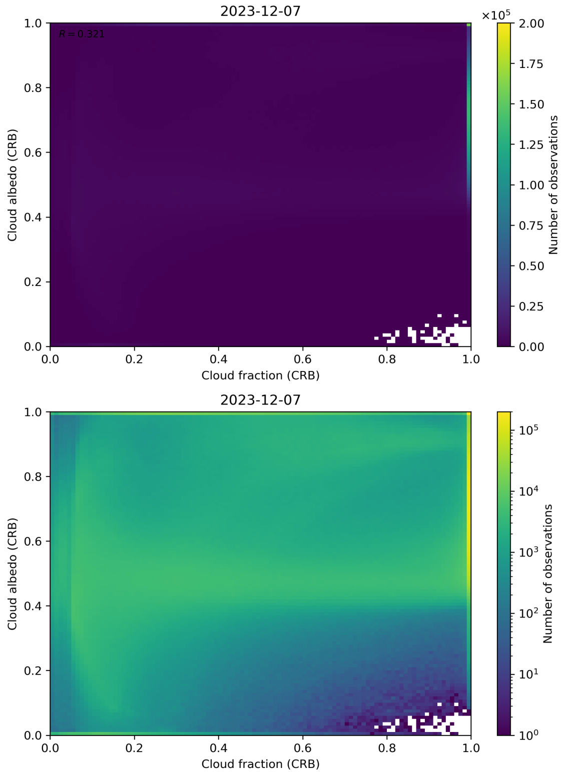
Figure 77: Scatter density plot of “Cloud fraction (CRB)” against “Cloud albedo (CRB)” for 2023-12-06 to 2023-12-08.
