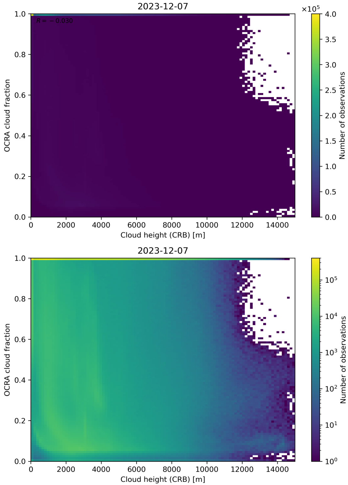
Figure 81: Scatter density plot of “Cloud height (CRB)” against “OCRA cloud fraction” for 2023-12-06 to 2023-12-08.
