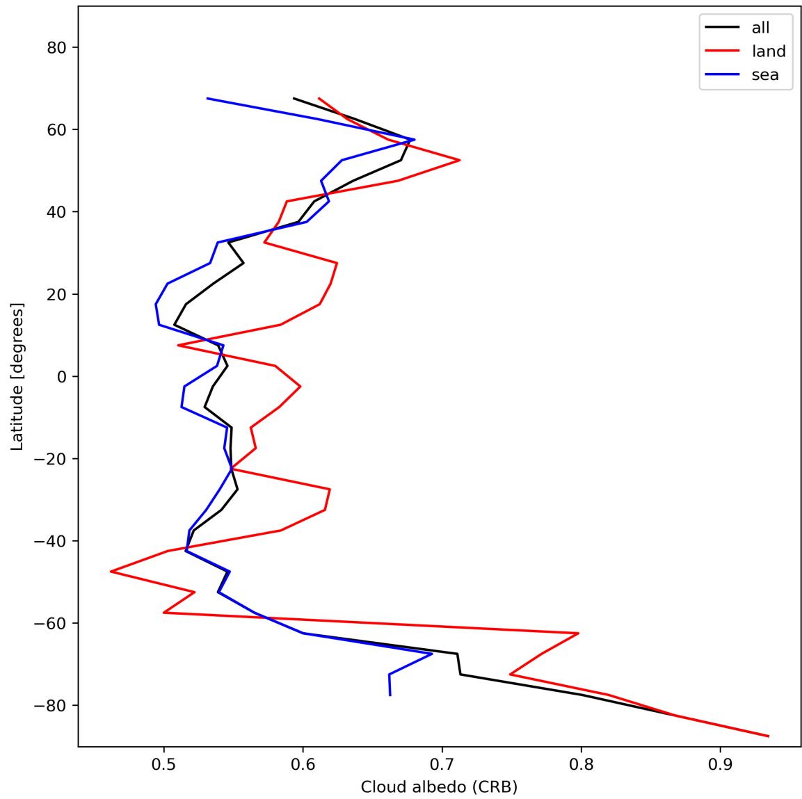
Figure 28: Zonal average of “Cloud albedo (CRB)” for 2023-12-06 to 2023-12-08.
