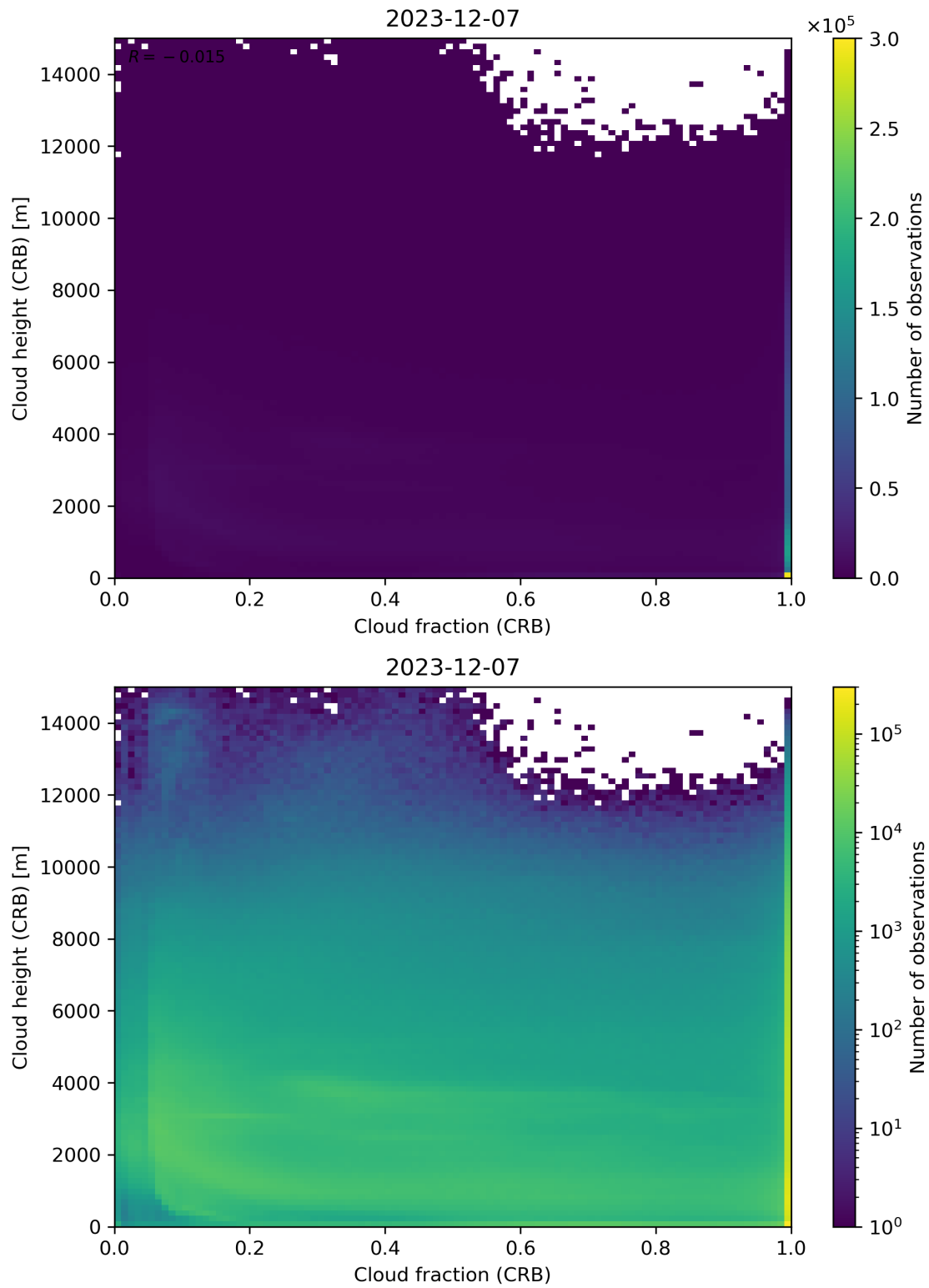
Figure 79: Scatter density plot of “Cloud fraction (CRB)” against “Cloud height (CRB)” for 2023-12-06 to 2023-12-08.
