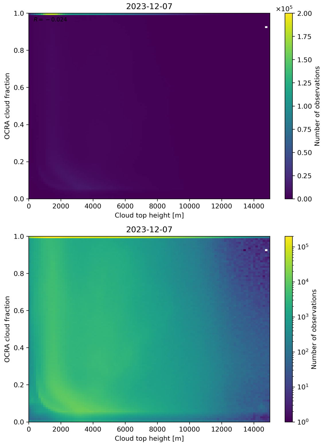
Figure 87: Scatter density plot of “Cloud top height” against “OCRA cloud fraction” for 2023-12-06 to 2023-12-08.
