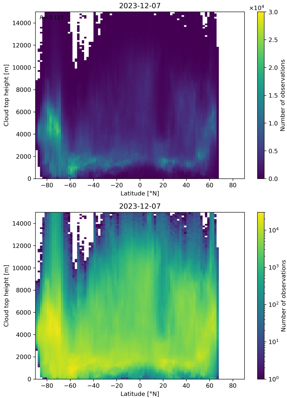
Figure 97: Scatter density plot of “Latitude” against “Cloud top height” for 2023-12-06 to 2023-12-08.
