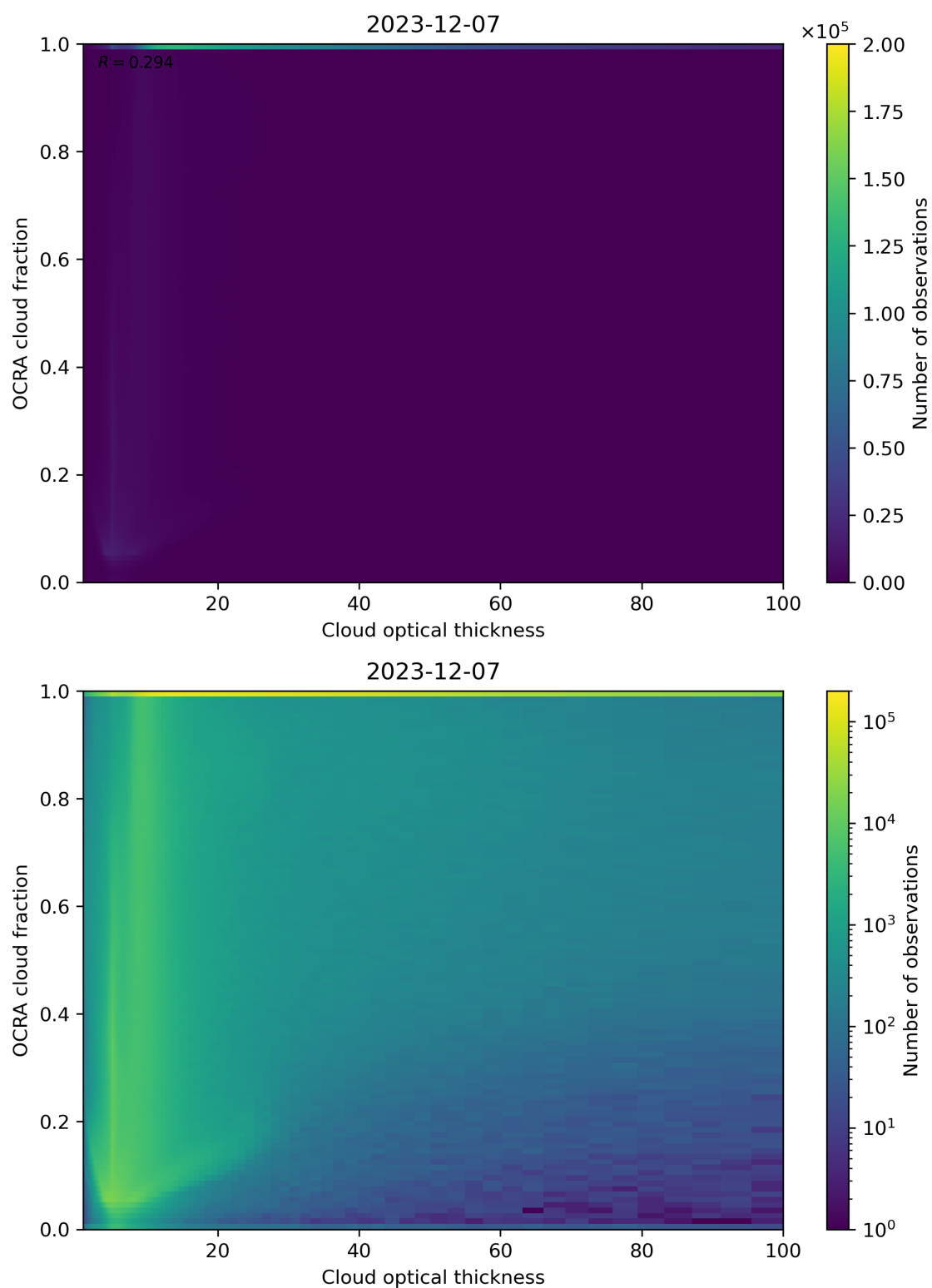
Figure 83: Scatter density plot of “Cloud optical thickness” against “OCRA cloud fraction” for 2023-12-06 to 2023-12-08.
