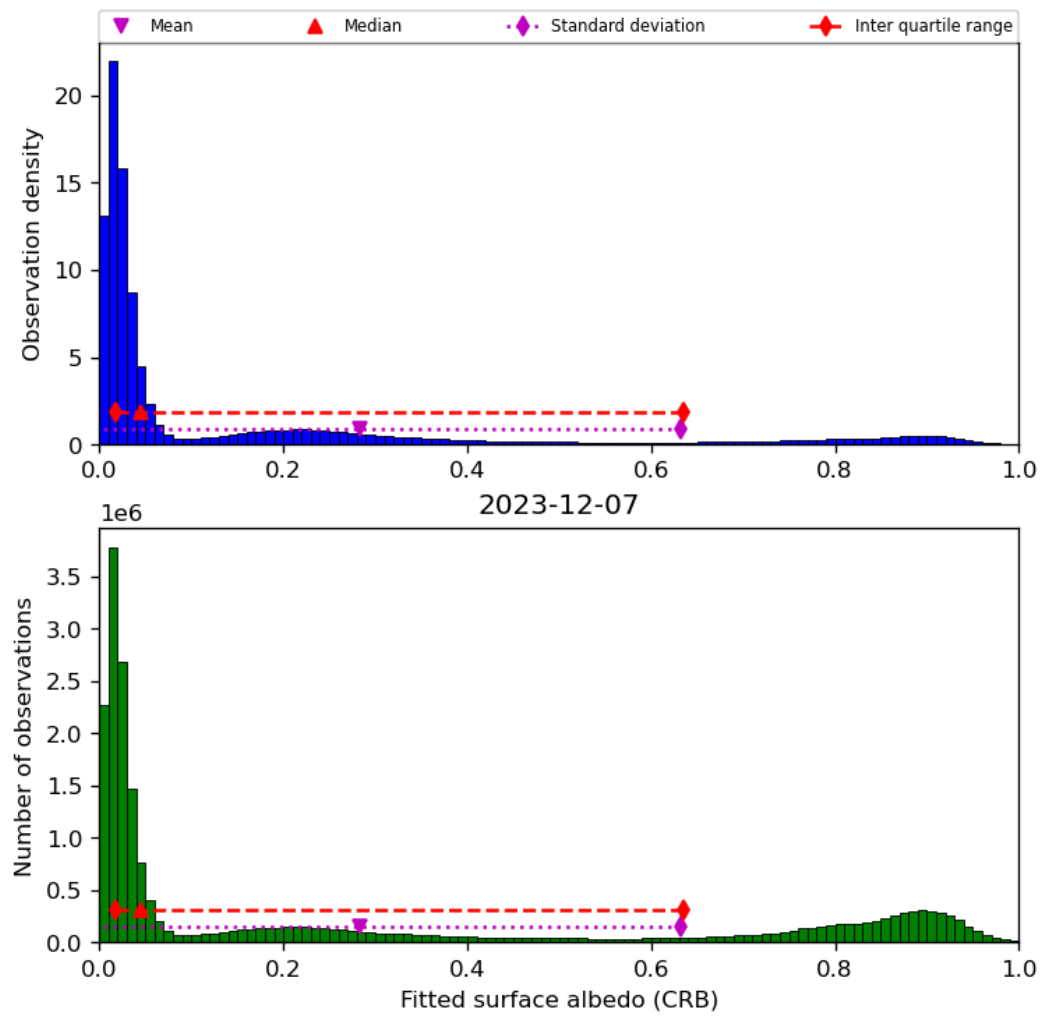
Figure 46: Histogram of “Fitted surface albedo (CRB)” for 2023-12-06 to 2023-12-08
