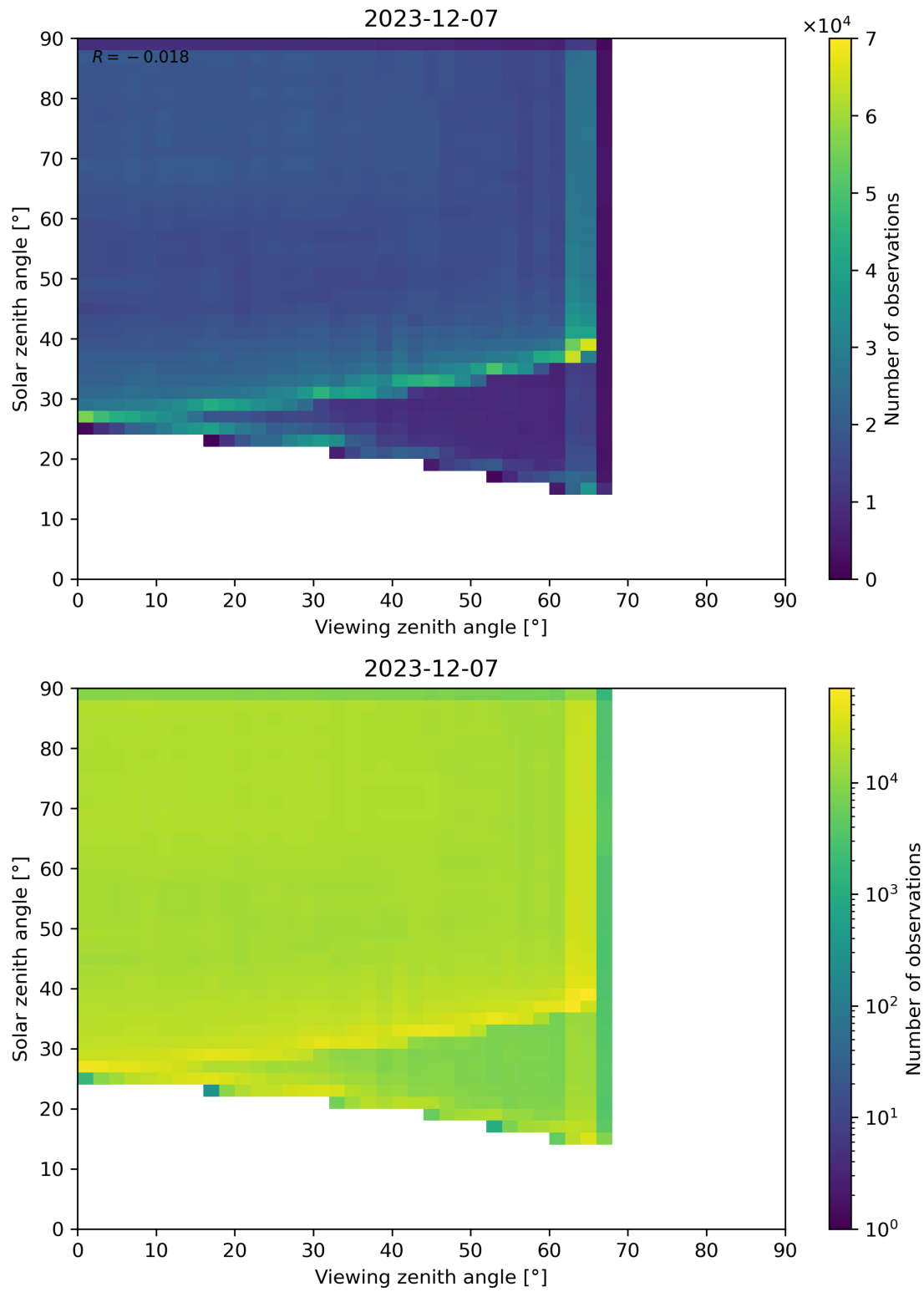
Figure 114: Scatter density plot of “Viewing zenith angle” against “Solar zenith angle” for 2023-12-06 to 2023-12-08.
