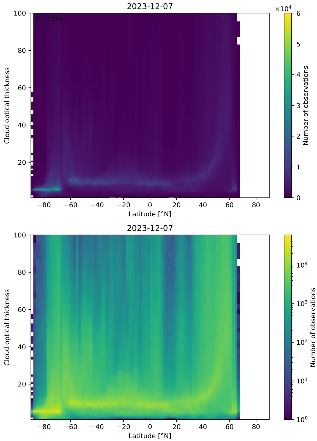
Figure 96: Scatter density plot of “Latitude” against “Cloud optical thickness” for 2023-12-06 to 2023-12-08.
