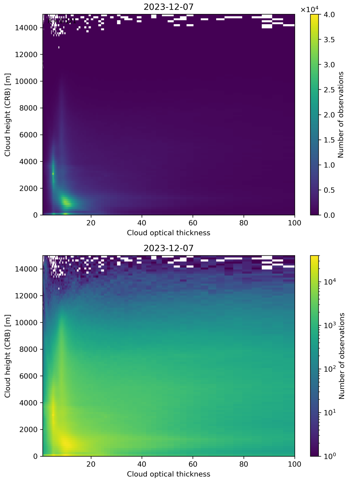
Figure 85: Scatter density plot of “Cloud optical thickness” against “Cloud height (CRB)” for 2023-12-06 to 2023-12-08.
