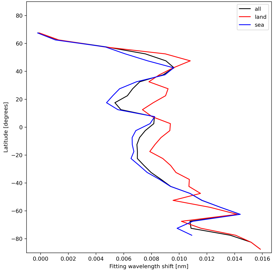
Figure 33: Zonal average of “Fitting wavelength shift” for 2023-12-06 to 2023-12-08.
