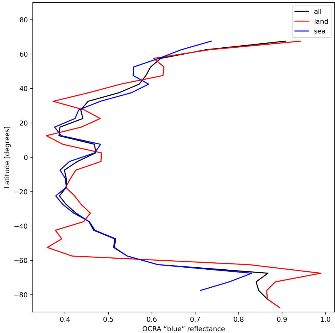
Figure 35: Zonal average of “OCRA “blue” reflectance” for 2023-12-06 to 2023-12-08.
