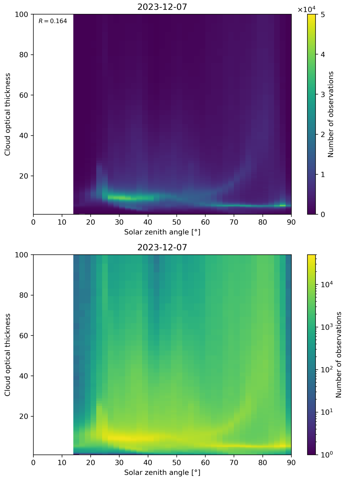
Figure 103: Scatter density plot of “Solar zenith angle” against “Cloud optical thickness” for 2023-12-06 to 2023-12-08.
