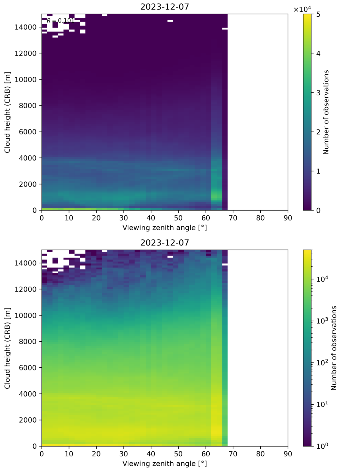
Figure 110: Scatter density plot of “Viewing zenith angle” against “Cloud height (CRB)” for 2023-12-06 to 2023-12-08.
