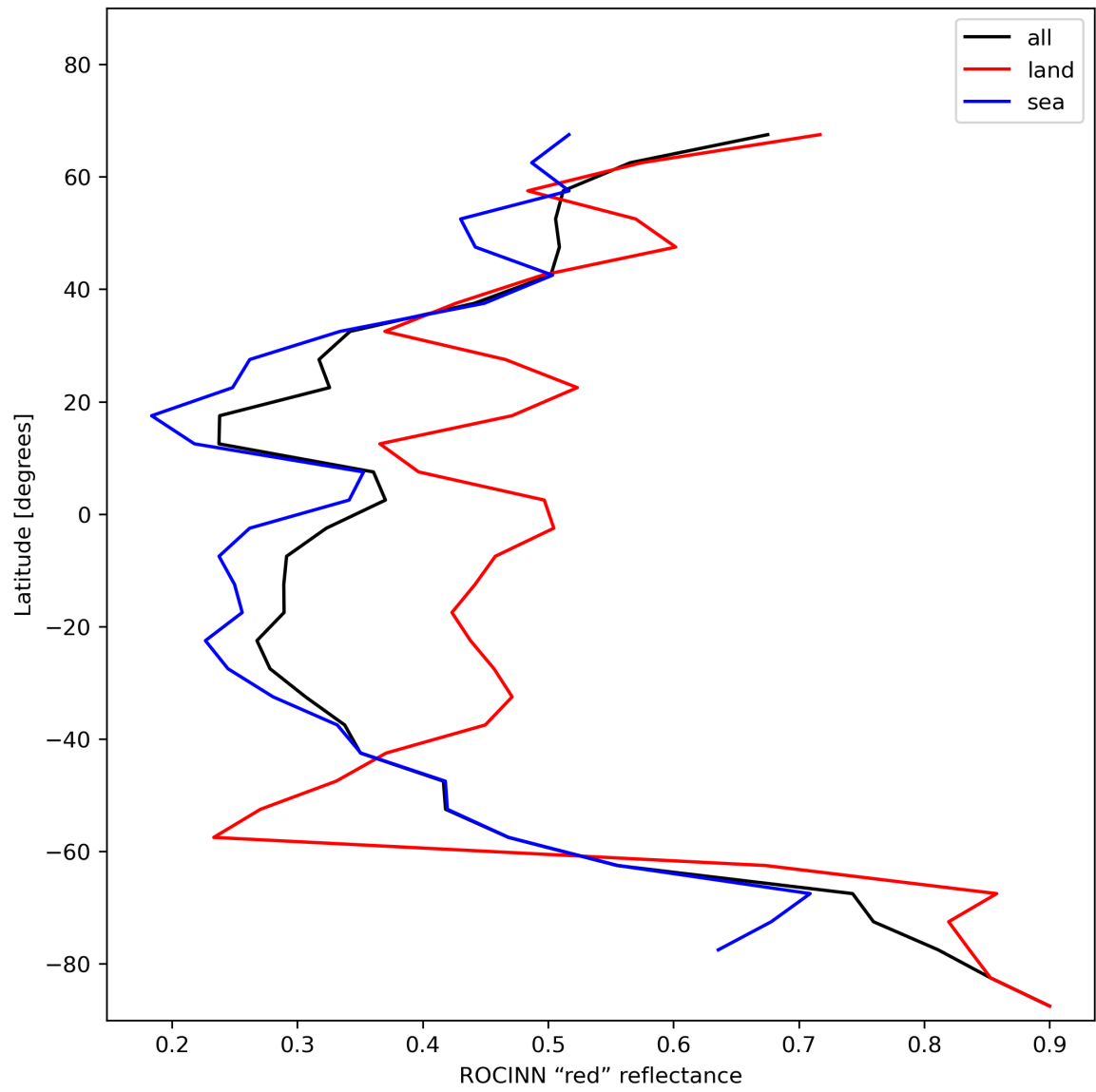
Figure 37: Zonal average of “ROCINN “red” reflectance” for 2023-12-06 to 2023-12-08.
