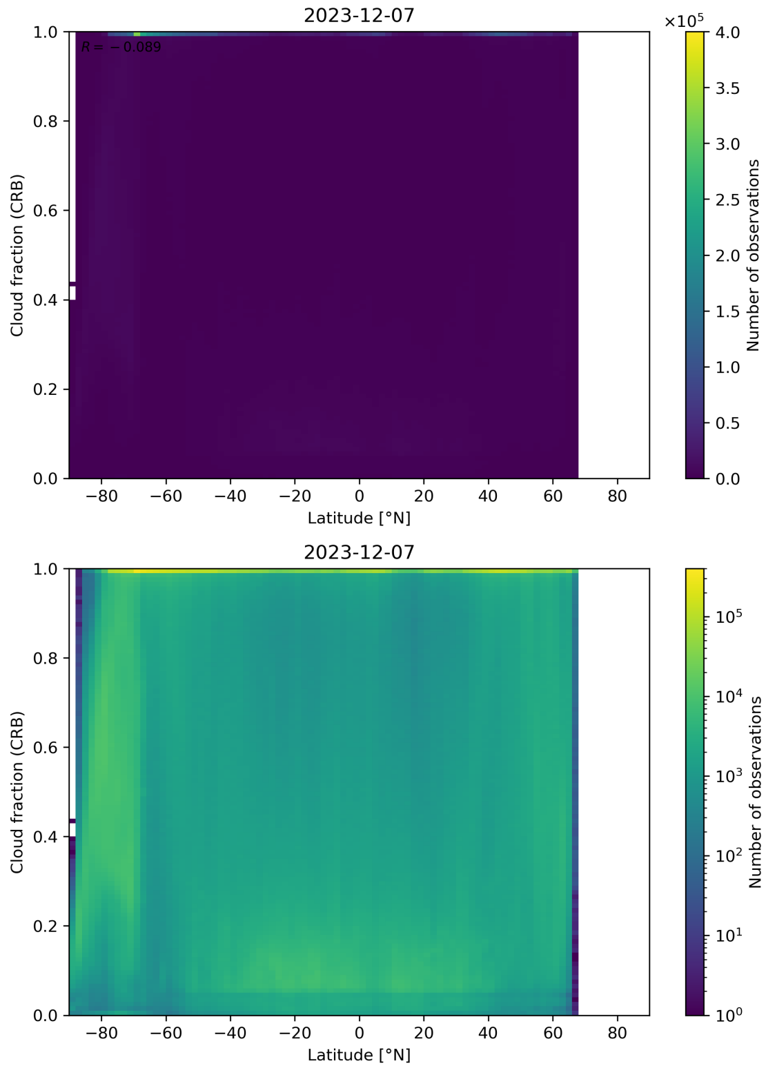
Figure 94: Scatter density plot of “Latitude” against “Cloud fraction (CRB)” for 2023-12-06 to 2023-12-08.
