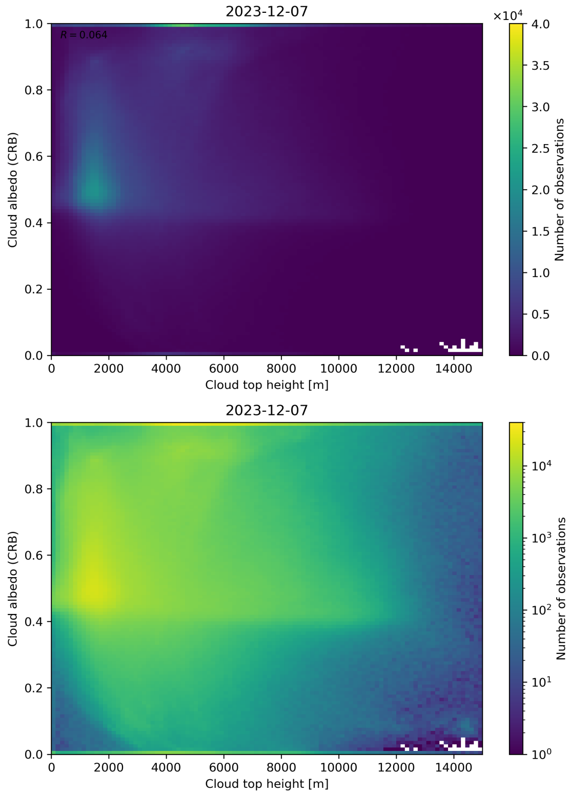
Figure 86: Scatter density plot of “Cloud top height” against “Cloud albedo (CRB)” for 2023-12-06 to 2023-12-08.
