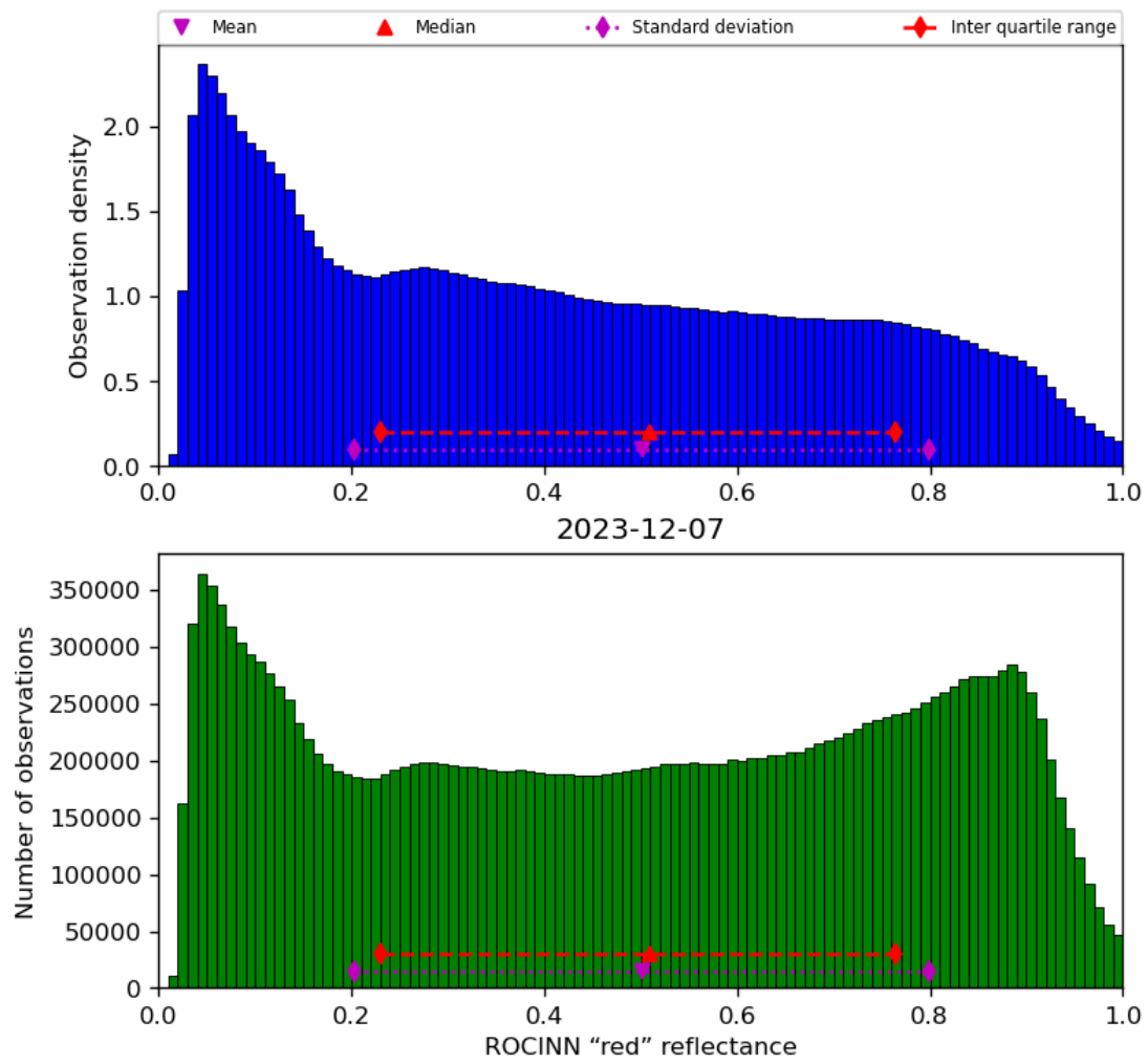
Figure 53: Histogram of “ROCINN “red” reflectance” for 2023-12-06 to 2023-12-08
