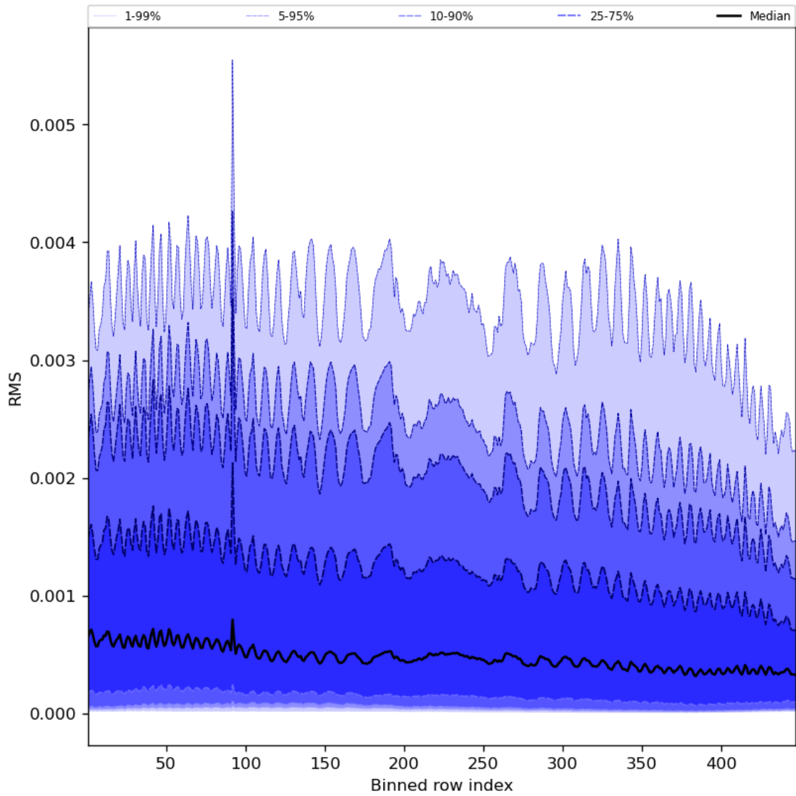
Figure 63: Along track statistics of “RMS” for 2023-12-06 to 2023-12-08
