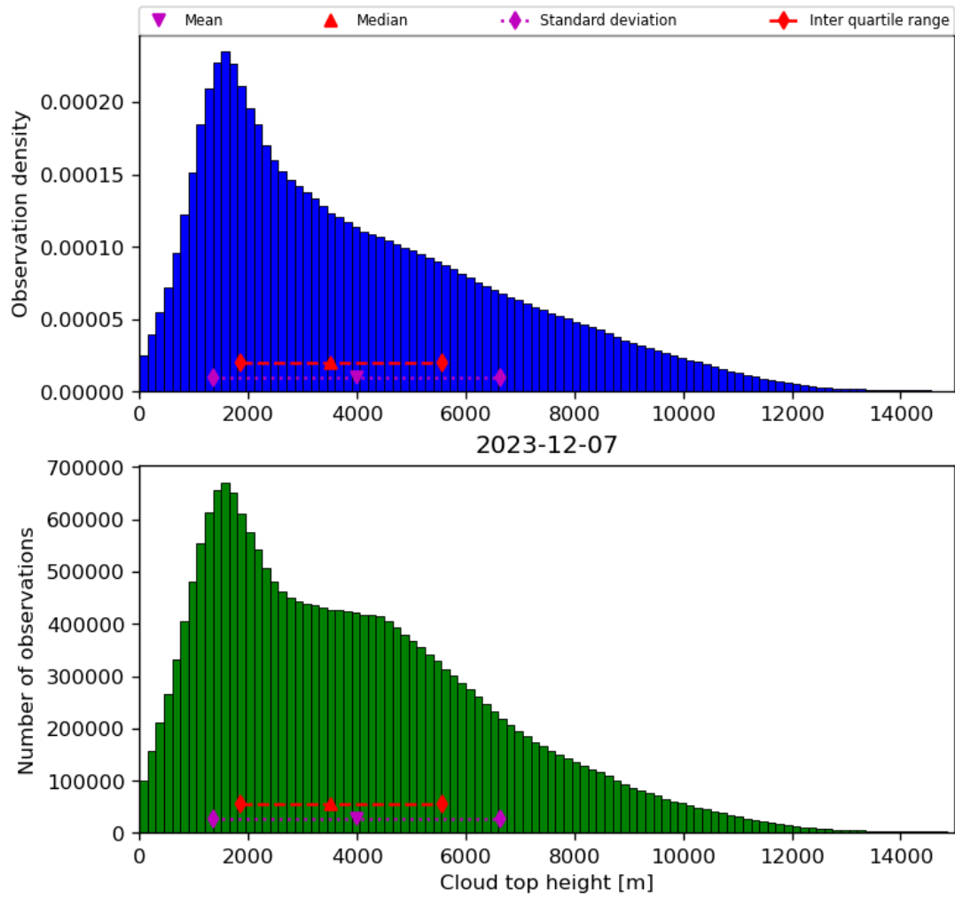
Figure 40: Histogram of “Cloud top height” for 2023-12-06 to 2023-12-08
