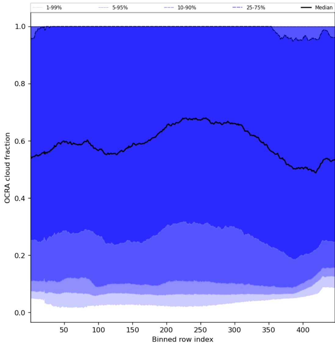
Figure 66: Along track statistics of “OCRA cloud fraction” for 2023-12-06 to 2023-12-08
