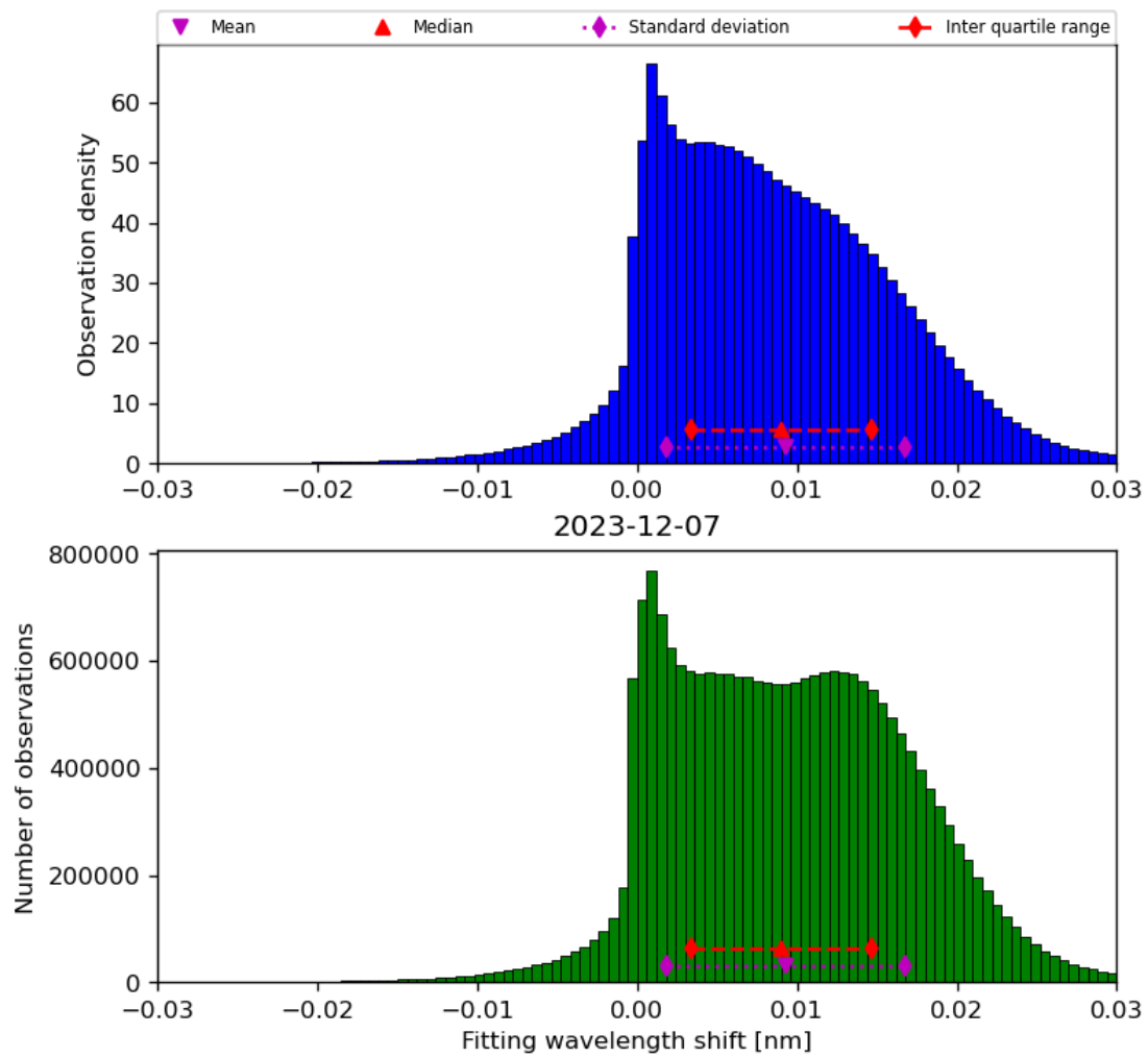
Figure 49: Histogram of “Fitting wavelength shift” for 2023-12-06 to 2023-12-08
