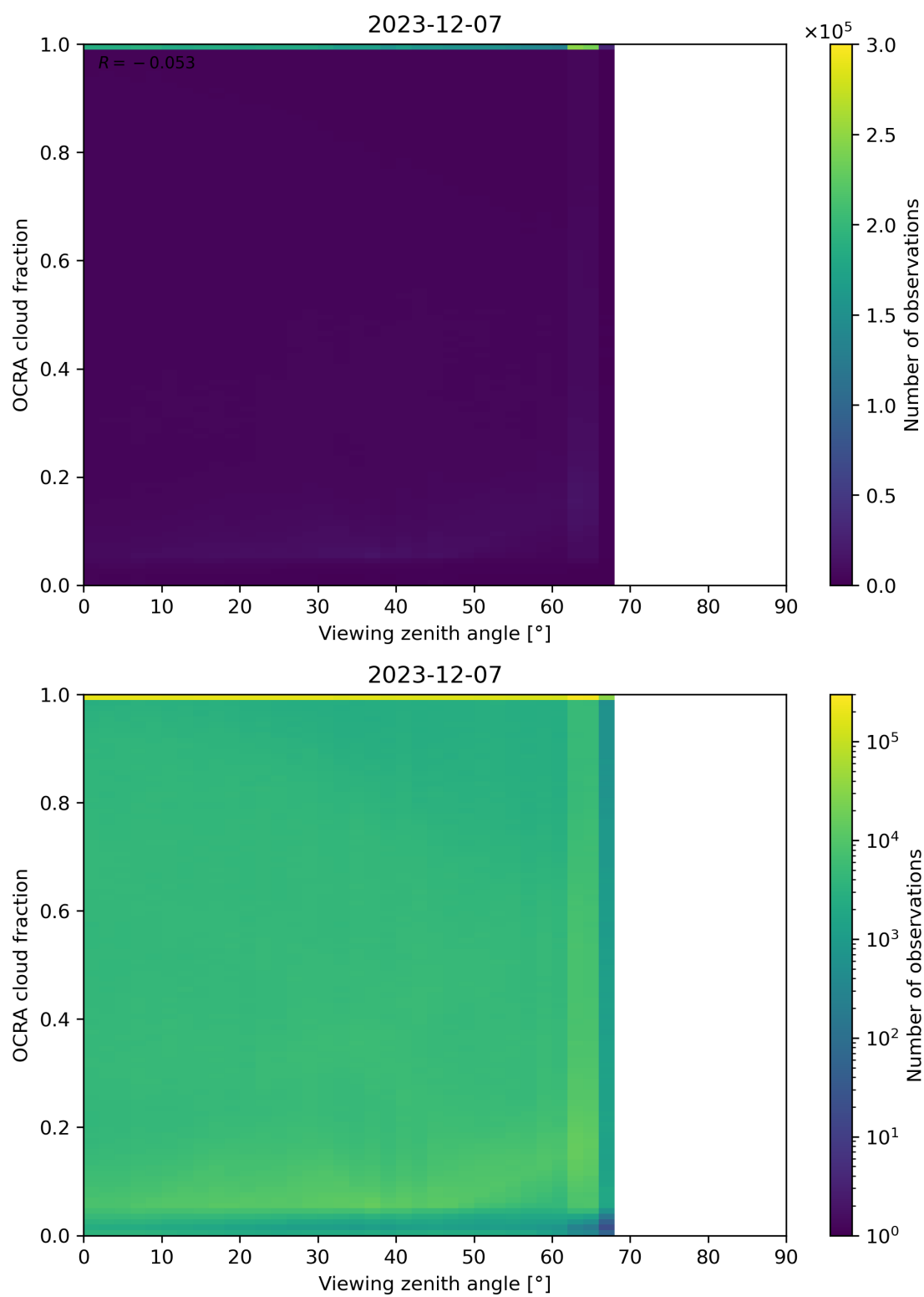
Figure 108: Scatter density plot of “Viewing zenith angle” against “OCRA cloud fraction” for 2023-12-06 to 2023-12-08.
