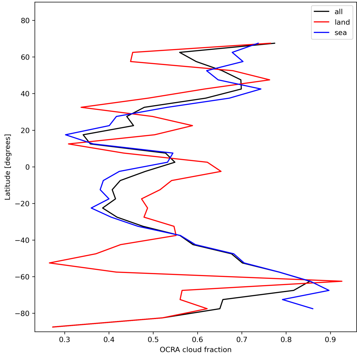
Figure 34: Zonal average of “OCRA cloud fraction” for 2023-12-06 to 2023-12-08.
