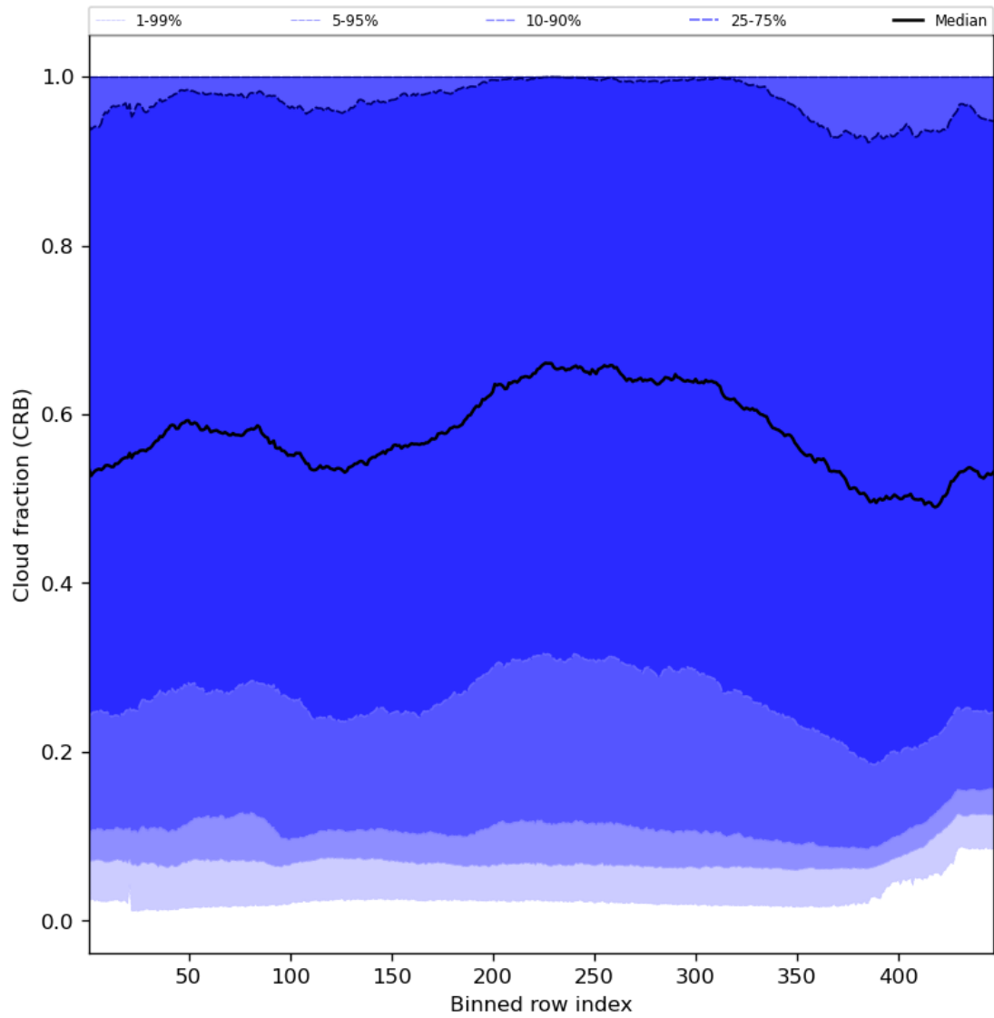
Figure 58: Along track statistics of “Cloud fraction (CRB)” for 2023-12-06 to 2023-12-08
