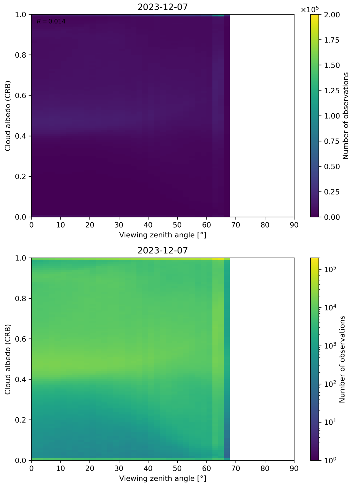
Figure 106: Scatter density plot of “Viewing zenith angle” against “Cloud albedo (CRB)” for 2023-12-06 to 2023-12-08.
