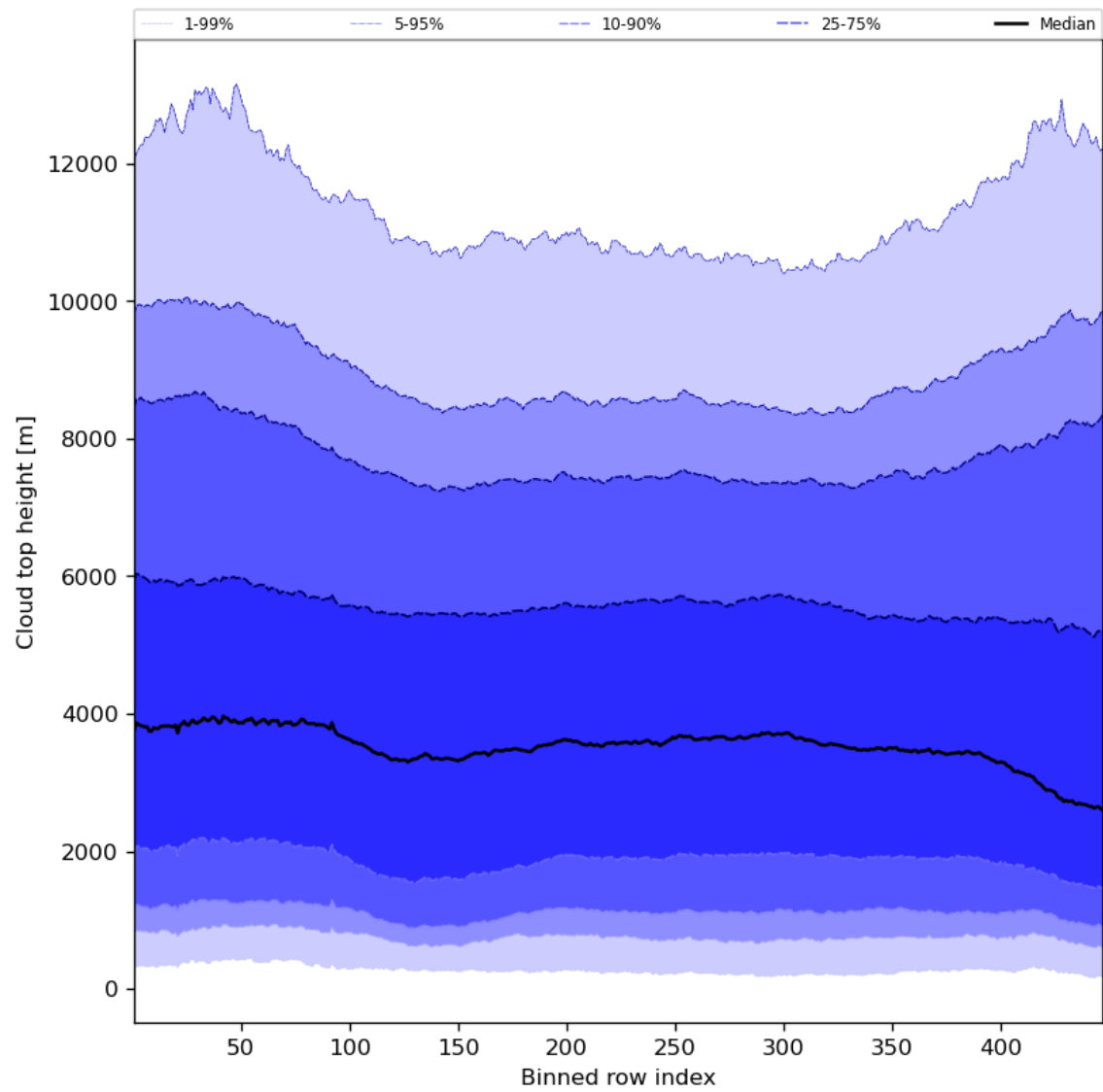
Figure 56: Along track statistics of “Cloud top height” for 2023-12-06 to 2023-12-08
