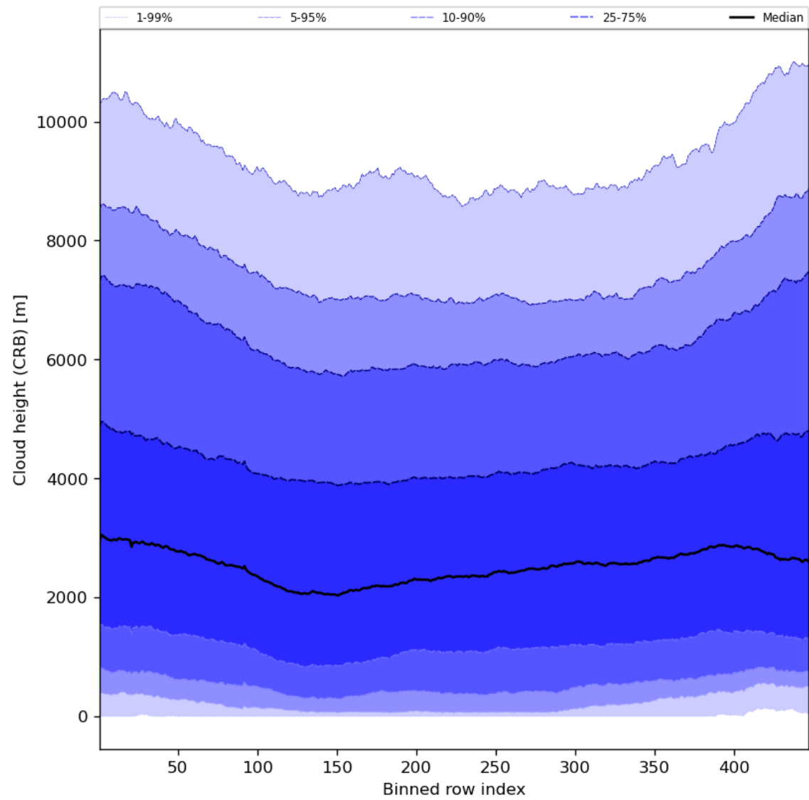
Figure 59: Along track statistics of “Cloud height (CRB)” for 2023-12-06 to 2023-12-08
