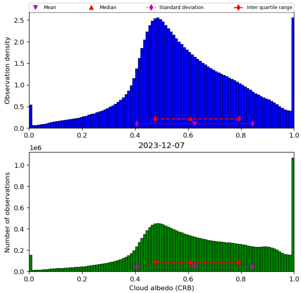
Figure 44: Histogram of “Cloud albedo (CRB)” for 2023-12-06 to 2023-12-08
