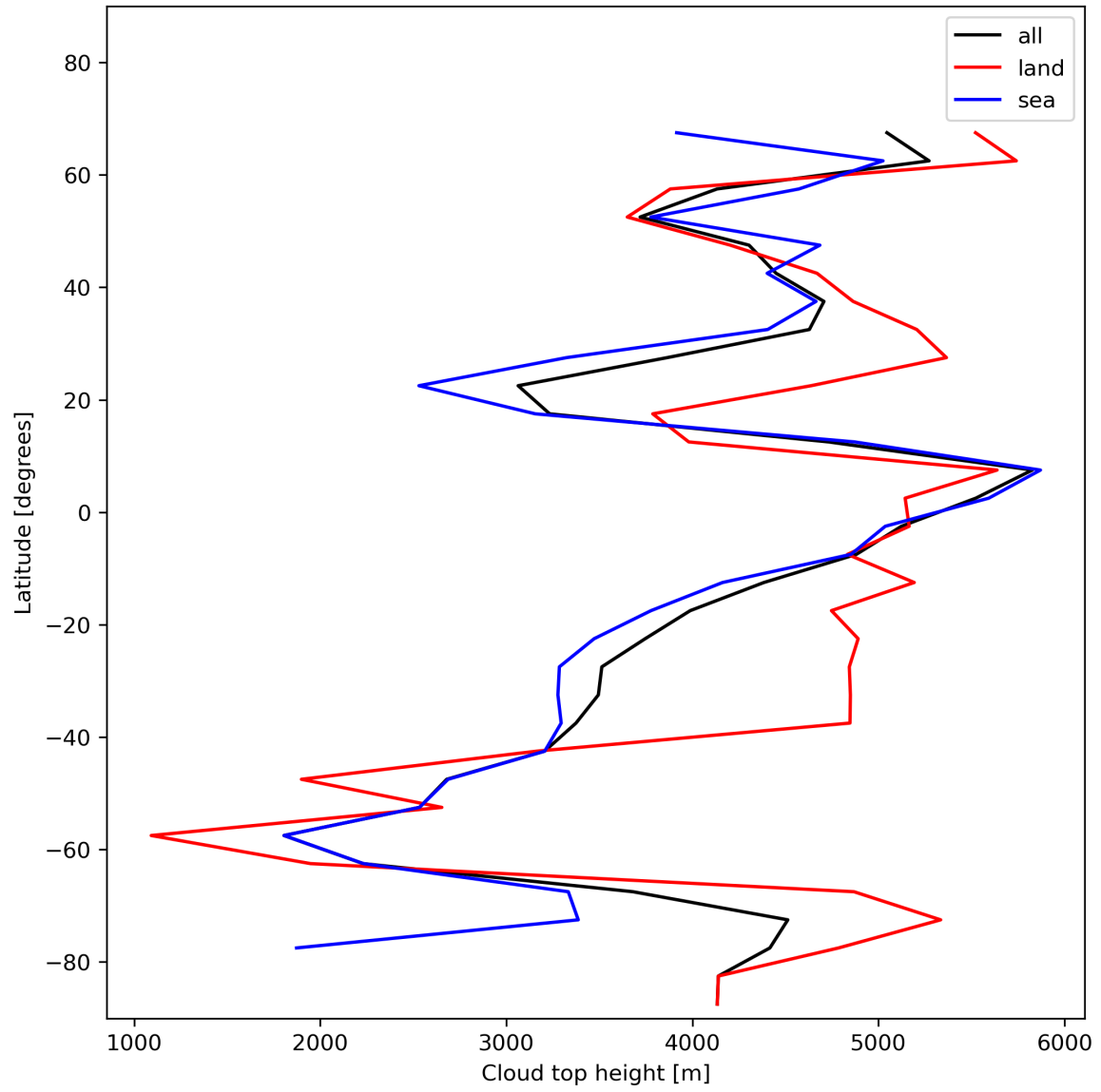
Figure 24: Zonal average of “Cloud top height” for 2023-12-06 to 2023-12-08.
