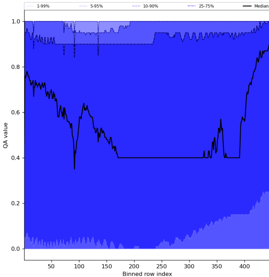
Figure 54: Along track statistics of “QA value” for 2023-12-06 to 2023-12-08
