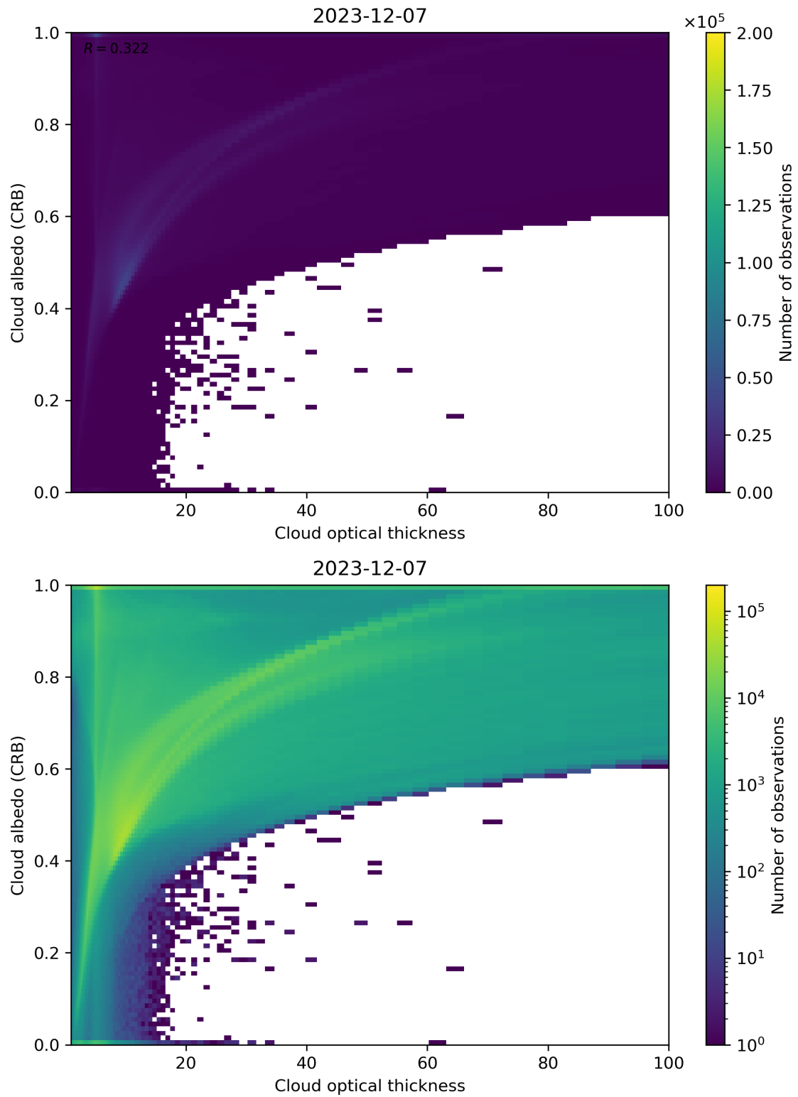
Figure 82: Scatter density plot of “Cloud optical thickness” against “Cloud albedo (CRB)” for 2023-12-06 to 2023-12-08.
