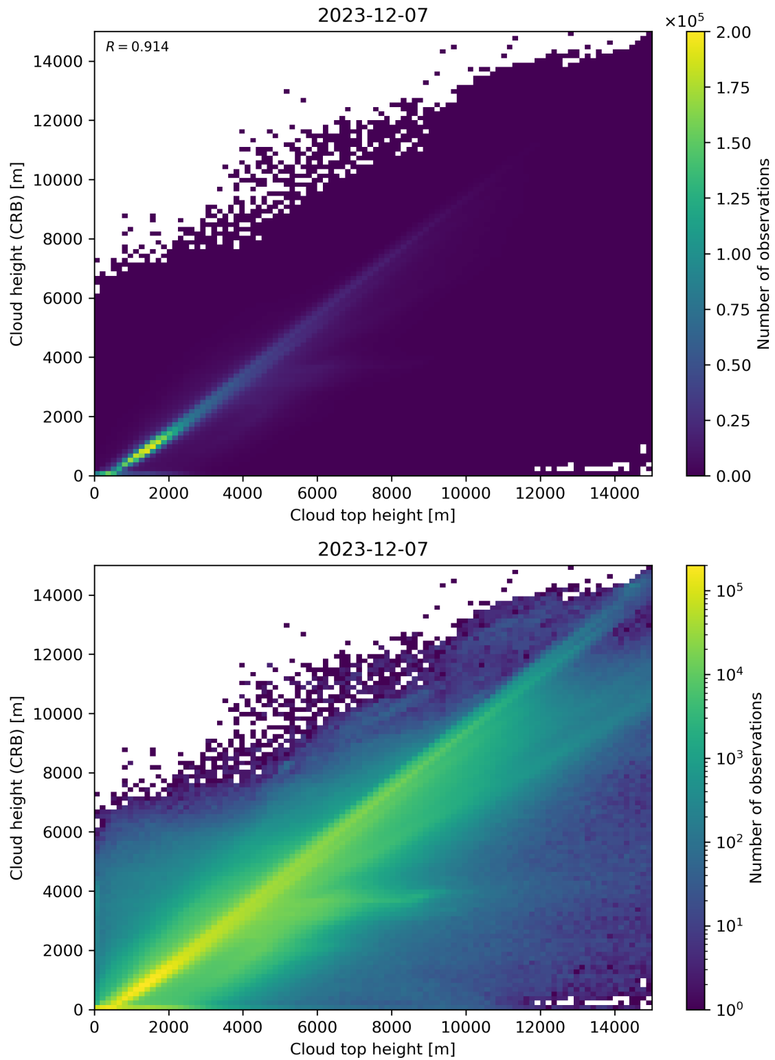
Figure 89: Scatter density plot of “Cloud top height” against “Cloud height (CRB)” for 2023-12-06 to 2023-12-08.
