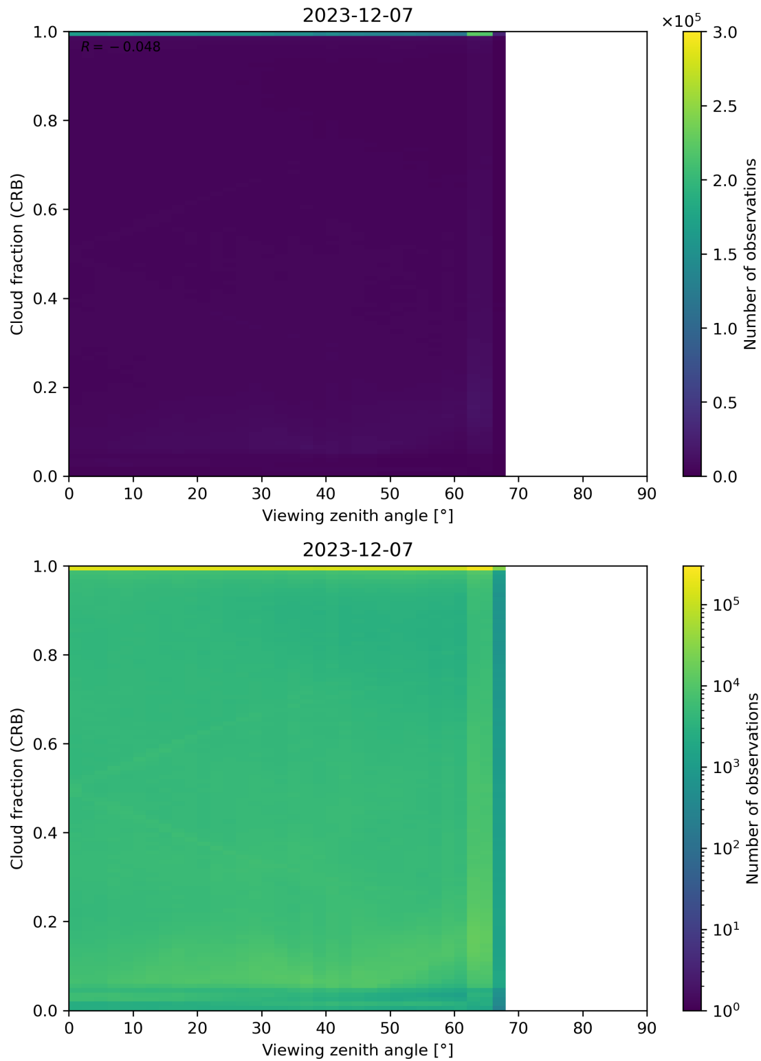
Figure 109: Scatter density plot of “Viewing zenith angle” against “Cloud fraction (CRB)” for 2023-12-06 to 2023-12-08.
