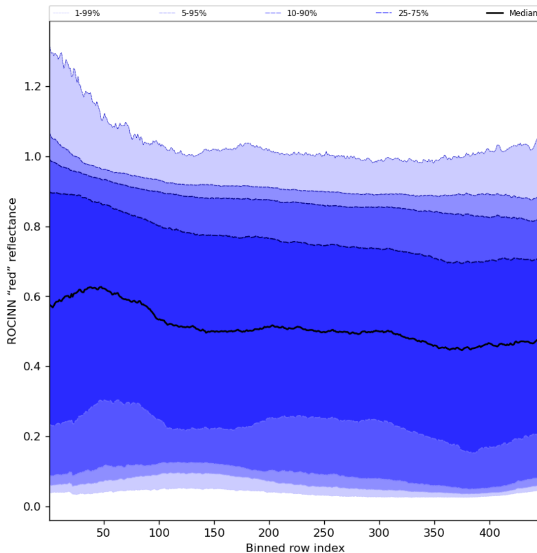
Figure 69: Along track statistics of “ROCINN “red” reflectance” for 2023-12-06 to 2023-12-08
