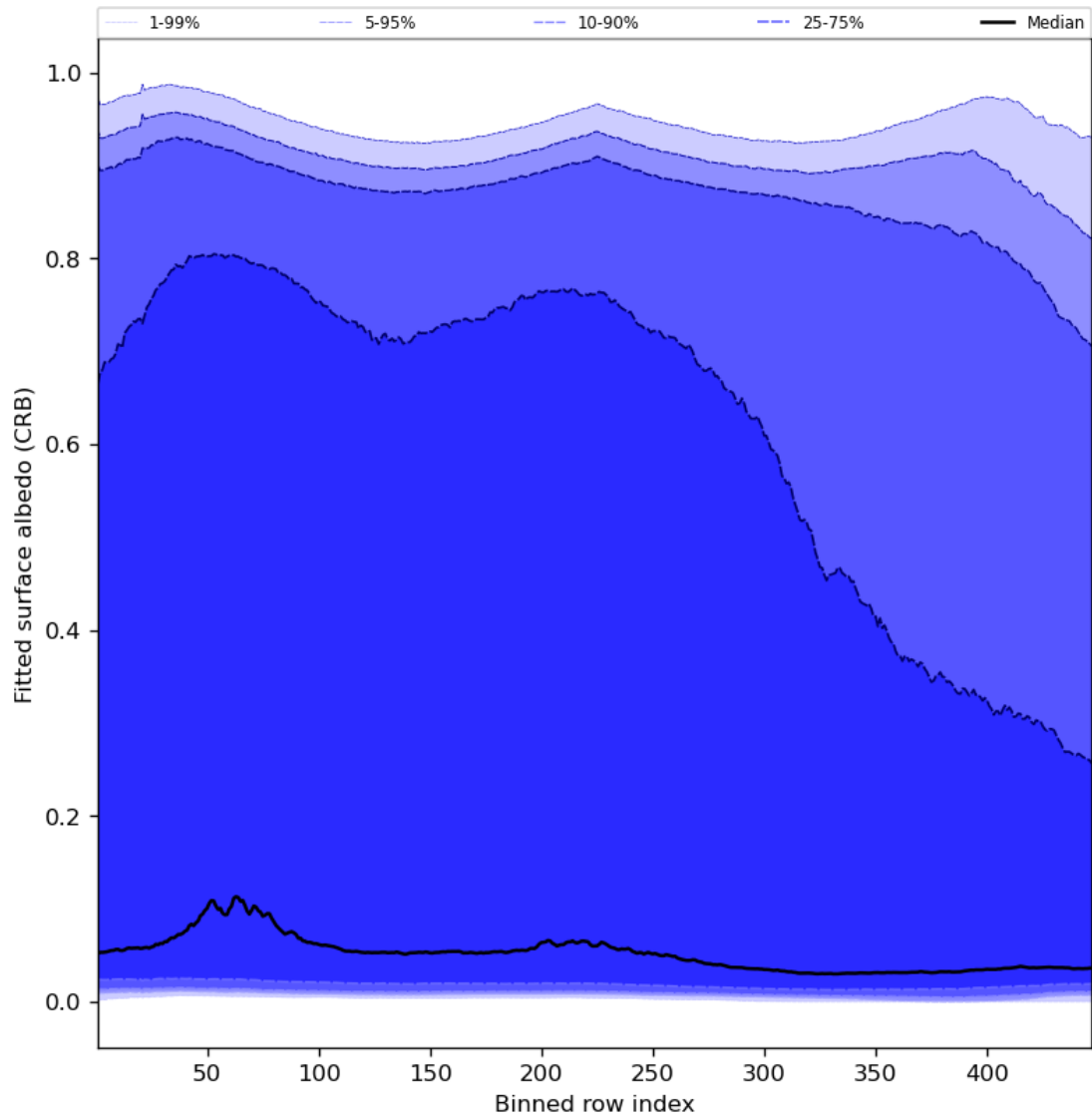
Figure 62: Along track statistics of “Fitted surface albedo (CRB)” for 2023-12-06 to 2023-12-08
