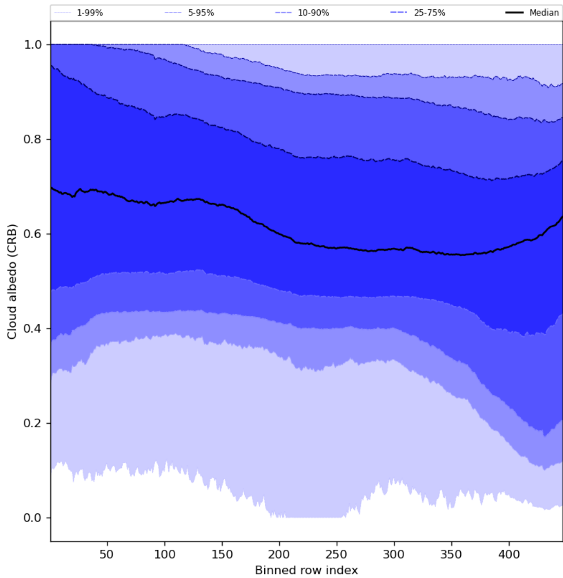
Figure 60: Along track statistics of “Cloud albedo (CRB)” for 2023-12-06 to 2023-12-08
