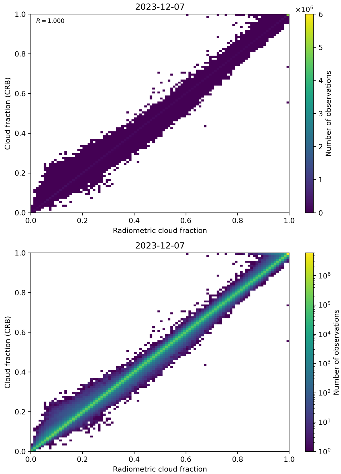
Figure 73: Scatter density plot of “Radiometric cloud fraction” against “Cloud fraction (CRB)” for 2023-12-06 to 2023-12-08.
