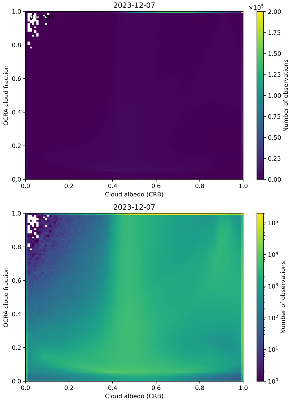
Figure 70: Scatter density plot of “Cloud albedo (CRB)” against “OCRA cloud fraction” for 2023-12-06 to 2023-12-08.
