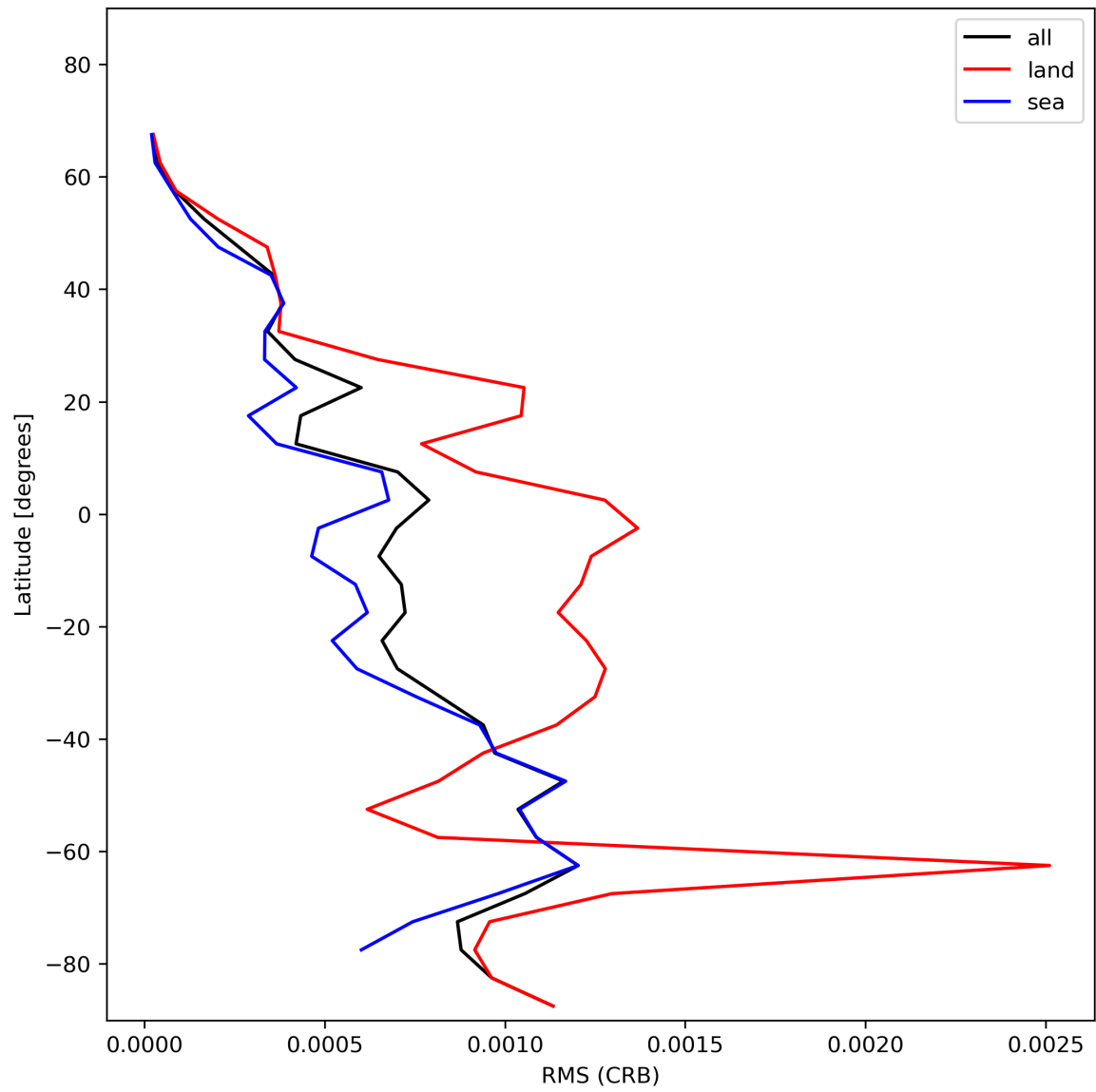
Figure 32: Zonal average of “RMS (CRB)” for 2023-12-06 to 2023-12-08.
