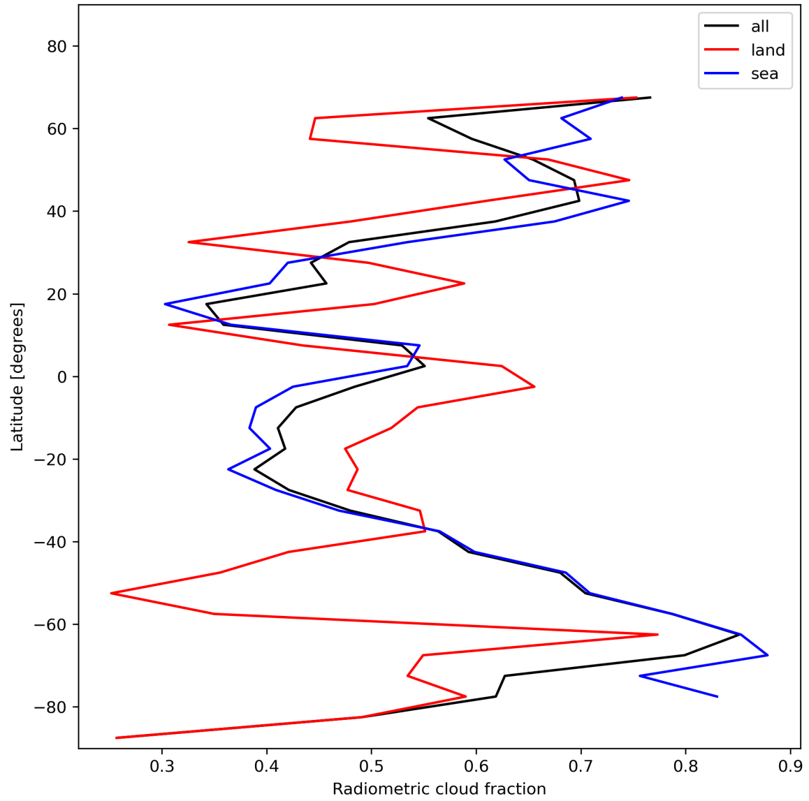
Figure 23: Zonal average of “Radiometric cloud fraction” for 2023-12-06 to 2023-12-08.
