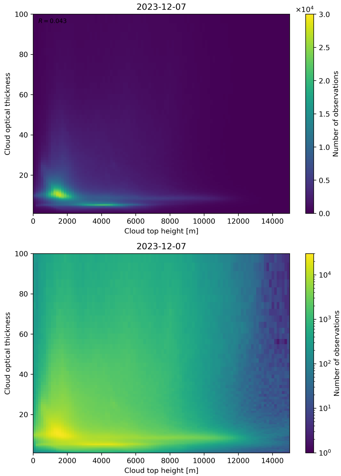
Figure 90: Scatter density plot of “Cloud top height” against “Cloud optical thickness” for 2023-12-06 to 2023-12-08.
