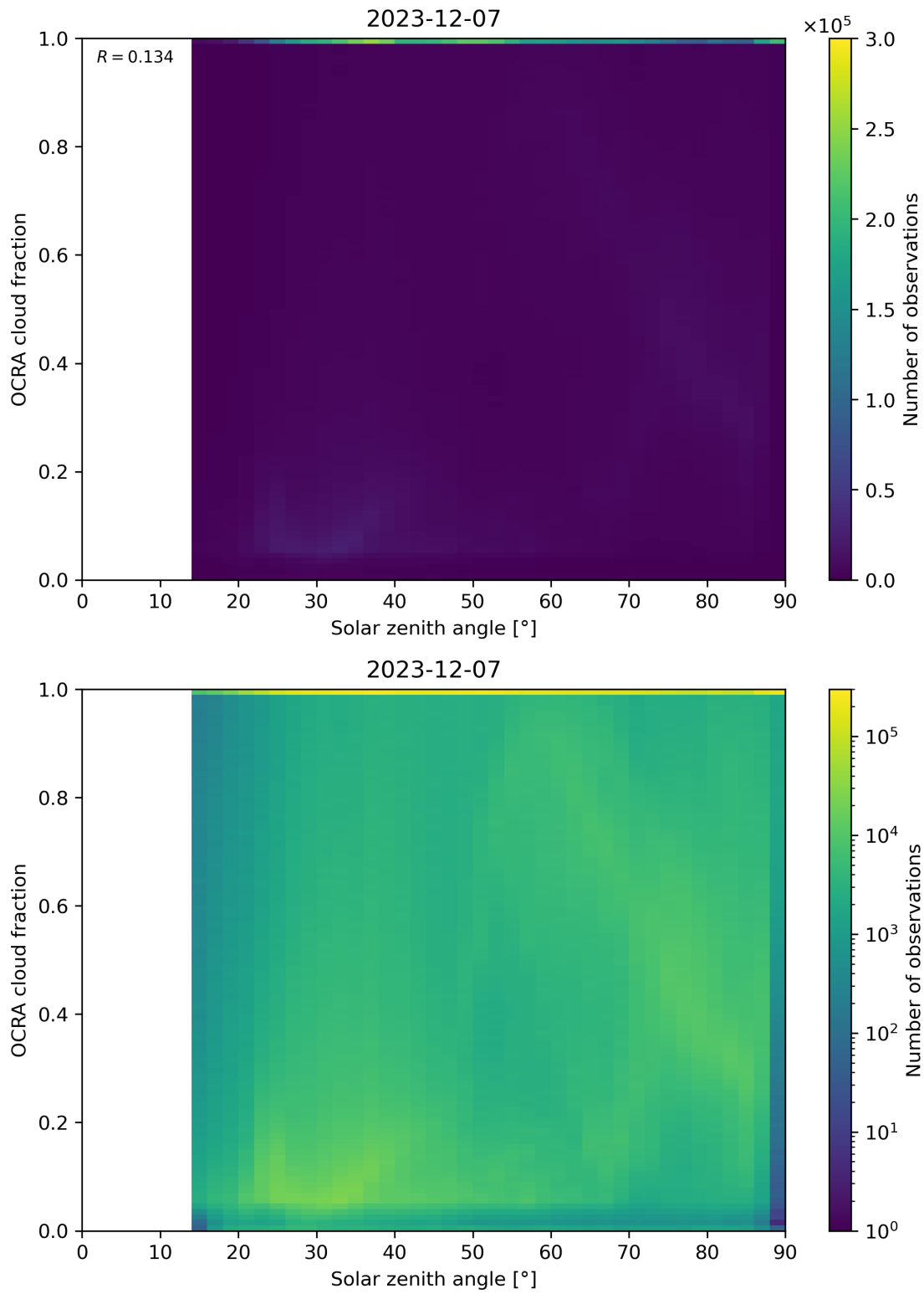
Figure 100: Scatter density plot of “Solar zenith angle” against “OCRA cloud fraction” for 2023-12-06 to 2023-12-08.
