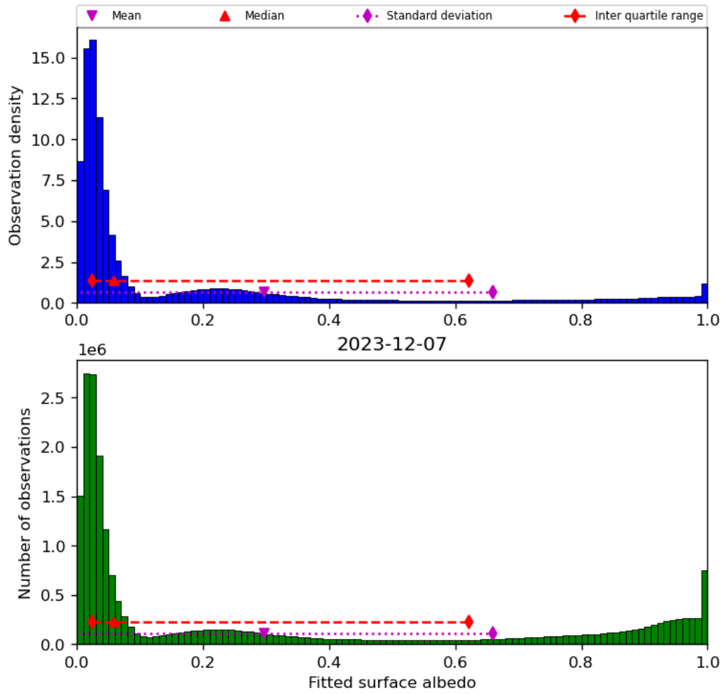
Figure 45: Histogram of “Fitted surface albedo” for 2023-12-06 to 2023-12-08
