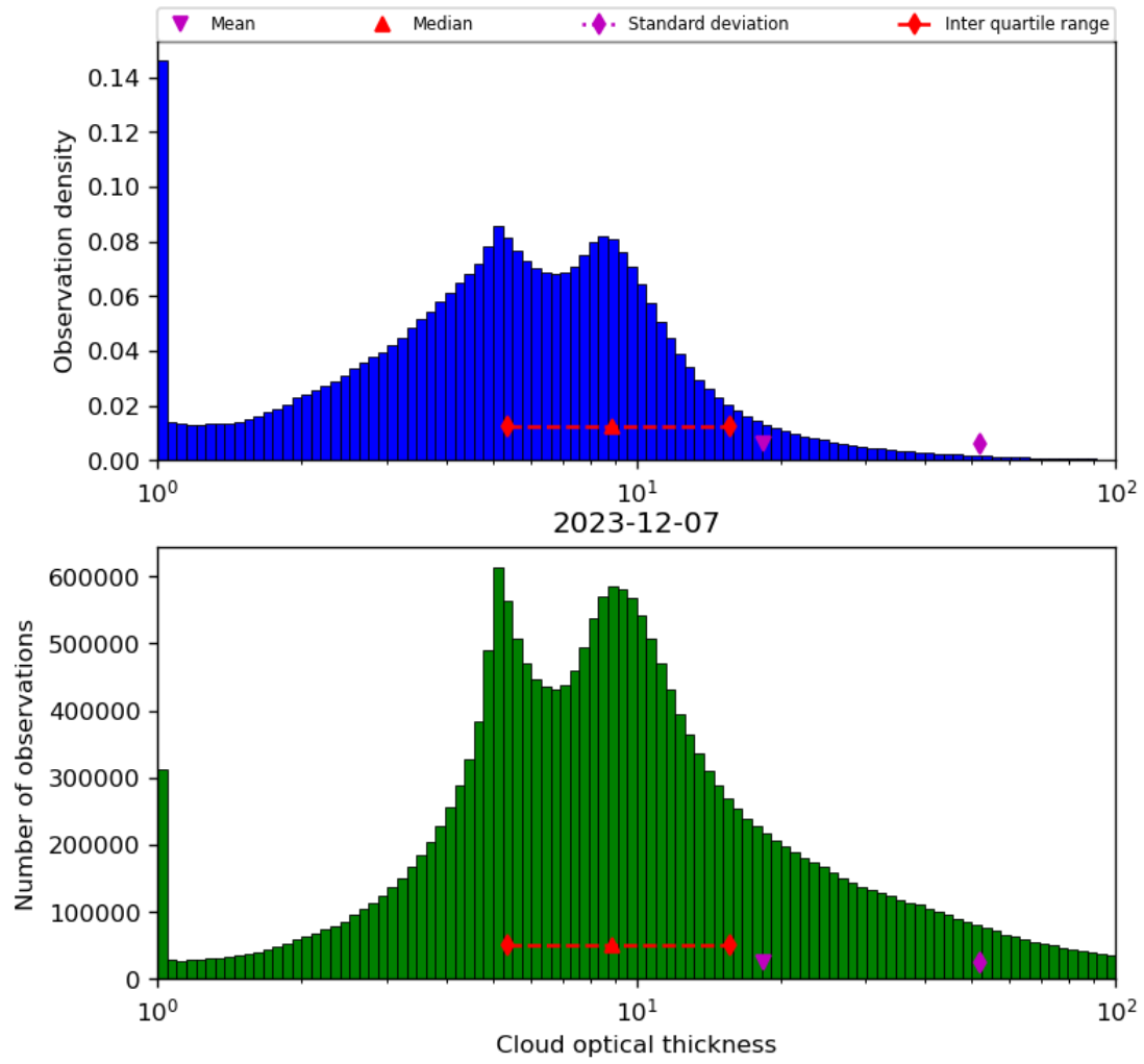
Figure 41: Histogram of “Cloud optical thickness” for 2023-12-06 to 2023-12-08
