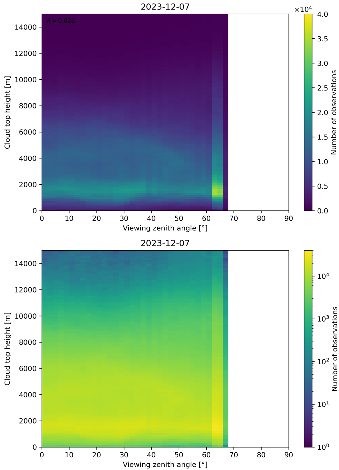
Figure 112: Scatter density plot of “Viewing zenith angle” against “Cloud top height” for 2023-12-06 to 2023-12-08.
