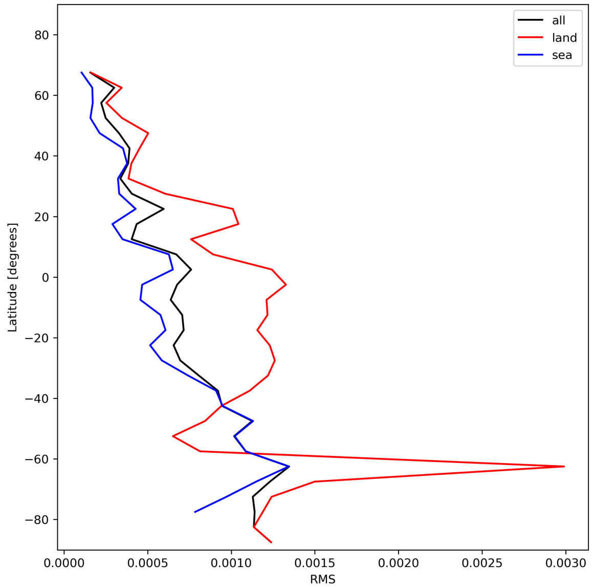
Figure 31: Zonal average of “RMS” for 2023-12-06 to 2023-12-08.
