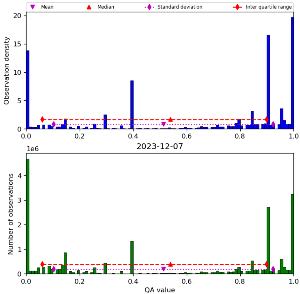
Figure 38: Histogram of “QA value” for 2023-12-06 to 2023-12-08
