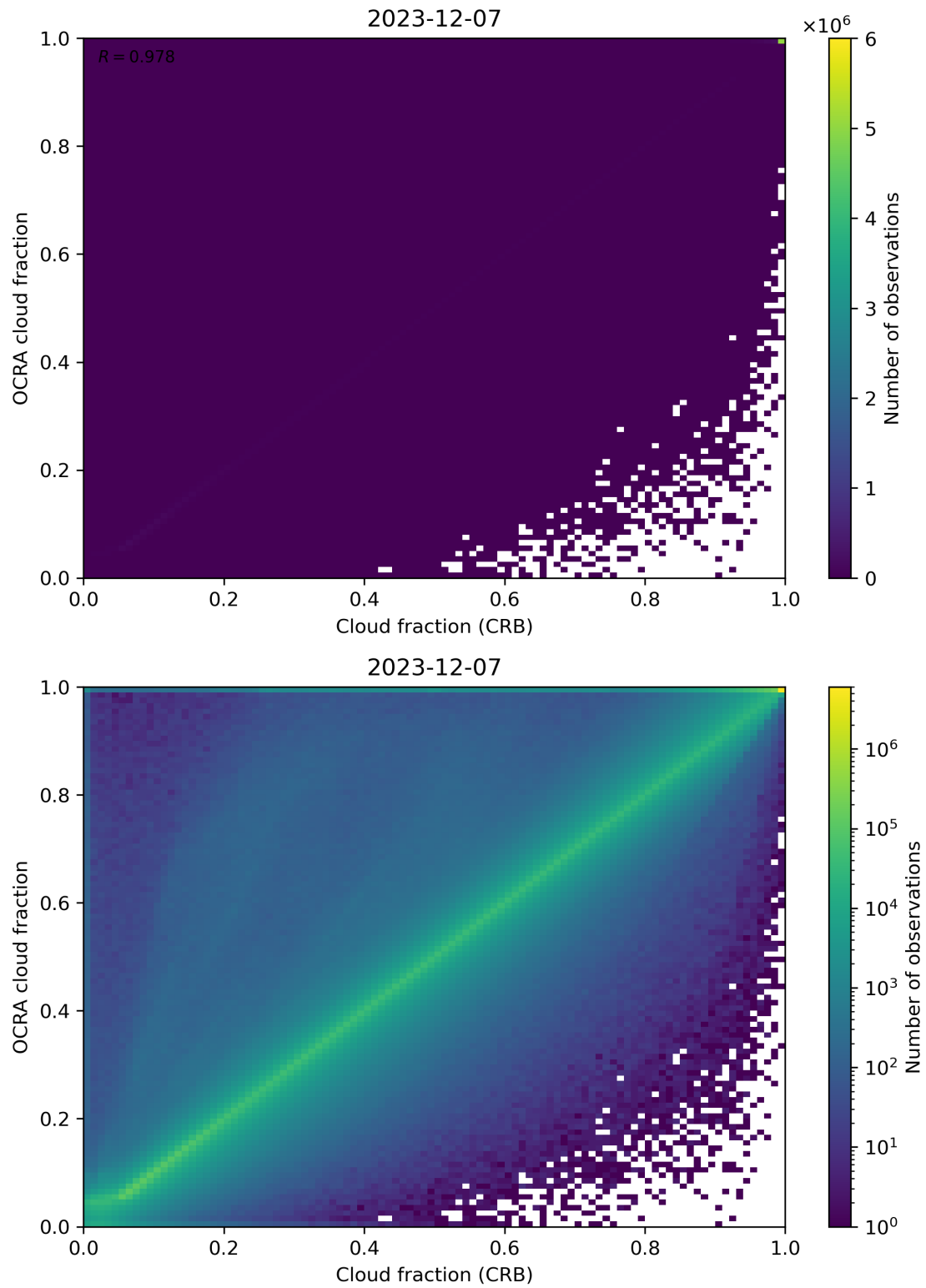
Figure 78: Scatter density plot of “Cloud fraction (CRB)” against “OCRA cloud fraction” for 2023-12-06 to 2023-12-08.
