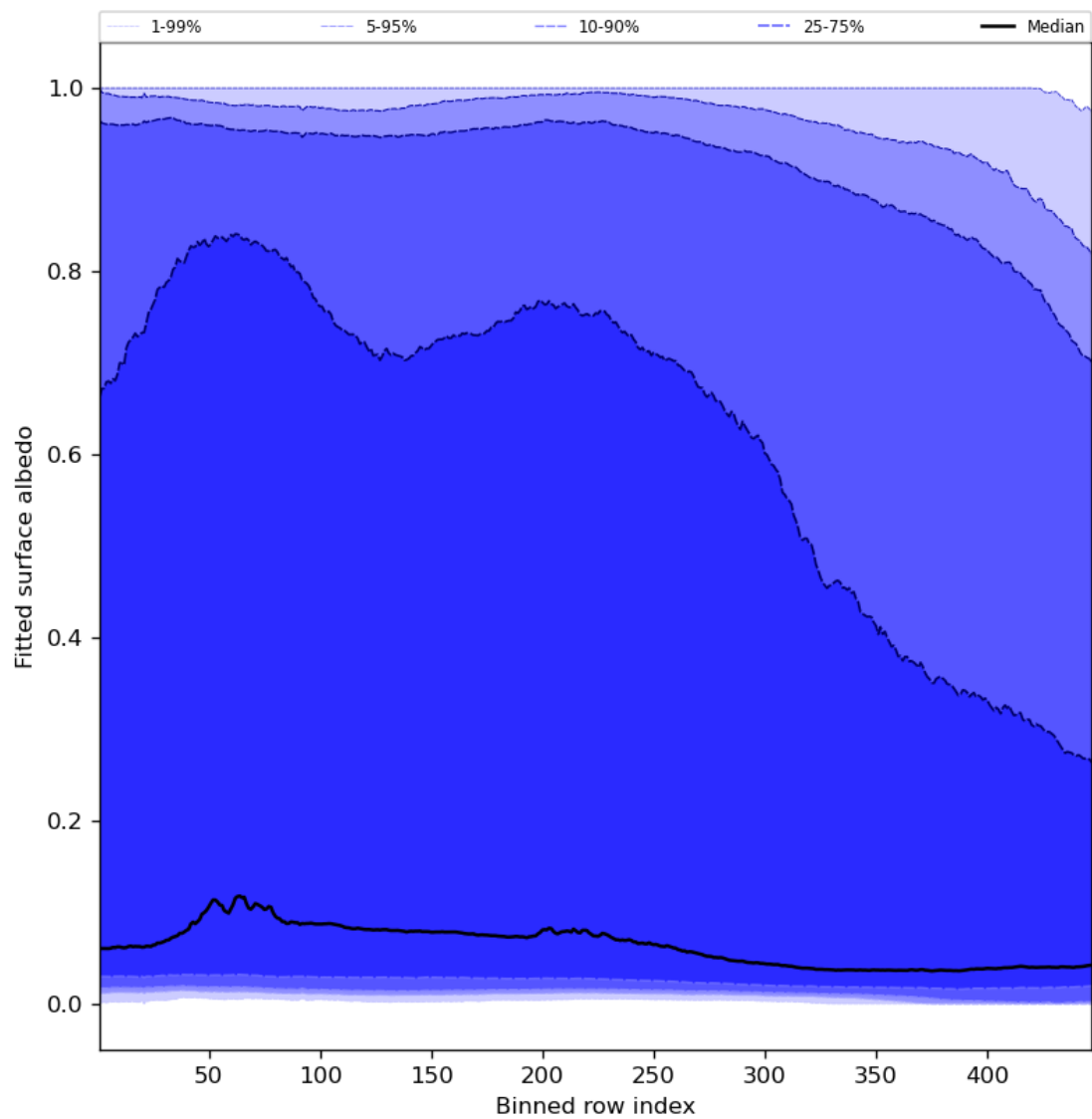
Figure 61: Along track statistics of “Fitted surface albedo” for 2023-12-06 to 2023-12-08
