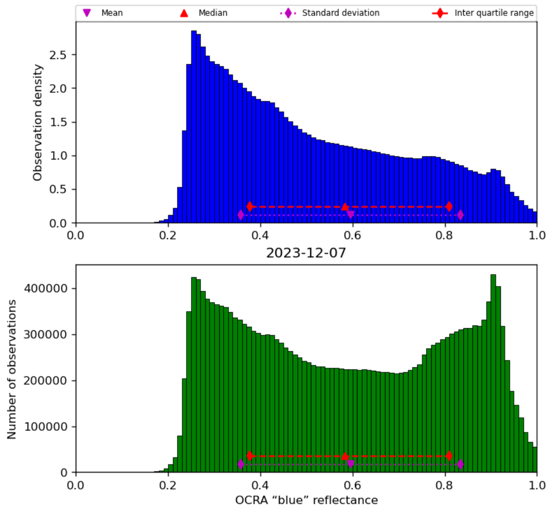
Figure 51: Histogram of “OCRA “blue” reflectance” for 2023-12-06 to 2023-12-08
