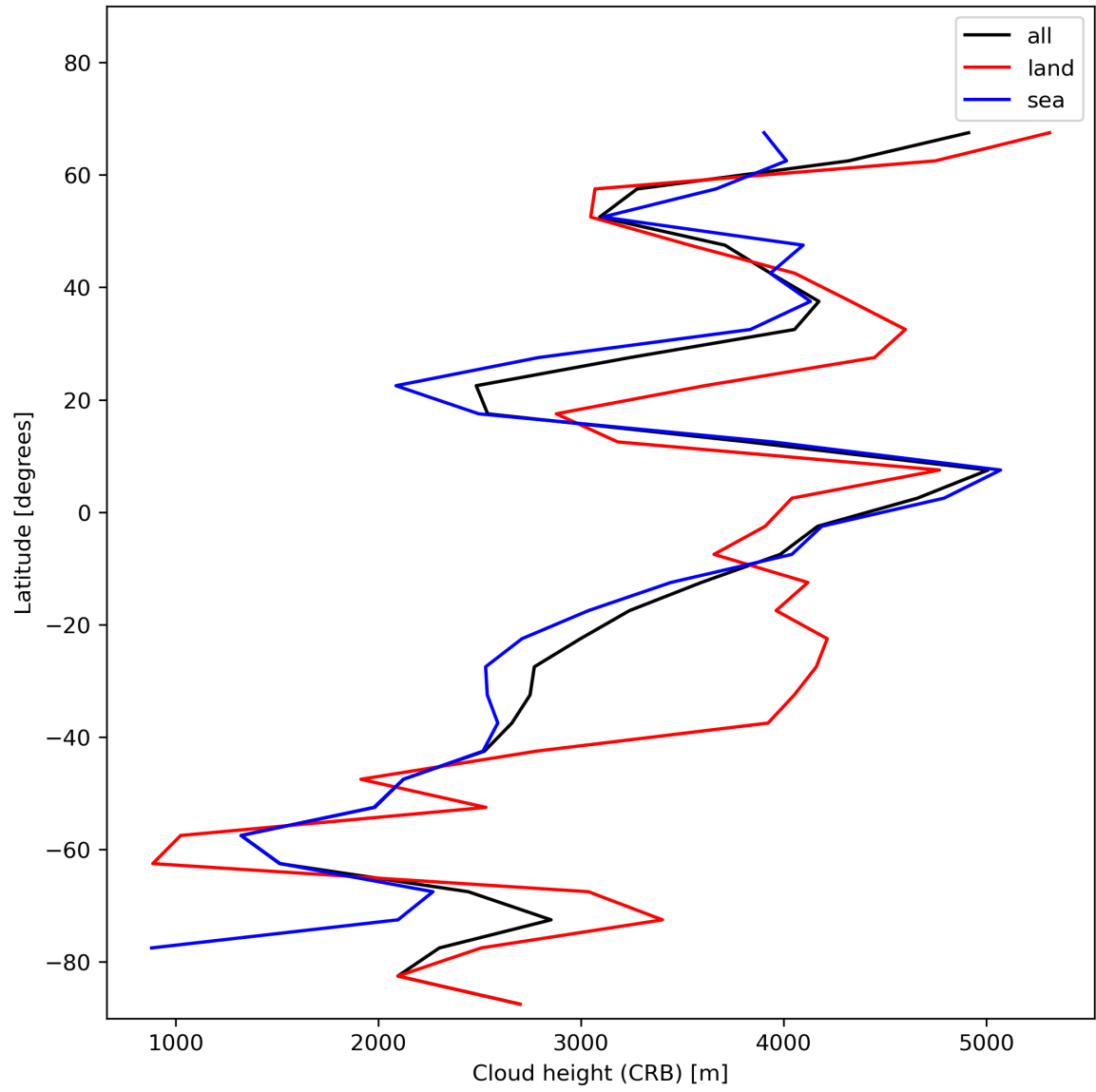
Figure 27: Zonal average of “Cloud height (CRB)” for 2023-12-06 to 2023-12-08.
