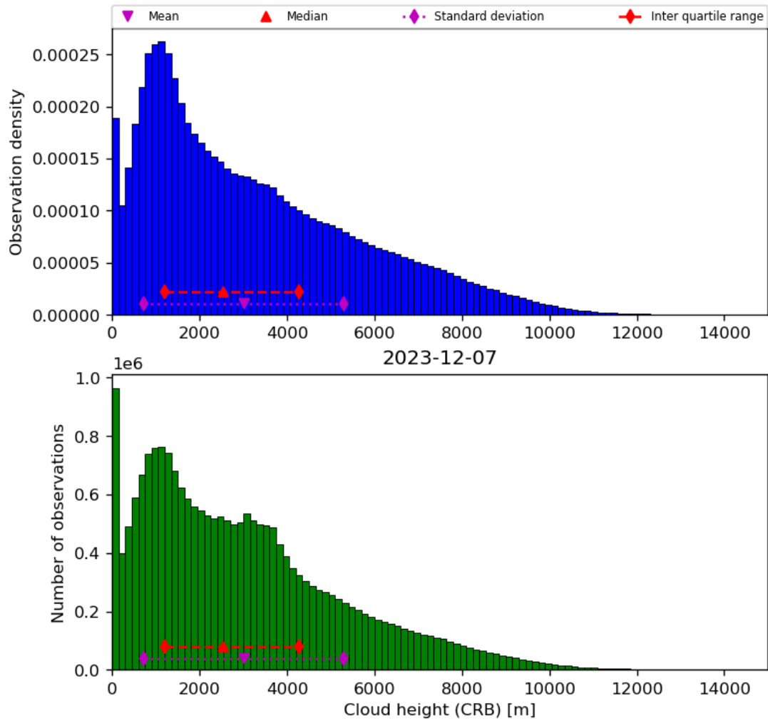
Figure 43: Histogram of “Cloud height (CRB)” for 2023-12-06 to 2023-12-08
