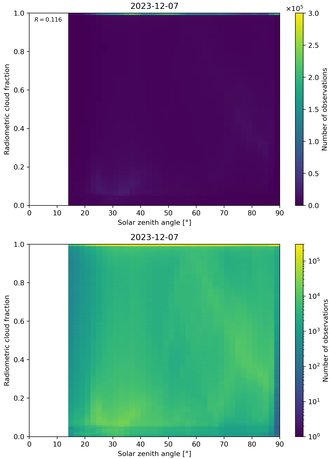
Figure 99: Scatter density plot of “Solar zenith angle” against “Radiometric cloud fraction” for 2023-12-06 to 2023-12-08.
