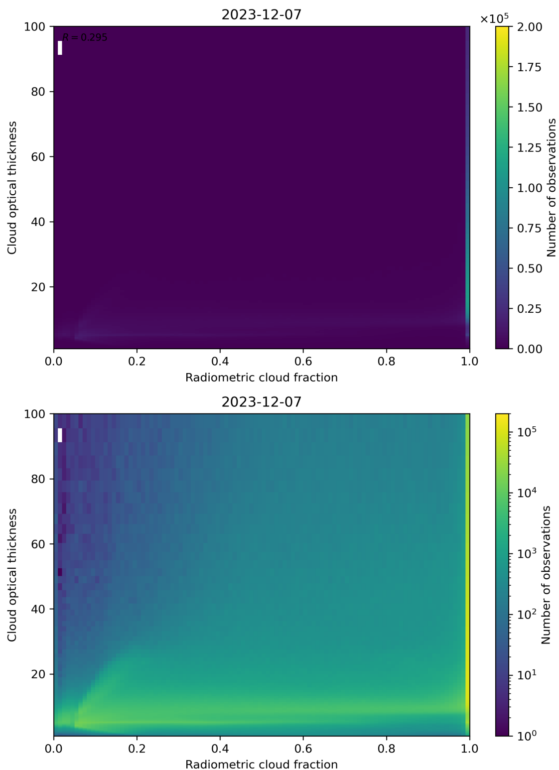
Figure 75: Scatter density plot of “Radiometric cloud fraction” against “Cloud optical thickness” for 2023-12-06 to 2023-12-08.
