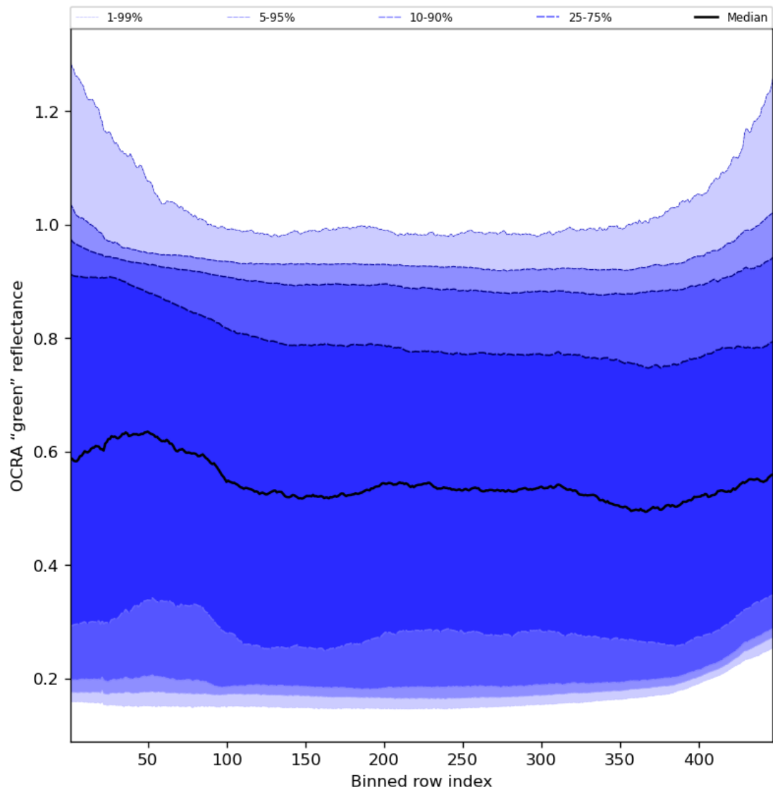
Figure 68: Along track statistics of “OCRA “green” reflectance” for 2023-12-06 to 2023-12-08
