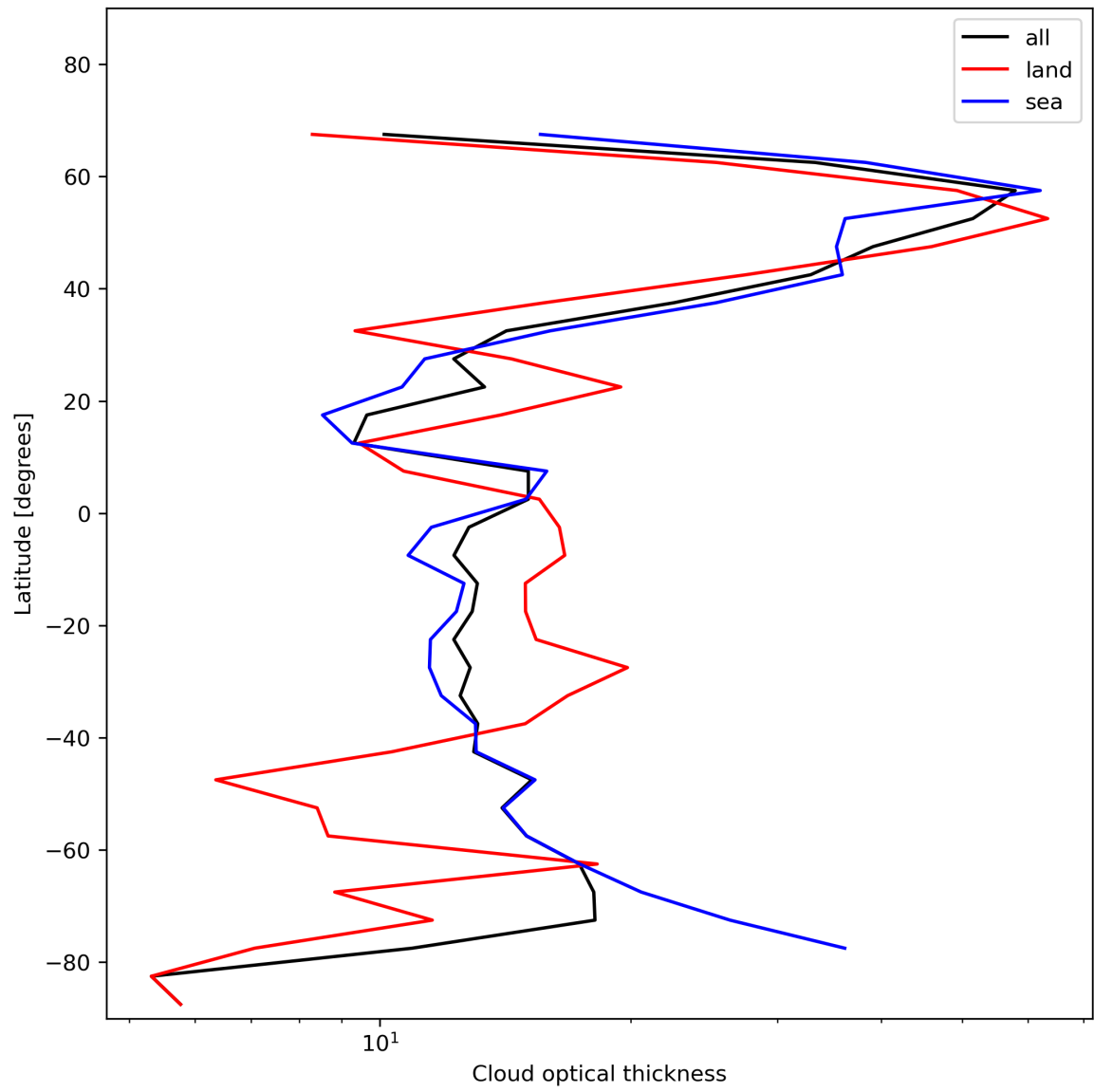
Figure 25: Zonal average of “Cloud optical thickness” for 2023-12-06 to 2023-12-08.
