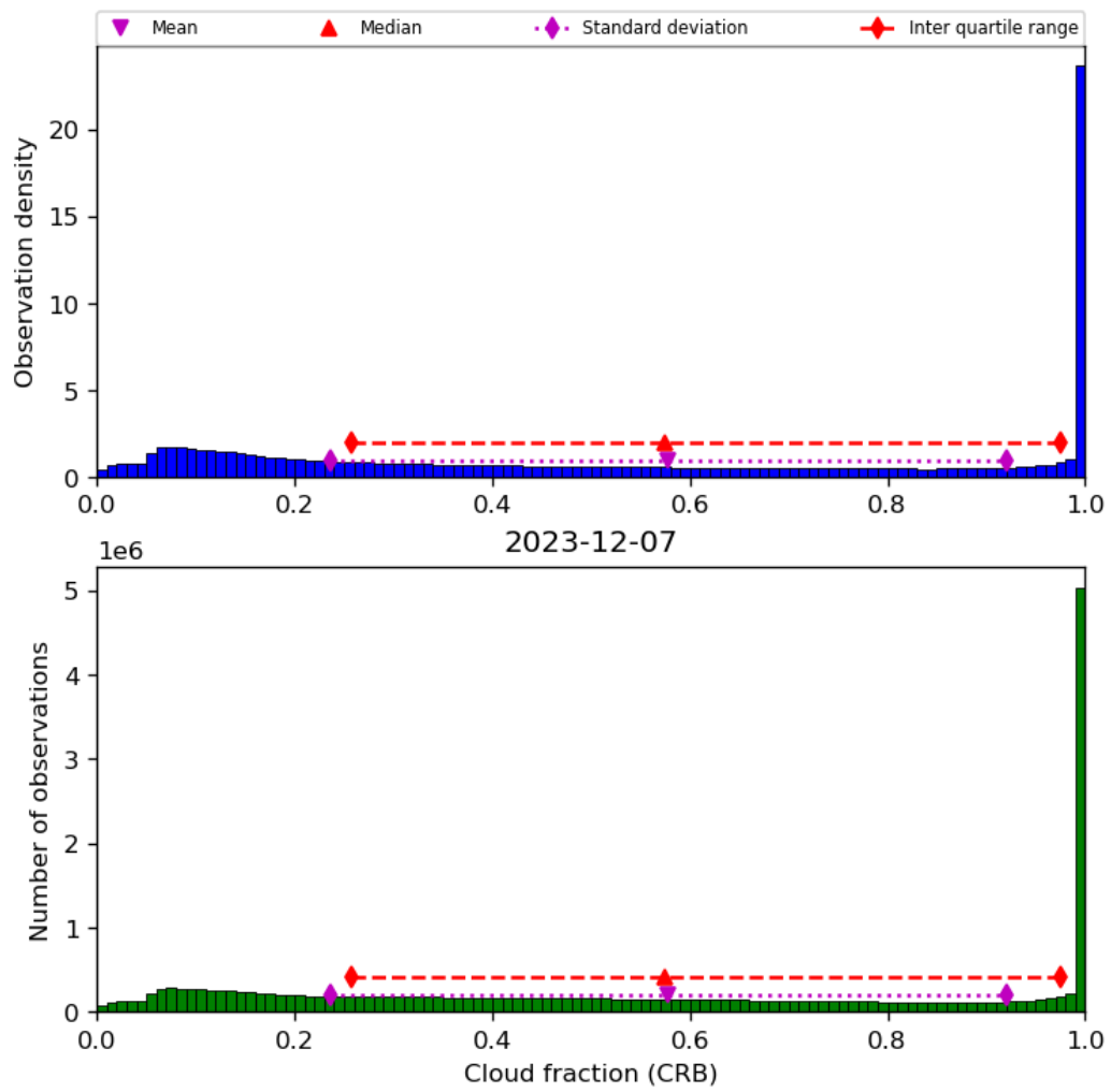
Figure 42: Histogram of “Cloud fraction (CRB)” for 2023-12-06 to 2023-12-08
