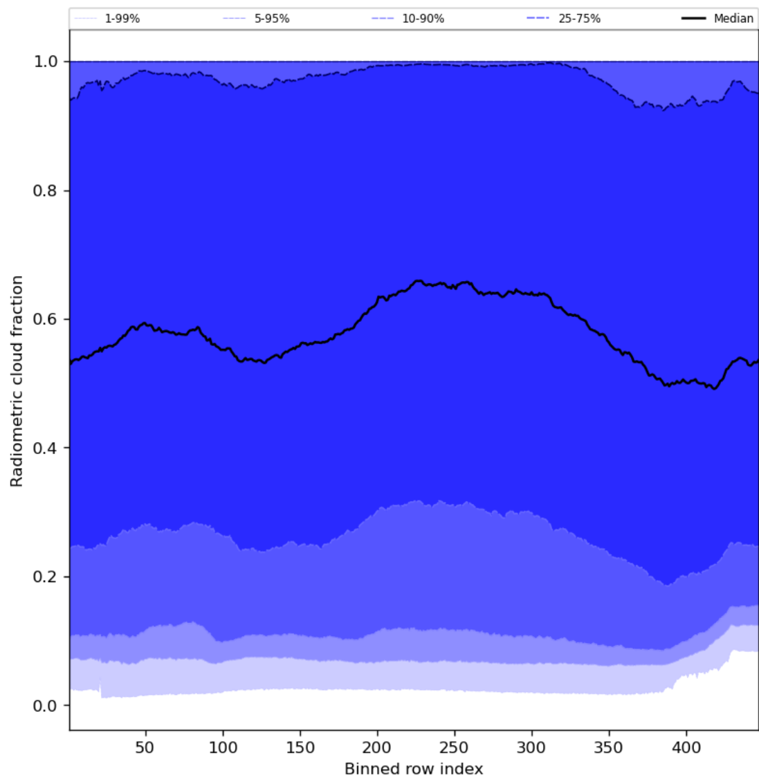
Figure 55: Along track statistics of “Radiometric cloud fraction” for 2023-12-06 to 2023-12-08
