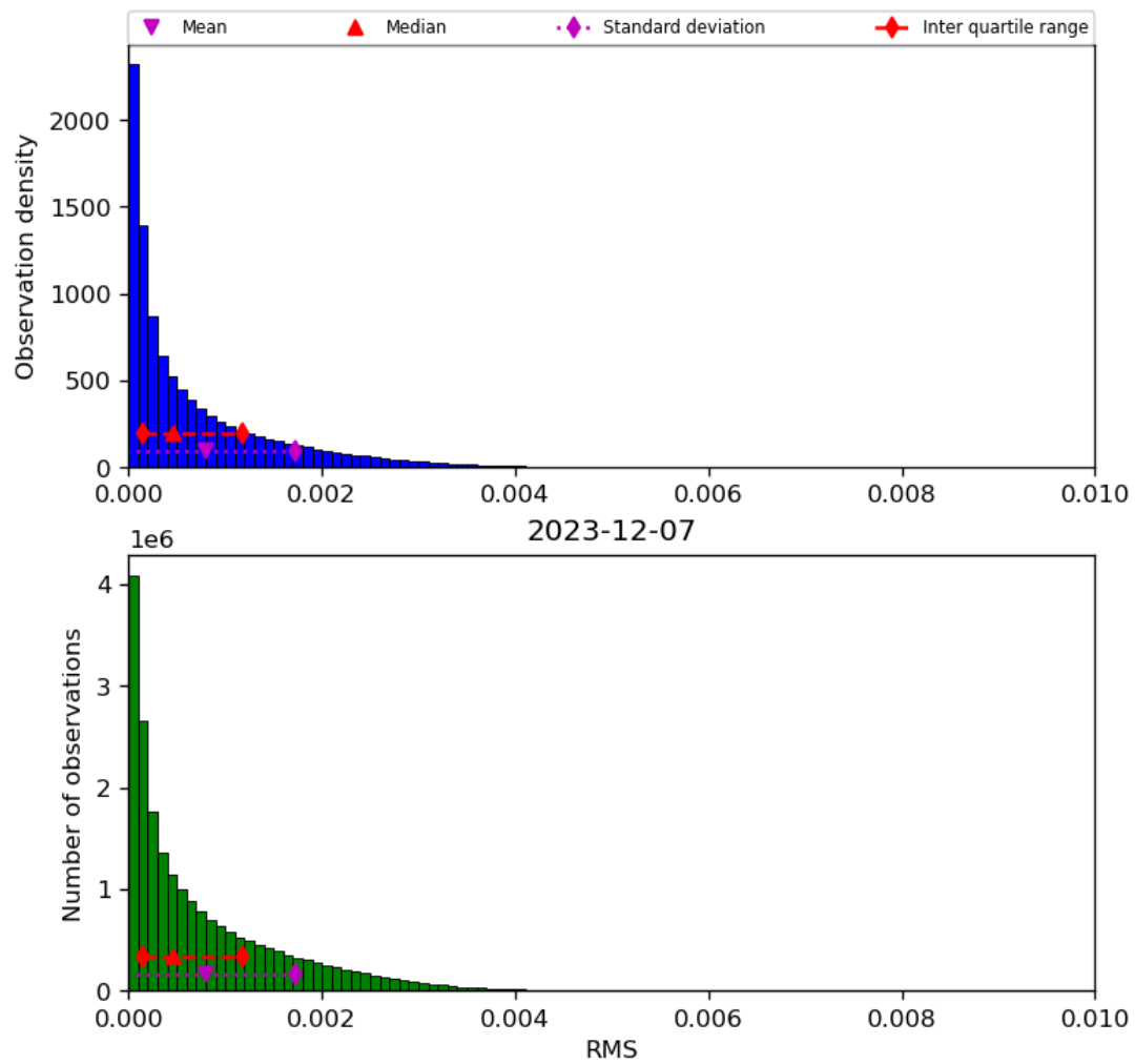
Figure 47: Histogram of “RMS” for 2023-12-06 to 2023-12-08
