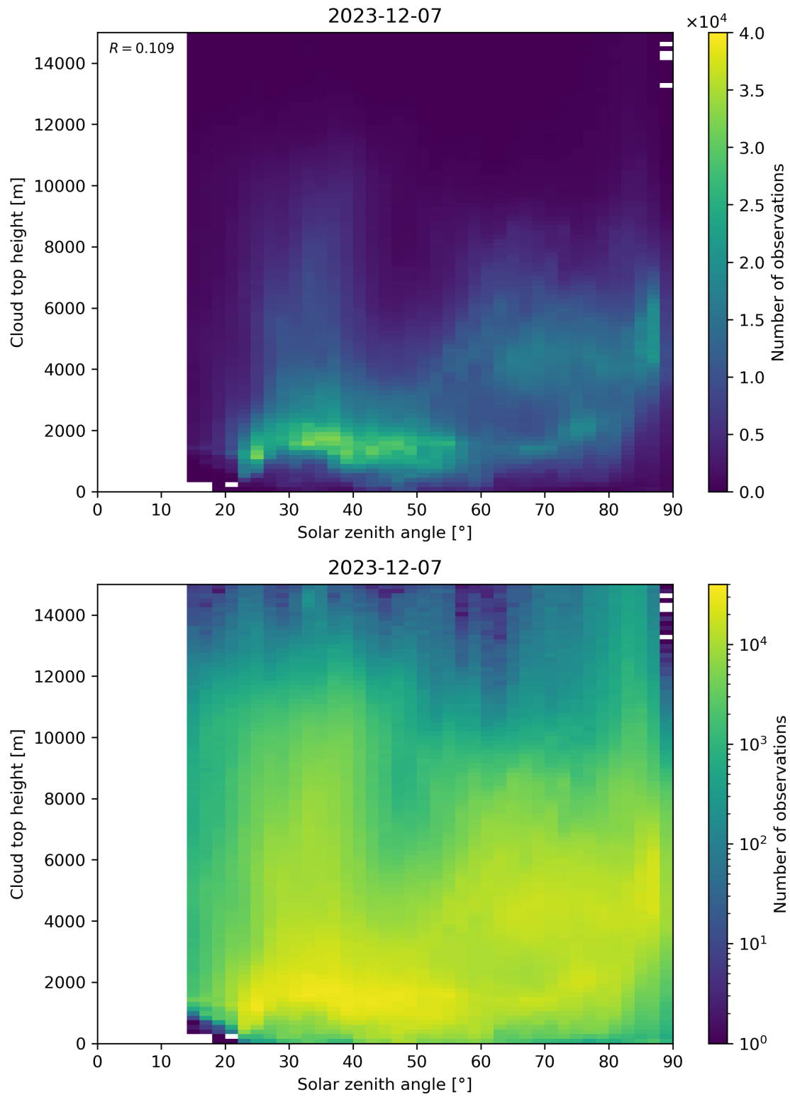
Figure 104: Scatter density plot of “Solar zenith angle” against “Cloud top height” for 2023-12-06 to 2023-12-08.
