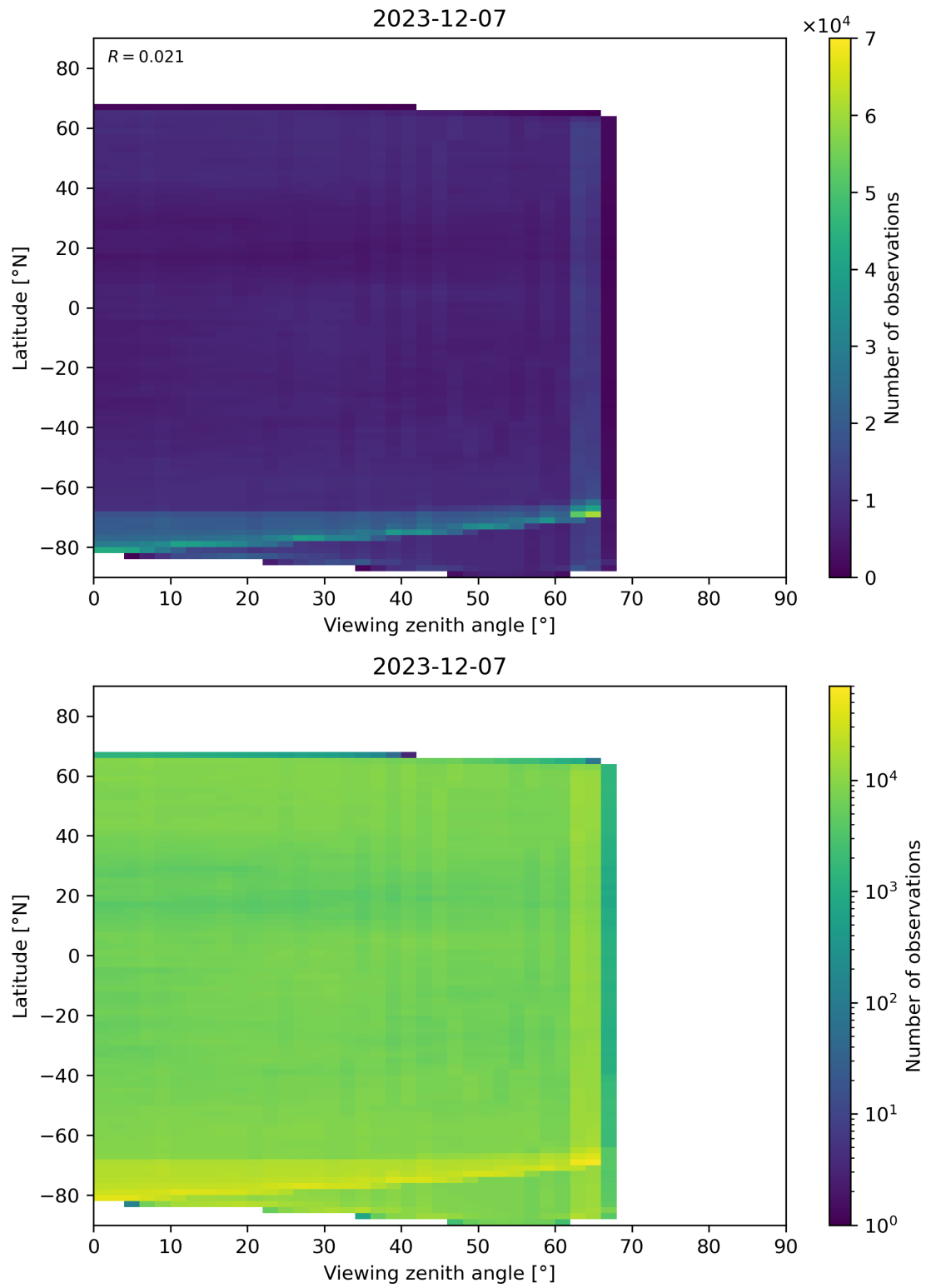
Figure 113: Scatter density plot of “Viewing zenith angle” against “Latitude” for 2023-12-06 to 2023-12-08.
