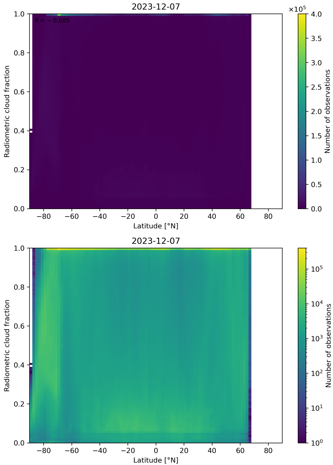
Figure 92: Scatter density plot of “Latitude” against “Radiometric cloud fraction” for 2023-12-06 to 2023-12-08.
