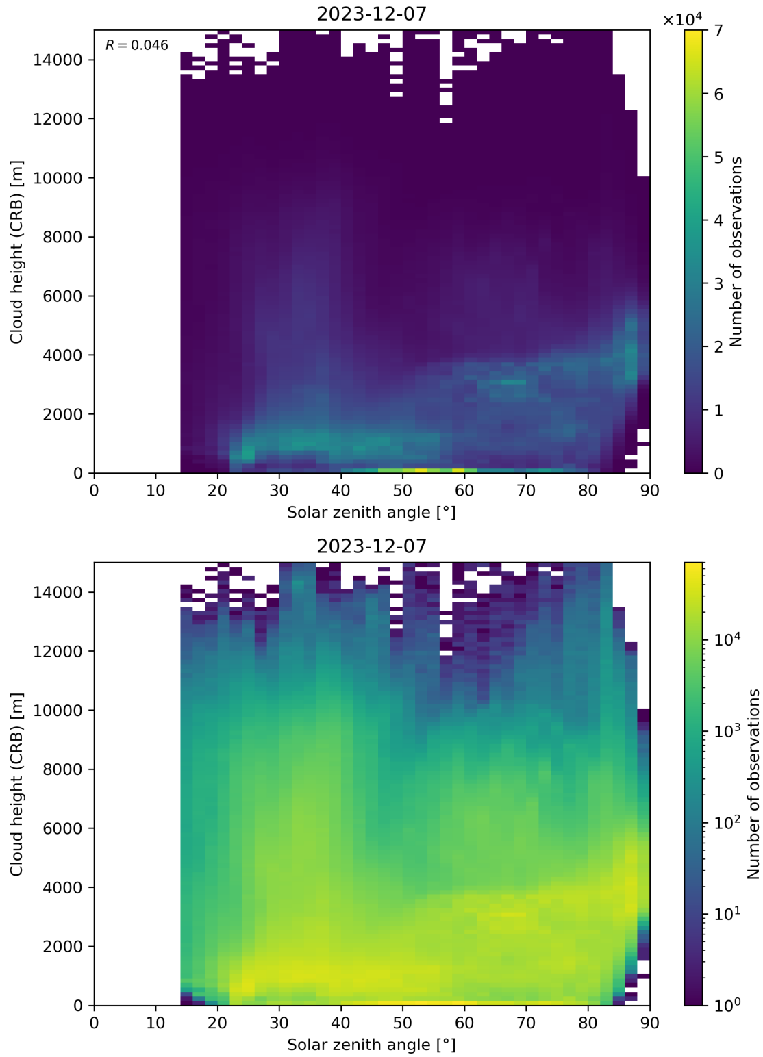
Figure 102: Scatter density plot of “Solar zenith angle” against “Cloud height (CRB)” for 2023-12-06 to 2023-12-08.
