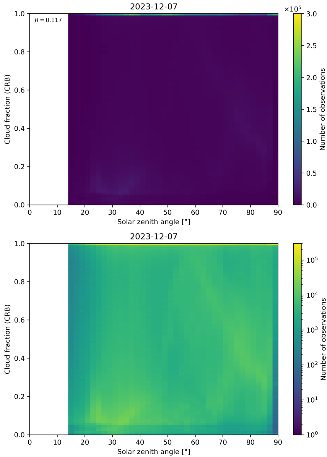
Figure 101: Scatter density plot of “Solar zenith angle” against “Cloud fraction (CRB)” for 2023-12-06 to 2023-12-08.
