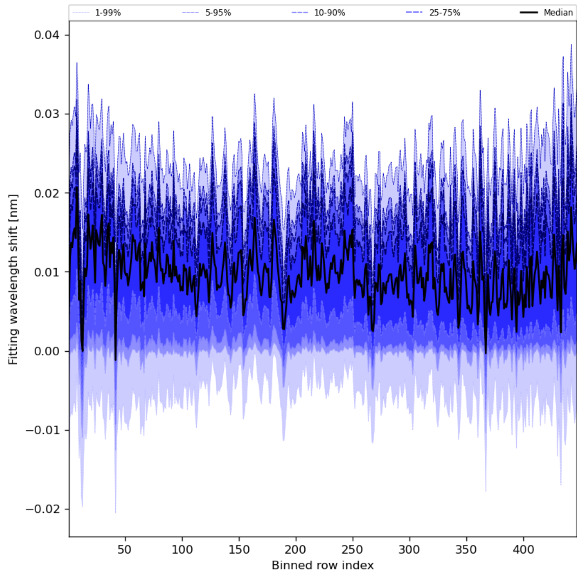
Figure 65: Along track statistics of “Fitting wavelength shift” for 2023-12-06 to 2023-12-08
