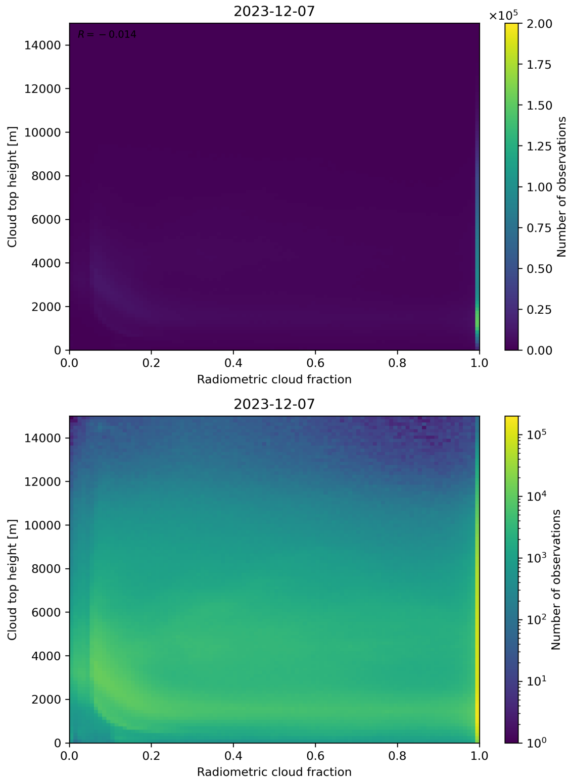
Figure 76: Scatter density plot of “Radiometric cloud fraction” against “Cloud top height” for 2023-12-06 to 2023-12-08.
