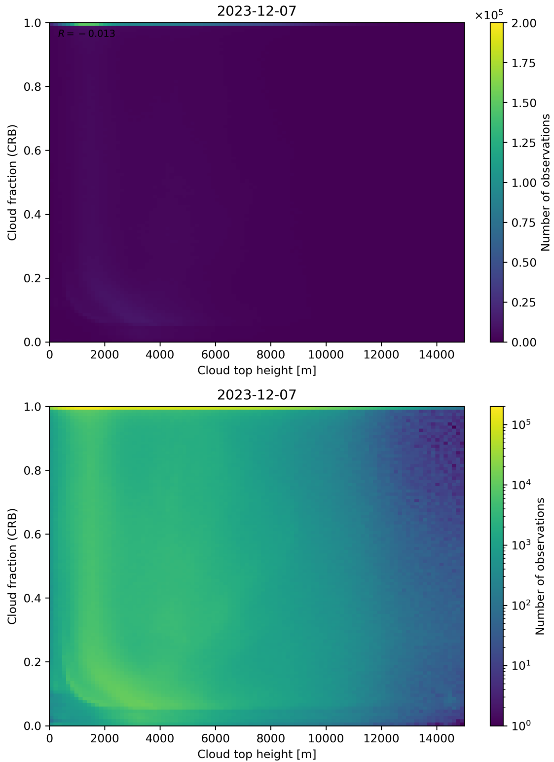
Figure 88: Scatter density plot of “Cloud top height” against “Cloud fraction (CRB)” for 2023-12-06 to 2023-12-08.
