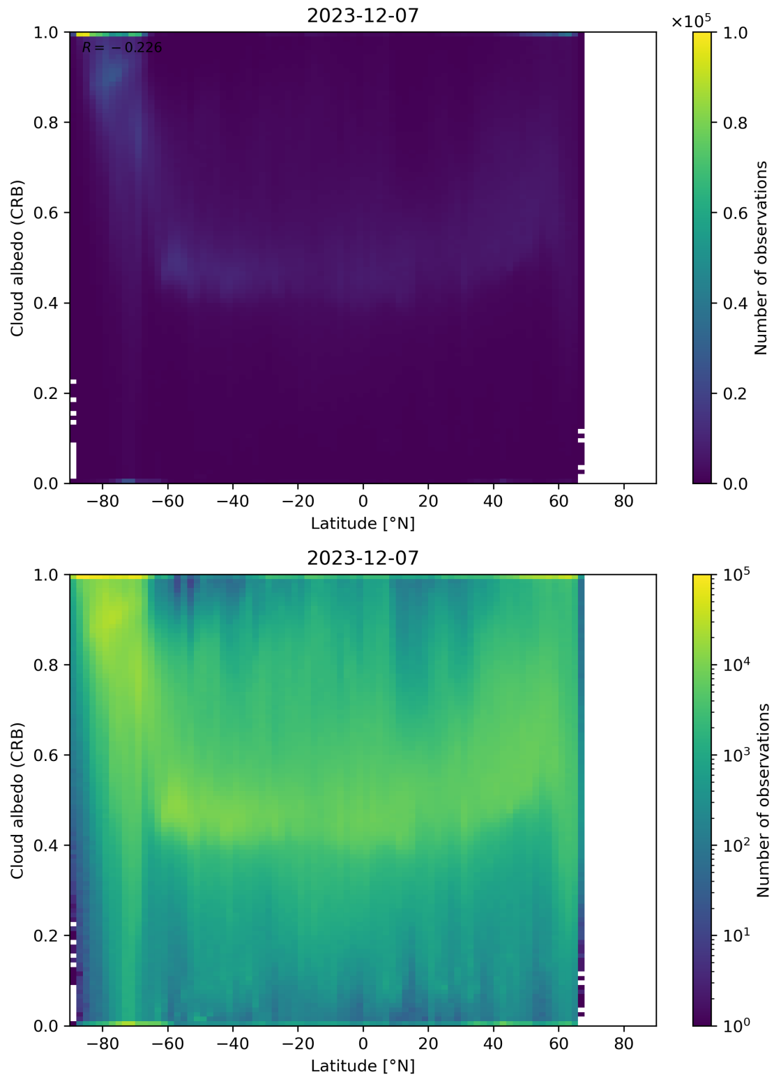
Figure 91: Scatter density plot of “Latitude” against “Cloud albedo (CRB)” for 2023-12-06 to 2023-12-08.
