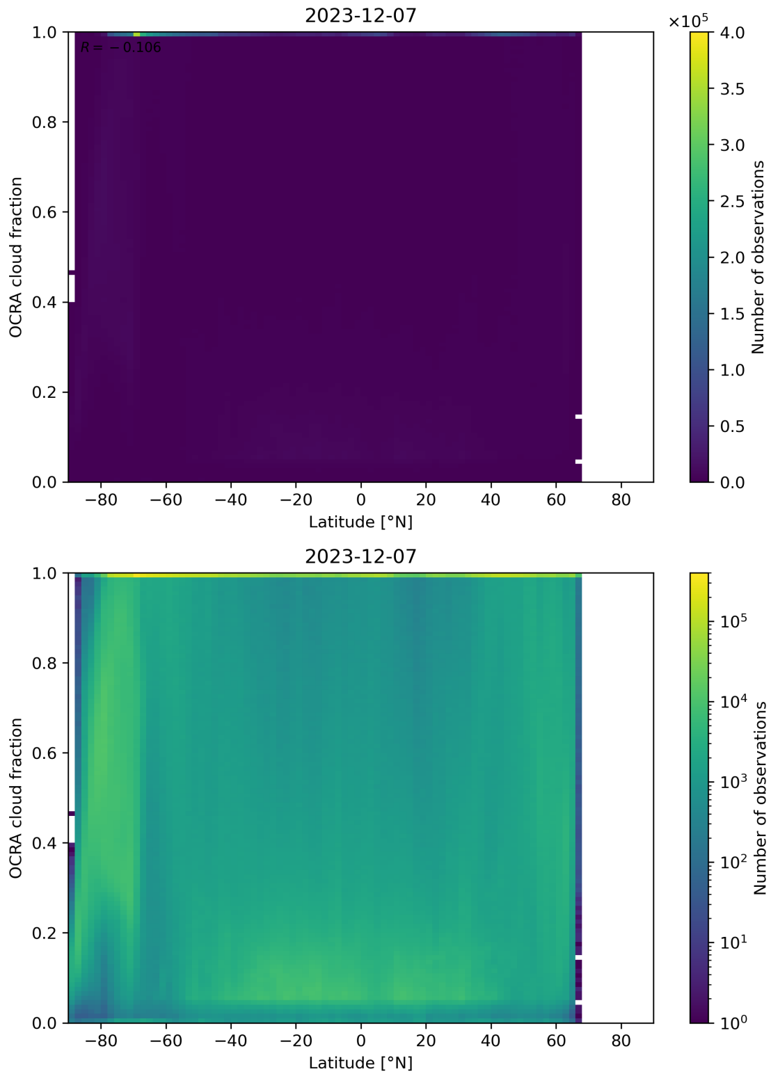
Figure 93: Scatter density plot of “Latitude” against “OCRA cloud fraction” for 2023-12-06 to 2023-12-08.
