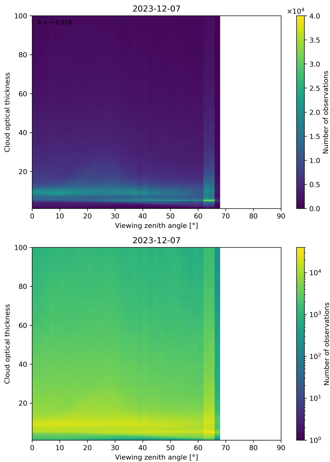
Figure 111: Scatter density plot of “Viewing zenith angle” against “Cloud optical thickness” for 2023-12-06 to 2023-12-08.
