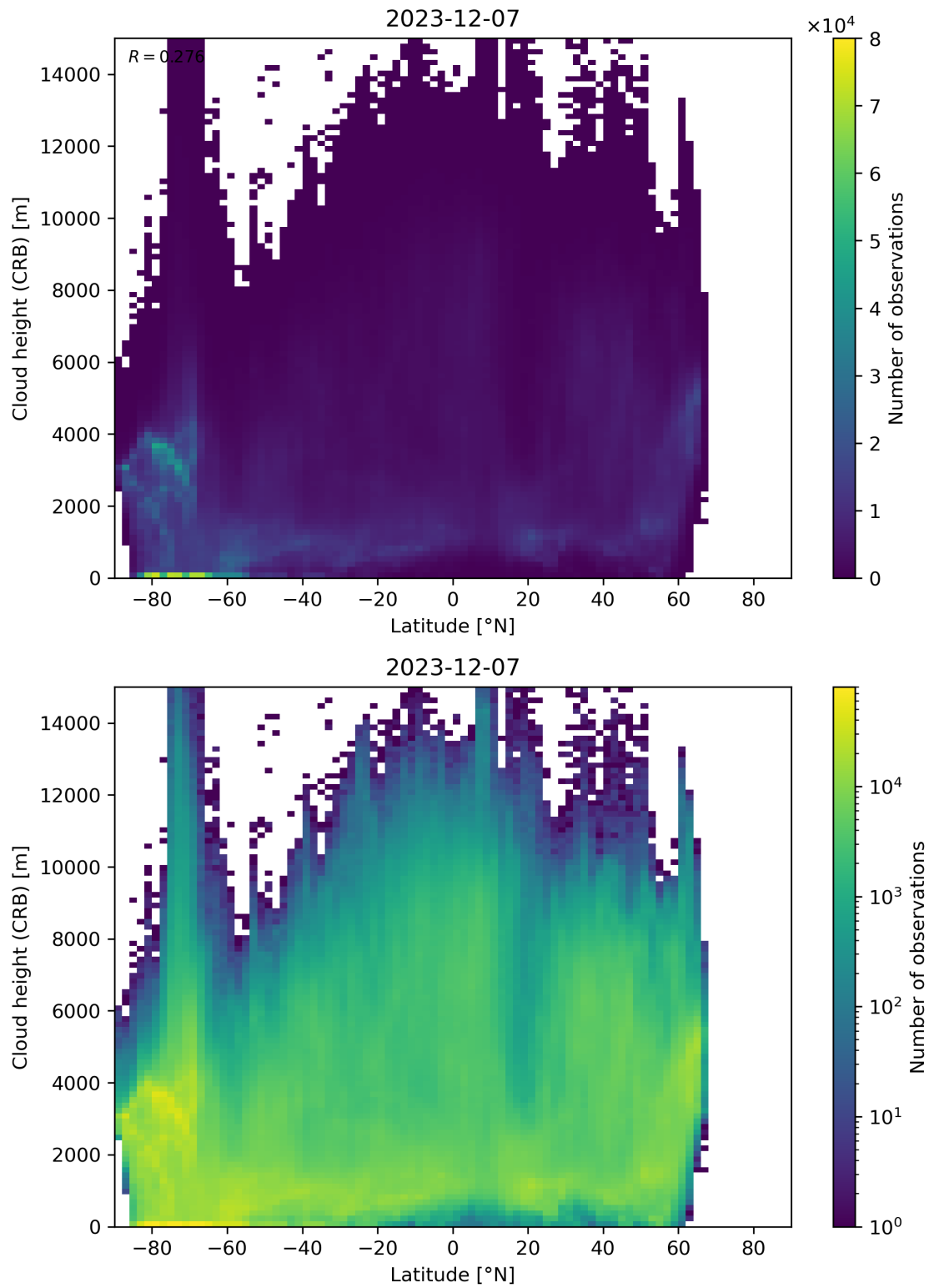
Figure 95: Scatter density plot of “Latitude” against “Cloud height (CRB)” for 2023-12-06 to 2023-12-08.
