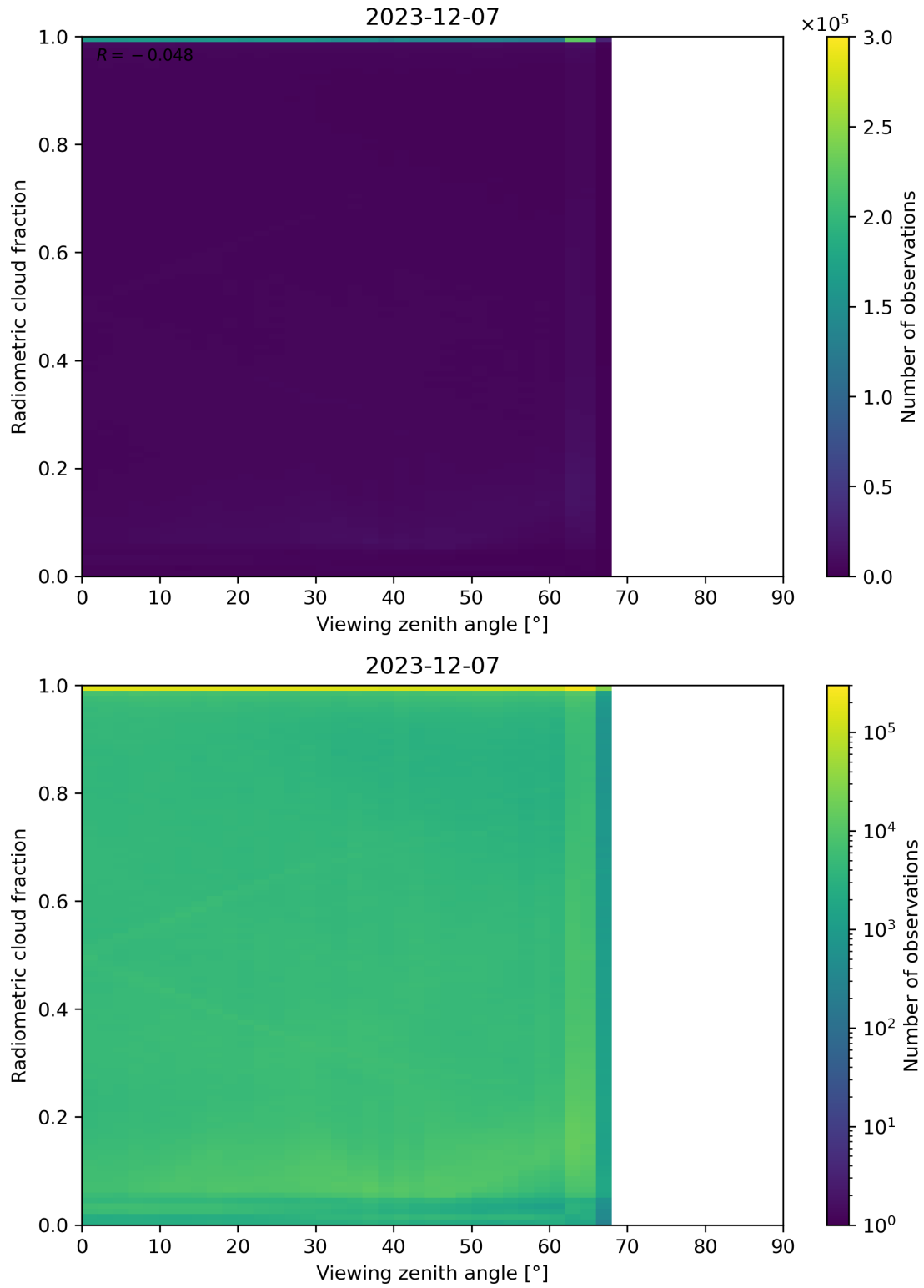
Figure 107: Scatter density plot of “Viewing zenith angle” against “Radiometric cloud fraction” for 2023-12-06 to 2023-12-08.
