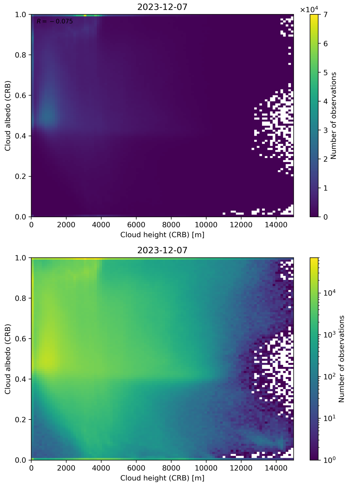
Figure 80: Scatter density plot of “Cloud height (CRB)” against “Cloud albedo (CRB)” for 2023-12-06 to 2023-12-08.
