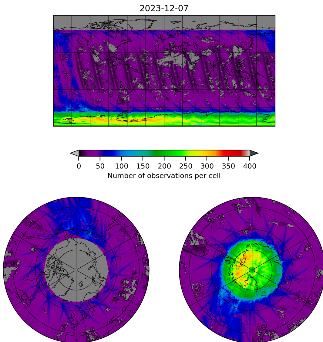
Figure 21: Map of the number of observations for 2023-12-06 to 2023-12-08
