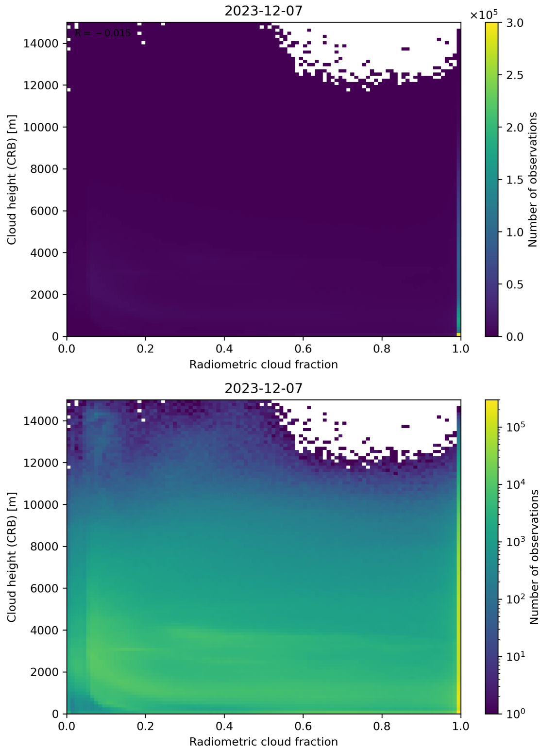
Figure 74: Scatter density plot of “Radiometric cloud fraction” against “Cloud height (CRB)” for 2023-12-06 to 2023-12-08.
