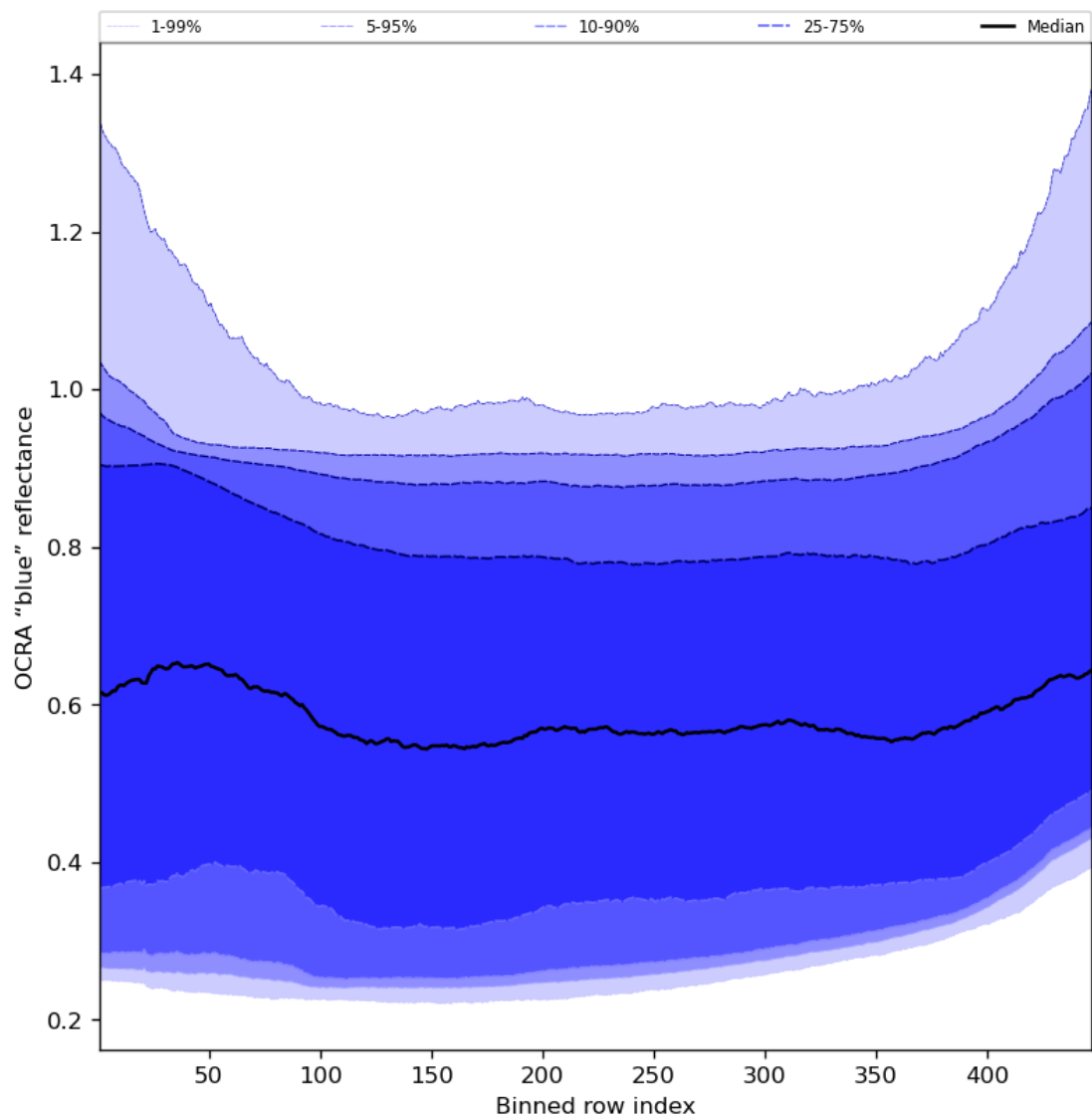
Figure 67: Along track statistics of “OCRA “blue” reflectance” for 2023-12-06 to 2023-12-08
