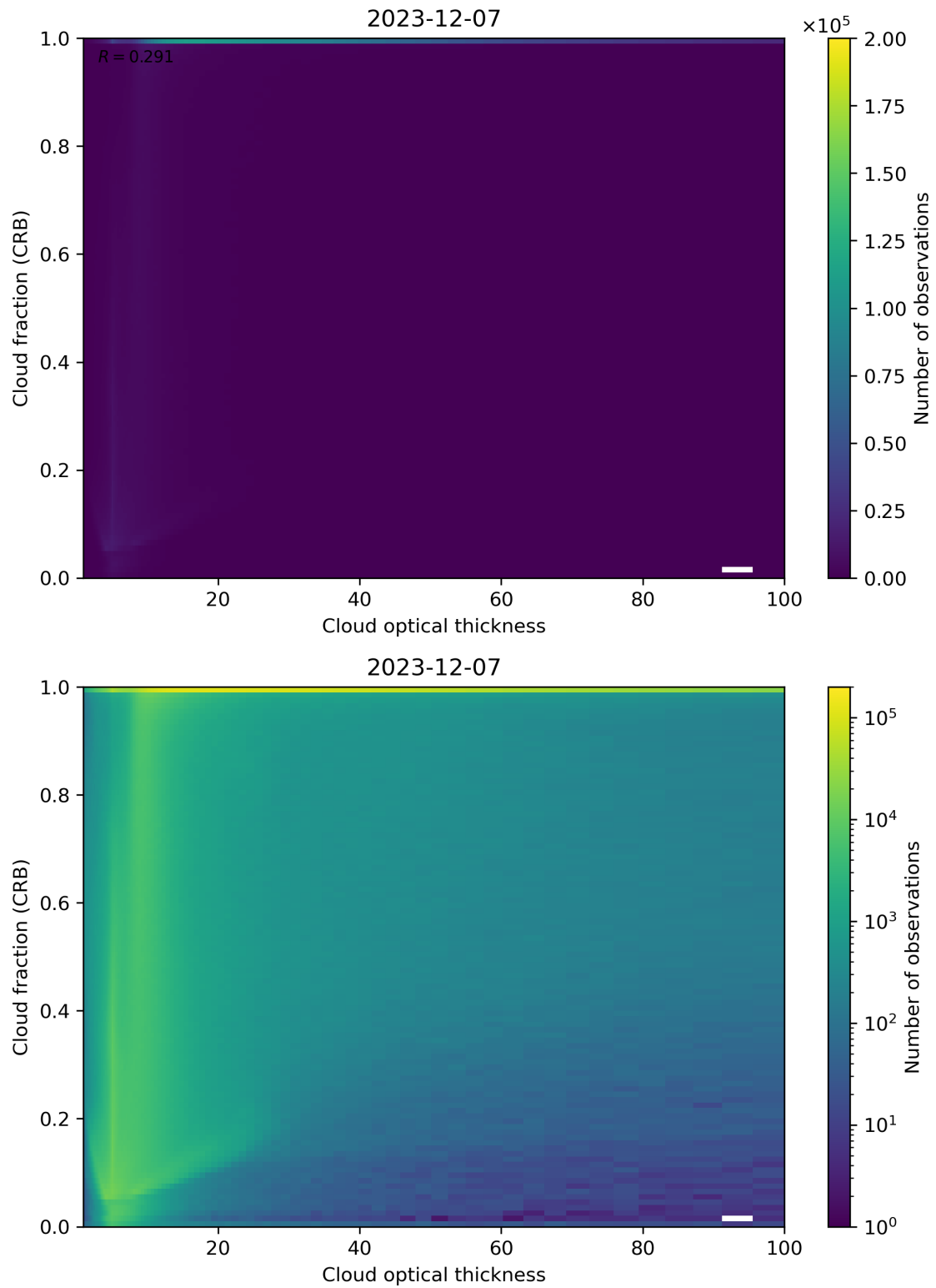
Figure 84: Scatter density plot of “Cloud optical thickness” against “Cloud fraction (CRB)” for 2023-12-06 to 2023-12-08.
