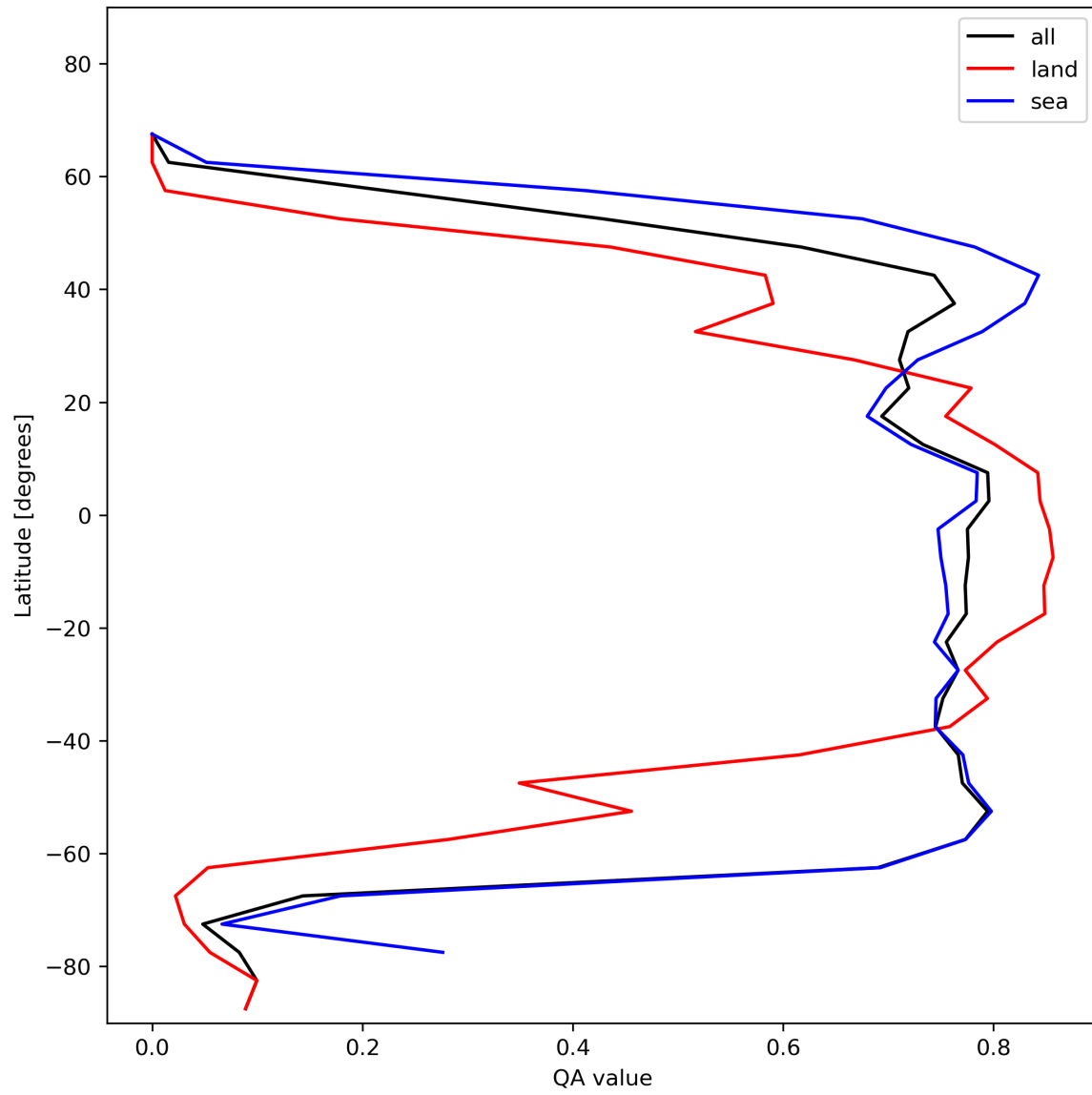
Figure 22: Zonal average of “QA value” for 2023-12-06 to 2023-12-08.
