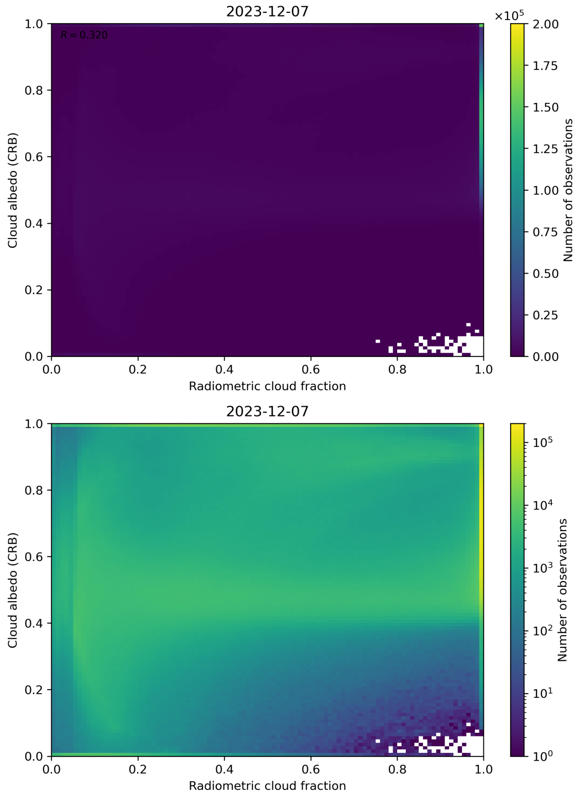
Figure 71: Scatter density plot of “Radiometric cloud fraction” against “Cloud albedo (CRB)” for 2023-12-06 to 2023-12-08.
