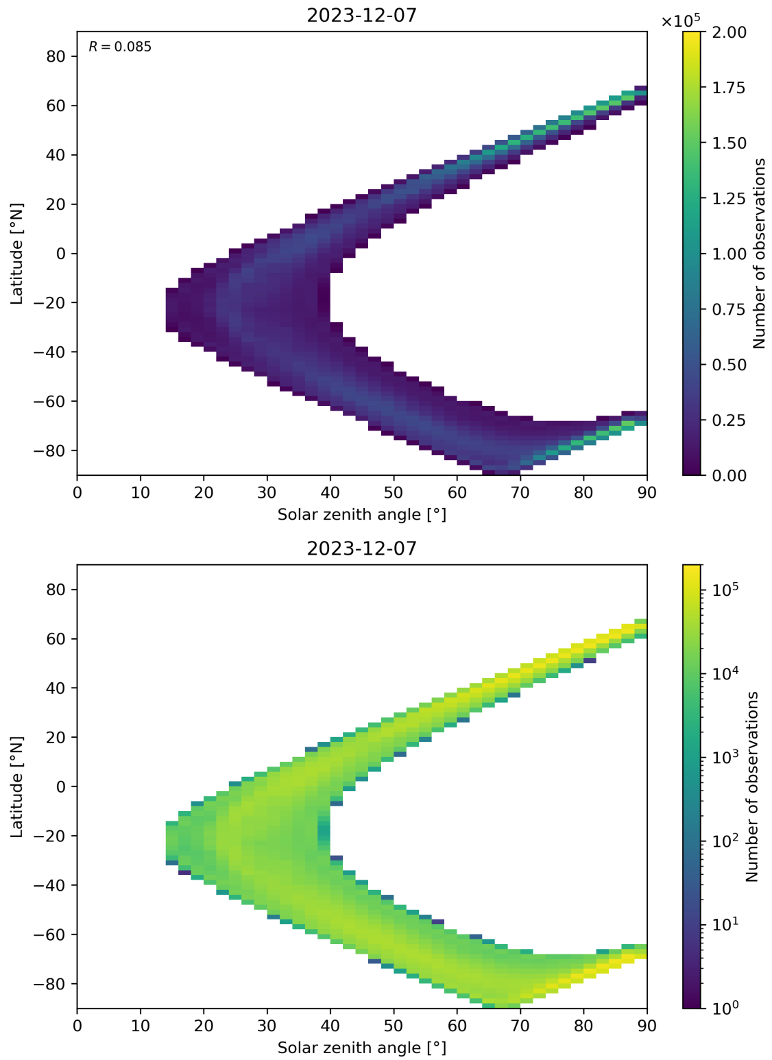
Figure 105: Scatter density plot of “Solar zenith angle” against “Latitude” for 2023-12-06 to 2023-12-08.
