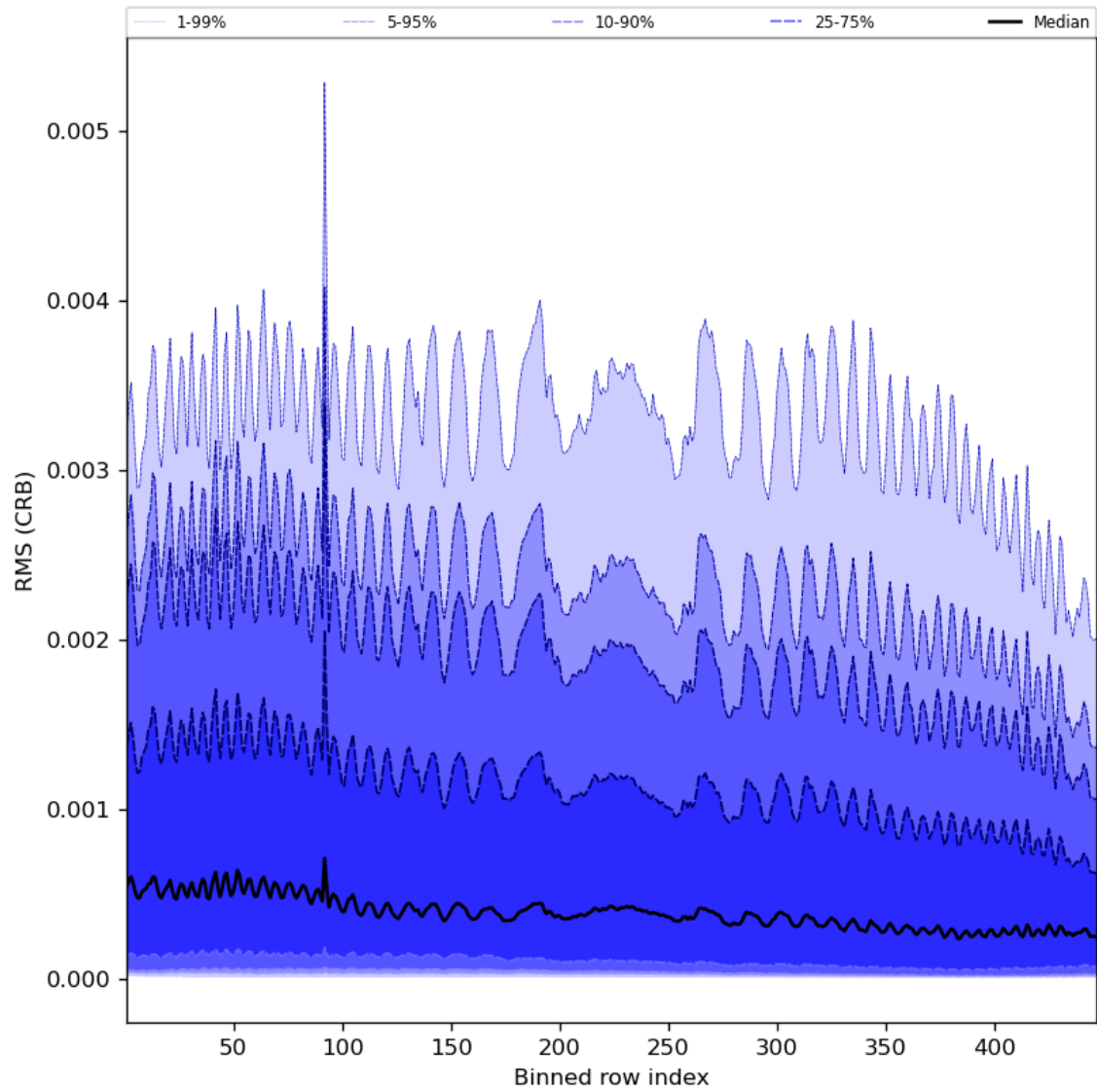
Figure 64: Along track statistics of “RMS (CRB)” for 2023-12-06 to 2023-12-08
