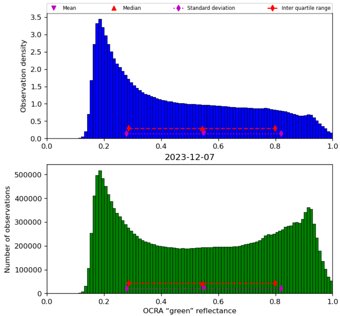
Figure 52: Histogram of “OCRA “green” reflectance” for 2023-12-06 to 2023-12-08
