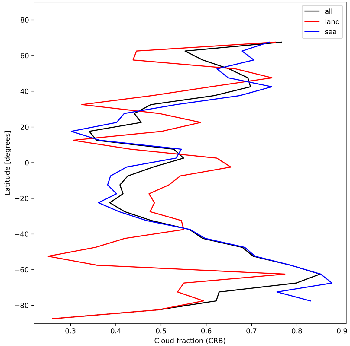
Figure 26: Zonal average of “Cloud fraction (CRB)” for 2023-12-06 to 2023-12-08.
