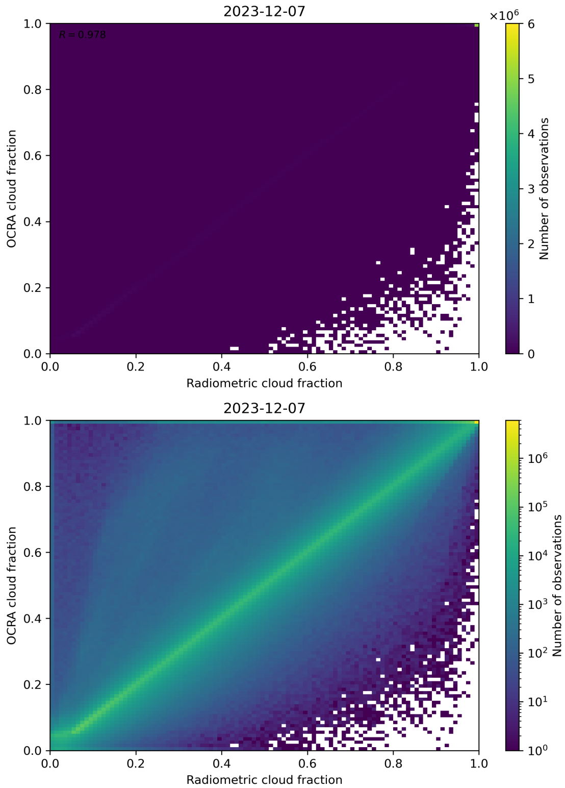
Figure 72: Scatter density plot of “Radiometric cloud fraction” against “OCRA cloud fraction” for 2023-12-06 to 2023-12-08.
