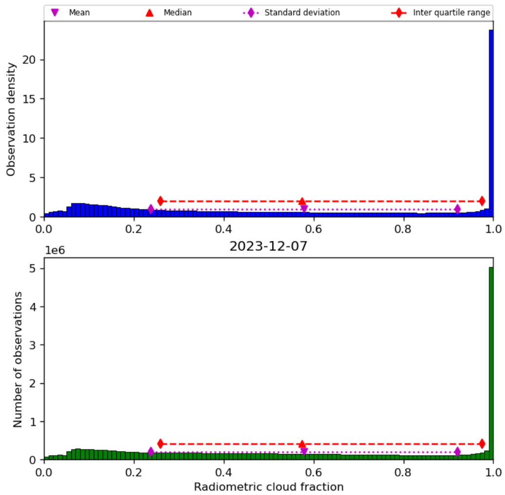
Figure 39: Histogram of “Radiometric cloud fraction” for 2023-12-06 to 2023-12-08
