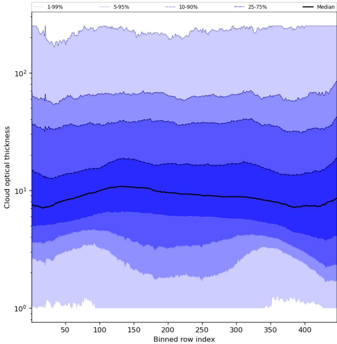
Figure 57: Along track statistics of “Cloud optical thickness” for 2023-12-06 to 2023-12-08
