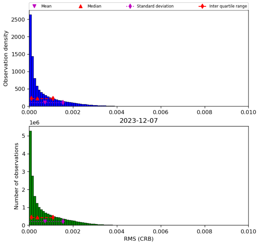
Figure 48: Histogram of “RMS (CRB)” for 2023-12-06 to 2023-12-08
