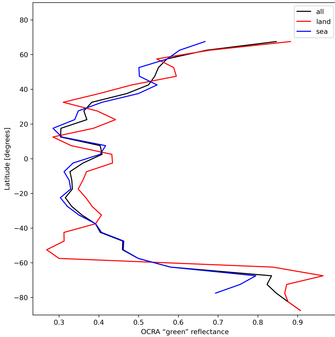
Figure 36: Zonal average of “OCRA “green” reflectance” for 2023-12-06 to 2023-12-08.
