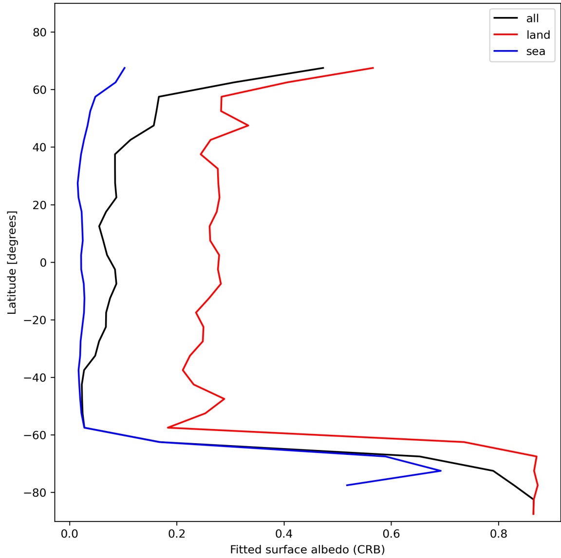
Figure 30: Zonal average of “Fitted surface albedo (CRB)” for 2023-12-06 to 2023-12-08.
