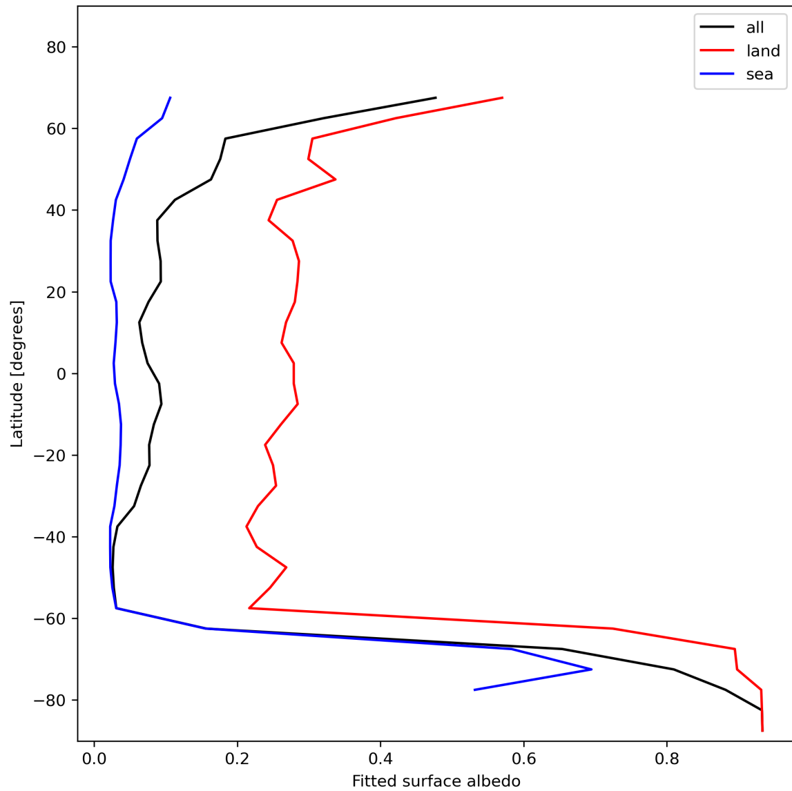
Figure 29: Zonal average of “Fitted surface albedo” for 2023-12-06 to 2023-12-08.
