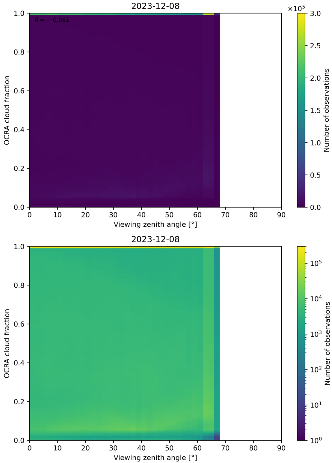
Figure 108: Scatter density plot of “Viewing zenith angle” against “OCRA cloud fraction” for 2023-12-07 to 2023-12-09.
