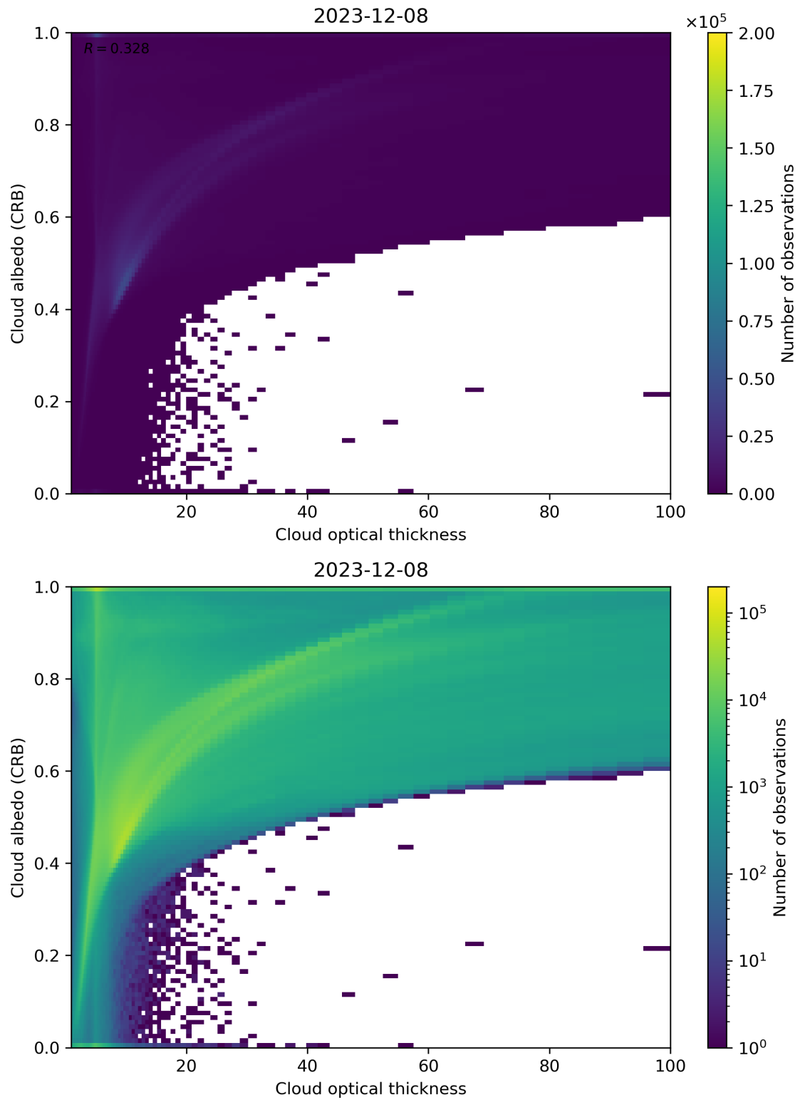
Figure 82: Scatter density plot of “Cloud optical thickness” against “Cloud albedo (CRB)” for 2023-12-07 to 2023-12-09.
