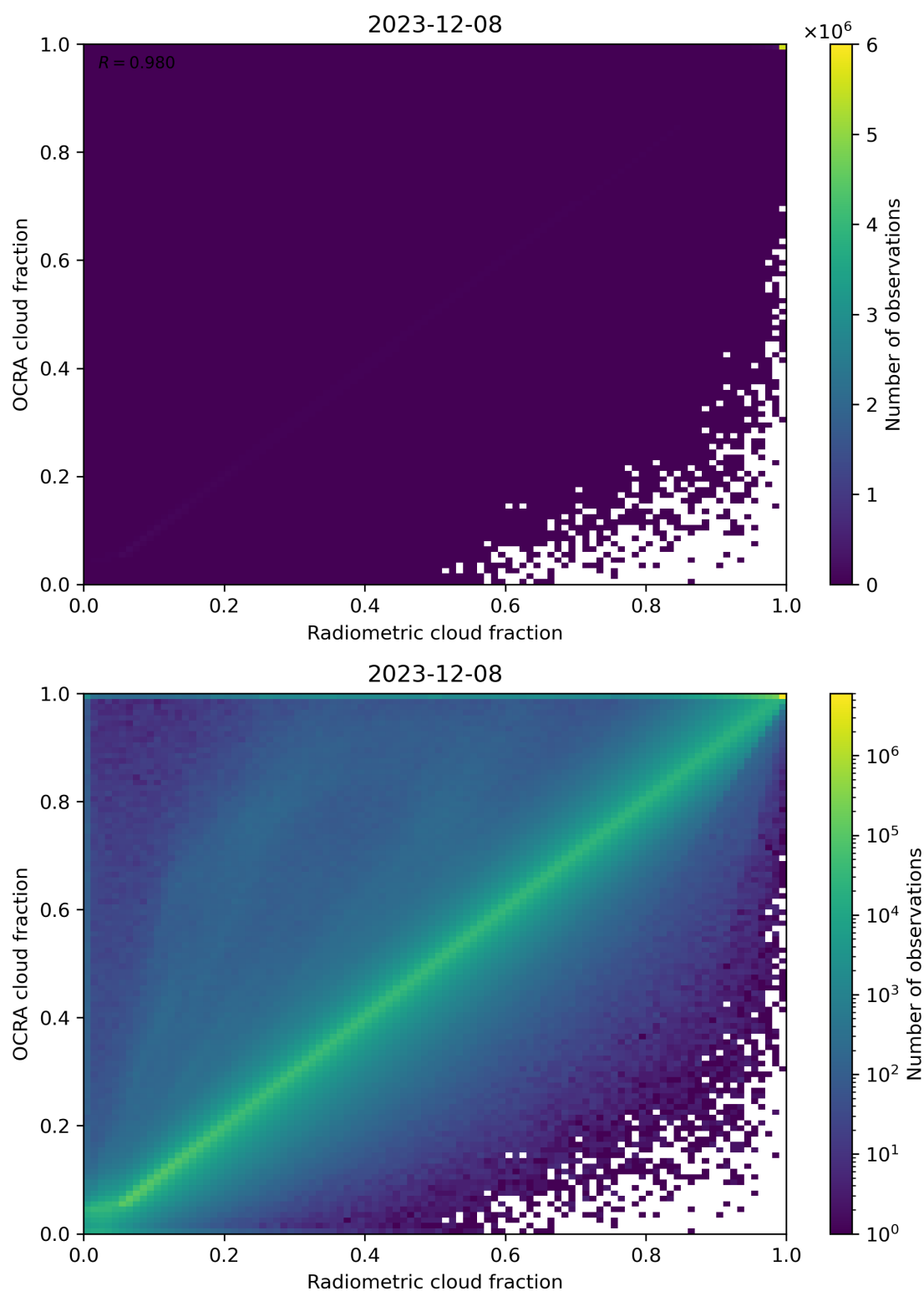
Figure 72: Scatter density plot of “Radiometric cloud fraction” against “OCRA cloud fraction” for 2023-12-07 to 2023-12-09.
