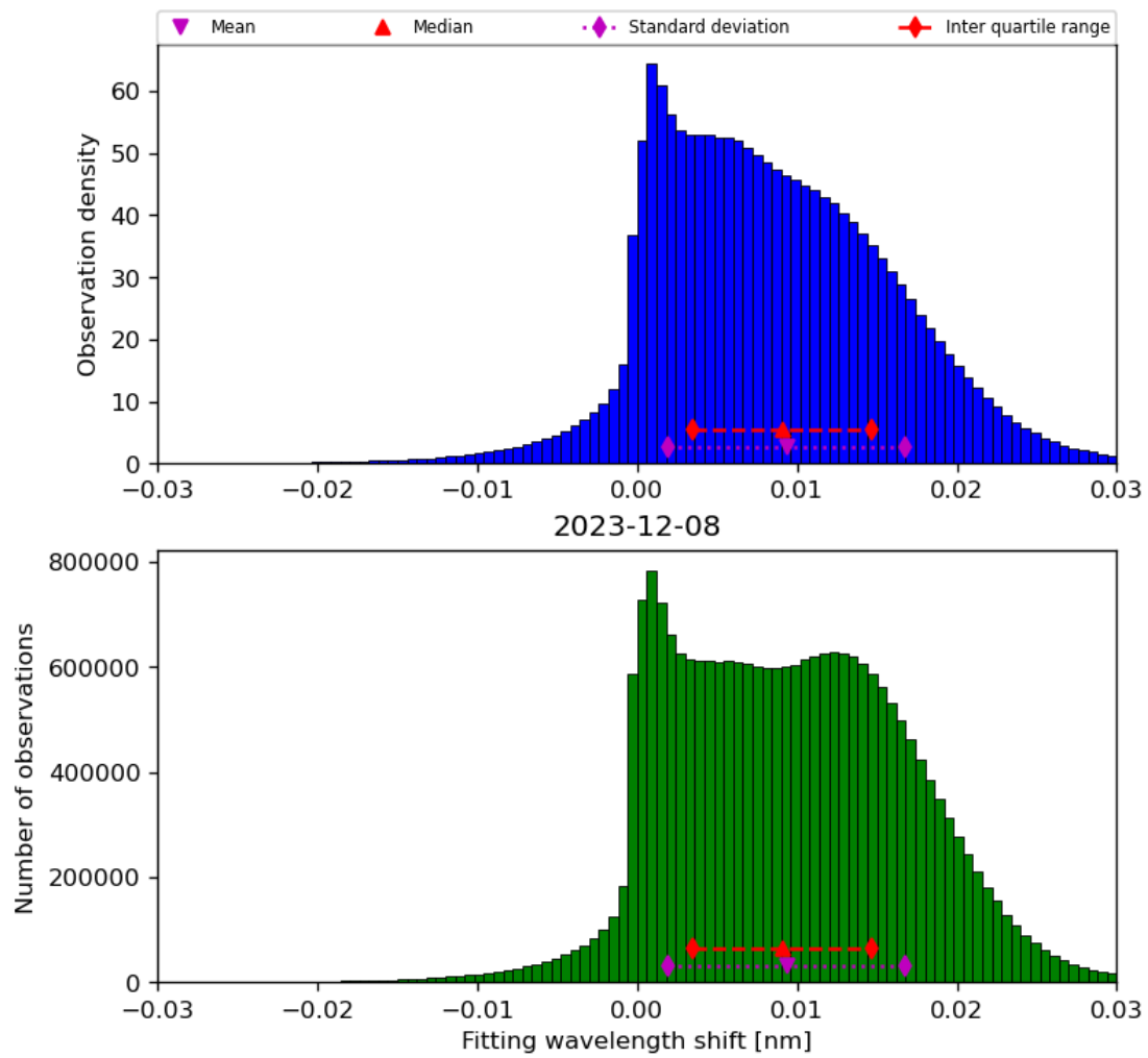
Figure 49: Histogram of “Fitting wavelength shift” for 2023-12-07 to 2023-12-09
