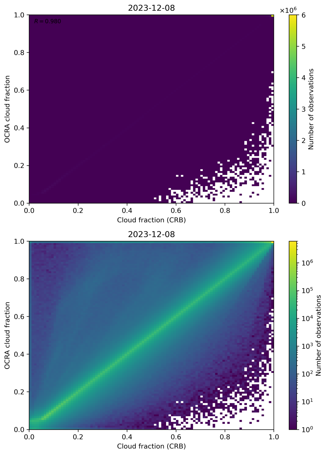
Figure 78: Scatter density plot of “Cloud fraction (CRB)” against “OCRA cloud fraction” for 2023-12-07 to 2023-12-09.
