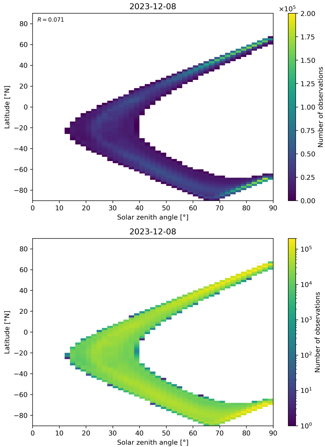
Figure 105: Scatter density plot of “Solar zenith angle” against “Latitude” for 2023-12-07 to 2023-12-09.
