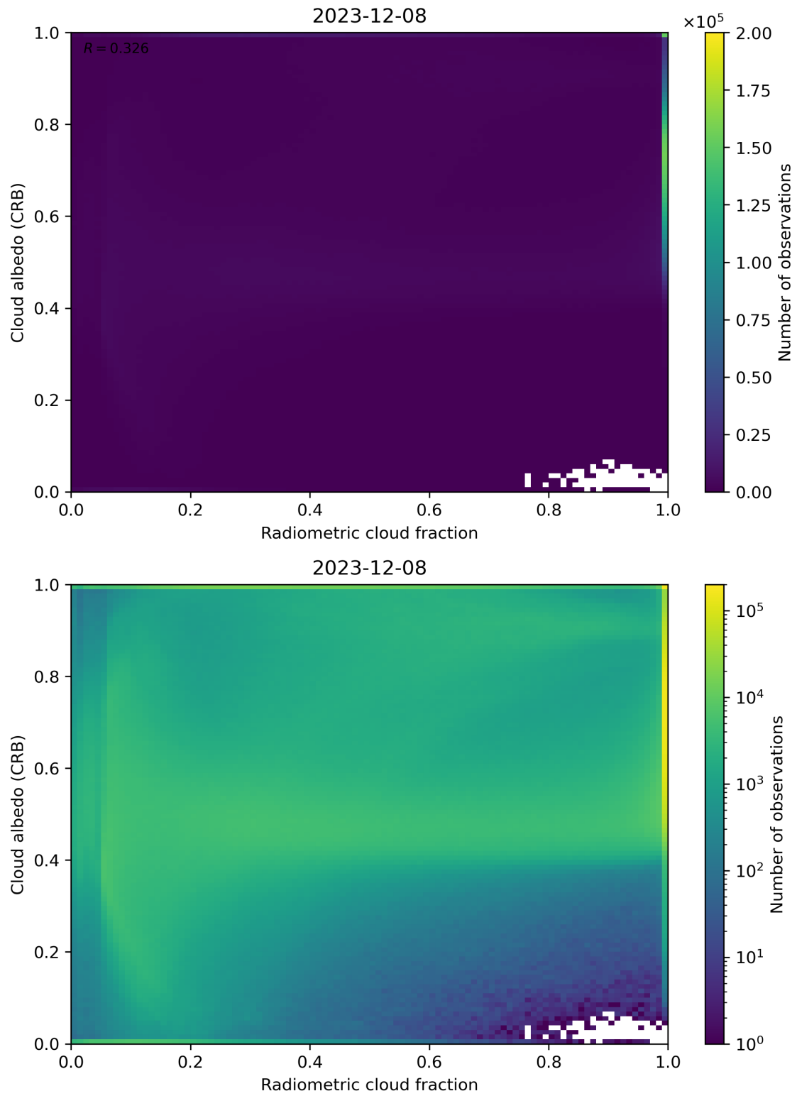
Figure 71: Scatter density plot of “Radiometric cloud fraction” against “Cloud albedo (CRB)” for 2023-12-07 to 2023-12-09.
