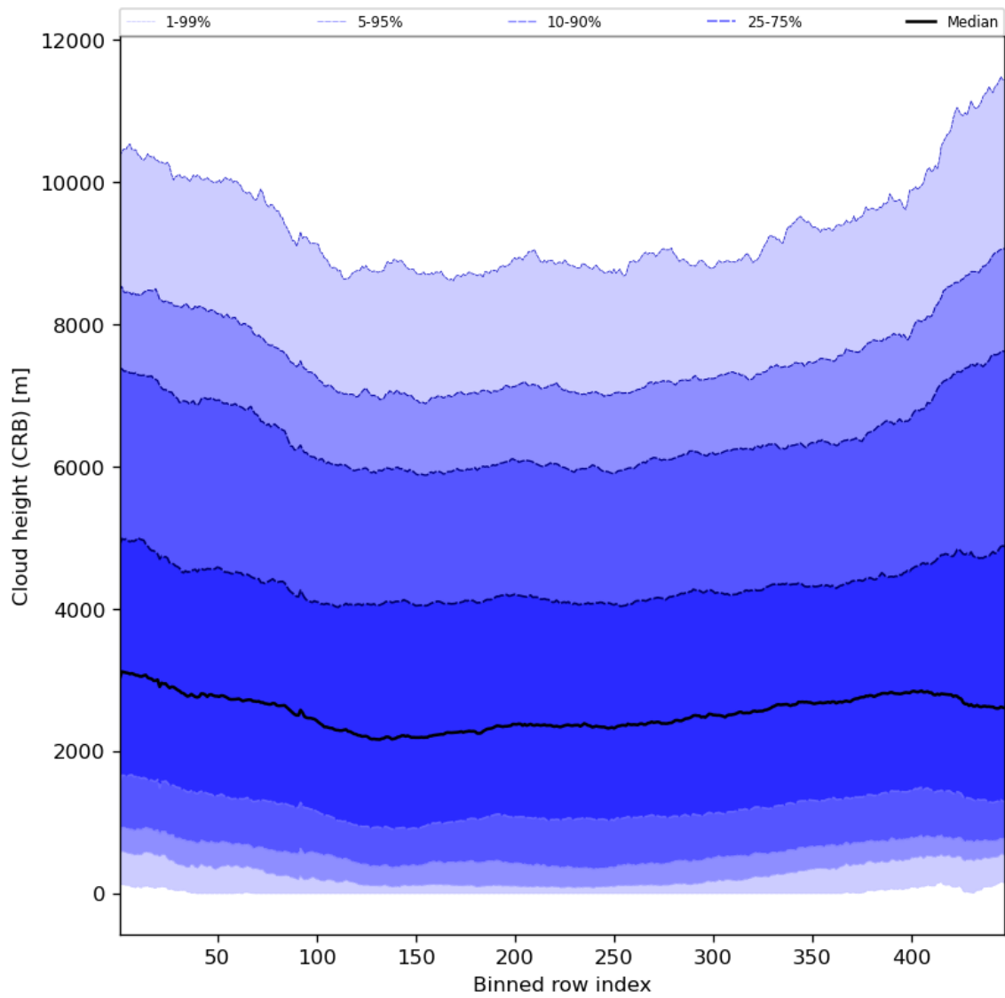
Figure 59: Along track statistics of “Cloud height (CRB)” for 2023-12-07 to 2023-12-09
