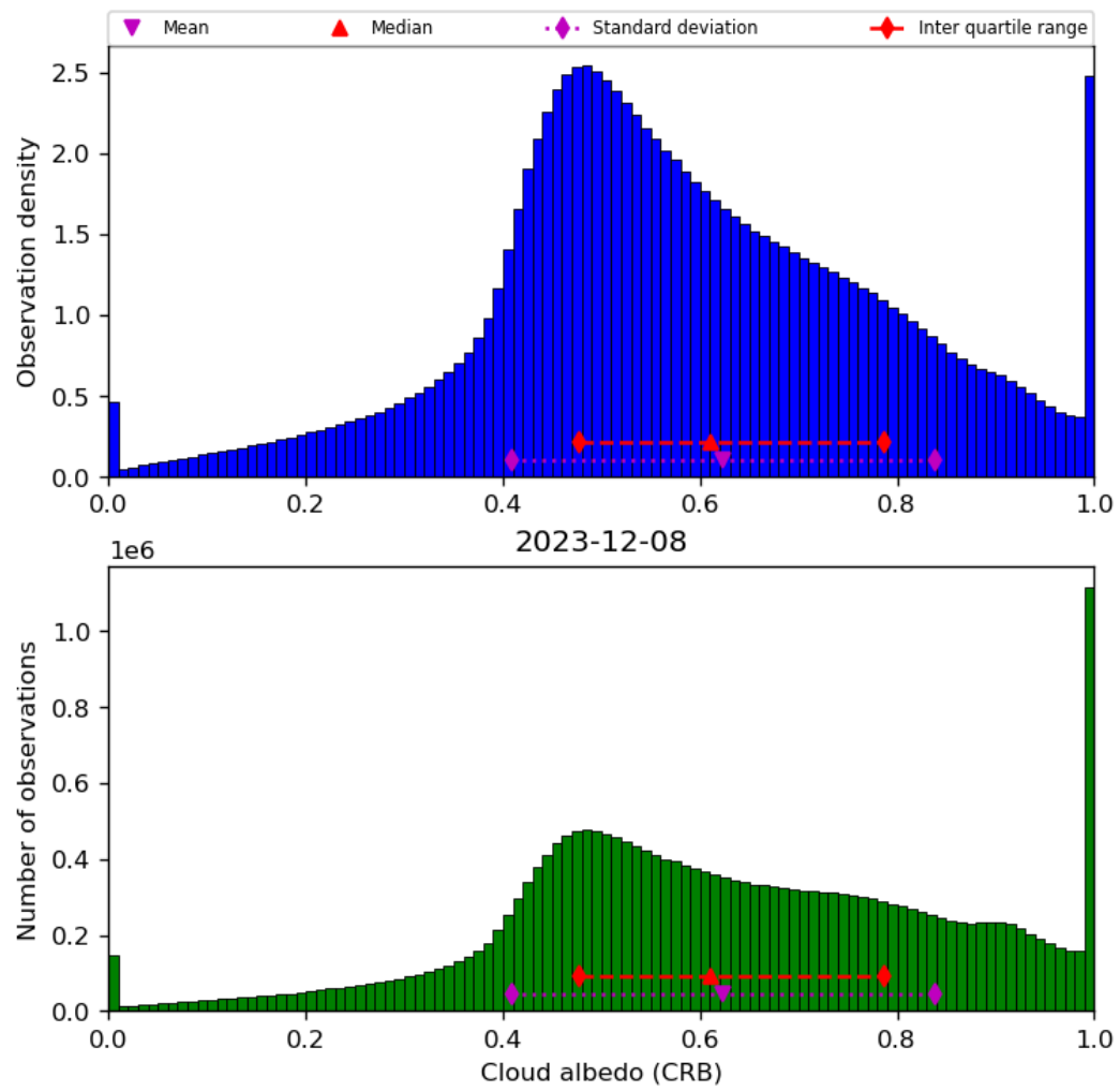
Figure 44: Histogram of “Cloud albedo (CRB)” for 2023-12-07 to 2023-12-09
