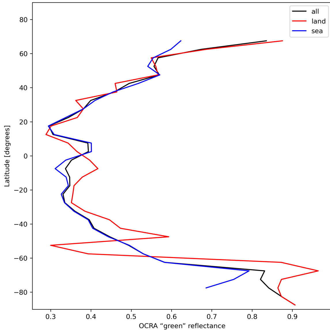
Figure 36: Zonal average of “OCRA “green” reflectance” for 2023-12-07 to 2023-12-09.
