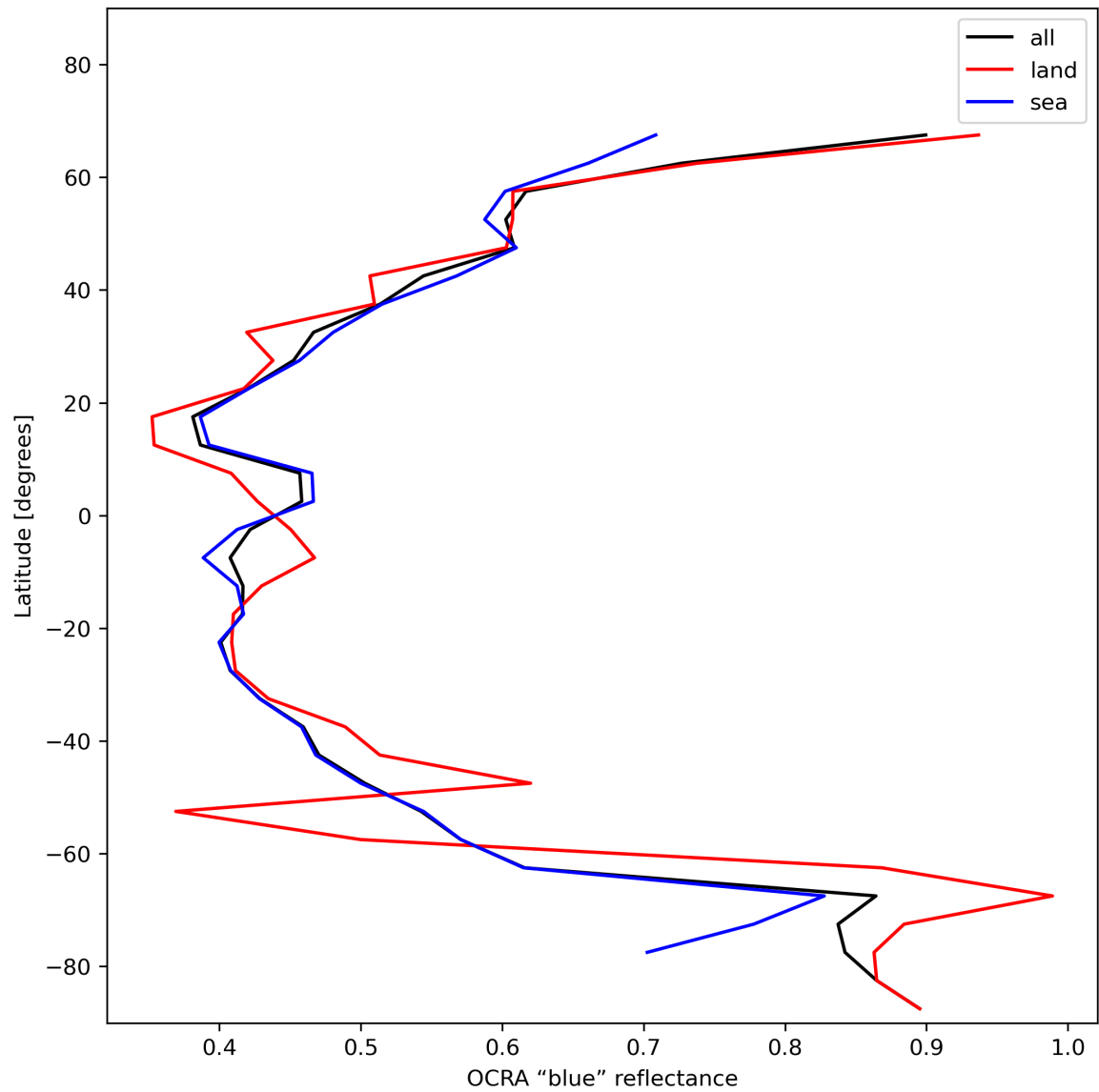
Figure 35: Zonal average of “OCRA “blue” reflectance” for 2023-12-07 to 2023-12-09.
