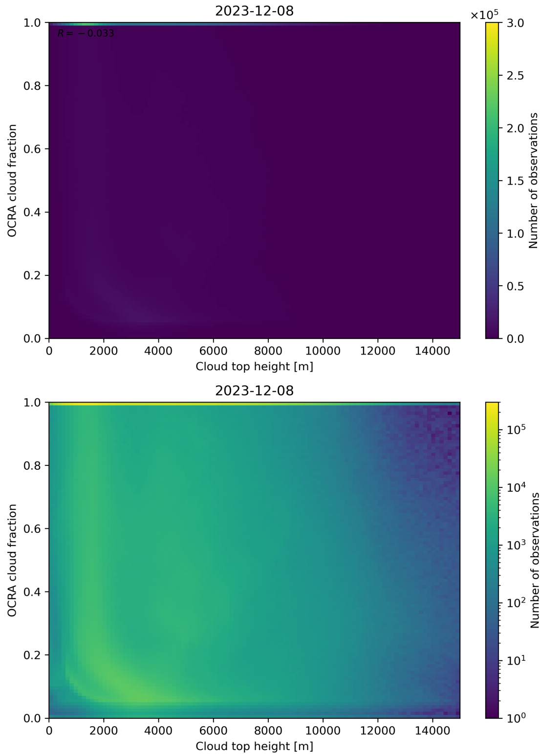
Figure 87: Scatter density plot of “Cloud top height” against “OCRA cloud fraction” for 2023-12-07 to 2023-12-09.
