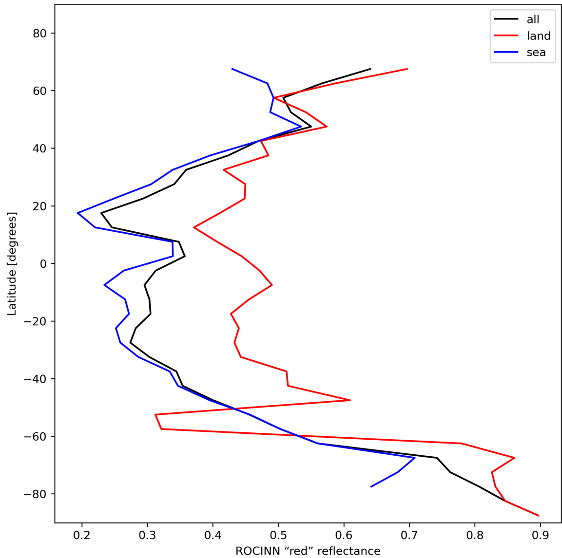
Figure 37: Zonal average of “ROCINN “red” reflectance” for 2023-12-07 to 2023-12-09.
