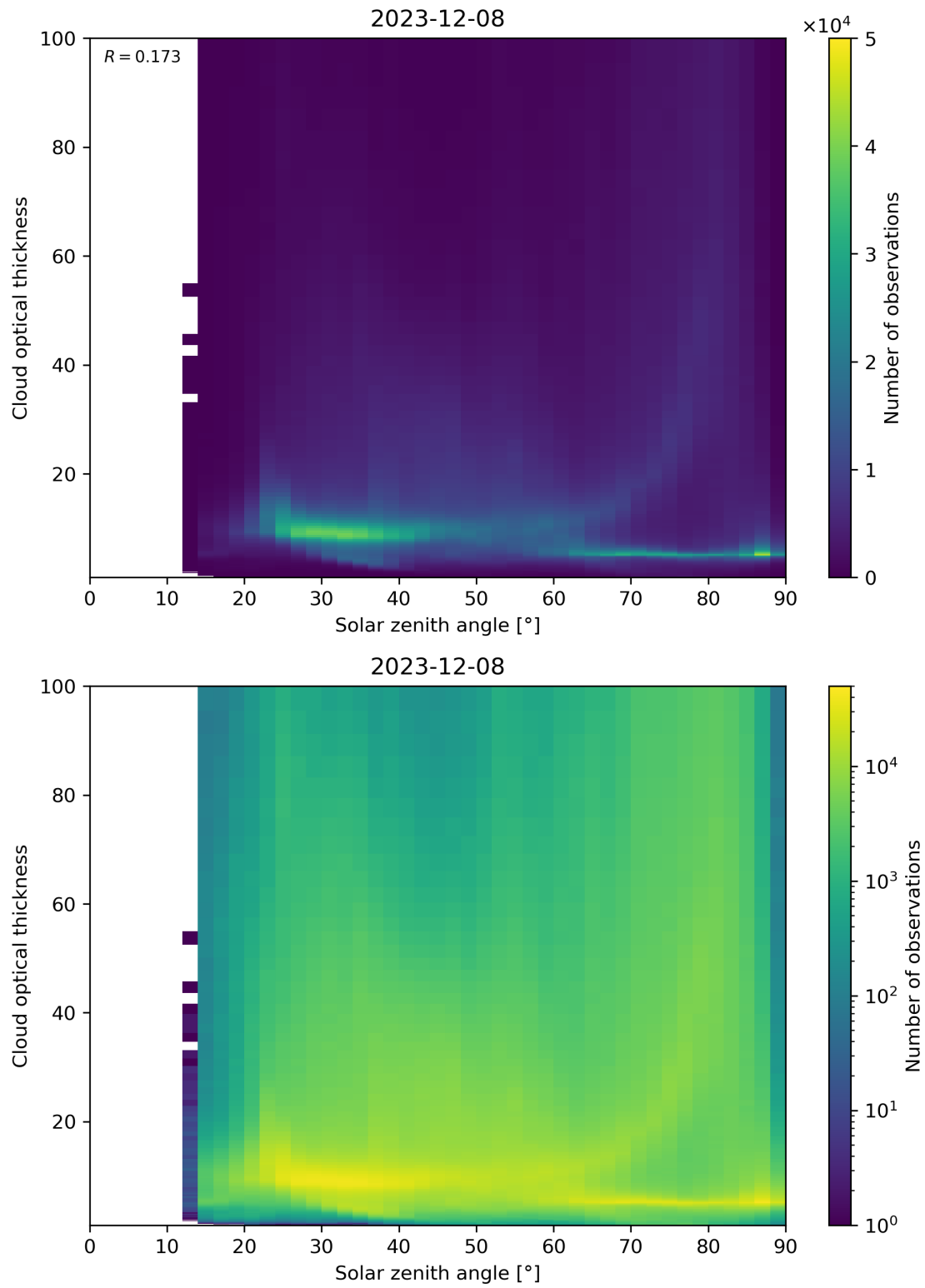
Figure 103: Scatter density plot of “Solar zenith angle” against “Cloud optical thickness” for 2023-12-07 to 2023-12-09.
