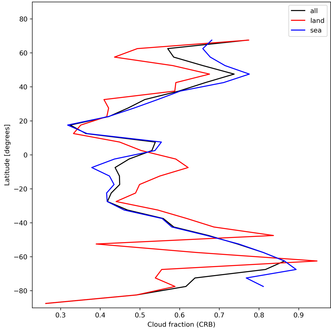
Figure 26: Zonal average of “Cloud fraction (CRB)” for 2023-12-07 to 2023-12-09.
