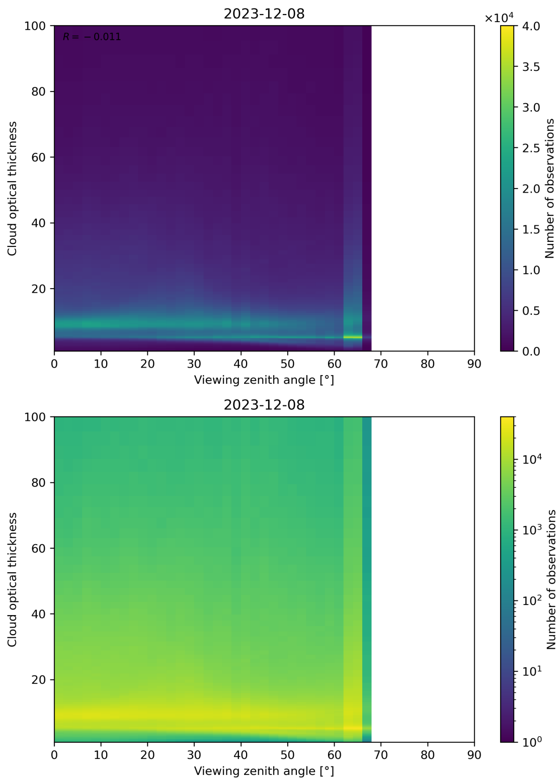
Figure 111: Scatter density plot of “Viewing zenith angle” against “Cloud optical thickness” for 2023-12-07 to 2023-12-09.
