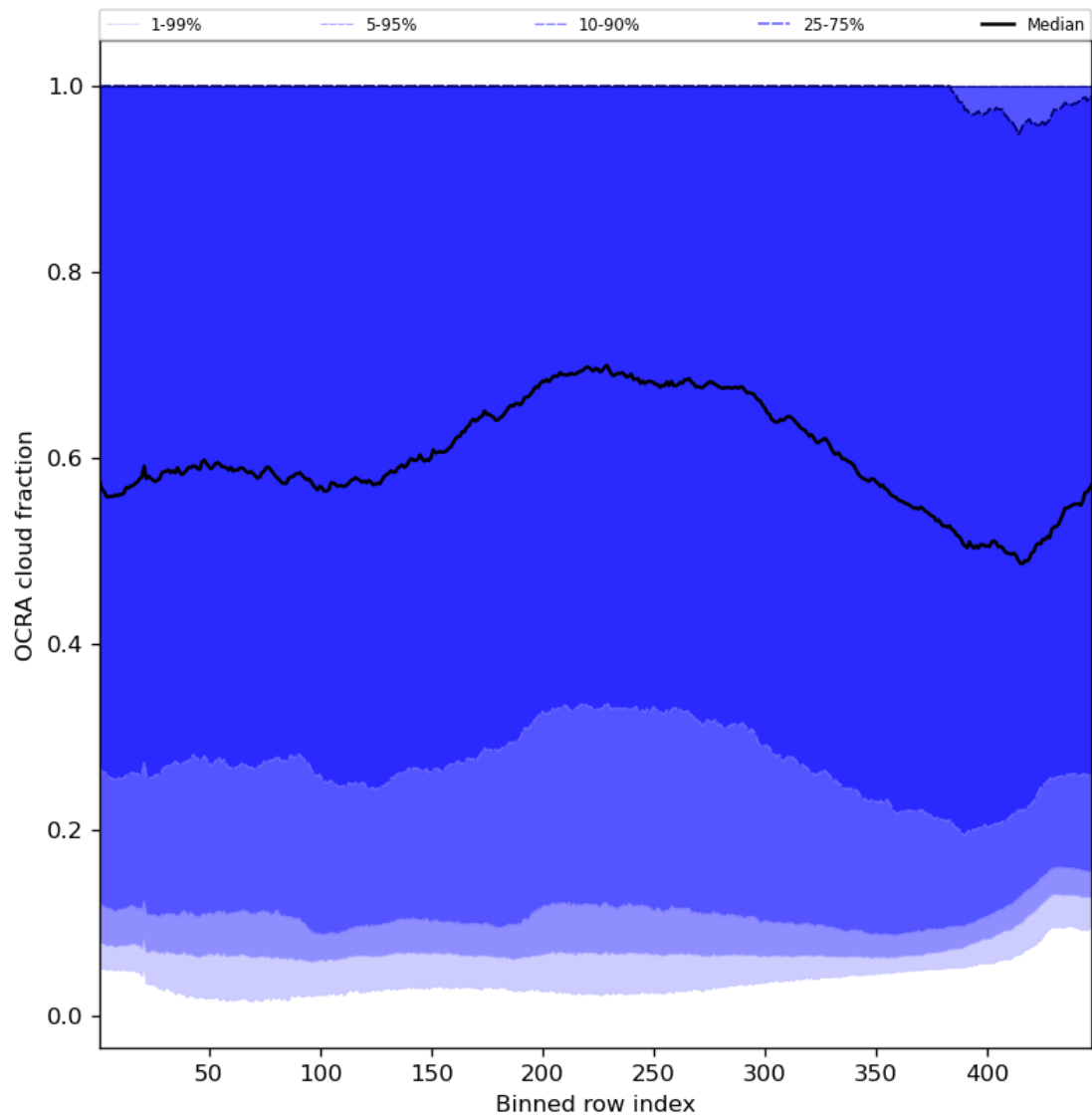
Figure 66: Along track statistics of “OCRA cloud fraction” for 2023-12-07 to 2023-12-09
