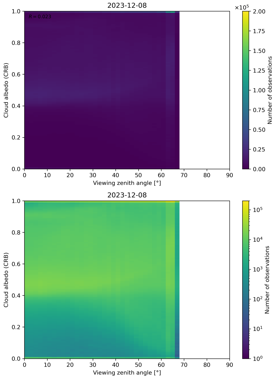
Figure 106: Scatter density plot of “Viewing zenith angle” against “Cloud albedo (CRB)” for 2023-12-07 to 2023-12-09.
