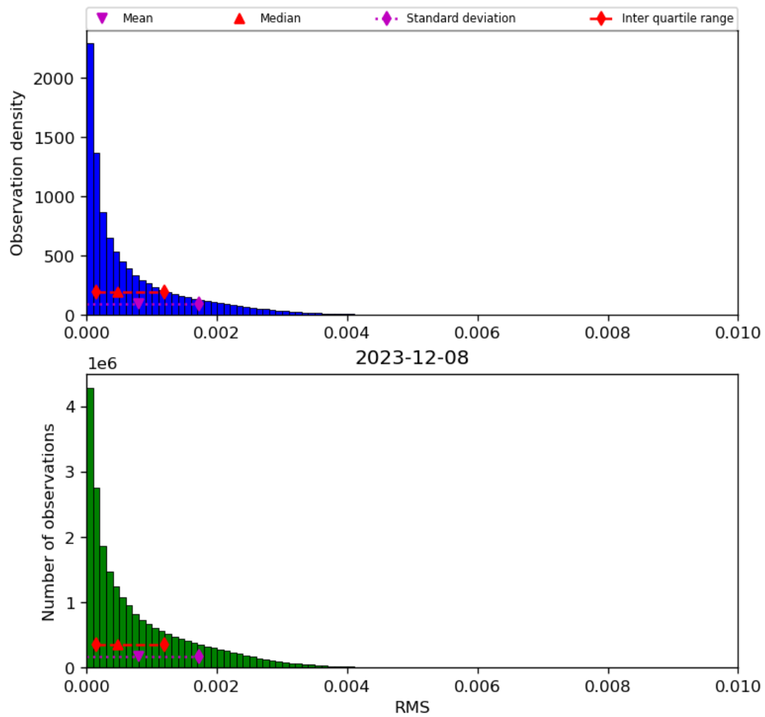
Figure 47: Histogram of “RMS” for 2023-12-07 to 2023-12-09
