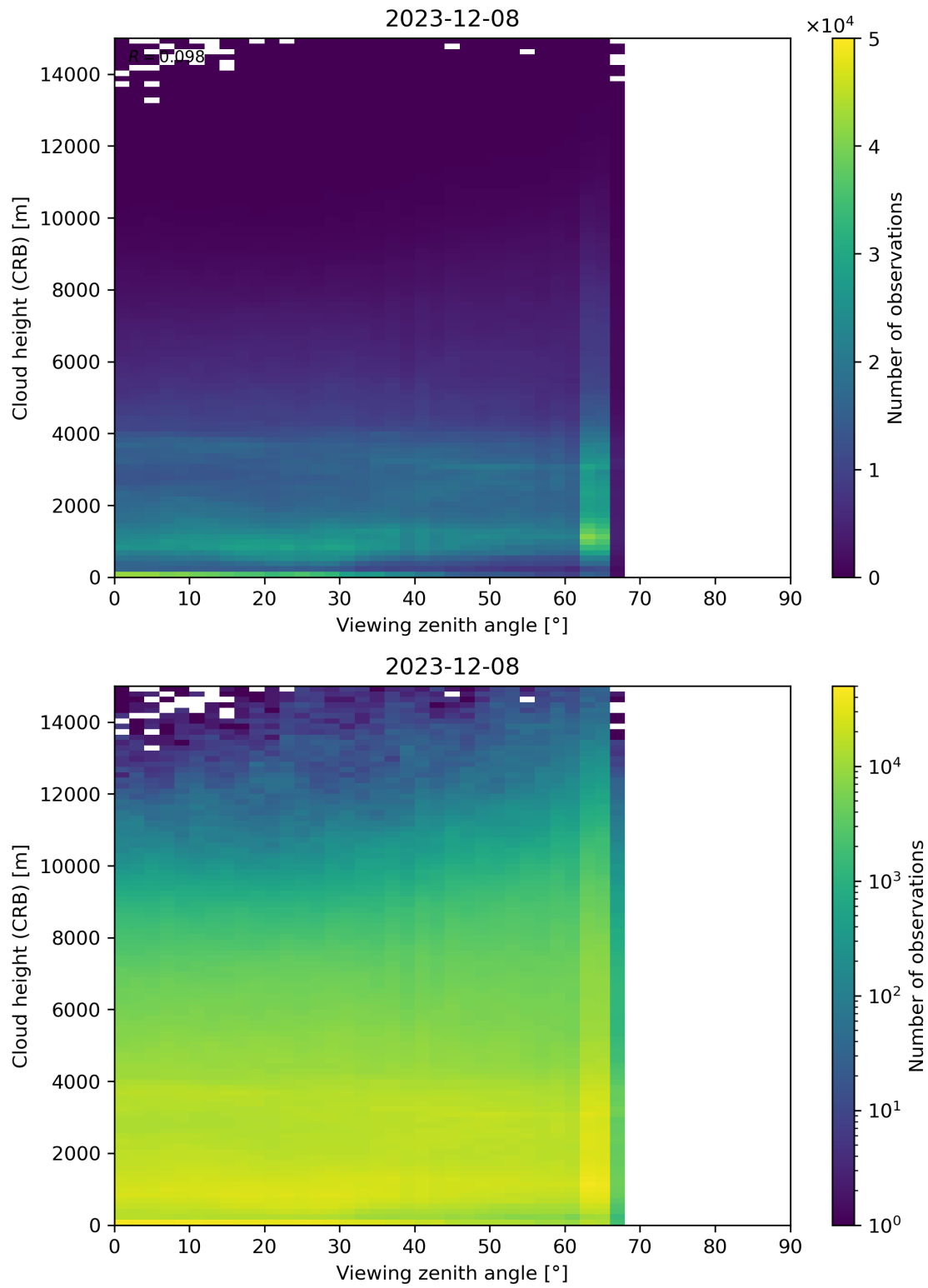
Figure 110: Scatter density plot of “Viewing zenith angle” against “Cloud height (CRB)” for 2023-12-07 to 2023-12-09.
