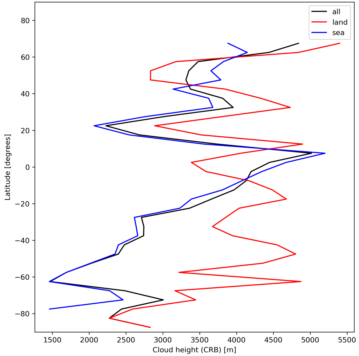
Figure 27: Zonal average of “Cloud height (CRB)” for 2023-12-07 to 2023-12-09.
