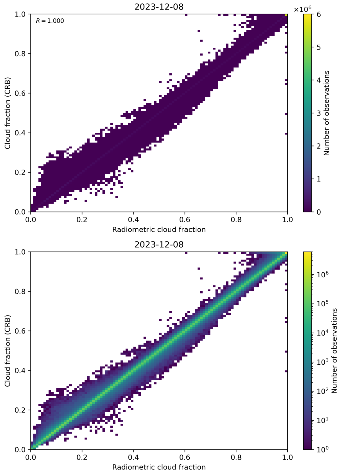
Figure 73: Scatter density plot of “Radiometric cloud fraction” against “Cloud fraction (CRB)” for 2023-12-07 to 2023-12-09.
