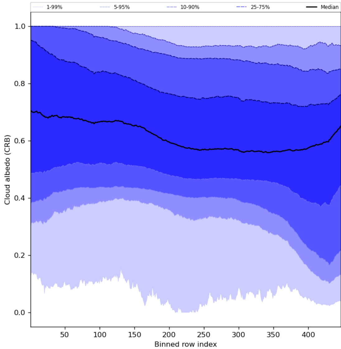
Figure 60: Along track statistics of “Cloud albedo (CRB)” for 2023-12-07 to 2023-12-09
