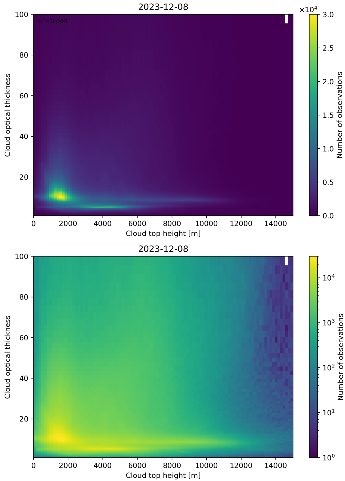
Figure 90: Scatter density plot of “Cloud top height” against “Cloud optical thickness” for 2023-12-07 to 2023-12-09.
