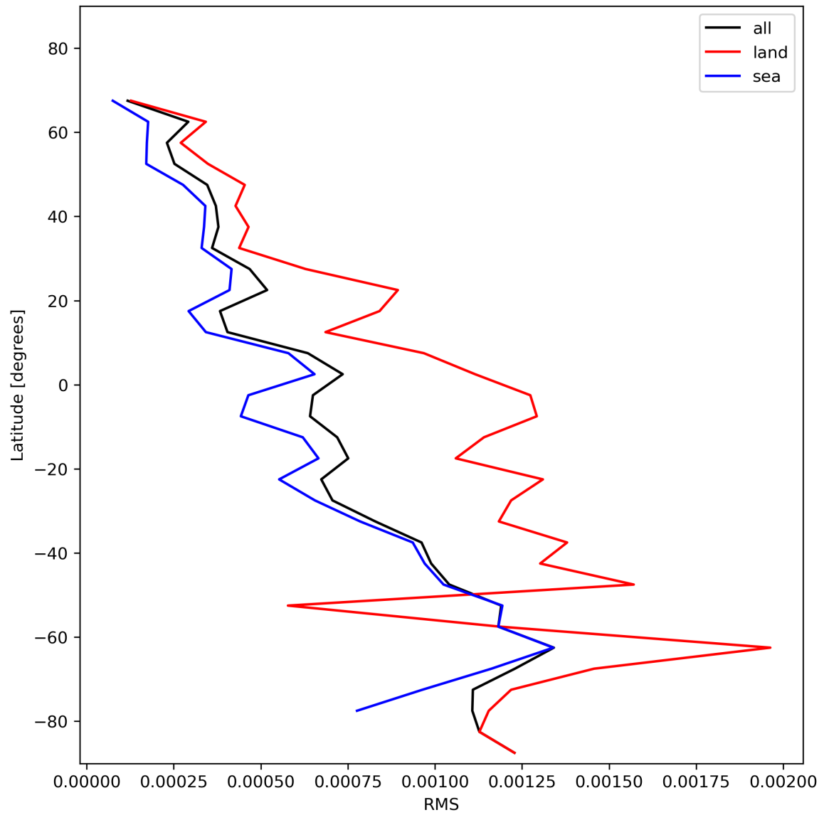
Figure 31: Zonal average of “RMS” for 2023-12-07 to 2023-12-09.
