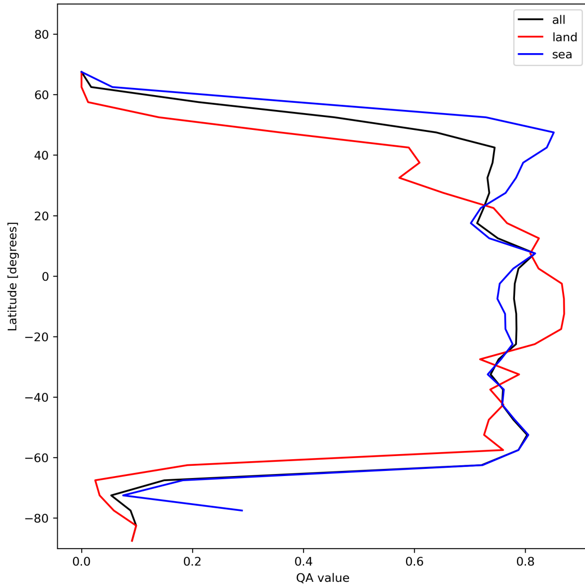
Figure 22: Zonal average of “QA value” for 2023-12-07 to 2023-12-09.
