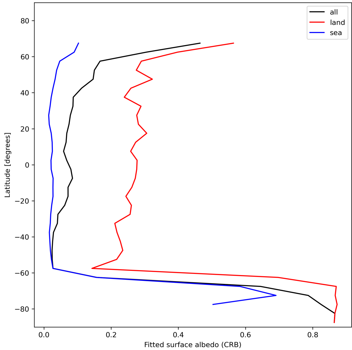
Figure 30: Zonal average of “Fitted surface albedo (CRB)” for 2023-12-07 to 2023-12-09.
