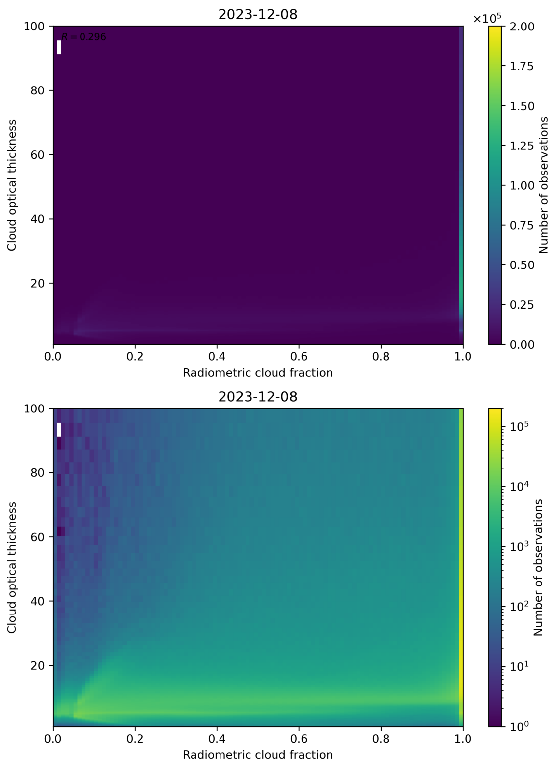
Figure 75: Scatter density plot of “Radiometric cloud fraction” against “Cloud optical thickness” for 2023-12-07 to 2023-12-09.
