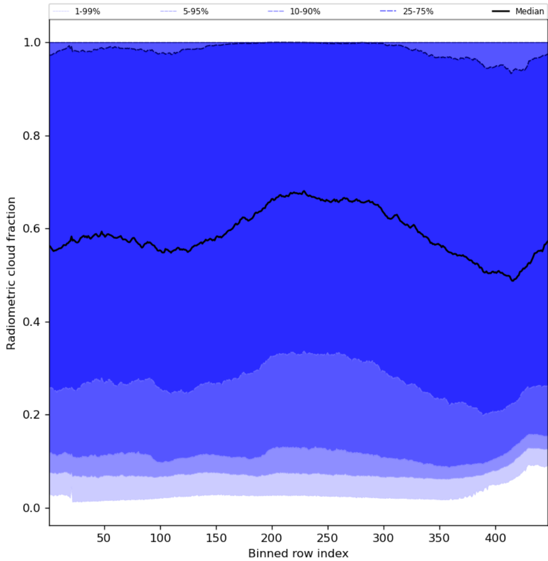
Figure 55: Along track statistics of “Radiometric cloud fraction” for 2023-12-07 to 2023-12-09
