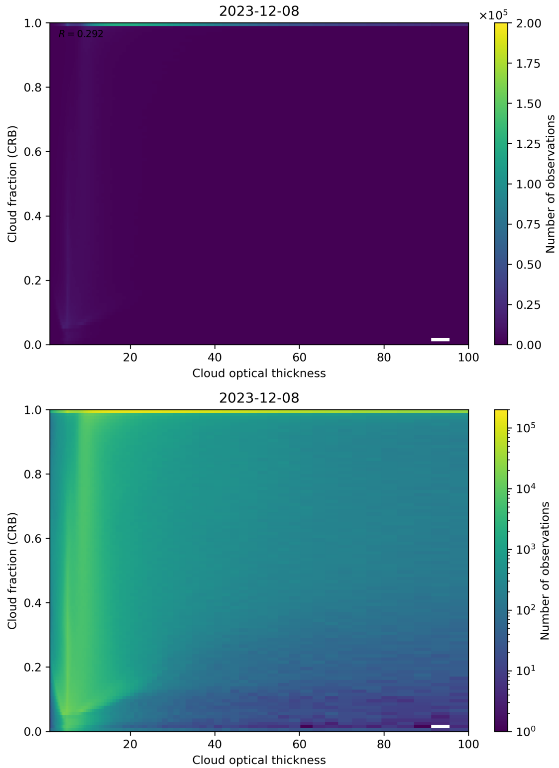
Figure 84: Scatter density plot of “Cloud optical thickness” against “Cloud fraction (CRB)” for 2023-12-07 to 2023-12-09.
