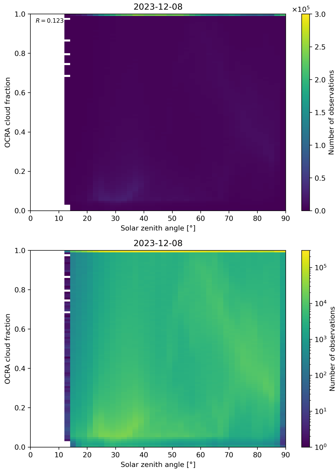
Figure 100: Scatter density plot of “Solar zenith angle” against “OCRA cloud fraction” for 2023-12-07 to 2023-12-09.
