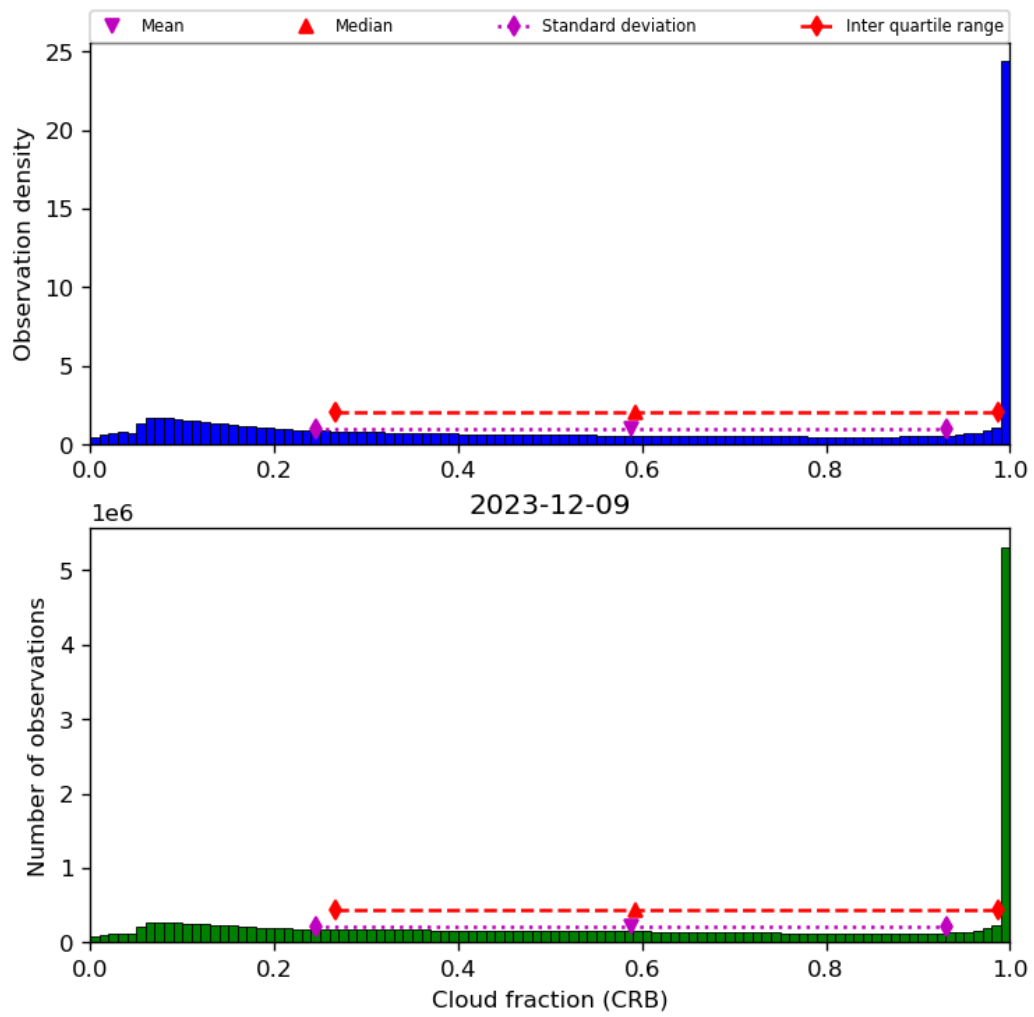
Figure 42: Histogram of “Cloud fraction (CRB)” for 2023-12-09 to 2023-12-10
