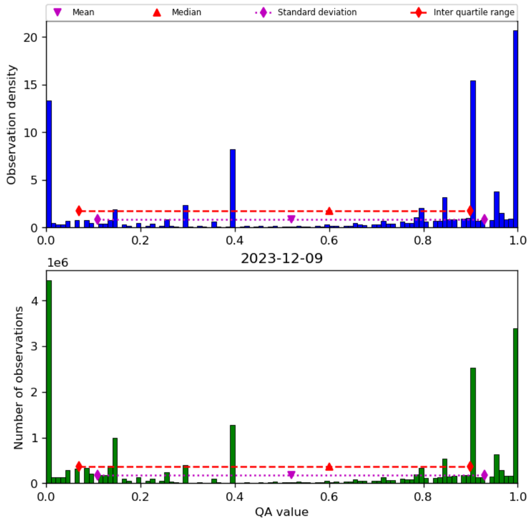
Figure 38: Histogram of “QA value” for 2023-12-09 to 2023-12-10
