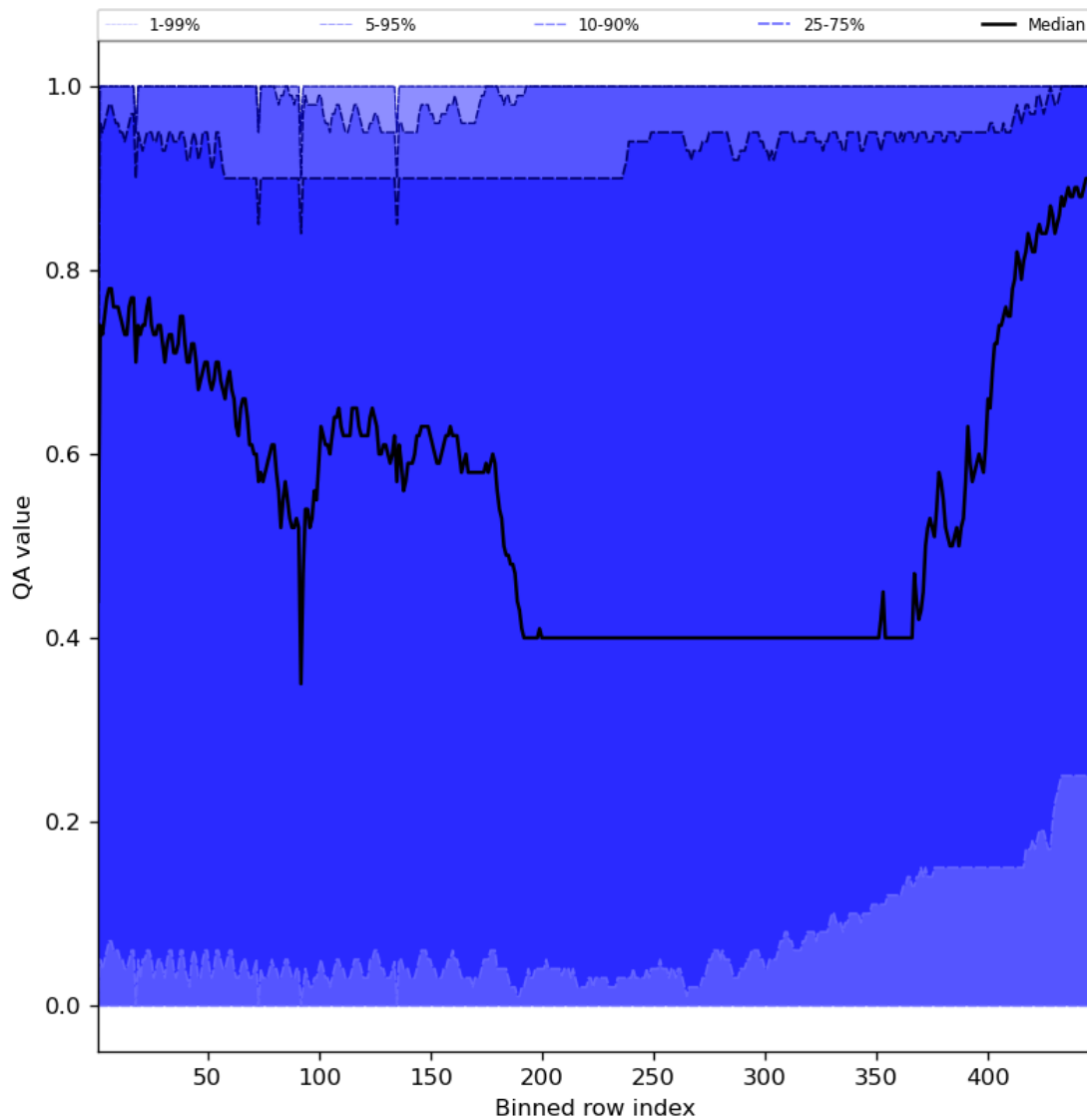
Figure 54: Along track statistics of “QA value” for 2023-12-09 to 2023-12-10
