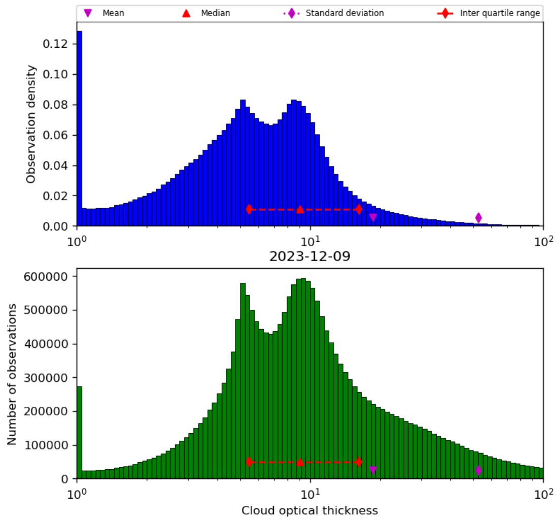
Figure 41: Histogram of “Cloud optical thickness” for 2023-12-09 to 2023-12-10
