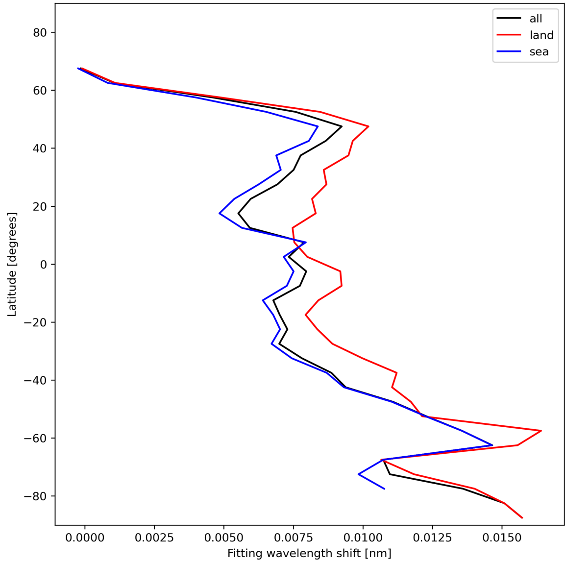
Figure 33: Zonal average of “Fitting wavelength shift” for 2023-12-09 to 2023-12-10.
