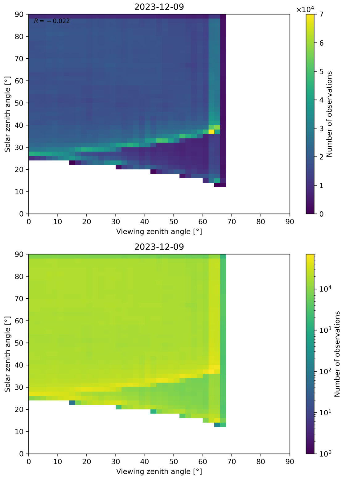
Figure 114: Scatter density plot of “Viewing zenith angle” against “Solar zenith angle” for 2023-12-09 to 2023-12-10.
