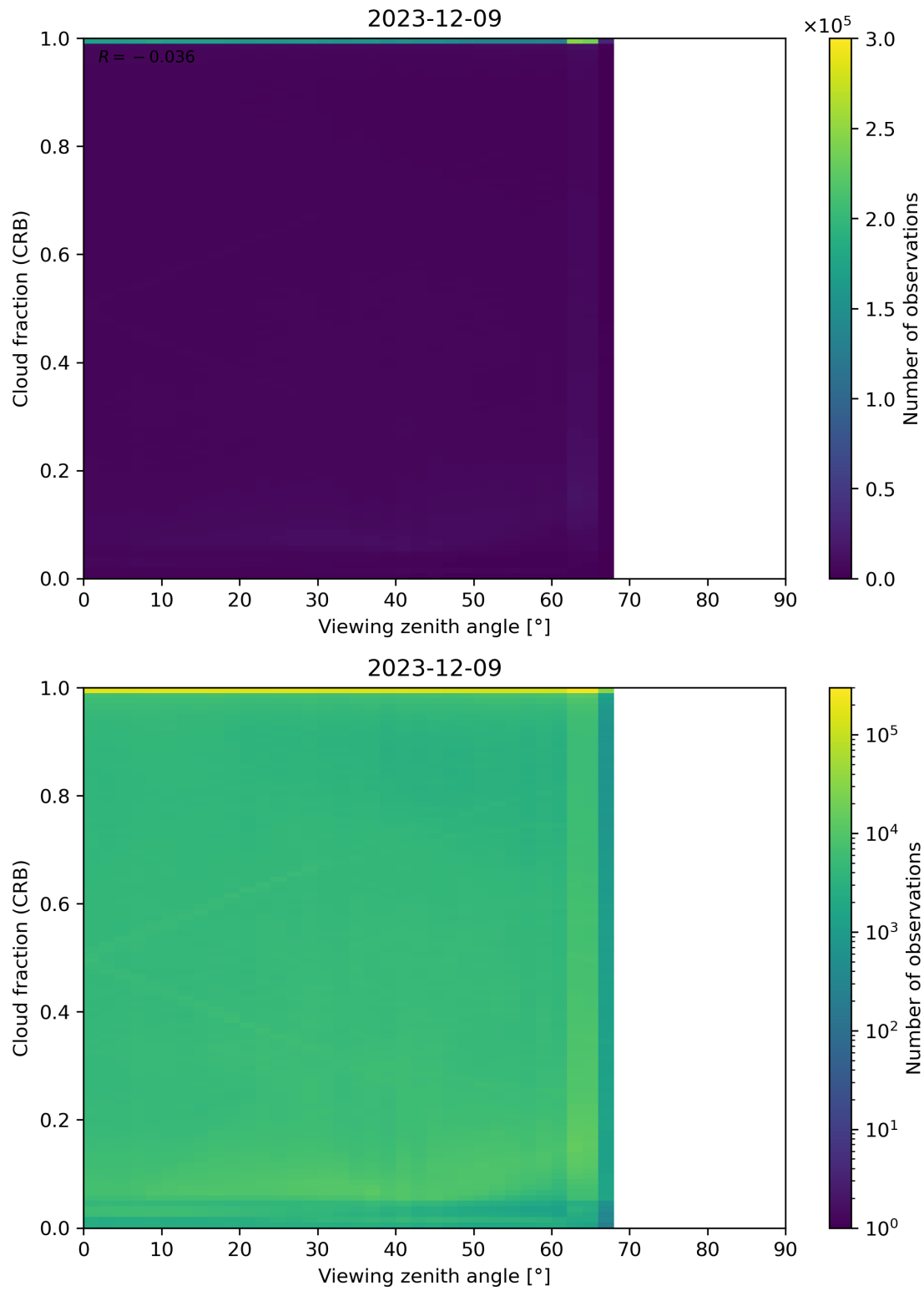
Figure 109: Scatter density plot of “Viewing zenith angle” against “Cloud fraction (CRB)” for 2023-12-09 to 2023-12-10.
