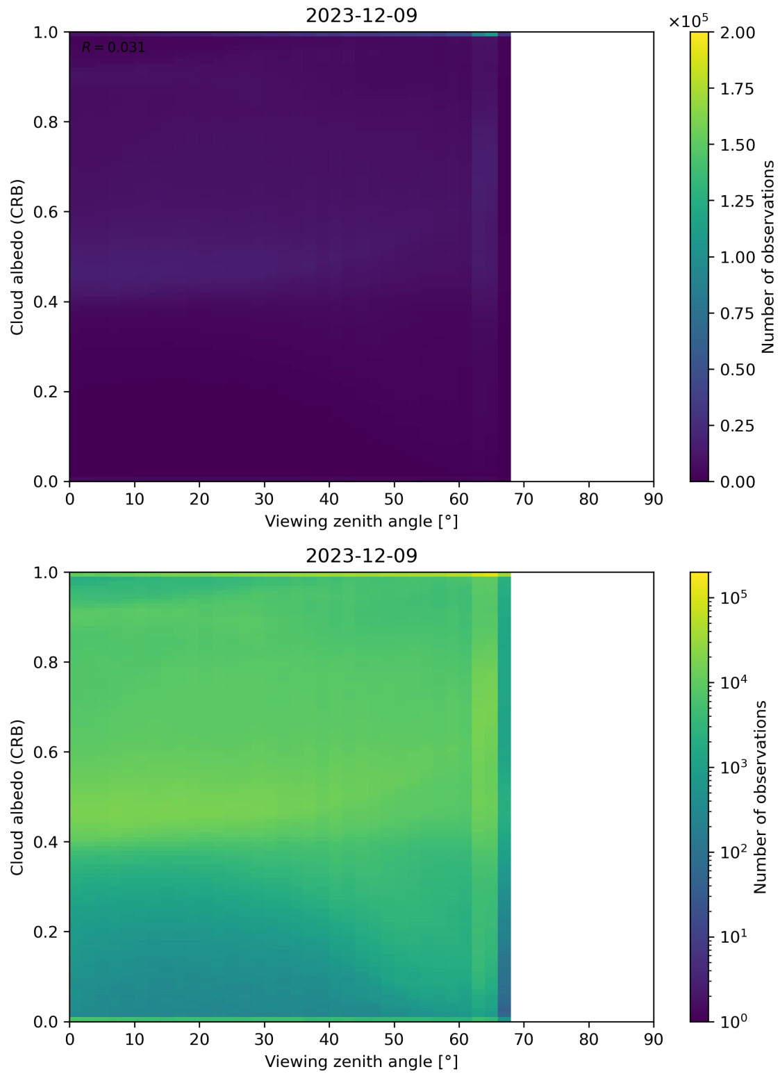
Figure 106: Scatter density plot of “Viewing zenith angle” against “Cloud albedo (CRB)” for 2023-12-09 to 2023-12-10.
