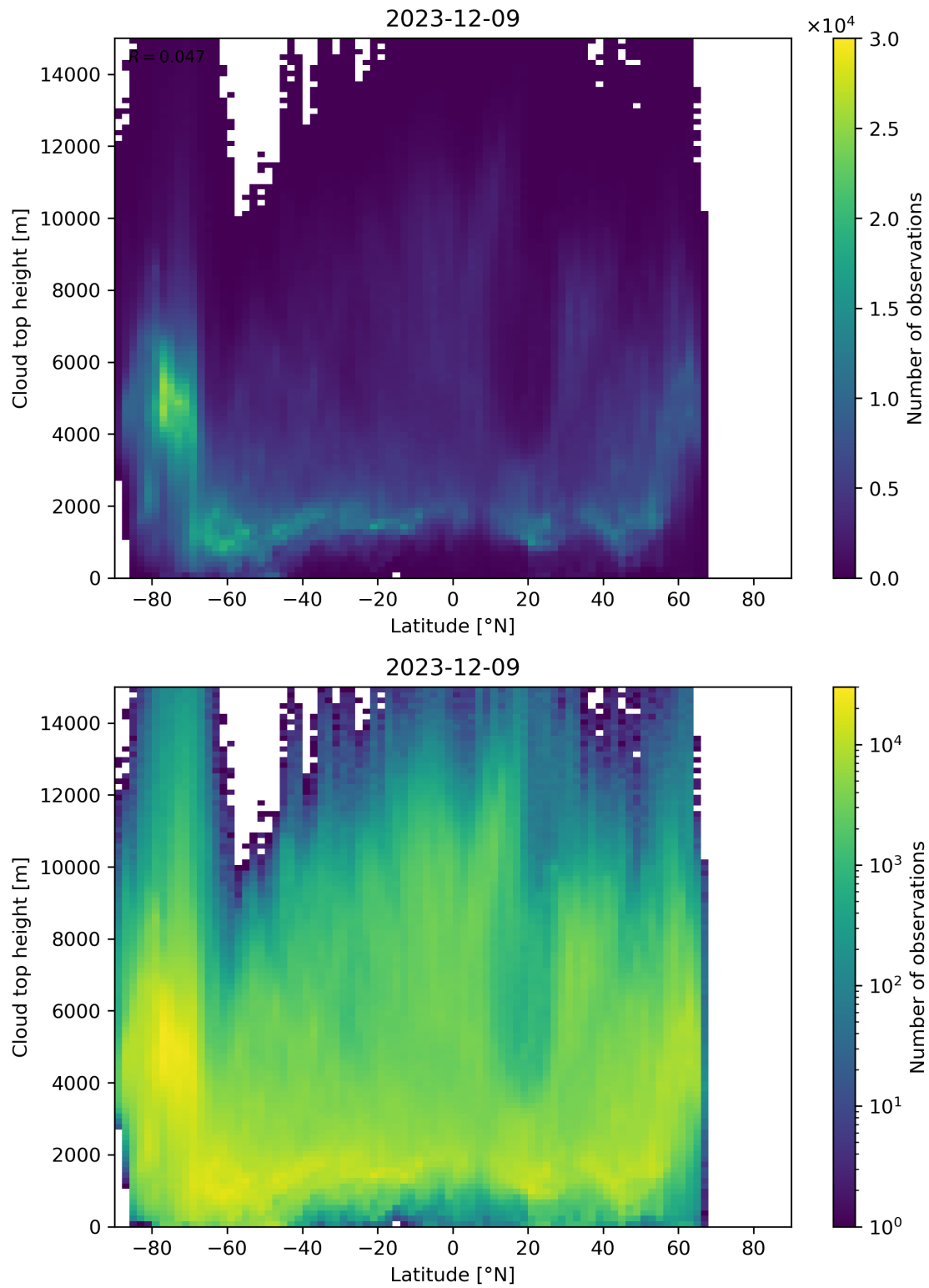
Figure 97: Scatter density plot of “Latitude” against “Cloud top height” for 2023-12-09 to 2023-12-10.
