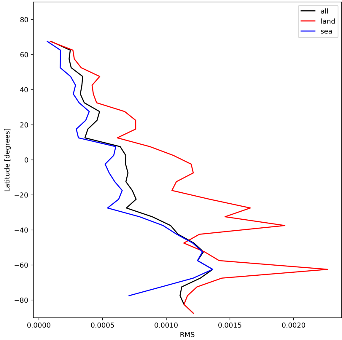
Figure 31: Zonal average of “RMS” for 2023-12-09 to 2023-12-10.
