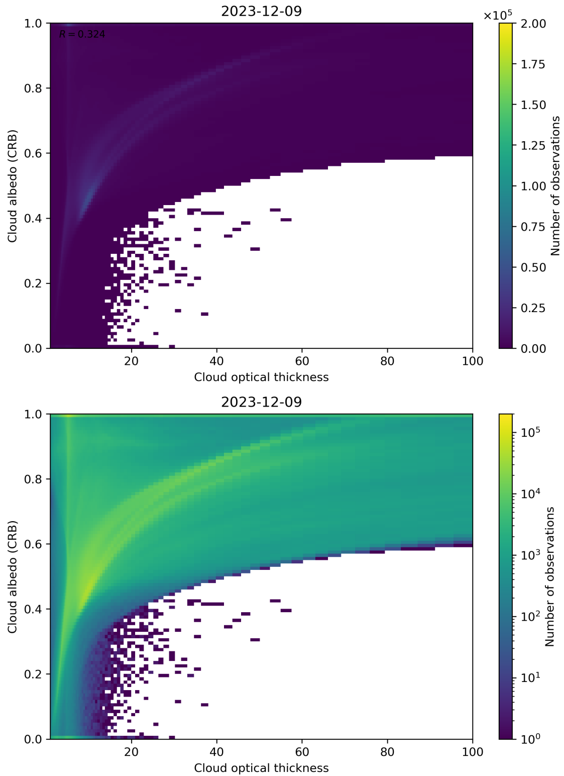
Figure 82: Scatter density plot of “Cloud optical thickness” against “Cloud albedo (CRB)” for 2023-12-09 to 2023-12-10.
