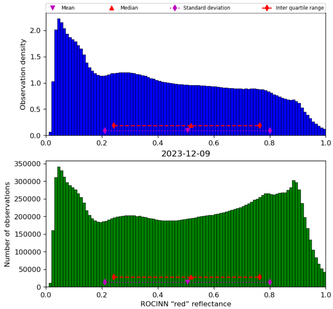
Figure 53: Histogram of “ROCINN “red” reflectance” for 2023-12-09 to 2023-12-10
