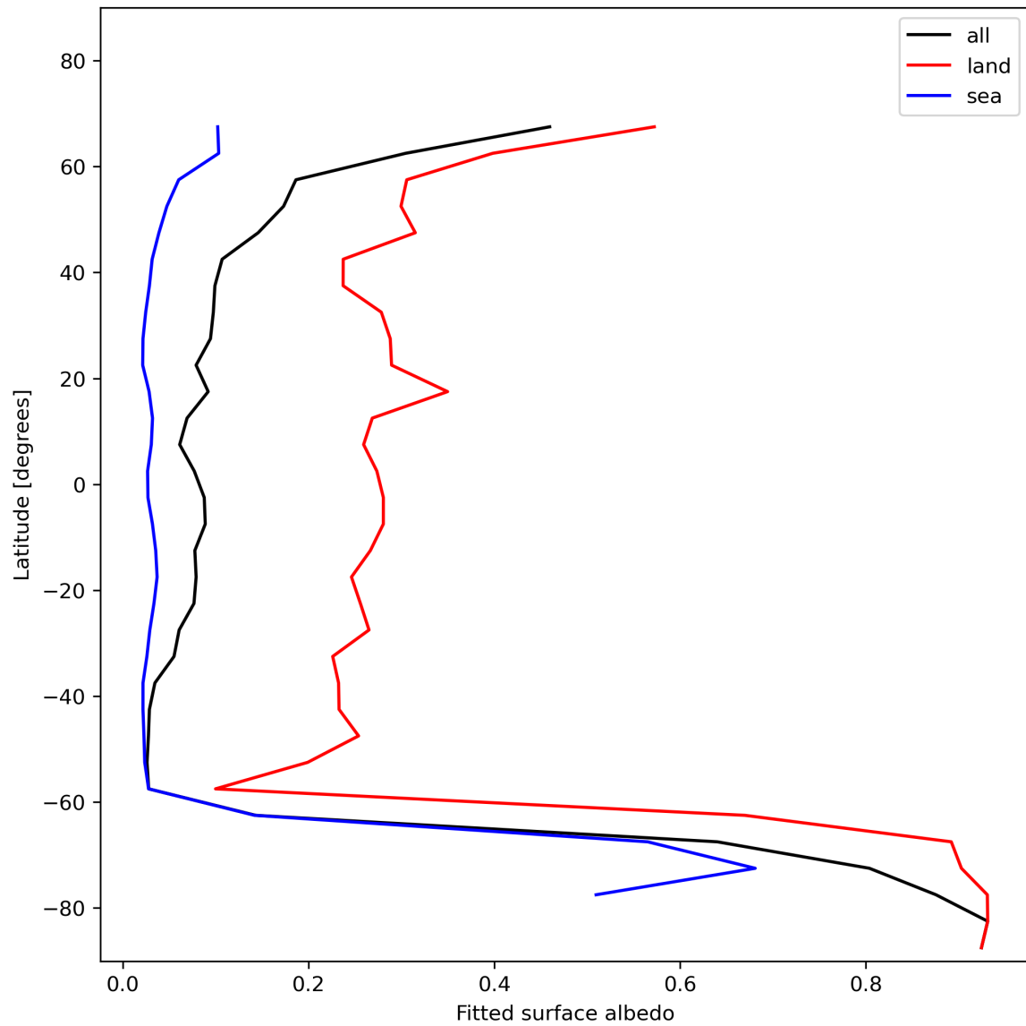
Figure 29: Zonal average of “Fitted surface albedo” for 2023-12-09 to 2023-12-10.
