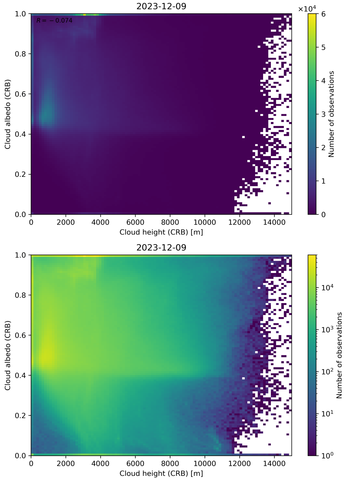
Figure 80: Scatter density plot of “Cloud height (CRB)” against “Cloud albedo (CRB)” for 2023-12-09 to 2023-12-10.
