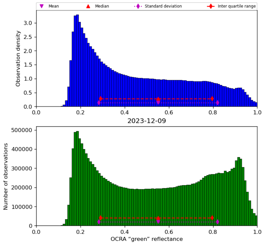
Figure 52: Histogram of “OCRA “green” reflectance” for 2023-12-09 to 2023-12-10
