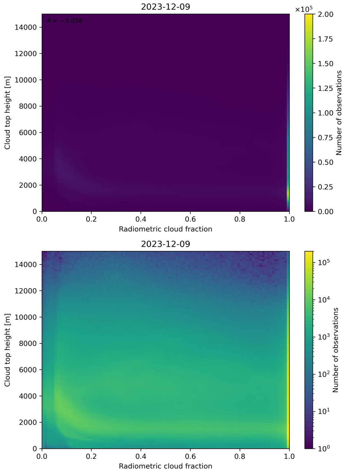
Figure 76: Scatter density plot of “Radiometric cloud fraction” against “Cloud top height” for 2023-12-09 to 2023-12-10.
