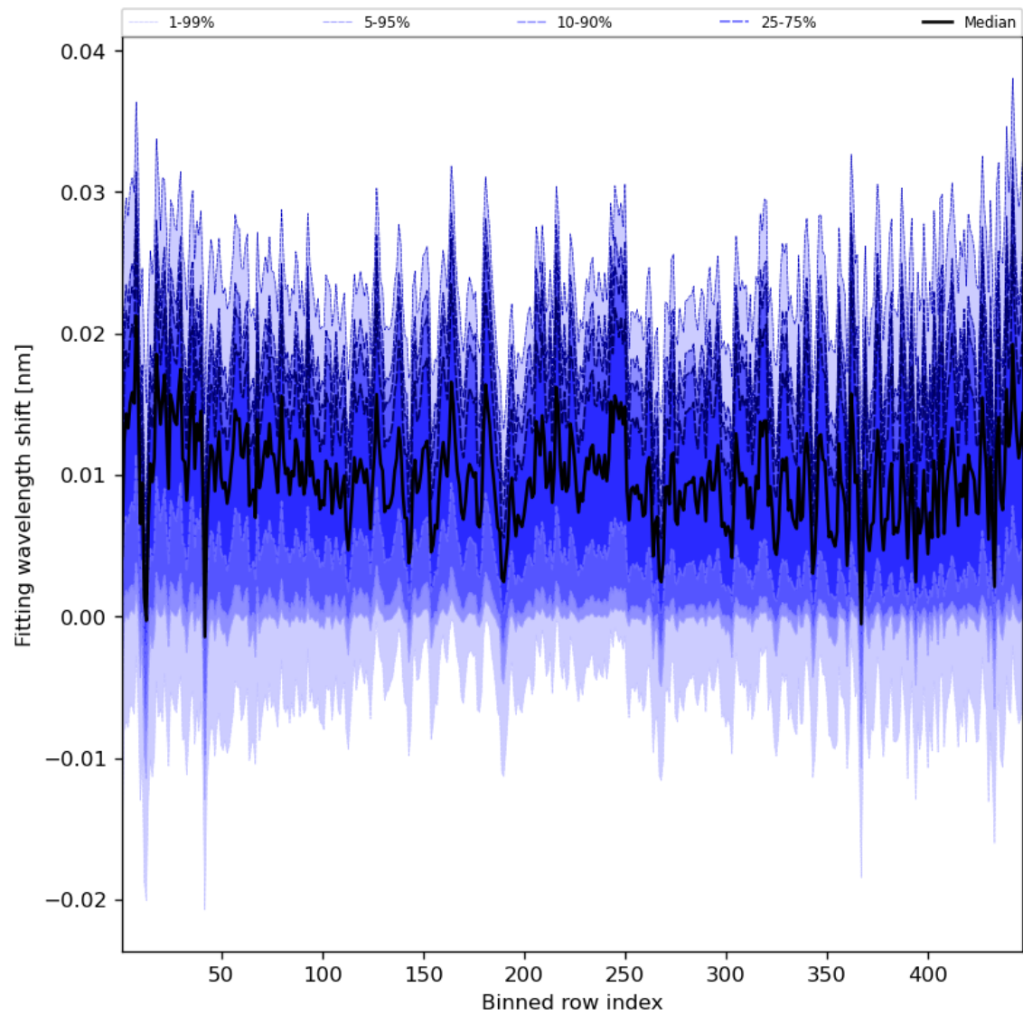
Figure 65: Along track statistics of “Fitting wavelength shift” for 2023-12-09 to 2023-12-10
