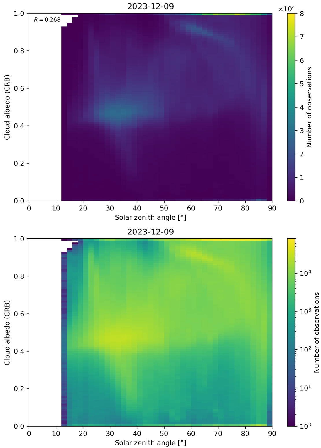
Figure 98: Scatter density plot of “Solar zenith angle” against “Cloud albedo (CRB)” for 2023-12-09 to 2023-12-10.
