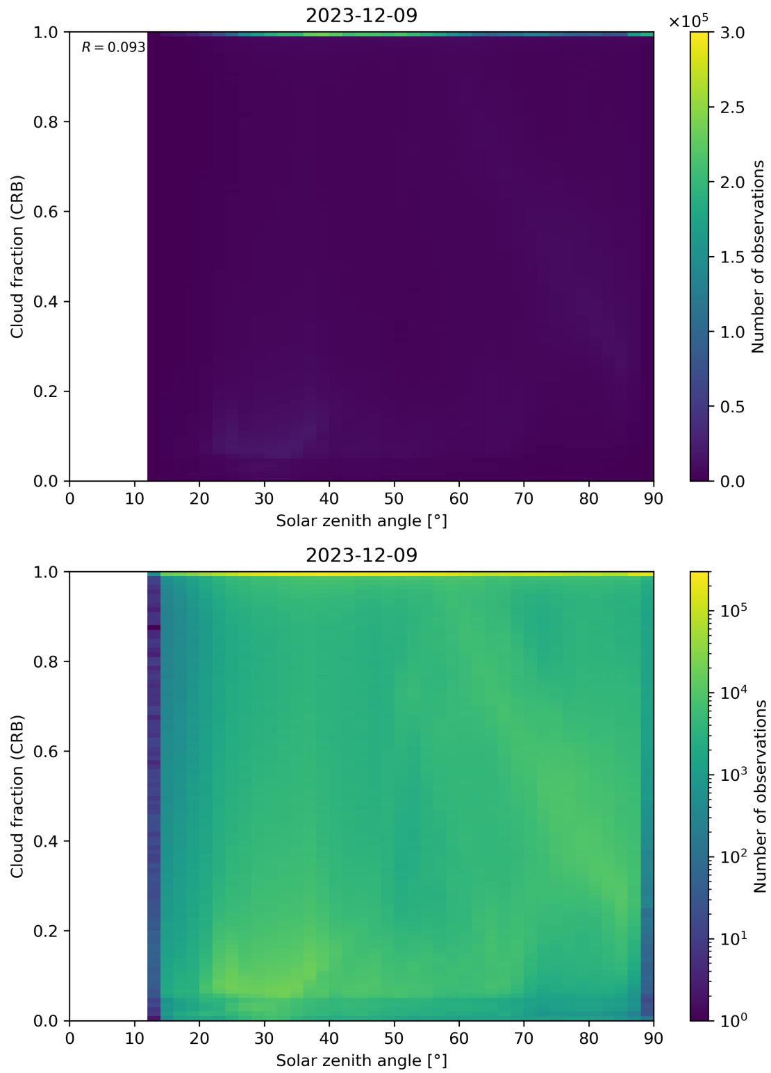
Figure 101: Scatter density plot of “Solar zenith angle” against “Cloud fraction (CRB)” for 2023-12-09 to 2023-12-10.
