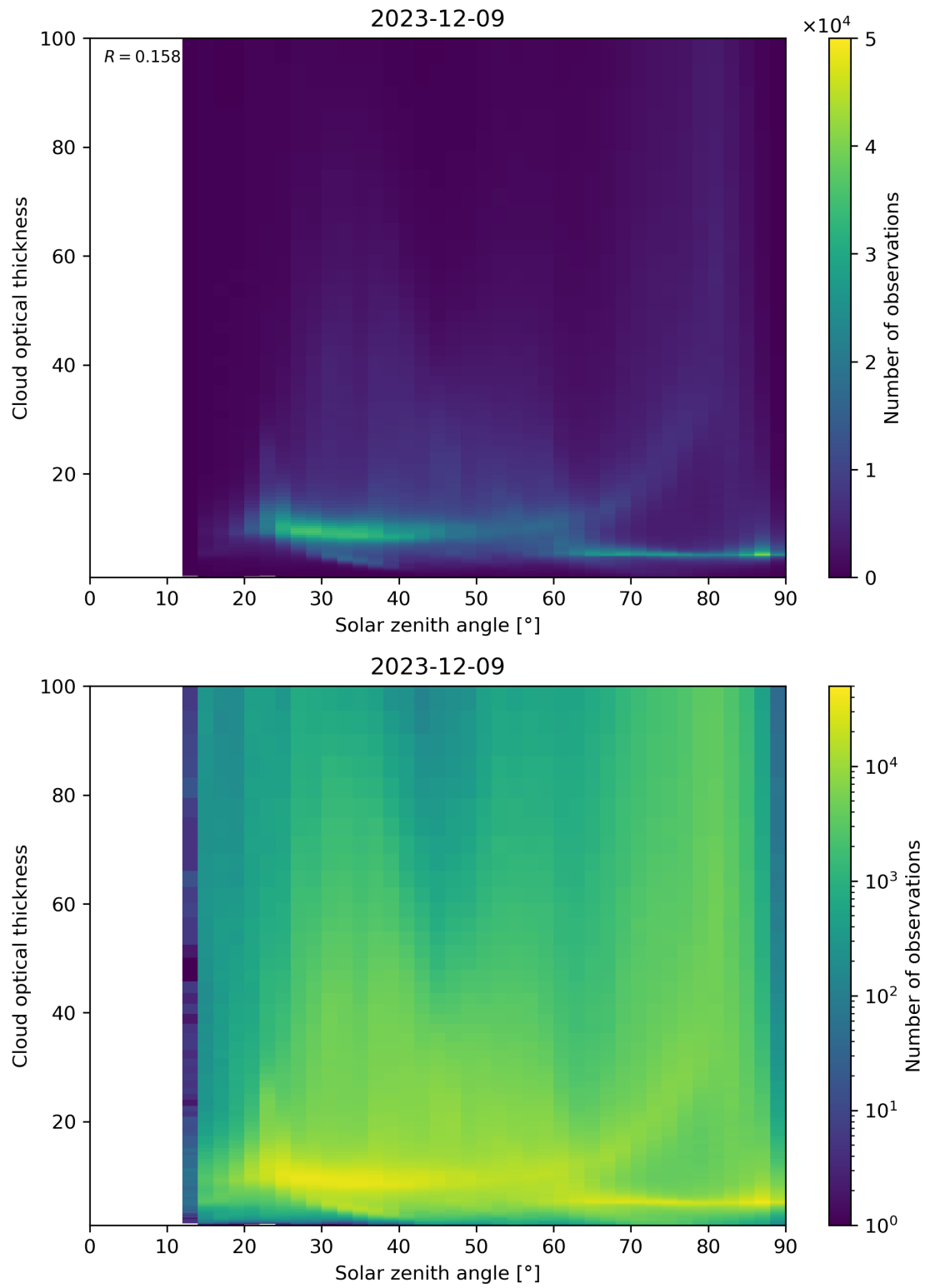
Figure 103: Scatter density plot of “Solar zenith angle” against “Cloud optical thickness” for 2023-12-09 to 2023-12-10.
