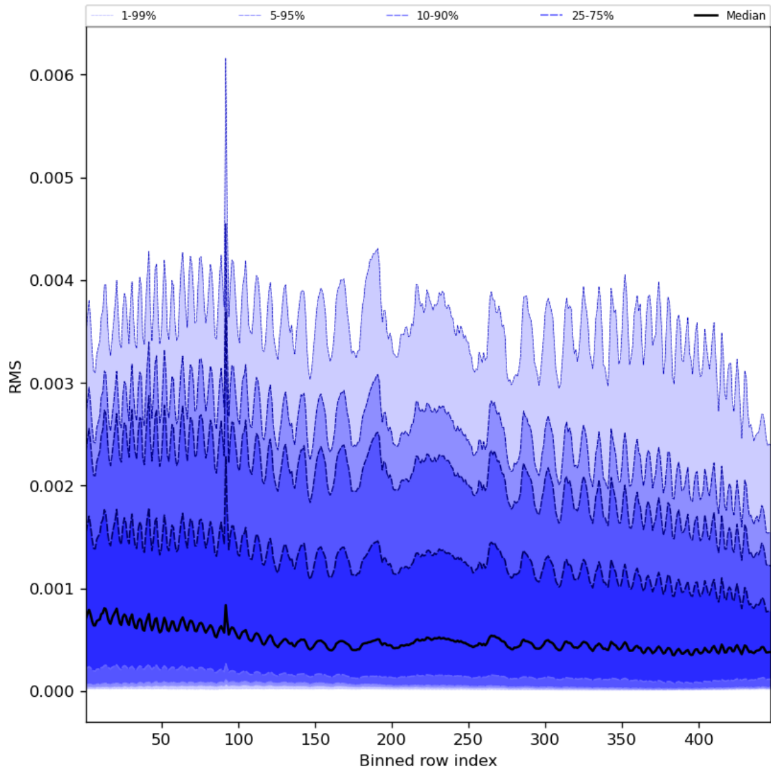
Figure 63: Along track statistics of “RMS” for 2023-12-09 to 2023-12-10
