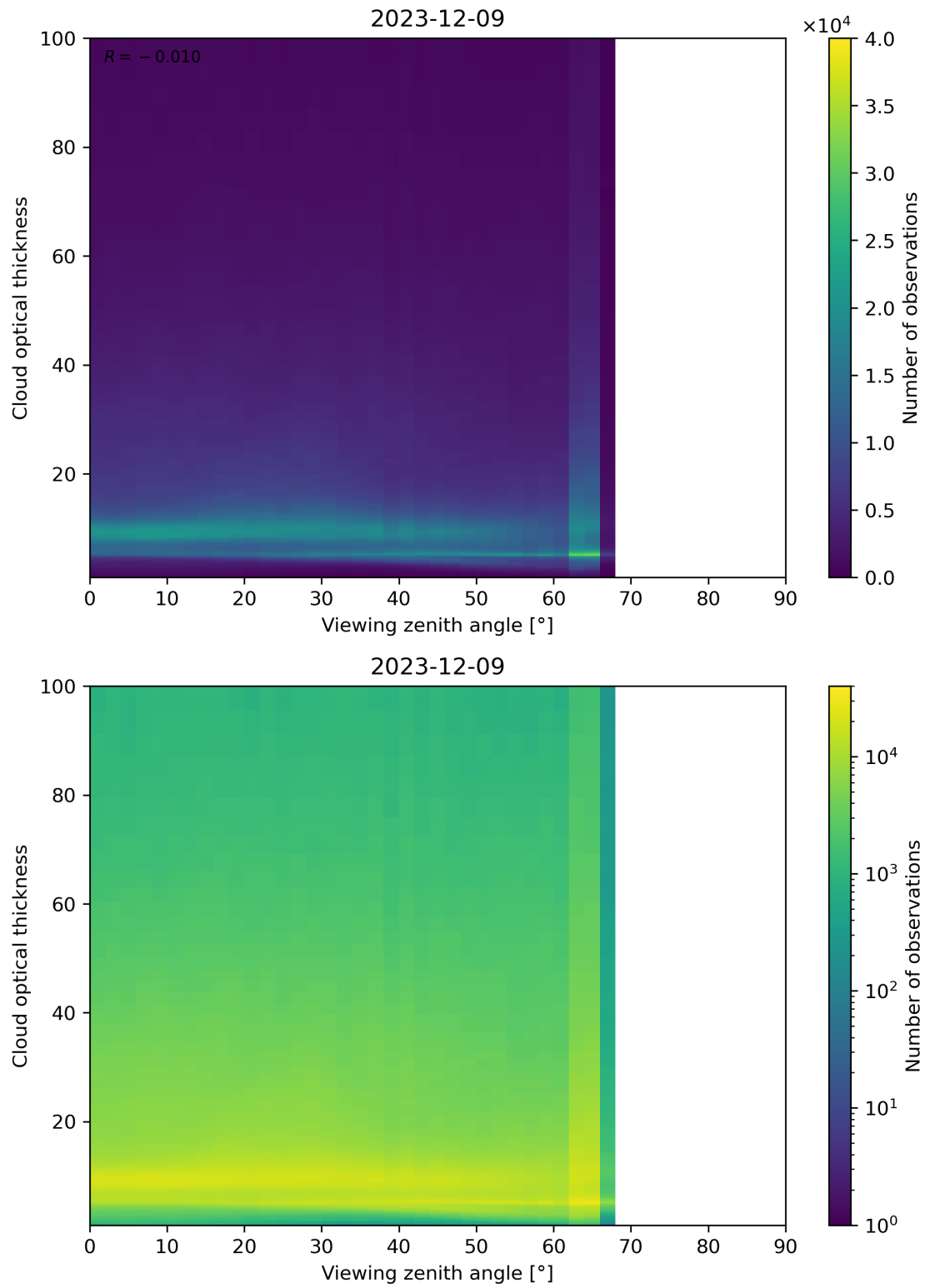
Figure 111: Scatter density plot of “Viewing zenith angle” against “Cloud optical thickness” for 2023-12-09 to 2023-12-10.
