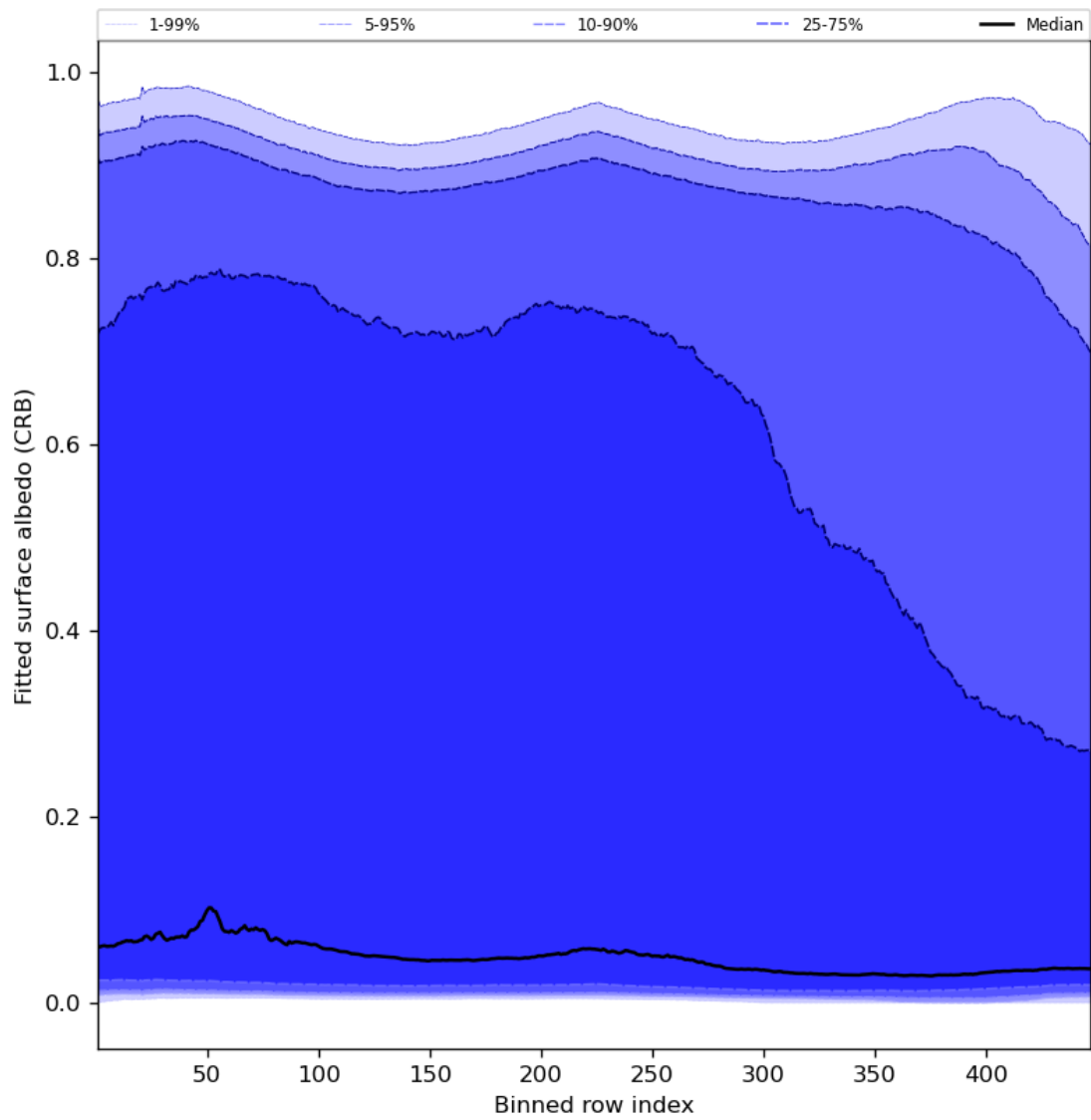
Figure 62: Along track statistics of “Fitted surface albedo (CRB)” for 2023-12-09 to 2023-12-10
