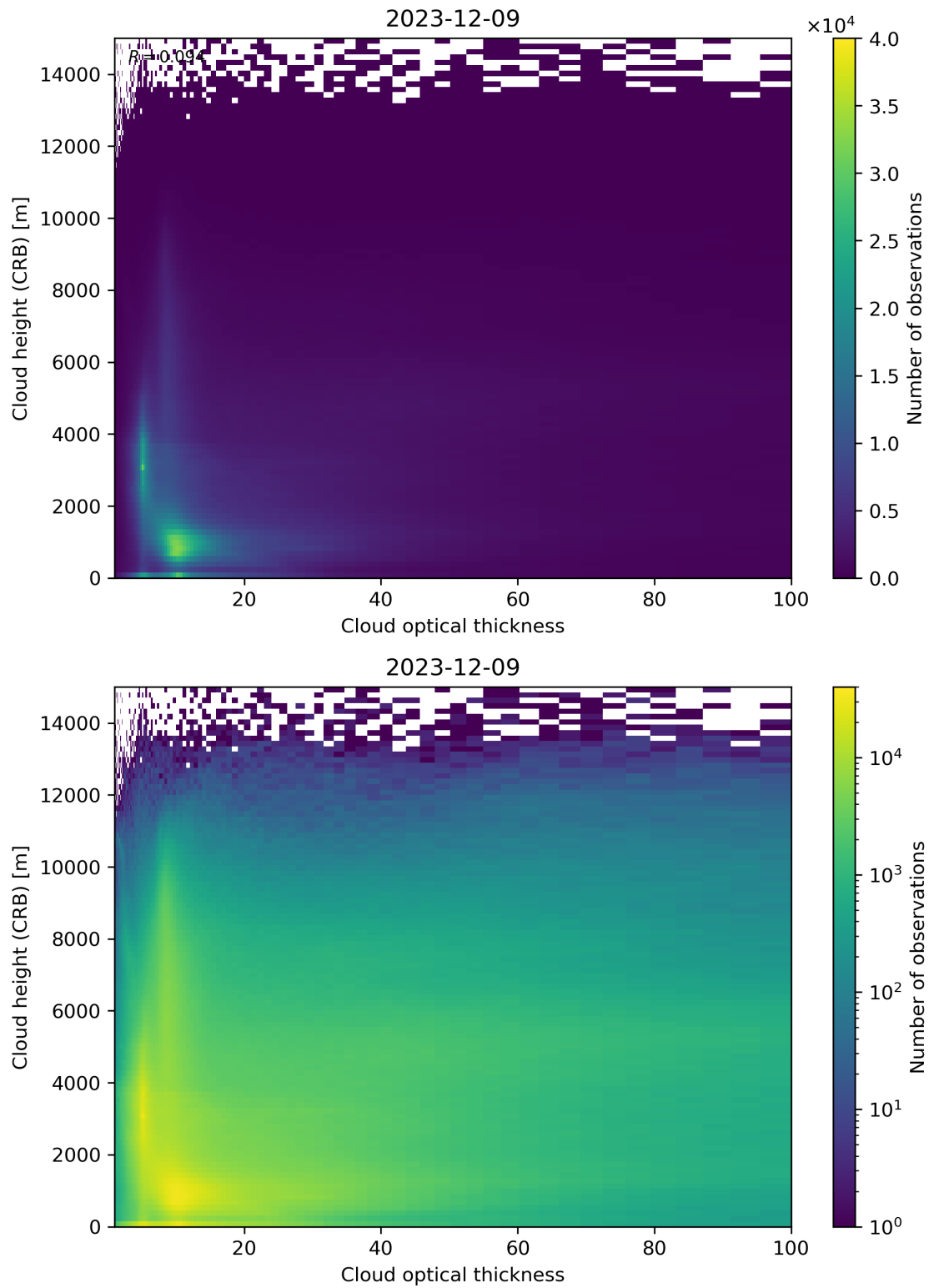
Figure 85: Scatter density plot of “Cloud optical thickness” against “Cloud height (CRB)” for 2023-12-09 to 2023-12-10.
