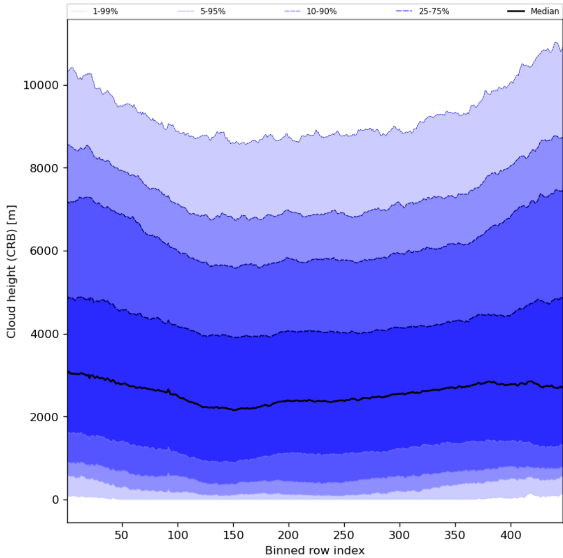
Figure 59: Along track statistics of “Cloud height (CRB)” for 2023-12-09 to 2023-12-10
