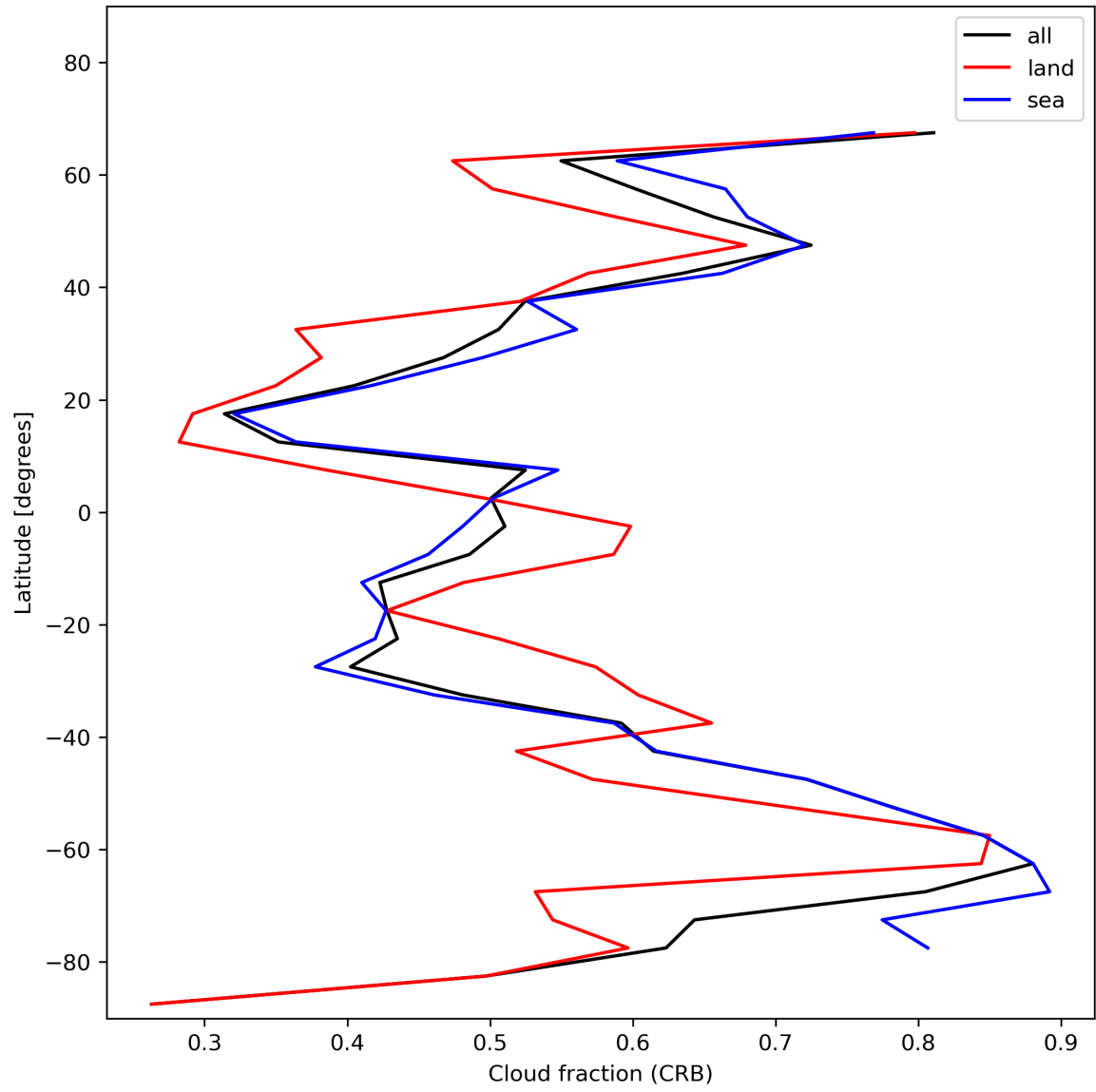
Figure 26: Zonal average of “Cloud fraction (CRB)” for 2023-12-09 to 2023-12-10.
