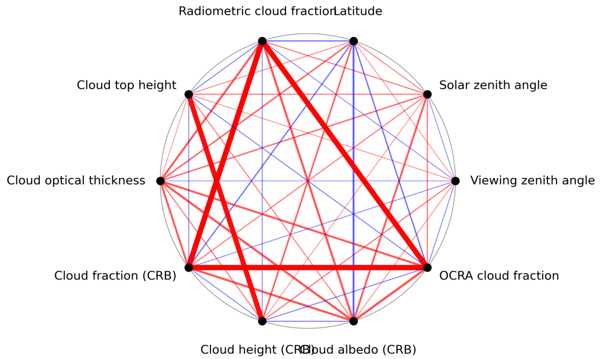
Figure 1: Map of correlation graph for 2023-12-09 to 2023-12-10.
