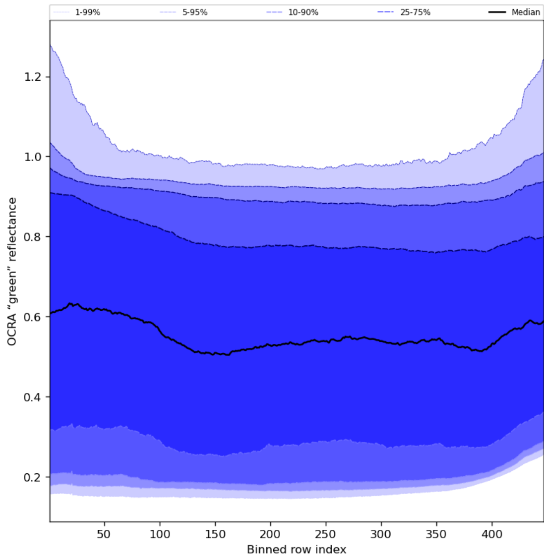
Figure 68: Along track statistics of “OCRA “green” reflectance” for 2023-12-09 to 2023-12-10
