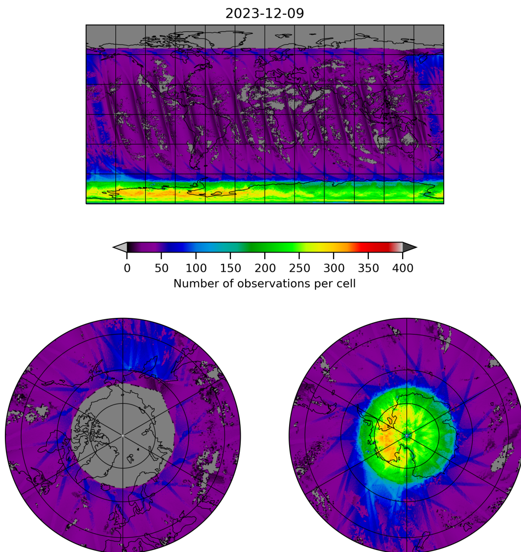
Figure 21: Map of the number of observations for 2023-12-09 to 2023-12-10
