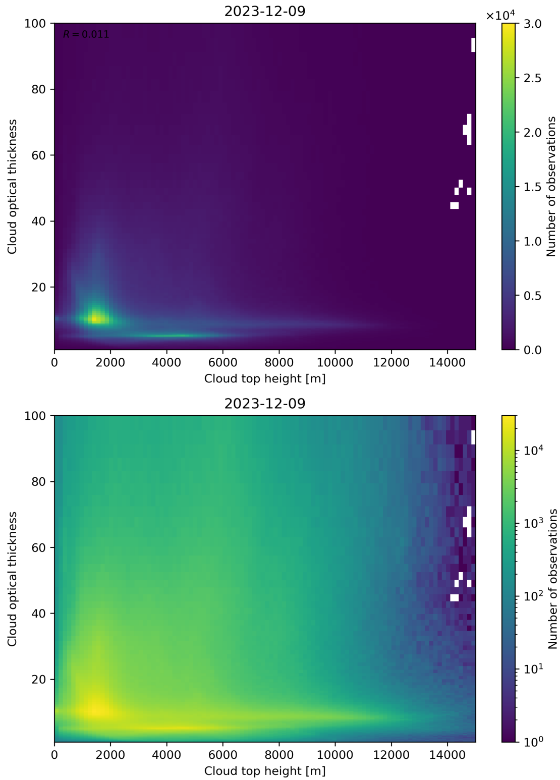
Figure 90: Scatter density plot of “Cloud top height” against “Cloud optical thickness” for 2023-12-09 to 2023-12-10.
