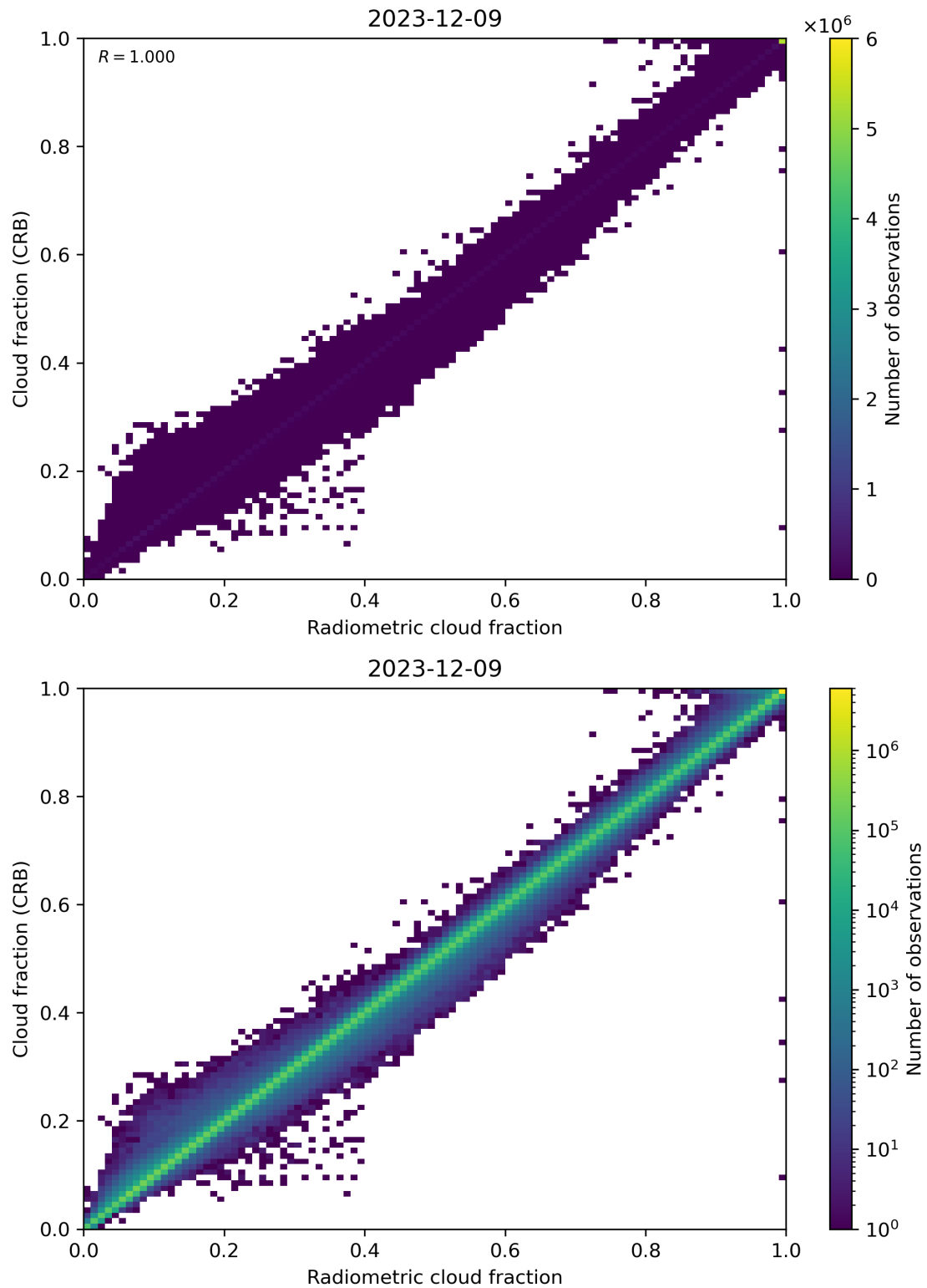
Figure 73: Scatter density plot of “Radiometric cloud fraction” against “Cloud fraction (CRB)” for 2023-12-09 to 2023-12-10.
