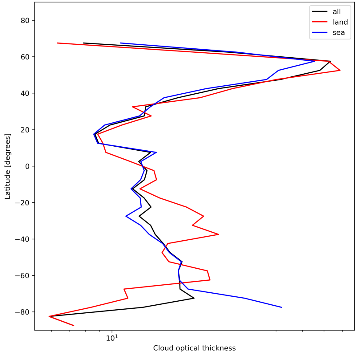
Figure 25: Zonal average of “Cloud optical thickness” for 2023-12-09 to 2023-12-10.
