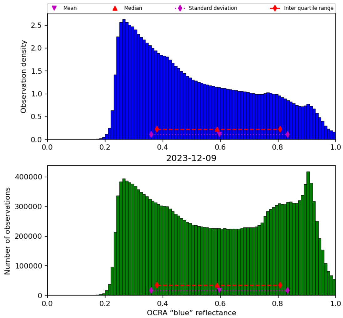
Figure 51: Histogram of “OCRA “blue” reflectance” for 2023-12-09 to 2023-12-10
