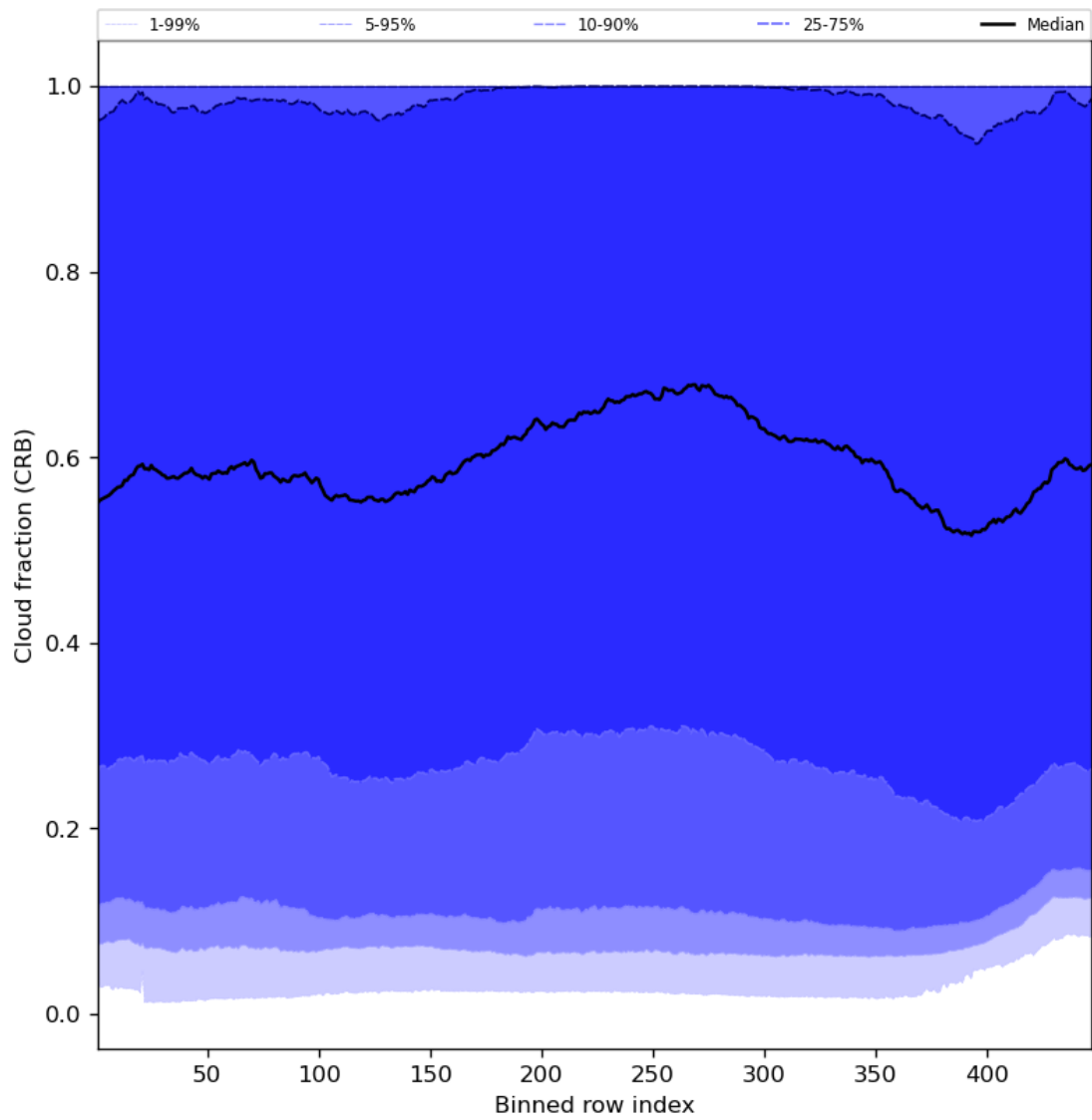
Figure 58: Along track statistics of “Cloud fraction (CRB)” for 2023-12-09 to 2023-12-10
