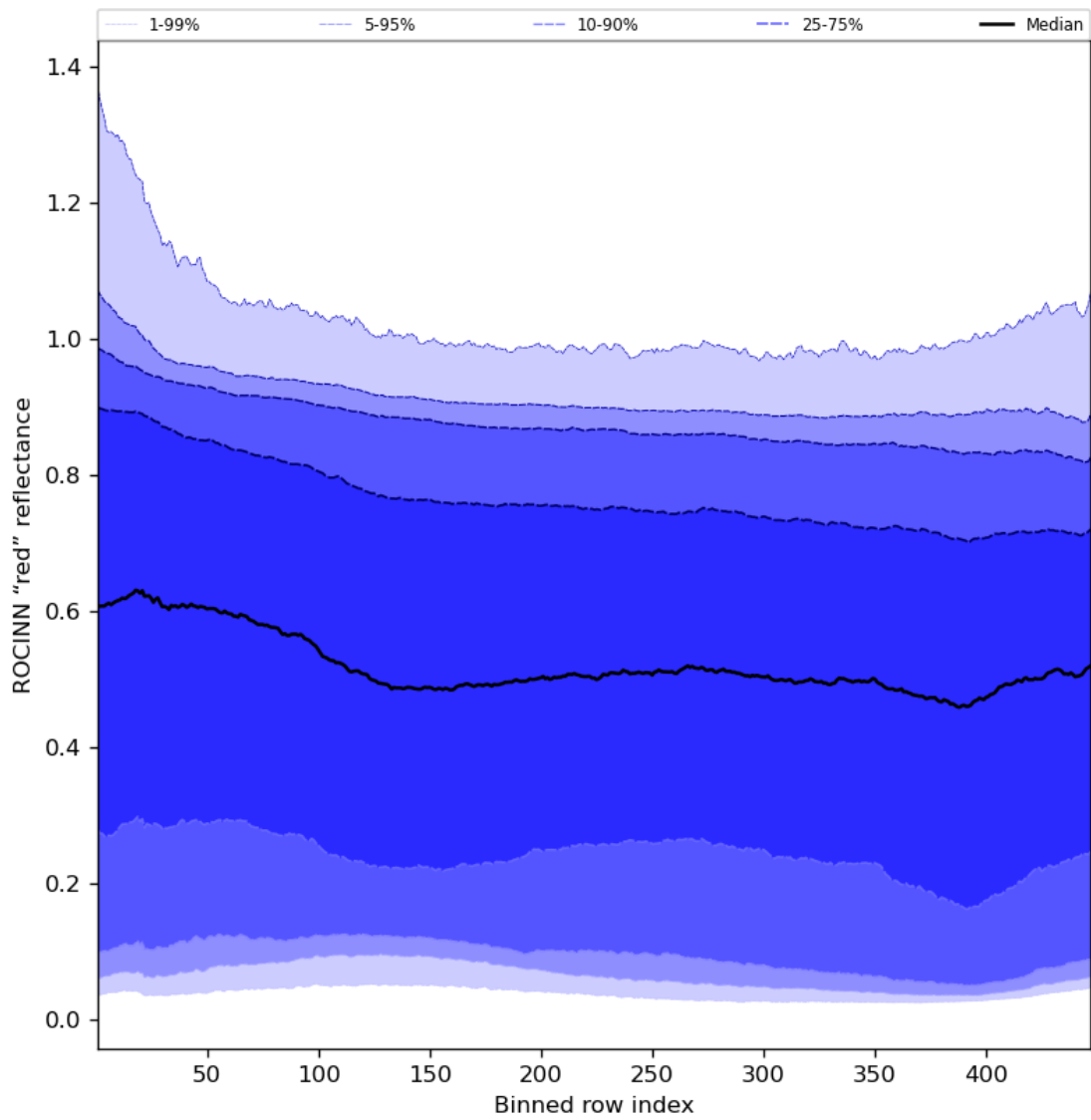
Figure 69: Along track statistics of “ROCINN “red” reflectance” for 2023-12-09 to 2023-12-10
