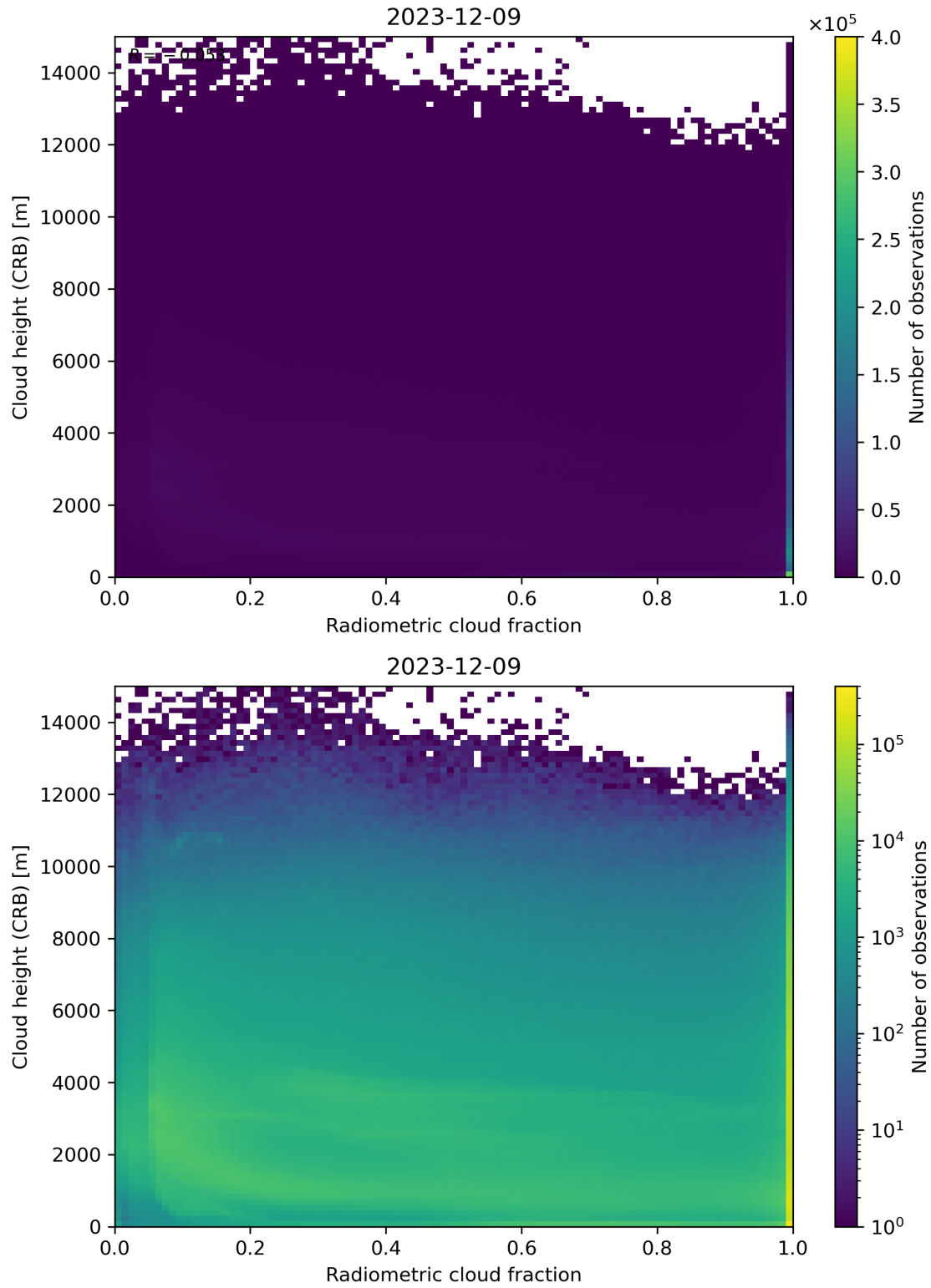
Figure 74: Scatter density plot of “Radiometric cloud fraction” against “Cloud height (CRB)” for 2023-12-09 to 2023-12-10.
