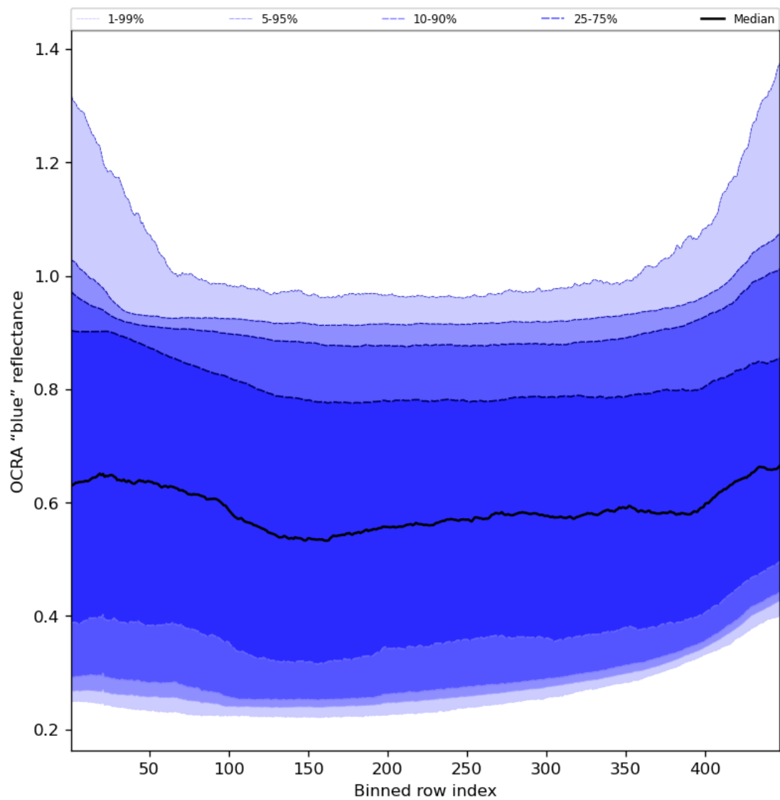
Figure 67: Along track statistics of “OCRA “blue” reflectance” for 2023-12-09 to 2023-12-10
