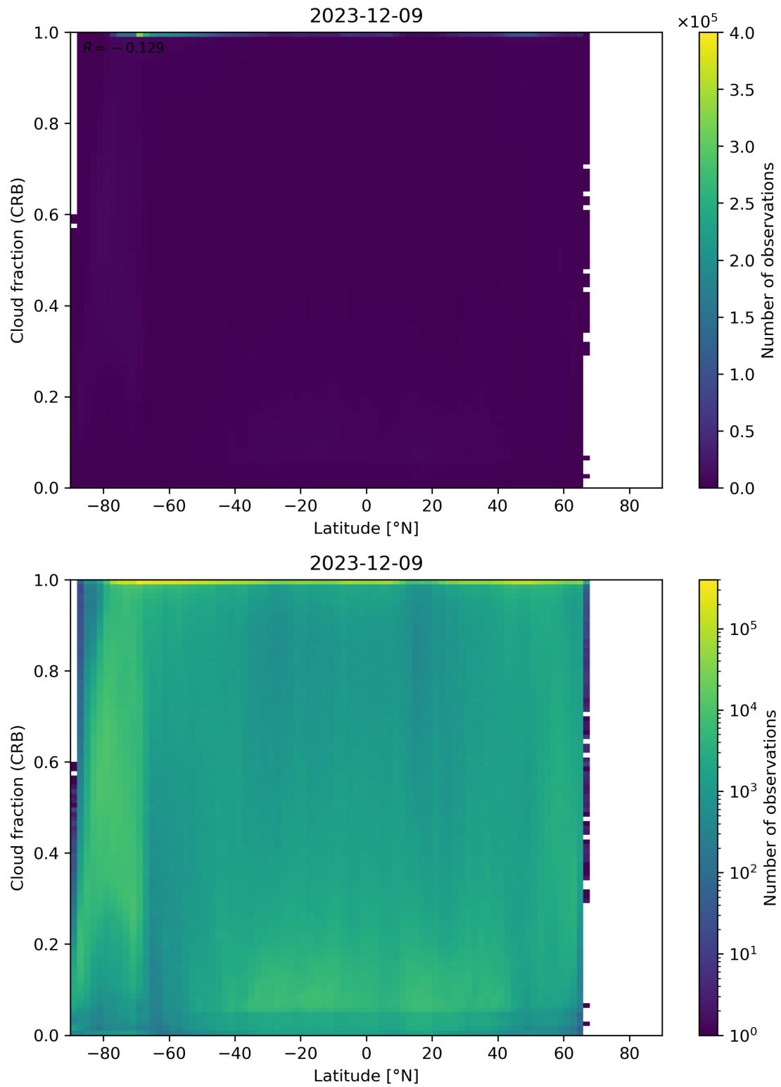
Figure 94: Scatter density plot of “Latitude” against “Cloud fraction (CRB)” for 2023-12-09 to 2023-12-10.
