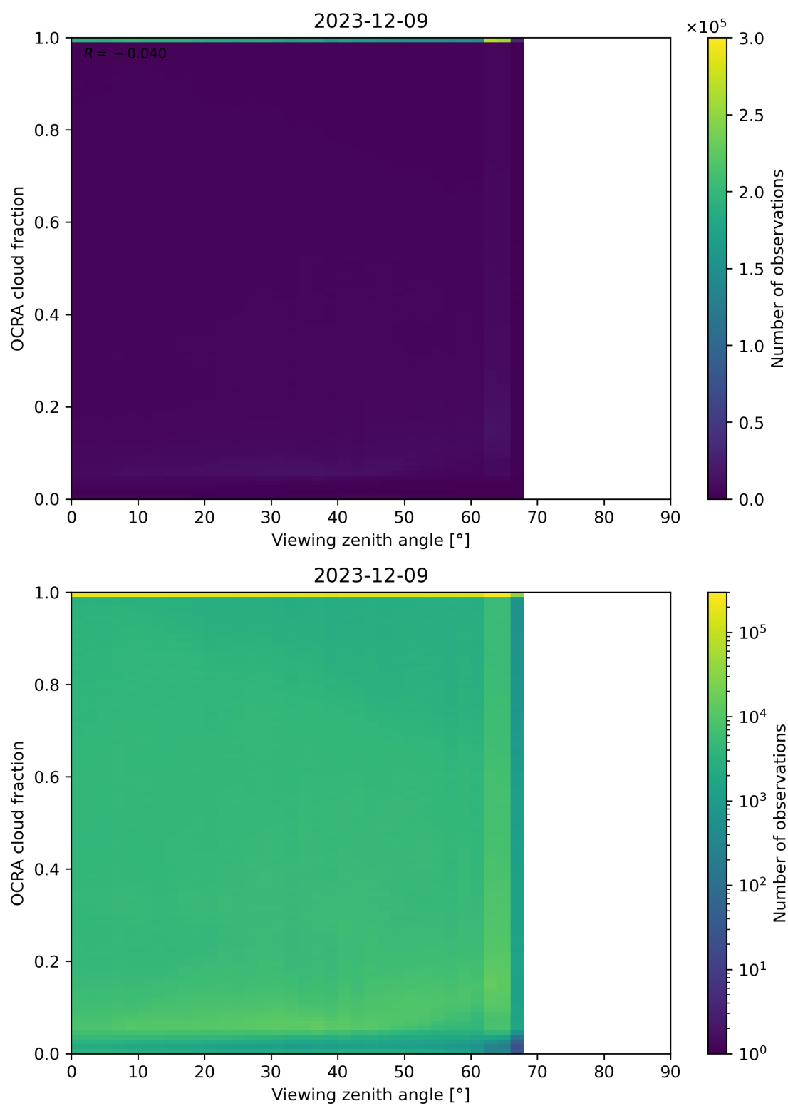
Figure 108: Scatter density plot of “Viewing zenith angle” against “OCRA cloud fraction” for 2023-12-09 to 2023-12-10.
