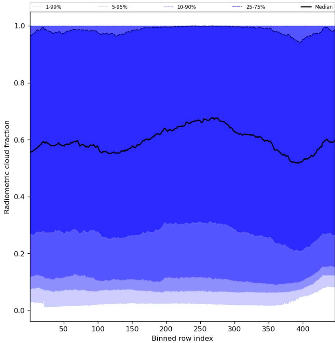
Figure 55: Along track statistics of “Radiometric cloud fraction” for 2023-12-09 to 2023-12-10
