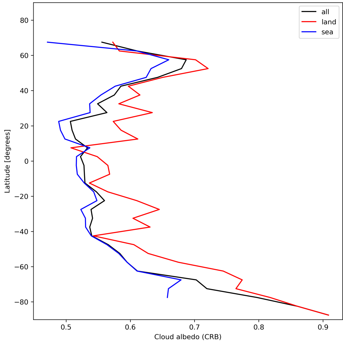
Figure 28: Zonal average of “Cloud albedo (CRB)” for 2023-12-09 to 2023-12-10.
