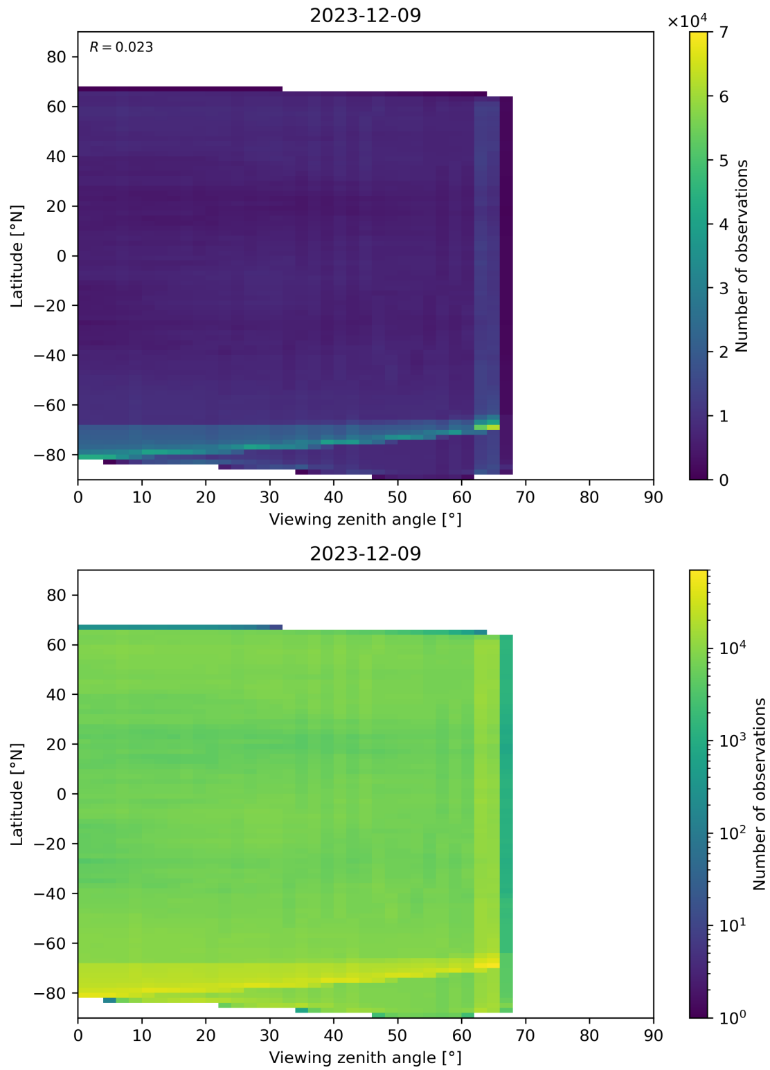
Figure 113: Scatter density plot of “Viewing zenith angle” against “Latitude” for 2023-12-09 to 2023-12-10.
