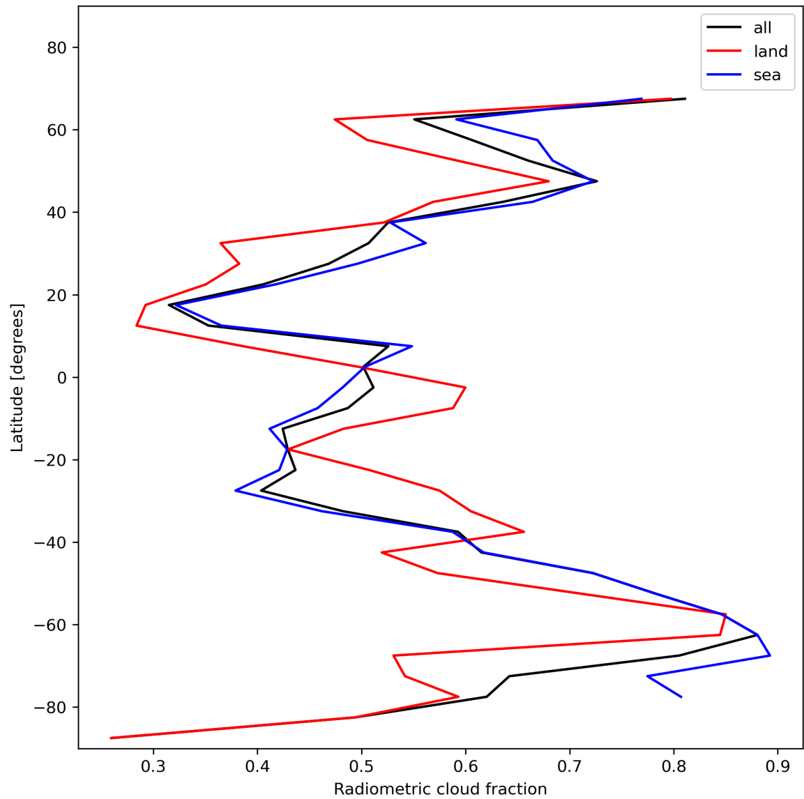
Figure 23: Zonal average of “Radiometric cloud fraction” for 2023-12-09 to 2023-12-10.
