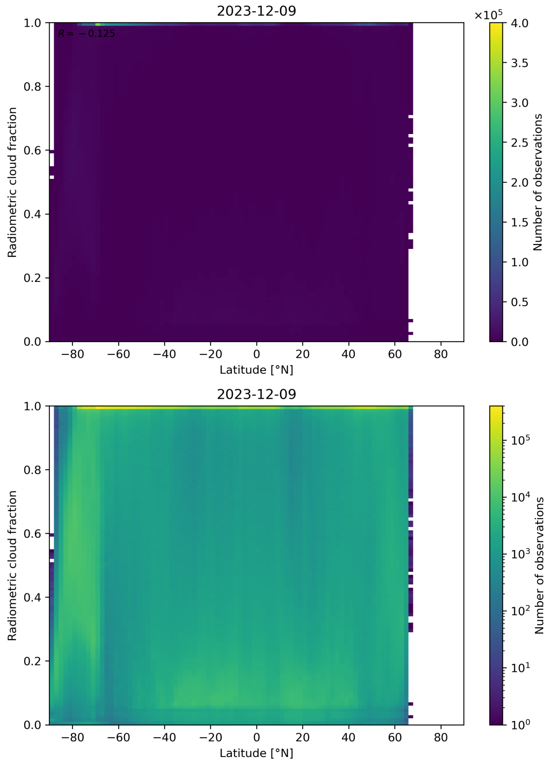
Figure 92: Scatter density plot of “Latitude” against “Radiometric cloud fraction” for 2023-12-09 to 2023-12-10.
