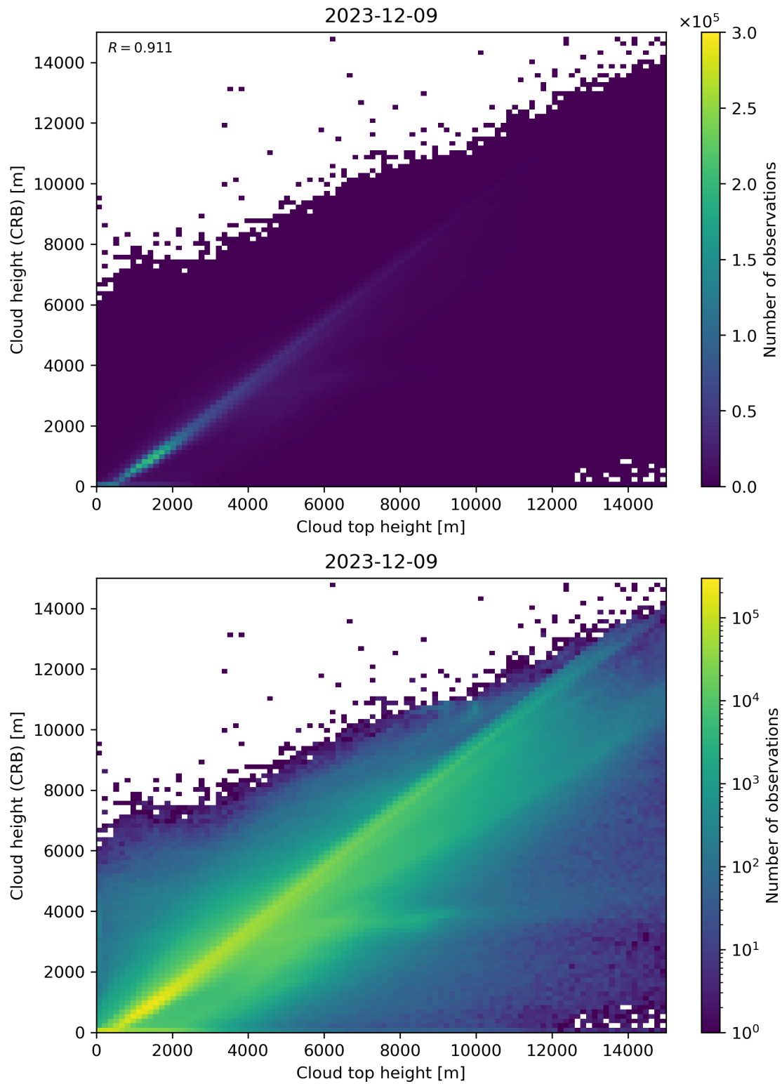
Figure 89: Scatter density plot of “Cloud top height” against “Cloud height (CRB)” for 2023-12-09 to 2023-12-10.
