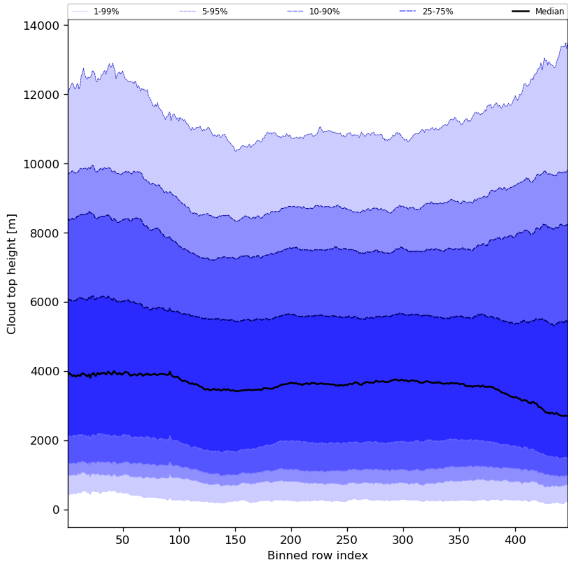
Figure 56: Along track statistics of “Cloud top height” for 2023-12-09 to 2023-12-10
