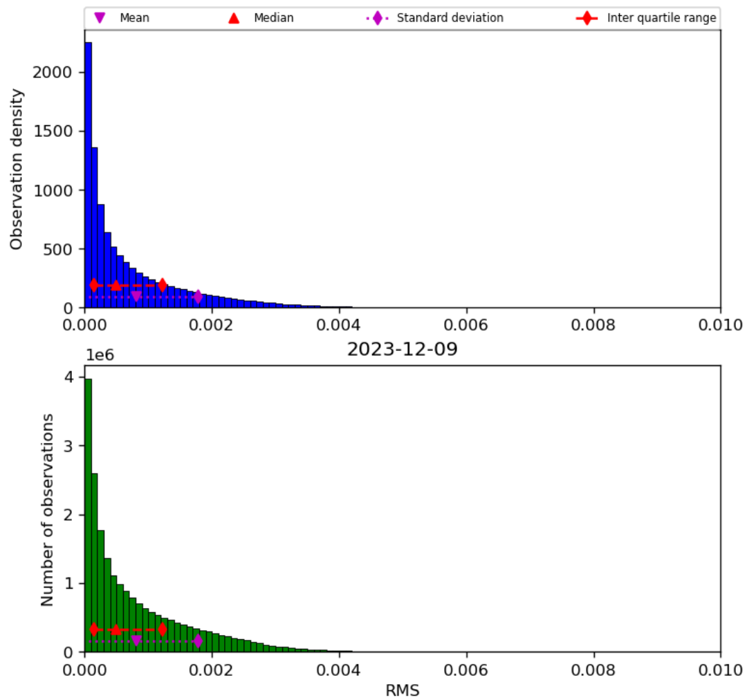
Figure 47: Histogram of “RMS” for 2023-12-09 to 2023-12-10
