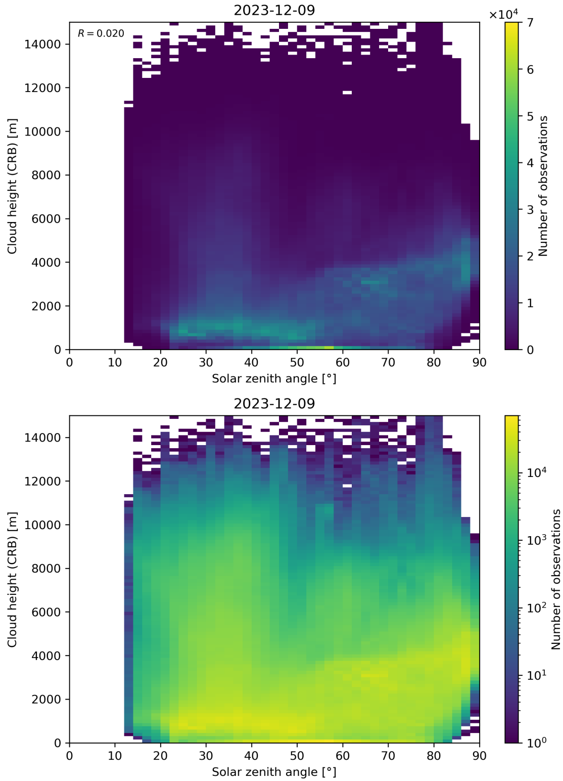
Figure 102: Scatter density plot of “Solar zenith angle” against “Cloud height (CRB)” for 2023-12-09 to 2023-12-10.
