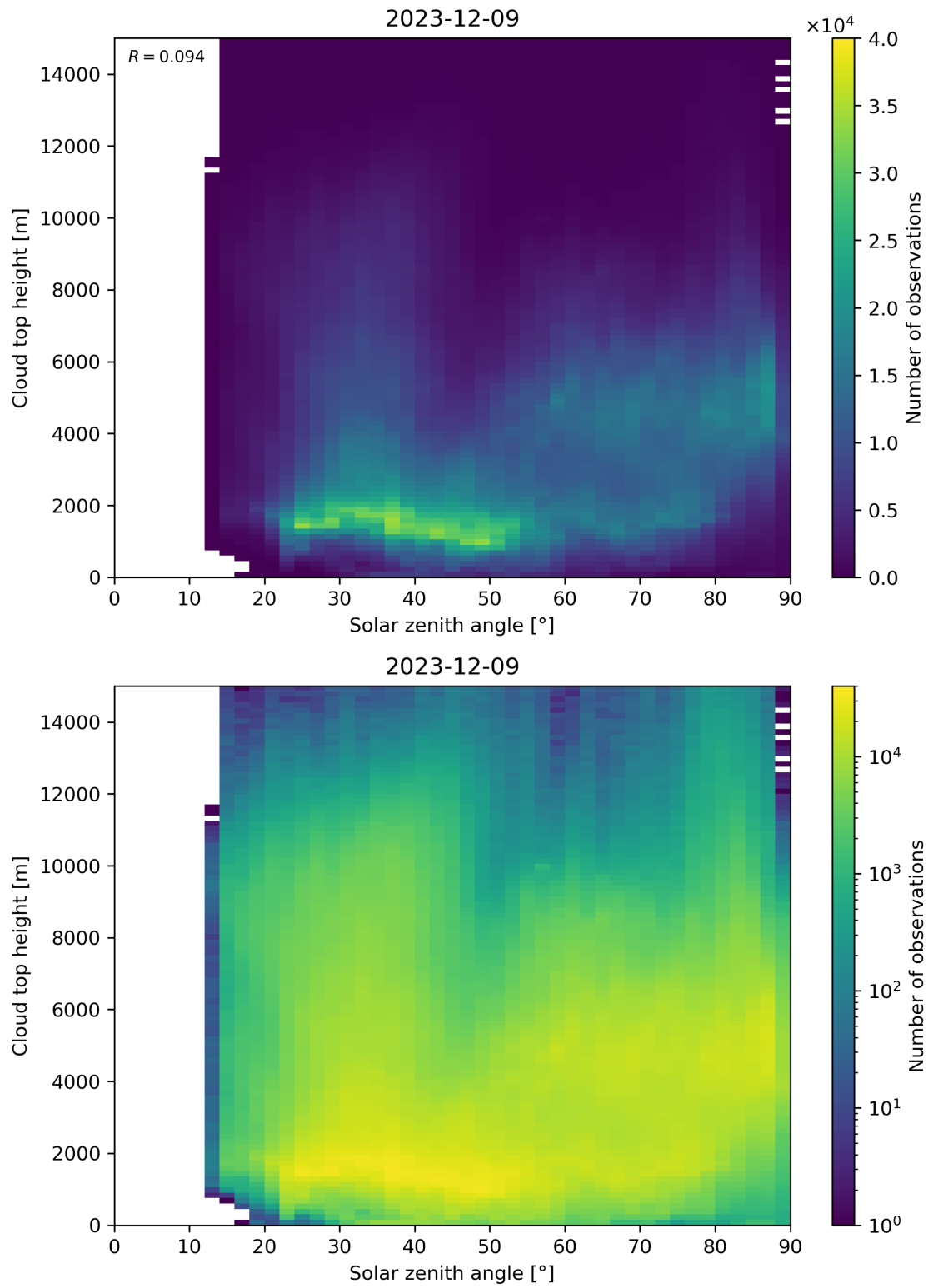
Figure 104: Scatter density plot of “Solar zenith angle” against “Cloud top height” for 2023-12-09 to 2023-12-10.
