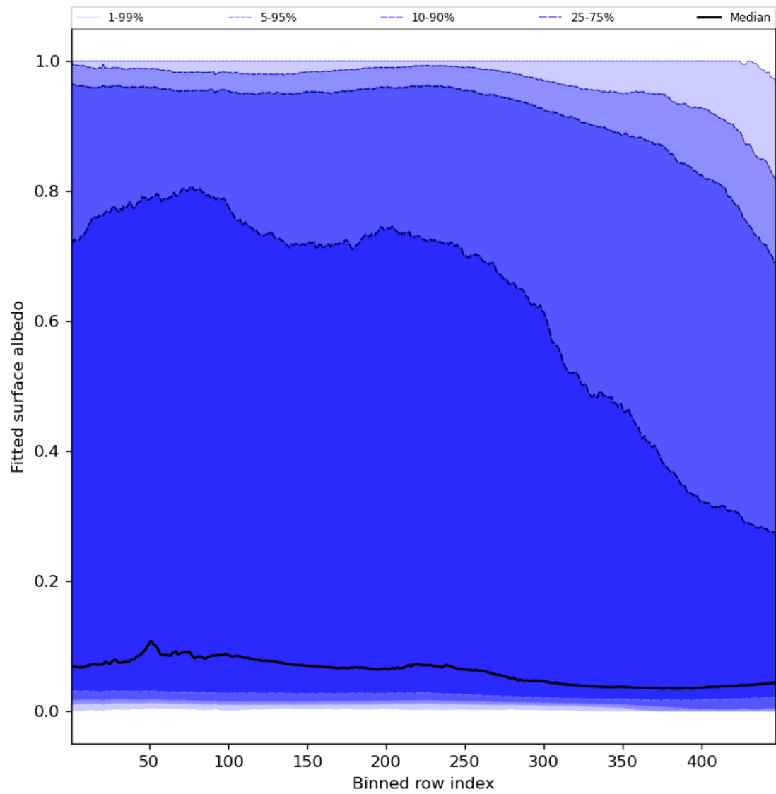
Figure 61: Along track statistics of “Fitted surface albedo” for 2023-12-09 to 2023-12-10
