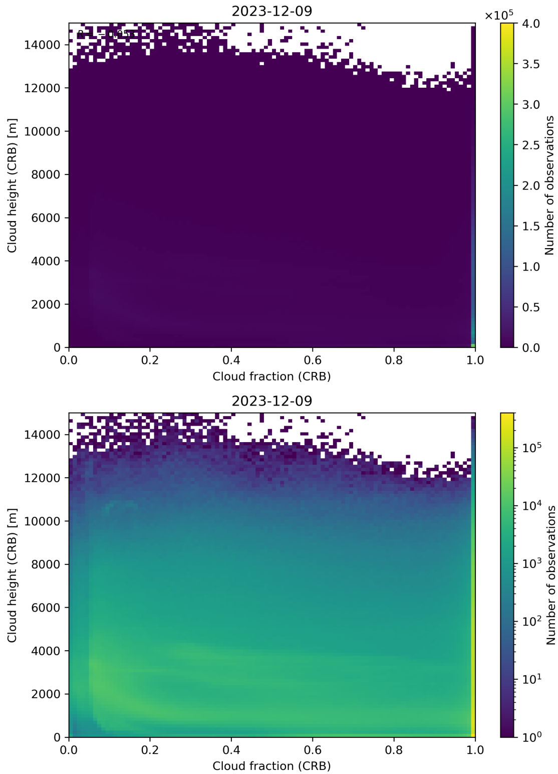
Figure 79: Scatter density plot of “Cloud fraction (CRB)” against “Cloud height (CRB)” for 2023-12-09 to 2023-12-10.
