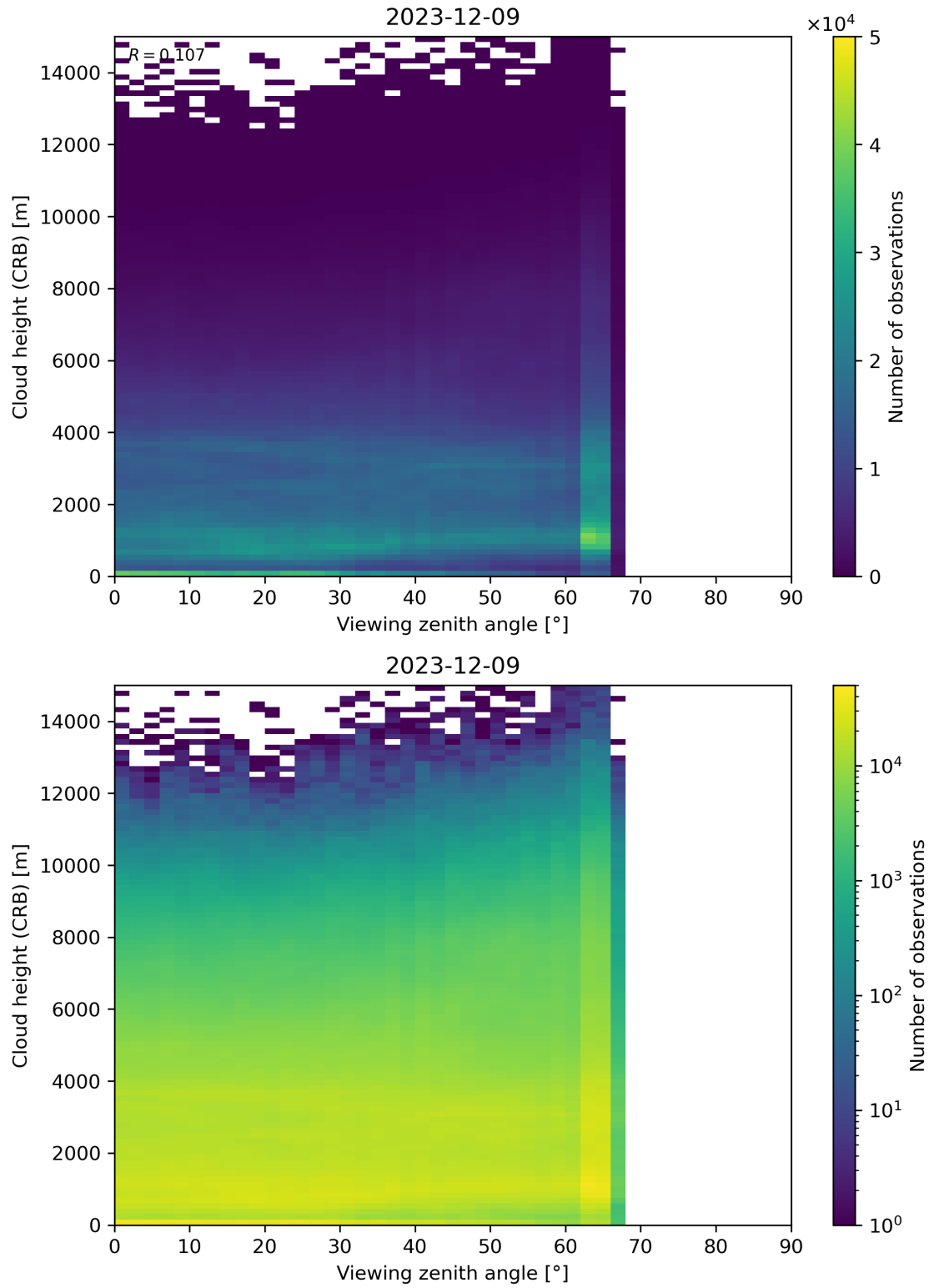
Figure 110: Scatter density plot of “Viewing zenith angle” against “Cloud height (CRB)” for 2023-12-09 to 2023-12-10.
