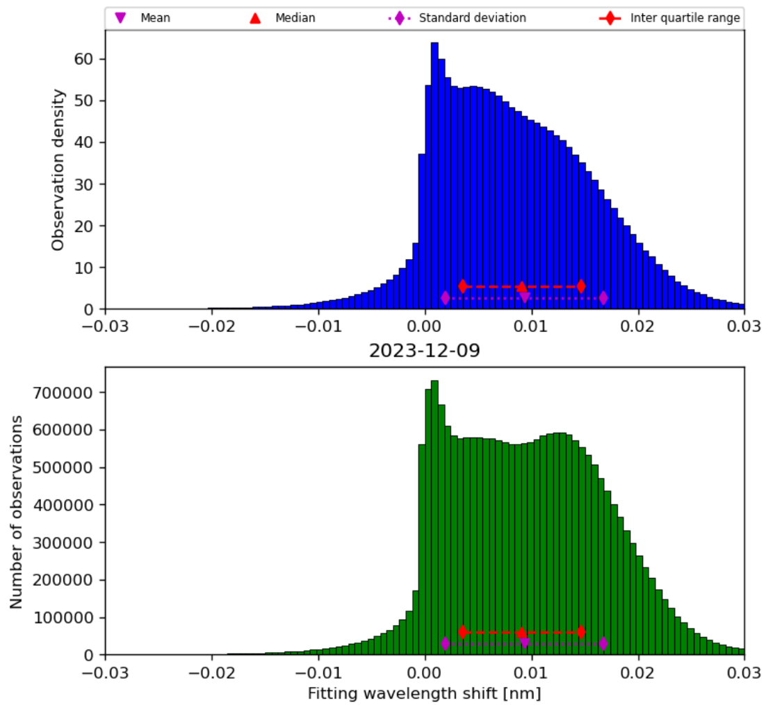
Figure 49: Histogram of “Fitting wavelength shift” for 2023-12-09 to 2023-12-10
