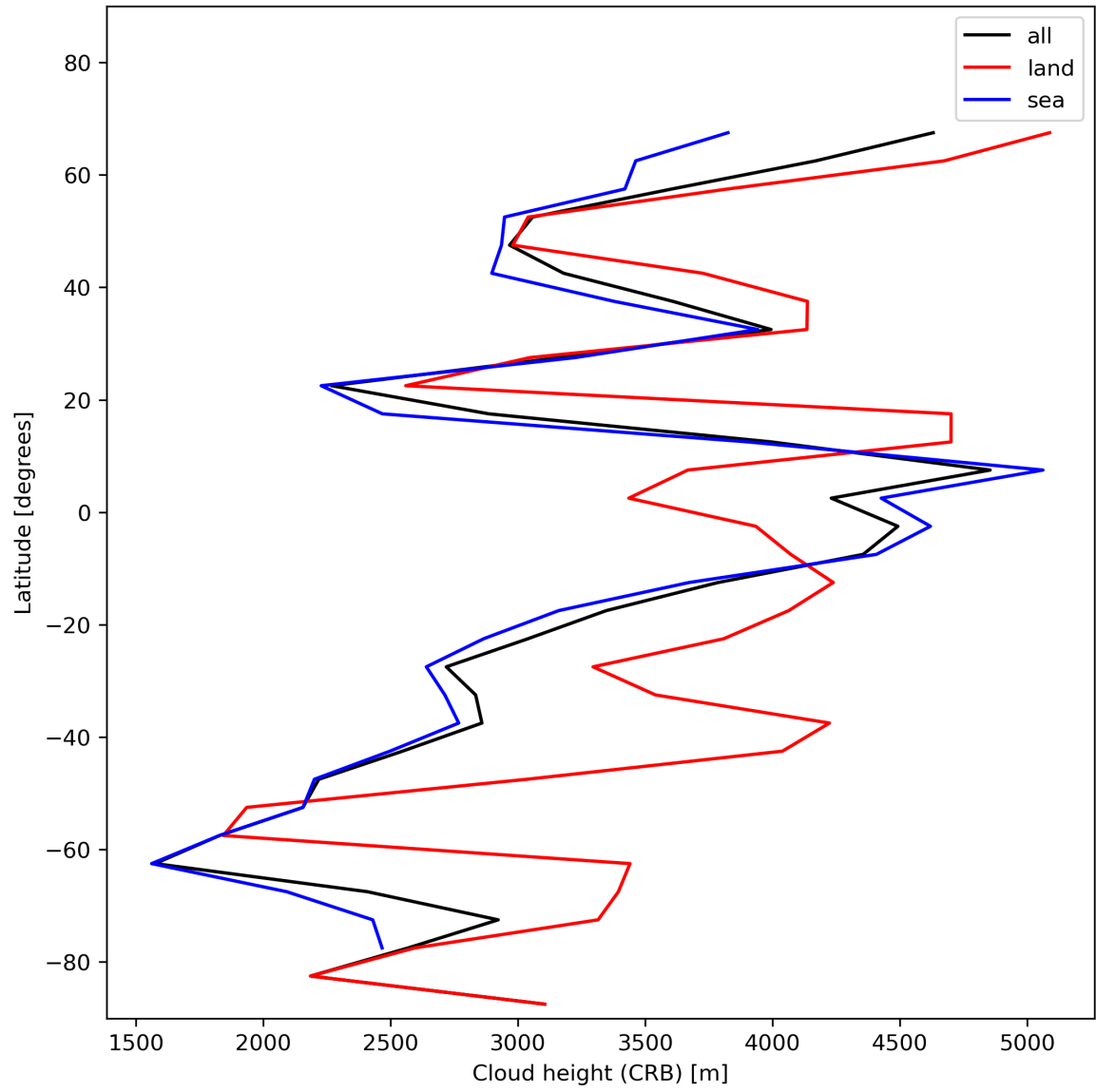
Figure 27: Zonal average of “Cloud height (CRB)” for 2023-12-09 to 2023-12-10.
