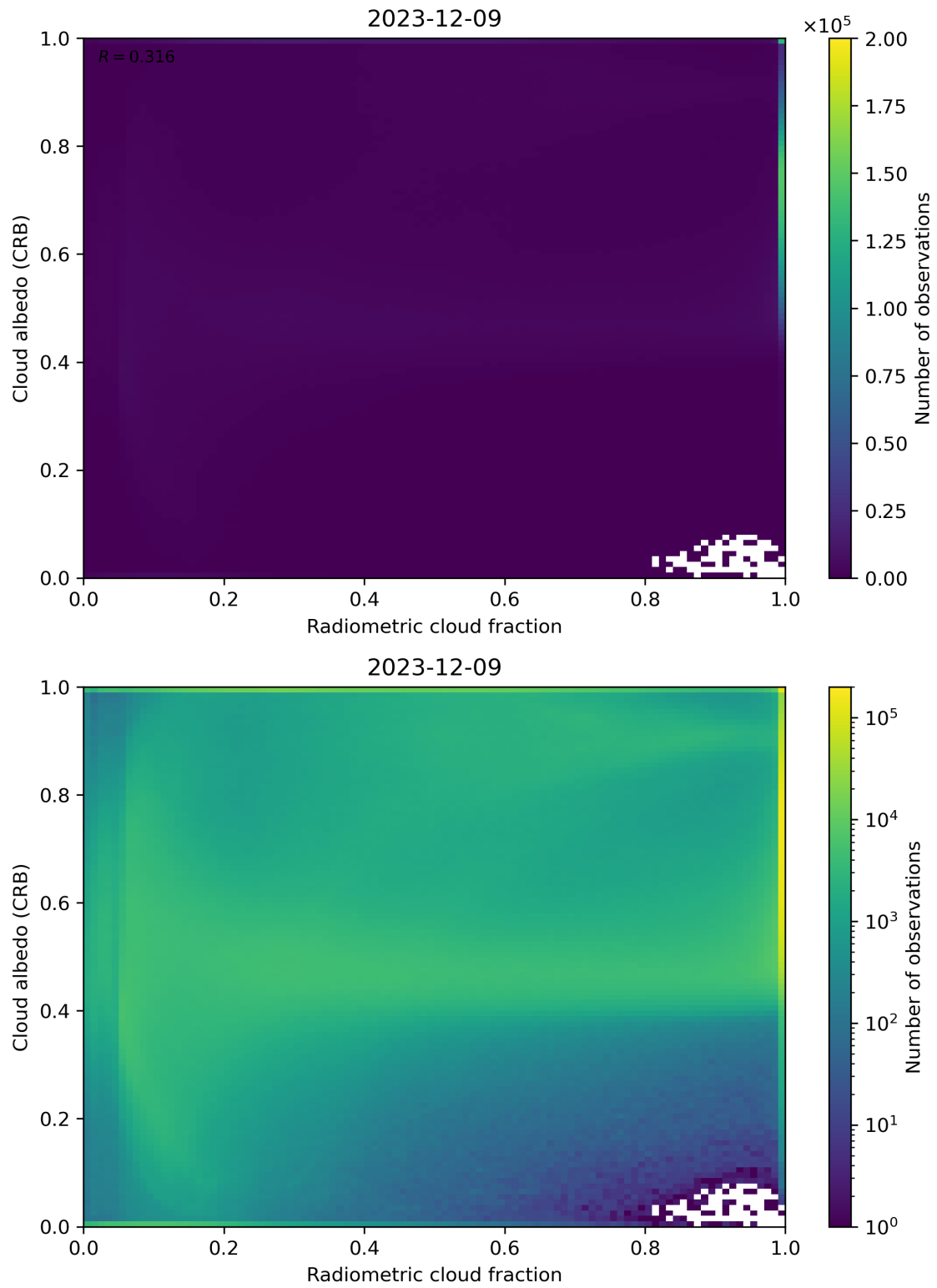
Figure 71: Scatter density plot of “Radiometric cloud fraction” against “Cloud albedo (CRB)” for 2023-12-09 to 2023-12-10.
