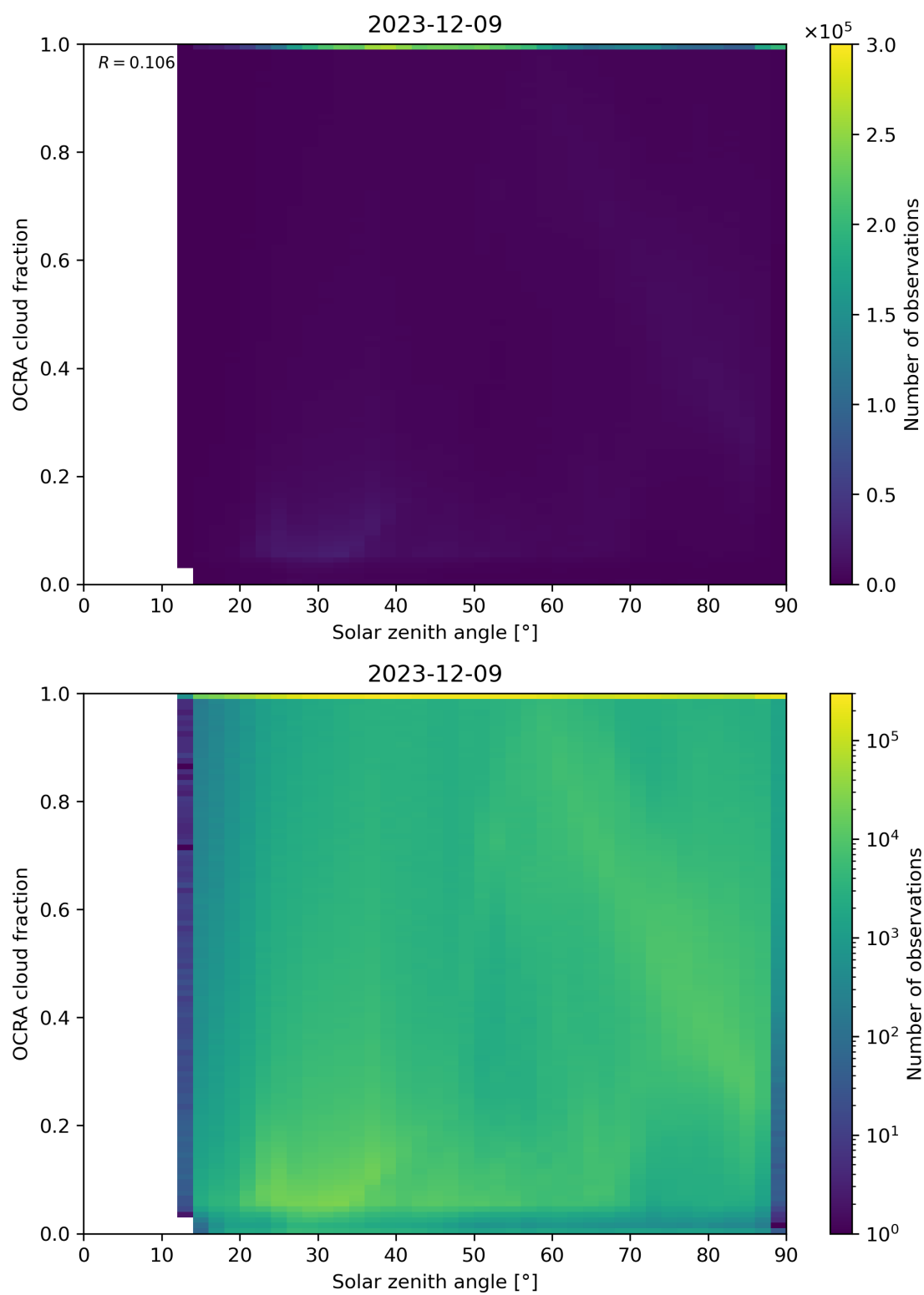
Figure 100: Scatter density plot of “Solar zenith angle” against “OCRA cloud fraction” for 2023-12-09 to 2023-12-10.
