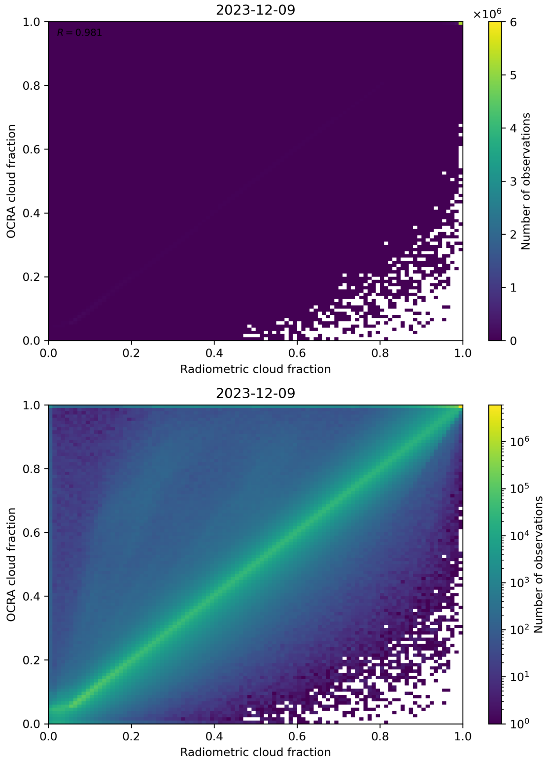
Figure 72: Scatter density plot of “Radiometric cloud fraction” against “OCRA cloud fraction” for 2023-12-09 to 2023-12-10.
