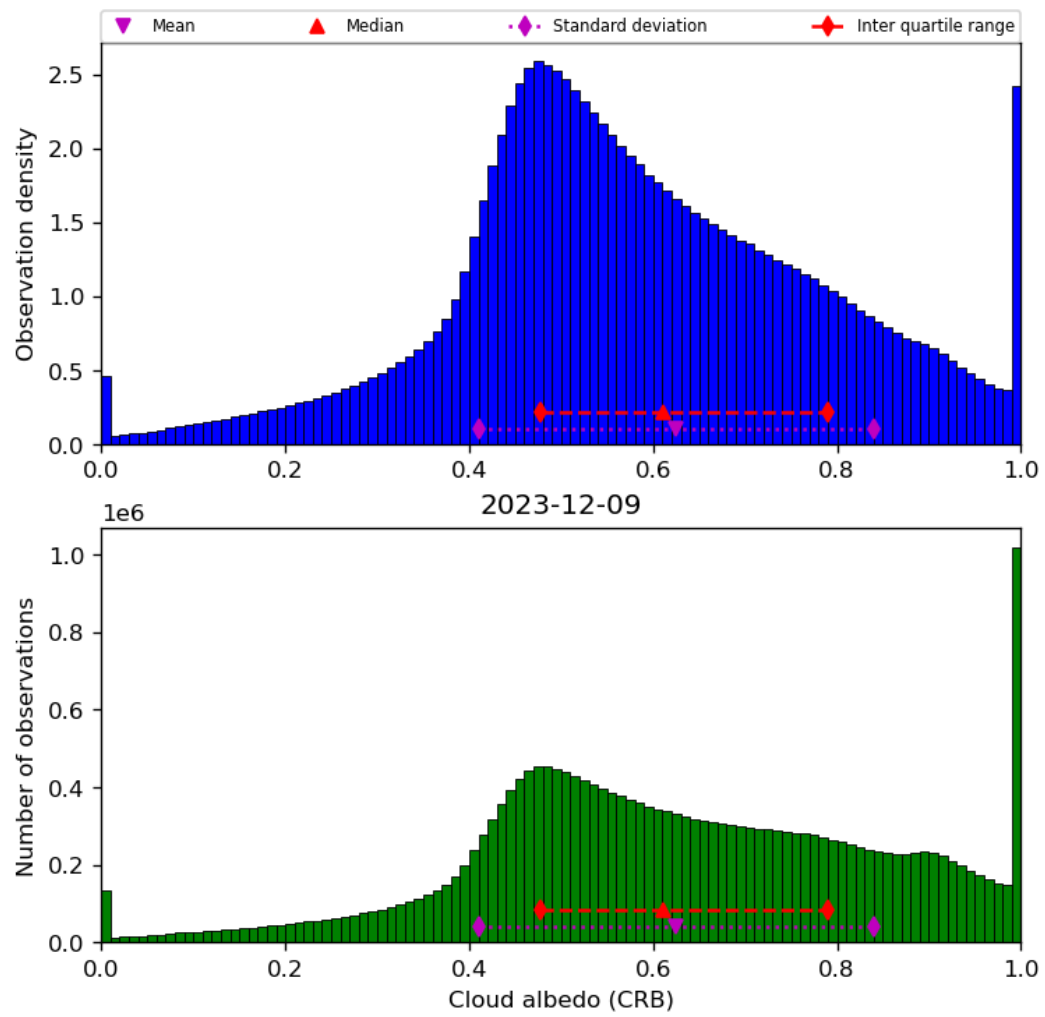
Figure 44: Histogram of “Cloud albedo (CRB)” for 2023-12-09 to 2023-12-10
