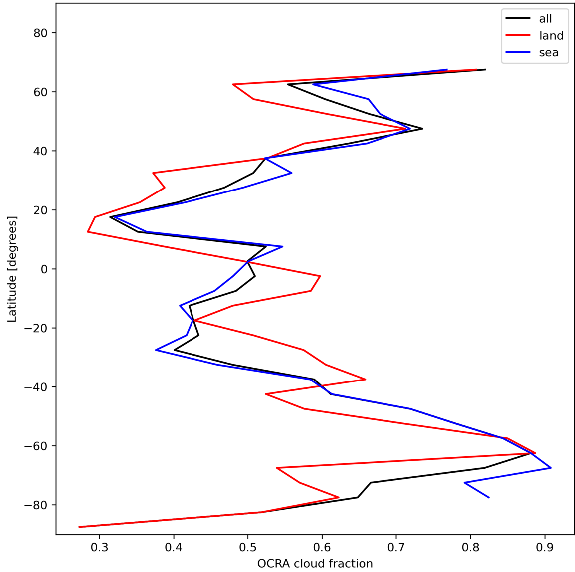
Figure 34: Zonal average of “OCRA cloud fraction” for 2023-12-09 to 2023-12-10.
