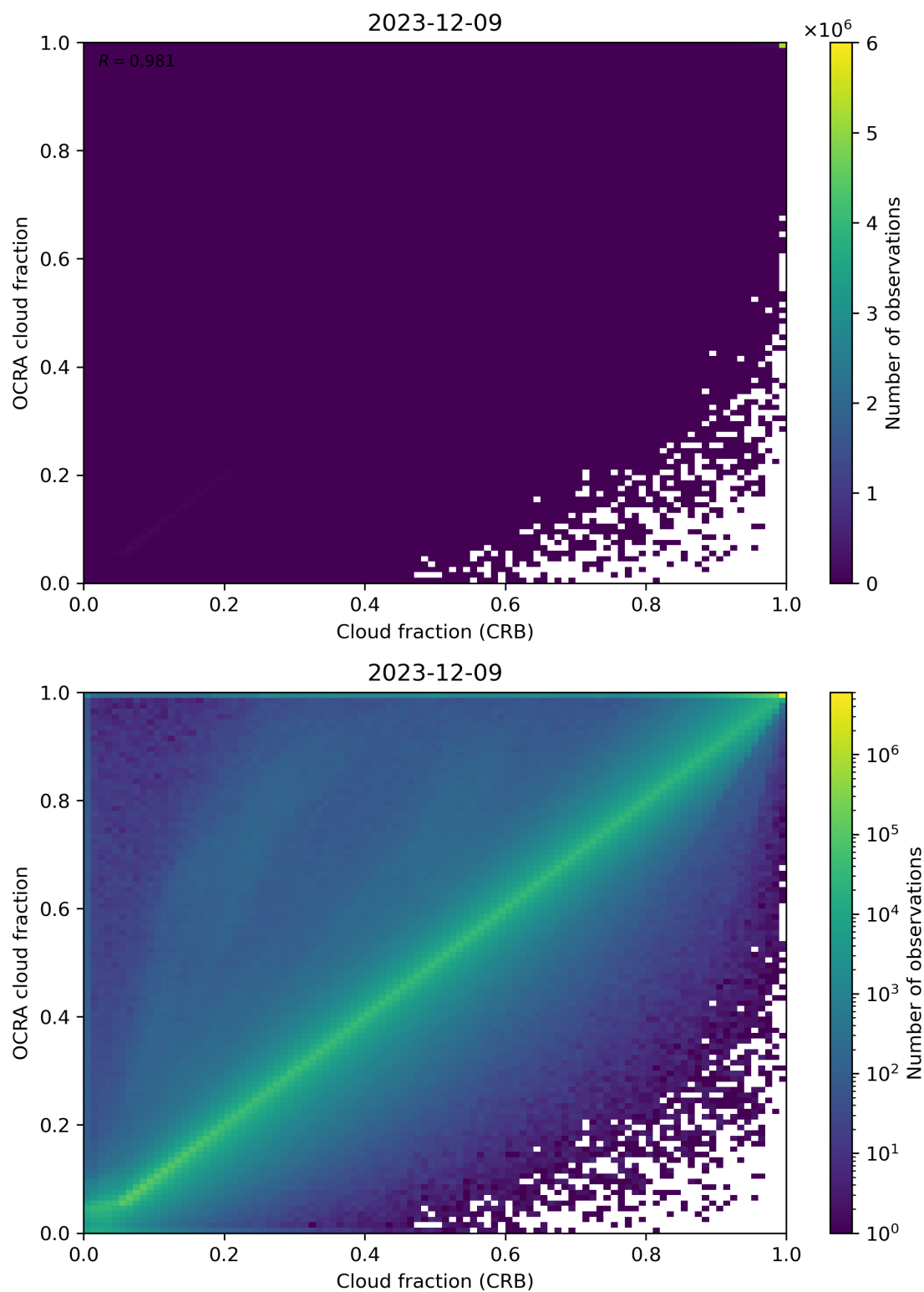
Figure 78: Scatter density plot of “Cloud fraction (CRB)” against “OCRA cloud fraction” for 2023-12-09 to 2023-12-10.
