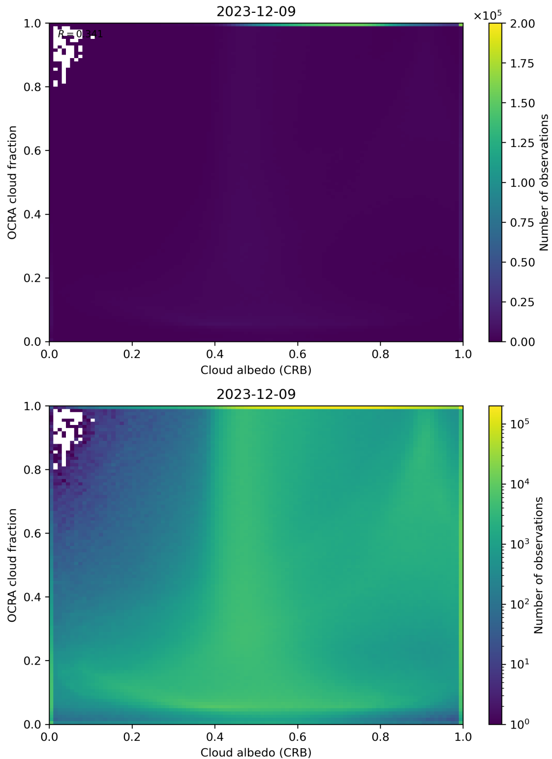
Figure 70: Scatter density plot of “Cloud albedo (CRB)” against “OCRA cloud fraction” for 2023-12-09 to 2023-12-10.
