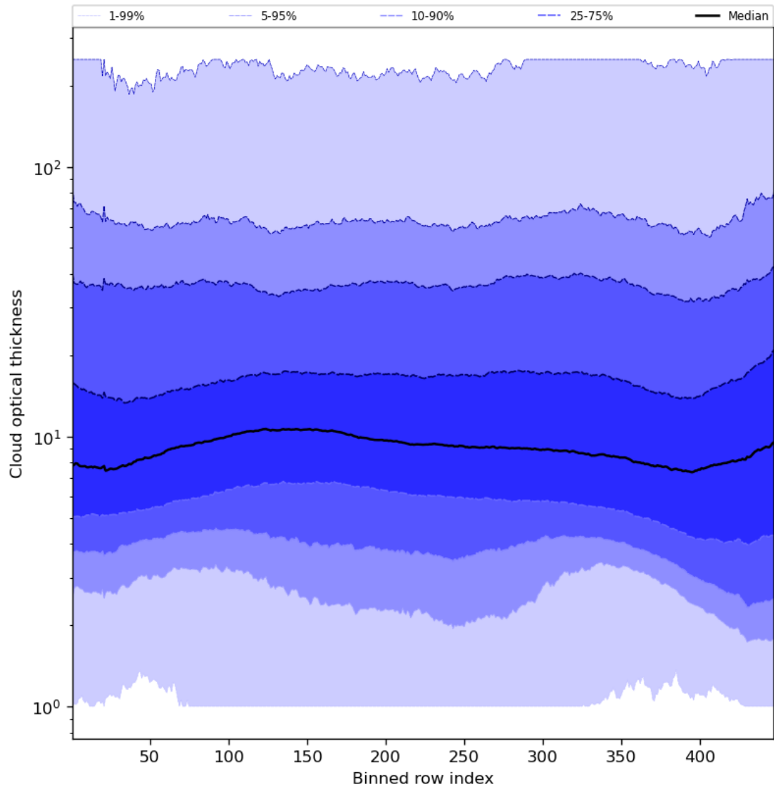
Figure 57: Along track statistics of “Cloud optical thickness” for 2023-12-09 to 2023-12-10
