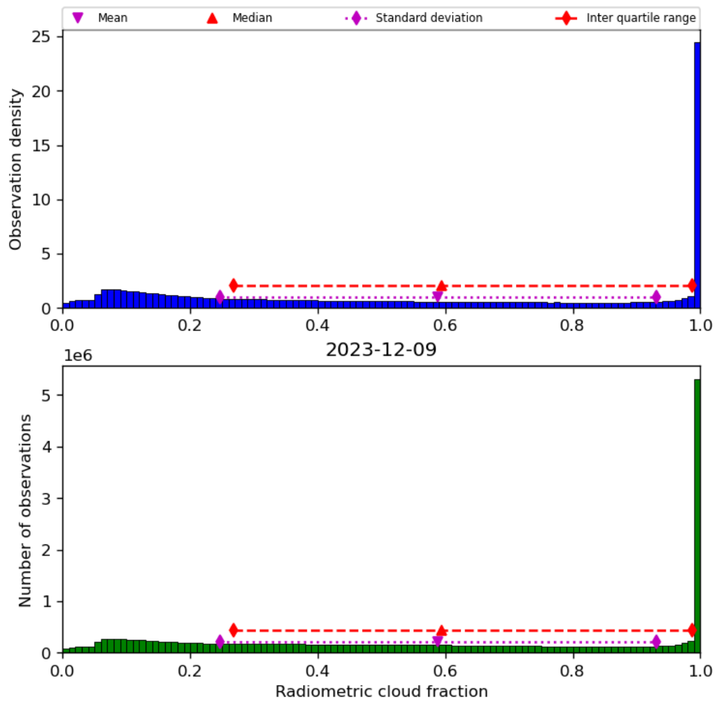
Figure 39: Histogram of “Radiometric cloud fraction” for 2023-12-09 to 2023-12-10
