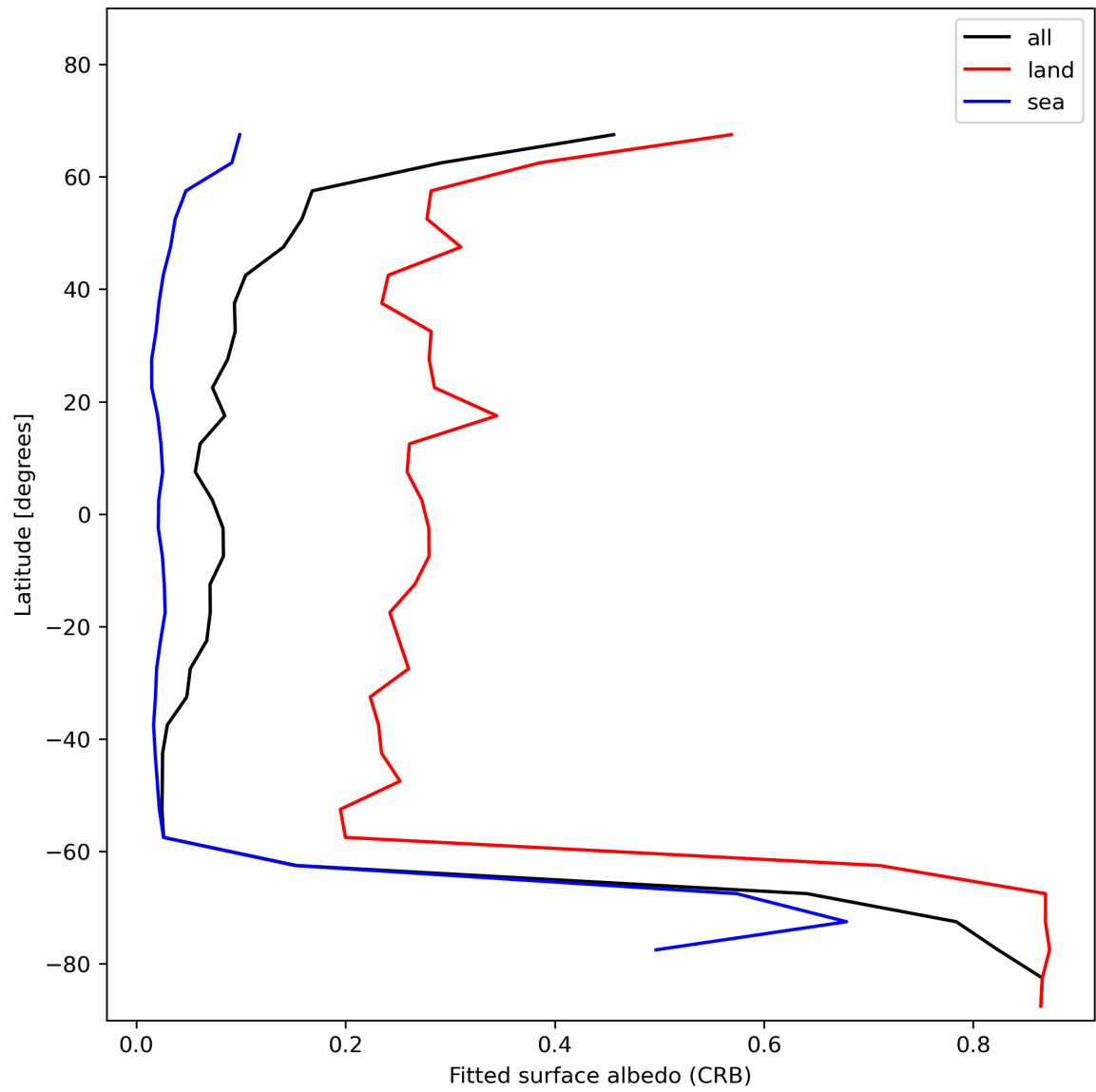
Figure 30: Zonal average of “Fitted surface albedo (CRB)” for 2023-12-09 to 2023-12-10.
