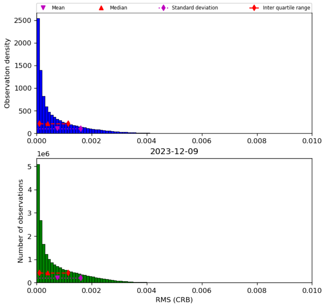
Figure 48: Histogram of “RMS (CRB)” for 2023-12-09 to 2023-12-10
