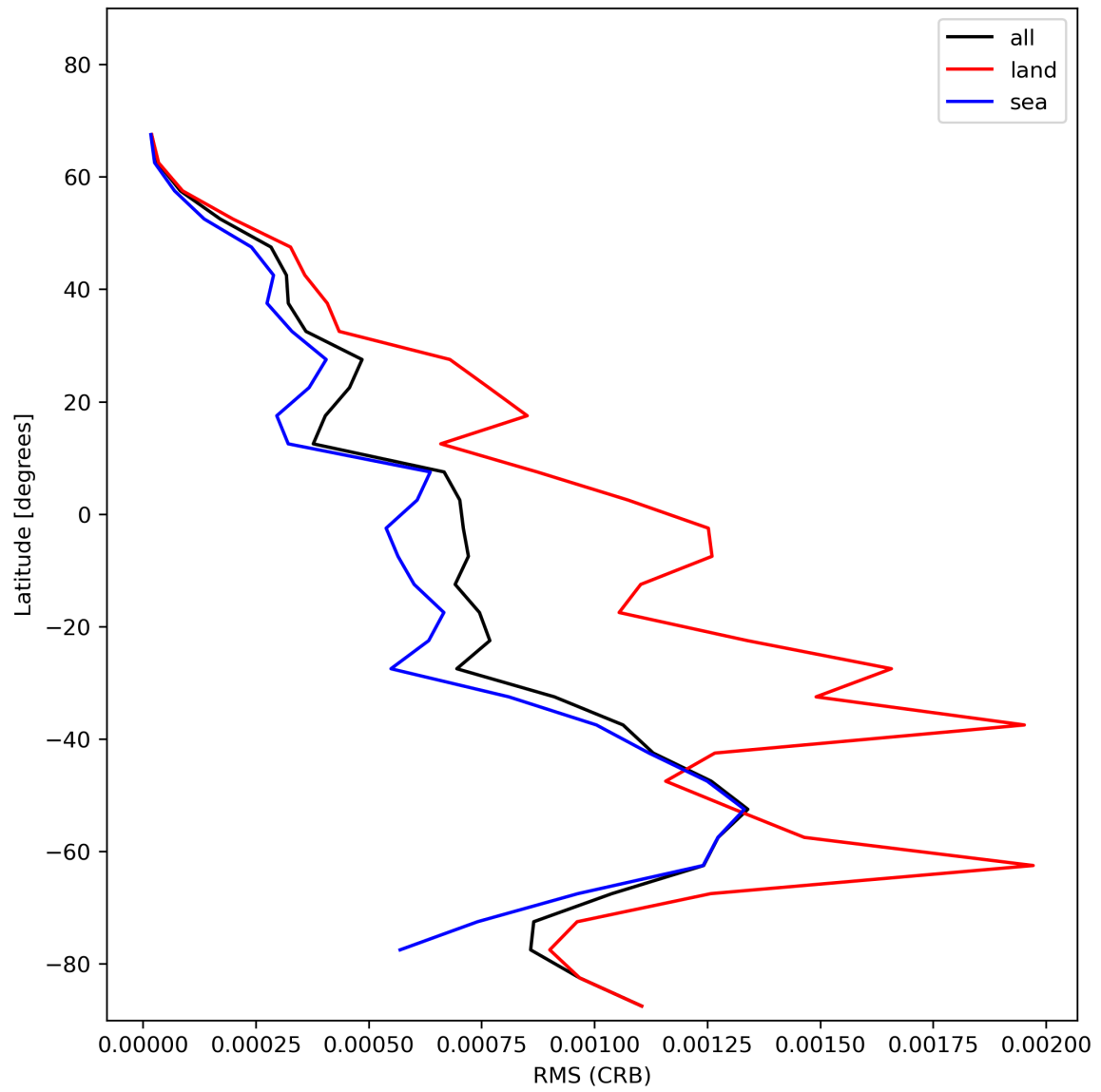
Figure 32: Zonal average of “RMS (CRB)” for 2023-12-09 to 2023-12-10.
