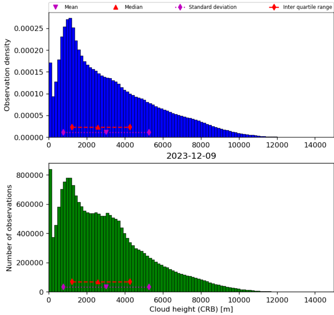
Figure 43: Histogram of “Cloud height (CRB)” for 2023-12-09 to 2023-12-10
