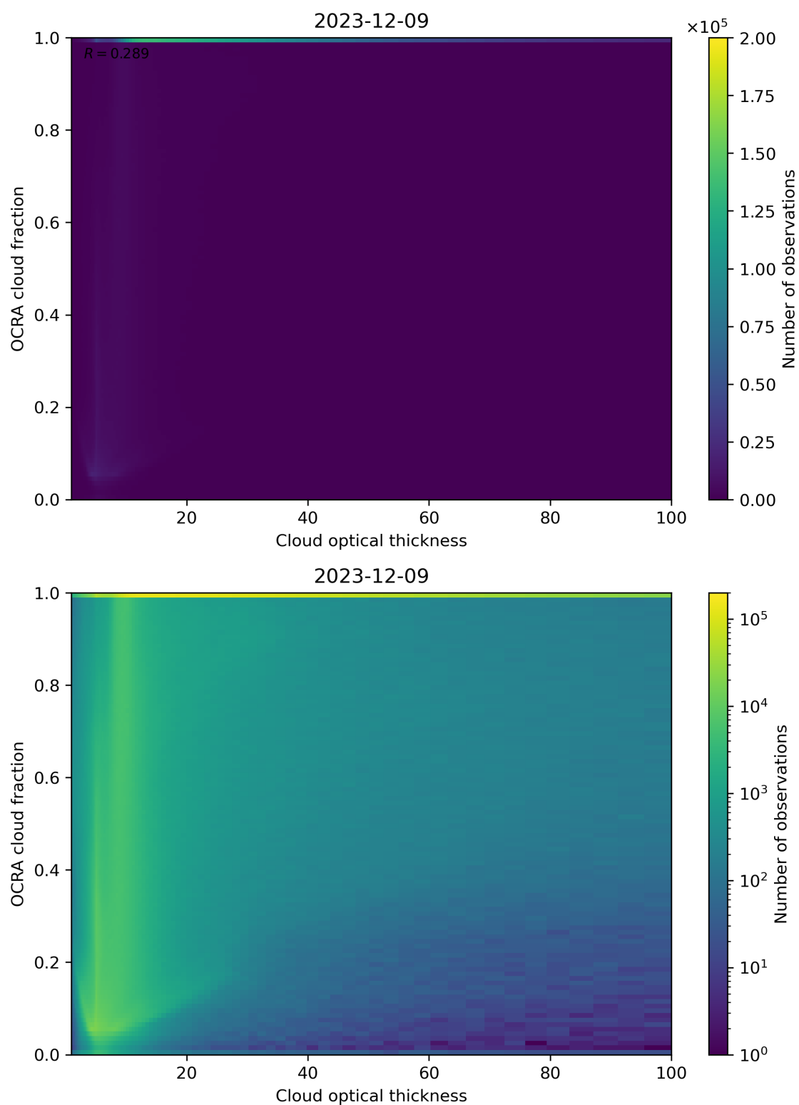
Figure 83: Scatter density plot of “Cloud optical thickness” against “OCRA cloud fraction” for 2023-12-09 to 2023-12-10.
