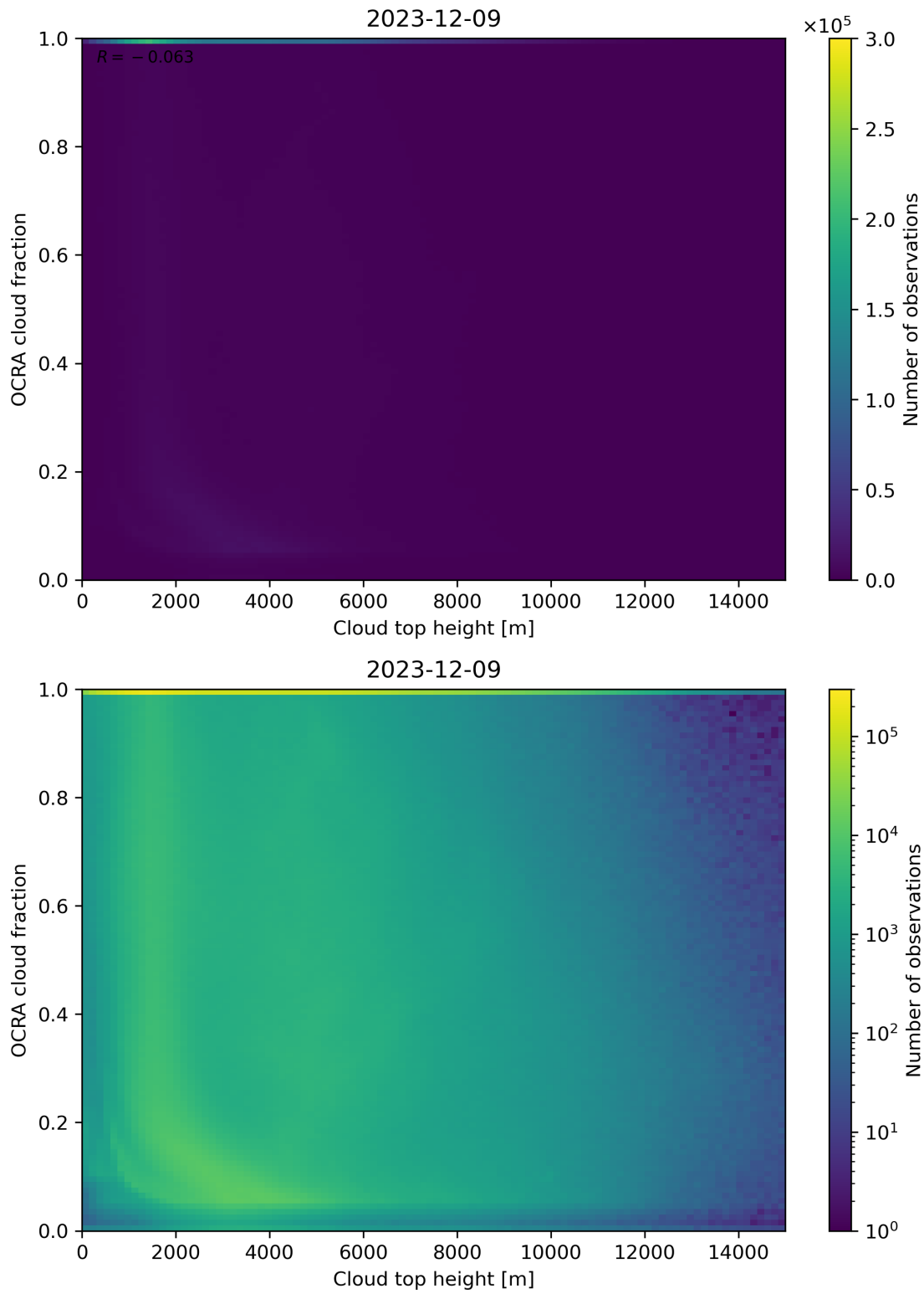
Figure 87: Scatter density plot of “Cloud top height” against “OCRA cloud fraction” for 2023-12-09 to 2023-12-10.
