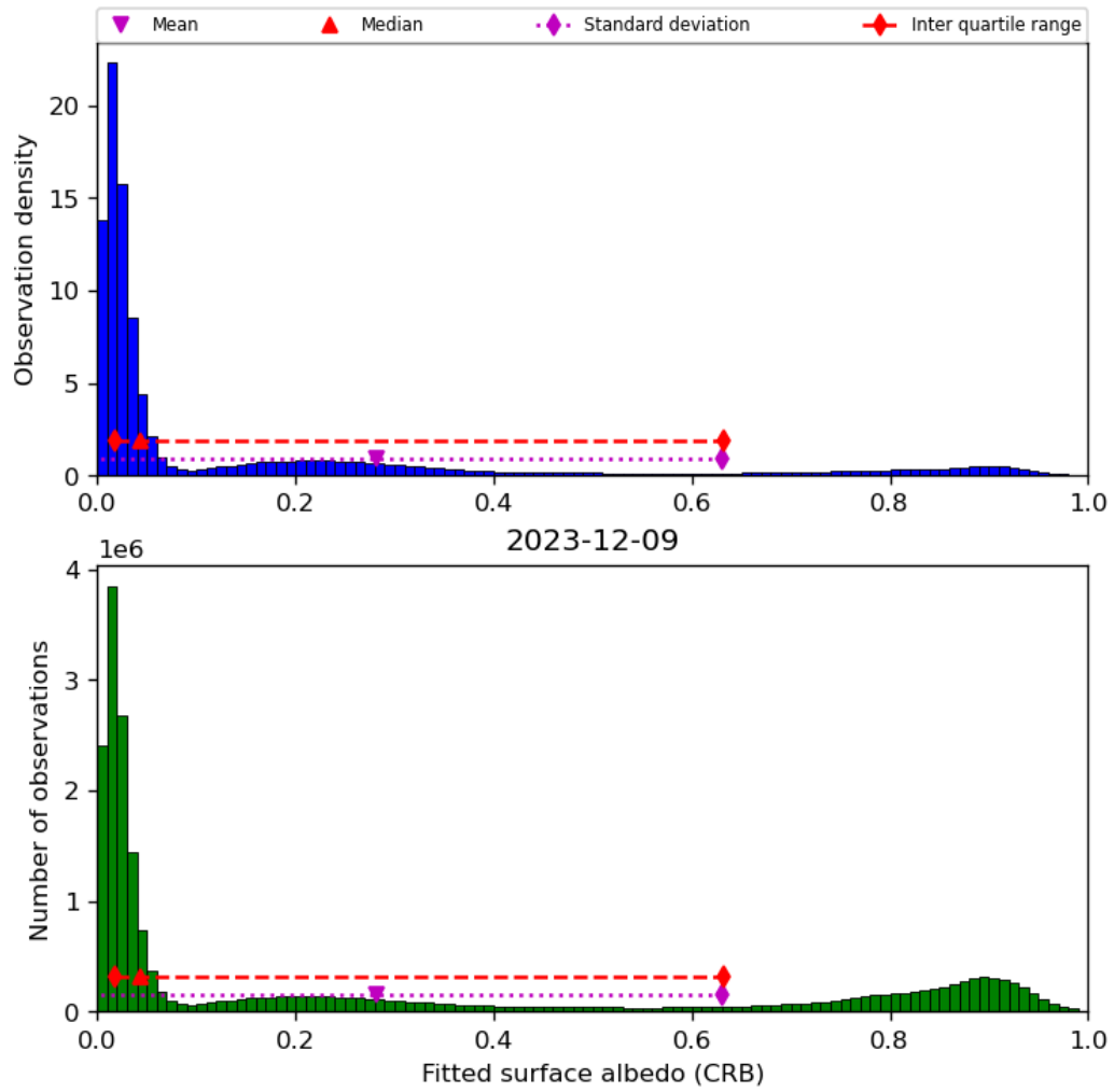
Figure 46: Histogram of “Fitted surface albedo (CRB)” for 2023-12-09 to 2023-12-10
