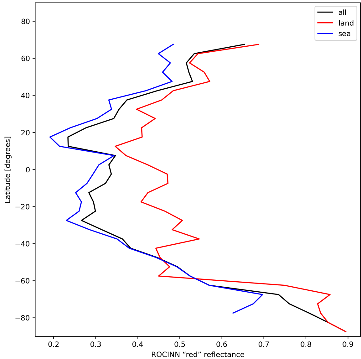
Figure 37: Zonal average of “ROCINN “red” reflectance” for 2023-12-09 to 2023-12-10.
