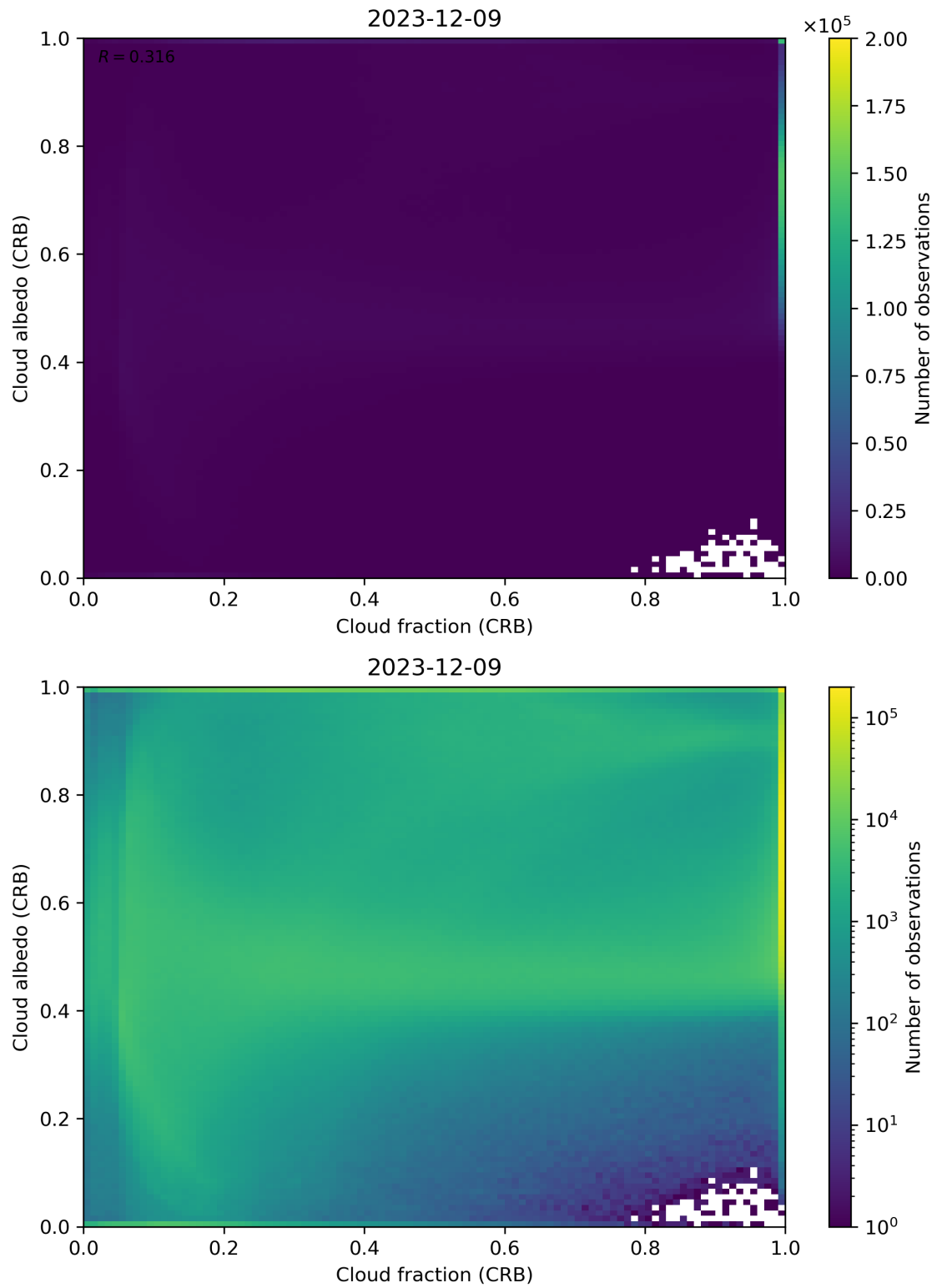
Figure 77: Scatter density plot of “Cloud fraction (CRB)” against “Cloud albedo (CRB)” for 2023-12-09 to 2023-12-10.
