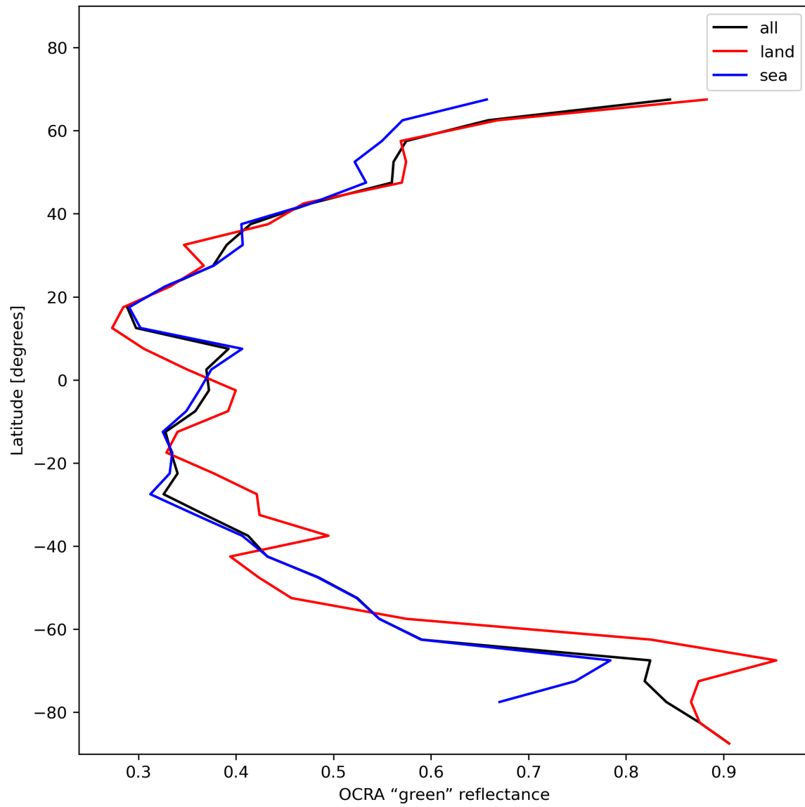
Figure 36: Zonal average of “OCRA “green” reflectance” for 2023-12-09 to 2023-12-10.
