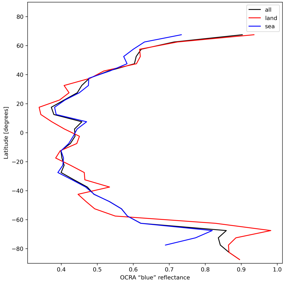
Figure 35: Zonal average of “OCRA “blue” reflectance” for 2023-12-09 to 2023-12-10.
