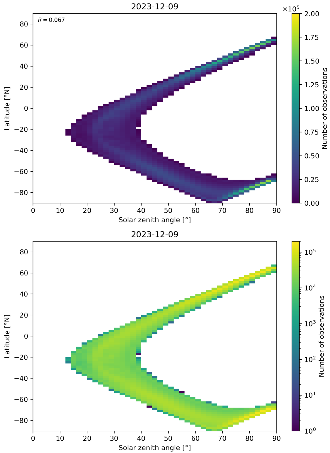
Figure 105: Scatter density plot of “Solar zenith angle” against “Latitude” for 2023-12-09 to 2023-12-10.
