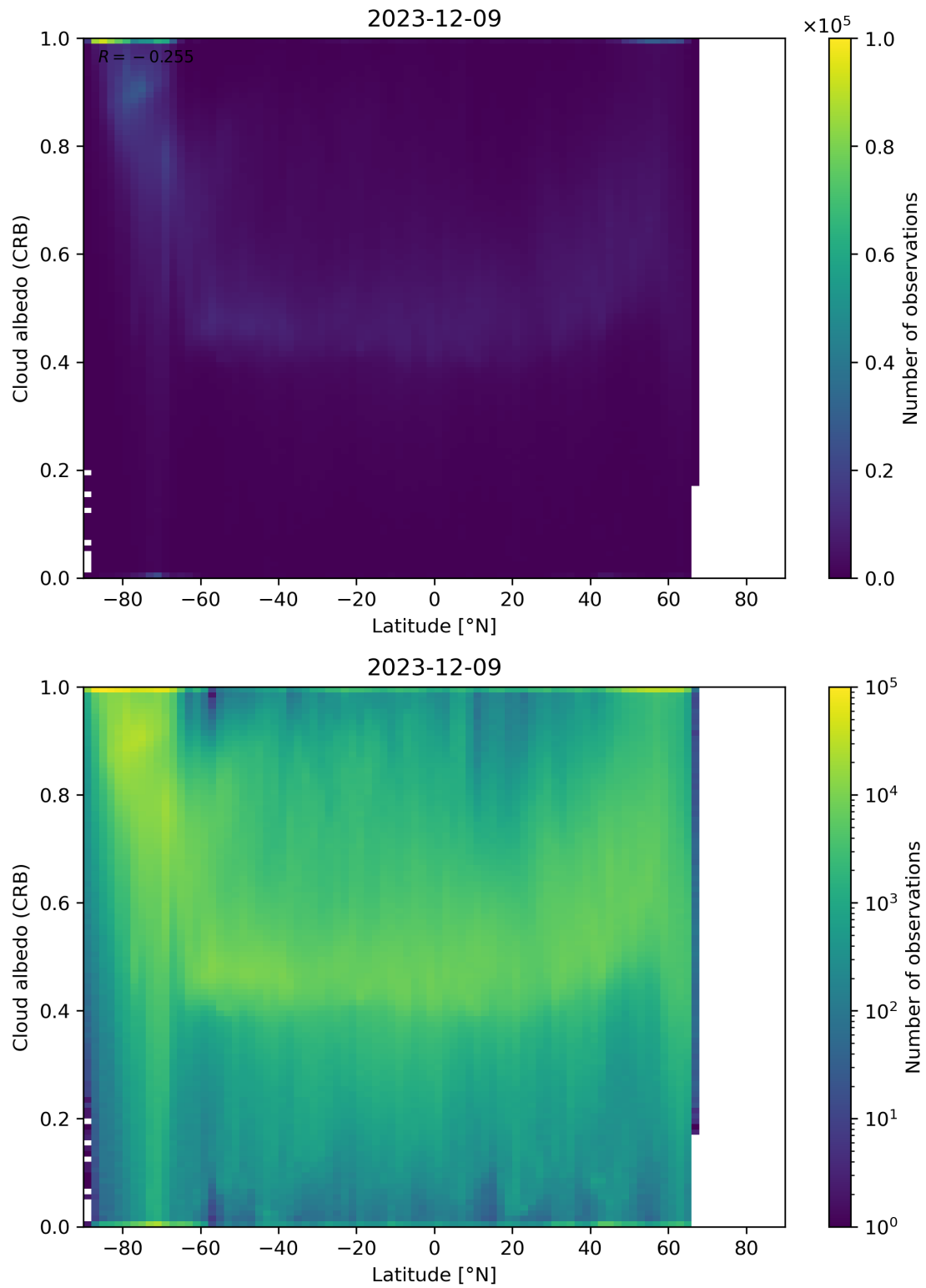
Figure 91: Scatter density plot of “Latitude” against “Cloud albedo (CRB)” for 2023-12-09 to 2023-12-10.
