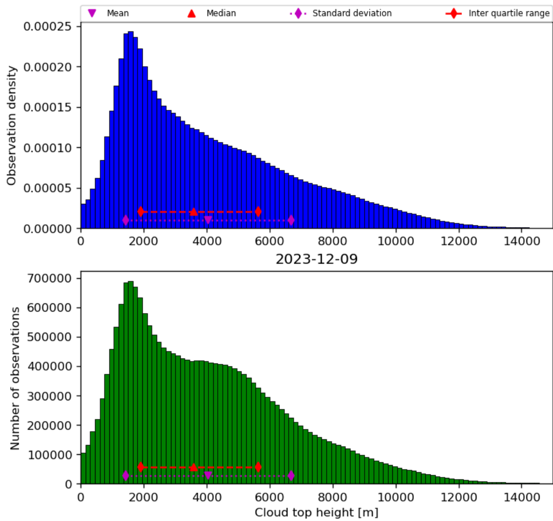
Figure 40: Histogram of “Cloud top height” for 2023-12-09 to 2023-12-10
