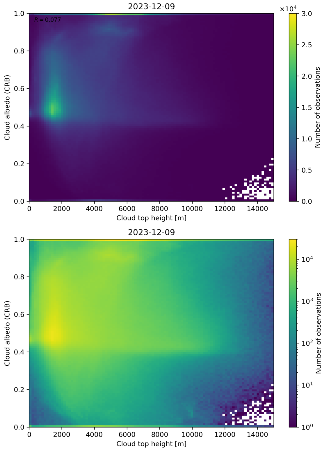
Figure 86: Scatter density plot of “Cloud top height” against “Cloud albedo (CRB)” for 2023-12-09 to 2023-12-10.
