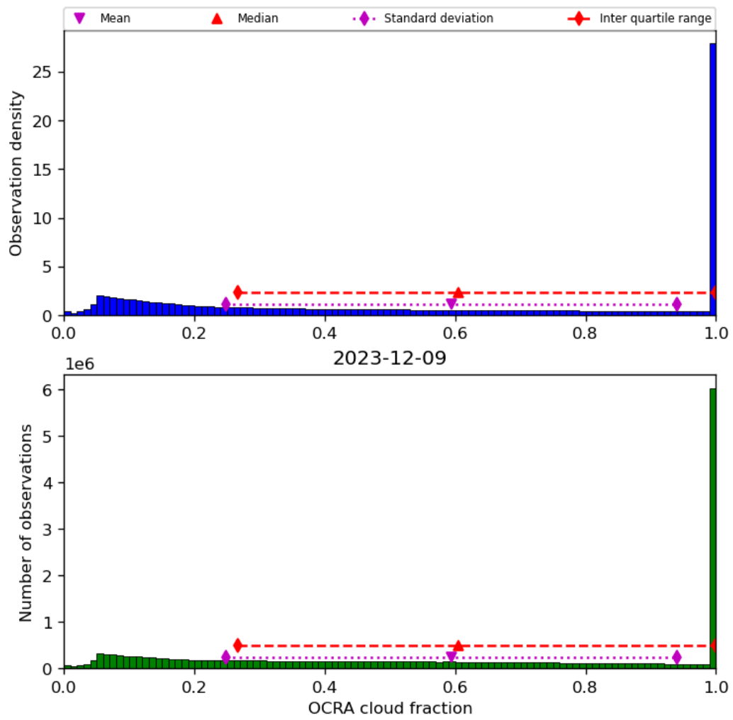
Figure 50: Histogram of “OCRA cloud fraction” for 2023-12-09 to 2023-12-10
