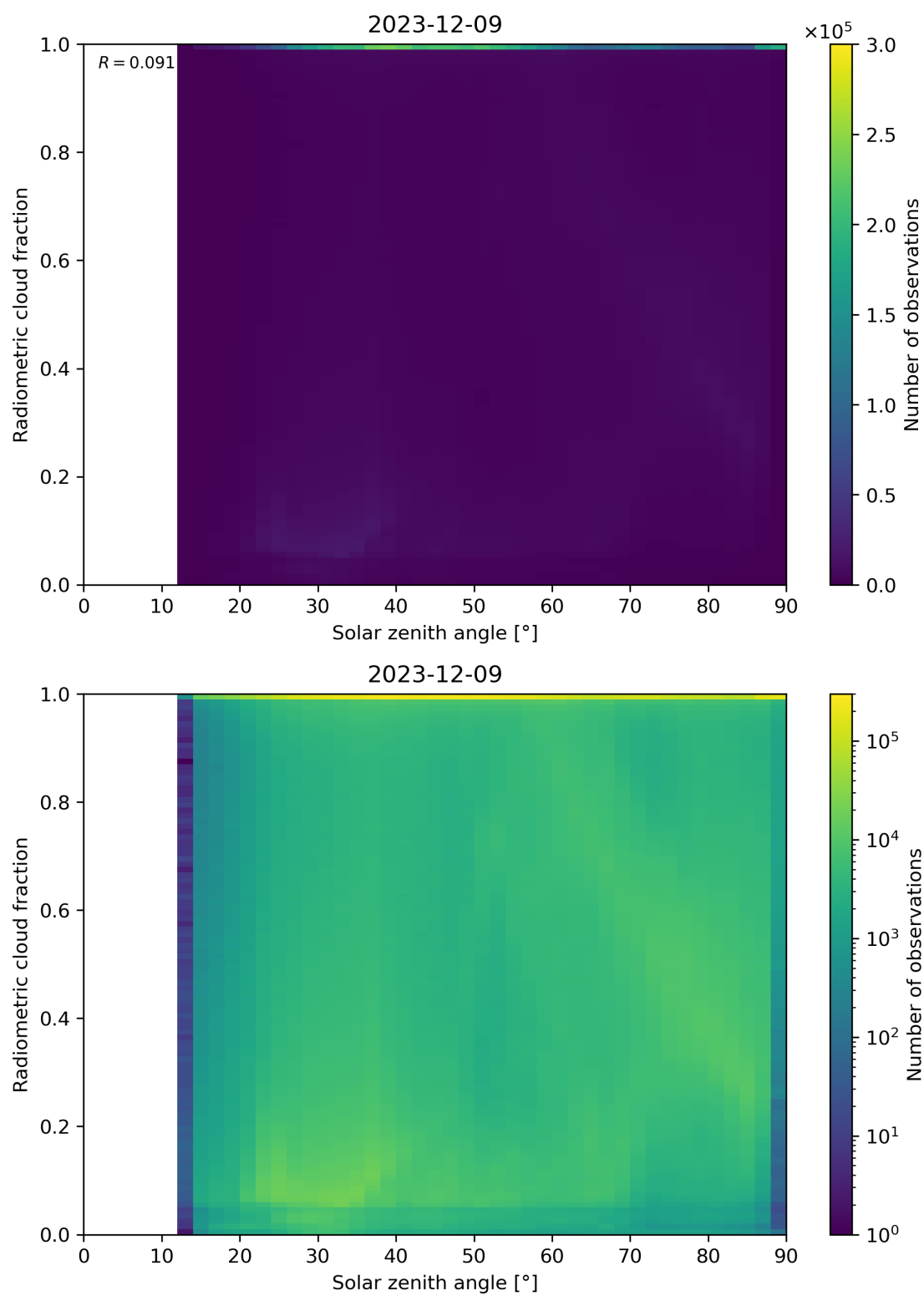
Figure 99: Scatter density plot of “Solar zenith angle” against “Radiometric cloud fraction” for 2023-12-09 to 2023-12-10.
