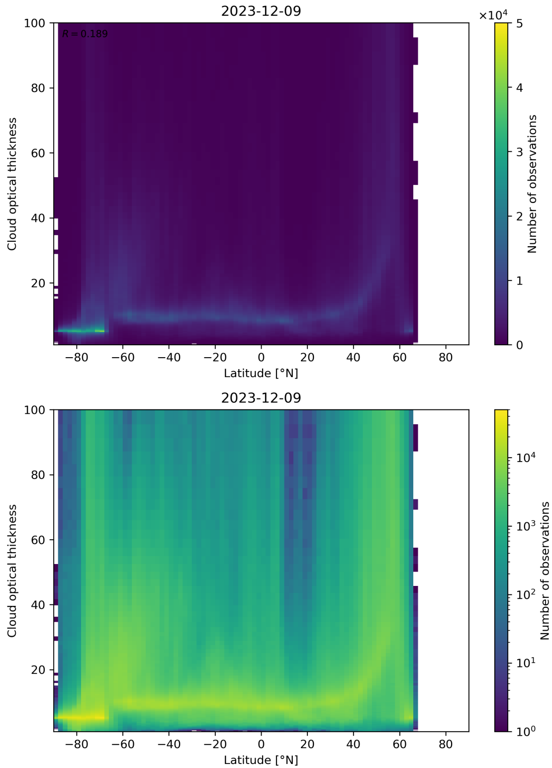
Figure 96: Scatter density plot of “Latitude” against “Cloud optical thickness” for 2023-12-09 to 2023-12-10.
