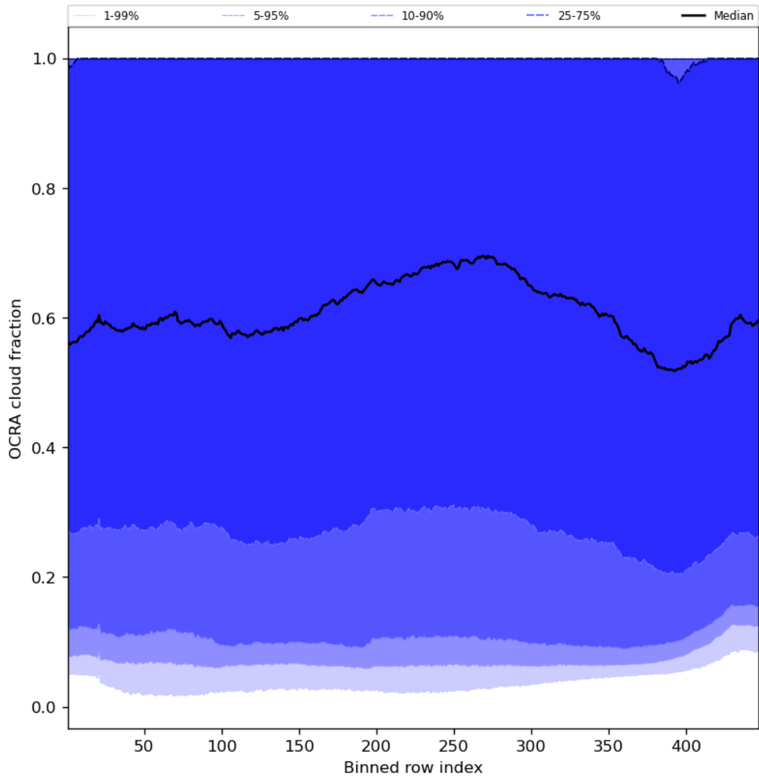
Figure 66: Along track statistics of “OCRA cloud fraction” for 2023-12-09 to 2023-12-10
