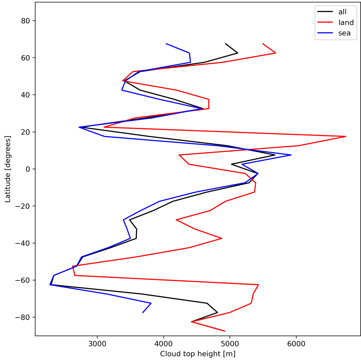
Figure 24: Zonal average of “Cloud top height” for 2023-12-09 to 2023-12-10.
