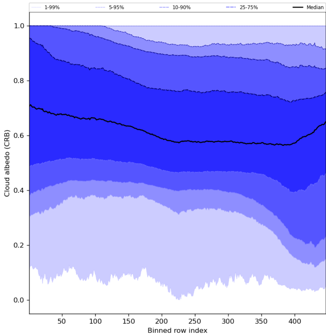
Figure 60: Along track statistics of “Cloud albedo (CRB)” for 2023-12-09 to 2023-12-10
