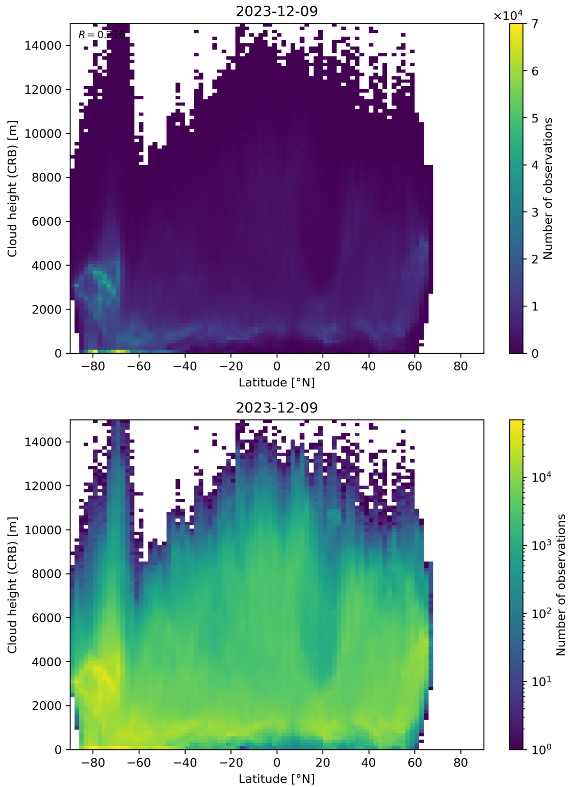
Figure 95: Scatter density plot of “Latitude” against “Cloud height (CRB)” for 2023-12-09 to 2023-12-10.
