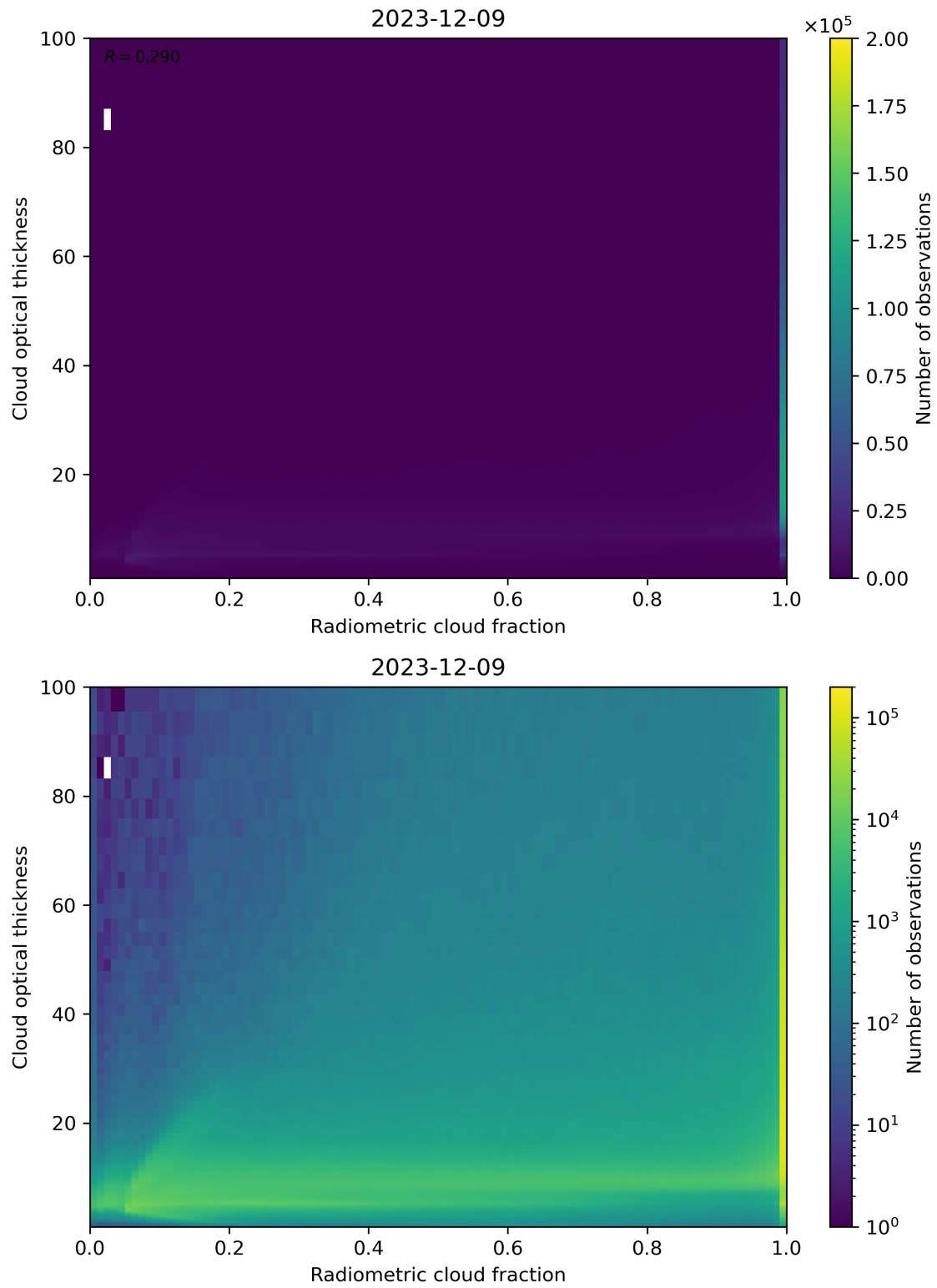
Figure 75: Scatter density plot of “Radiometric cloud fraction” against “Cloud optical thickness” for 2023-12-09 to 2023-12-10.
