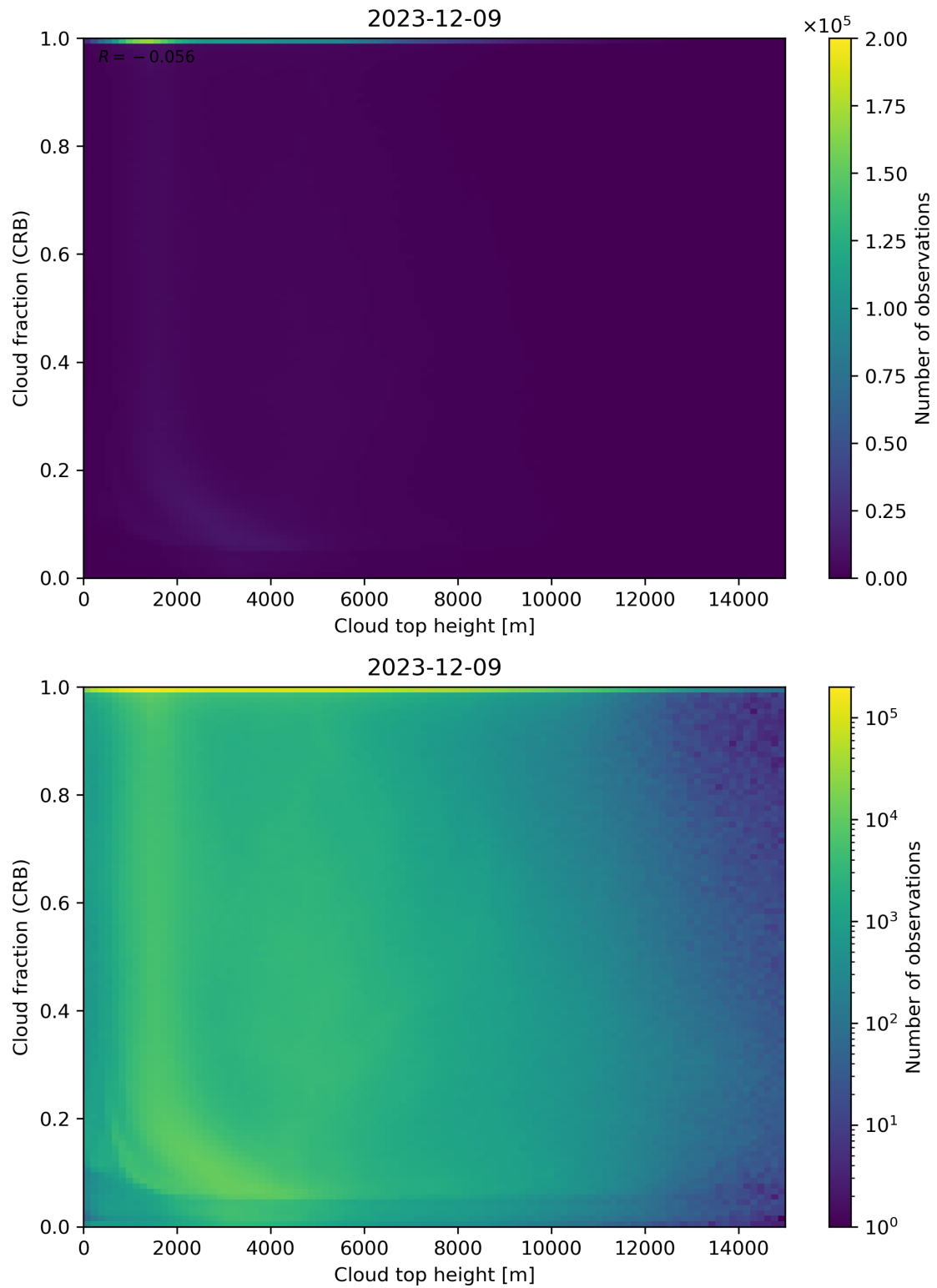
Figure 88: Scatter density plot of “Cloud top height” against “Cloud fraction (CRB)” for 2023-12-09 to 2023-12-10.
