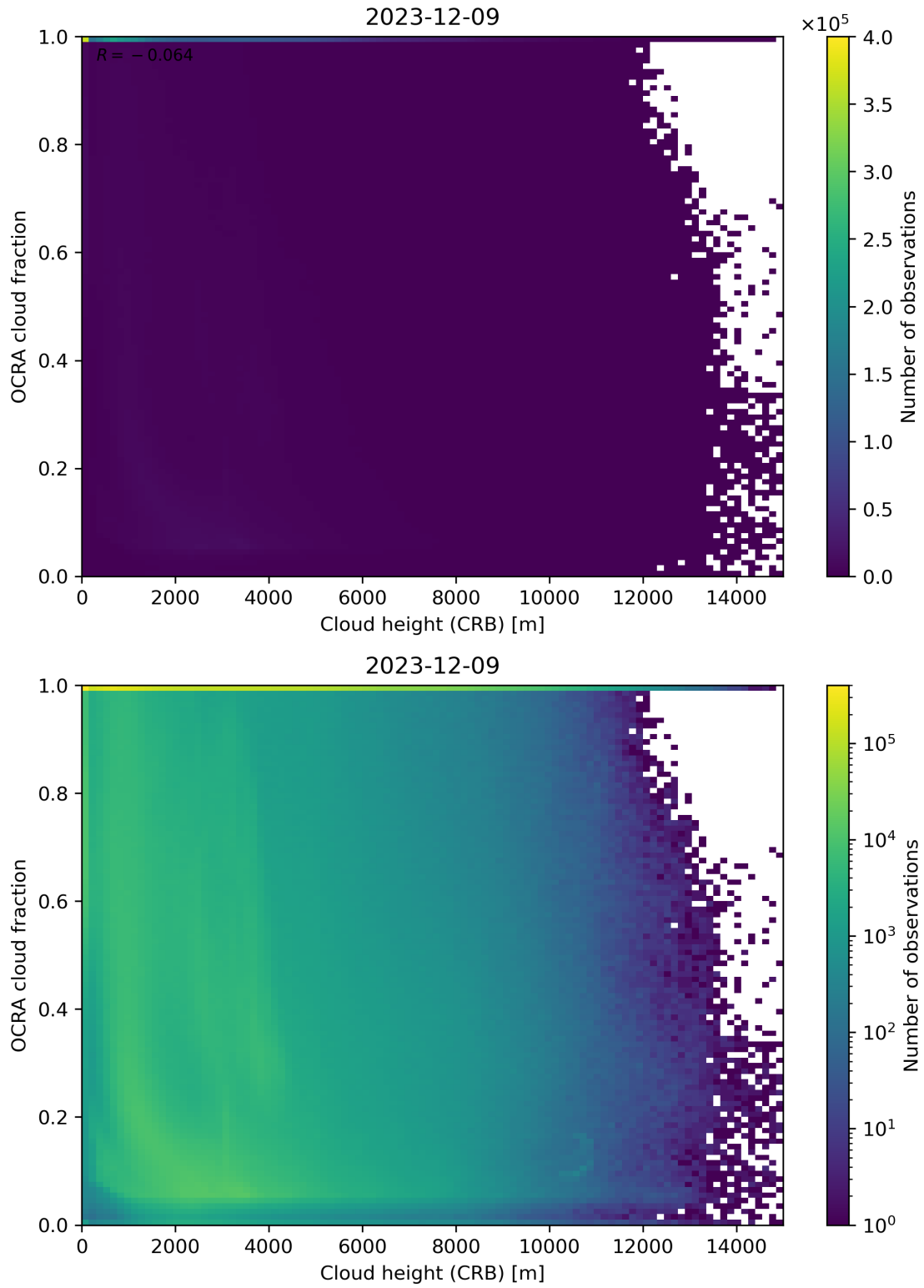
Figure 81: Scatter density plot of “Cloud height (CRB)” against “OCRA cloud fraction” for 2023-12-09 to 2023-12-10.
