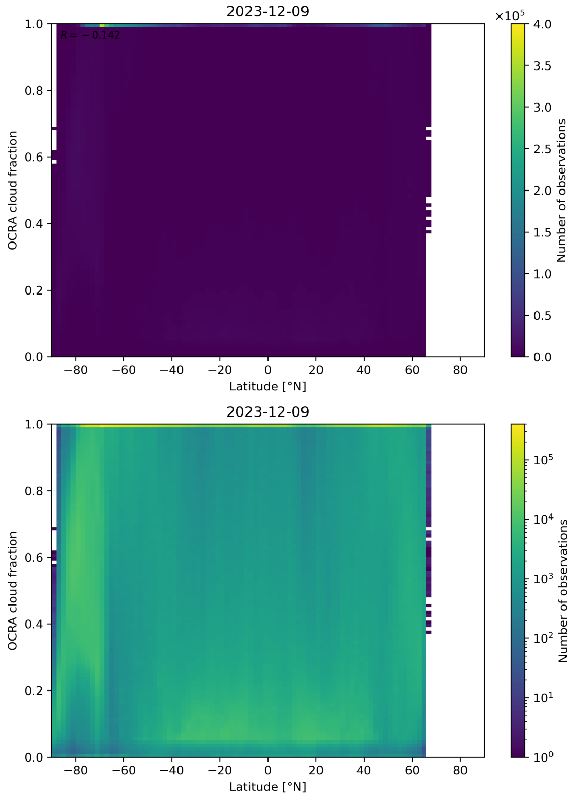
Figure 93: Scatter density plot of “Latitude” against “OCRA cloud fraction” for 2023-12-09 to 2023-12-10.
