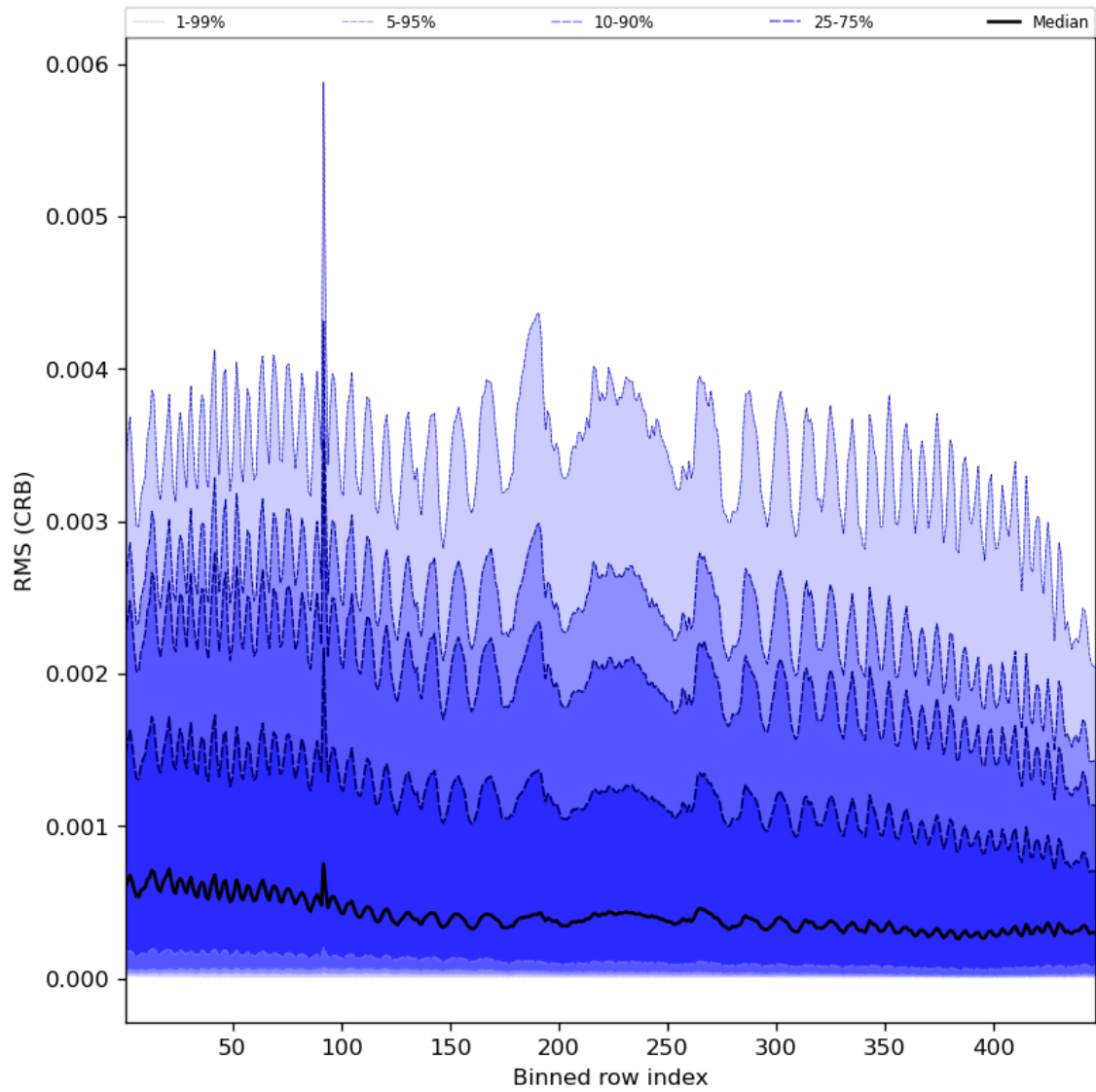
Figure 64: Along track statistics of “RMS (CRB)” for 2023-12-09 to 2023-12-10
