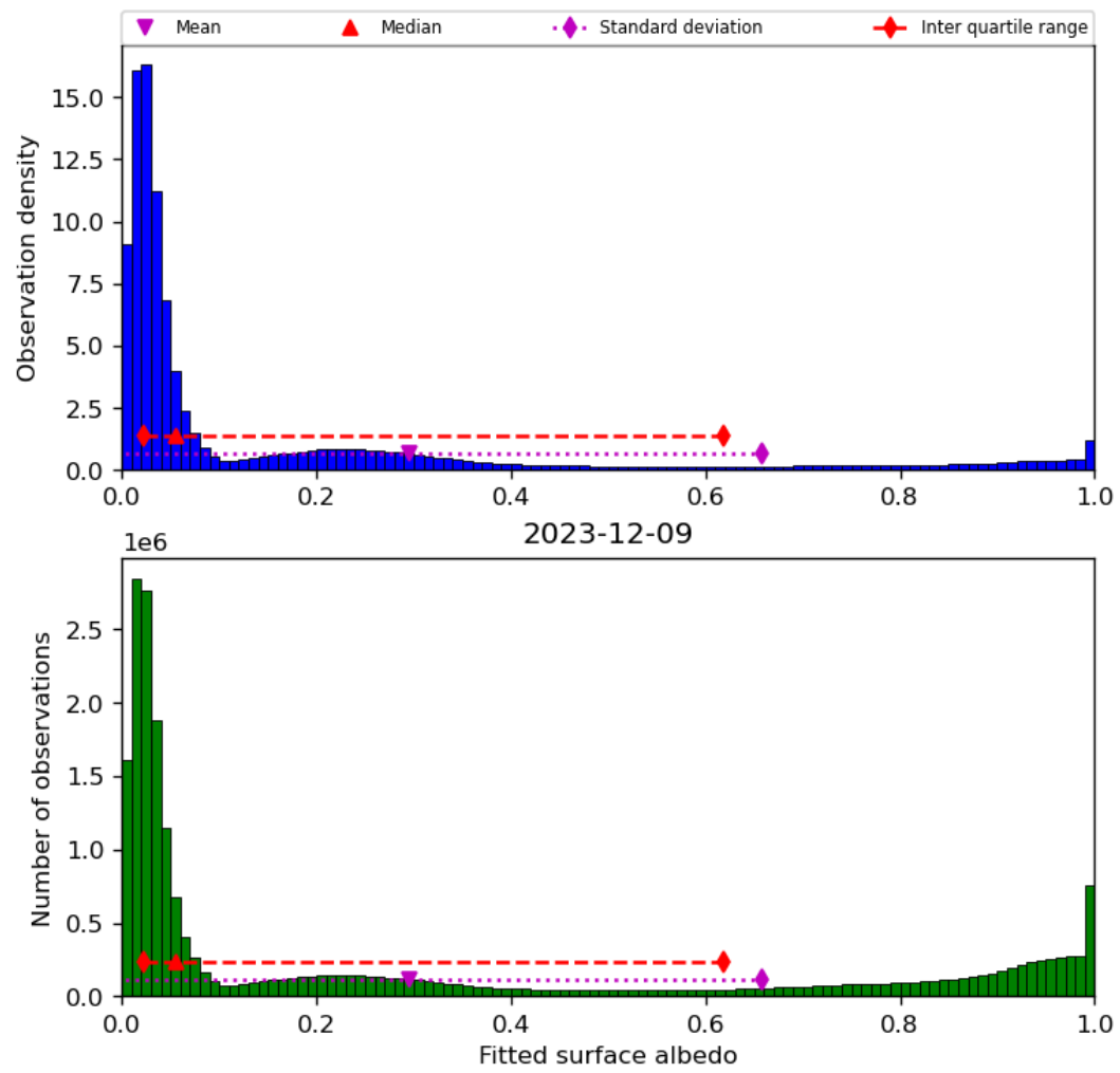
Figure 45: Histogram of “Fitted surface albedo” for 2023-12-09 to 2023-12-10
