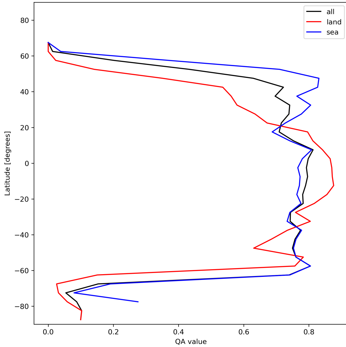
Figure 22: Zonal average of “QA value” for 2023-12-09 to 2023-12-10.
