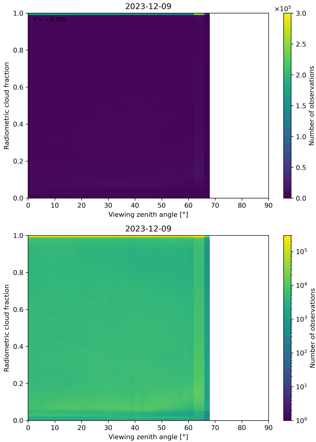
Figure 107: Scatter density plot of “Viewing zenith angle” against “Radiometric cloud fraction” for 2023-12-09 to 2023-12-10.
