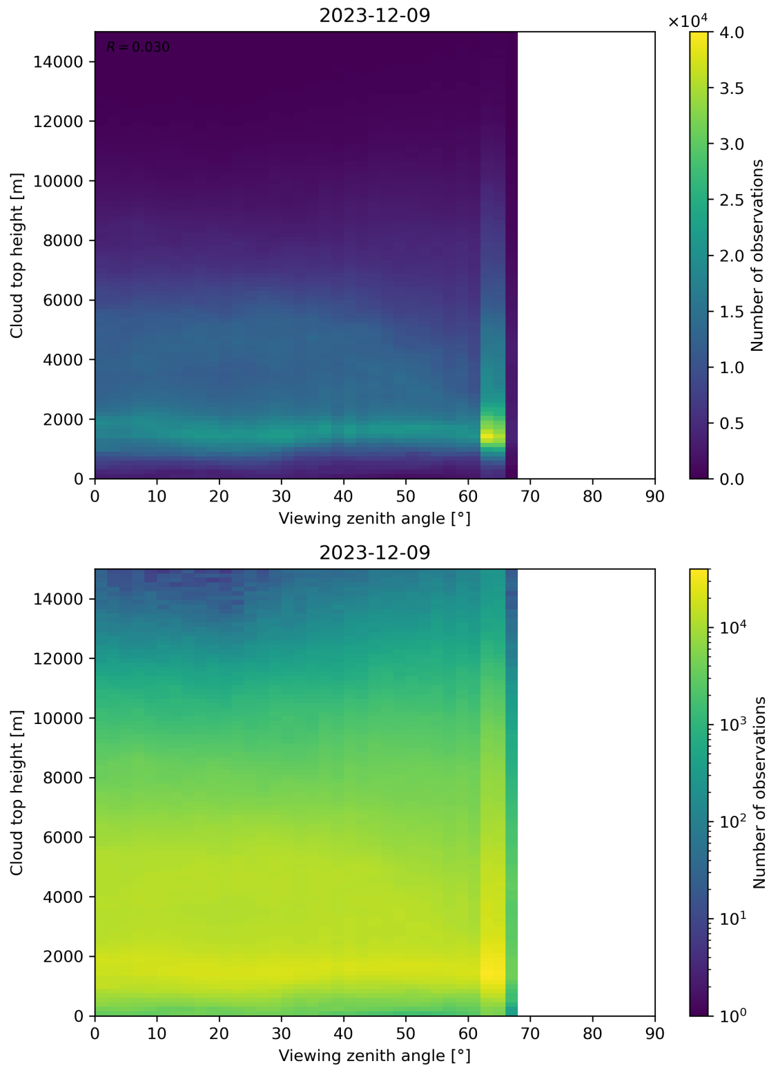
Figure 112: Scatter density plot of “Viewing zenith angle” against “Cloud top height” for 2023-12-09 to 2023-12-10.
