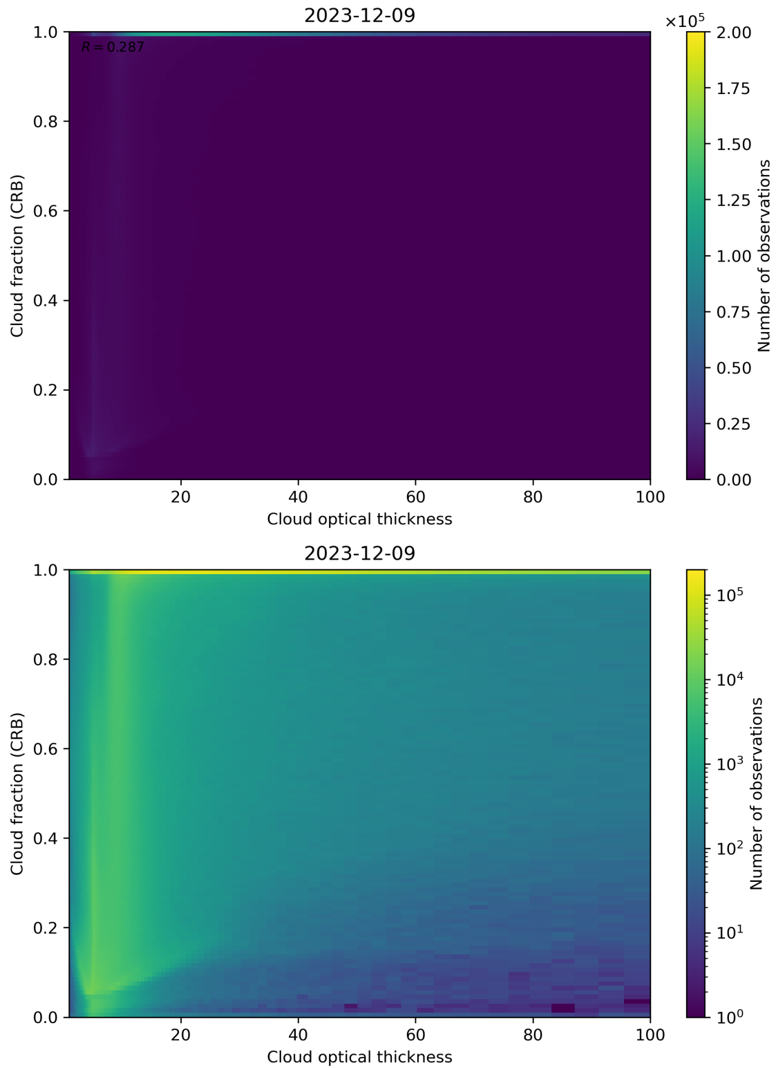
Figure 84: Scatter density plot of “Cloud optical thickness” against “Cloud fraction (CRB)” for 2023-12-09 to 2023-12-10.
