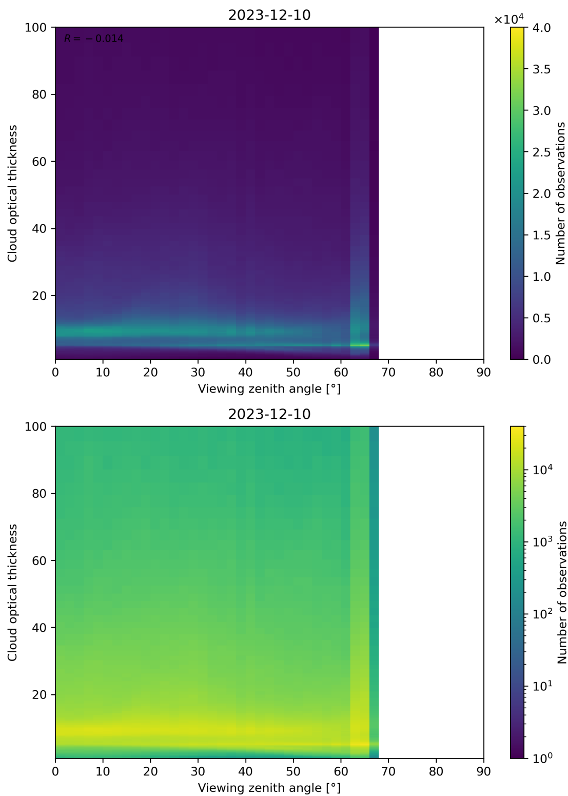
Figure 111: Scatter density plot of “Viewing zenith angle” against “Cloud optical thickness” for 2023-12-09 to 2023-12-11.
