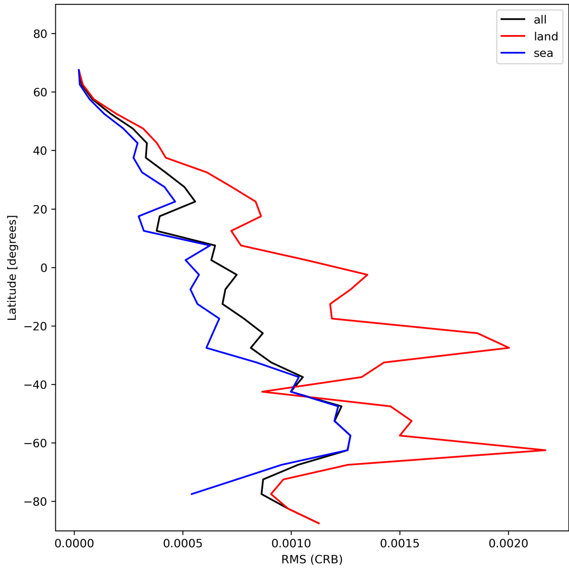
Figure 32: Zonal average of “RMS (CRB)” for 2023-12-09 to 2023-12-11.
