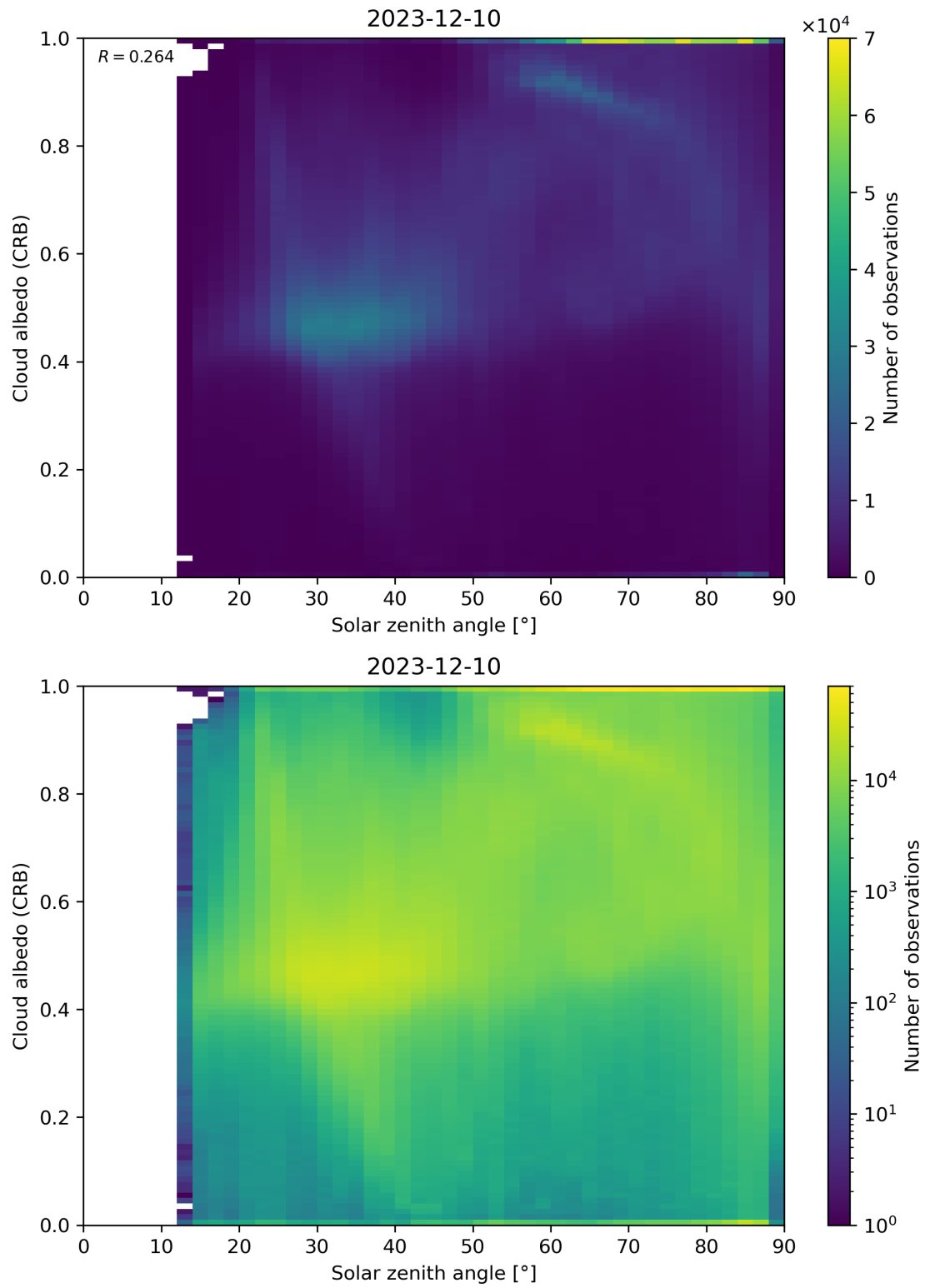
Figure 98: Scatter density plot of “Solar zenith angle” against “Cloud albedo (CRB)” for 2023-12-09 to 2023-12-11.
