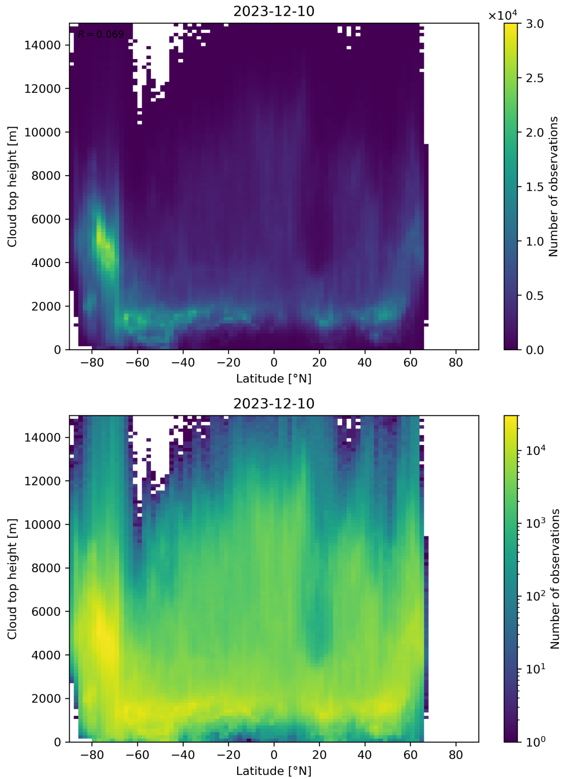
Figure 97: Scatter density plot of “Latitude” against “Cloud top height” for 2023-12-09 to 2023-12-11.
