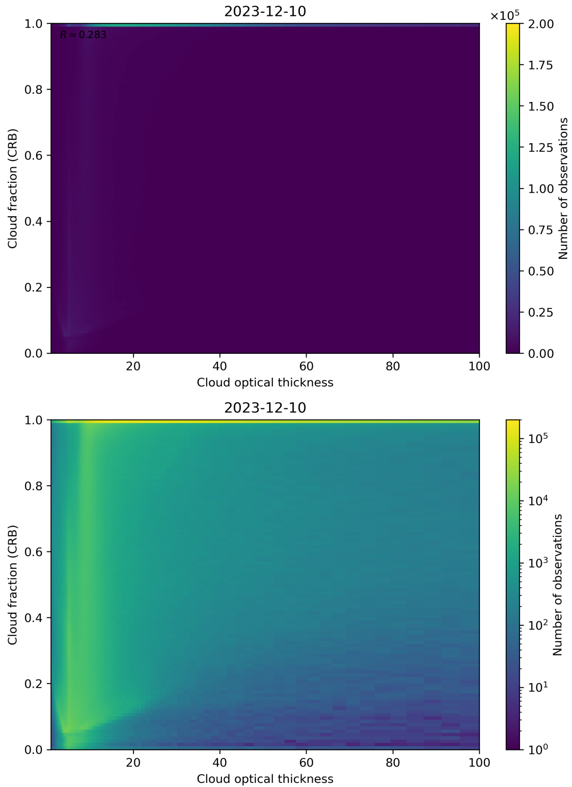
Figure 84: Scatter density plot of “Cloud optical thickness” against “Cloud fraction (CRB)” for 2023-12-09 to 2023-12-11.
