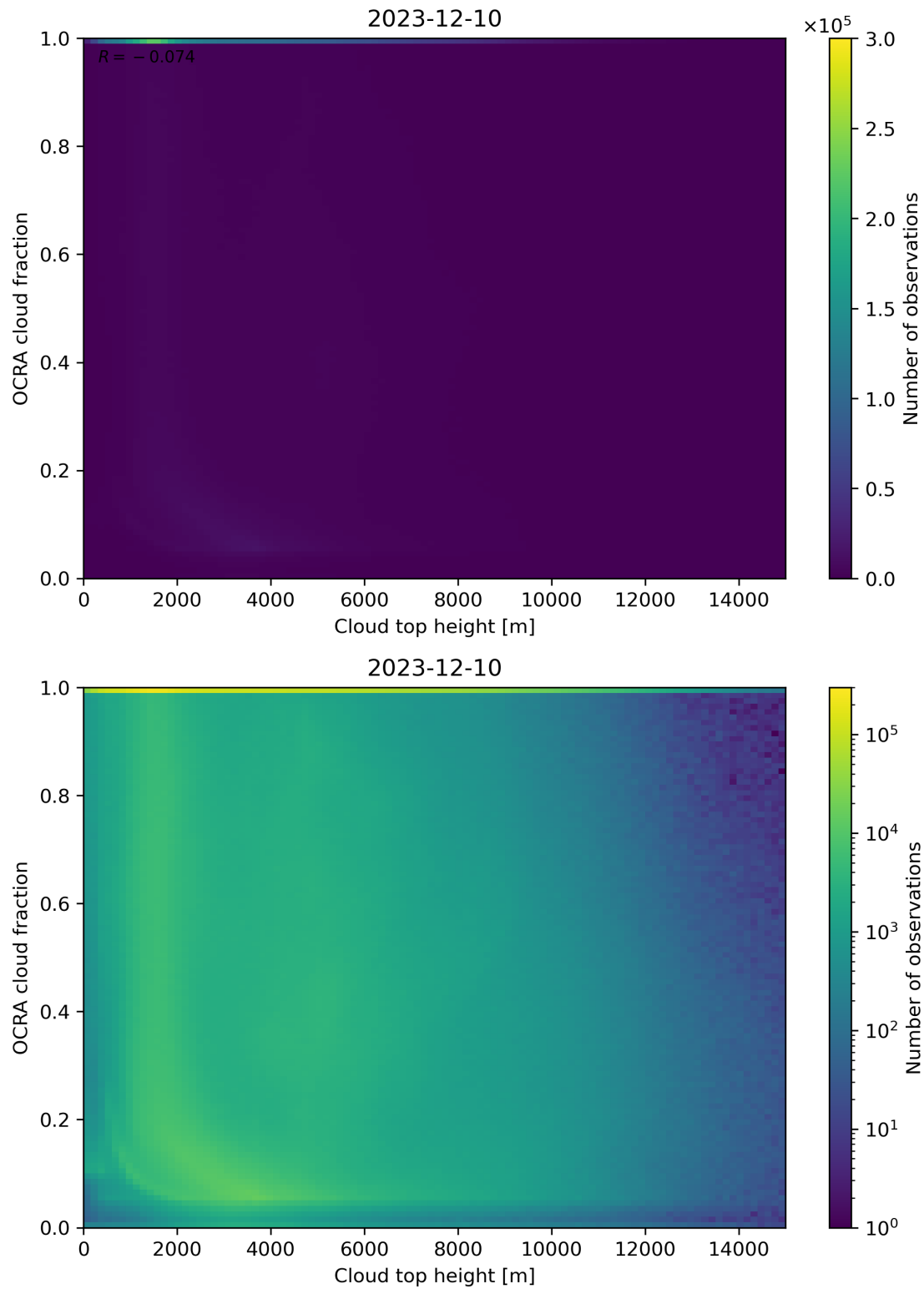
Figure 87: Scatter density plot of “Cloud top height” against “OCRA cloud fraction” for 2023-12-09 to 2023-12-11.
