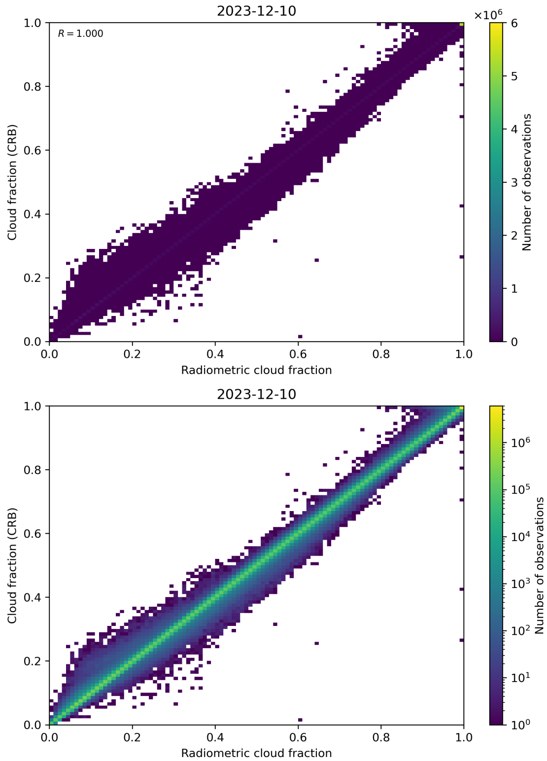
Figure 73: Scatter density plot of “Radiometric cloud fraction” against “Cloud fraction (CRB)” for 2023-12-09 to 2023-12-11.
