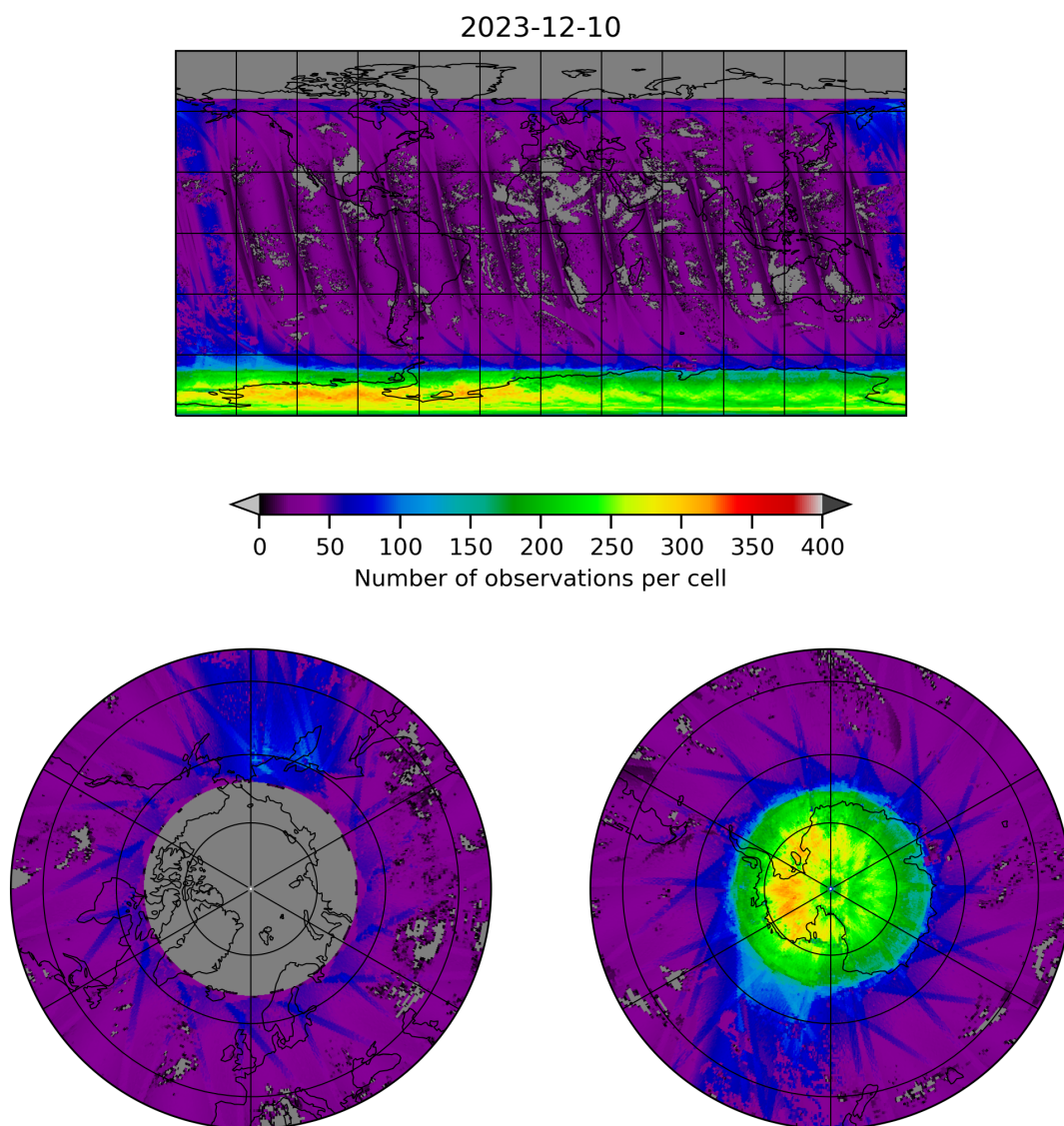
Figure 21: Map of the number of observations for 2023-12-09 to 2023-12-11
