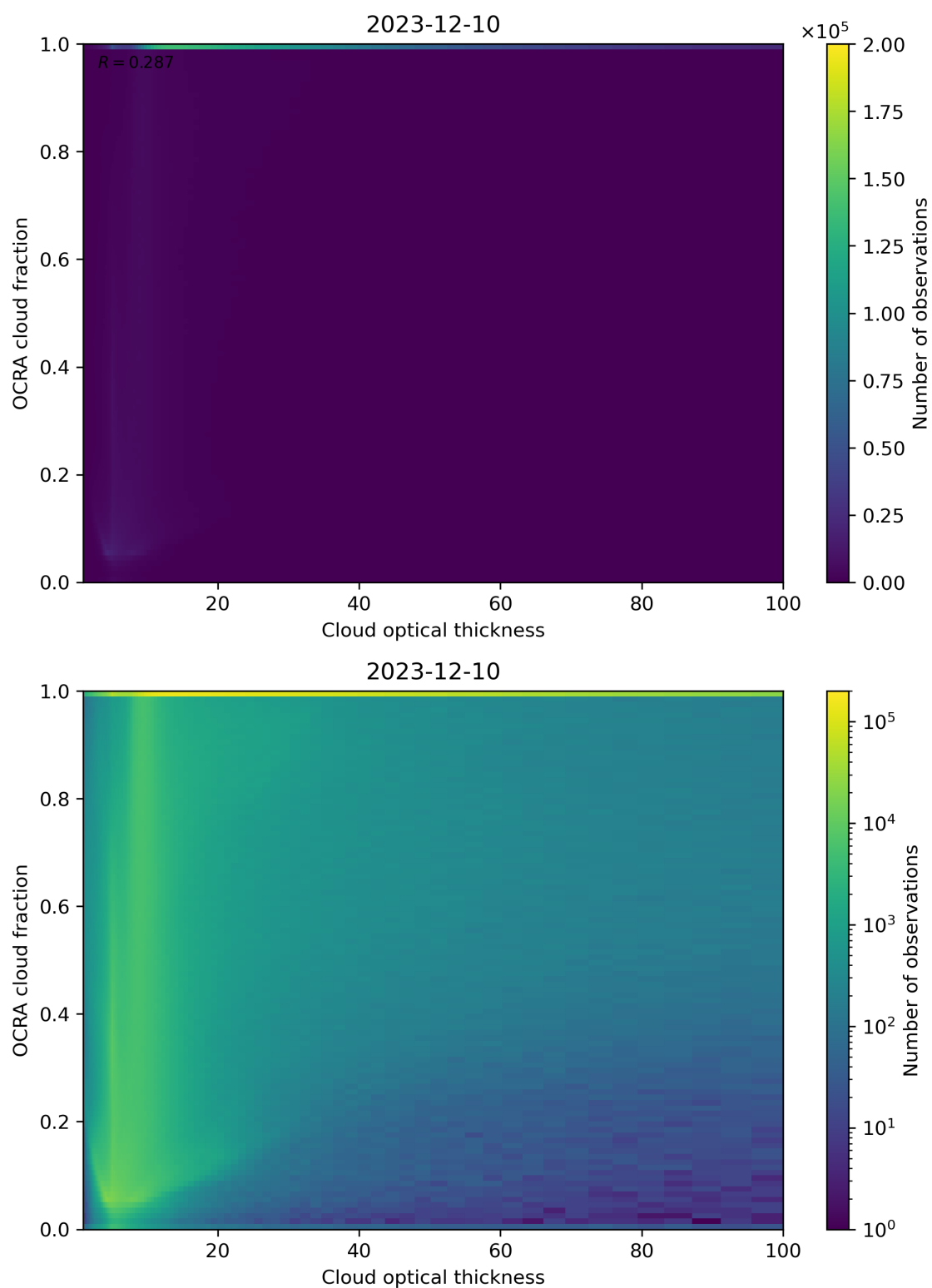
Figure 83: Scatter density plot of “Cloud optical thickness” against “OCRA cloud fraction” for 2023-12-09 to 2023-12-11.
