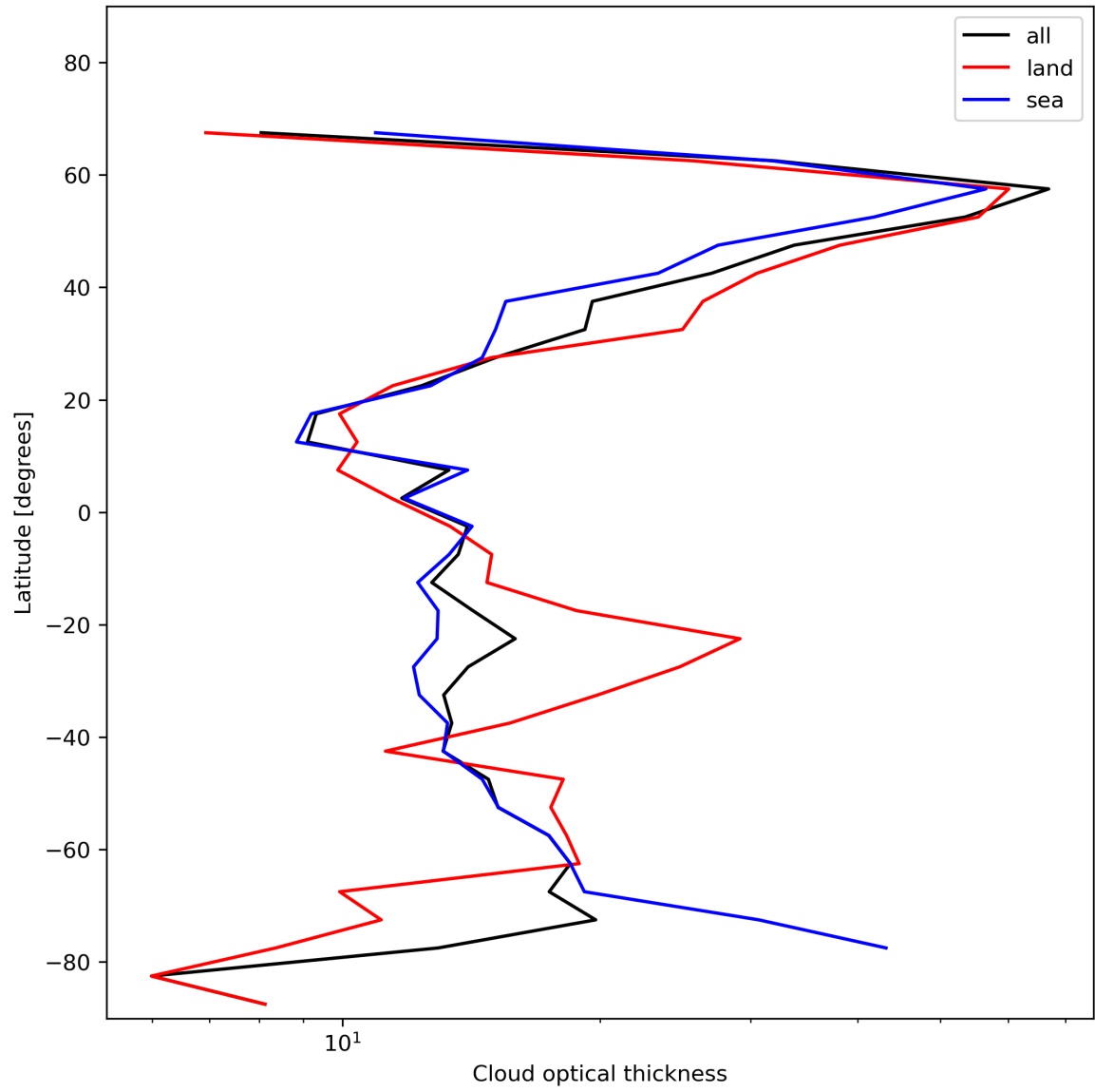
Figure 25: Zonal average of “Cloud optical thickness” for 2023-12-09 to 2023-12-11.
