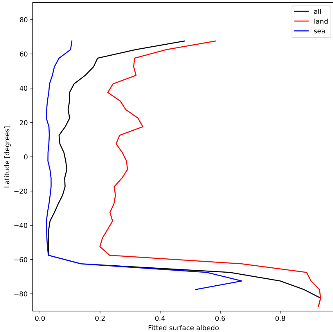
Figure 29: Zonal average of “Fitted surface albedo” for 2023-12-09 to 2023-12-11.
