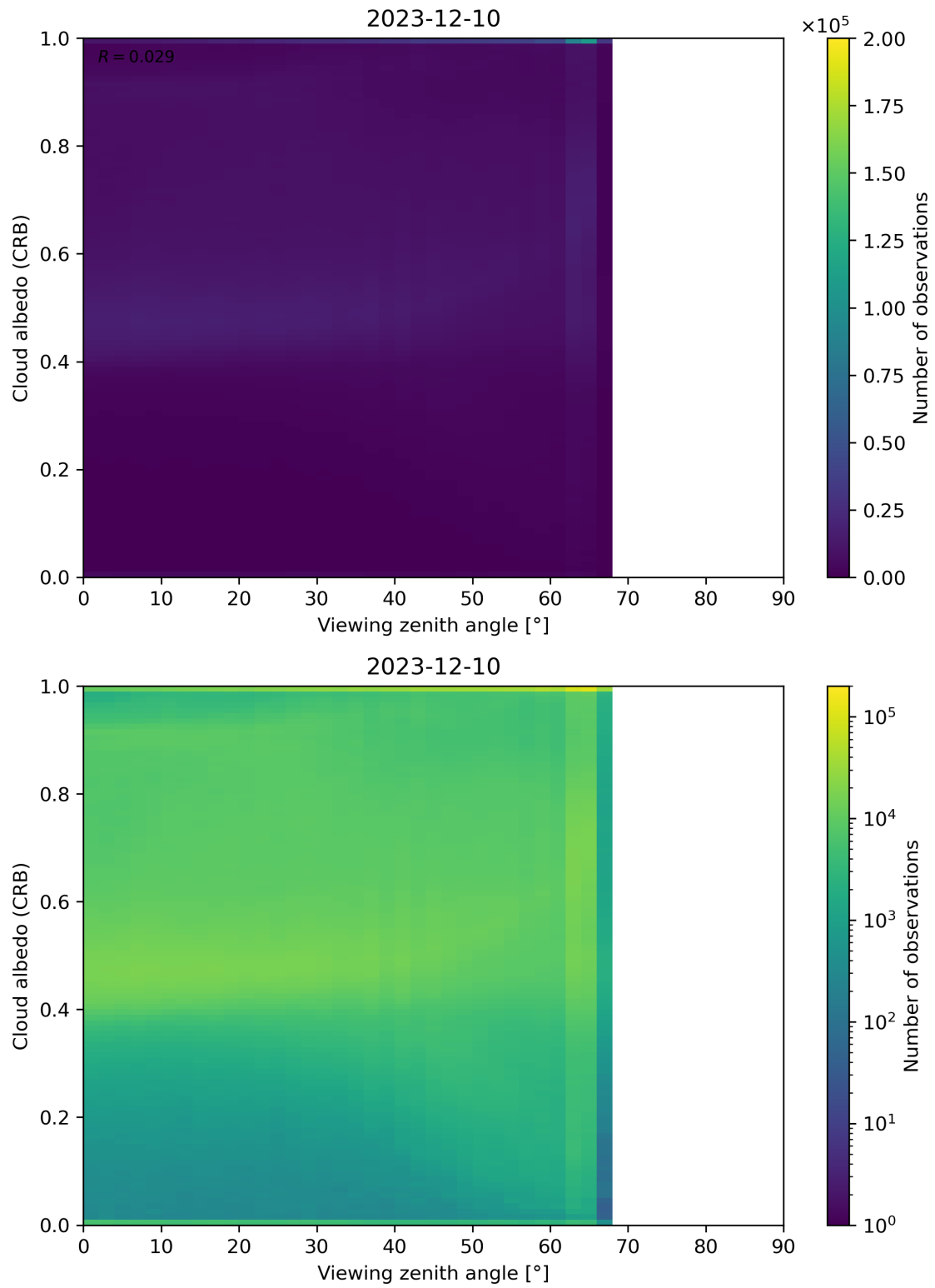
Figure 106: Scatter density plot of “Viewing zenith angle” against “Cloud albedo (CRB)” for 2023-12-09 to 2023-12-11.
