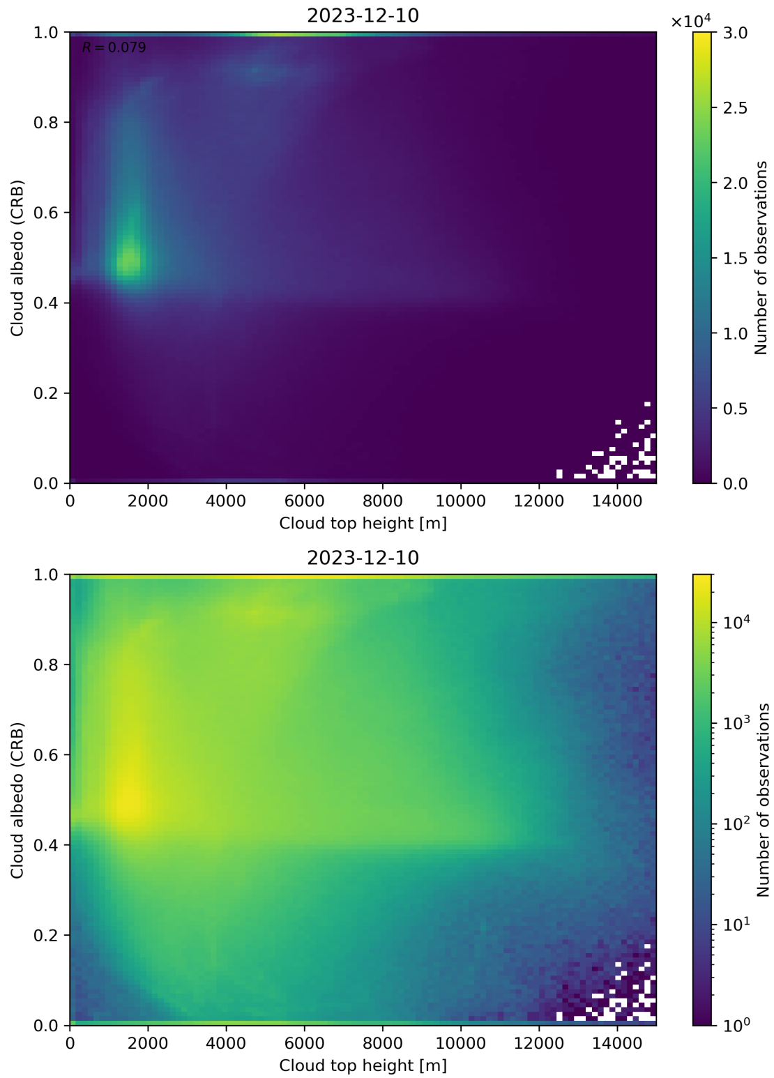
Figure 86: Scatter density plot of “Cloud top height” against “Cloud albedo (CRB)” for 2023-12-09 to 2023-12-11.
