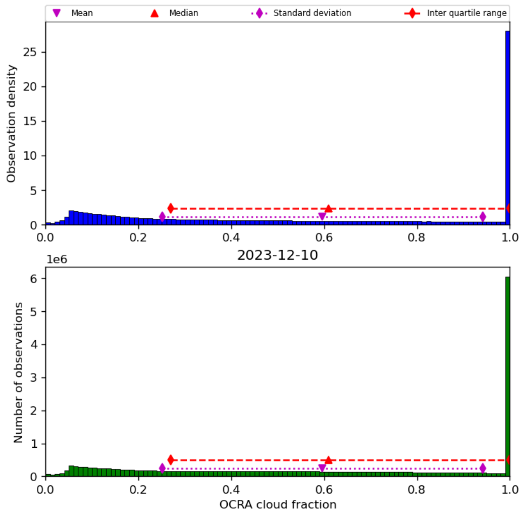
Figure 50: Histogram of “OCRA cloud fraction” for 2023-12-09 to 2023-12-11
