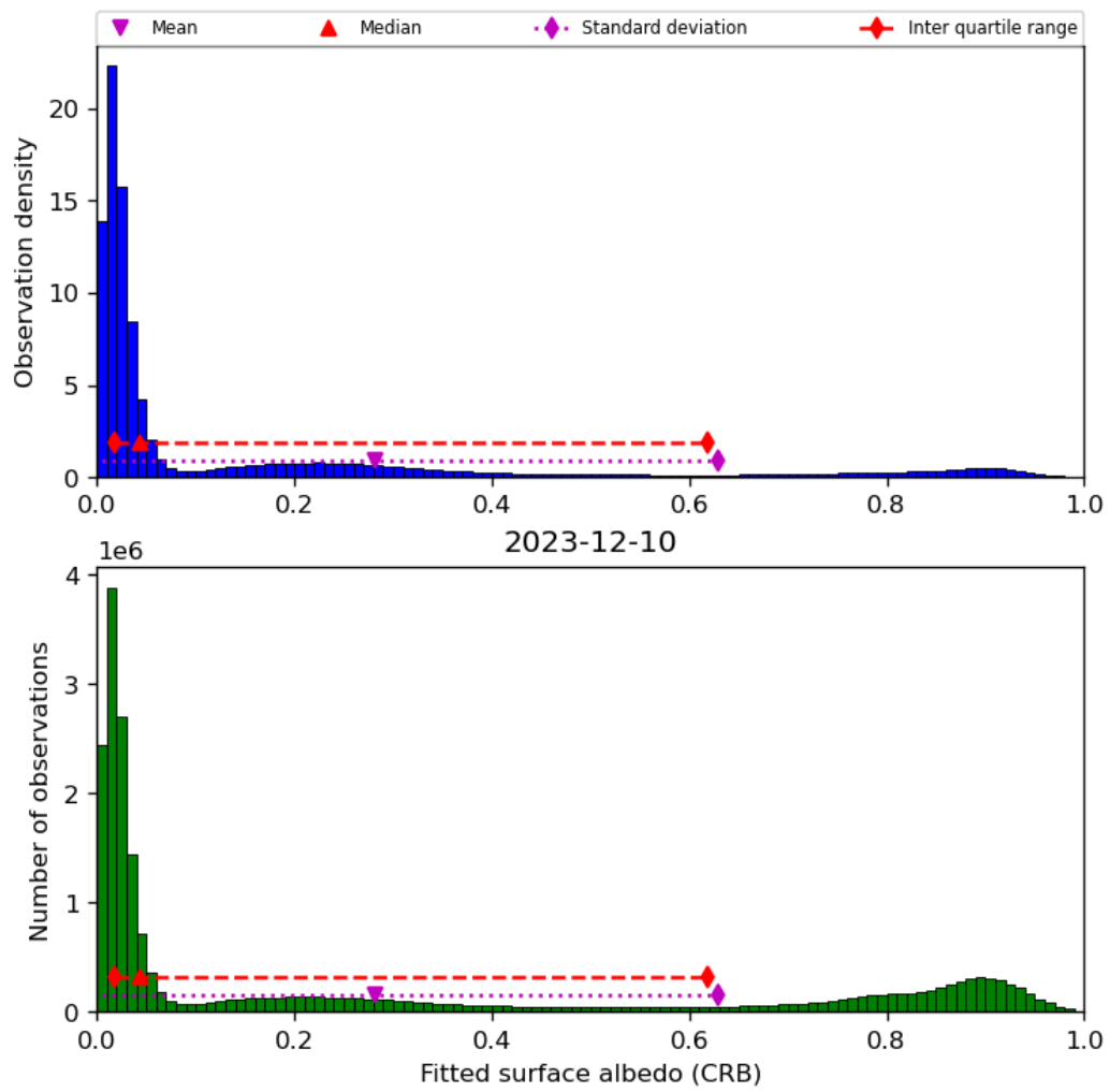
Figure 46: Histogram of “Fitted surface albedo (CRB)” for 2023-12-09 to 2023-12-11
