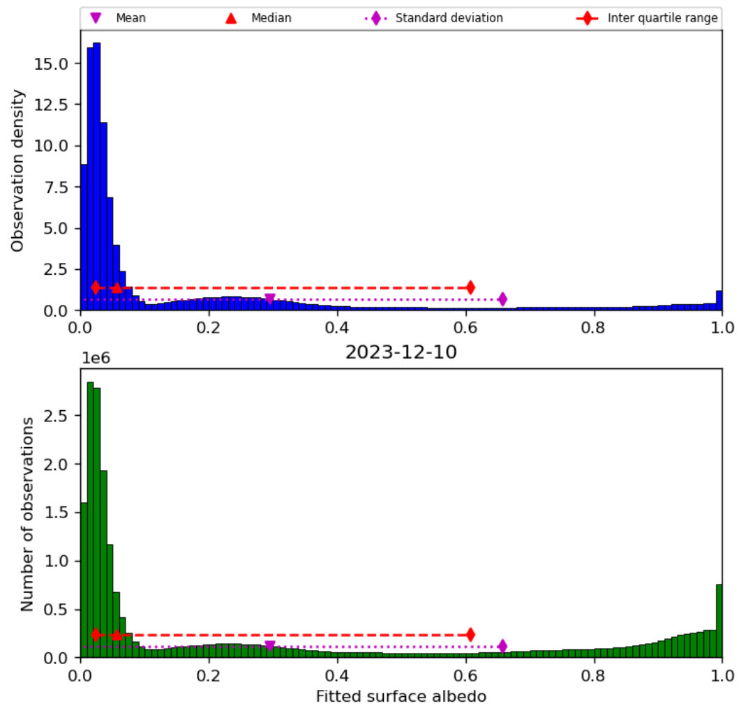
Figure 45: Histogram of “Fitted surface albedo” for 2023-12-09 to 2023-12-11
