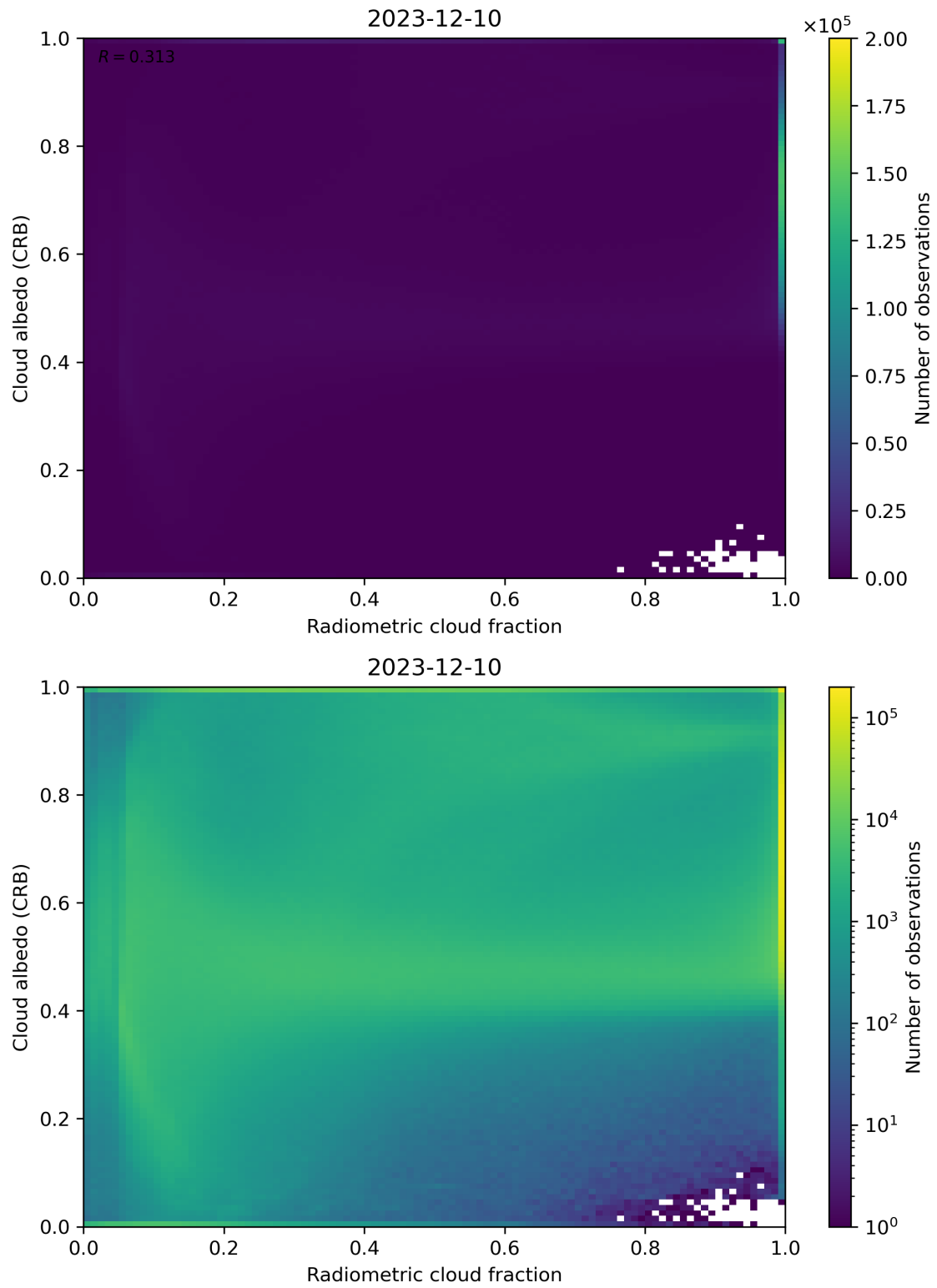
Figure 71: Scatter density plot of “Radiometric cloud fraction” against “Cloud albedo (CRB)” for 2023-12-09 to 2023-12-11.
