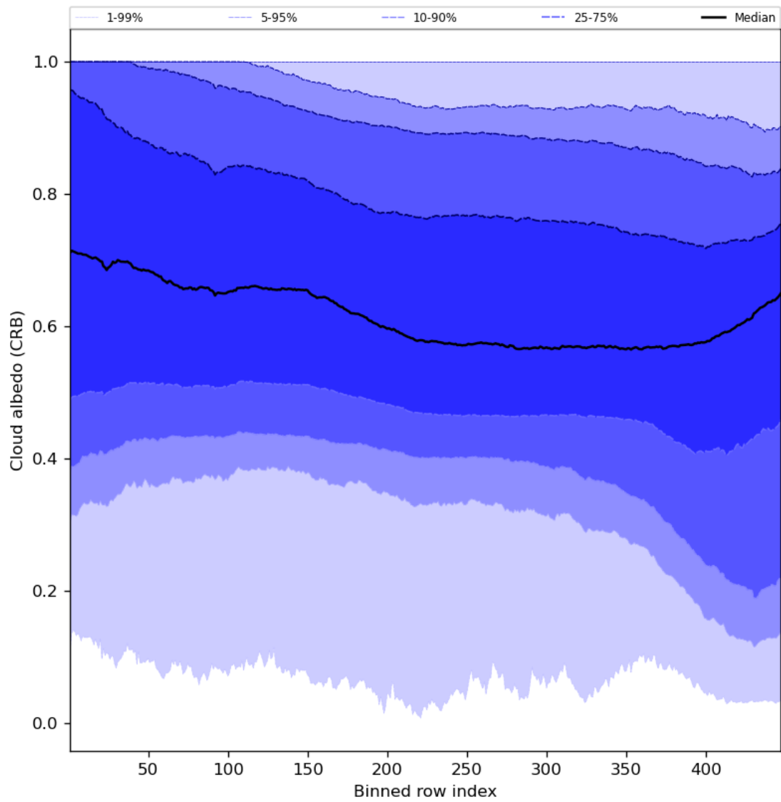
Figure 60: Along track statistics of “Cloud albedo (CRB)” for 2023-12-09 to 2023-12-11
