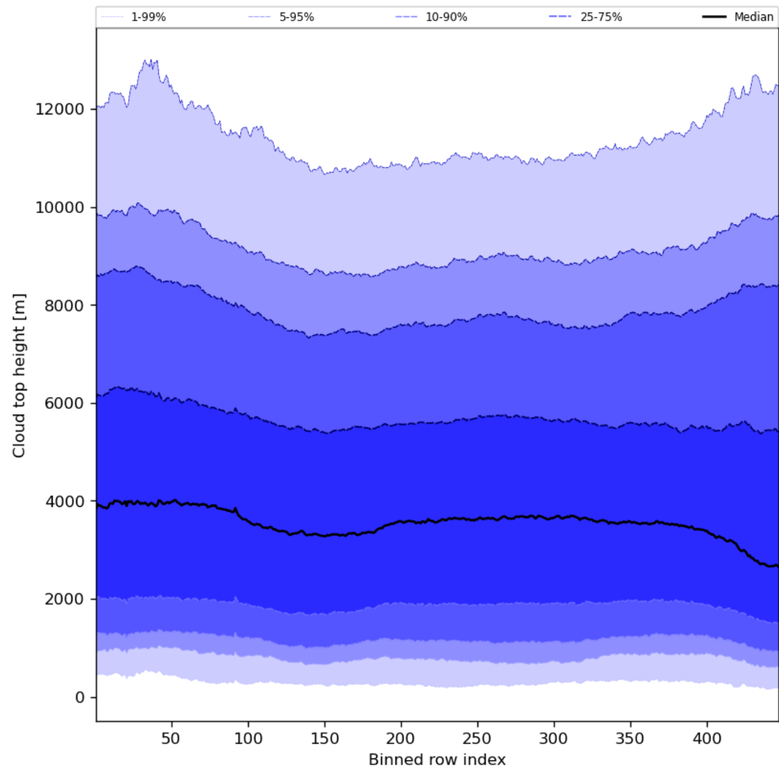
Figure 56: Along track statistics of “Cloud top height” for 2023-12-09 to 2023-12-11
