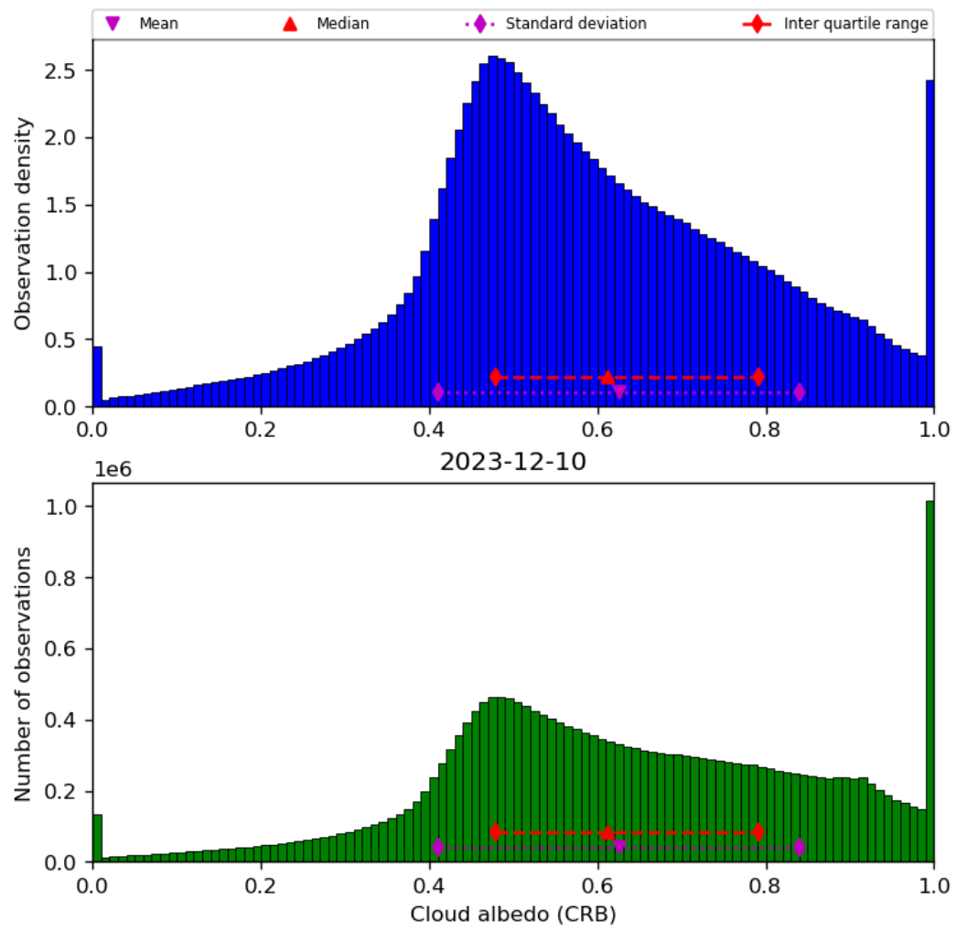
Figure 44: Histogram of “Cloud albedo (CRB)” for 2023-12-09 to 2023-12-11
