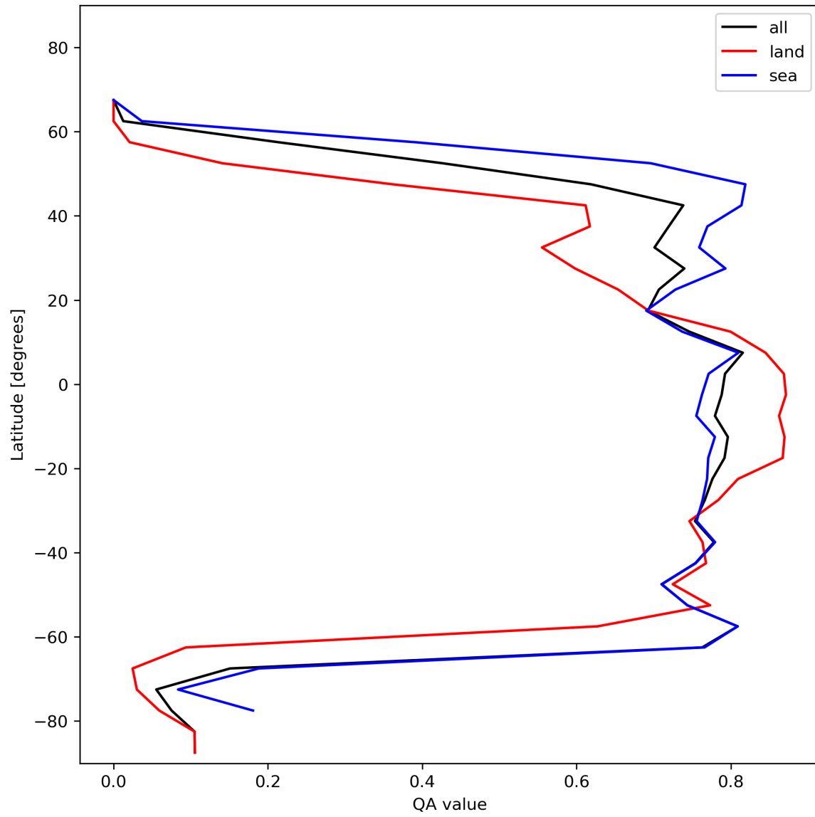
Figure 22: Zonal average of “QA value” for 2023-12-09 to 2023-12-11.
