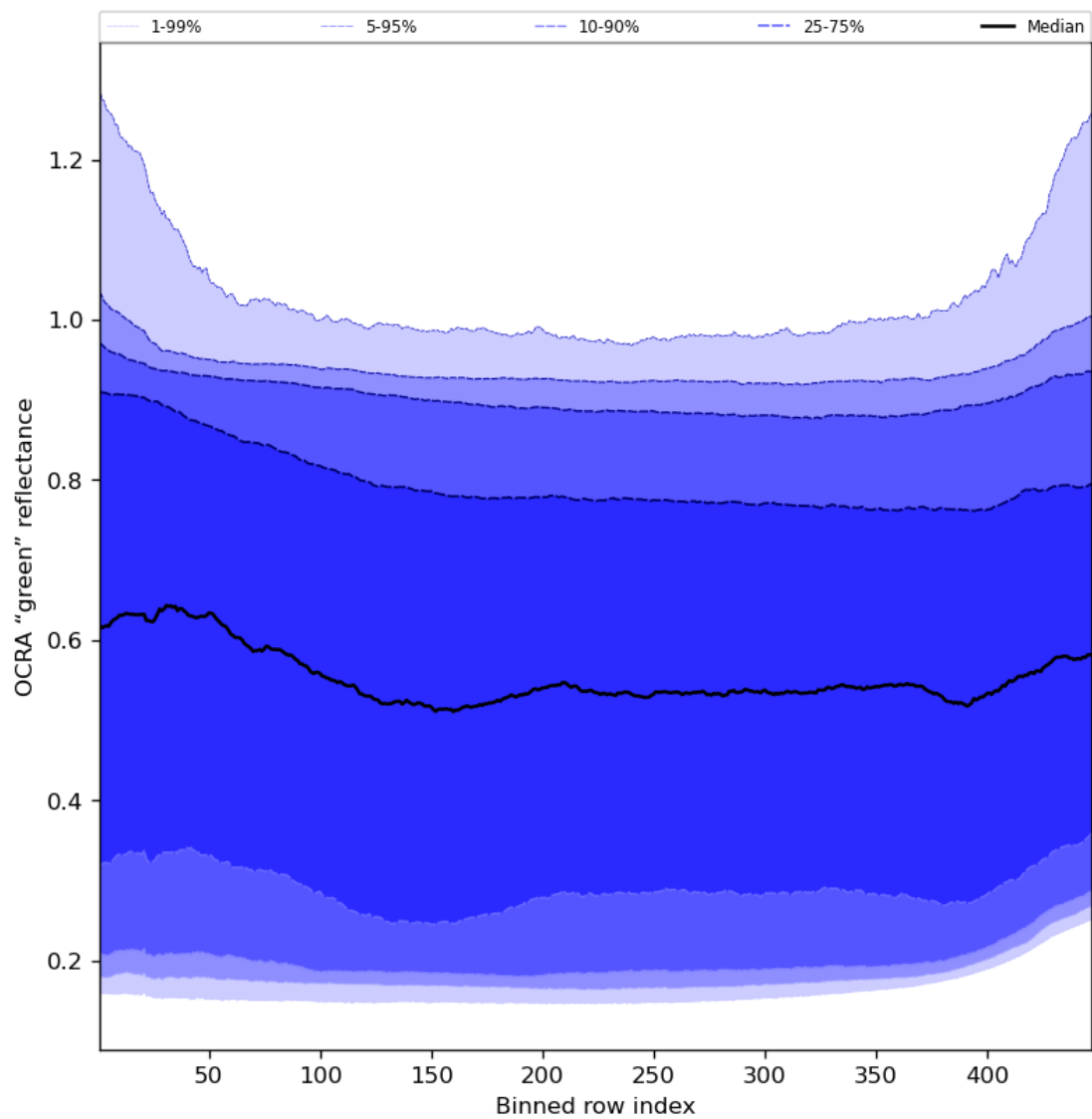
Figure 68: Along track statistics of “OCRA “green” reflectance” for 2023-12-09 to 2023-12-11
