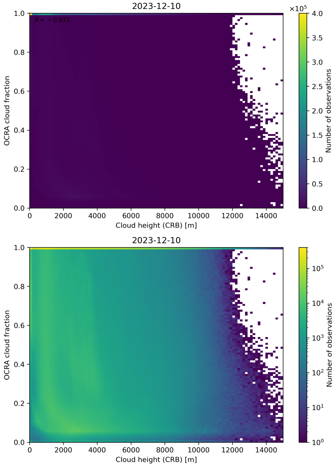
Figure 81: Scatter density plot of “Cloud height (CRB)” against “OCRA cloud fraction” for 2023-12-09 to 2023-12-11.
