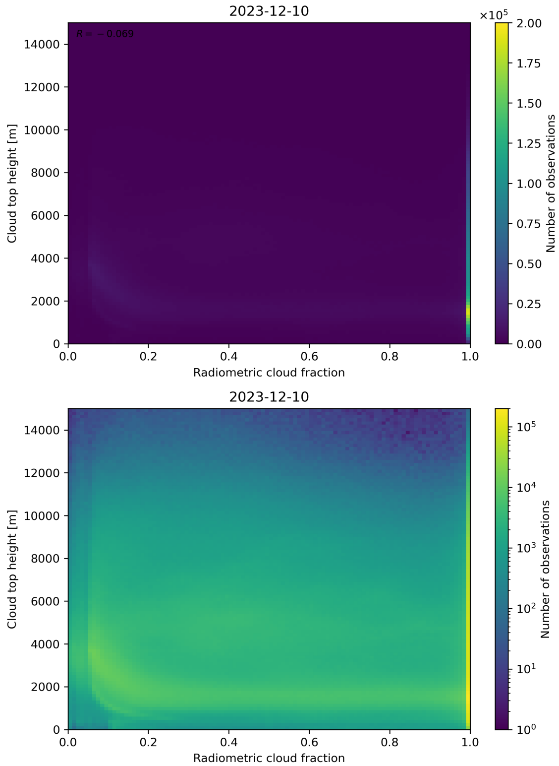
Figure 76: Scatter density plot of “Radiometric cloud fraction” against “Cloud top height” for 2023-12-09 to 2023-12-11.
