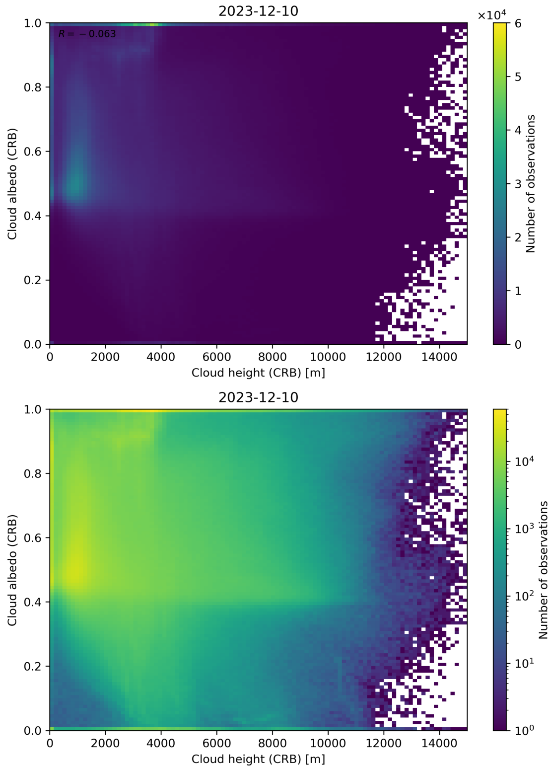
Figure 80: Scatter density plot of “Cloud height (CRB)” against “Cloud albedo (CRB)” for 2023-12-09 to 2023-12-11.
