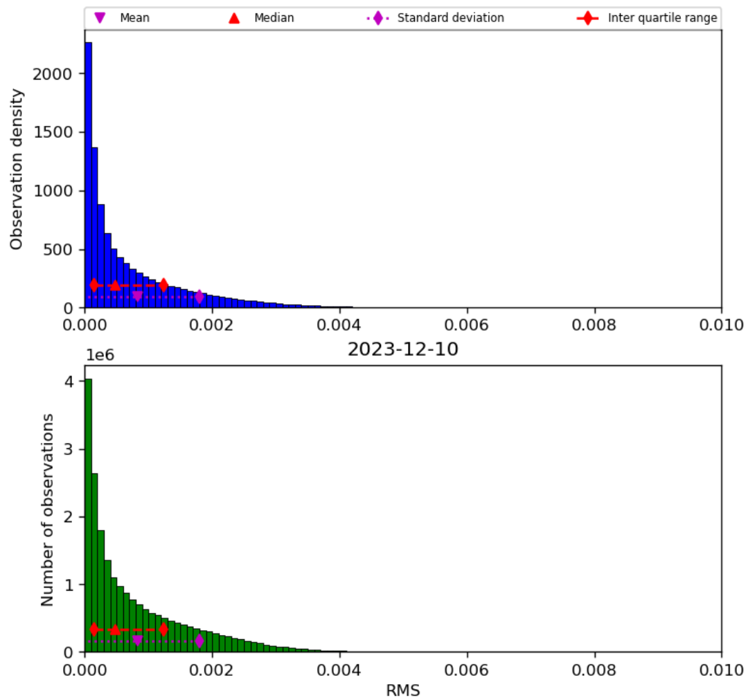
Figure 47: Histogram of “RMS” for 2023-12-09 to 2023-12-11
