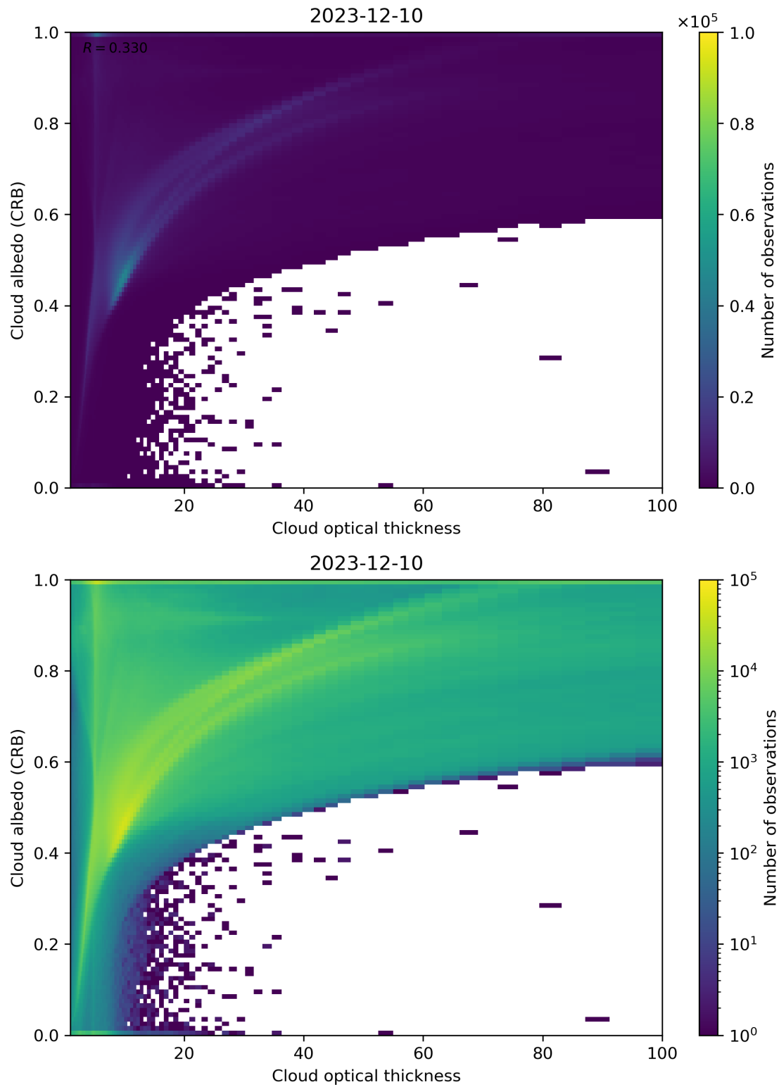
Figure 82: Scatter density plot of “Cloud optical thickness” against “Cloud albedo (CRB)” for 2023-12-09 to 2023-12-11.
