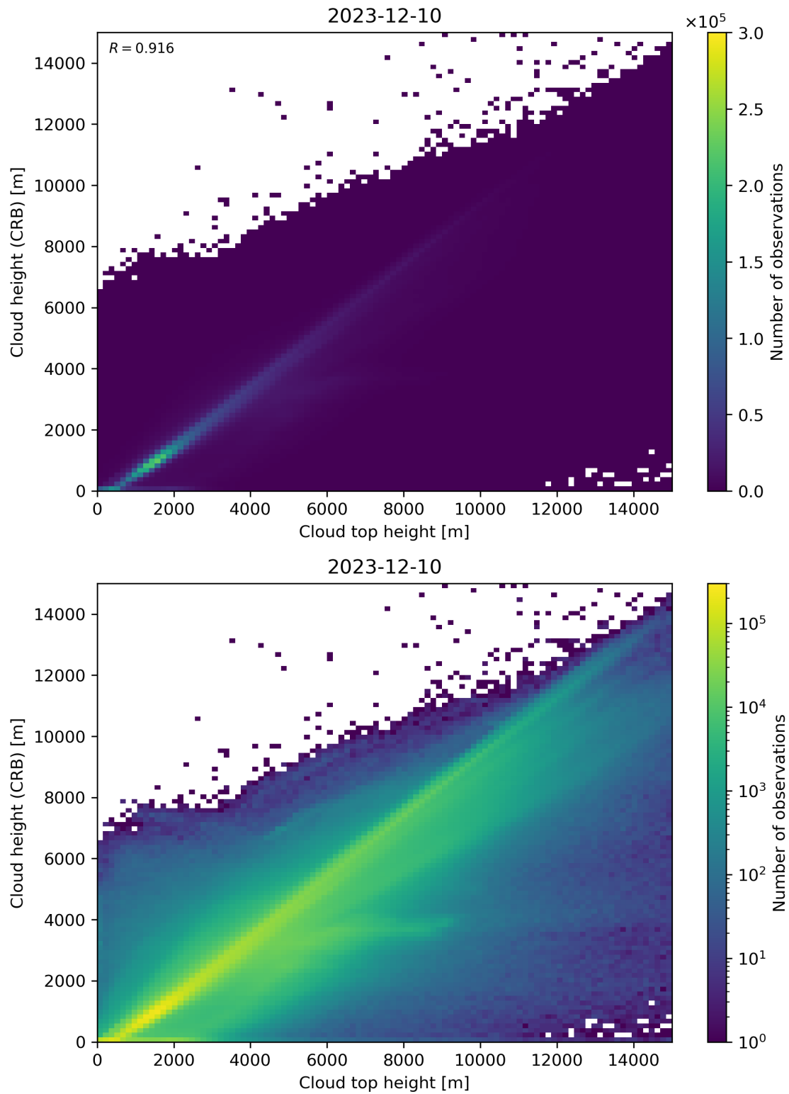
Figure 89: Scatter density plot of “Cloud top height” against “Cloud height (CRB)” for 2023-12-09 to 2023-12-11.
