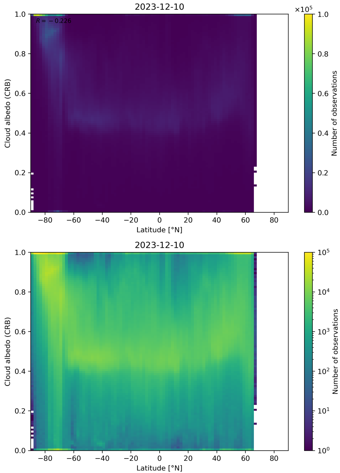
Figure 91: Scatter density plot of “Latitude” against “Cloud albedo (CRB)” for 2023-12-09 to 2023-12-11.
