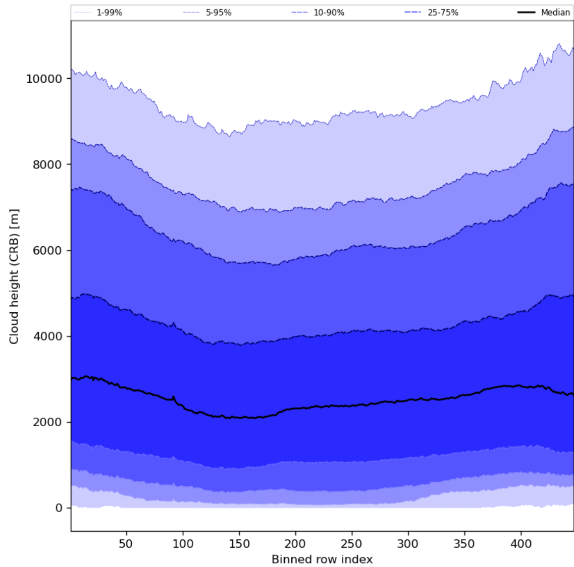
Figure 59: Along track statistics of “Cloud height (CRB)” for 2023-12-09 to 2023-12-11
