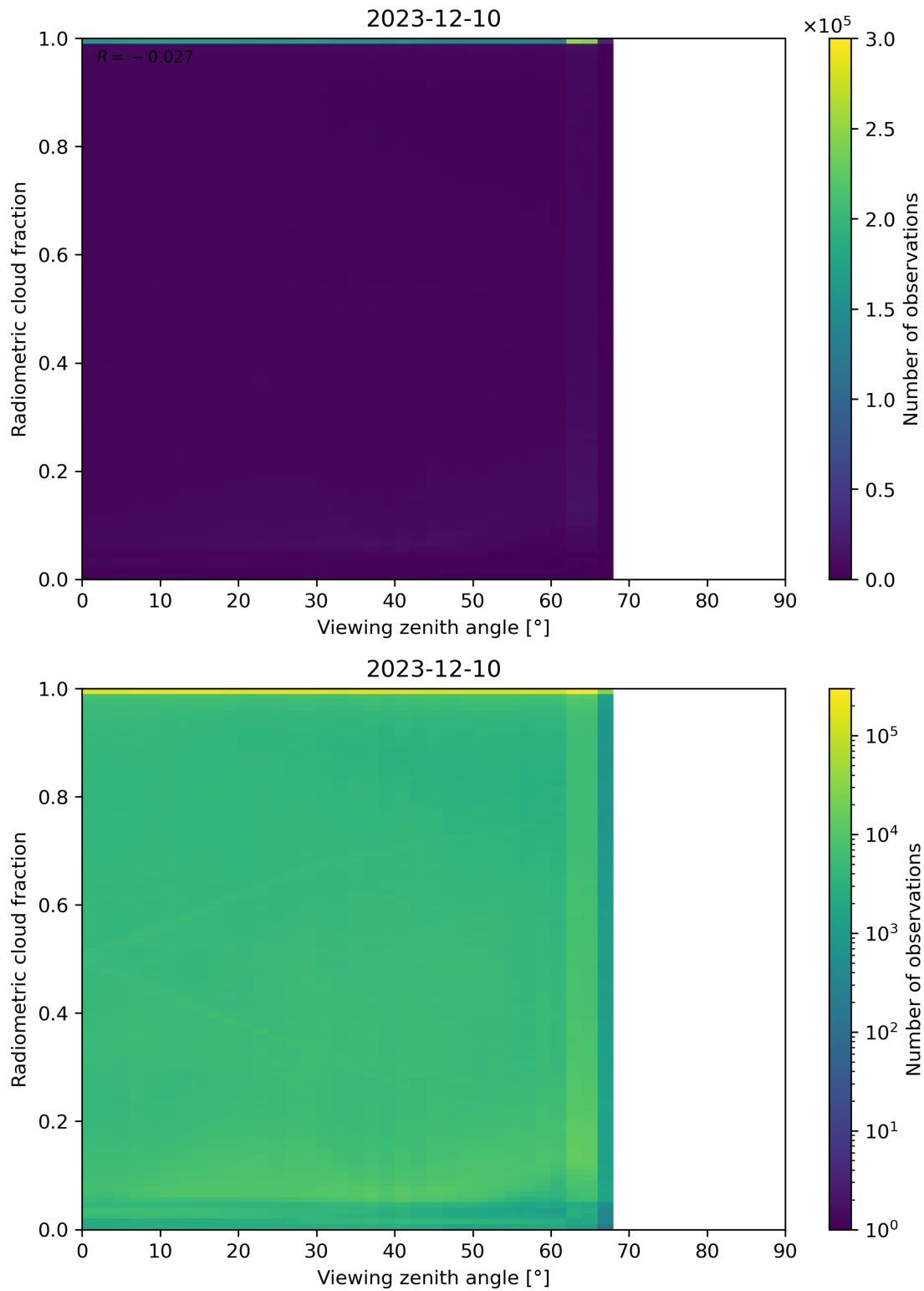
Figure 107: Scatter density plot of “Viewing zenith angle” against “Radiometric cloud fraction” for 2023-12-09 to 2023-12-11.
