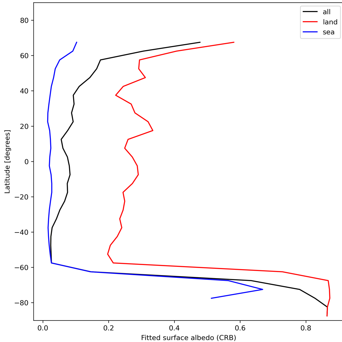
Figure 30: Zonal average of “Fitted surface albedo (CRB)” for 2023-12-09 to 2023-12-11.
