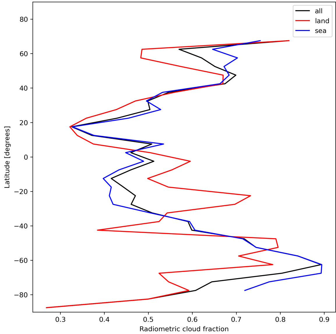
Figure 23: Zonal average of “Radiometric cloud fraction” for 2023-12-09 to 2023-12-11.
