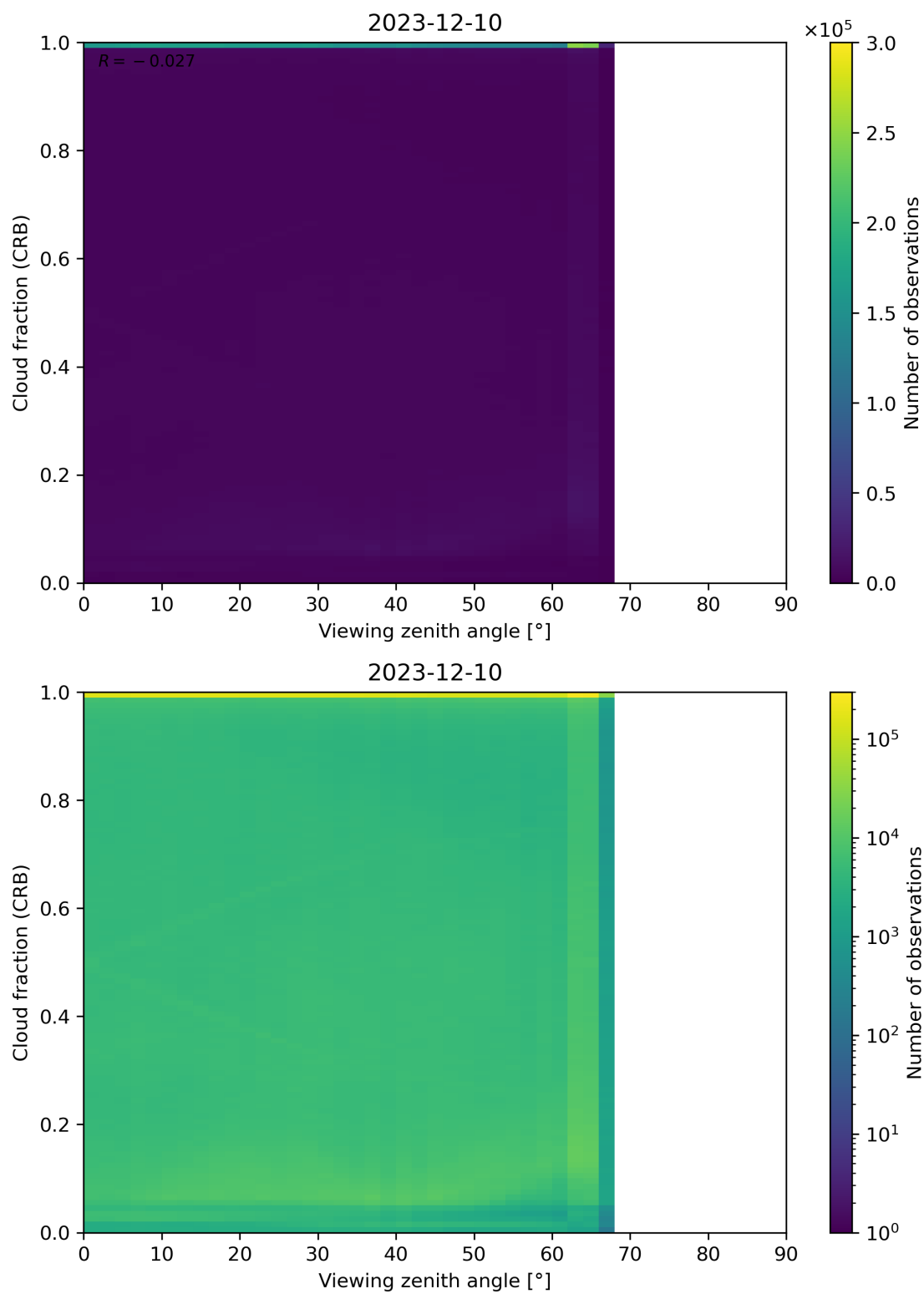
Figure 109: Scatter density plot of “Viewing zenith angle” against “Cloud fraction (CRB)” for 2023-12-09 to 2023-12-11.
