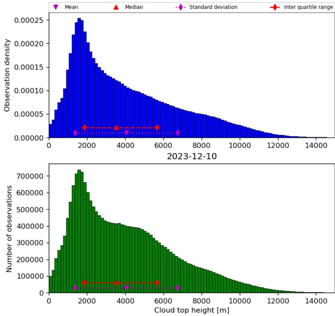
Figure 40: Histogram of “Cloud top height” for 2023-12-09 to 2023-12-11
