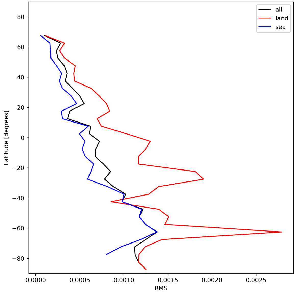
Figure 31: Zonal average of “RMS” for 2023-12-09 to 2023-12-11.
