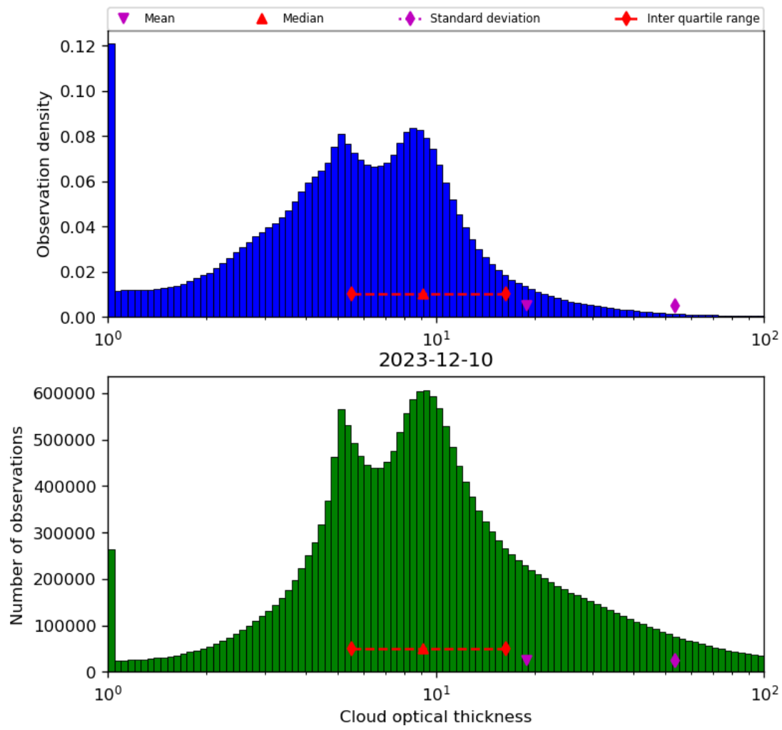
Figure 41: Histogram of “Cloud optical thickness” for 2023-12-09 to 2023-12-11
