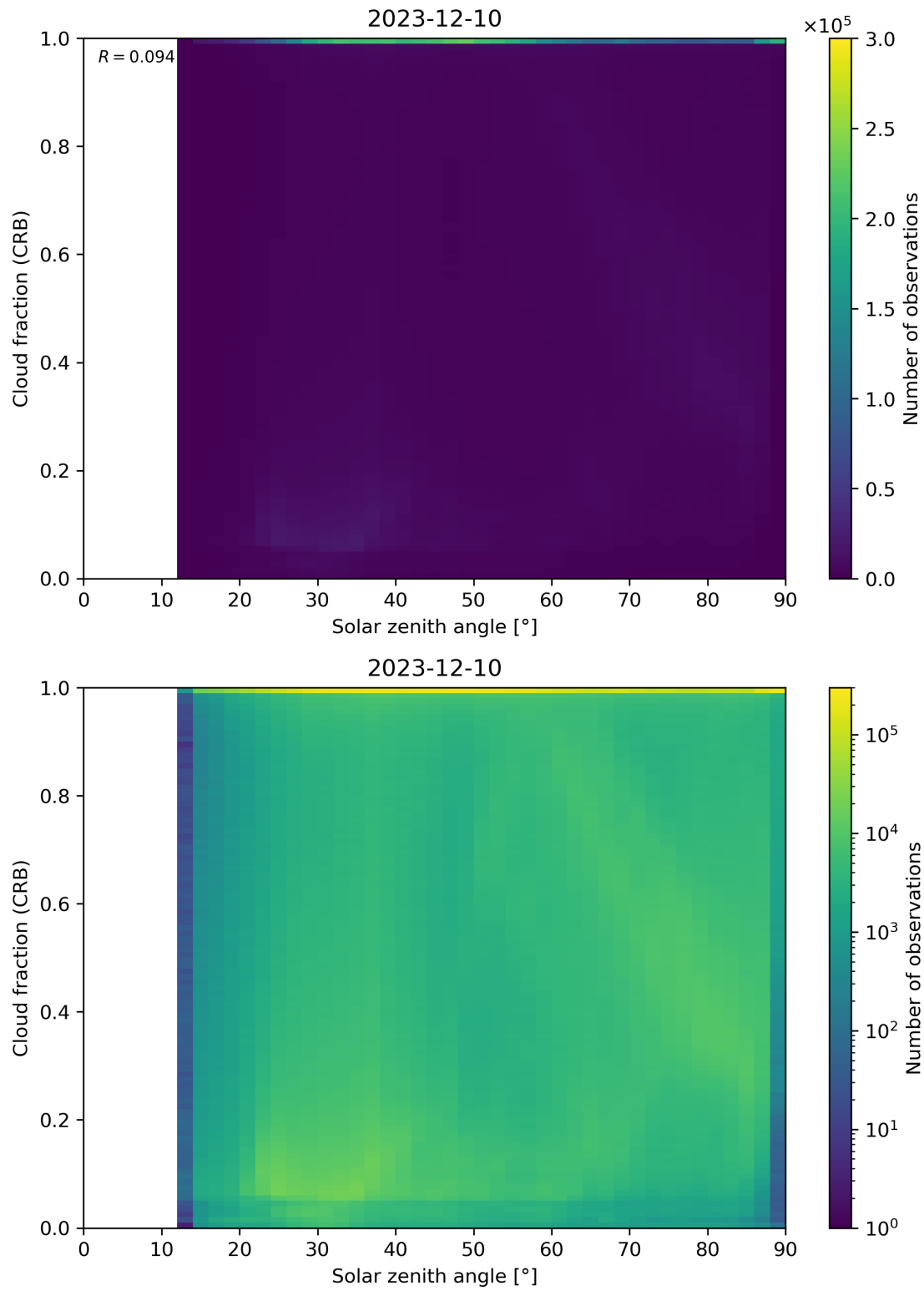
Figure 101: Scatter density plot of “Solar zenith angle” against “Cloud fraction (CRB)” for 2023-12-09 to 2023-12-11.
