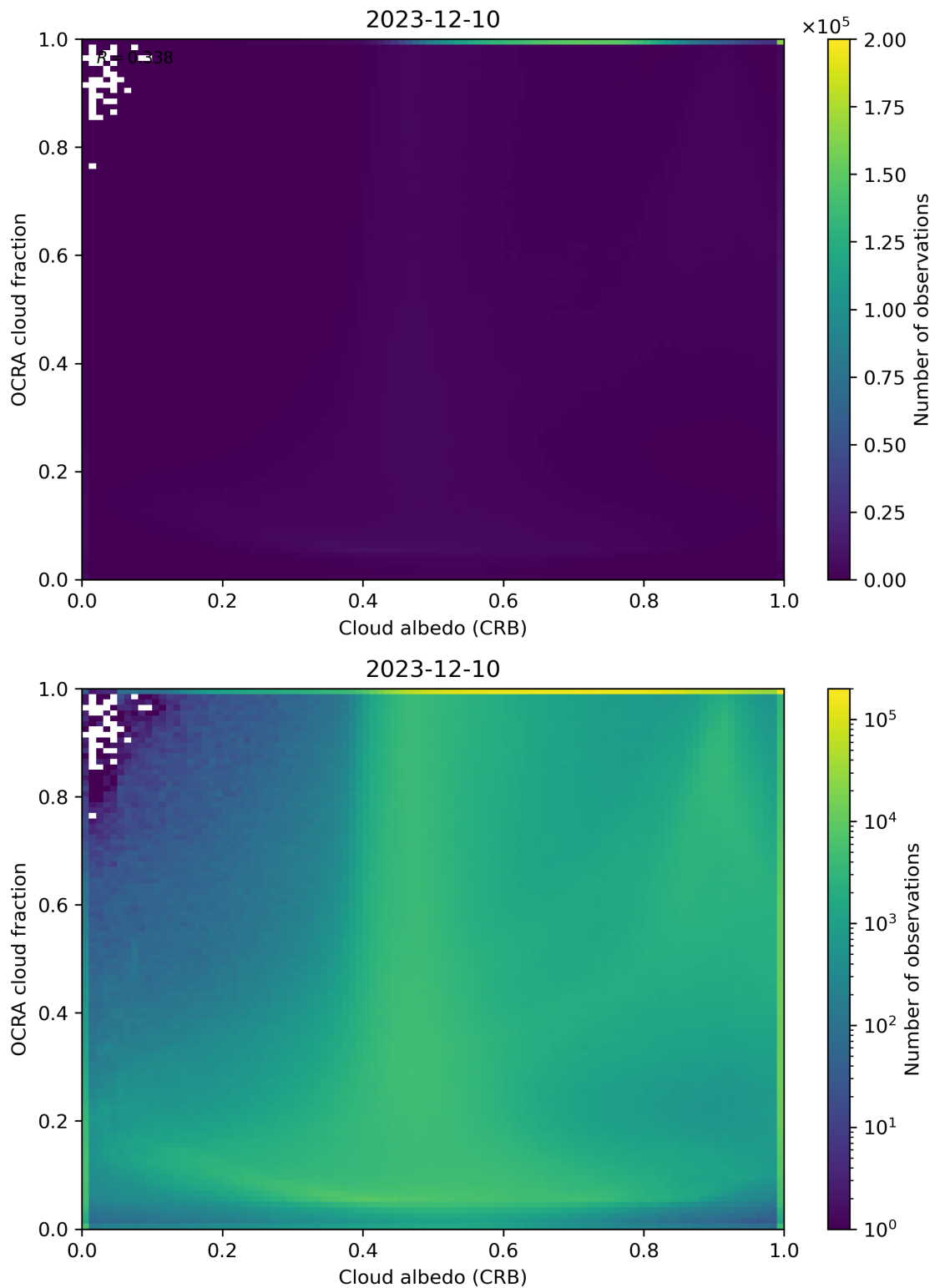
Figure 70: Scatter density plot of “Cloud albedo (CRB)” against “OCRA cloud fraction” for 2023-12-09 to 2023-12-11.
