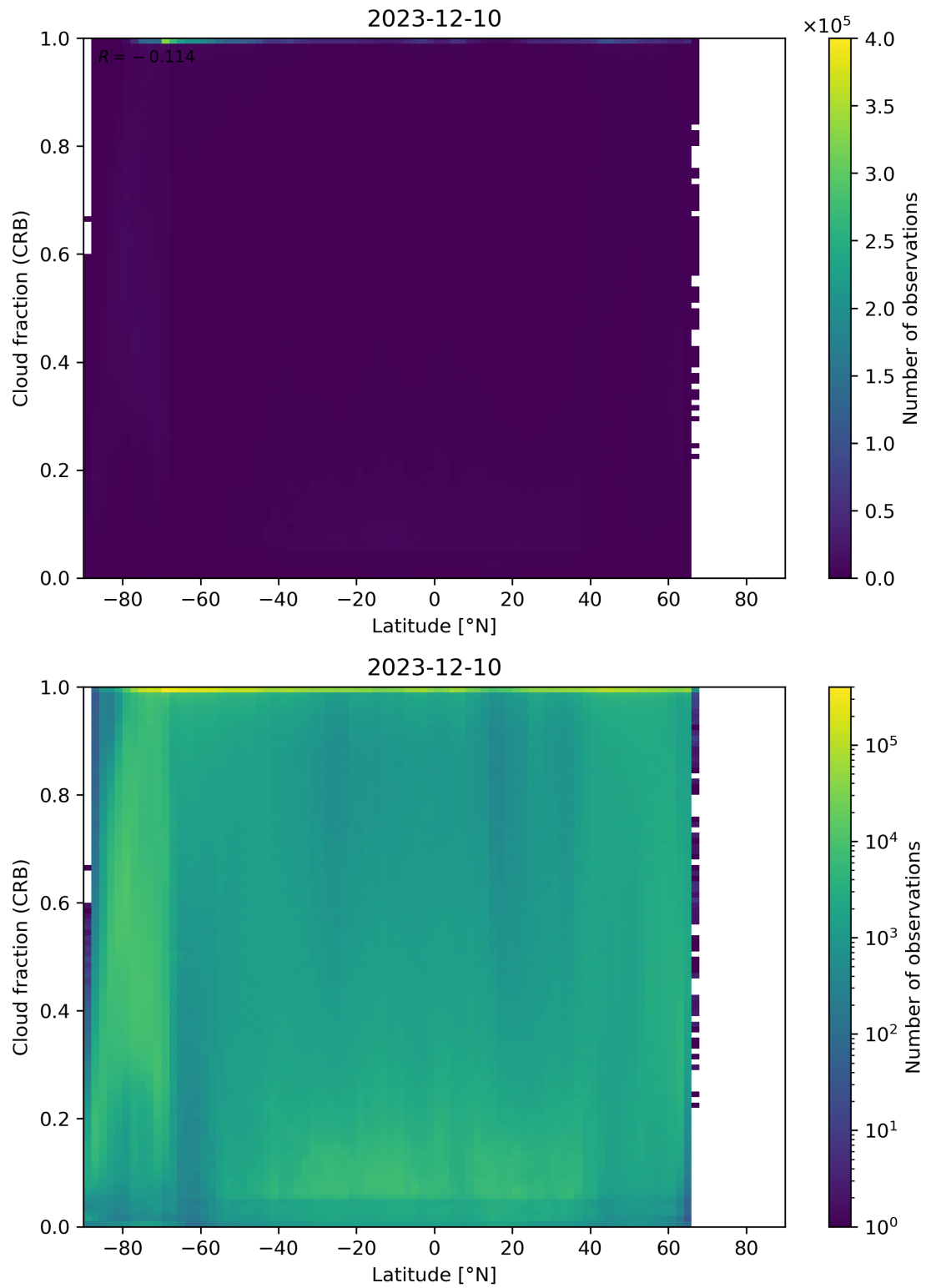
Figure 94: Scatter density plot of “Latitude” against “Cloud fraction (CRB)” for 2023-12-09 to 2023-12-11.
