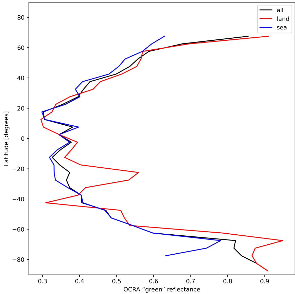
Figure 36: Zonal average of “OCRA “green” reflectance” for 2023-12-09 to 2023-12-11.
