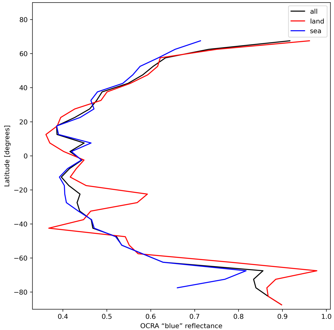
Figure 35: Zonal average of “OCRA “blue” reflectance” for 2023-12-09 to 2023-12-11.
