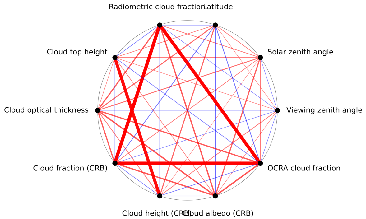
Figure 1: Map of correlation graph for 2023-12-09 to 2023-12-11.
