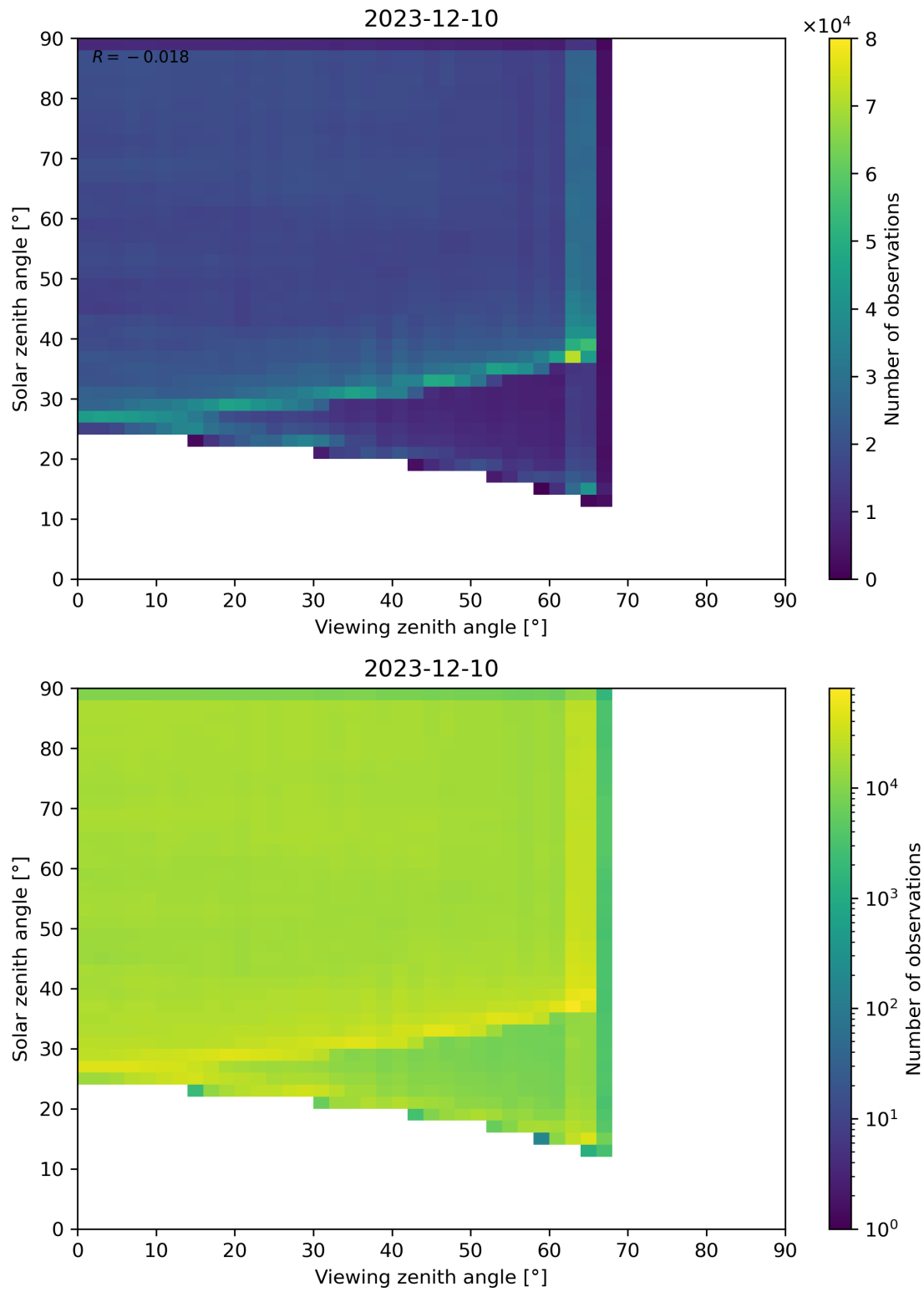
Figure 114: Scatter density plot of “Viewing zenith angle” against “Solar zenith angle” for 2023-12-09 to 2023-12-11.
