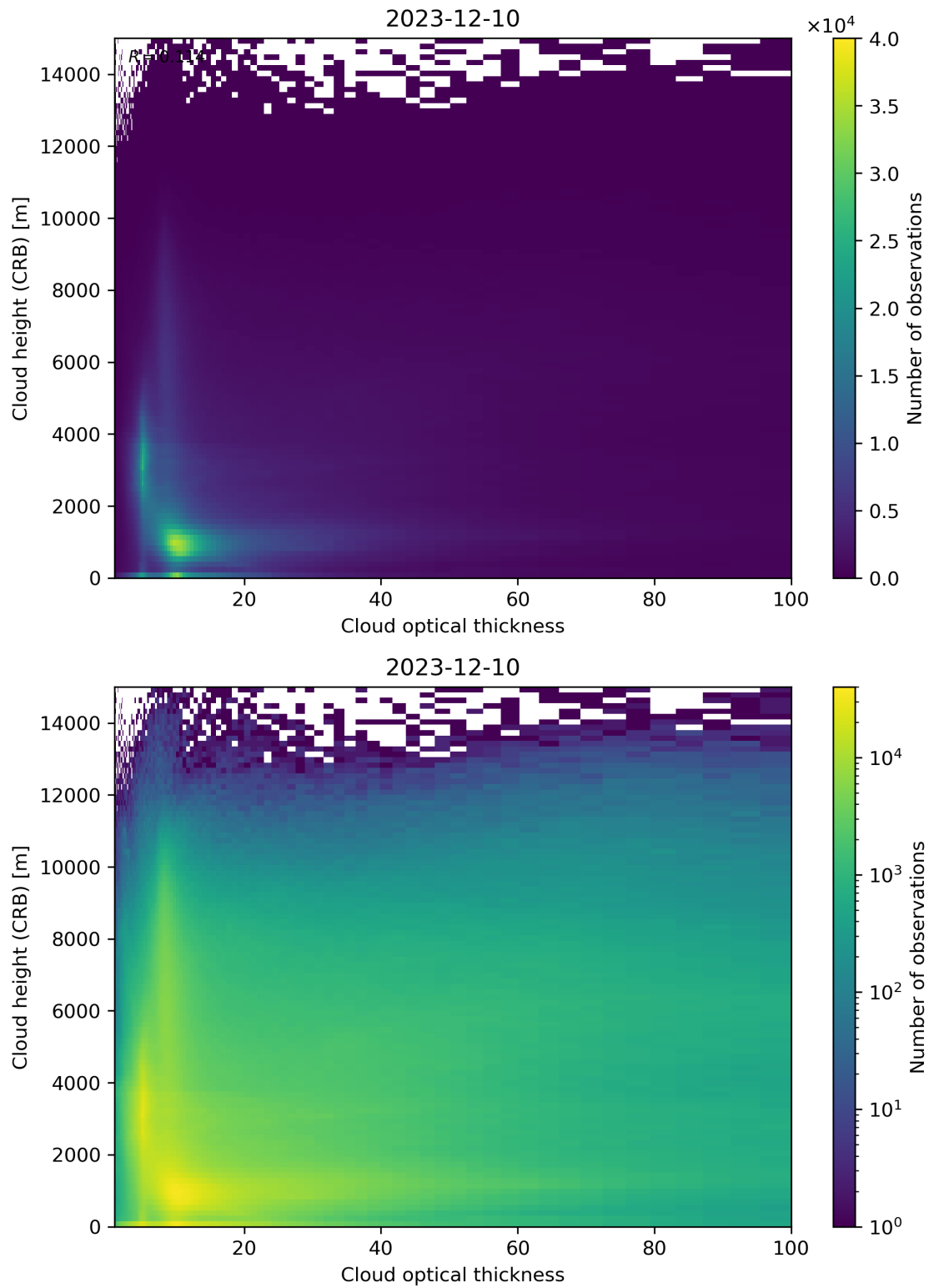
Figure 85: Scatter density plot of “Cloud optical thickness” against “Cloud height (CRB)” for 2023-12-09 to 2023-12-11.
