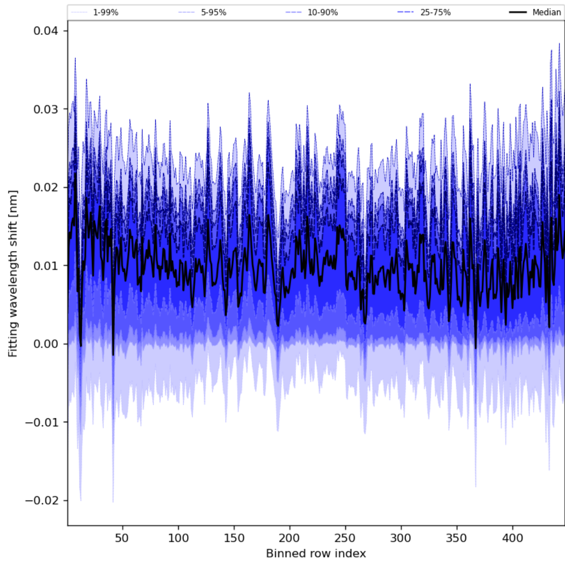
Figure 65: Along track statistics of “Fitting wavelength shift” for 2023-12-09 to 2023-12-11
