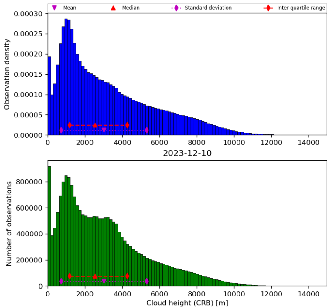
Figure 43: Histogram of “Cloud height (CRB)” for 2023-12-09 to 2023-12-11
