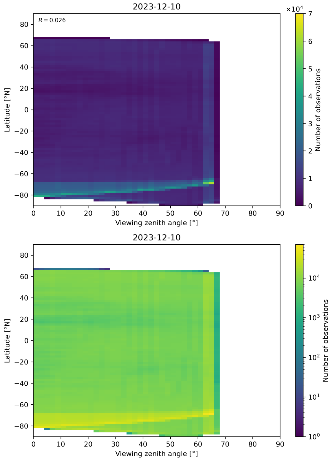
Figure 113: Scatter density plot of “Viewing zenith angle” against “Latitude” for 2023-12-09 to 2023-12-11.
