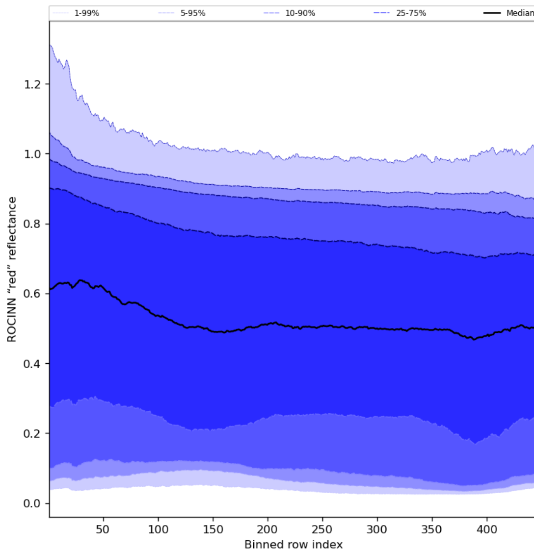
Figure 69: Along track statistics of “ROCINN “red” reflectance” for 2023-12-09 to 2023-12-11
