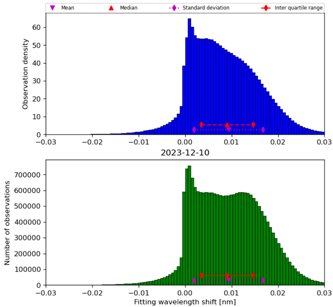
Figure 49: Histogram of “Fitting wavelength shift” for 2023-12-09 to 2023-12-11
