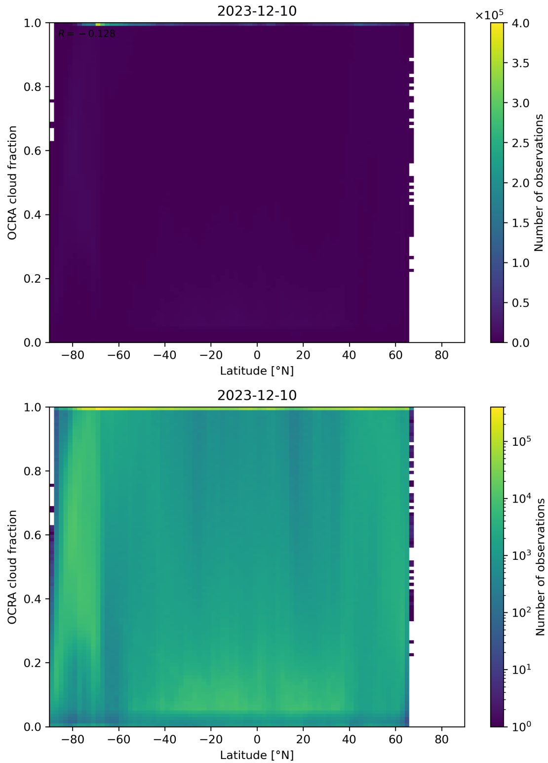
Figure 93: Scatter density plot of “Latitude” against “OCRA cloud fraction” for 2023-12-09 to 2023-12-11.
