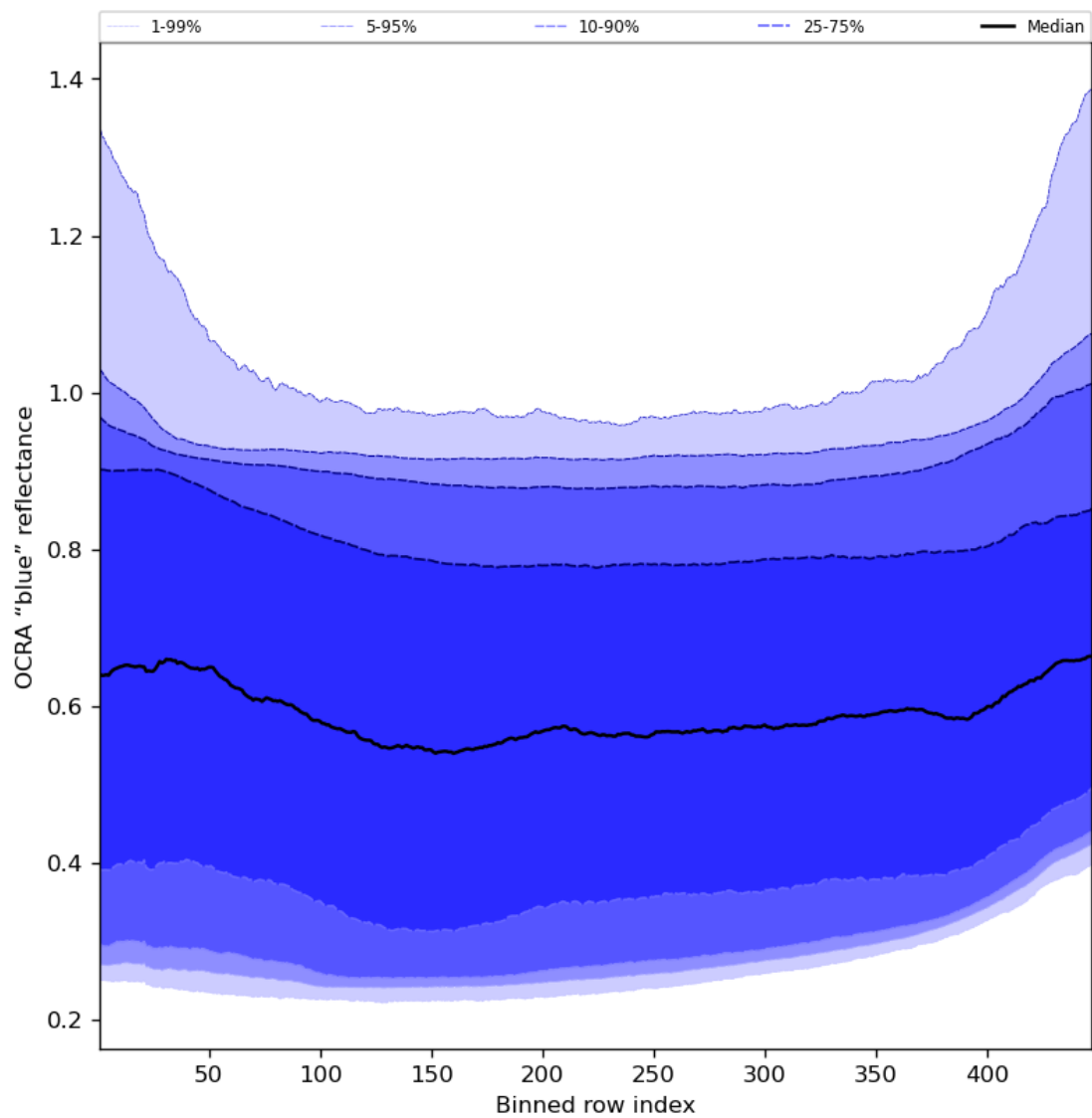
Figure 67: Along track statistics of “OCRA “blue” reflectance” for 2023-12-09 to 2023-12-11
