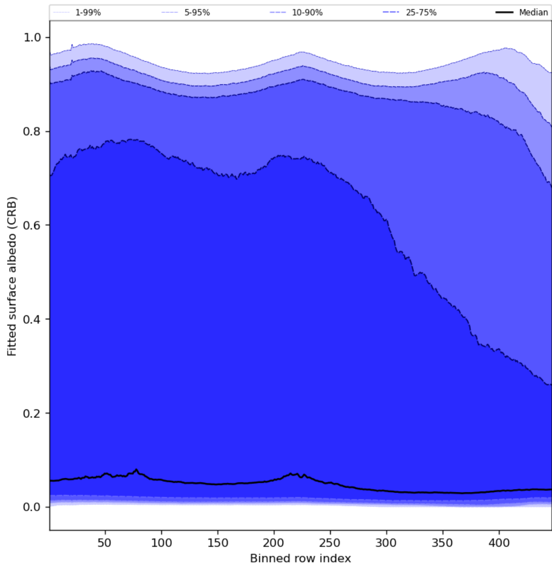
Figure 62: Along track statistics of “Fitted surface albedo (CRB)” for 2023-12-09 to 2023-12-11
