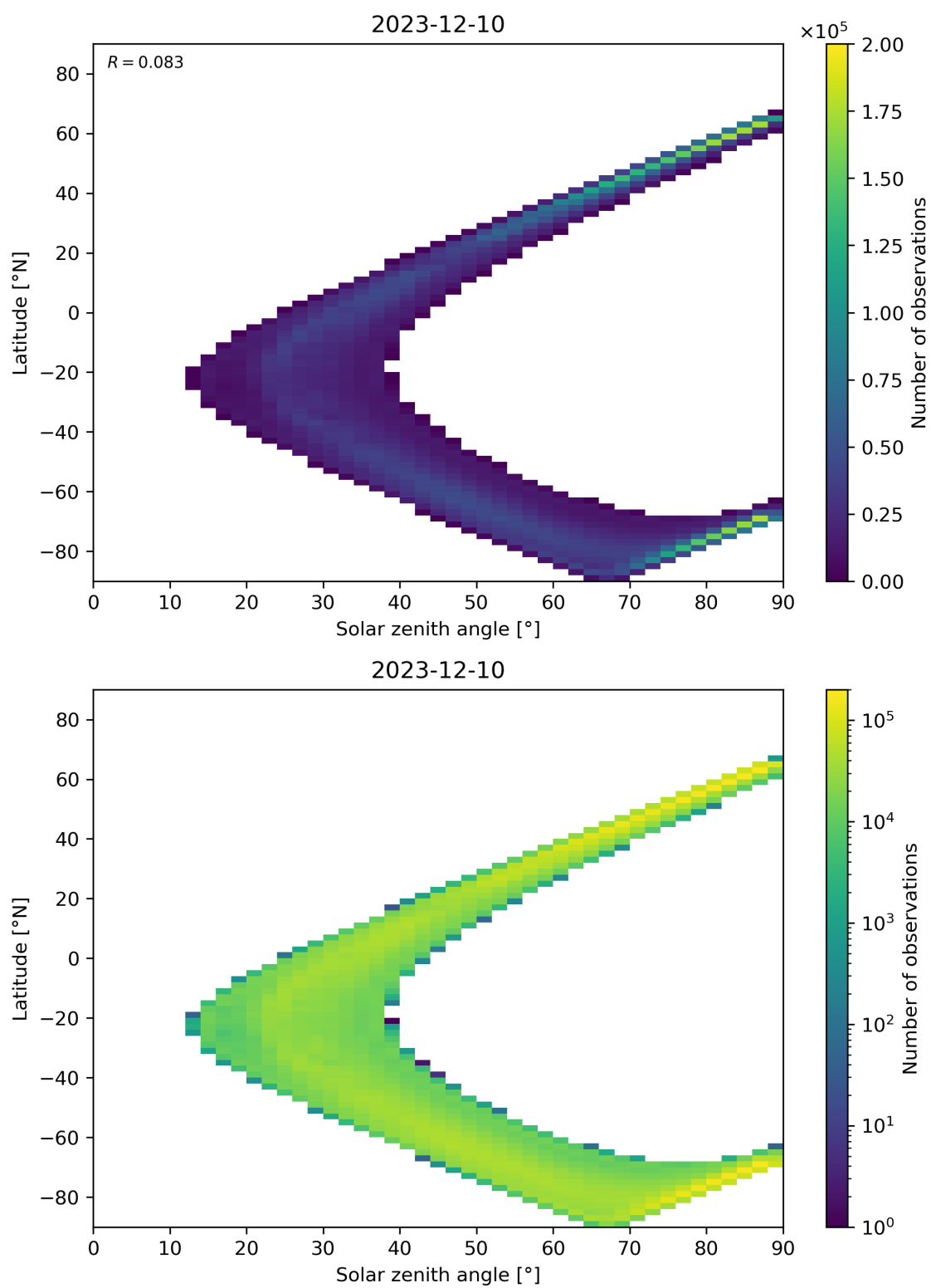
Figure 105: Scatter density plot of “Solar zenith angle” against “Latitude” for 2023-12-09 to 2023-12-11.
