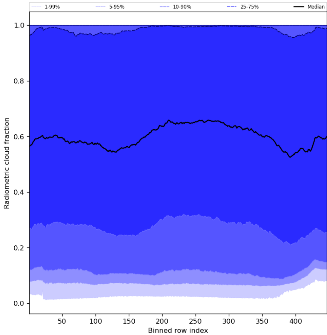
Figure 55: Along track statistics of “Radiometric cloud fraction” for 2023-12-09 to 2023-12-11
