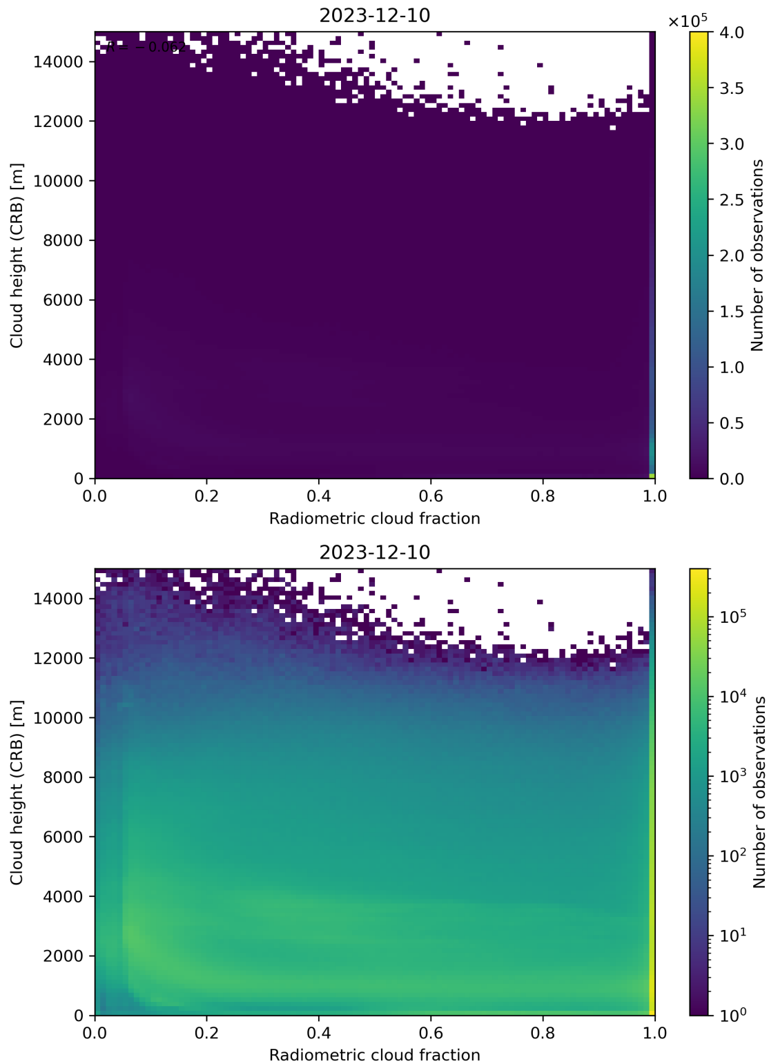
Figure 74: Scatter density plot of “Radiometric cloud fraction” against “Cloud height (CRB)” for 2023-12-09 to 2023-12-11.
