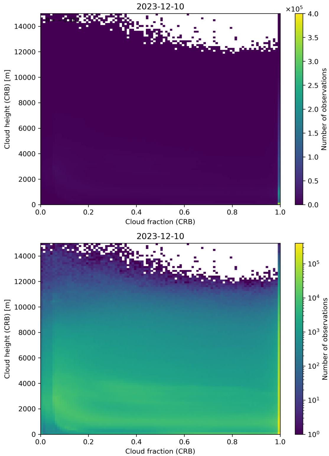
Figure 79: Scatter density plot of “Cloud fraction (CRB)” against “Cloud height (CRB)” for 2023-12-09 to 2023-12-11.
