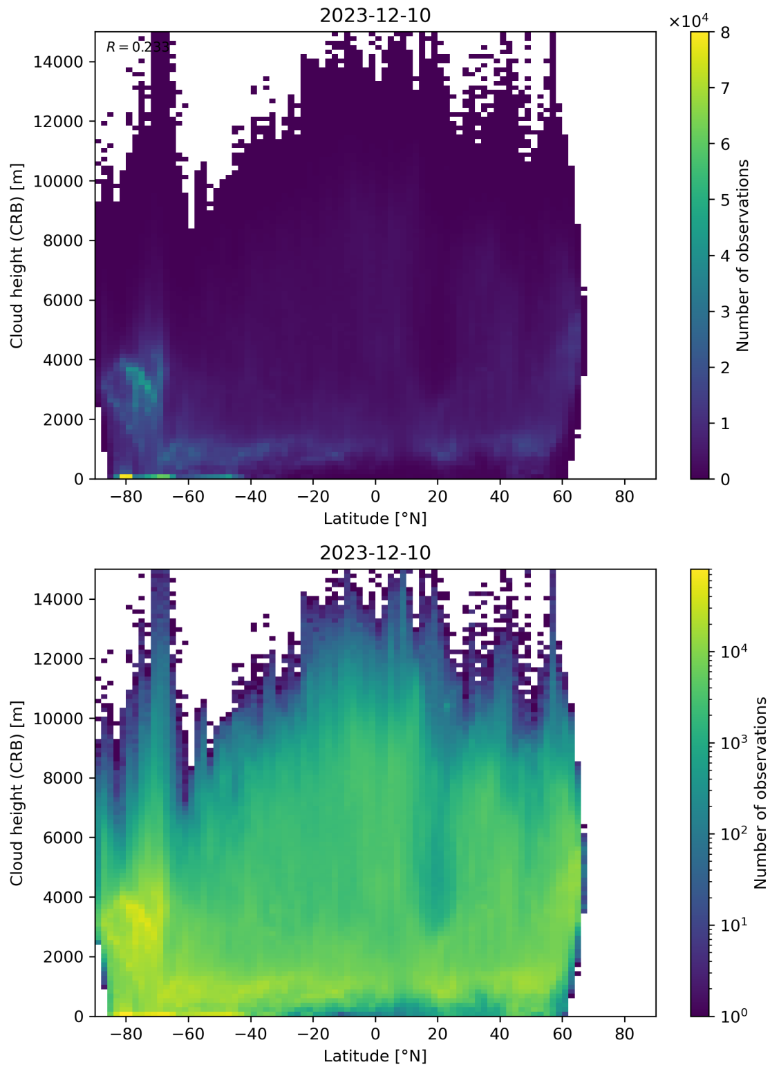
Figure 95: Scatter density plot of “Latitude” against “Cloud height (CRB)” for 2023-12-09 to 2023-12-11.
