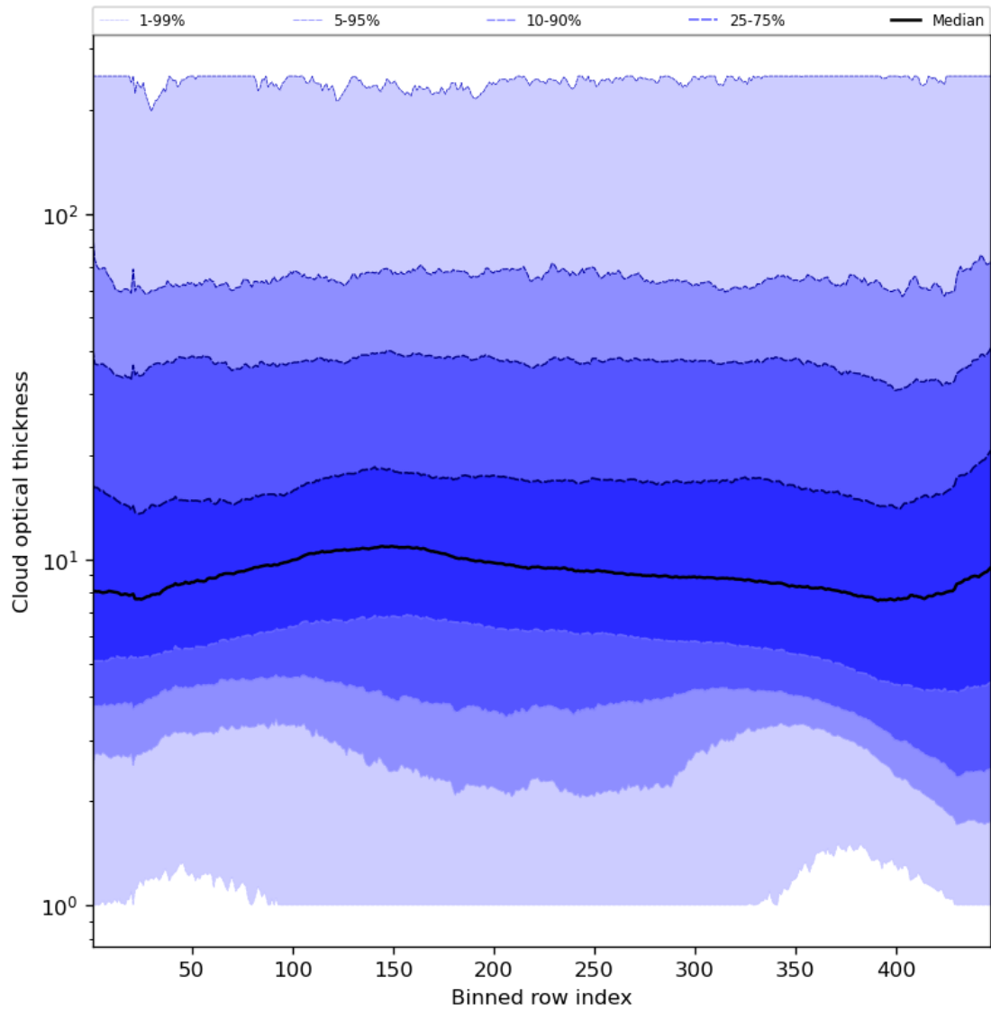
Figure 57: Along track statistics of “Cloud optical thickness” for 2023-12-09 to 2023-12-11
