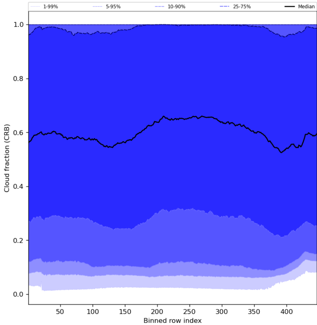
Figure 58: Along track statistics of “Cloud fraction (CRB)” for 2023-12-09 to 2023-12-11
