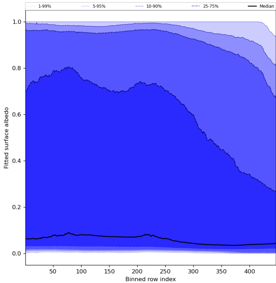
Figure 61: Along track statistics of “Fitted surface albedo” for 2023-12-09 to 2023-12-11
