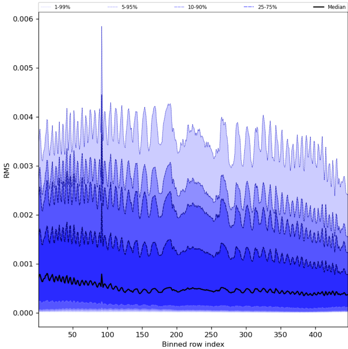
Figure 63: Along track statistics of “RMS” for 2023-12-09 to 2023-12-11
