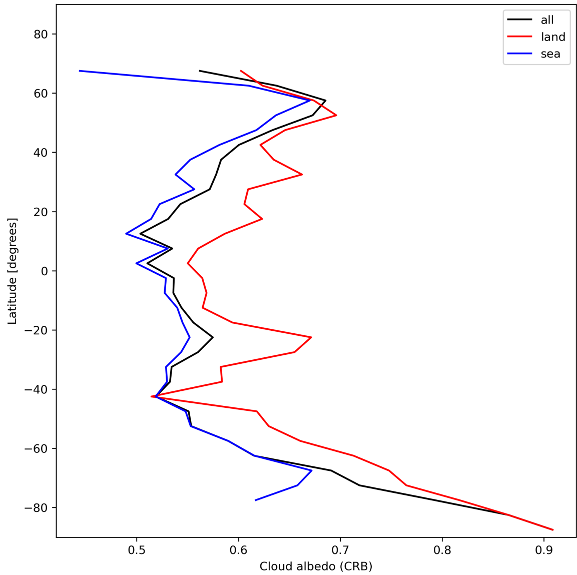
Figure 28: Zonal average of “Cloud albedo (CRB)” for 2023-12-09 to 2023-12-11.
