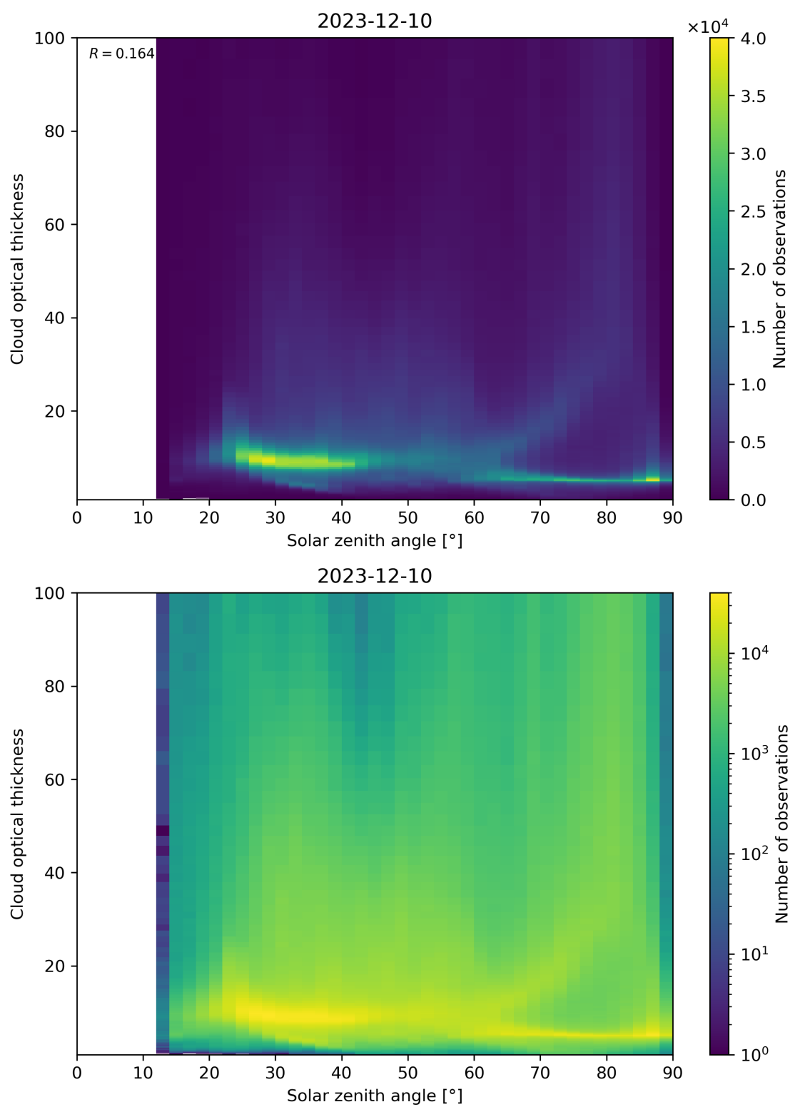
Figure 103: Scatter density plot of “Solar zenith angle” against “Cloud optical thickness” for 2023-12-09 to 2023-12-11.
