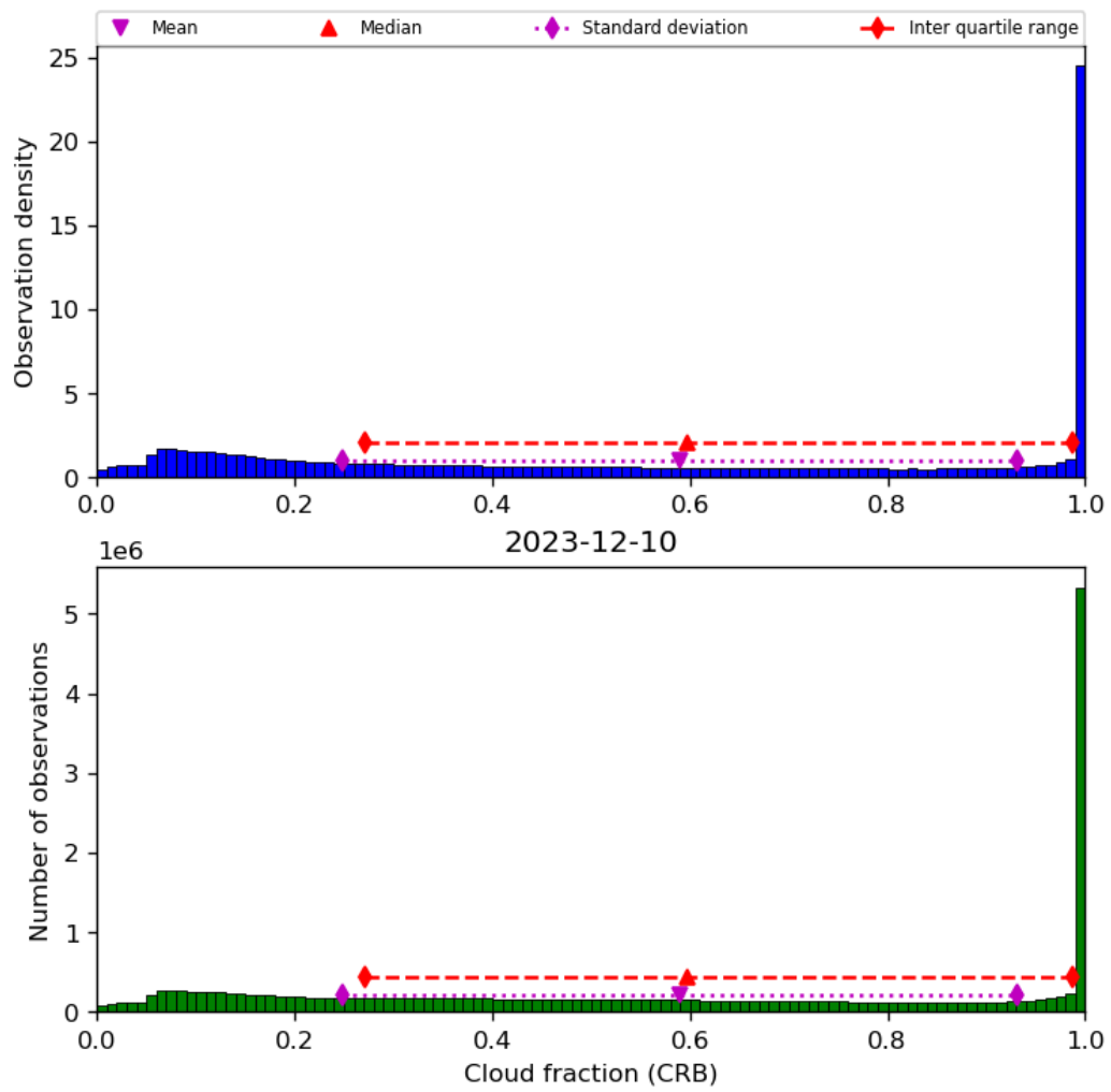
Figure 42: Histogram of “Cloud fraction (CRB)” for 2023-12-09 to 2023-12-11
