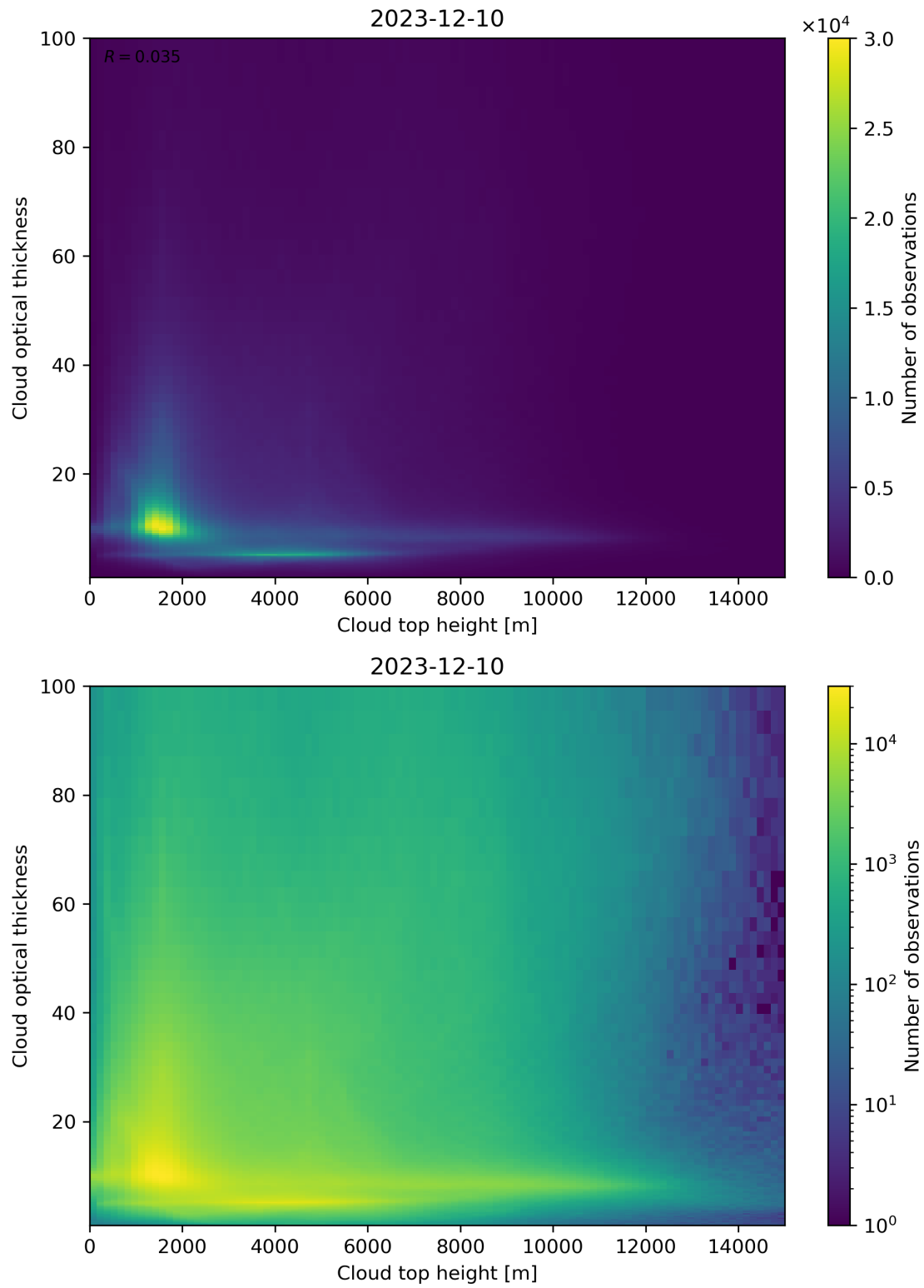
Figure 90: Scatter density plot of “Cloud top height” against “Cloud optical thickness” for 2023-12-09 to 2023-12-11.
