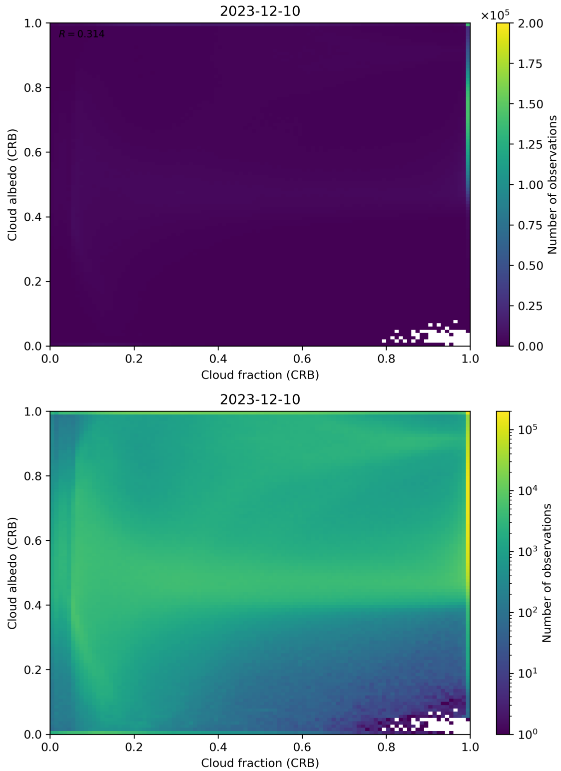
Figure 77: Scatter density plot of “Cloud fraction (CRB)” against “Cloud albedo (CRB)” for 2023-12-09 to 2023-12-11.
