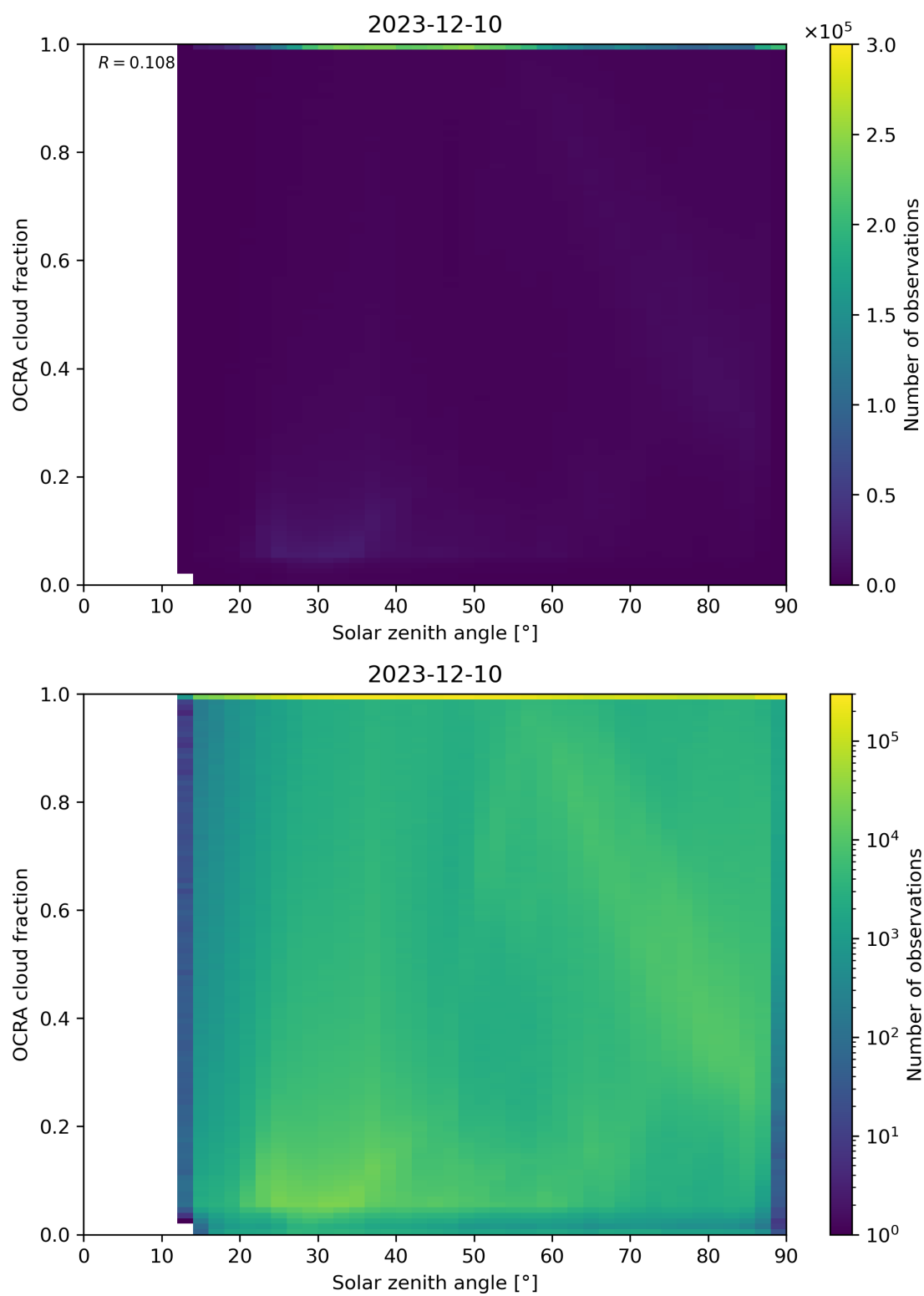
Figure 100: Scatter density plot of “Solar zenith angle” against “OCRA cloud fraction” for 2023-12-09 to 2023-12-11.
