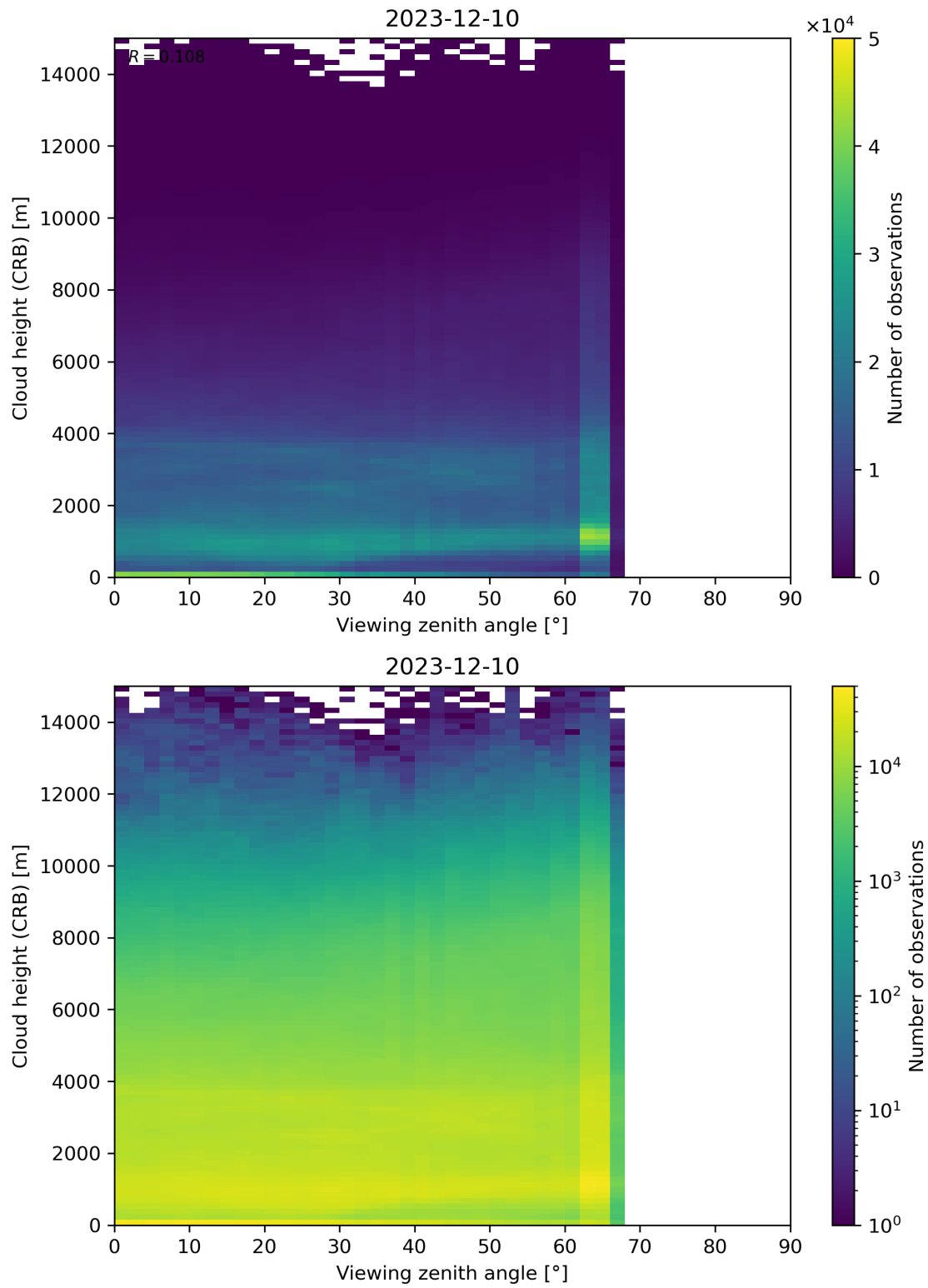
Figure 110: Scatter density plot of “Viewing zenith angle” against “Cloud height (CRB)” for 2023-12-09 to 2023-12-11.
