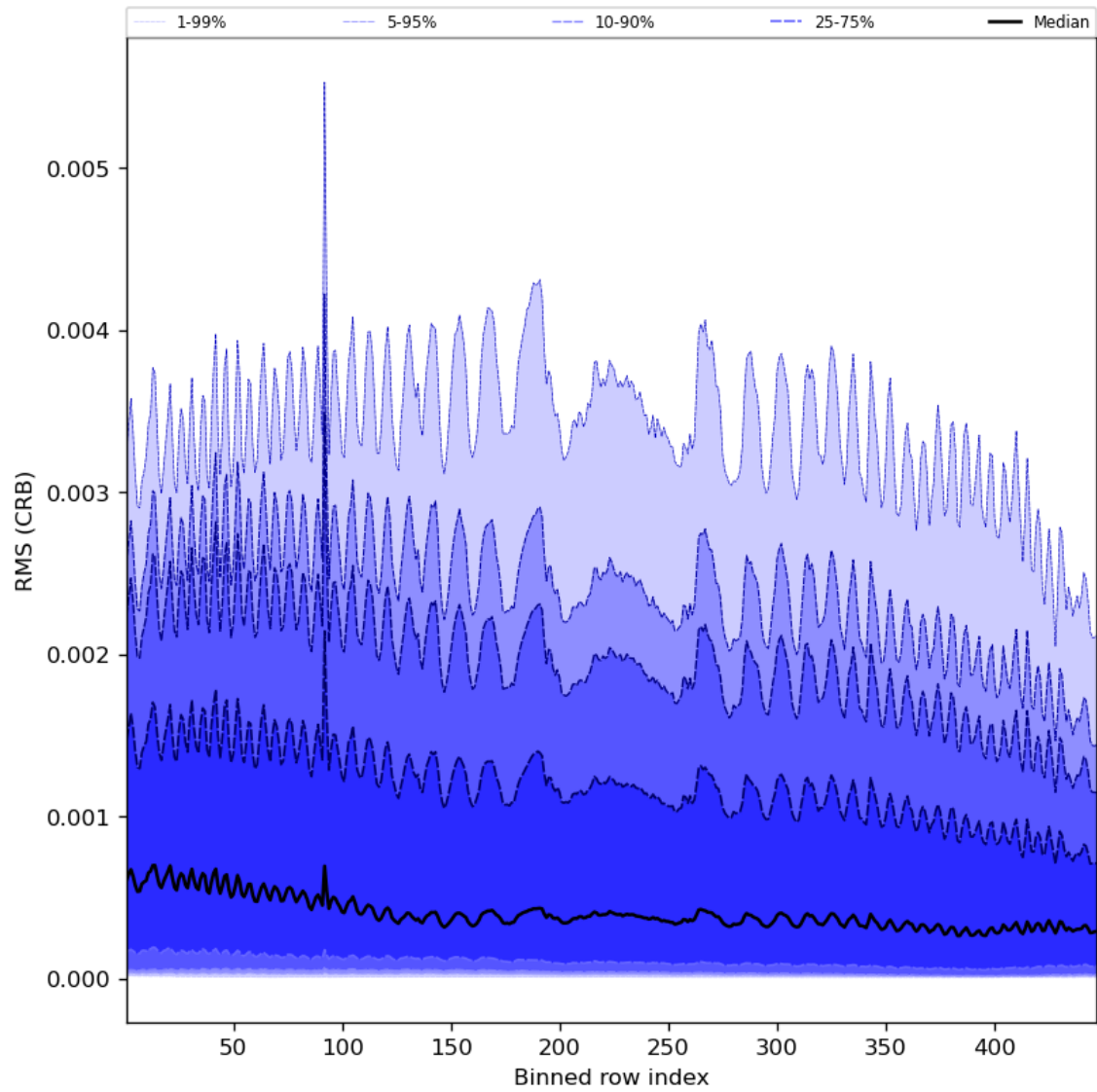
Figure 64: Along track statistics of “RMS (CRB)” for 2023-12-09 to 2023-12-11
