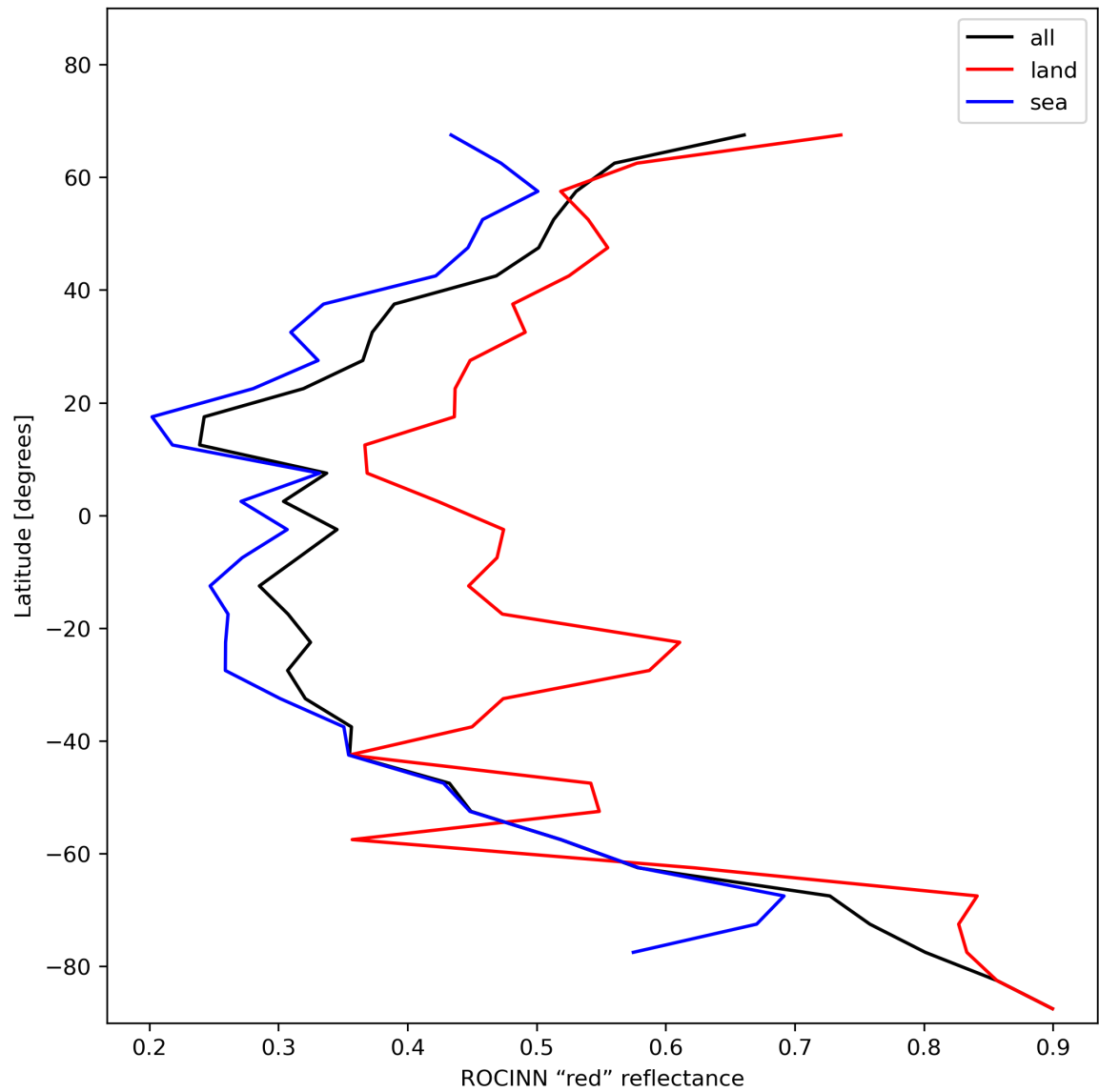
Figure 37: Zonal average of “ROCINN “red” reflectance” for 2023-12-09 to 2023-12-11.
