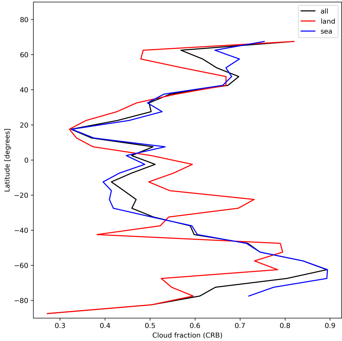
Figure 26: Zonal average of “Cloud fraction (CRB)” for 2023-12-09 to 2023-12-11.
