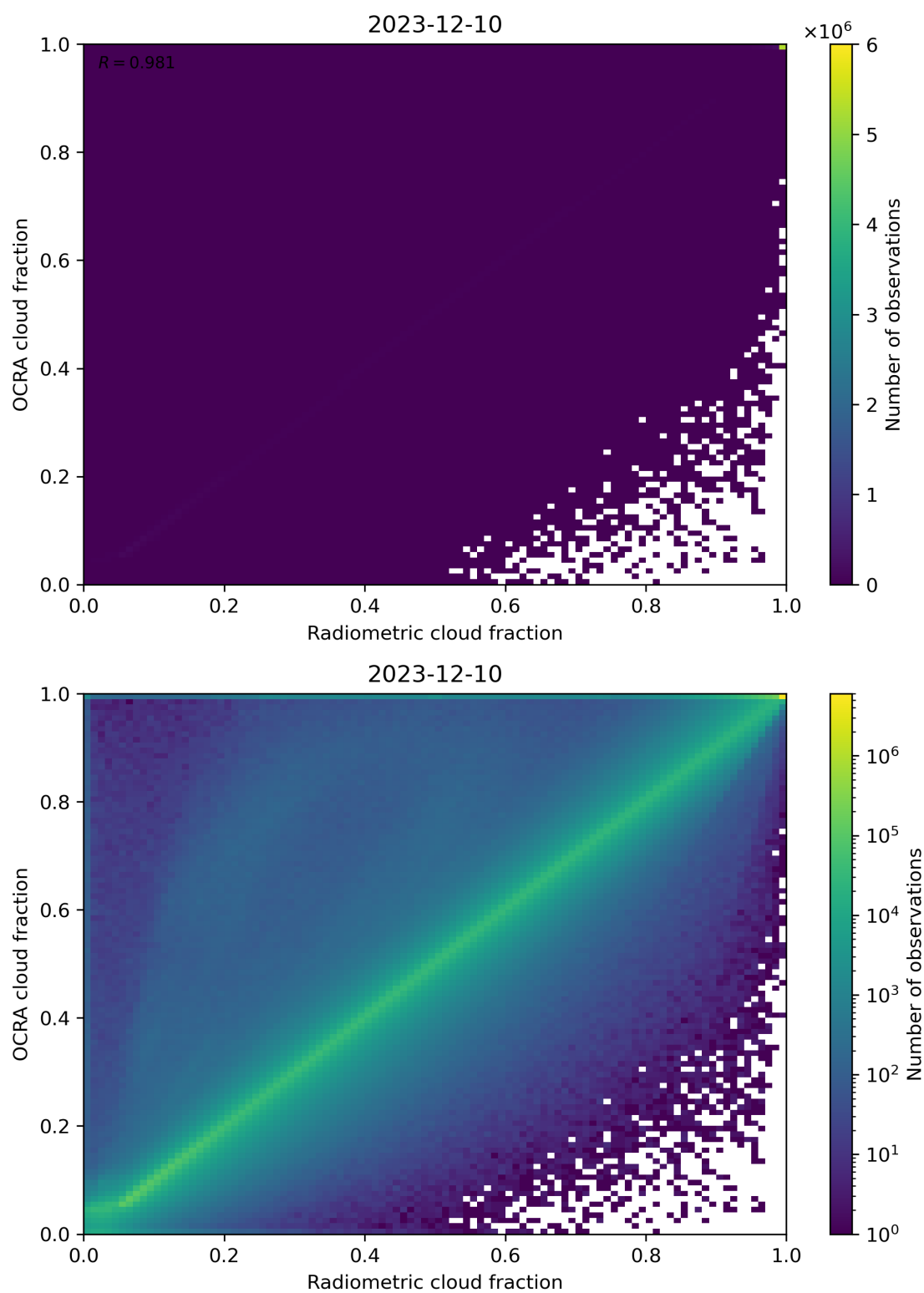
Figure 72: Scatter density plot of “Radiometric cloud fraction” against “OCRA cloud fraction” for 2023-12-09 to 2023-12-11.
