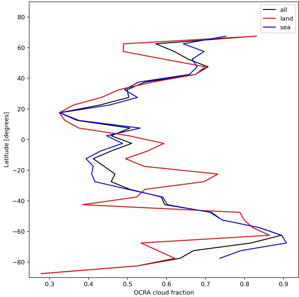
Figure 34: Zonal average of “OCRA cloud fraction” for 2023-12-09 to 2023-12-11.
