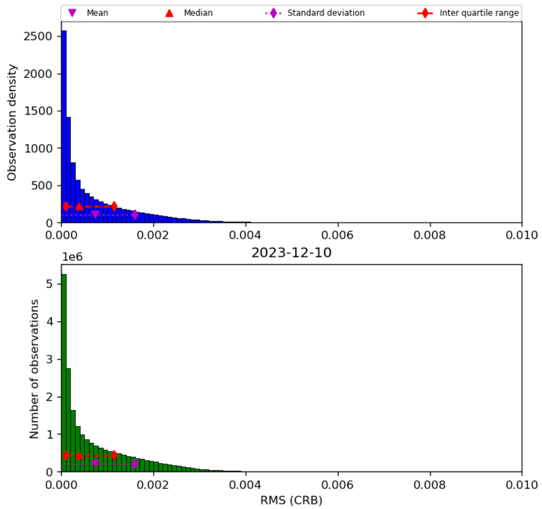
Figure 48: Histogram of “RMS (CRB)” for 2023-12-09 to 2023-12-11
