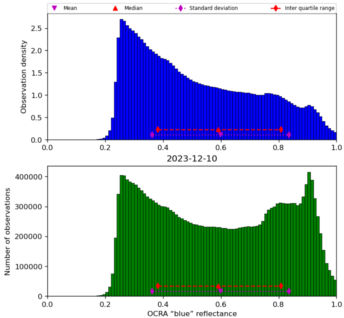
Figure 51: Histogram of “OCRA “blue” reflectance” for 2023-12-09 to 2023-12-11
