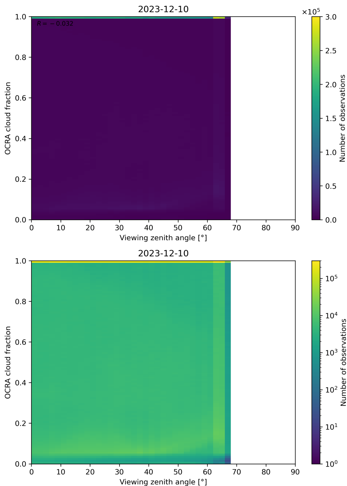
Figure 108: Scatter density plot of “Viewing zenith angle” against “OCRA cloud fraction” for 2023-12-09 to 2023-12-11.
