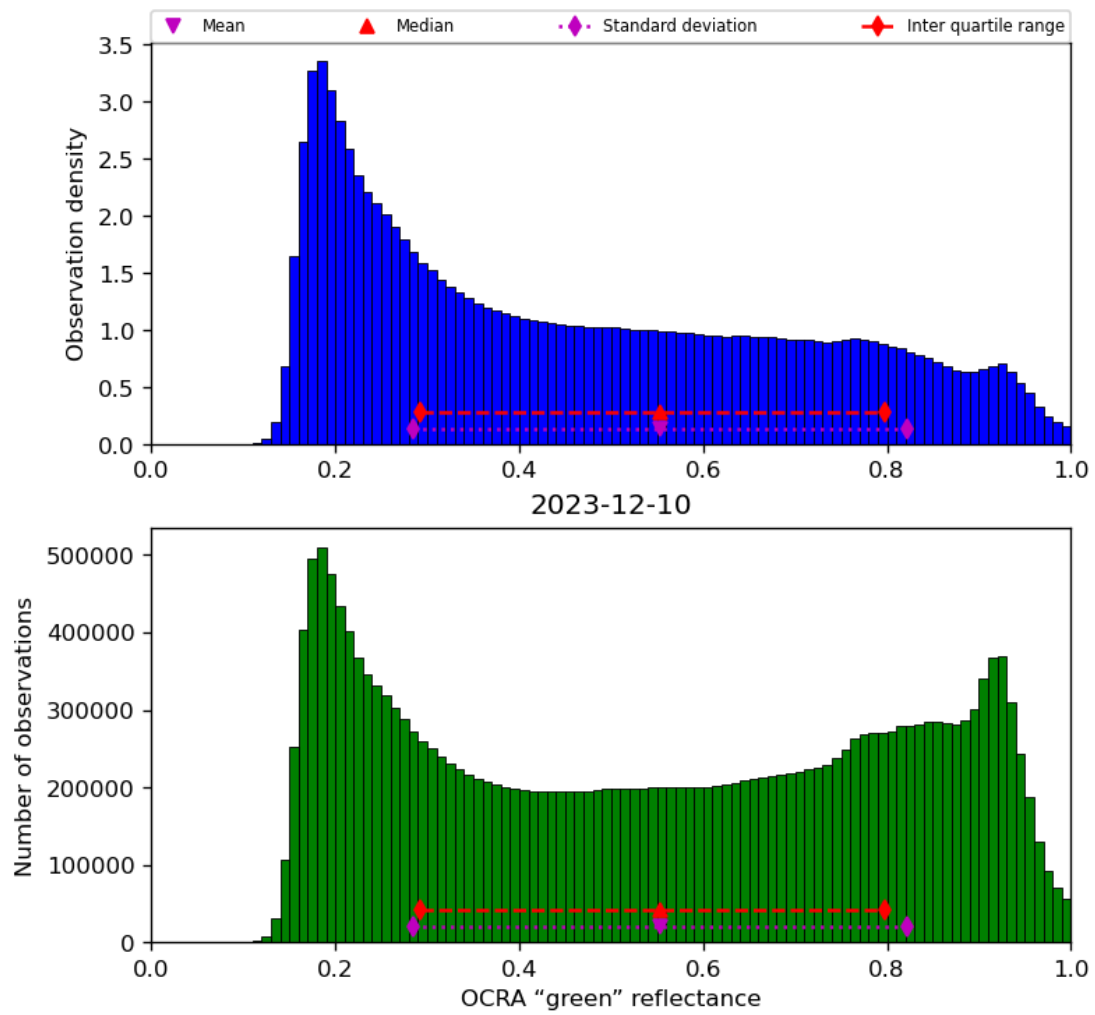
Figure 52: Histogram of “OCRA “green” reflectance” for 2023-12-09 to 2023-12-11
