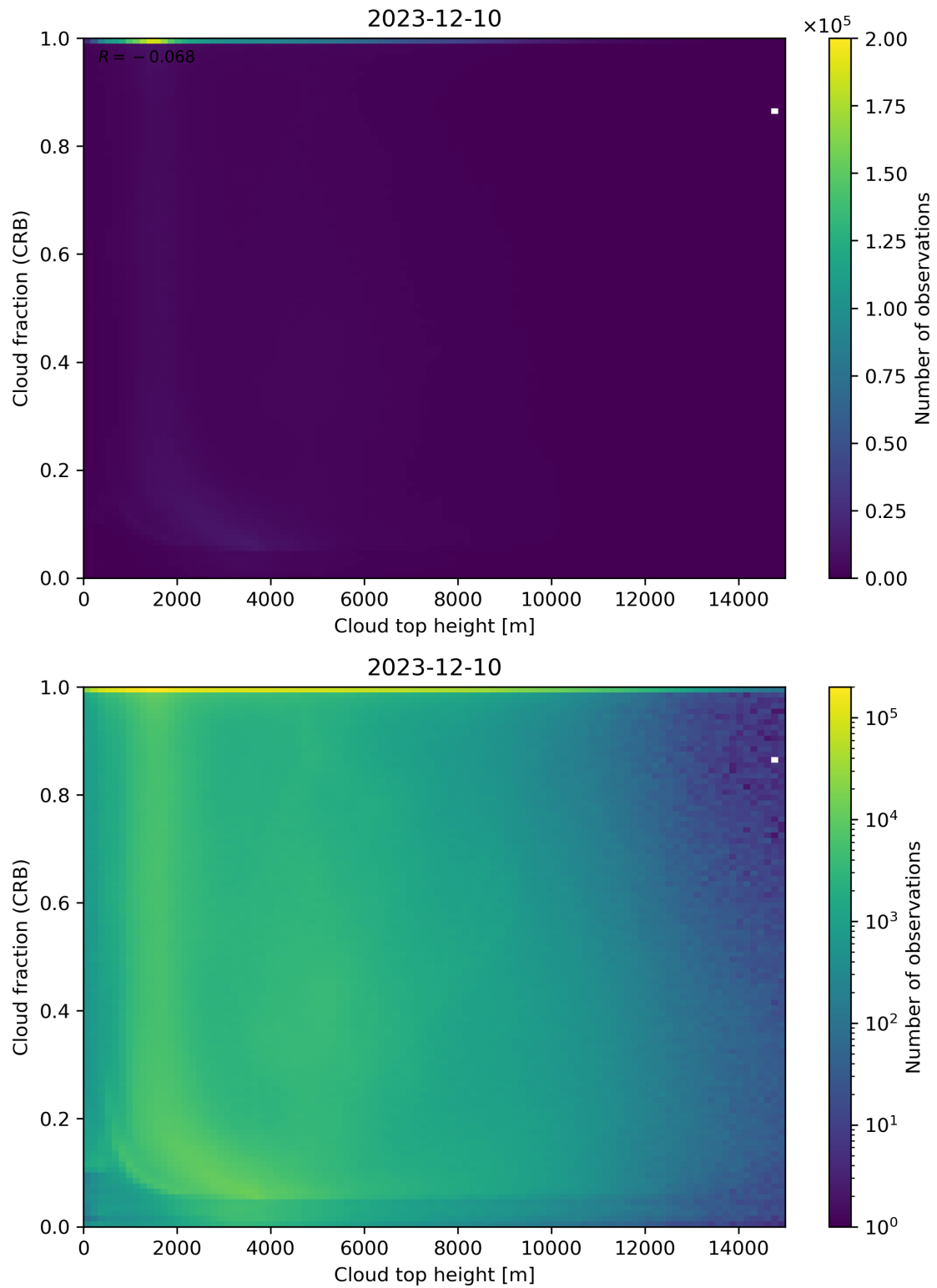
Figure 88: Scatter density plot of “Cloud top height” against “Cloud fraction (CRB)” for 2023-12-09 to 2023-12-11.
