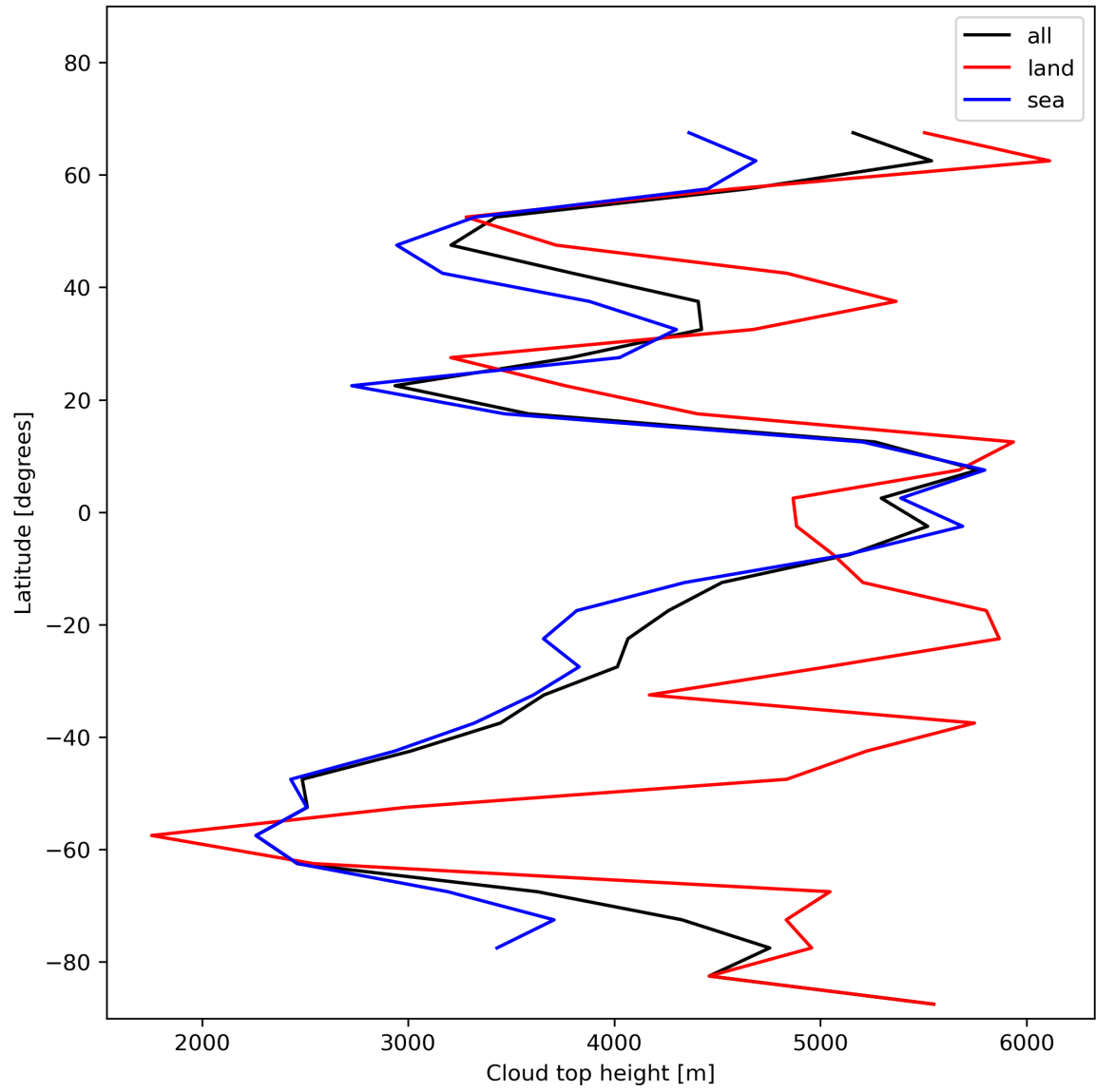
Figure 24: Zonal average of “Cloud top height” for 2023-12-09 to 2023-12-11.
