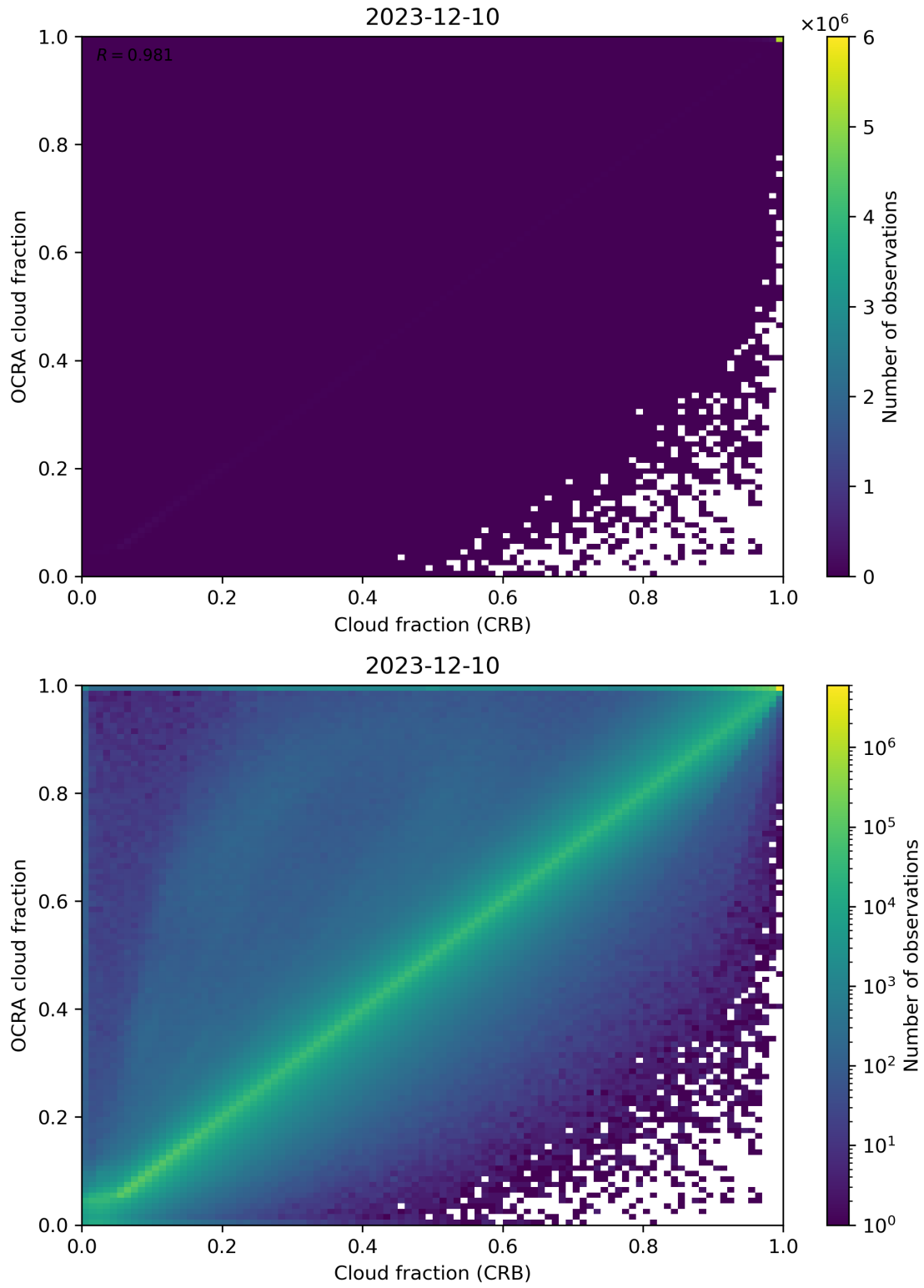
Figure 78: Scatter density plot of “Cloud fraction (CRB)” against “OCRA cloud fraction” for 2023-12-09 to 2023-12-11.
