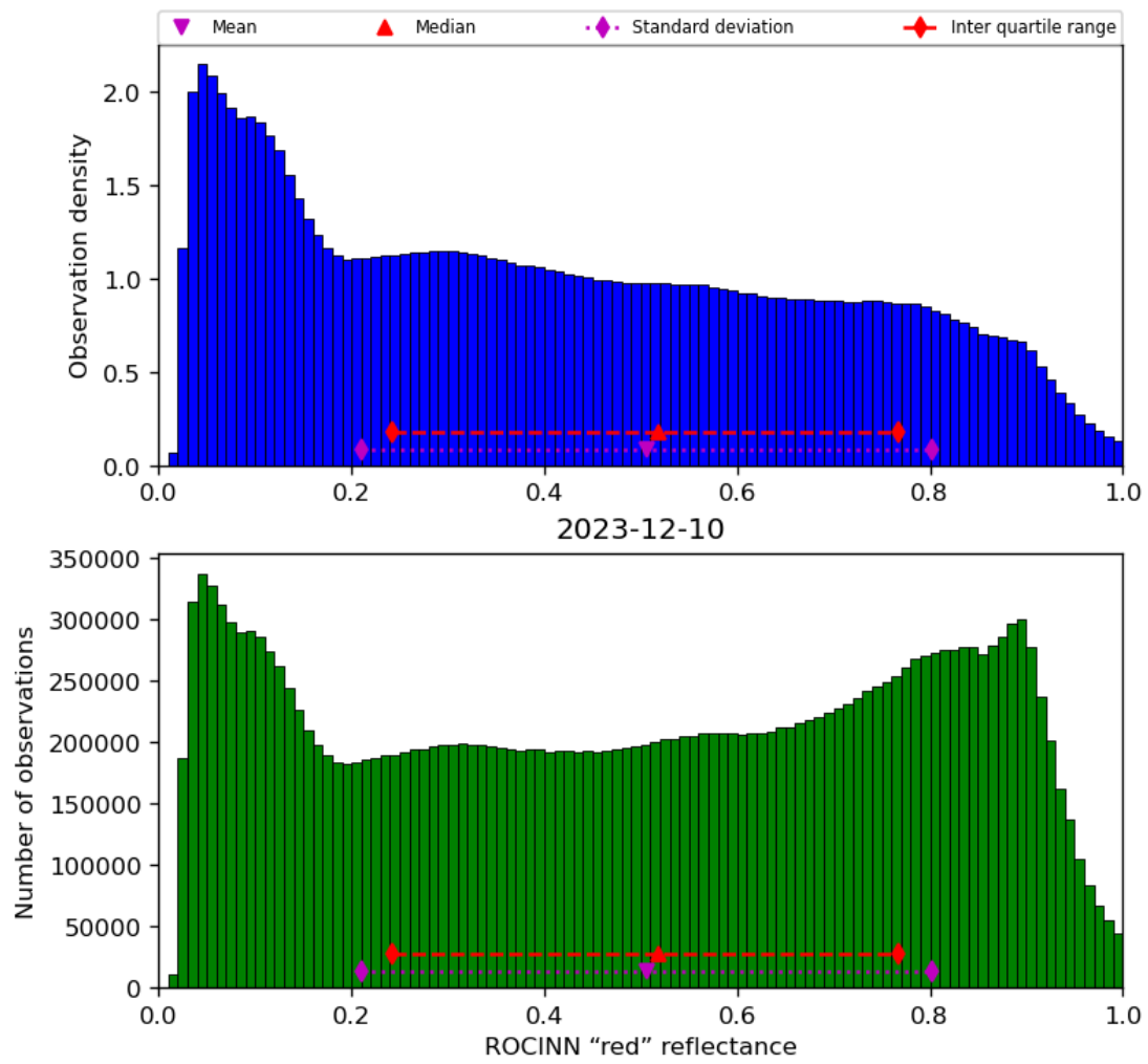
Figure 53: Histogram of “ROCINN “red” reflectance” for 2023-12-09 to 2023-12-11
