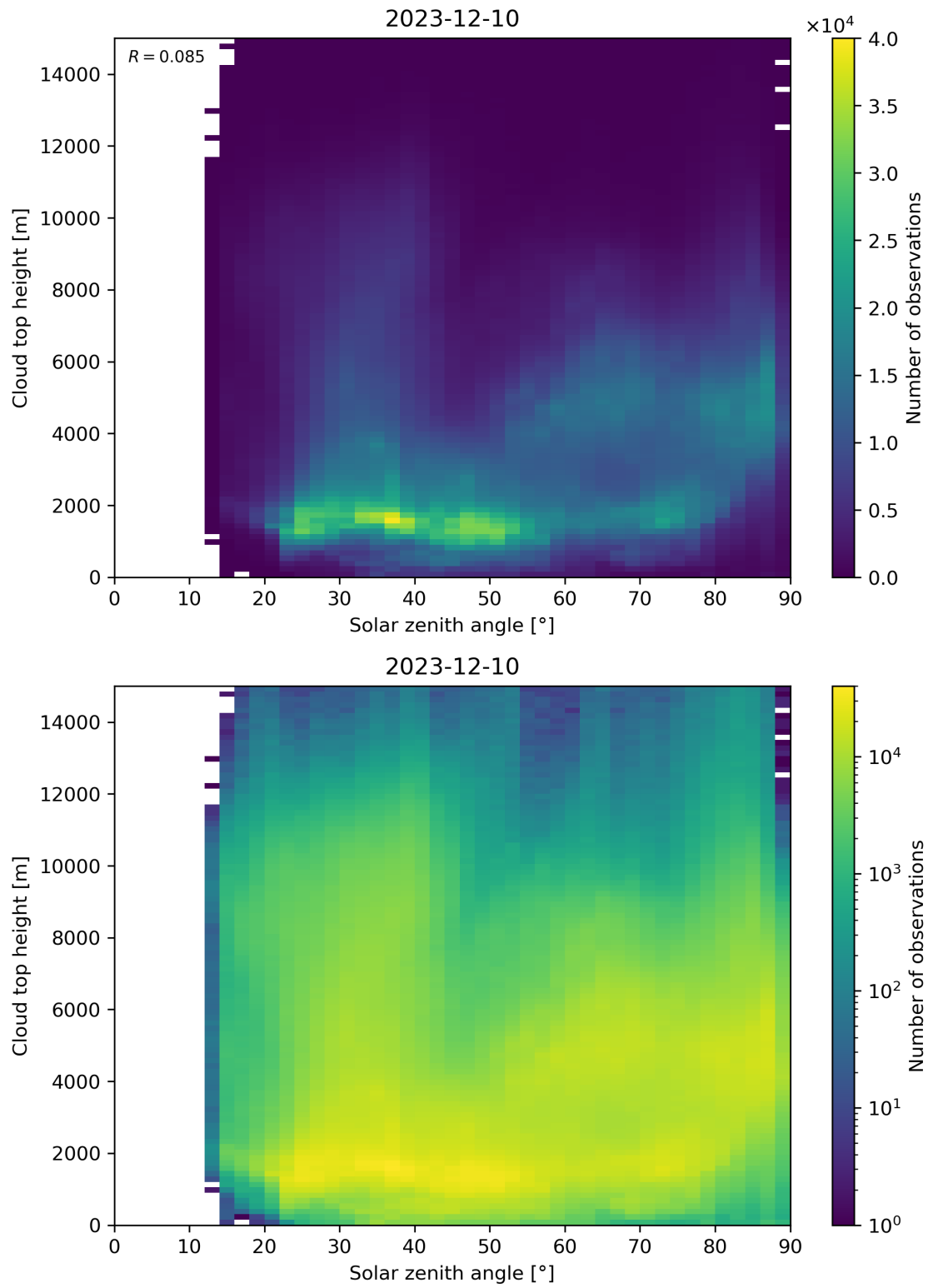
Figure 104: Scatter density plot of “Solar zenith angle” against “Cloud top height” for 2023-12-09 to 2023-12-11.
