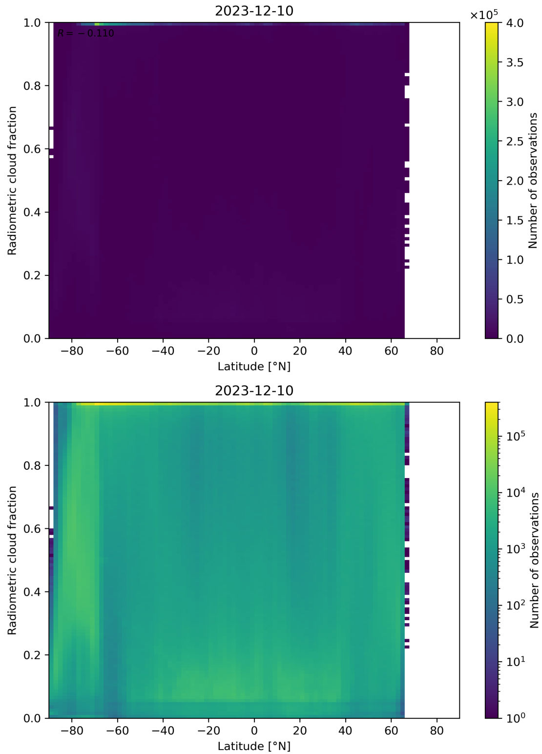
Figure 92: Scatter density plot of “Latitude” against “Radiometric cloud fraction” for 2023-12-09 to 2023-12-11.
