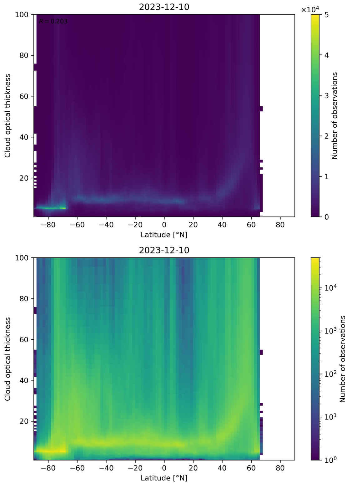
Figure 96: Scatter density plot of “Latitude” against “Cloud optical thickness” for 2023-12-09 to 2023-12-11.
