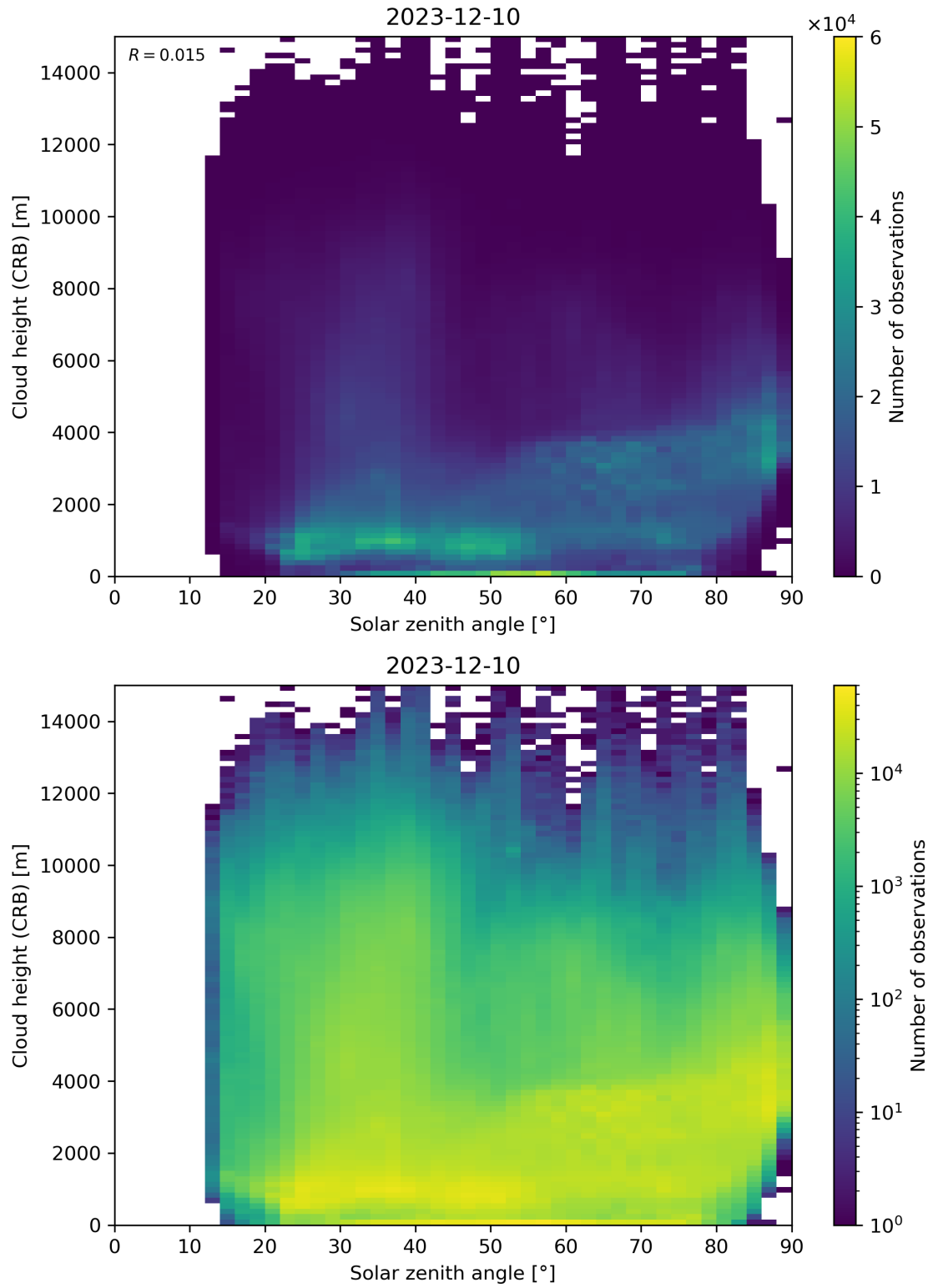
Figure 102: Scatter density plot of “Solar zenith angle” against “Cloud height (CRB)” for 2023-12-09 to 2023-12-11.
