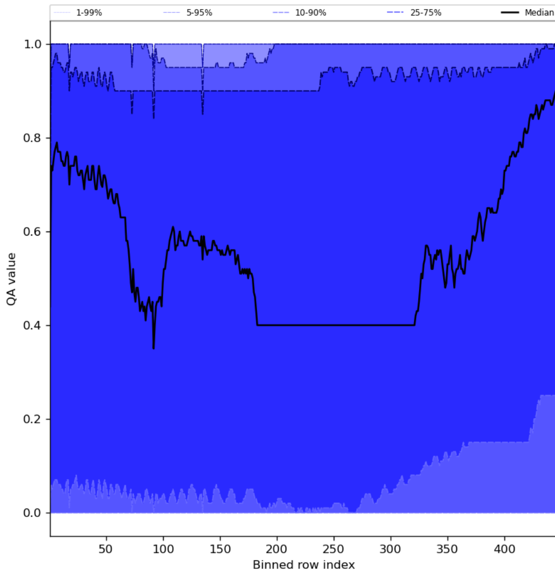
Figure 54: Along track statistics of “QA value” for 2023-12-09 to 2023-12-11
