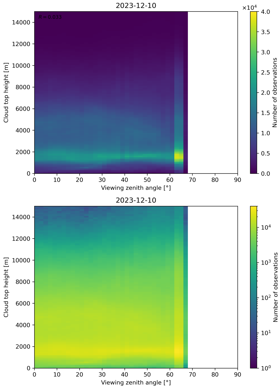
Figure 112: Scatter density plot of “Viewing zenith angle” against “Cloud top height” for 2023-12-09 to 2023-12-11.
