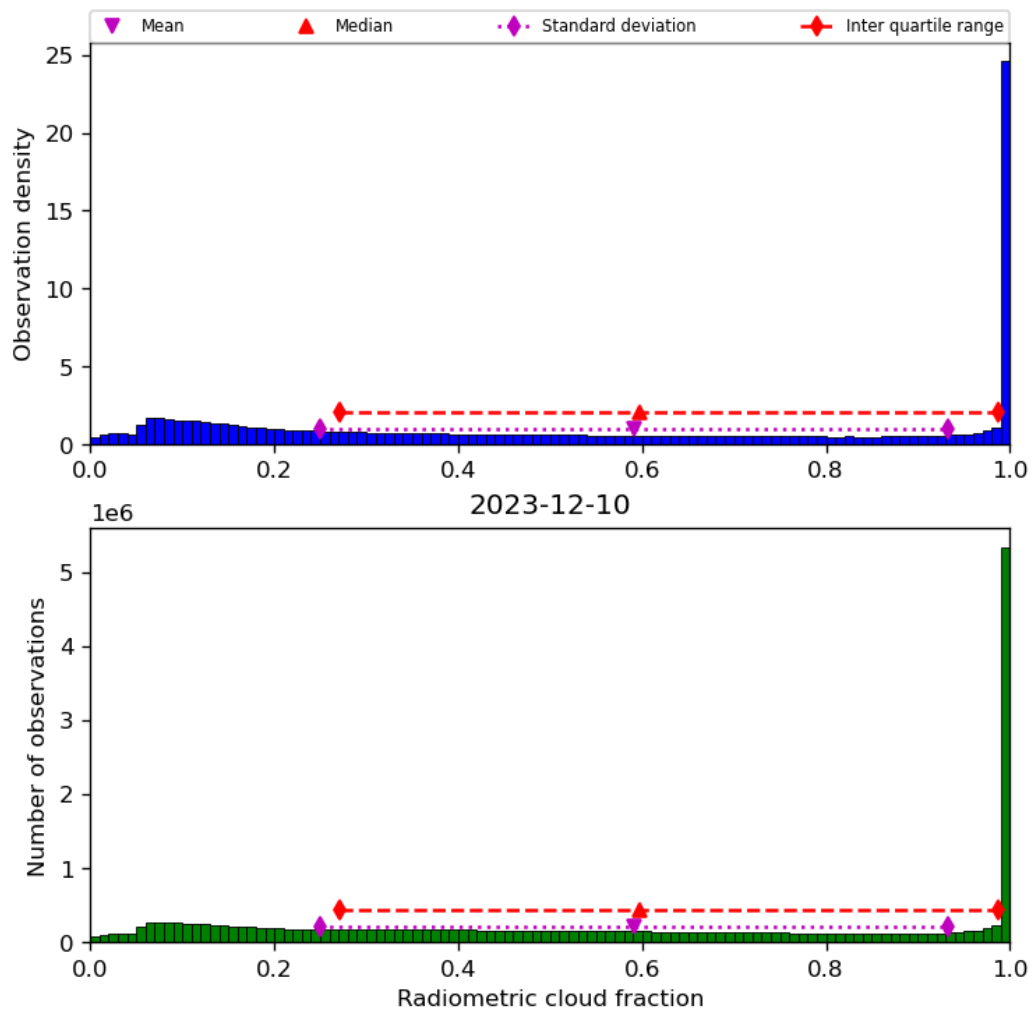
Figure 39: Histogram of “Radiometric cloud fraction” for 2023-12-09 to 2023-12-11
