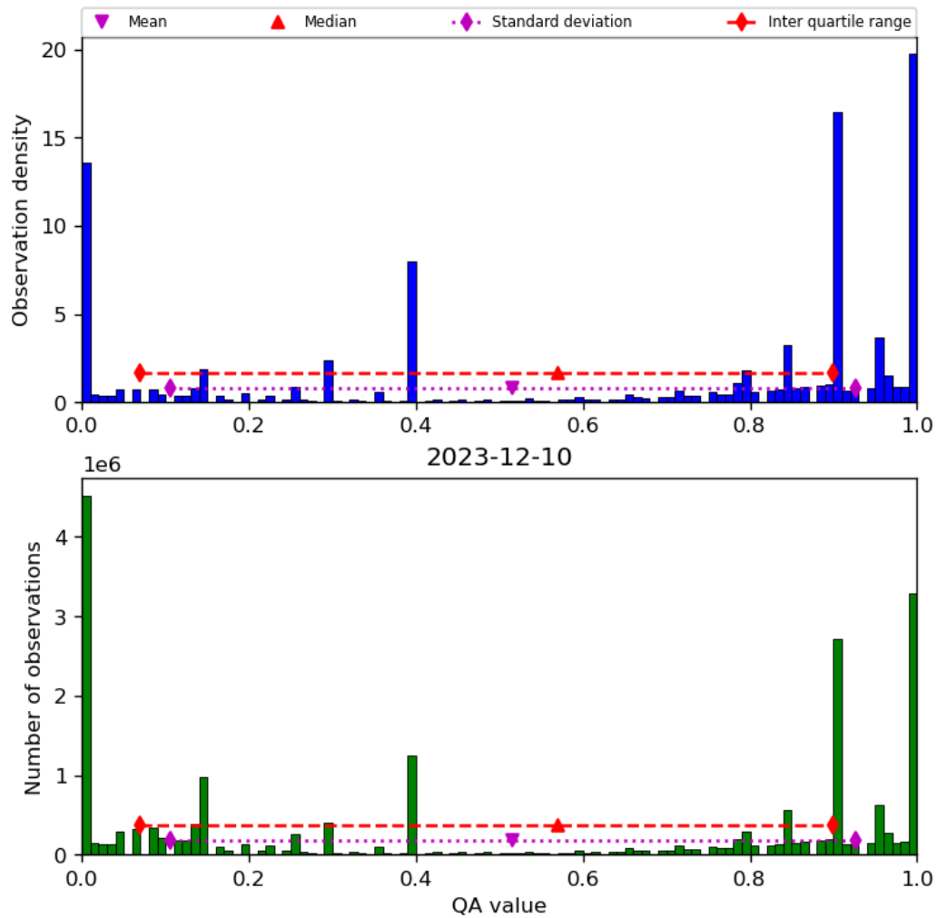
Figure 38: Histogram of “QA value” for 2023-12-09 to 2023-12-11
