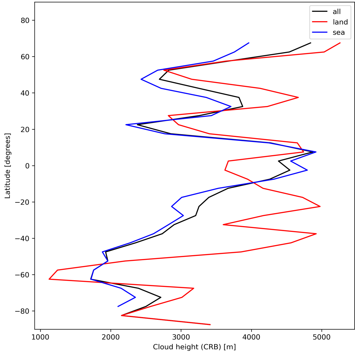
Figure 27: Zonal average of “Cloud height (CRB)” for 2023-12-09 to 2023-12-11.
