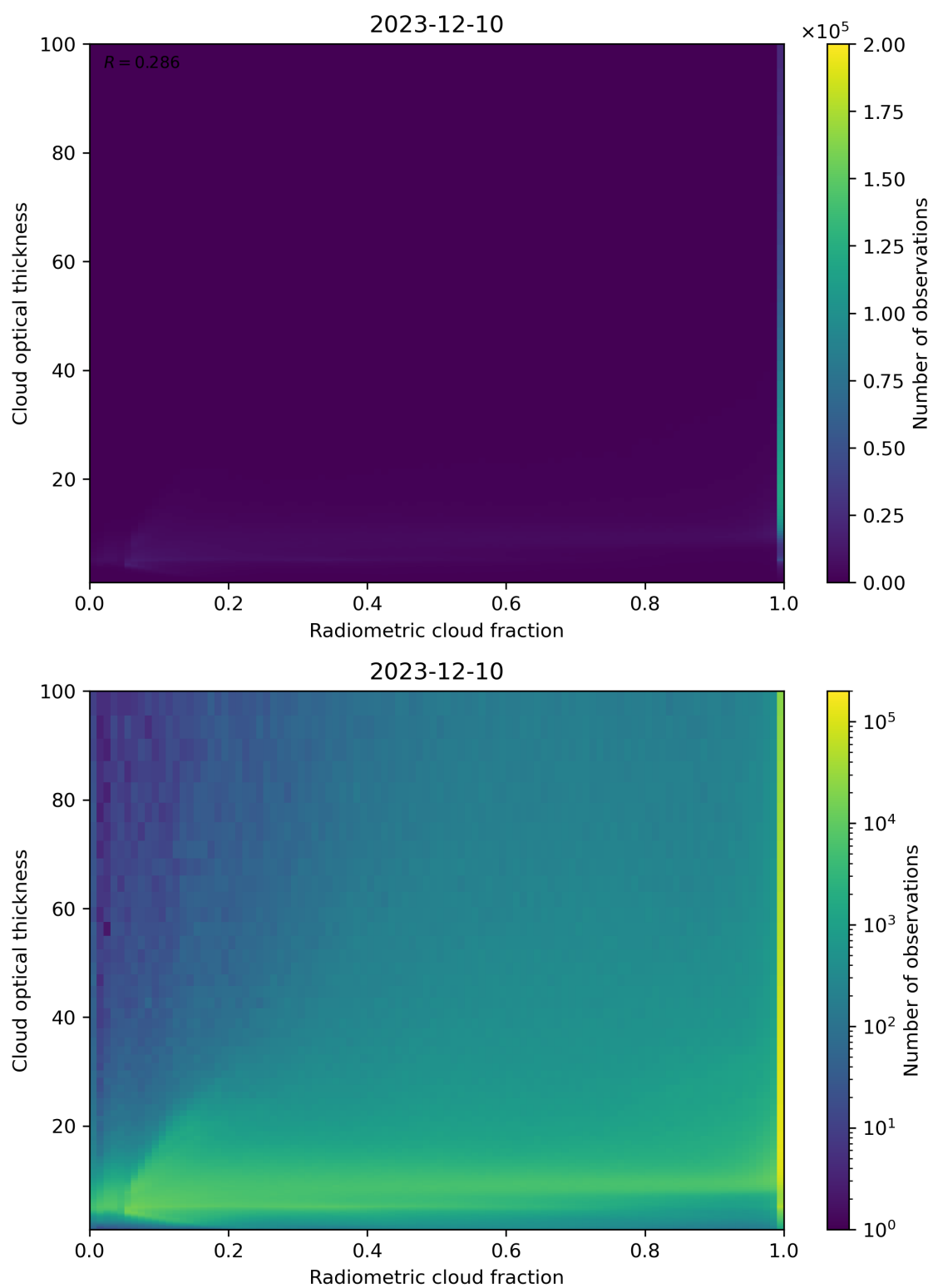
Figure 75: Scatter density plot of “Radiometric cloud fraction” against “Cloud optical thickness” for 2023-12-09 to 2023-12-11.
