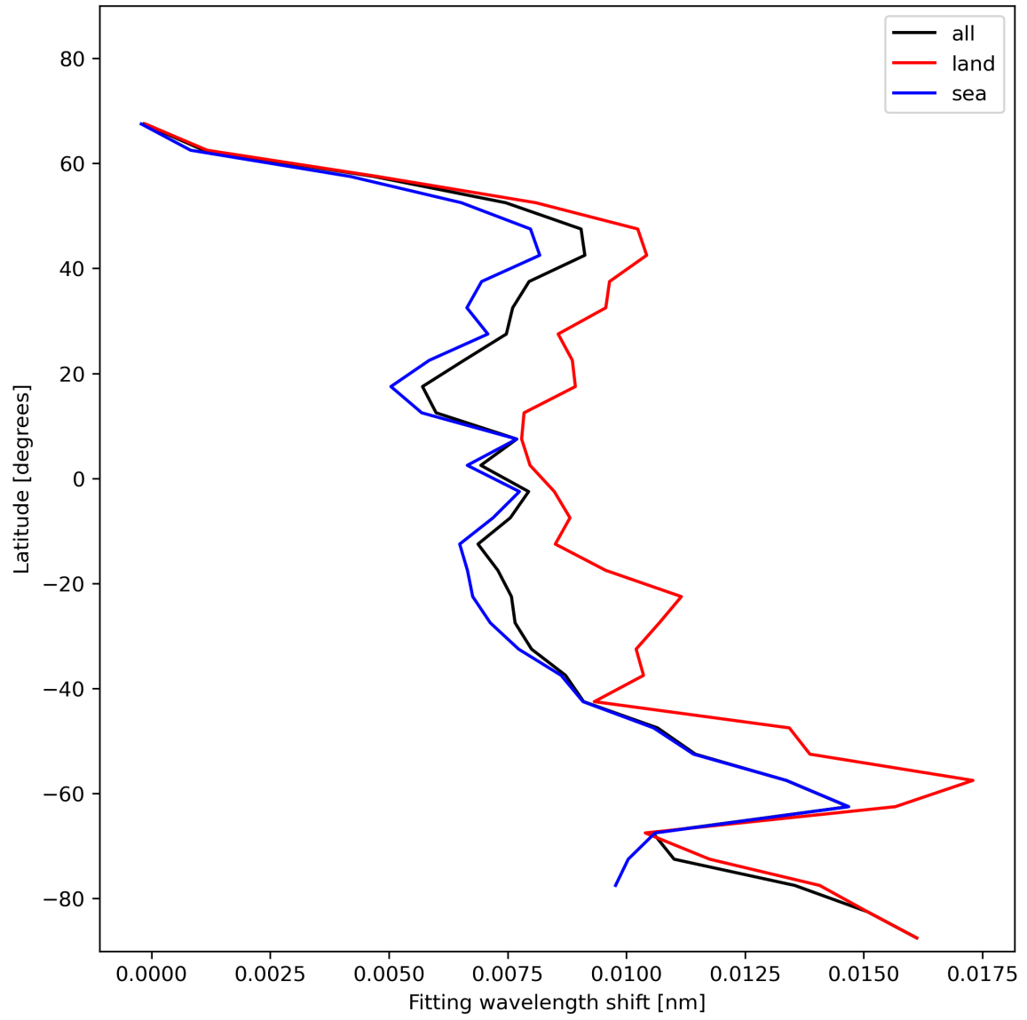
Figure 33: Zonal average of “Fitting wavelength shift” for 2023-12-09 to 2023-12-11.
