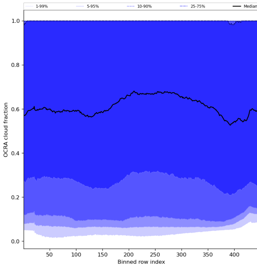
Figure 66: Along track statistics of “OCRA cloud fraction” for 2023-12-09 to 2023-12-11
