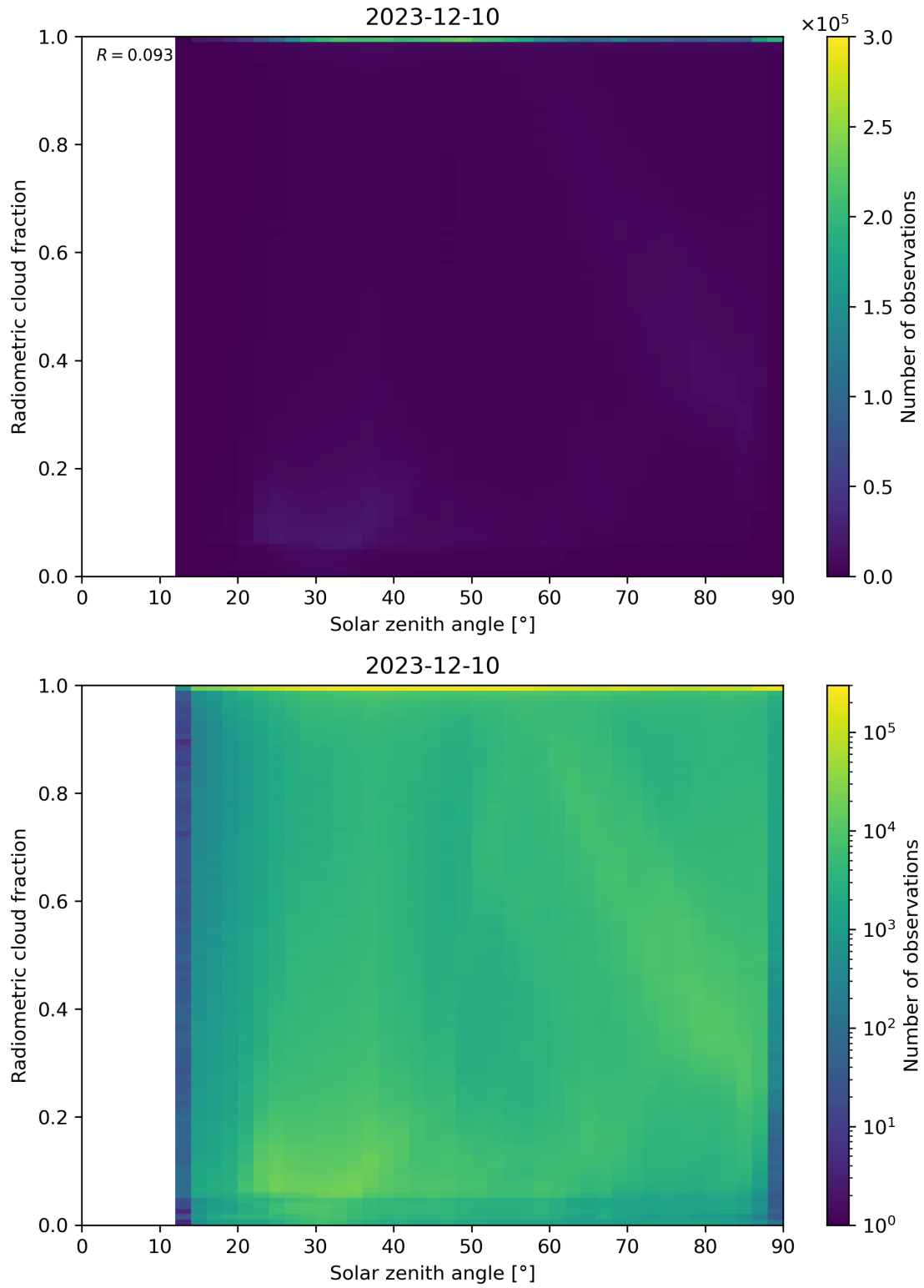
Figure 99: Scatter density plot of “Solar zenith angle” against “Radiometric cloud fraction” for 2023-12-09 to 2023-12-11.
