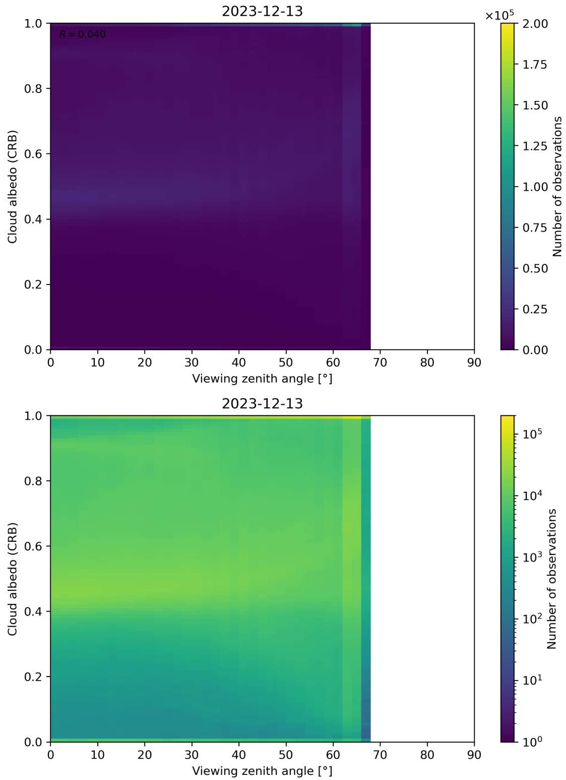
Figure 106: Scatter density plot of “Viewing zenith angle” against “Cloud albedo (CRB)” for 2023-12-12 to 2023-12-14.
