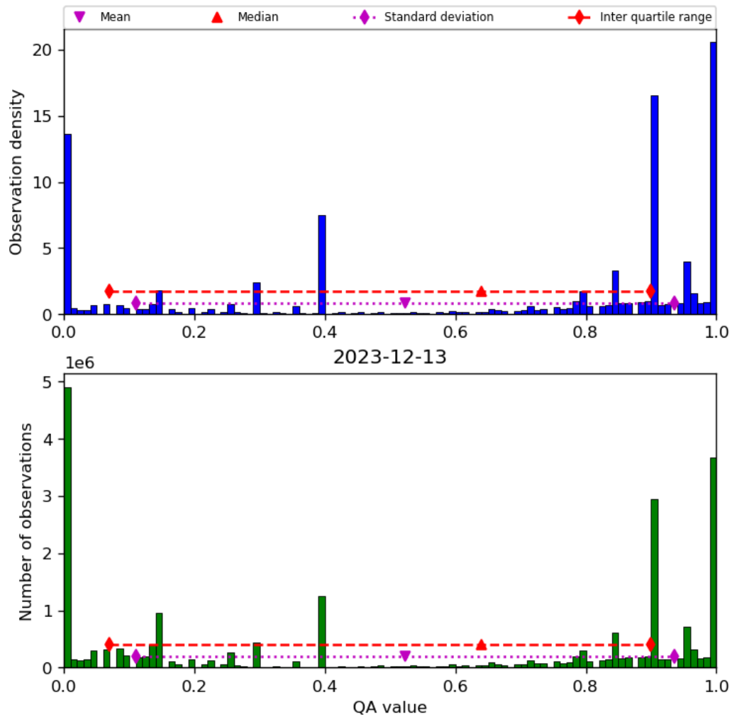
Figure 38: Histogram of “QA value” for 2023-12-12 to 2023-12-14
