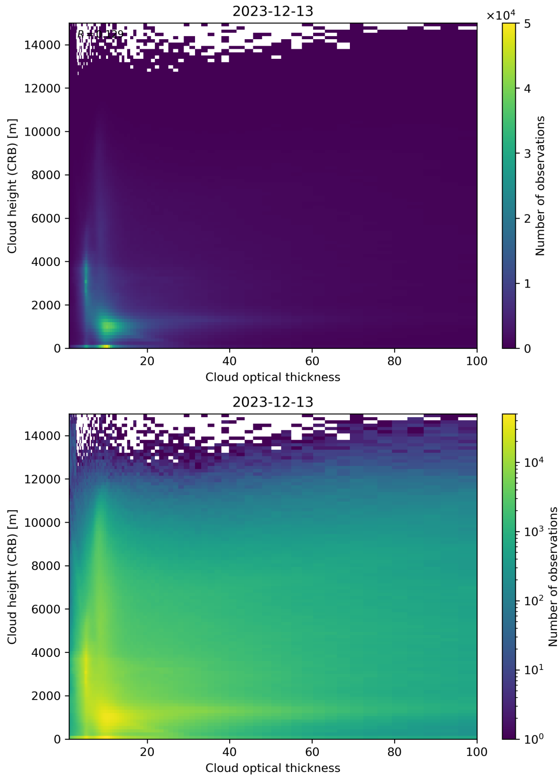
Figure 85: Scatter density plot of “Cloud optical thickness” against “Cloud height (CRB)” for 2023-12-12 to 2023-12-14.
