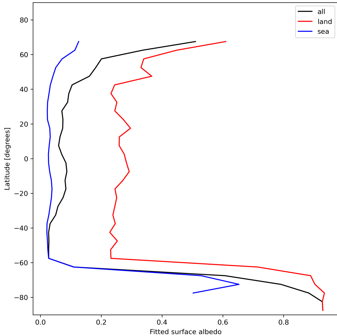
Figure 29: Zonal average of “Fitted surface albedo” for 2023-12-12 to 2023-12-14.
