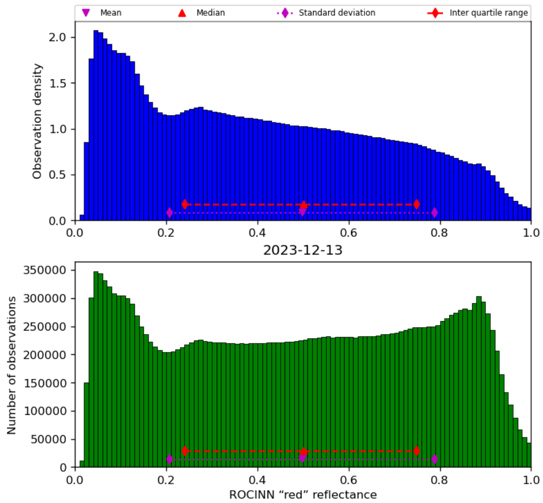
Figure 53: Histogram of “ROCINN “red” reflectance” for 2023-12-12 to 2023-12-14
