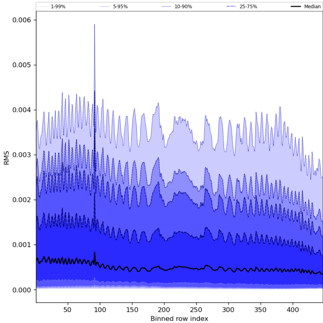
Figure 63: Along track statistics of “RMS” for 2023-12-12 to 2023-12-14
