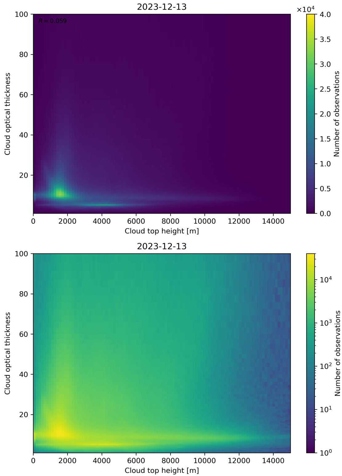
Figure 90: Scatter density plot of “Cloud top height” against “Cloud optical thickness” for 2023-12-12 to 2023-12-14.
