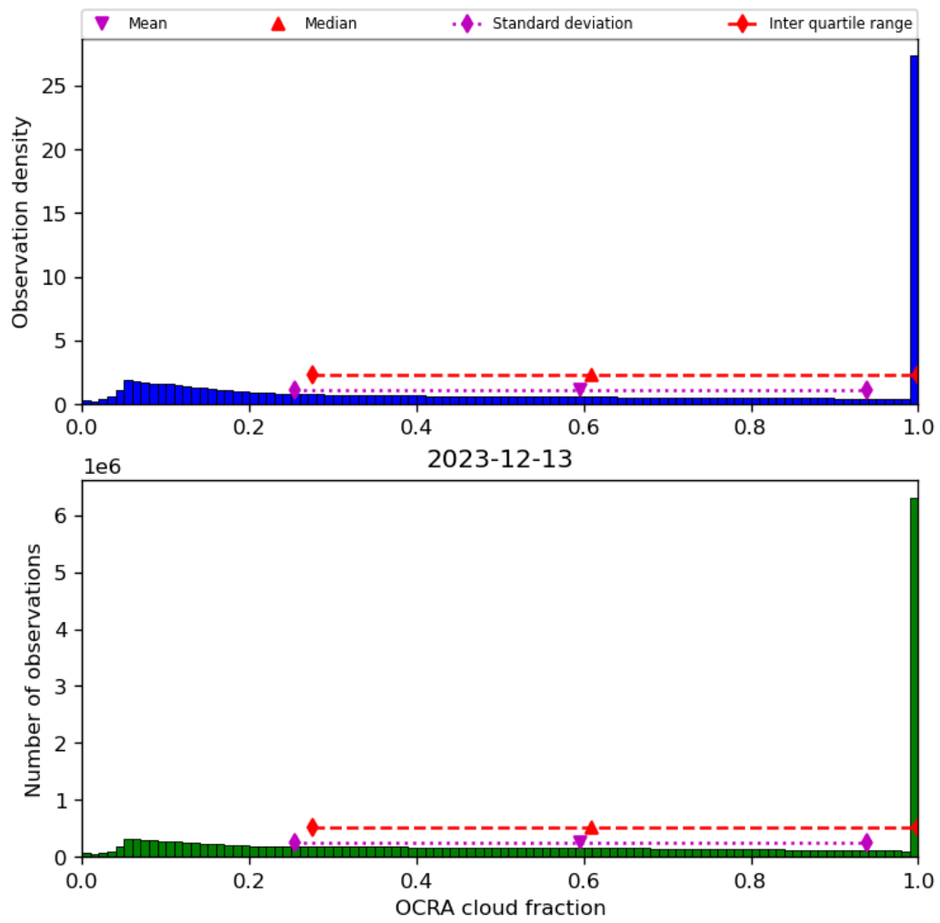
Figure 50: Histogram of “OCRA cloud fraction” for 2023-12-12 to 2023-12-14
