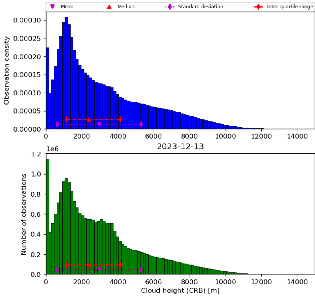
Figure 43: Histogram of “Cloud height (CRB)” for 2023-12-12 to 2023-12-14
