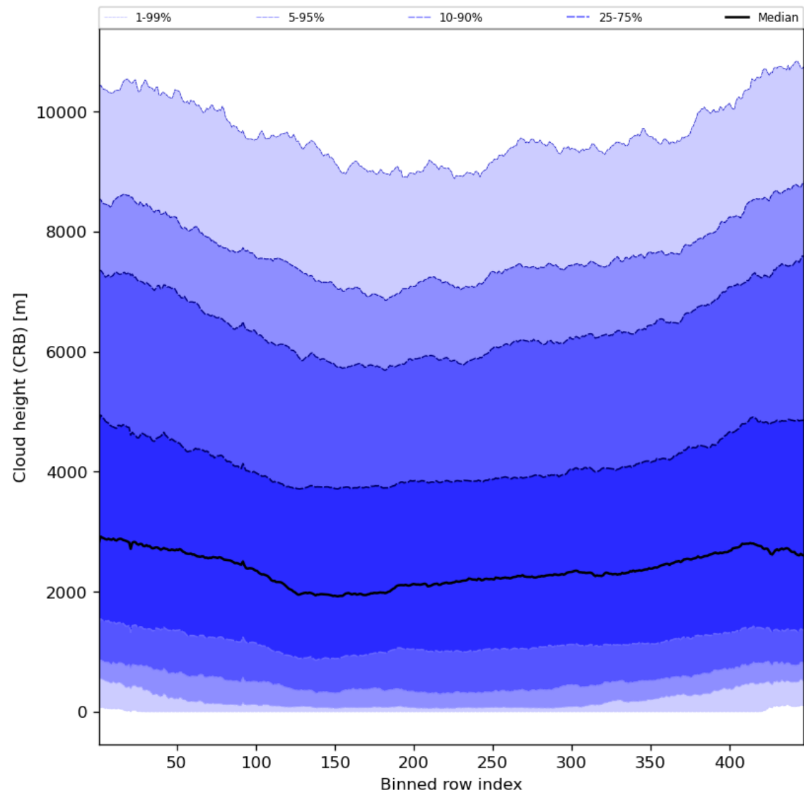
Figure 59: Along track statistics of “Cloud height (CRB)” for 2023-12-12 to 2023-12-14
