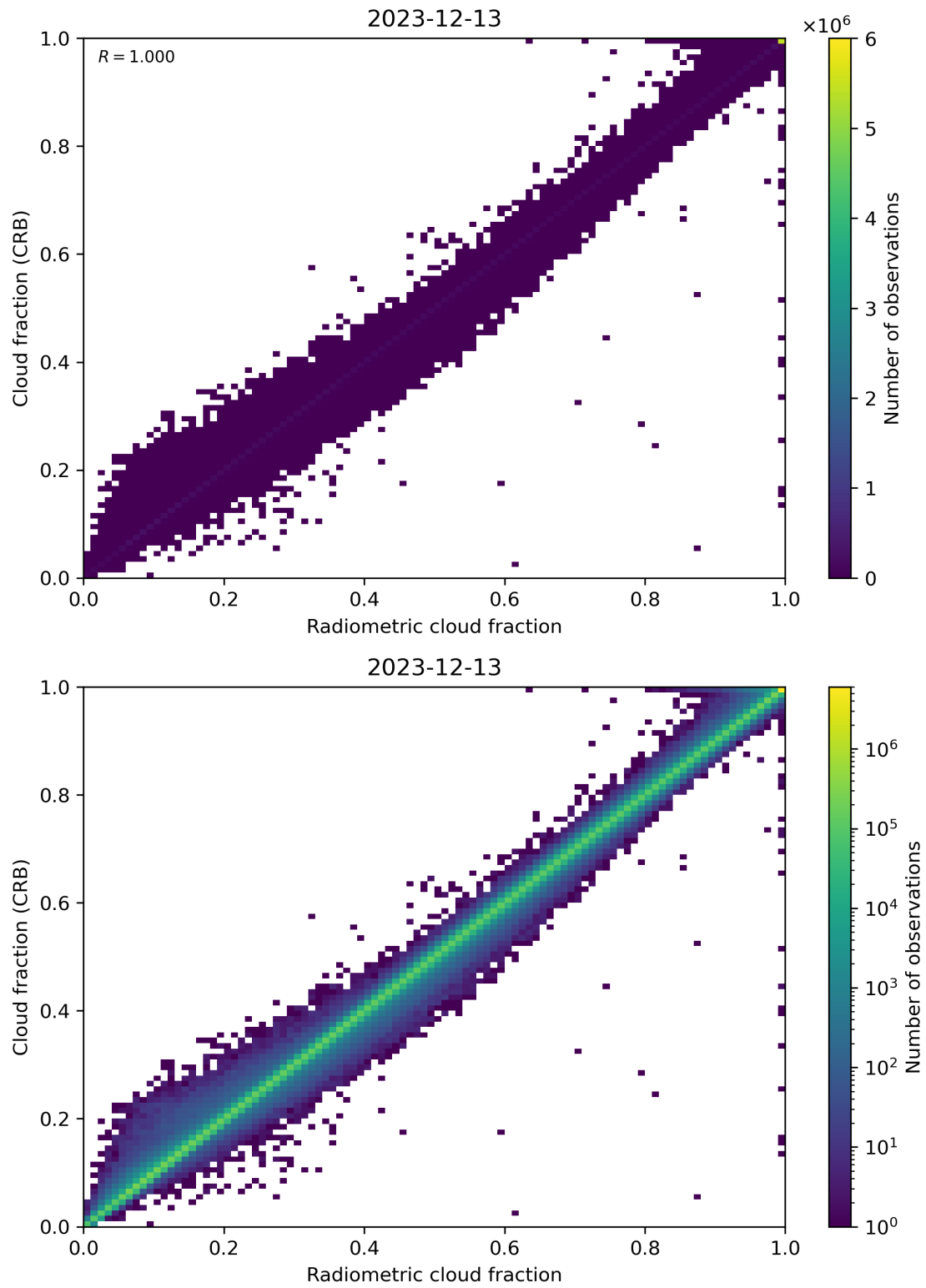
Figure 73: Scatter density plot of “Radiometric cloud fraction” against “Cloud fraction (CRB)” for 2023-12-12 to 2023-12-14.
