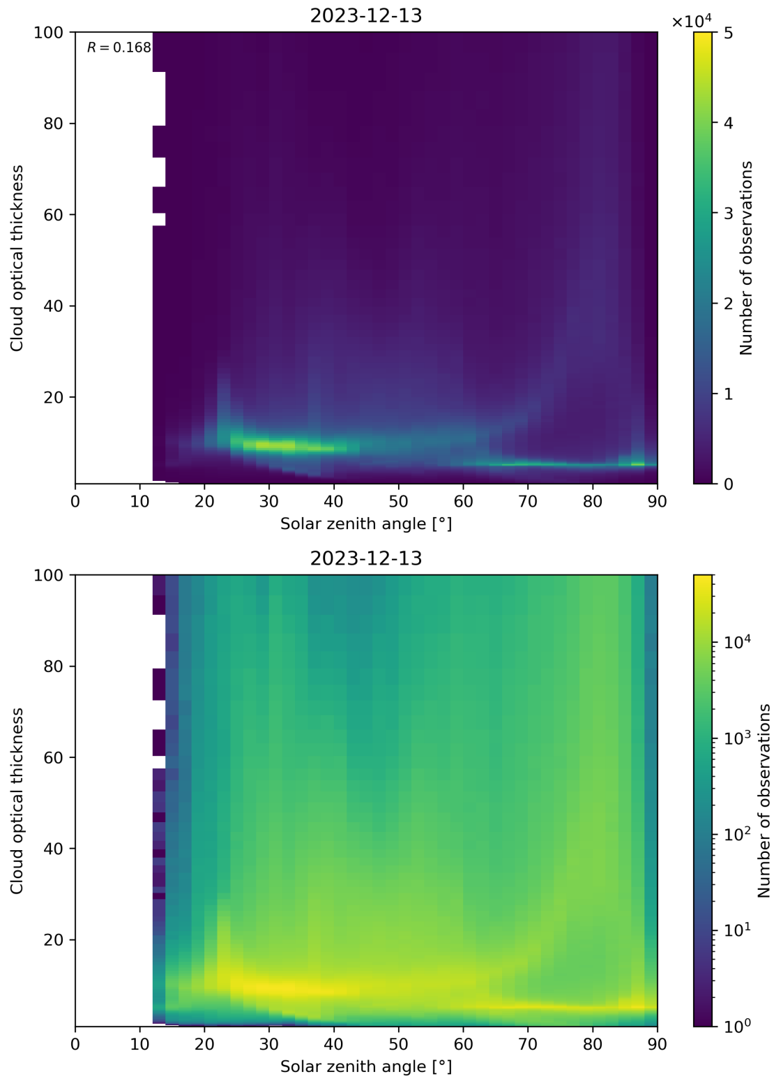
Figure 103: Scatter density plot of “Solar zenith angle” against “Cloud optical thickness” for 2023-12-12 to 2023-12-14.
