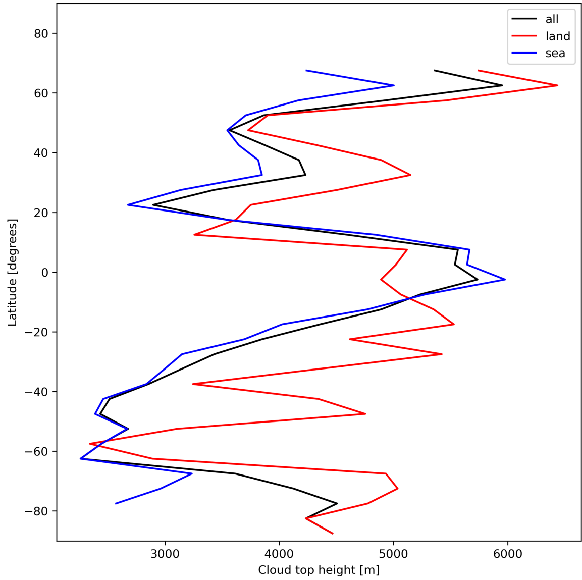
Figure 24: Zonal average of “Cloud top height” for 2023-12-12 to 2023-12-14.
