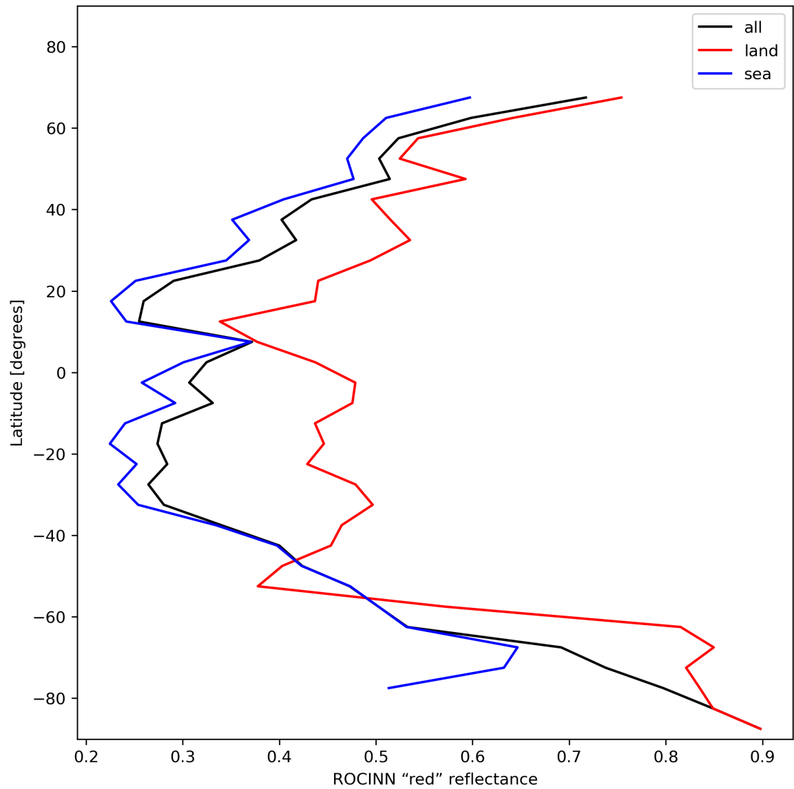
Figure 37: Zonal average of “ROCINN “red” reflectance” for 2023-12-12 to 2023-12-14.
