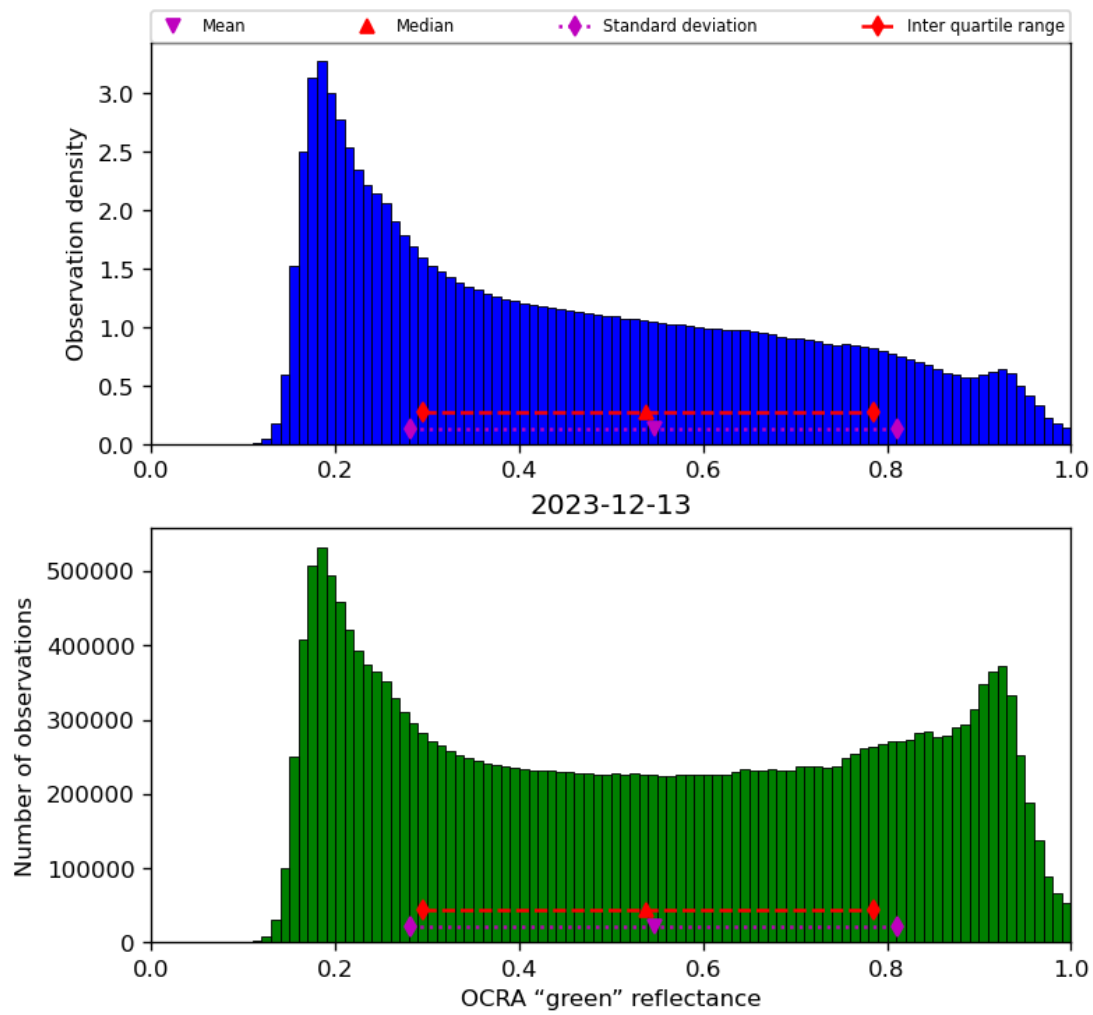
Figure 52: Histogram of “OCRA “green” reflectance” for 2023-12-12 to 2023-12-14
