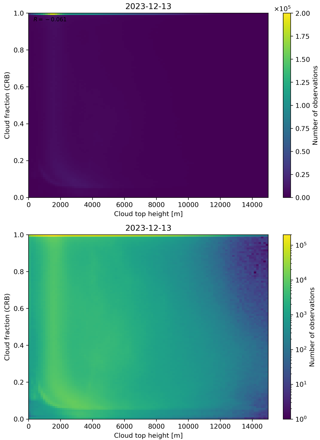
Figure 88: Scatter density plot of “Cloud top height” against “Cloud fraction (CRB)” for 2023-12-12 to 2023-12-14.
