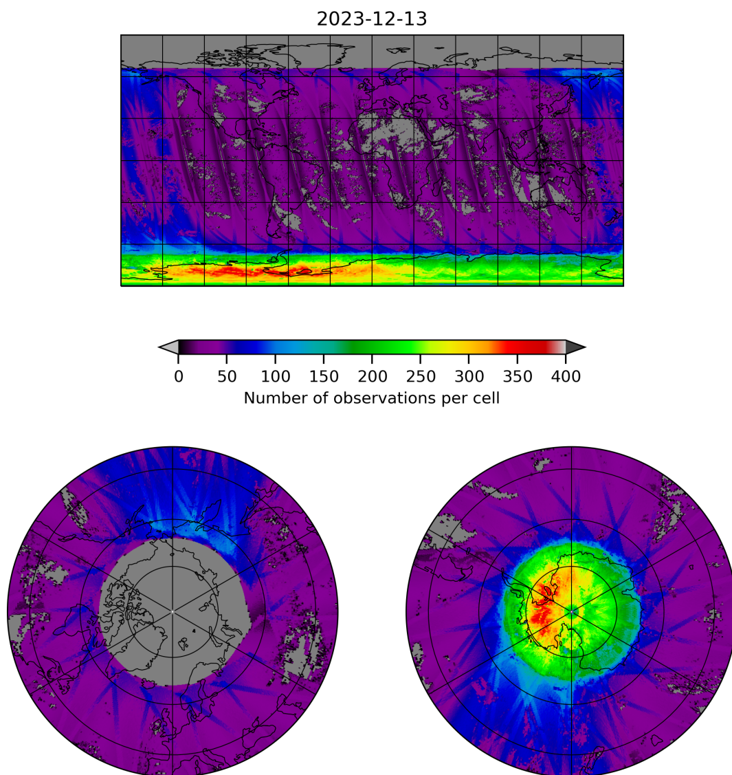
Figure 21: Map of the number of observations for 2023-12-12 to 2023-12-14
