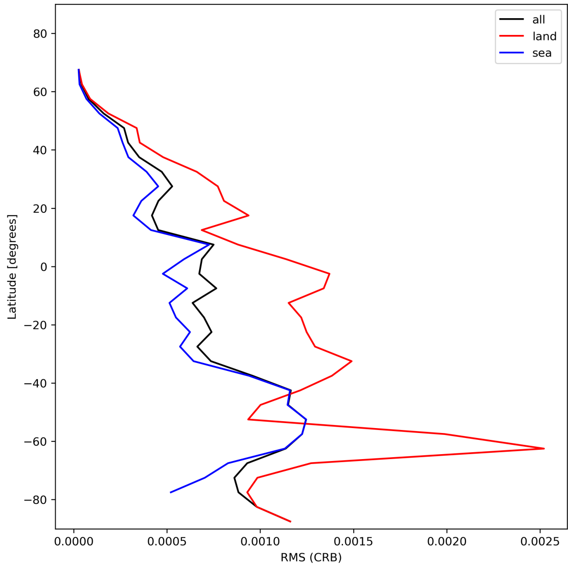
Figure 32: Zonal average of “RMS (CRB)” for 2023-12-12 to 2023-12-14.
