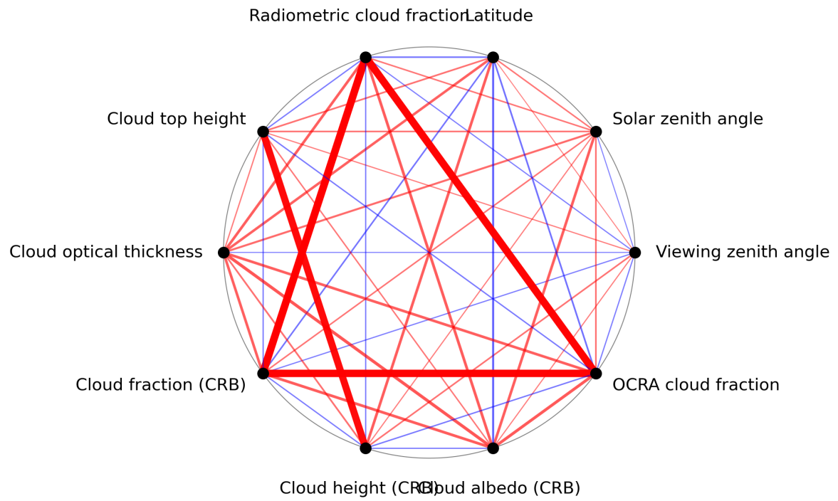
Figure 1: Map of correlation graph for 2023-12-12 to 2023-12-14.
