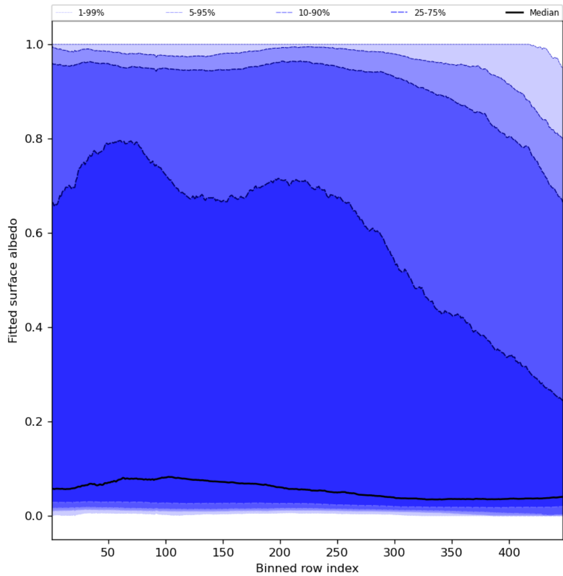
Figure 61: Along track statistics of “Fitted surface albedo” for 2023-12-12 to 2023-12-14
