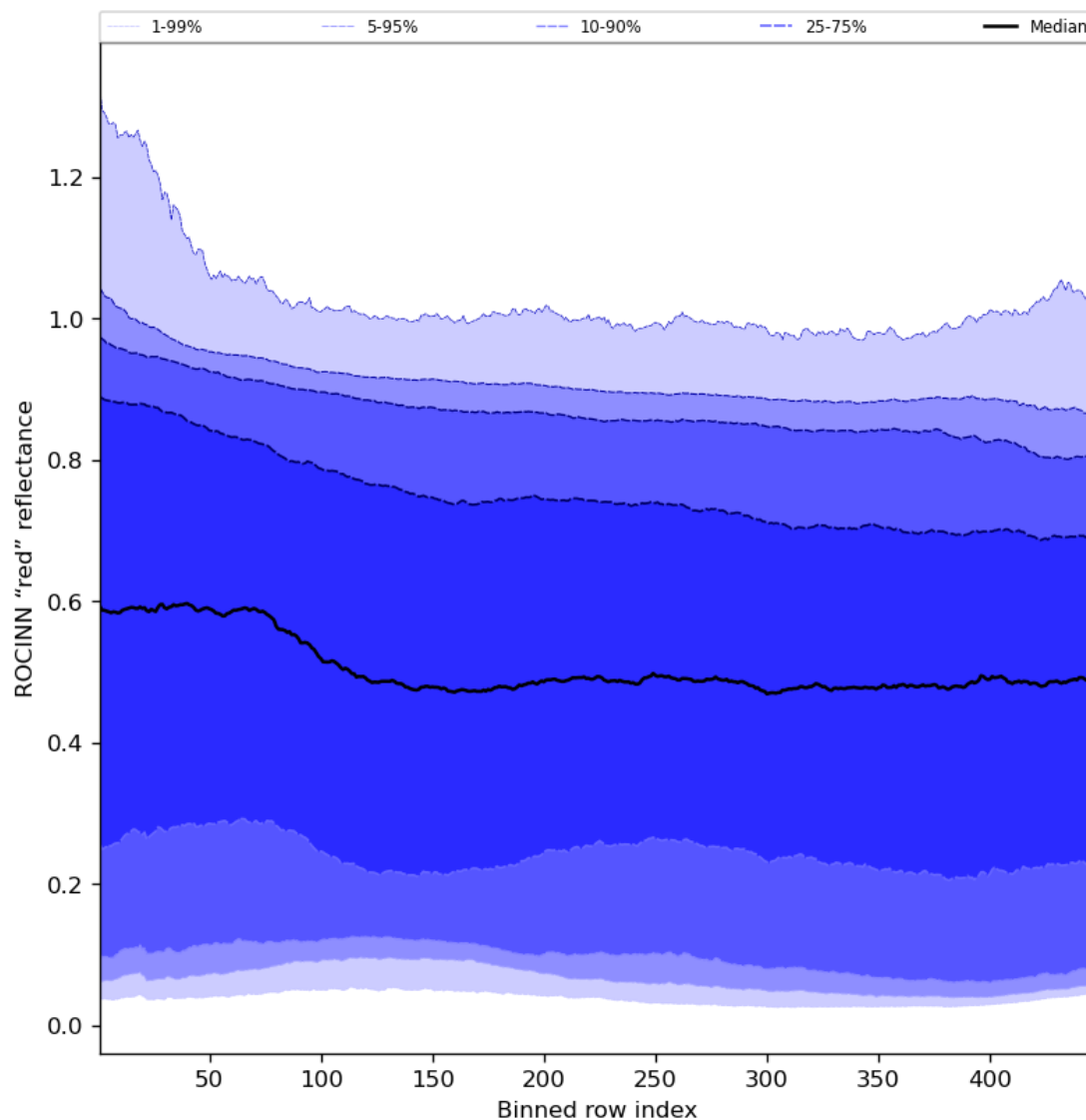
Figure 69: Along track statistics of "ROCINN "red" reflectance" for 2023-12-12 to 2023-12-14
