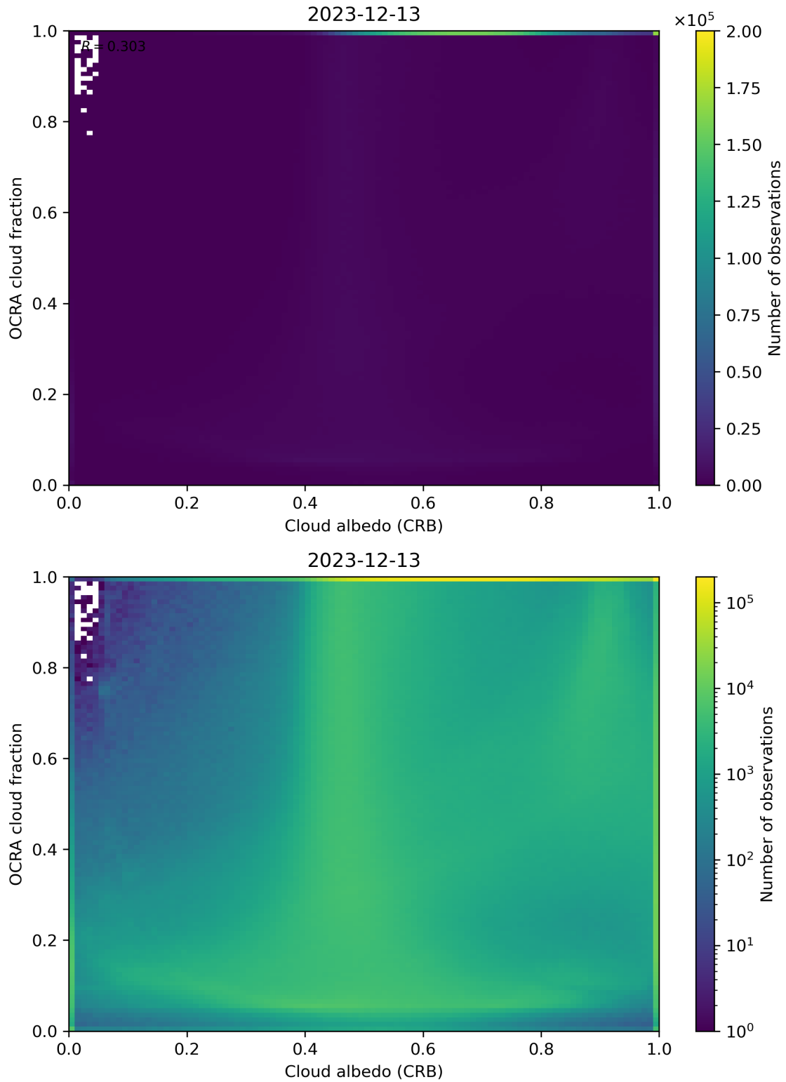
Figure 70: Scatter density plot of “Cloud albedo (CRB)” against “OCRA cloud fraction” for 2023-12-12 to 2023-12-14.
