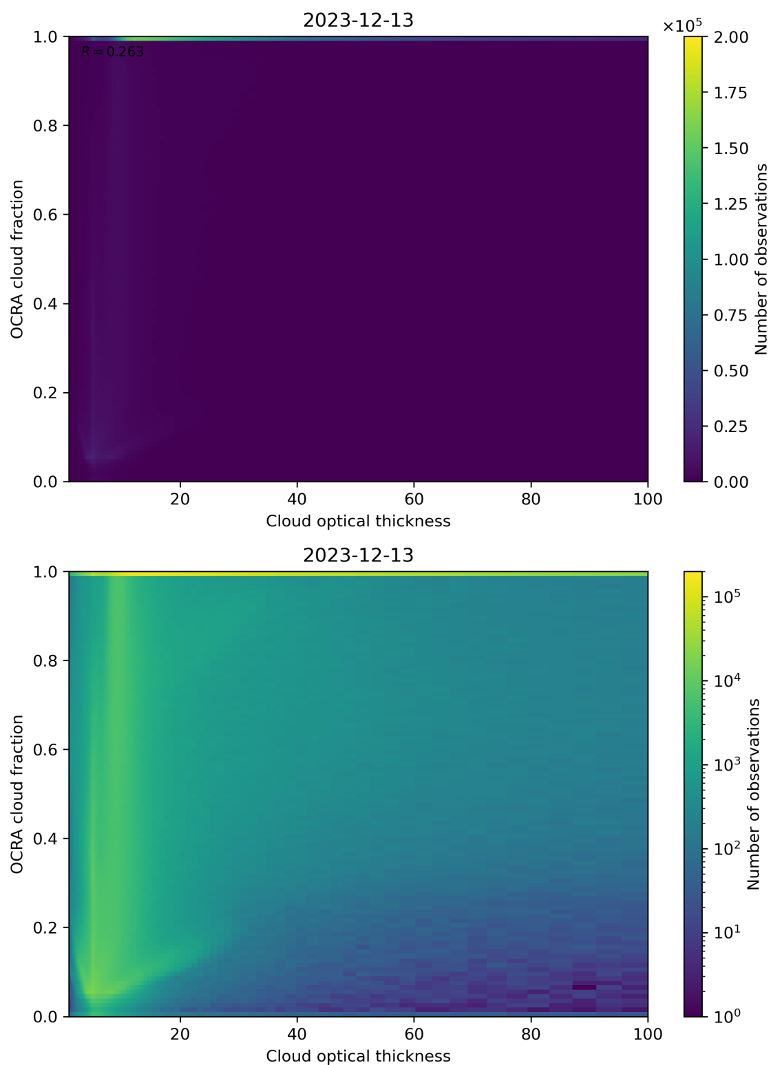
Figure 83: Scatter density plot of “Cloud optical thickness” against “OCRA cloud fraction” for 2023-12-12 to 2023-12-14.
