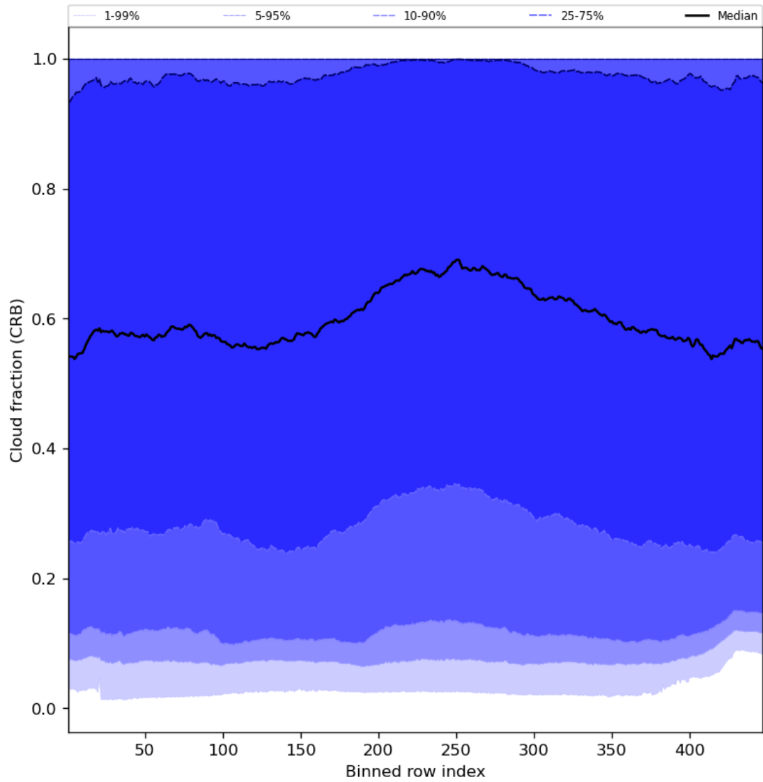
Figure 58: Along track statistics of “Cloud fraction (CRB)” for 2023-12-12 to 2023-12-14
