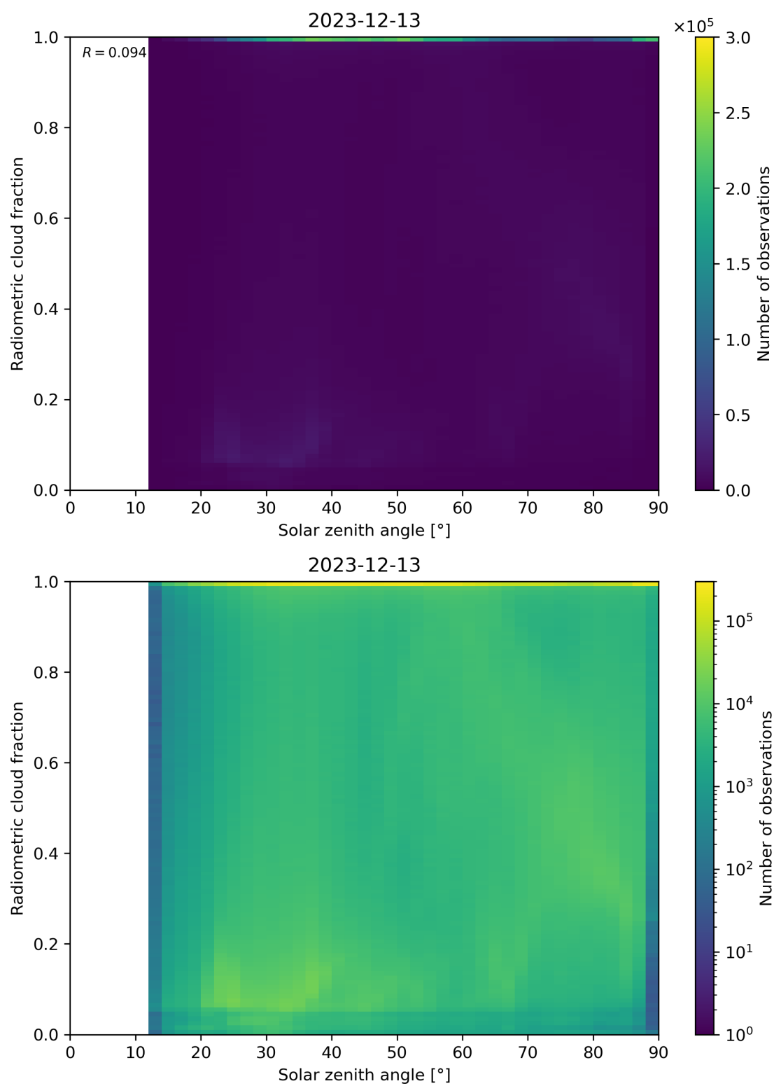
Figure 99: Scatter density plot of “Solar zenith angle” against “Radiometric cloud fraction” for 2023-12-12 to 2023-12-14.
