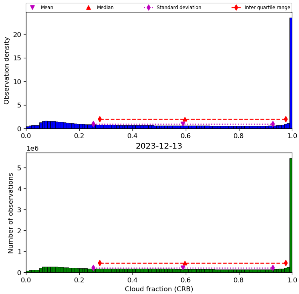
Figure 42: Histogram of “Cloud fraction (CRB)” for 2023-12-12 to 2023-12-14
