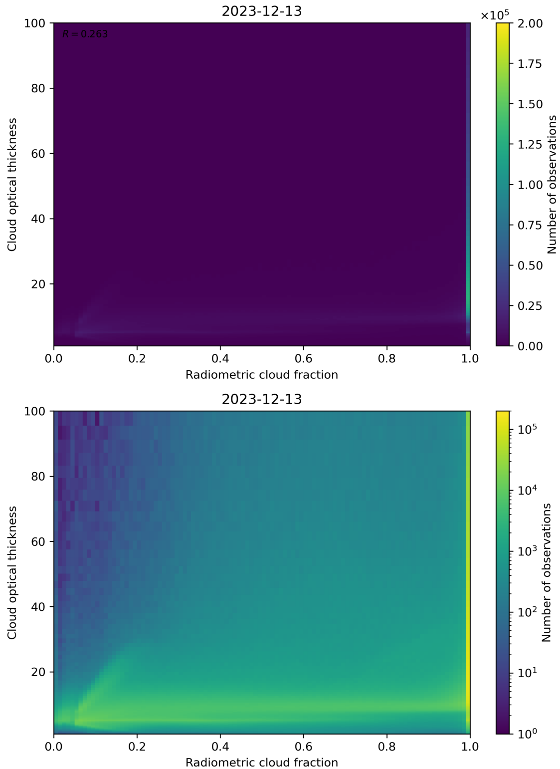
Figure 75: Scatter density plot of “Radiometric cloud fraction” against “Cloud optical thickness” for 2023-12-12 to 2023-12-14.
