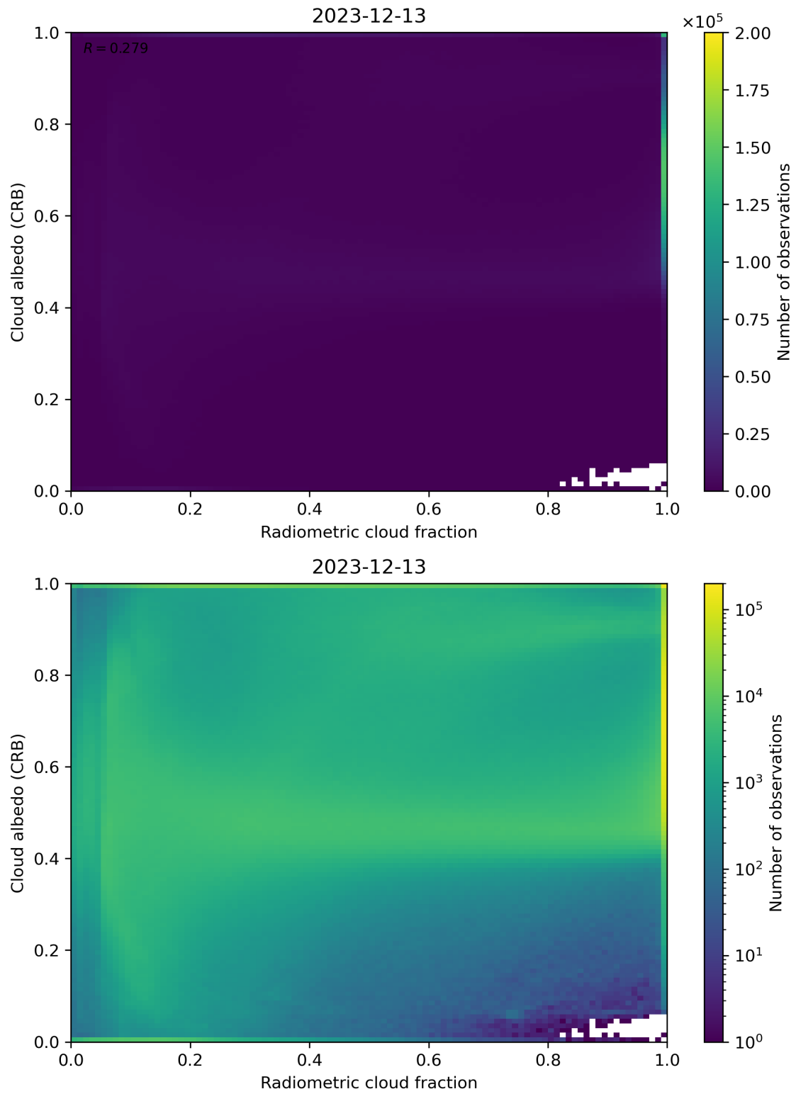
Figure 71: Scatter density plot of “Radiometric cloud fraction” against “Cloud albedo (CRB)” for 2023-12-12 to 2023-12-14.
