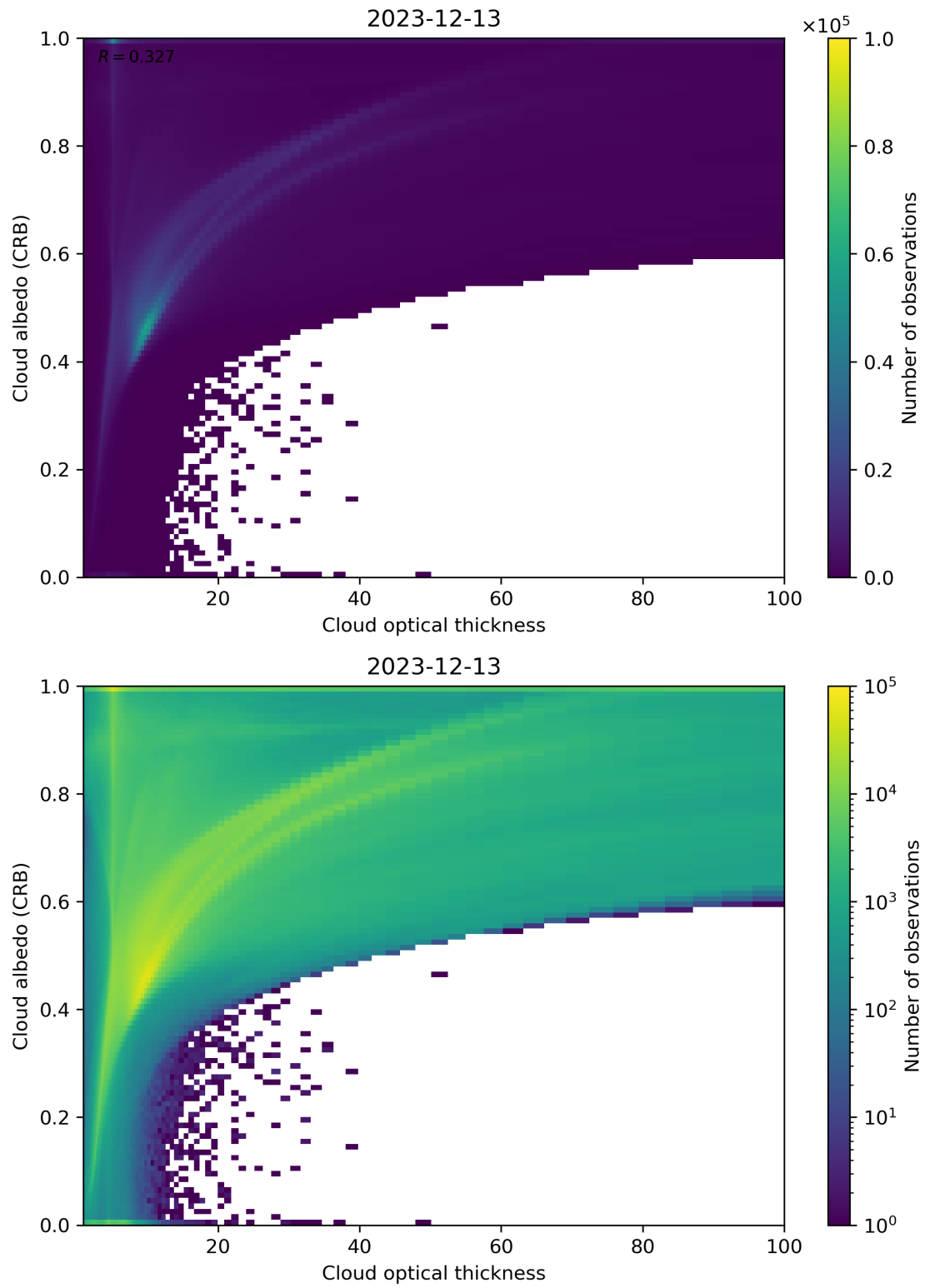
Figure 82: Scatter density plot of “Cloud optical thickness” against “Cloud albedo (CRB)” for 2023-12-12 to 2023-12-14.
