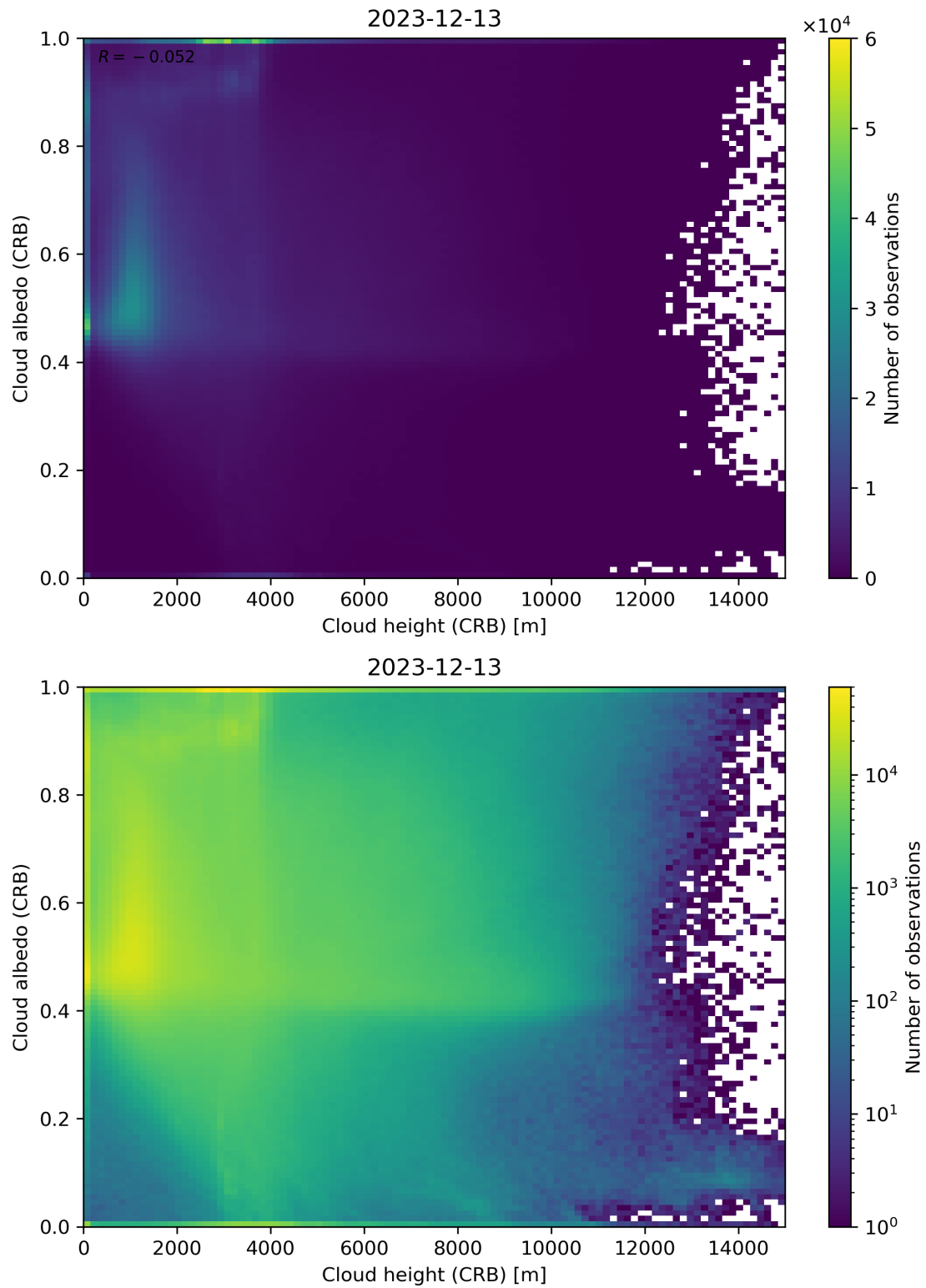
Figure 80: Scatter density plot of “Cloud height (CRB)” against “Cloud albedo (CRB)” for 2023-12-12 to 2023-12-14.
