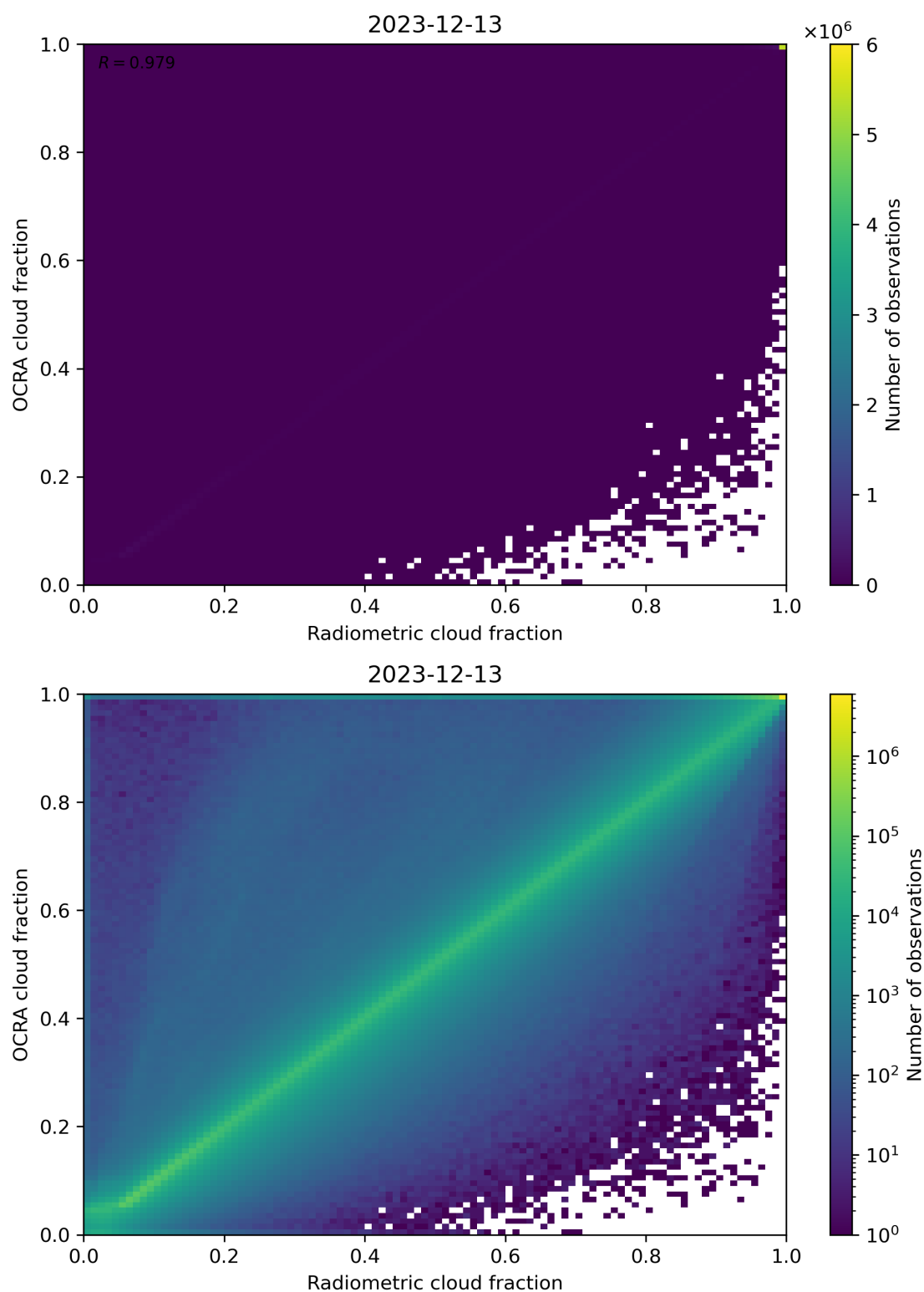
Figure 72: Scatter density plot of “Radiometric cloud fraction” against “OCRA cloud fraction” for 2023-12-12 to 2023-12-14.
