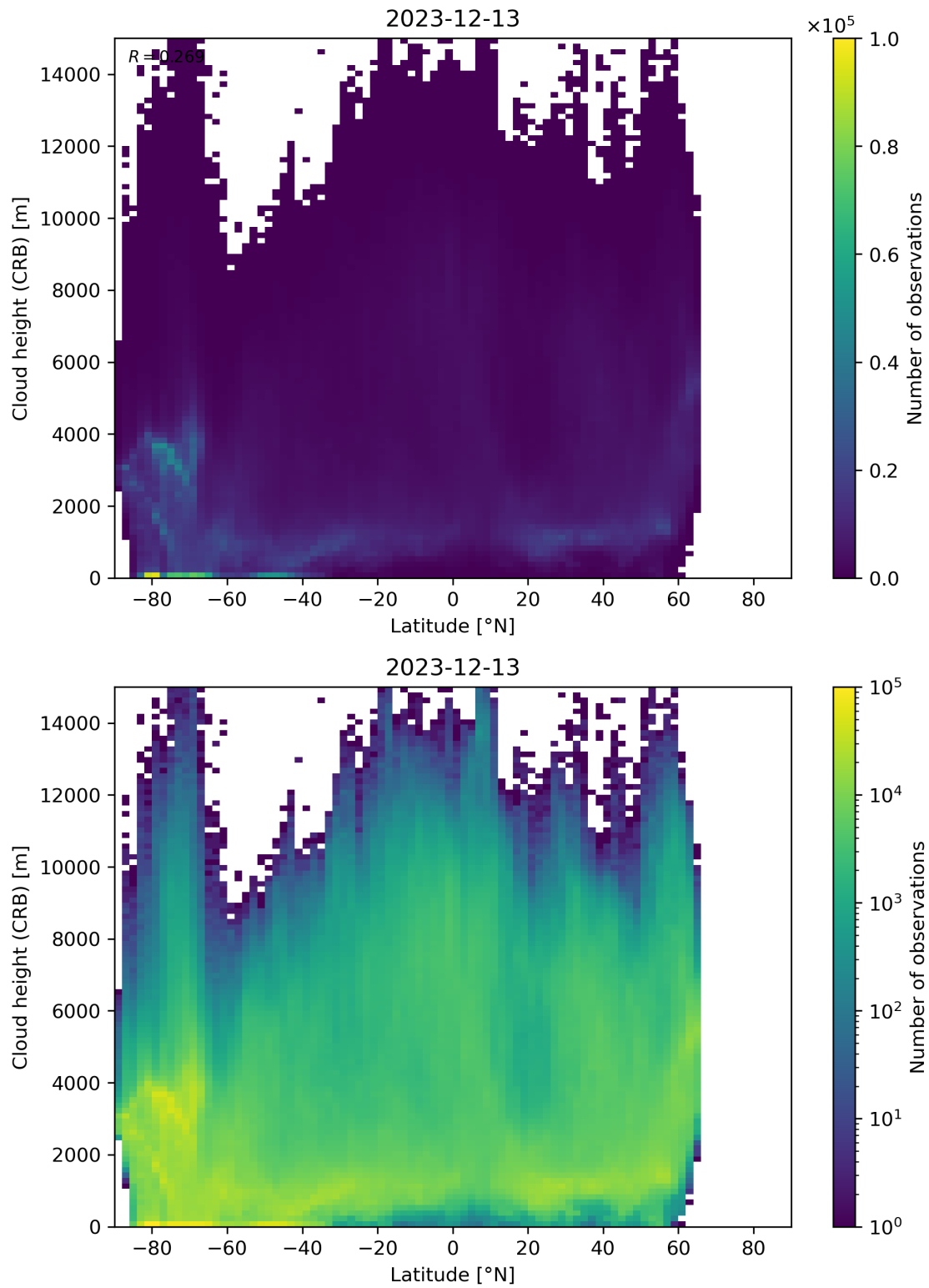
Figure 95: Scatter density plot of “Latitude” against “Cloud height (CRB)” for 2023-12-12 to 2023-12-14.
