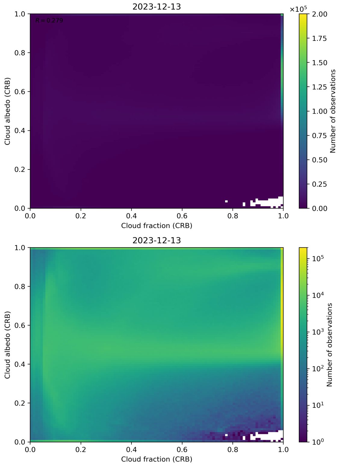
Figure 77: Scatter density plot of “Cloud fraction (CRB)” against “Cloud albedo (CRB)” for 2023-12-12 to 2023-12-14.
