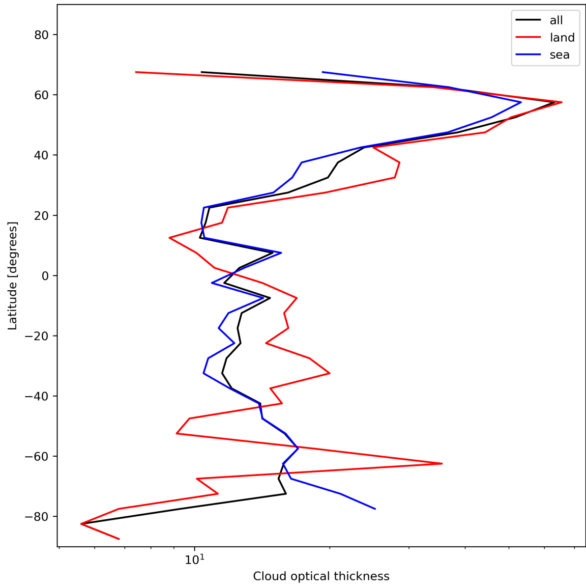
Figure 25: Zonal average of “Cloud optical thickness” for 2023-12-12 to 2023-12-14.
