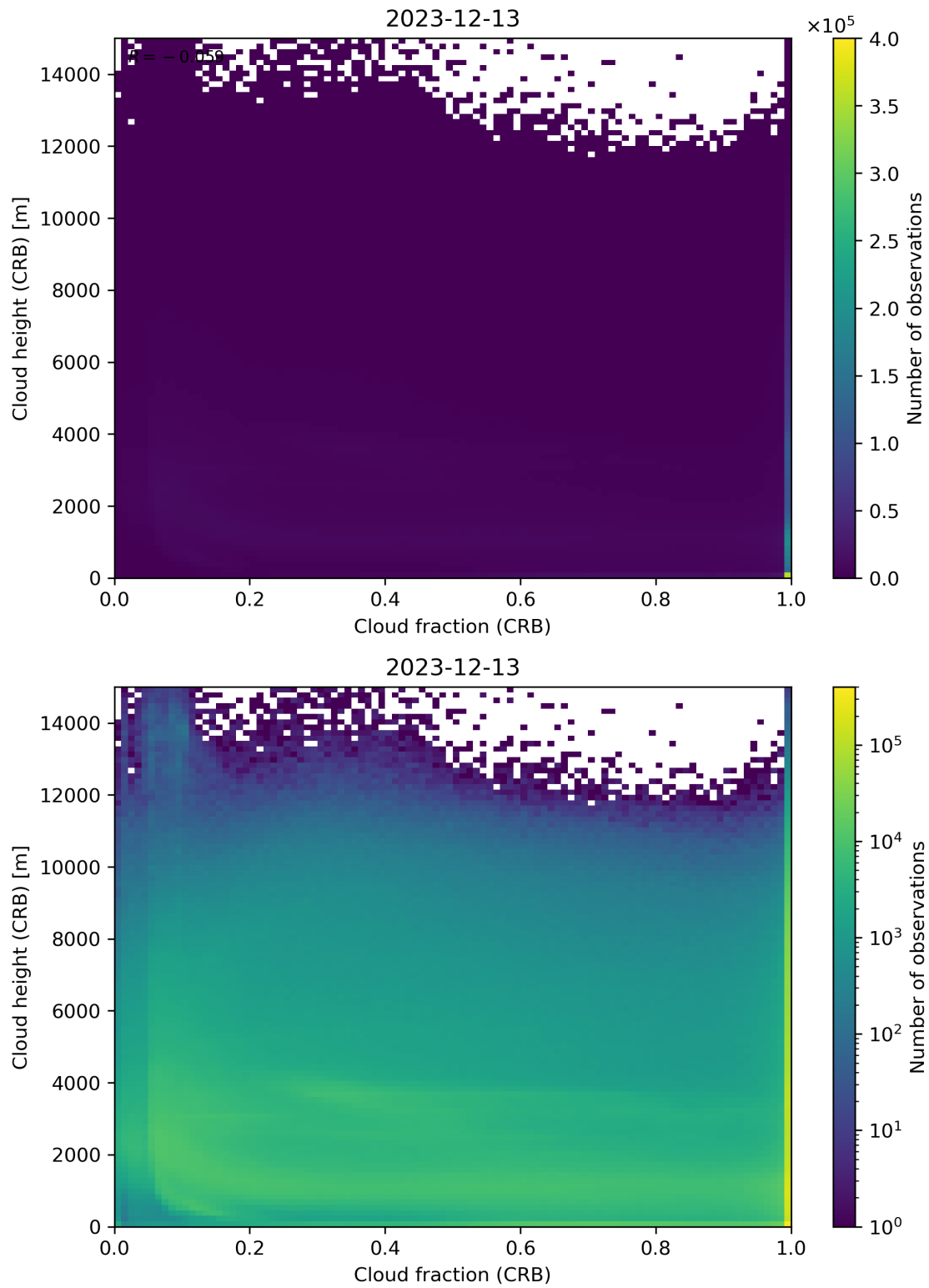
Figure 79: Scatter density plot of “Cloud fraction (CRB)” against “Cloud height (CRB)” for 2023-12-12 to 2023-12-14.
