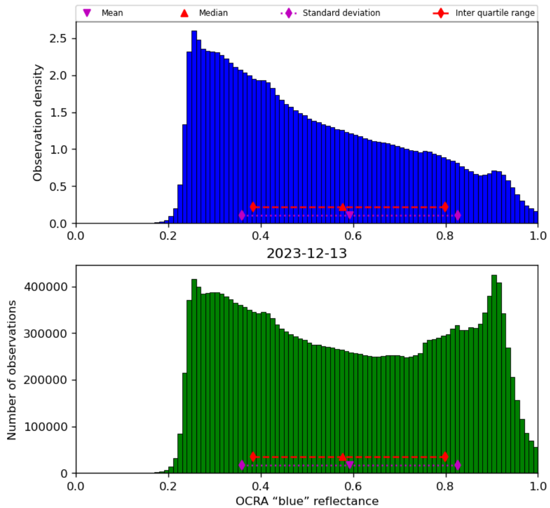
Figure 51: Histogram of “OCRA “blue” reflectance” for 2023-12-12 to 2023-12-14
