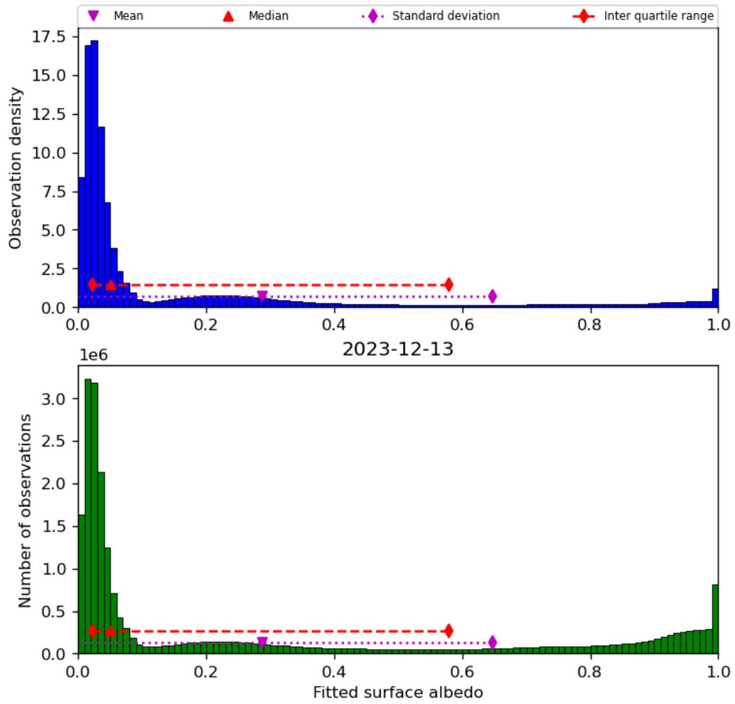
Figure 45: Histogram of “Fitted surface albedo” for 2023-12-12 to 2023-12-14
