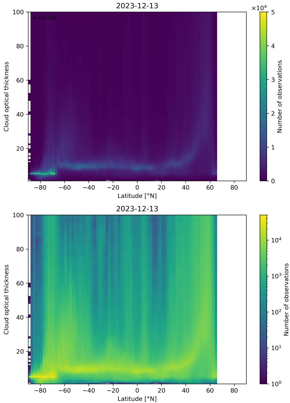
Figure 96: Scatter density plot of “Latitude” against “Cloud optical thickness” for 2023-12-12 to 2023-12-14.
