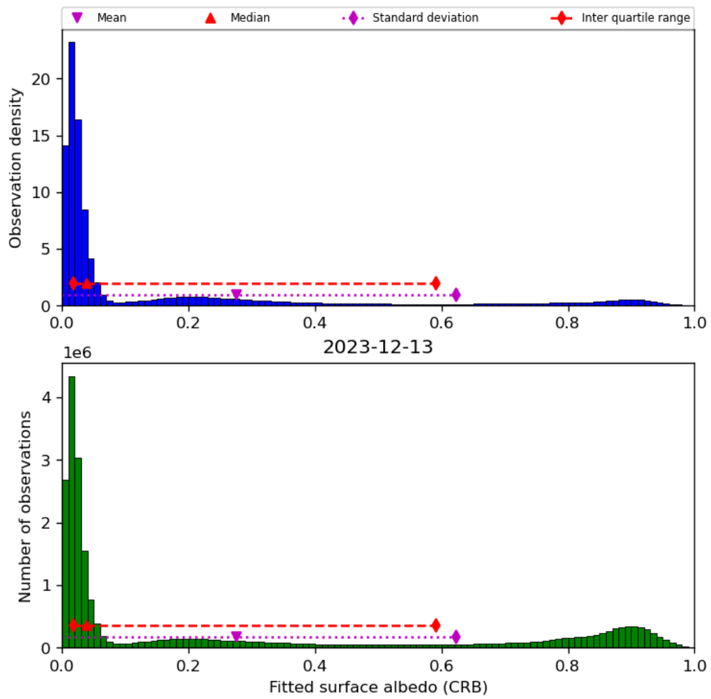
Figure 46: Histogram of “Fitted surface albedo (CRB)” for 2023-12-12 to 2023-12-14
