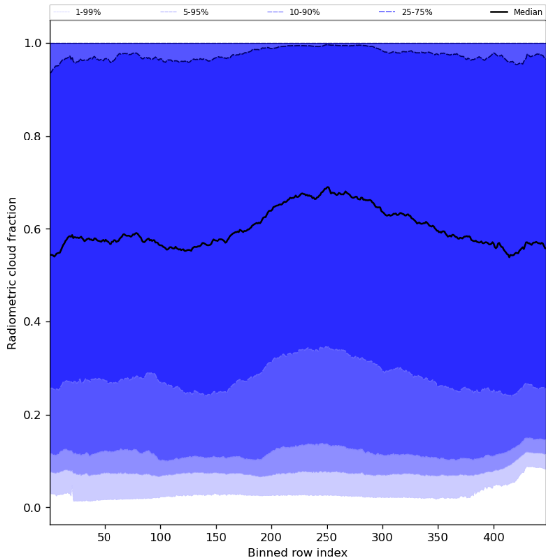
Figure 55: Along track statistics of “Radiometric cloud fraction” for 2023-12-12 to 2023-12-14
