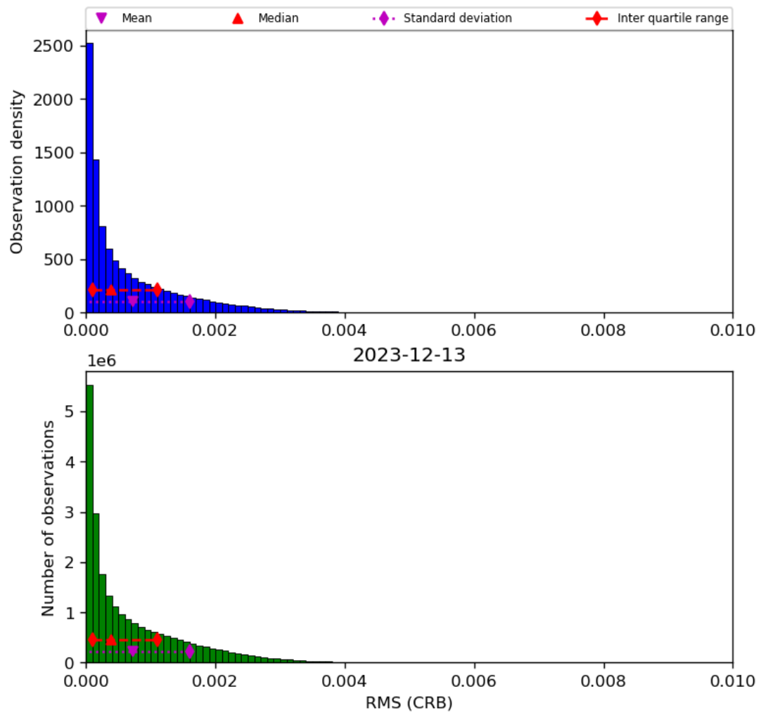
Figure 48: Histogram of “RMS (CRB)” for 2023-12-12 to 2023-12-14
