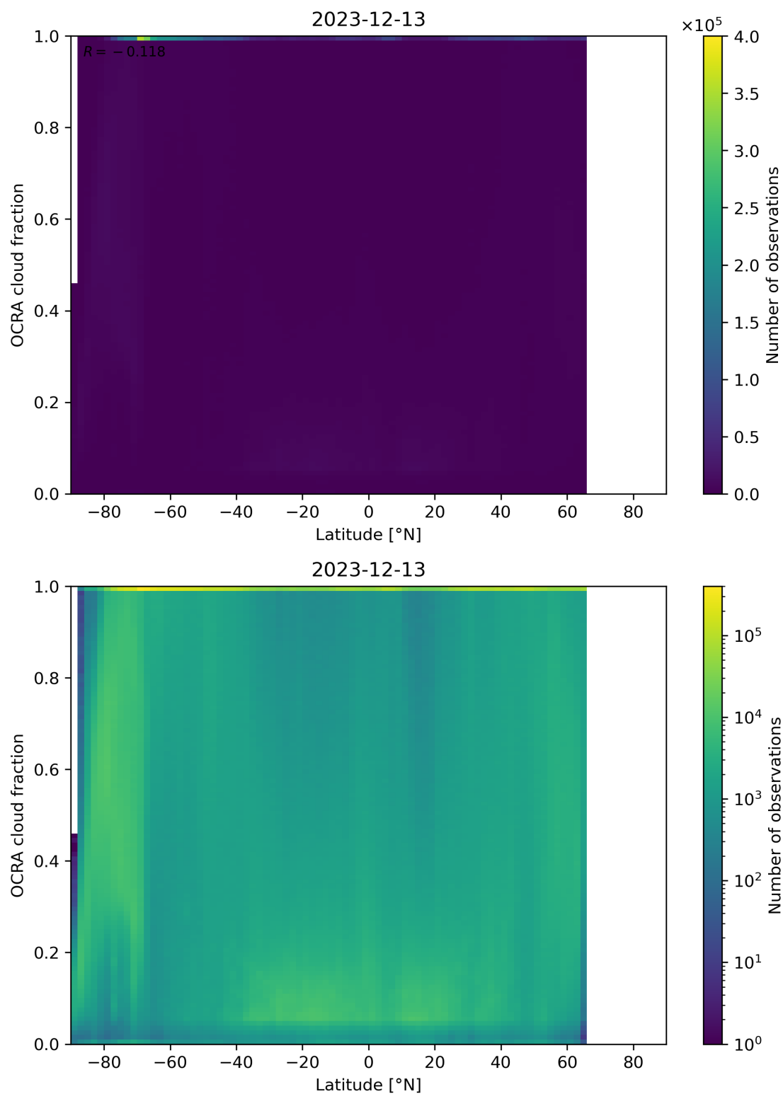
Figure 93: Scatter density plot of “Latitude” against “OCRA cloud fraction” for 2023-12-12 to 2023-12-14.
