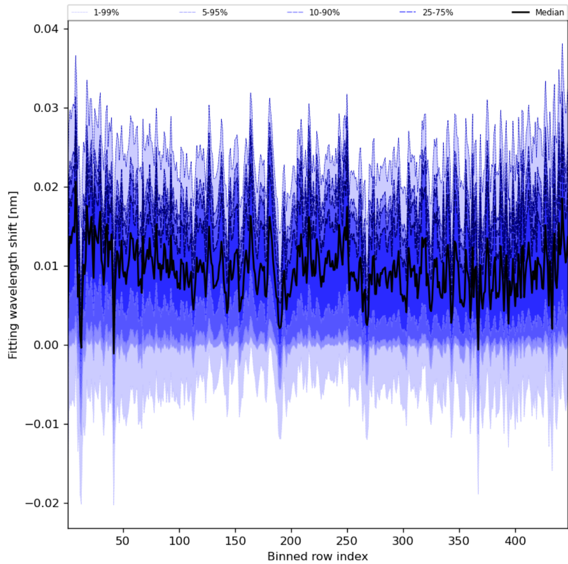
Figure 65: Along track statistics of “Fitting wavelength shift” for 2023-12-12 to 2023-12-14
