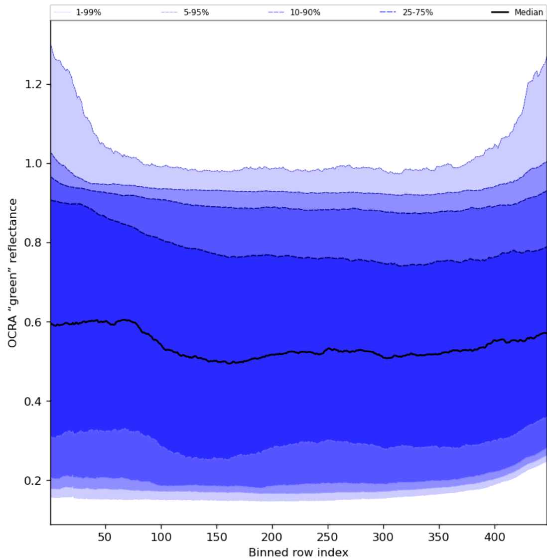
Figure 68: Along track statistics of “OCRA “green” reflectance” for 2023-12-12 to 2023-12-14
