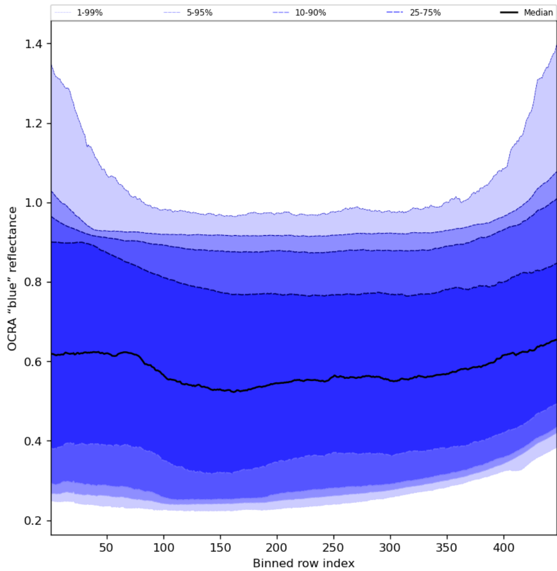
Figure 67: Along track statistics of “OCRA “blue” reflectance” for 2023-12-12 to 2023-12-14
