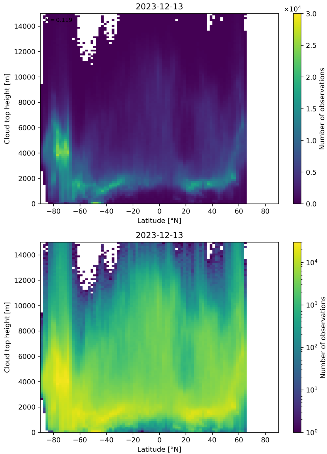
Figure 97: Scatter density plot of “Latitude” against “Cloud top height” for 2023-12-12 to 2023-12-14.
