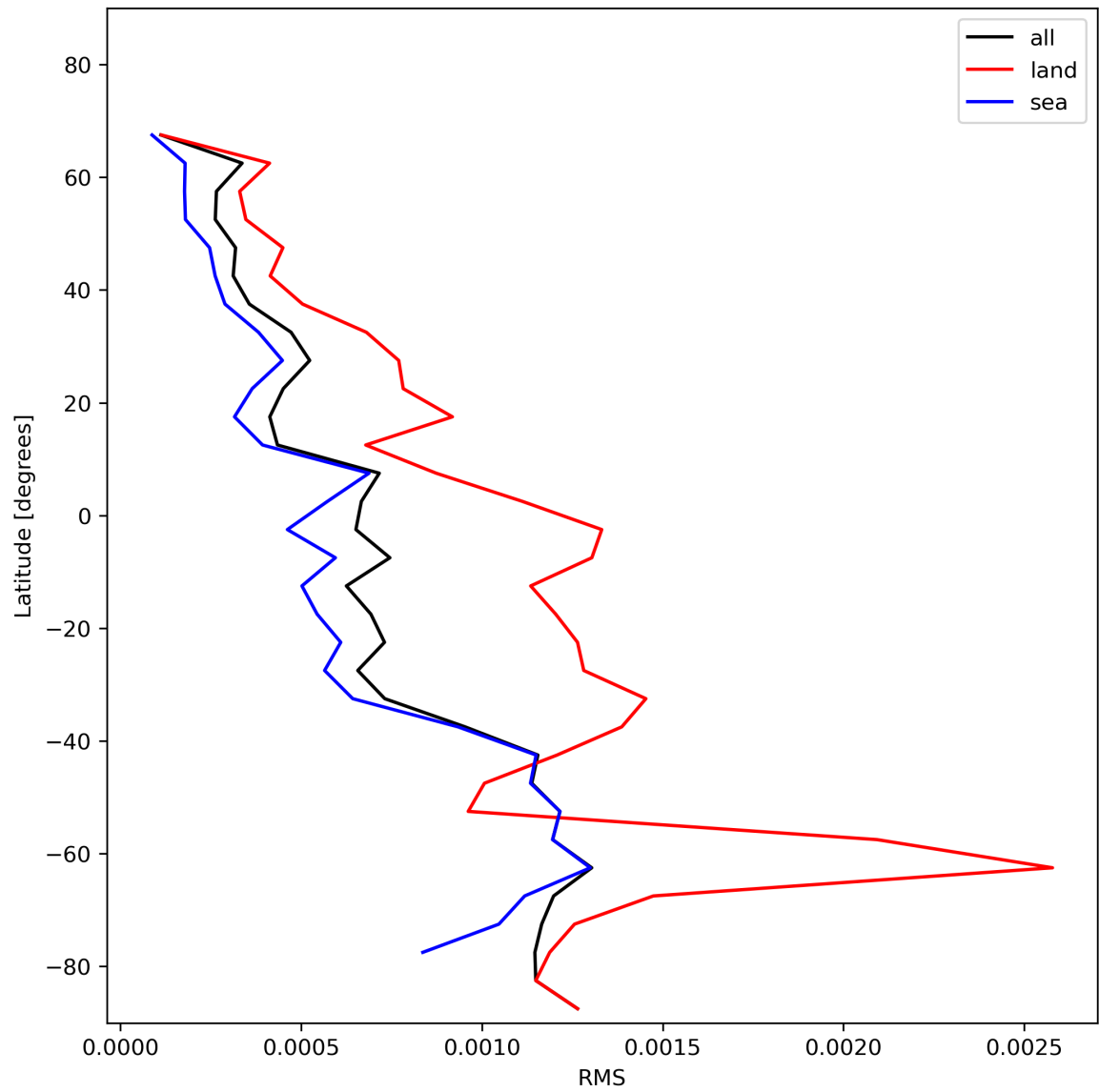
Figure 31: Zonal average of “RMS” for 2023-12-12 to 2023-12-14.
