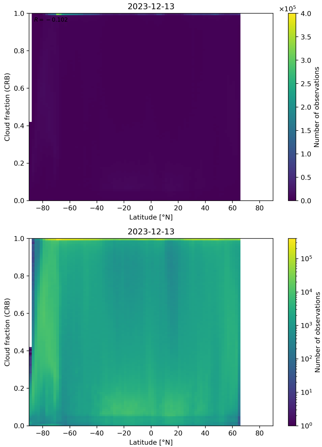
Figure 94: Scatter density plot of “Latitude” against “Cloud fraction (CRB)” for 2023-12-12 to 2023-12-14.
