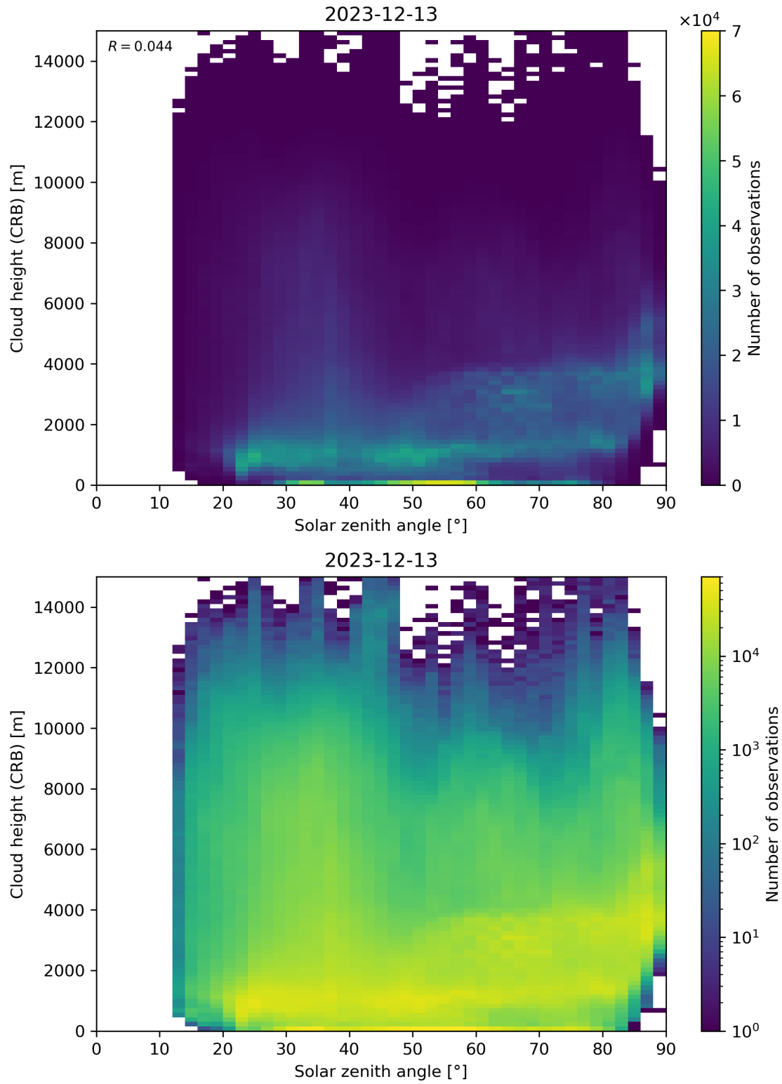
Figure 102: Scatter density plot of “Solar zenith angle” against “Cloud height (CRB)” for 2023-12-12 to 2023-12-14.
