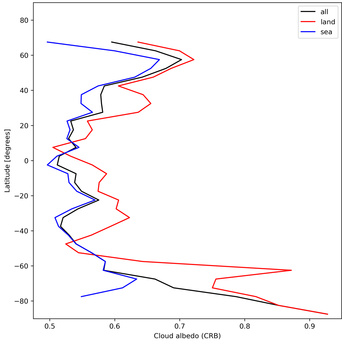
Figure 28: Zonal average of “Cloud albedo (CRB)” for 2023-12-12 to 2023-12-14.
