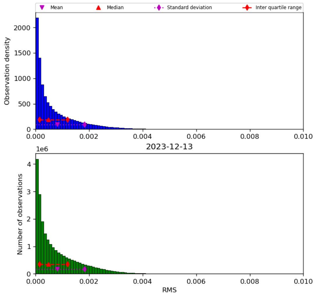
Figure 47: Histogram of “RMS” for 2023-12-12 to 2023-12-14
