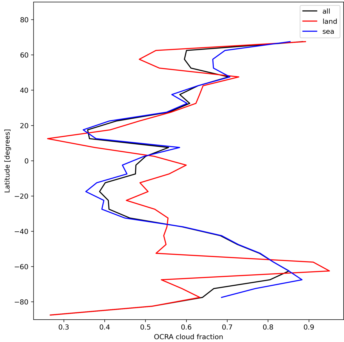
Figure 34: Zonal average of “OCRA cloud fraction” for 2023-12-12 to 2023-12-14.
