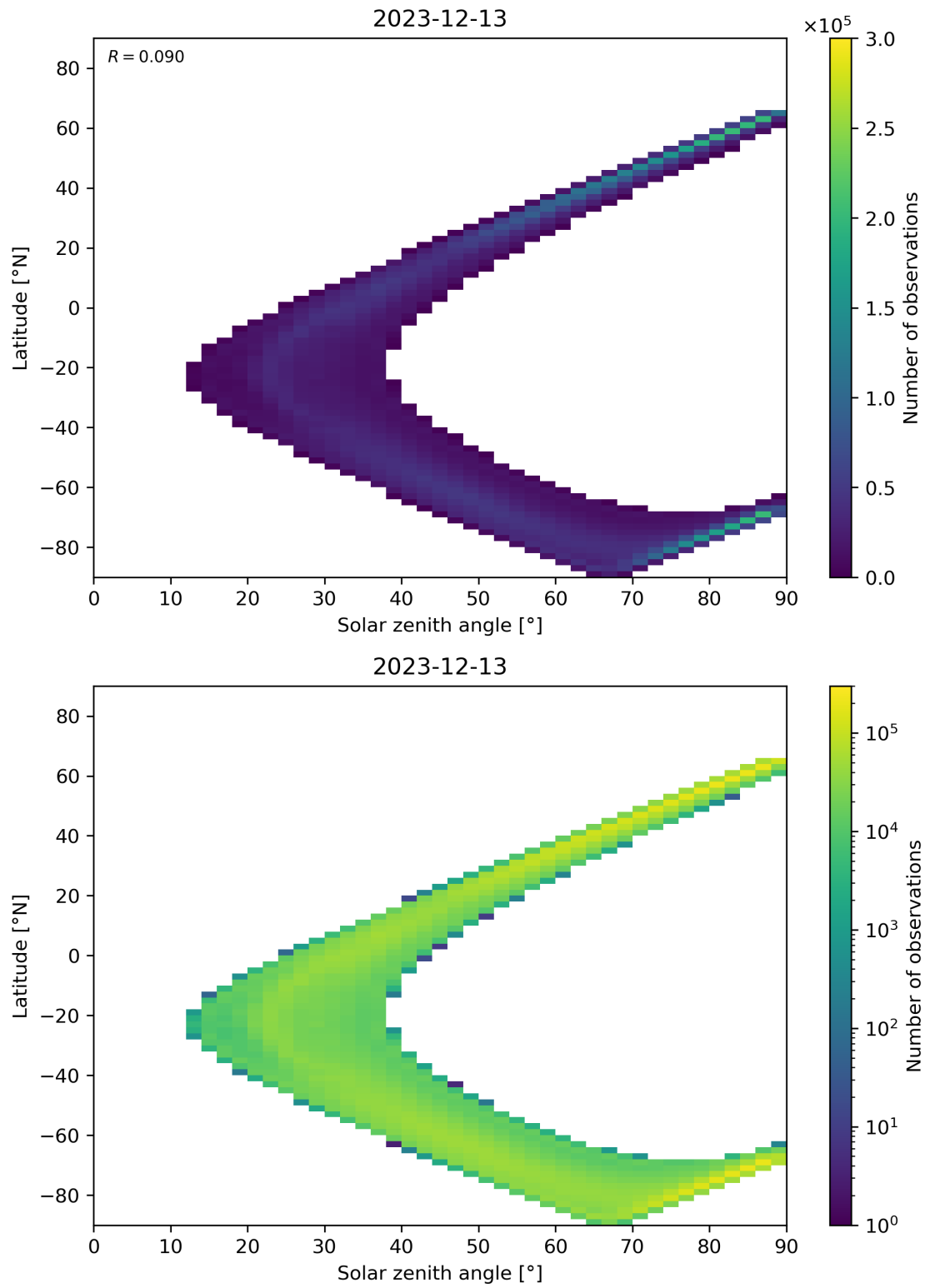
Figure 105: Scatter density plot of “Solar zenith angle” against “Latitude” for 2023-12-12 to 2023-12-14.
