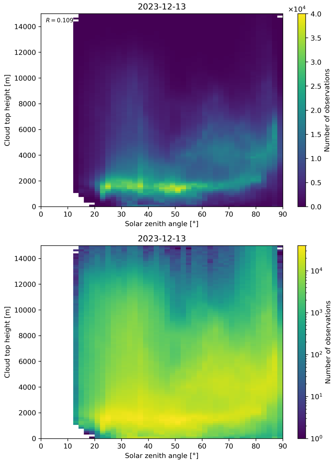
Figure 104: Scatter density plot of “Solar zenith angle” against “Cloud top height” for 2023-12-12 to 2023-12-14.
