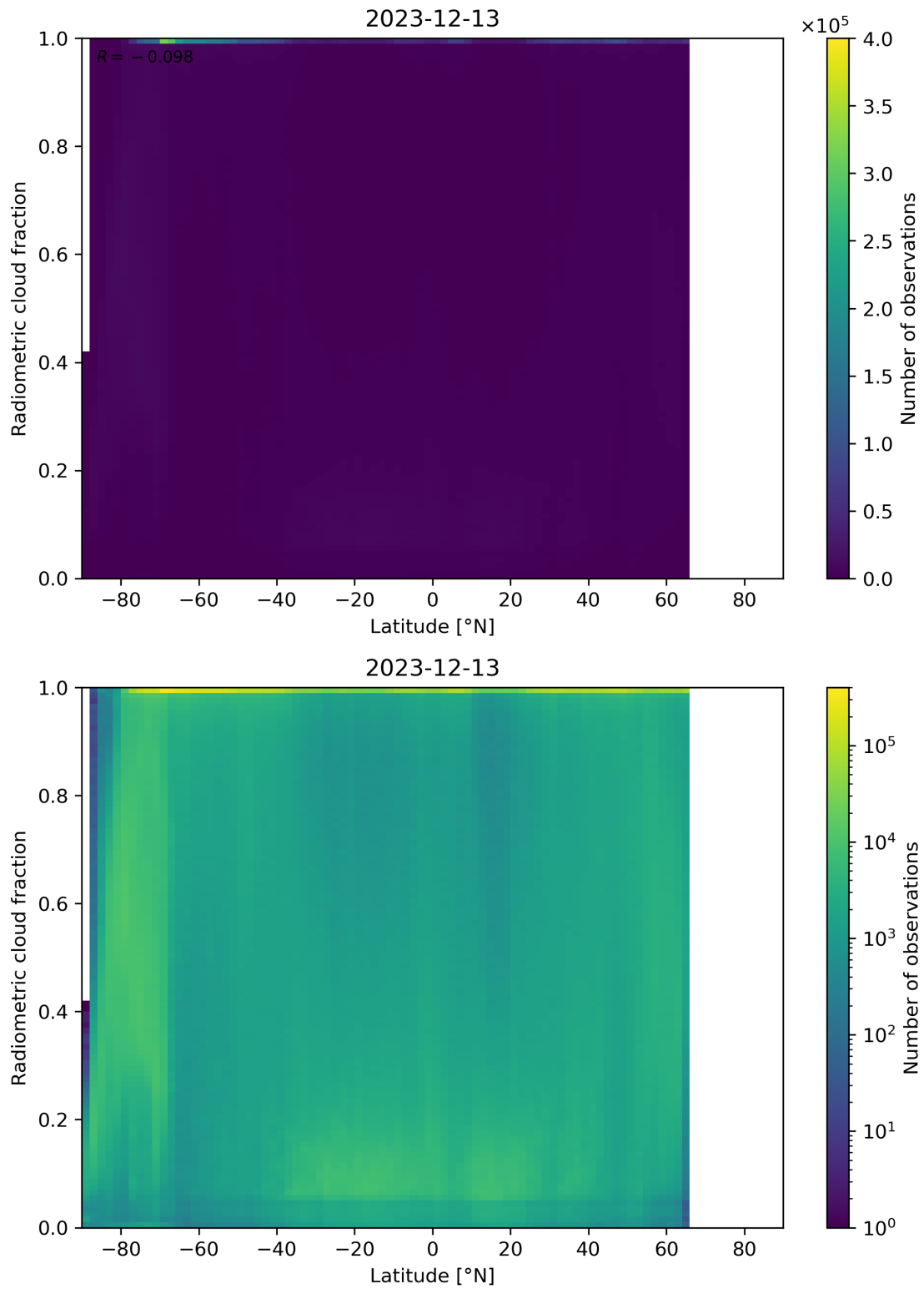
Figure 92: Scatter density plot of “Latitude” against “Radiometric cloud fraction” for 2023-12-12 to 2023-12-14.
