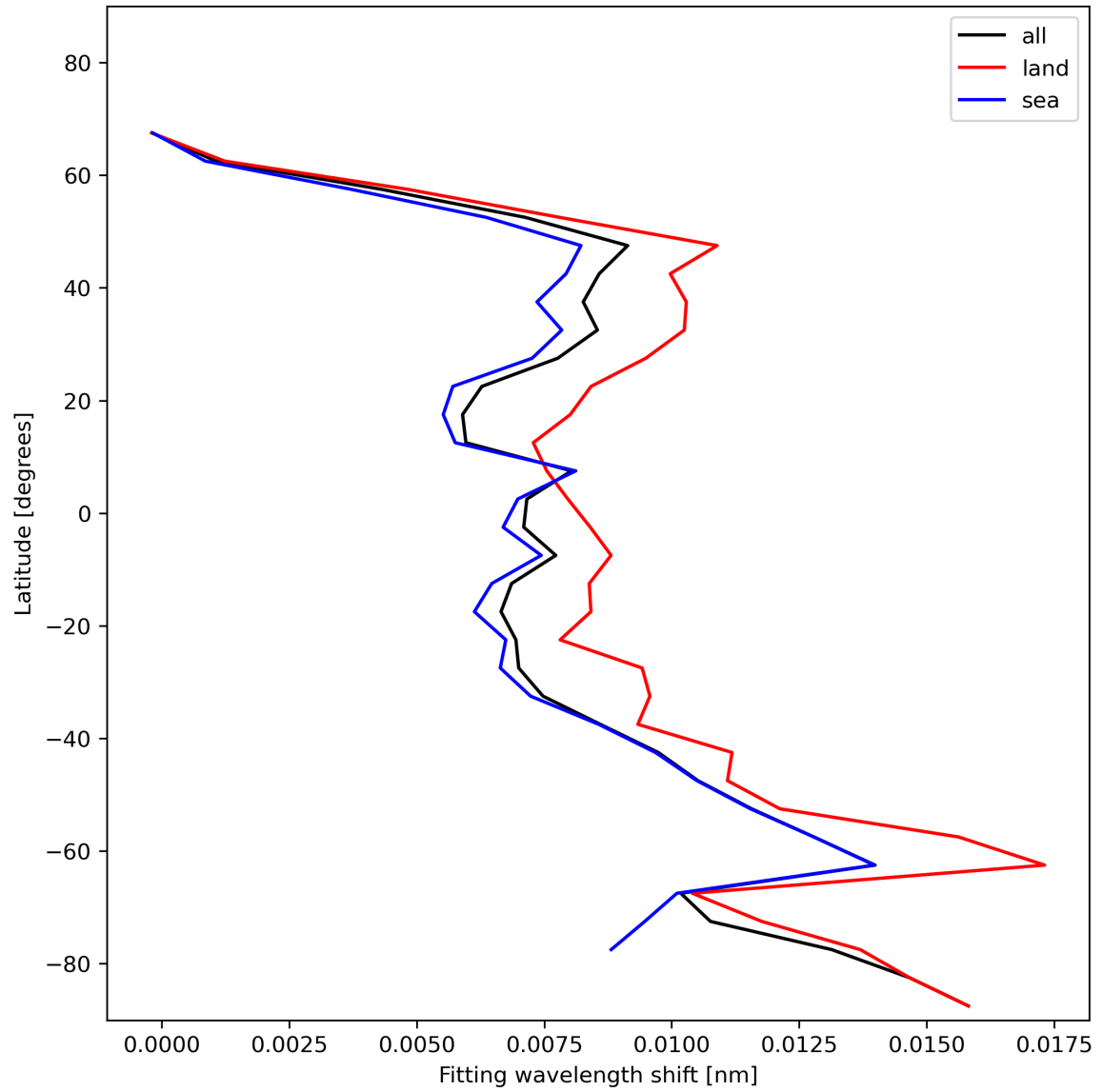
Figure 33: Zonal average of “Fitting wavelength shift” for 2023-12-12 to 2023-12-14.
