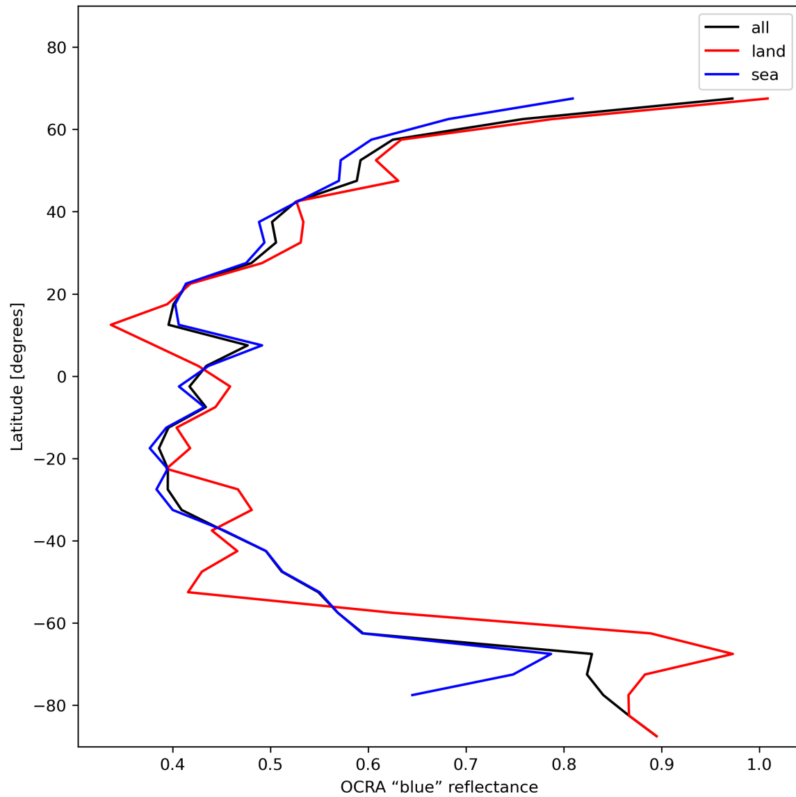
Figure 35: Zonal average of “OCRA “blue” reflectance” for 2023-12-12 to 2023-12-14.
