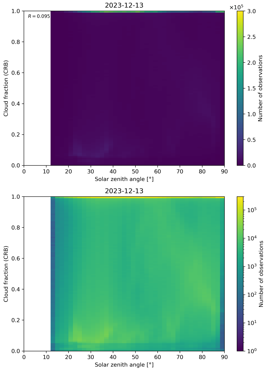
Figure 101: Scatter density plot of “Solar zenith angle” against “Cloud fraction (CRB)” for 2023-12-12 to 2023-12-14.
