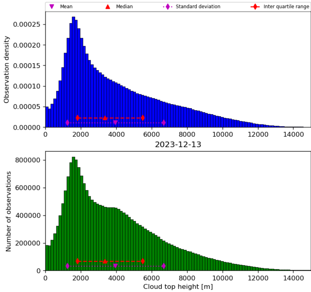
Figure 40: Histogram of “Cloud top height” for 2023-12-12 to 2023-12-14
