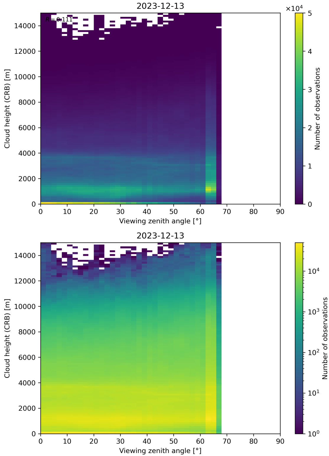
Figure 110: Scatter density plot of “Viewing zenith angle” against “Cloud height (CRB)” for 2023-12-12 to 2023-12-14.
