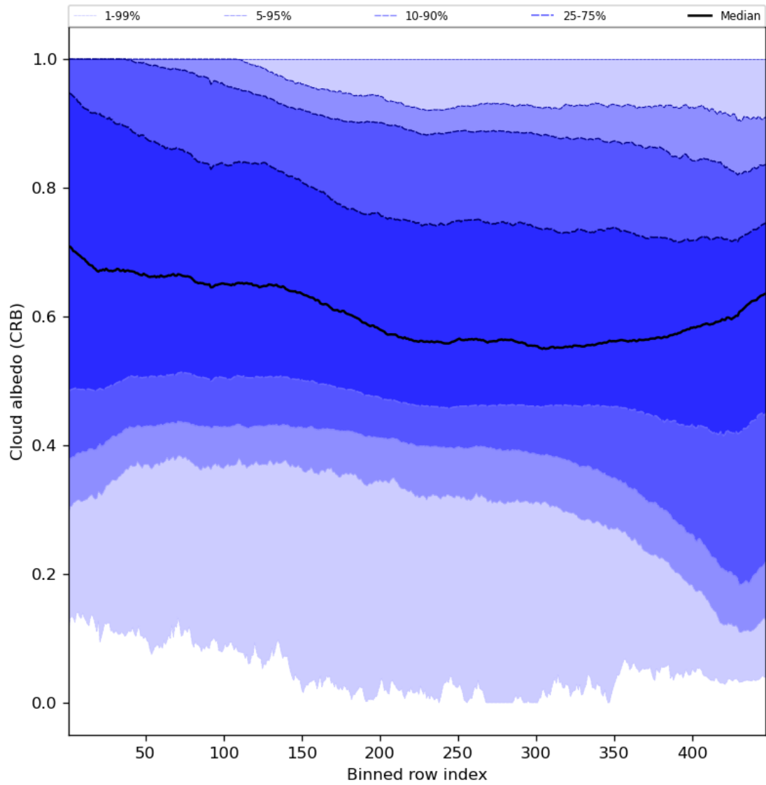
Figure 60: Along track statistics of “Cloud albedo (CRB)” for 2023-12-12 to 2023-12-14
