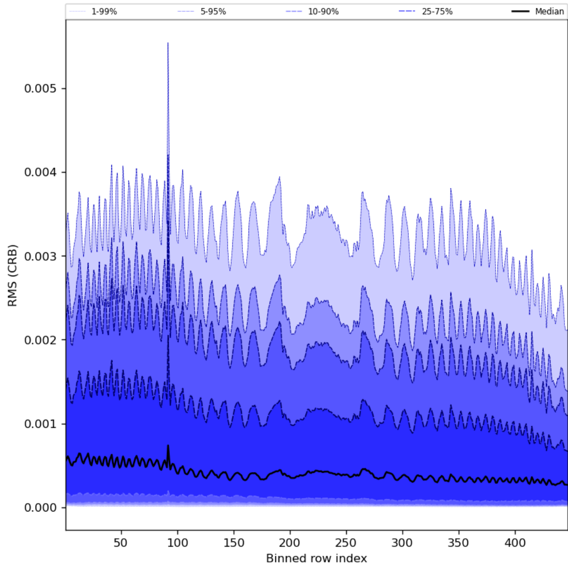
Figure 64: Along track statistics of “RMS (CRB)” for 2023-12-12 to 2023-12-14
