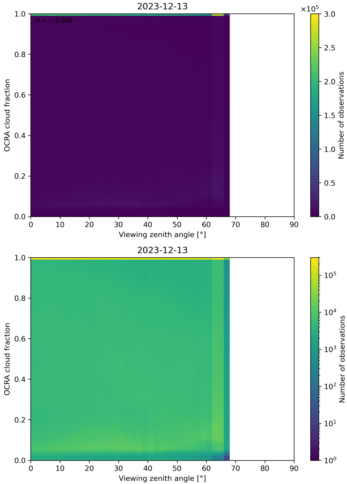
Figure 108: Scatter density plot of “Viewing zenith angle” against “OCRA cloud fraction” for 2023-12-12 to 2023-12-14.
