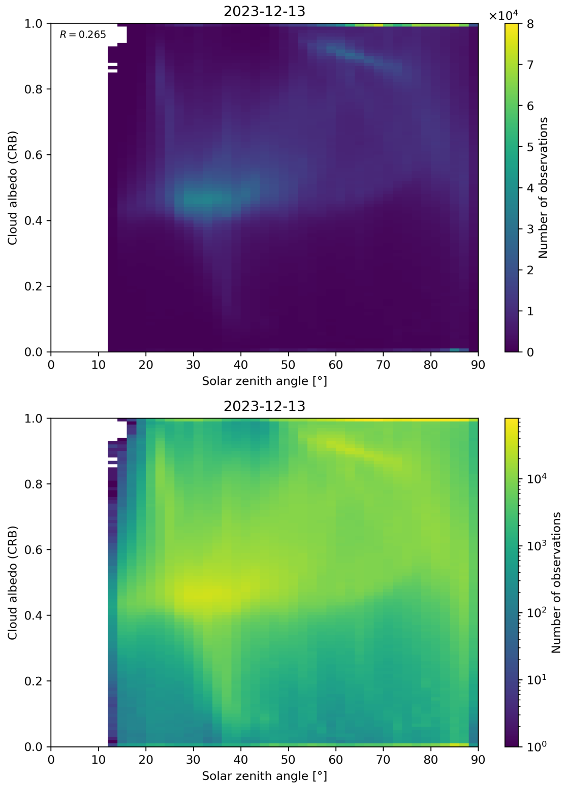
Figure 98: Scatter density plot of “Solar zenith angle” against “Cloud albedo (CRB)” for 2023-12-12 to 2023-12-14.
