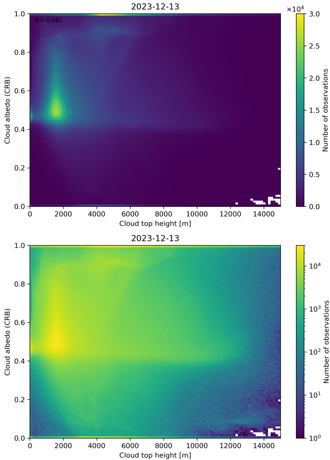
Figure 86: Scatter density plot of “Cloud top height” against “Cloud albedo (CRB)” for 2023-12-12 to 2023-12-14.
