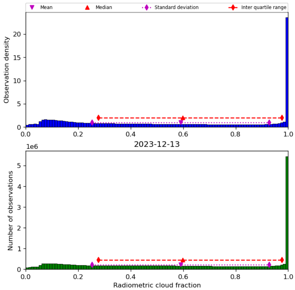
Figure 39: Histogram of “Radiometric cloud fraction” for 2023-12-12 to 2023-12-14
