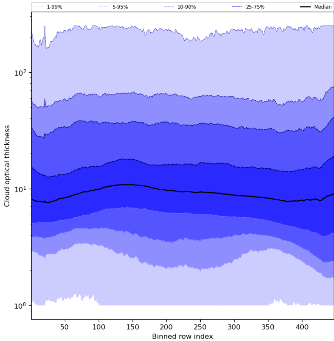
Figure 57: Along track statistics of “Cloud optical thickness” for 2023-12-12 to 2023-12-14
