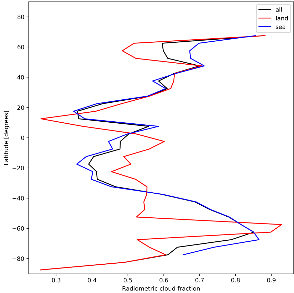
Figure 23: Zonal average of “Radiometric cloud fraction” for 2023-12-12 to 2023-12-14.
