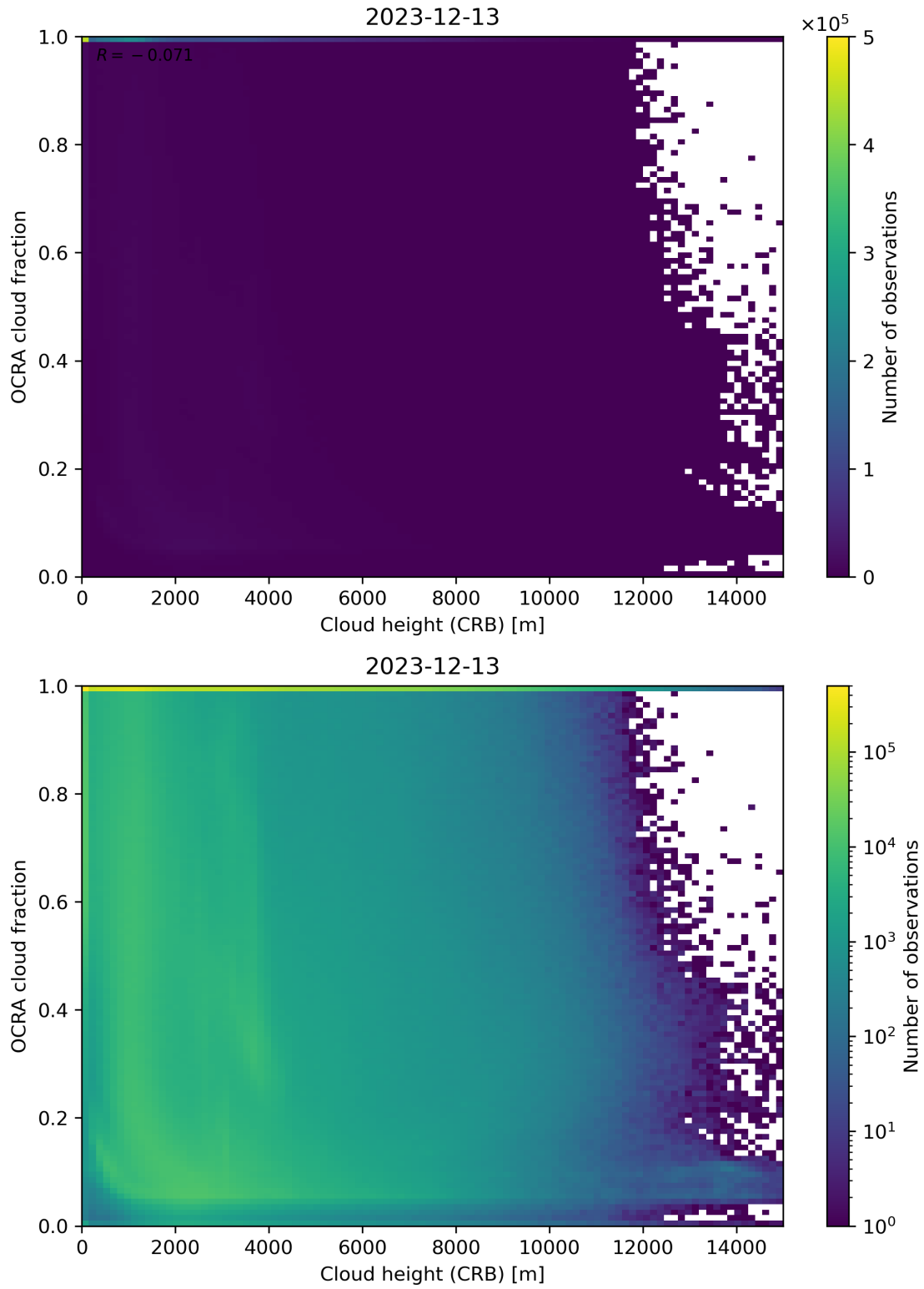
Figure 81: Scatter density plot of “Cloud height (CRB)” against “OCRA cloud fraction” for 2023-12-12 to 2023-12-14.
