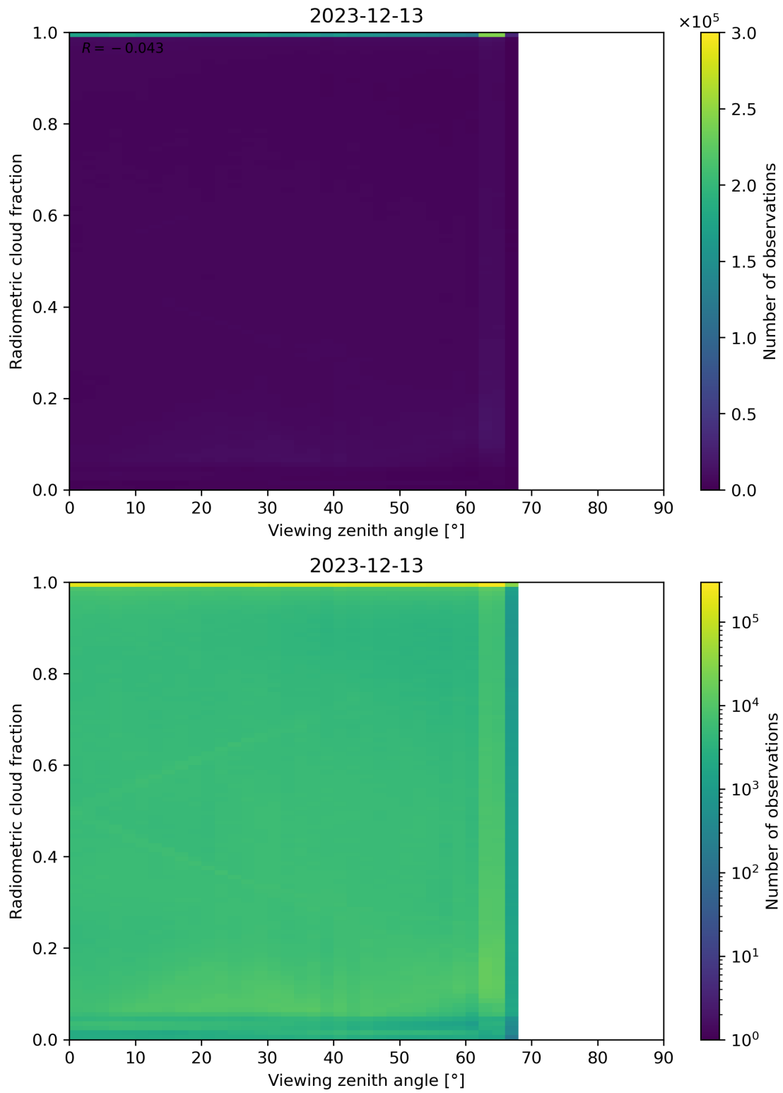
Figure 107: Scatter density plot of “Viewing zenith angle” against “Radiometric cloud fraction” for 2023-12-12 to 2023-12-14.
