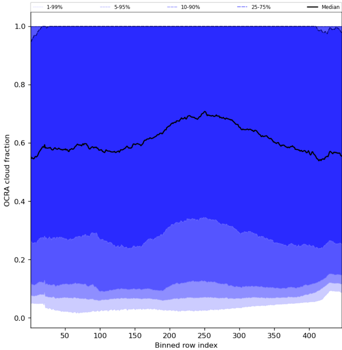
Figure 66: Along track statistics of “OCRA cloud fraction” for 2023-12-12 to 2023-12-14
