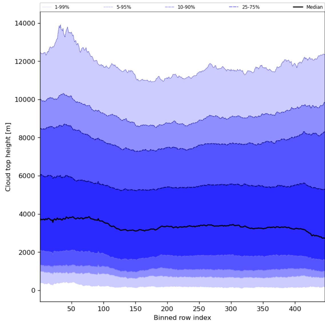
Figure 56: Along track statistics of “Cloud top height” for 2023-12-12 to 2023-12-14
