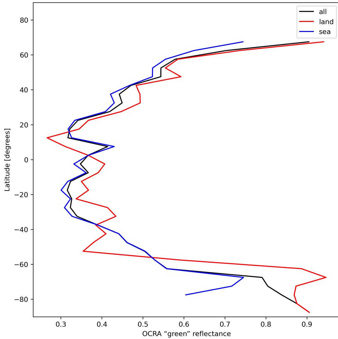
Figure 36: Zonal average of “OCRA “green” reflectance” for 2023-12-12 to 2023-12-14.
