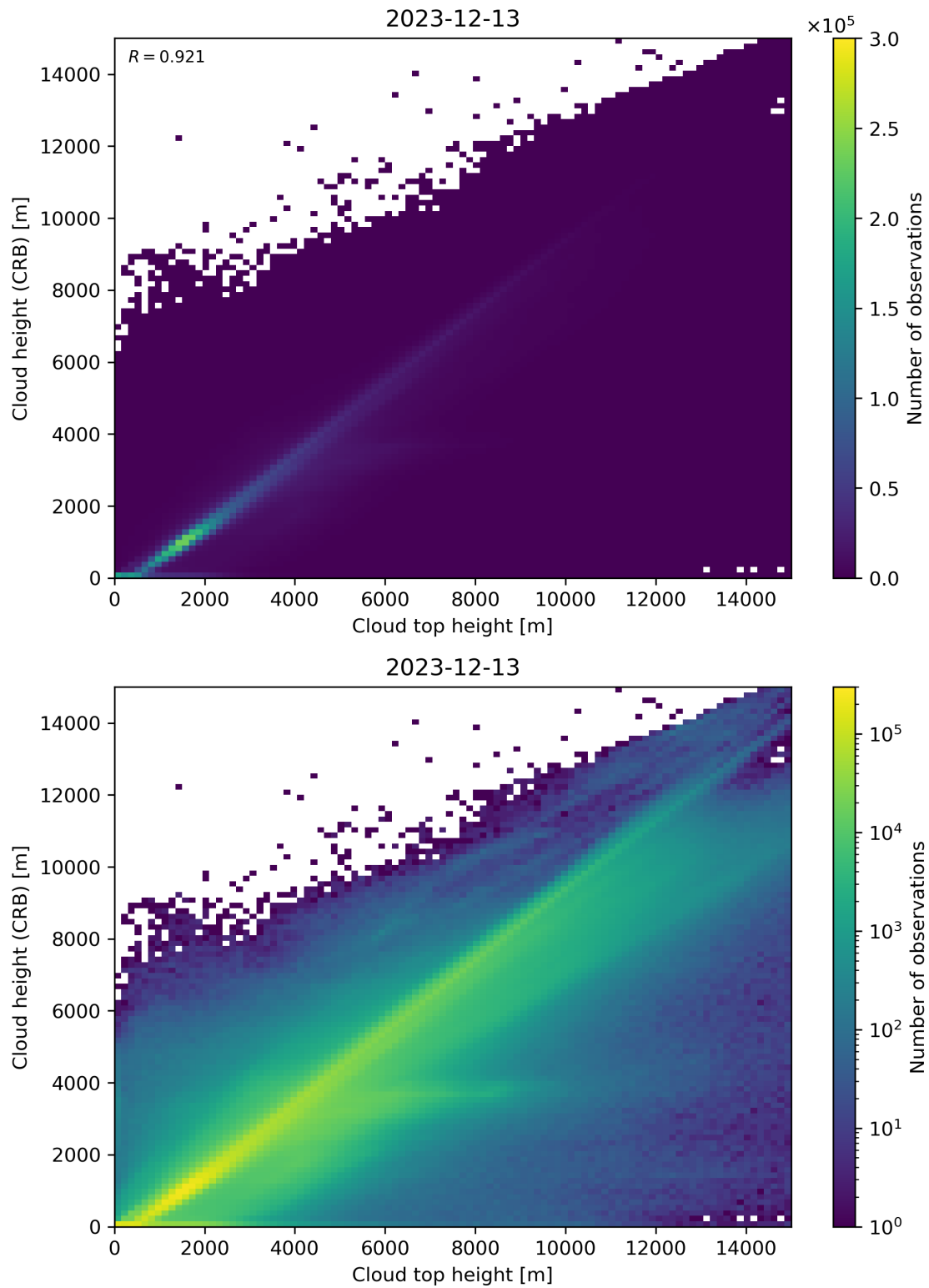
Figure 89: Scatter density plot of “Cloud top height” against “Cloud height (CRB)” for 2023-12-12 to 2023-12-14.
