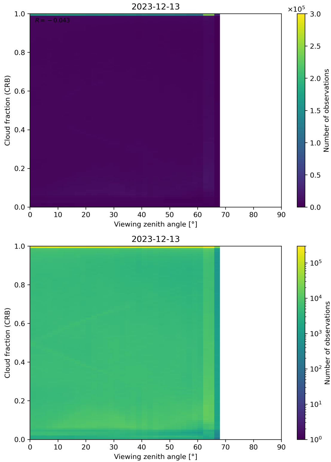
Figure 109: Scatter density plot of “Viewing zenith angle” against “Cloud fraction (CRB)” for 2023-12-12 to 2023-12-14.
