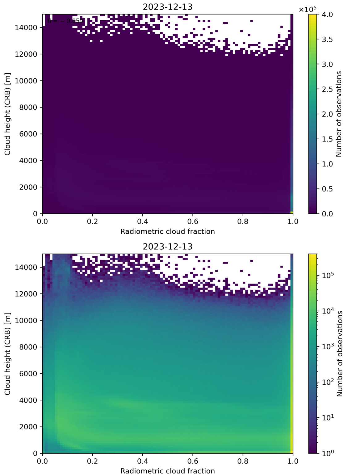
Figure 74: Scatter density plot of “Radiometric cloud fraction” against “Cloud height (CRB)” for 2023-12-12 to 2023-12-14.
