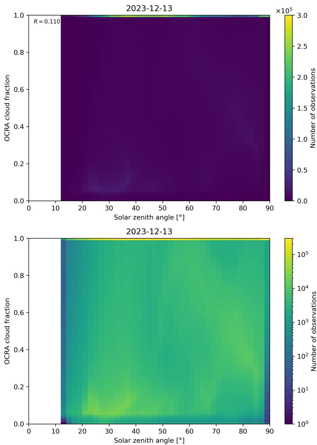
Figure 100: Scatter density plot of “Solar zenith angle” against “OCRA cloud fraction” for 2023-12-12 to 2023-12-14.
