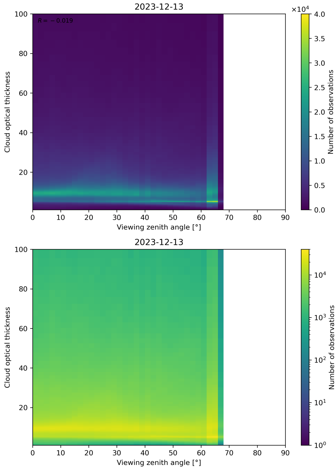
Figure 111: Scatter density plot of “Viewing zenith angle” against “Cloud optical thickness” for 2023-12-12 to 2023-12-14.
