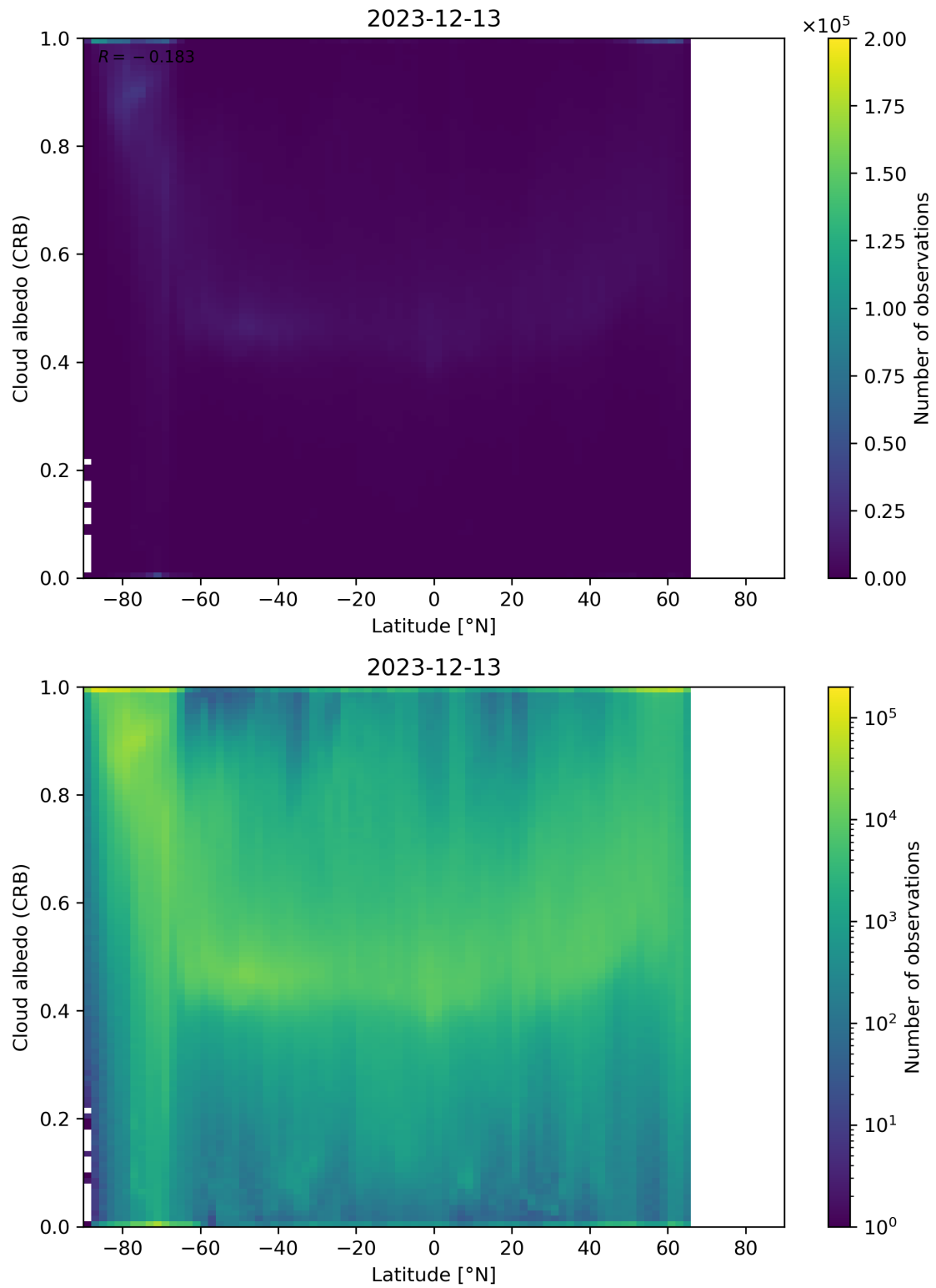
Figure 91: Scatter density plot of “Latitude” against “Cloud albedo (CRB)” for 2023-12-12 to 2023-12-14.
