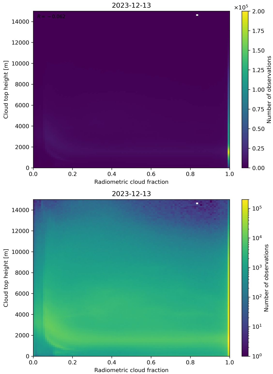
Figure 76: Scatter density plot of “Radiometric cloud fraction” against “Cloud top height” for 2023-12-12 to 2023-12-14.
