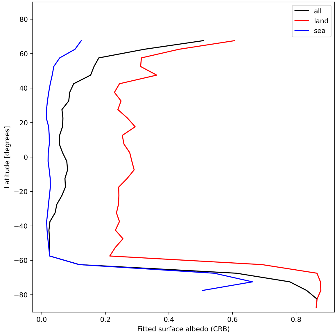
Figure 30: Zonal average of “Fitted surface albedo (CRB)” for 2023-12-12 to 2023-12-14.
