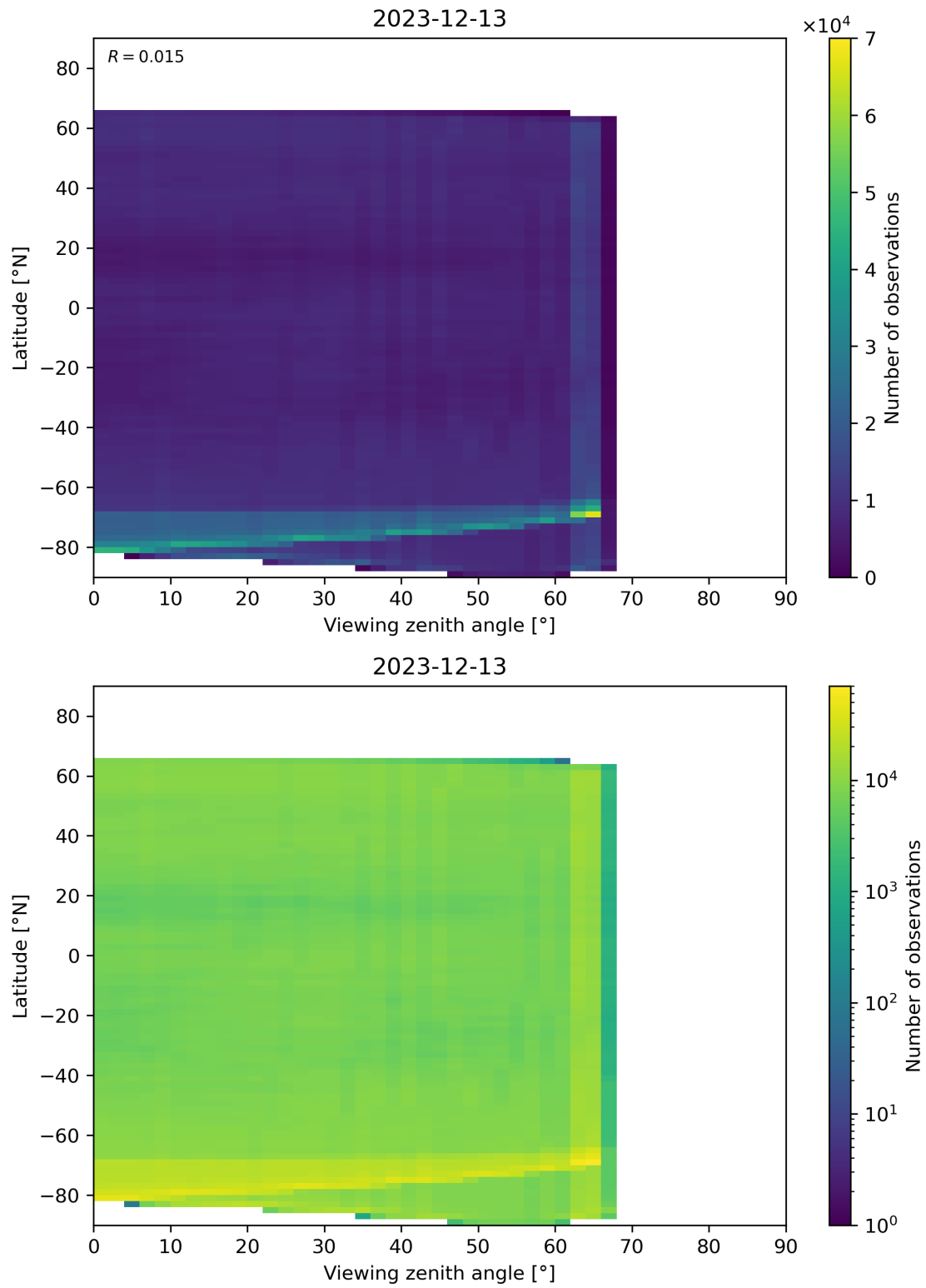
Figure 113: Scatter density plot of “Viewing zenith angle” against “Latitude” for 2023-12-12 to 2023-12-14.
