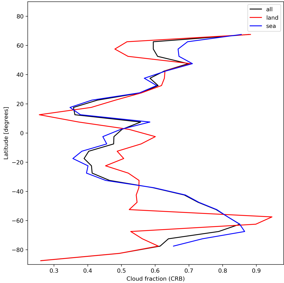
Figure 26: Zonal average of “Cloud fraction (CRB)” for 2023-12-12 to 2023-12-14.
