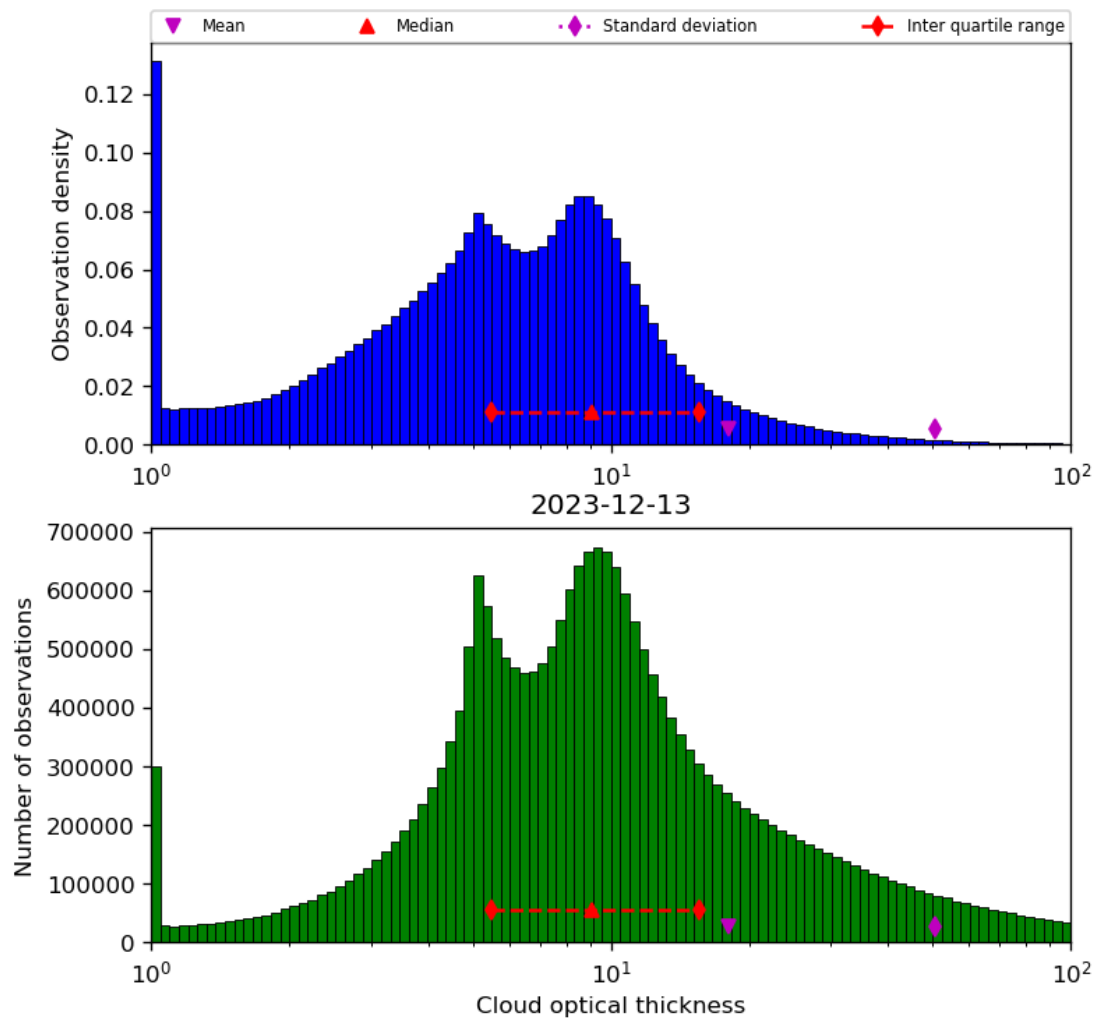
Figure 41: Histogram of “Cloud optical thickness” for 2023-12-12 to 2023-12-14
