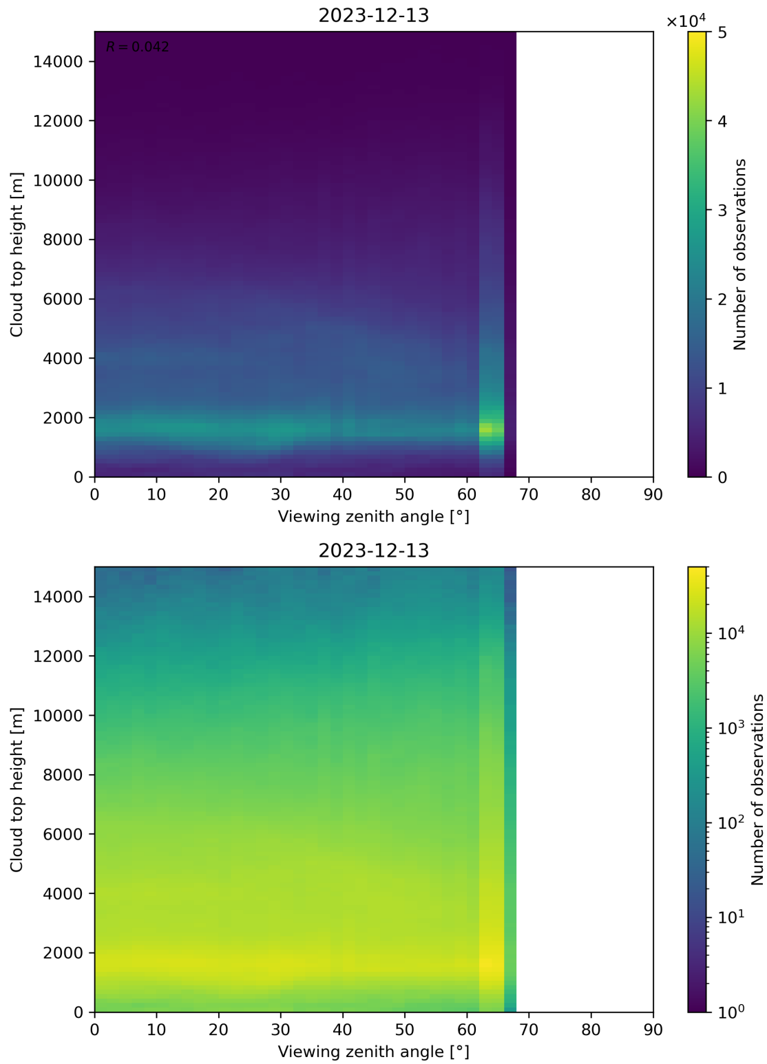
Figure 112: Scatter density plot of “Viewing zenith angle” against “Cloud top height” for 2023-12-12 to 2023-12-14.
