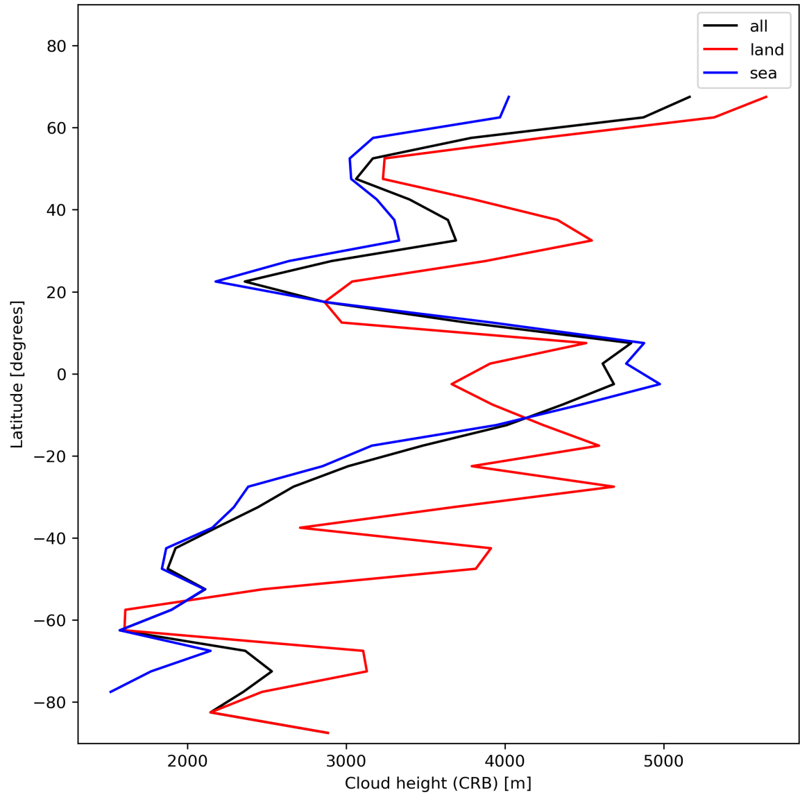
Figure 27: Zonal average of “Cloud height (CRB)” for 2023-12-12 to 2023-12-14.
