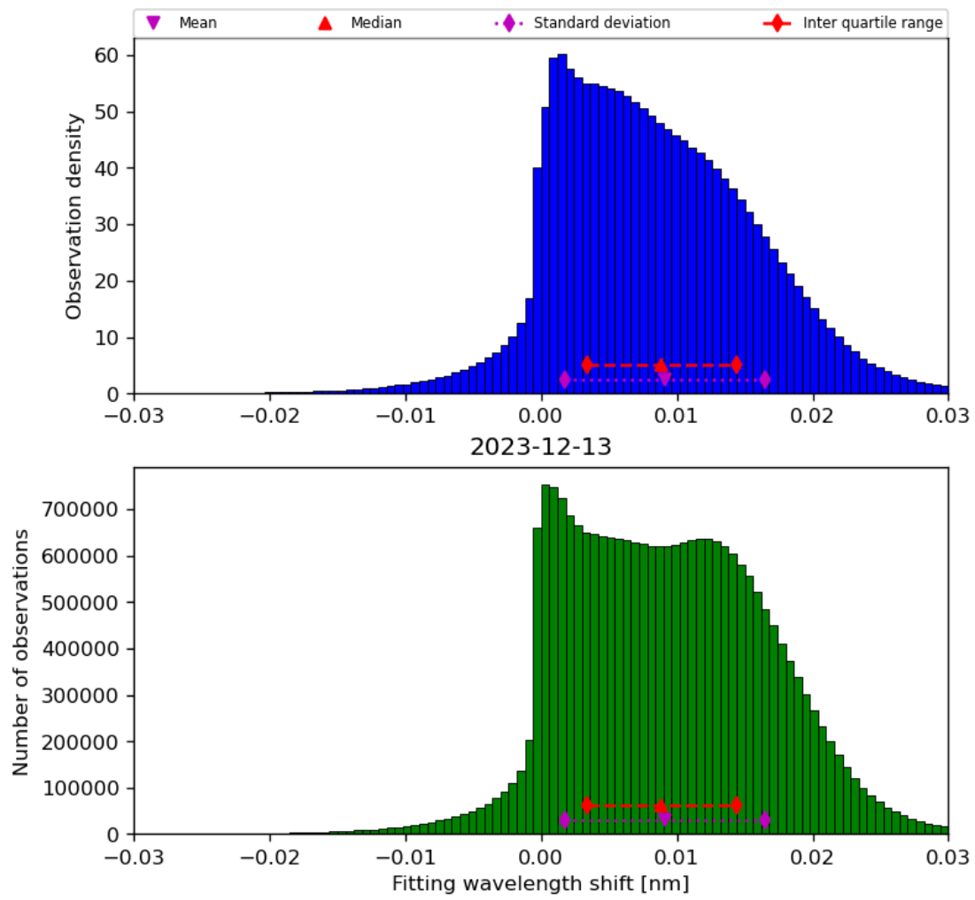
Figure 49: Histogram of “Fitting wavelength shift” for 2023-12-12 to 2023-12-14
