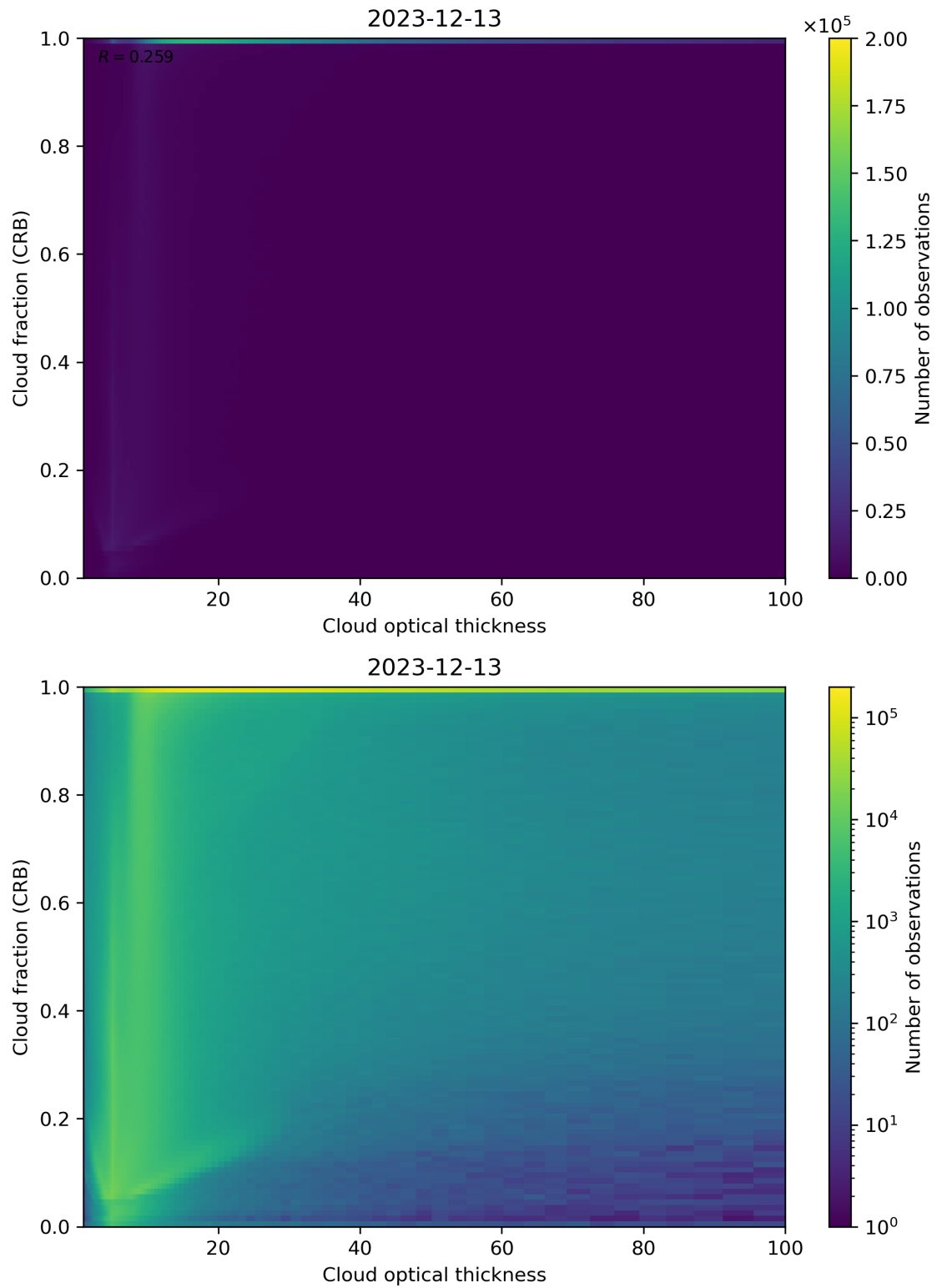
Figure 84: Scatter density plot of “Cloud optical thickness” against “Cloud fraction (CRB)” for 2023-12-12 to 2023-12-14.
