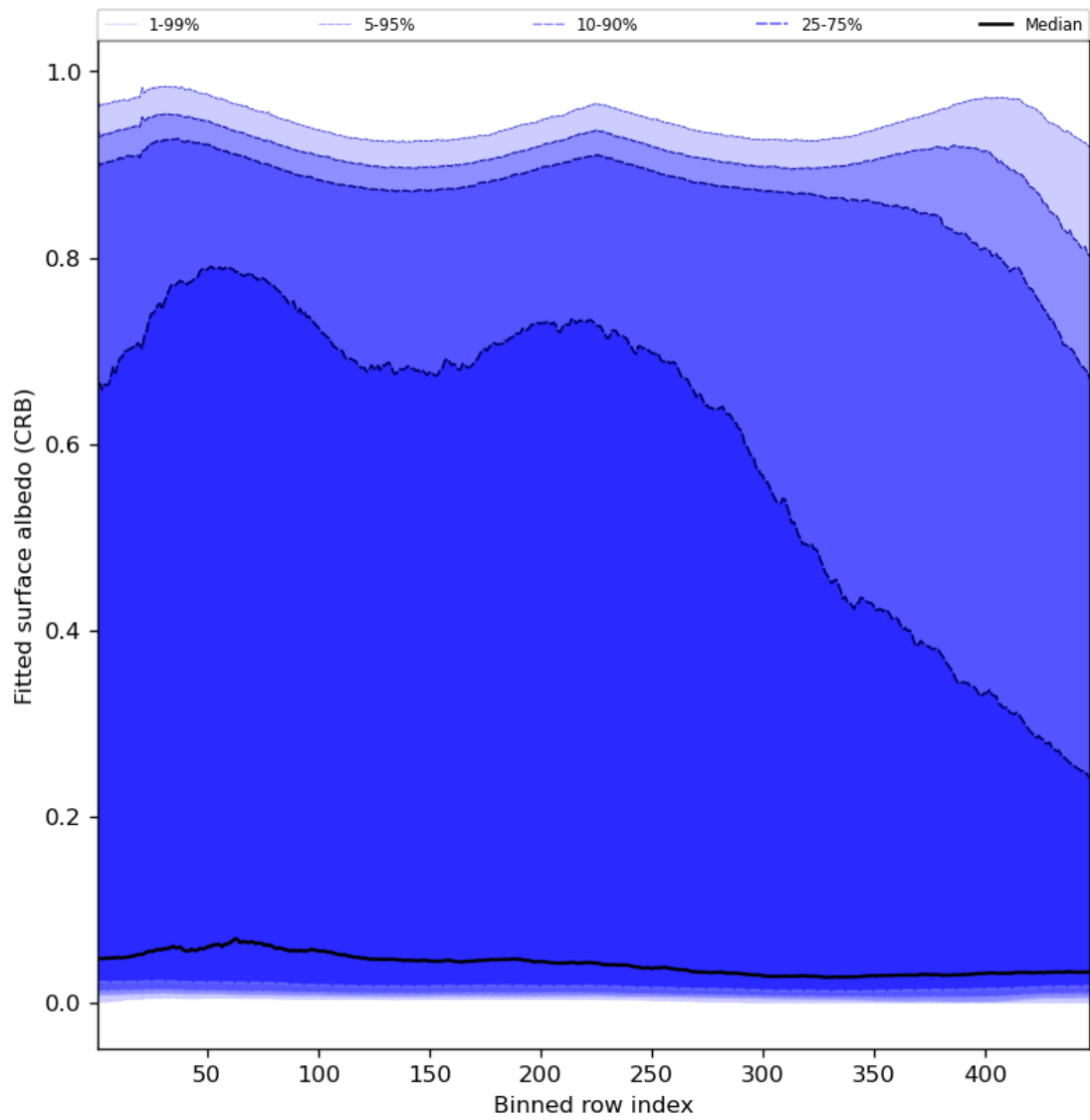
Figure 62: Along track statistics of “Fitted surface albedo (CRB)” for 2023-12-12 to 2023-12-14
