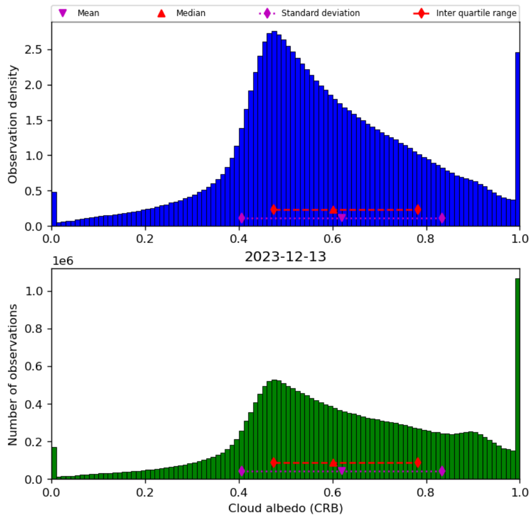
Figure 44: Histogram of “Cloud albedo (CRB)” for 2023-12-12 to 2023-12-14
