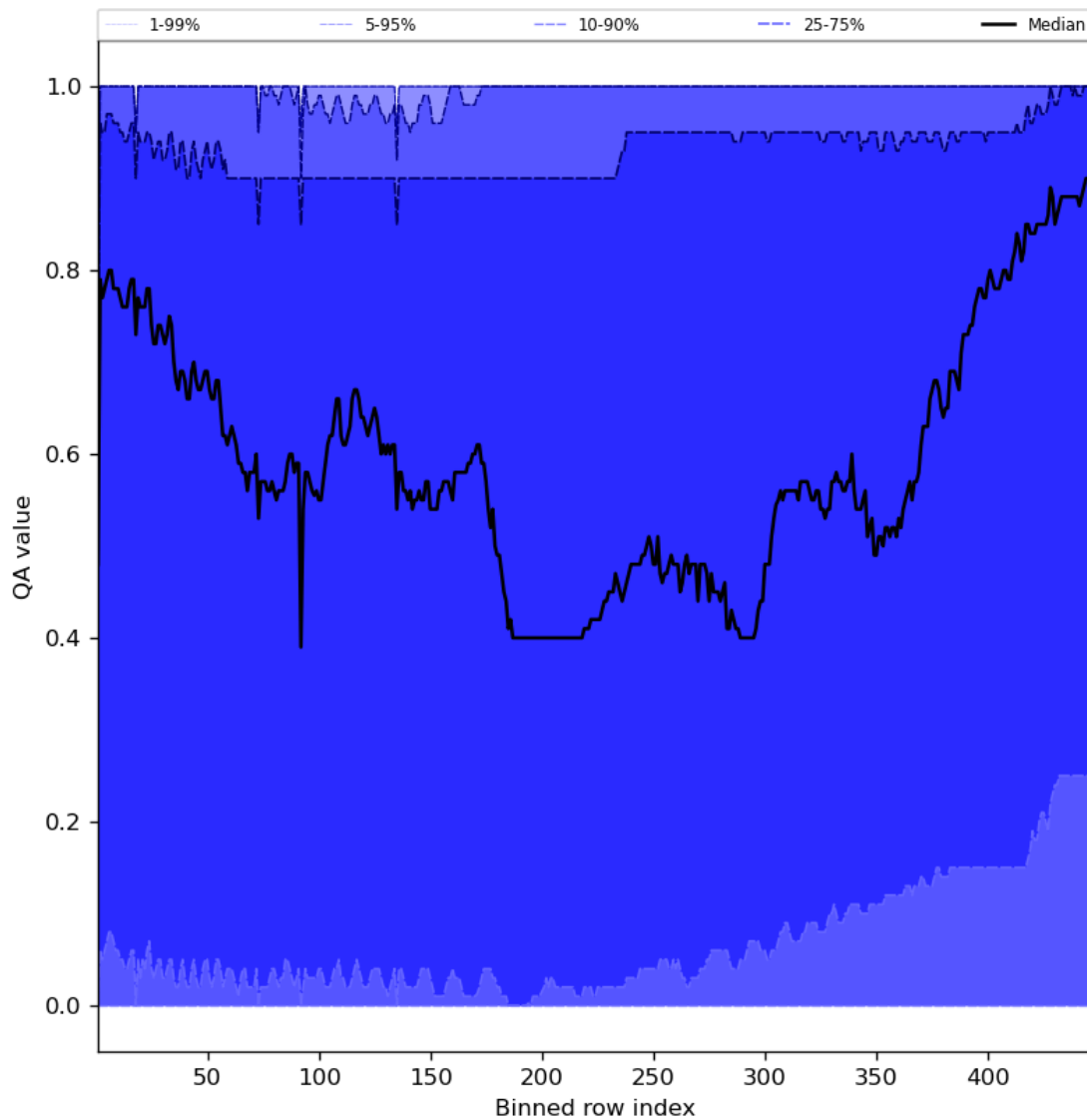
Figure 54: Along track statistics of “QA value” for 2023-12-12 to 2023-12-14
