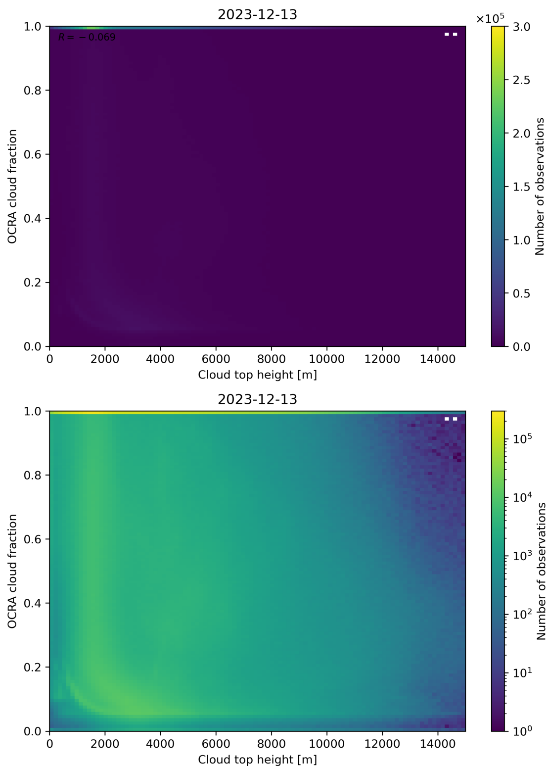
Figure 87: Scatter density plot of “Cloud top height” against “OCRA cloud fraction” for 2023-12-12 to 2023-12-14.
