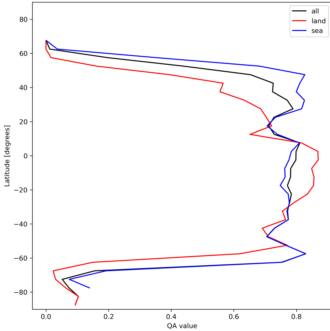
Figure 22: Zonal average of “QA value” for 2023-12-12 to 2023-12-14.
