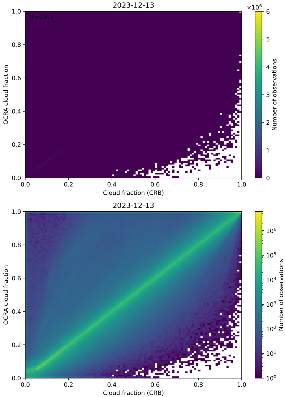
Figure 78: Scatter density plot of “Cloud fraction (CRB)” against “OCRA cloud fraction” for 2023-12-12 to 2023-12-14.
