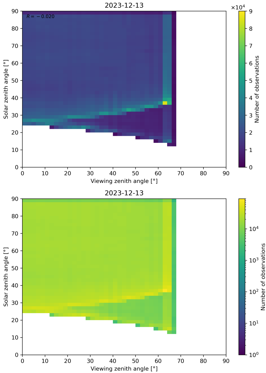
Figure 114: Scatter density plot of “Viewing zenith angle” against “Solar zenith angle” for 2023-12-12 to 2023-12-14.
