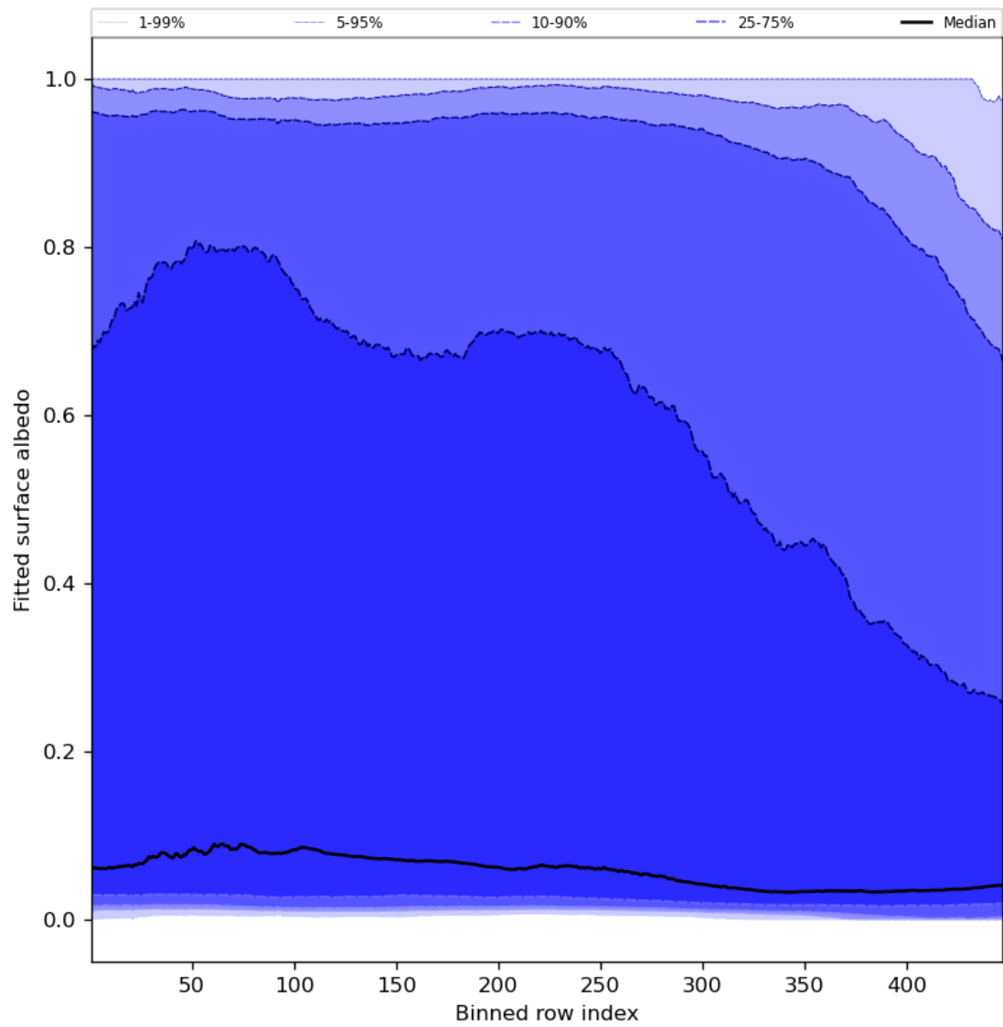
Figure 61: Along track statistics of “Fitted surface albedo” for 2023-12-14 to 2023-12-15
