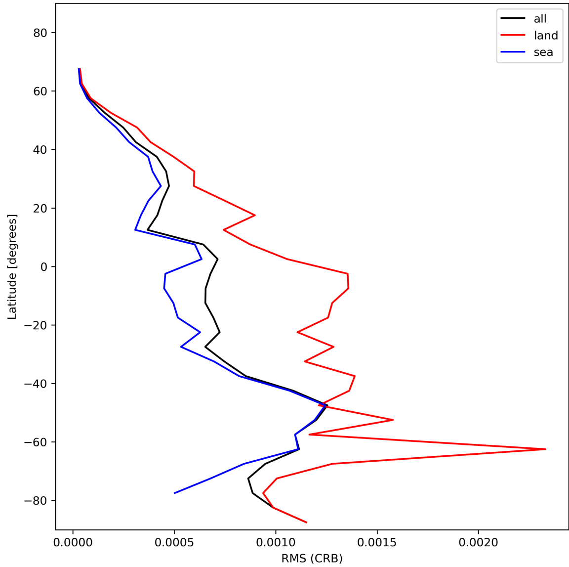
Figure 32: Zonal average of “RMS (CRB)” for 2023-12-14 to 2023-12-15.
