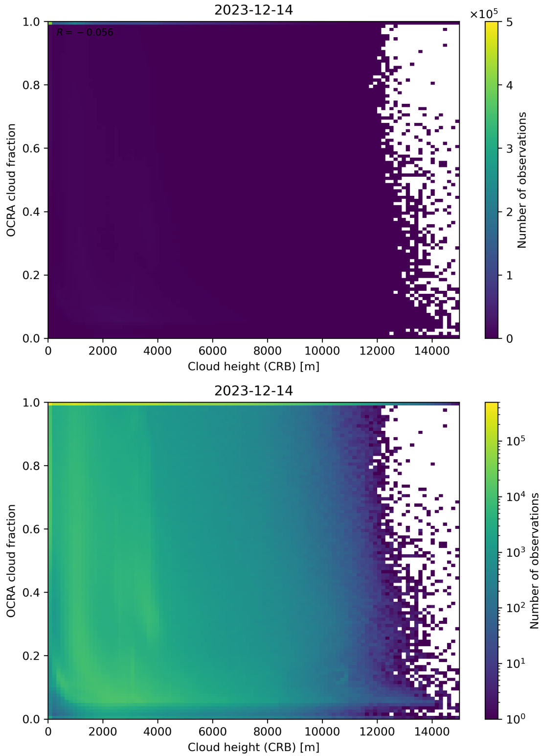
Figure 81: Scatter density plot of “Cloud height (CRB)” against “OCRA cloud fraction” for 2023-12-14 to 2023-12-15.
