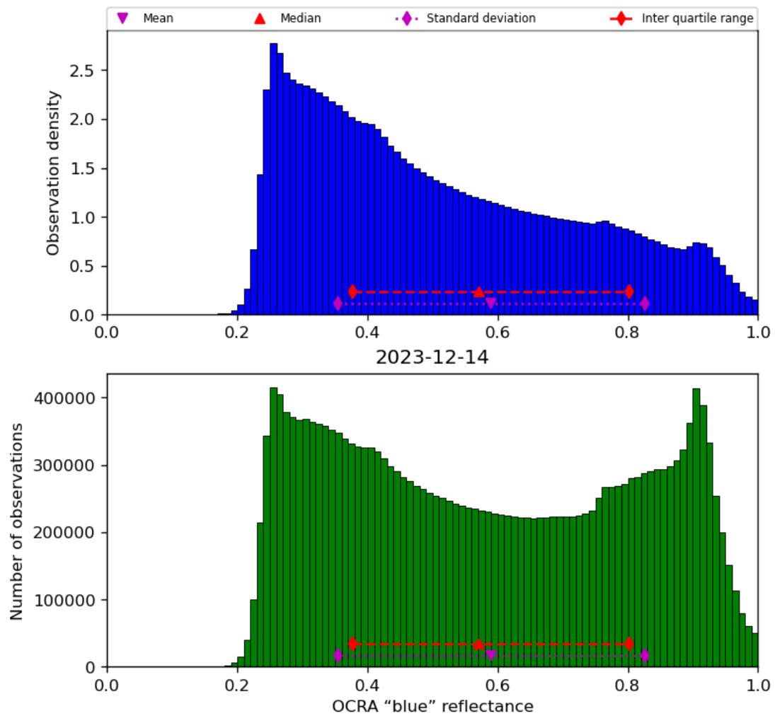
Figure 51: Histogram of “OCRA “blue” reflectance” for 2023-12-14 to 2023-12-15
