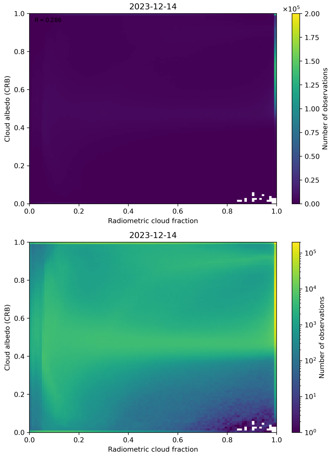
Figure 71: Scatter density plot of “Radiometric cloud fraction” against “Cloud albedo (CRB)” for 2023-12-14 to 2023-12-15.
