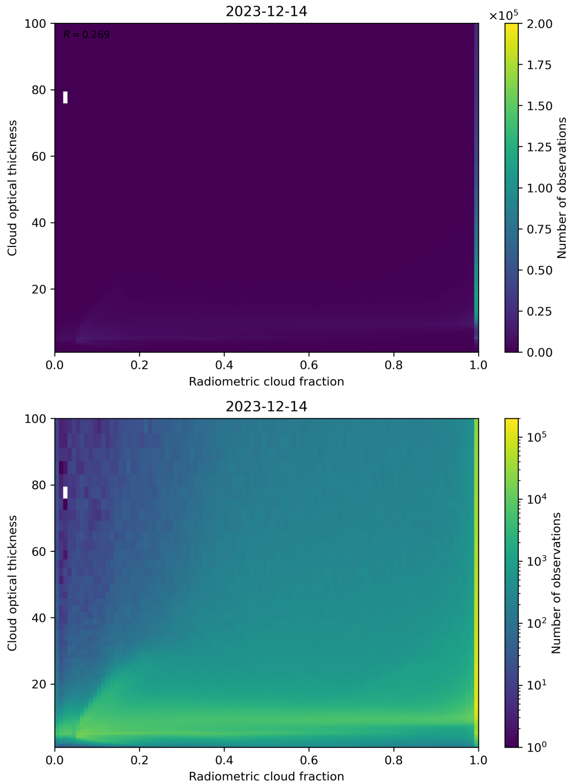
Figure 75: Scatter density plot of “Radiometric cloud fraction” against “Cloud optical thickness” for 2023-12-14 to 2023-12-15.
