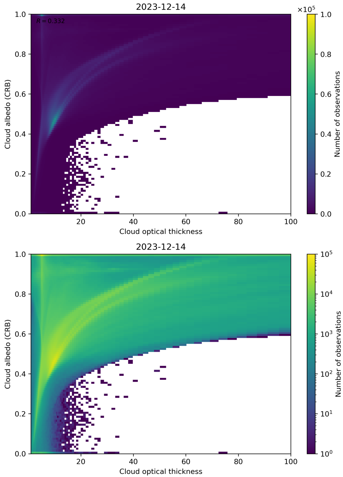
Figure 82: Scatter density plot of “Cloud optical thickness” against “Cloud albedo (CRB)” for 2023-12-14 to 2023-12-15.
