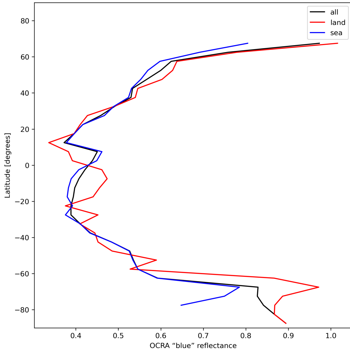
Figure 35: Zonal average of “OCRA “blue” reflectance” for 2023-12-14 to 2023-12-15.
