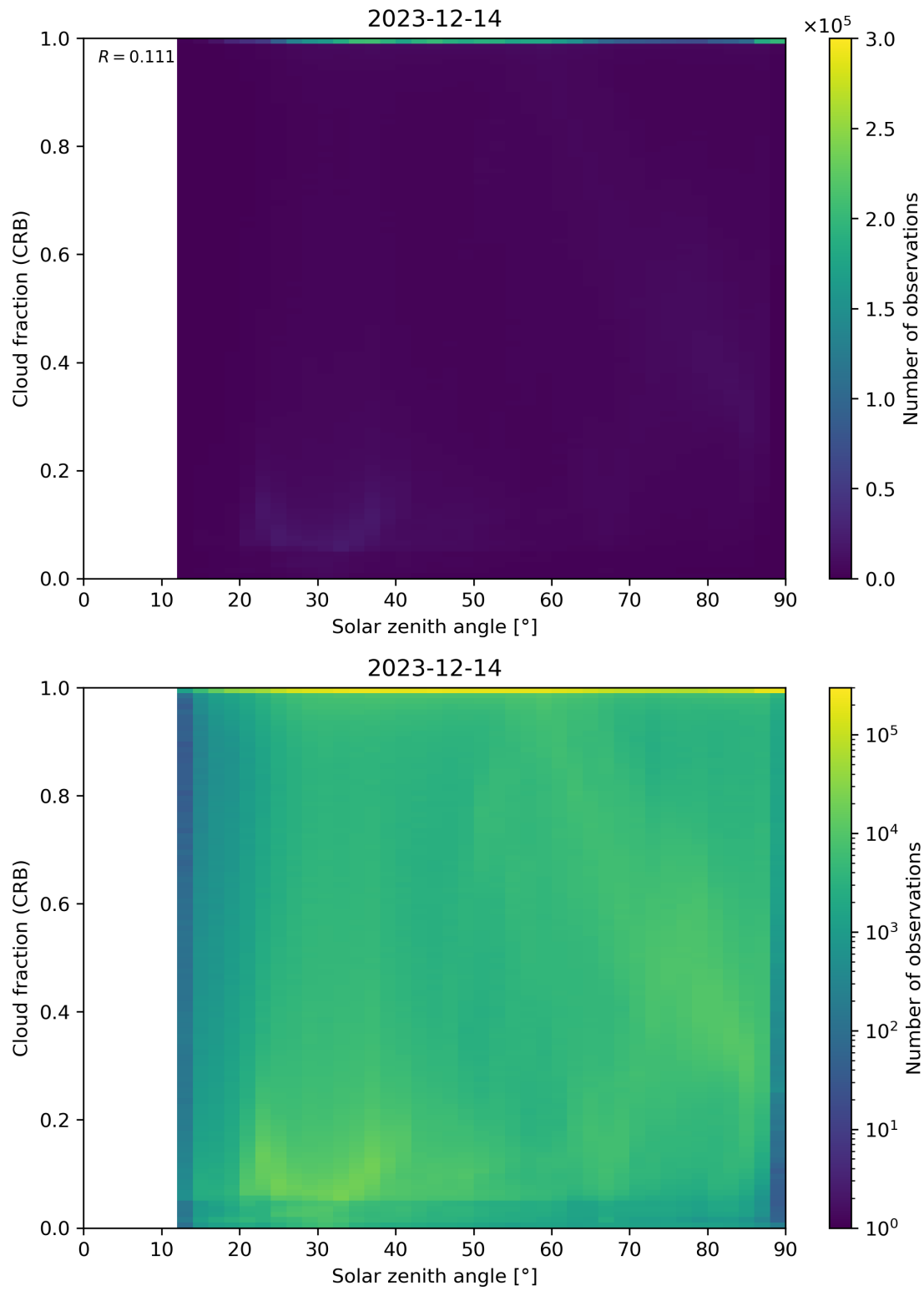
Figure 101: Scatter density plot of “Solar zenith angle” against “Cloud fraction (CRB)” for 2023-12-14 to 2023-12-15.
