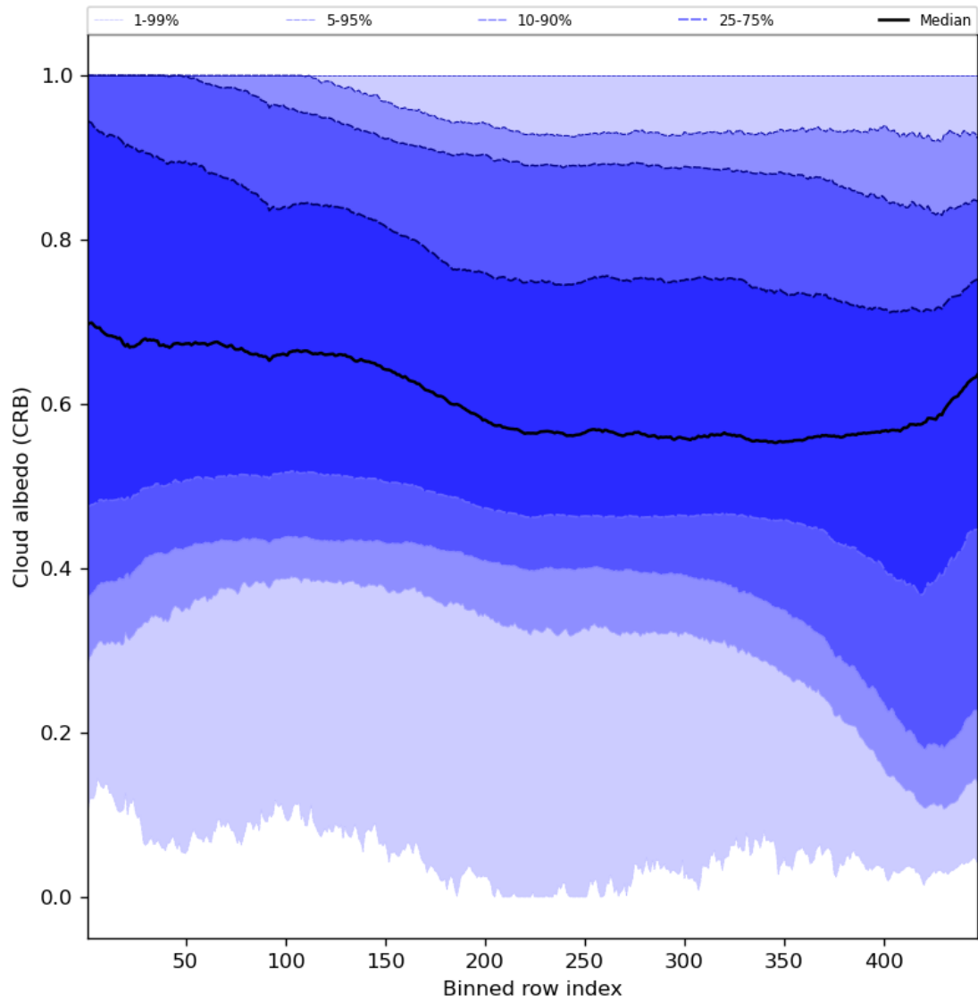
Figure 60: Along track statistics of “Cloud albedo (CRB)” for 2023-12-14 to 2023-12-15
