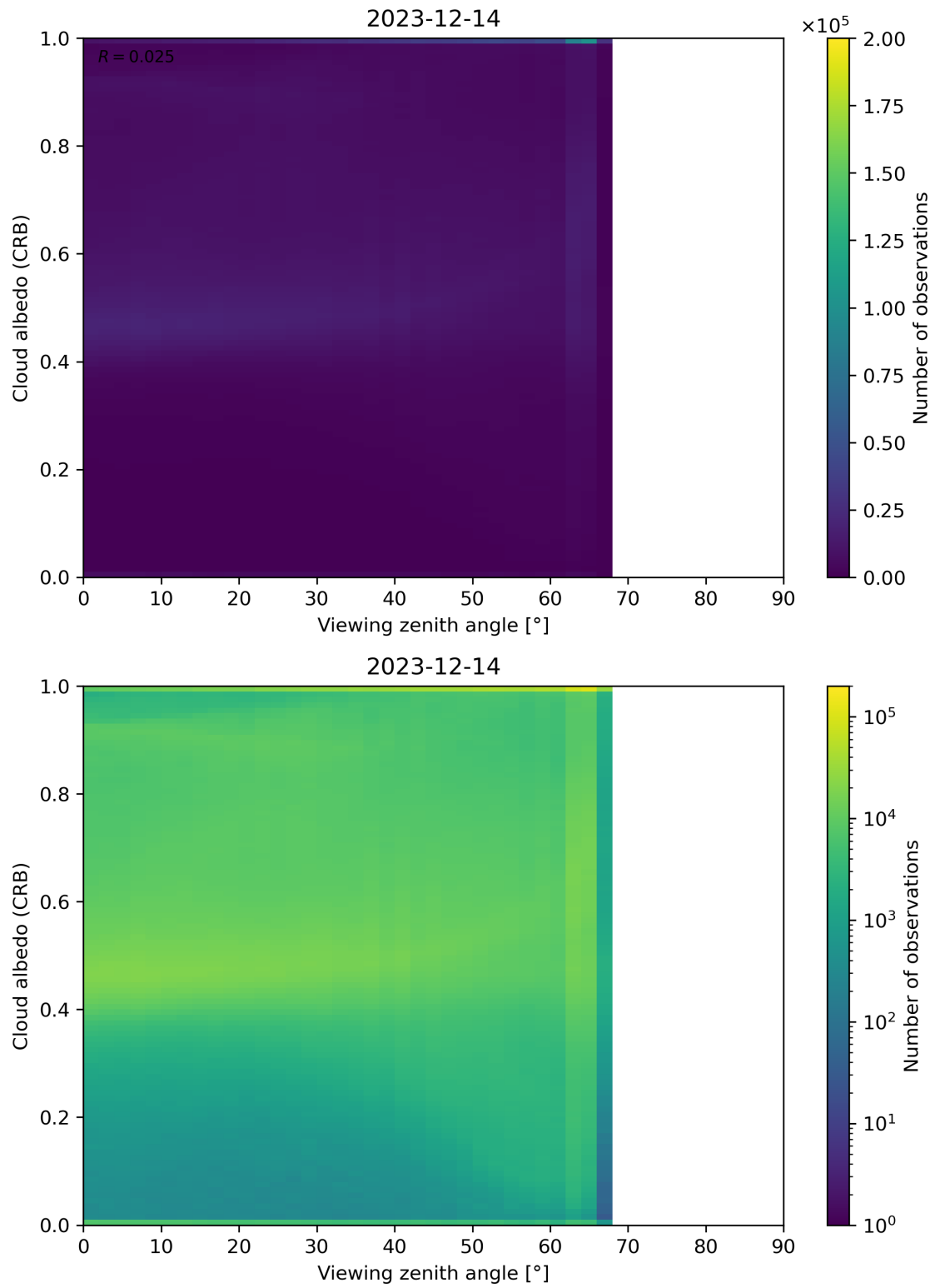
Figure 106: Scatter density plot of “Viewing zenith angle” against “Cloud albedo (CRB)” for 2023-12-14 to 2023-12-15.
