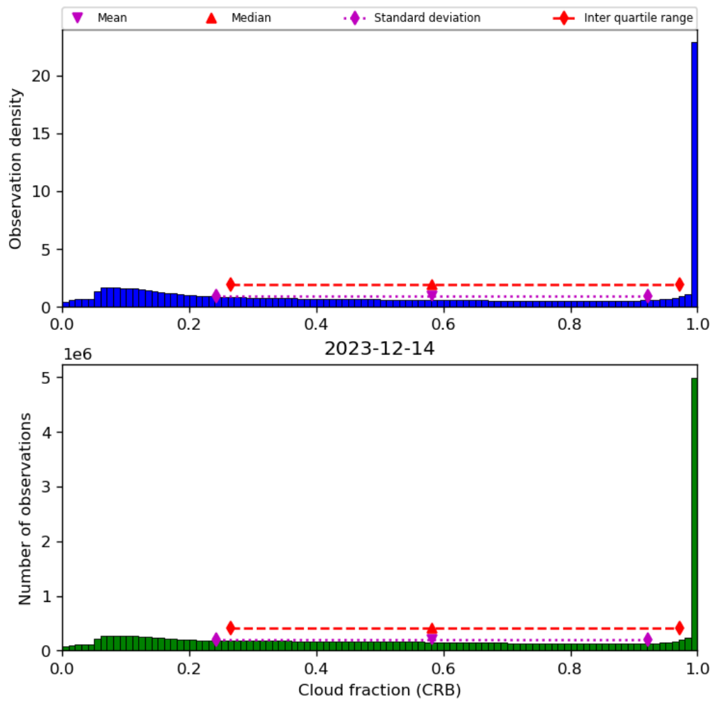
Figure 42: Histogram of “Cloud fraction (CRB)” for 2023-12-14 to 2023-12-15
