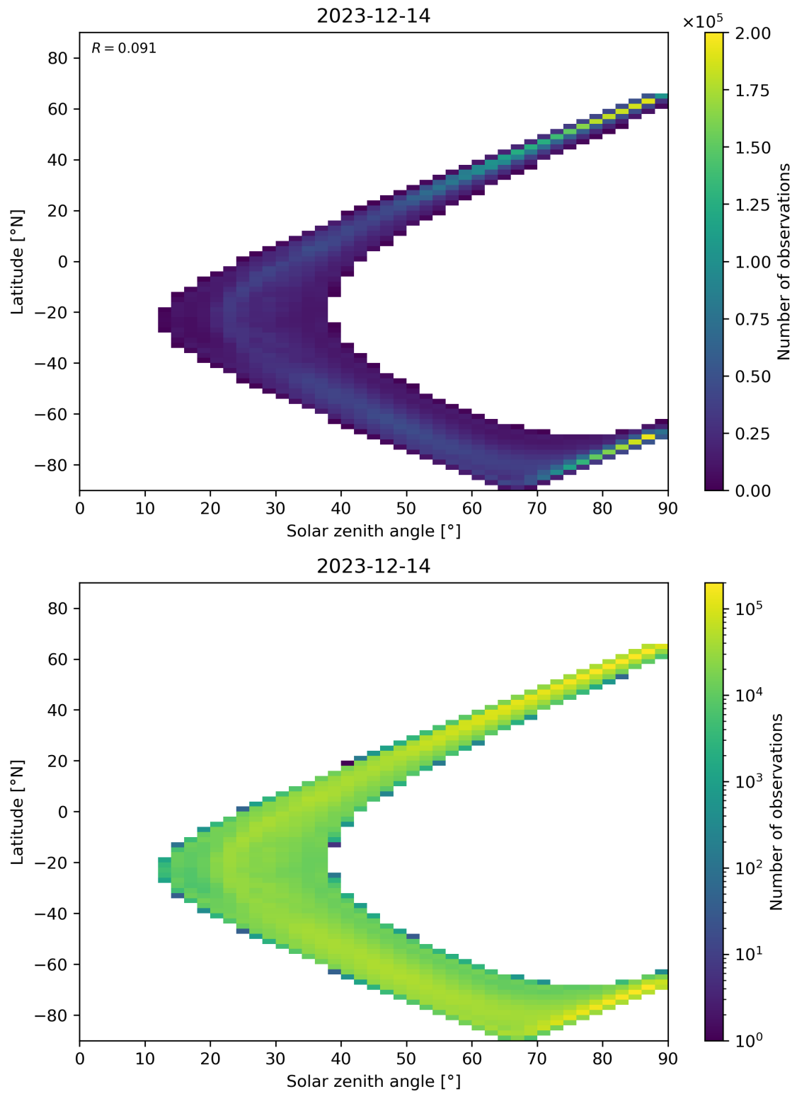
Figure 105: Scatter density plot of “Solar zenith angle” against “Latitude” for 2023-12-14 to 2023-12-15.
