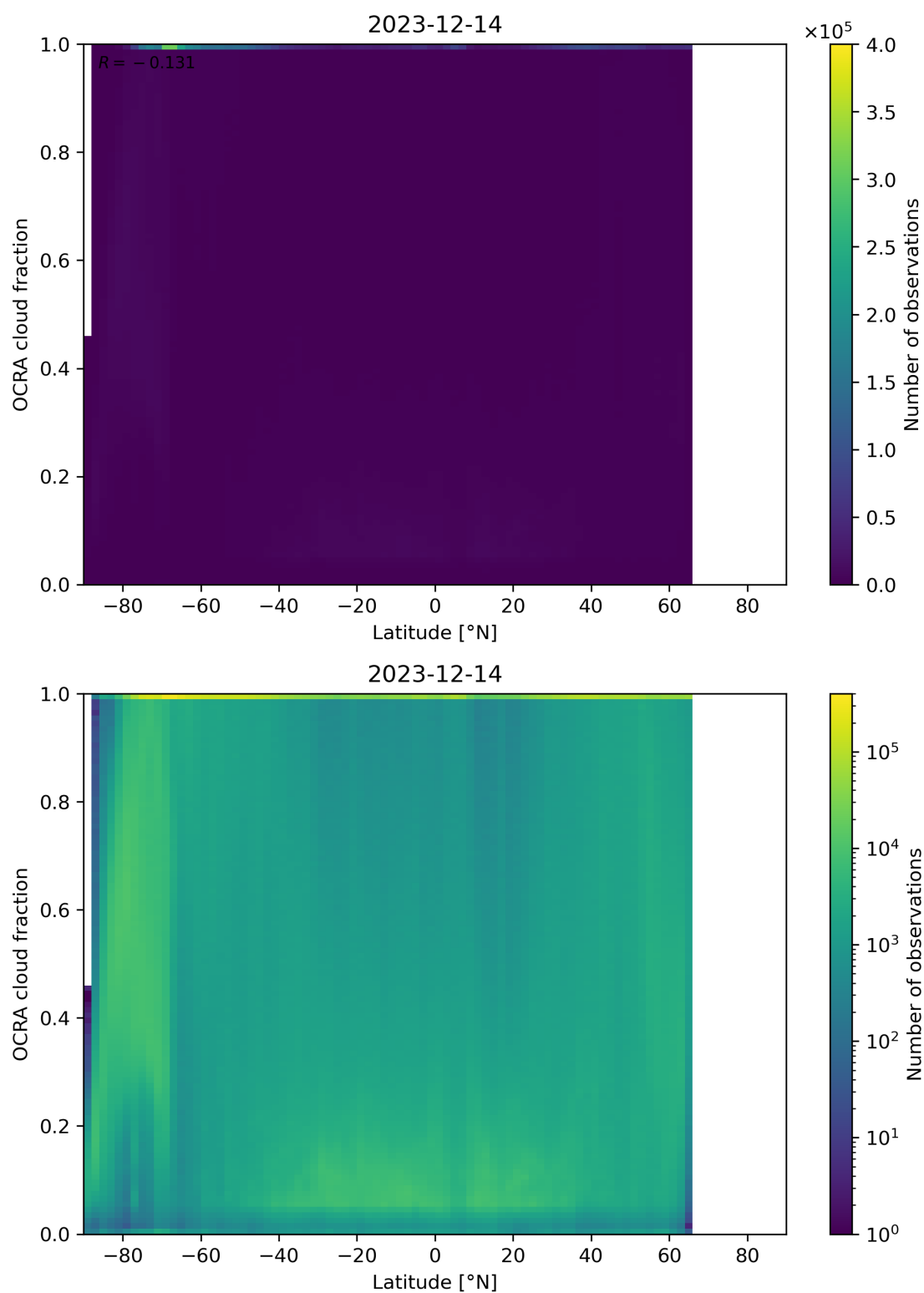
Figure 93: Scatter density plot of “Latitude” against “OCRA cloud fraction” for 2023-12-14 to 2023-12-15.
