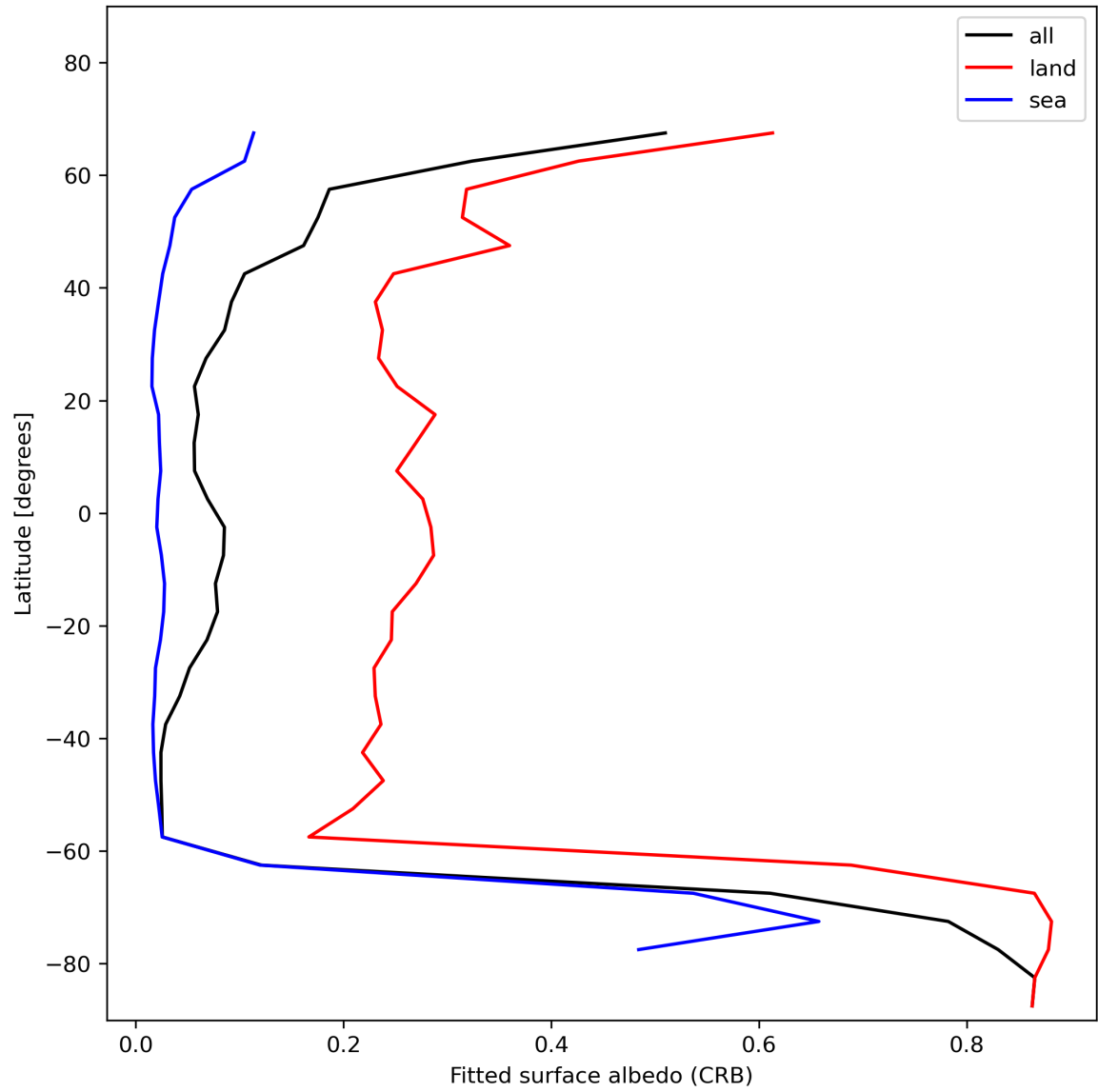
Figure 30: Zonal average of “Fitted surface albedo (CRB)” for 2023-12-14 to 2023-12-15.
