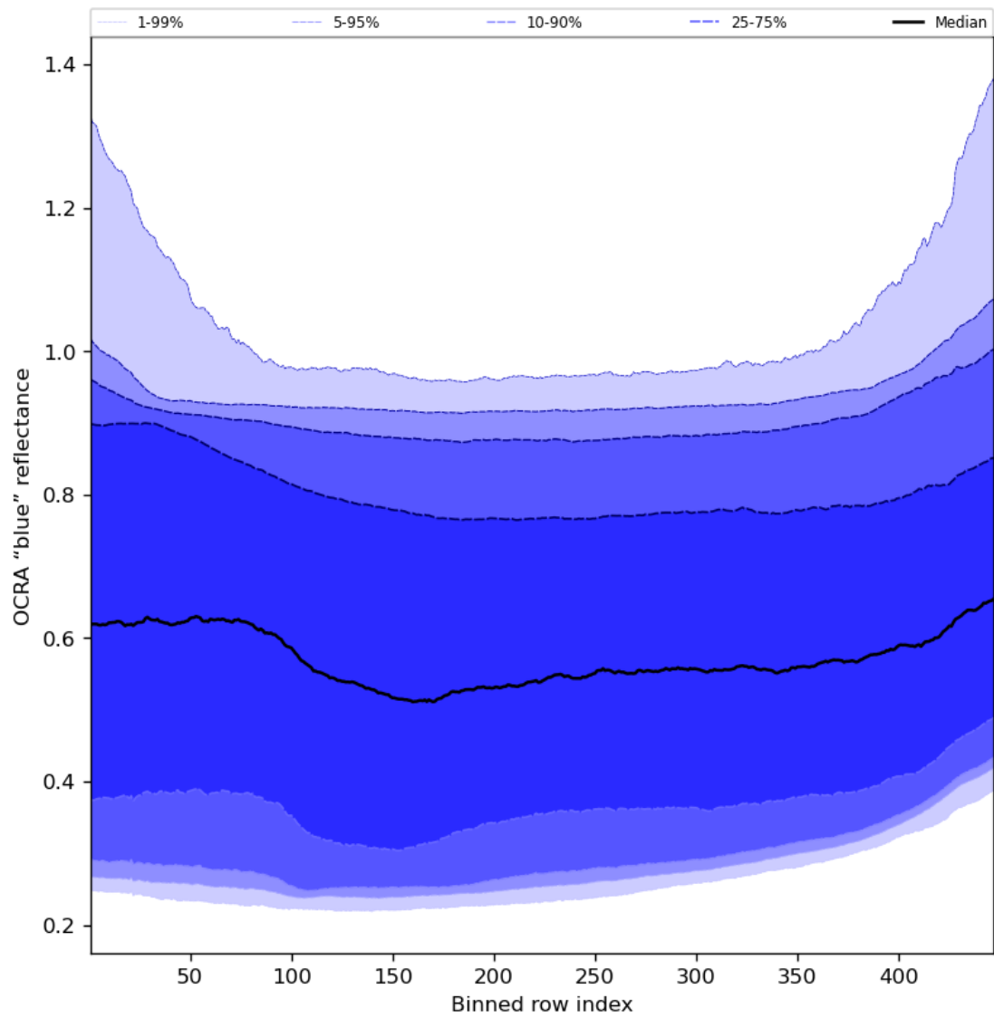
Figure 67: Along track statistics of “OCRA “blue” reflectance” for 2023-12-14 to 2023-12-15
