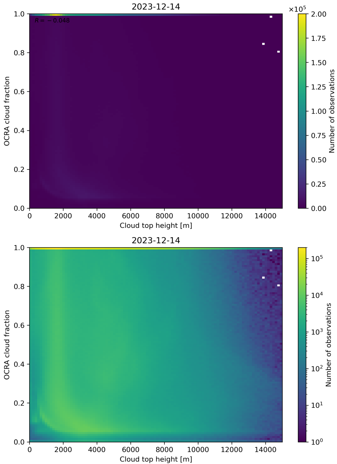
Figure 87: Scatter density plot of “Cloud top height” against “OCRA cloud fraction” for 2023-12-14 to 2023-12-15.
