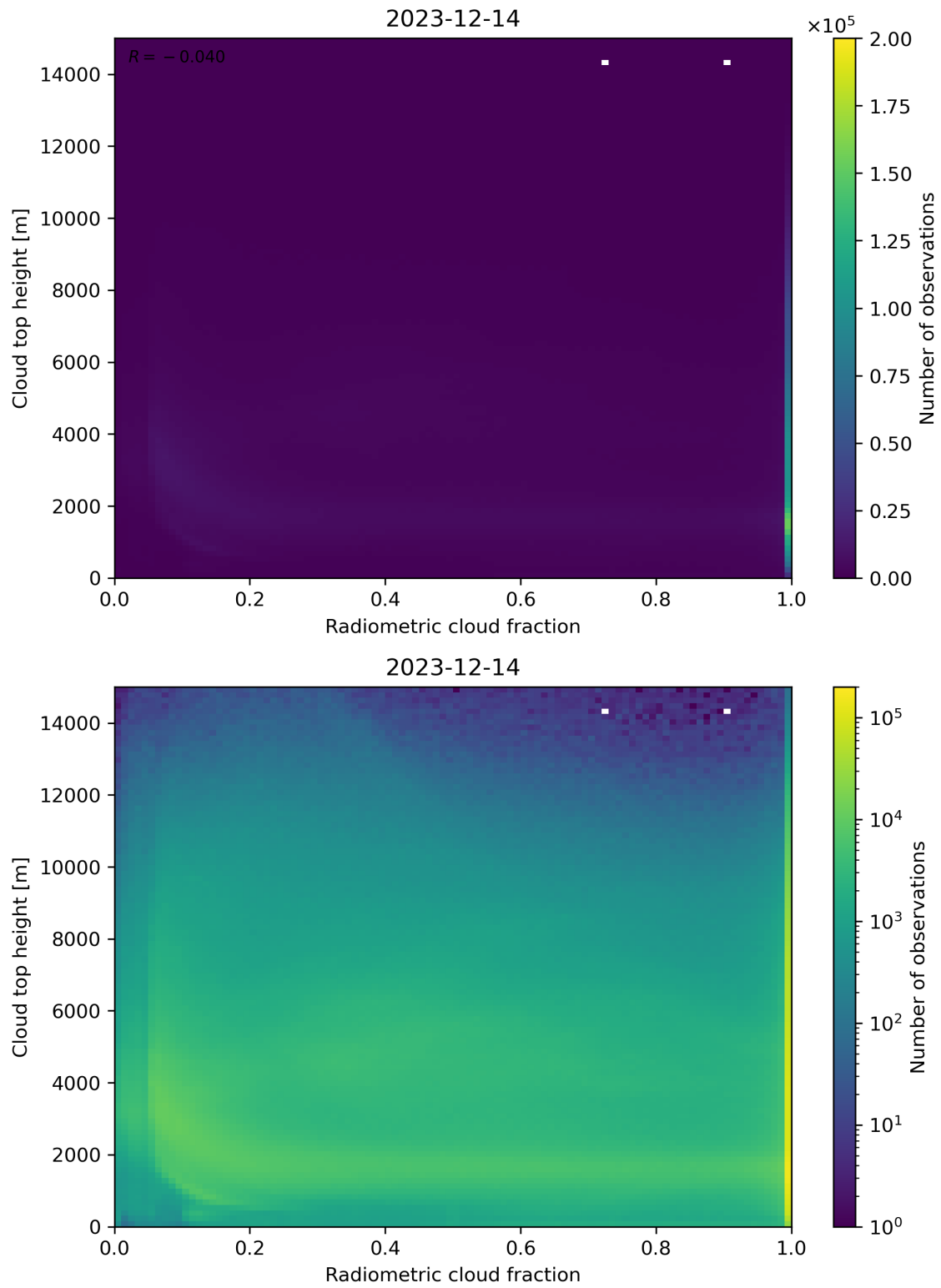
Figure 76: Scatter density plot of “Radiometric cloud fraction” against “Cloud top height” for 2023-12-14 to 2023-12-15.
