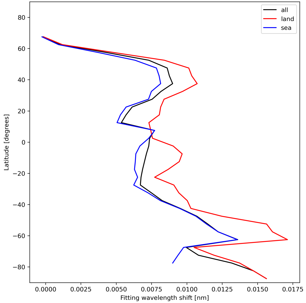
Figure 33: Zonal average of “Fitting wavelength shift” for 2023-12-14 to 2023-12-15.
