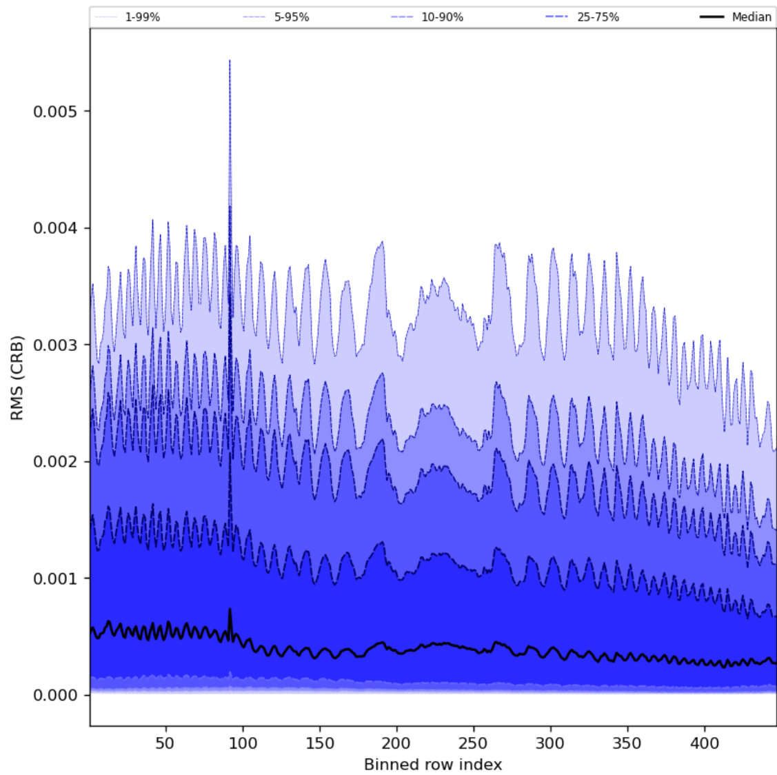
Figure 64: Along track statistics of “RMS (CRB)” for 2023-12-14 to 2023-12-15
