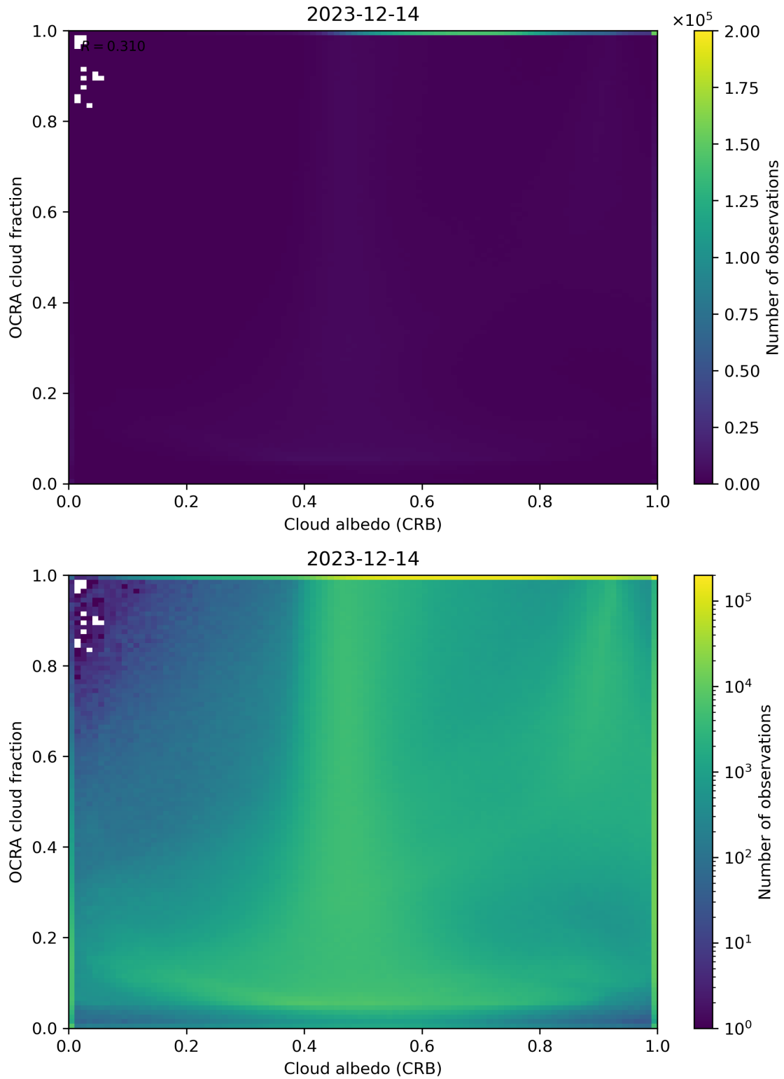
Figure 70: Scatter density plot of “Cloud albedo (CRB)” against “OCRA cloud fraction” for 2023-12-14 to 2023-12-15.
