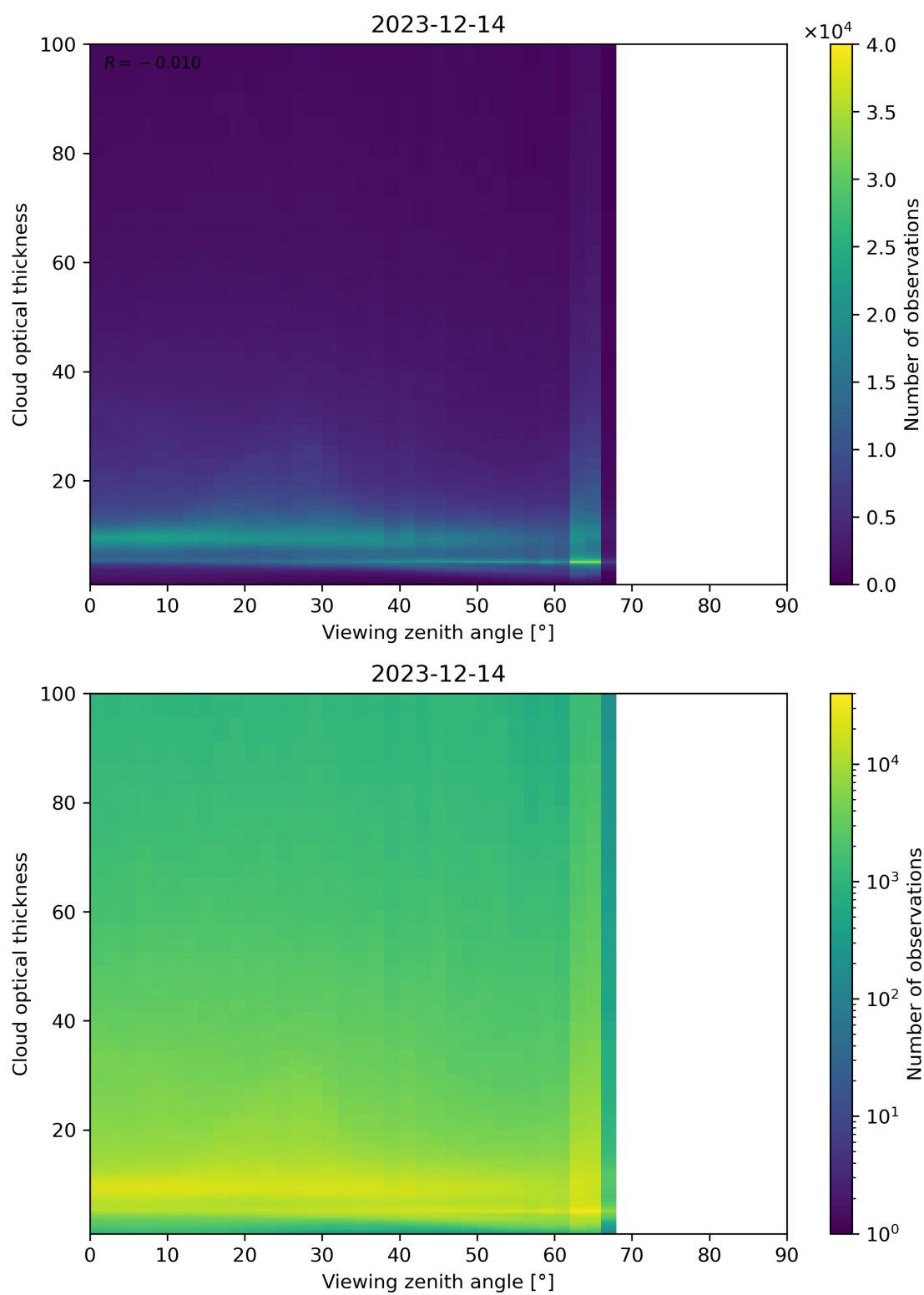
Figure 111: Scatter density plot of “Viewing zenith angle” against “Cloud optical thickness” for 2023-12-14 to 2023-12-15.
