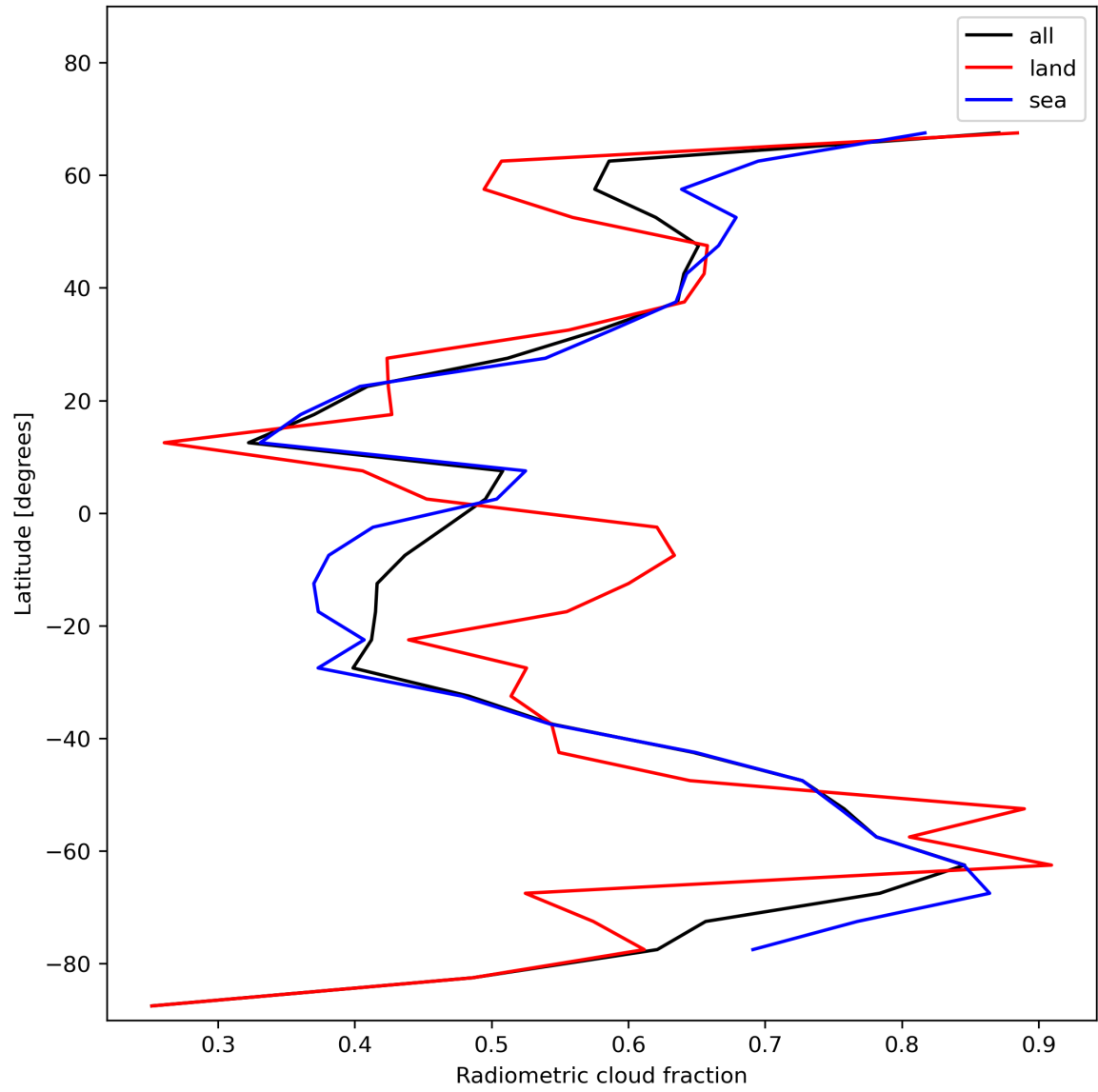
Figure 23: Zonal average of “Radiometric cloud fraction” for 2023-12-14 to 2023-12-15.
