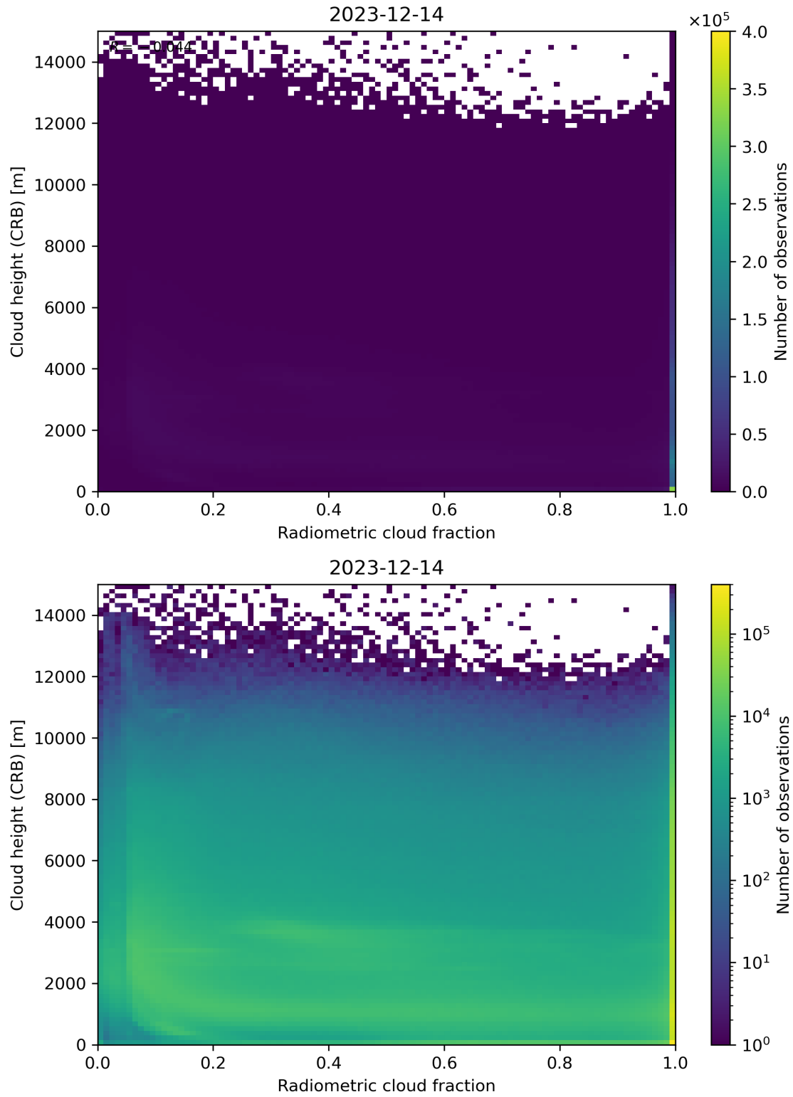
Figure 74: Scatter density plot of “Radiometric cloud fraction” against “Cloud height (CRB)” for 2023-12-14 to 2023-12-15.
