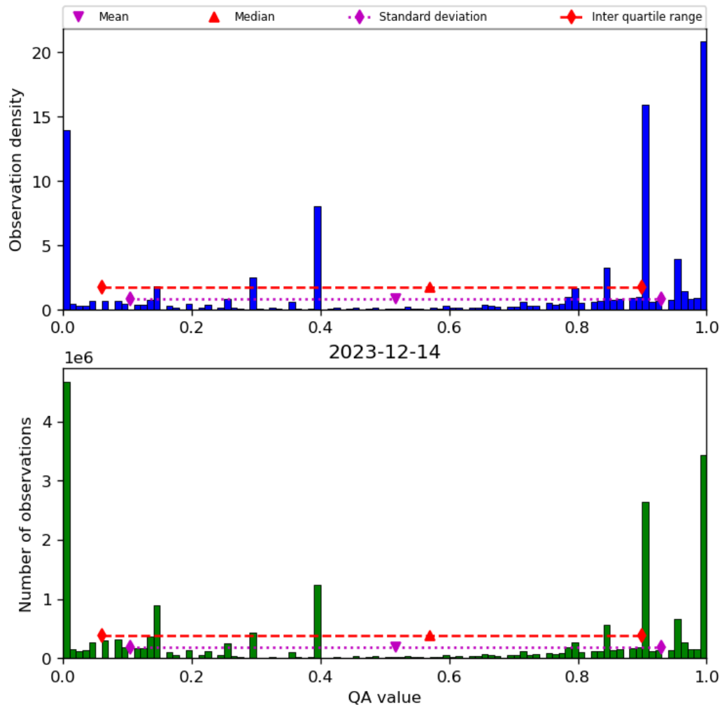
Figure 38: Histogram of “QA value” for 2023-12-14 to 2023-12-15
