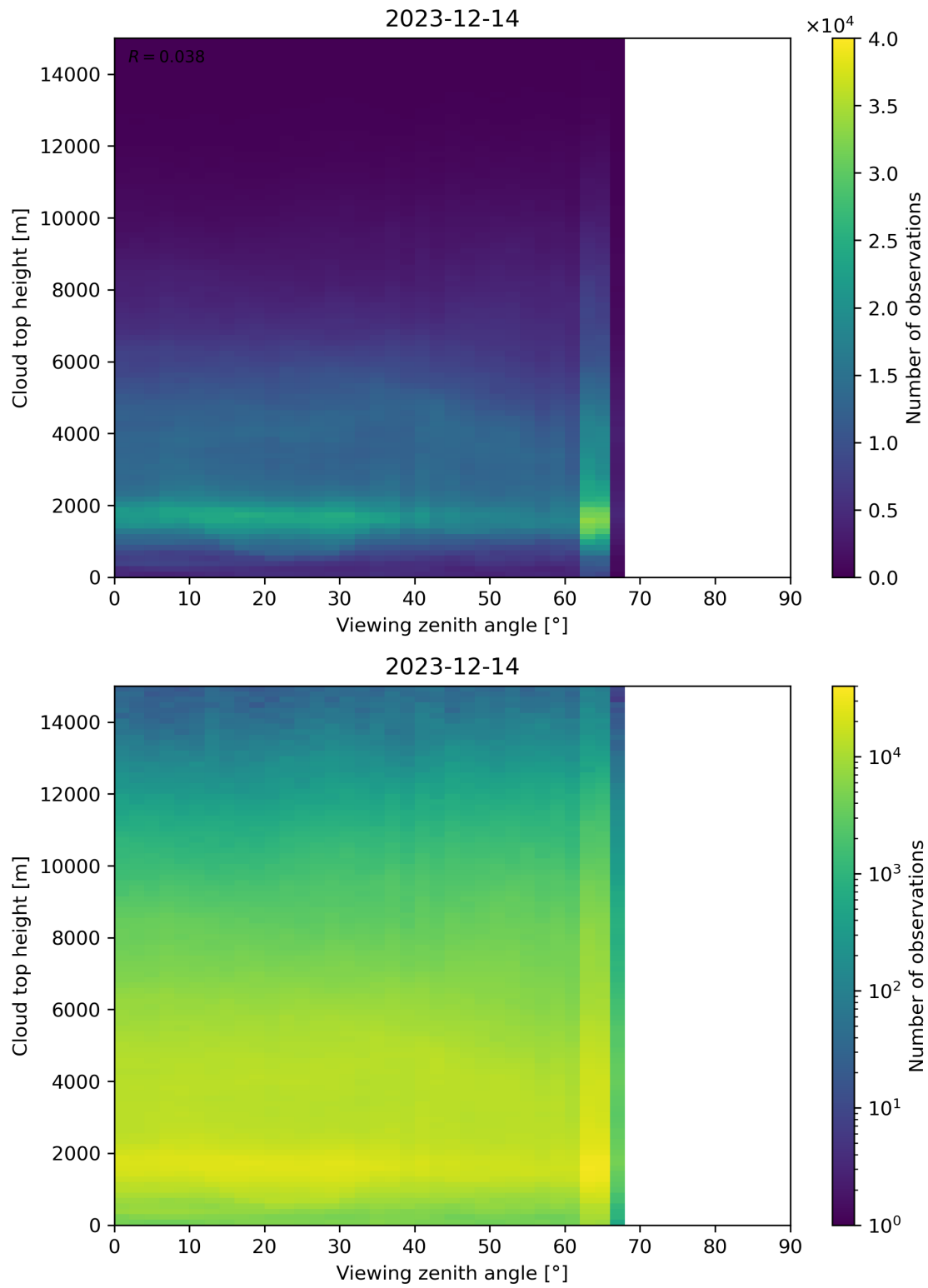
Figure 112: Scatter density plot of “Viewing zenith angle” against “Cloud top height” for 2023-12-14 to 2023-12-15.
