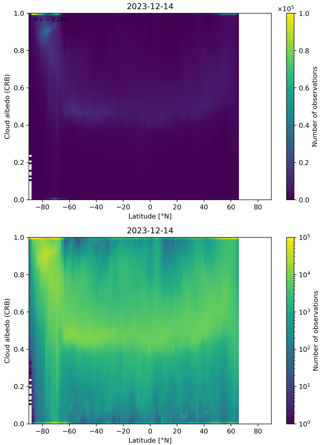
Figure 91: Scatter density plot of “Latitude” against “Cloud albedo (CRB)” for 2023-12-14 to 2023-12-15.
