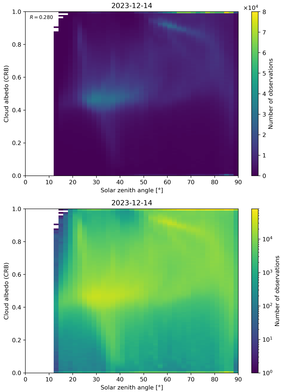
Figure 98: Scatter density plot of “Solar zenith angle” against “Cloud albedo (CRB)” for 2023-12-14 to 2023-12-15.
