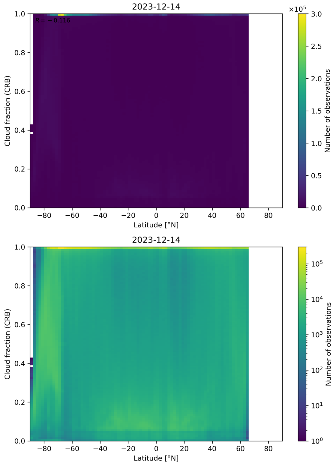
Figure 94: Scatter density plot of “Latitude” against “Cloud fraction (CRB)” for 2023-12-14 to 2023-12-15.
