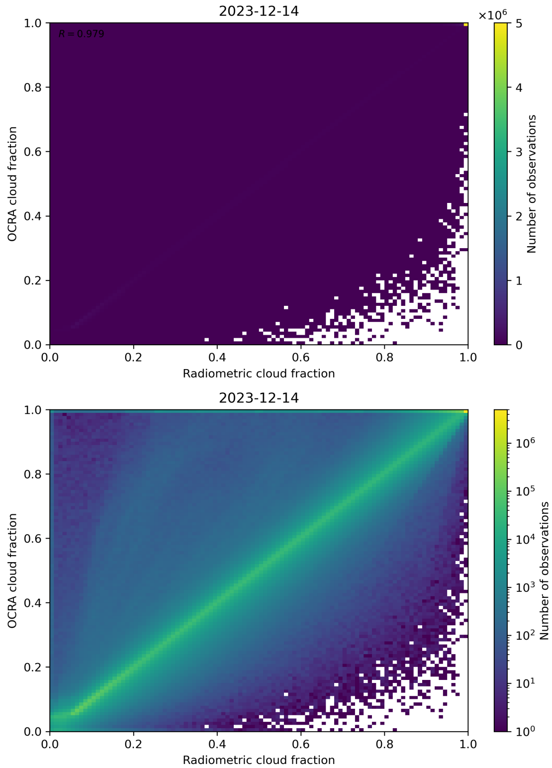
Figure 72: Scatter density plot of “Radiometric cloud fraction” against “OCRA cloud fraction” for 2023-12-14 to 2023-12-15.
