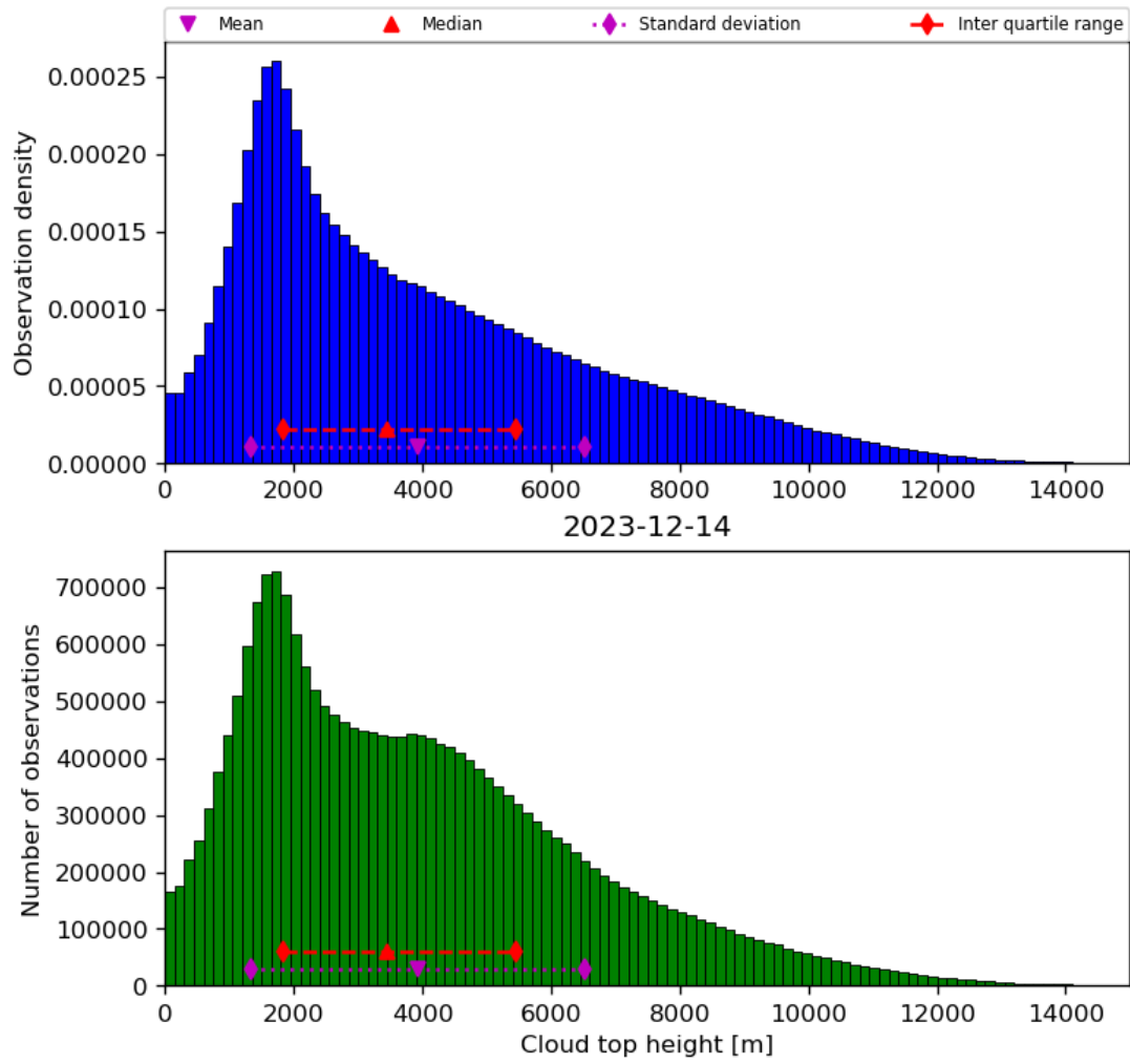
Figure 40: Histogram of “Cloud top height” for 2023-12-14 to 2023-12-15
