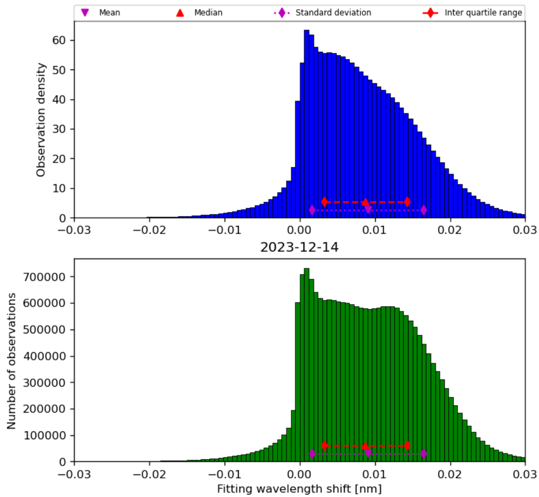
Figure 49: Histogram of “Fitting wavelength shift” for 2023-12-14 to 2023-12-15
