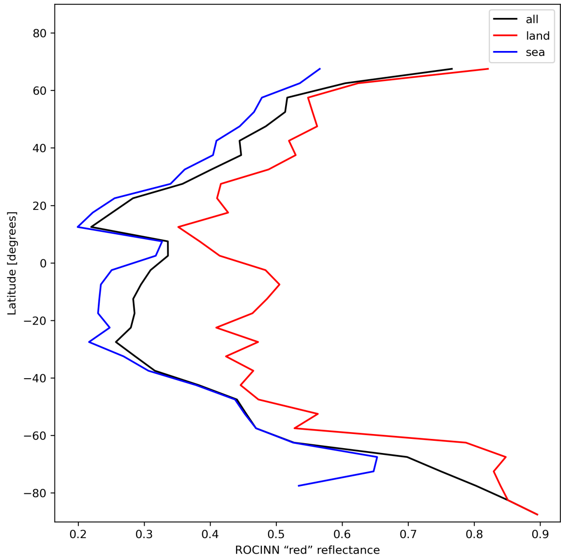
Figure 37: Zonal average of “ROCINN “red” reflectance” for 2023-12-14 to 2023-12-15.
