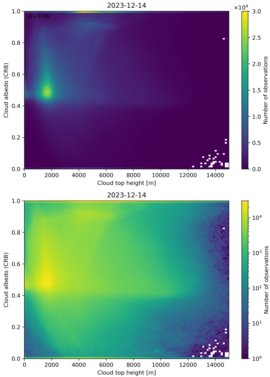
Figure 86: Scatter density plot of “Cloud top height” against “Cloud albedo (CRB)” for 2023-12-14 to 2023-12-15.
