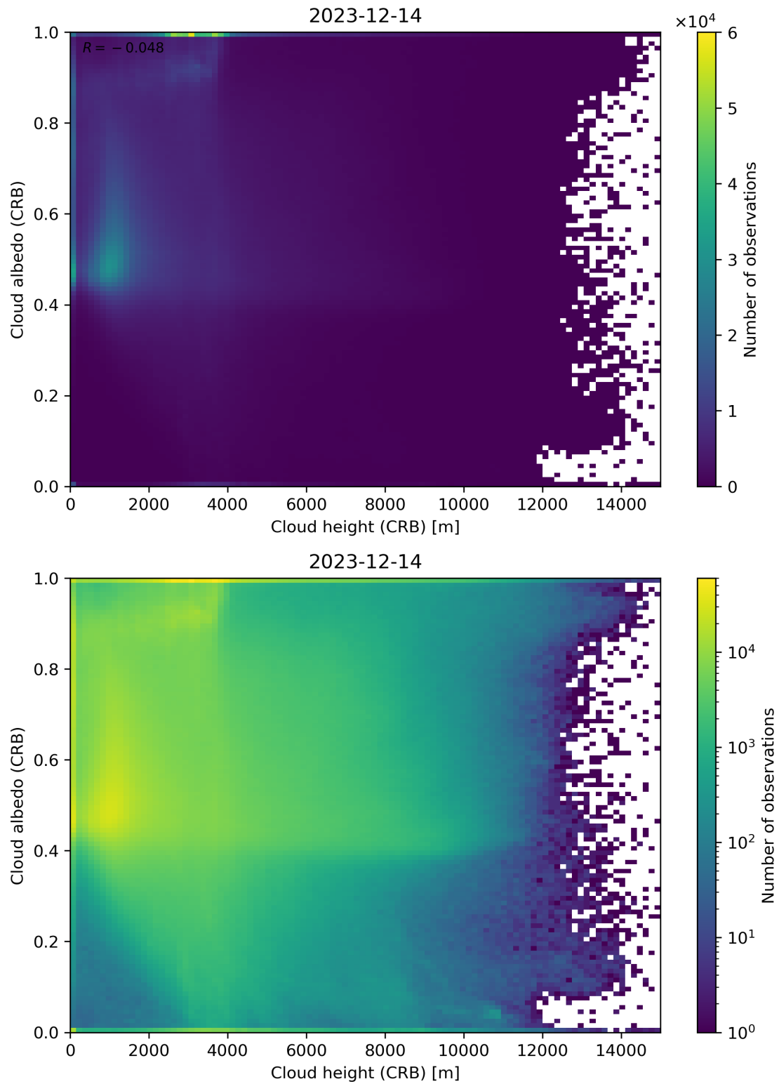
Figure 80: Scatter density plot of “Cloud height (CRB)” against “Cloud albedo (CRB)” for 2023-12-14 to 2023-12-15.
