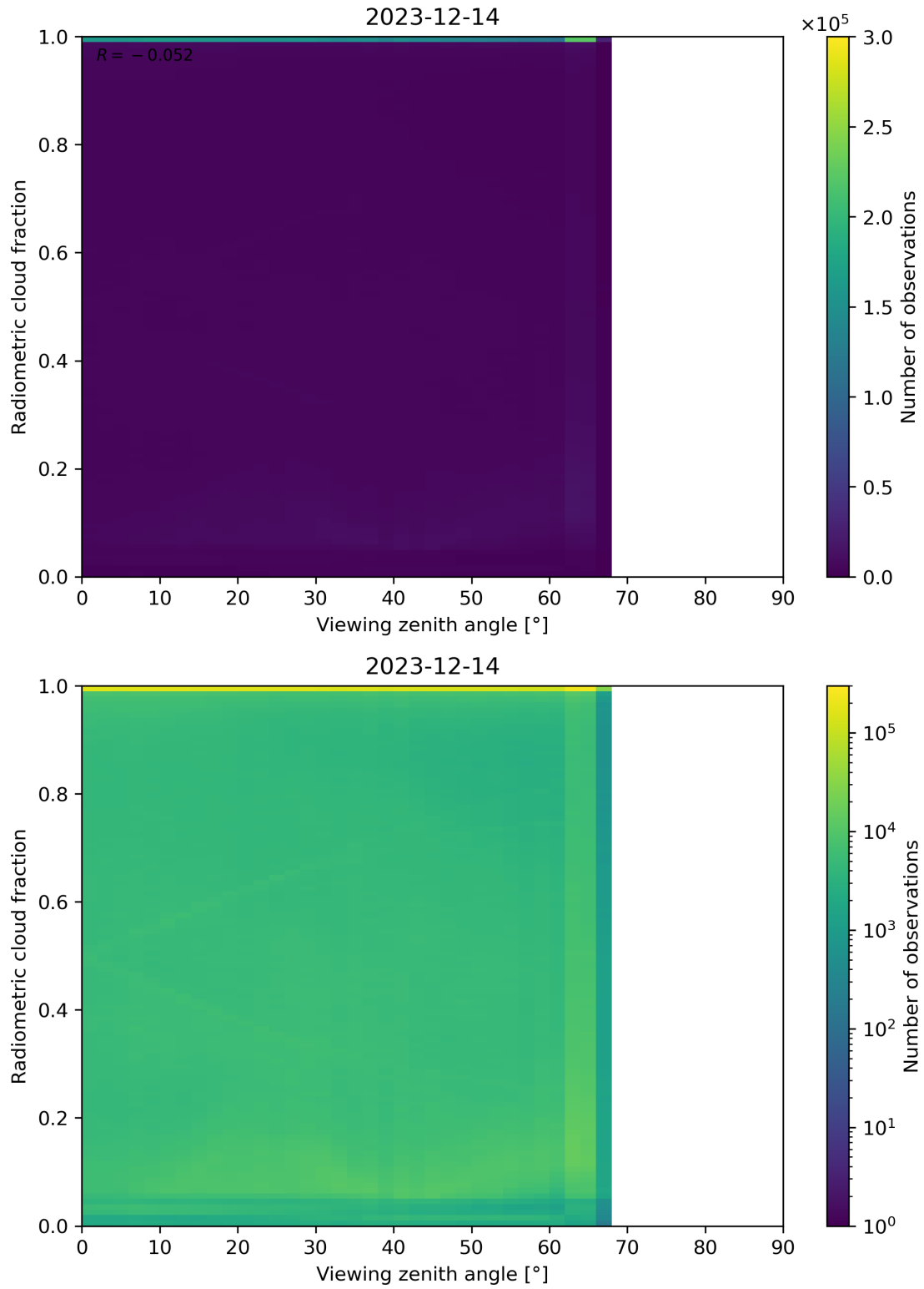
Figure 107: Scatter density plot of “Viewing zenith angle” against “Radiometric cloud fraction” for 2023-12-14 to 2023-12-15.
