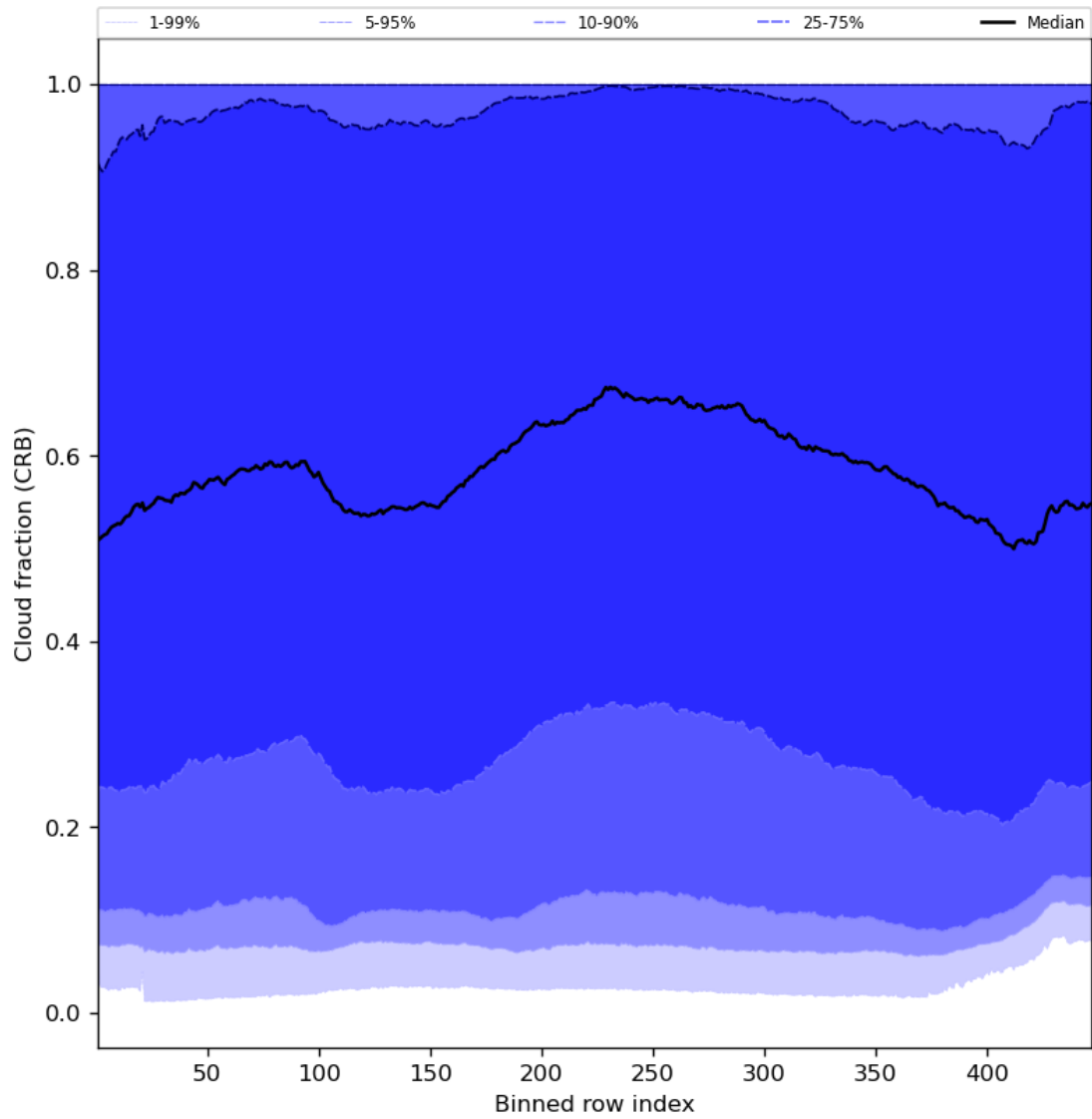
Figure 58: Along track statistics of “Cloud fraction (CRB)” for 2023-12-14 to 2023-12-15
