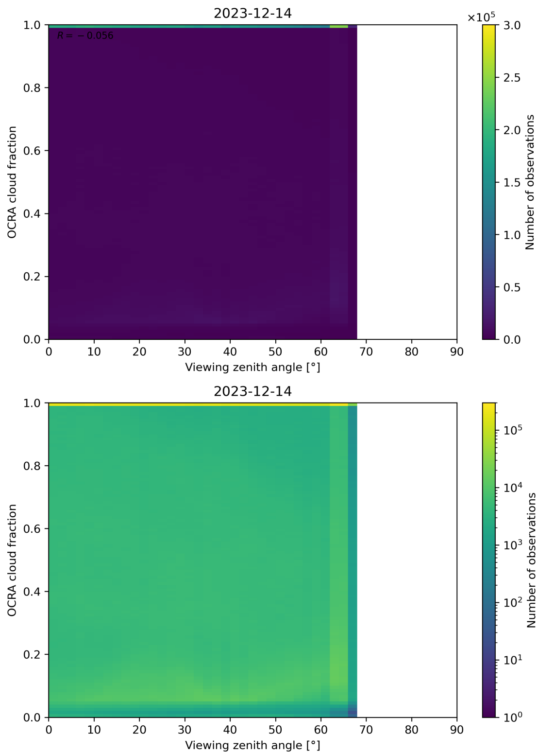
Figure 108: Scatter density plot of “Viewing zenith angle” against “OCRA cloud fraction” for 2023-12-14 to 2023-12-15.
