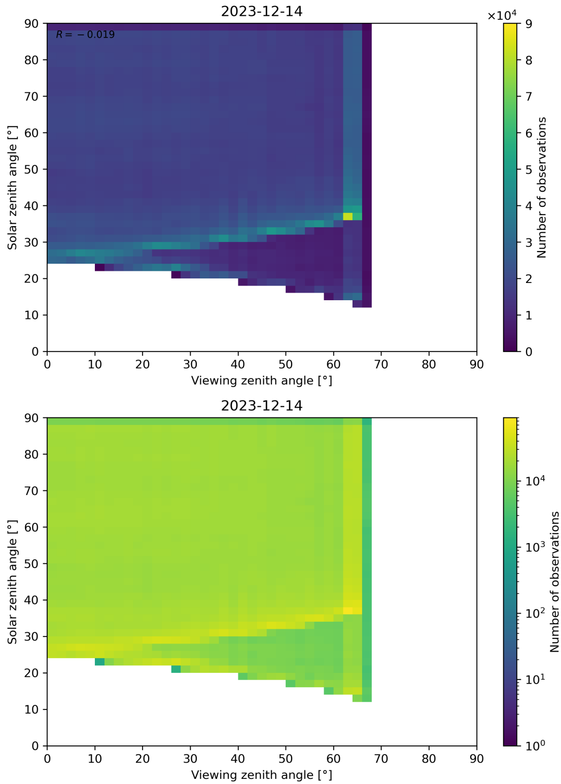
Figure 114: Scatter density plot of “Viewing zenith angle” against “Solar zenith angle” for 2023-12-14 to 2023-12-15.
