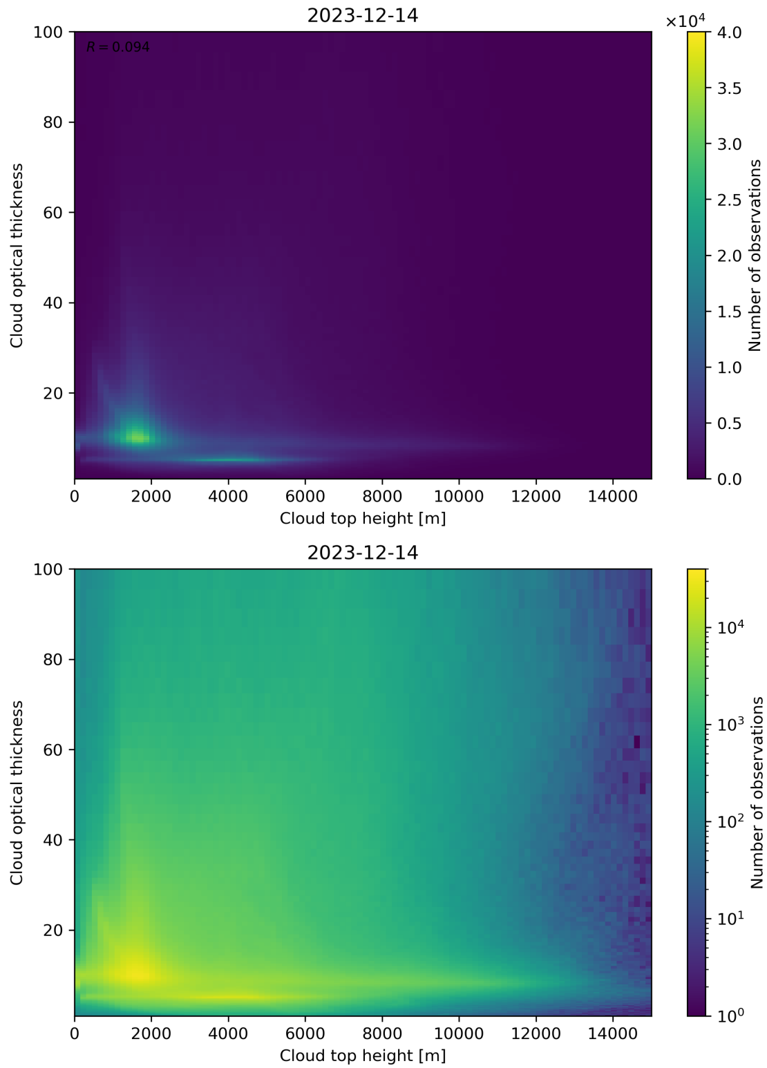
Figure 90: Scatter density plot of “Cloud top height” against “Cloud optical thickness” for 2023-12-14 to 2023-12-15.
