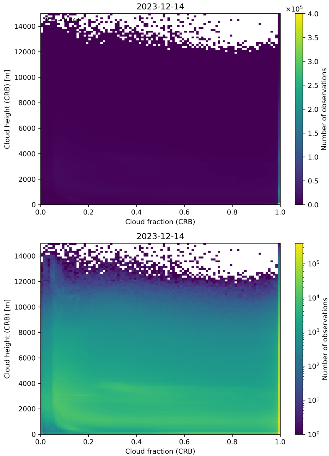
Figure 79: Scatter density plot of “Cloud fraction (CRB)” against “Cloud height (CRB)” for 2023-12-14 to 2023-12-15.
