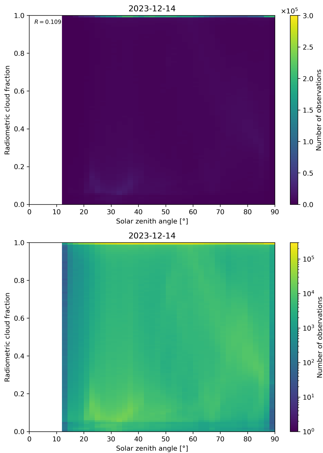
Figure 99: Scatter density plot of “Solar zenith angle” against “Radiometric cloud fraction” for 2023-12-14 to 2023-12-15.
