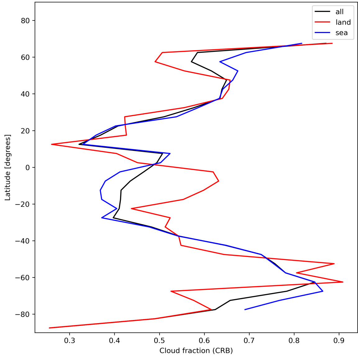
Figure 26: Zonal average of “Cloud fraction (CRB)” for 2023-12-14 to 2023-12-15.
