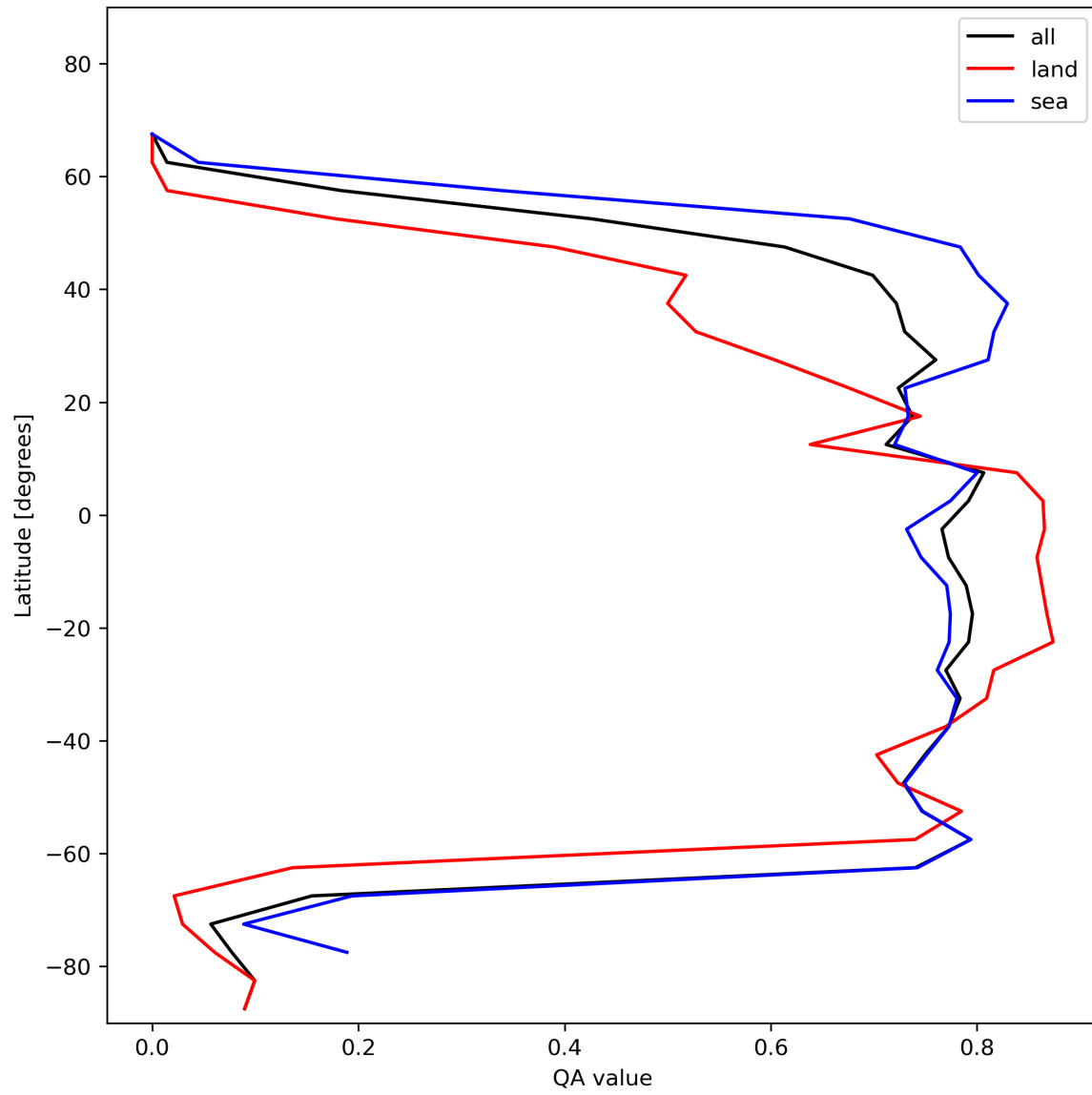
Figure 22: Zonal average of “QA value” for 2023-12-14 to 2023-12-15.
