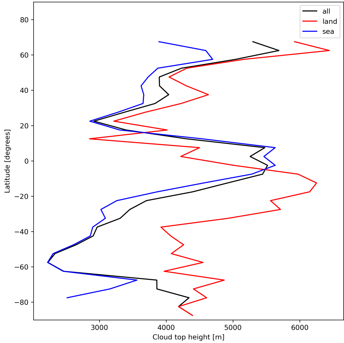
Figure 24: Zonal average of “Cloud top height” for 2023-12-14 to 2023-12-15.
