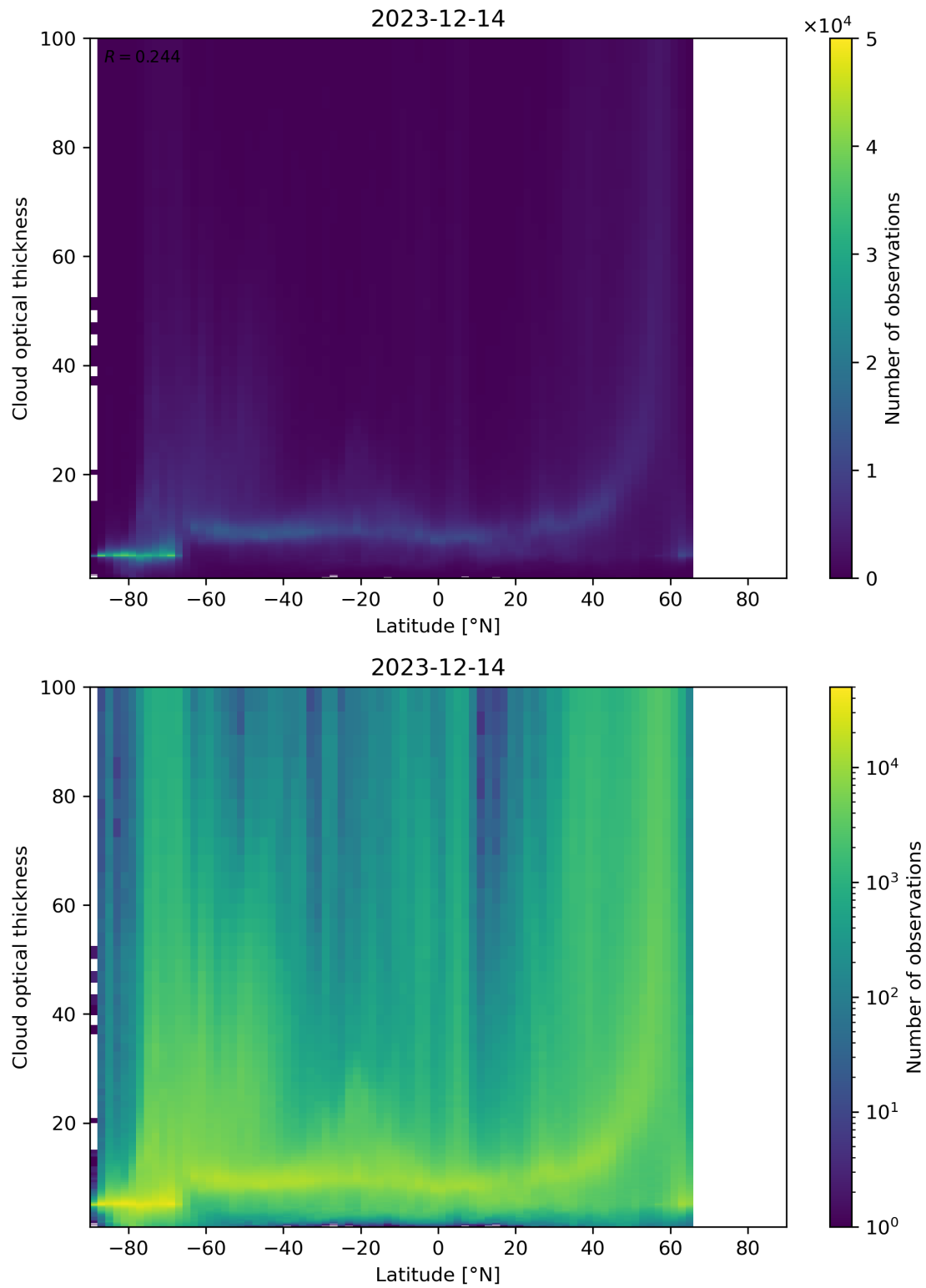
Figure 96: Scatter density plot of “Latitude” against “Cloud optical thickness” for 2023-12-14 to 2023-12-15.
