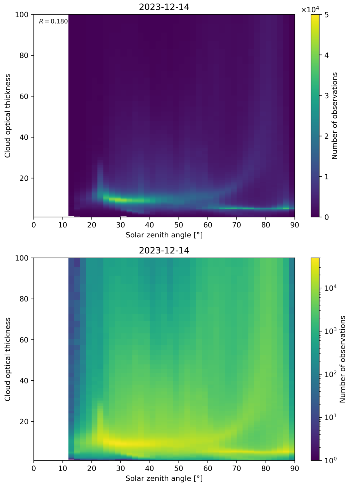
Figure 103: Scatter density plot of “Solar zenith angle” against “Cloud optical thickness” for 2023-12-14 to 2023-12-15.
