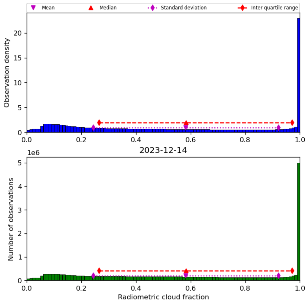
Figure 39: Histogram of “Radiometric cloud fraction” for 2023-12-14 to 2023-12-15
