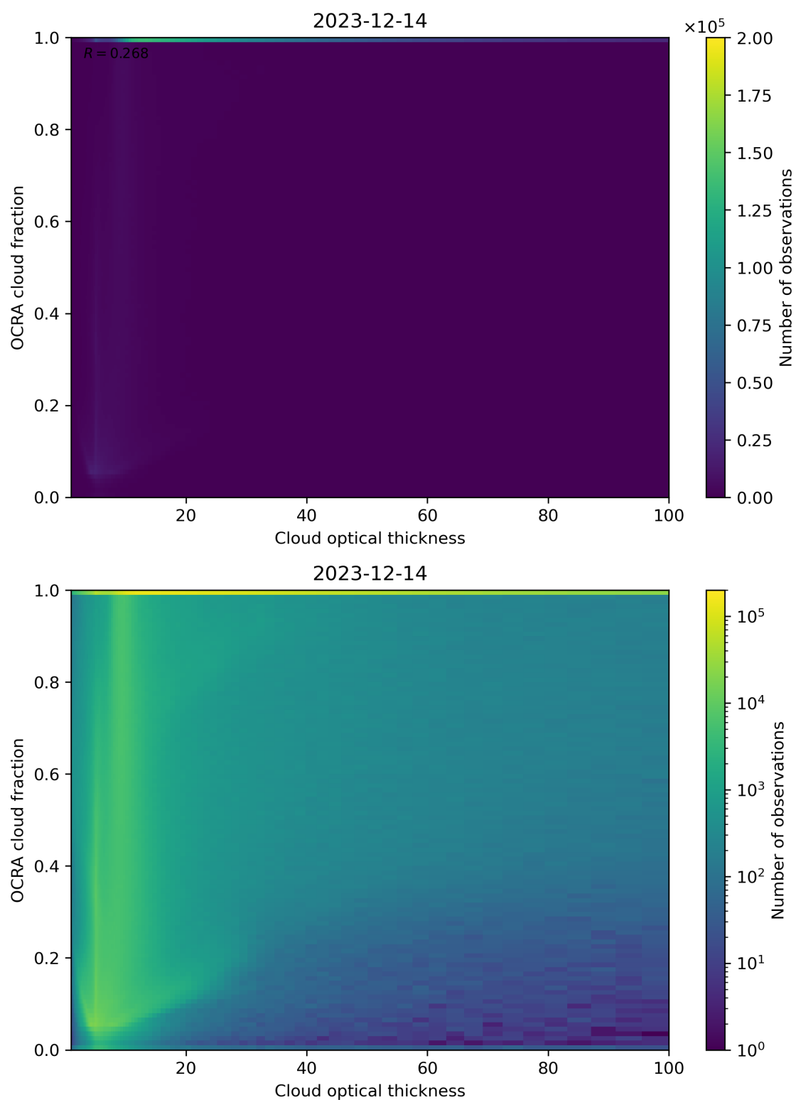
Figure 83: Scatter density plot of “Cloud optical thickness” against “OCRA cloud fraction” for 2023-12-14 to 2023-12-15.
