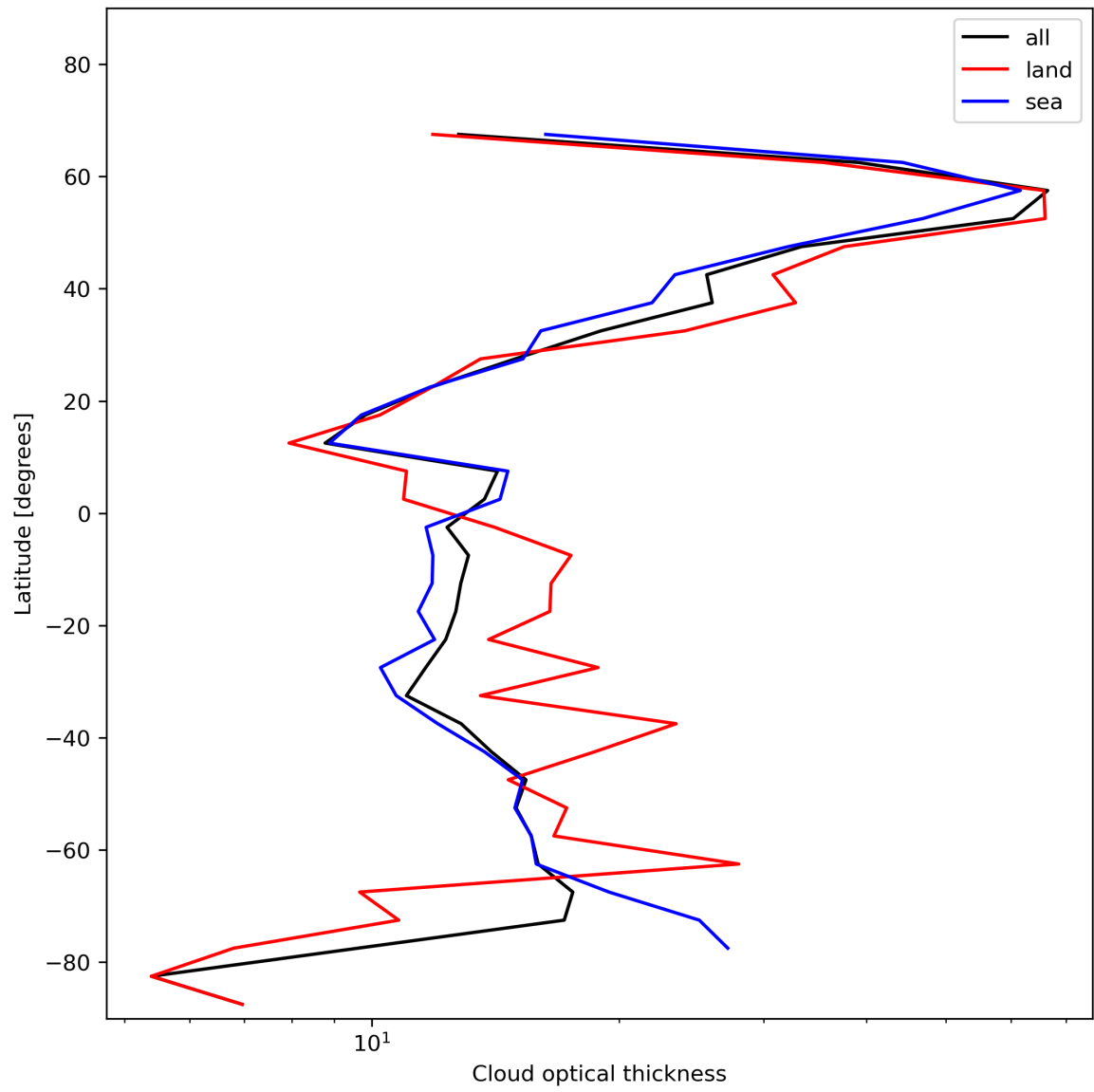
Figure 25: Zonal average of “Cloud optical thickness” for 2023-12-14 to 2023-12-15.
