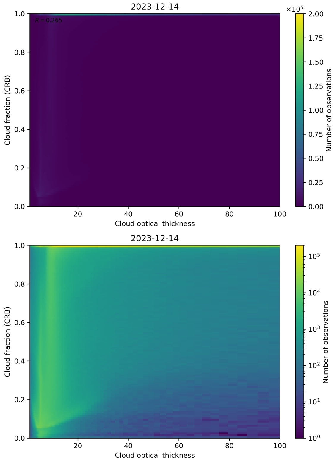
Figure 84: Scatter density plot of “Cloud optical thickness” against “Cloud fraction (CRB)” for 2023-12-14 to 2023-12-15.
