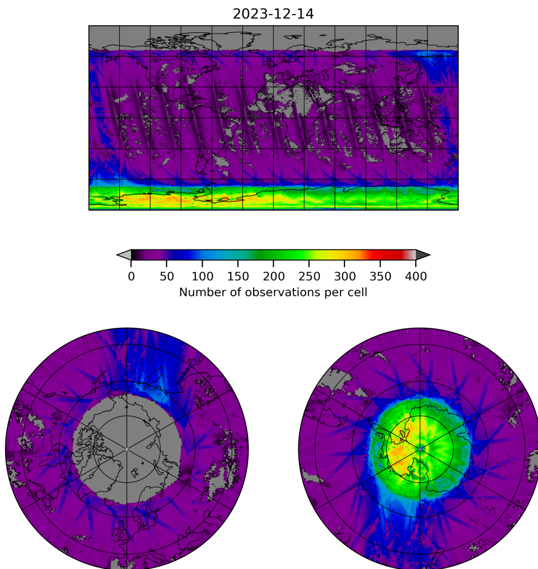
Figure 21: Map of the number of observations for 2023-12-14 to 2023-12-15
