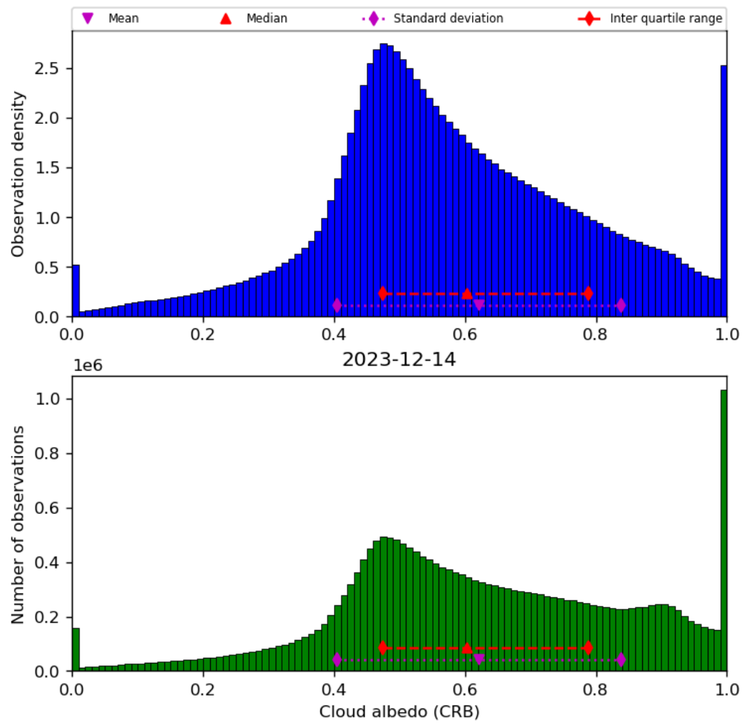
Figure 44: Histogram of “Cloud albedo (CRB)” for 2023-12-14 to 2023-12-15
