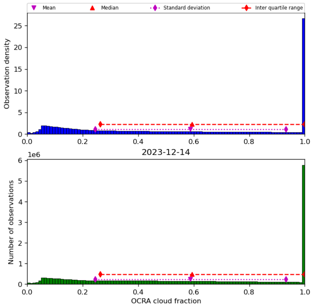
Figure 50: Histogram of “OCRA cloud fraction” for 2023-12-14 to 2023-12-15
