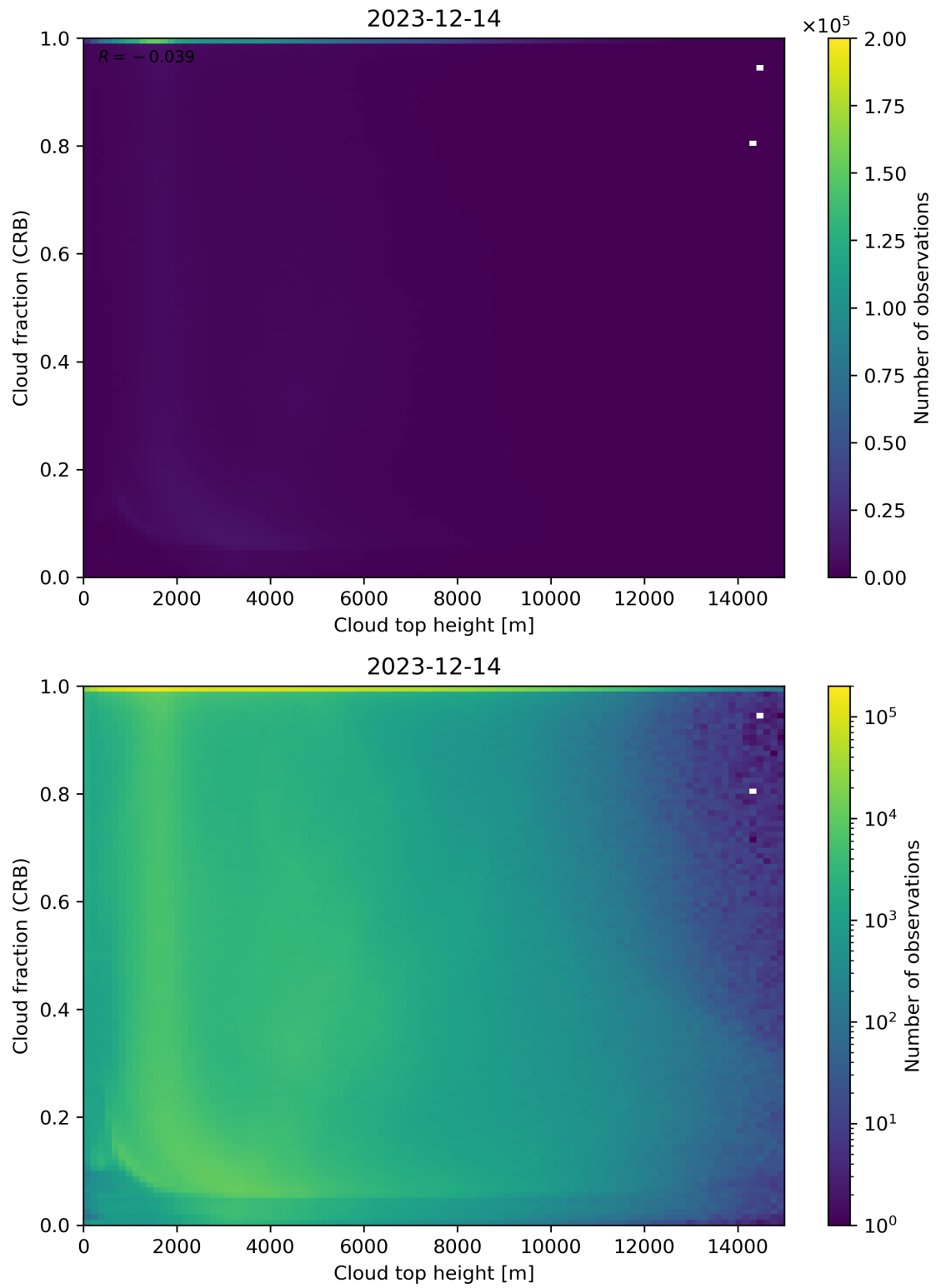
Figure 88: Scatter density plot of “Cloud top height” against “Cloud fraction (CRB)” for 2023-12-14 to 2023-12-15.
