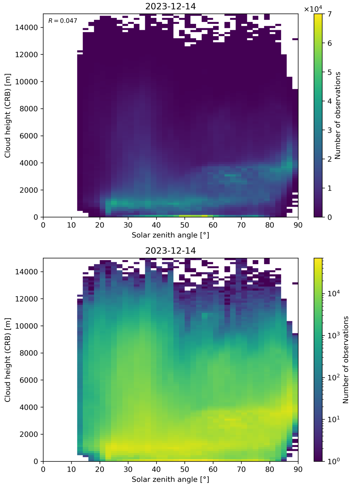
Figure 102: Scatter density plot of “Solar zenith angle” against “Cloud height (CRB)” for 2023-12-14 to 2023-12-15.
