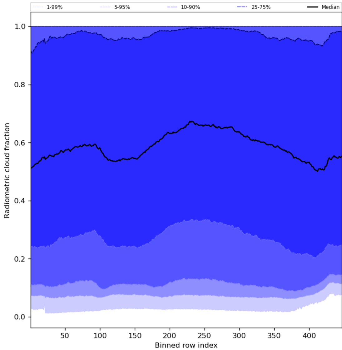
Figure 55: Along track statistics of “Radiometric cloud fraction” for 2023-12-14 to 2023-12-15
