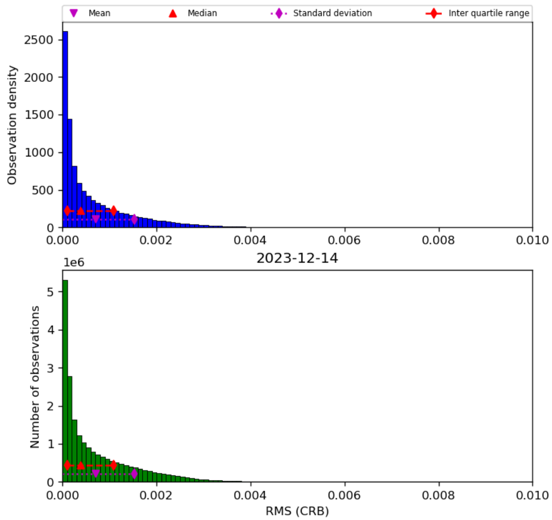
Figure 48: Histogram of “RMS (CRB)” for 2023-12-14 to 2023-12-15
