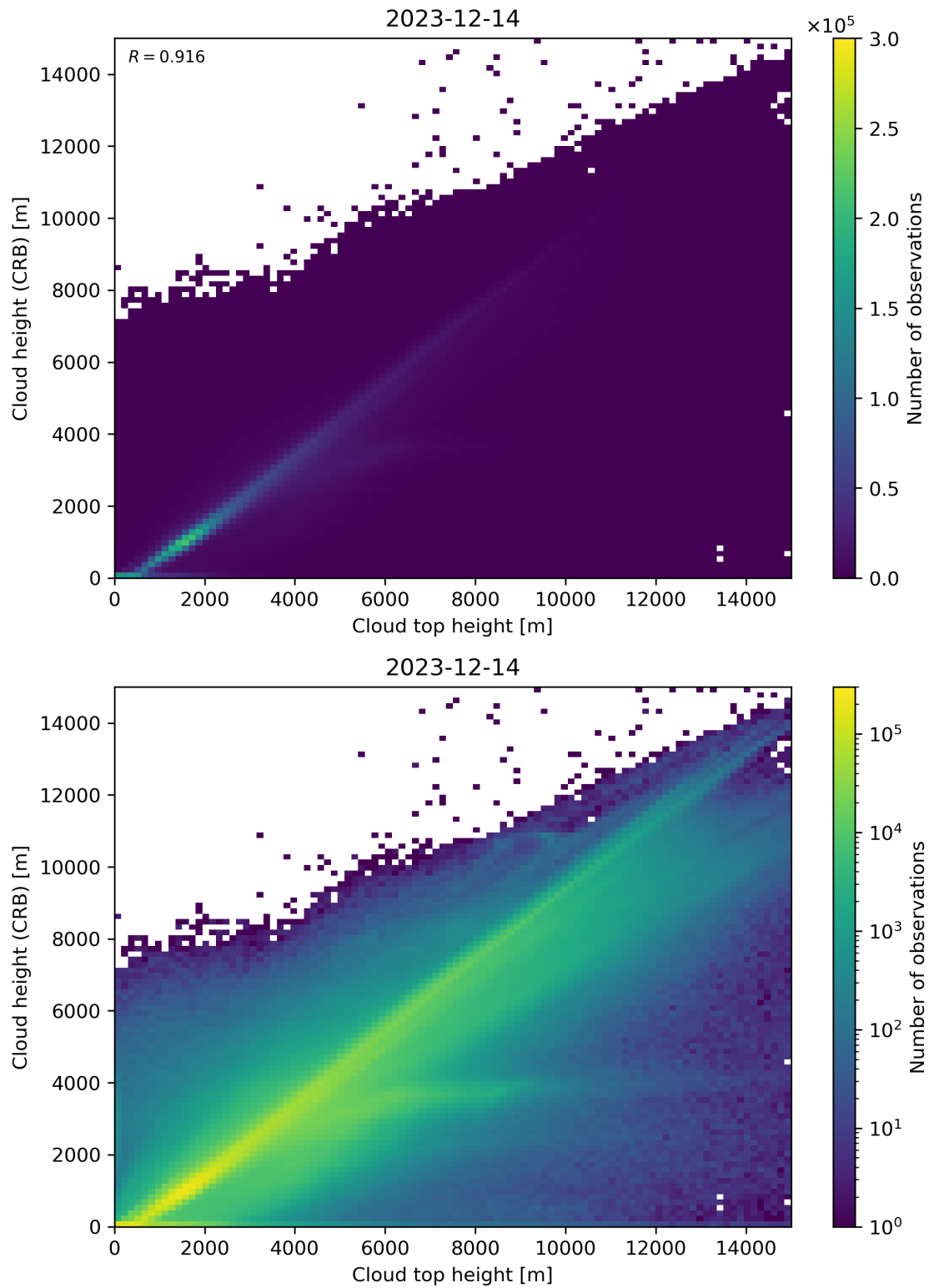
Figure 89: Scatter density plot of “Cloud top height” against “Cloud height (CRB)” for 2023-12-14 to 2023-12-15.
