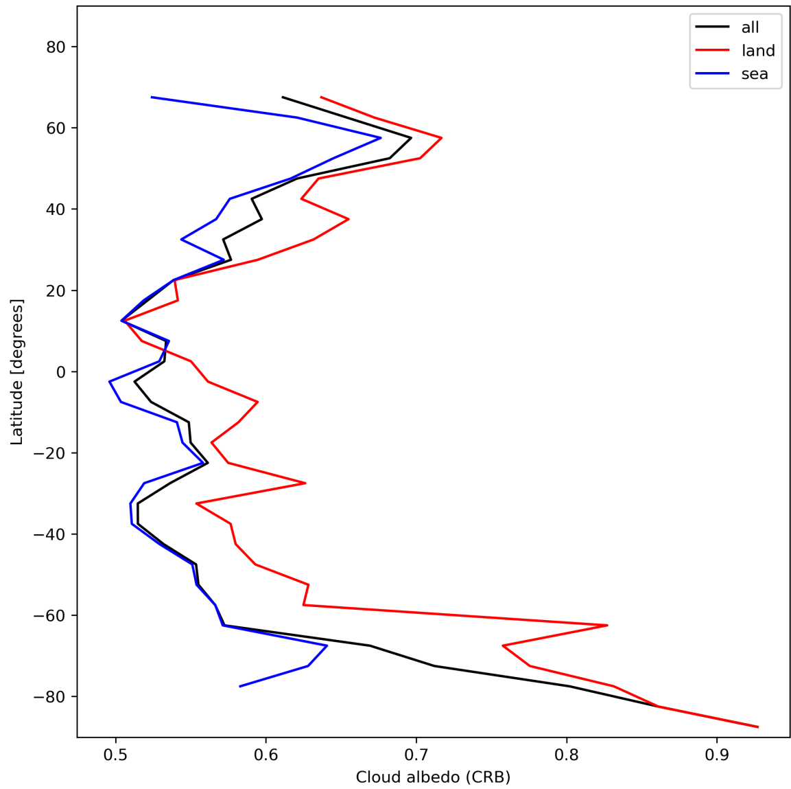
Figure 28: Zonal average of “Cloud albedo (CRB)” for 2023-12-14 to 2023-12-15.
