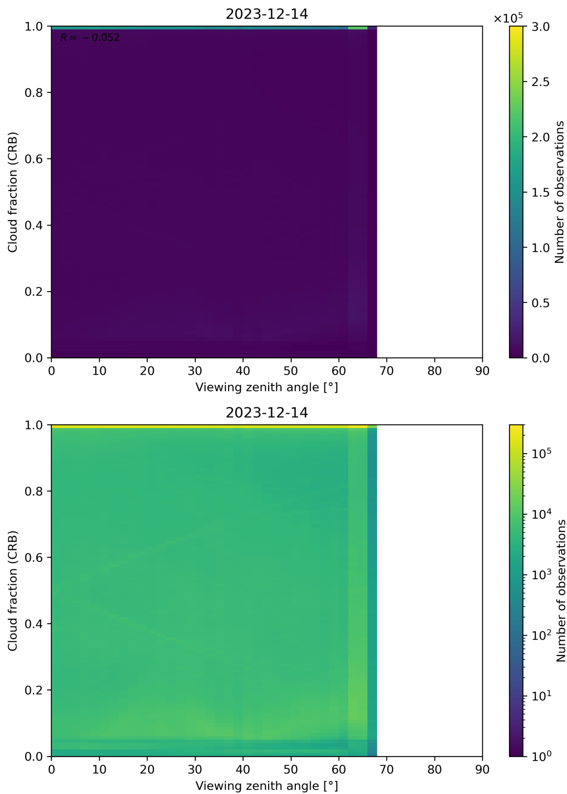
Figure 109: Scatter density plot of “Viewing zenith angle” against “Cloud fraction (CRB)” for 2023-12-14 to 2023-12-15.
