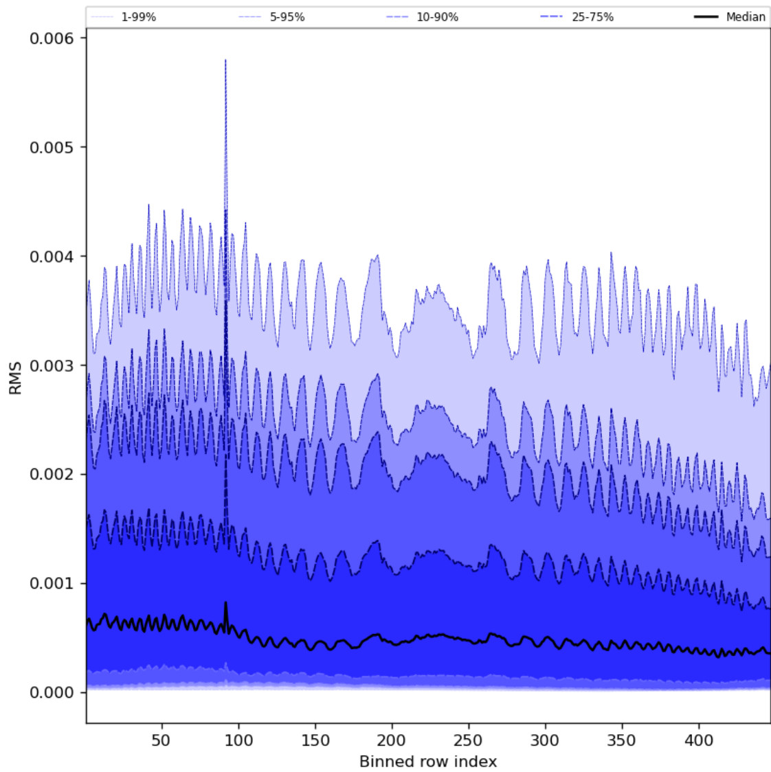
Figure 63: Along track statistics of “RMS” for 2023-12-14 to 2023-12-15
