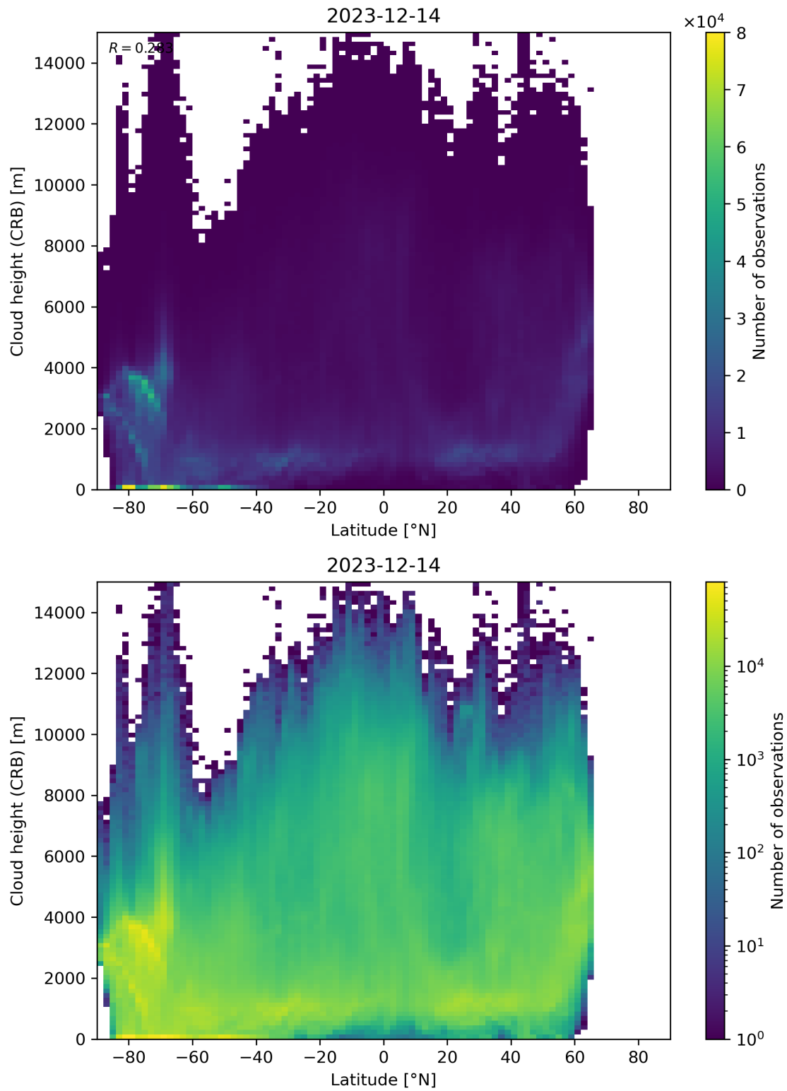
Figure 95: Scatter density plot of “Latitude” against “Cloud height (CRB)” for 2023-12-14 to 2023-12-15.
