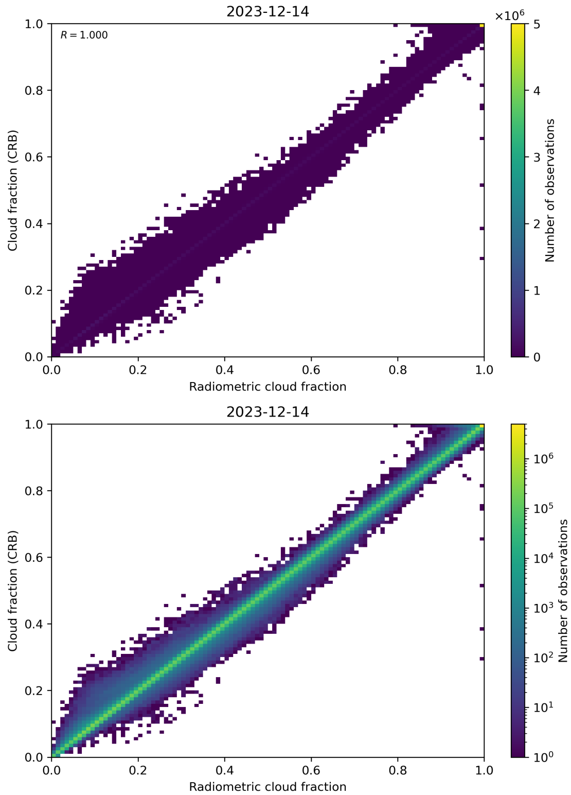
Figure 73: Scatter density plot of “Radiometric cloud fraction” against “Cloud fraction (CRB)” for 2023-12-14 to 2023-12-15.
