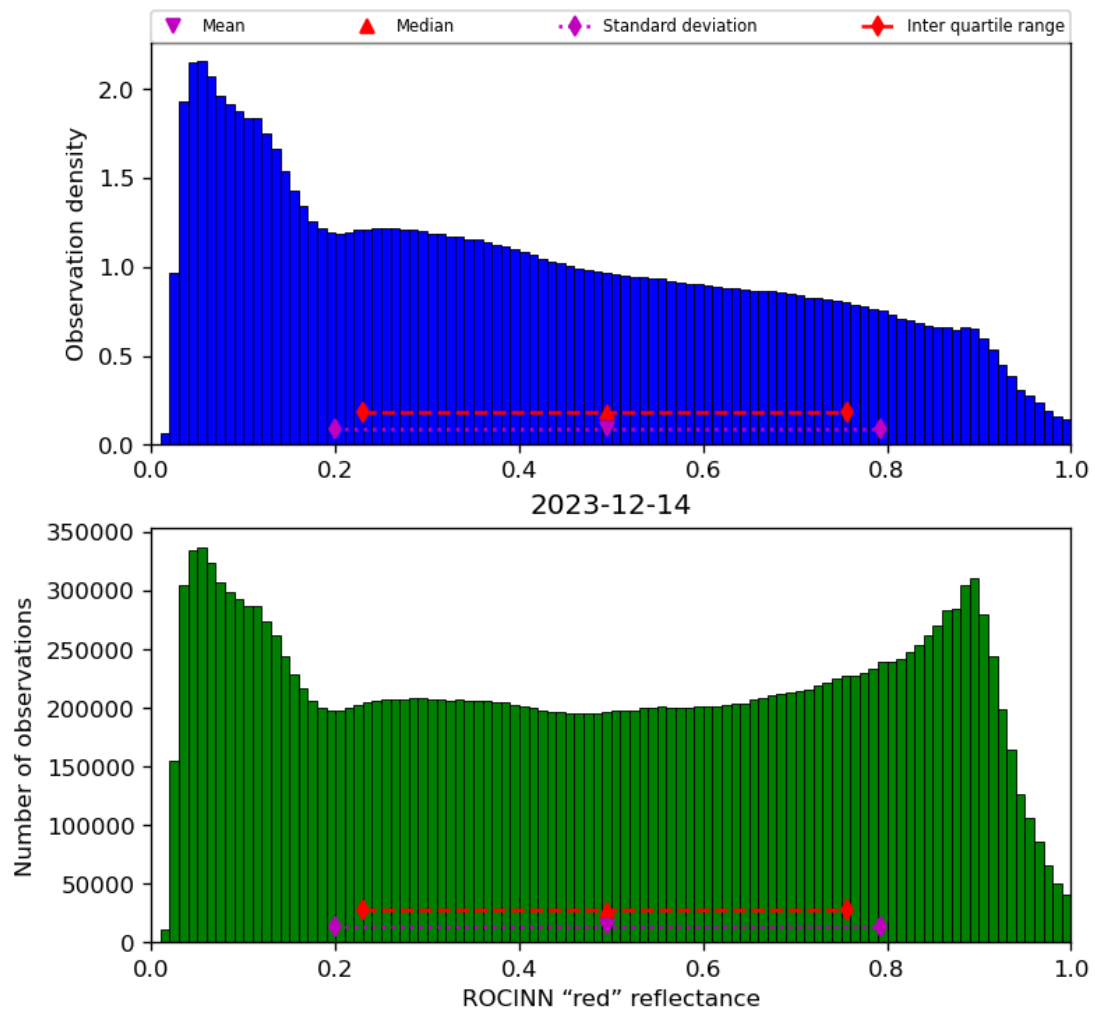
Figure 53: Histogram of “ROCINN “red” reflectance” for 2023-12-14 to 2023-12-15
