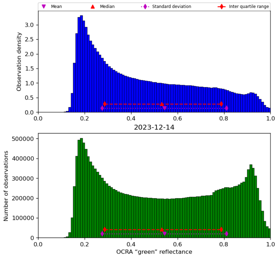
Figure 52: Histogram of “OCRA “green” reflectance” for 2023-12-14 to 2023-12-15
