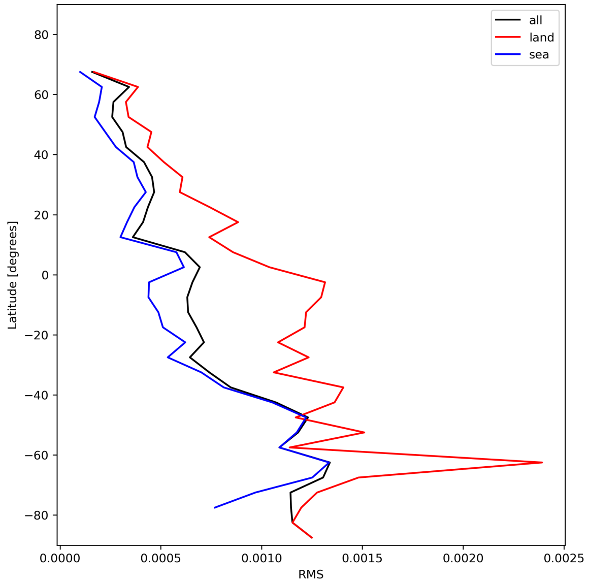
Figure 31: Zonal average of “RMS” for 2023-12-14 to 2023-12-15.
