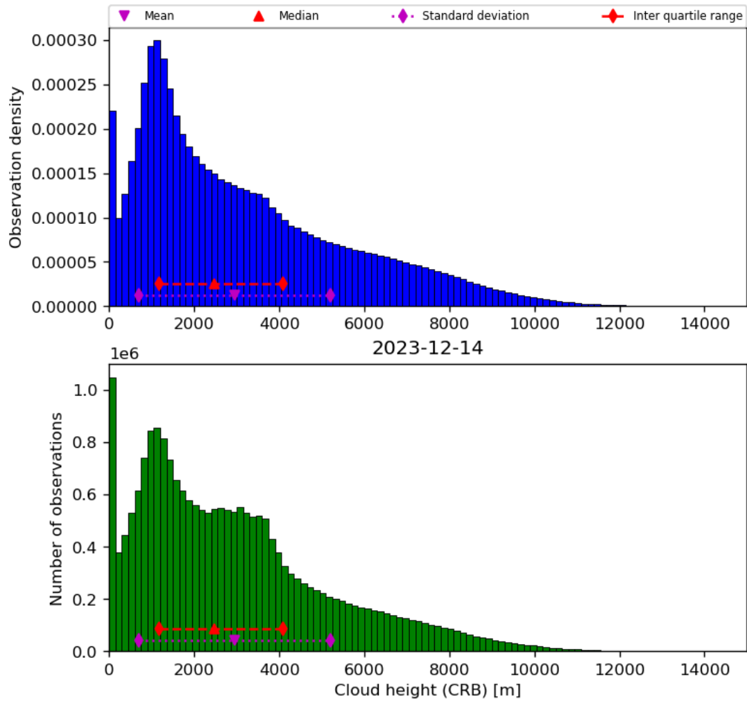
Figure 43: Histogram of “Cloud height (CRB)” for 2023-12-14 to 2023-12-15
