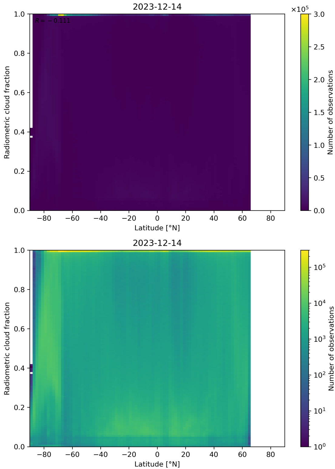
Figure 92: Scatter density plot of “Latitude” against “Radiometric cloud fraction” for 2023-12-14 to 2023-12-15.
