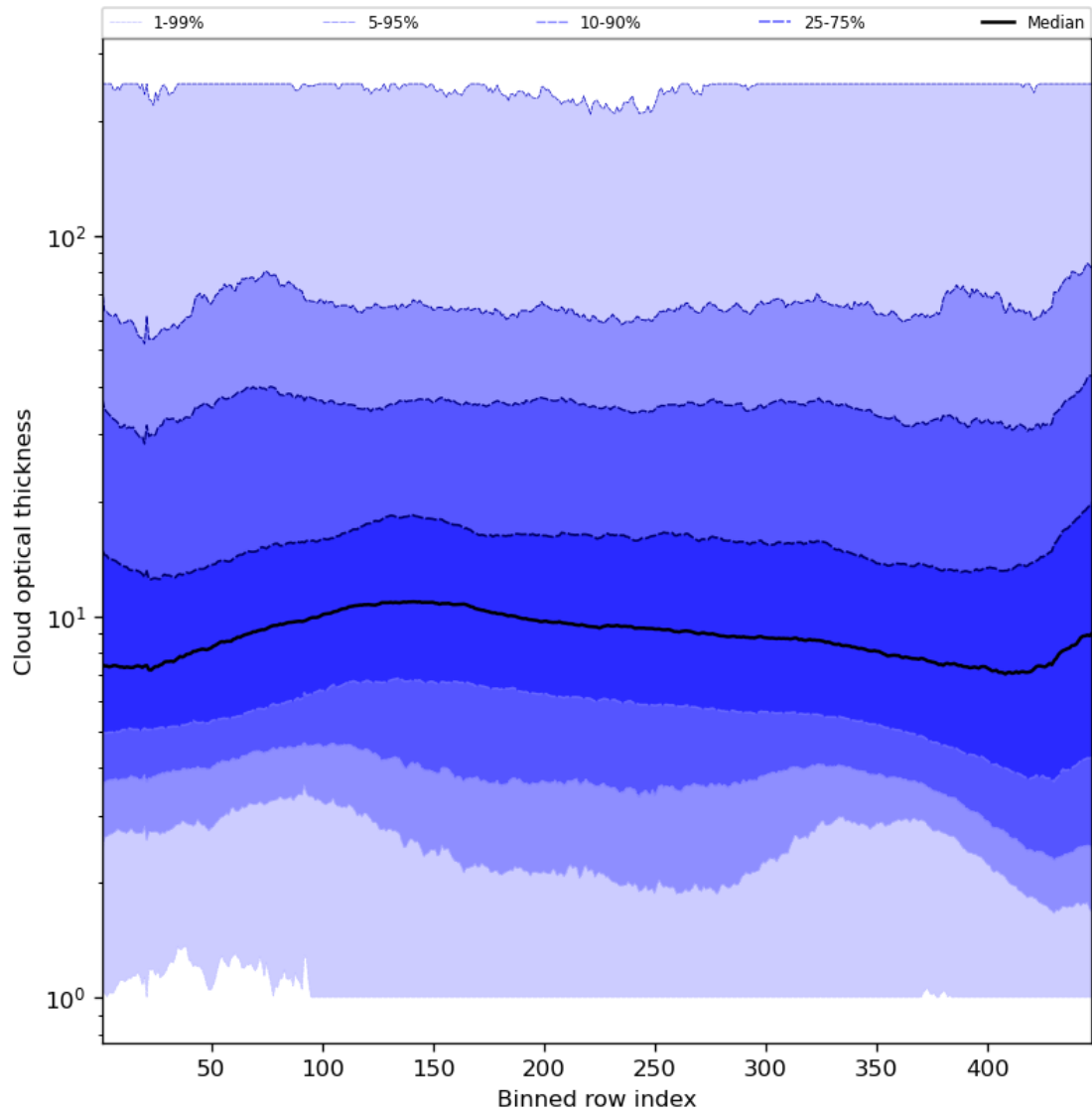
Figure 57: Along track statistics of “Cloud optical thickness” for 2023-12-14 to 2023-12-15
