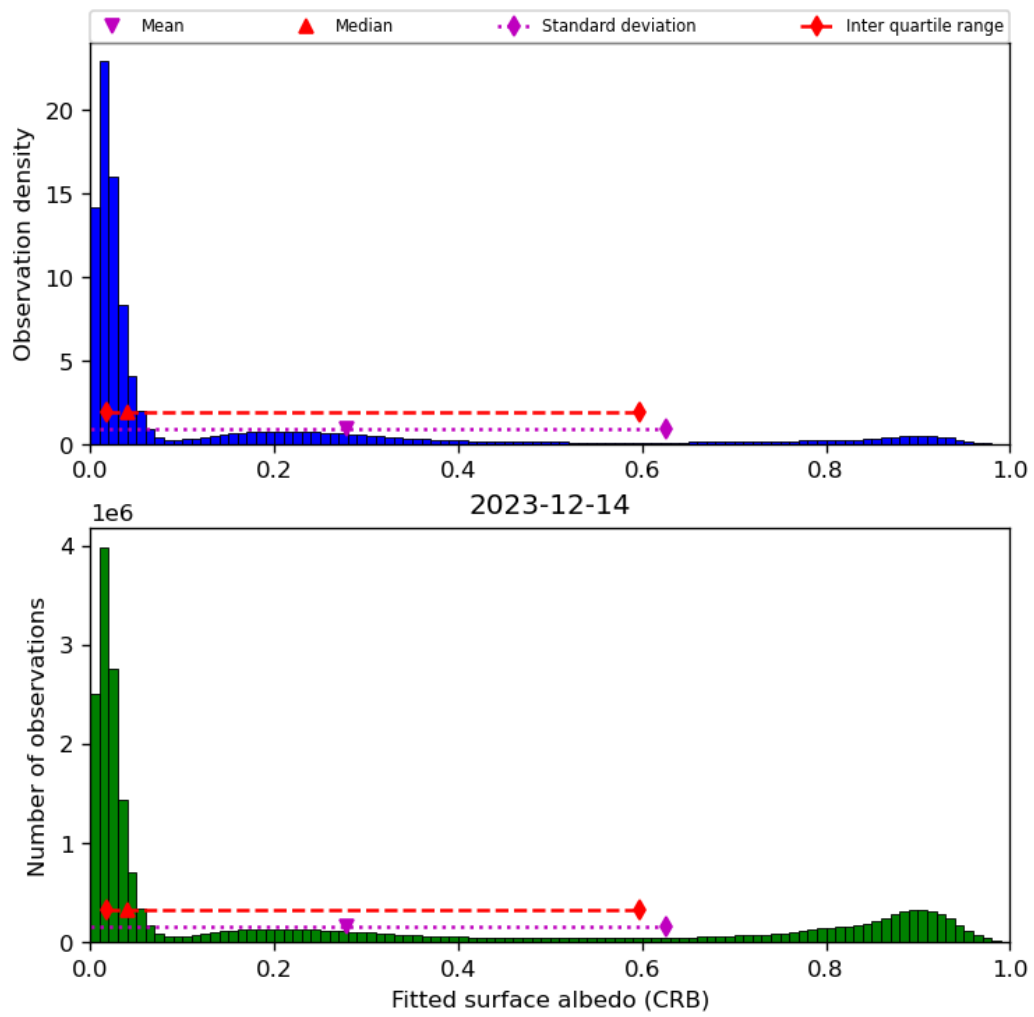
Figure 46: Histogram of “Fitted surface albedo (CRB)” for 2023-12-14 to 2023-12-15
