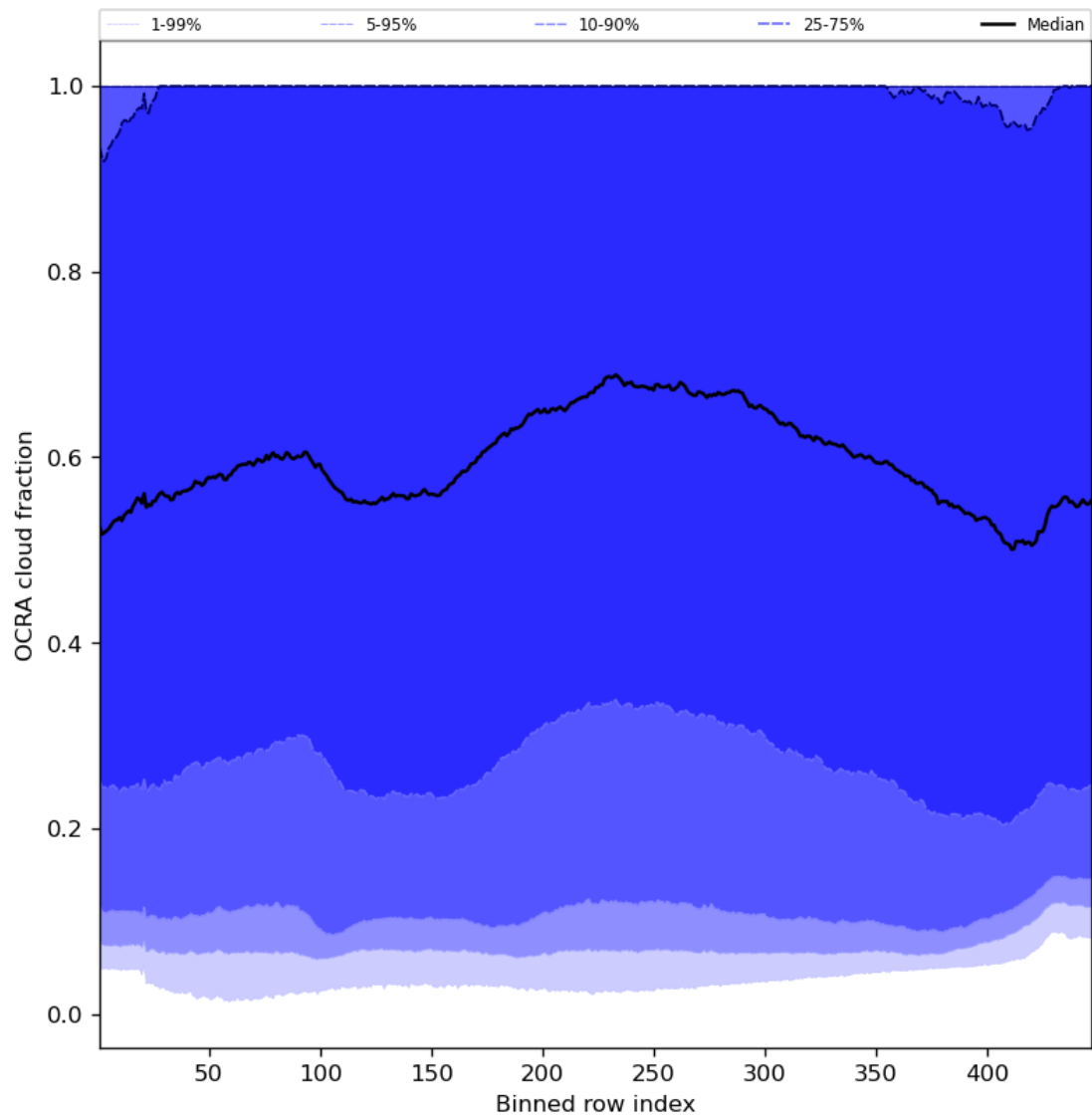
Figure 66: Along track statistics of “OCRA cloud fraction” for 2023-12-14 to 2023-12-15
