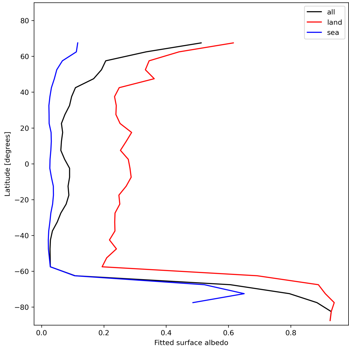
Figure 29: Zonal average of “Fitted surface albedo” for 2023-12-14 to 2023-12-15.
