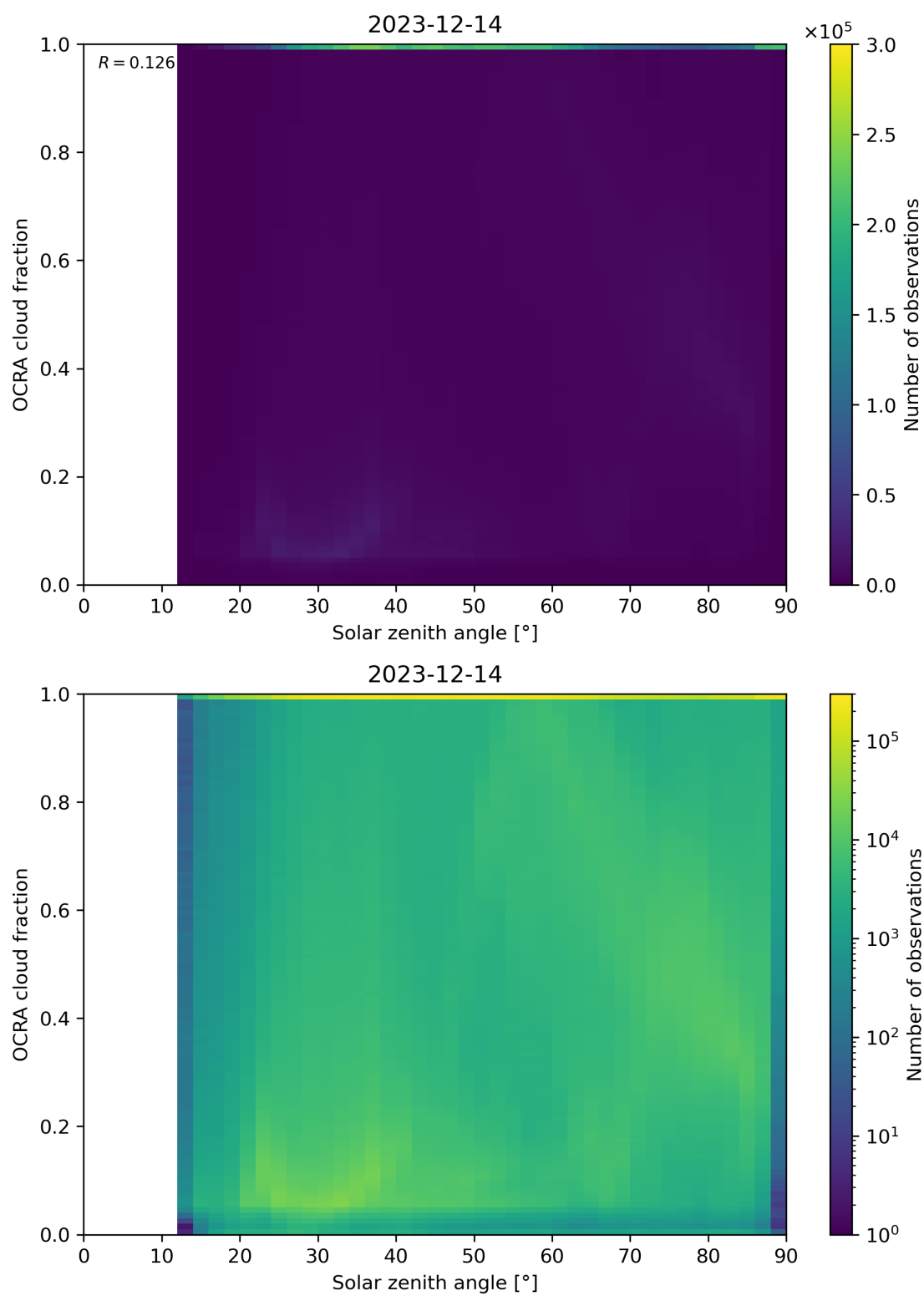
Figure 100: Scatter density plot of “Solar zenith angle” against “OCRA cloud fraction” for 2023-12-14 to 2023-12-15.
