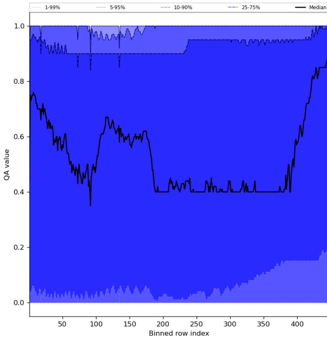
Figure 54: Along track statistics of “QA value” for 2023-12-14 to 2023-12-15
