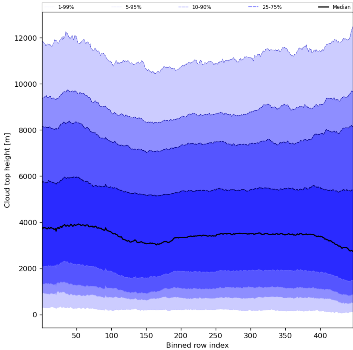
Figure 56: Along track statistics of “Cloud top height” for 2023-12-14 to 2023-12-15
