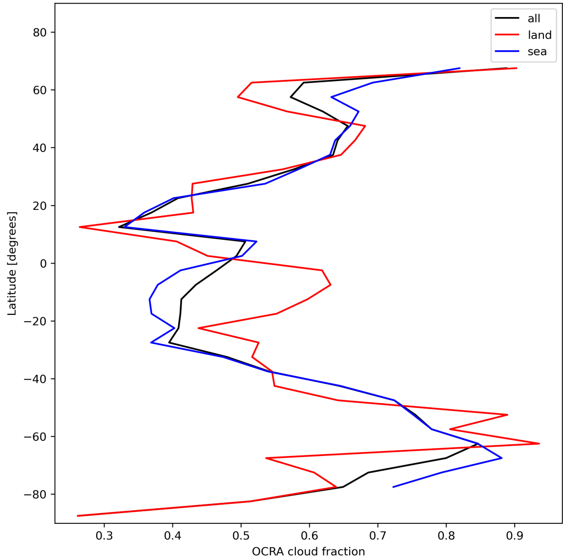
Figure 34: Zonal average of “OCRA cloud fraction” for 2023-12-14 to 2023-12-15.
