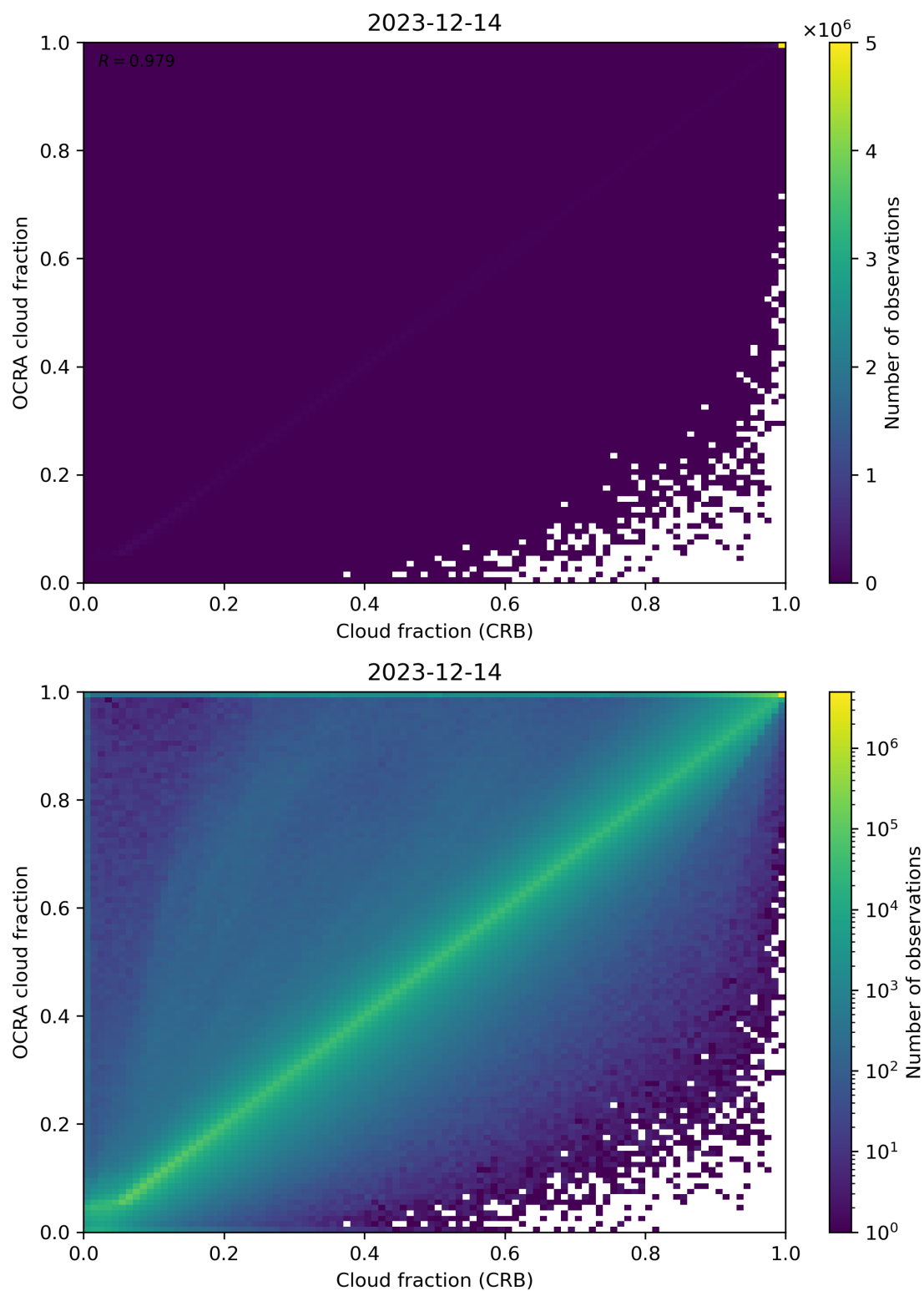
Figure 78: Scatter density plot of “Cloud fraction (CRB)” against “OCRA cloud fraction” for 2023-12-14 to 2023-12-15.
