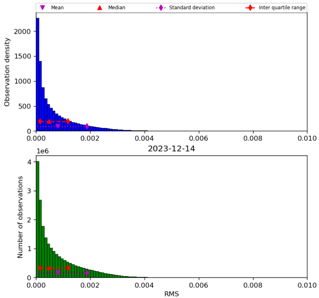
Figure 47: Histogram of “RMS” for 2023-12-14 to 2023-12-15
