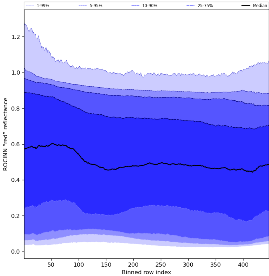
Figure 69: Along track statistics of “ROCINN “red” reflectance” for 2023-12-14 to 2023-12-15
