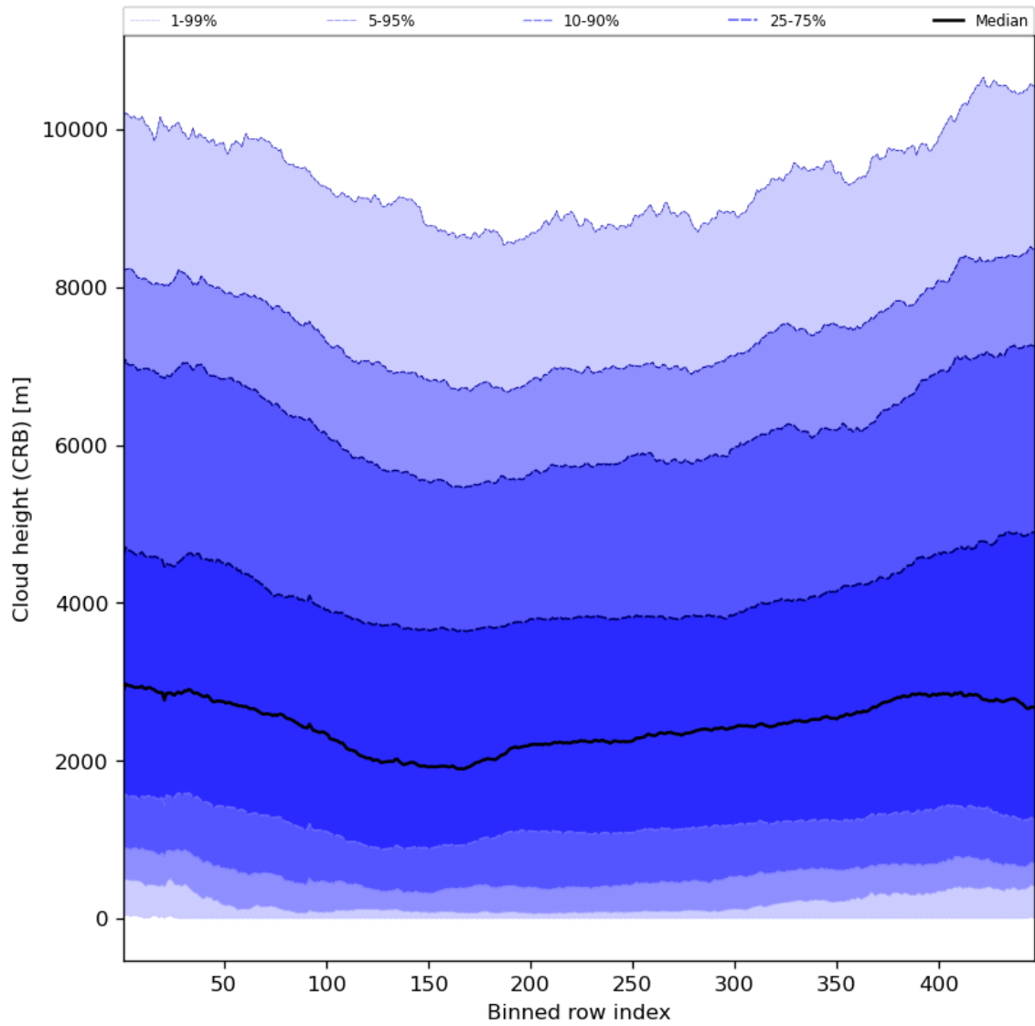
Figure 59: Along track statistics of “Cloud height (CRB)” for 2023-12-14 to 2023-12-15
