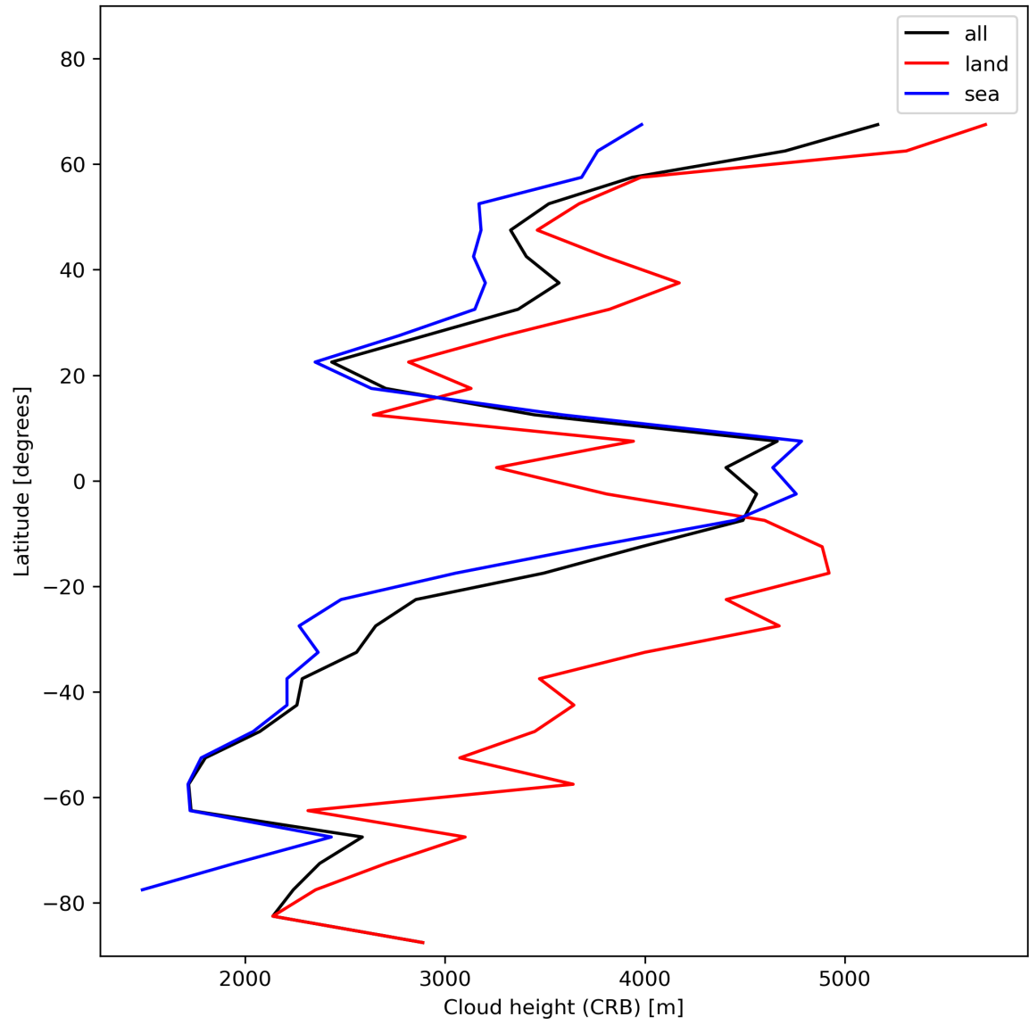
Figure 27: Zonal average of “Cloud height (CRB)” for 2023-12-14 to 2023-12-15.
