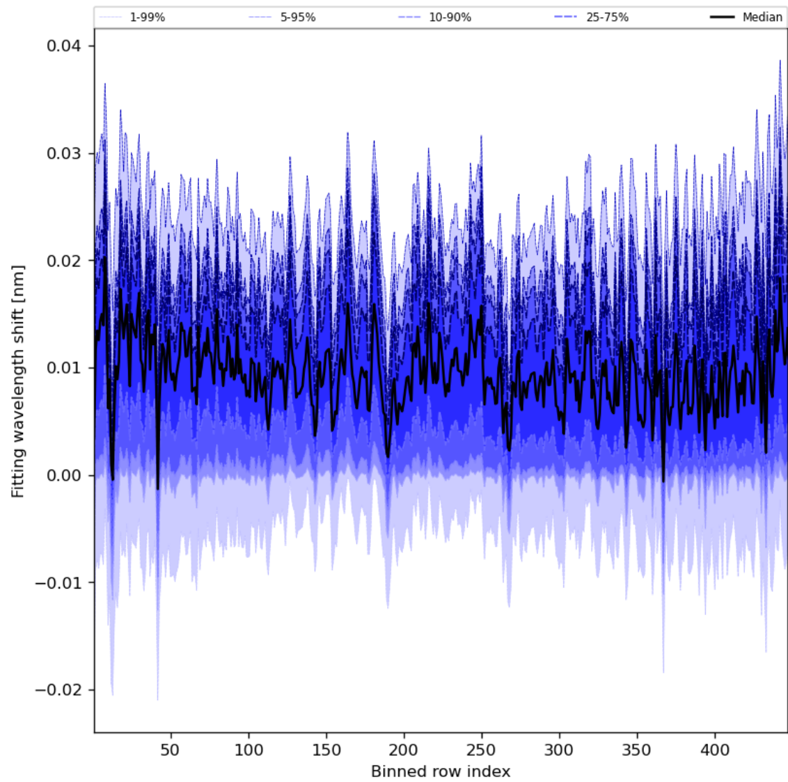
Figure 65: Along track statistics of “Fitting wavelength shift” for 2023-12-14 to 2023-12-15
