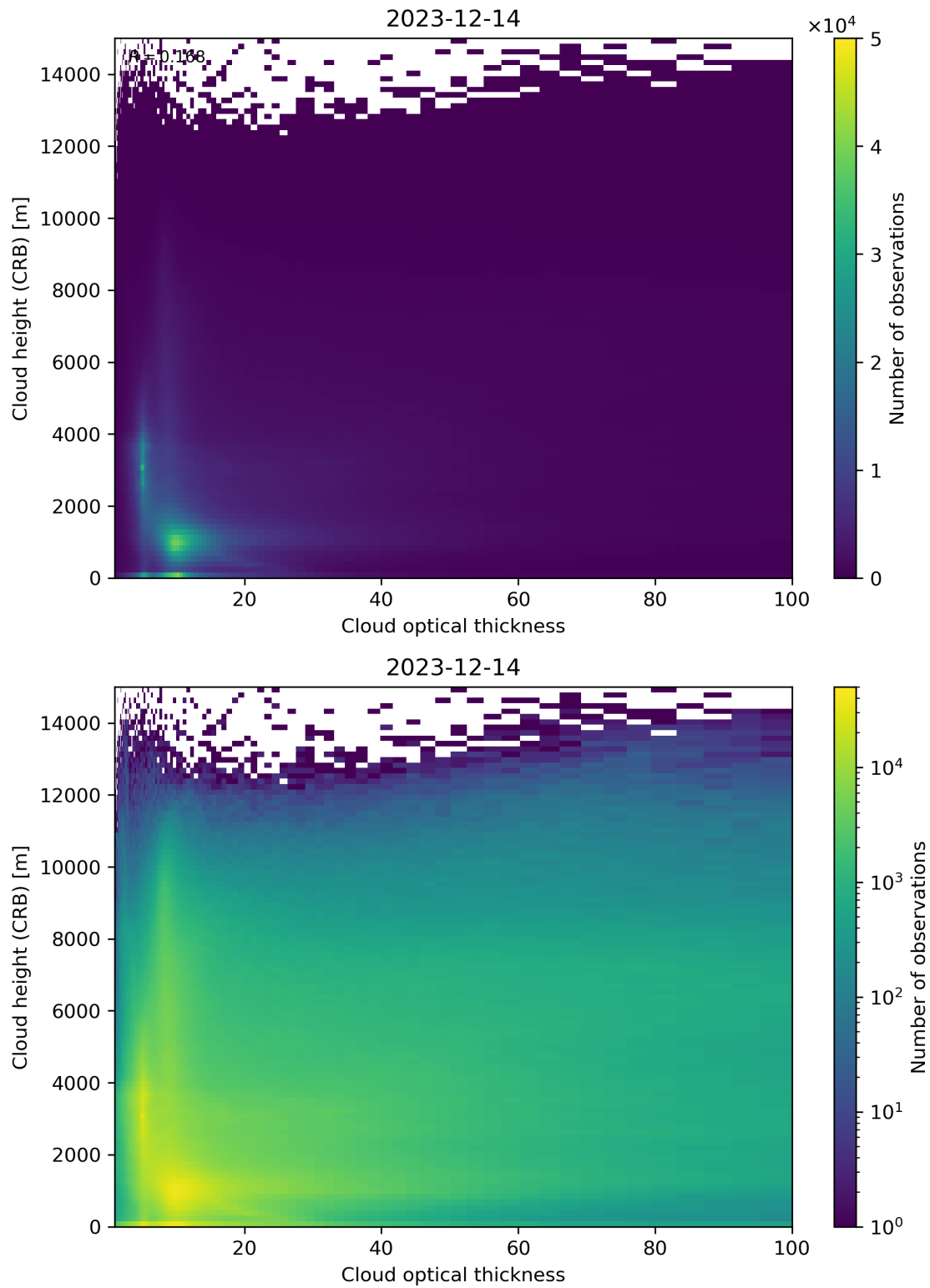
Figure 85: Scatter density plot of “Cloud optical thickness” against “Cloud height (CRB)” for 2023-12-14 to 2023-12-15.
