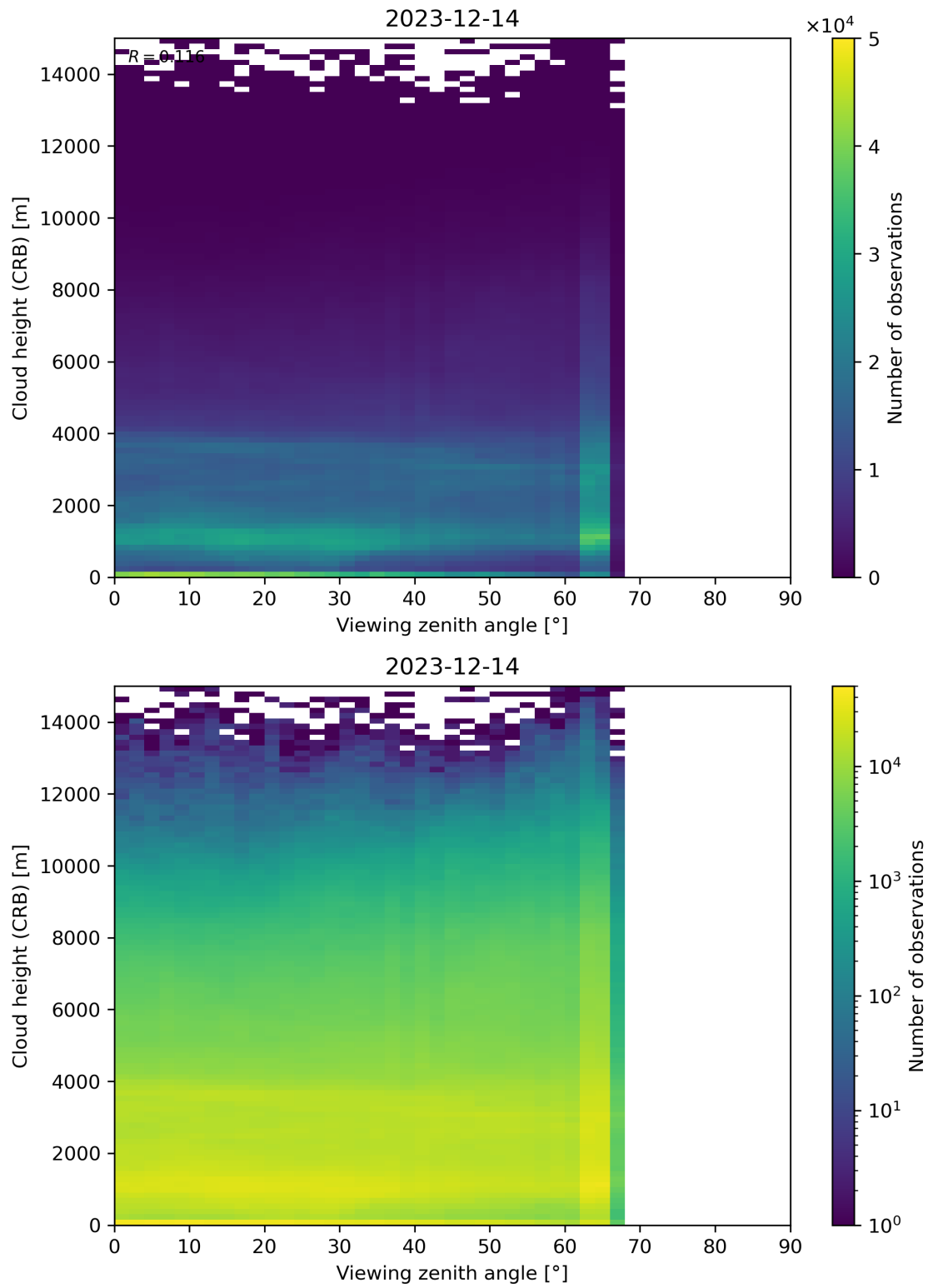
Figure 110: Scatter density plot of “Viewing zenith angle” against “Cloud height (CRB)” for 2023-12-14 to 2023-12-15.
