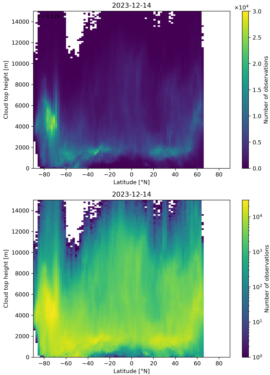
Figure 97: Scatter density plot of “Latitude” against “Cloud top height” for 2023-12-14 to 2023-12-15.
