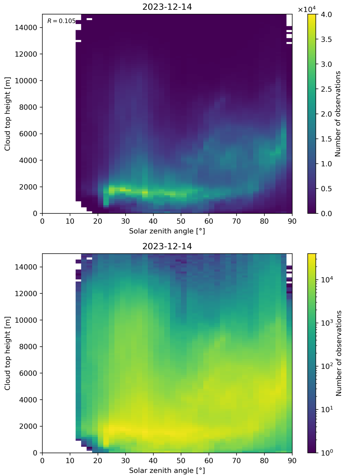
Figure 104: Scatter density plot of “Solar zenith angle” against “Cloud top height” for 2023-12-14 to 2023-12-15.
