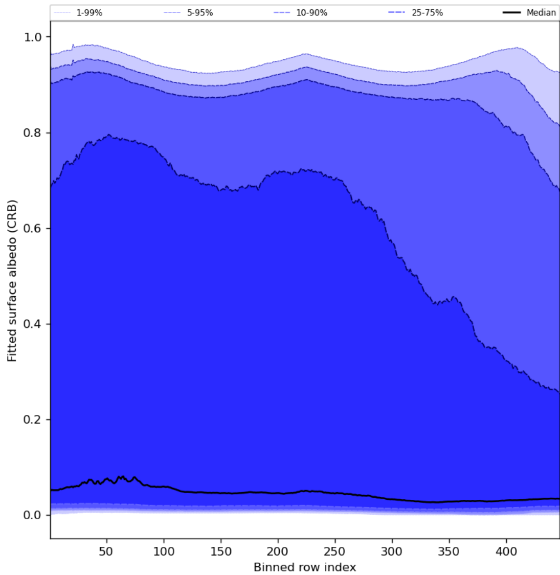
Figure 62: Along track statistics of “Fitted surface albedo (CRB)” for 2023-12-14 to 2023-12-15
