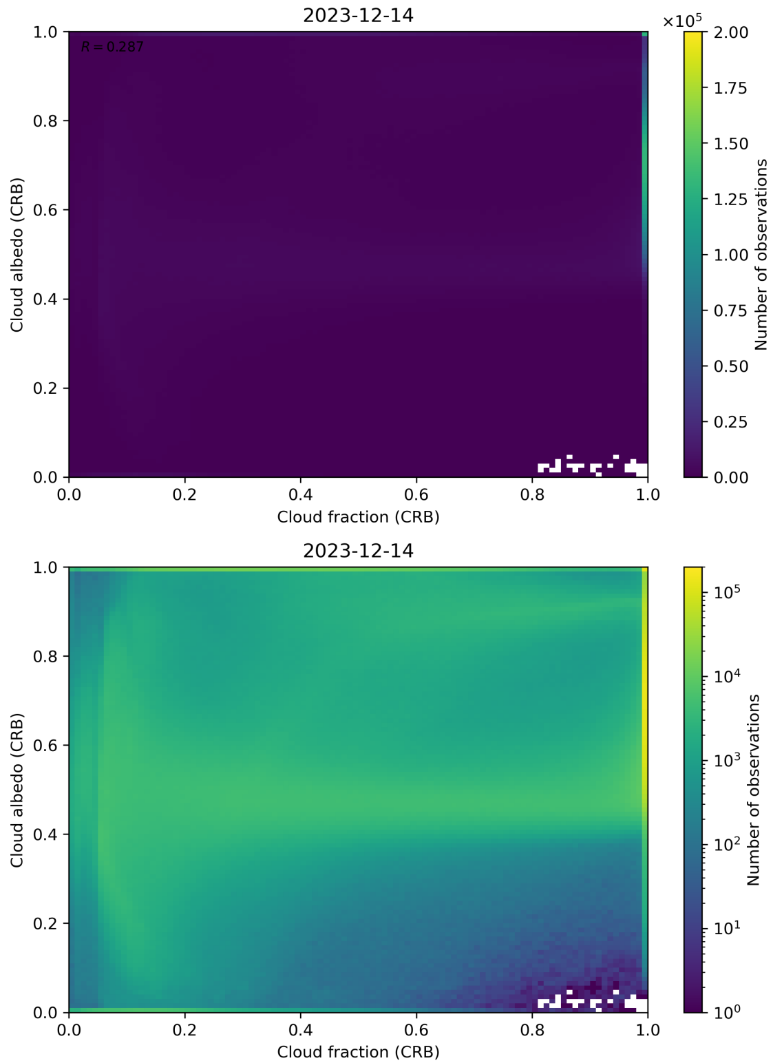
Figure 77: Scatter density plot of “Cloud fraction (CRB)” against “Cloud albedo (CRB)” for 2023-12-14 to 2023-12-15.
