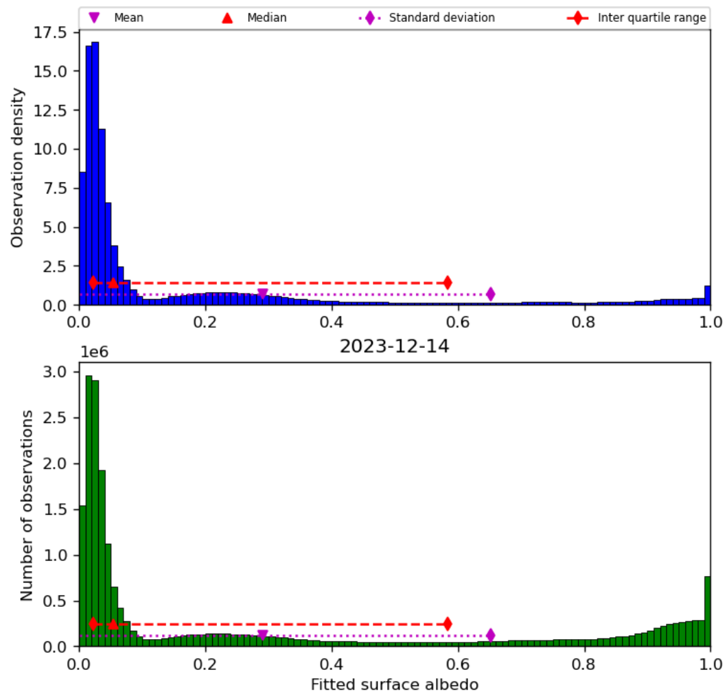
Figure 45: Histogram of “Fitted surface albedo” for 2023-12-14 to 2023-12-15
