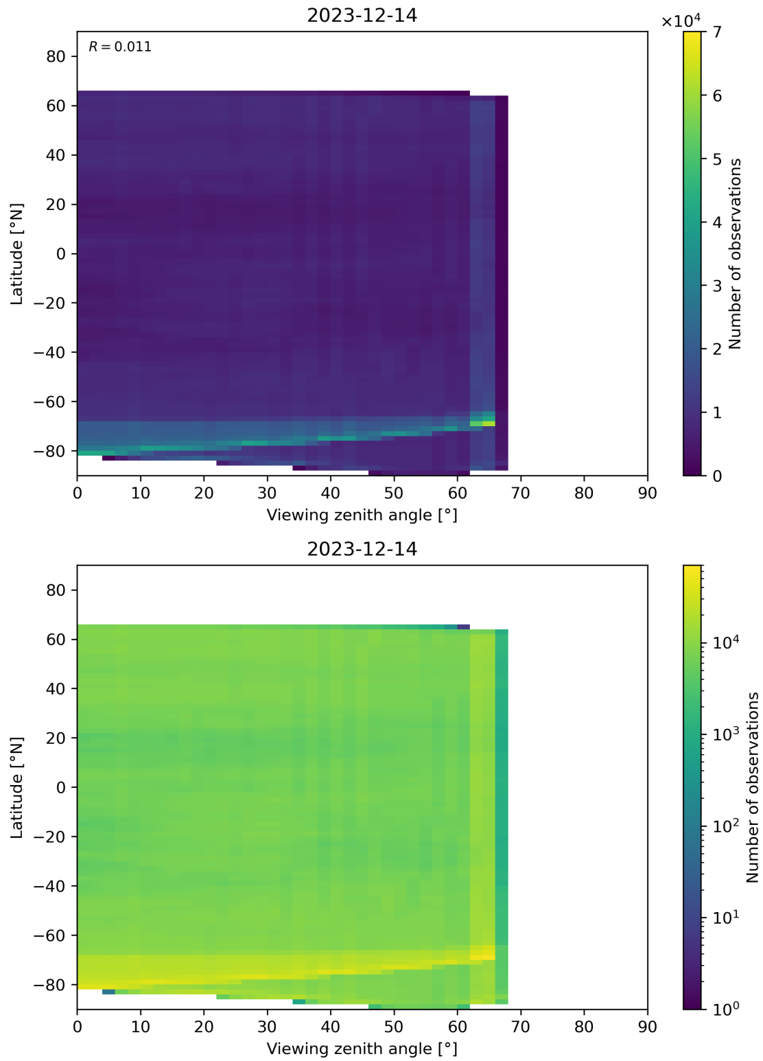
Figure 113: Scatter density plot of “Viewing zenith angle” against “Latitude” for 2023-12-14 to 2023-12-15.
