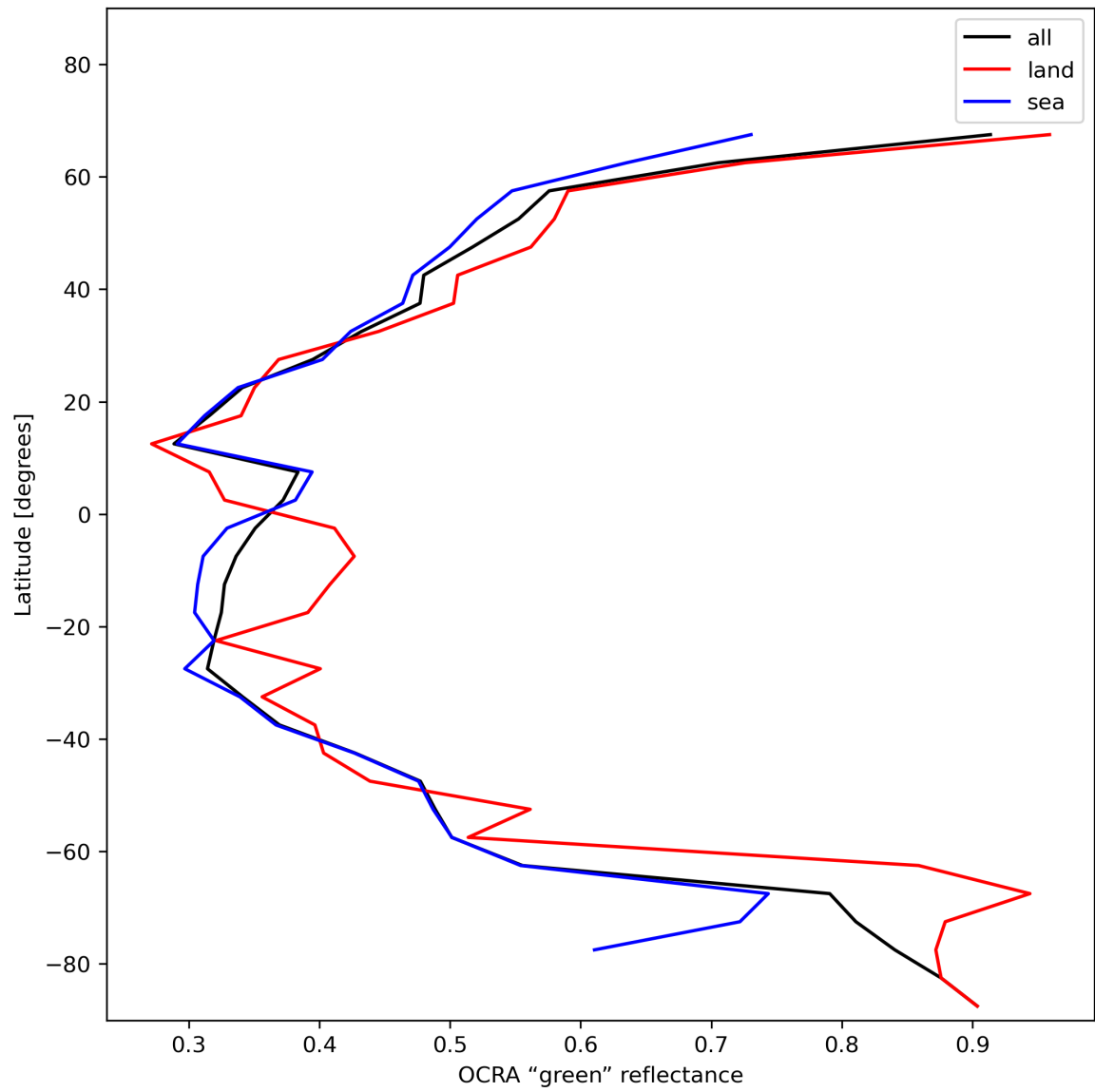
Figure 36: Zonal average of “OCRA “green” reflectance” for 2023-12-14 to 2023-12-15.
