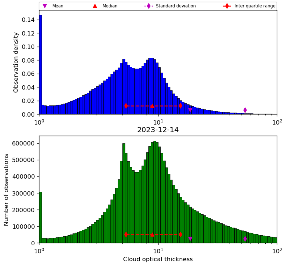
Figure 41: Histogram of “Cloud optical thickness” for 2023-12-14 to 2023-12-15
