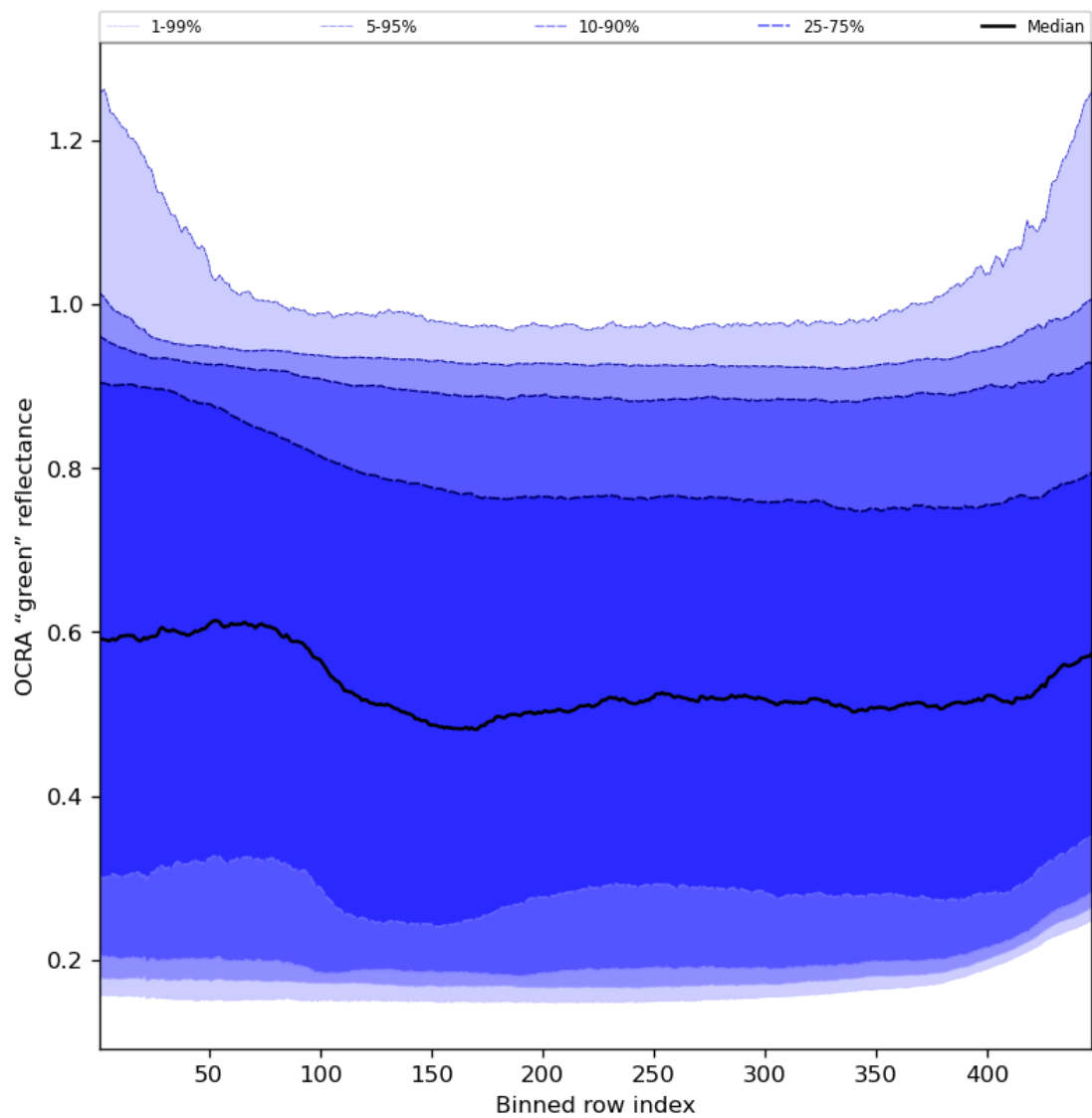
Figure 68: Along track statistics of "OCRA "green" reflectance" for 2023-12-14 to 2023-12-15
