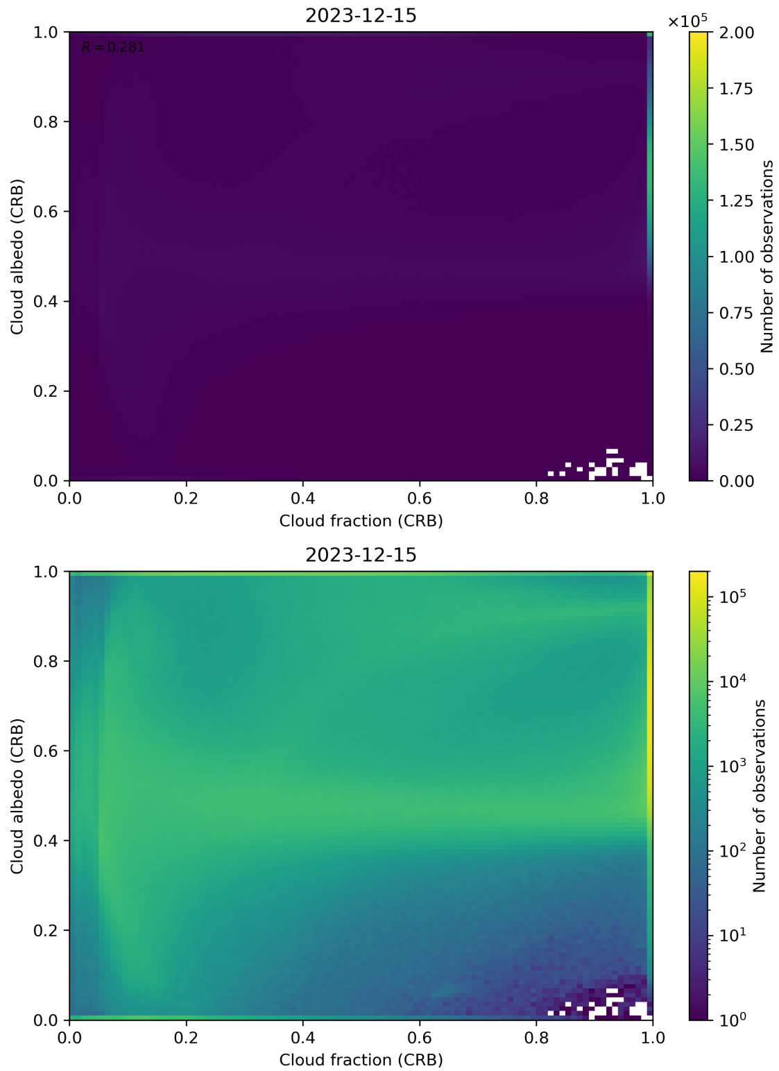
Figure 77: Scatter density plot of “Cloud fraction (CRB)” against “Cloud albedo (CRB)” for 2023-12-14 to 2023-12-16.
