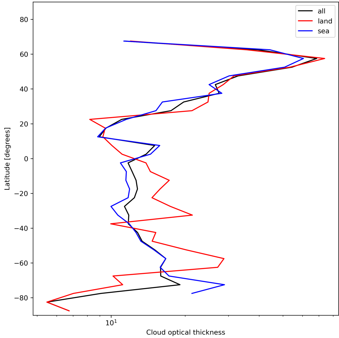
Figure 25: Zonal average of “Cloud optical thickness” for 2023-12-14 to 2023-12-16.
