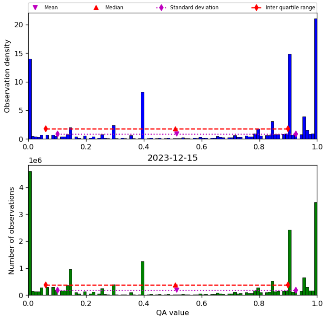
Figure 38: Histogram of “QA value” for 2023-12-14 to 2023-12-16
