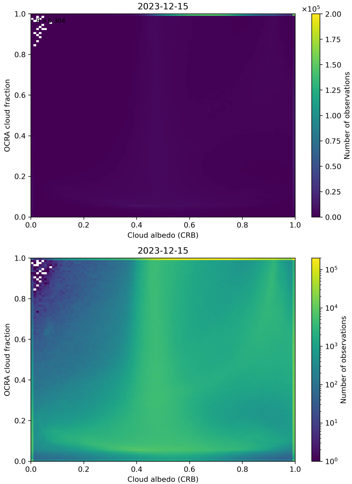
Figure 70: Scatter density plot of “Cloud albedo (CRB)” against “OCRA cloud fraction” for 2023-12-14 to 2023-12-16.
