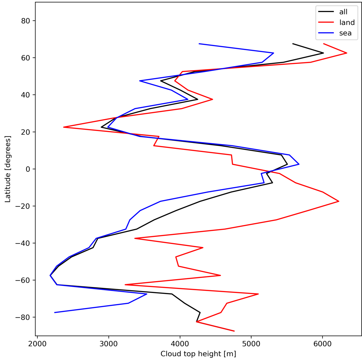
Figure 24: Zonal average of “Cloud top height” for 2023-12-14 to 2023-12-16.
