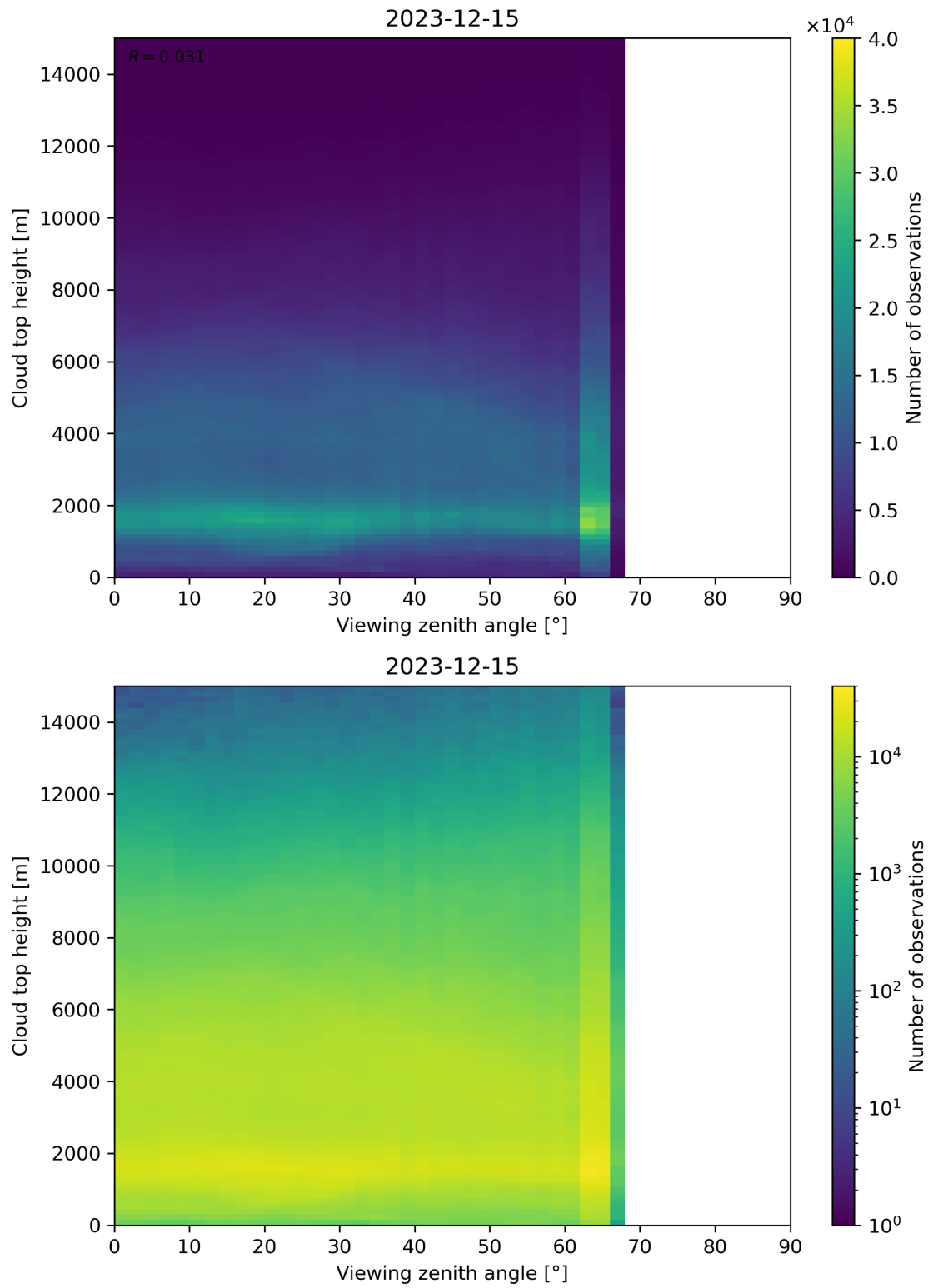
Figure 112: Scatter density plot of “Viewing zenith angle” against “Cloud top height” for 2023-12-14 to 2023-12-16.
