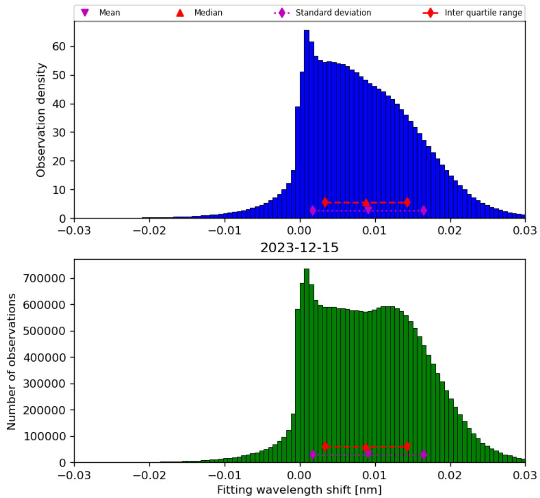
Figure 49: Histogram of “Fitting wavelength shift” for 2023-12-14 to 2023-12-16
