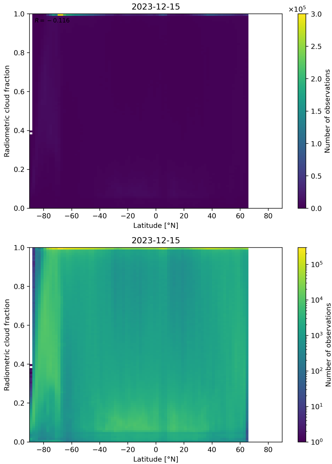
Figure 92: Scatter density plot of “Latitude” against “Radiometric cloud fraction” for 2023-12-14 to 2023-12-16.
