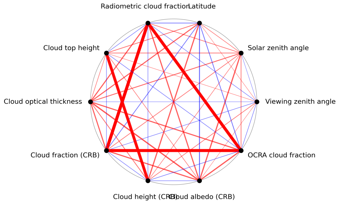
Figure 1: Map of correlation graph for 2023-12-14 to 2023-12-16.
