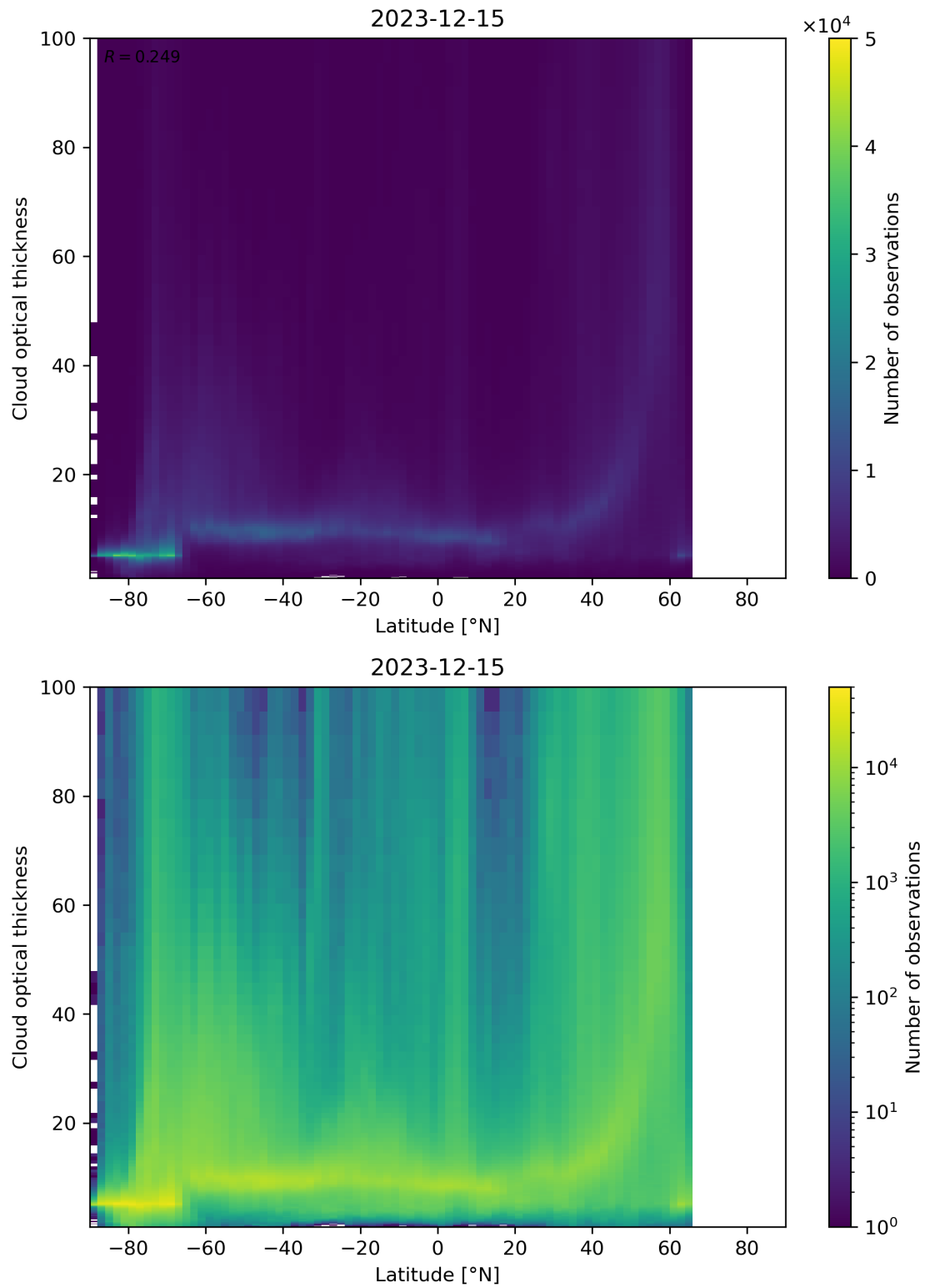
Figure 96: Scatter density plot of “Latitude” against “Cloud optical thickness” for 2023-12-14 to 2023-12-16.
