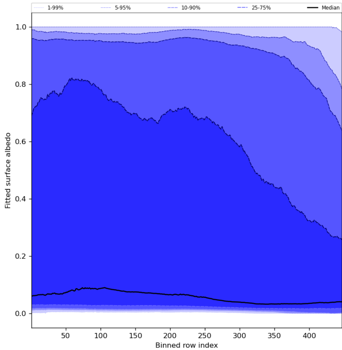
Figure 61: Along track statistics of “Fitted surface albedo” for 2023-12-14 to 2023-12-16
