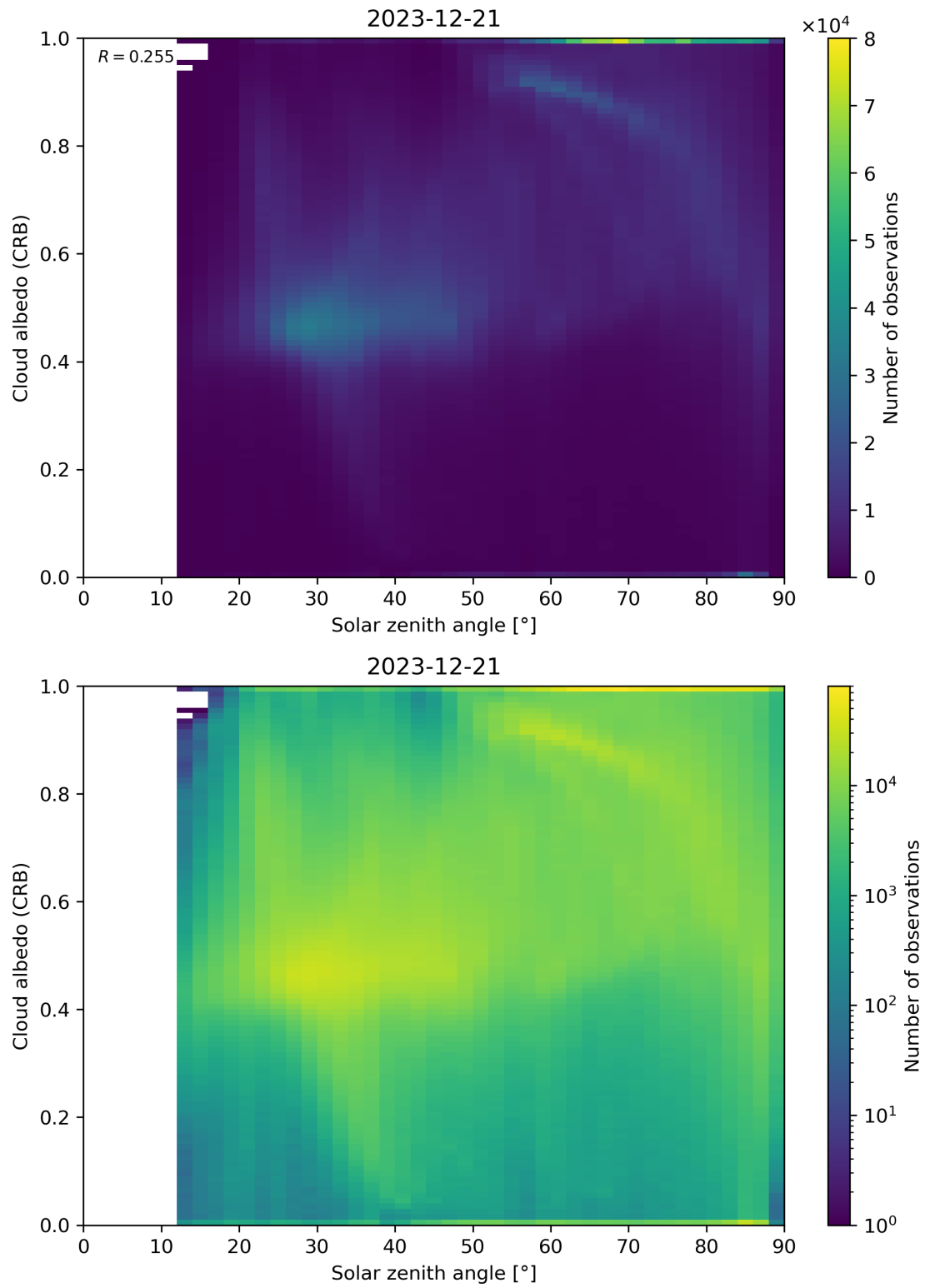
Figure 98: Scatter density plot of “Solar zenith angle” against “Cloud albedo (CRB)” for 2023-12-20 to 2023-12-22.
