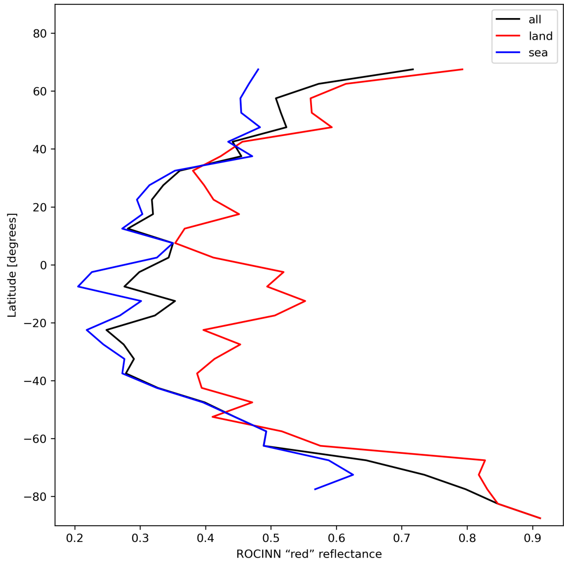
Figure 37: Zonal average of “ROCINN “red” reflectance” for 2023-12-20 to 2023-12-22.
