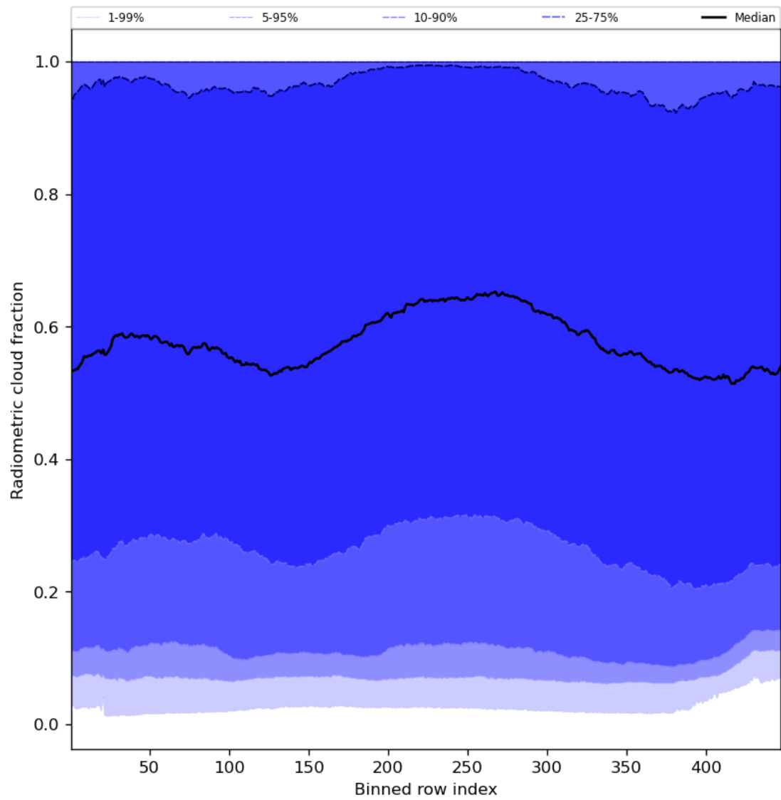
Figure 55: Along track statistics of “Radiometric cloud fraction” for 2023-12-20 to 2023-12-22
