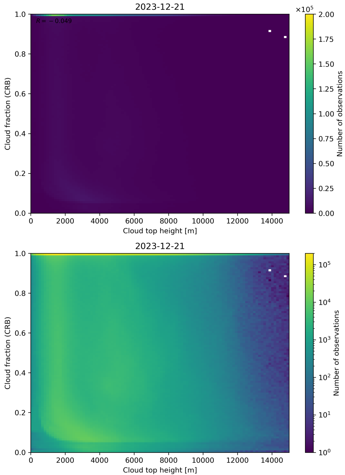
Figure 88: Scatter density plot of “Cloud top height” against “Cloud fraction (CRB)” for 2023-12-20 to 2023-12-22.
