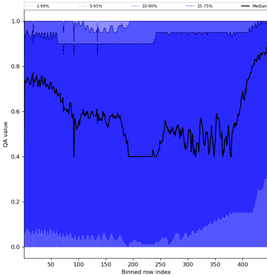
Figure 54: Along track statistics of “QA value” for 2023-12-20 to 2023-12-22
