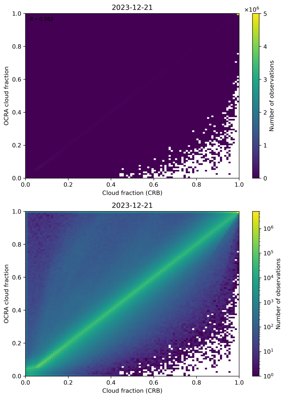
Figure 78: Scatter density plot of “Cloud fraction (CRB)” against “OCRA cloud fraction” for 2023-12-20 to 2023-12-22.
