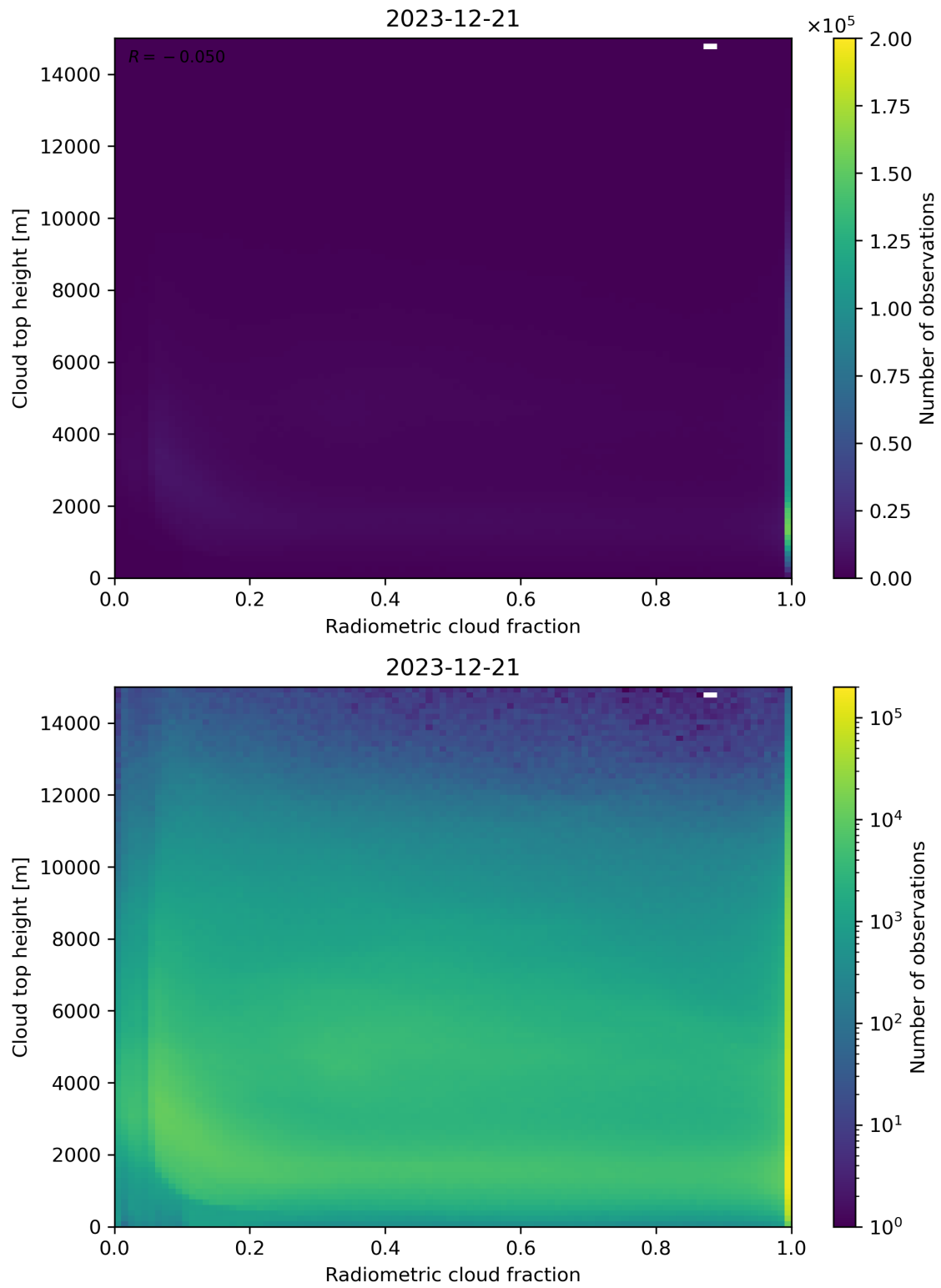
Figure 76: Scatter density plot of “Radiometric cloud fraction” against “Cloud top height” for 2023-12-20 to 2023-12-22.
