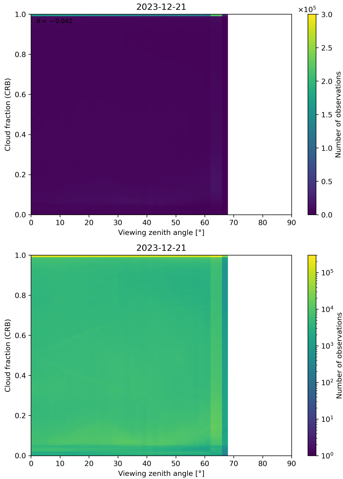
Figure 109: Scatter density plot of “Viewing zenith angle” against “Cloud fraction (CRB)” for 2023-12-20 to 2023-12-22.
