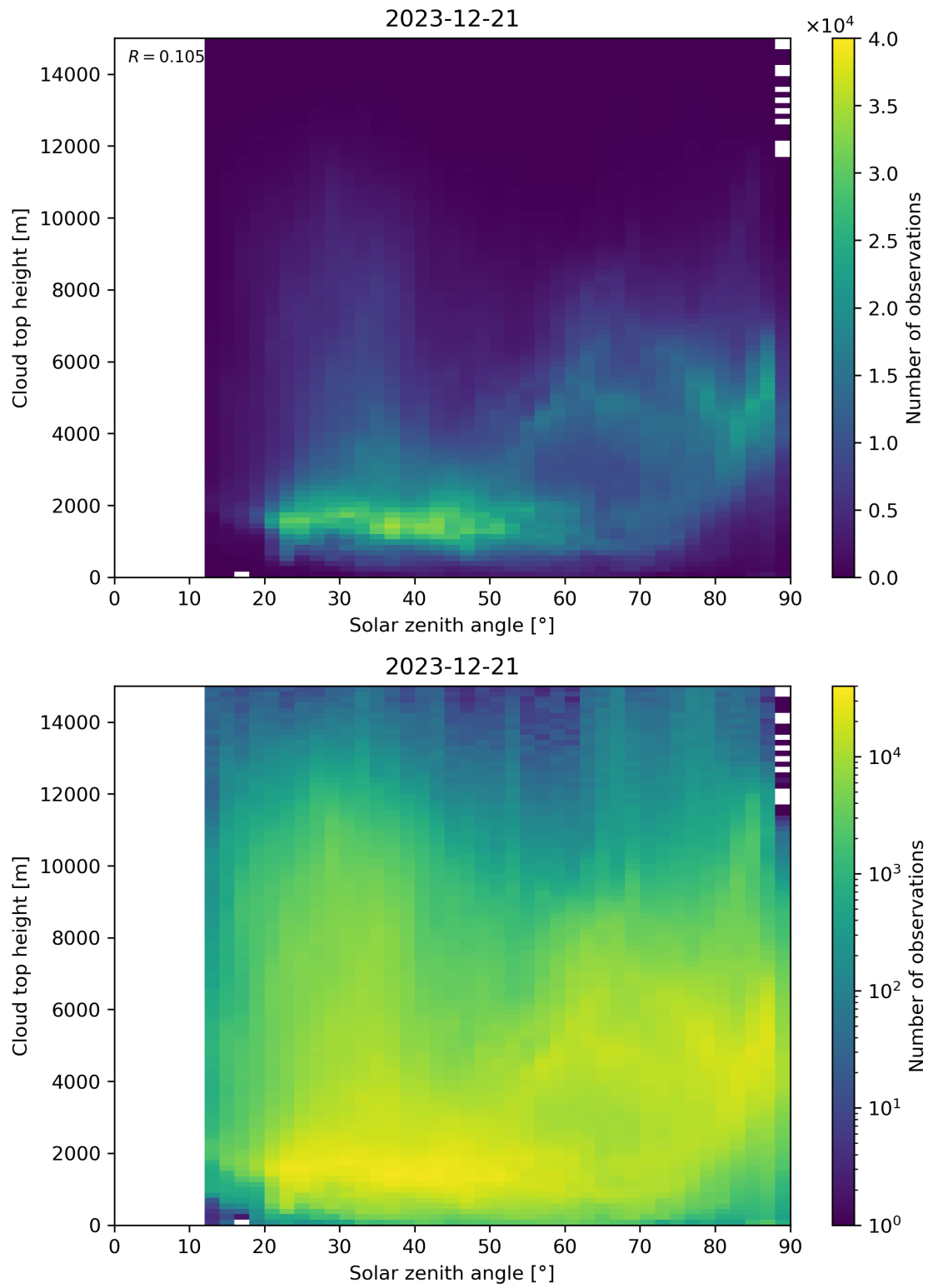
Figure 104: Scatter density plot of “Solar zenith angle” against “Cloud top height” for 2023-12-20 to 2023-12-22.
