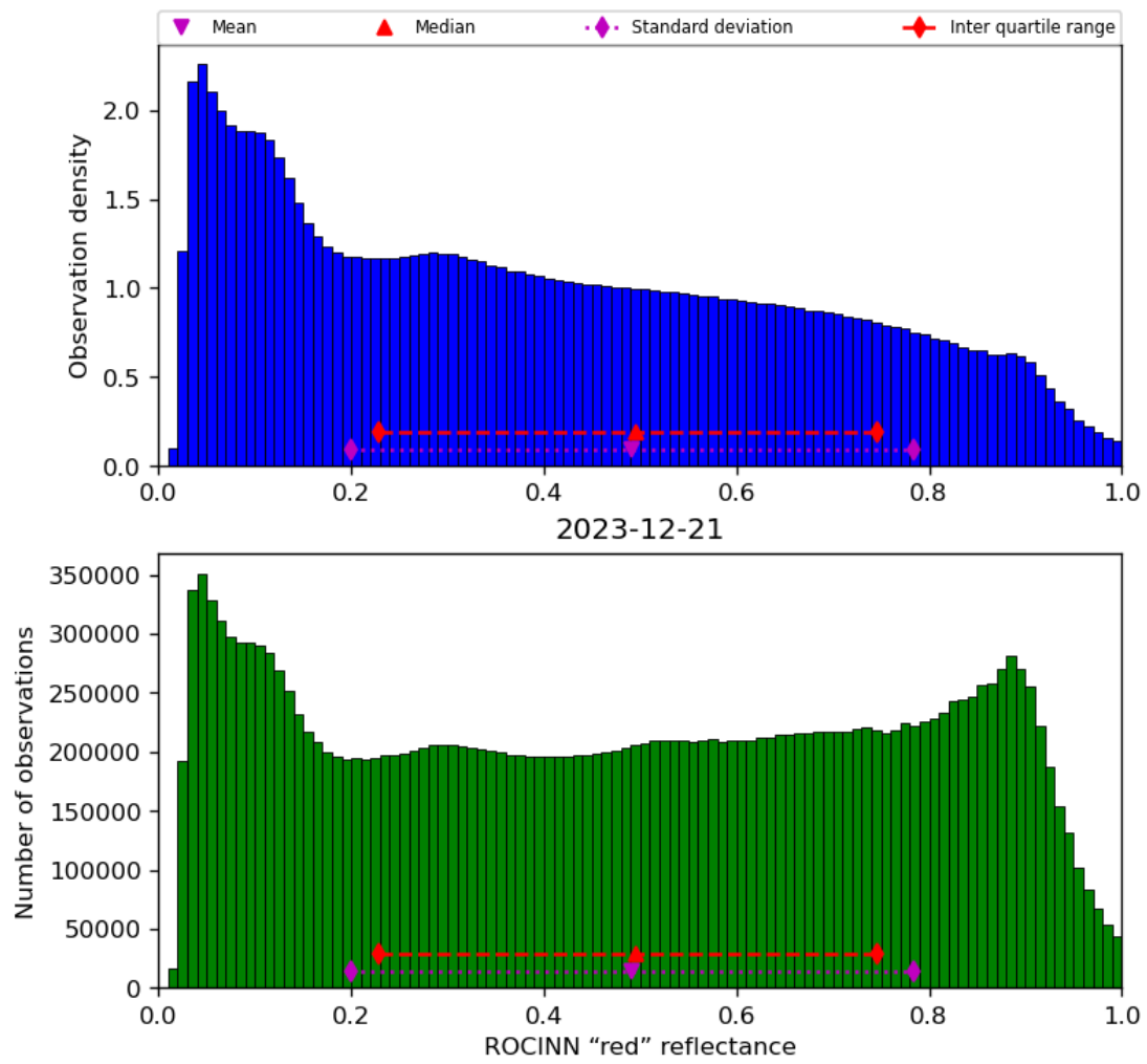
Figure 53: Histogram of “ROCINN “red” reflectance” for 2023-12-20 to 2023-12-22
