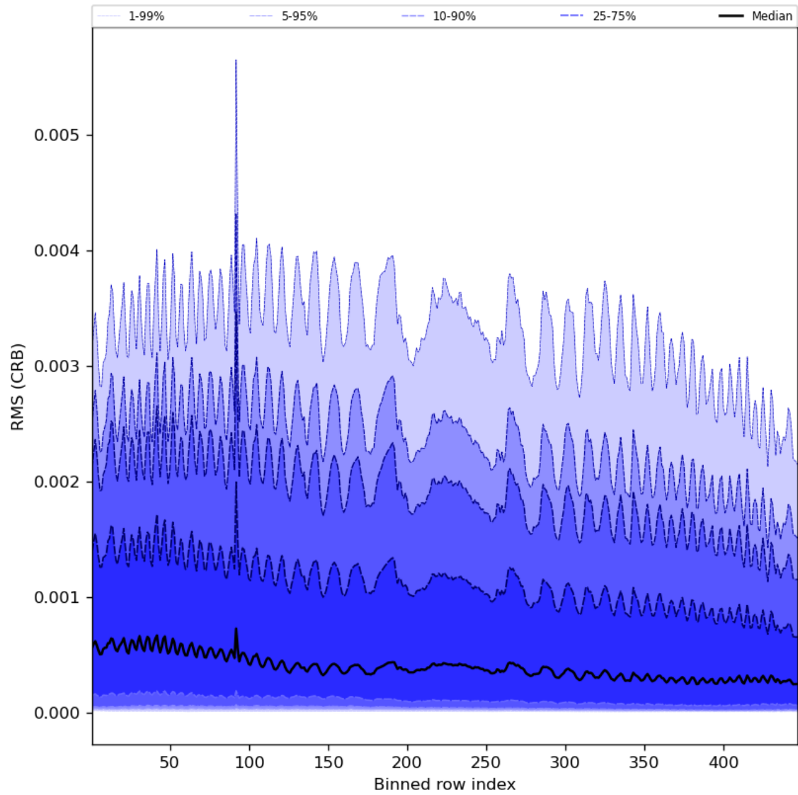
Figure 64: Along track statistics of “RMS (CRB)” for 2023-12-20 to 2023-12-22
