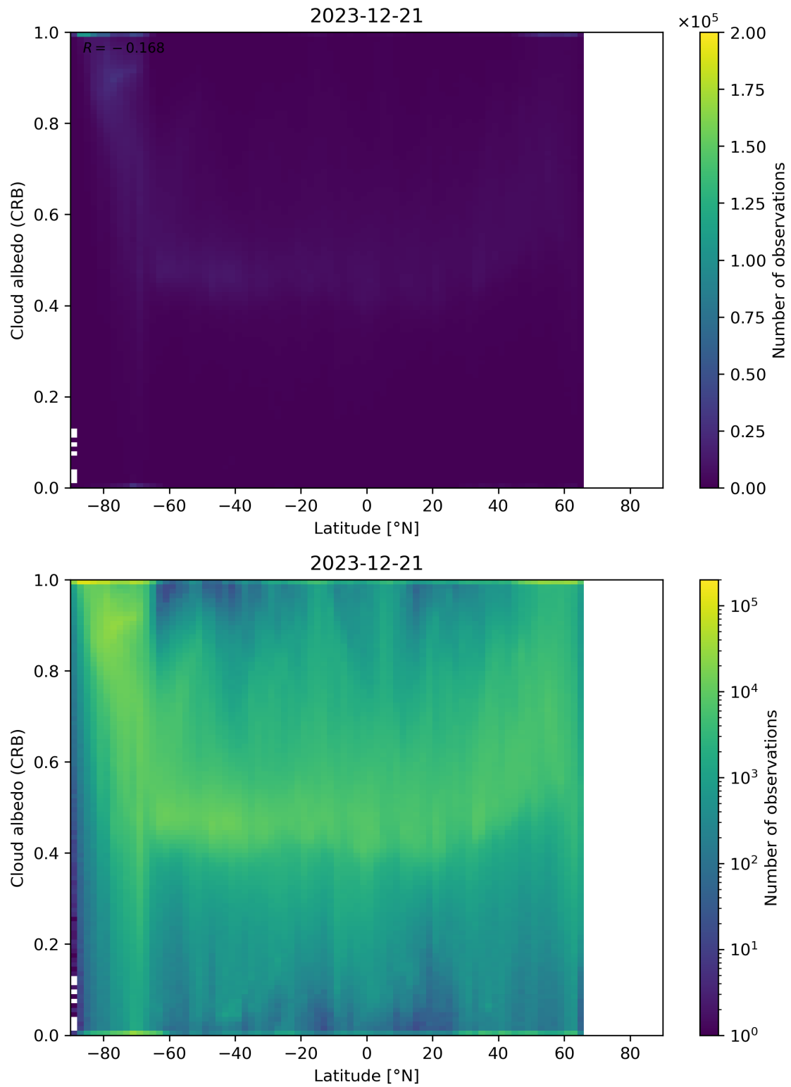
Figure 91: Scatter density plot of “Latitude” against “Cloud albedo (CRB)” for 2023-12-20 to 2023-12-22.
