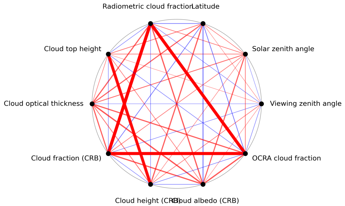
Figure 1: Map of correlation graph for 2023-12-20 to 2023-12-22.
