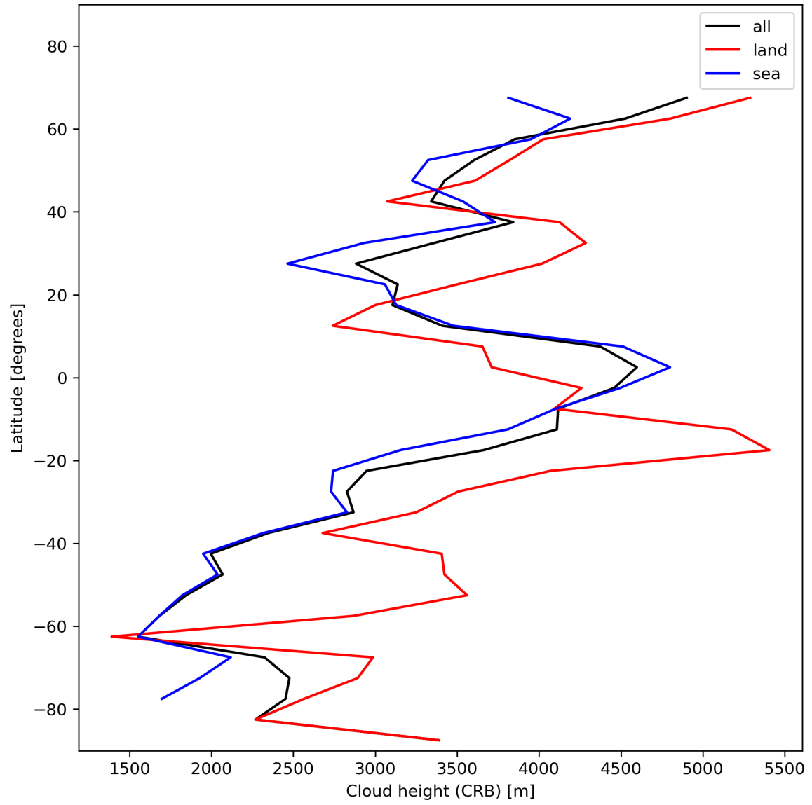
Figure 27: Zonal average of “Cloud height (CRB)” for 2023-12-20 to 2023-12-22.
