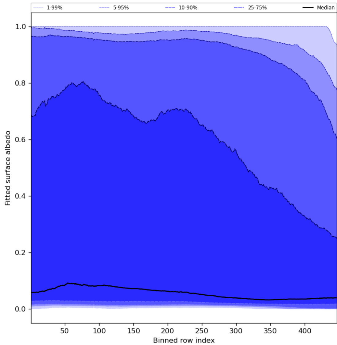
Figure 61: Along track statistics of “Fitted surface albedo” for 2023-12-20 to 2023-12-22
