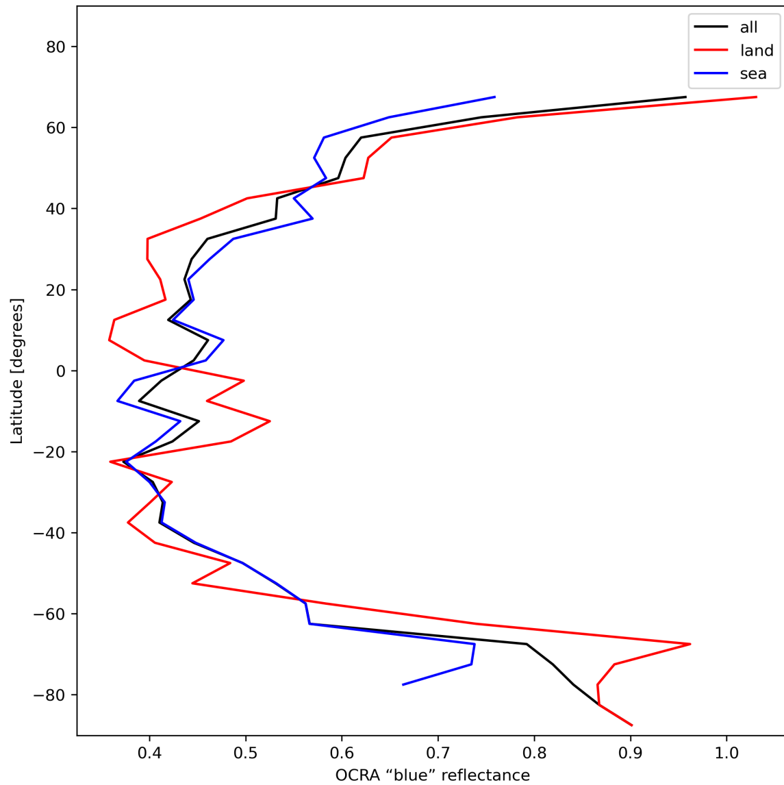
Figure 35: Zonal average of “OCRA “blue” reflectance” for 2023-12-20 to 2023-12-22.
