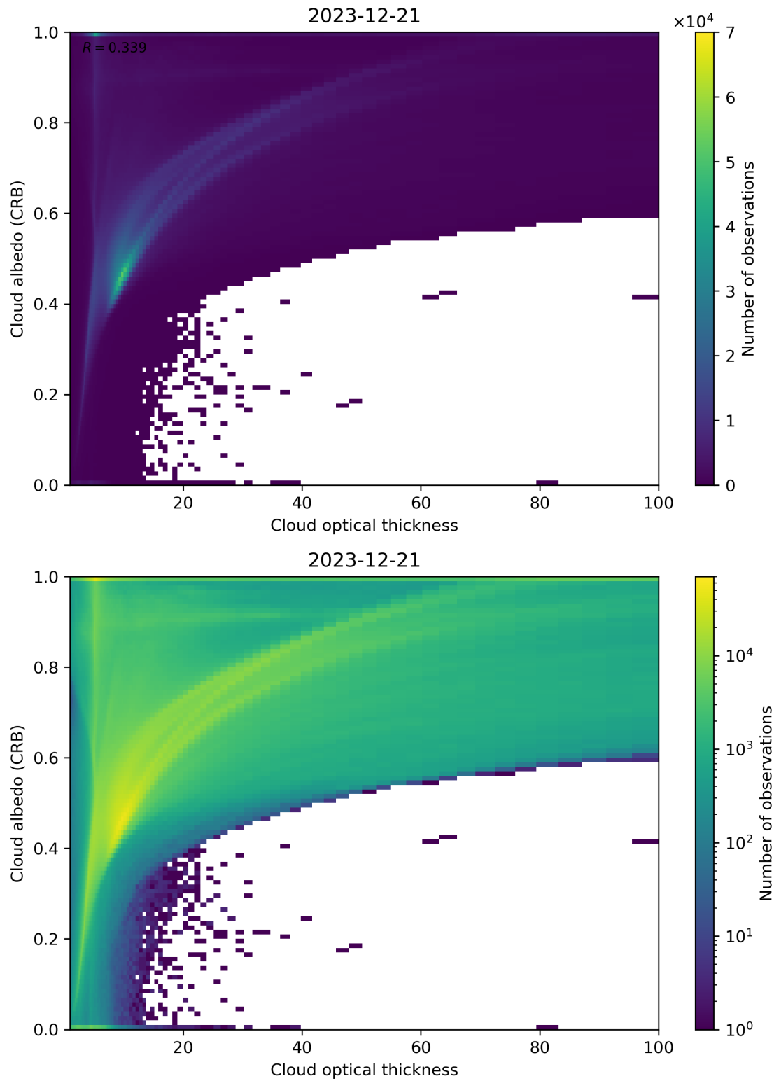
Figure 82: Scatter density plot of “Cloud optical thickness” against “Cloud albedo (CRB)” for 2023-12-20 to 2023-12-22.
