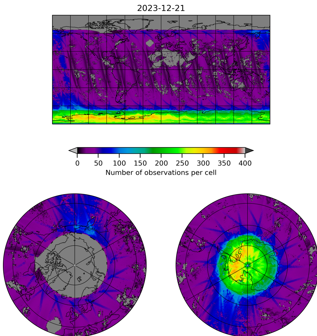
Figure 21: Map of the number of observations for 2023-12-20 to 2023-12-22
