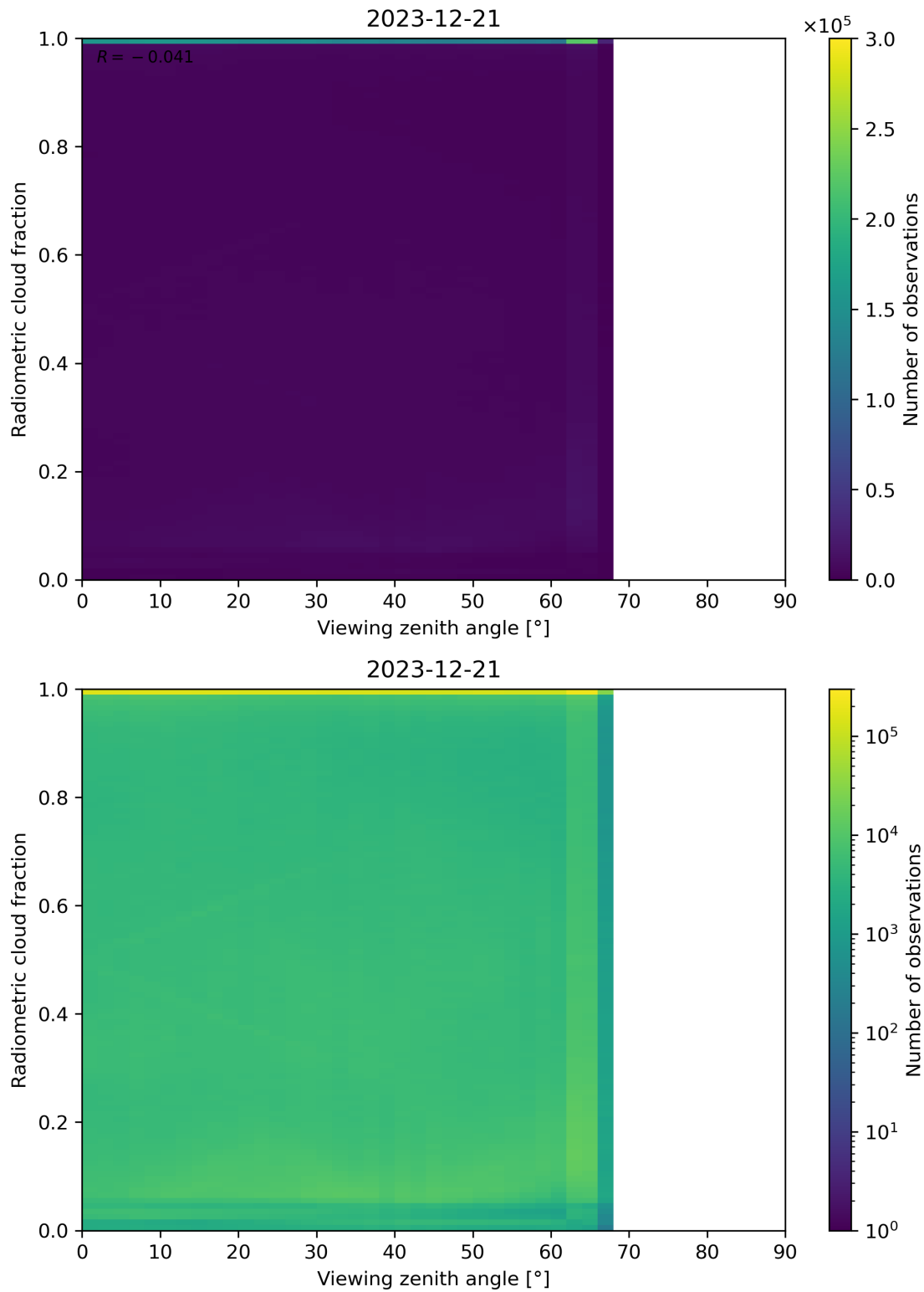
Figure 107: Scatter density plot of “Viewing zenith angle” against “Radiometric cloud fraction” for 2023-12-20 to 2023-12-22.
