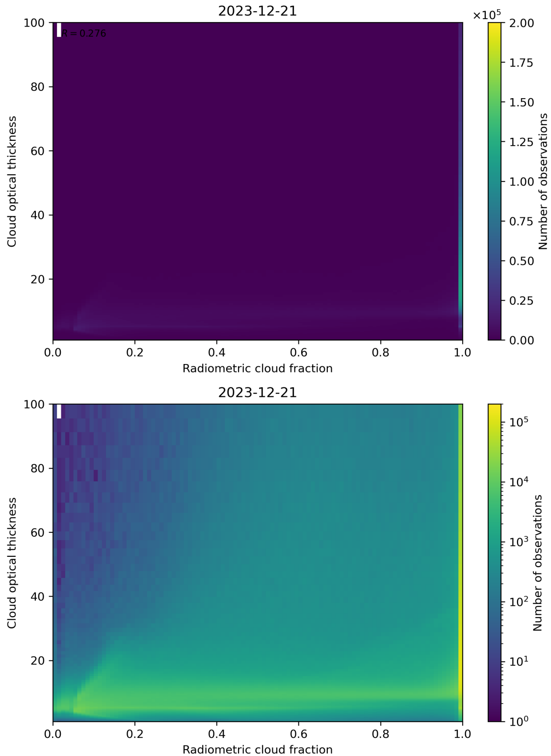
Figure 75: Scatter density plot of “Radiometric cloud fraction” against “Cloud optical thickness” for 2023-12-20 to 2023-12-22.
