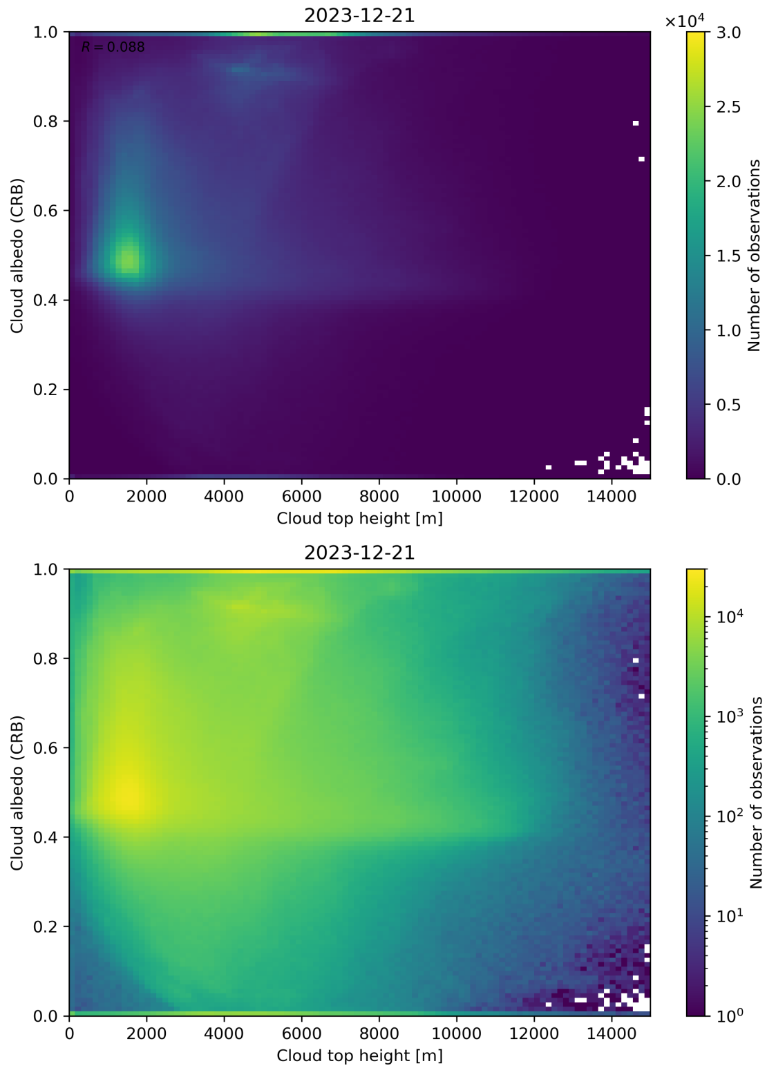
Figure 86: Scatter density plot of “Cloud top height” against “Cloud albedo (CRB)” for 2023-12-20 to 2023-12-22.
