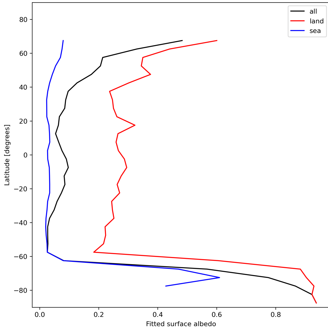
Figure 29: Zonal average of “Fitted surface albedo” for 2023-12-20 to 2023-12-22.
