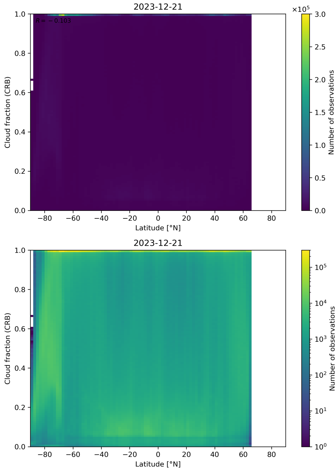
Figure 94: Scatter density plot of “Latitude” against “Cloud fraction (CRB)” for 2023-12-20 to 2023-12-22.
