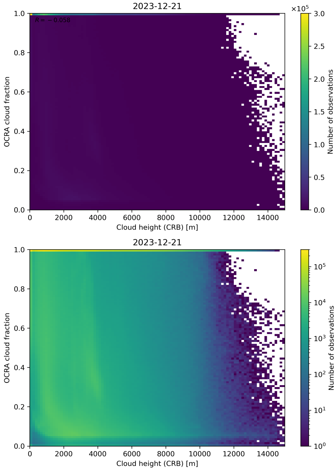
Figure 81: Scatter density plot of “Cloud height (CRB)” against “OCRA cloud fraction” for 2023-12-20 to 2023-12-22.
