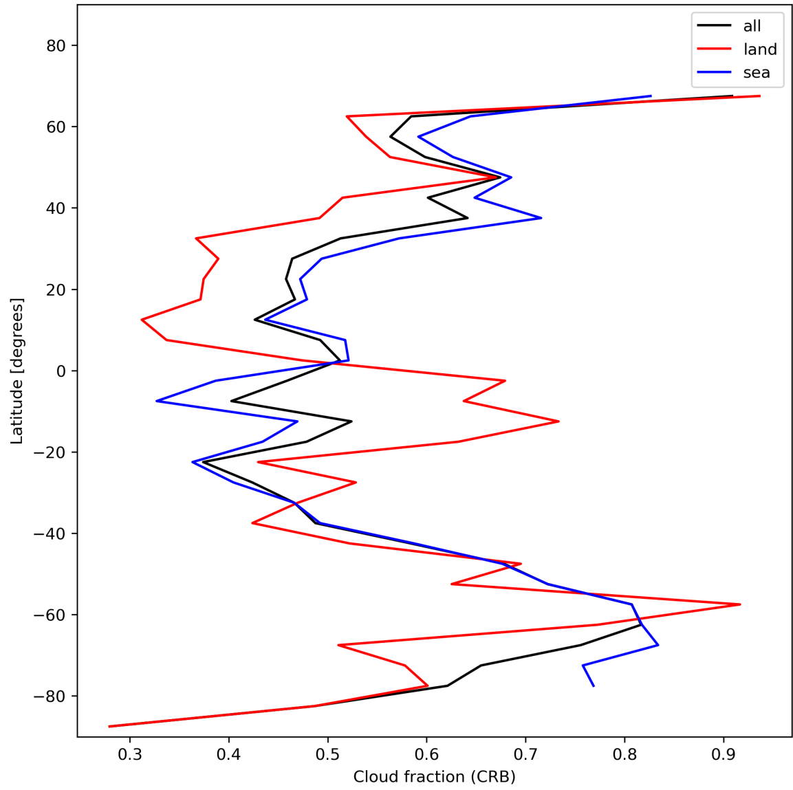
Figure 26: Zonal average of “Cloud fraction (CRB)” for 2023-12-20 to 2023-12-22.
