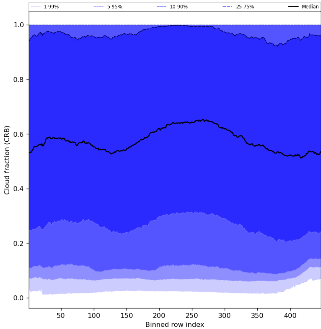
Figure 58: Along track statistics of “Cloud fraction (CRB)” for 2023-12-20 to 2023-12-22
