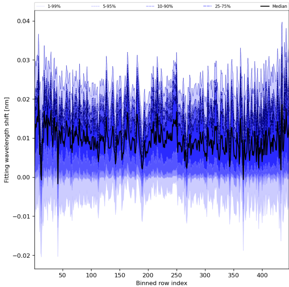
Figure 65: Along track statistics of “Fitting wavelength shift” for 2023-12-20 to 2023-12-22
