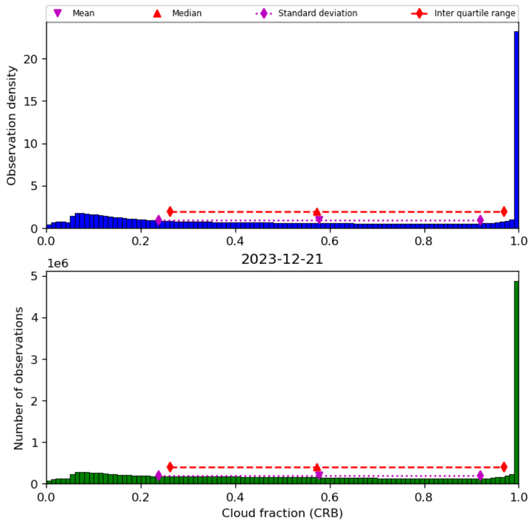
Figure 42: Histogram of “Cloud fraction (CRB)” for 2023-12-20 to 2023-12-22
