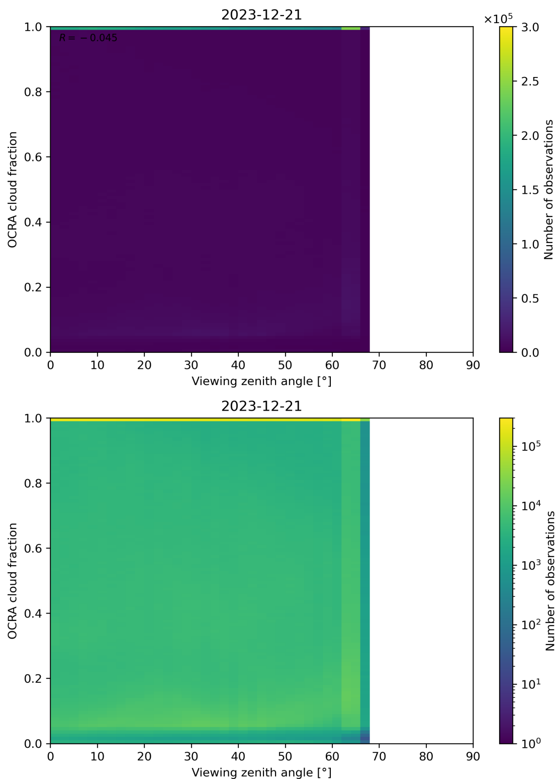
Figure 108: Scatter density plot of “Viewing zenith angle” against “OCRA cloud fraction” for 2023-12-20 to 2023-12-22.
