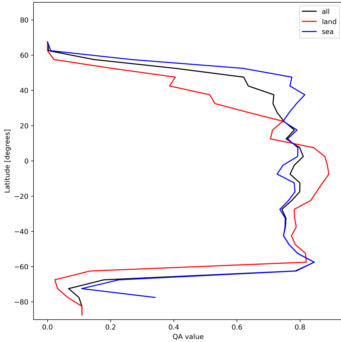
Figure 22: Zonal average of “QA value” for 2023-12-20 to 2023-12-22.
