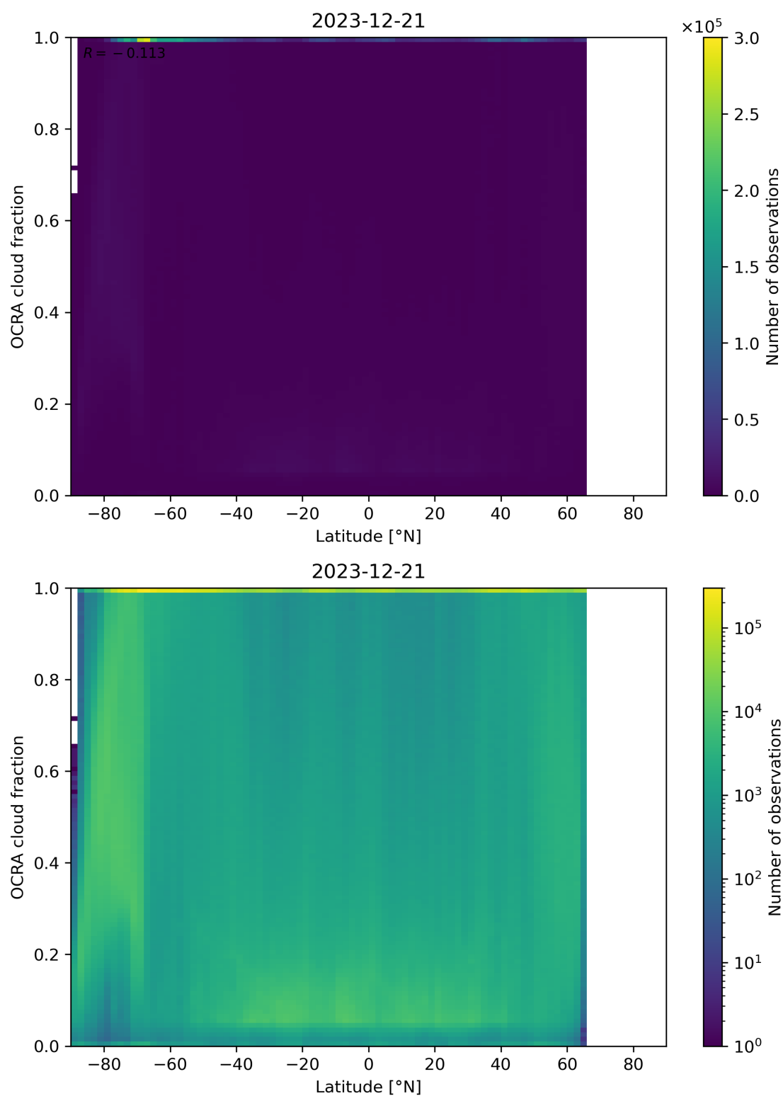
Figure 93: Scatter density plot of “Latitude” against “OCRA cloud fraction” for 2023-12-20 to 2023-12-22.
