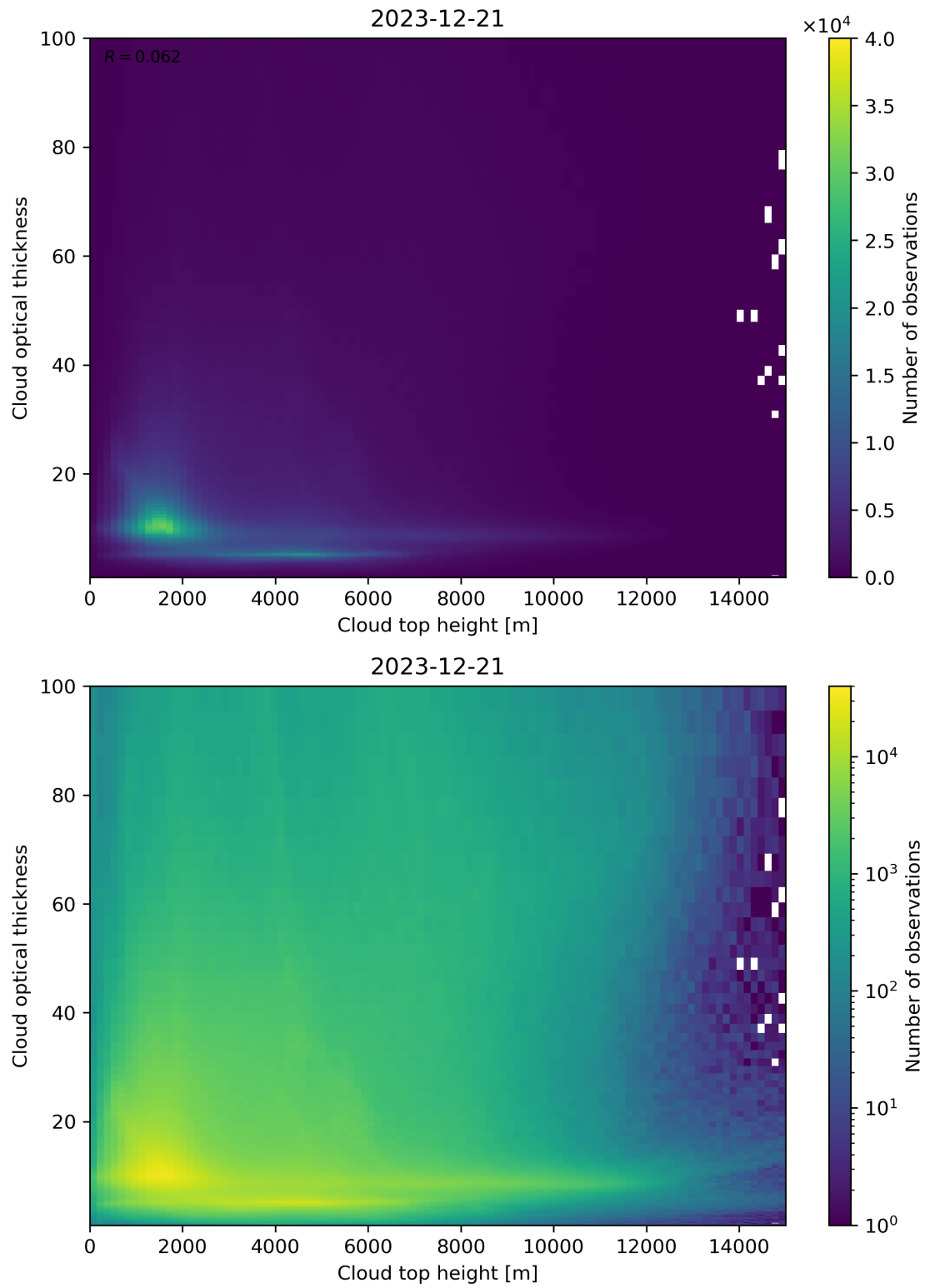
Figure 90: Scatter density plot of “Cloud top height” against “Cloud optical thickness” for 2023-12-20 to 2023-12-22.
