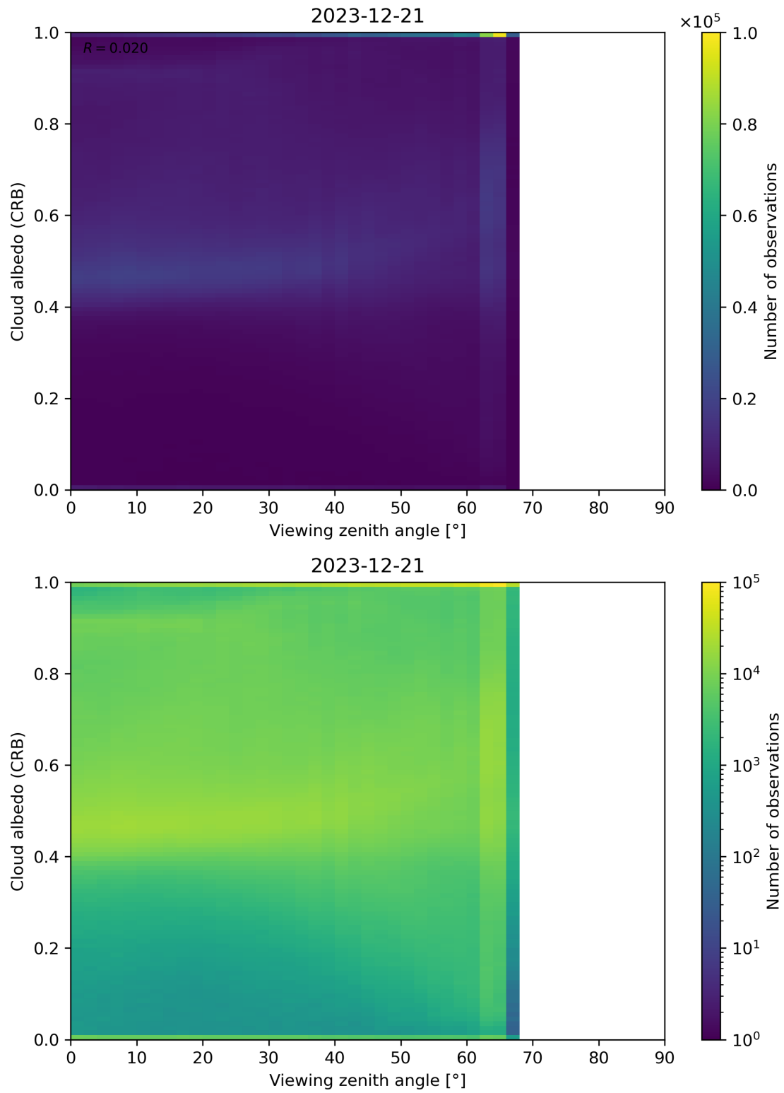
Figure 106: Scatter density plot of “Viewing zenith angle” against “Cloud albedo (CRB)” for 2023-12-20 to 2023-12-22.
