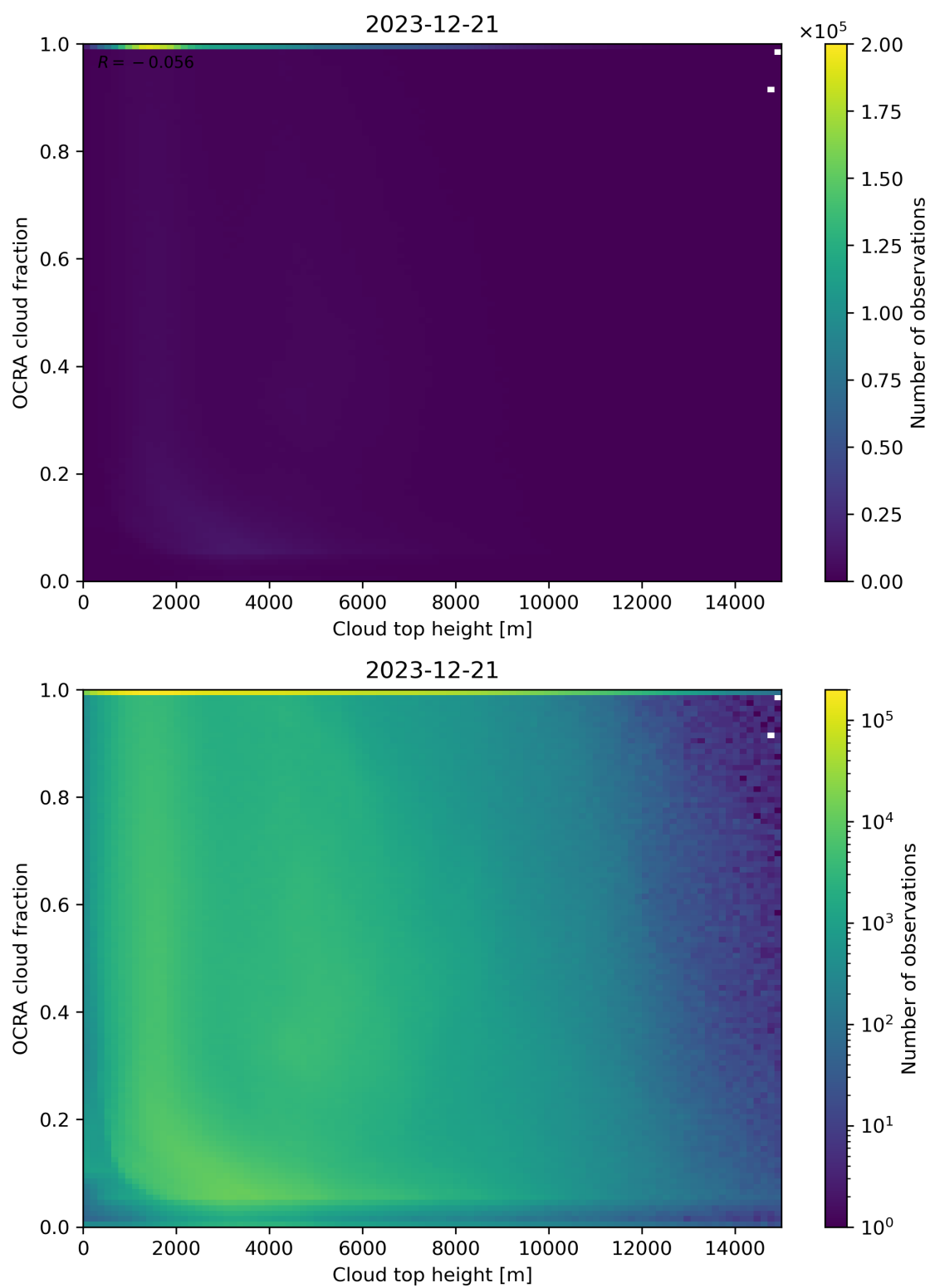
Figure 87: Scatter density plot of “Cloud top height” against “OCRA cloud fraction” for 2023-12-20 to 2023-12-22.
