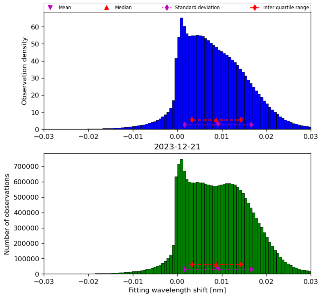
Figure 49: Histogram of “Fitting wavelength shift” for 2023-12-20 to 2023-12-22
