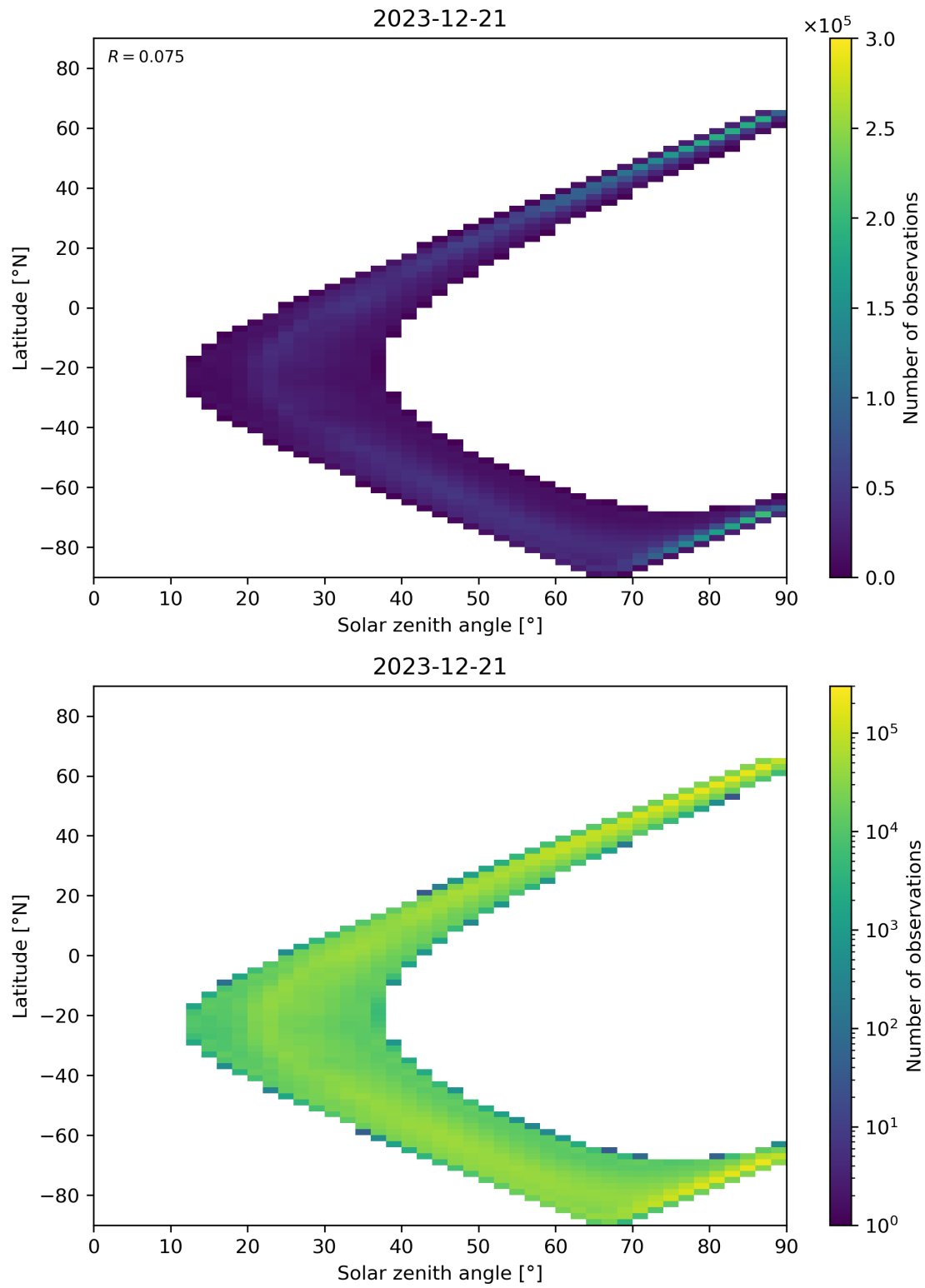
Figure 105: Scatter density plot of “Solar zenith angle” against “Latitude” for 2023-12-20 to 2023-12-22.
