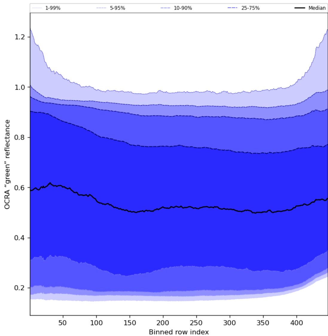
Figure 68: Along track statistics of “OCRA “green” reflectance” for 2023-12-20 to 2023-12-22
