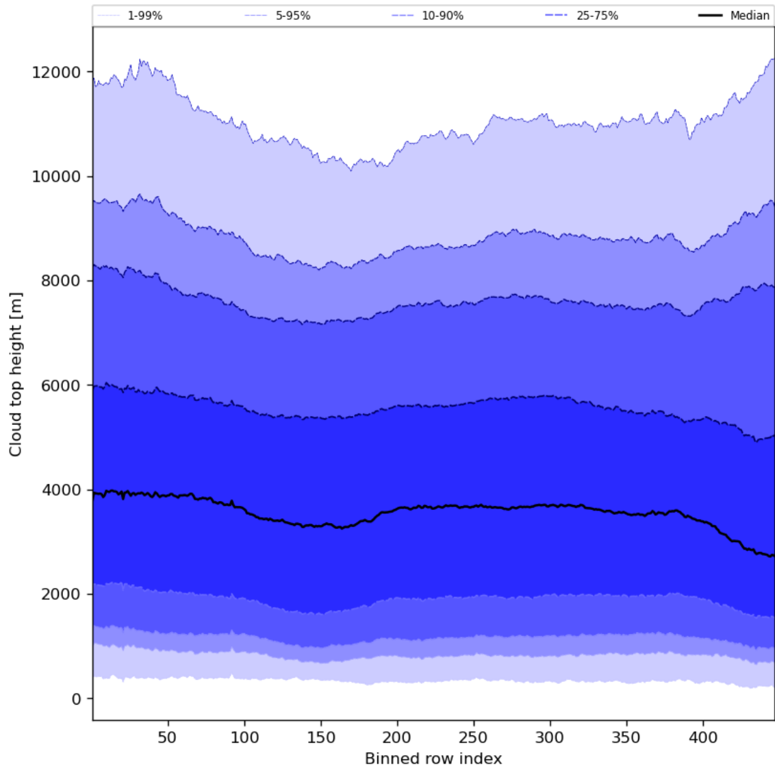
Figure 56: Along track statistics of “Cloud top height” for 2023-12-20 to 2023-12-22
