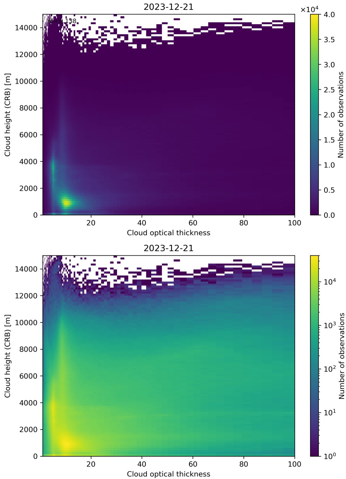
Figure 85: Scatter density plot of “Cloud optical thickness” against “Cloud height (CRB)” for 2023-12-20 to 2023-12-22.
