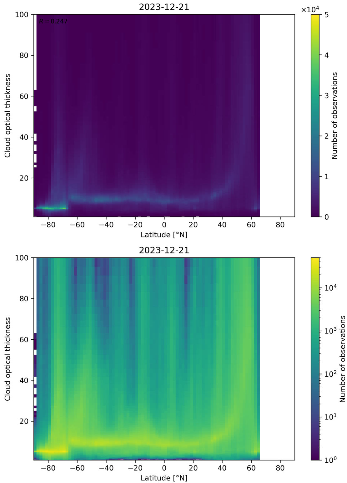
Figure 96: Scatter density plot of “Latitude” against “Cloud optical thickness” for 2023-12-20 to 2023-12-22.
