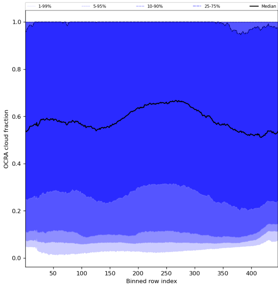
Figure 66: Along track statistics of “OCRA cloud fraction” for 2023-12-20 to 2023-12-22
