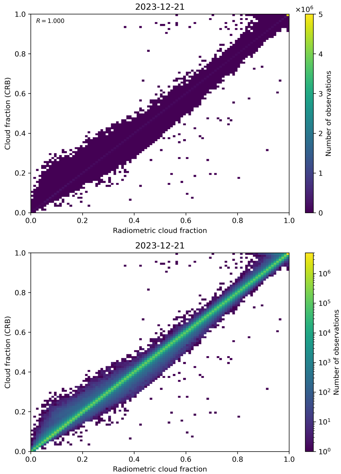
Figure 73: Scatter density plot of “Radiometric cloud fraction” against “Cloud fraction (CRB)” for 2023-12-20 to 2023-12-22.
