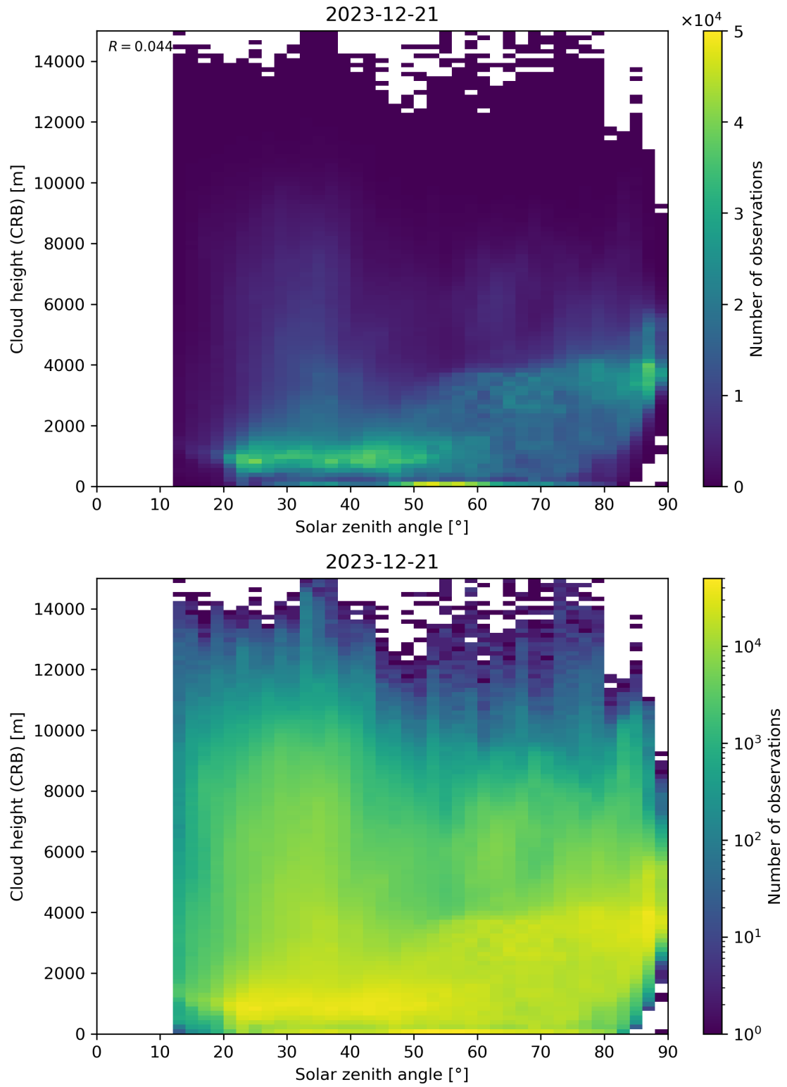
Figure 102: Scatter density plot of “Solar zenith angle” against “Cloud height (CRB)” for 2023-12-20 to 2023-12-22.
