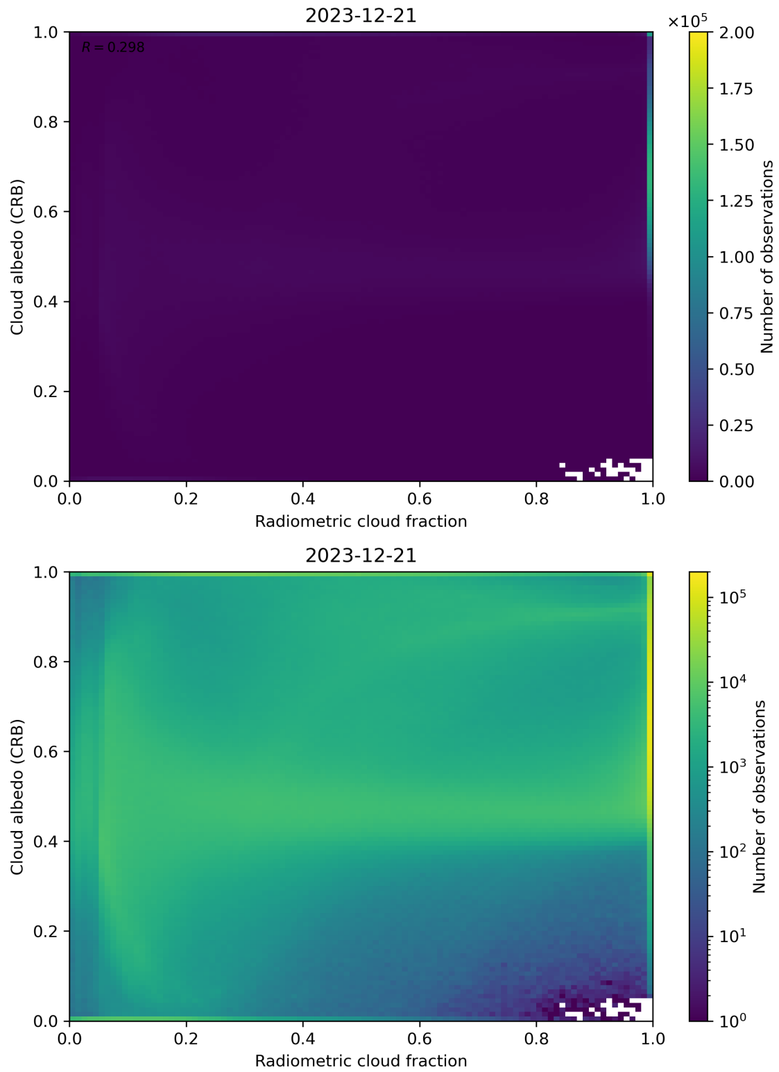
Figure 71: Scatter density plot of “Radiometric cloud fraction” against “Cloud albedo (CRB)” for 2023-12-20 to 2023-12-22.
