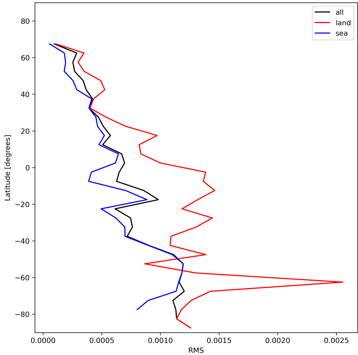
Figure 31: Zonal average of “RMS” for 2023-12-20 to 2023-12-22.
