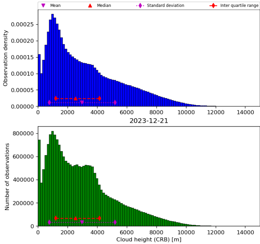
Figure 43: Histogram of “Cloud height (CRB)” for 2023-12-20 to 2023-12-22
