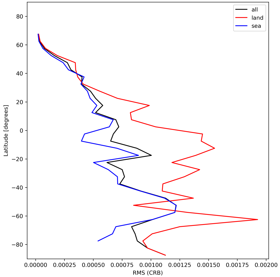
Figure 32: Zonal average of “RMS (CRB)” for 2023-12-20 to 2023-12-22.
