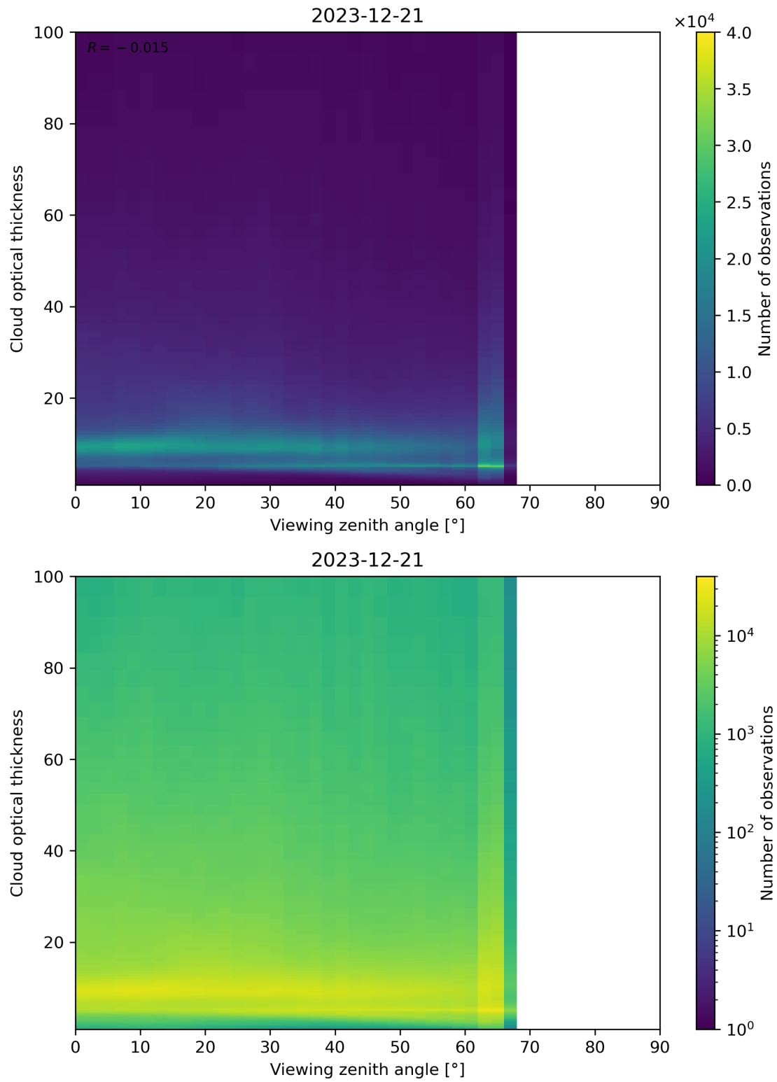
Figure 111: Scatter density plot of “Viewing zenith angle” against “Cloud optical thickness” for 2023-12-20 to 2023-12-22.
