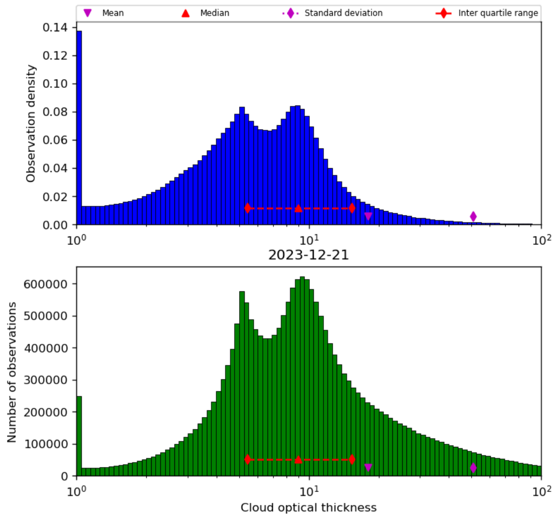
Figure 41: Histogram of “Cloud optical thickness” for 2023-12-20 to 2023-12-22
