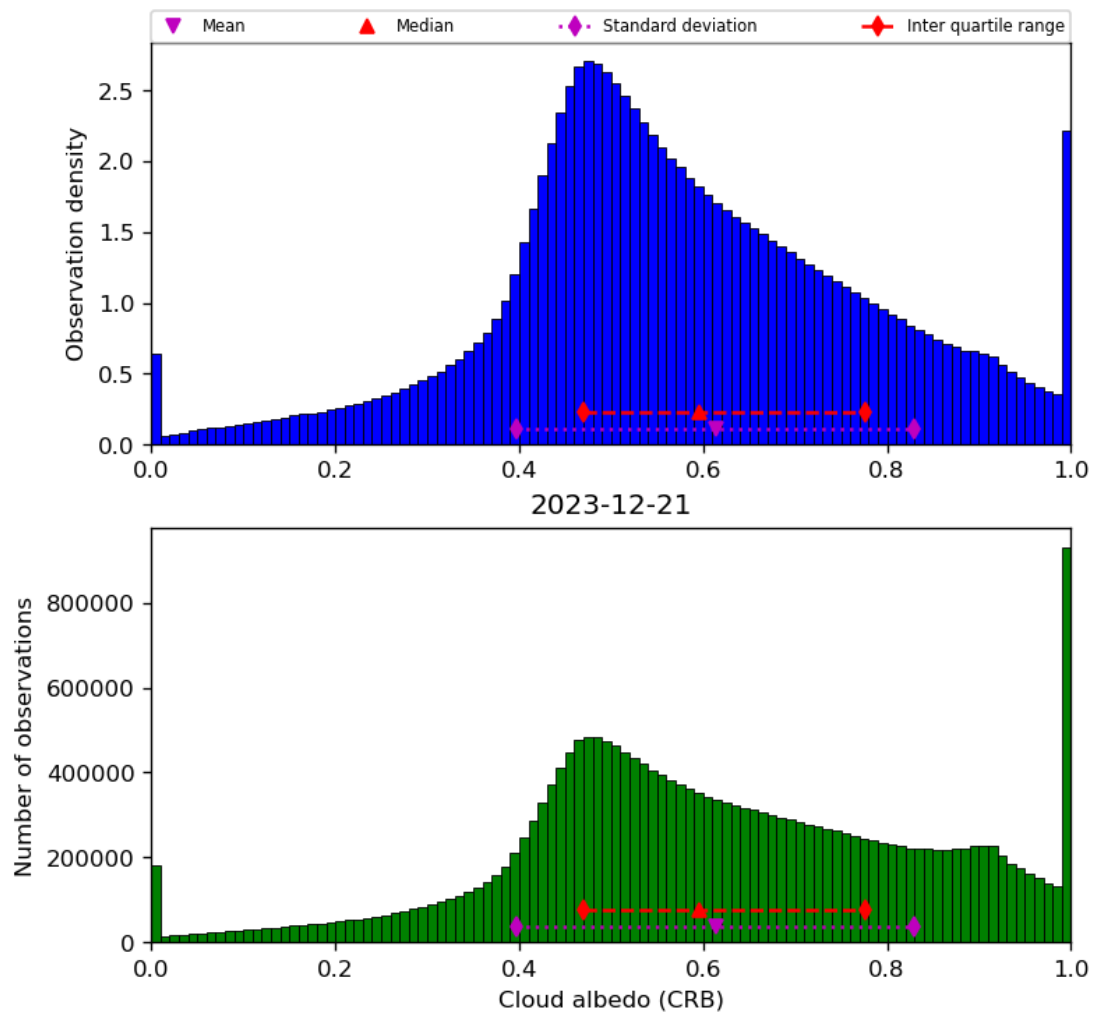
Figure 44: Histogram of “Cloud albedo (CRB)” for 2023-12-20 to 2023-12-22
