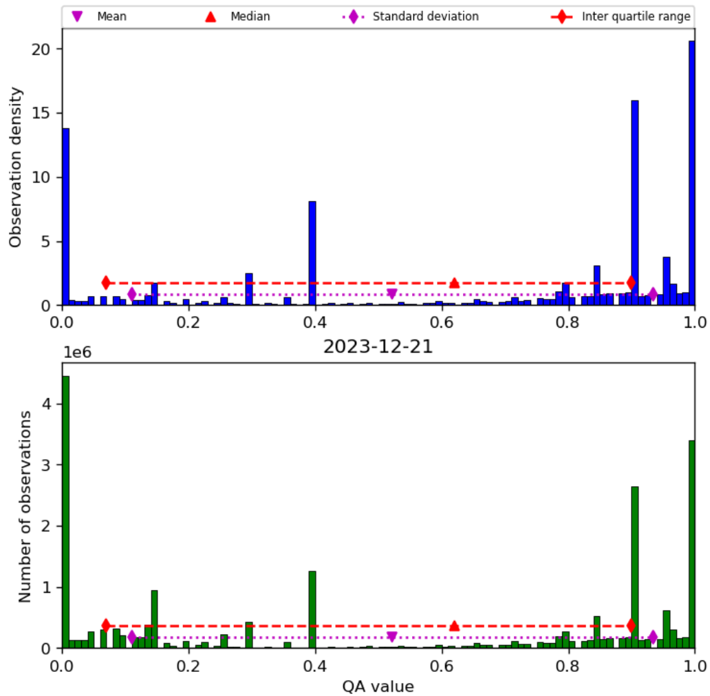
Figure 38: Histogram of “QA value” for 2023-12-20 to 2023-12-22
