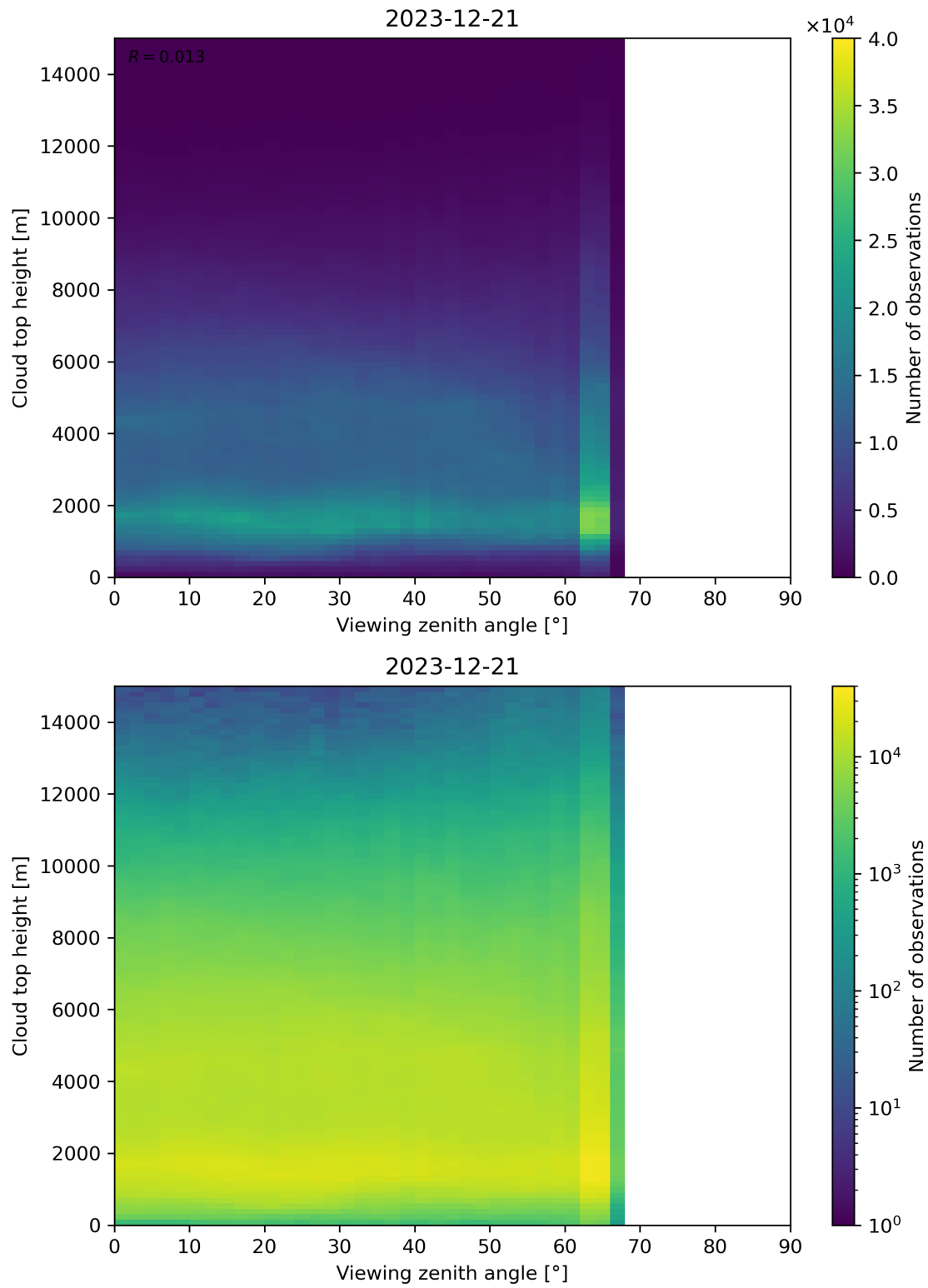
Figure 112: Scatter density plot of “Viewing zenith angle” against “Cloud top height” for 2023-12-20 to 2023-12-22.
