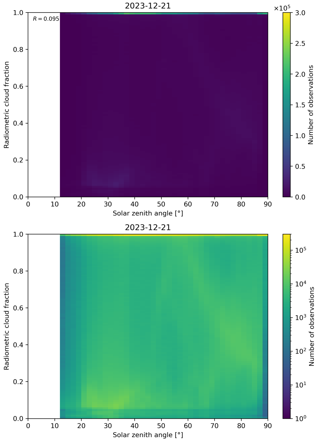
Figure 99: Scatter density plot of “Solar zenith angle” against “Radiometric cloud fraction” for 2023-12-20 to 2023-12-22.
