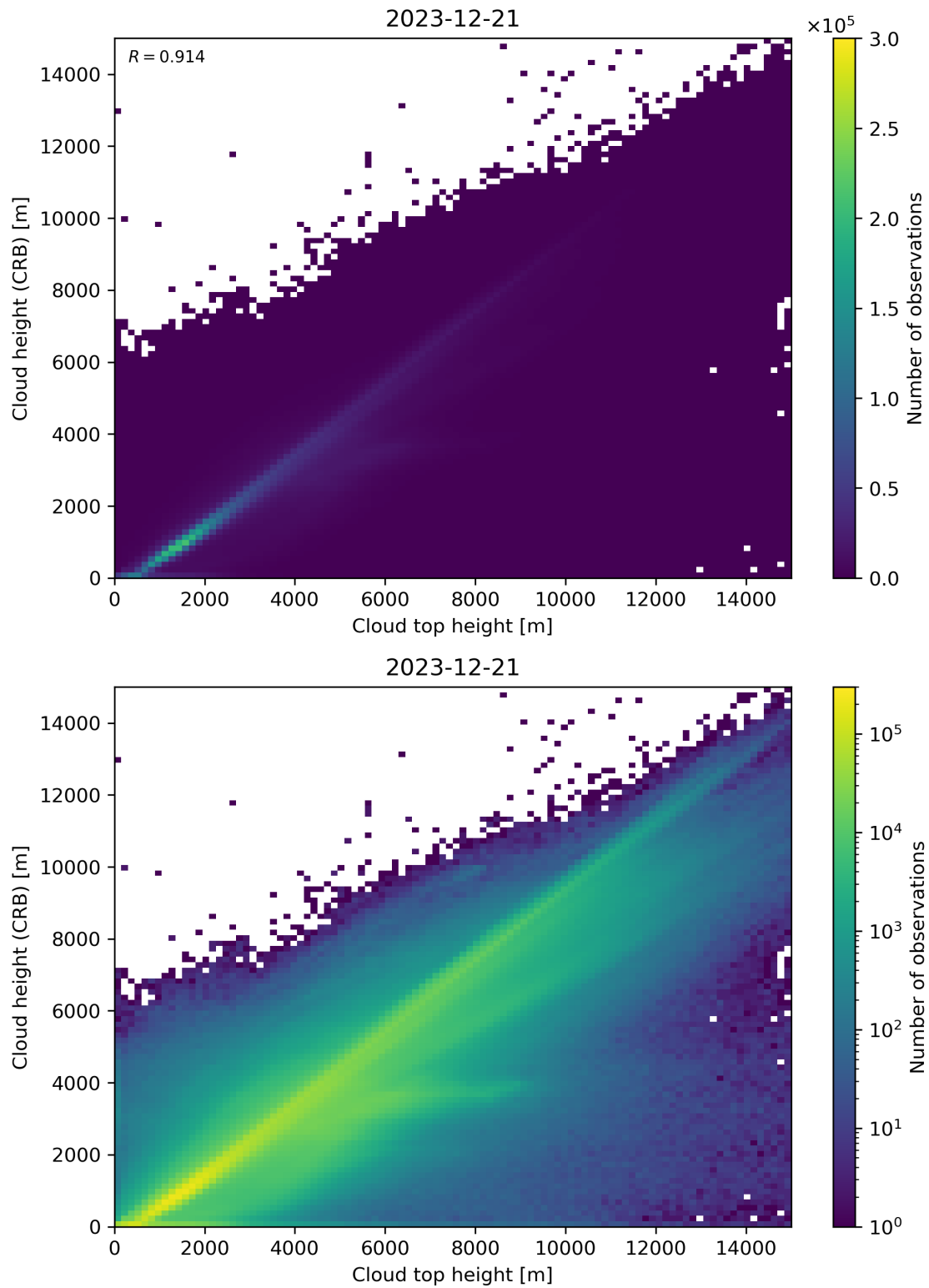
Figure 89: Scatter density plot of “Cloud top height” against “Cloud height (CRB)” for 2023-12-20 to 2023-12-22.
