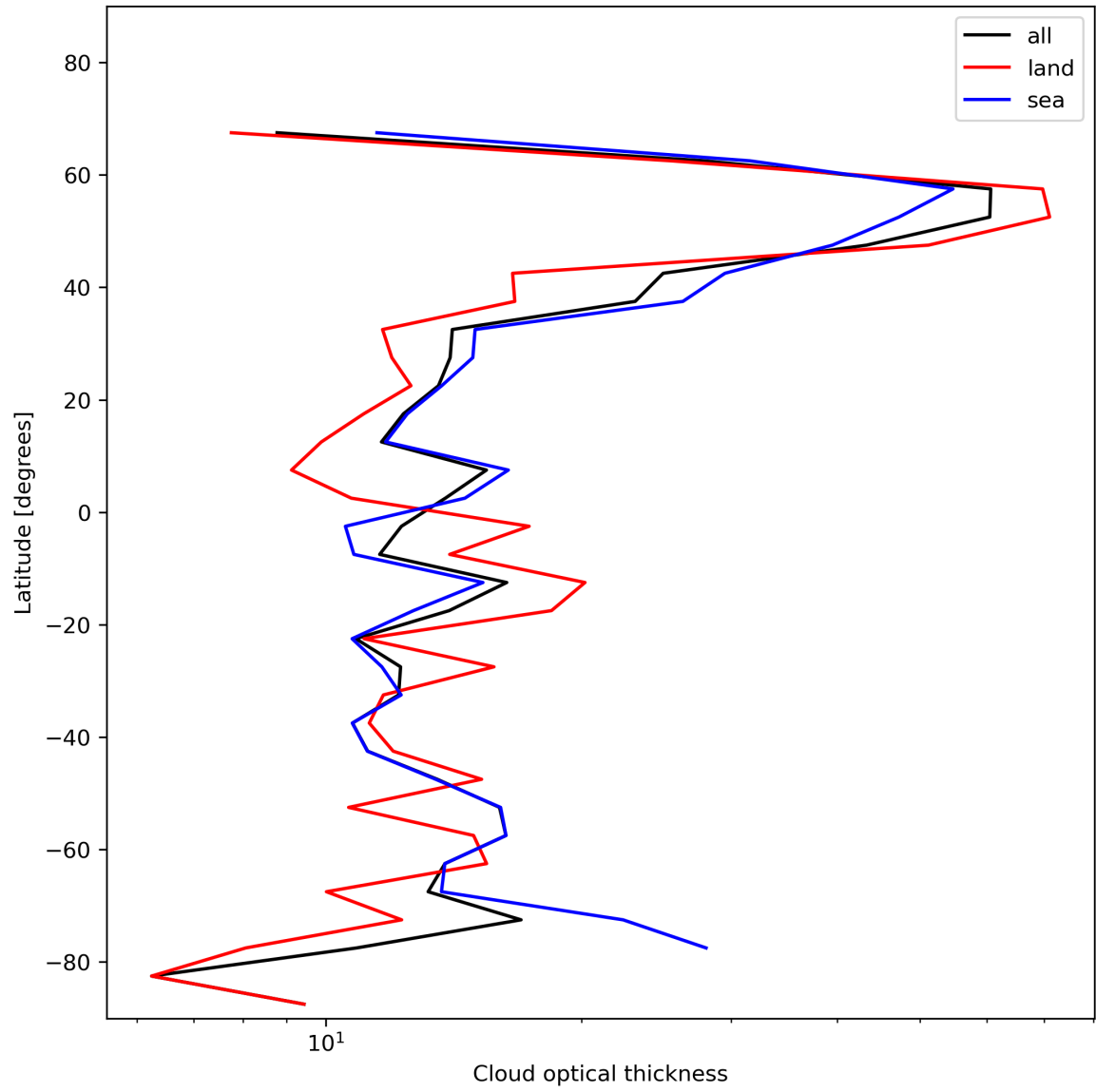
Figure 25: Zonal average of “Cloud optical thickness” for 2023-12-20 to 2023-12-22.
