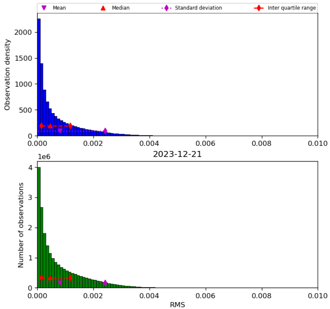
Figure 47: Histogram of “RMS” for 2023-12-20 to 2023-12-22
