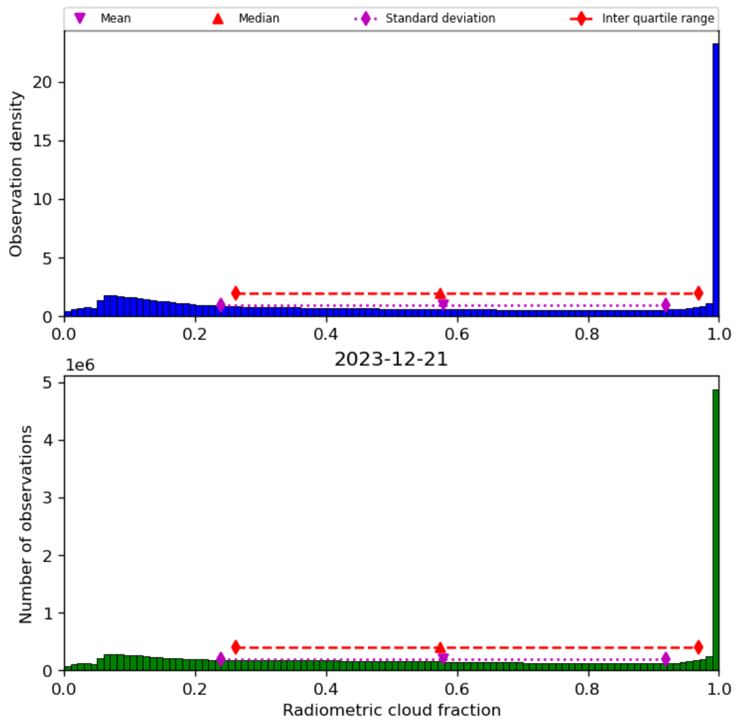
Figure 39: Histogram of “Radiometric cloud fraction” for 2023-12-20 to 2023-12-22
