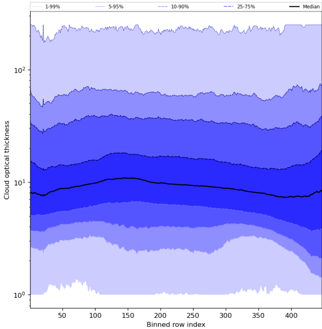
Figure 57: Along track statistics of “Cloud optical thickness” for 2023-12-20 to 2023-12-22
