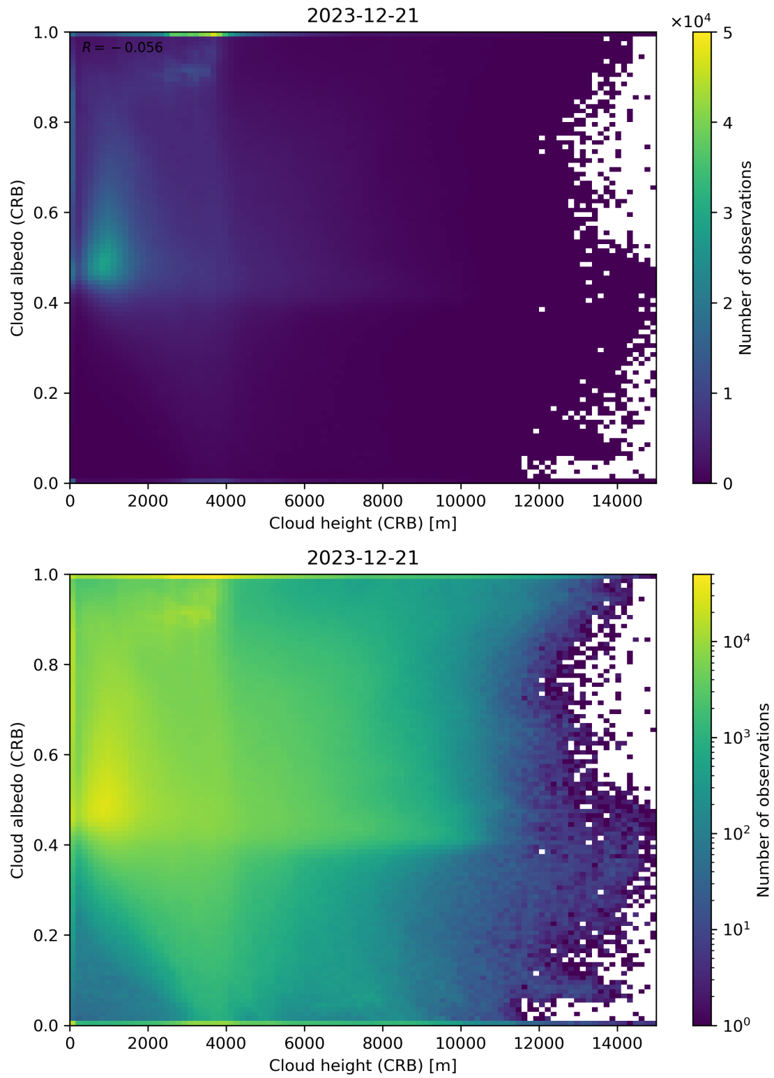
Figure 80: Scatter density plot of “Cloud height (CRB)” against “Cloud albedo (CRB)” for 2023-12-20 to 2023-12-22.
