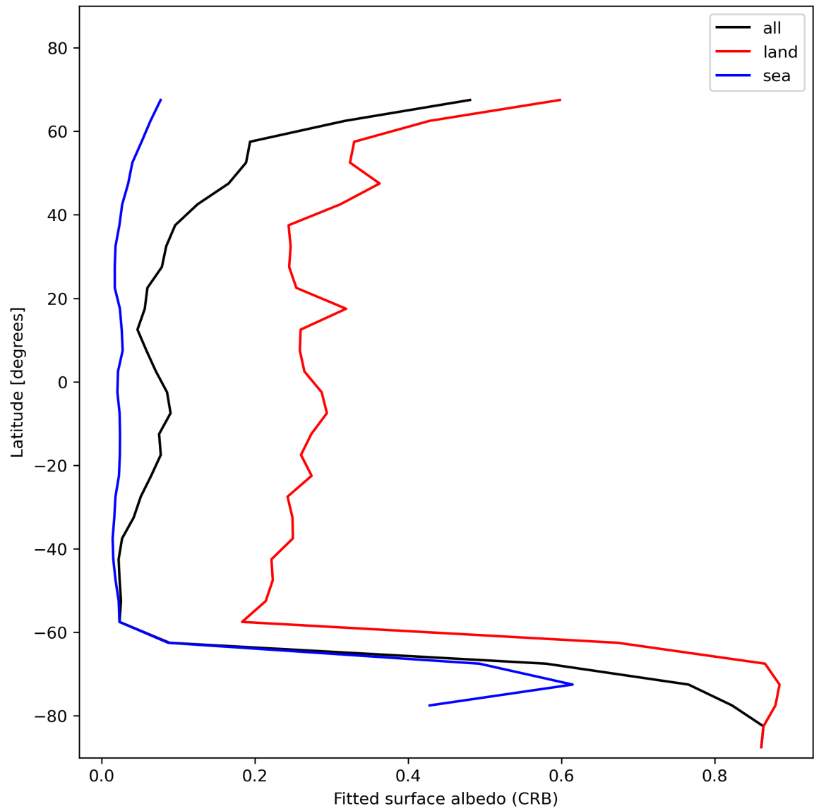
Figure 30: Zonal average of “Fitted surface albedo (CRB)” for 2023-12-20 to 2023-12-22.
