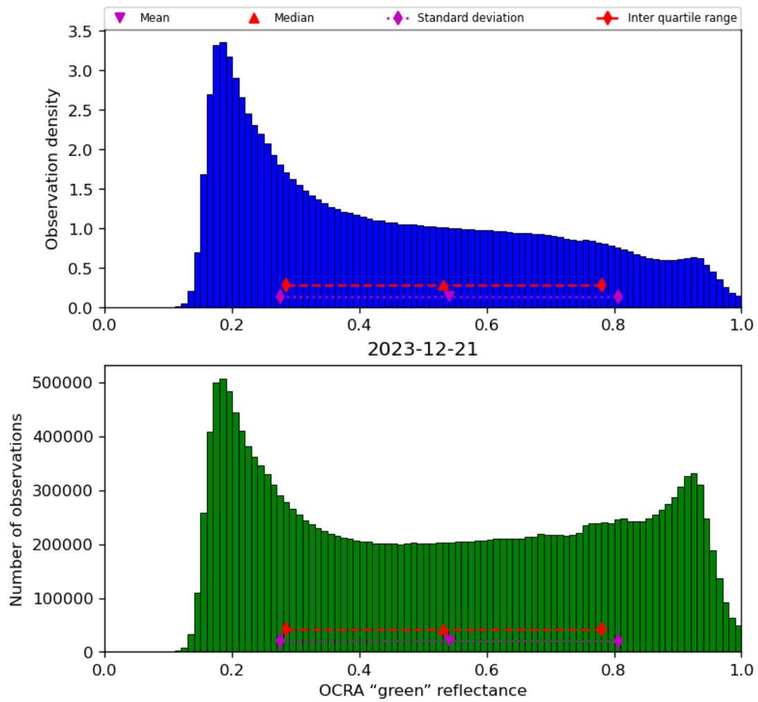
Figure 52: Histogram of “OCRA “green” reflectance” for 2023-12-20 to 2023-12-22
