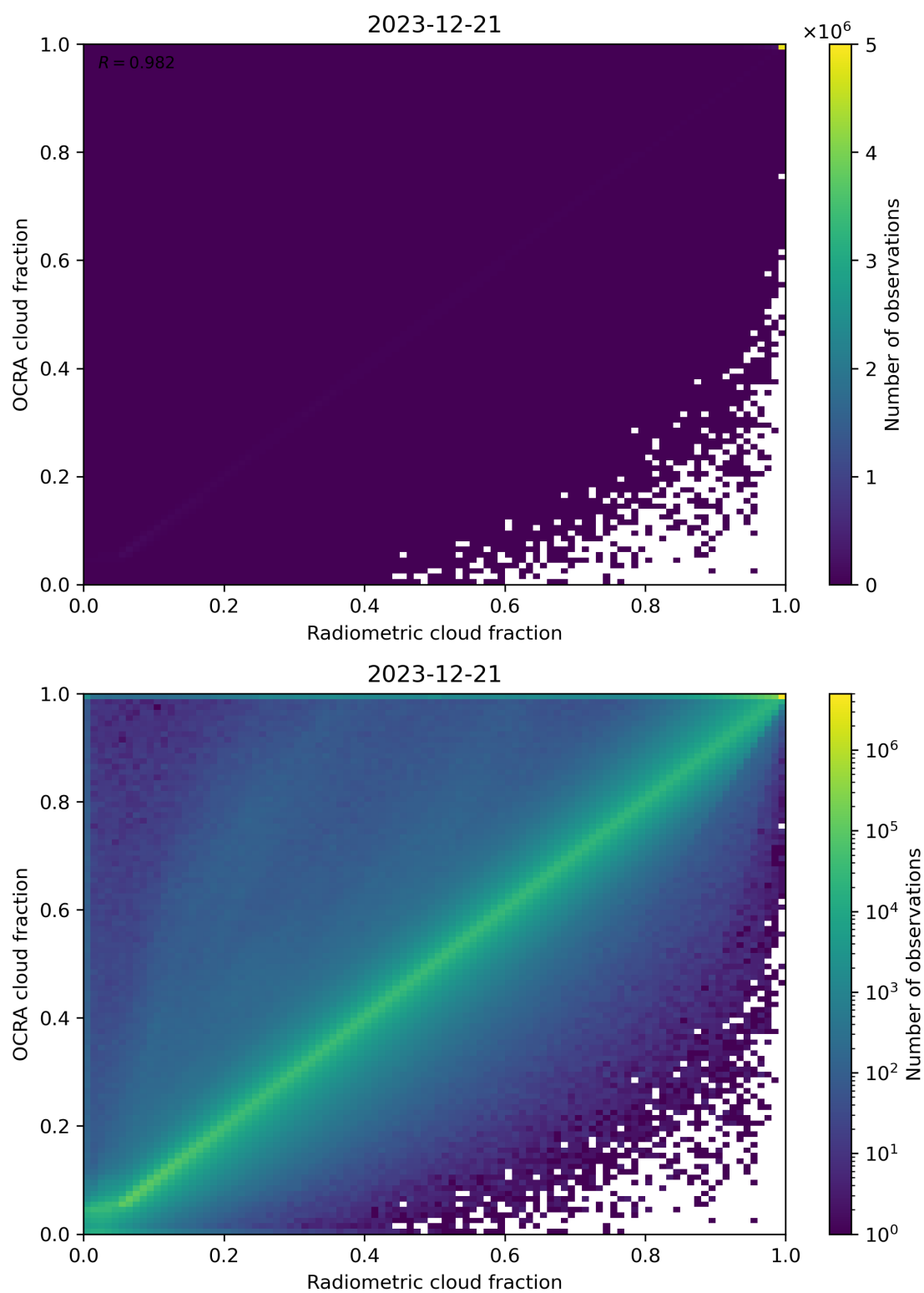
Figure 72: Scatter density plot of “Radiometric cloud fraction” against “OCRA cloud fraction” for 2023-12-20 to 2023-12-22.
