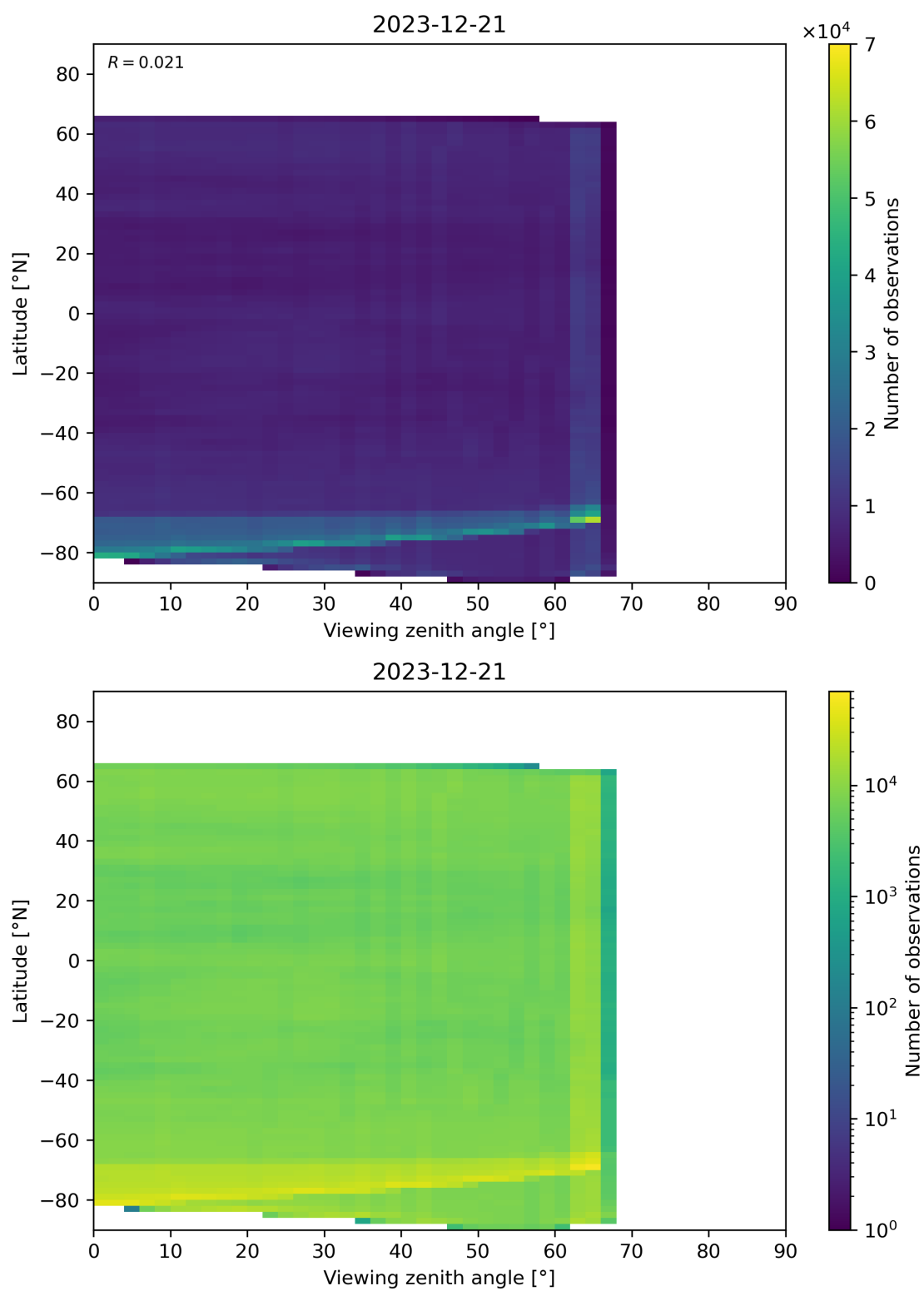
Figure 113: Scatter density plot of “Viewing zenith angle” against “Latitude” for 2023-12-20 to 2023-12-22.
