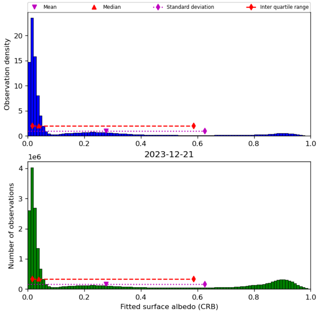
Figure 46: Histogram of “Fitted surface albedo (CRB)” for 2023-12-20 to 2023-12-22
