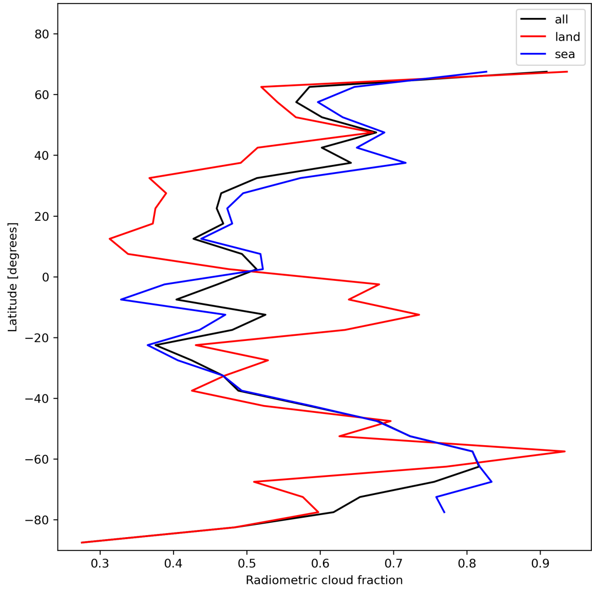
Figure 23: Zonal average of “Radiometric cloud fraction” for 2023-12-20 to 2023-12-22.
