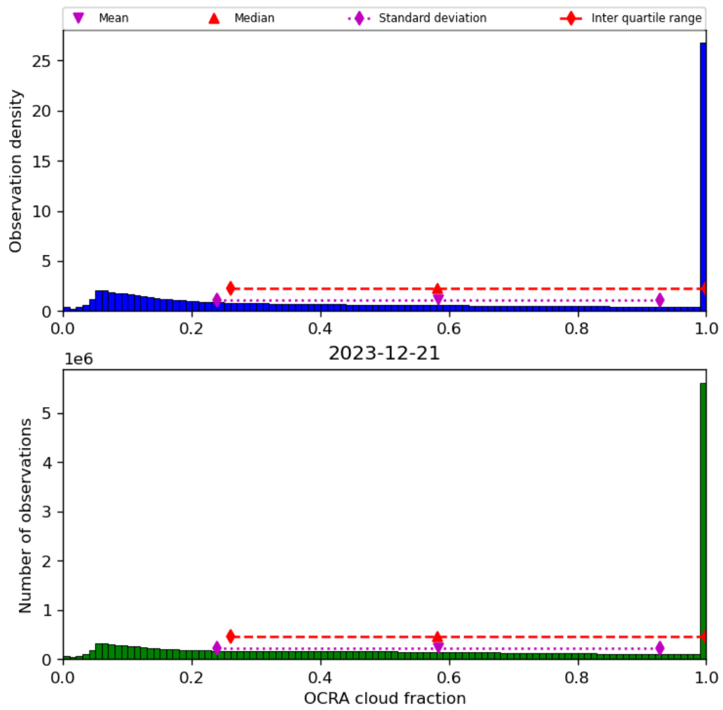
Figure 50: Histogram of “OCRA cloud fraction” for 2023-12-20 to 2023-12-22
