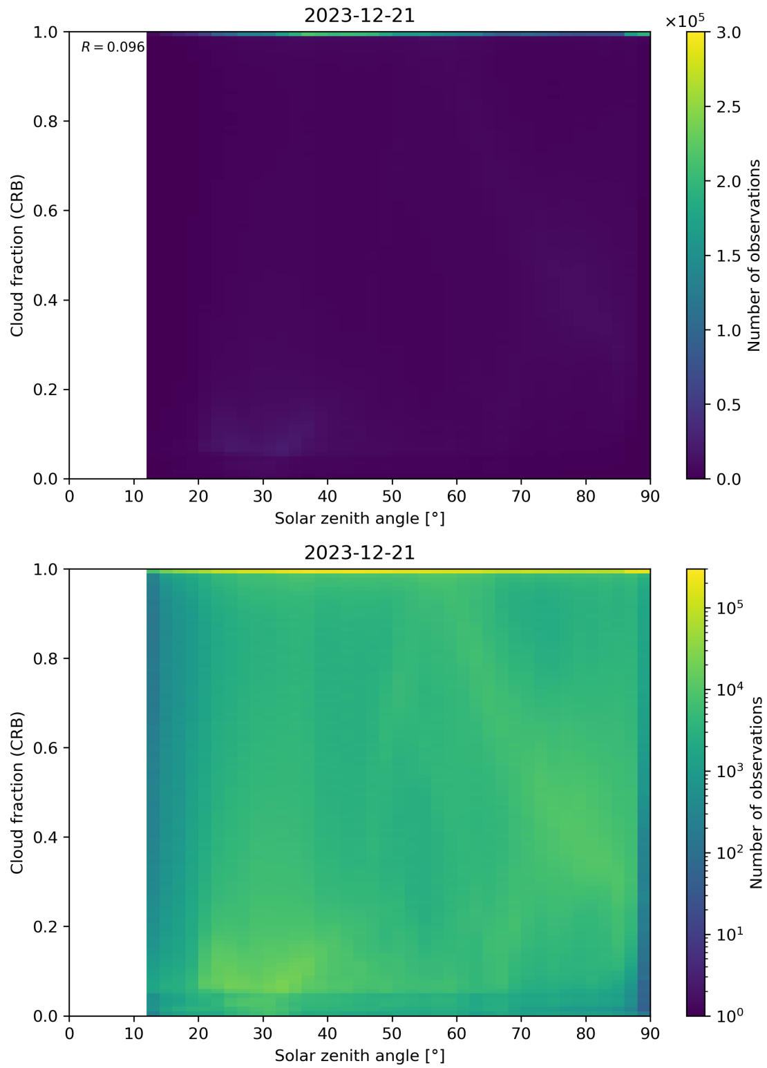
Figure 101: Scatter density plot of “Solar zenith angle” against “Cloud fraction (CRB)” for 2023-12-20 to 2023-12-22.
