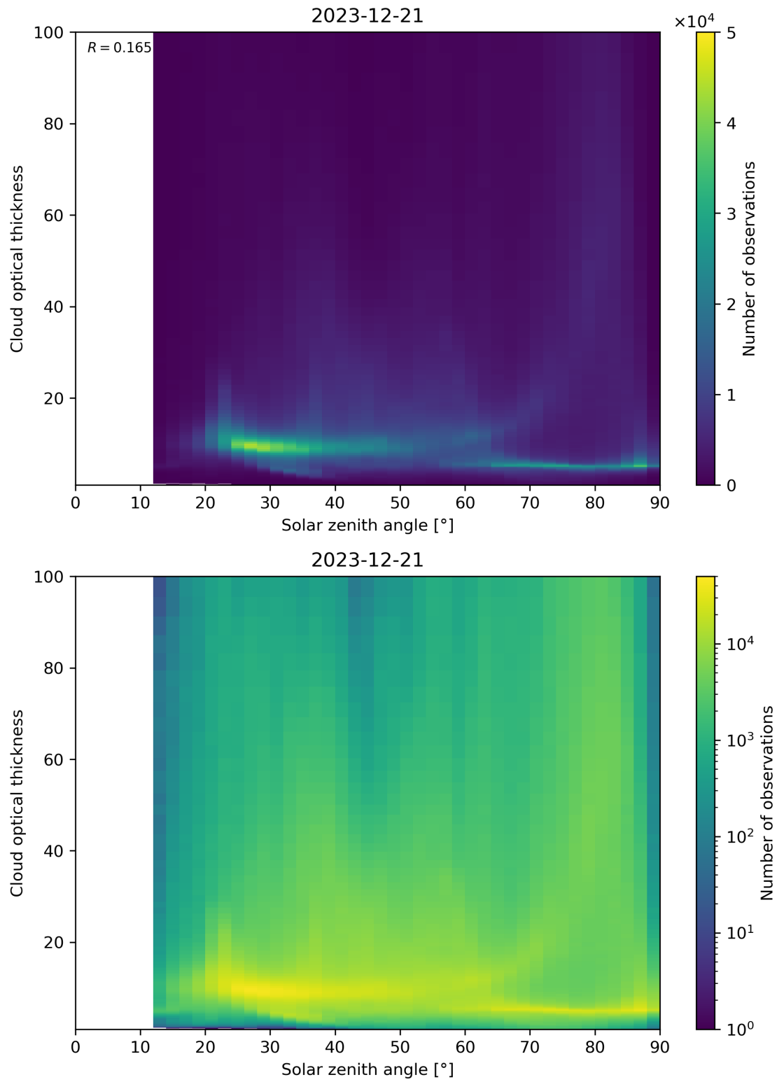
Figure 103: Scatter density plot of “Solar zenith angle” against “Cloud optical thickness” for 2023-12-20 to 2023-12-22.
