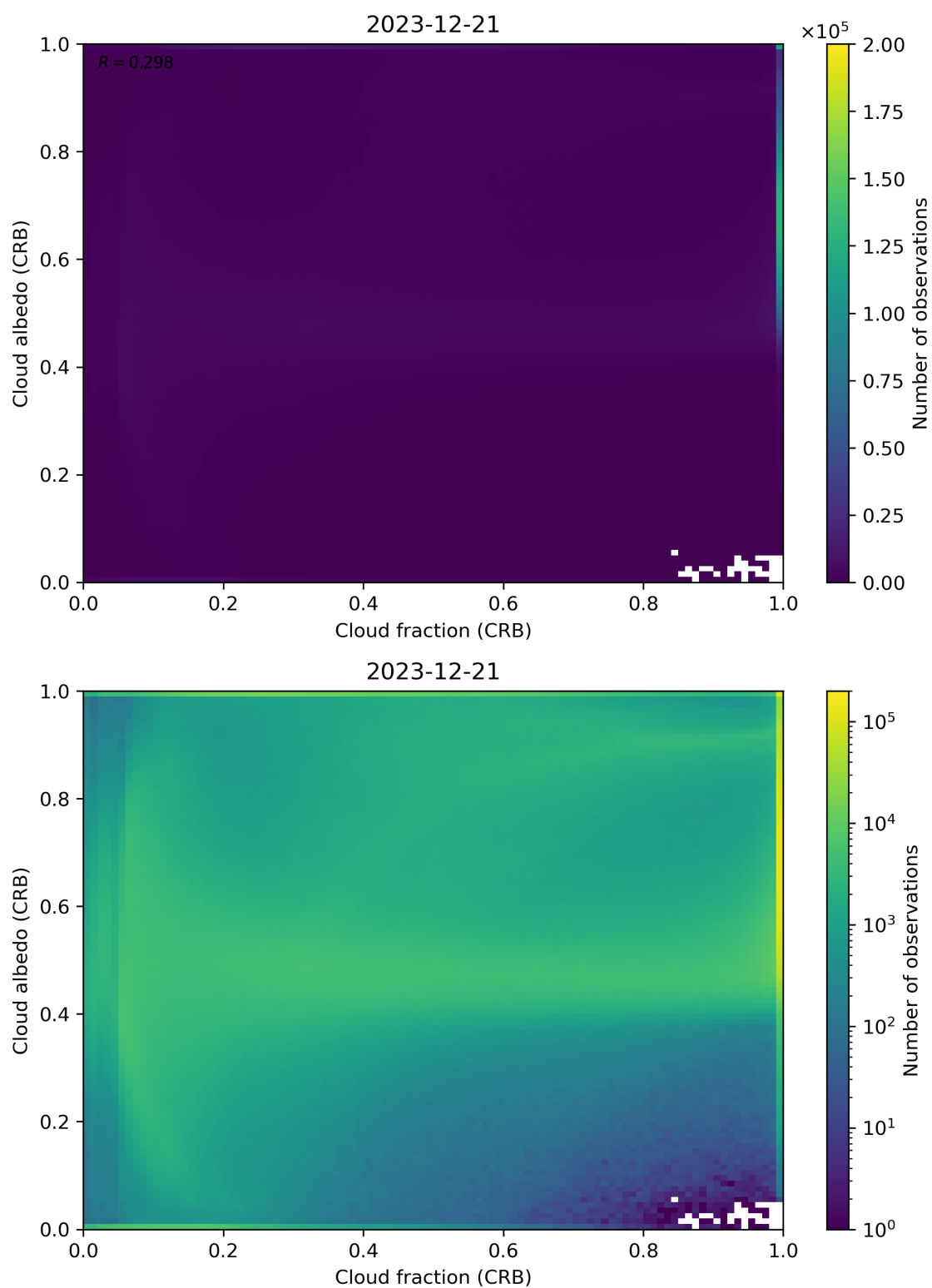
Figure 77: Scatter density plot of “Cloud fraction (CRB)” against “Cloud albedo (CRB)” for 2023-12-20 to 2023-12-22.
