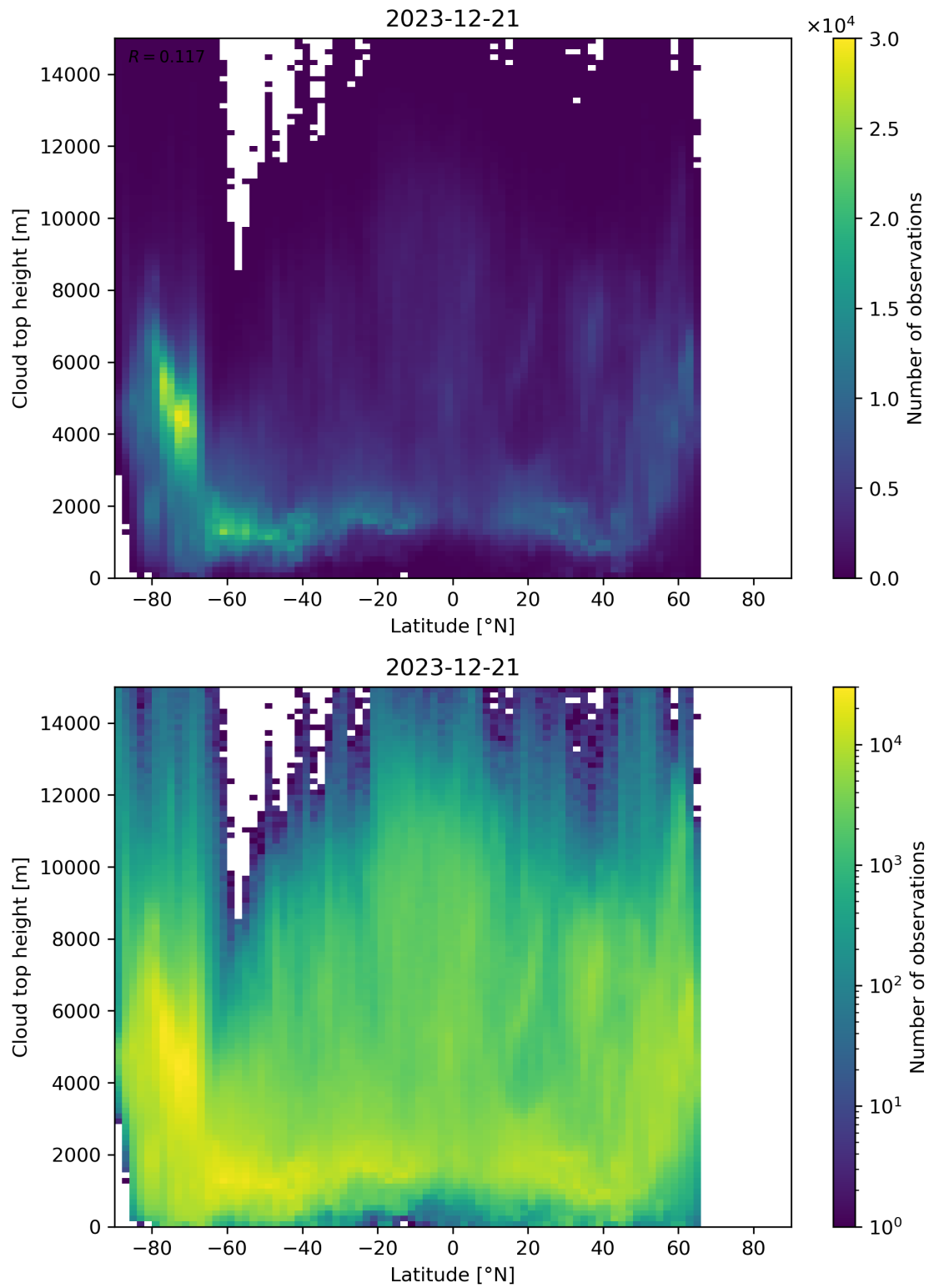
Figure 97: Scatter density plot of “Latitude” against “Cloud top height” for 2023-12-20 to 2023-12-22.
