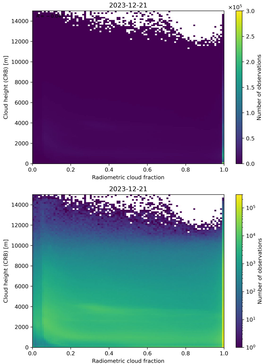
Figure 74: Scatter density plot of “Radiometric cloud fraction” against “Cloud height (CRB)” for 2023-12-20 to 2023-12-22.
