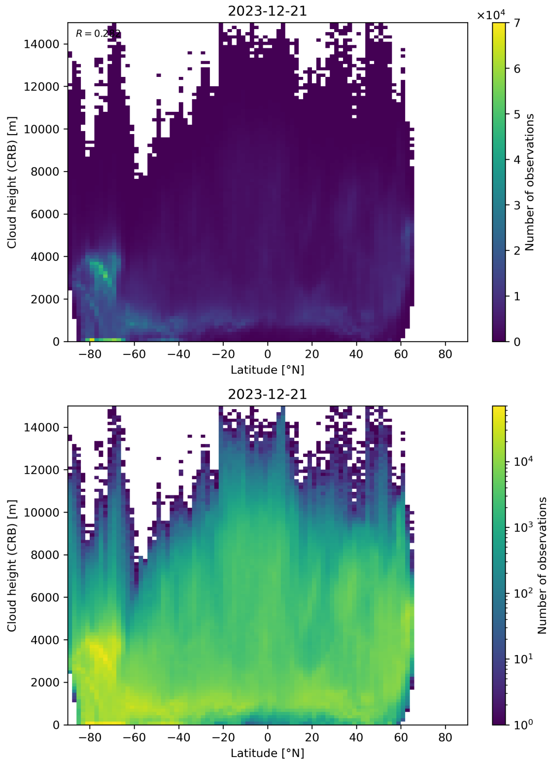
Figure 95: Scatter density plot of “Latitude” against “Cloud height (CRB)” for 2023-12-20 to 2023-12-22.
