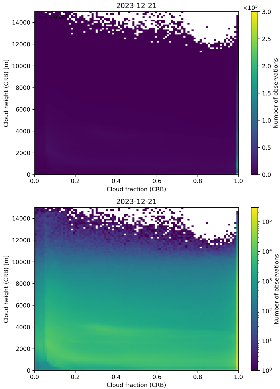
Figure 79: Scatter density plot of “Cloud fraction (CRB)” against “Cloud height (CRB)” for 2023-12-20 to 2023-12-22.
