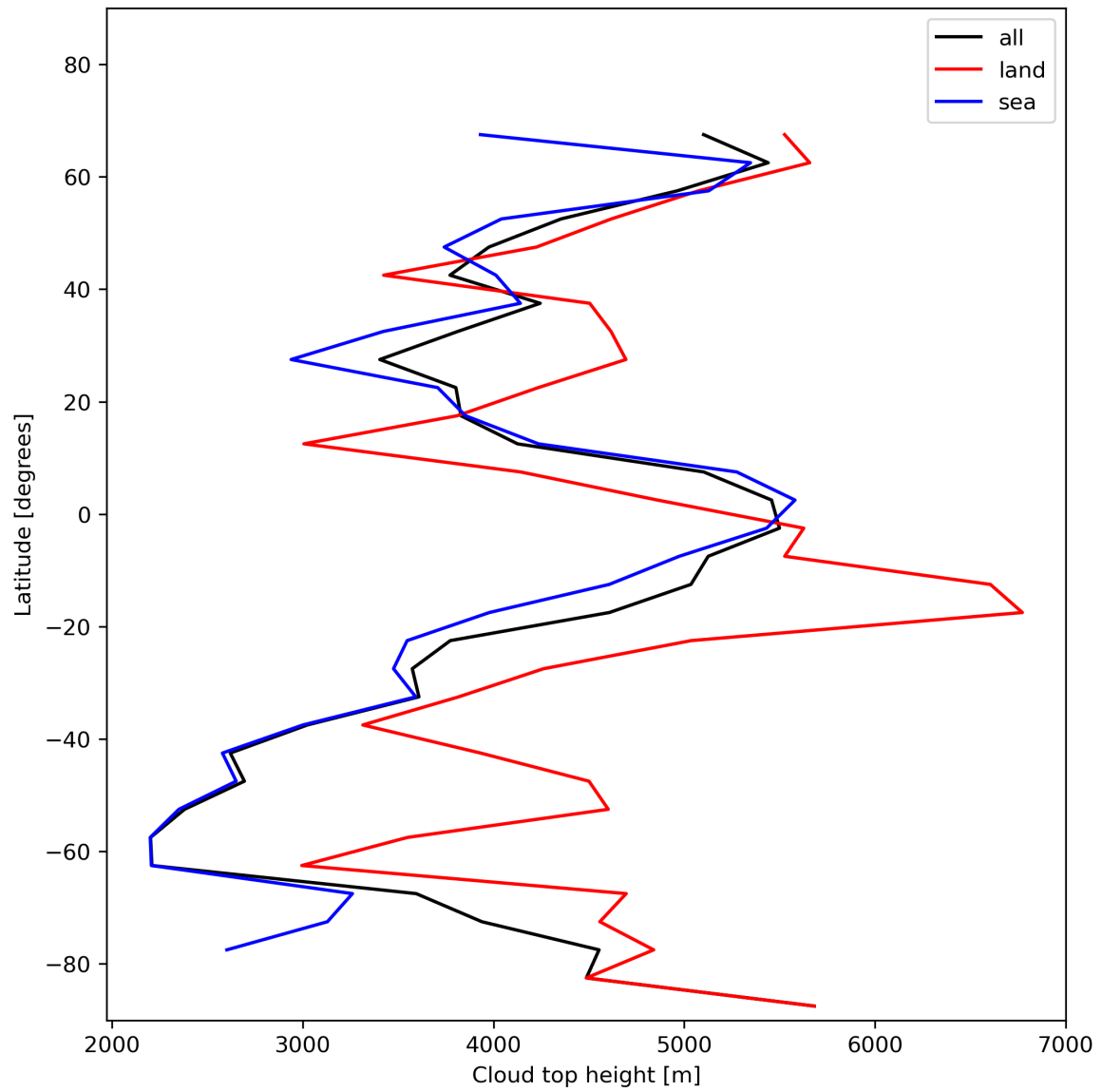
Figure 24: Zonal average of “Cloud top height” for 2023-12-20 to 2023-12-22.
