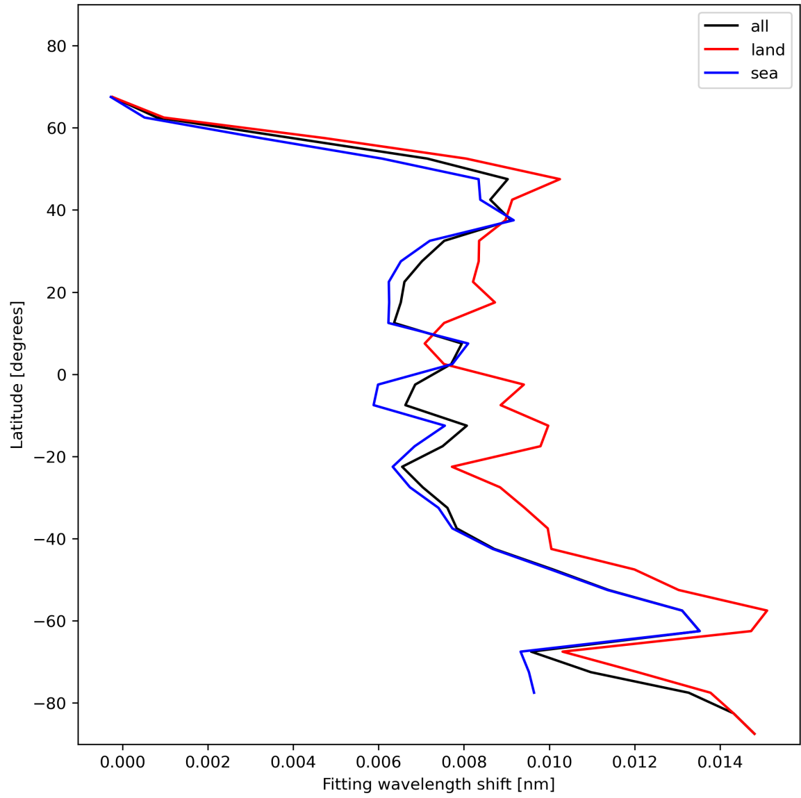
Figure 33: Zonal average of “Fitting wavelength shift” for 2023-12-20 to 2023-12-22.
