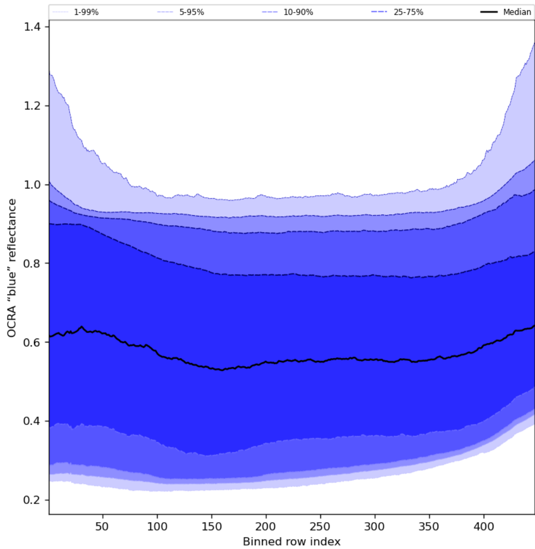
Figure 67: Along track statistics of “OCRA “blue” reflectance” for 2023-12-20 to 2023-12-22
