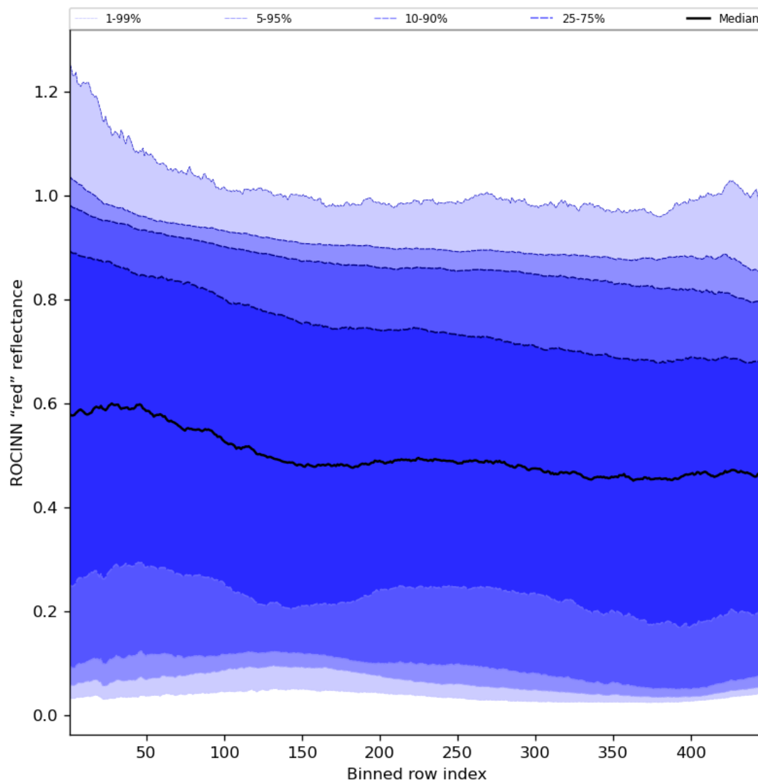
Figure 69: Along track statistics of “ROCINN “red” reflectance” for 2023-12-20 to 2023-12-22
