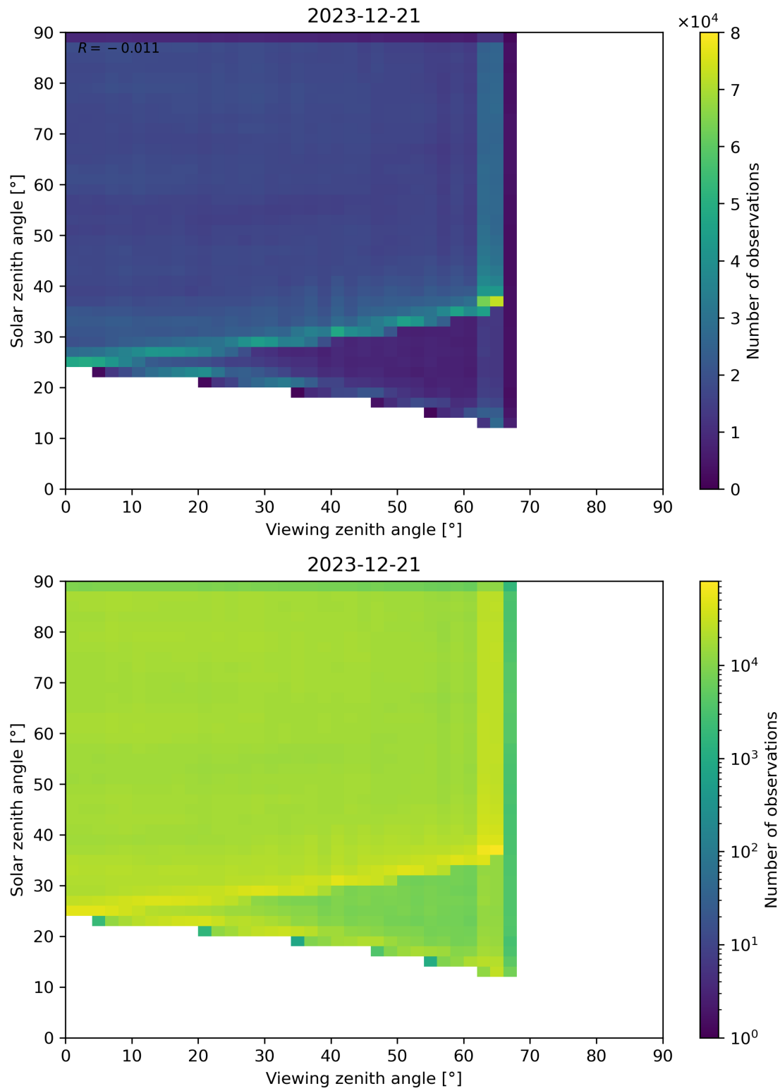
Figure 114: Scatter density plot of “Viewing zenith angle” against “Solar zenith angle” for 2023-12-20 to 2023-12-22.
