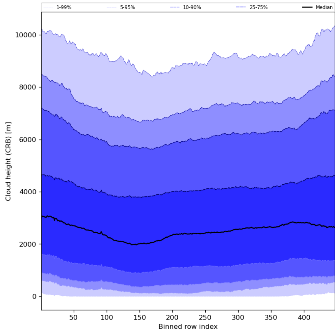
Figure 59: Along track statistics of “Cloud height (CRB)” for 2023-12-20 to 2023-12-22
