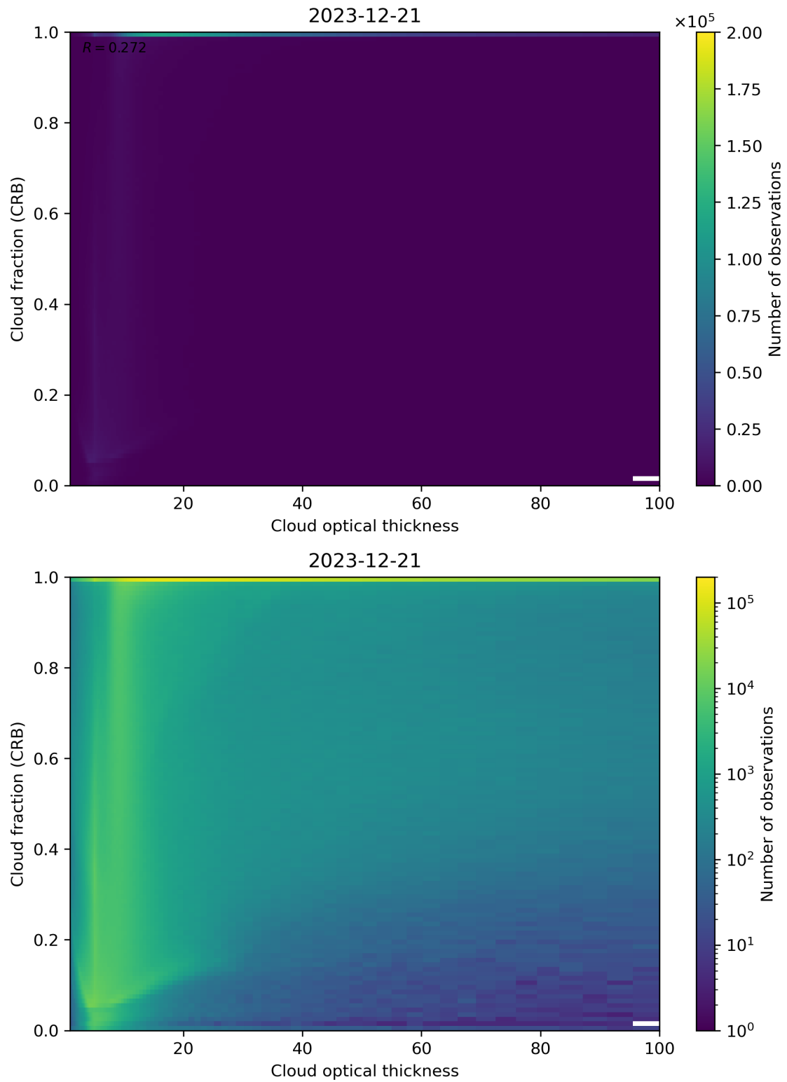
Figure 84: Scatter density plot of “Cloud optical thickness” against “Cloud fraction (CRB)” for 2023-12-20 to 2023-12-22.
