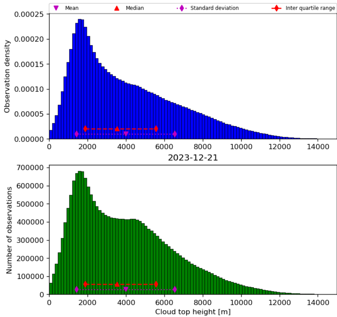
Figure 40: Histogram of “Cloud top height” for 2023-12-20 to 2023-12-22
