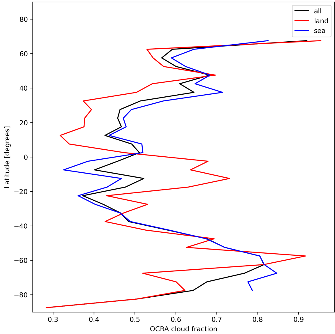
Figure 34: Zonal average of “OCRA cloud fraction” for 2023-12-20 to 2023-12-22.
