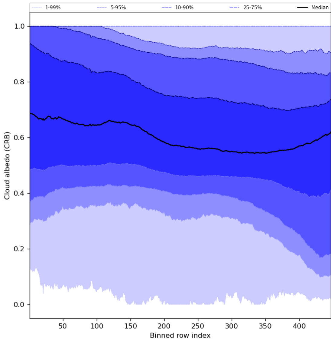
Figure 60: Along track statistics of “Cloud albedo (CRB)” for 2023-12-20 to 2023-12-22
