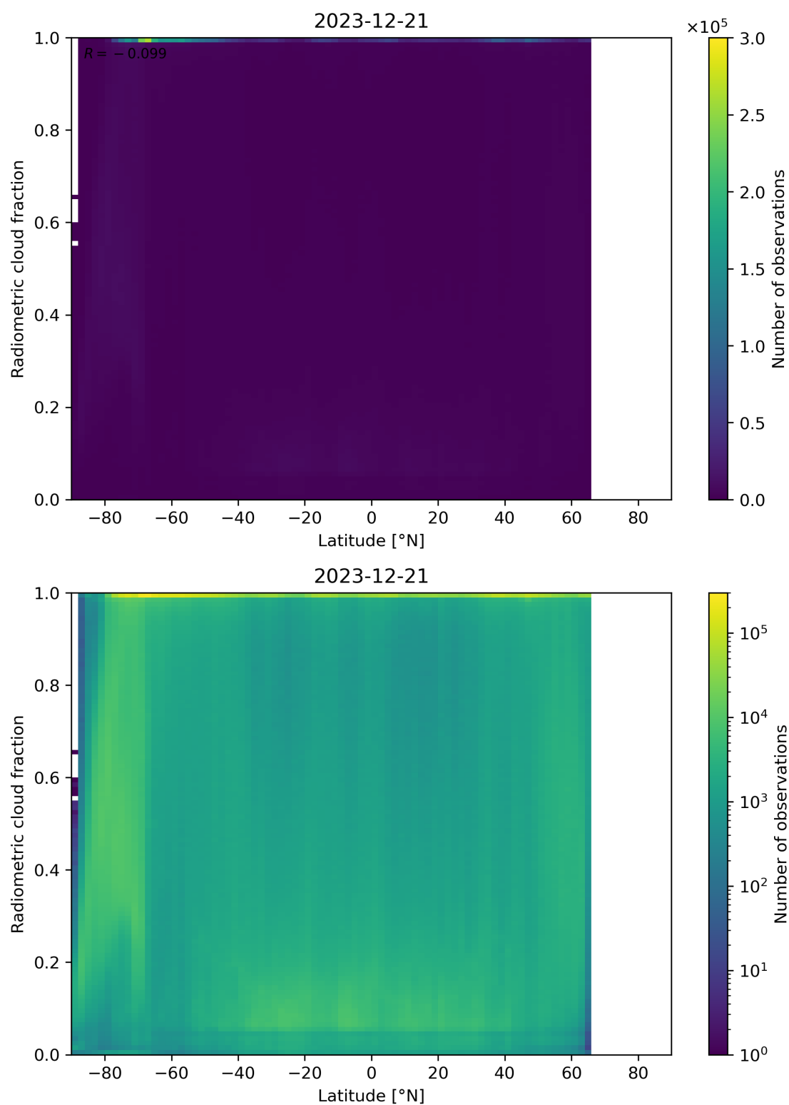
Figure 92: Scatter density plot of “Latitude” against “Radiometric cloud fraction” for 2023-12-20 to 2023-12-22.
