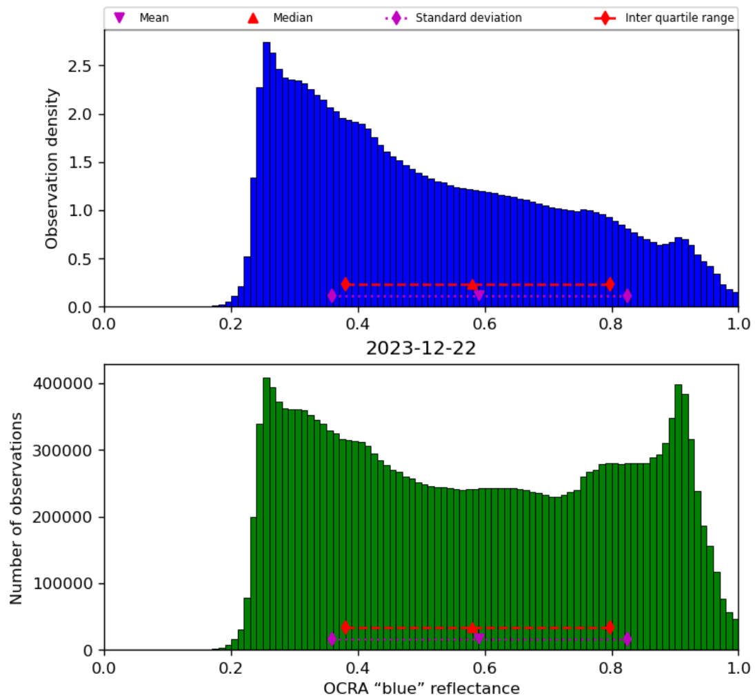
Figure 51: Histogram of “OCRA “blue” reflectance” for 2023-12-21 to 2023-12-23
