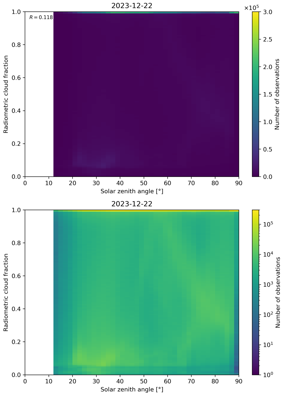
Figure 99: Scatter density plot of “Solar zenith angle” against “Radiometric cloud fraction” for 2023-12-21 to 2023-12-23.
