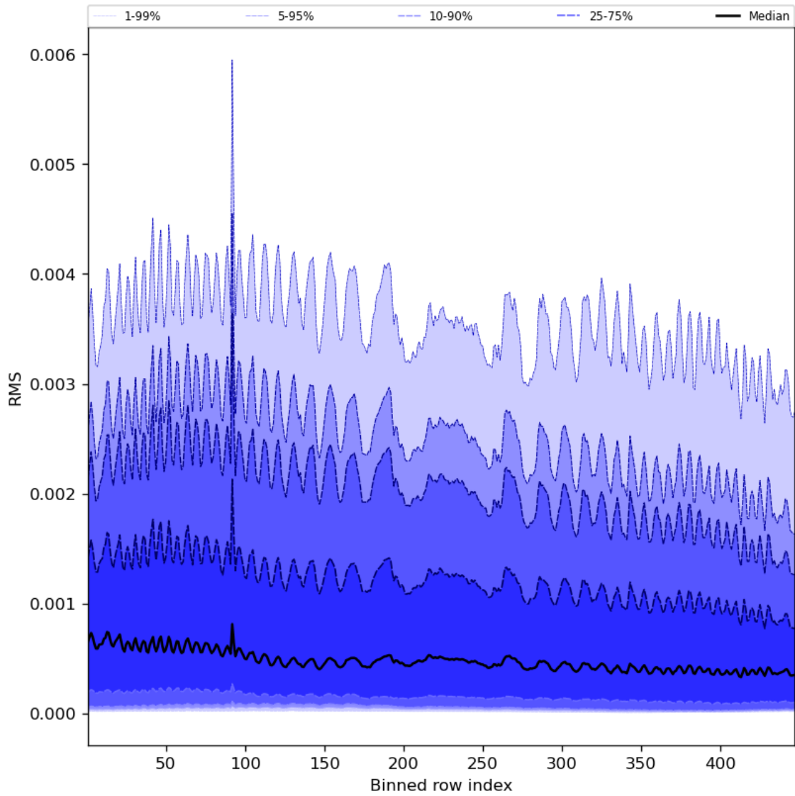
Figure 63: Along track statistics of “RMS” for 2023-12-21 to 2023-12-23
