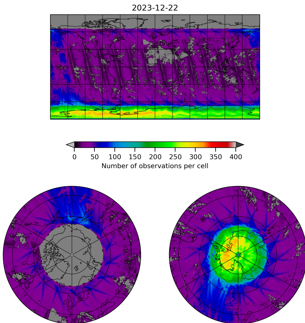
Figure 21: Map of the number of observations for 2023-12-21 to 2023-12-23
