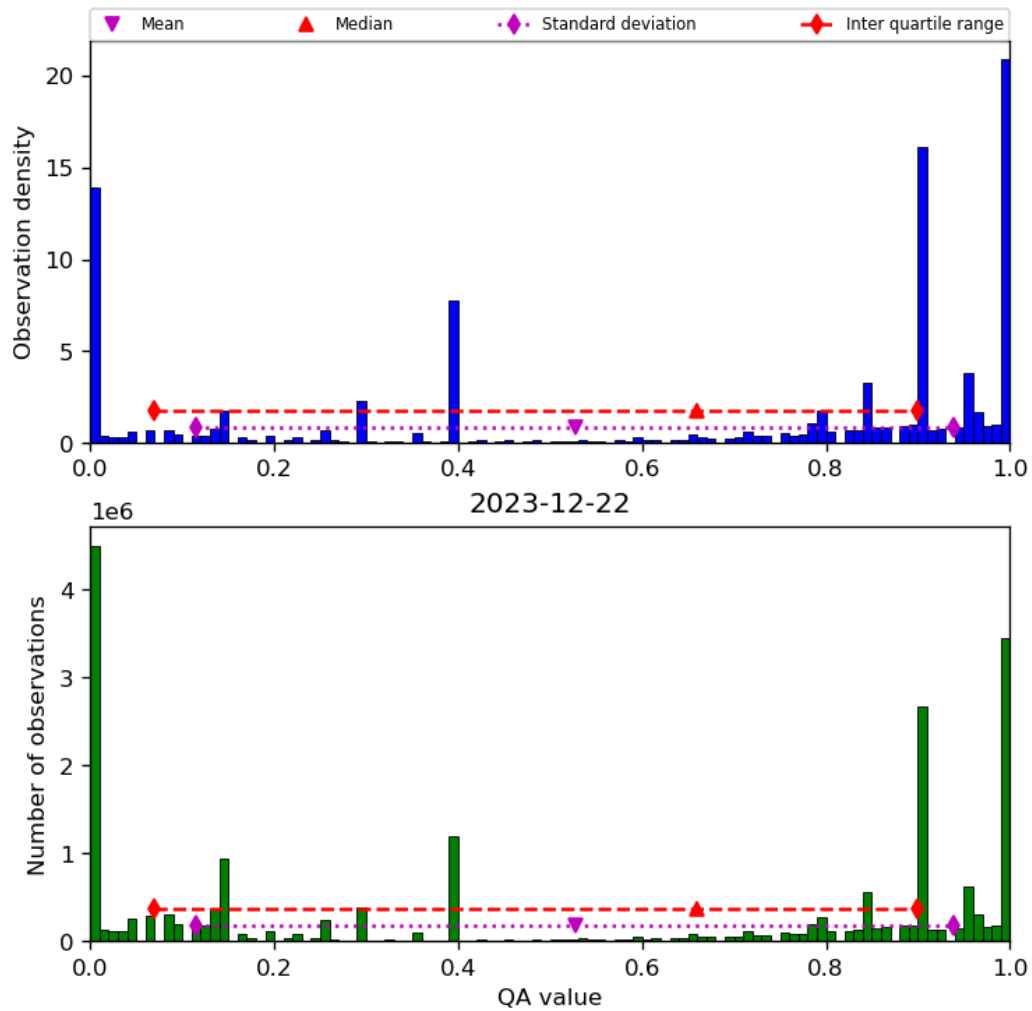
Figure 38: Histogram of “QA value” for 2023-12-21 to 2023-12-23
