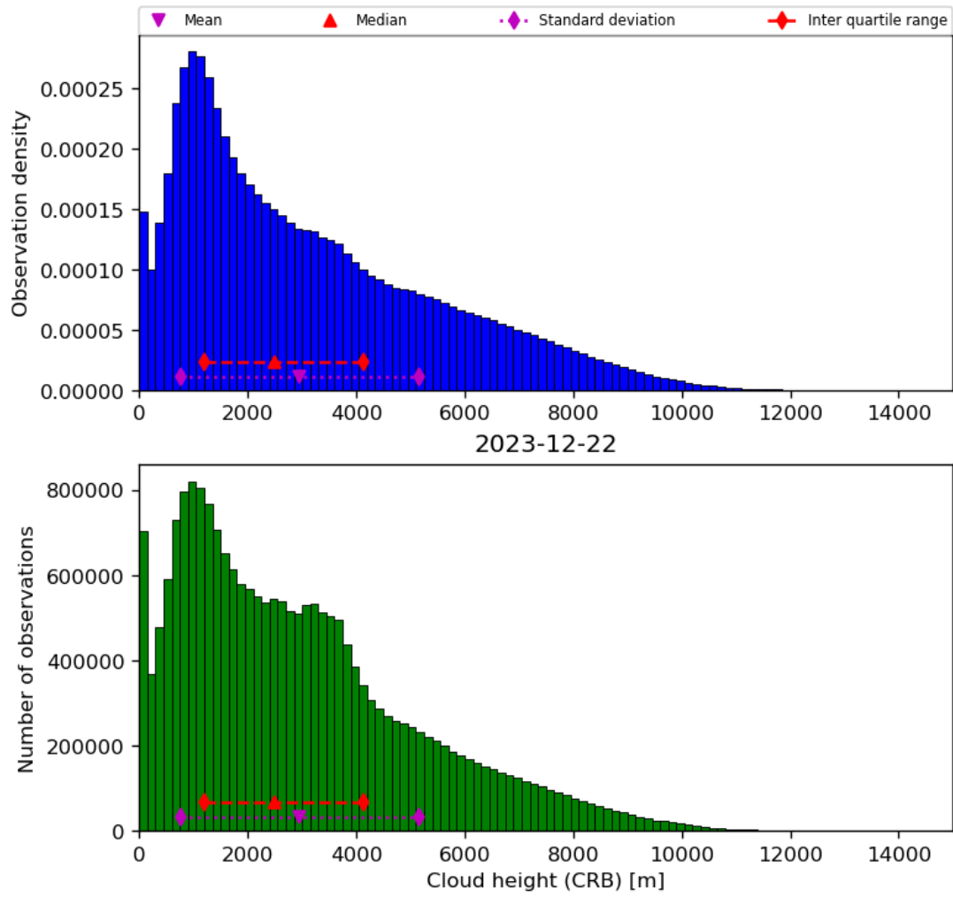
Figure 43: Histogram of “Cloud height (CRB)” for 2023-12-21 to 2023-12-23
