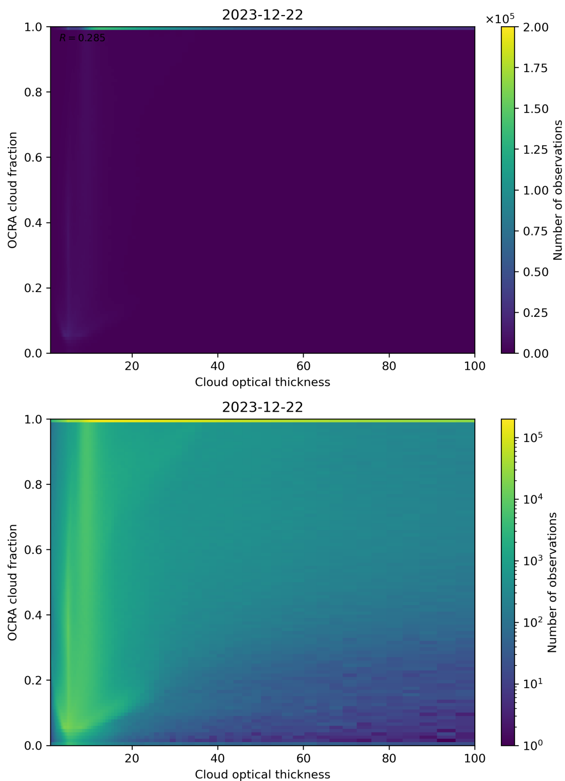
Figure 83: Scatter density plot of “Cloud optical thickness” against “OCRA cloud fraction” for 2023-12-21 to 2023-12-23.
