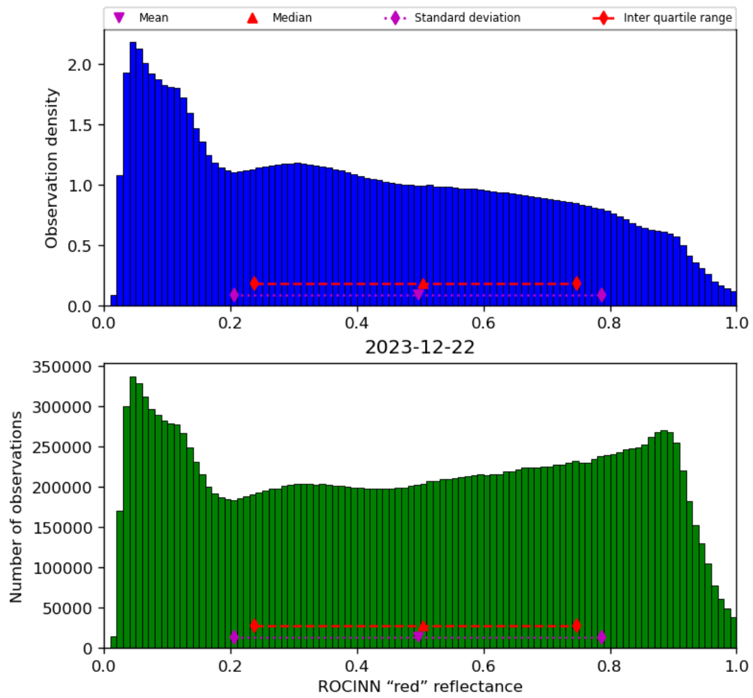
Figure 53: Histogram of “ROCINN “red” reflectance” for 2023-12-21 to 2023-12-23
