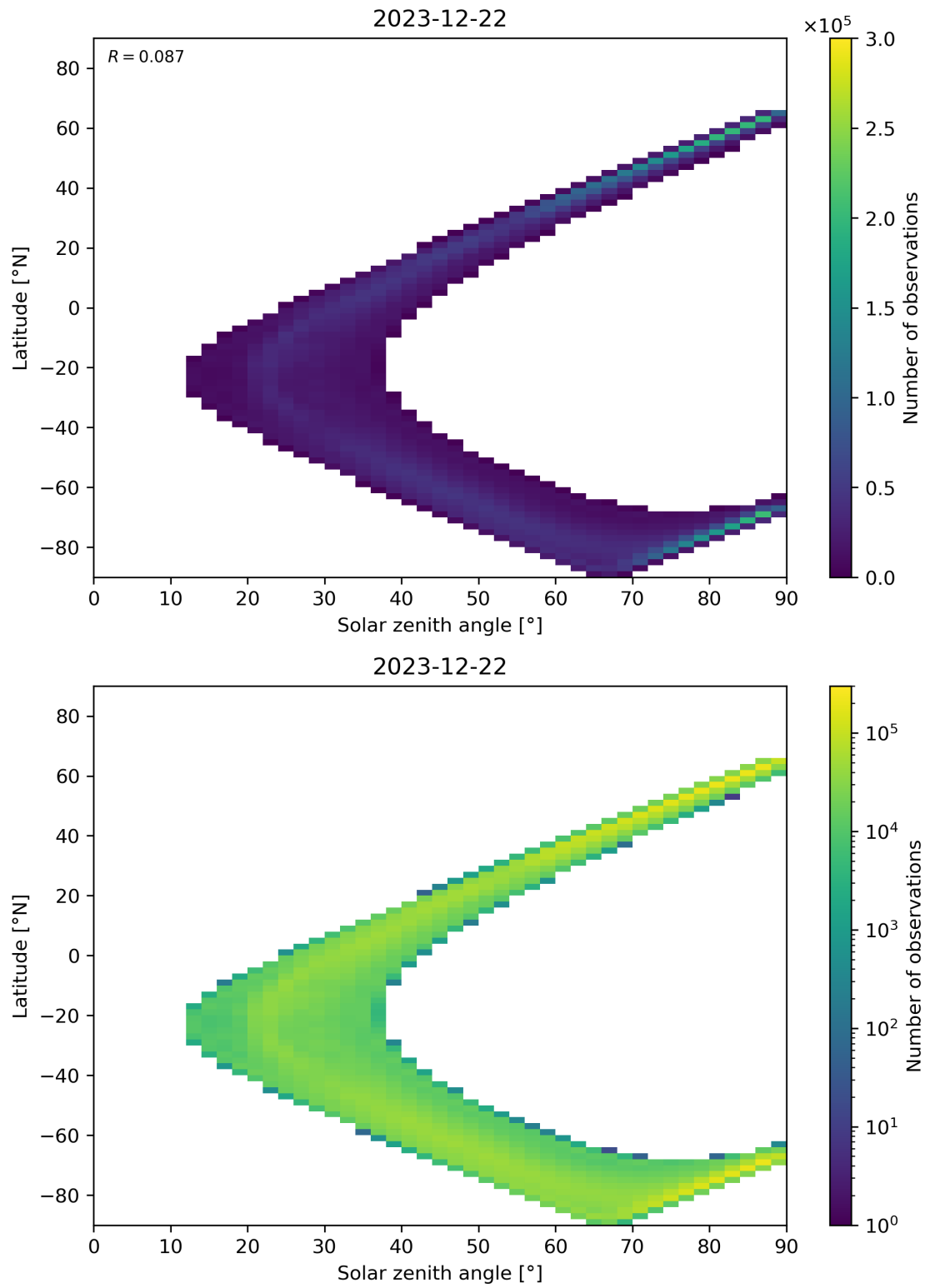
Figure 105: Scatter density plot of “Solar zenith angle” against “Latitude” for 2023-12-21 to 2023-12-23.
