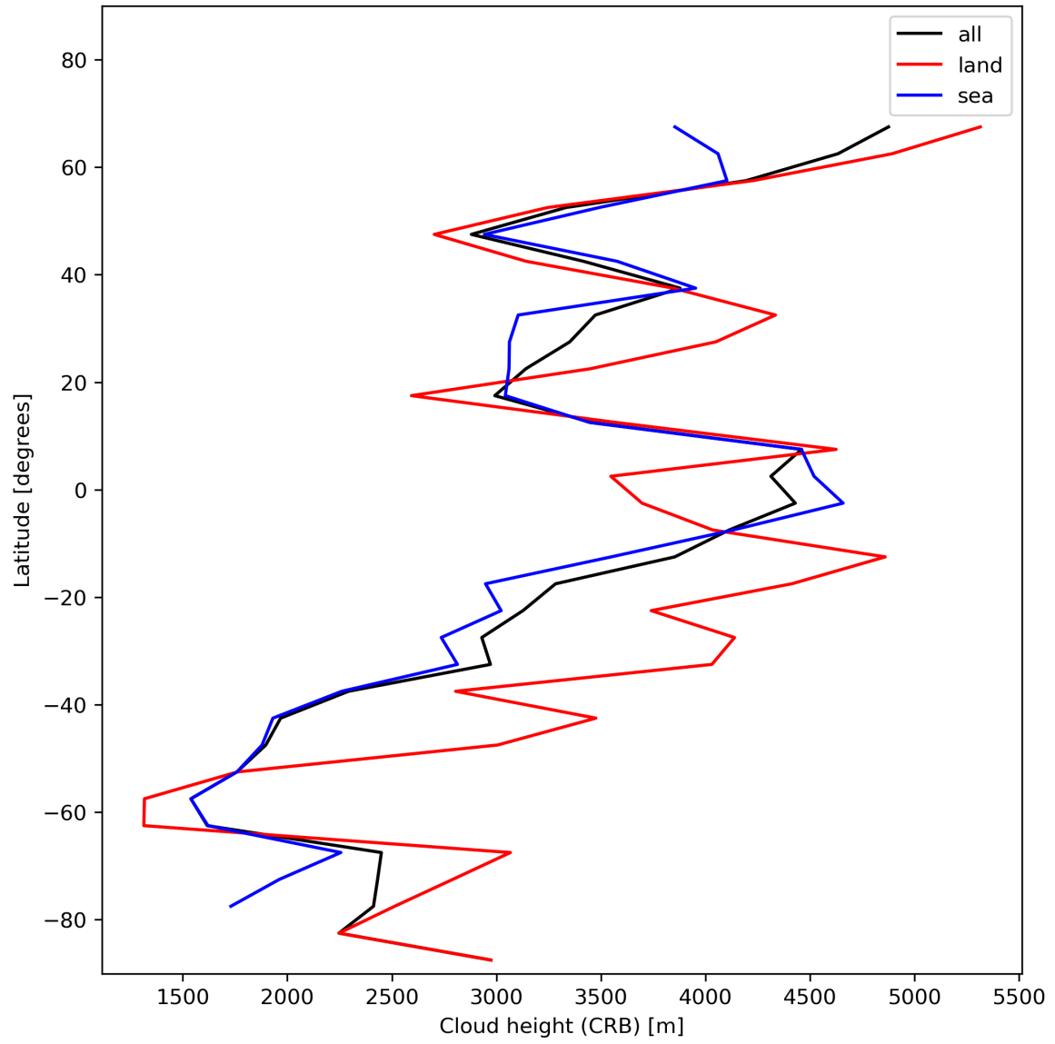
Figure 27: Zonal average of “Cloud height (CRB)” for 2023-12-21 to 2023-12-23.
