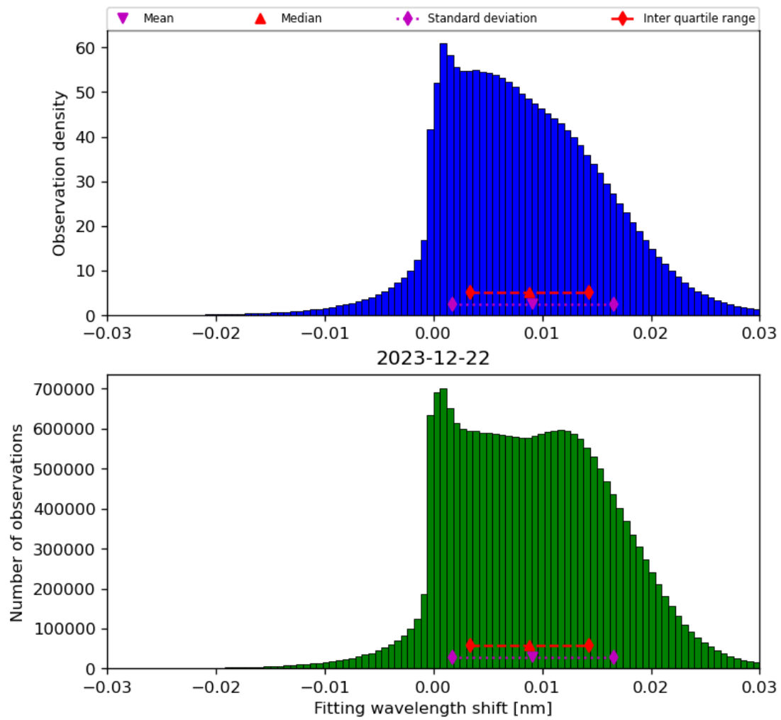
Figure 49: Histogram of “Fitting wavelength shift” for 2023-12-21 to 2023-12-23
