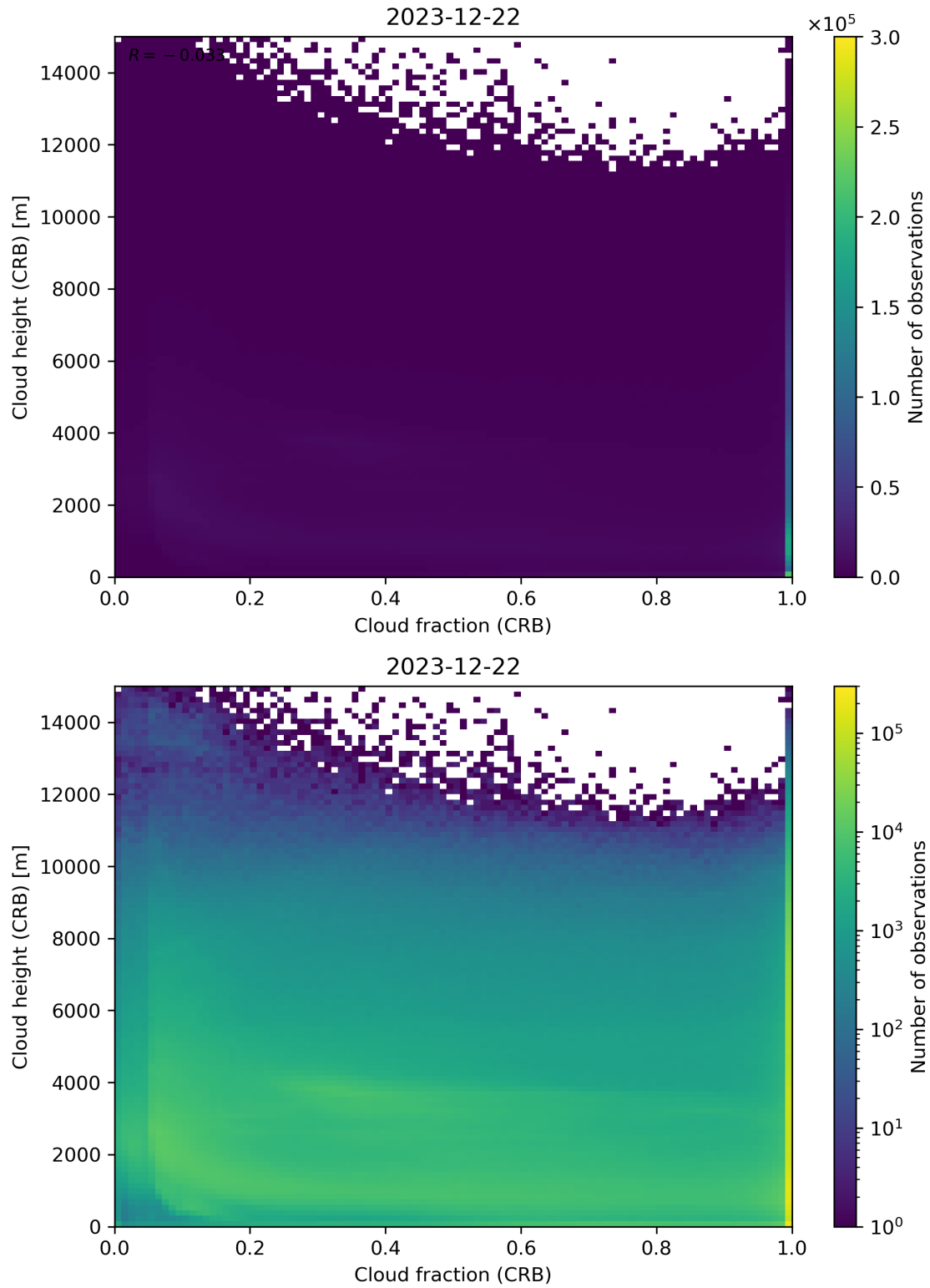
Figure 79: Scatter density plot of “Cloud fraction (CRB)” against “Cloud height (CRB)” for 2023-12-21 to 2023-12-23.
