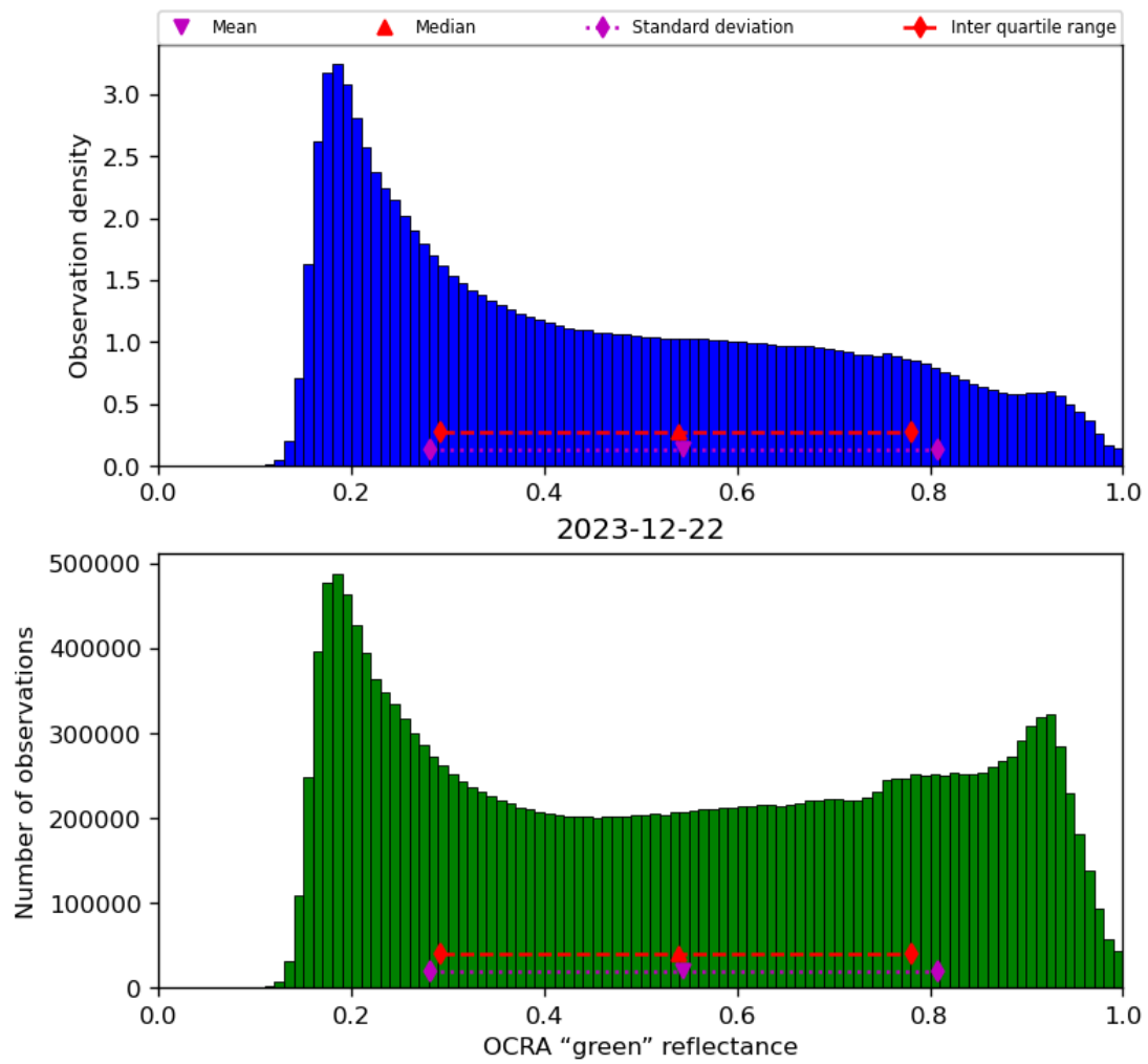
Figure 52: Histogram of “OCRA “green” reflectance” for 2023-12-21 to 2023-12-23
