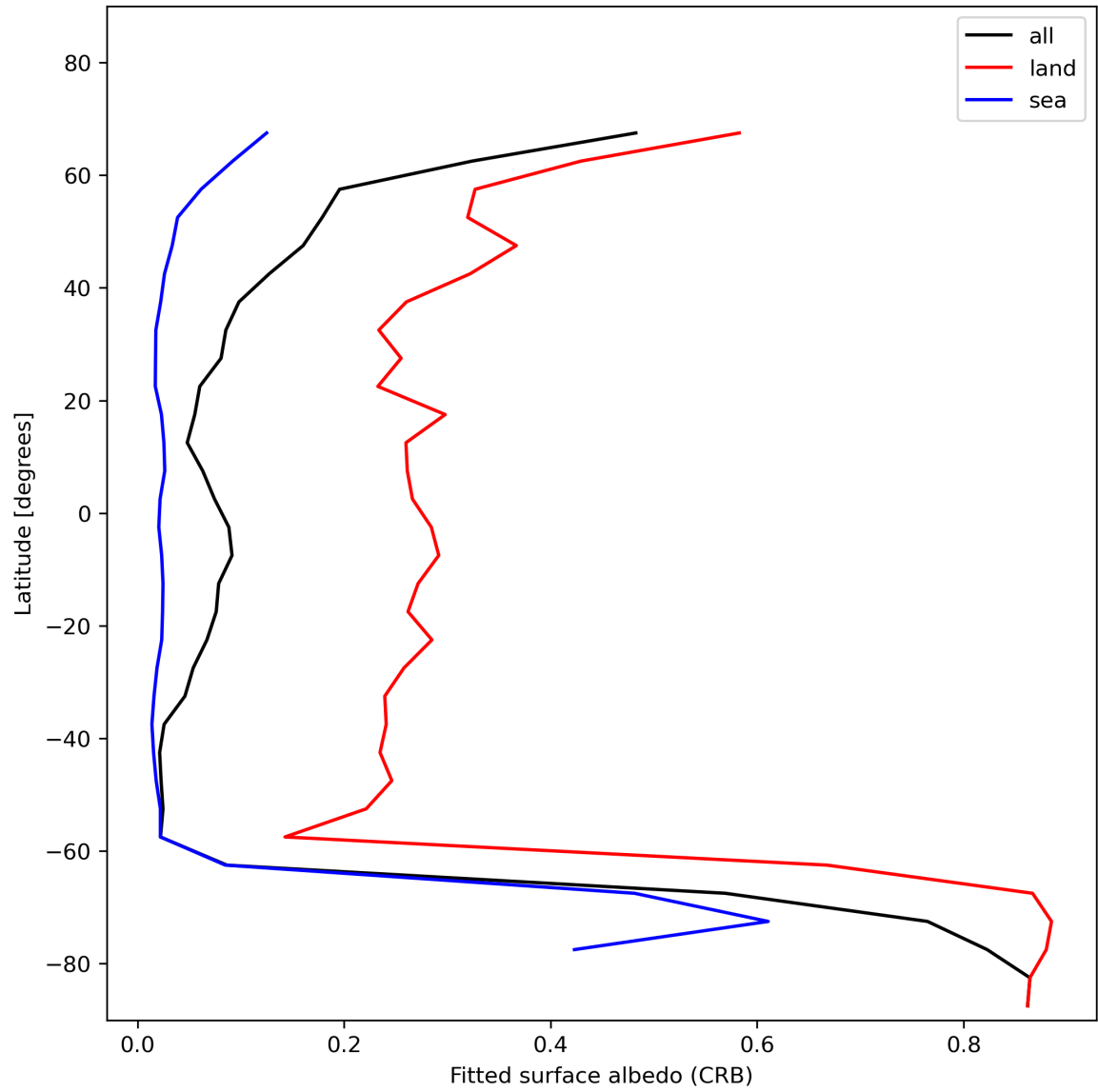
Figure 30: Zonal average of “Fitted surface albedo (CRB)” for 2023-12-21 to 2023-12-23.
