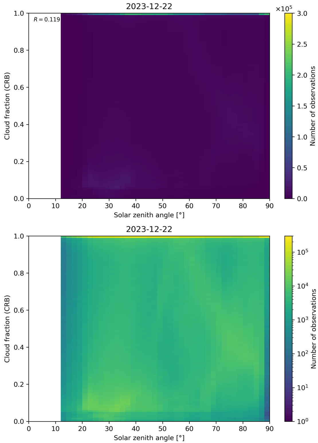
Figure 101: Scatter density plot of “Solar zenith angle” against “Cloud fraction (CRB)” for 2023-12-21 to 2023-12-23.
