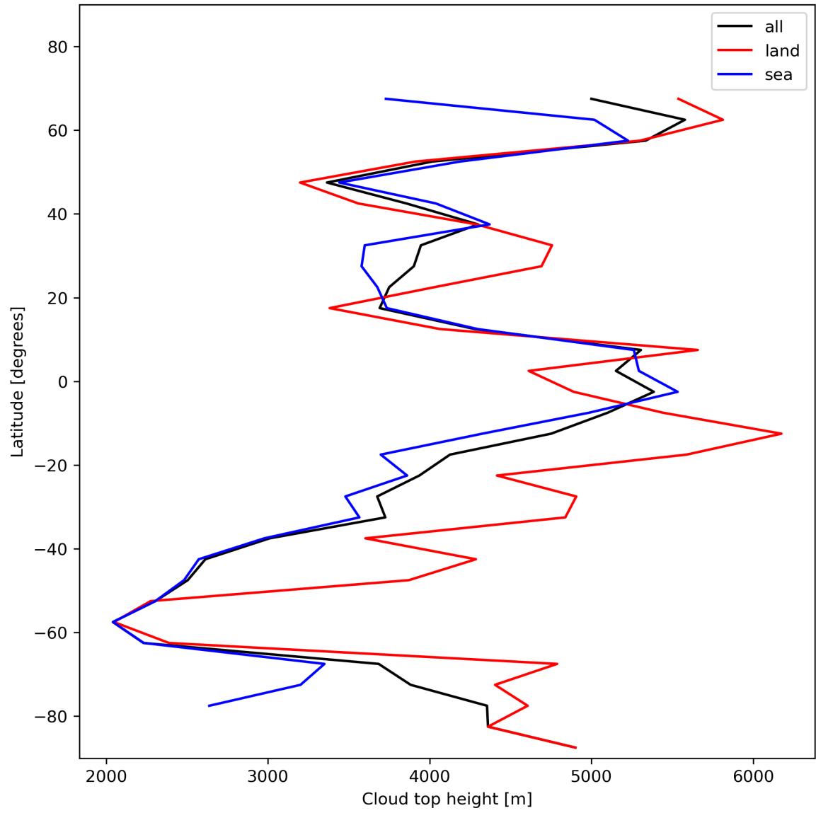
Figure 24: Zonal average of “Cloud top height” for 2023-12-21 to 2023-12-23.
