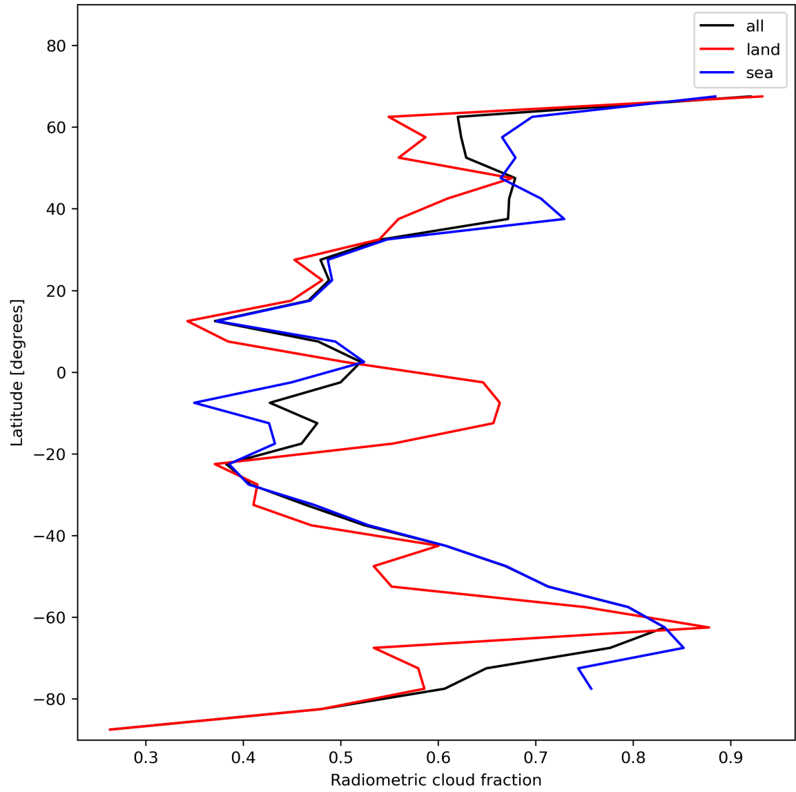
Figure 23: Zonal average of “Radiometric cloud fraction” for 2023-12-21 to 2023-12-23.
