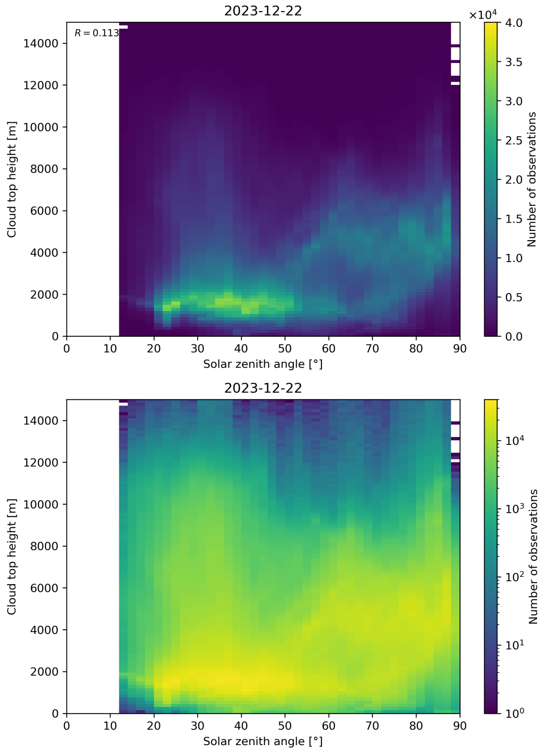
Figure 104: Scatter density plot of “Solar zenith angle” against “Cloud top height” for 2023-12-21 to 2023-12-23.
