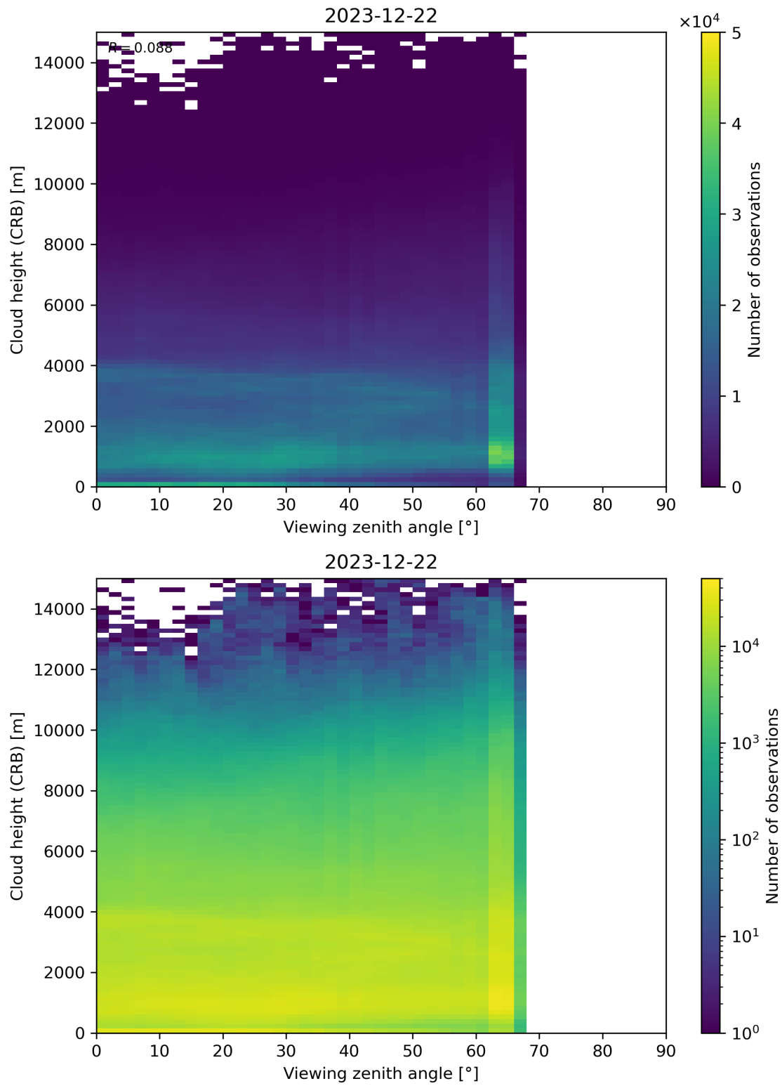
Figure 110: Scatter density plot of “Viewing zenith angle” against “Cloud height (CRB)” for 2023-12-21 to 2023-12-23.
