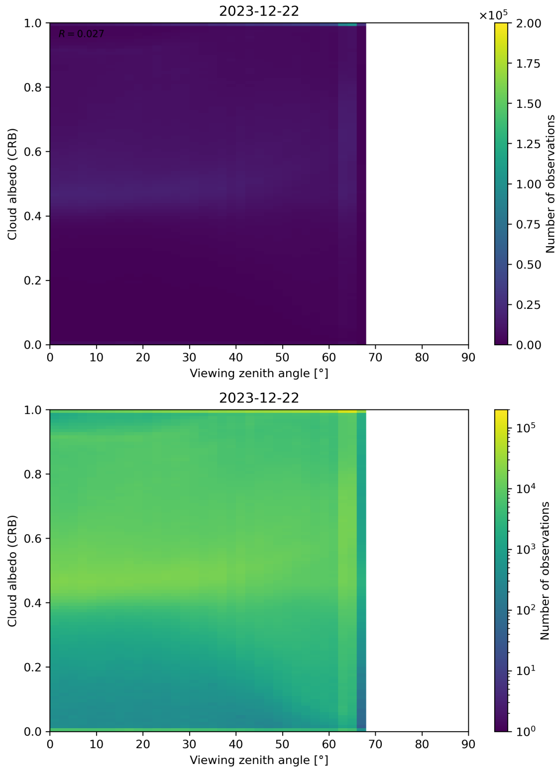
Figure 106: Scatter density plot of “Viewing zenith angle” against “Cloud albedo (CRB)” for 2023-12-21 to 2023-12-23.
