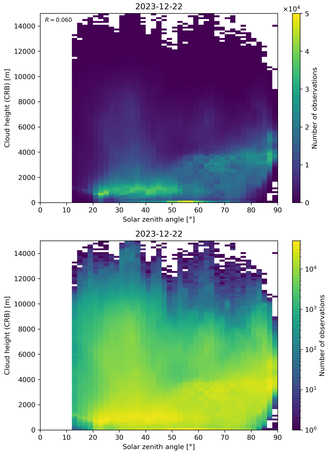
Figure 102: Scatter density plot of “Solar zenith angle” against “Cloud height (CRB)” for 2023-12-21 to 2023-12-23.
