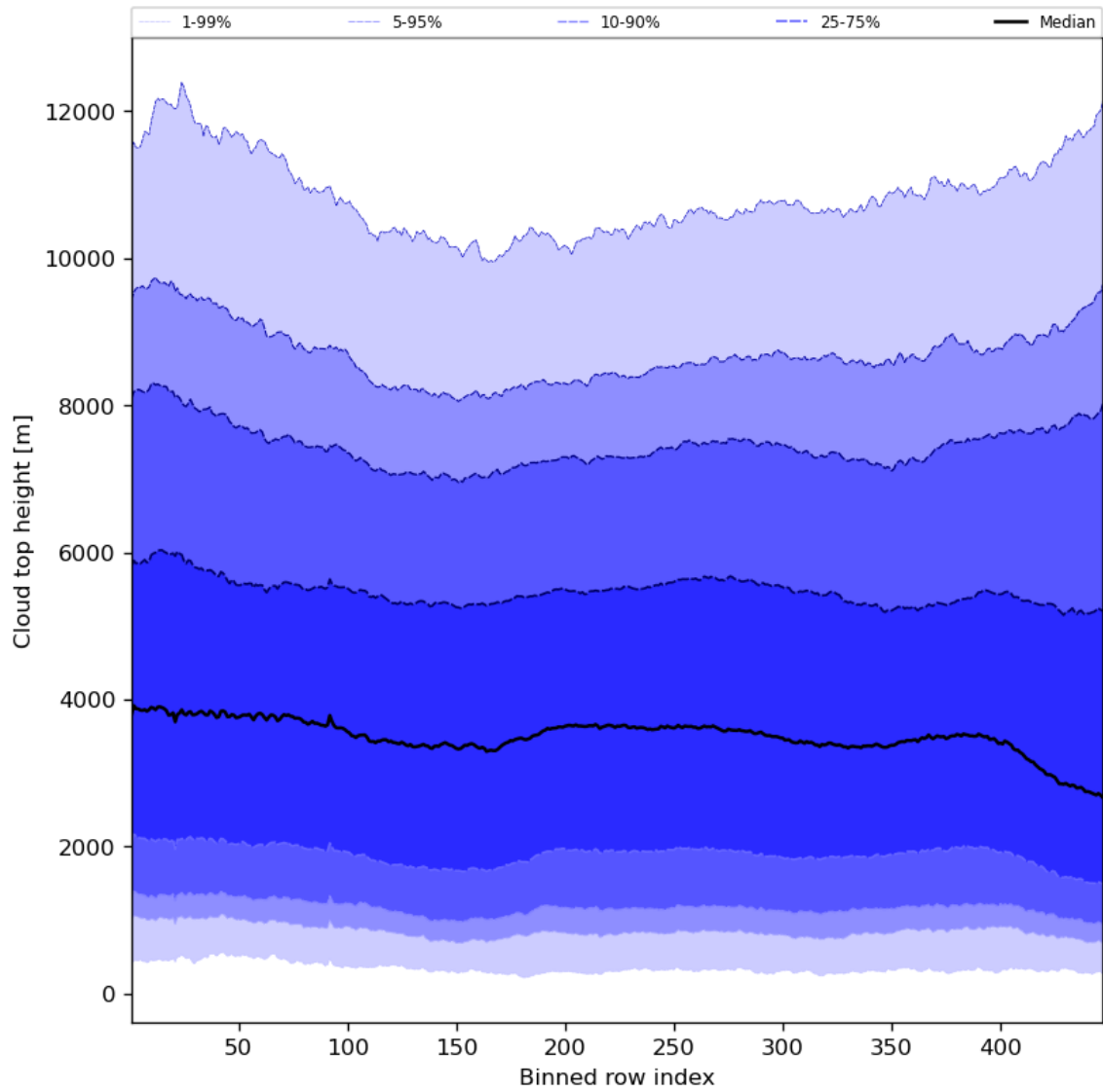
Figure 56: Along track statistics of “Cloud top height” for 2023-12-21 to 2023-12-23
