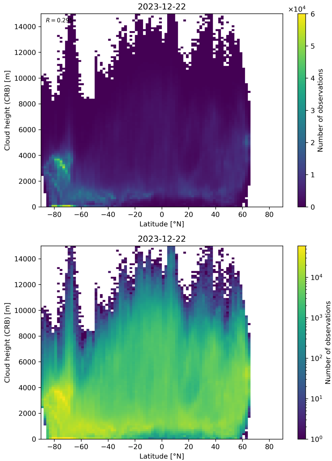
Figure 95: Scatter density plot of “Latitude” against “Cloud height (CRB)” for 2023-12-21 to 2023-12-23.
