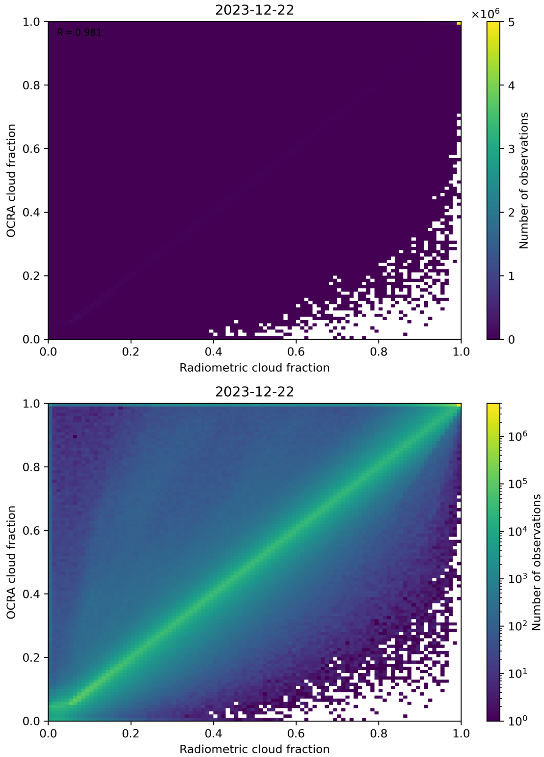
Figure 72: Scatter density plot of “Radiometric cloud fraction” against “OCRA cloud fraction” for 2023-12-21 to 2023-12-23.
