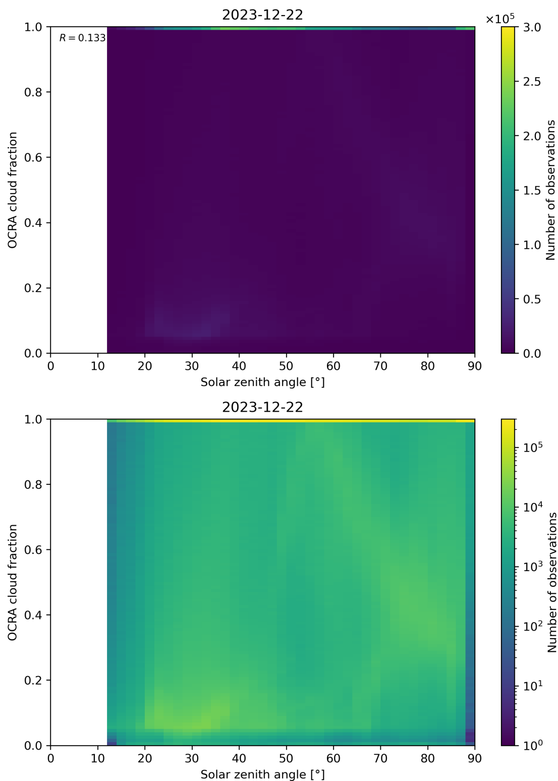
Figure 100: Scatter density plot of “Solar zenith angle” against “OCRA cloud fraction” for 2023-12-21 to 2023-12-23.
