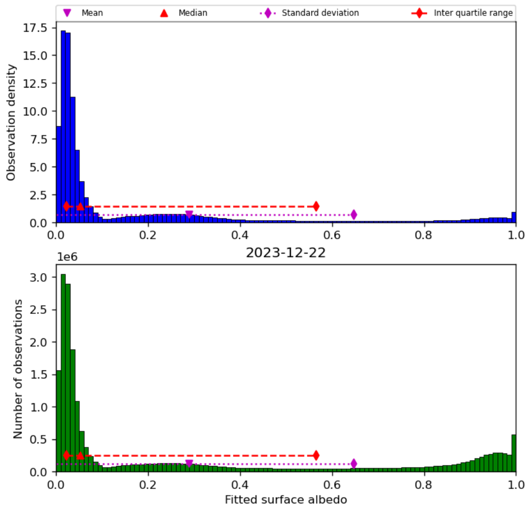
Figure 45: Histogram of “Fitted surface albedo” for 2023-12-21 to 2023-12-23
