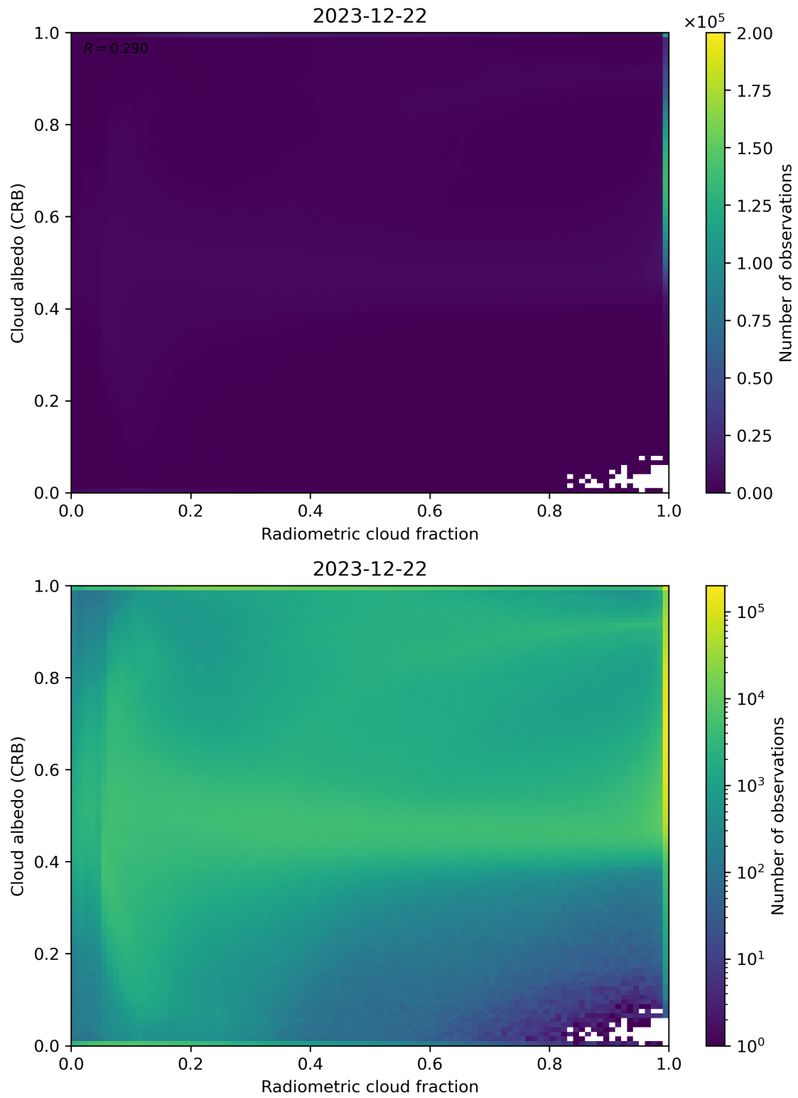
Figure 71: Scatter density plot of “Radiometric cloud fraction” against “Cloud albedo (CRB)” for 2023-12-21 to 2023-12-23.
