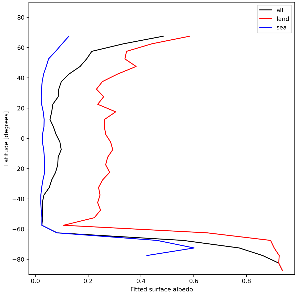
Figure 29: Zonal average of “Fitted surface albedo” for 2023-12-21 to 2023-12-23.
