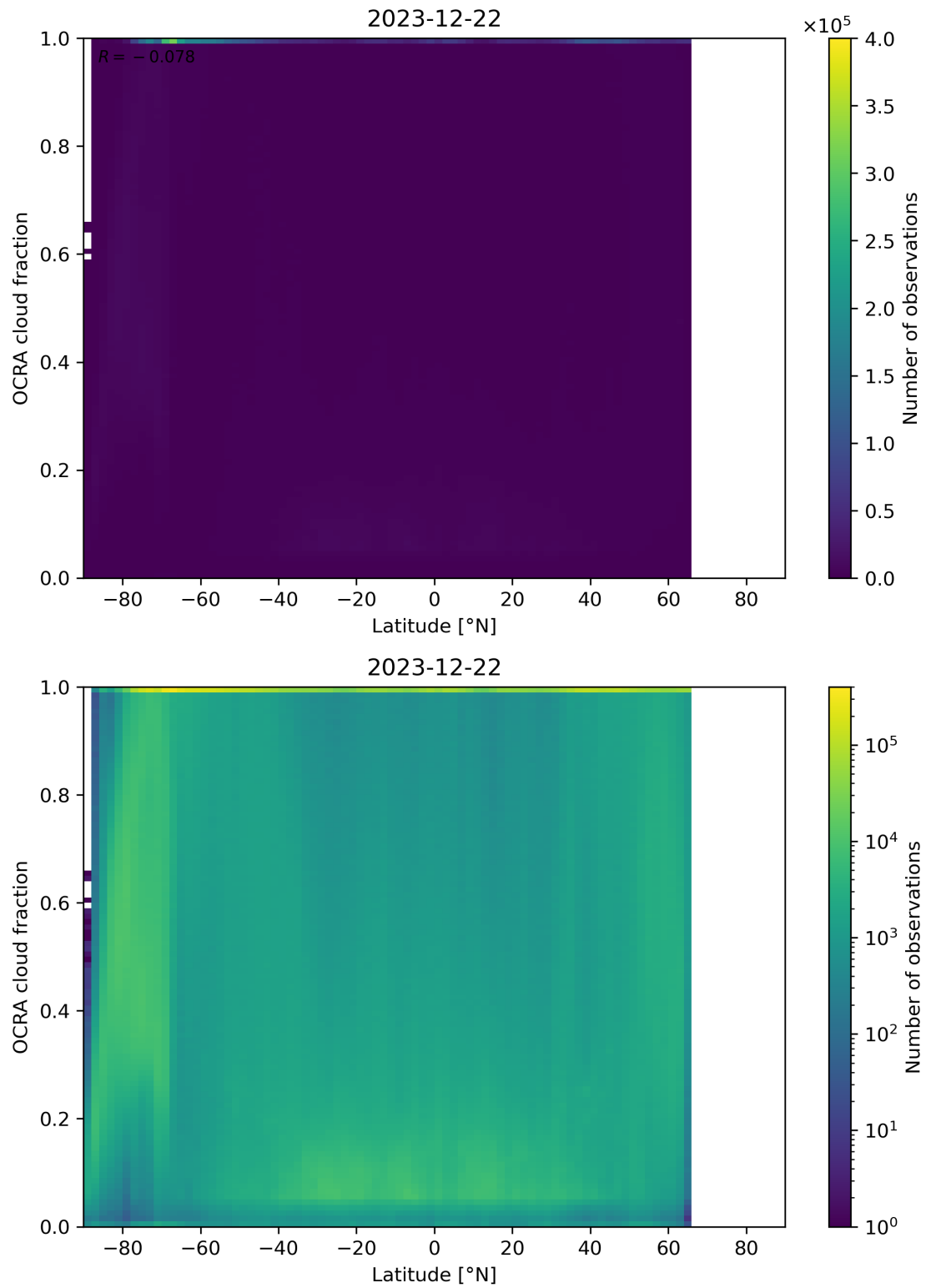
Figure 93: Scatter density plot of “Latitude” against “OCRA cloud fraction” for 2023-12-21 to 2023-12-23.
