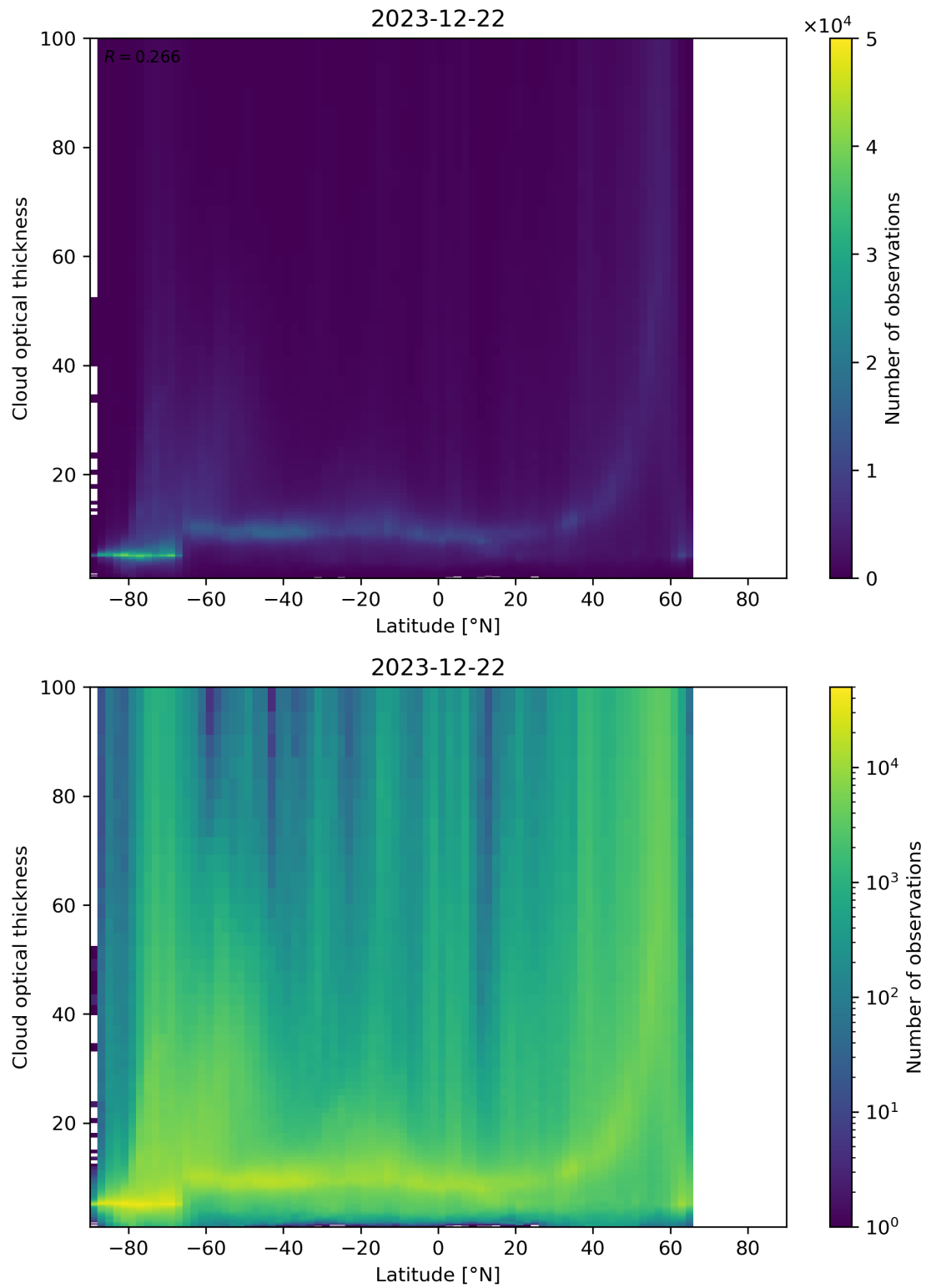
Figure 96: Scatter density plot of “Latitude” against “Cloud optical thickness” for 2023-12-21 to 2023-12-23.
