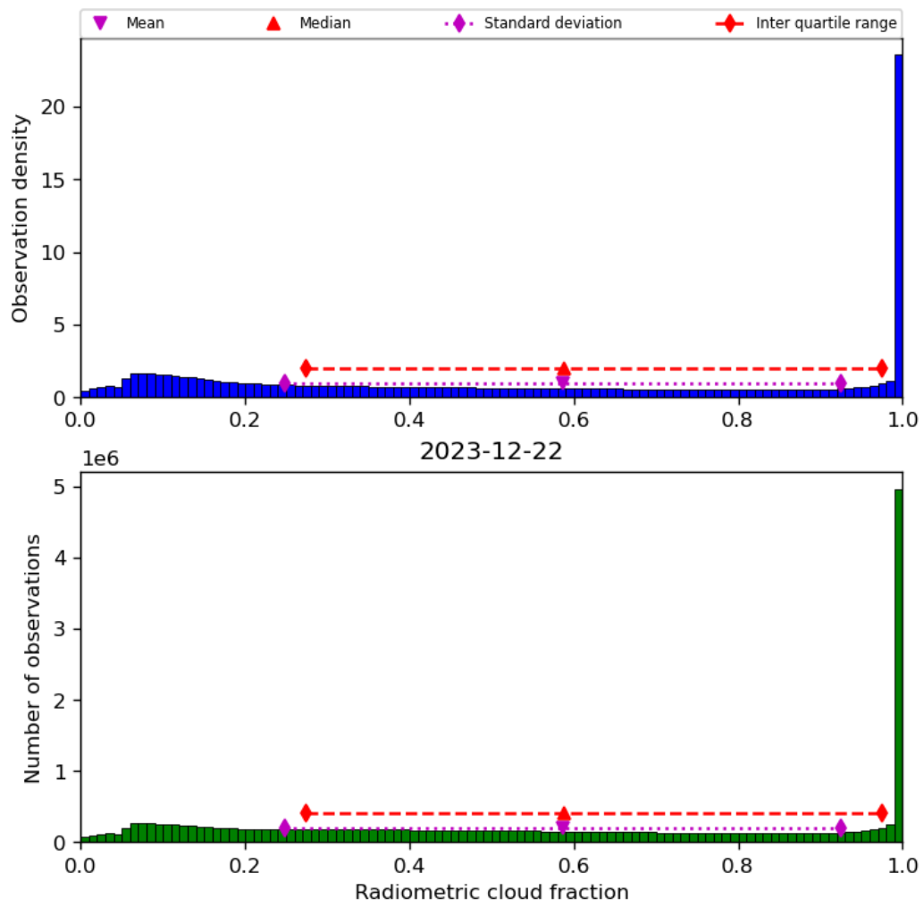
Figure 39: Histogram of “Radiometric cloud fraction” for 2023-12-21 to 2023-12-23
