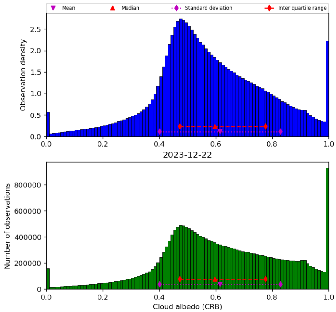
Figure 44: Histogram of “Cloud albedo (CRB)” for 2023-12-21 to 2023-12-23
