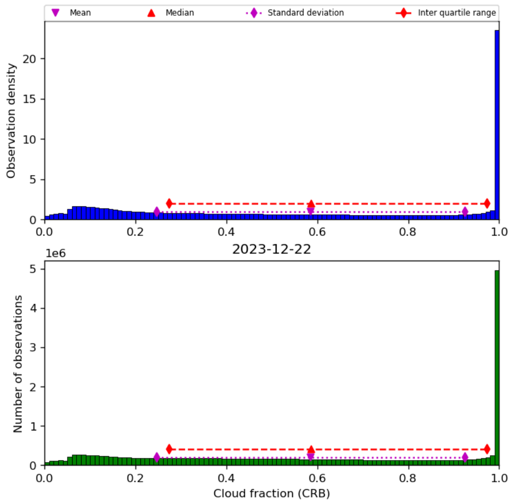
Figure 42: Histogram of “Cloud fraction (CRB)” for 2023-12-21 to 2023-12-23
