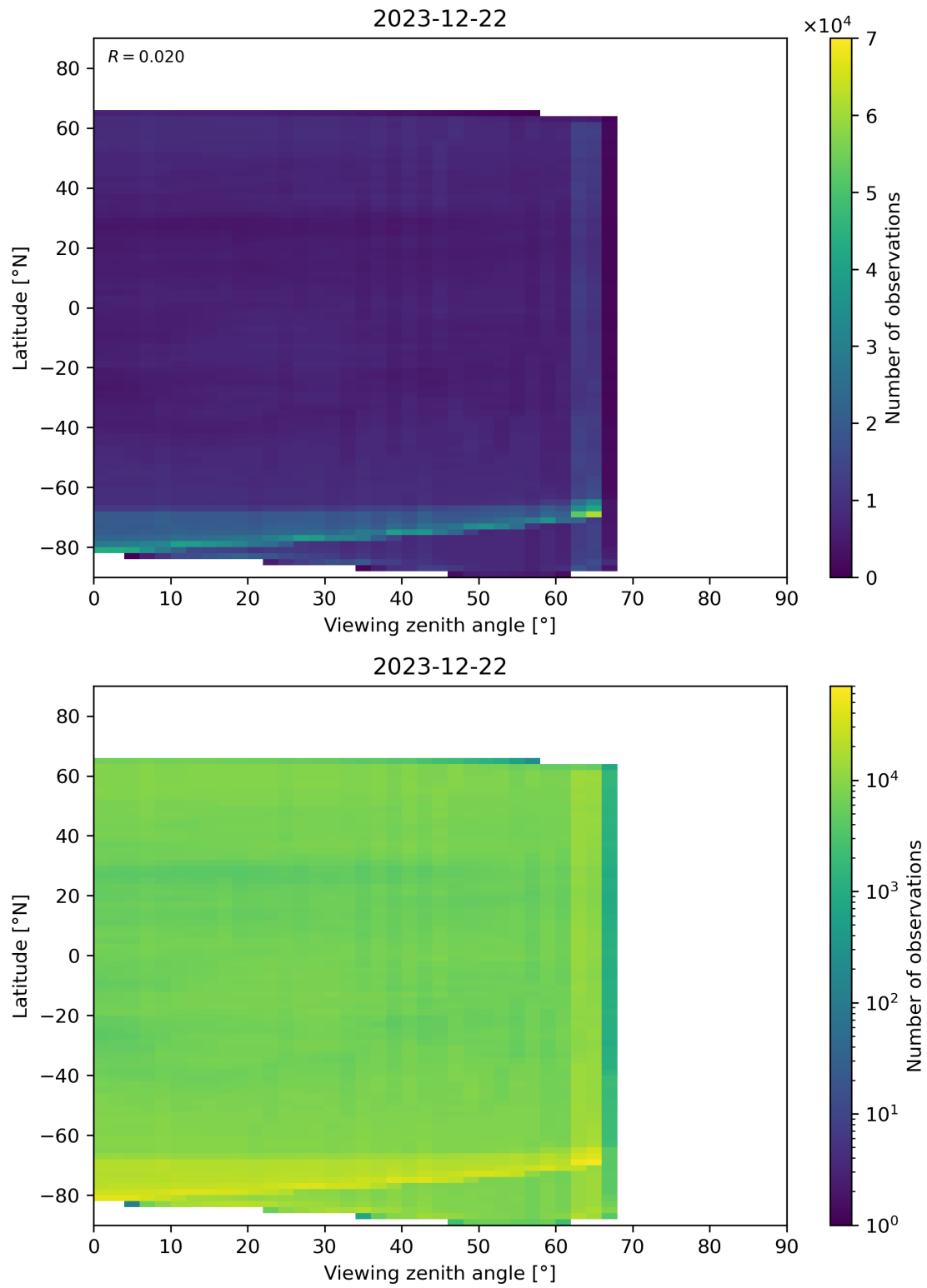
Figure 113: Scatter density plot of “Viewing zenith angle” against “Latitude” for 2023-12-21 to 2023-12-23.
