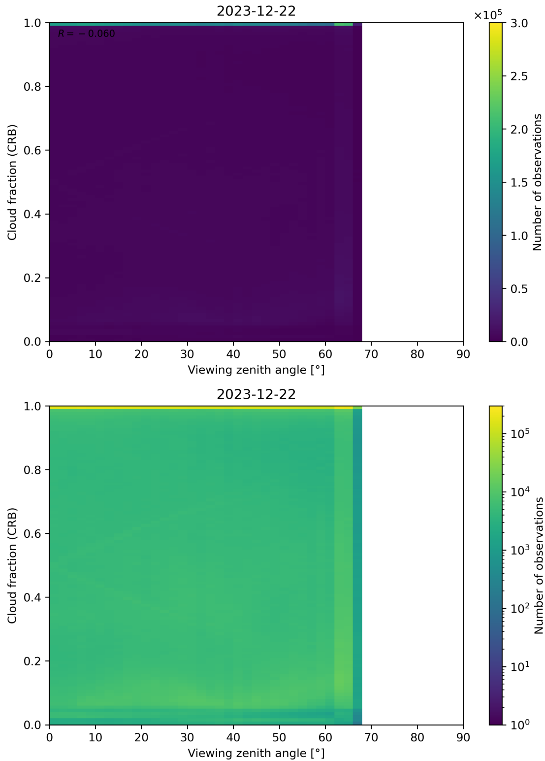
Figure 109: Scatter density plot of “Viewing zenith angle” against “Cloud fraction (CRB)” for 2023-12-21 to 2023-12-23.
