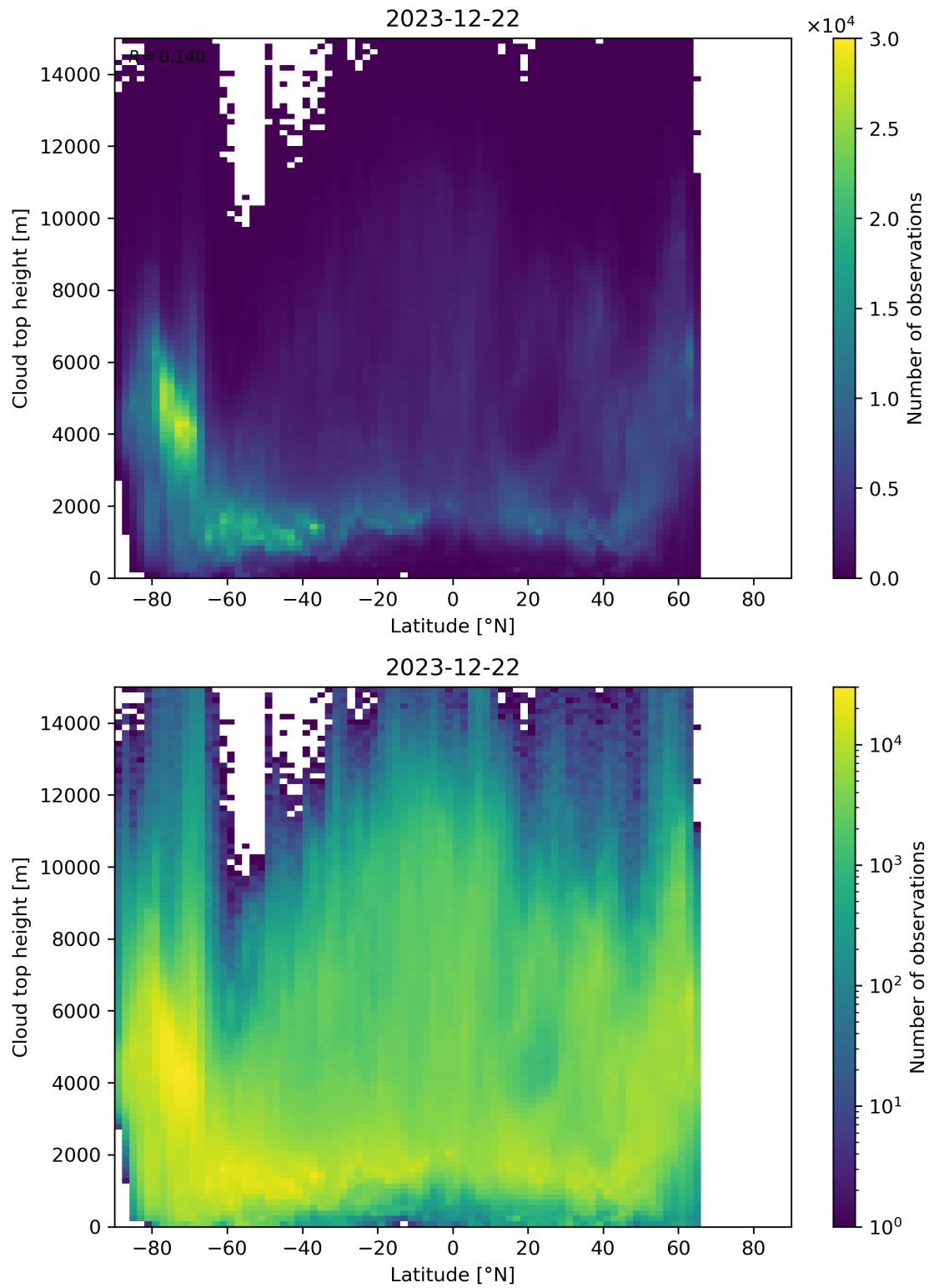
Figure 97: Scatter density plot of “Latitude” against “Cloud top height” for 2023-12-21 to 2023-12-23.
