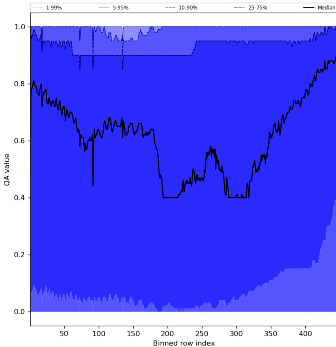
Figure 54: Along track statistics of “QA value” for 2023-12-21 to 2023-12-23
