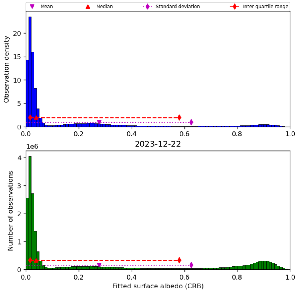
Figure 46: Histogram of “Fitted surface albedo (CRB)” for 2023-12-21 to 2023-12-23
