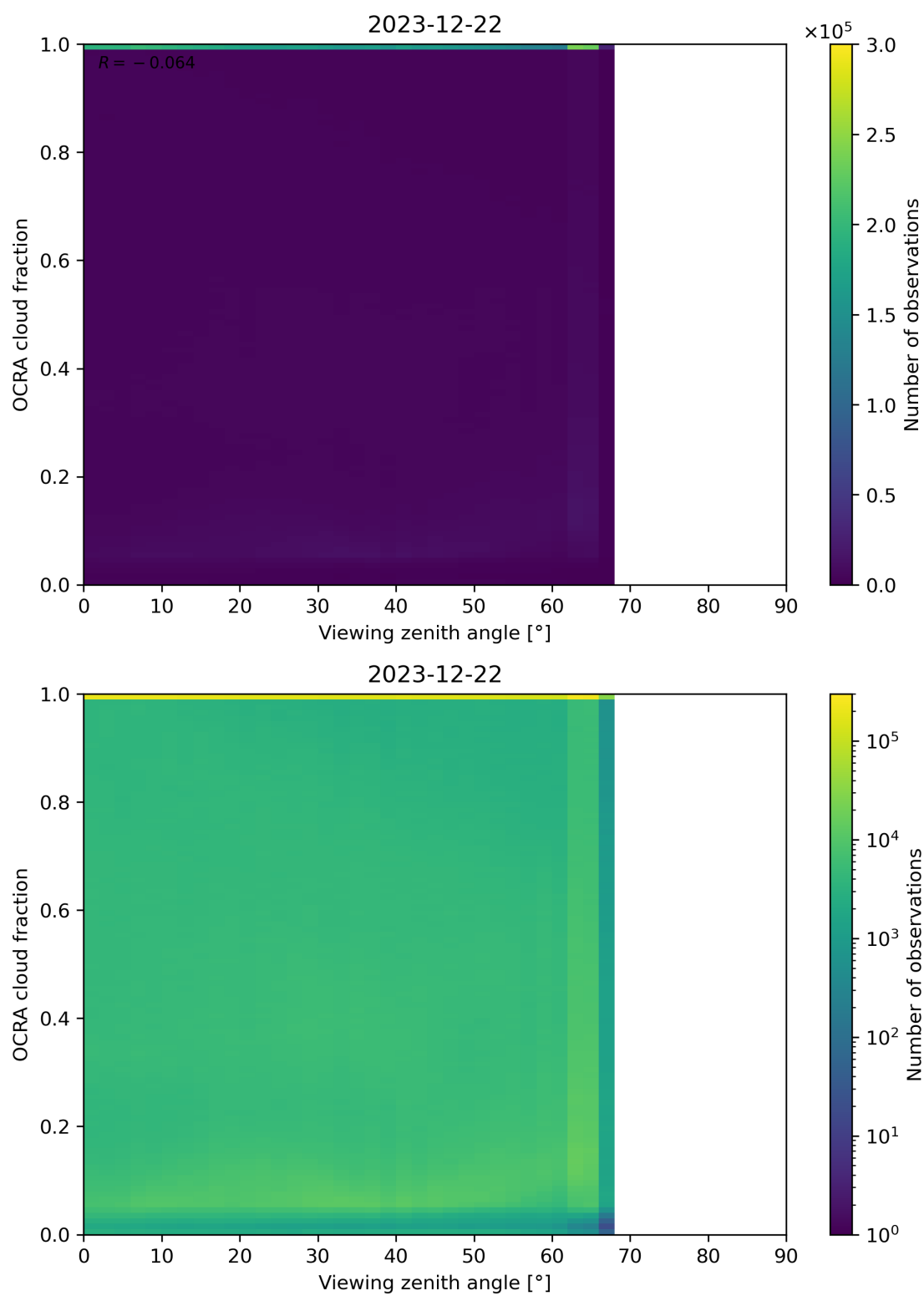
Figure 108: Scatter density plot of “Viewing zenith angle” against “OCRA cloud fraction” for 2023-12-21 to 2023-12-23.
