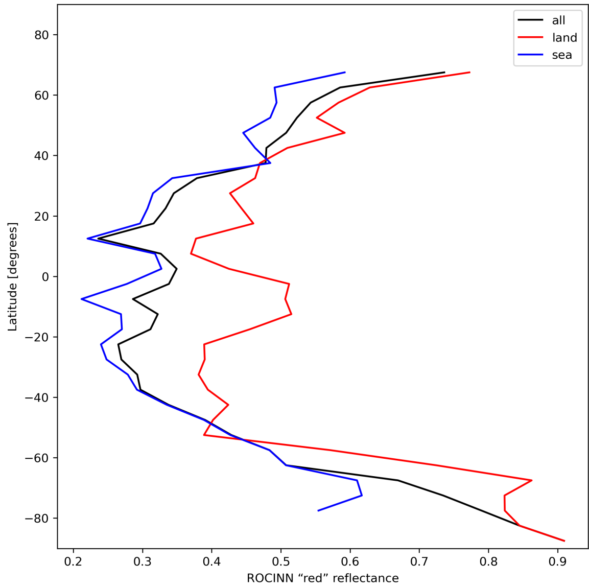
Figure 37: Zonal average of "ROCINN "red" reflectance" for 2023-12-21 to 2023-12-23.
