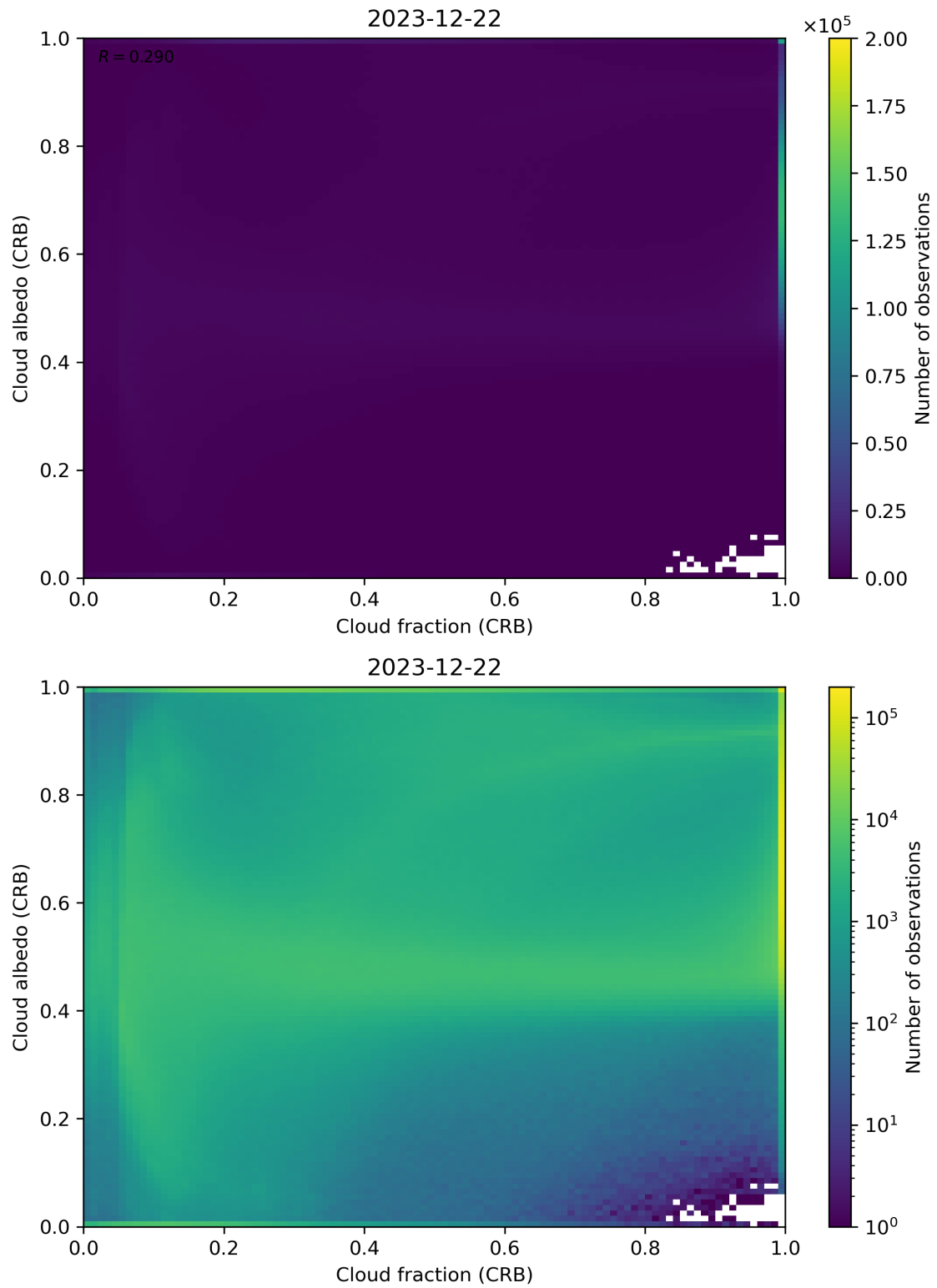
Figure 77: Scatter density plot of “Cloud fraction (CRB)” against “Cloud albedo (CRB)” for 2023-12-21 to 2023-12-23.
