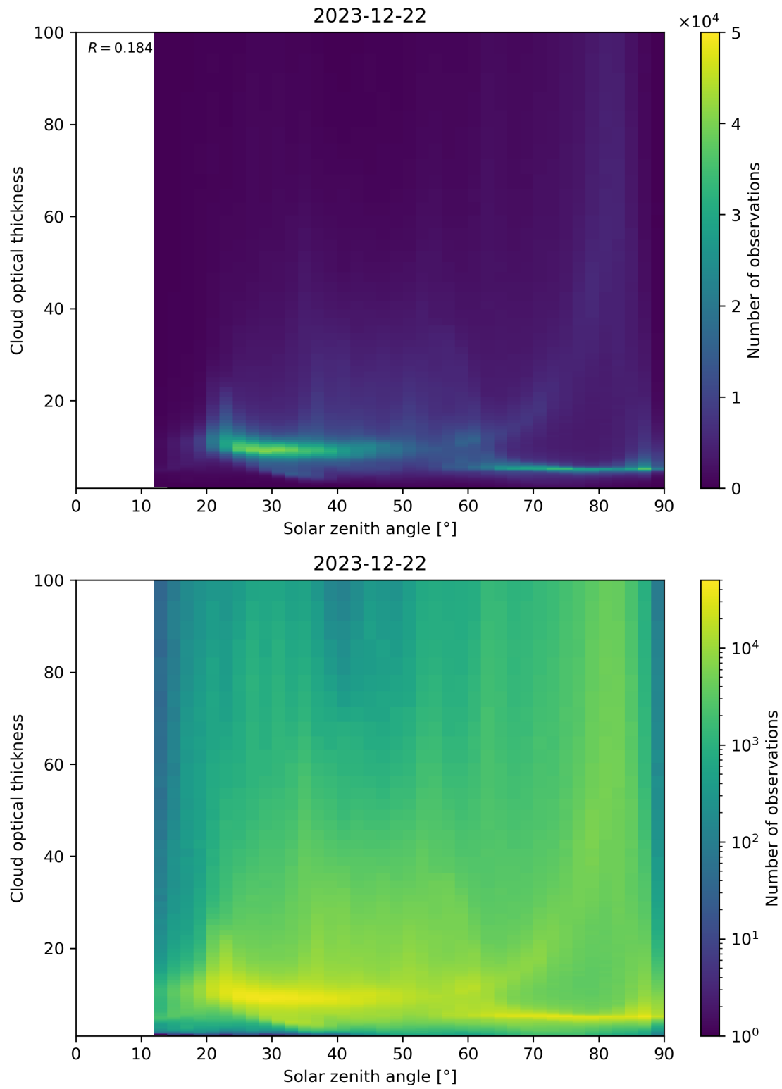
Figure 103: Scatter density plot of “Solar zenith angle” against “Cloud optical thickness” for 2023-12-21 to 2023-12-23.
