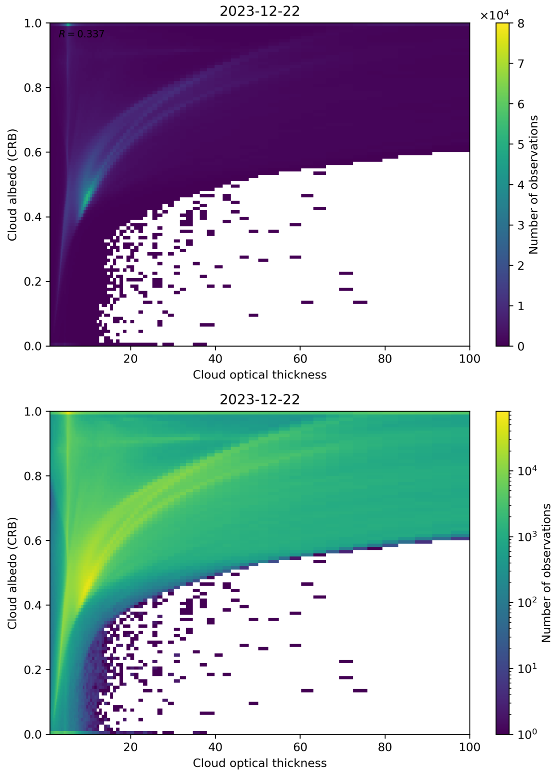
Figure 82: Scatter density plot of “Cloud optical thickness” against “Cloud albedo (CRB)” for 2023-12-21 to 2023-12-23.
