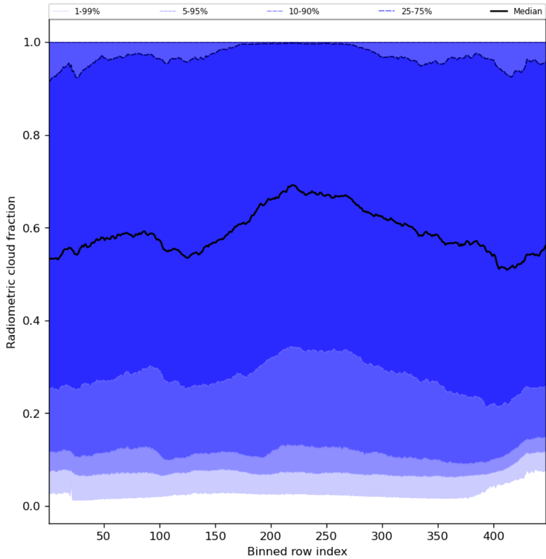
Figure 55: Along track statistics of “Radiometric cloud fraction” for 2023-12-21 to 2023-12-23
