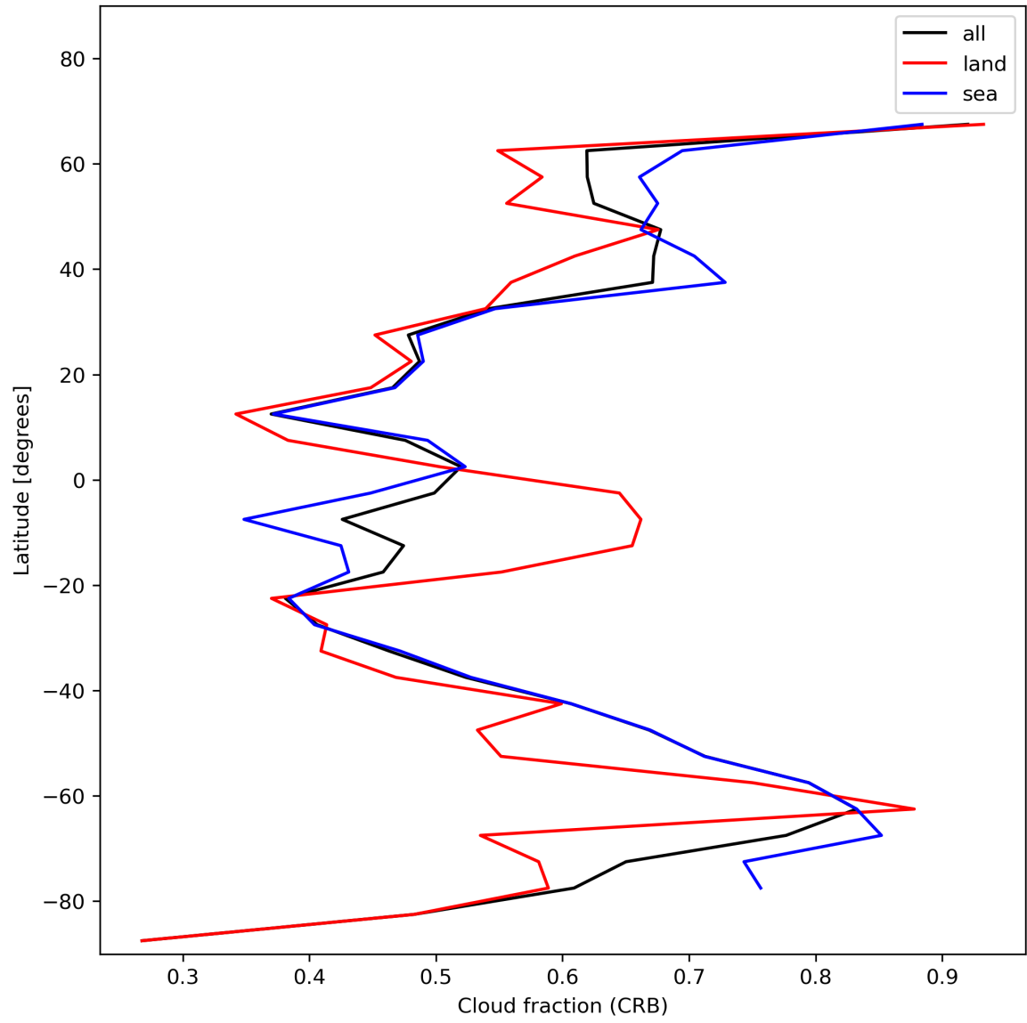
Figure 26: Zonal average of “Cloud fraction (CRB)” for 2023-12-21 to 2023-12-23.
