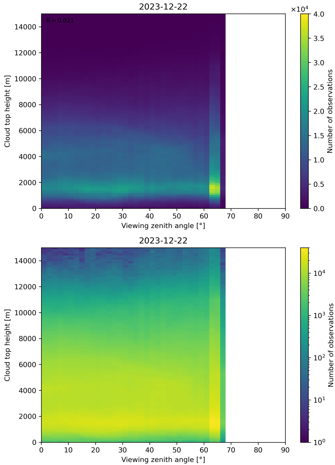
Figure 112: Scatter density plot of “Viewing zenith angle” against “Cloud top height” for 2023-12-21 to 2023-12-23.
