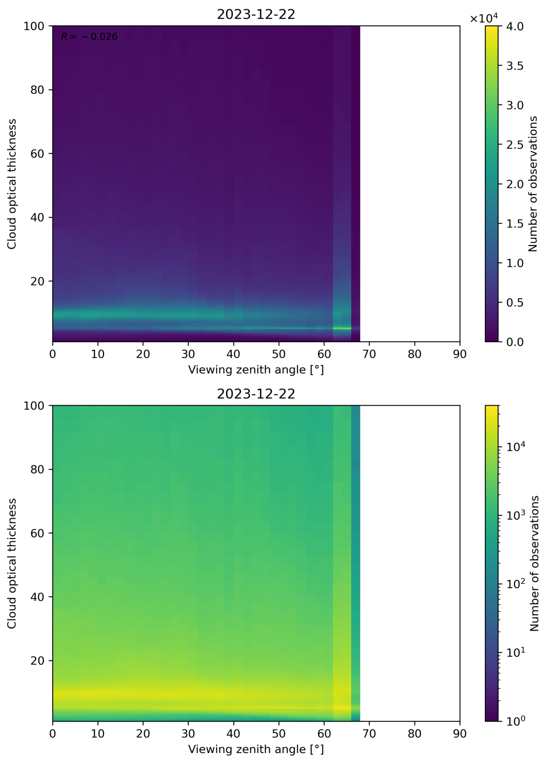
Figure 111: Scatter density plot of “Viewing zenith angle” against “Cloud optical thickness” for 2023-12-21 to 2023-12-23.
