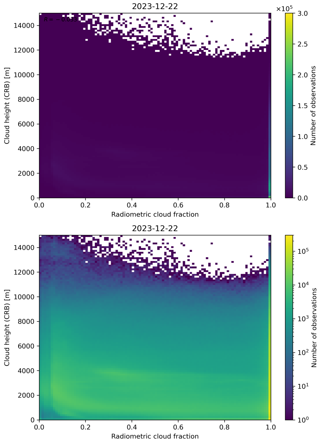
Figure 74: Scatter density plot of “Radiometric cloud fraction” against “Cloud height (CRB)” for 2023-12-21 to 2023-12-23.
