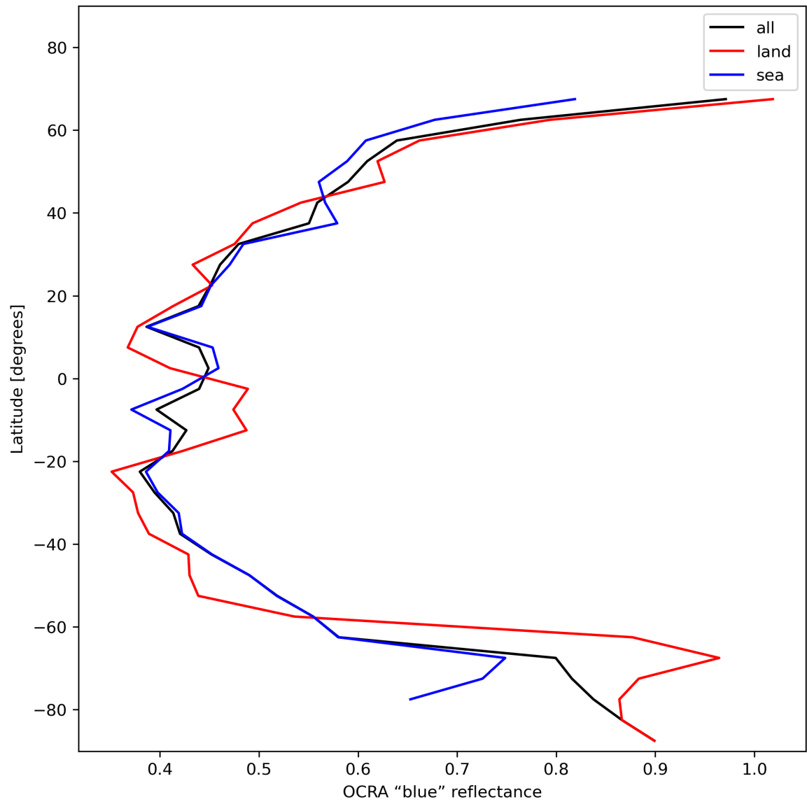
Figure 35: Zonal average of “OCRA “blue” reflectance” for 2023-12-21 to 2023-12-23.
