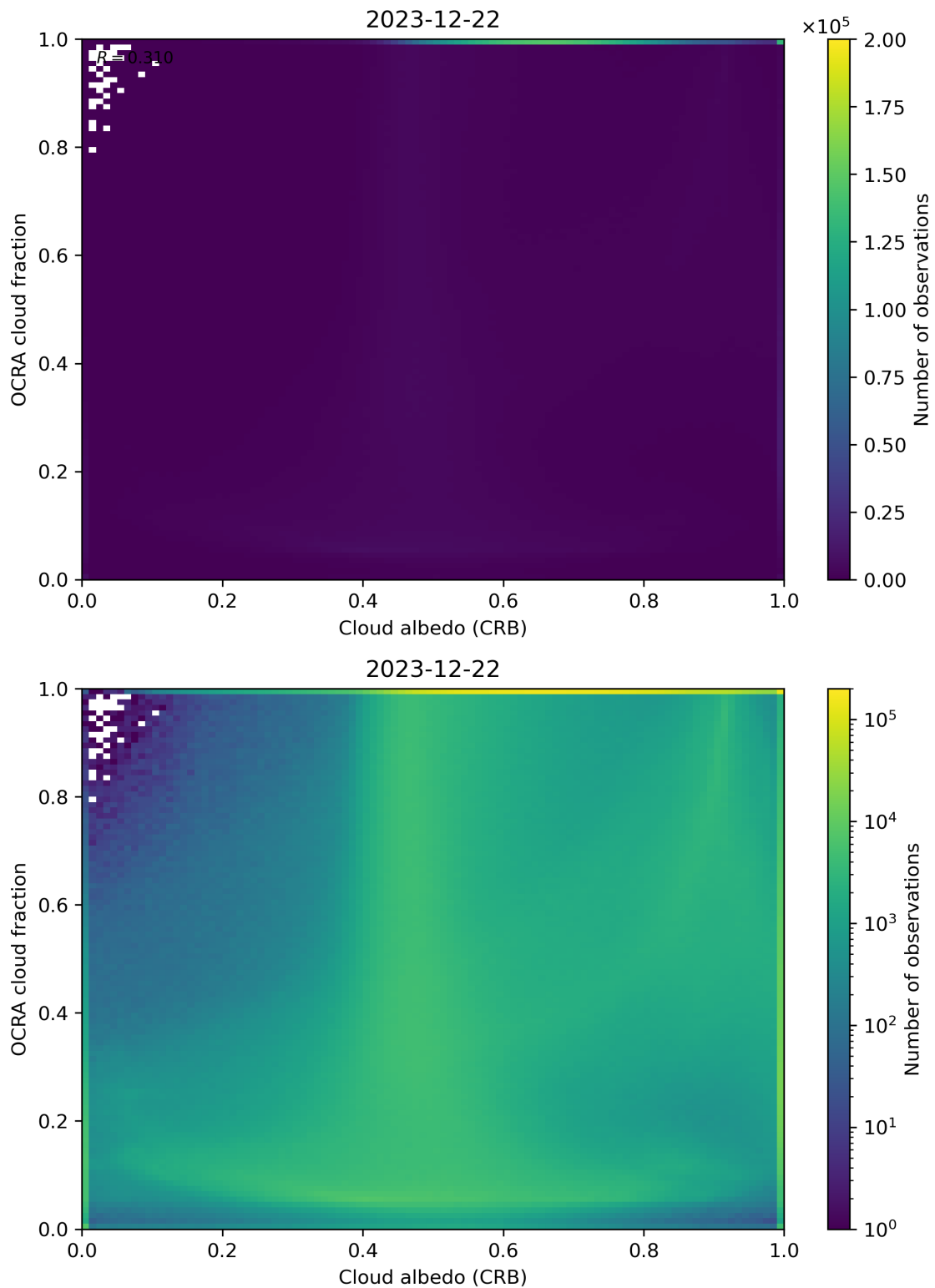
Figure 70: Scatter density plot of “Cloud albedo (CRB)” against “OCRA cloud fraction” for 2023-12-21 to 2023-12-23.
