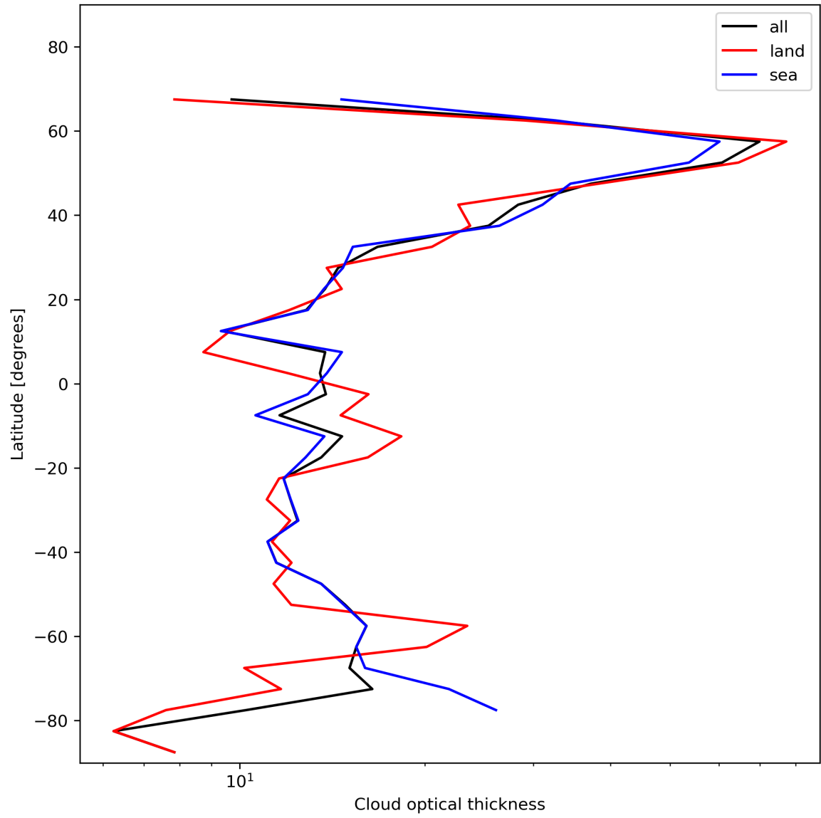
Figure 25: Zonal average of “Cloud optical thickness” for 2023-12-21 to 2023-12-23.
