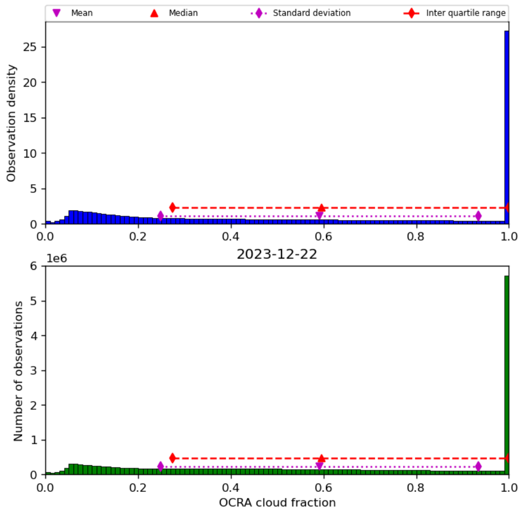
Figure 50: Histogram of “OCRA cloud fraction” for 2023-12-21 to 2023-12-23
