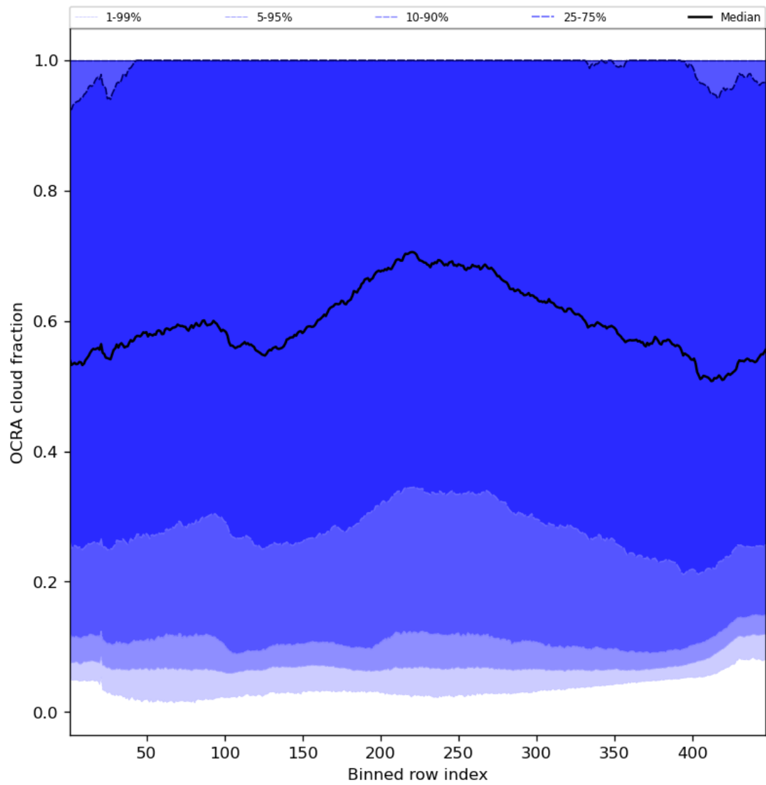
Figure 66: Along track statistics of “OCRA cloud fraction” for 2023-12-21 to 2023-12-23
