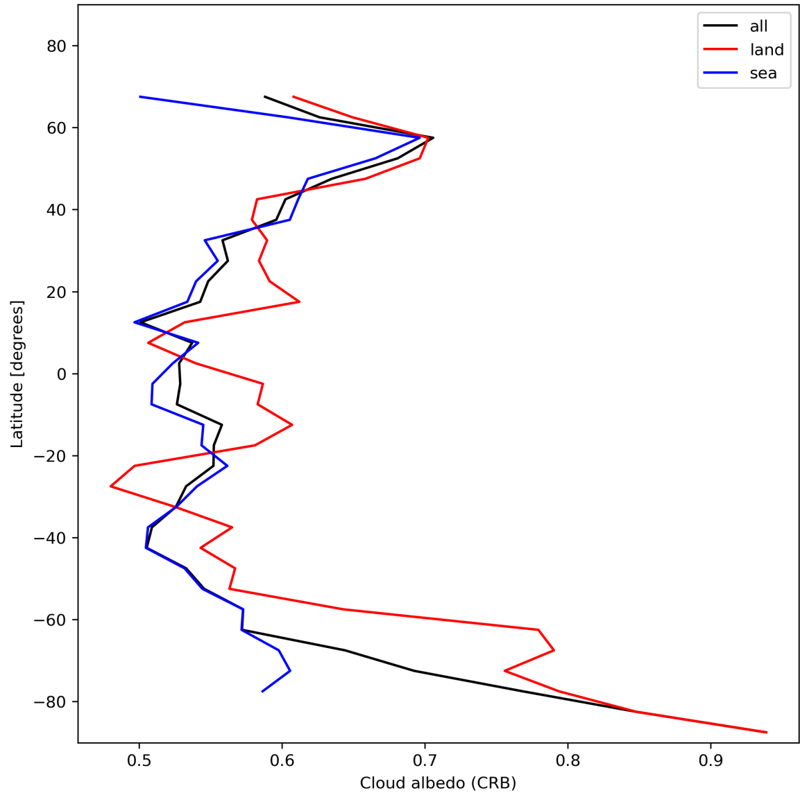
Figure 28: Zonal average of “Cloud albedo (CRB)” for 2023-12-21 to 2023-12-23.
