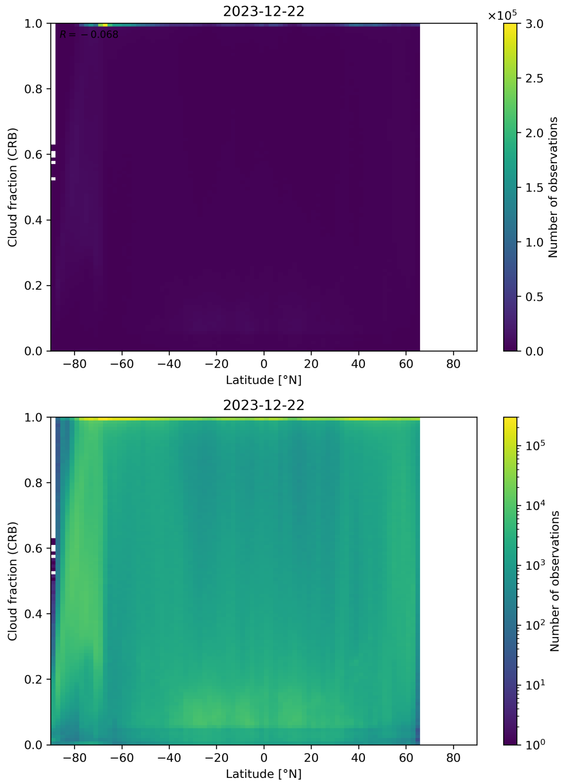
Figure 94: Scatter density plot of “Latitude” against “Cloud fraction (CRB)” for 2023-12-21 to 2023-12-23.
