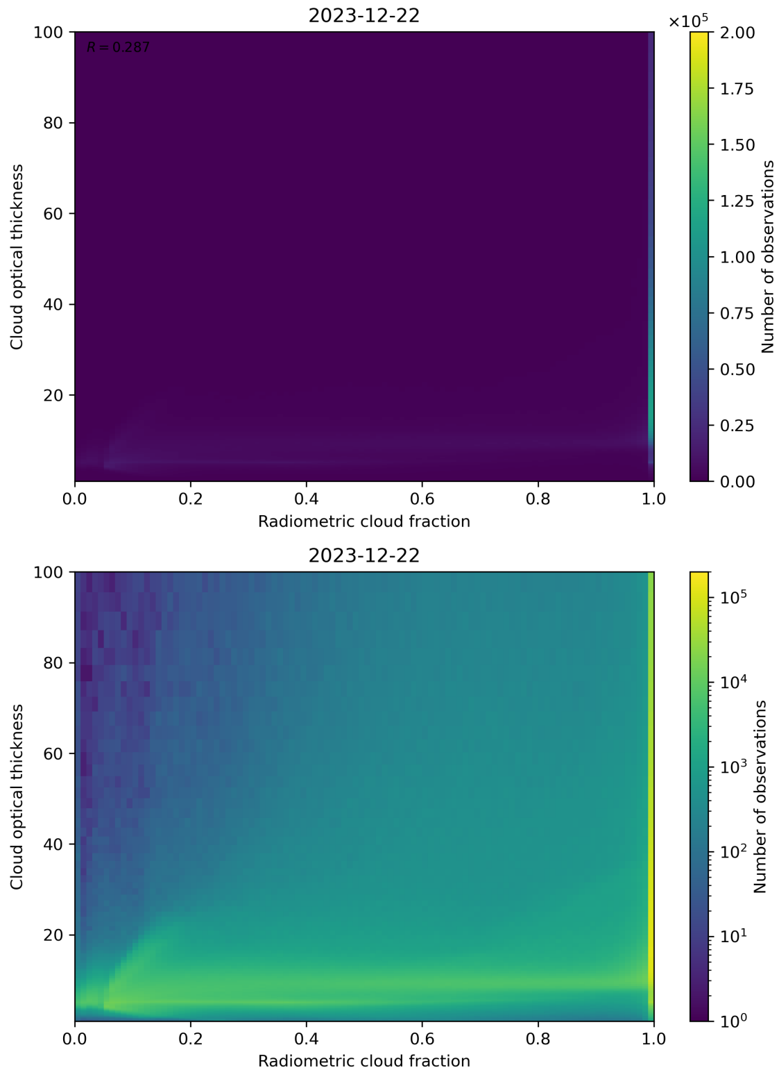
Figure 75: Scatter density plot of “Radiometric cloud fraction” against “Cloud optical thickness” for 2023-12-21 to 2023-12-23.
