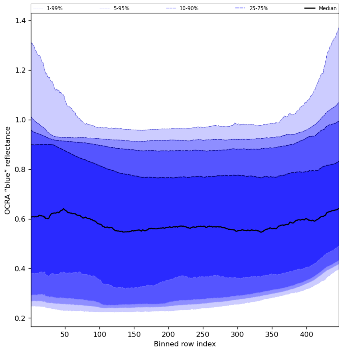
Figure 67: Along track statistics of “OCRA “blue” reflectance” for 2023-12-21 to 2023-12-23
