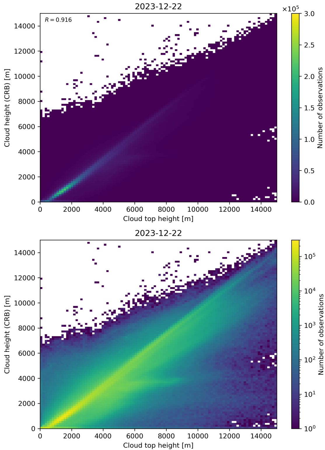
Figure 89: Scatter density plot of “Cloud top height” against “Cloud height (CRB)” for 2023-12-21 to 2023-12-23.
