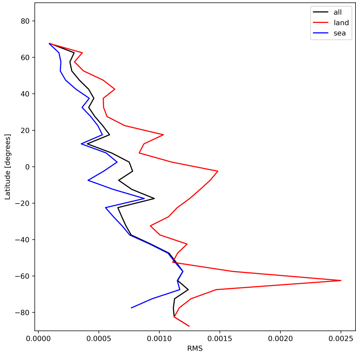
Figure 31: Zonal average of “RMS” for 2023-12-21 to 2023-12-23.
