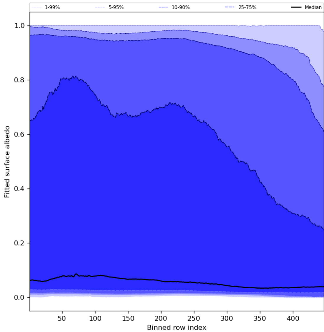
Figure 61: Along track statistics of “Fitted surface albedo” for 2023-12-21 to 2023-12-23
