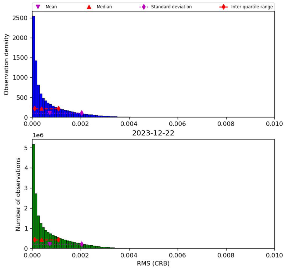
Figure 48: Histogram of “RMS (CRB)” for 2023-12-21 to 2023-12-23
