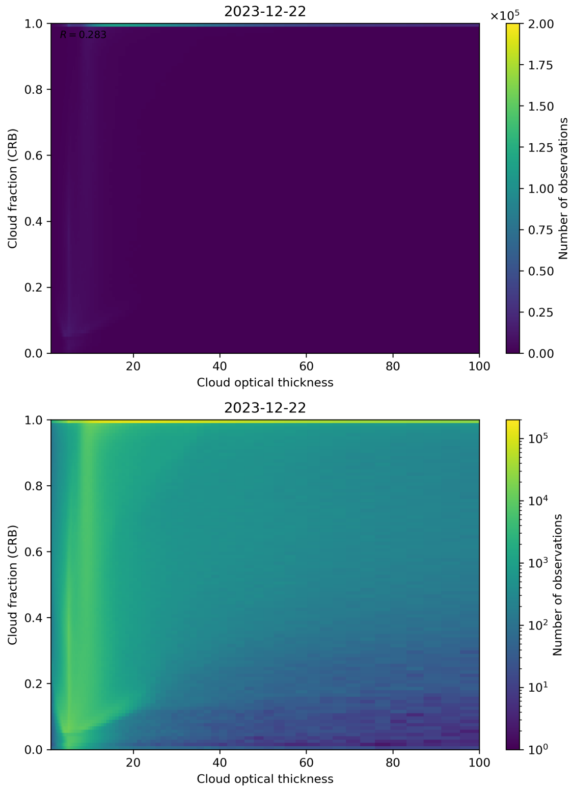
Figure 84: Scatter density plot of “Cloud optical thickness” against “Cloud fraction (CRB)” for 2023-12-21 to 2023-12-23.
