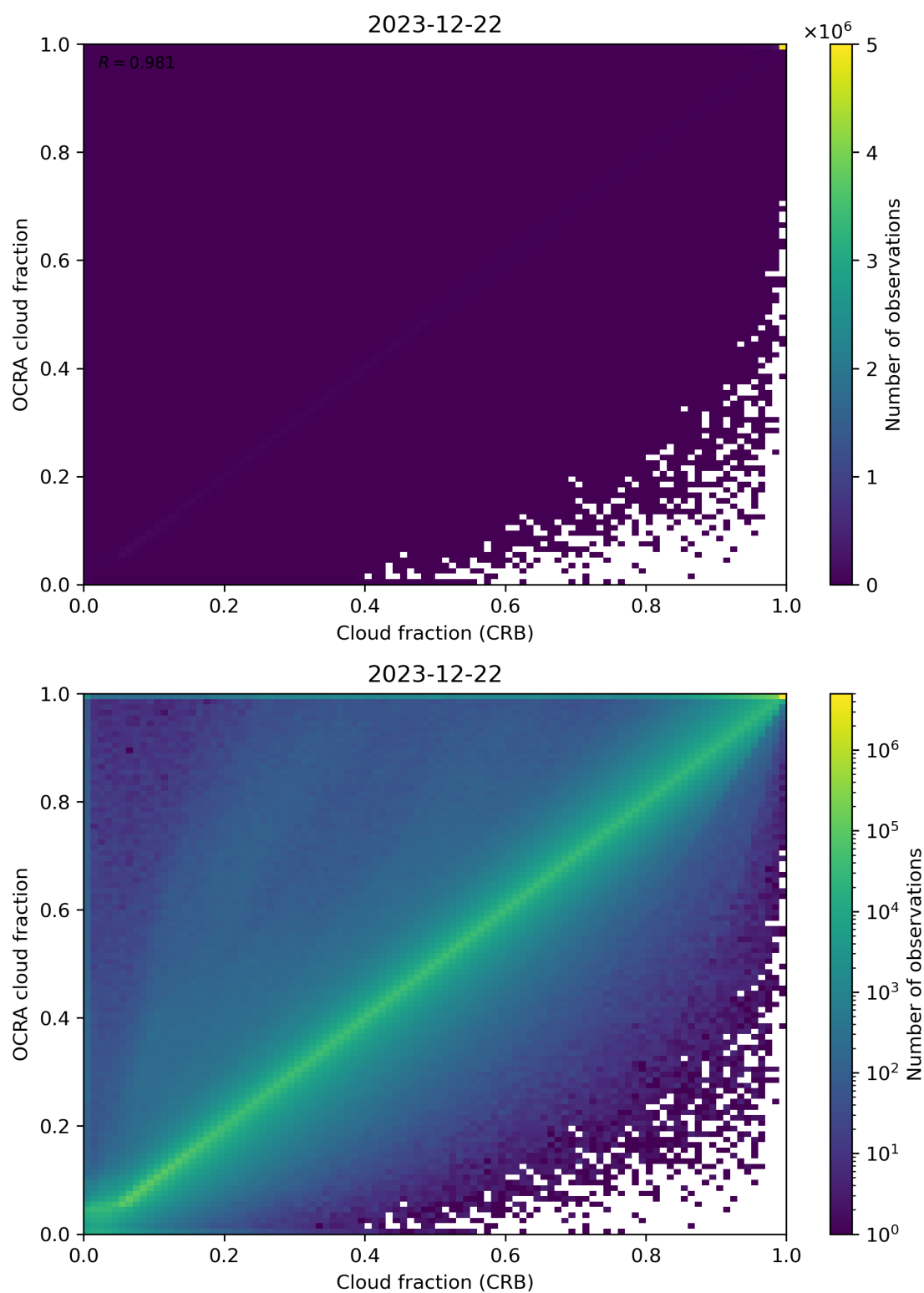
Figure 78: Scatter density plot of “Cloud fraction (CRB)” against “OCRA cloud fraction” for 2023-12-21 to 2023-12-23.
