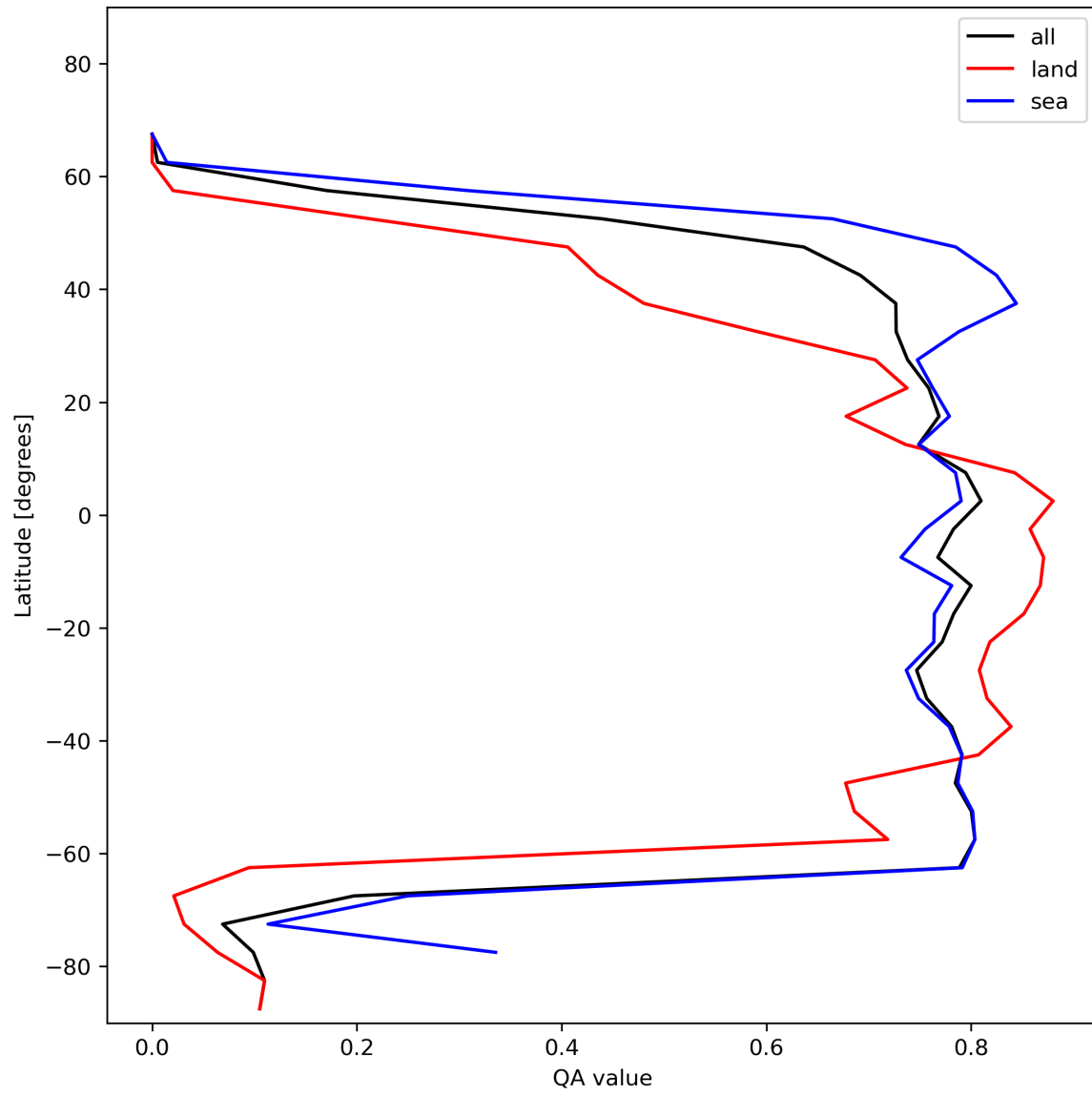
Figure 22: Zonal average of “QA value” for 2023-12-21 to 2023-12-23.
