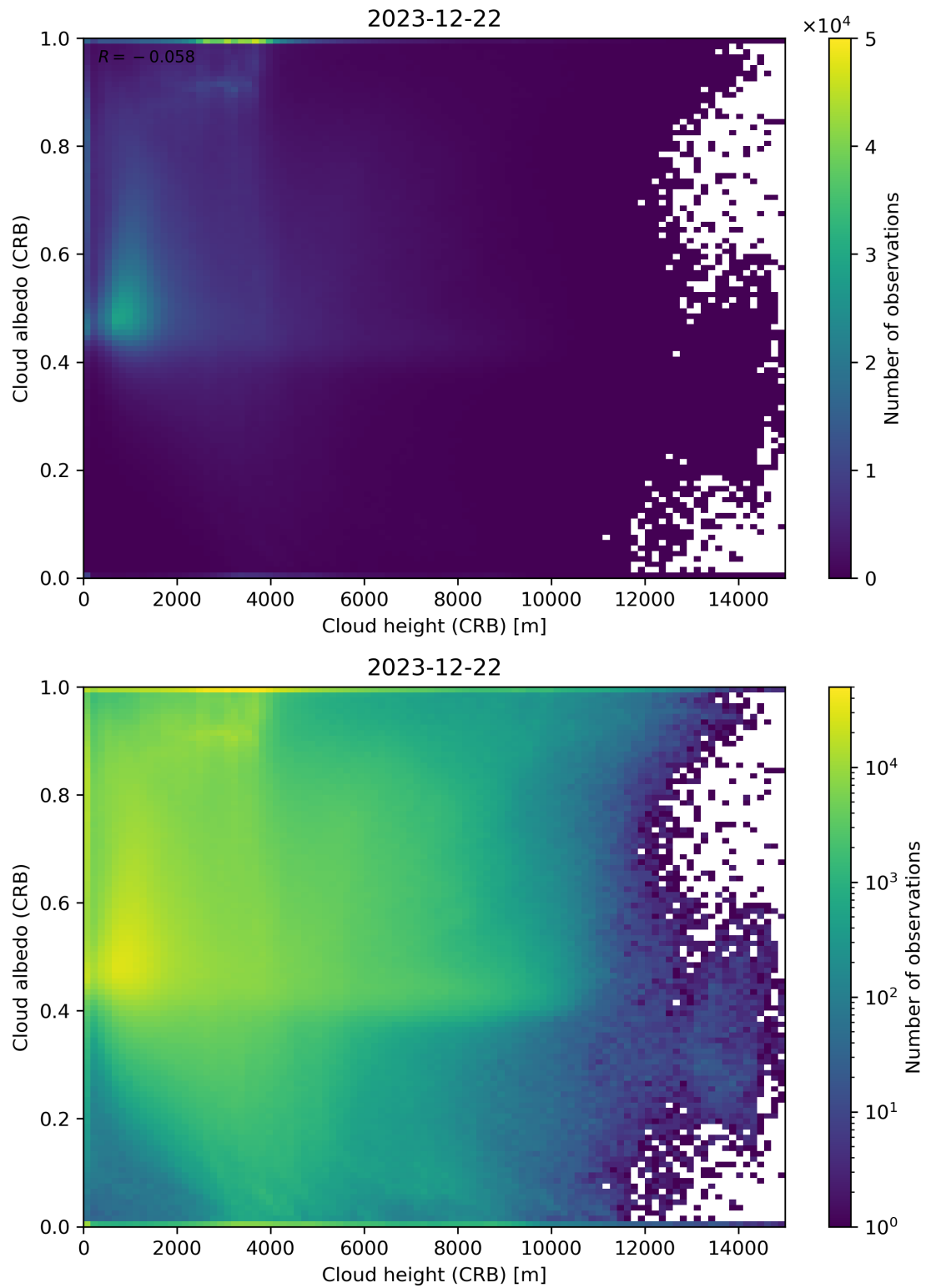
Figure 80: Scatter density plot of “Cloud height (CRB)” against “Cloud albedo (CRB)” for 2023-12-21 to 2023-12-23.
