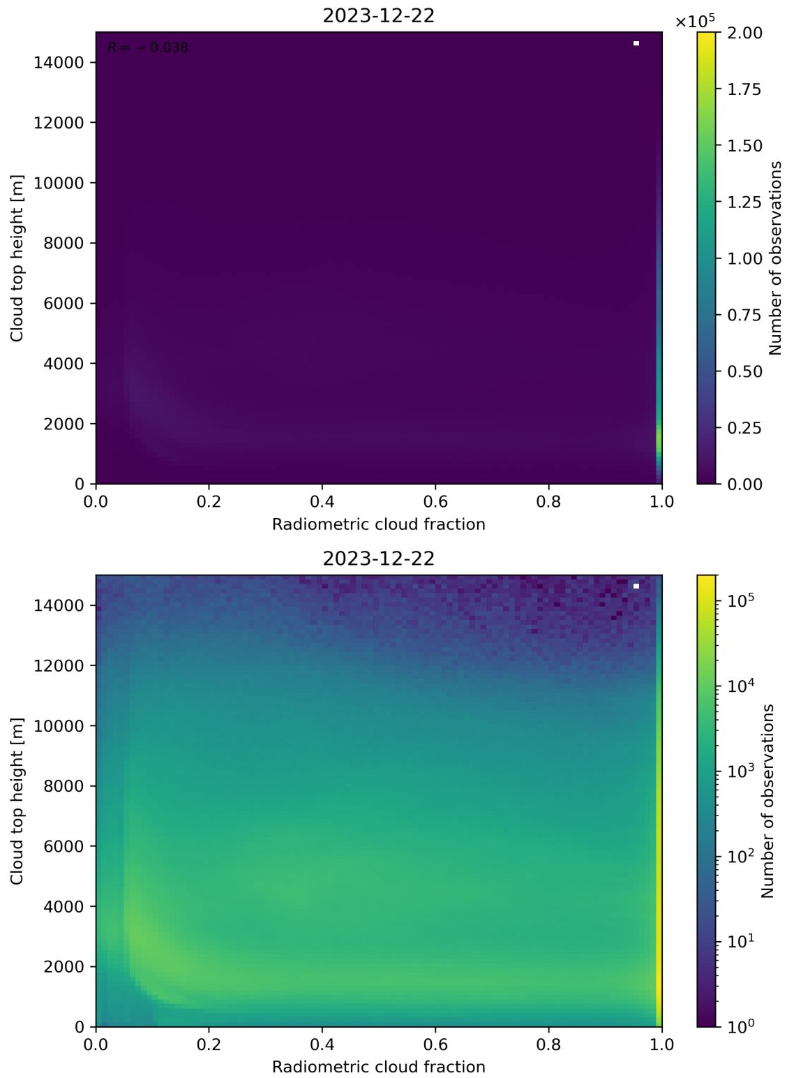
Figure 76: Scatter density plot of “Radiometric cloud fraction” against “Cloud top height” for 2023-12-21 to 2023-12-23.
