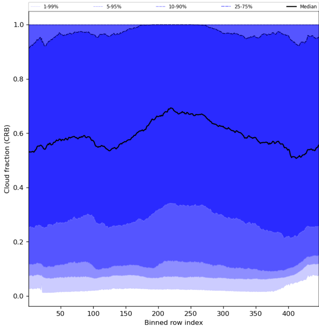
Figure 58: Along track statistics of “Cloud fraction (CRB)” for 2023-12-21 to 2023-12-23
