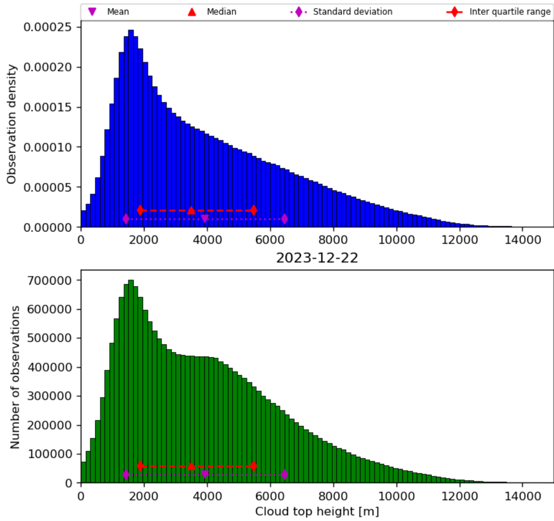
Figure 40: Histogram of “Cloud top height” for 2023-12-21 to 2023-12-23
