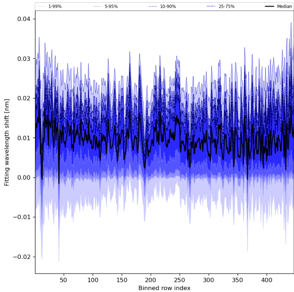
Figure 65: Along track statistics of “Fitting wavelength shift” for 2023-12-21 to 2023-12-23
