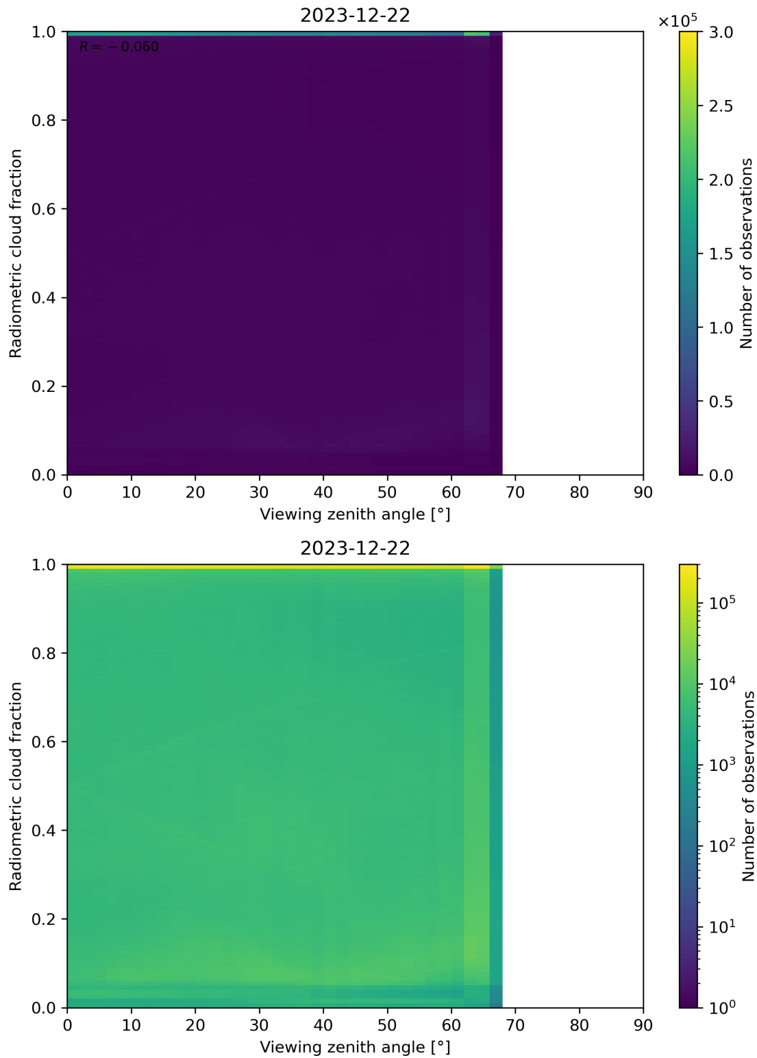
Figure 107: Scatter density plot of “Viewing zenith angle” against “Radiometric cloud fraction” for 2023-12-21 to 2023-12-23.
