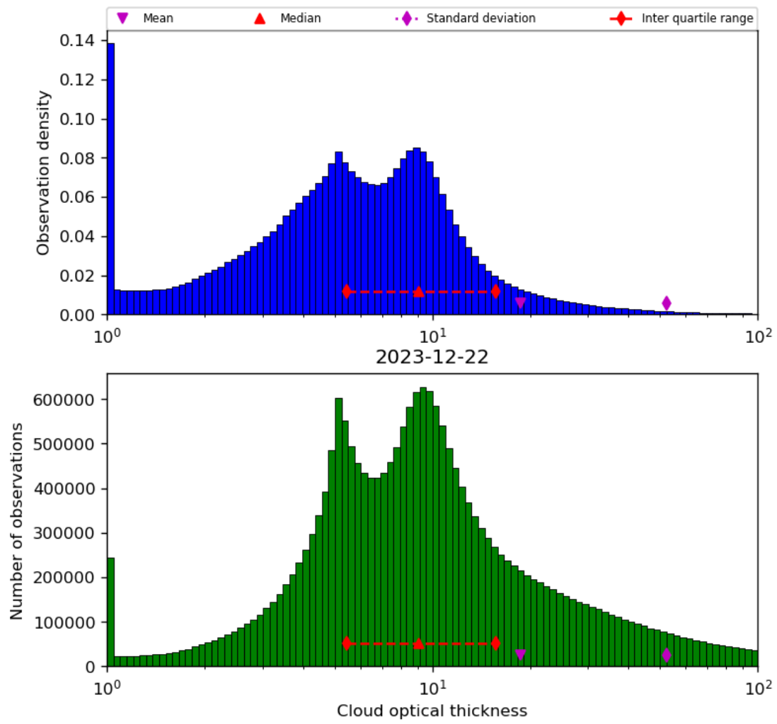
Figure 41: Histogram of “Cloud optical thickness” for 2023-12-21 to 2023-12-23
