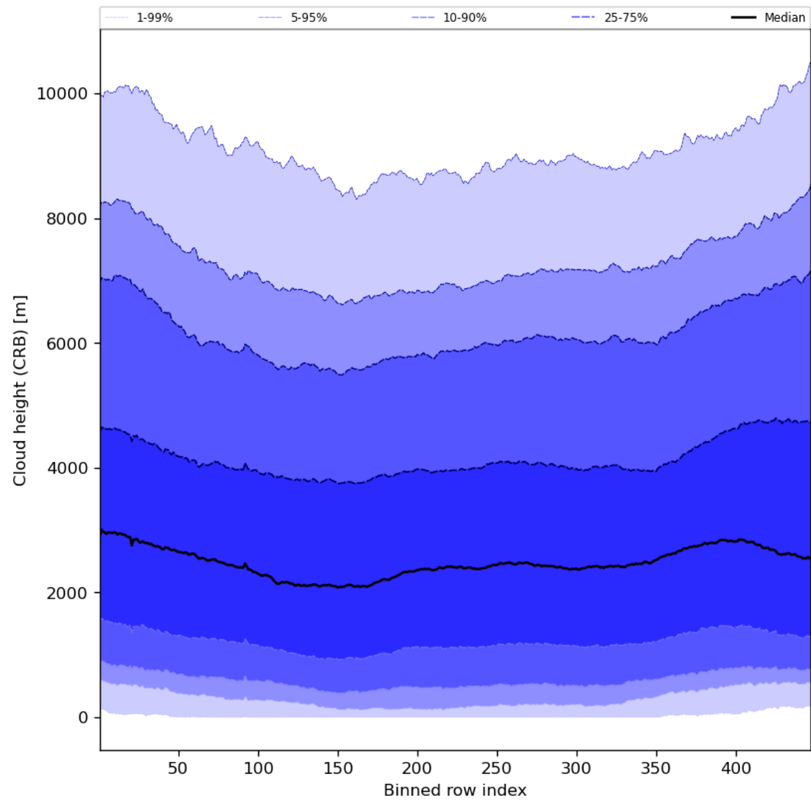
Figure 59: Along track statistics of “Cloud height (CRB)” for 2023-12-21 to 2023-12-23
