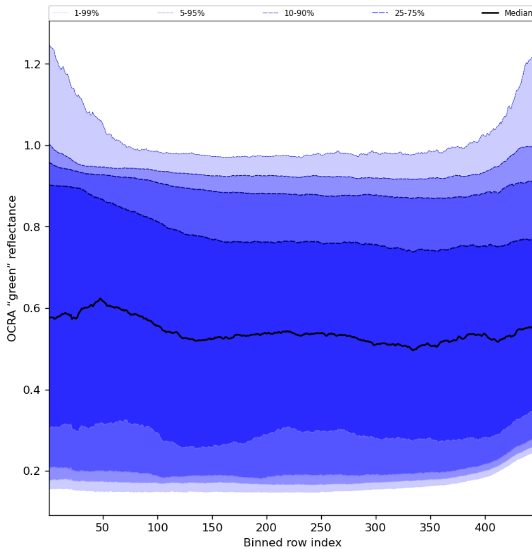
Figure 68: Along track statistics of “OCRA “green” reflectance” for 2023-12-21 to 2023-12-23
