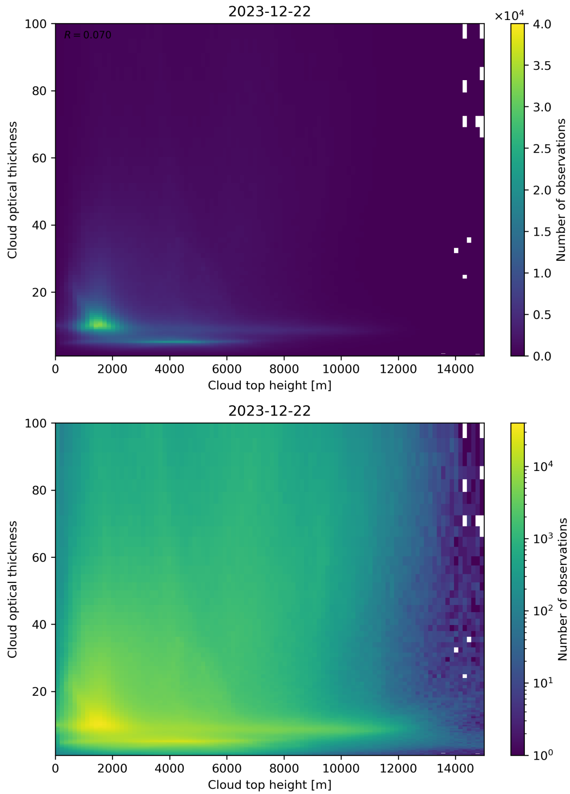
Figure 90: Scatter density plot of “Cloud top height” against “Cloud optical thickness” for 2023-12-21 to 2023-12-23.
