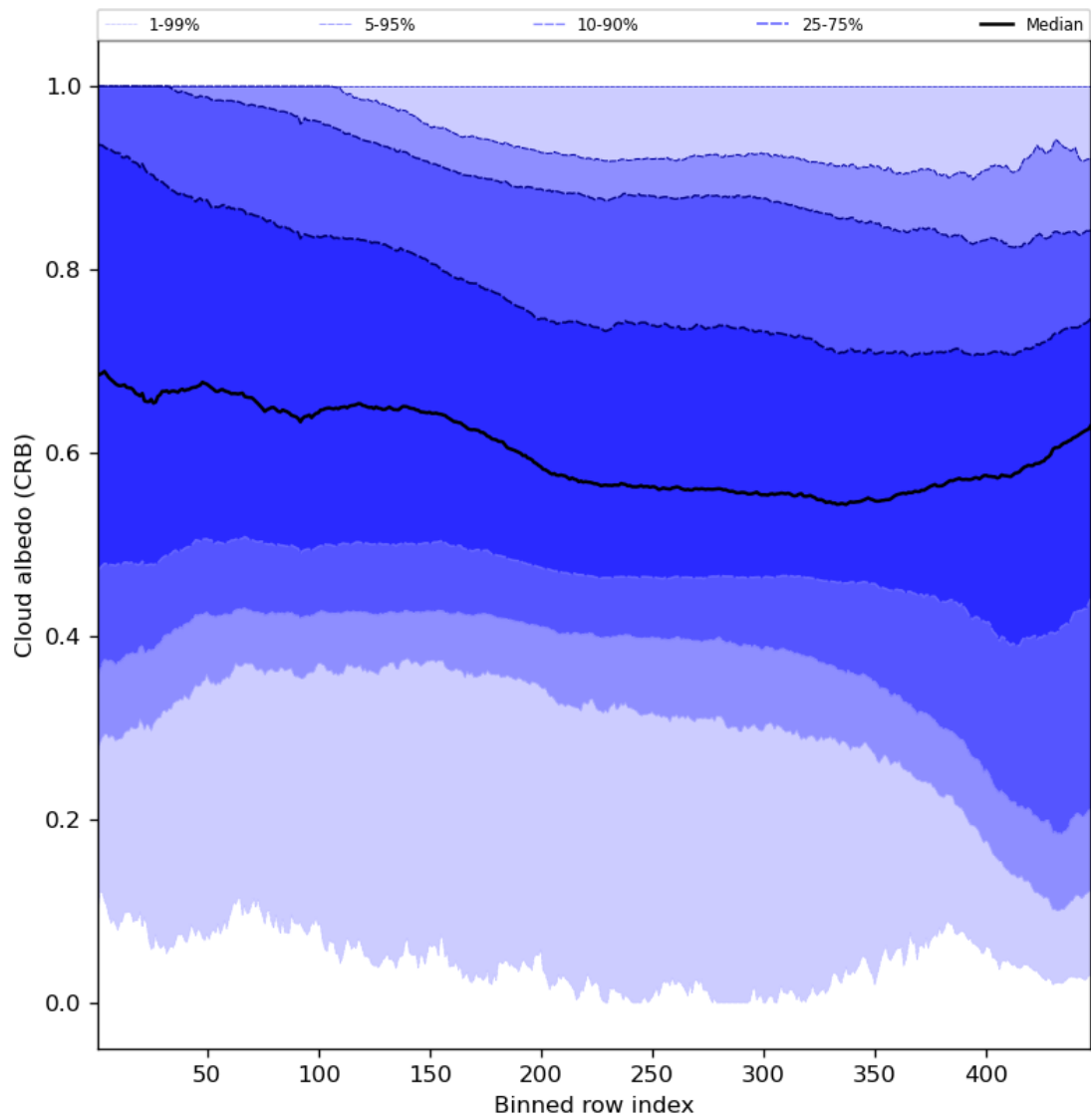
Figure 60: Along track statistics of “Cloud albedo (CRB)” for 2023-12-21 to 2023-12-23
