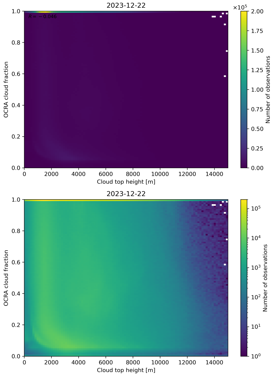
Figure 87: Scatter density plot of “Cloud top height” against “OCRA cloud fraction” for 2023-12-21 to 2023-12-23.
