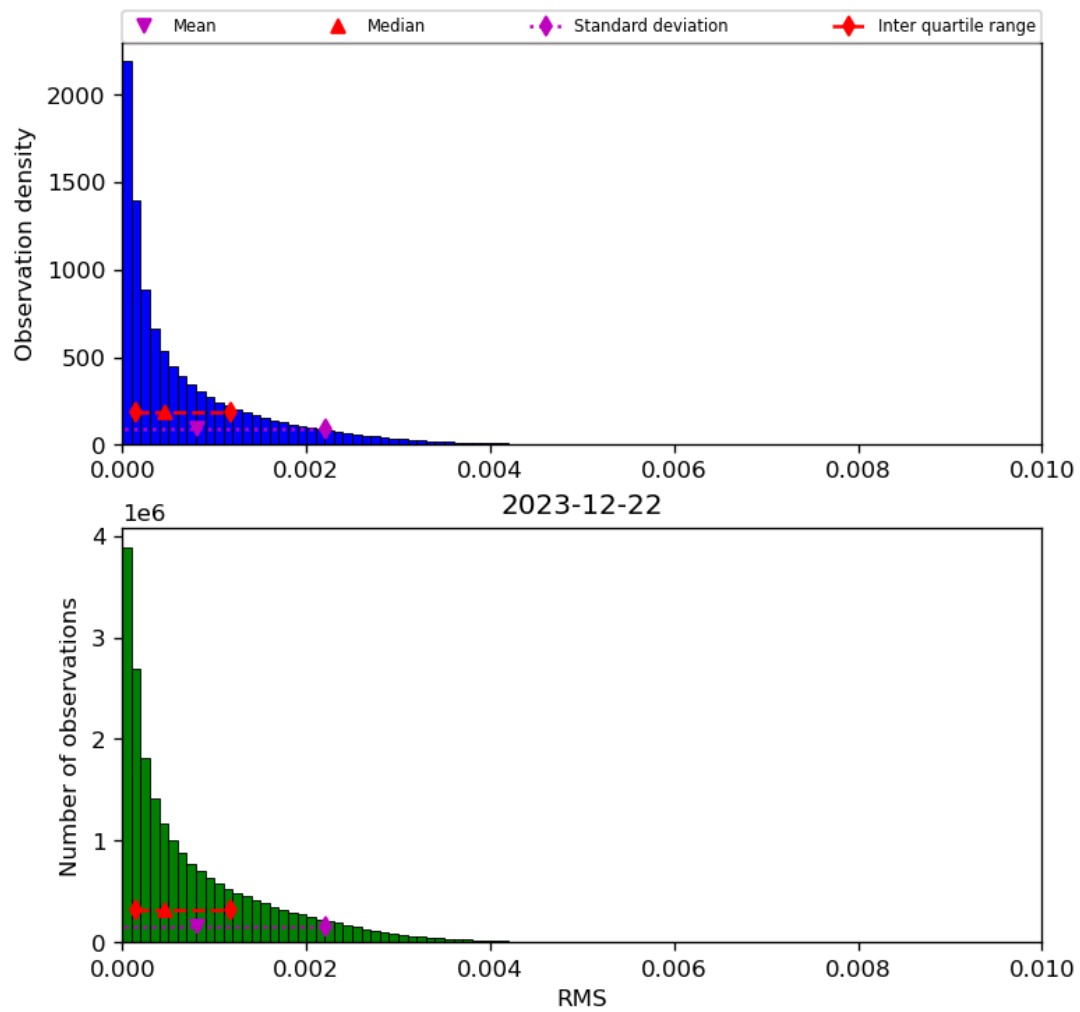
Figure 47: Histogram of “RMS” for 2023-12-21 to 2023-12-23
