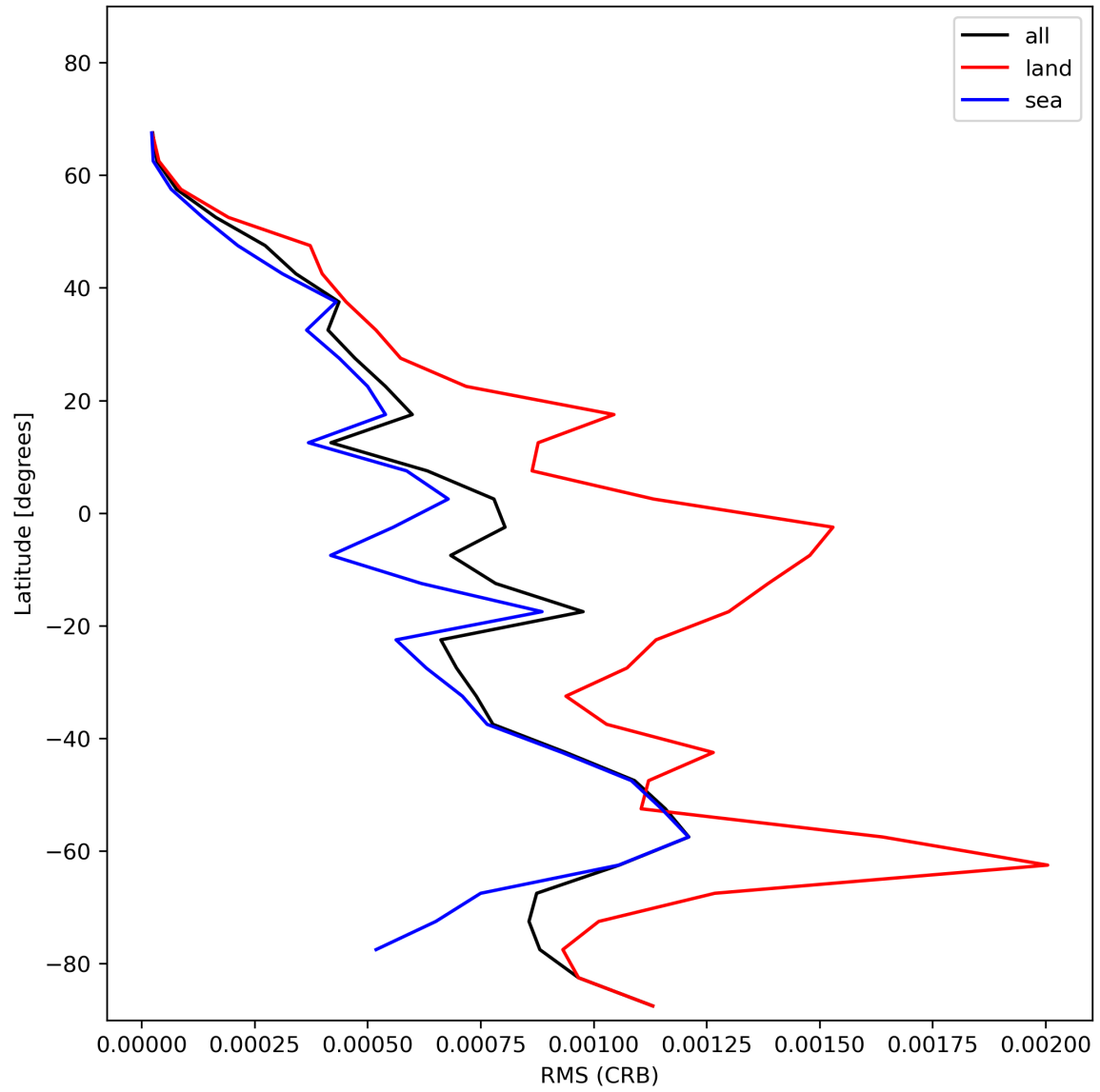
Figure 32: Zonal average of “RMS (CRB)” for 2023-12-21 to 2023-12-23.
