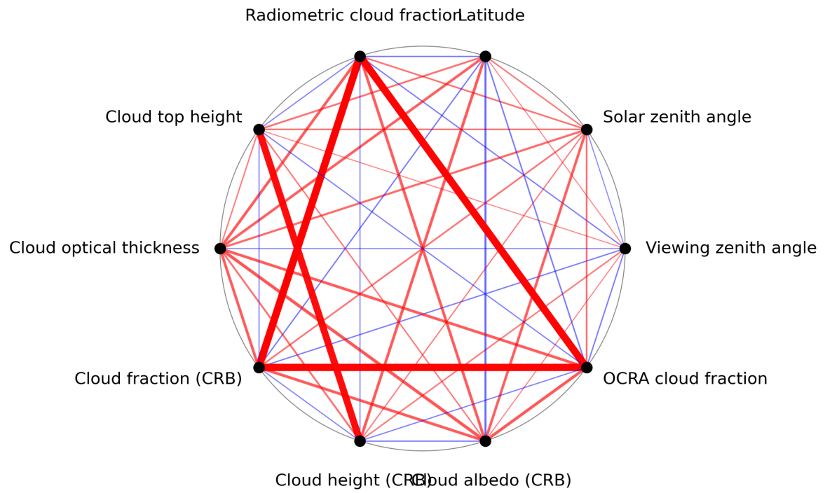
Figure 1: Map of correlation graph for 2023-12-21 to 2023-12-23.
