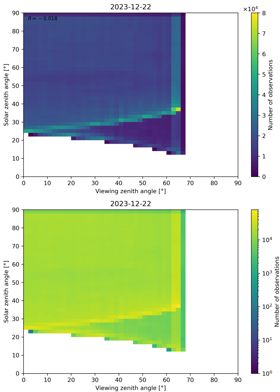
Figure 114: Scatter density plot of “Viewing zenith angle” against “Solar zenith angle” for 2023-12-21 to 2023-12-23.
