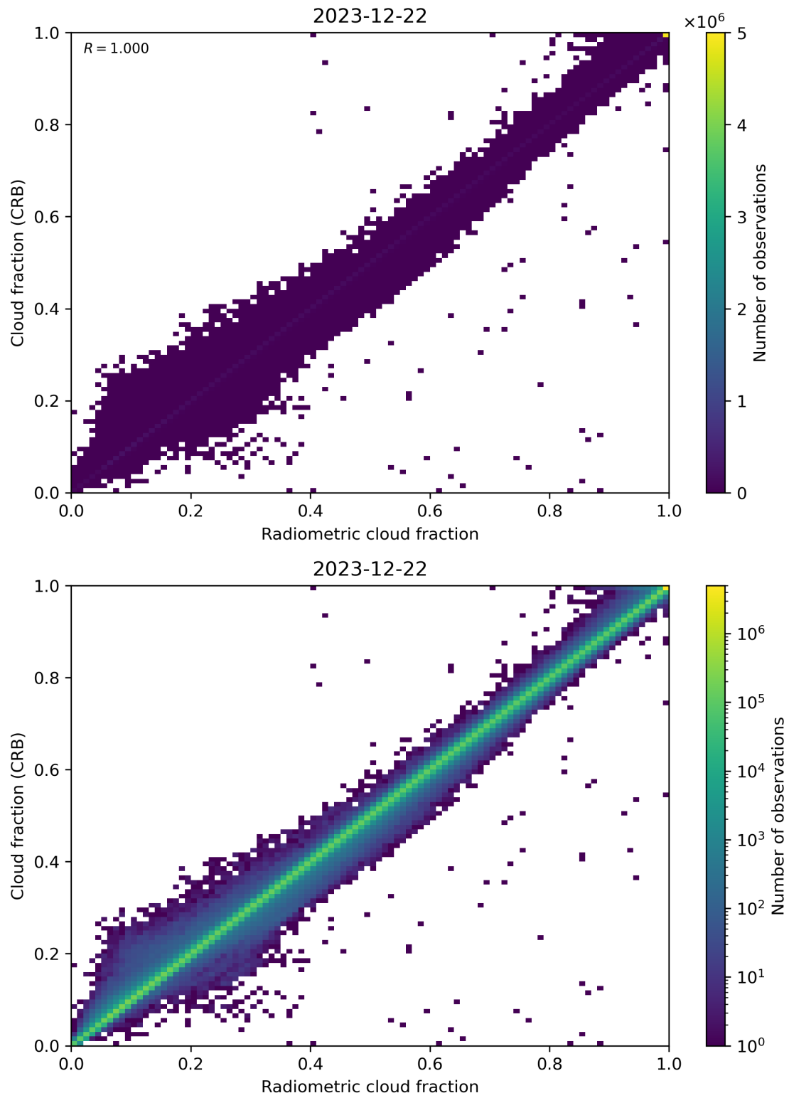
Figure 73: Scatter density plot of “Radiometric cloud fraction” against “Cloud fraction (CRB)” for 2023-12-21 to 2023-12-23.
