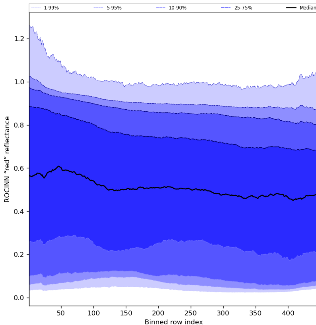
Figure 69: Along track statistics of “ROCINN “red” reflectance” for 2023-12-21 to 2023-12-23
