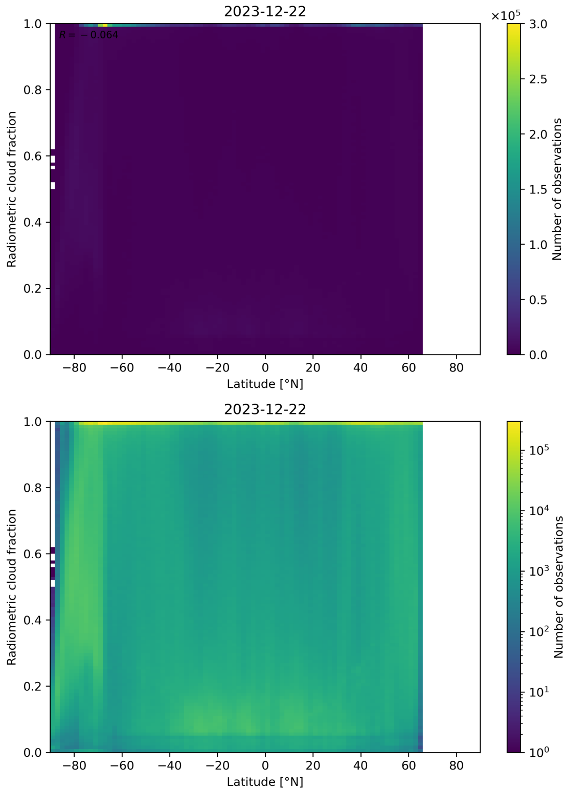
Figure 92: Scatter density plot of “Latitude” against “Radiometric cloud fraction” for 2023-12-21 to 2023-12-23.
