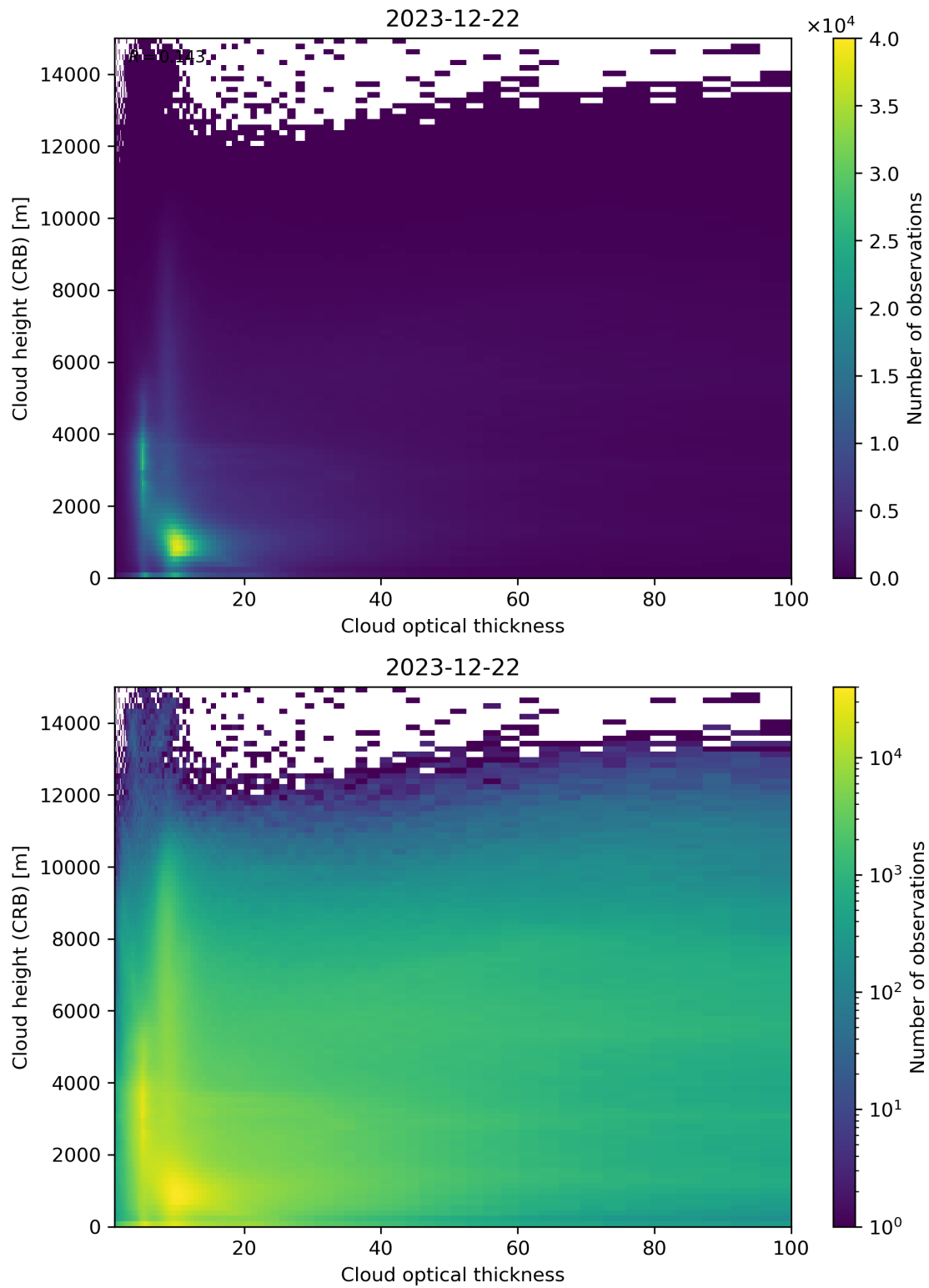
Figure 85: Scatter density plot of “Cloud optical thickness” against “Cloud height (CRB)” for 2023-12-21 to 2023-12-23.
