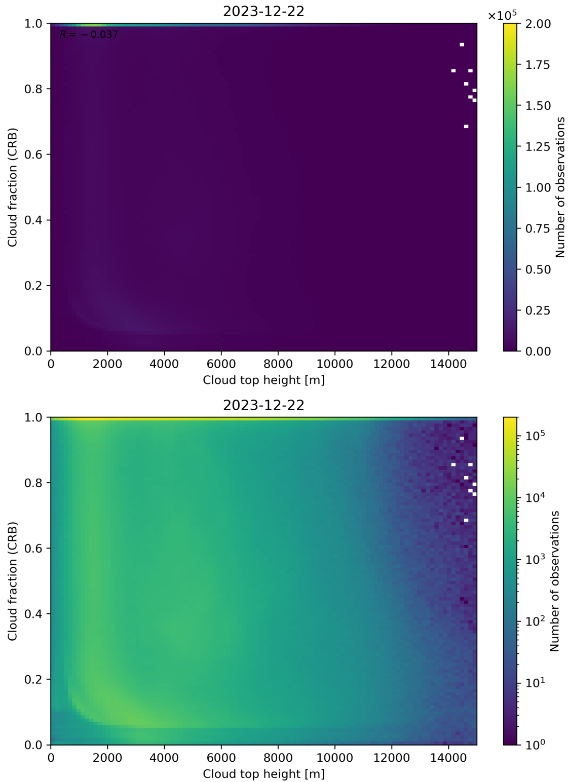
Figure 88: Scatter density plot of “Cloud top height” against “Cloud fraction (CRB)” for 2023-12-21 to 2023-12-23.
