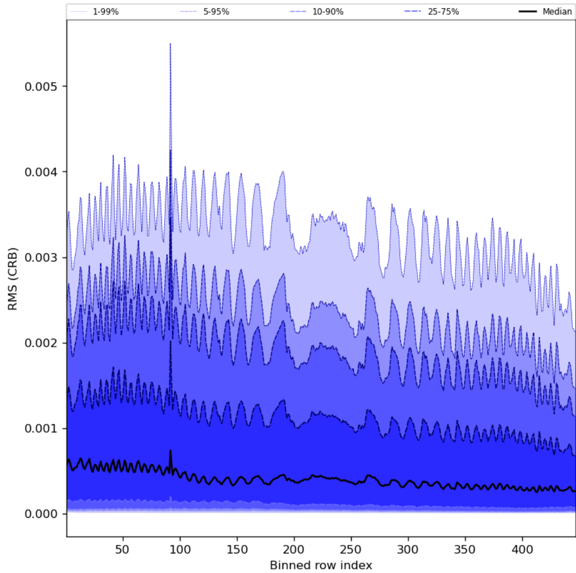
Figure 64: Along track statistics of “RMS (CRB)” for 2023-12-21 to 2023-12-23
