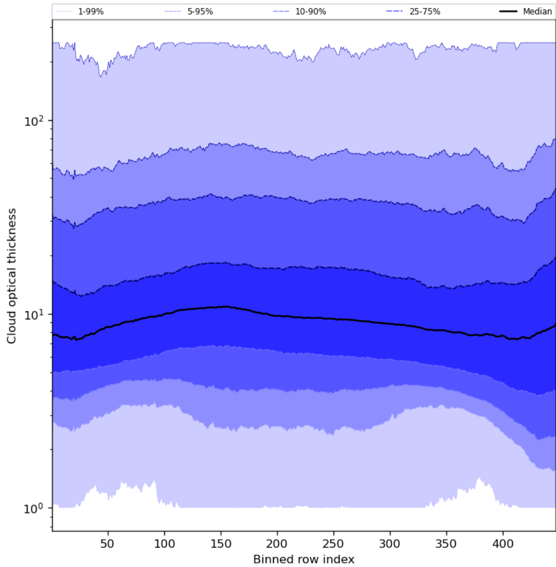
Figure 57: Along track statistics of “Cloud optical thickness” for 2023-12-21 to 2023-12-23
