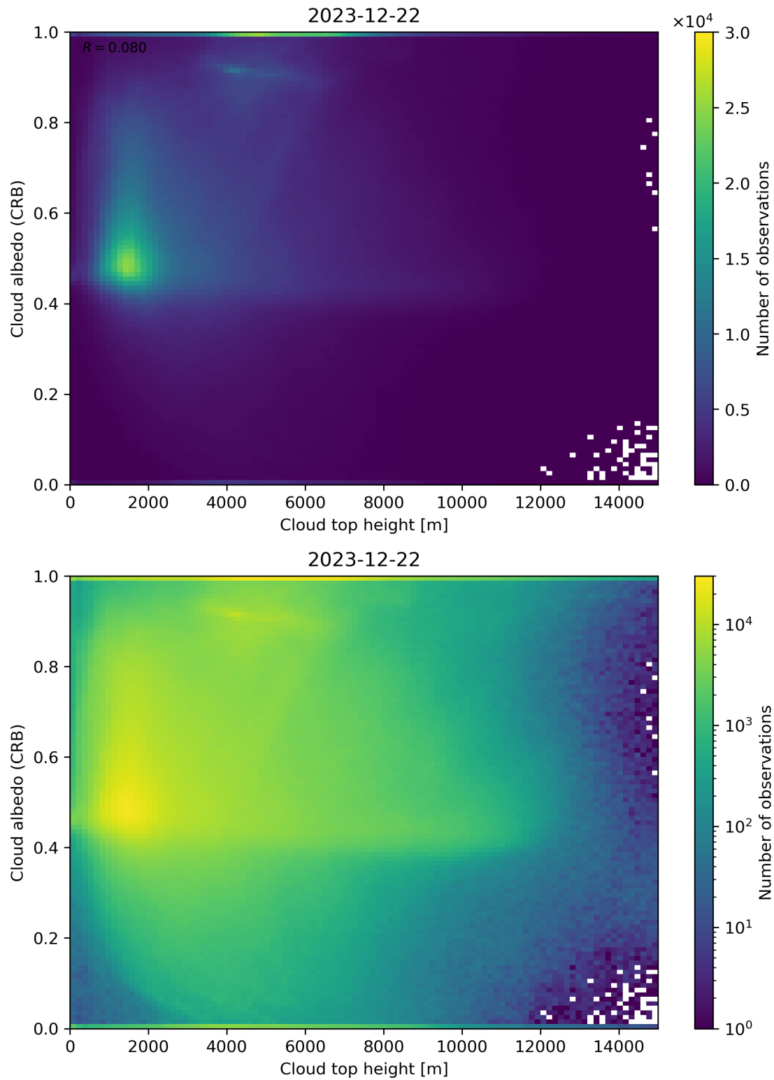
Figure 86: Scatter density plot of “Cloud top height” against “Cloud albedo (CRB)” for 2023-12-21 to 2023-12-23.
