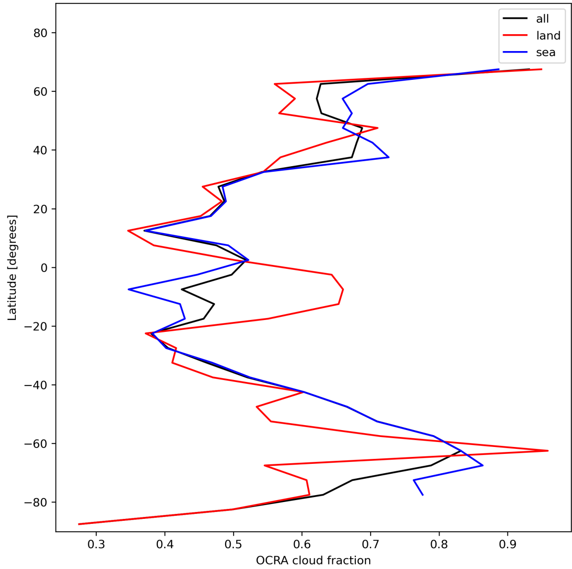
Figure 34: Zonal average of “OCRA cloud fraction” for 2023-12-21 to 2023-12-23.
