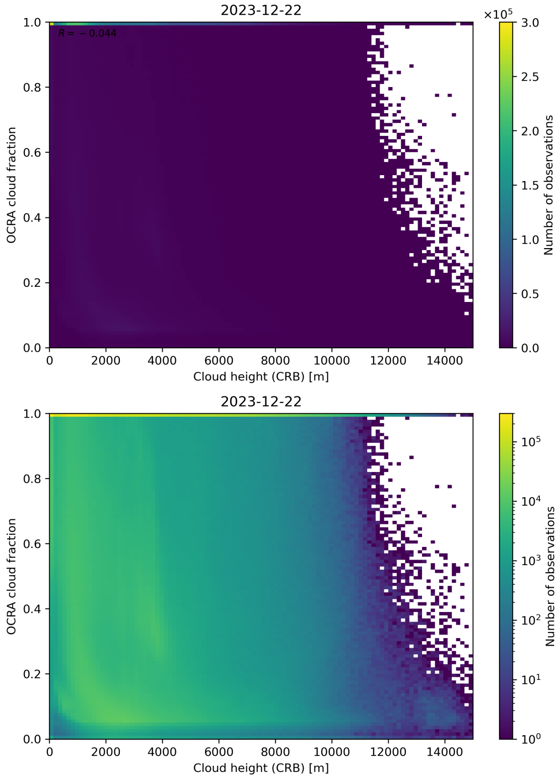
Figure 81: Scatter density plot of “Cloud height (CRB)” against “OCRA cloud fraction” for 2023-12-21 to 2023-12-23.
