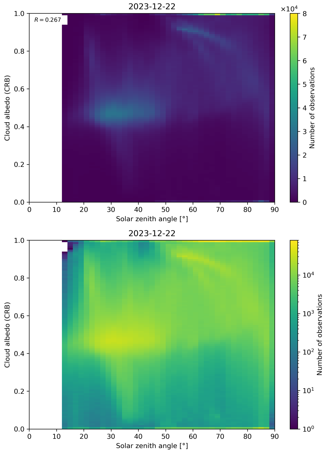
Figure 98: Scatter density plot of “Solar zenith angle” against “Cloud albedo (CRB)” for 2023-12-21 to 2023-12-23.
