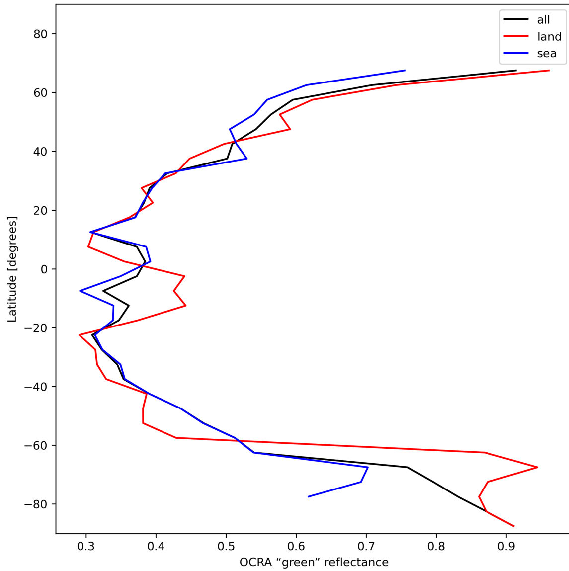
Figure 36: Zonal average of “OCRA “green” reflectance” for 2023-12-21 to 2023-12-23.
