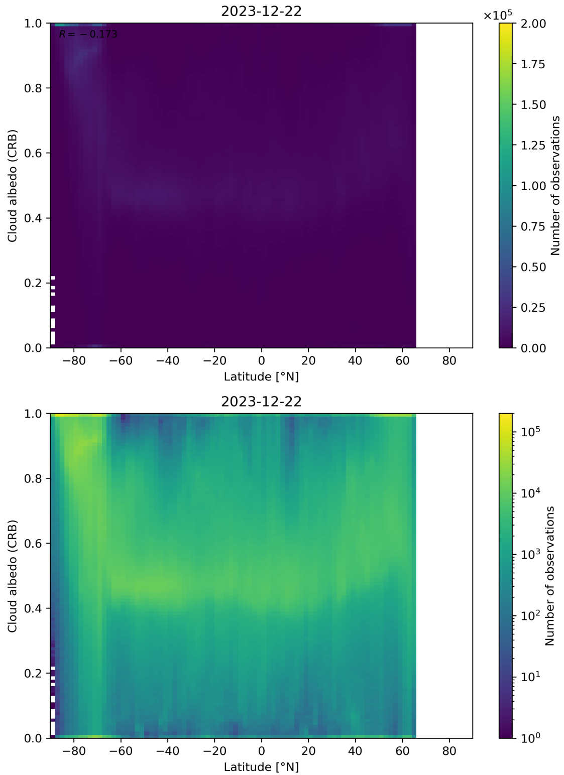
Figure 91: Scatter density plot of “Latitude” against “Cloud albedo (CRB)” for 2023-12-21 to 2023-12-23.
