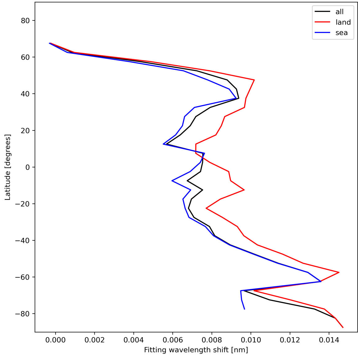
Figure 33: Zonal average of “Fitting wavelength shift” for 2023-12-21 to 2023-12-23.
