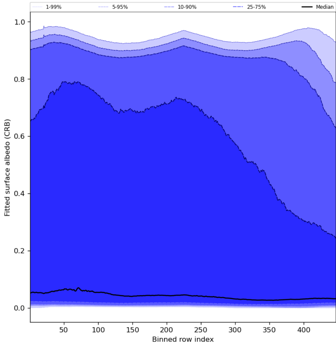
Figure 62: Along track statistics of “Fitted surface albedo (CRB)” for 2023-12-21 to 2023-12-23
