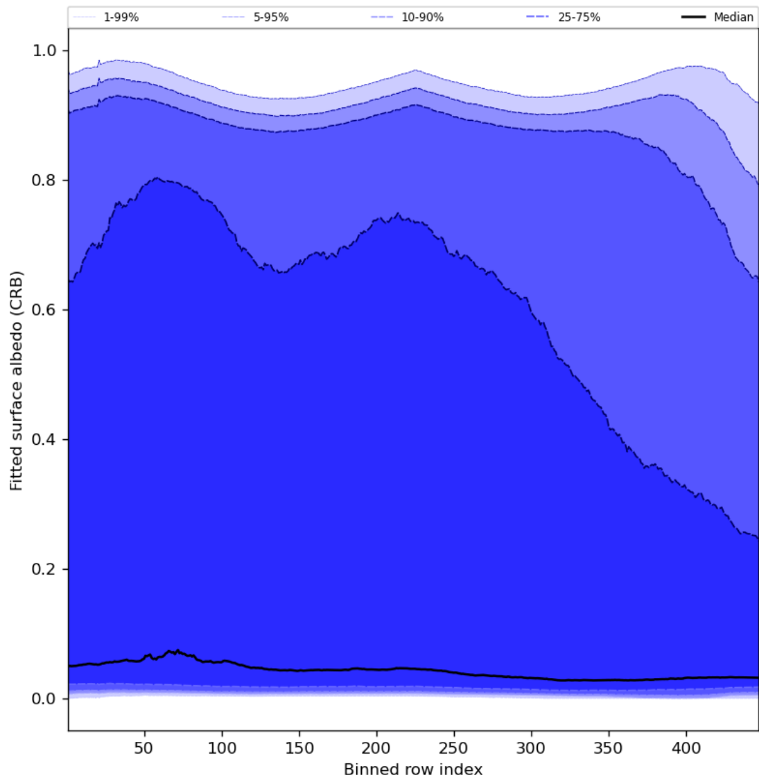
Figure 62: Along track statistics of “Fitted surface albedo (CRB)” for 2023-12-22 to 2023-12-24
