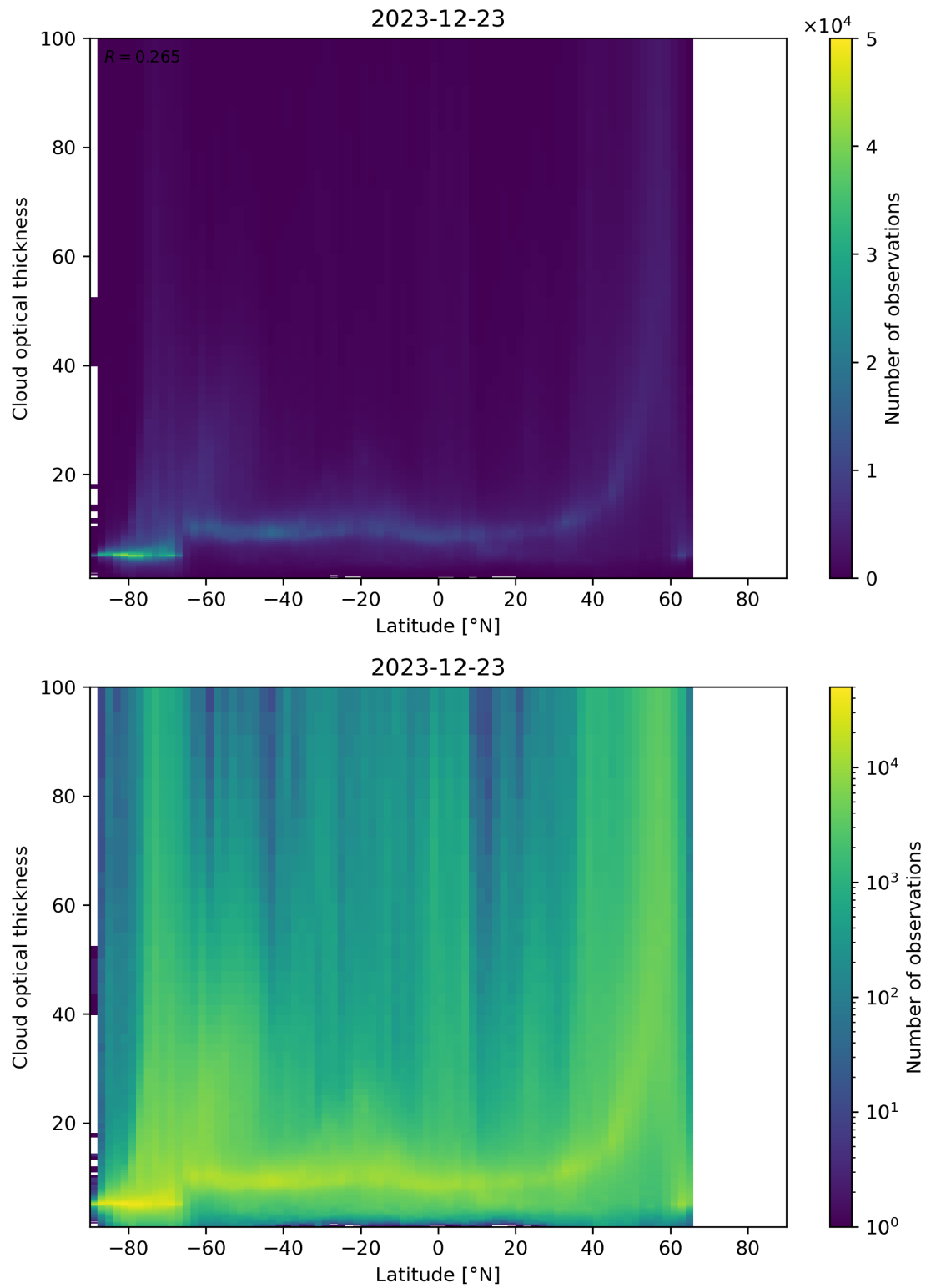
Figure 96: Scatter density plot of “Latitude” against “Cloud optical thickness” for 2023-12-22 to 2023-12-24.
