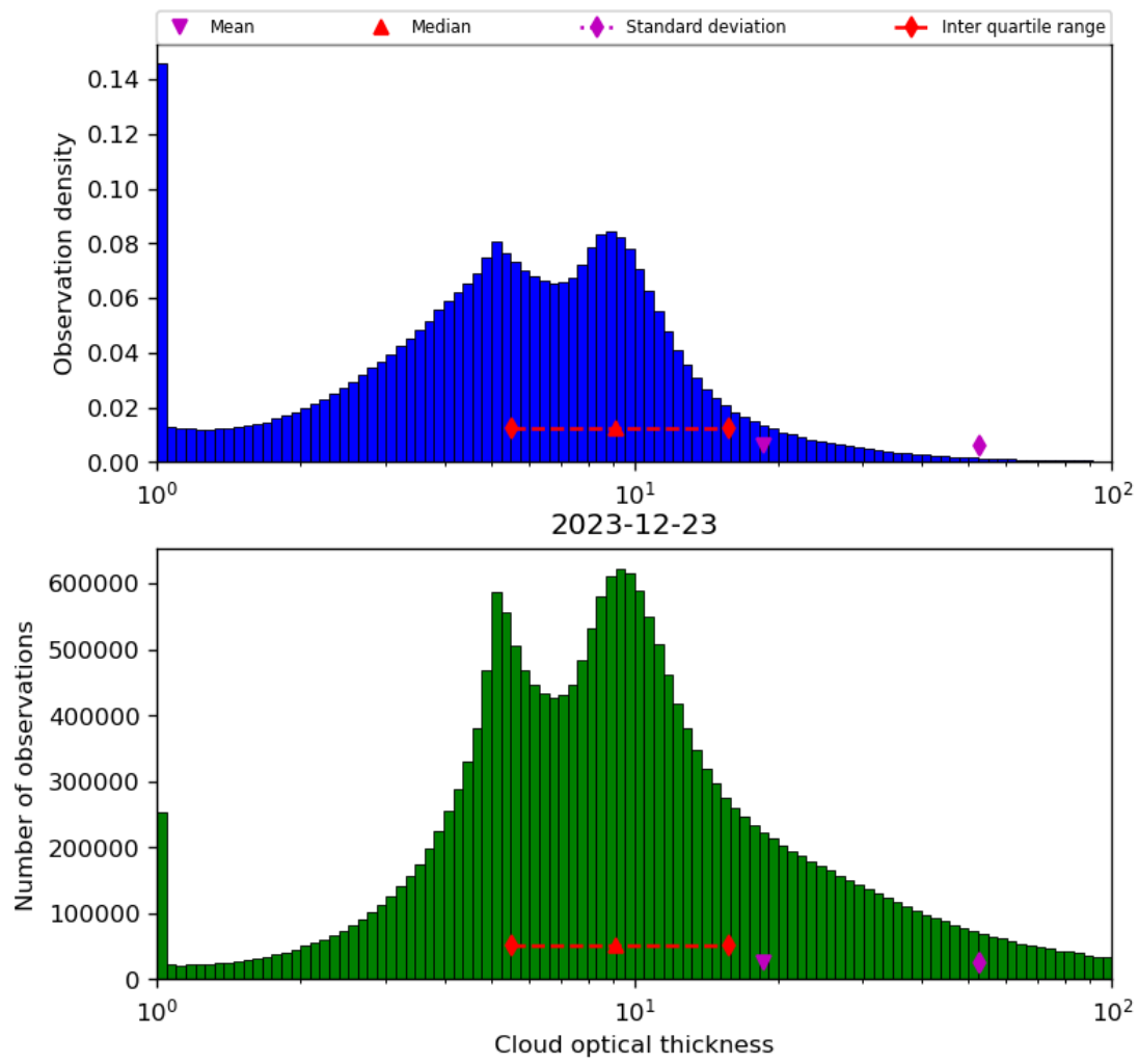
Figure 41: Histogram of “Cloud optical thickness” for 2023-12-22 to 2023-12-24
