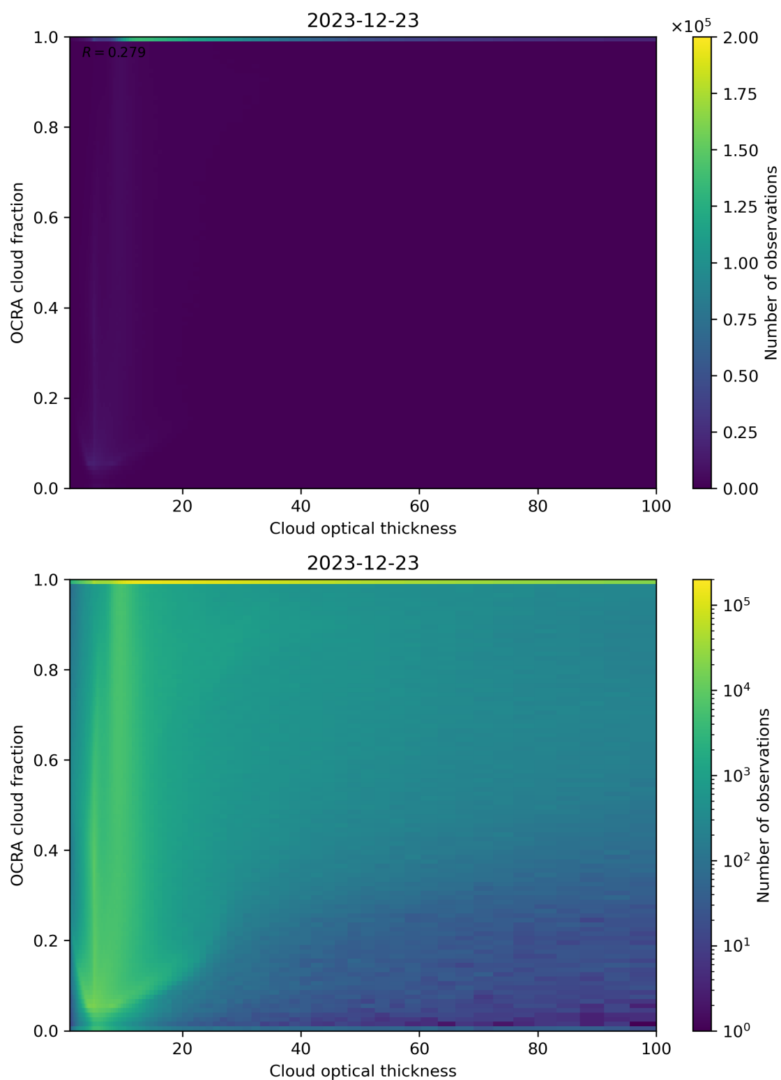
Figure 83: Scatter density plot of “Cloud optical thickness” against “OCRA cloud fraction” for 2023-12-22 to 2023-12-24.
