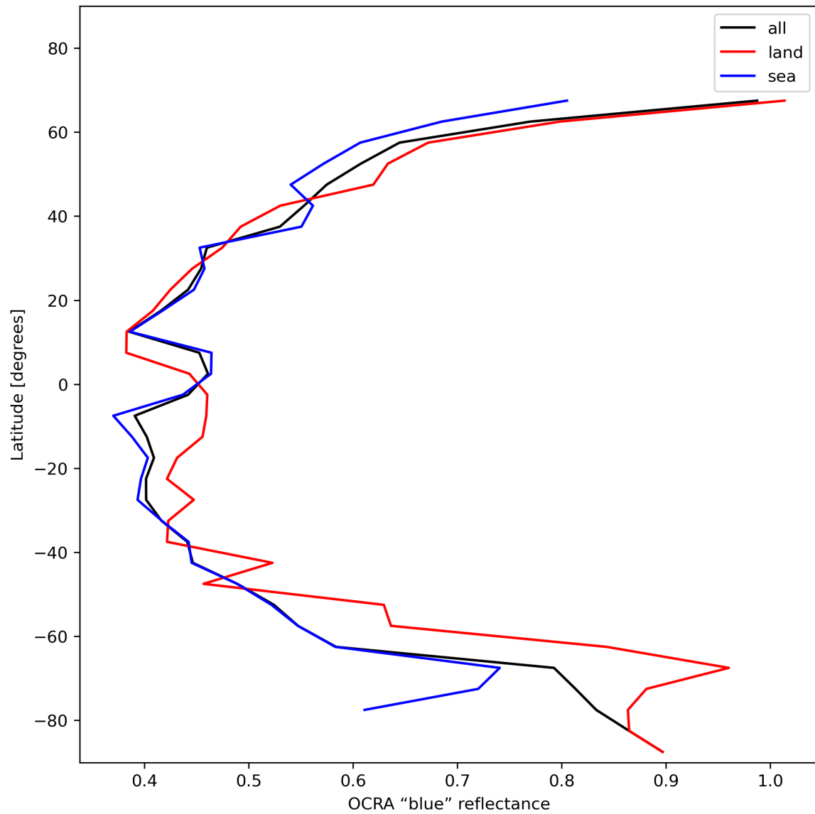
Figure 35: Zonal average of “OCRA “blue” reflectance” for 2023-12-22 to 2023-12-24.
