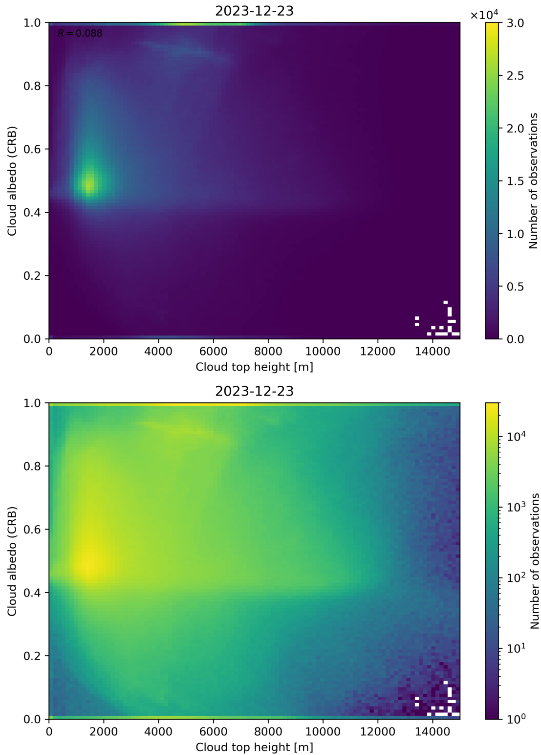
Figure 86: Scatter density plot of “Cloud top height” against “Cloud albedo (CRB)” for 2023-12-22 to 2023-12-24.
