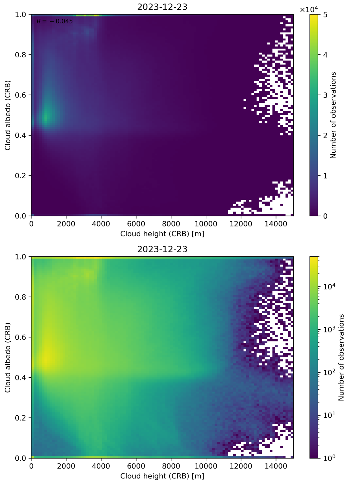
Figure 80: Scatter density plot of “Cloud height (CRB)” against “Cloud albedo (CRB)” for 2023-12-22 to 2023-12-24.
