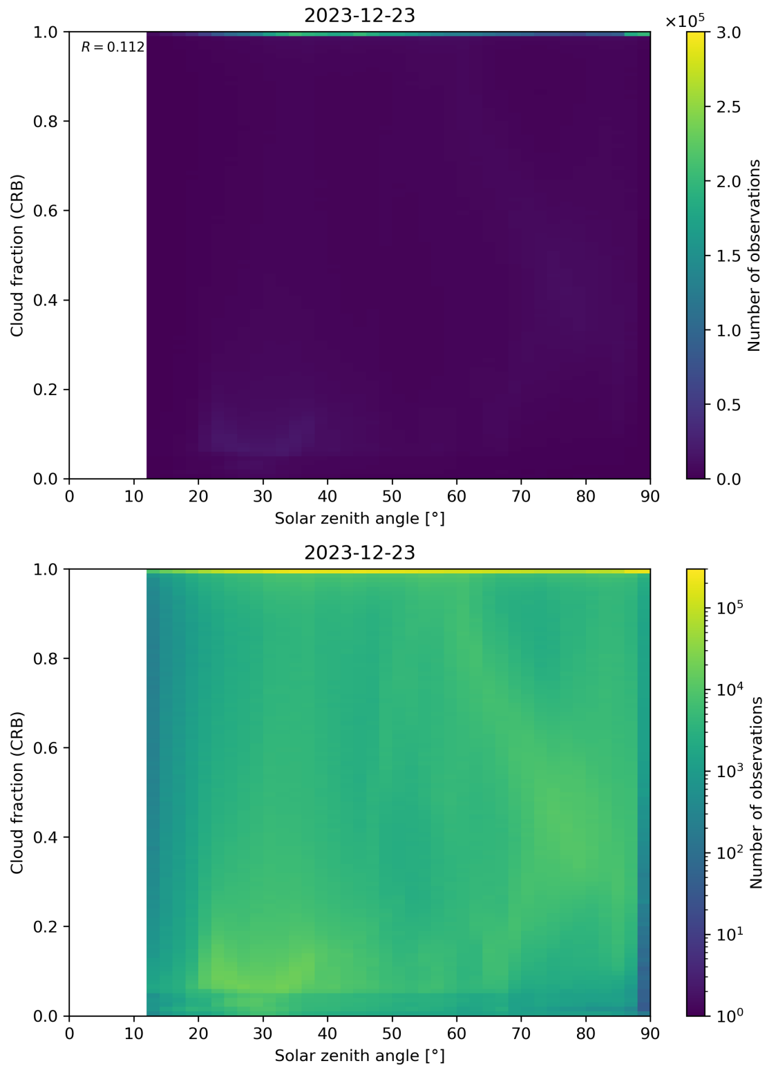
Figure 101: Scatter density plot of “Solar zenith angle” against “Cloud fraction (CRB)” for 2023-12-22 to 2023-12-24.
