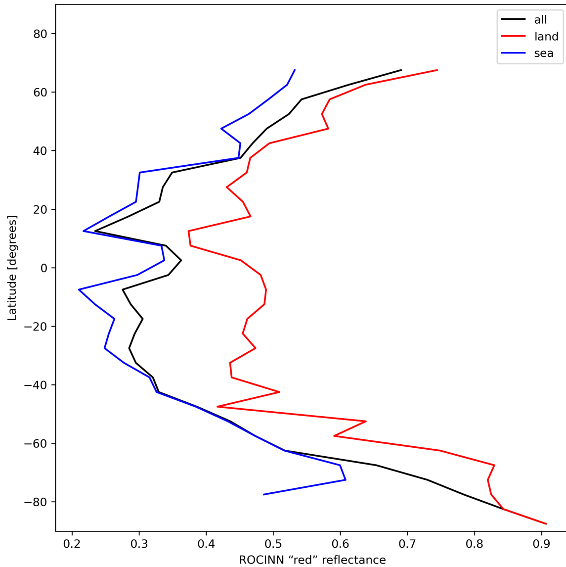
Figure 37: Zonal average of “ROCINN “red” reflectance” for 2023-12-22 to 2023-12-24.
