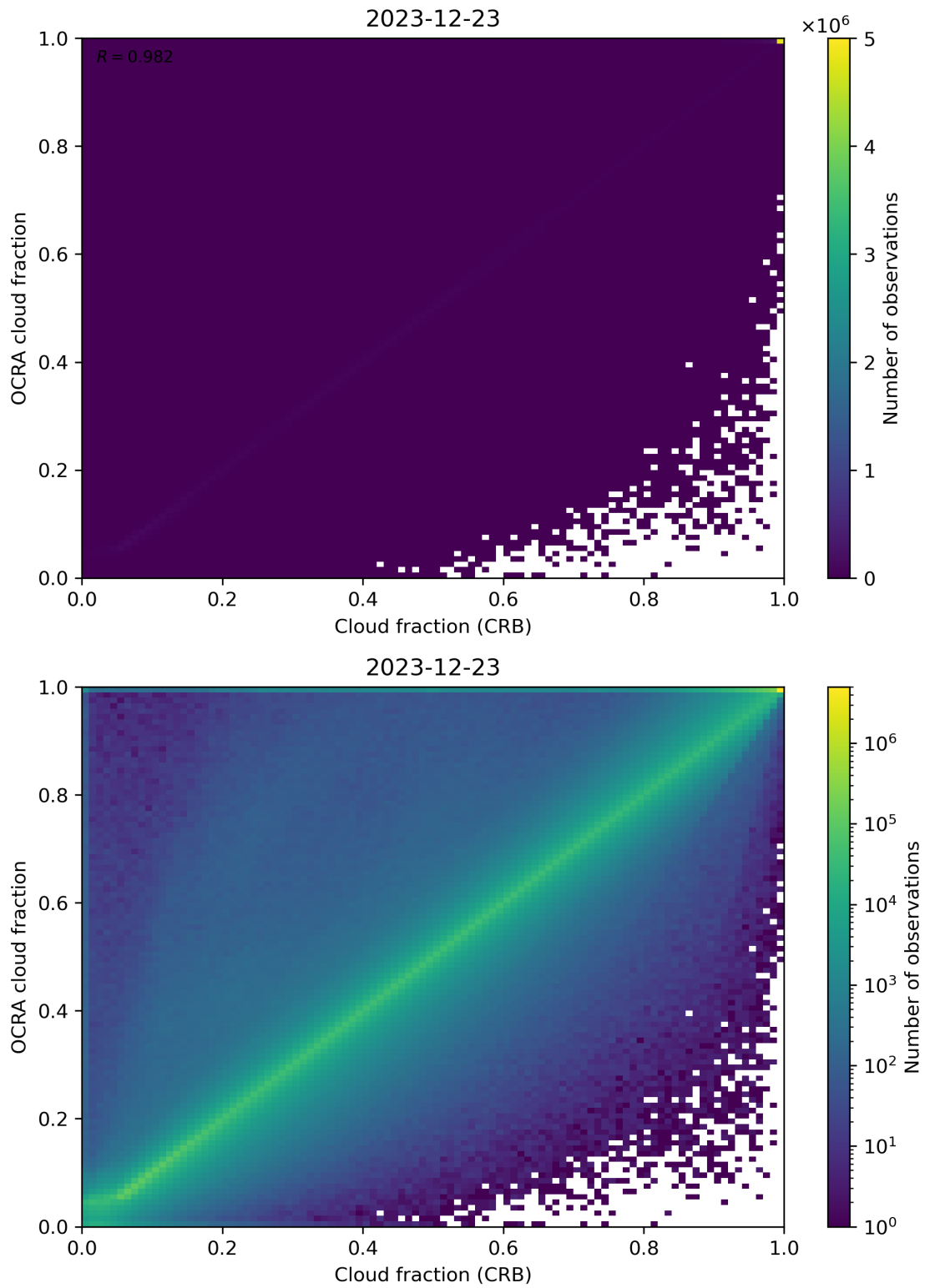
Figure 78: Scatter density plot of “Cloud fraction (CRB)” against “OCRA cloud fraction” for 2023-12-22 to 2023-12-24.
