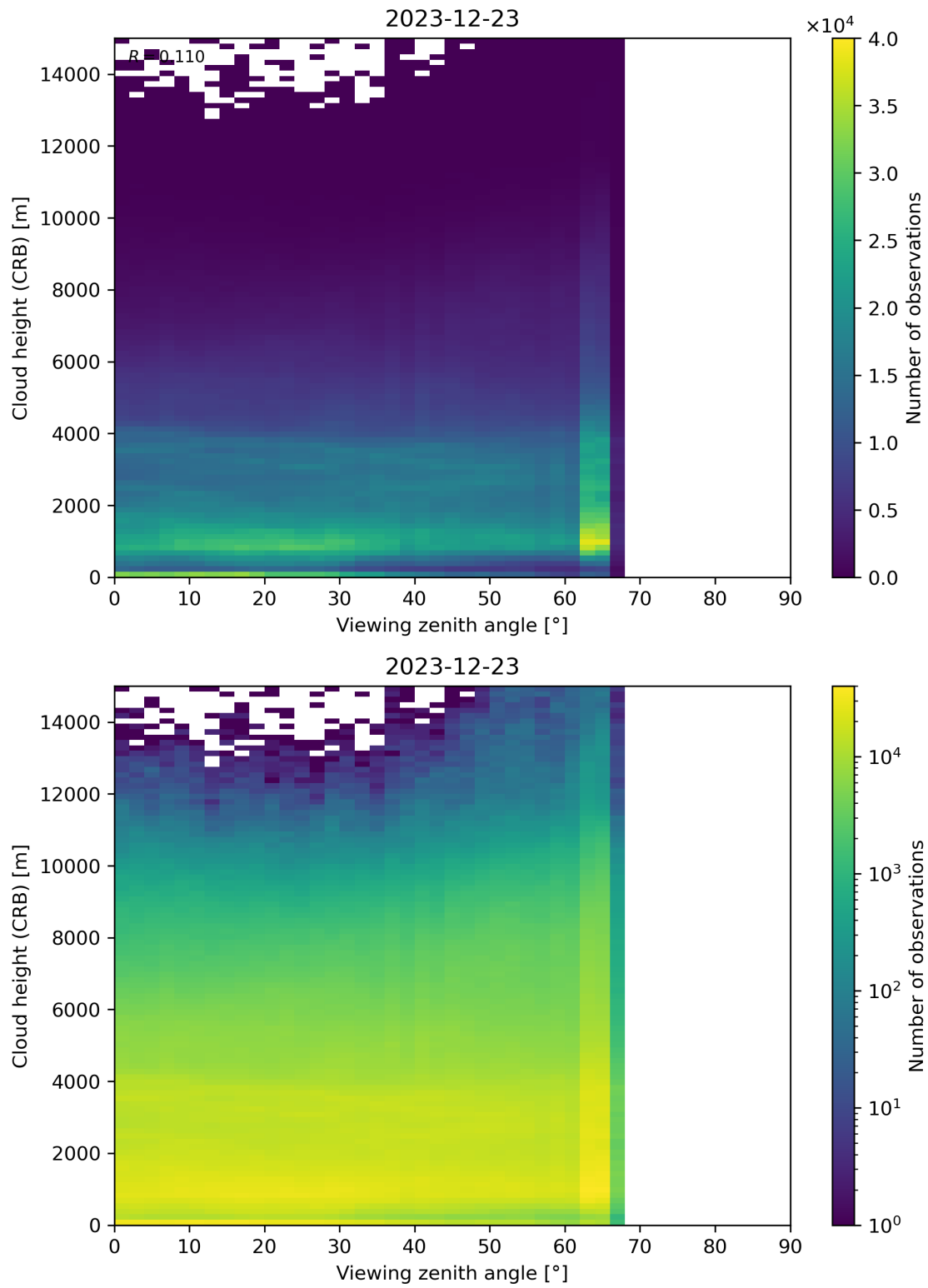
Figure 110: Scatter density plot of “Viewing zenith angle” against “Cloud height (CRB)” for 2023-12-22 to 2023-12-24.
