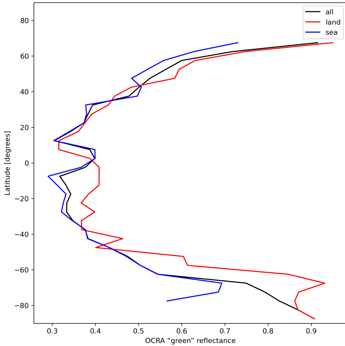
Figure 36: Zonal average of “OCRA “green” reflectance” for 2023-12-22 to 2023-12-24.
