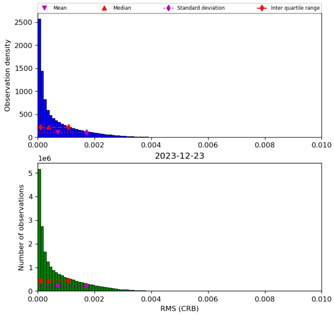
Figure 48: Histogram of “RMS (CRB)” for 2023-12-22 to 2023-12-24
