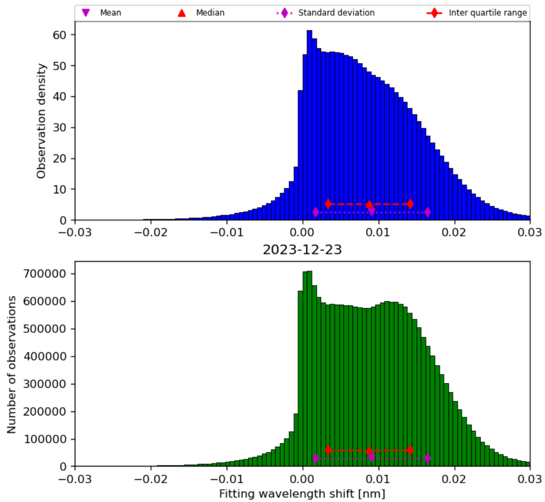
Figure 49: Histogram of “Fitting wavelength shift” for 2023-12-22 to 2023-12-24
