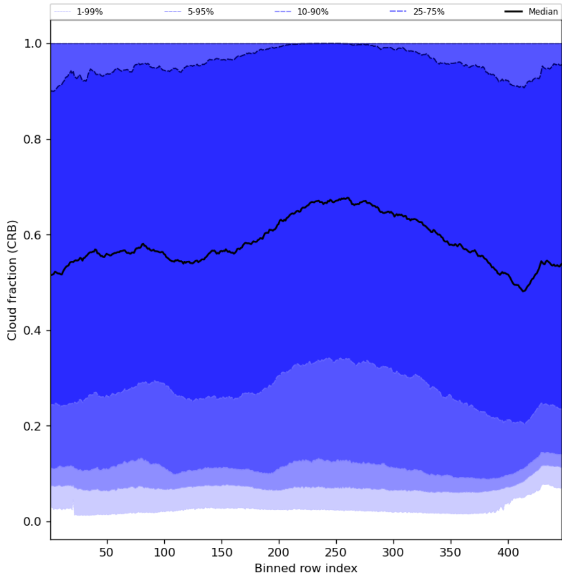
Figure 58: Along track statistics of “Cloud fraction (CRB)” for 2023-12-22 to 2023-12-24
