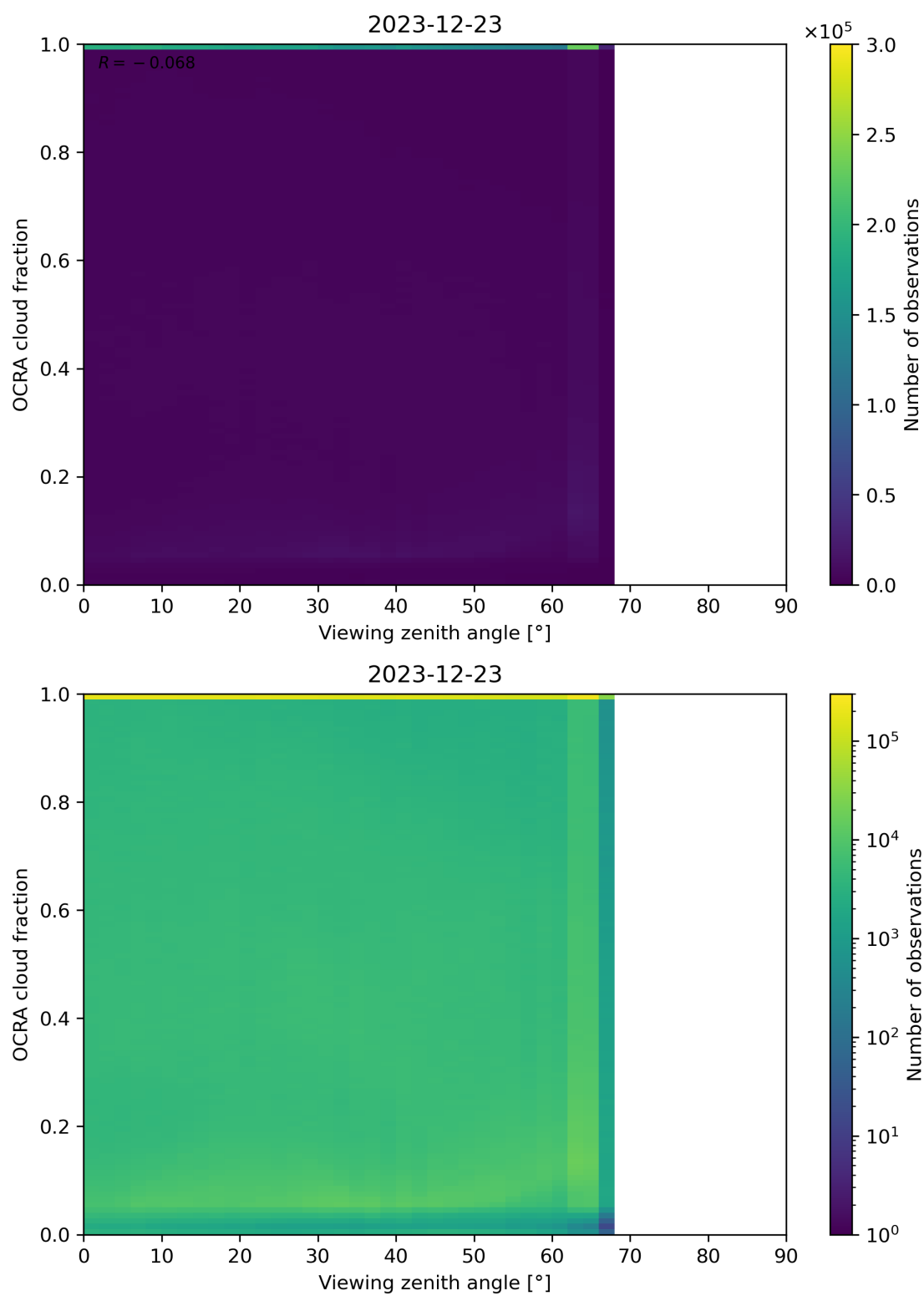
Figure 108: Scatter density plot of “Viewing zenith angle” against “OCRA cloud fraction” for 2023-12-22 to 2023-12-24.
