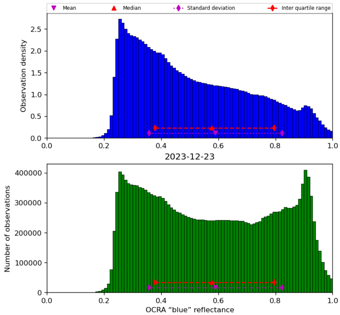
Figure 51: Histogram of “OCRA “blue” reflectance” for 2023-12-22 to 2023-12-24
