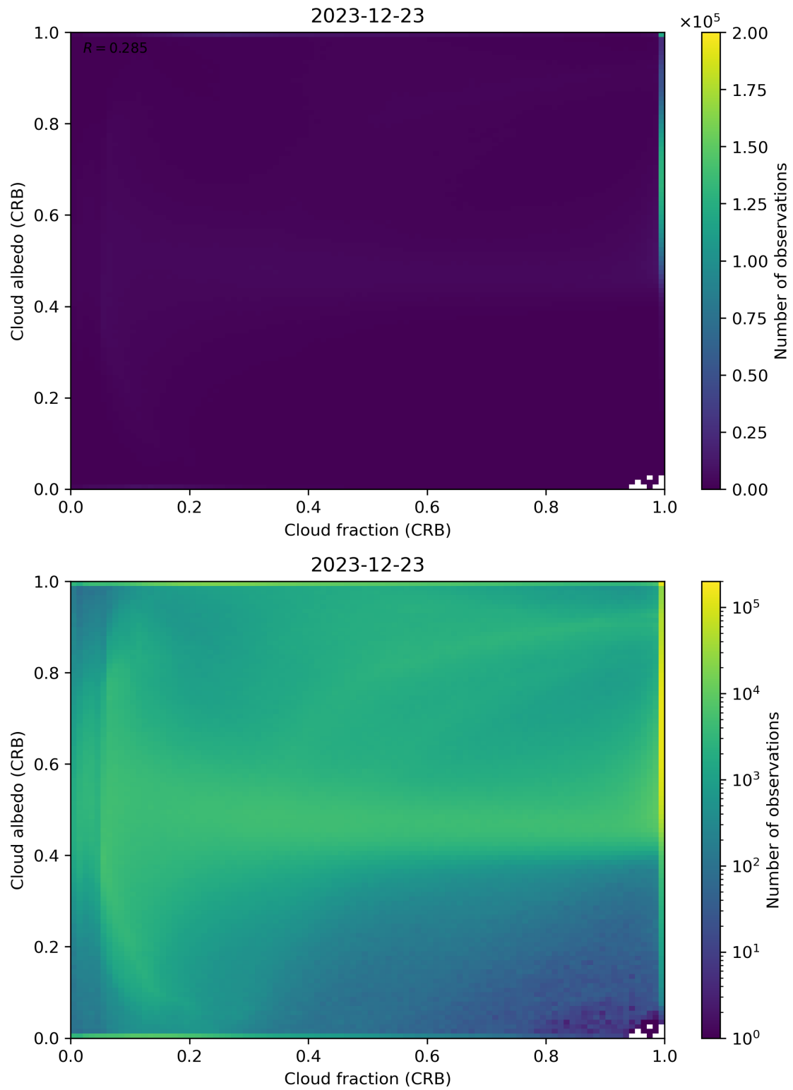
Figure 77: Scatter density plot of “Cloud fraction (CRB)” against “Cloud albedo (CRB)” for 2023-12-22 to 2023-12-24.
