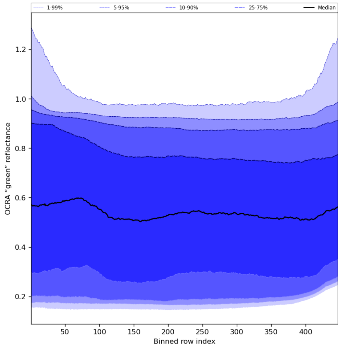
Figure 68: Along track statistics of “OCRA “green” reflectance” for 2023-12-22 to 2023-12-24
