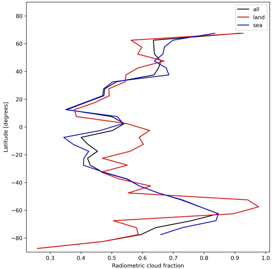
Figure 23: Zonal average of “Radiometric cloud fraction” for 2023-12-22 to 2023-12-24.
