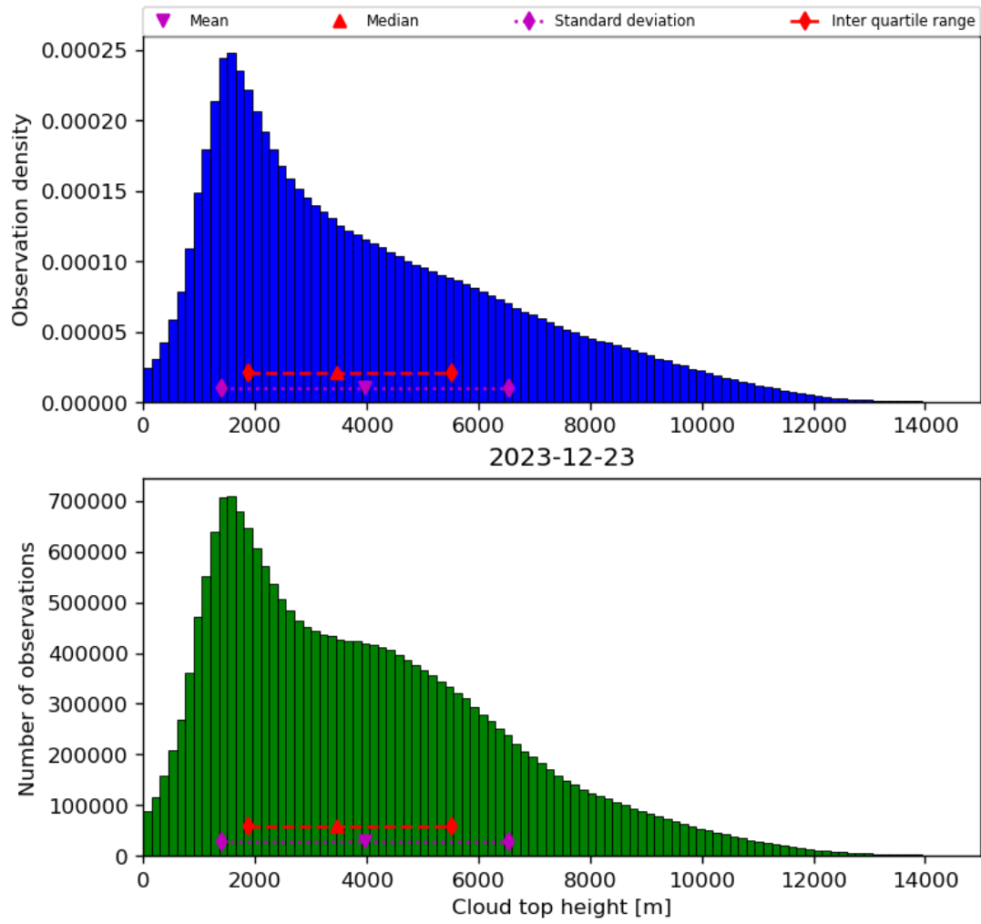
Figure 40: Histogram of “Cloud top height” for 2023-12-22 to 2023-12-24
