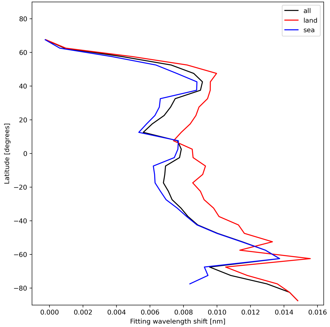
Figure 33: Zonal average of “Fitting wavelength shift” for 2023-12-22 to 2023-12-24.
