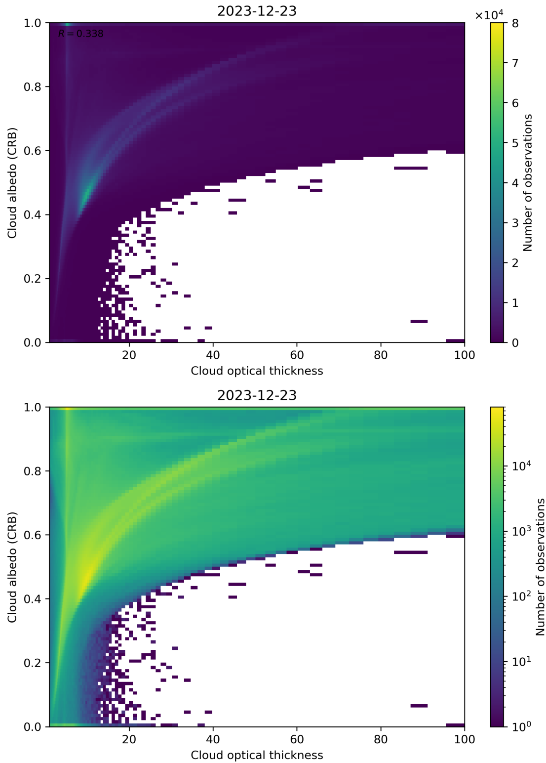
Figure 82: Scatter density plot of “Cloud optical thickness” against “Cloud albedo (CRB)” for 2023-12-22 to 2023-12-24.
