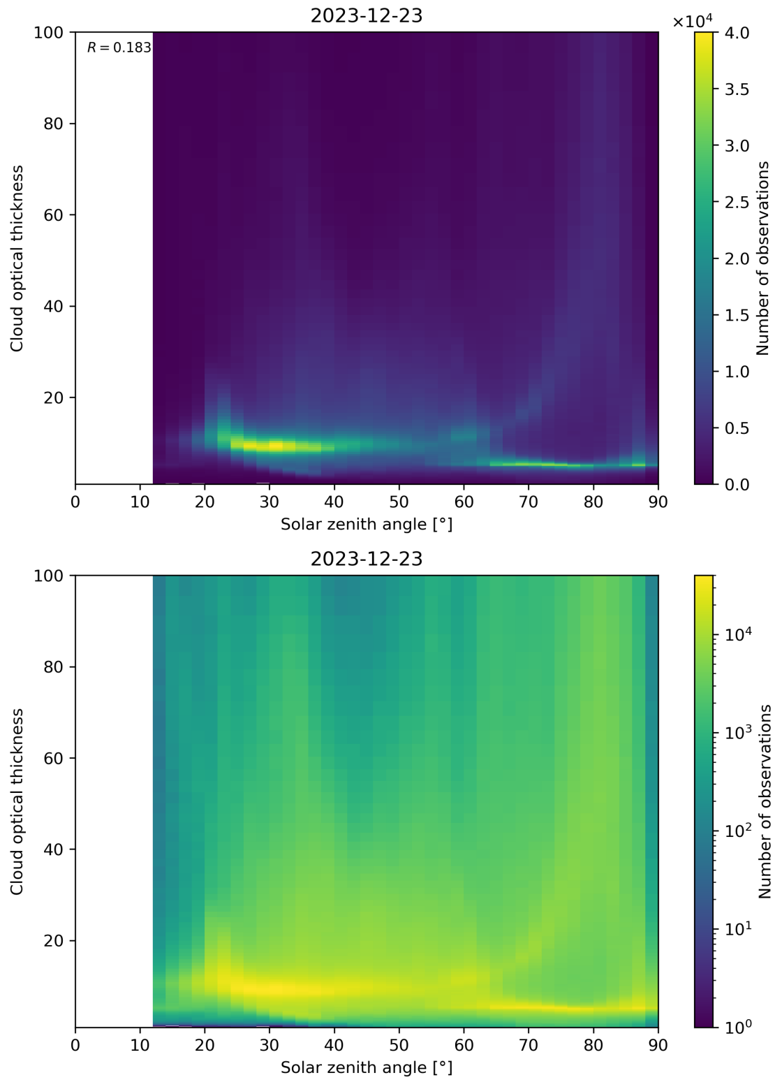
Figure 103: Scatter density plot of “Solar zenith angle” against “Cloud optical thickness” for 2023-12-22 to 2023-12-24.
