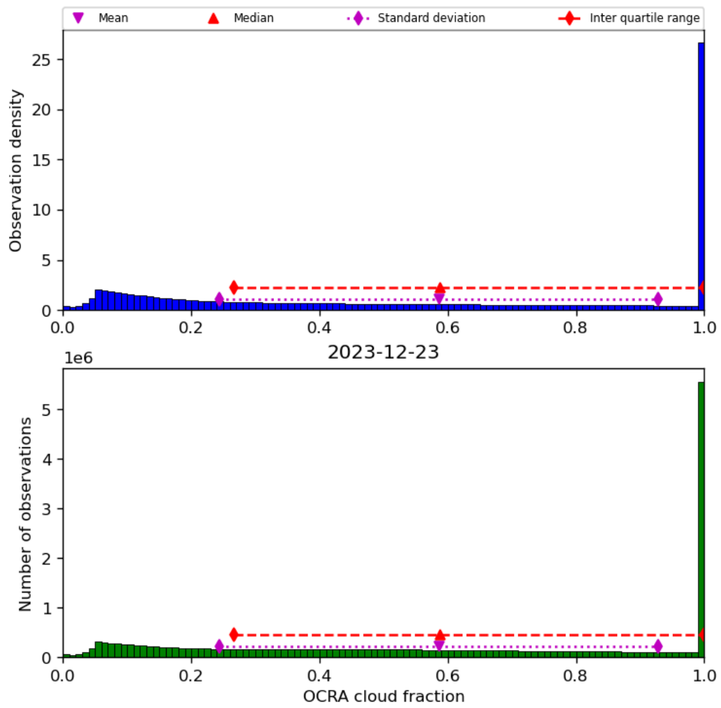
Figure 50: Histogram of “OCRA cloud fraction” for 2023-12-22 to 2023-12-24
