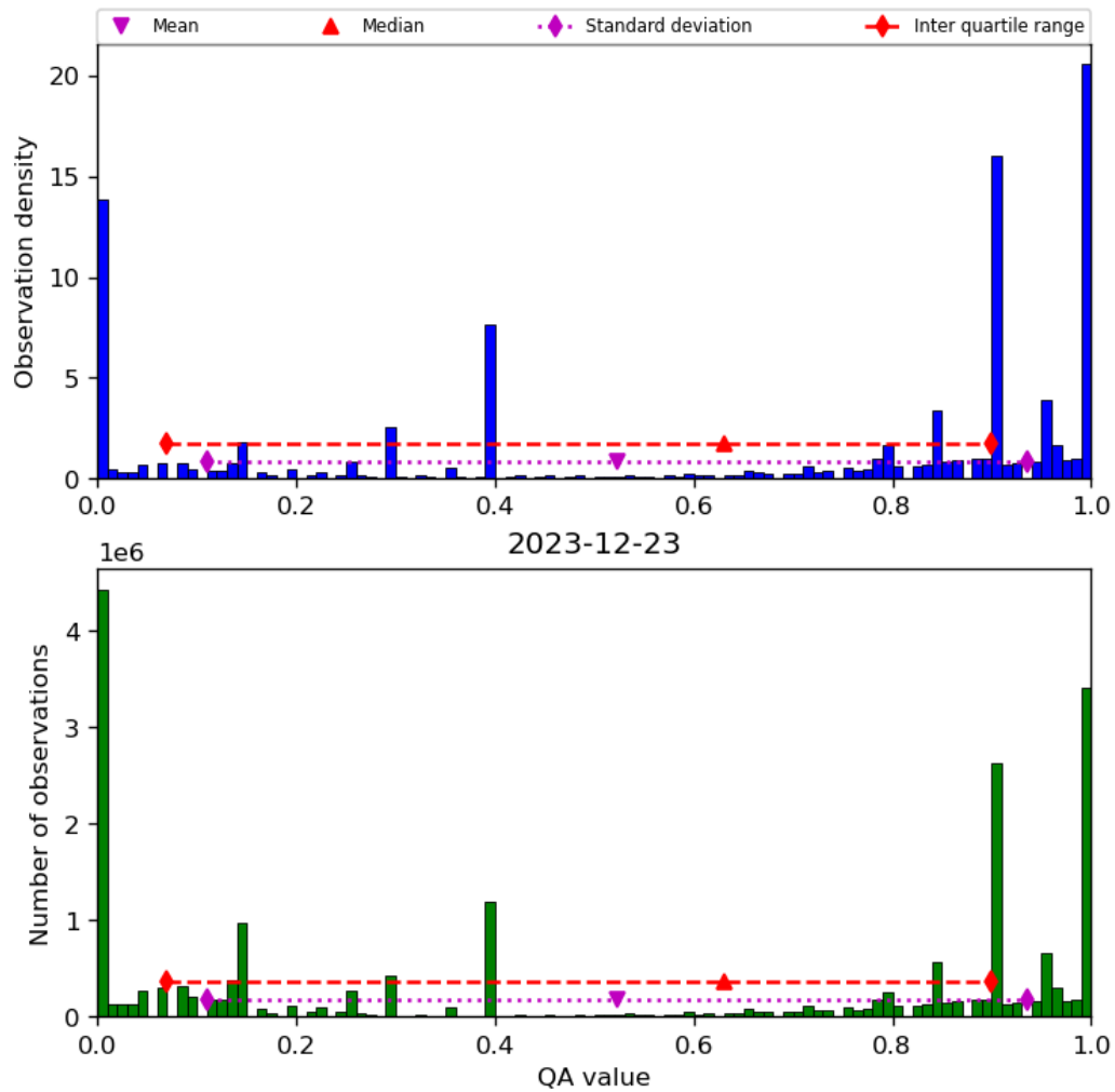
Figure 38: Histogram of “QA value” for 2023-12-22 to 2023-12-24
