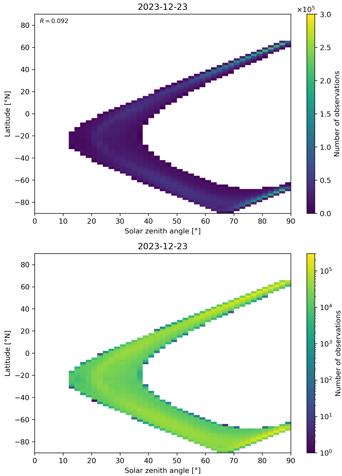
Figure 105: Scatter density plot of “Solar zenith angle” against “Latitude” for 2023-12-22 to 2023-12-24.
