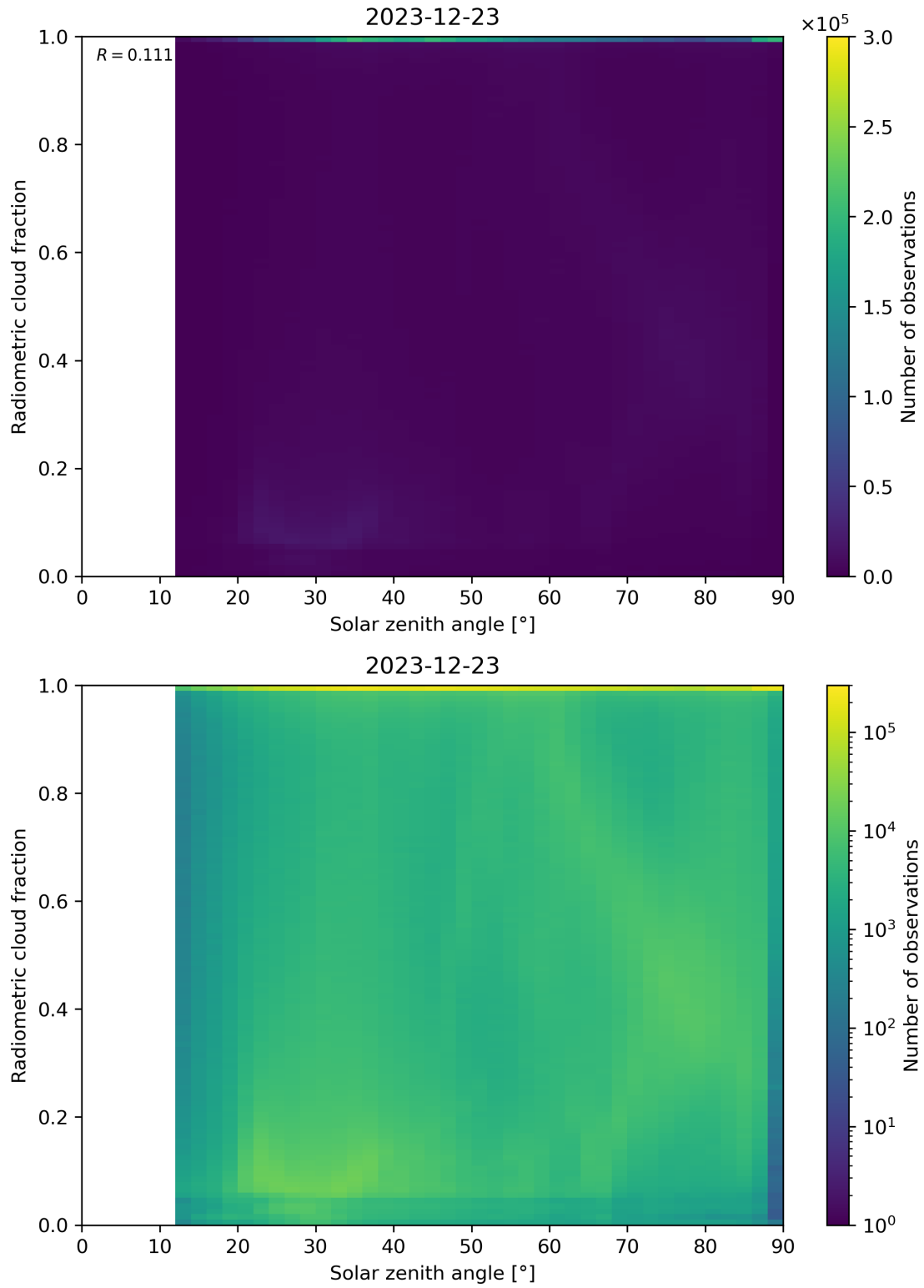
Figure 99: Scatter density plot of “Solar zenith angle” against “Radiometric cloud fraction” for 2023-12-22 to 2023-12-24.
