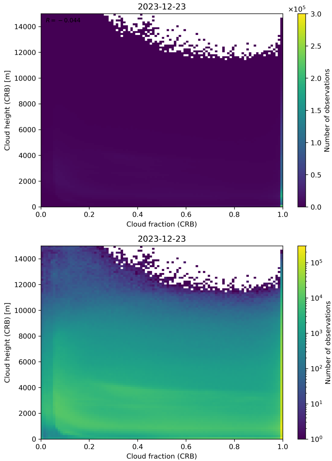
Figure 79: Scatter density plot of “Cloud fraction (CRB)” against “Cloud height (CRB)” for 2023-12-22 to 2023-12-24.
