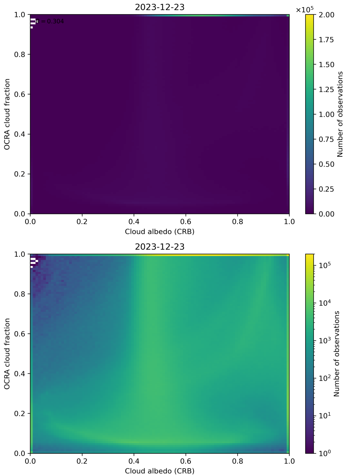
Figure 70: Scatter density plot of “Cloud albedo (CRB)” against “OCRA cloud fraction” for 2023-12-22 to 2023-12-24.
