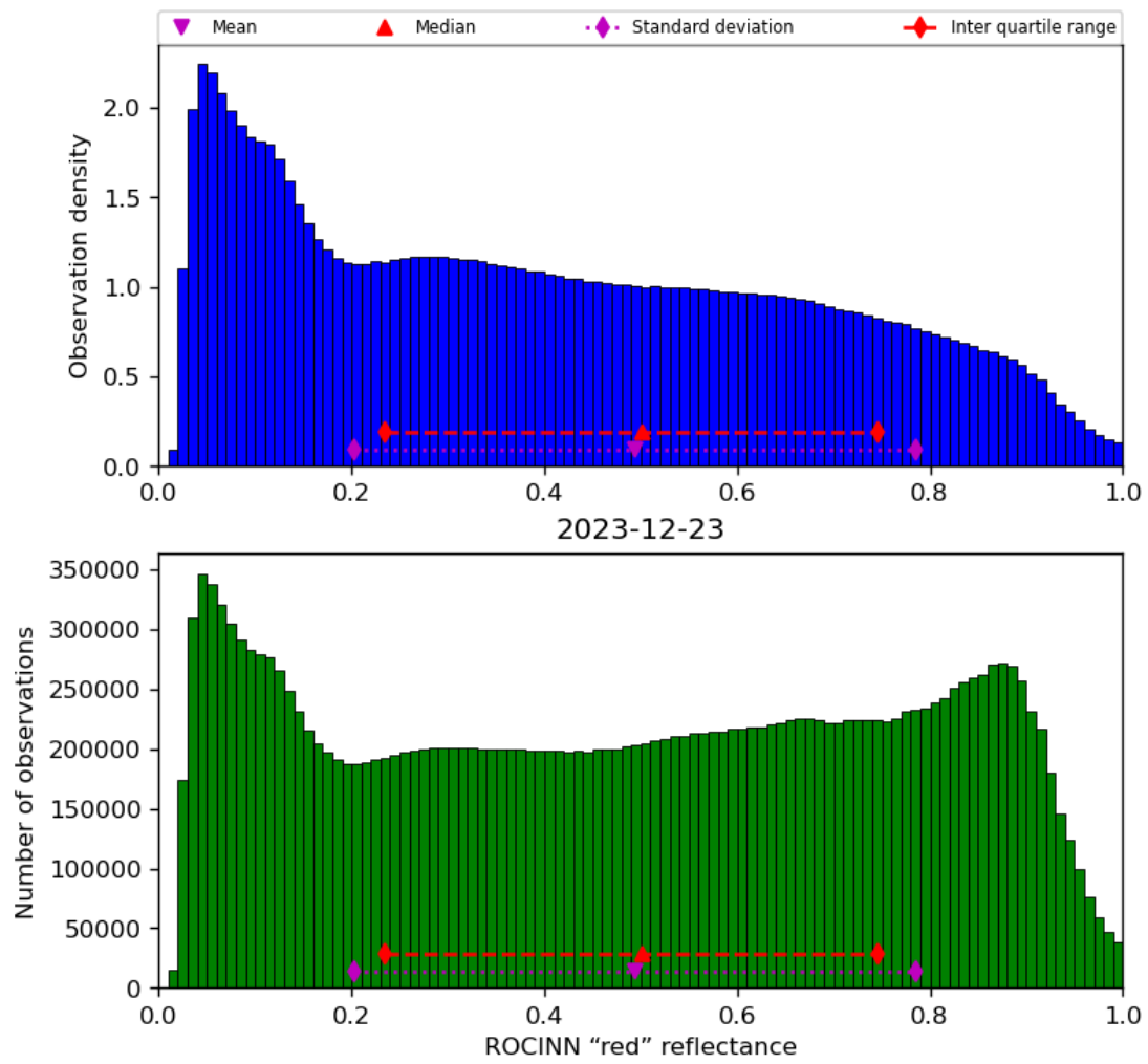
Figure 53: Histogram of “ROCINN “red” reflectance” for 2023-12-22 to 2023-12-24
