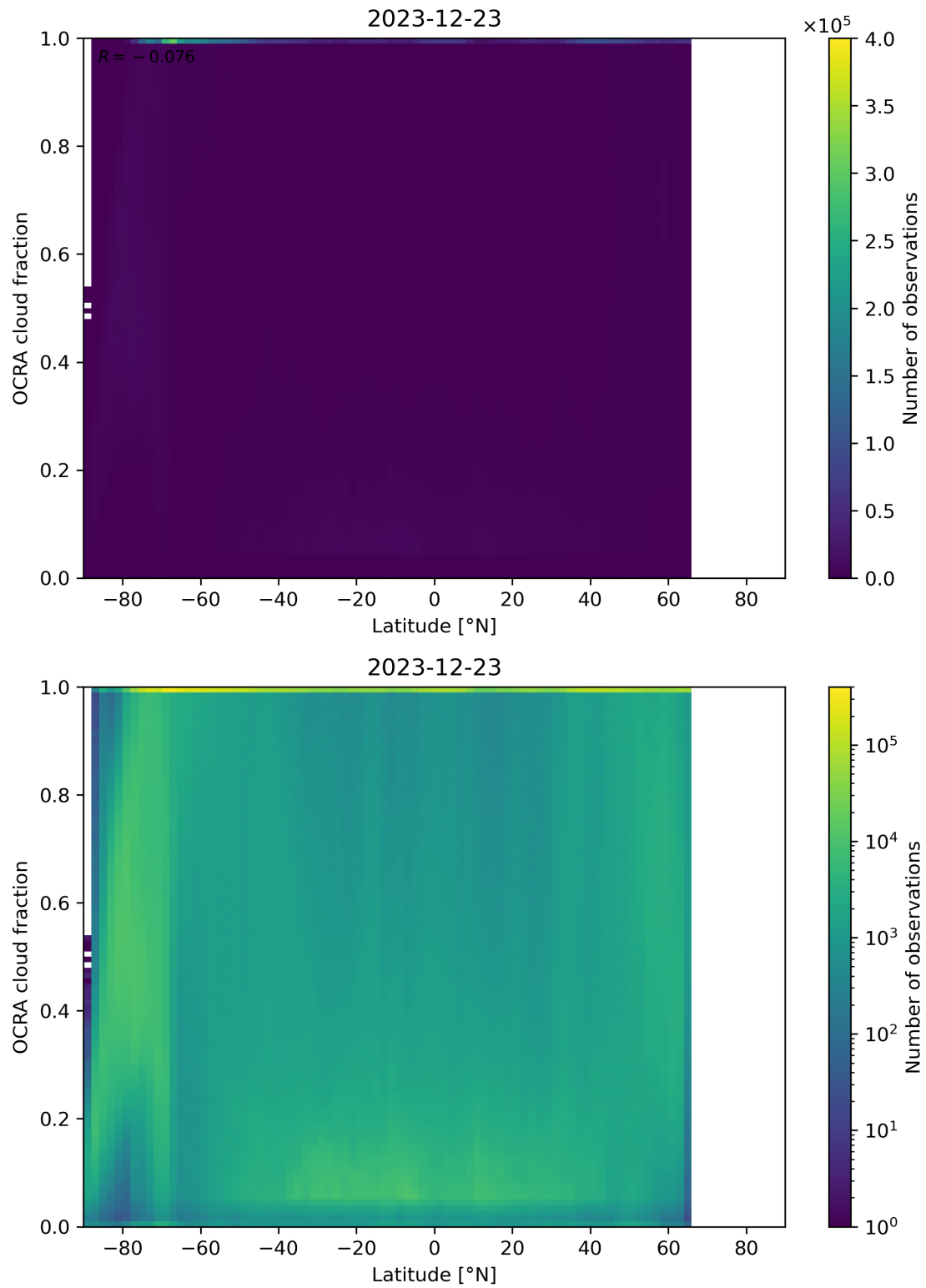
Figure 93: Scatter density plot of “Latitude” against “OCRA cloud fraction” for 2023-12-22 to 2023-12-24.
