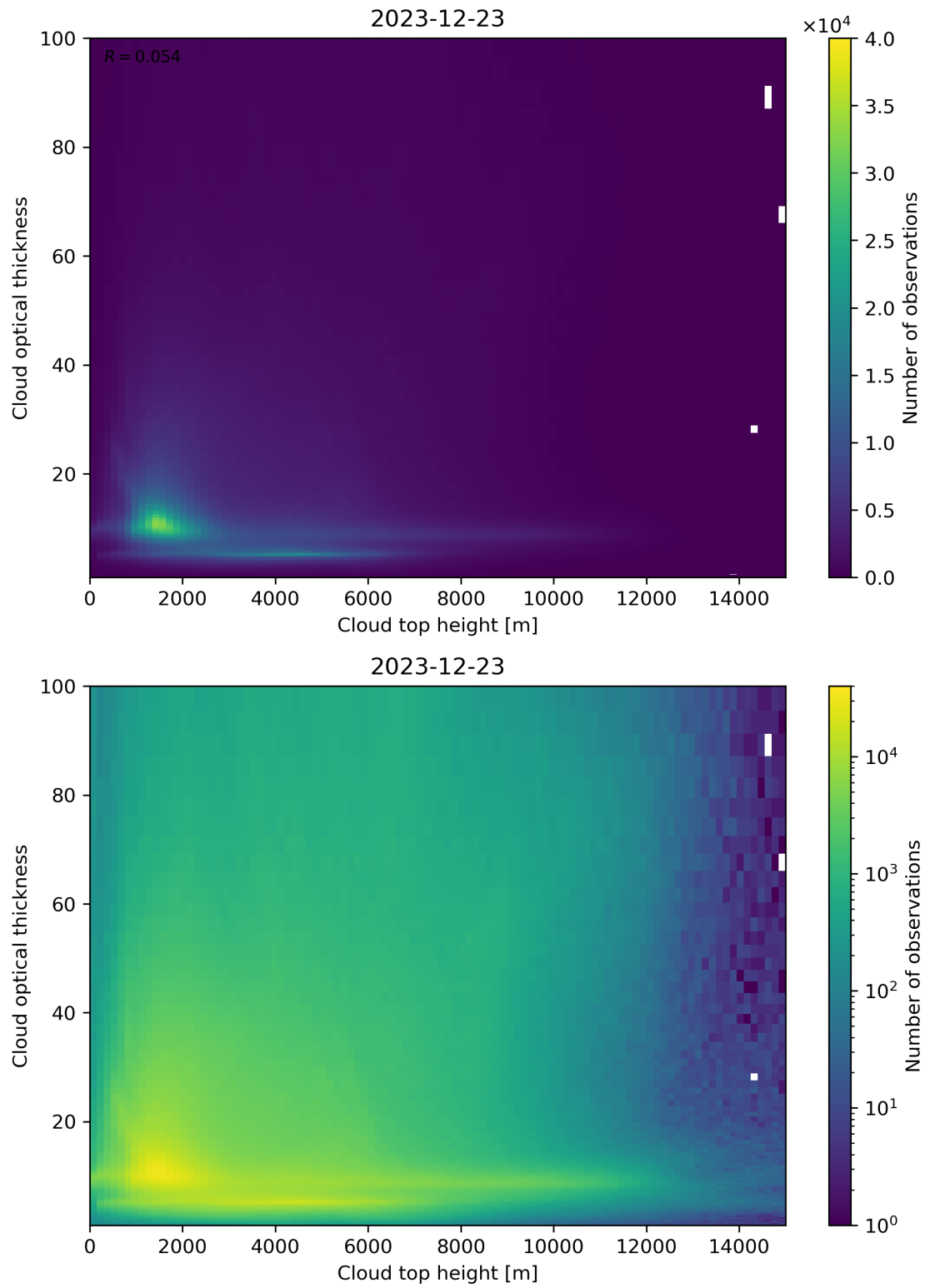
Figure 90: Scatter density plot of “Cloud top height” against “Cloud optical thickness” for 2023-12-22 to 2023-12-24.
