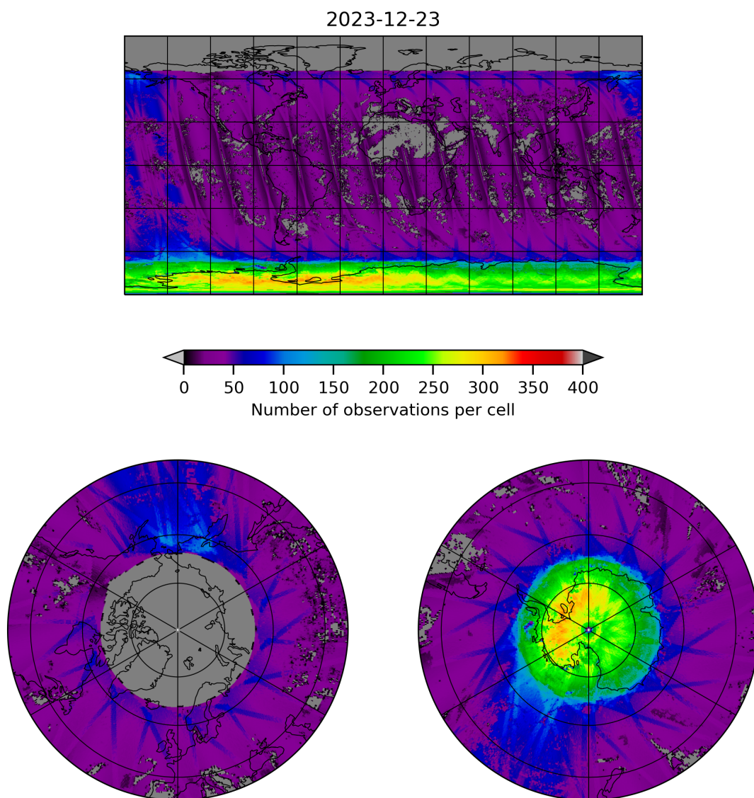
Figure 21: Map of the number of observations for 2023-12-22 to 2023-12-24
