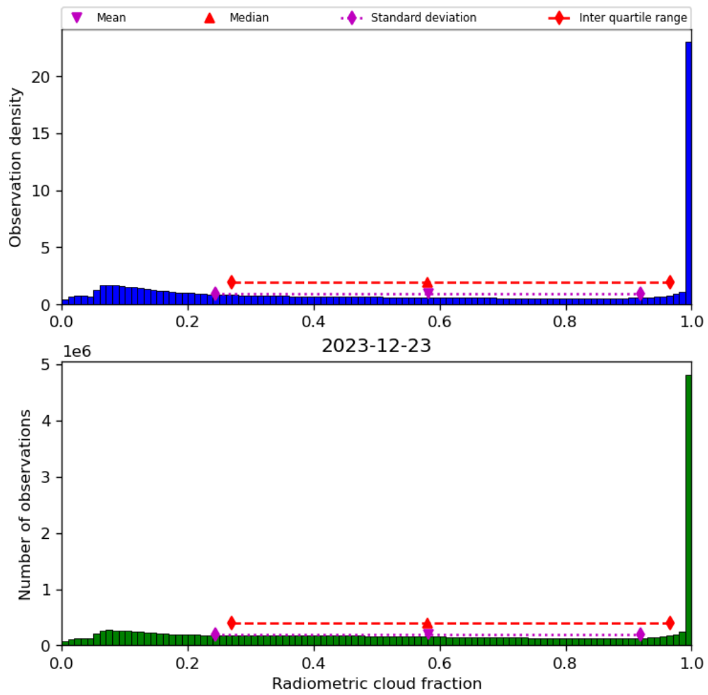
Figure 39: Histogram of “Radiometric cloud fraction” for 2023-12-22 to 2023-12-24
