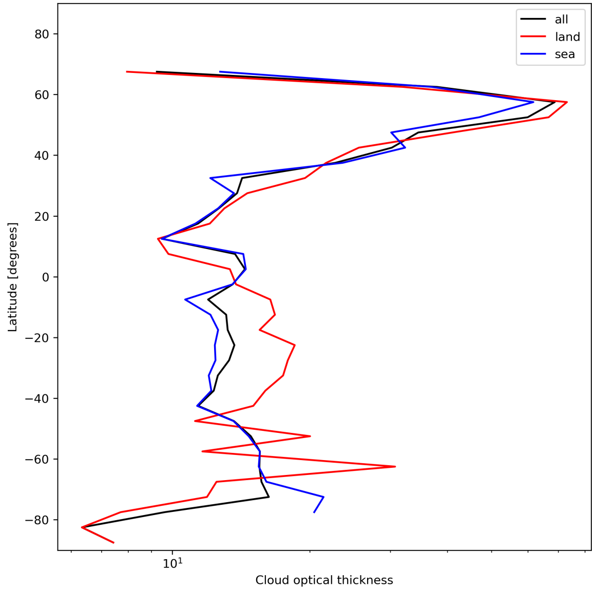
Figure 25: Zonal average of “Cloud optical thickness” for 2023-12-22 to 2023-12-24.
