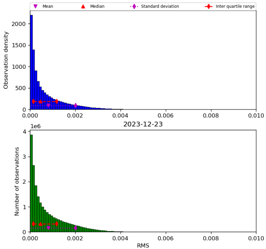
Figure 47: Histogram of “RMS” for 2023-12-22 to 2023-12-24
