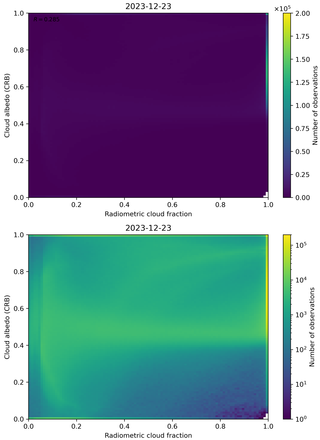
Figure 71: Scatter density plot of “Radiometric cloud fraction” against “Cloud albedo (CRB)” for 2023-12-22 to 2023-12-24.
