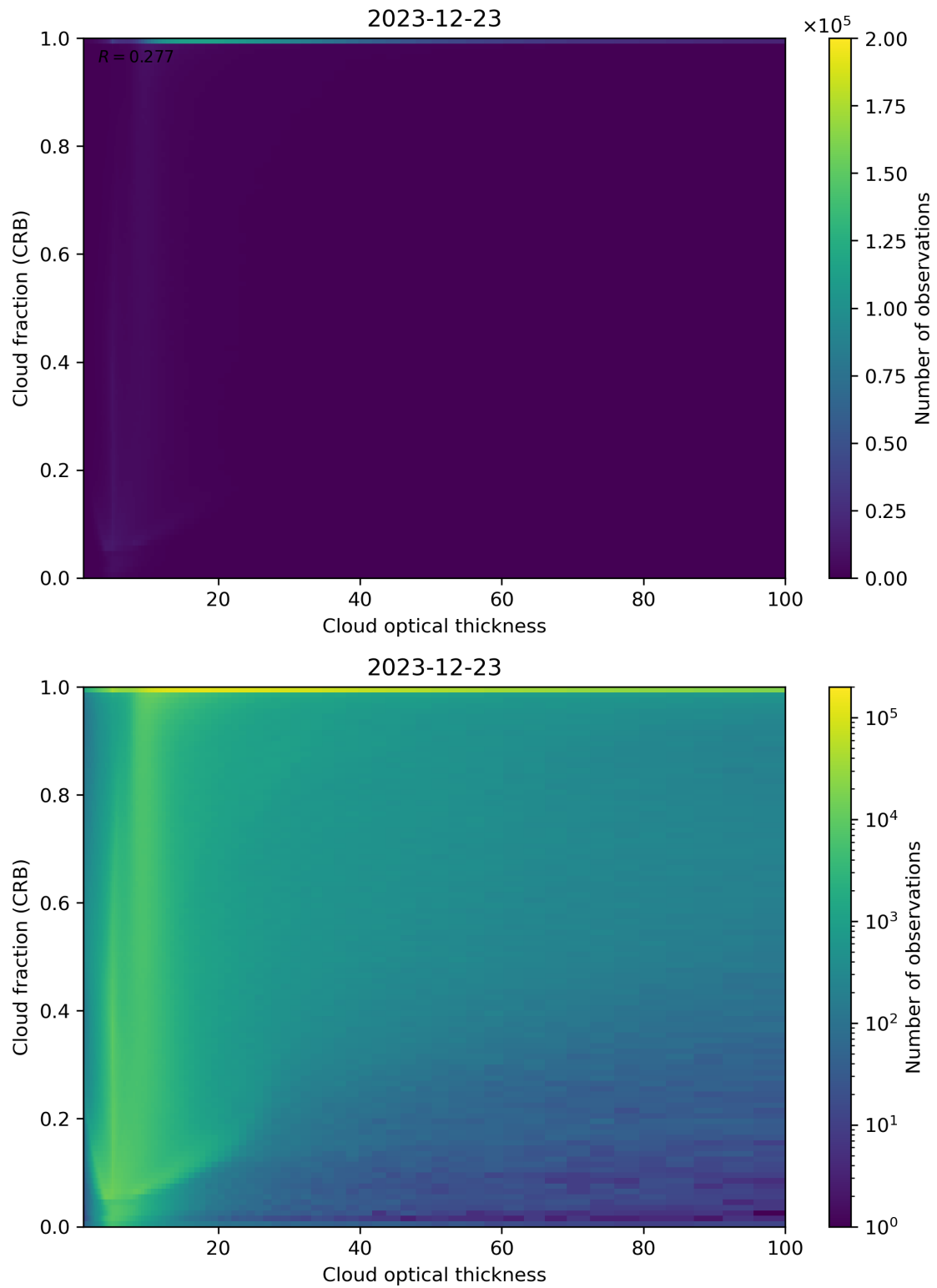
Figure 84: Scatter density plot of “Cloud optical thickness” against “Cloud fraction (CRB)” for 2023-12-22 to 2023-12-24.
