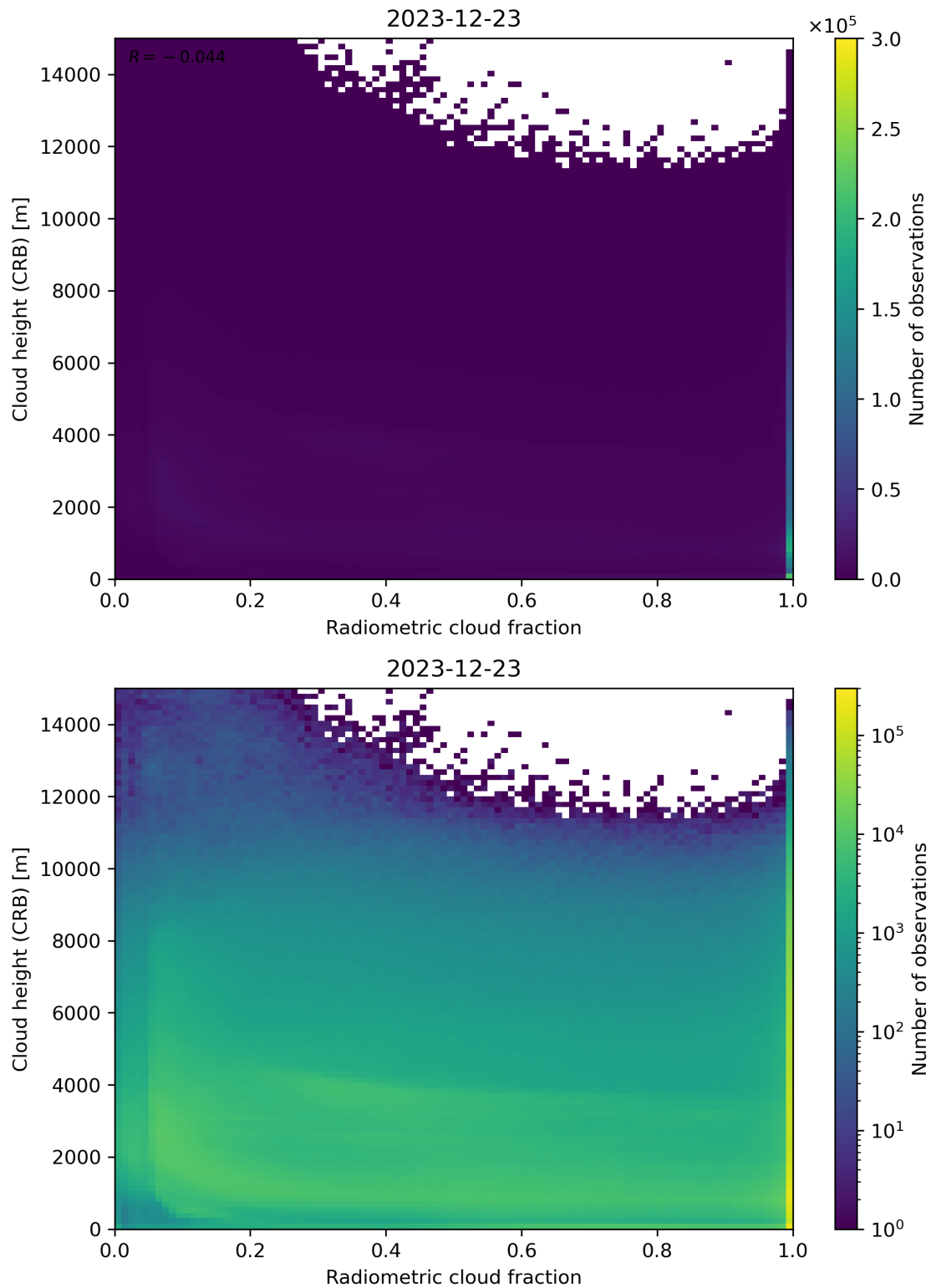
Figure 74: Scatter density plot of “Radiometric cloud fraction” against “Cloud height (CRB)” for 2023-12-22 to 2023-12-24.
