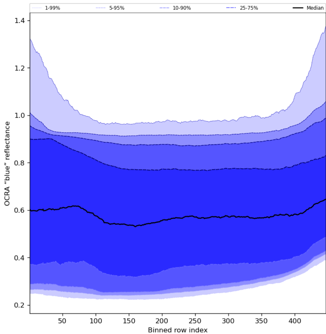
Figure 67: Along track statistics of "OCRA "blue" reflectance" for 2023-12-22 to 2023-12-24
