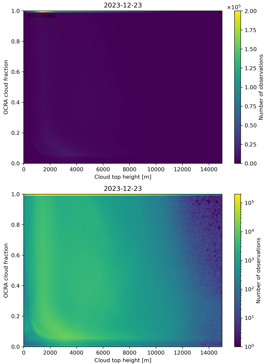
Figure 87: Scatter density plot of “Cloud top height” against “OCRA cloud fraction” for 2023-12-22 to 2023-12-24.
