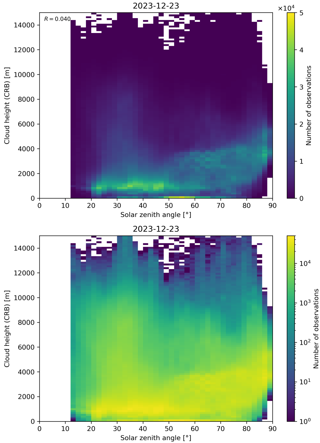
Figure 102: Scatter density plot of “Solar zenith angle” against “Cloud height (CRB)” for 2023-12-22 to 2023-12-24.
