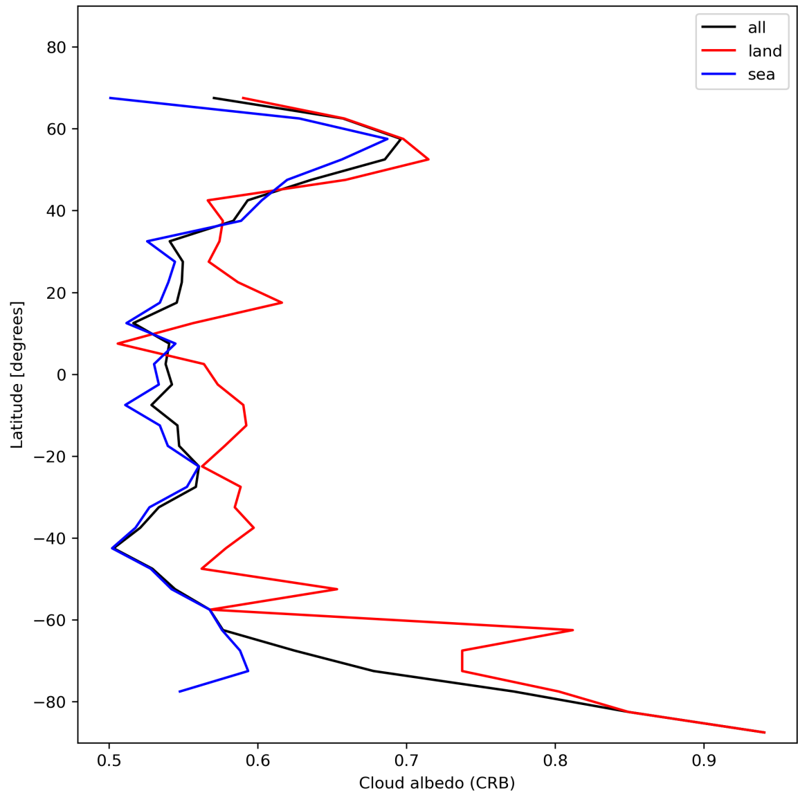
Figure 28: Zonal average of “Cloud albedo (CRB)” for 2023-12-22 to 2023-12-24.
