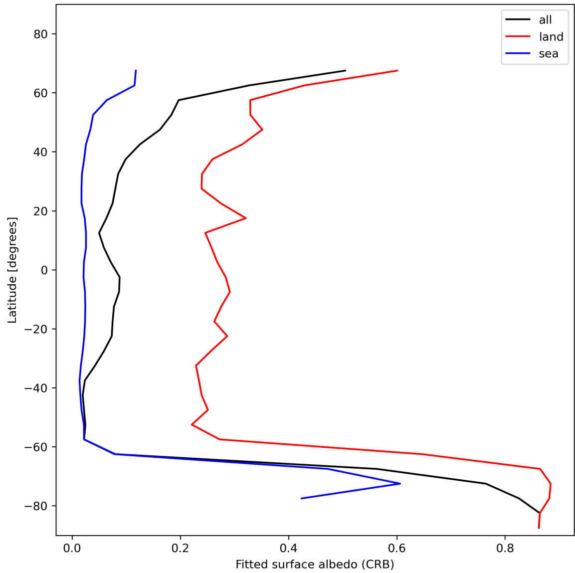
Figure 30: Zonal average of “Fitted surface albedo (CRB)” for 2023-12-22 to 2023-12-24.
