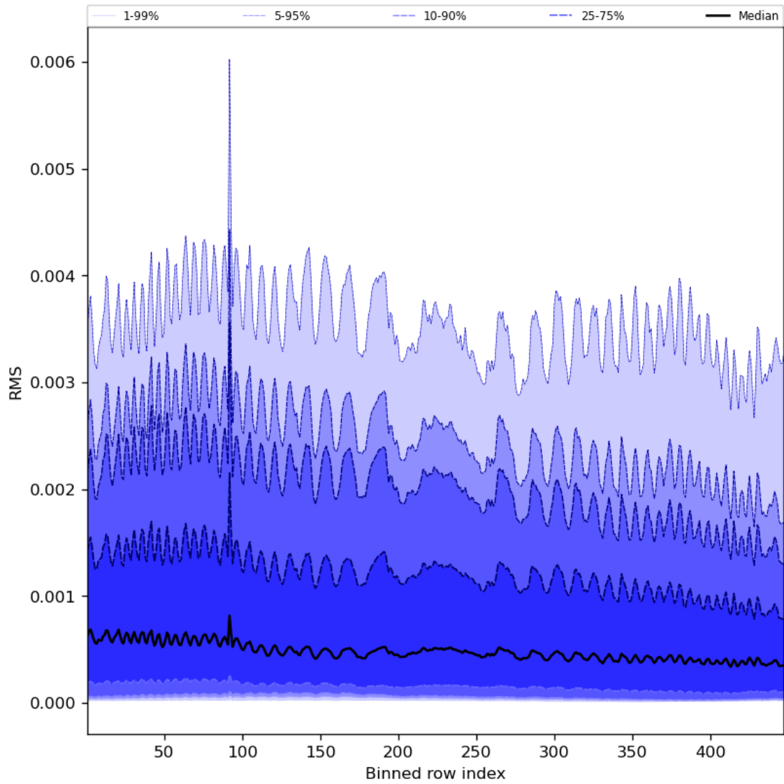
Figure 63: Along track statistics of “RMS” for 2023-12-22 to 2023-12-24
