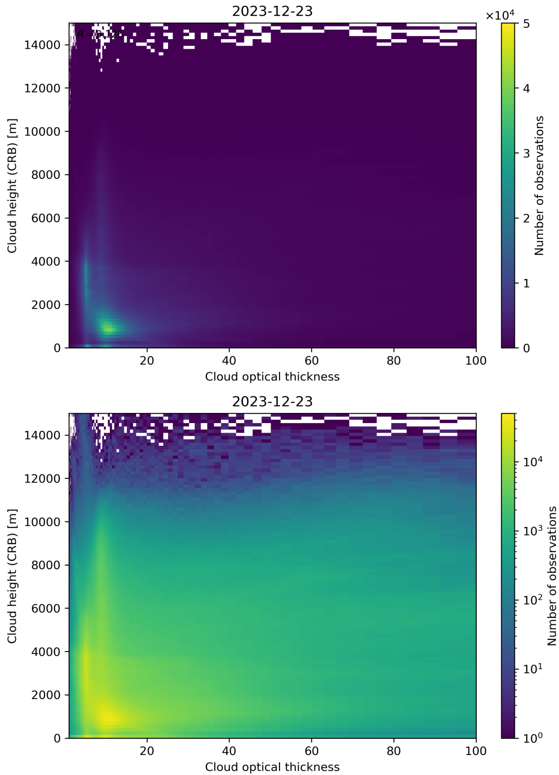
Figure 85: Scatter density plot of “Cloud optical thickness” against “Cloud height (CRB)” for 2023-12-22 to 2023-12-24.
