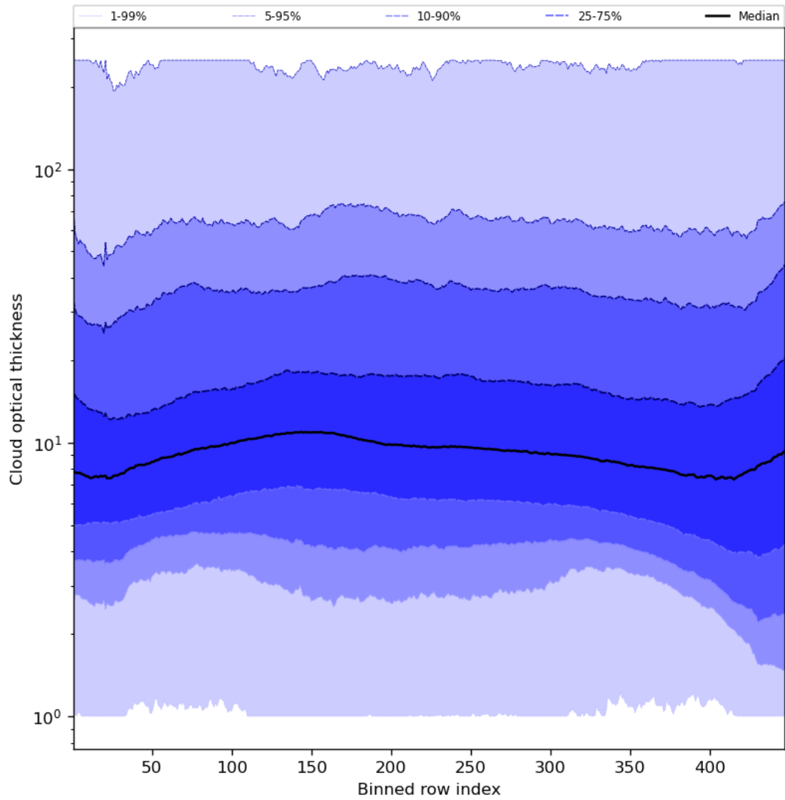
Figure 57: Along track statistics of “Cloud optical thickness” for 2023-12-22 to 2023-12-24
