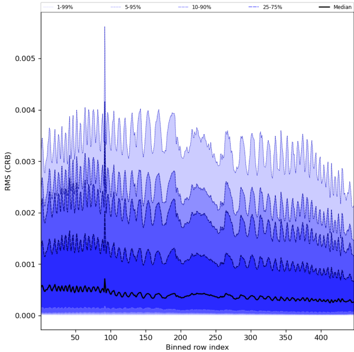
Figure 64: Along track statistics of “RMS (CRB)” for 2023-12-22 to 2023-12-24
