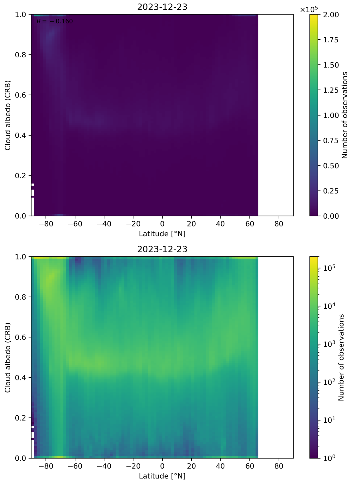
Figure 91: Scatter density plot of “Latitude” against “Cloud albedo (CRB)” for 2023-12-22 to 2023-12-24.
