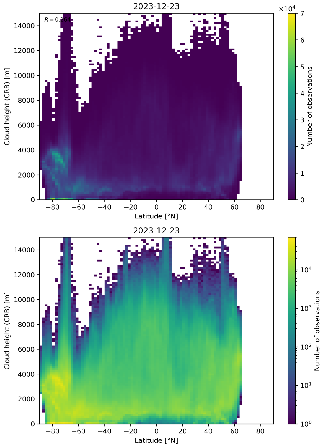
Figure 95: Scatter density plot of “Latitude” against “Cloud height (CRB)” for 2023-12-22 to 2023-12-24.
