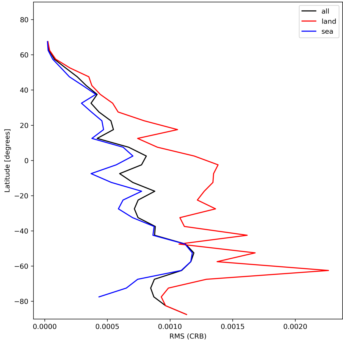
Figure 32: Zonal average of “RMS (CRB)” for 2023-12-22 to 2023-12-24.
