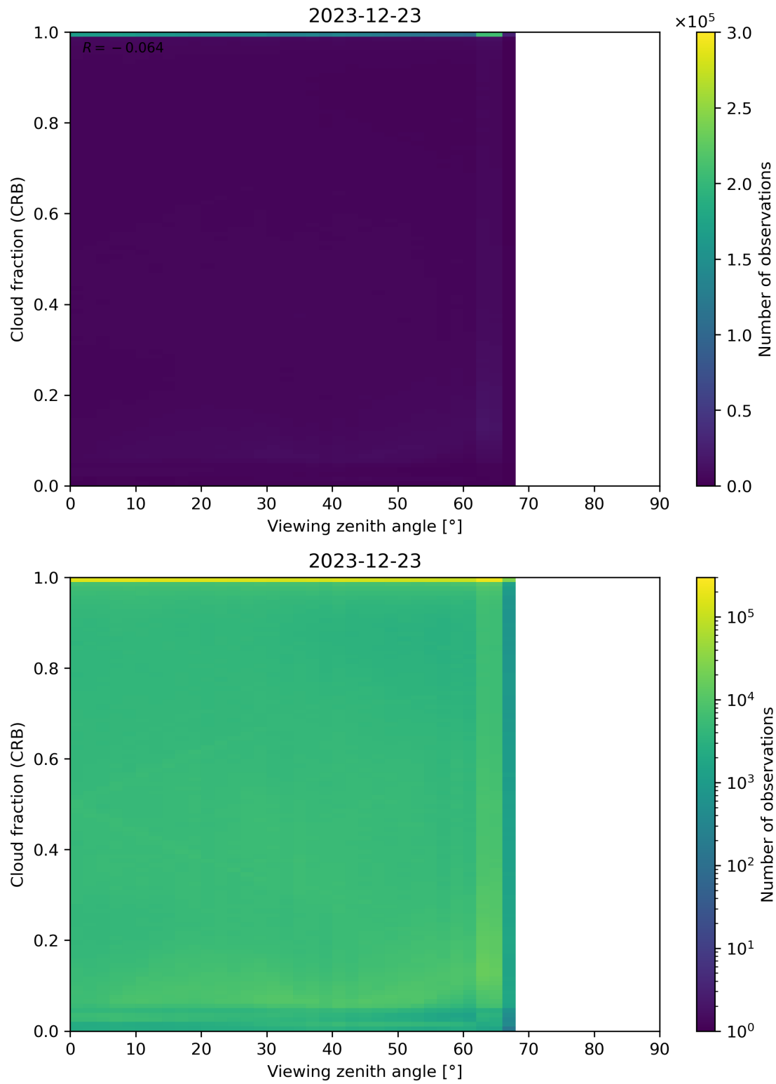
Figure 109: Scatter density plot of “Viewing zenith angle” against “Cloud fraction (CRB)” for 2023-12-22 to 2023-12-24.
