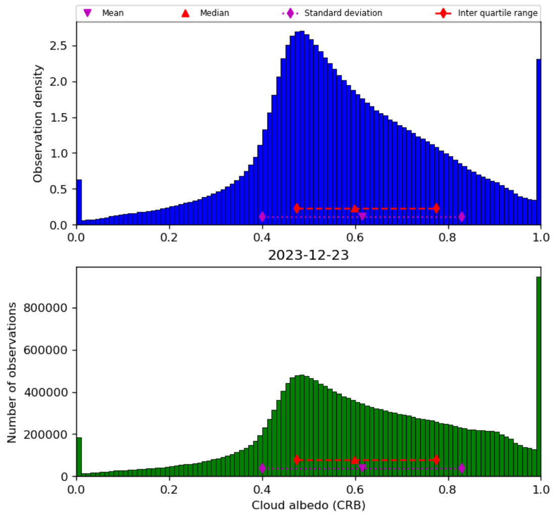
Figure 44: Histogram of “Cloud albedo (CRB)” for 2023-12-22 to 2023-12-24
