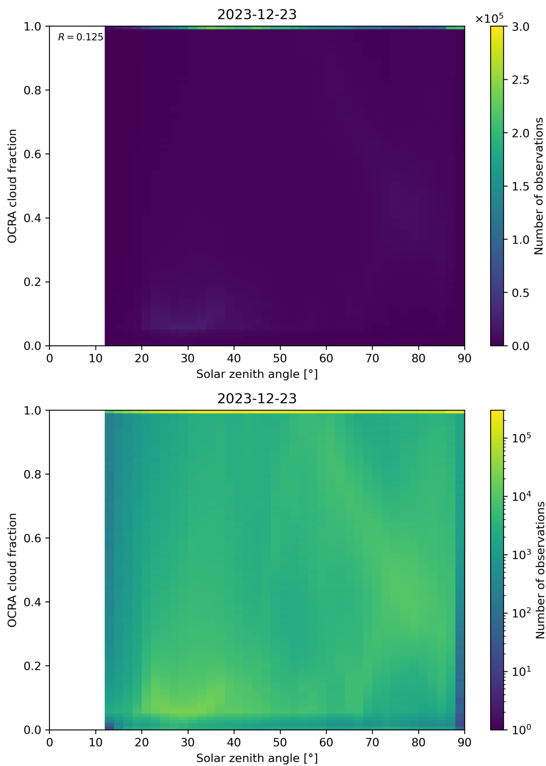
Figure 100: Scatter density plot of “Solar zenith angle” against “OCRA cloud fraction” for 2023-12-22 to 2023-12-24.
