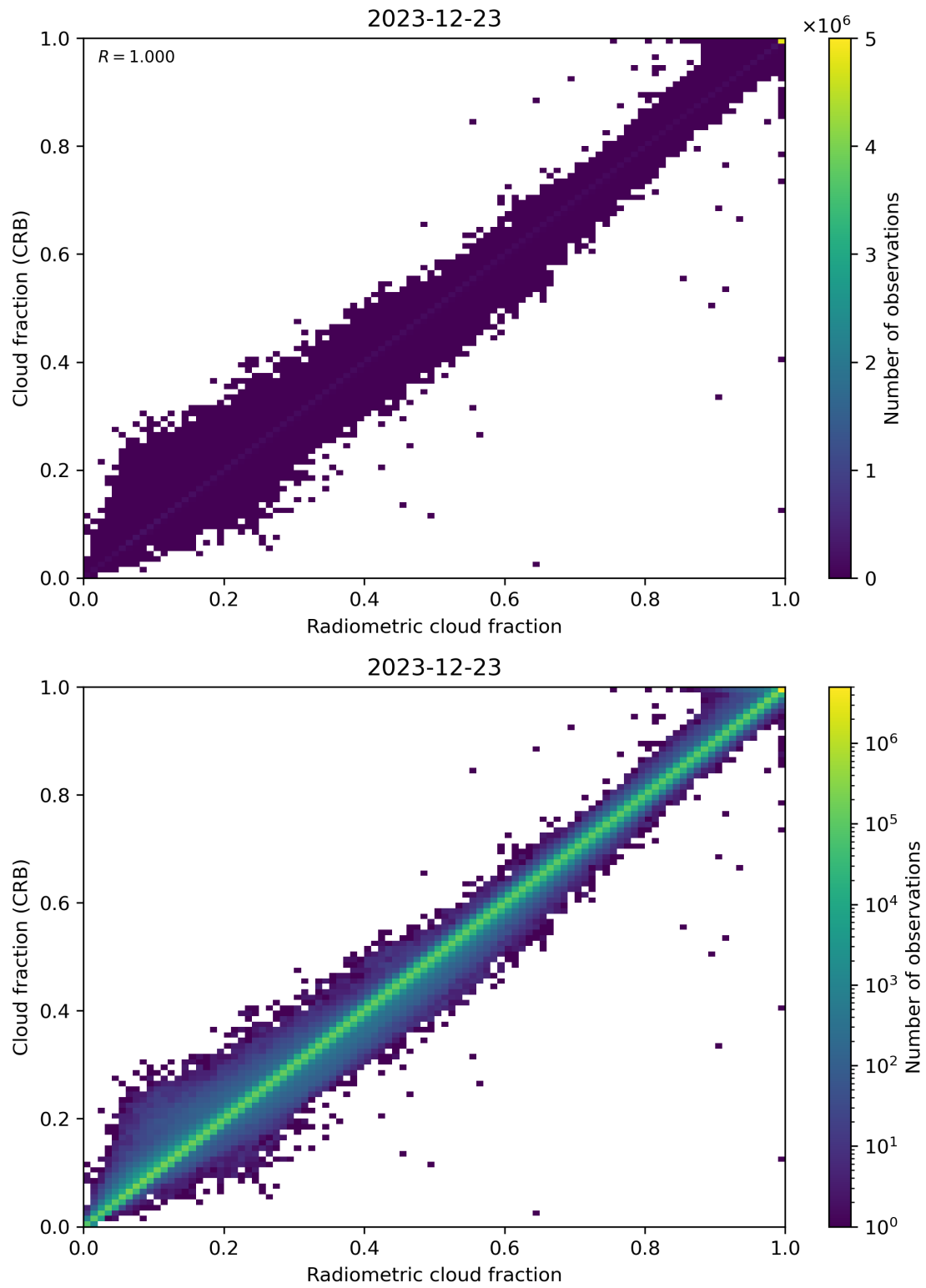
Figure 73: Scatter density plot of “Radiometric cloud fraction” against “Cloud fraction (CRB)” for 2023-12-22 to 2023-12-24.
