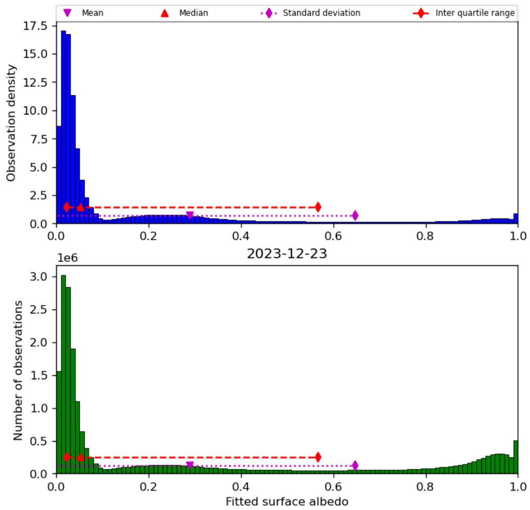
Figure 45: Histogram of “Fitted surface albedo” for 2023-12-22 to 2023-12-24
