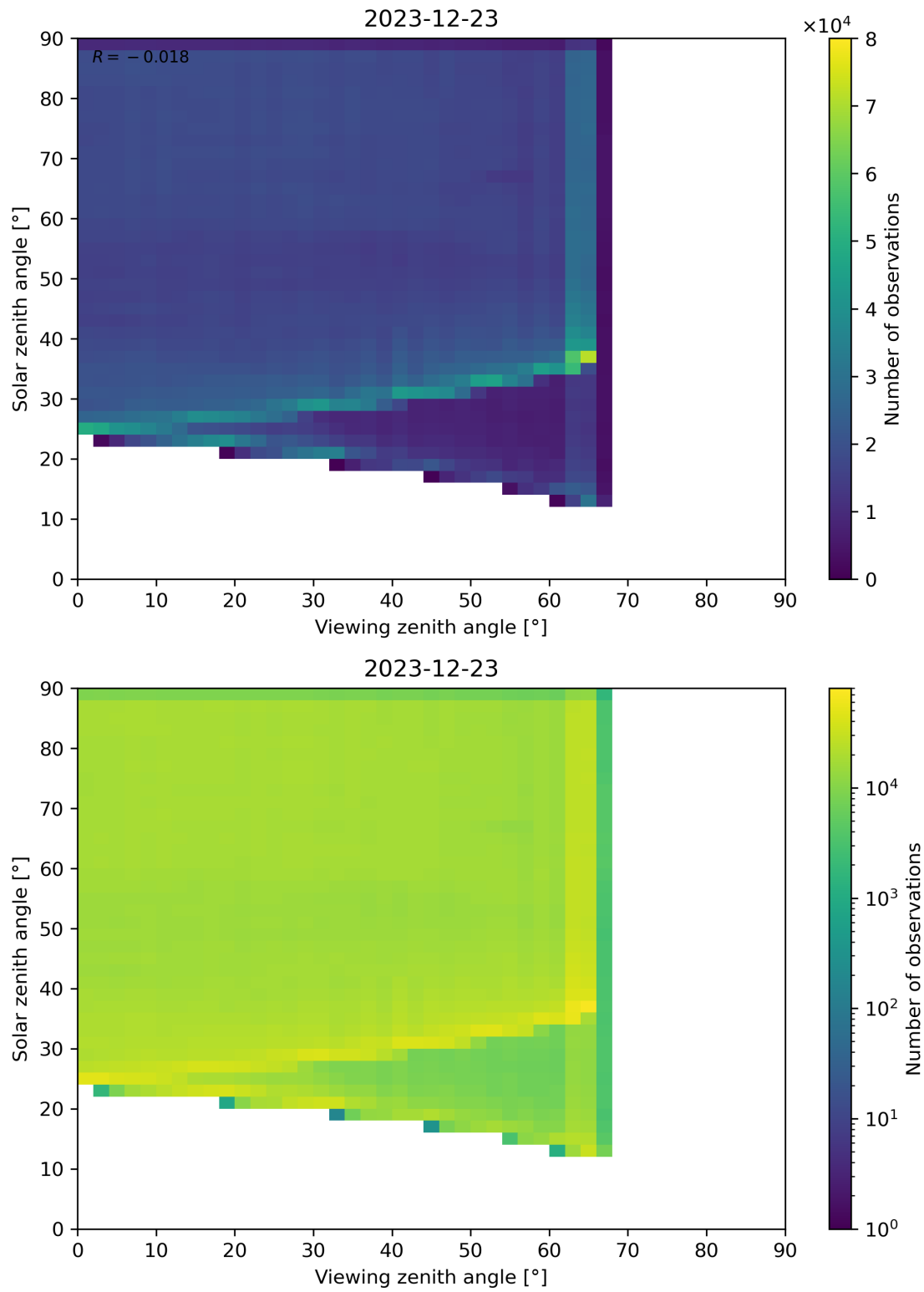
Figure 114: Scatter density plot of “Viewing zenith angle” against “Solar zenith angle” for 2023-12-22 to 2023-12-24.
