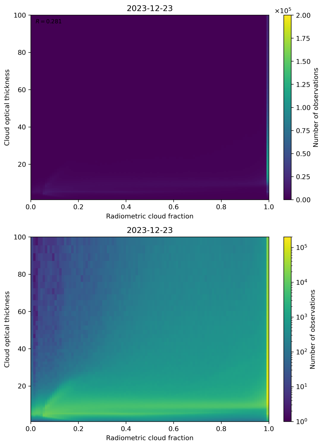
Figure 75: Scatter density plot of “Radiometric cloud fraction” against “Cloud optical thickness” for 2023-12-22 to 2023-12-24.
