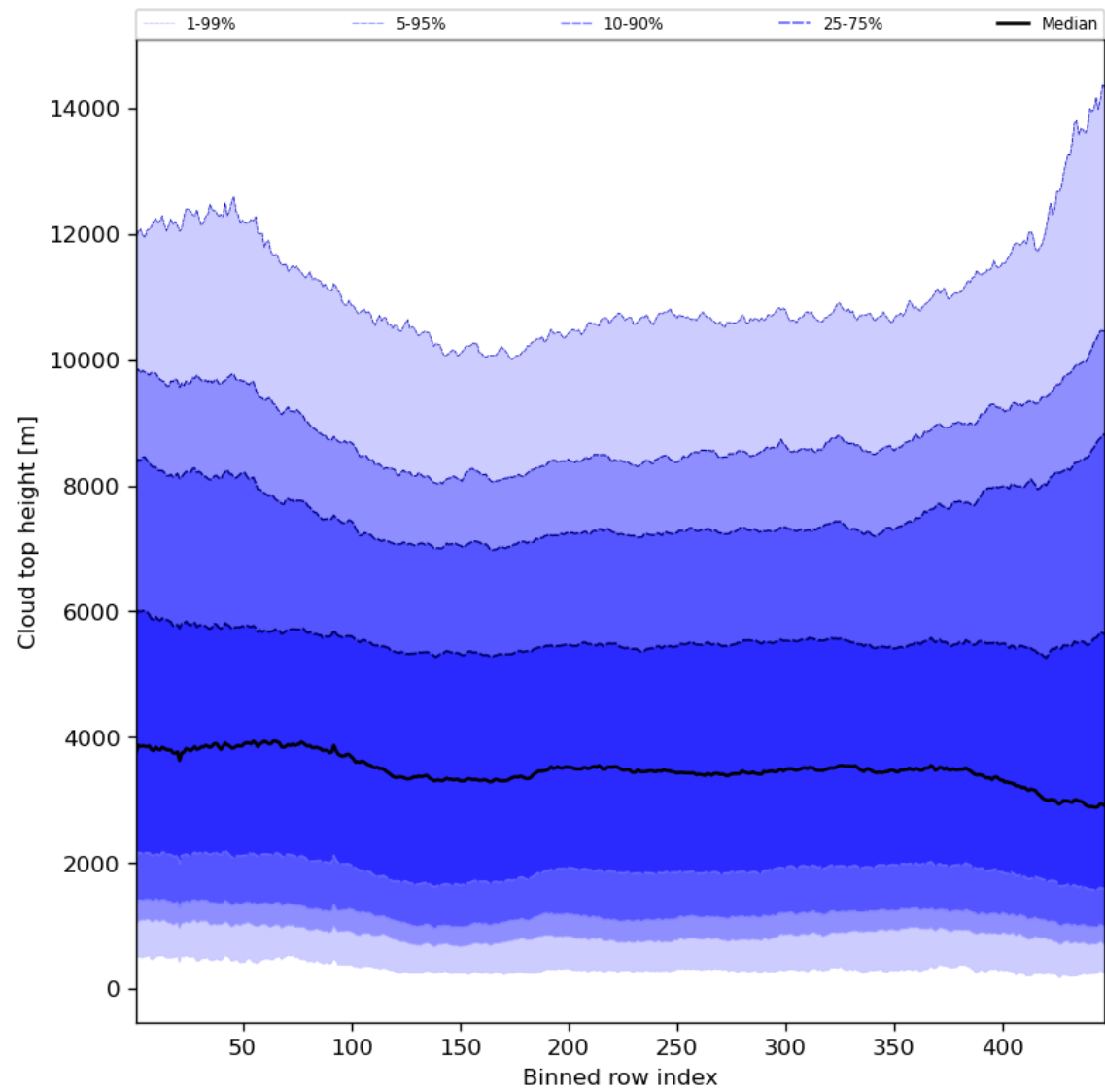
Figure 56: Along track statistics of “Cloud top height” for 2023-12-22 to 2023-12-24
