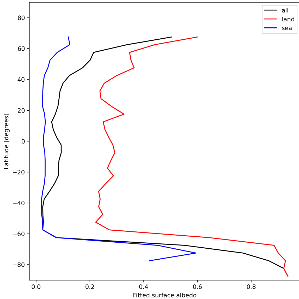
Figure 29: Zonal average of “Fitted surface albedo” for 2023-12-22 to 2023-12-24.
