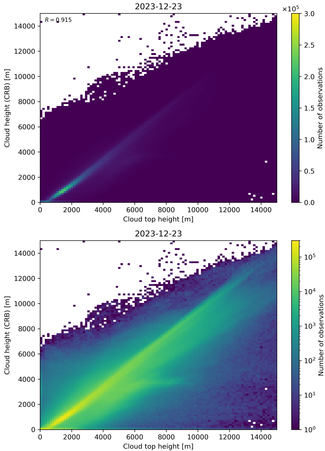
Figure 89: Scatter density plot of “Cloud top height” against “Cloud height (CRB)” for 2023-12-22 to 2023-12-24.
