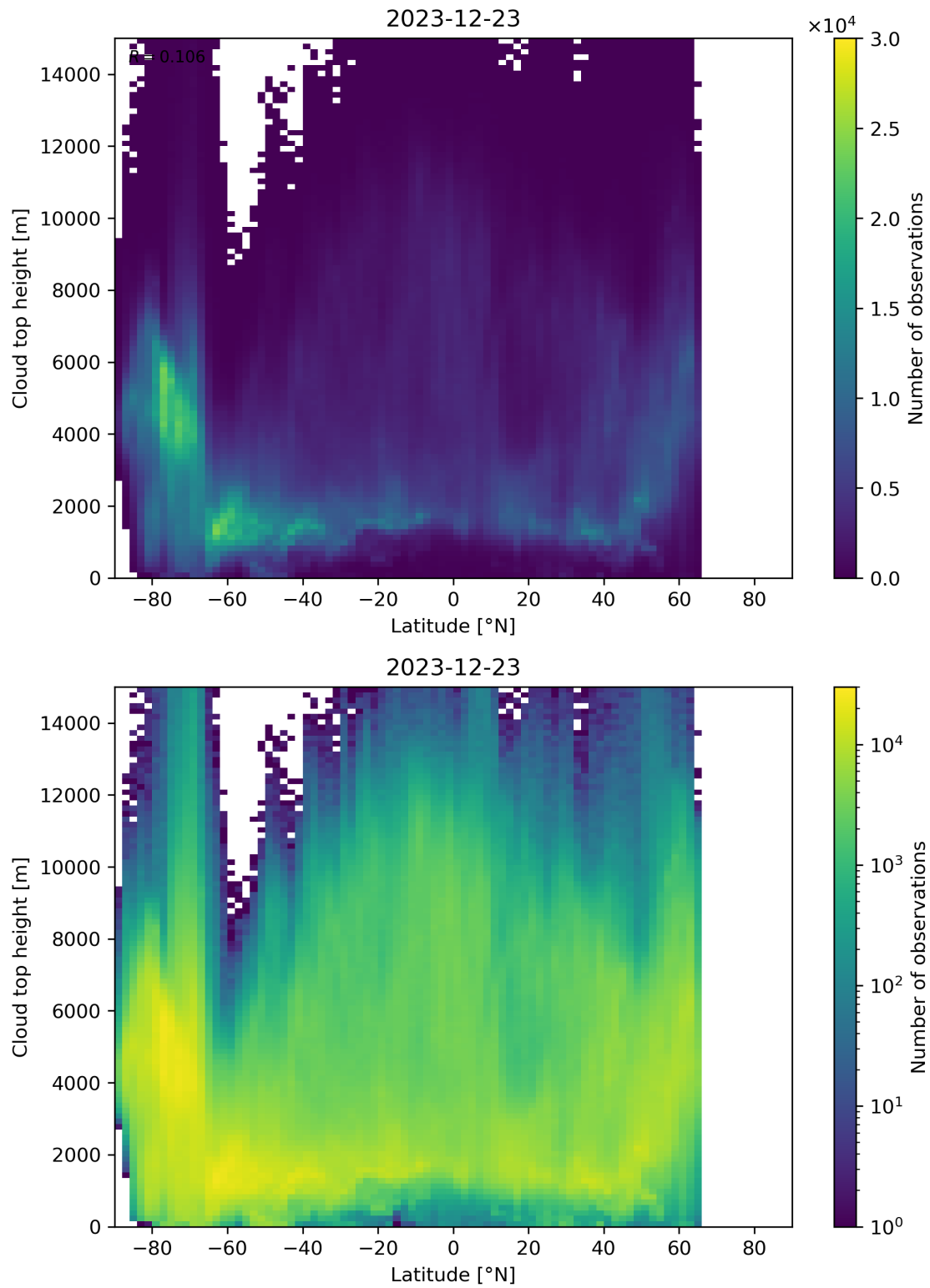
Figure 97: Scatter density plot of “Latitude” against “Cloud top height” for 2023-12-22 to 2023-12-24.
