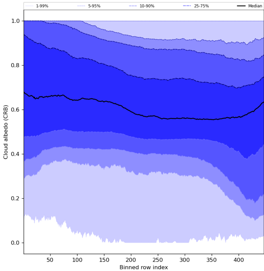
Figure 60: Along track statistics of “Cloud albedo (CRB)” for 2023-12-22 to 2023-12-24
