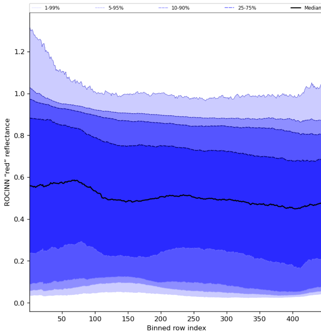
Figure 69: Along track statistics of “ROCINN “red” reflectance” for 2023-12-22 to 2023-12-24
