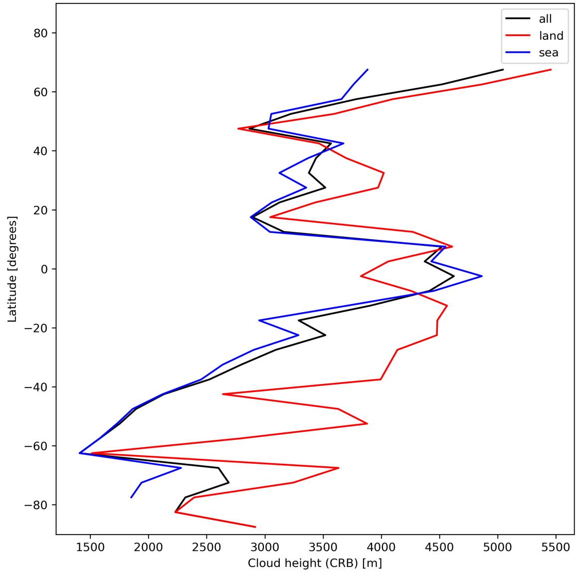
Figure 27: Zonal average of “Cloud height (CRB)” for 2023-12-22 to 2023-12-24.
