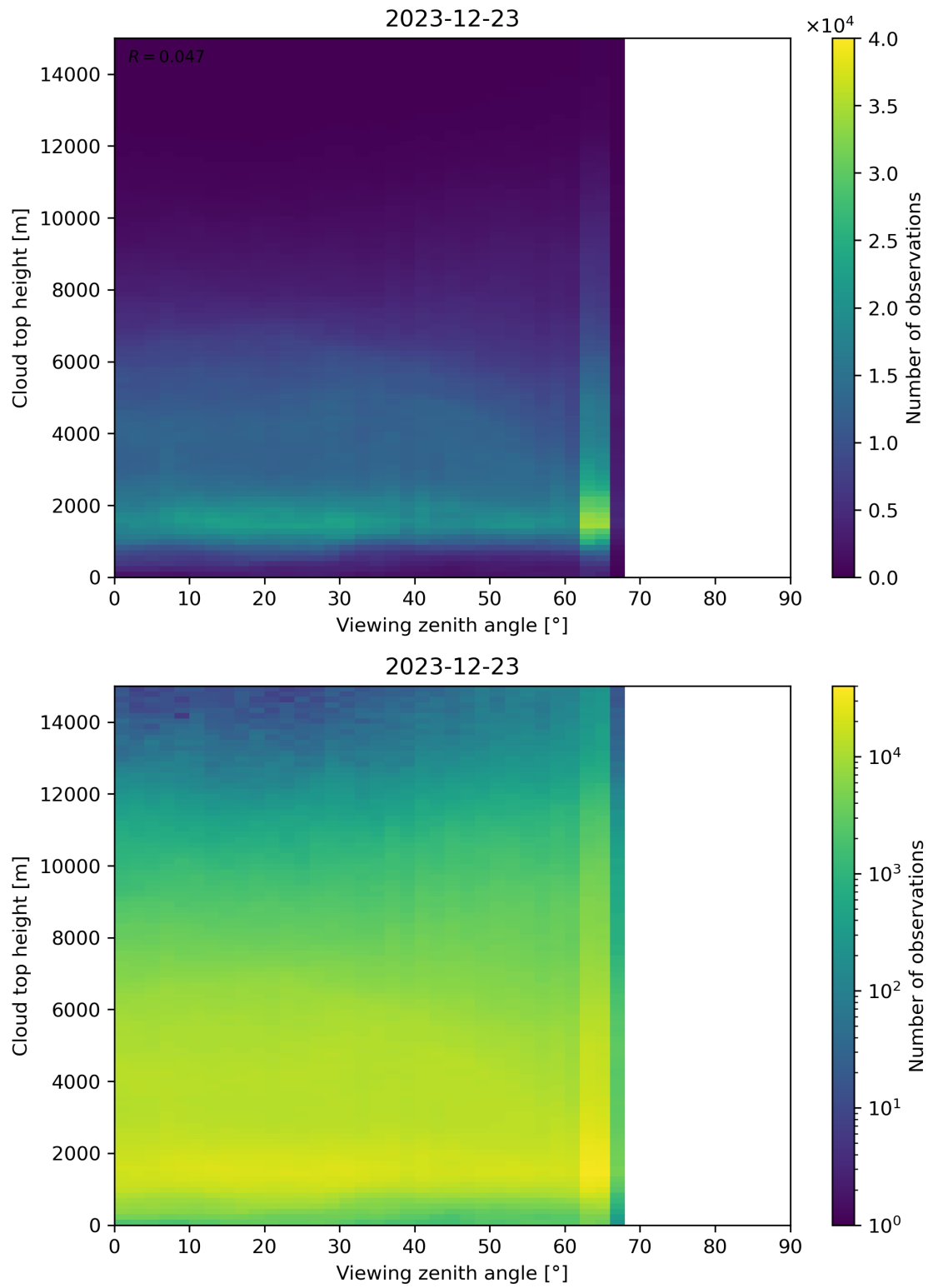
Figure 112: Scatter density plot of “Viewing zenith angle” against “Cloud top height” for 2023-12-22 to 2023-12-24.
