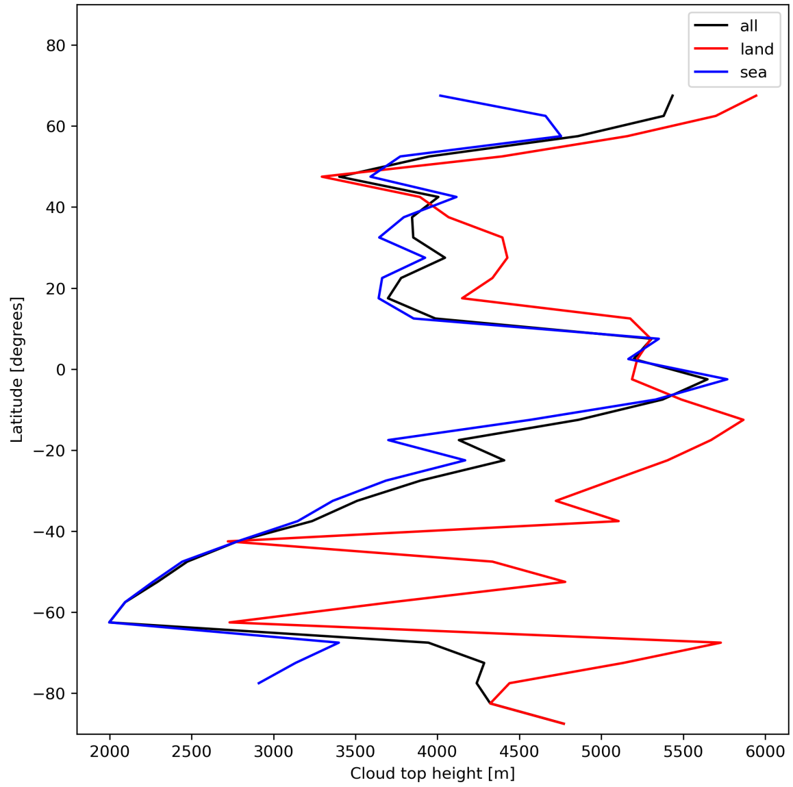
Figure 24: Zonal average of “Cloud top height” for 2023-12-22 to 2023-12-24.
