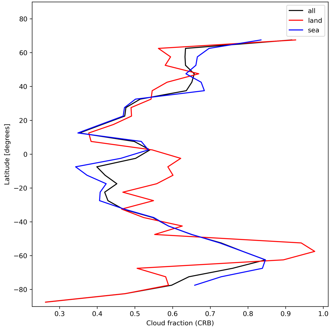
Figure 26: Zonal average of “Cloud fraction (CRB)” for 2023-12-22 to 2023-12-24.
