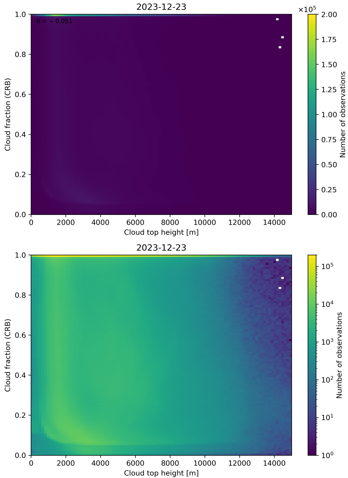
Figure 88: Scatter density plot of “Cloud top height” against “Cloud fraction (CRB)” for 2023-12-22 to 2023-12-24.
