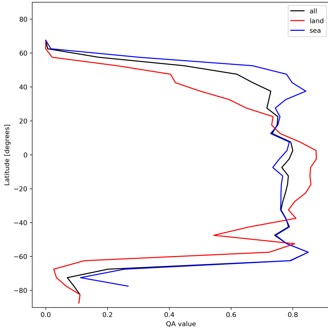
Figure 22: Zonal average of “QA value” for 2023-12-22 to 2023-12-24.
