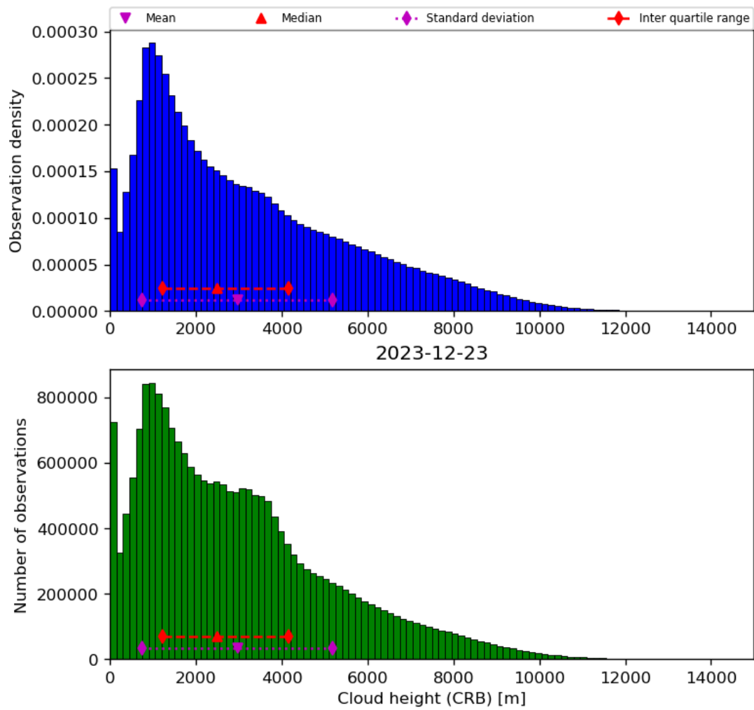
Figure 43: Histogram of “Cloud height (CRB)” for 2023-12-22 to 2023-12-24
