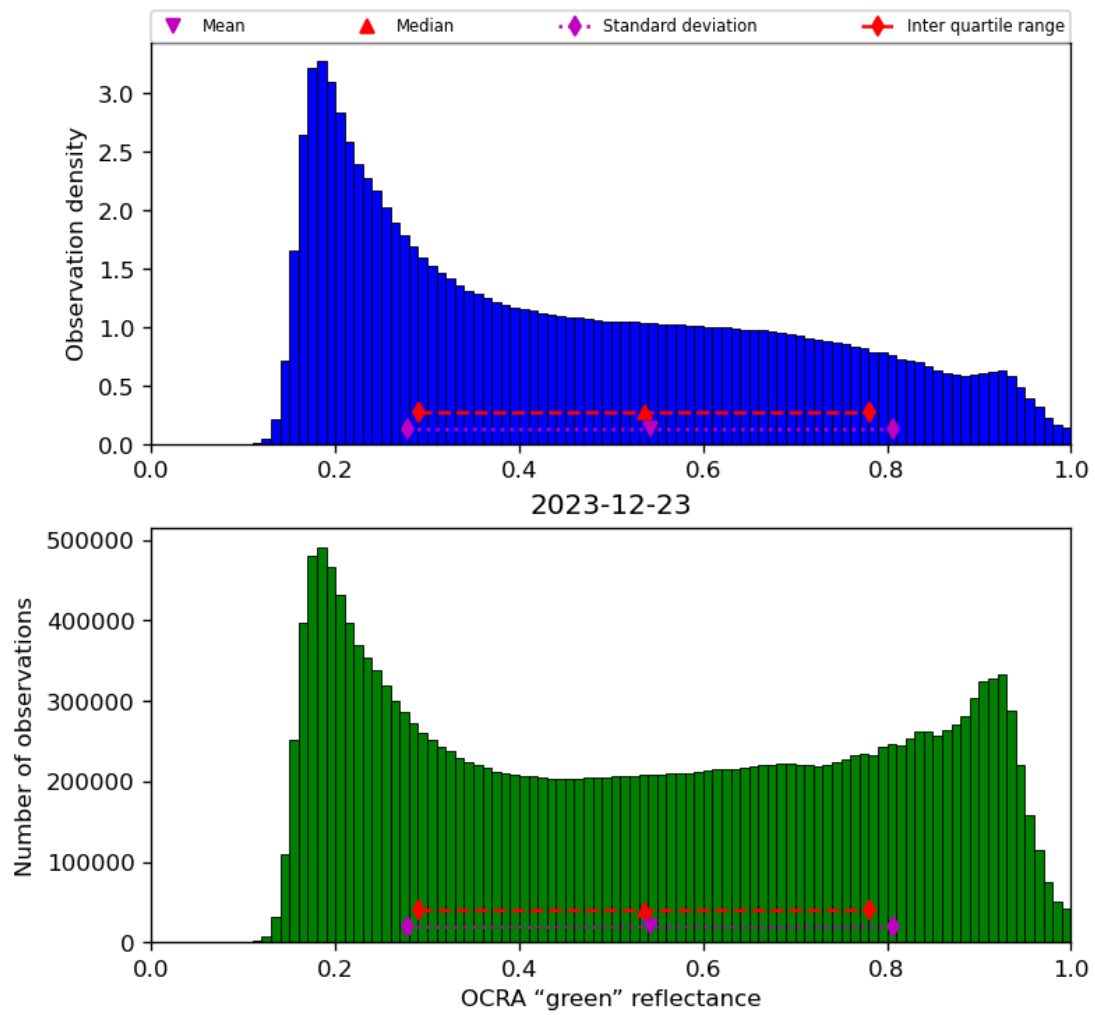
Figure 52: Histogram of “OCRA “green” reflectance” for 2023-12-22 to 2023-12-24
