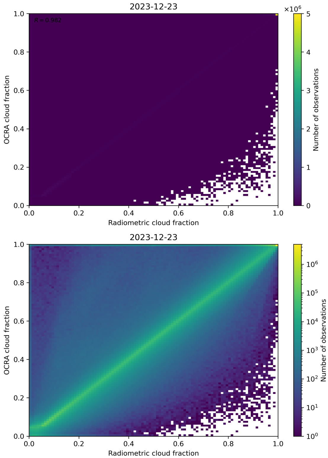
Figure 72: Scatter density plot of “Radiometric cloud fraction” against “OCRA cloud fraction” for 2023-12-22 to 2023-12-24.
