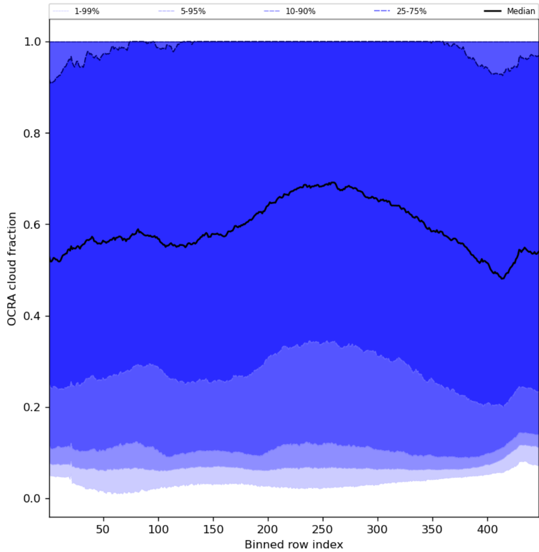
Figure 66: Along track statistics of “OCRA cloud fraction” for 2023-12-22 to 2023-12-24
