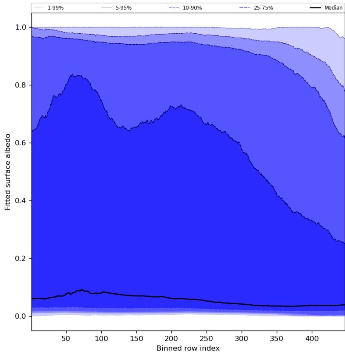
Figure 61: Along track statistics of “Fitted surface albedo” for 2023-12-22 to 2023-12-24
