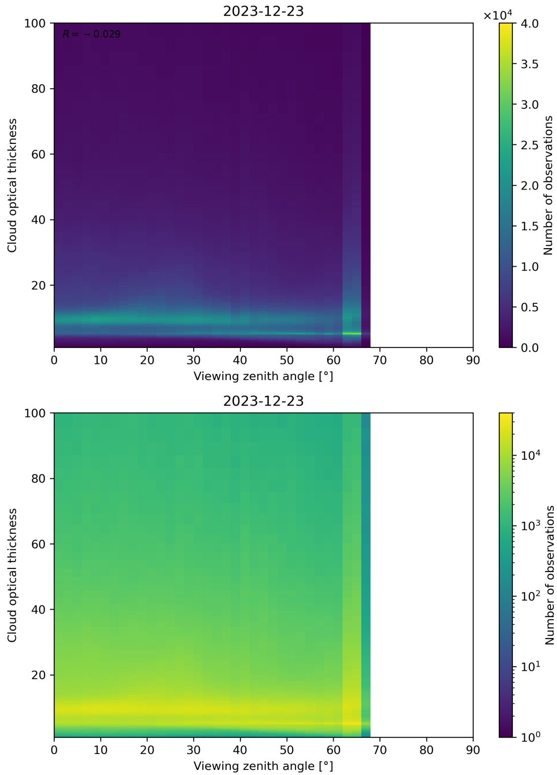
Figure 111: Scatter density plot of “Viewing zenith angle” against “Cloud optical thickness” for 2023-12-22 to 2023-12-24.
