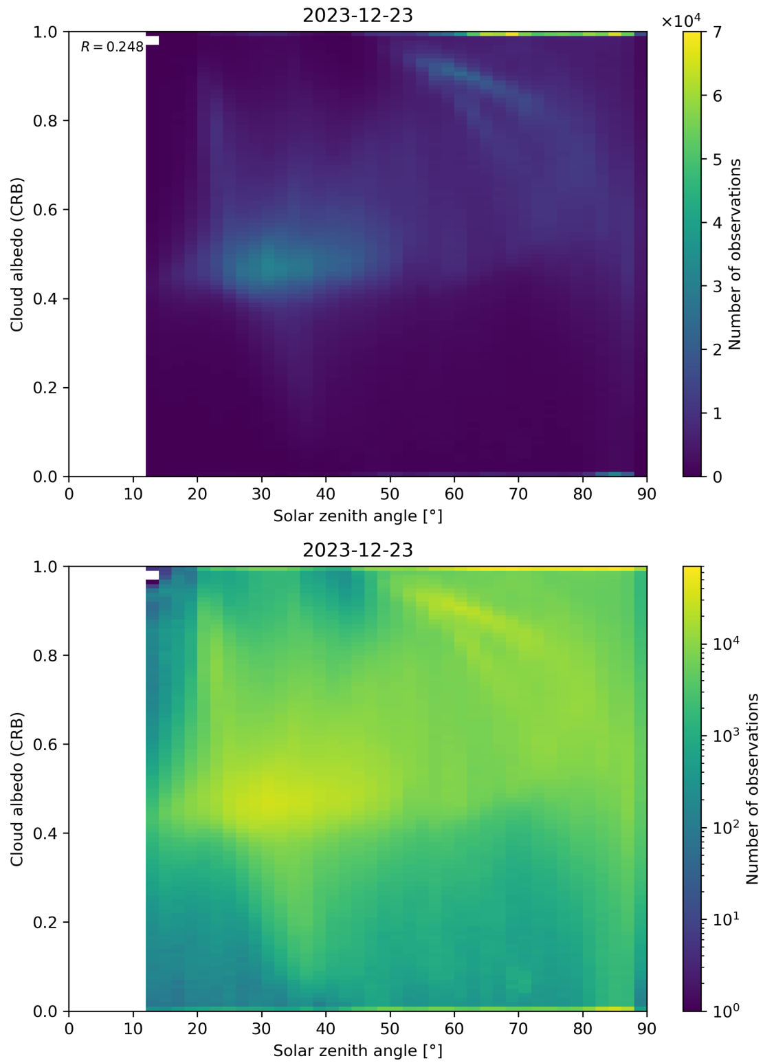
Figure 98: Scatter density plot of “Solar zenith angle” against “Cloud albedo (CRB)” for 2023-12-22 to 2023-12-24.
