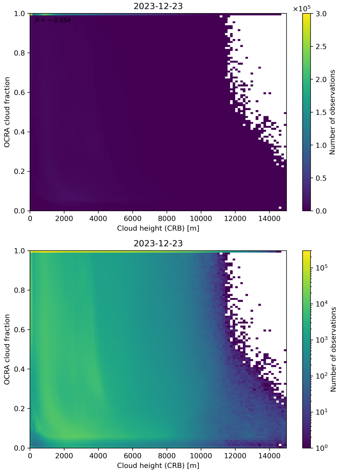
Figure 81: Scatter density plot of “Cloud height (CRB)” against “OCRA cloud fraction” for 2023-12-22 to 2023-12-24.
