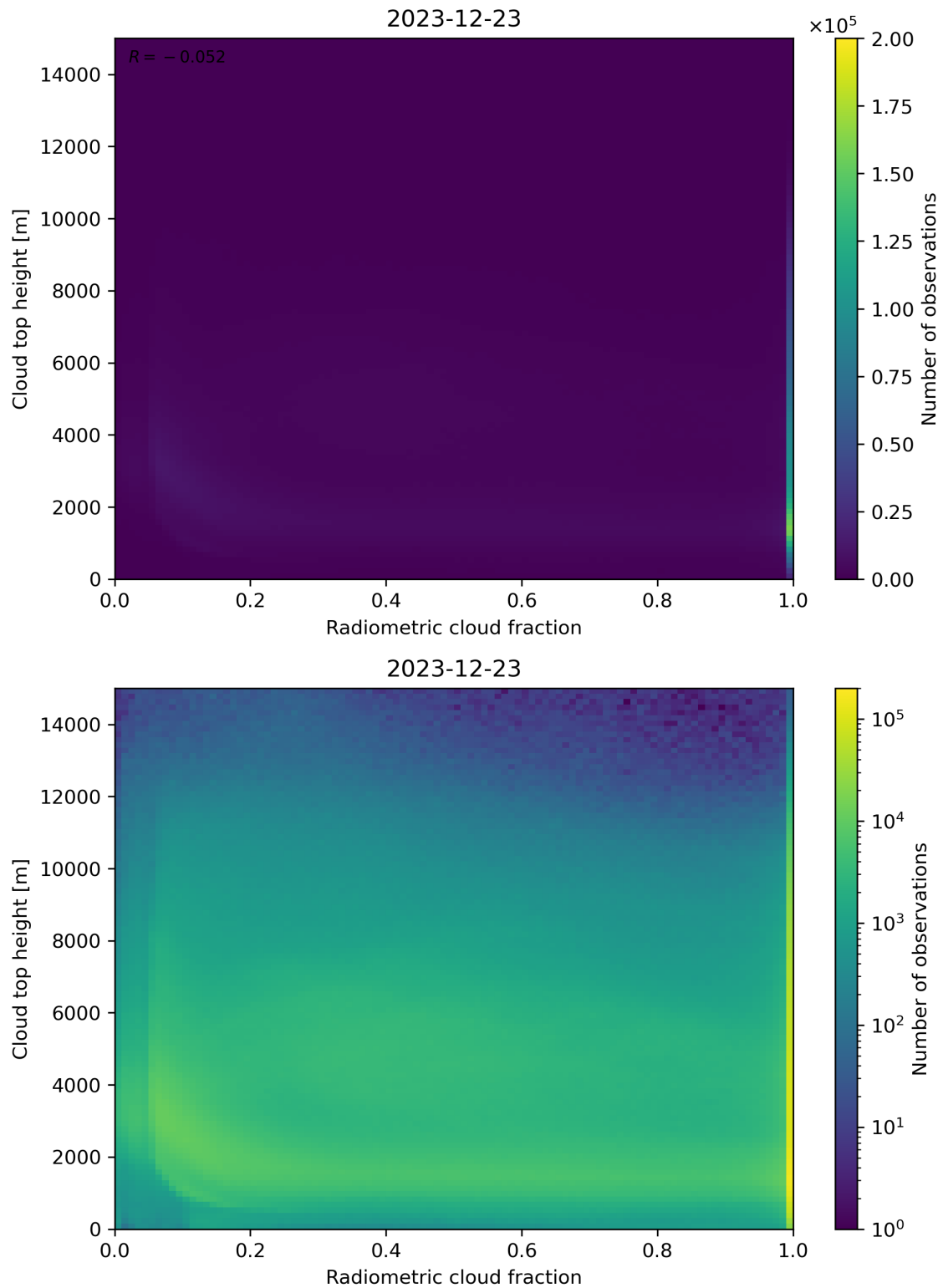
Figure 76: Scatter density plot of “Radiometric cloud fraction” against “Cloud top height” for 2023-12-22 to 2023-12-24.
