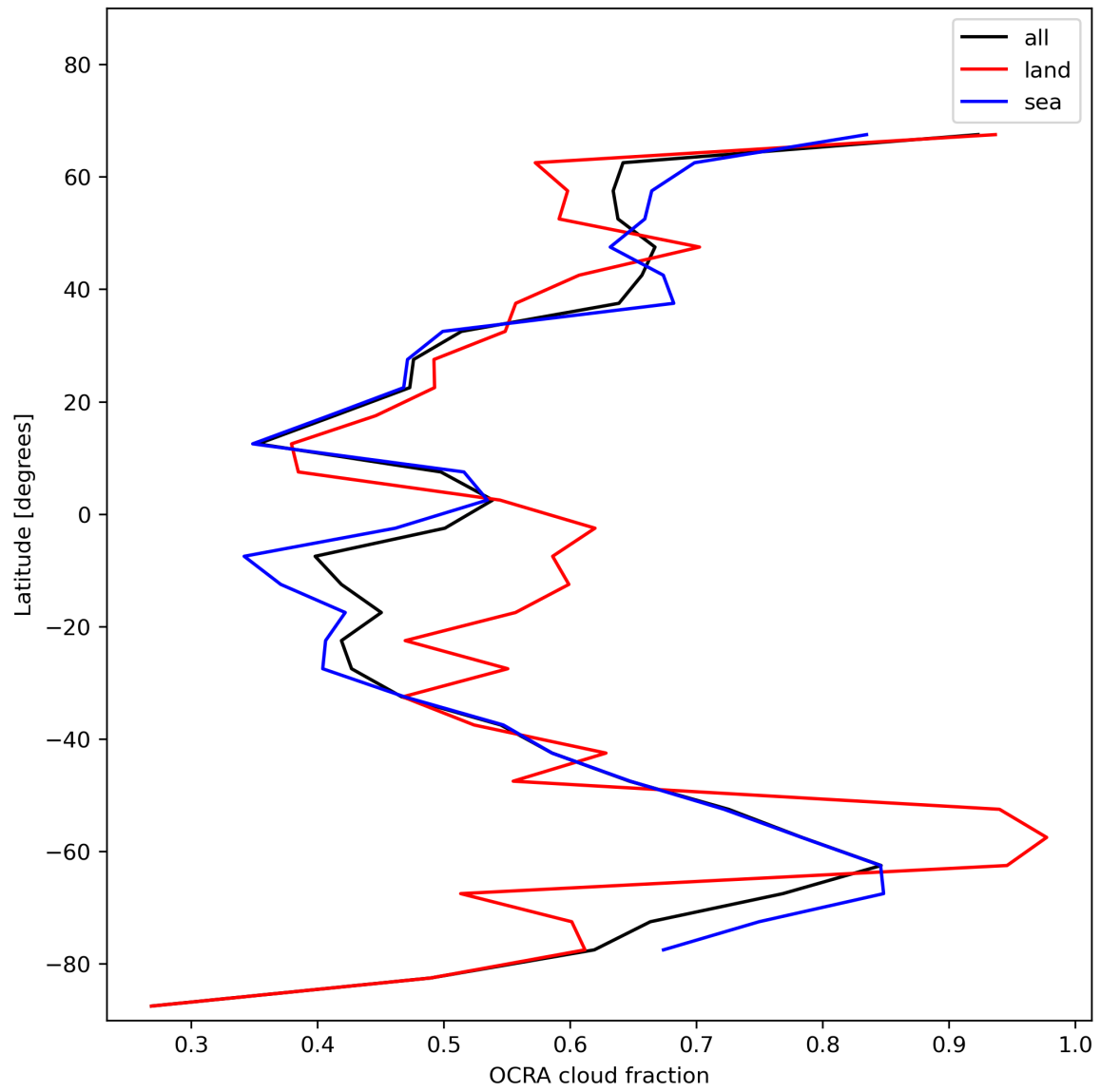
Figure 34: Zonal average of “OCRA cloud fraction” for 2023-12-22 to 2023-12-24.
