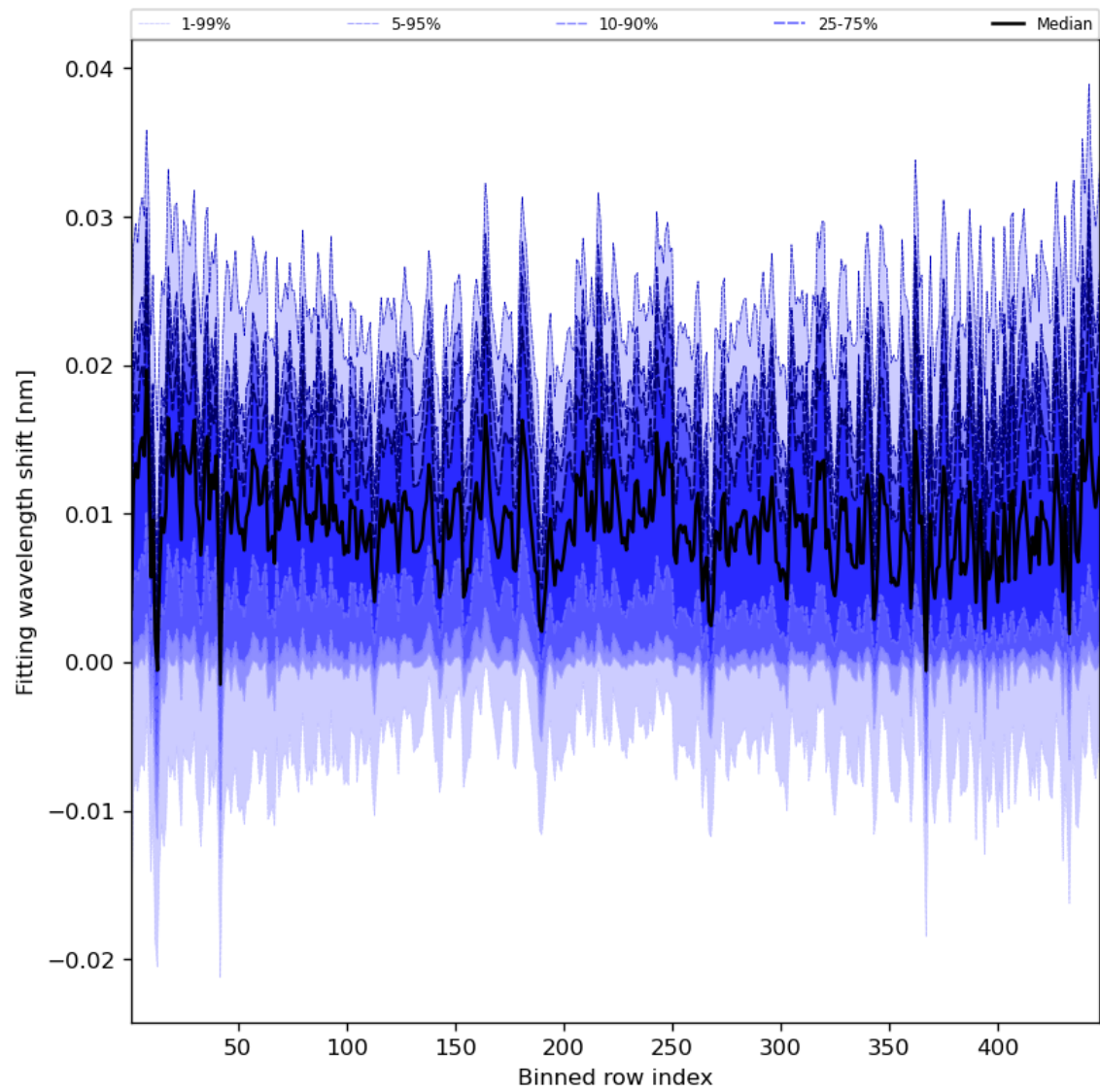
Figure 65: Along track statistics of “Fitting wavelength shift” for 2023-12-22 to 2023-12-24
