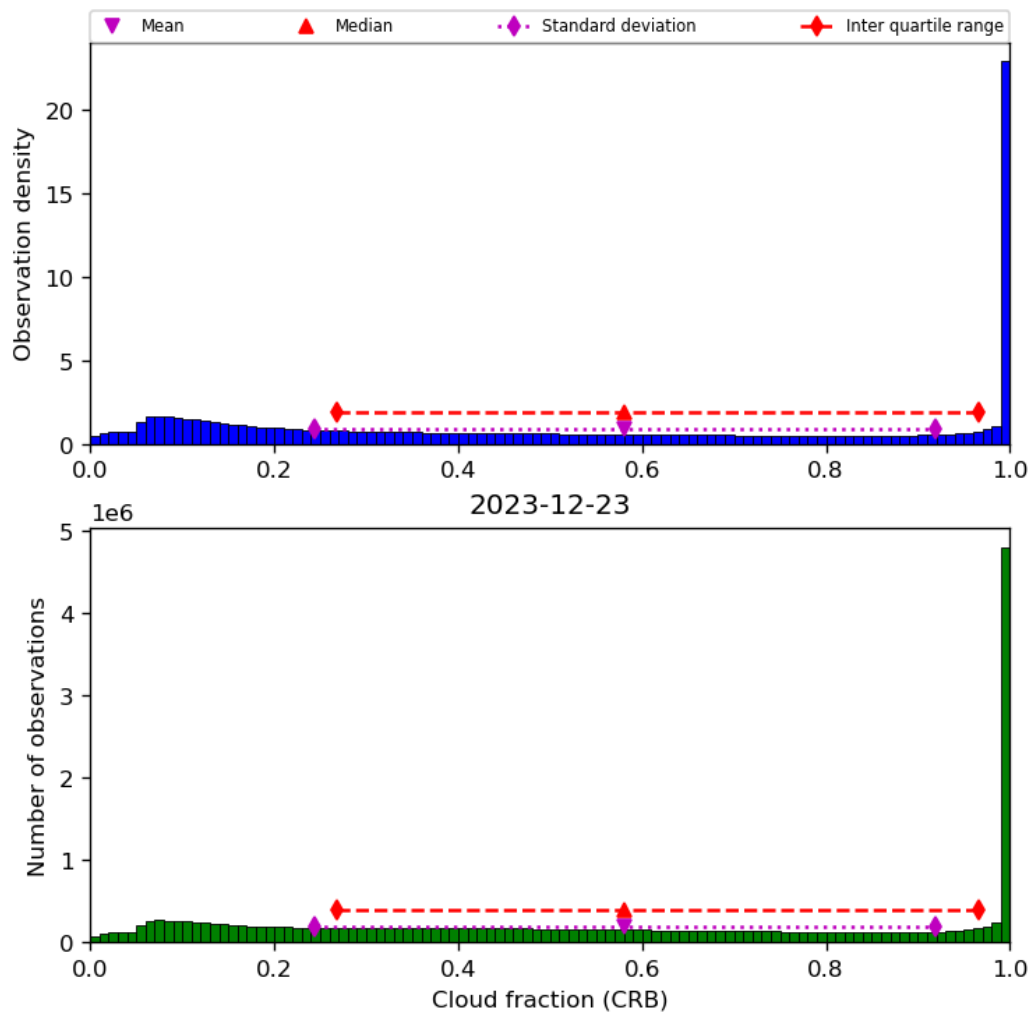
Figure 42: Histogram of “Cloud fraction (CRB)” for 2023-12-22 to 2023-12-24
