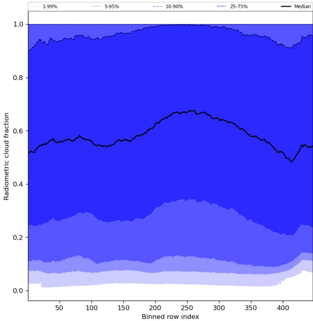
Figure 55: Along track statistics of “Radiometric cloud fraction” for 2023-12-22 to 2023-12-24
