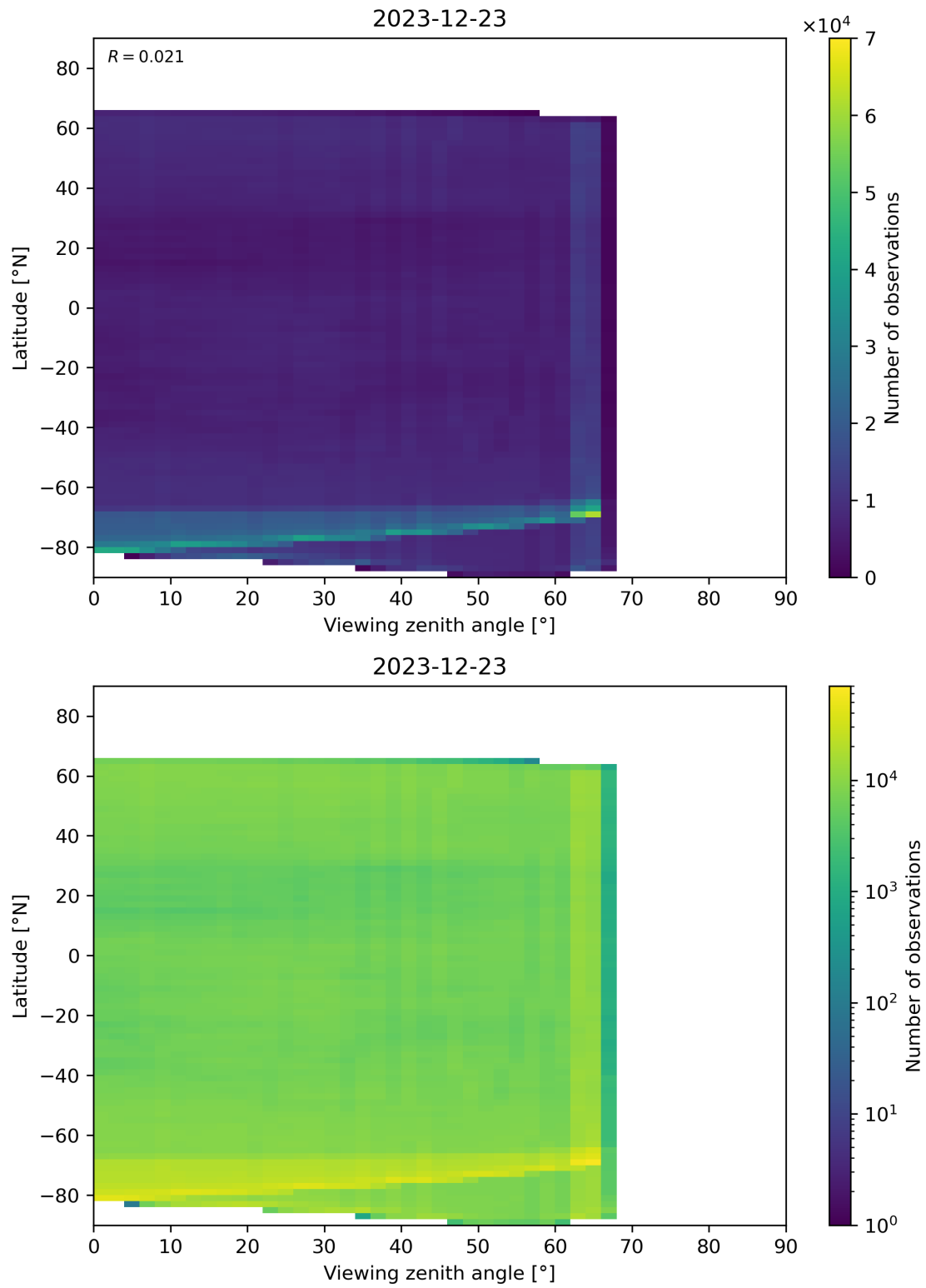
Figure 113: Scatter density plot of “Viewing zenith angle” against “Latitude” for 2023-12-22 to 2023-12-24.
