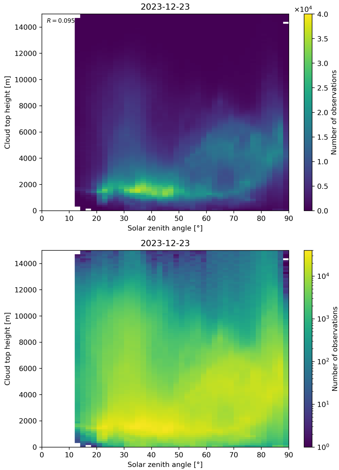
Figure 104: Scatter density plot of “Solar zenith angle” against “Cloud top height” for 2023-12-22 to 2023-12-24.
