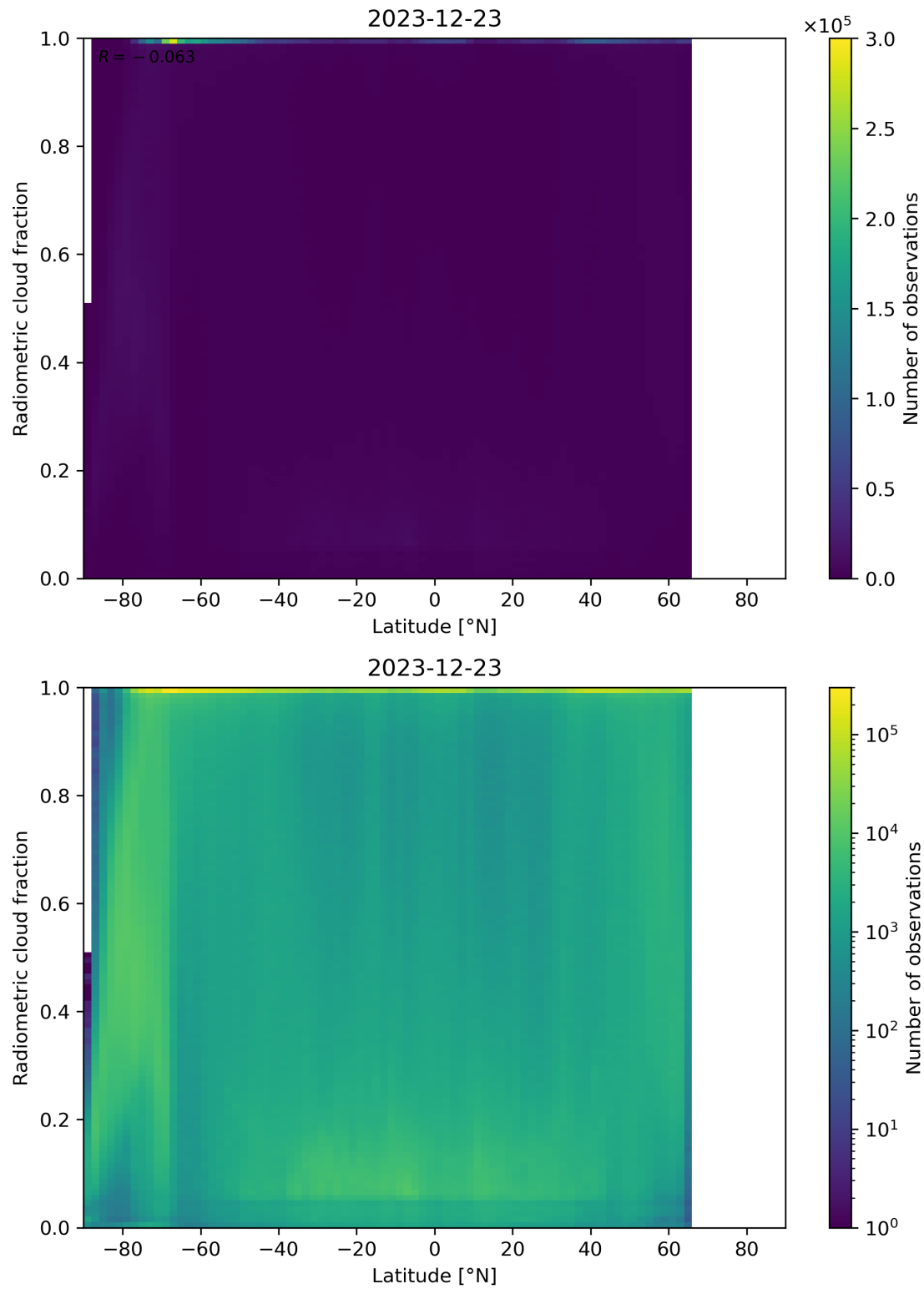
Figure 92: Scatter density plot of “Latitude” against “Radiometric cloud fraction” for 2023-12-22 to 2023-12-24.
