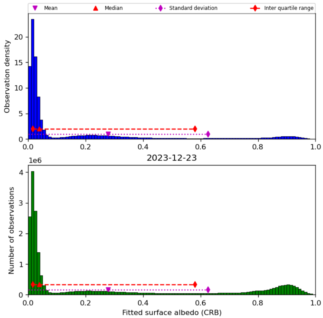
Figure 46: Histogram of “Fitted surface albedo (CRB)” for 2023-12-22 to 2023-12-24
