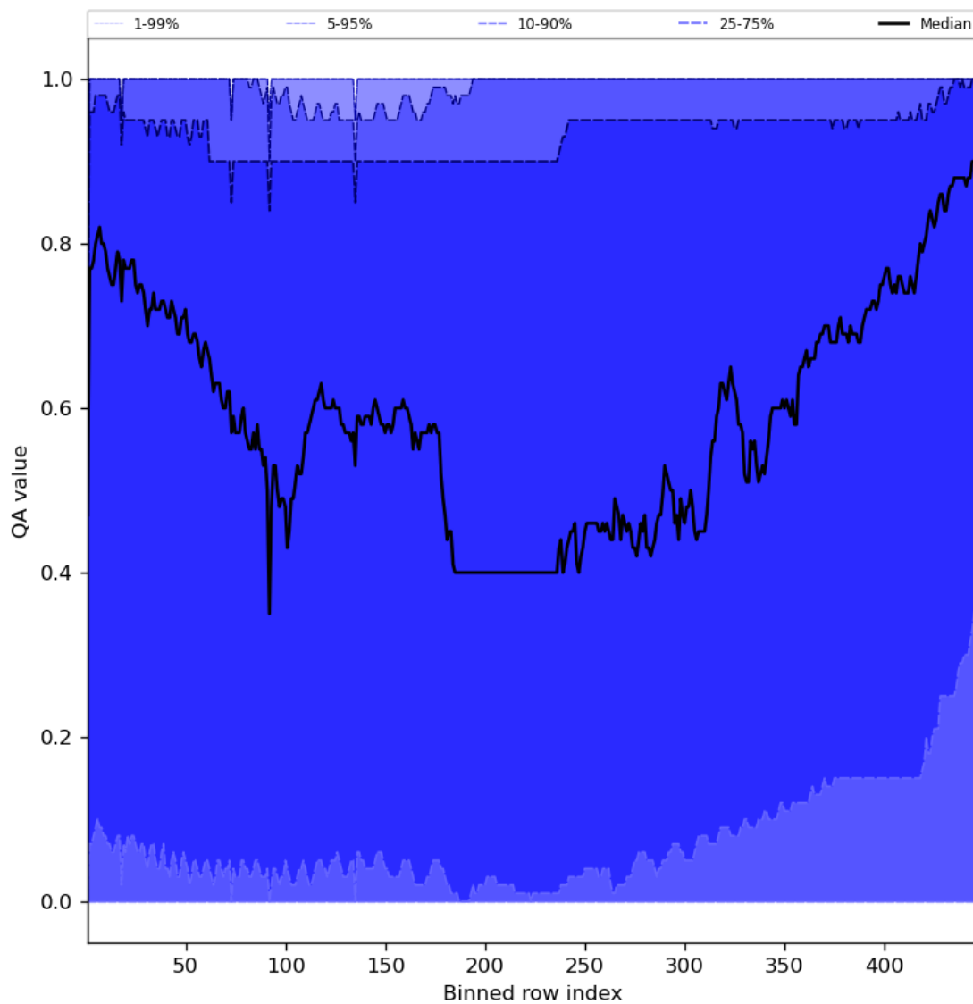
Figure 54: Along track statistics of “QA value” for 2023-12-22 to 2023-12-24
