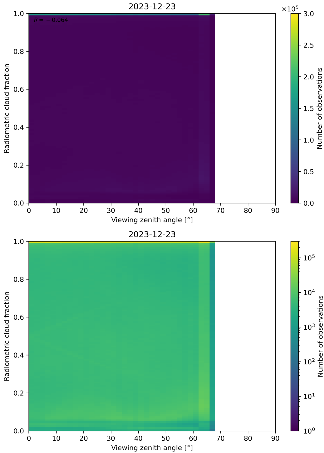
Figure 107: Scatter density plot of “Viewing zenith angle” against “Radiometric cloud fraction” for 2023-12-22 to 2023-12-24.
