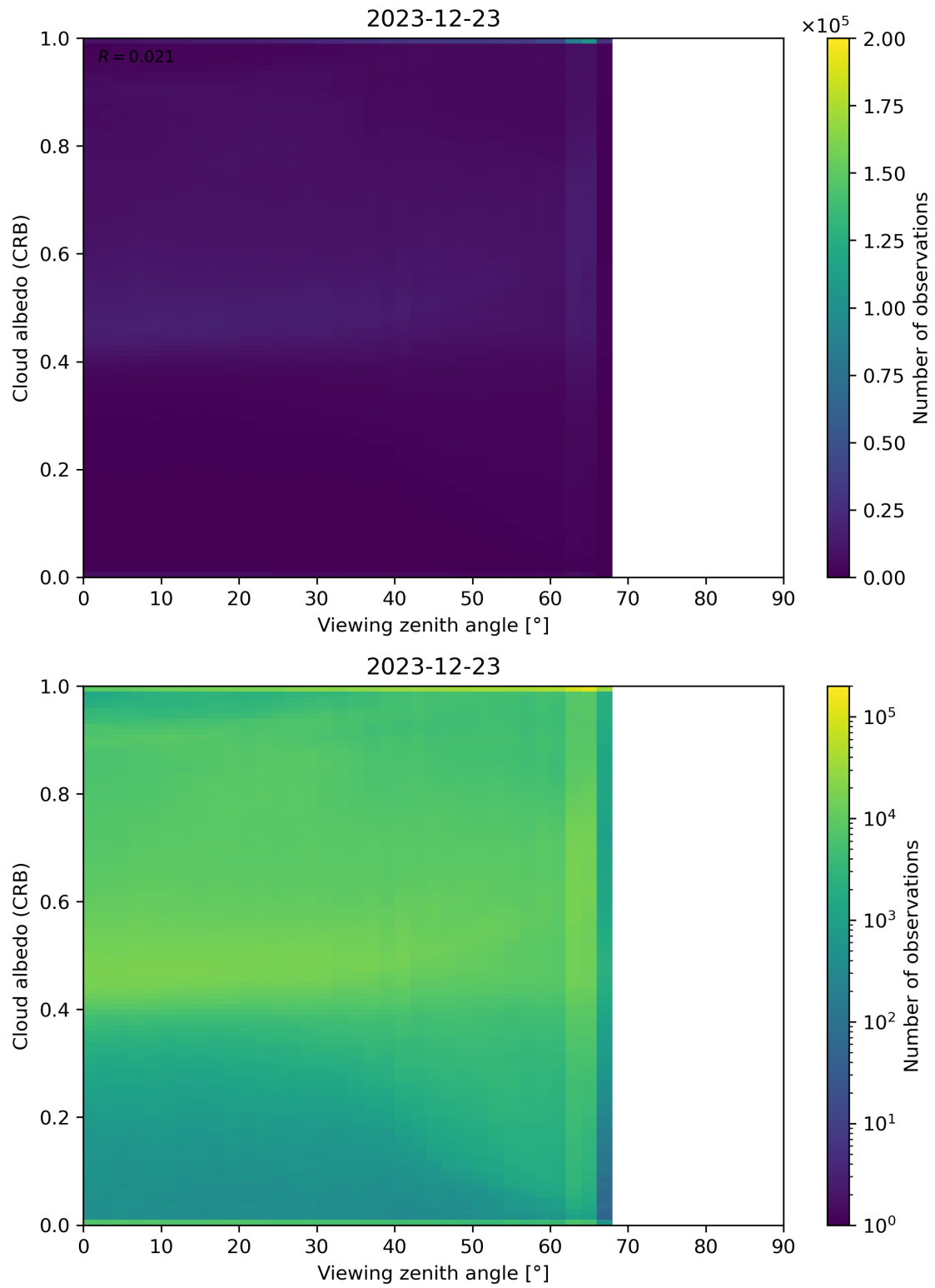
Figure 106: Scatter density plot of “Viewing zenith angle” against “Cloud albedo (CRB)” for 2023-12-22 to 2023-12-24.
