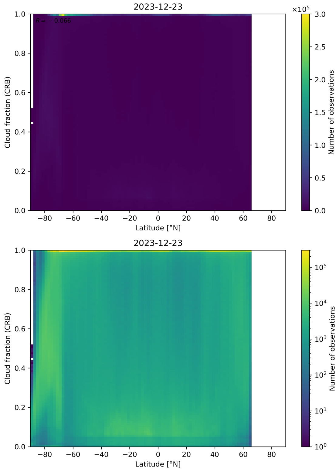
Figure 94: Scatter density plot of “Latitude” against “Cloud fraction (CRB)” for 2023-12-22 to 2023-12-24.
