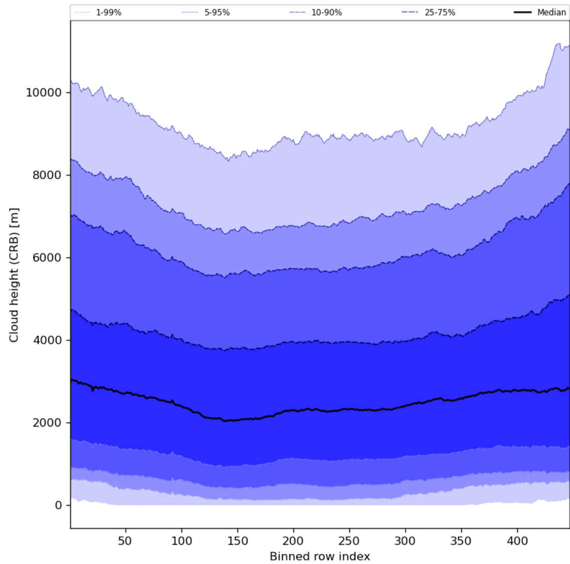
Figure 59: Along track statistics of “Cloud height (CRB)” for 2023-12-22 to 2023-12-24
