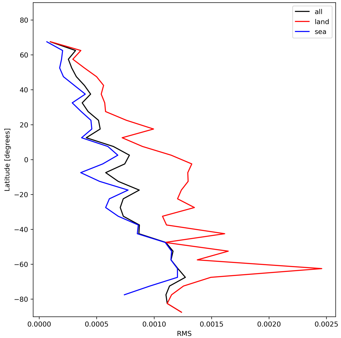
Figure 31: Zonal average of “RMS” for 2023-12-22 to 2023-12-24.
