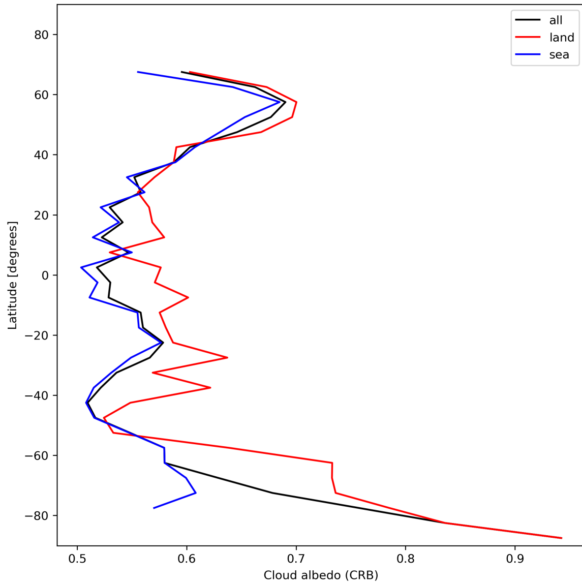
Figure 28: Zonal average of “Cloud albedo (CRB)” for 2023-12-23 to 2023-12-25.
