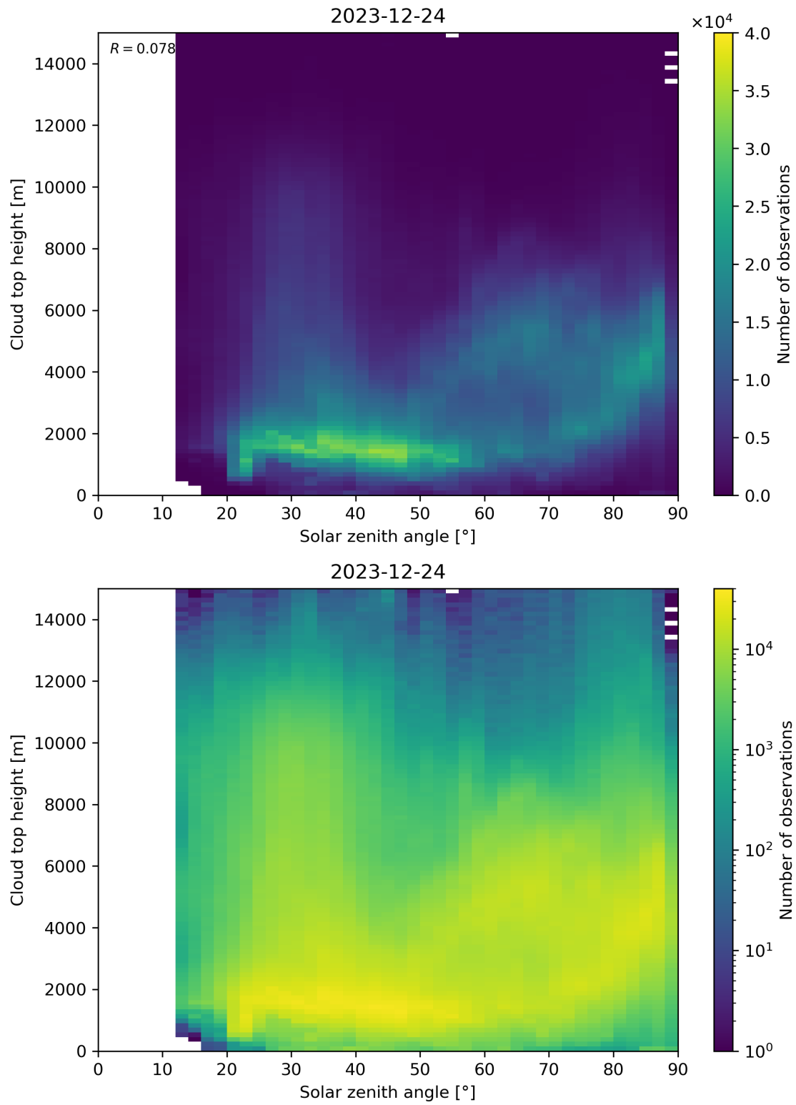
Figure 104: Scatter density plot of “Solar zenith angle” against “Cloud top height” for 2023-12-23 to 2023-12-25.
