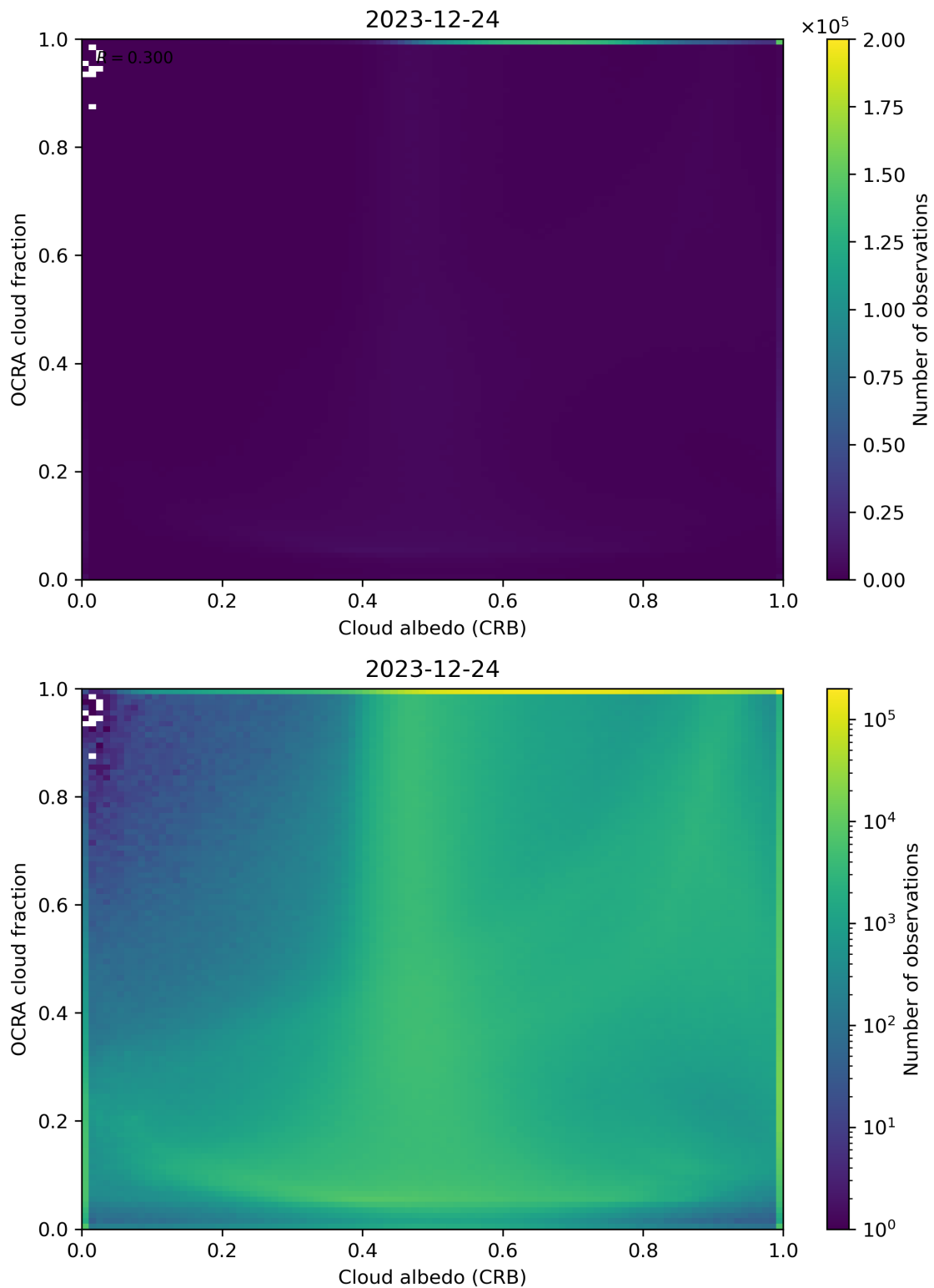
Figure 70: Scatter density plot of “Cloud albedo (CRB)” against “OCRA cloud fraction” for 2023-12-23 to 2023-12-25.
