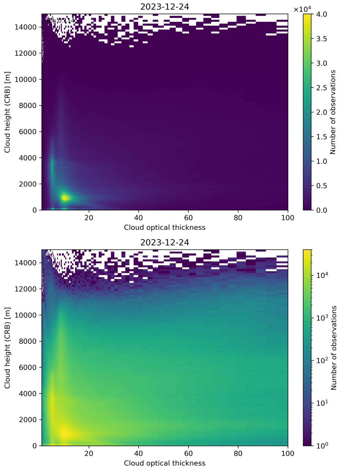
Figure 85: Scatter density plot of “Cloud optical thickness” against “Cloud height (CRB)” for 2023-12-23 to 2023-12-25.
