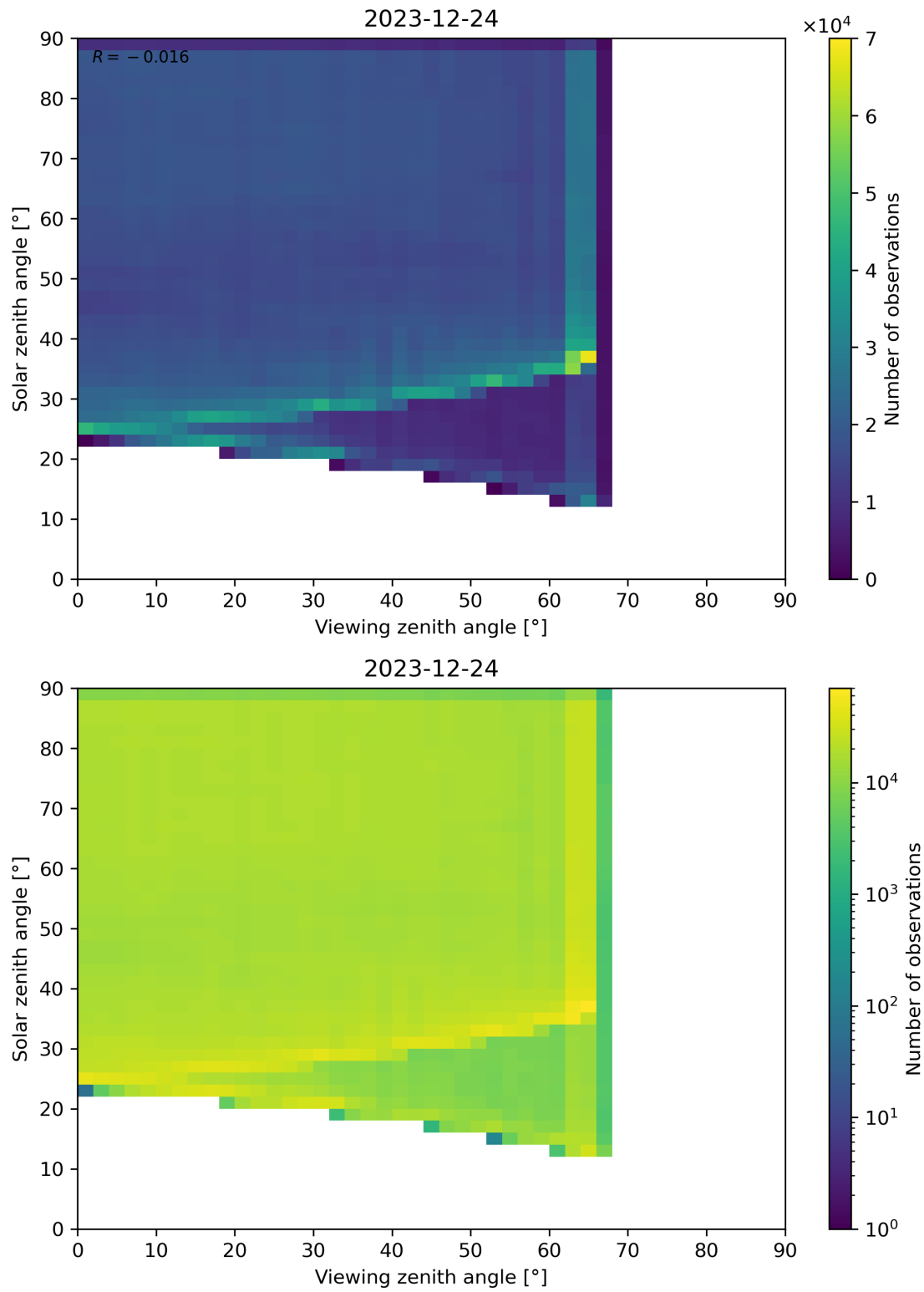
Figure 114: Scatter density plot of “Viewing zenith angle” against “Solar zenith angle” for 2023-12-23 to 2023-12-25.
