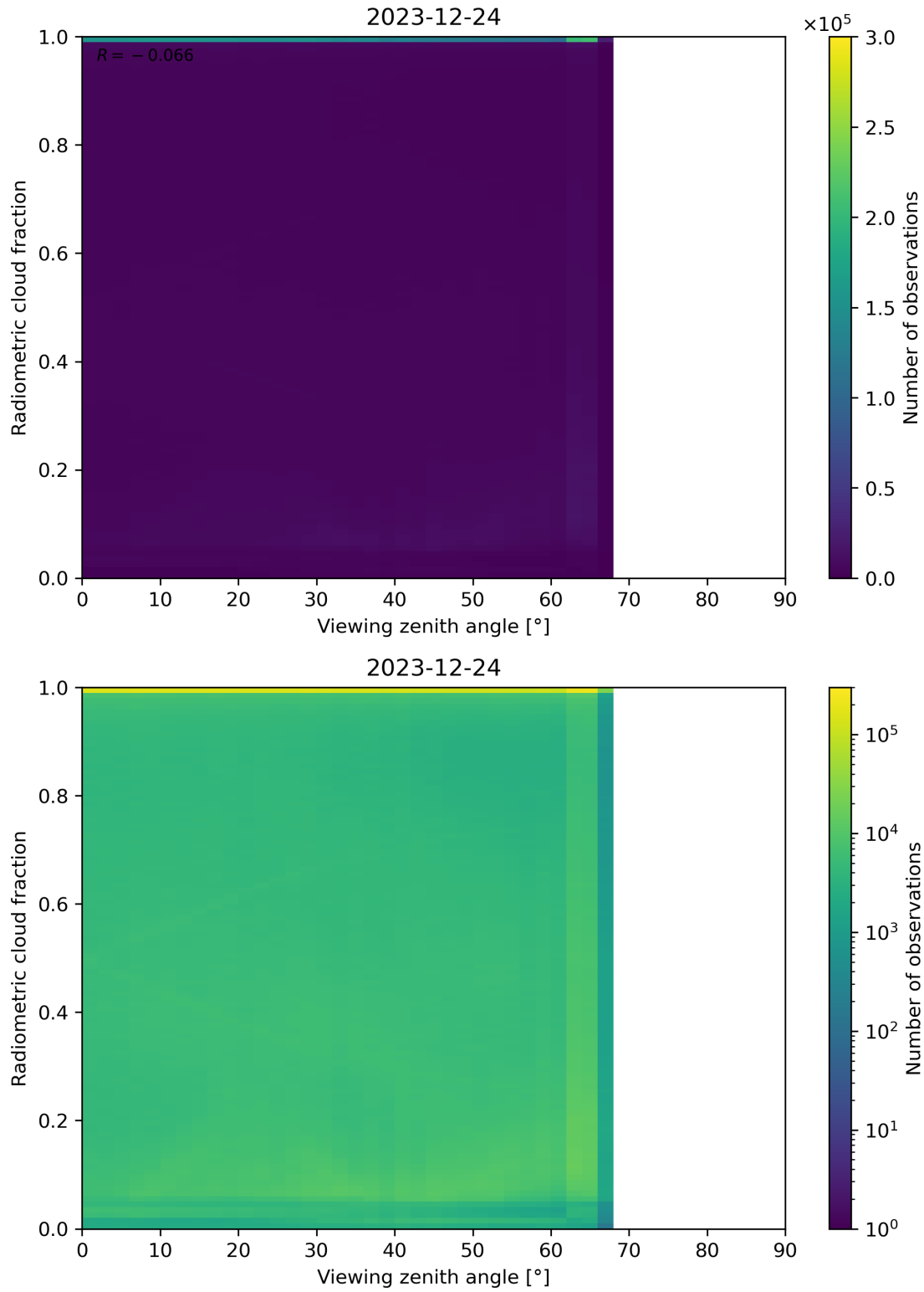
Figure 107: Scatter density plot of “Viewing zenith angle” against “Radiometric cloud fraction” for 2023-12-23 to 2023-12-25.
