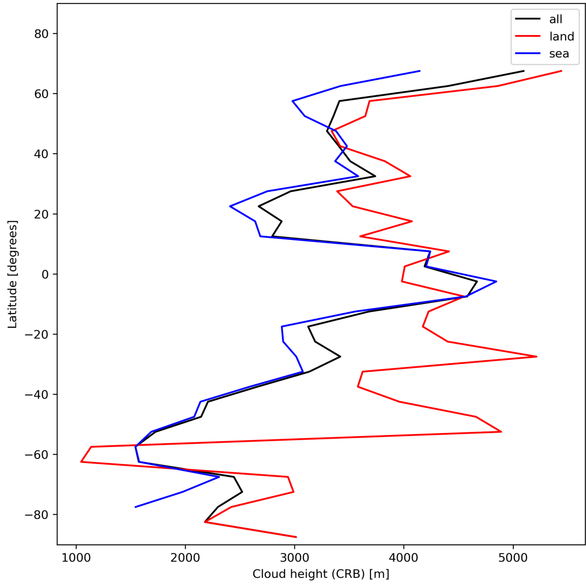
Figure 27: Zonal average of “Cloud height (CRB)” for 2023-12-23 to 2023-12-25.
