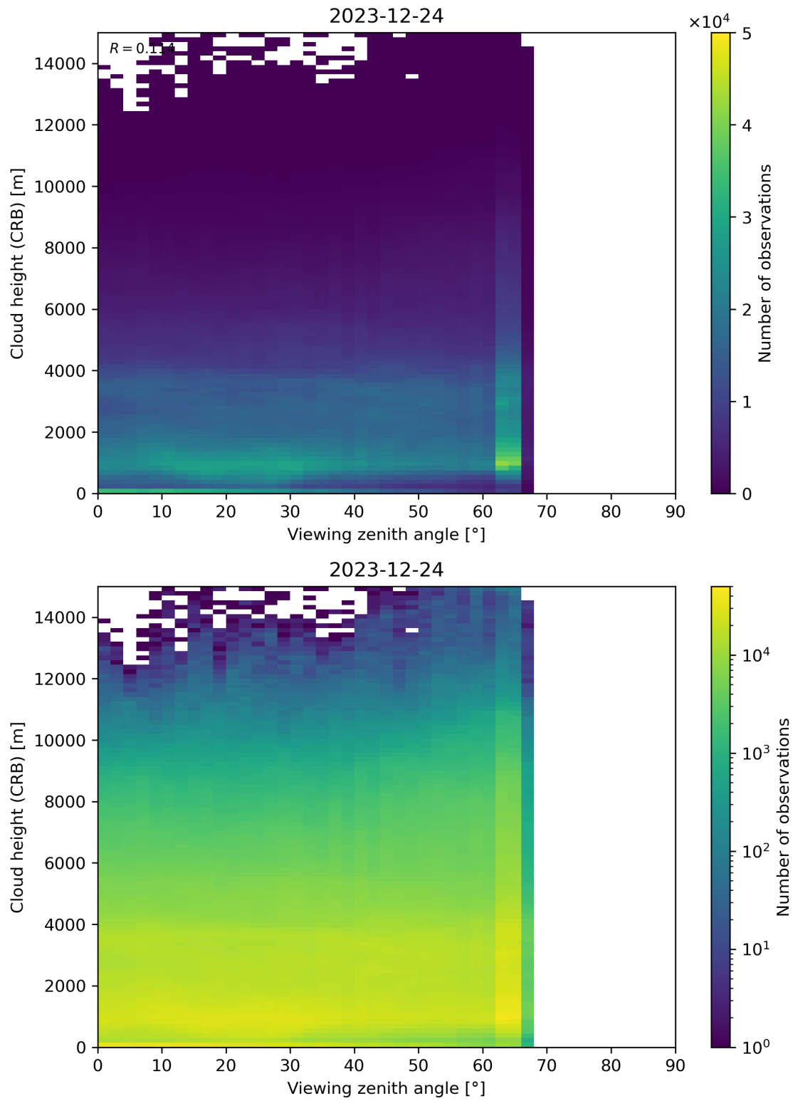
Figure 110: Scatter density plot of “Viewing zenith angle” against “Cloud height (CRB)” for 2023-12-23 to 2023-12-25.
