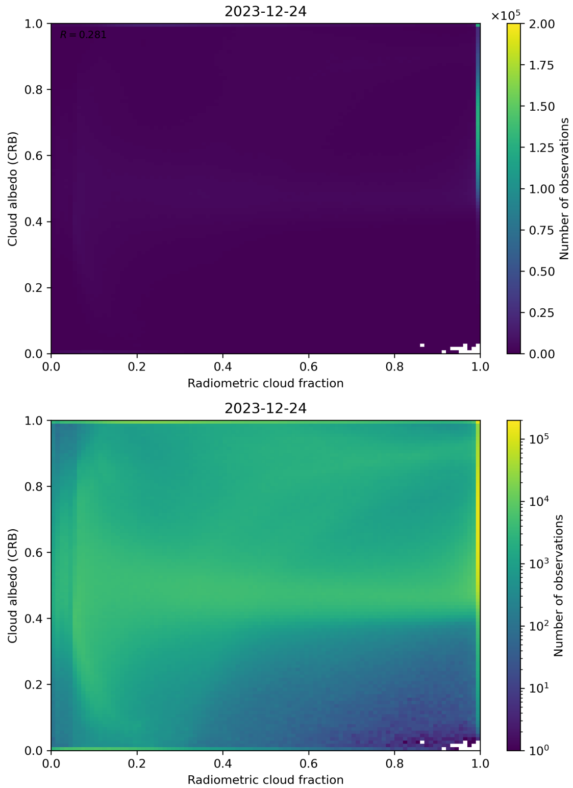
Figure 71: Scatter density plot of “Radiometric cloud fraction” against “Cloud albedo (CRB)” for 2023-12-23 to 2023-12-25.
