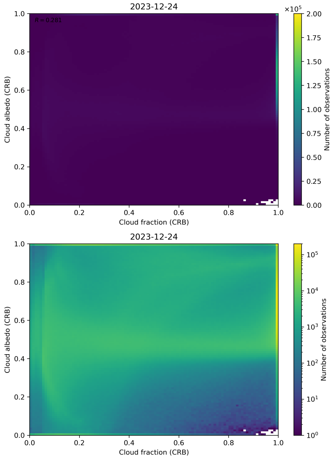
Figure 77: Scatter density plot of “Cloud fraction (CRB)” against “Cloud albedo (CRB)” for 2023-12-23 to 2023-12-25.
