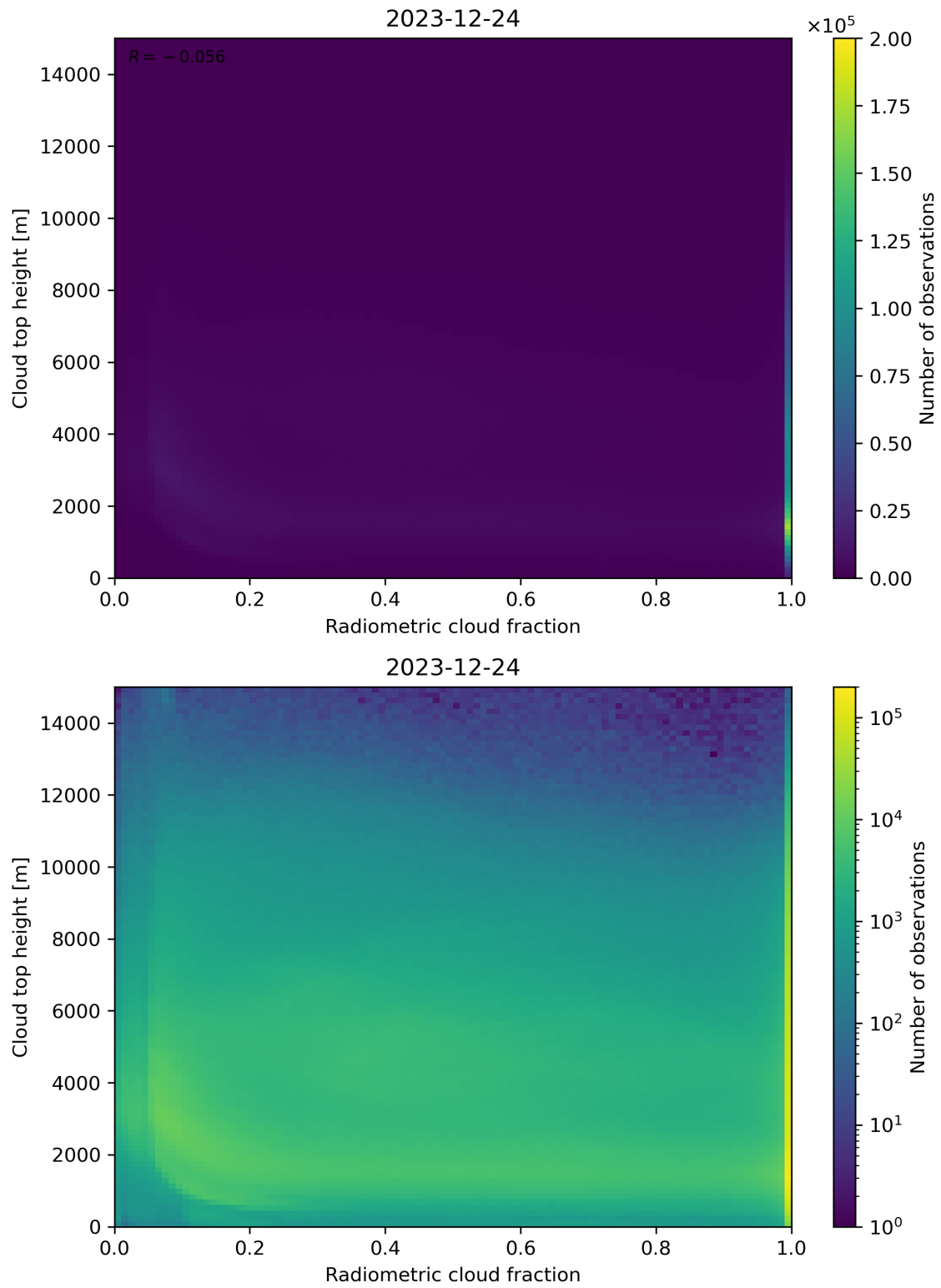
Figure 76: Scatter density plot of “Radiometric cloud fraction” against “Cloud top height” for 2023-12-23 to 2023-12-25.
