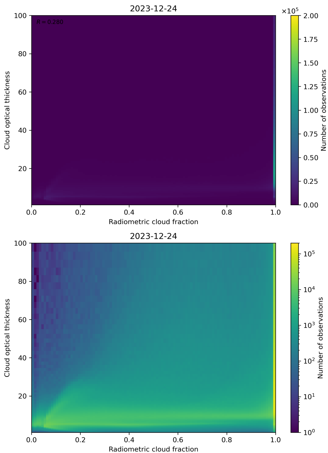
Figure 75: Scatter density plot of “Radiometric cloud fraction” against “Cloud optical thickness” for 2023-12-23 to 2023-12-25.
