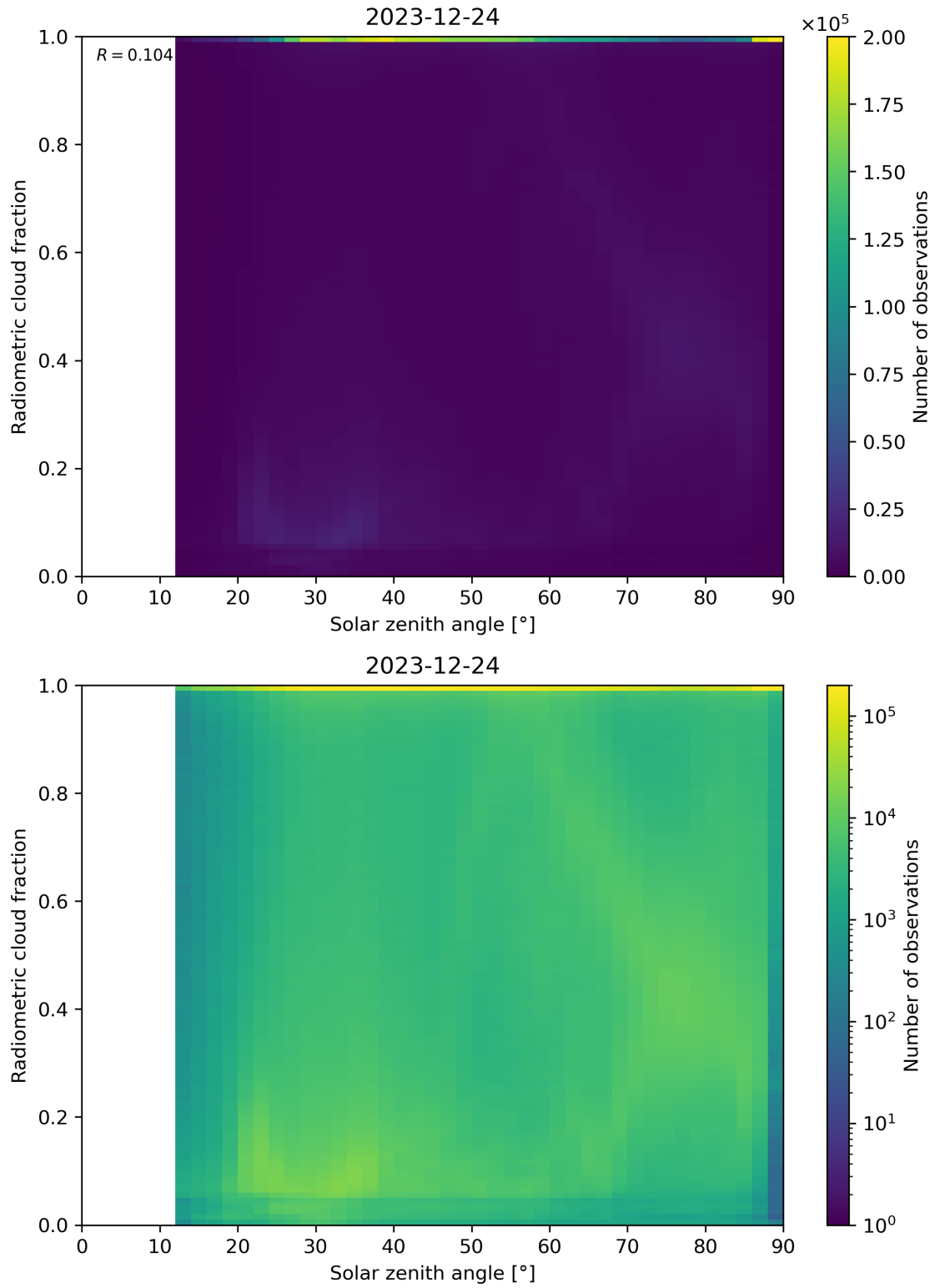
Figure 99: Scatter density plot of “Solar zenith angle” against “Radiometric cloud fraction” for 2023-12-23 to 2023-12-25.
