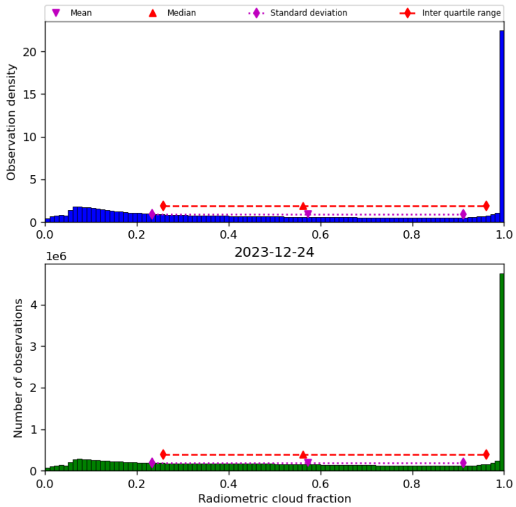
Figure 39: Histogram of “Radiometric cloud fraction” for 2023-12-23 to 2023-12-25
