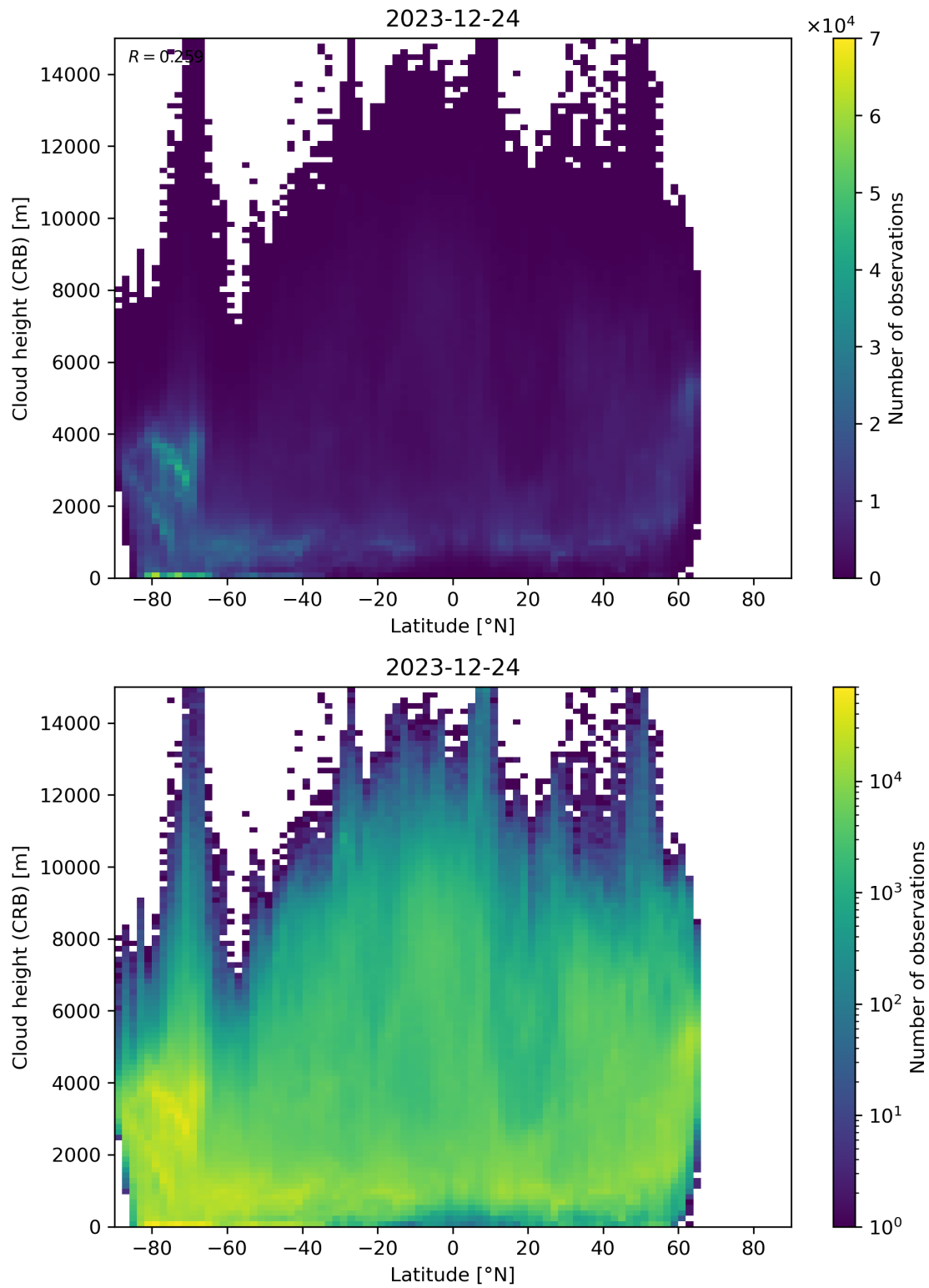
Figure 95: Scatter density plot of “Latitude” against “Cloud height (CRB)” for 2023-12-23 to 2023-12-25.
