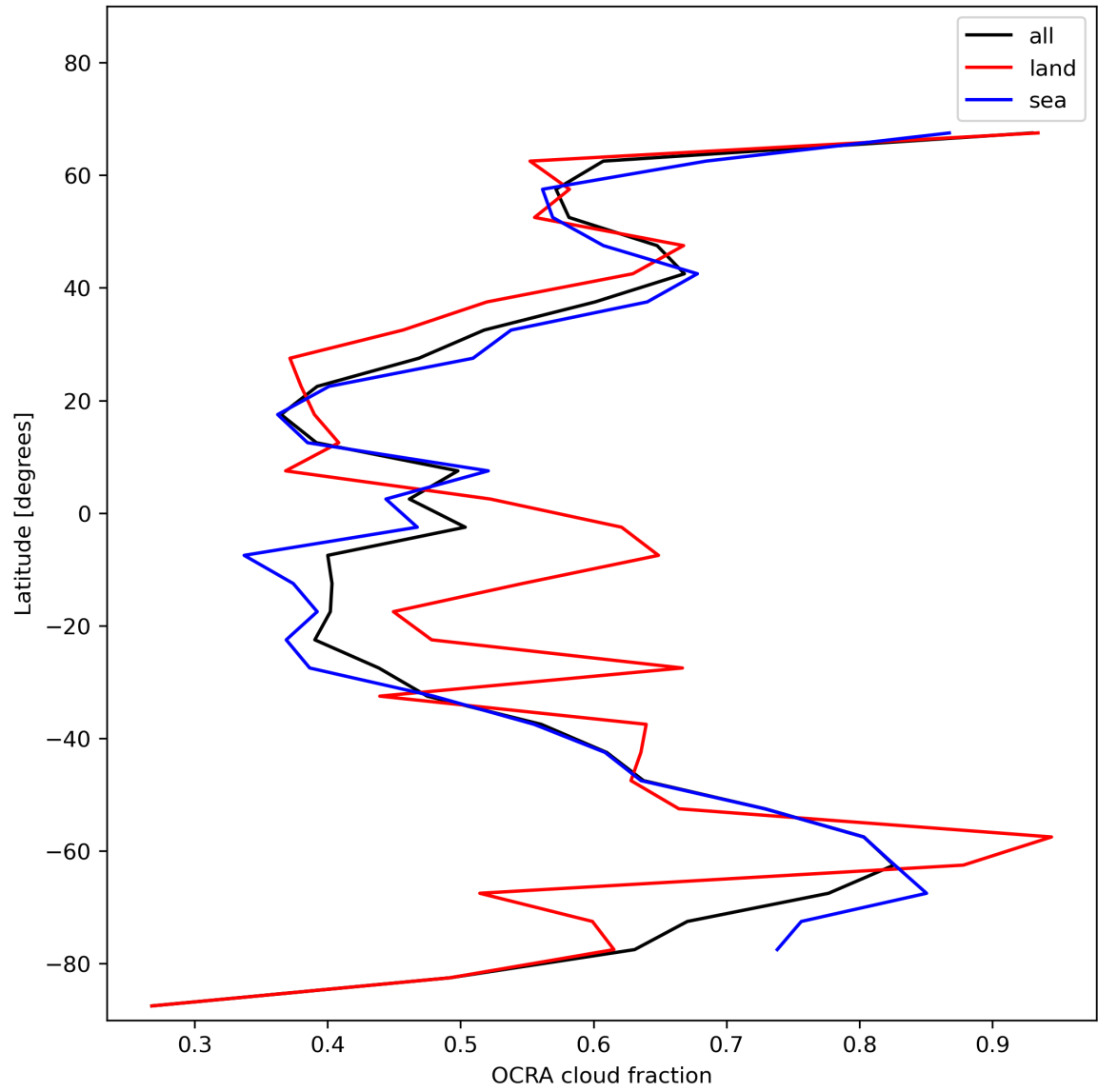
Figure 34: Zonal average of “OCRA cloud fraction” for 2023-12-23 to 2023-12-25.
