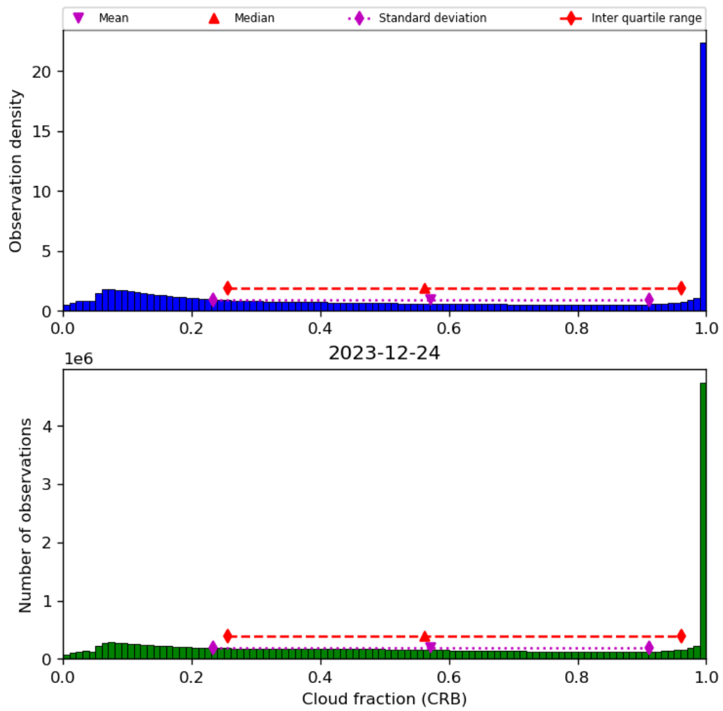
Figure 42: Histogram of “Cloud fraction (CRB)” for 2023-12-23 to 2023-12-25
