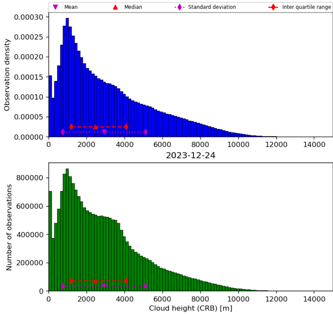
Figure 43: Histogram of “Cloud height (CRB)” for 2023-12-23 to 2023-12-25
