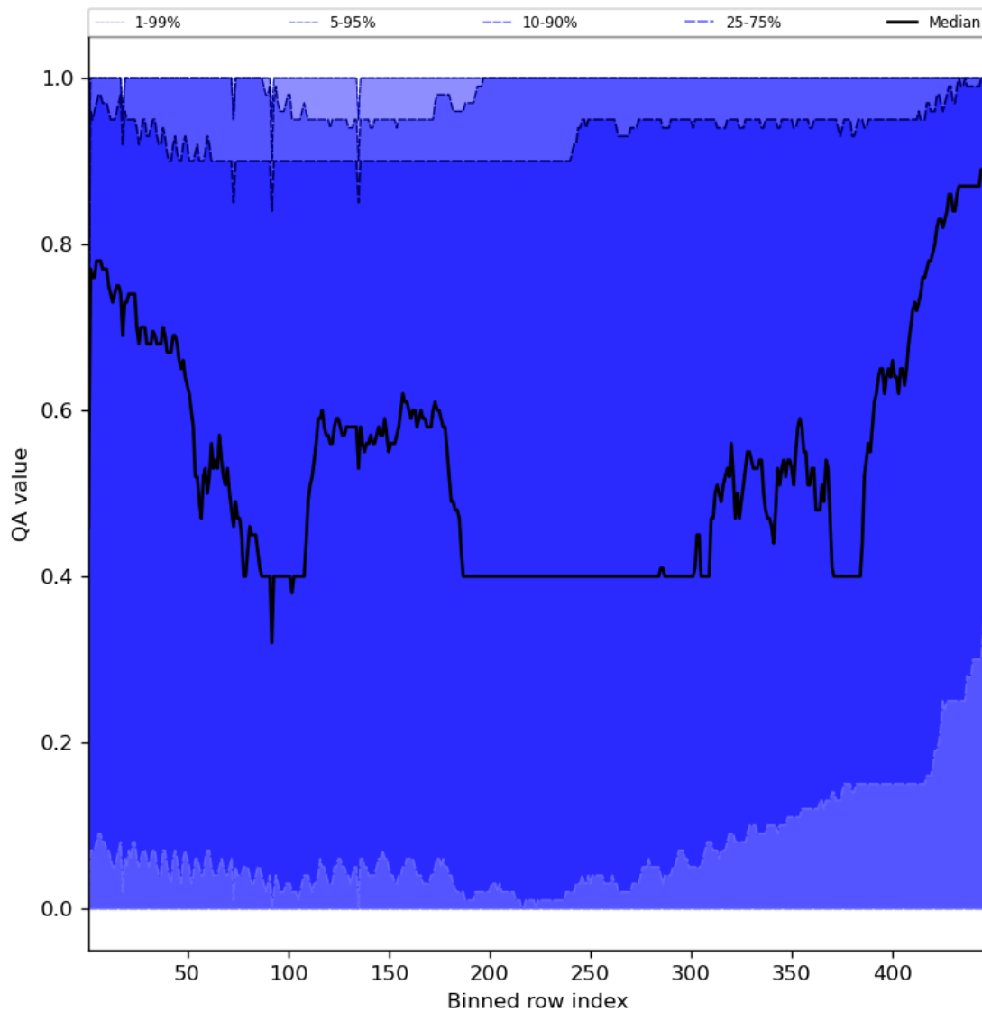
Figure 54: Along track statistics of “QA value” for 2023-12-23 to 2023-12-25
