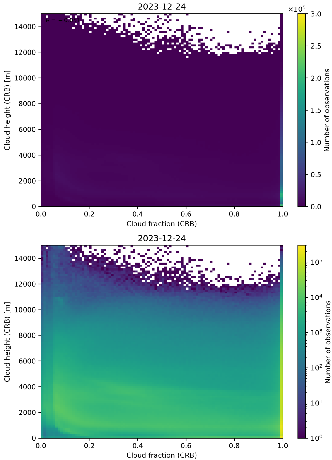
Figure 79: Scatter density plot of “Cloud fraction (CRB)” against “Cloud height (CRB)” for 2023-12-23 to 2023-12-25.
