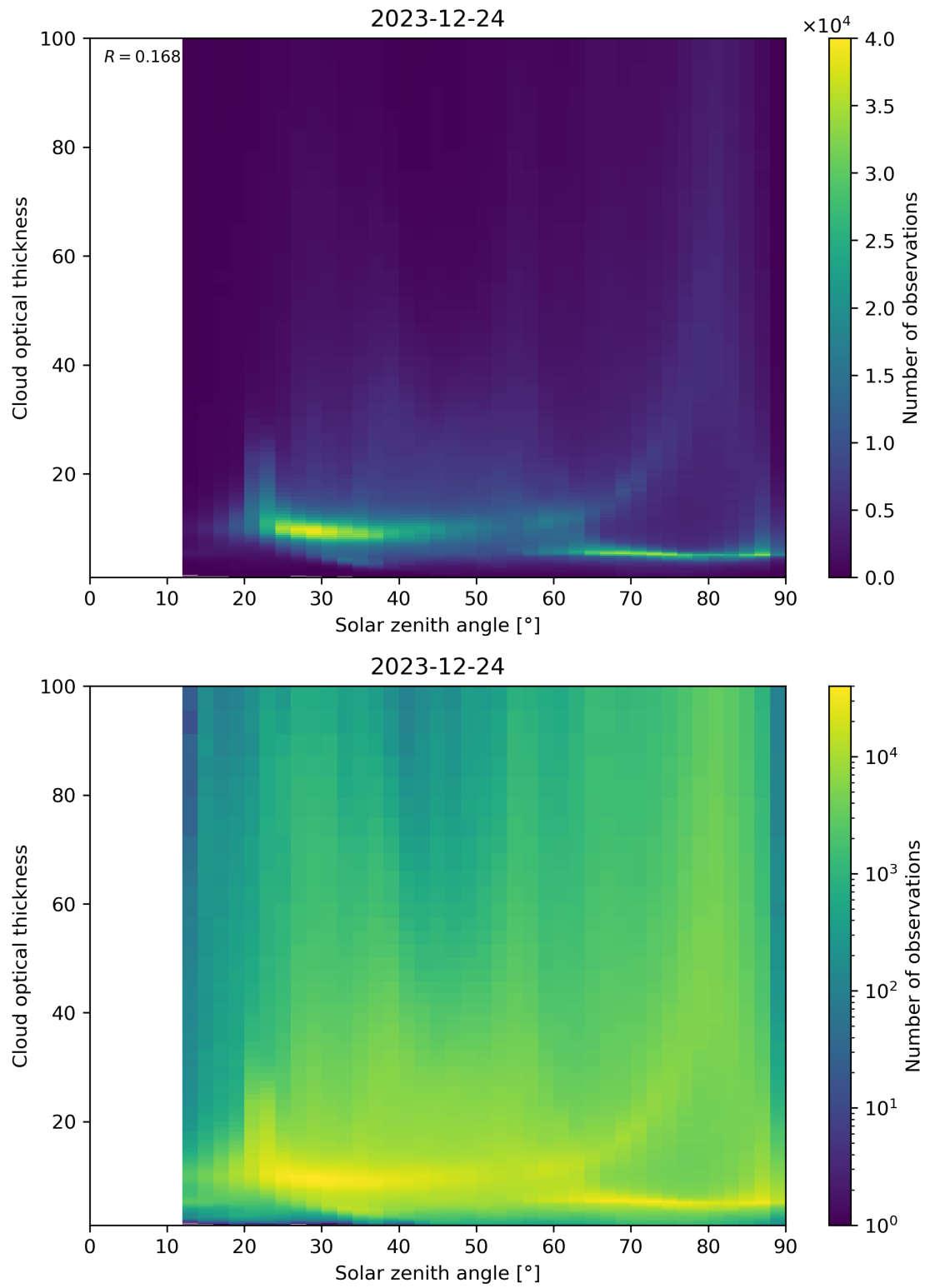
Figure 103: Scatter density plot of “Solar zenith angle” against “Cloud optical thickness” for 2023-12-23 to 2023-12-25.
