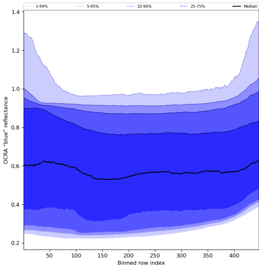
Figure 67: Along track statistics of “OCRA “blue” reflectance” for 2023-12-23 to 2023-12-25
