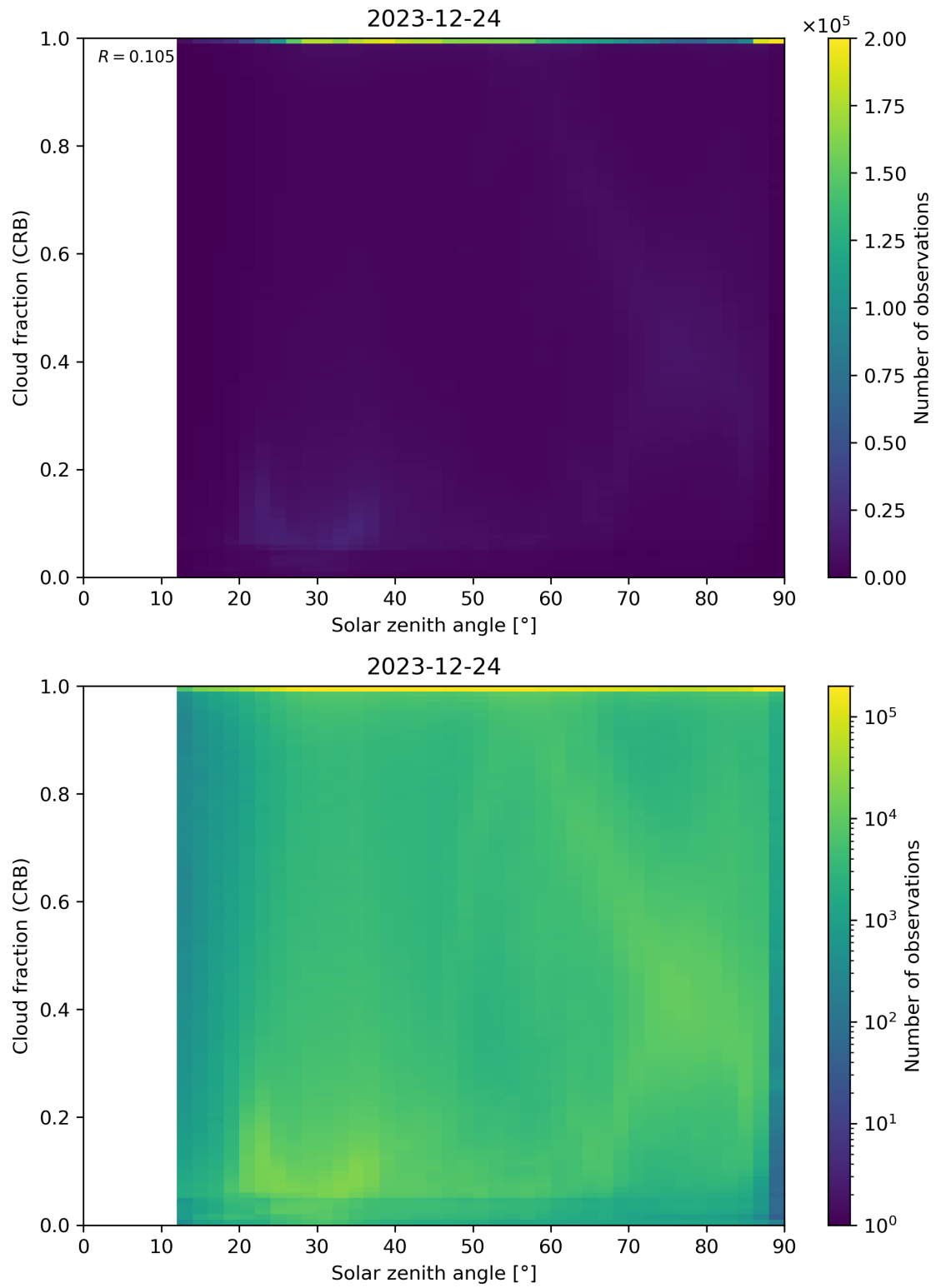
Figure 101: Scatter density plot of “Solar zenith angle” against “Cloud fraction (CRB)” for 2023-12-23 to 2023-12-25.
