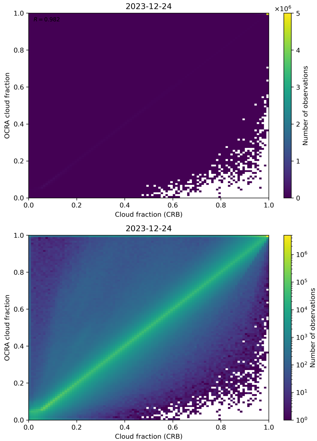
Figure 78: Scatter density plot of “Cloud fraction (CRB)” against “OCRA cloud fraction” for 2023-12-23 to 2023-12-25.
