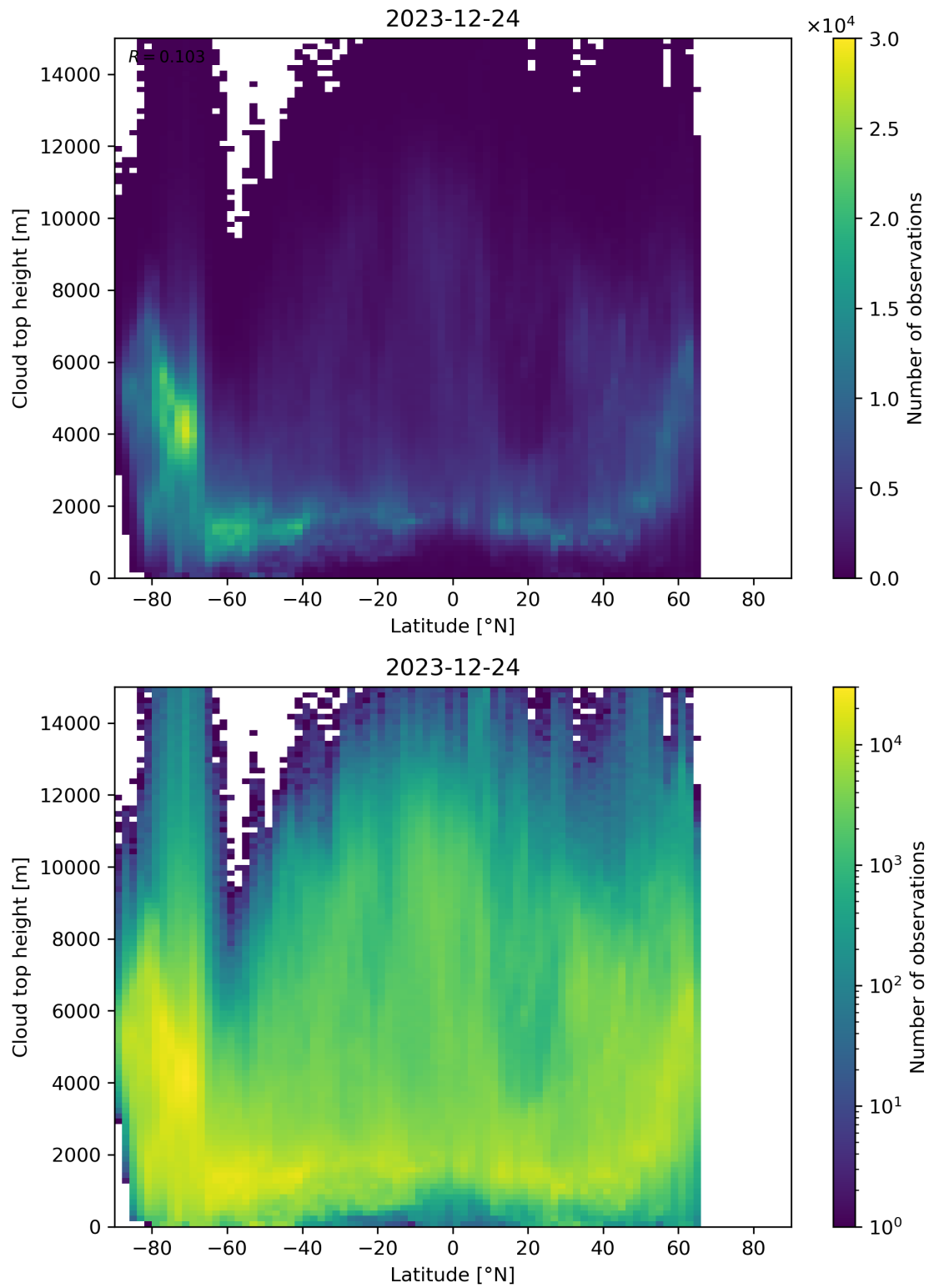
Figure 97: Scatter density plot of “Latitude” against “Cloud top height” for 2023-12-23 to 2023-12-25.
