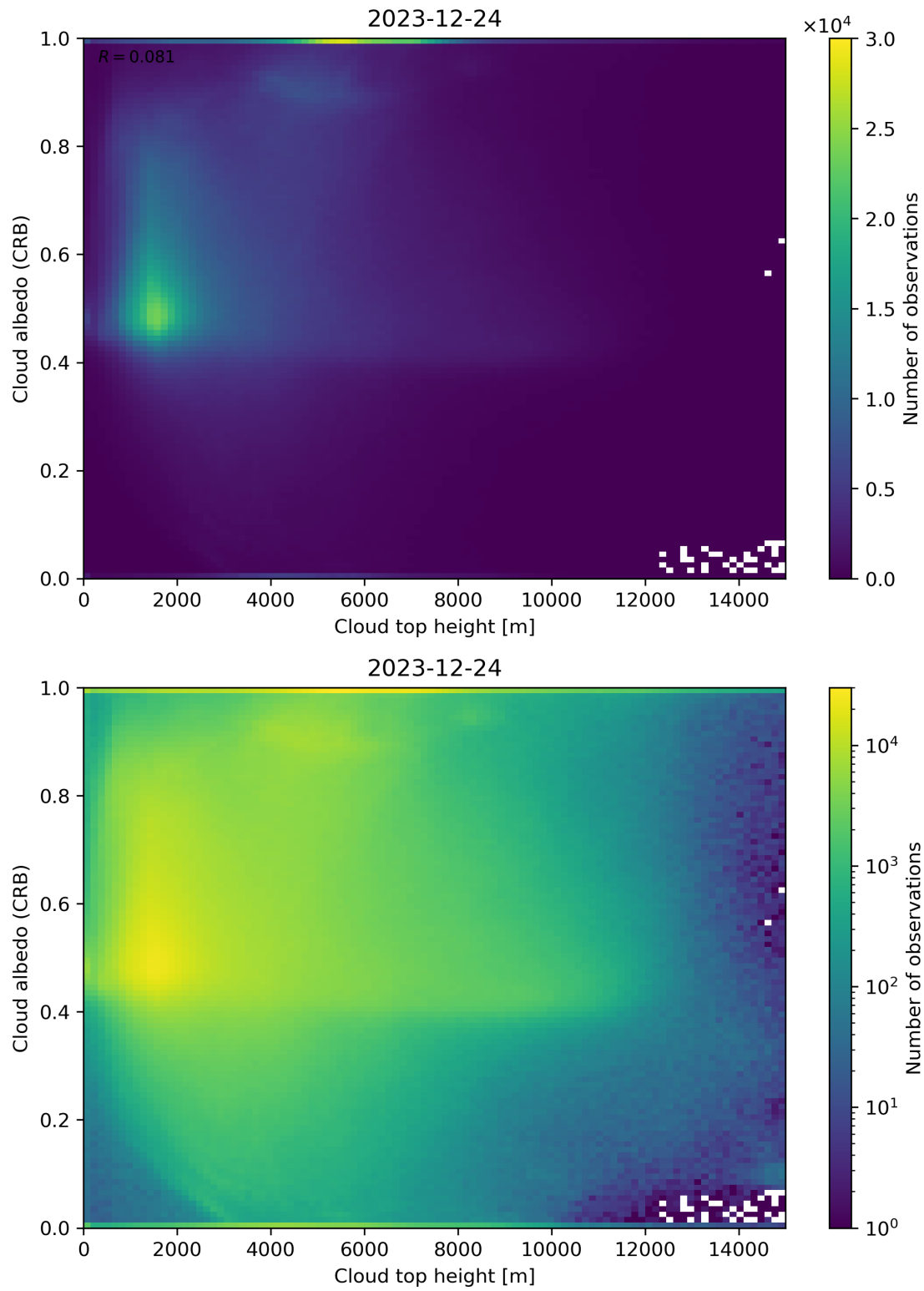
Figure 86: Scatter density plot of “Cloud top height” against “Cloud albedo (CRB)” for 2023-12-23 to 2023-12-25.
