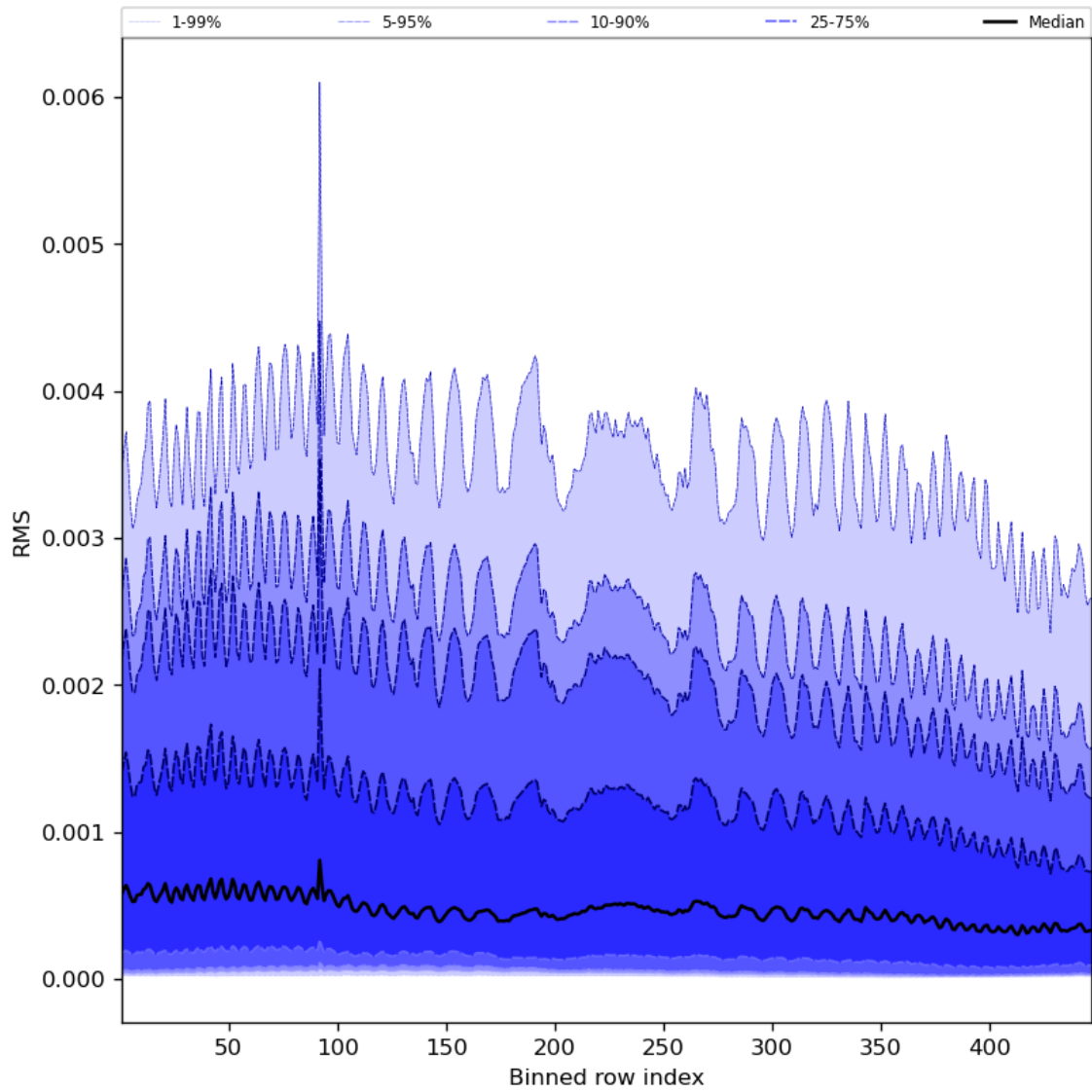
Figure 63: Along track statistics of “RMS” for 2023-12-23 to 2023-12-25
