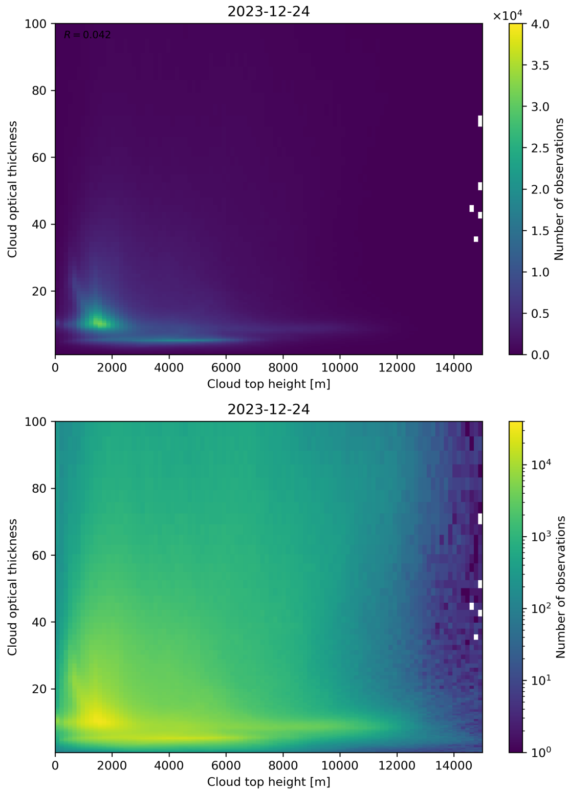
Figure 90: Scatter density plot of “Cloud top height” against “Cloud optical thickness” for 2023-12-23 to 2023-12-25.
