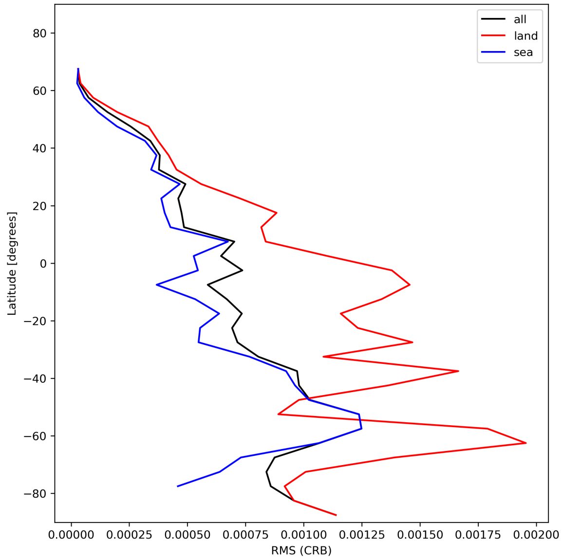
Figure 32: Zonal average of “RMS (CRB)” for 2023-12-23 to 2023-12-25.
