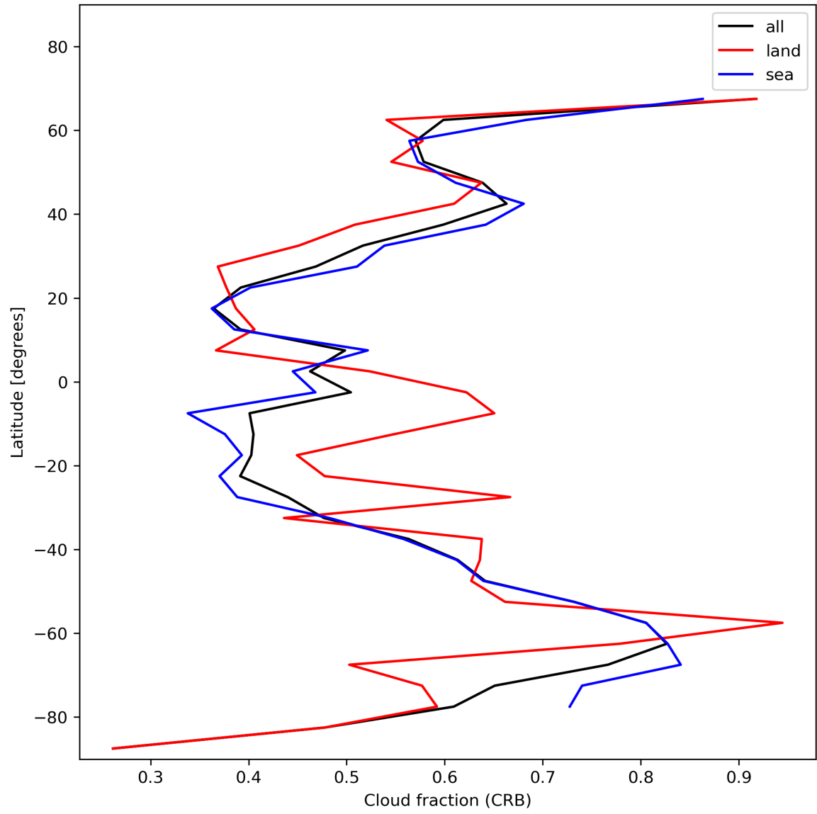
Figure 26: Zonal average of “Cloud fraction (CRB)” for 2023-12-23 to 2023-12-25.
