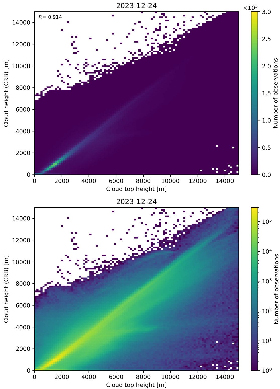
Figure 89: Scatter density plot of “Cloud top height” against “Cloud height (CRB)” for 2023-12-23 to 2023-12-25.
