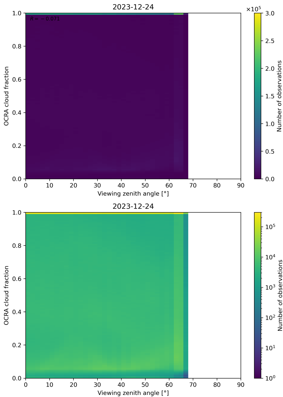
Figure 108: Scatter density plot of “Viewing zenith angle” against “OCRA cloud fraction” for 2023-12-23 to 2023-12-25.
