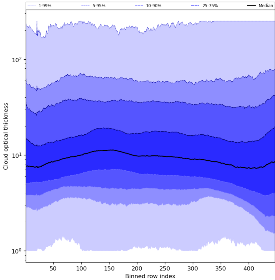
Figure 57: Along track statistics of “Cloud optical thickness” for 2023-12-23 to 2023-12-25
