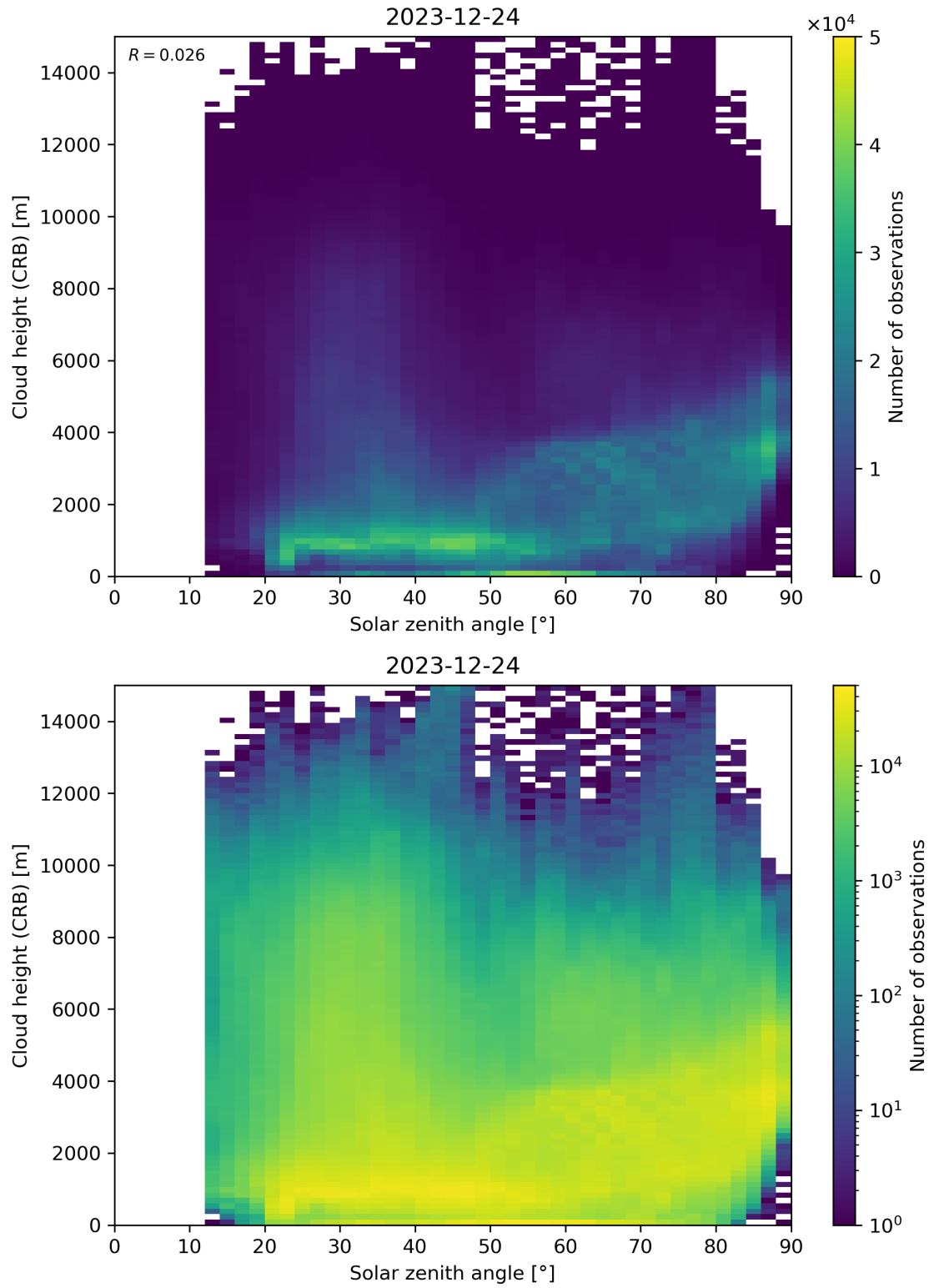
Figure 102: Scatter density plot of “Solar zenith angle” against “Cloud height (CRB)” for 2023-12-23 to 2023-12-25.
