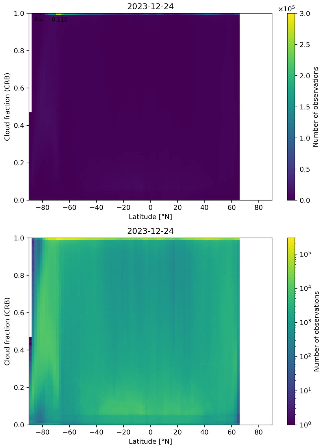
Figure 94: Scatter density plot of “Latitude” against “Cloud fraction (CRB)” for 2023-12-23 to 2023-12-25.
