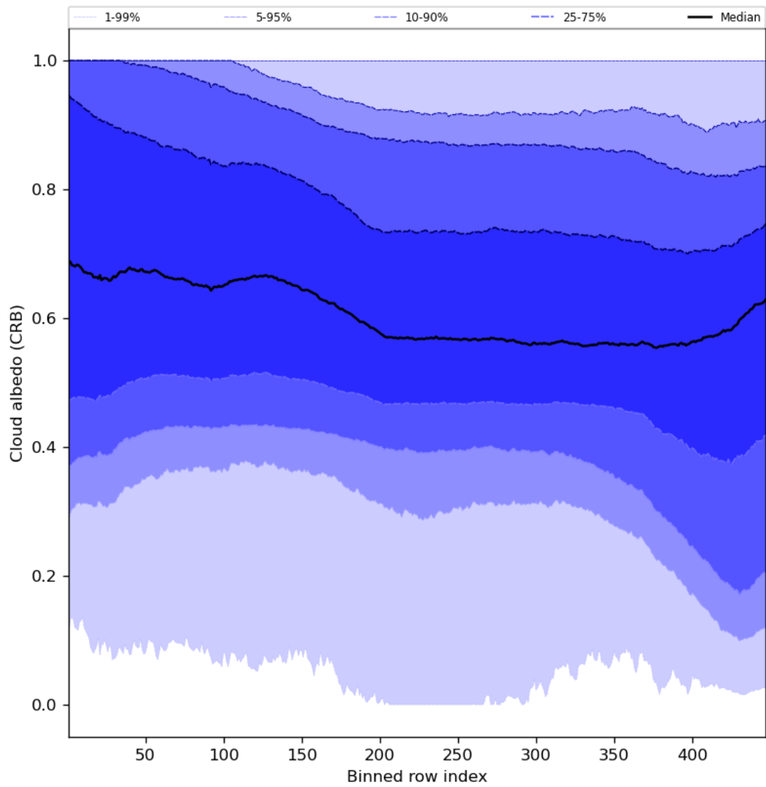
Figure 60: Along track statistics of “Cloud albedo (CRB)” for 2023-12-23 to 2023-12-25
