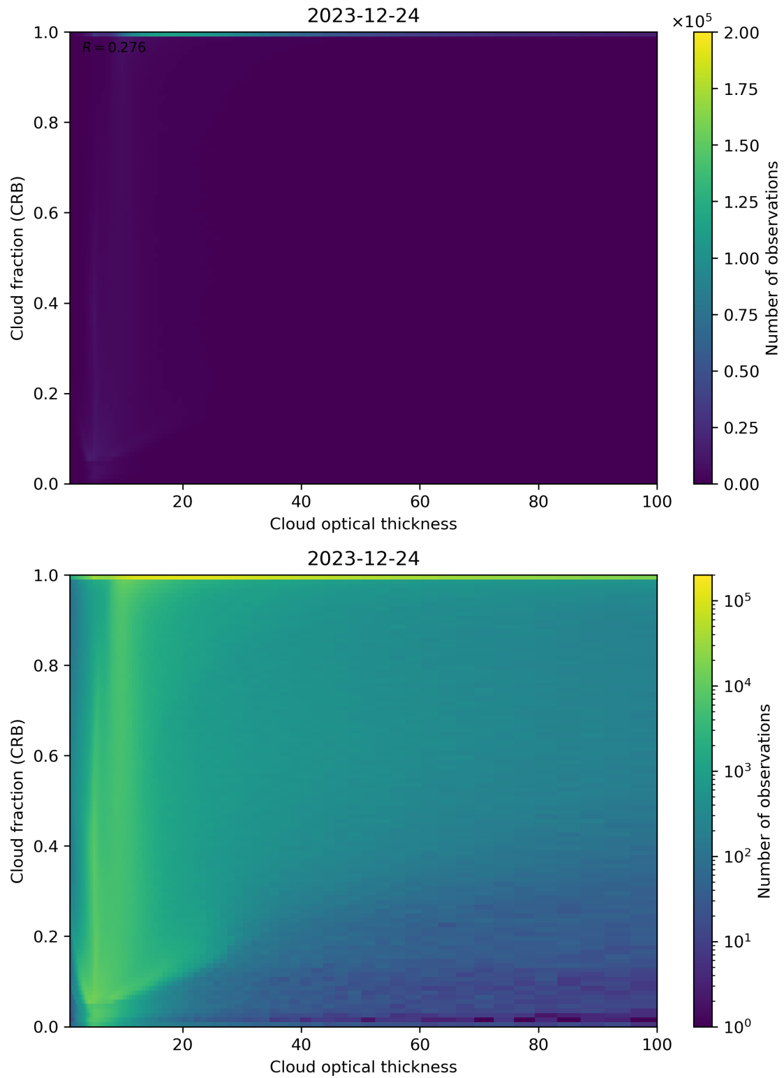
Figure 84: Scatter density plot of “Cloud optical thickness” against “Cloud fraction (CRB)” for 2023-12-23 to 2023-12-25.
