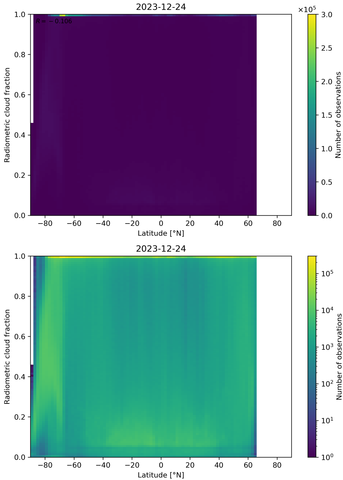
Figure 92: Scatter density plot of “Latitude” against “Radiometric cloud fraction” for 2023-12-23 to 2023-12-25.
