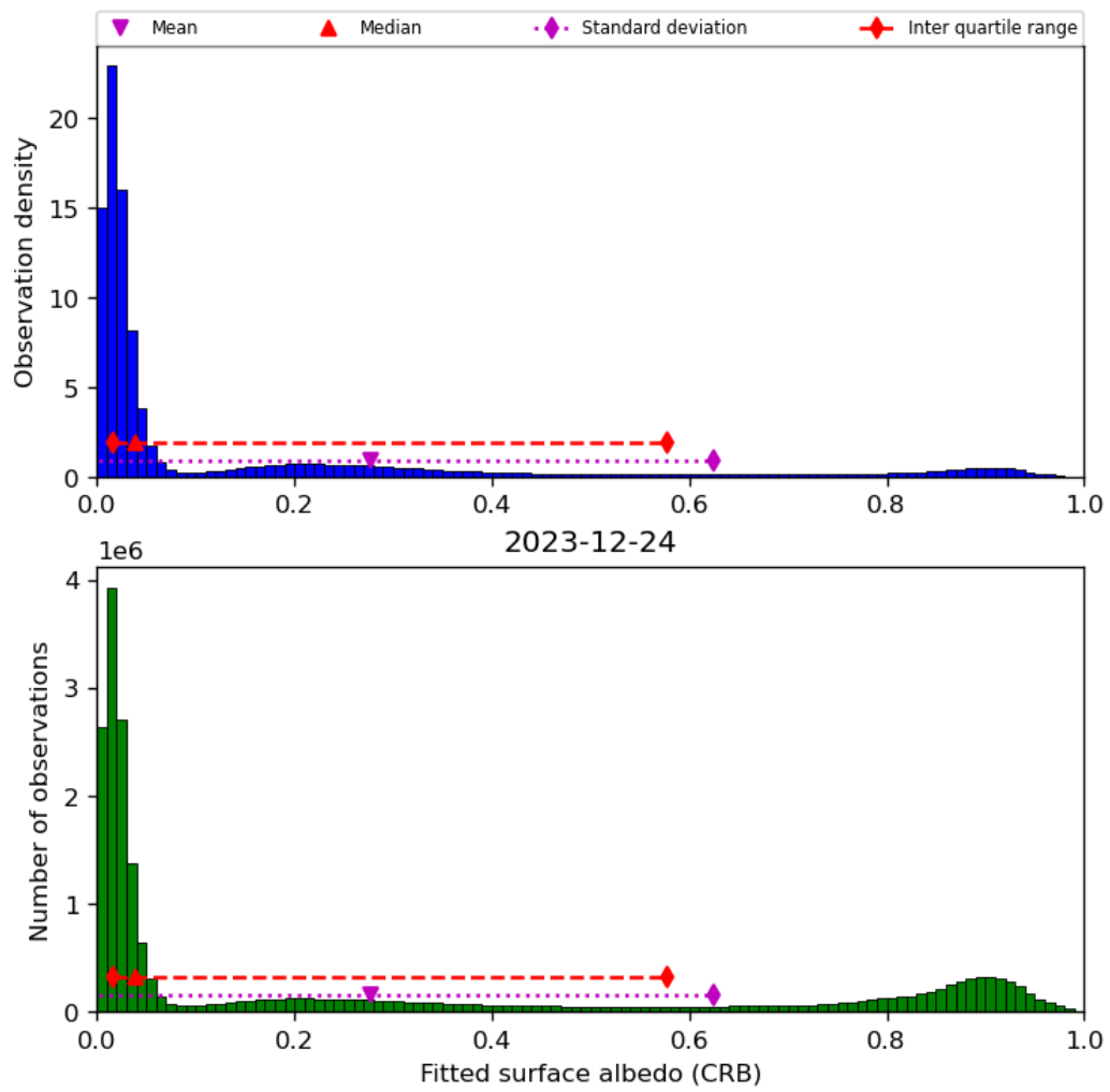
Figure 46: Histogram of “Fitted surface albedo (CRB)” for 2023-12-23 to 2023-12-25
