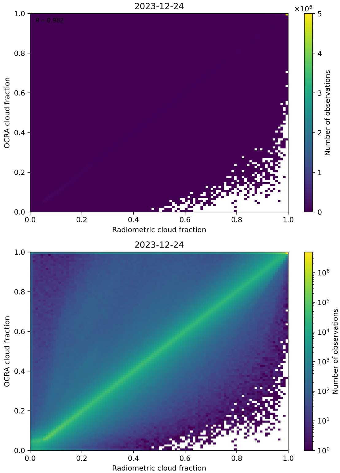
Figure 72: Scatter density plot of “Radiometric cloud fraction” against “OCRA cloud fraction” for 2023-12-23 to 2023-12-25.
