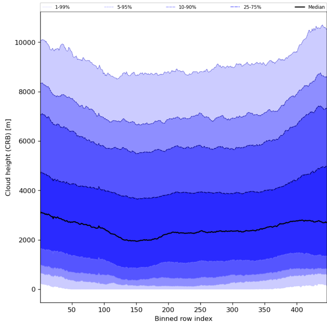
Figure 59: Along track statistics of “Cloud height (CRB)” for 2023-12-23 to 2023-12-25
