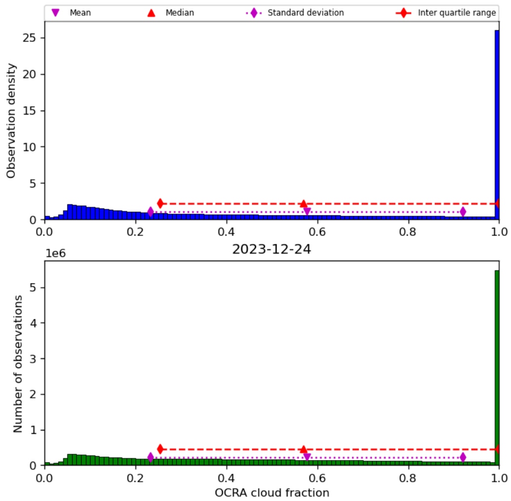
Figure 50: Histogram of “OCRA cloud fraction” for 2023-12-23 to 2023-12-25
