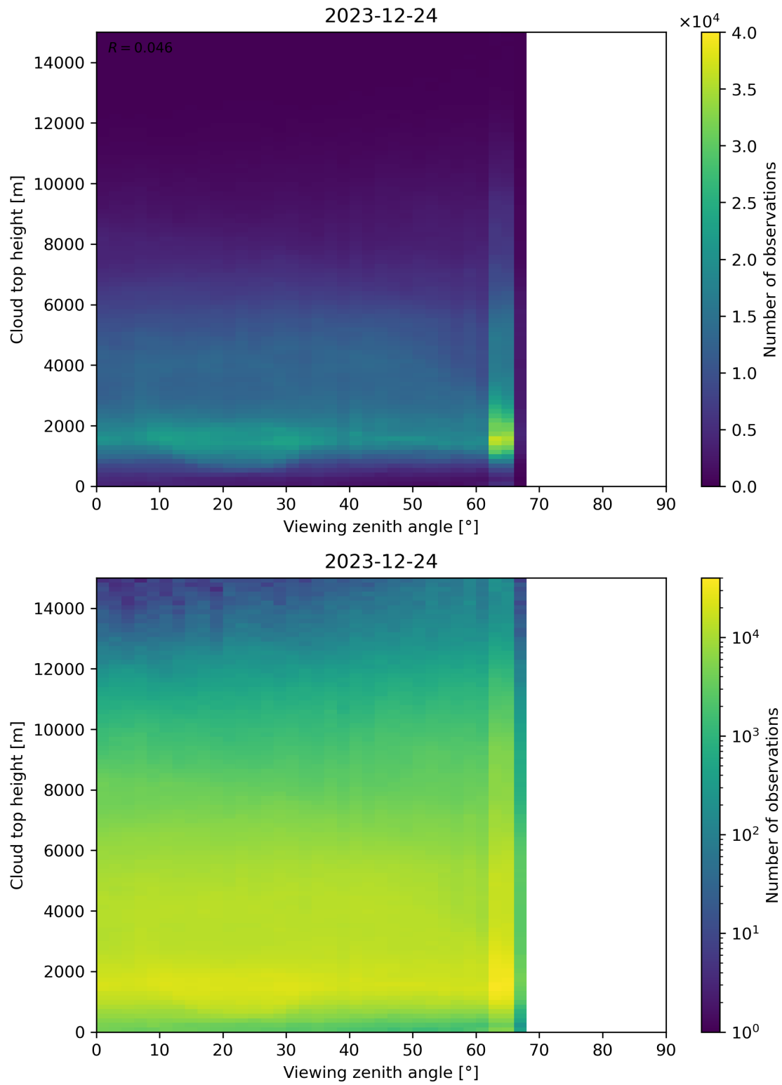
Figure 112: Scatter density plot of “Viewing zenith angle” against “Cloud top height” for 2023-12-23 to 2023-12-25.
