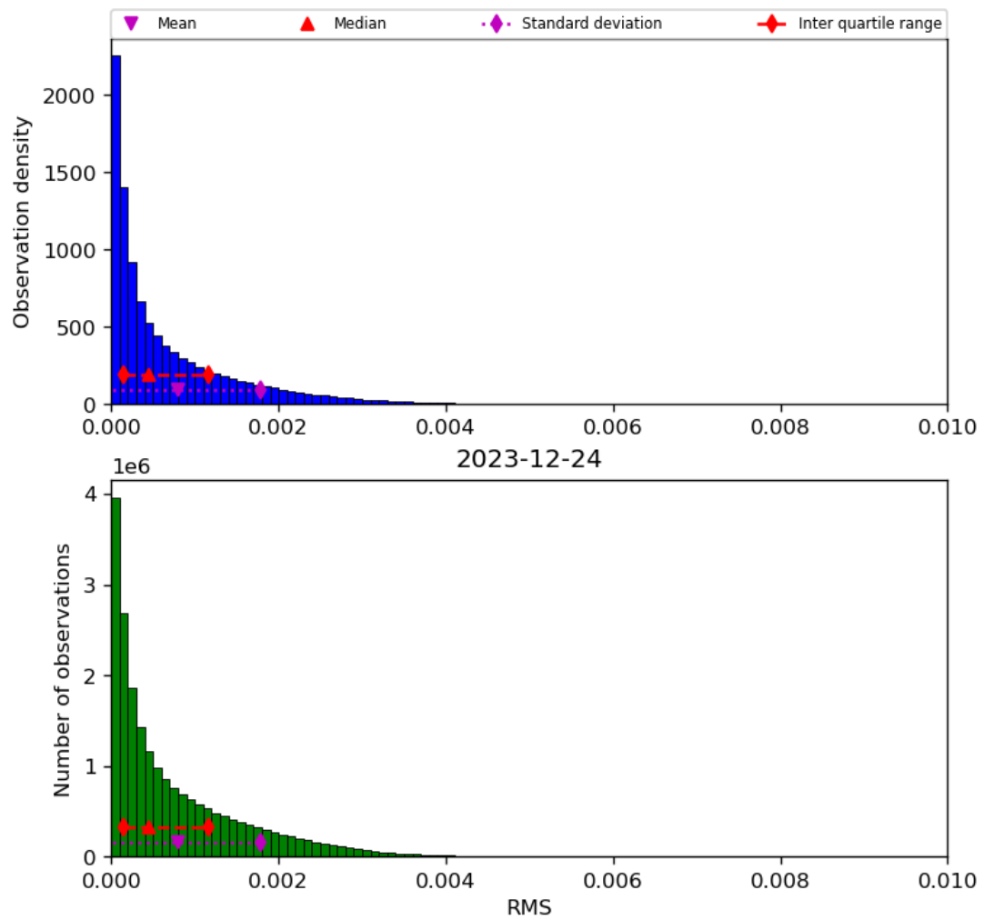
Figure 47: Histogram of “RMS” for 2023-12-23 to 2023-12-25
