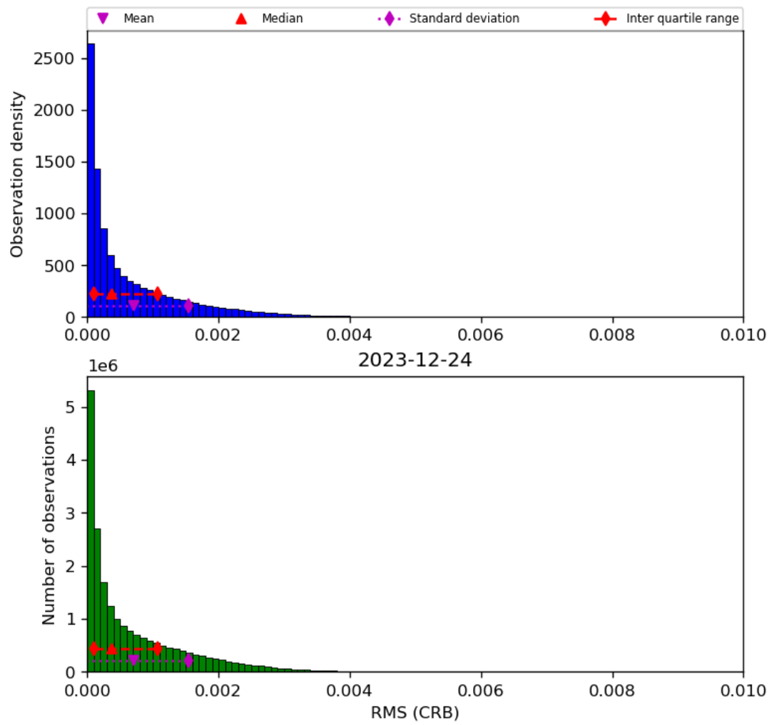
Figure 48: Histogram of “RMS (CRB)” for 2023-12-23 to 2023-12-25
