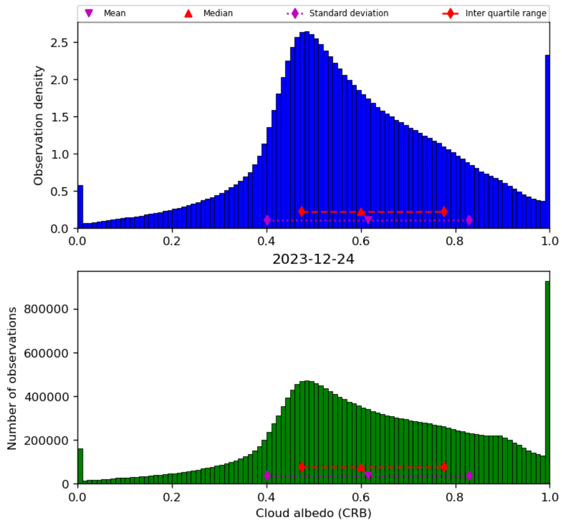
Figure 44: Histogram of “Cloud albedo (CRB)” for 2023-12-23 to 2023-12-25
