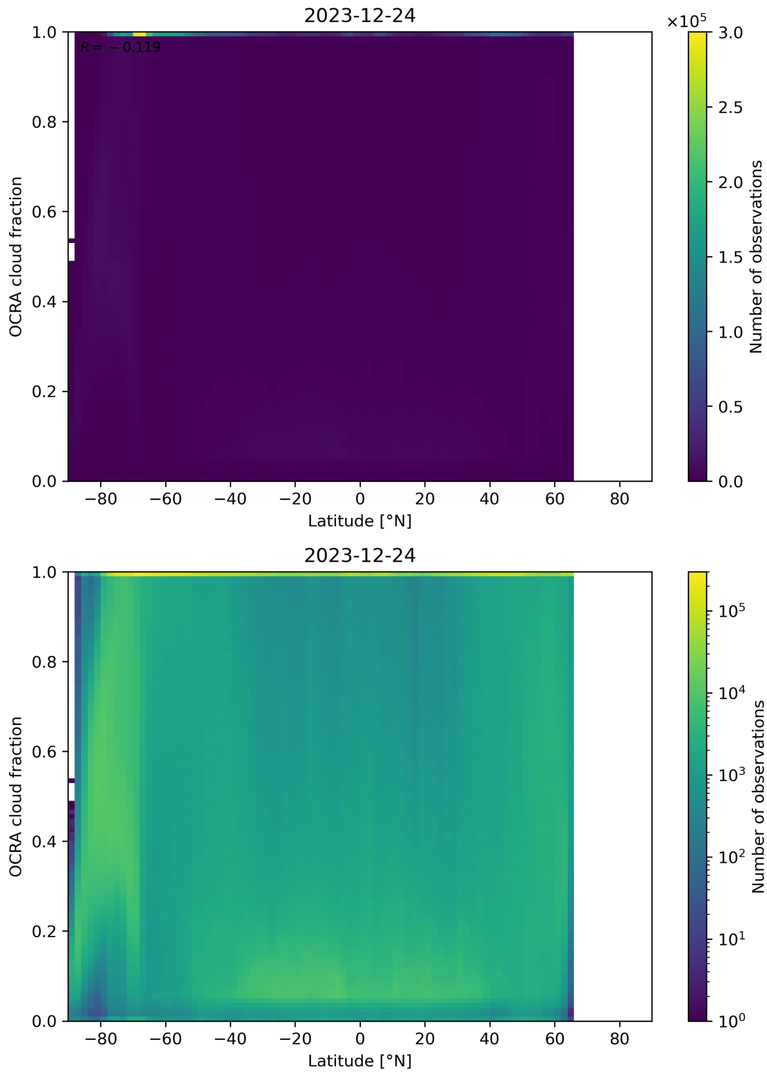
Figure 93: Scatter density plot of “Latitude” against “OCRA cloud fraction” for 2023-12-23 to 2023-12-25.
