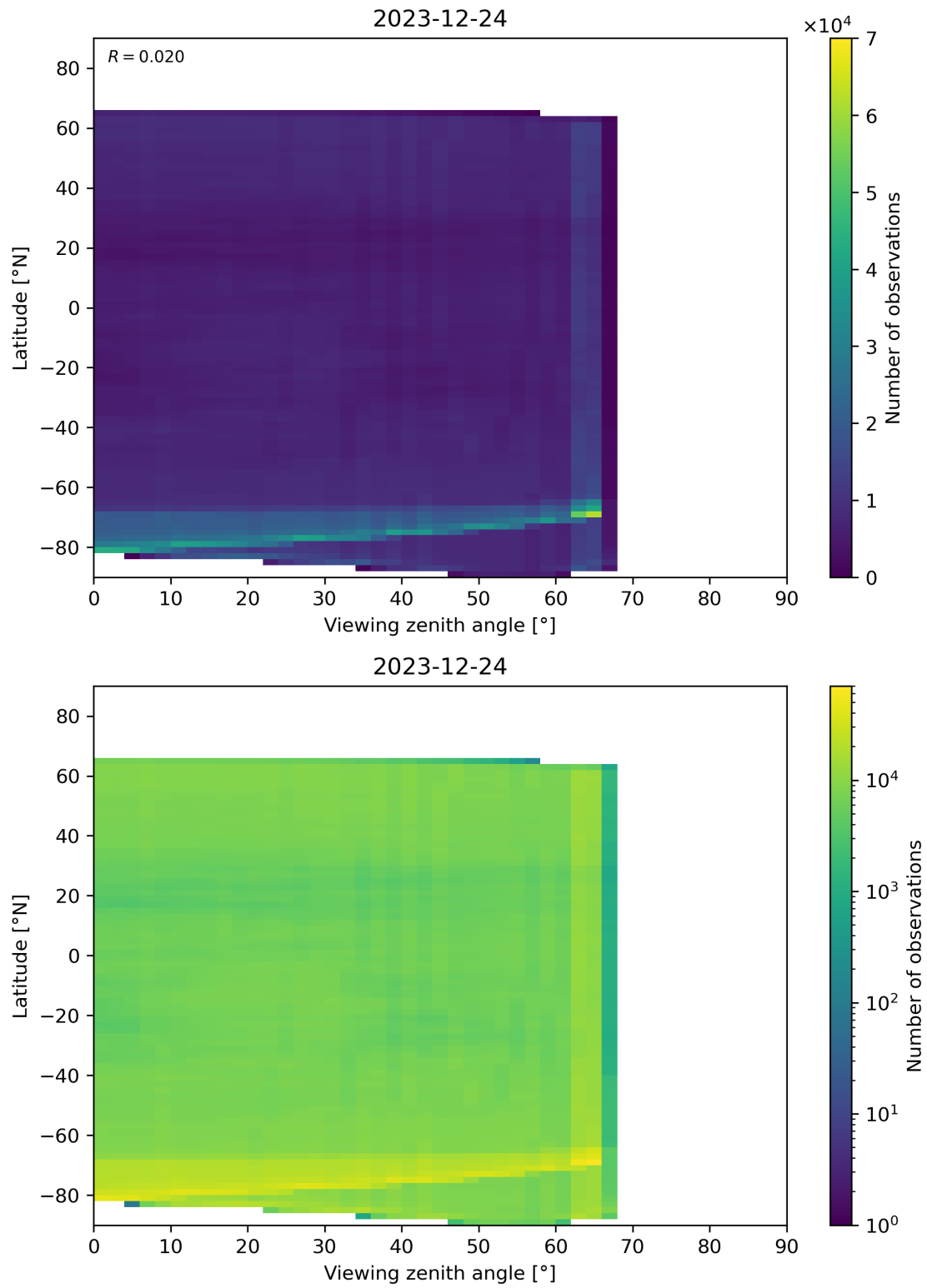
Figure 113: Scatter density plot of “Viewing zenith angle” against “Latitude” for 2023-12-23 to 2023-12-25.
