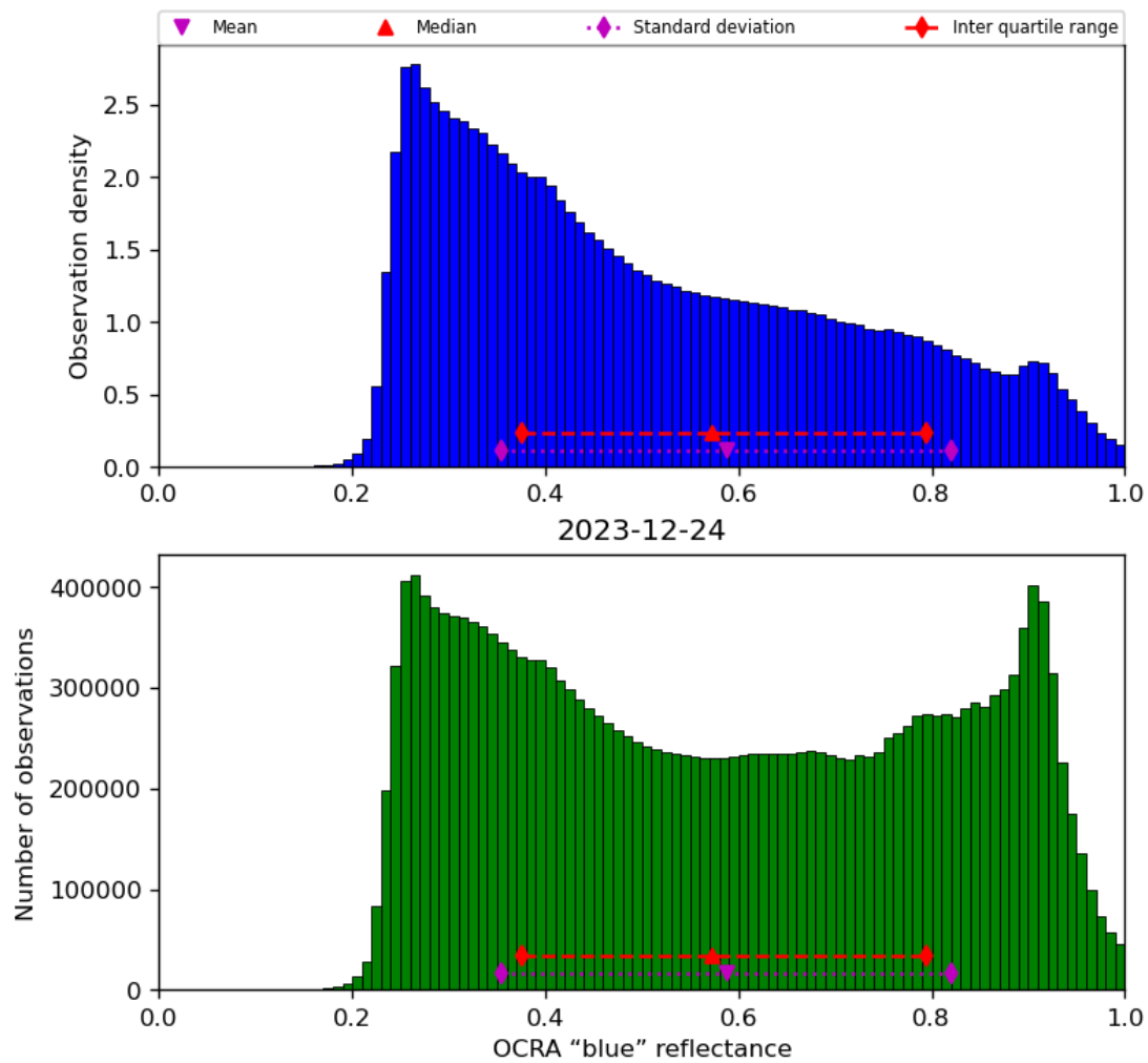
Figure 51: Histogram of “OCRA “blue” reflectance” for 2023-12-23 to 2023-12-25
