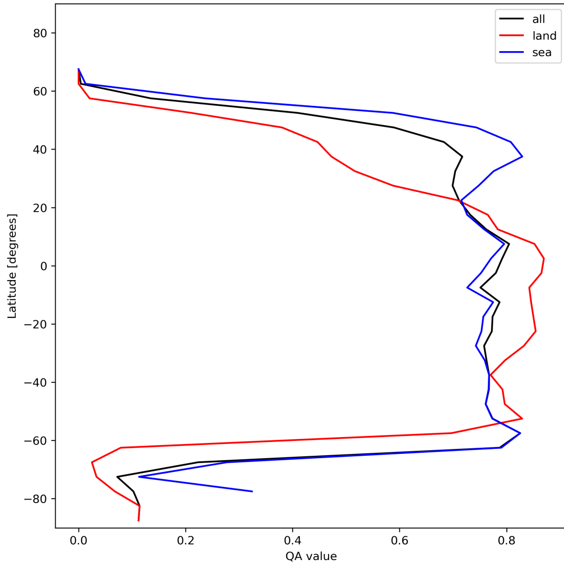
Figure 22: Zonal average of “QA value” for 2023-12-23 to 2023-12-25.
