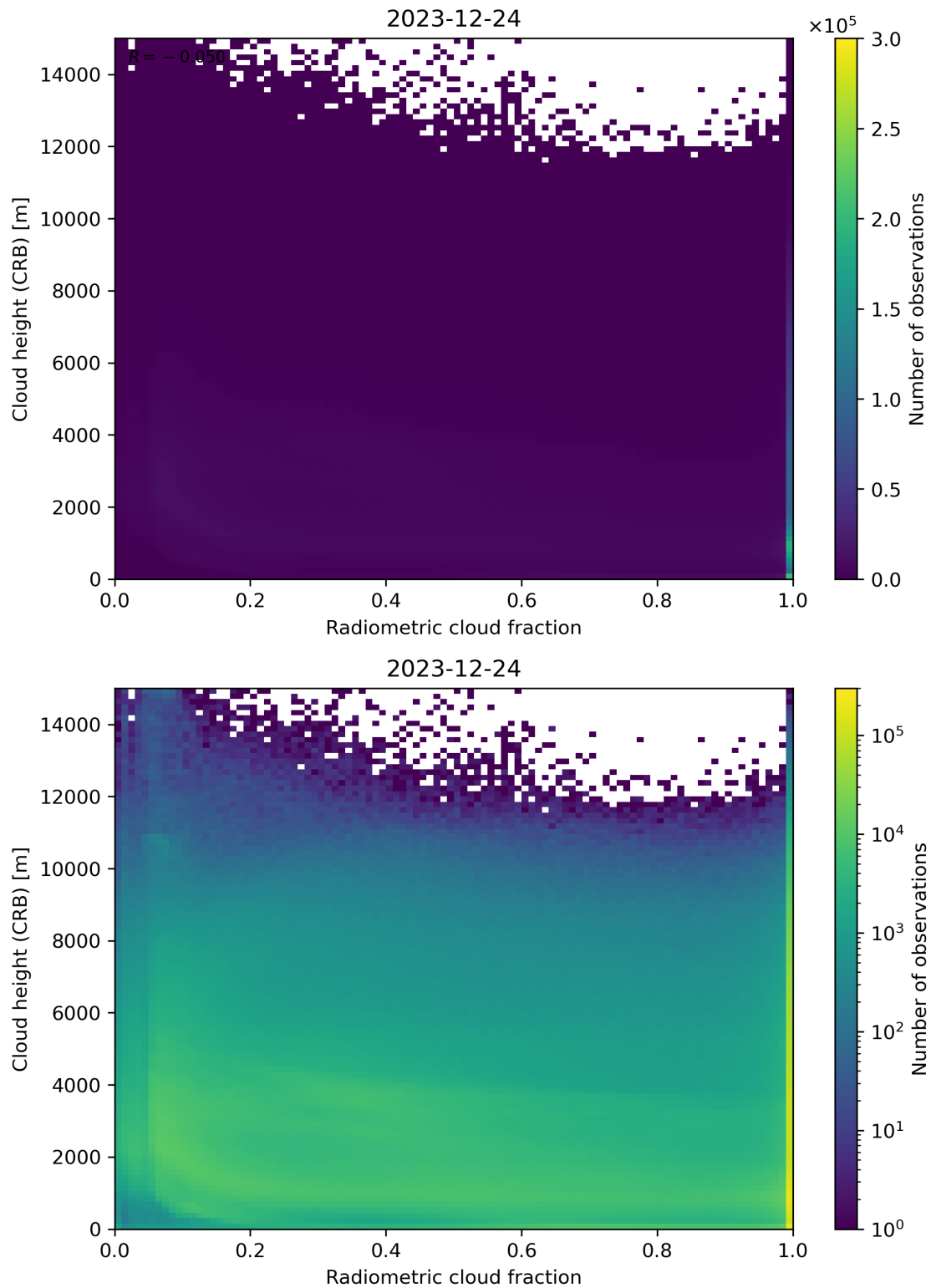
Figure 74: Scatter density plot of “Radiometric cloud fraction” against “Cloud height (CRB)” for 2023-12-23 to 2023-12-25.
