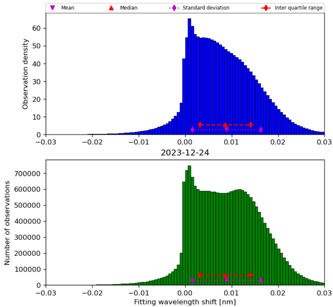
Figure 49: Histogram of “Fitting wavelength shift” for 2023-12-23 to 2023-12-25
