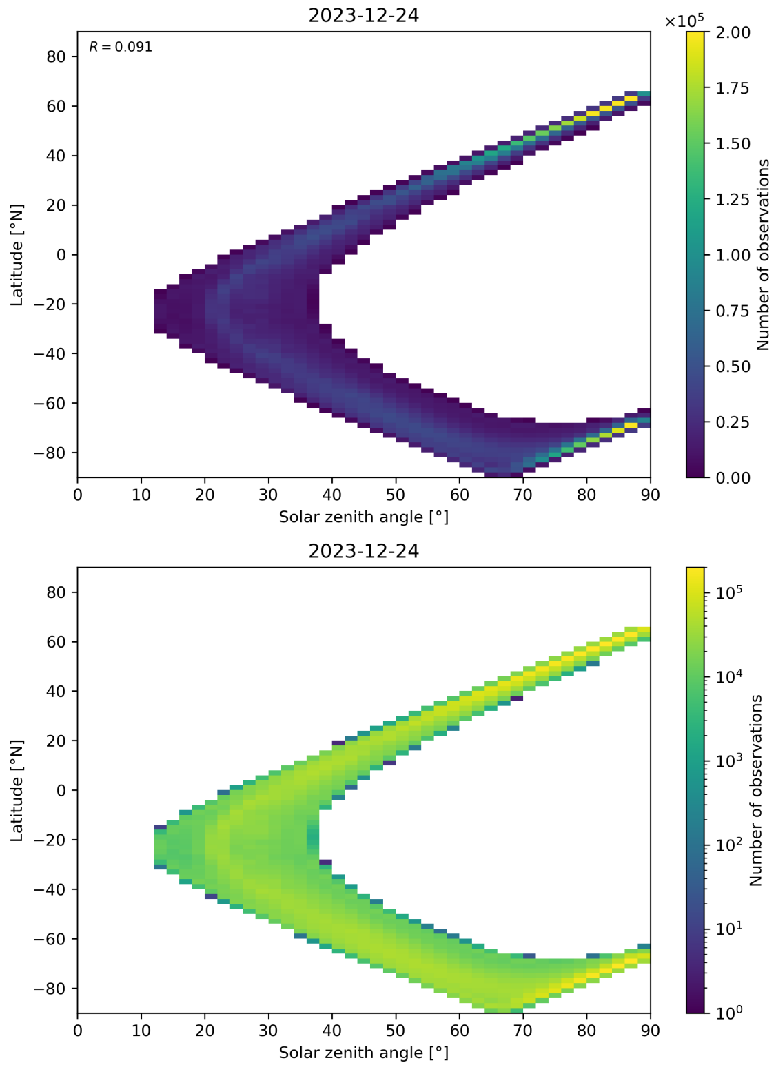
Figure 105: Scatter density plot of “Solar zenith angle” against “Latitude” for 2023-12-23 to 2023-12-25.
