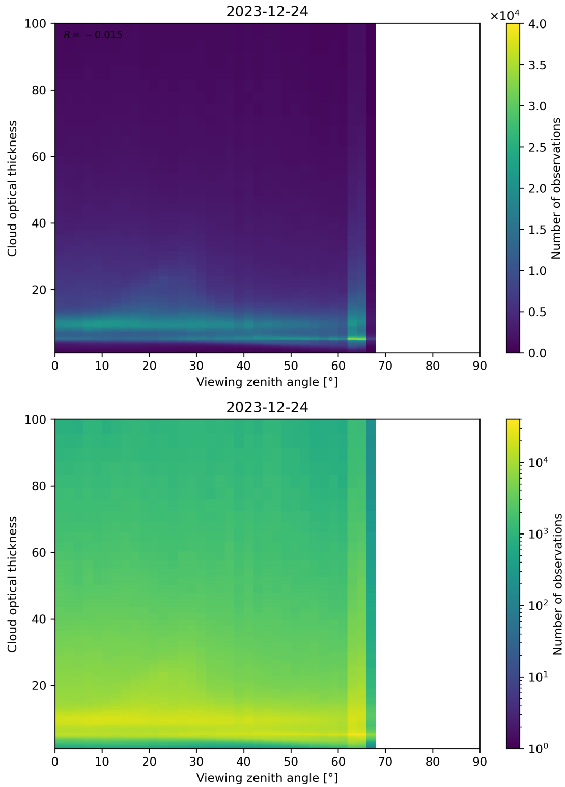
Figure 111: Scatter density plot of “Viewing zenith angle” against “Cloud optical thickness” for 2023-12-23 to 2023-12-25.
