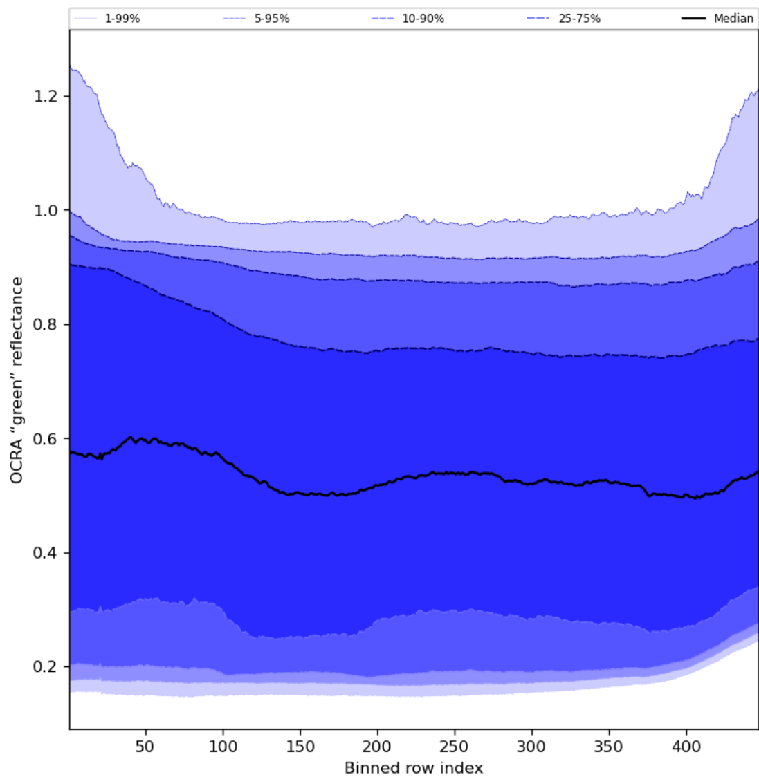
Figure 68: Along track statistics of “OCRA “green” reflectance” for 2023-12-23 to 2023-12-25
