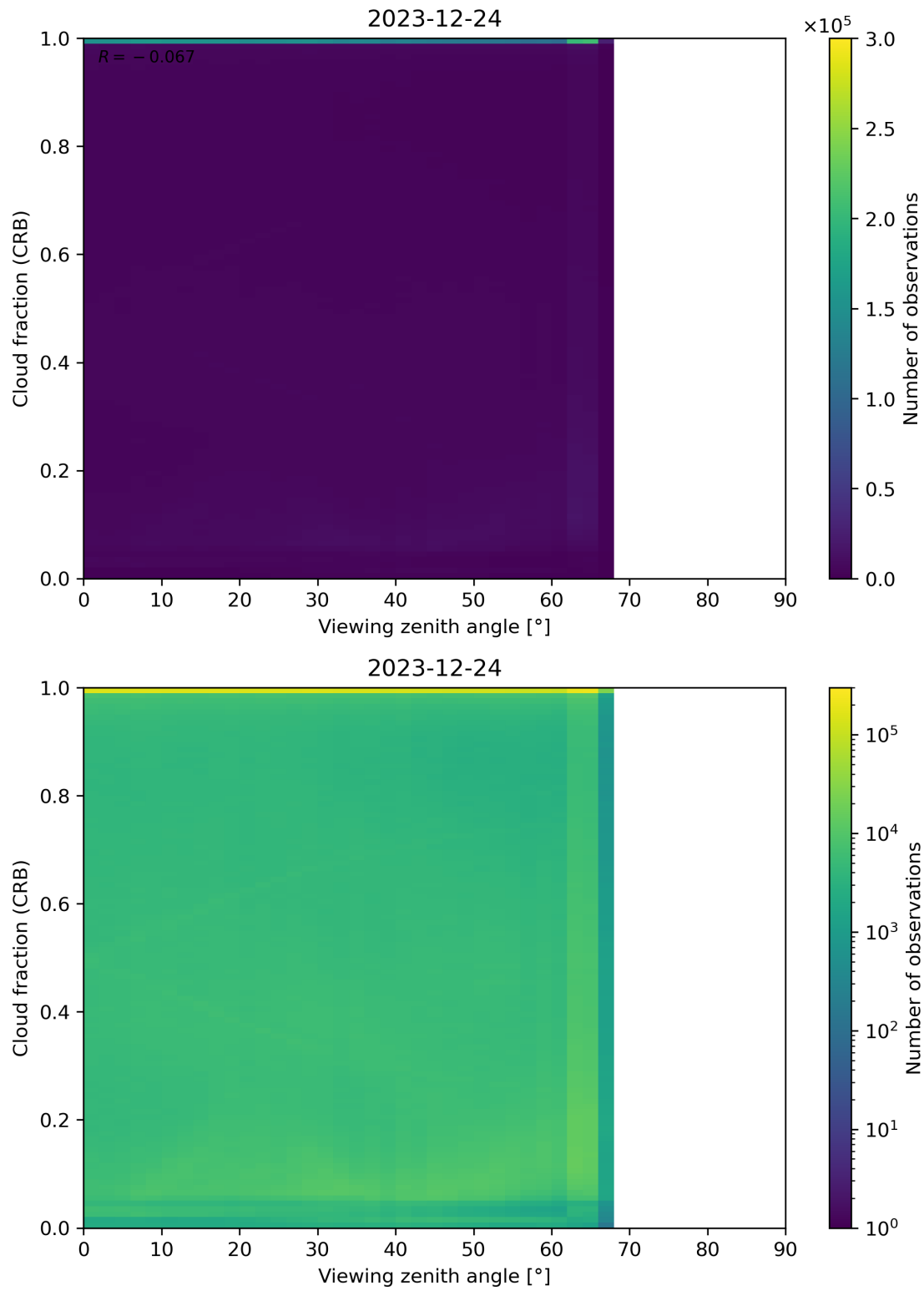
Figure 109: Scatter density plot of “Viewing zenith angle” against “Cloud fraction (CRB)” for 2023-12-23 to 2023-12-25.
