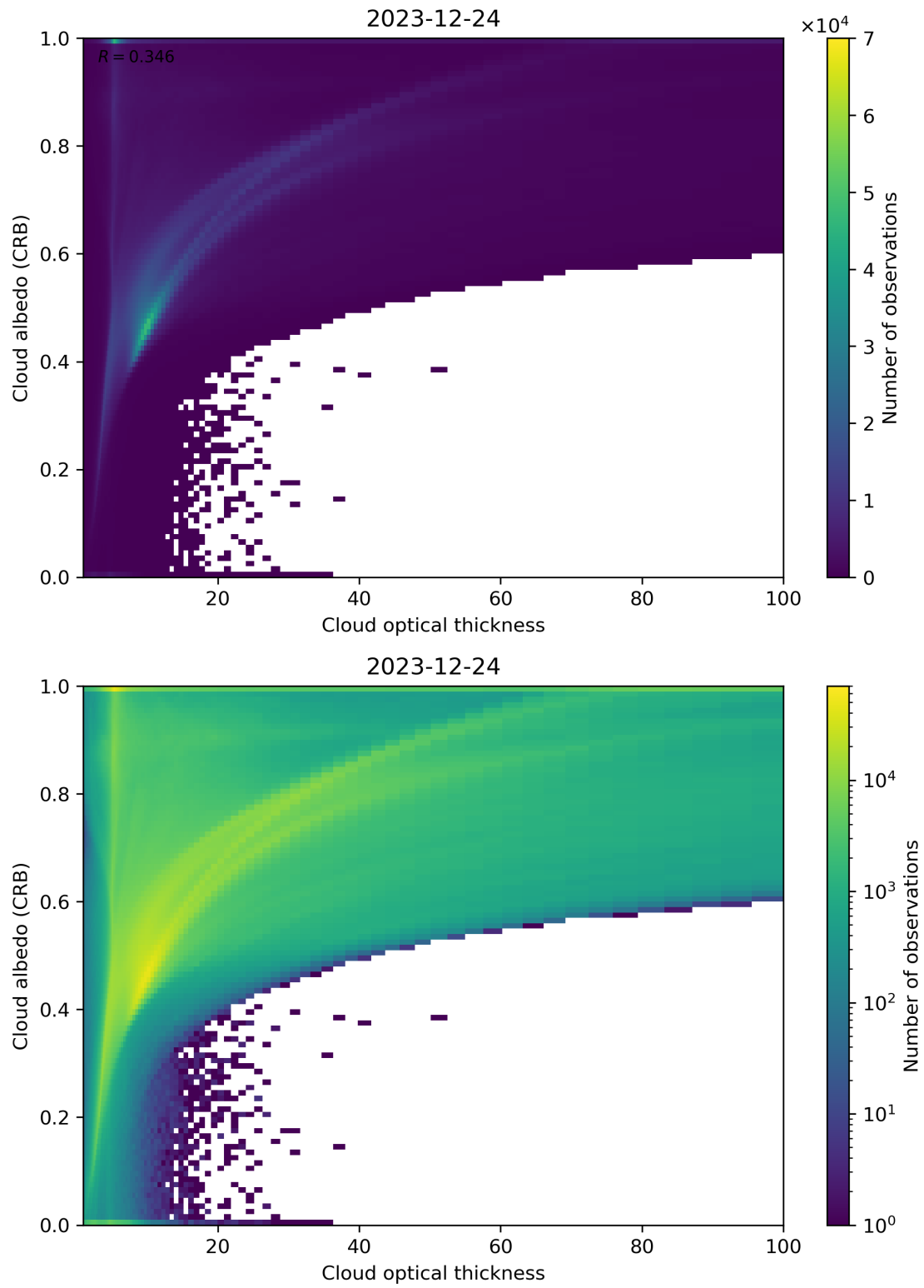
Figure 82: Scatter density plot of “Cloud optical thickness” against “Cloud albedo (CRB)” for 2023-12-23 to 2023-12-25.
