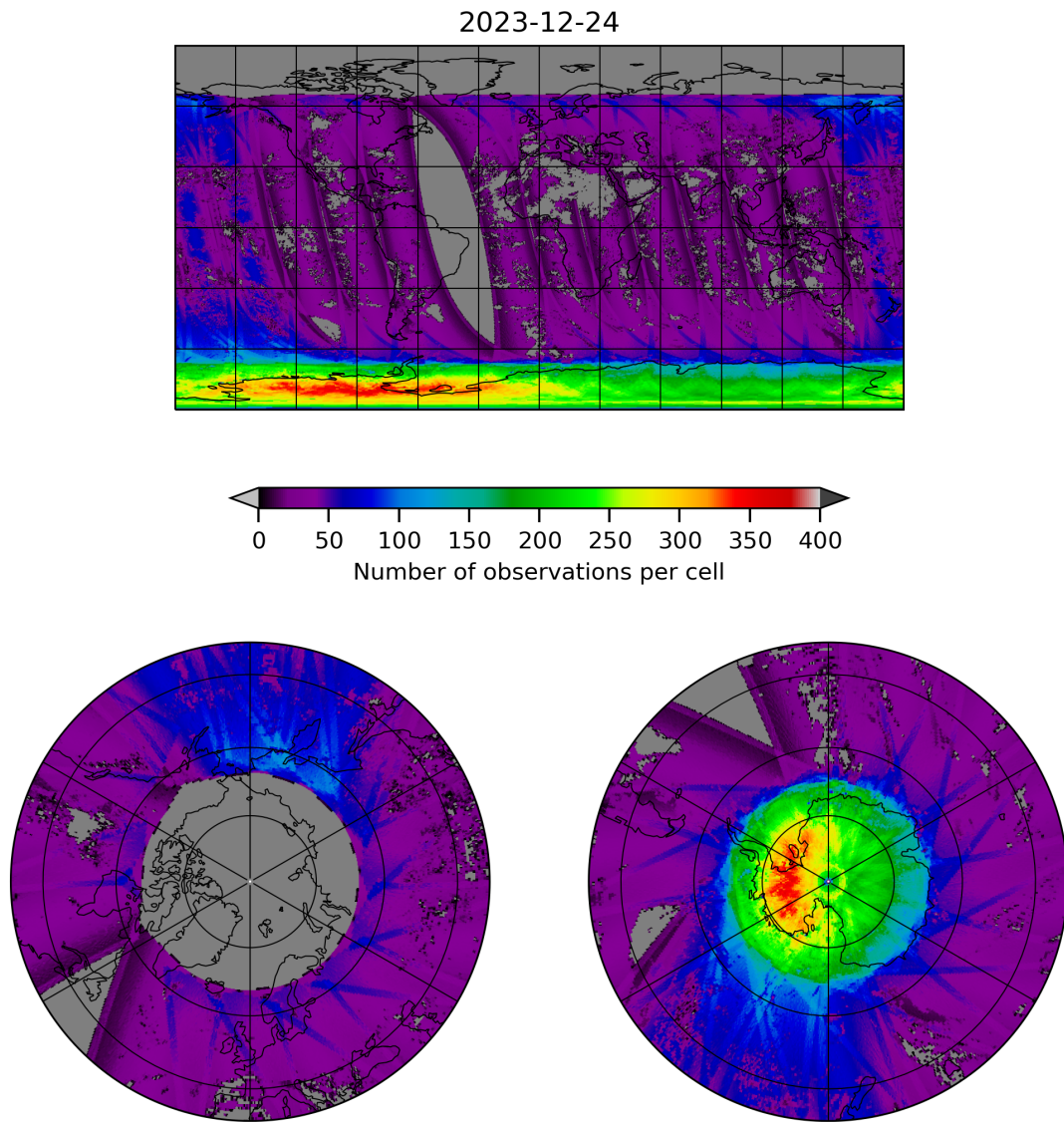
Figure 21: Map of the number of observations for 2023-12-23 to 2023-12-25
