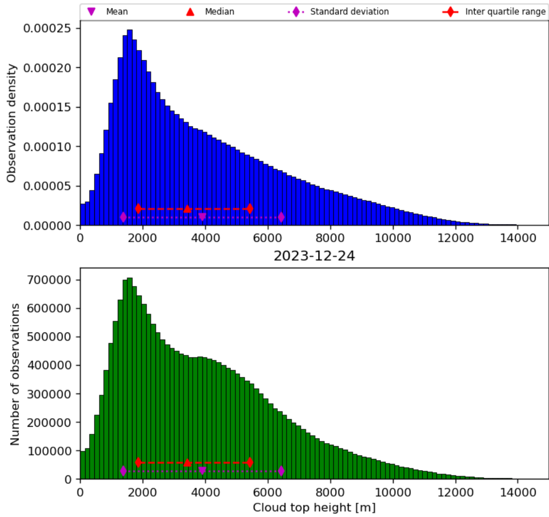
Figure 40: Histogram of “Cloud top height” for 2023-12-23 to 2023-12-25
