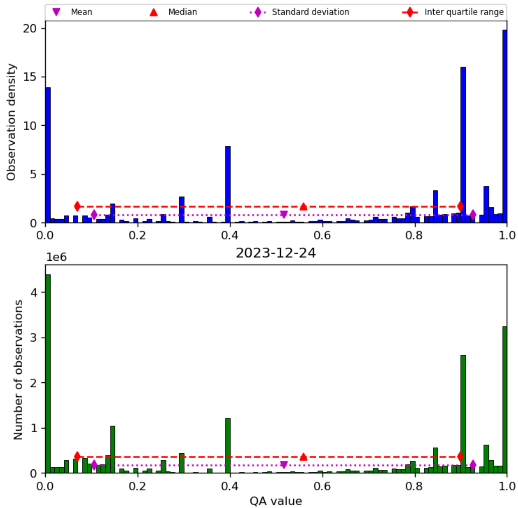
Figure 38: Histogram of “QA value” for 2023-12-23 to 2023-12-25
