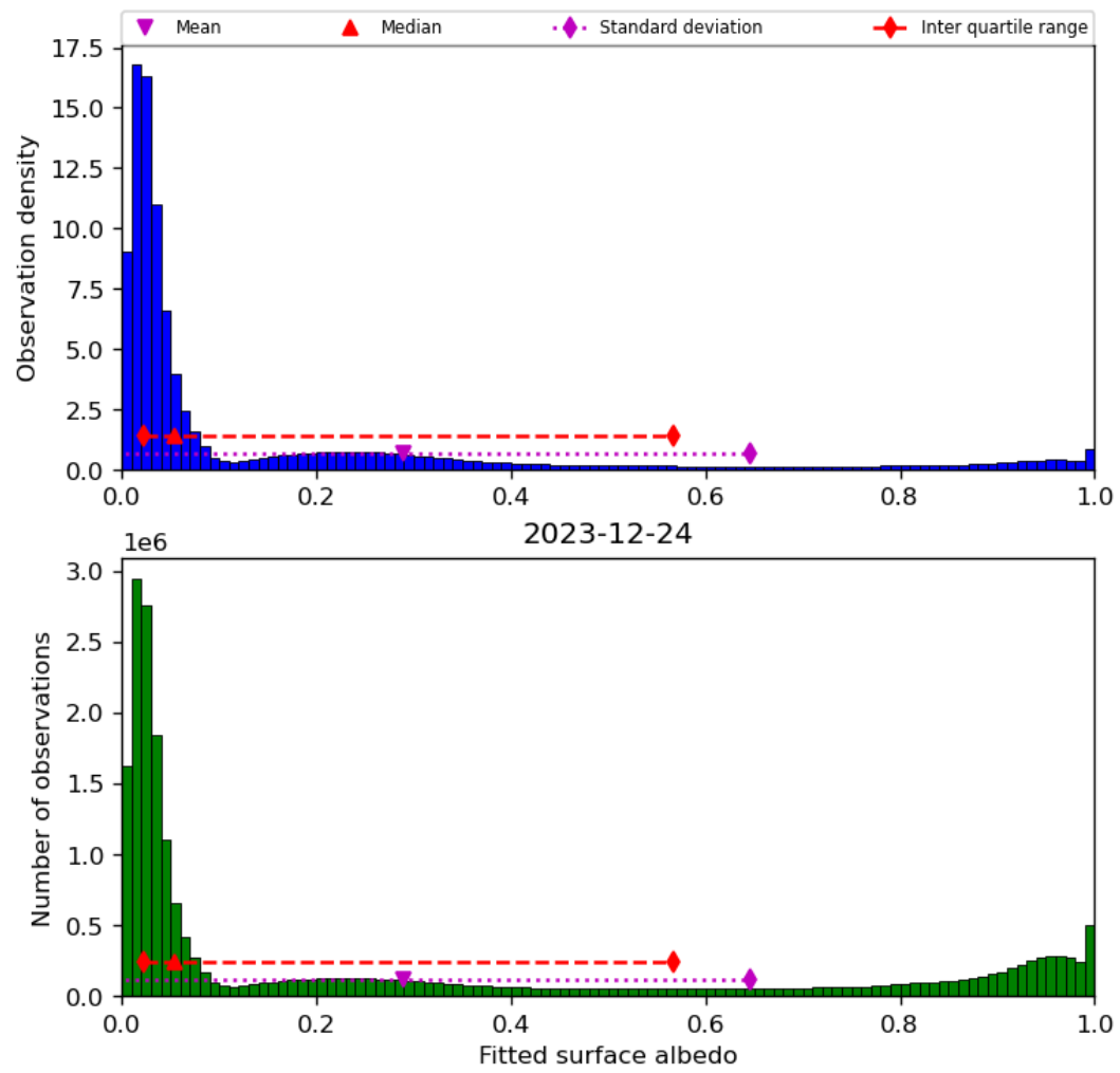
Figure 45: Histogram of “Fitted surface albedo” for 2023-12-23 to 2023-12-25
