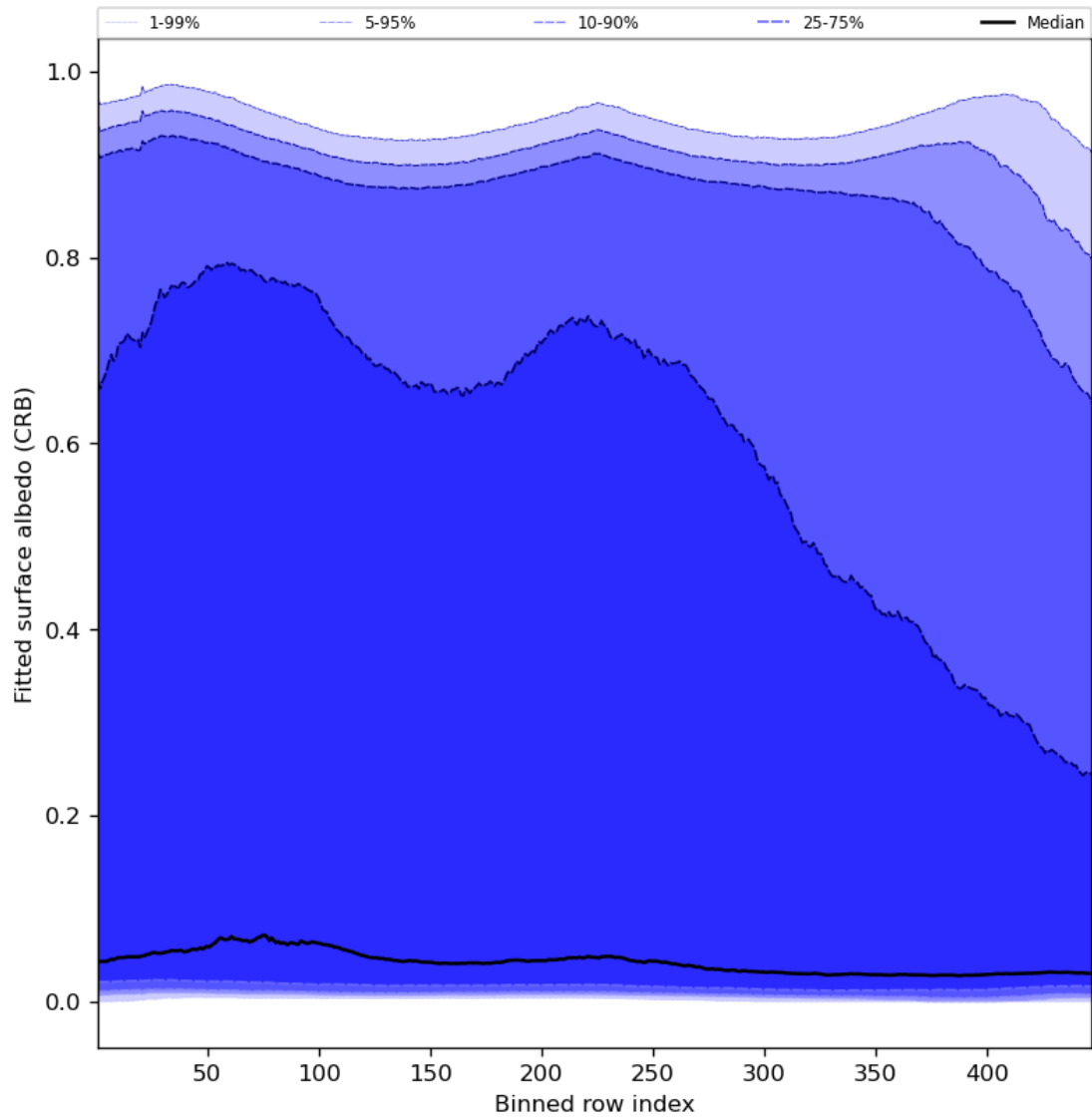
Figure 62: Along track statistics of “Fitted surface albedo (CRB)” for 2023-12-23 to 2023-12-25
