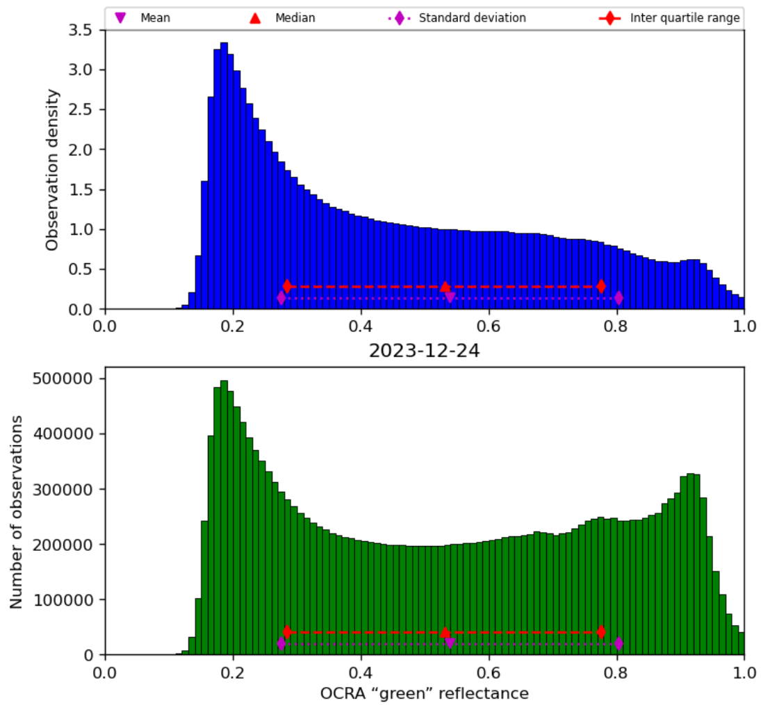
Figure 52: Histogram of “OCRA “green” reflectance” for 2023-12-23 to 2023-12-25
