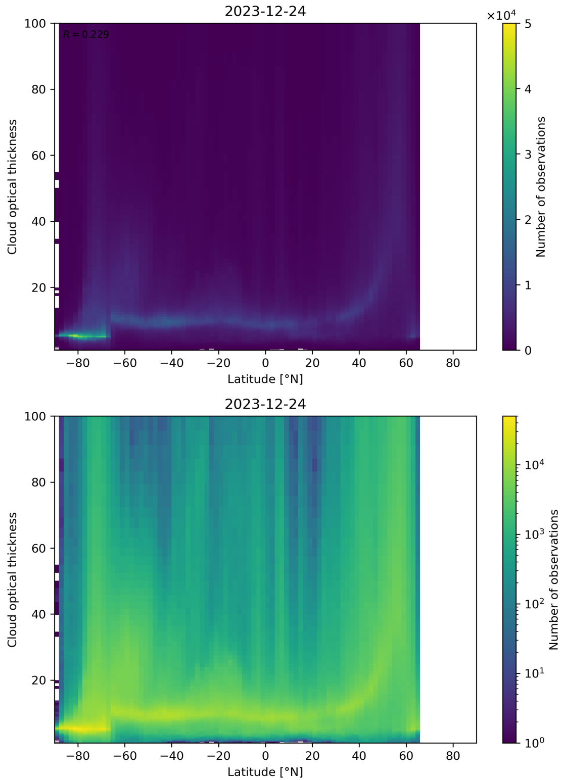
Figure 96: Scatter density plot of “Latitude” against “Cloud optical thickness” for 2023-12-23 to 2023-12-25.
