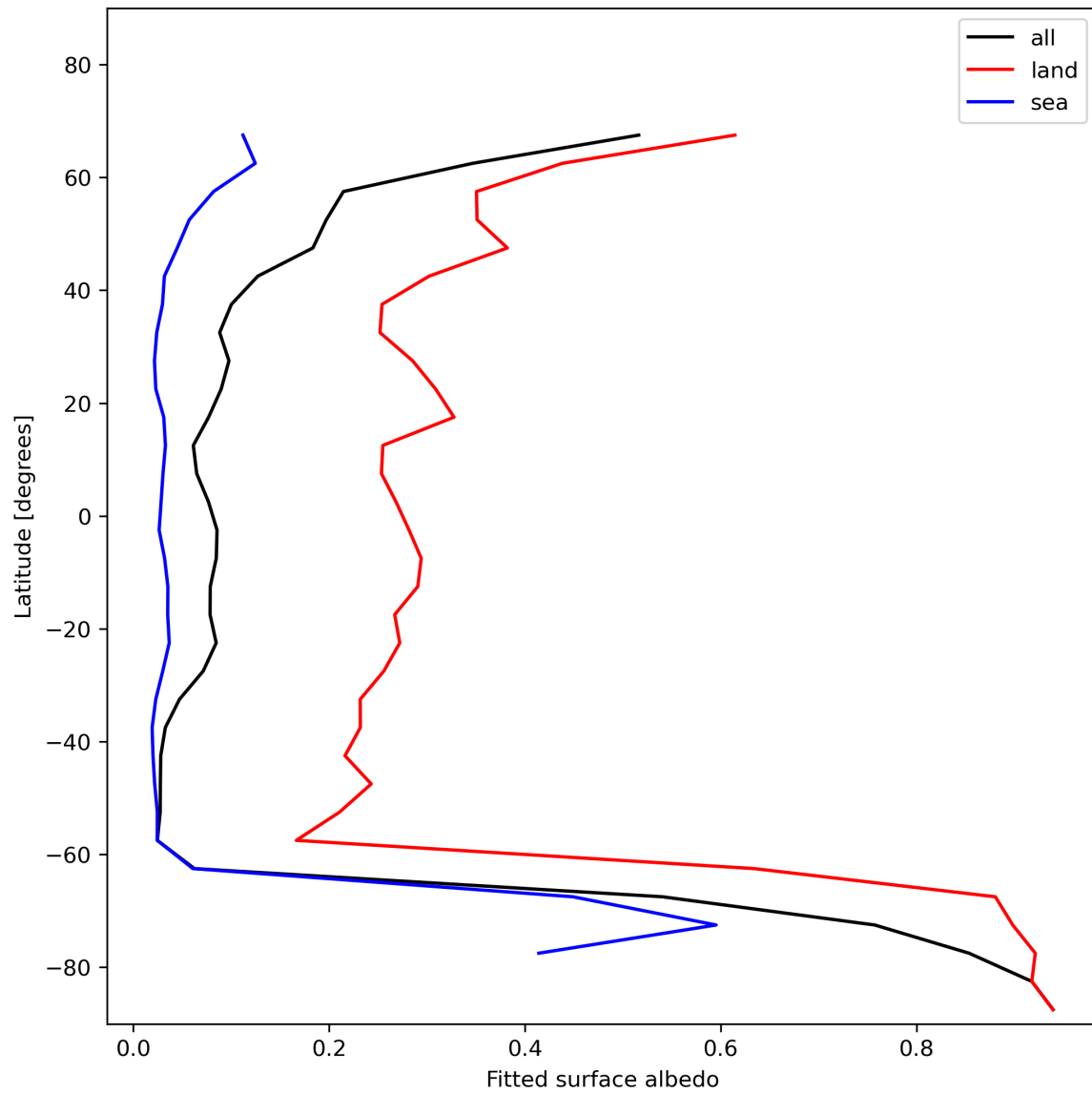
Figure 29: Zonal average of “Fitted surface albedo” for 2023-12-23 to 2023-12-25.
