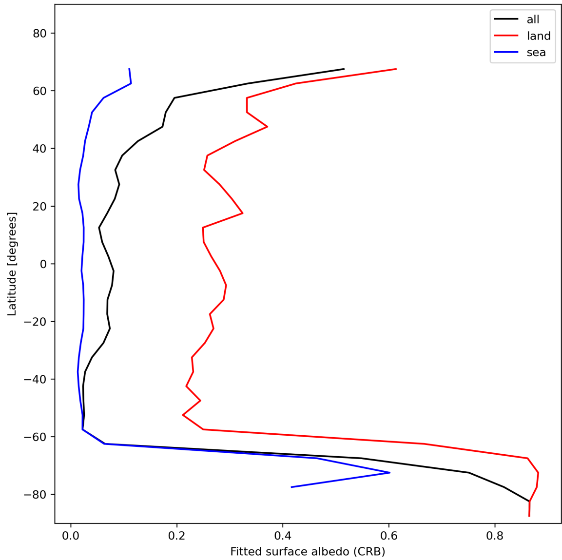
Figure 30: Zonal average of “Fitted surface albedo (CRB)” for 2023-12-23 to 2023-12-25.
