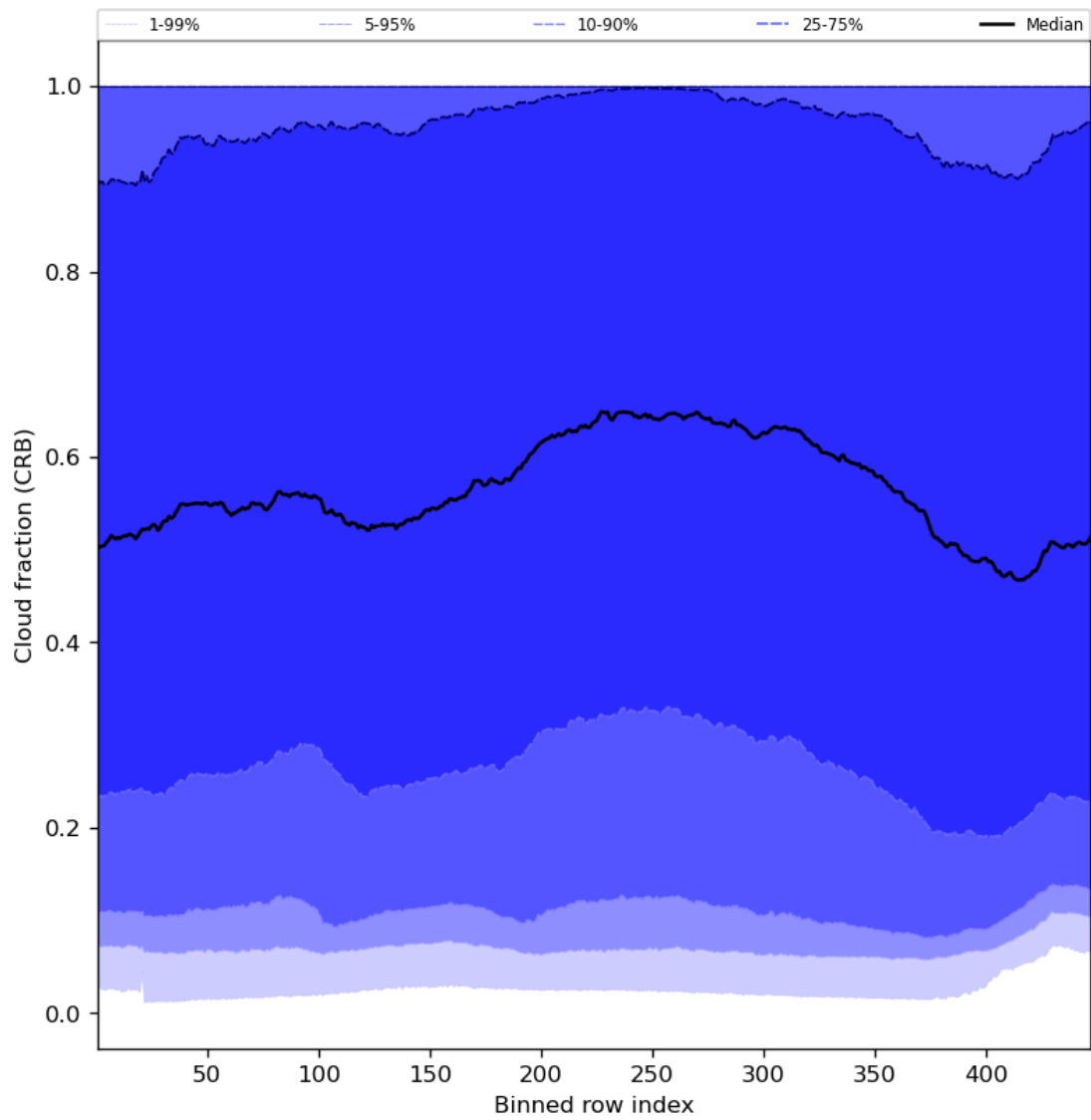
Figure 58: Along track statistics of “Cloud fraction (CRB)” for 2023-12-23 to 2023-12-25
