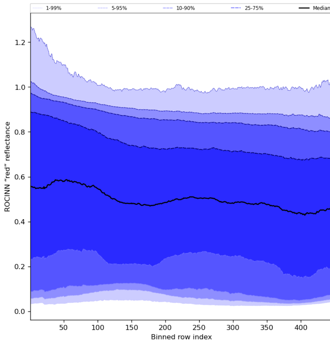
Figure 69: Along track statistics of “ROCINN “red” reflectance” for 2023-12-23 to 2023-12-25
