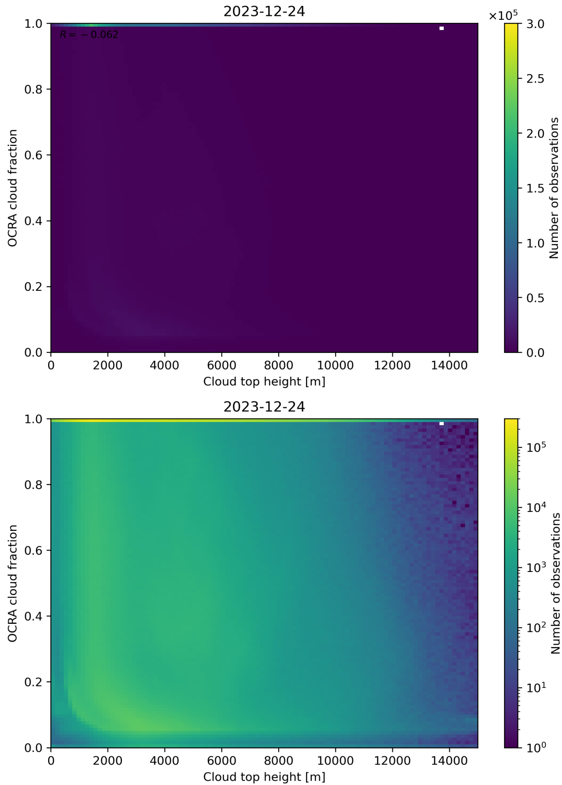
Figure 87: Scatter density plot of “Cloud top height” against “OCRA cloud fraction” for 2023-12-23 to 2023-12-25.
