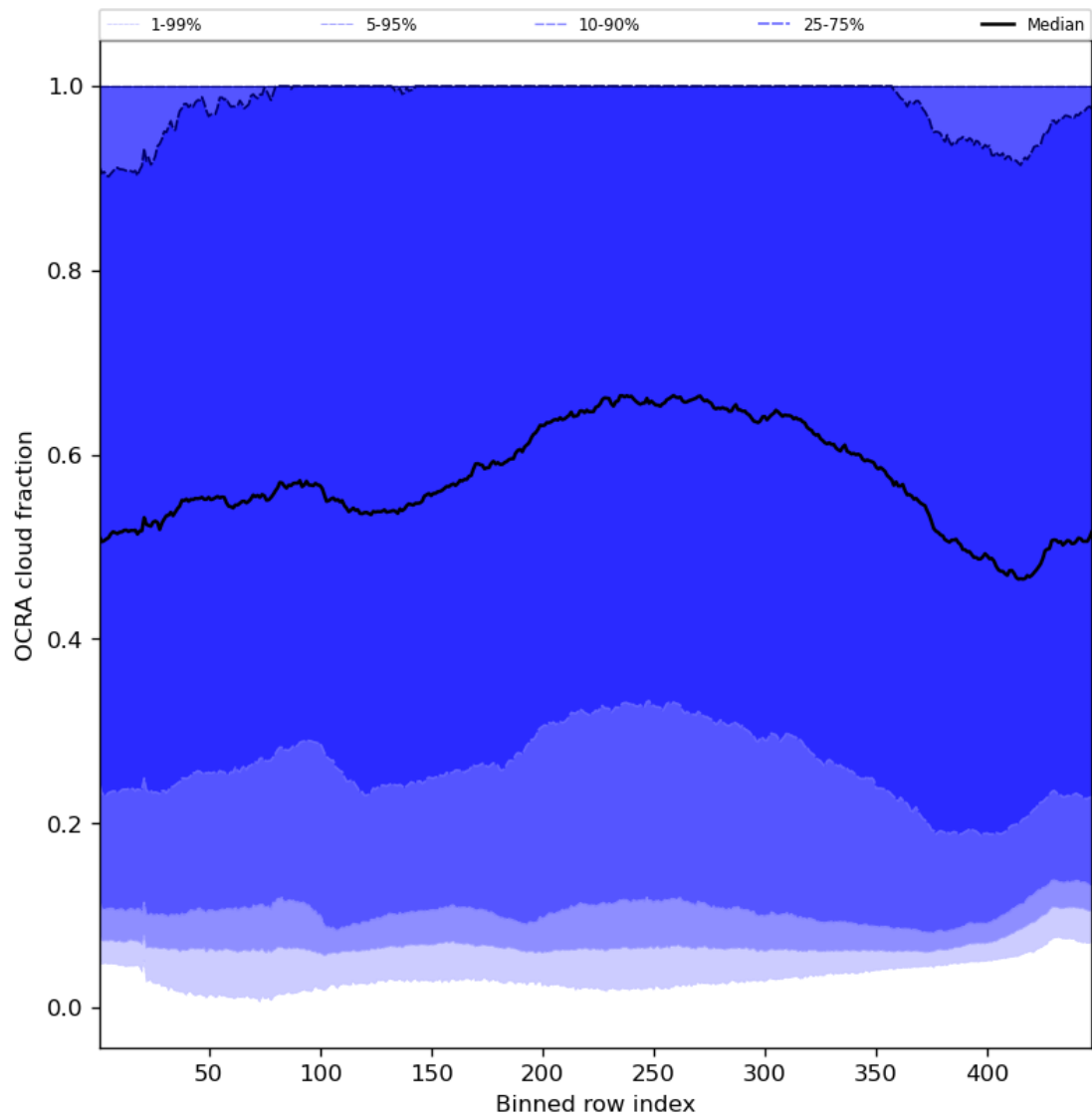
Figure 66: Along track statistics of “OCRA cloud fraction” for 2023-12-23 to 2023-12-25
