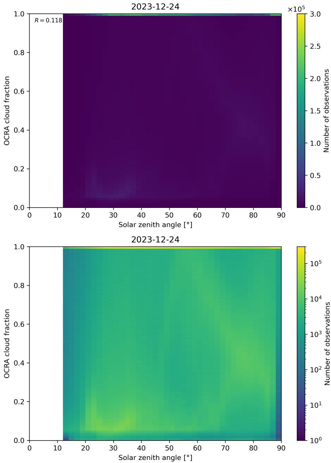
Figure 100: Scatter density plot of “Solar zenith angle” against “OCRA cloud fraction” for 2023-12-23 to 2023-12-25.
