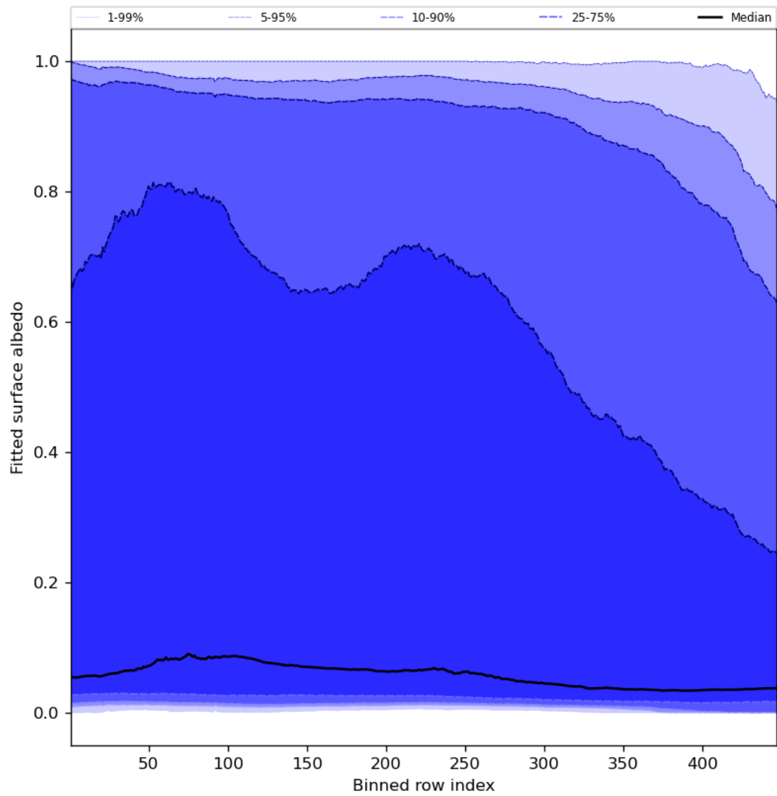
Figure 61: Along track statistics of “Fitted surface albedo” for 2023-12-23 to 2023-12-25
