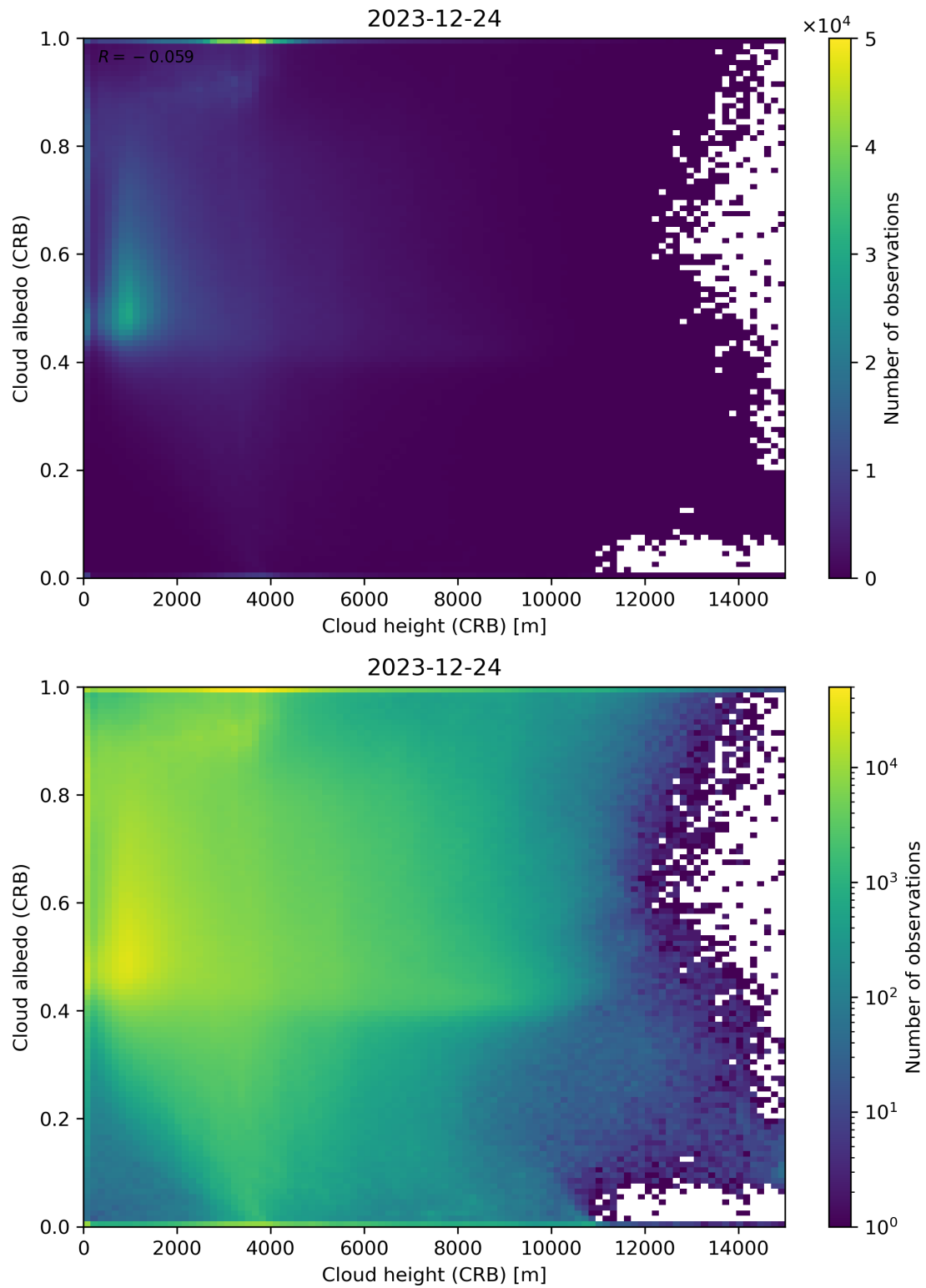
Figure 80: Scatter density plot of “Cloud height (CRB)” against “Cloud albedo (CRB)” for 2023-12-23 to 2023-12-25.
