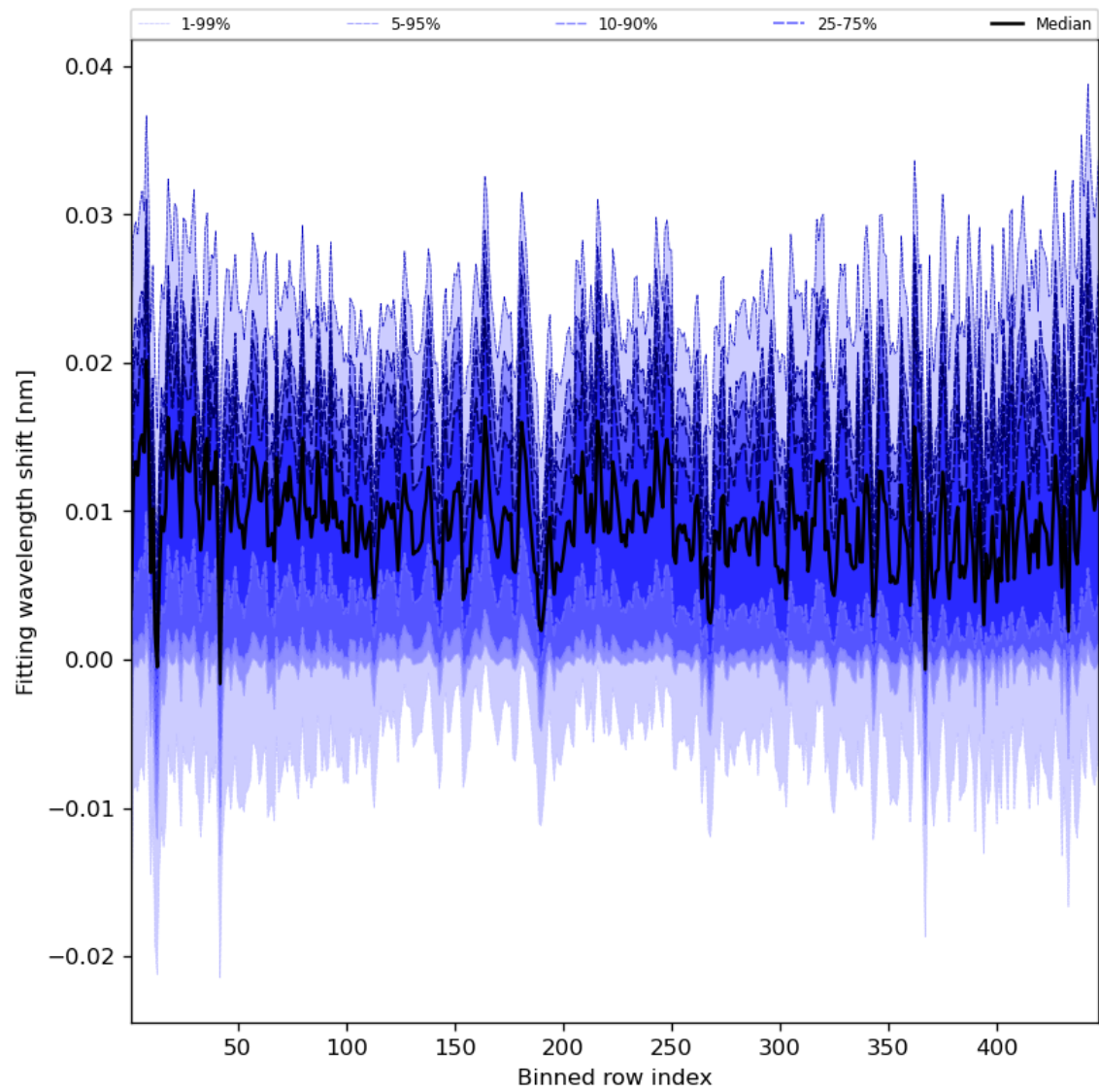
Figure 65: Along track statistics of “Fitting wavelength shift” for 2023-12-23 to 2023-12-25
