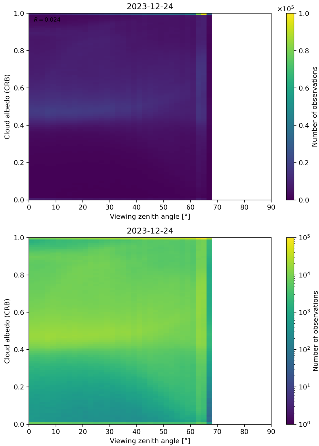
Figure 106: Scatter density plot of “Viewing zenith angle” against “Cloud albedo (CRB)” for 2023-12-23 to 2023-12-25.
