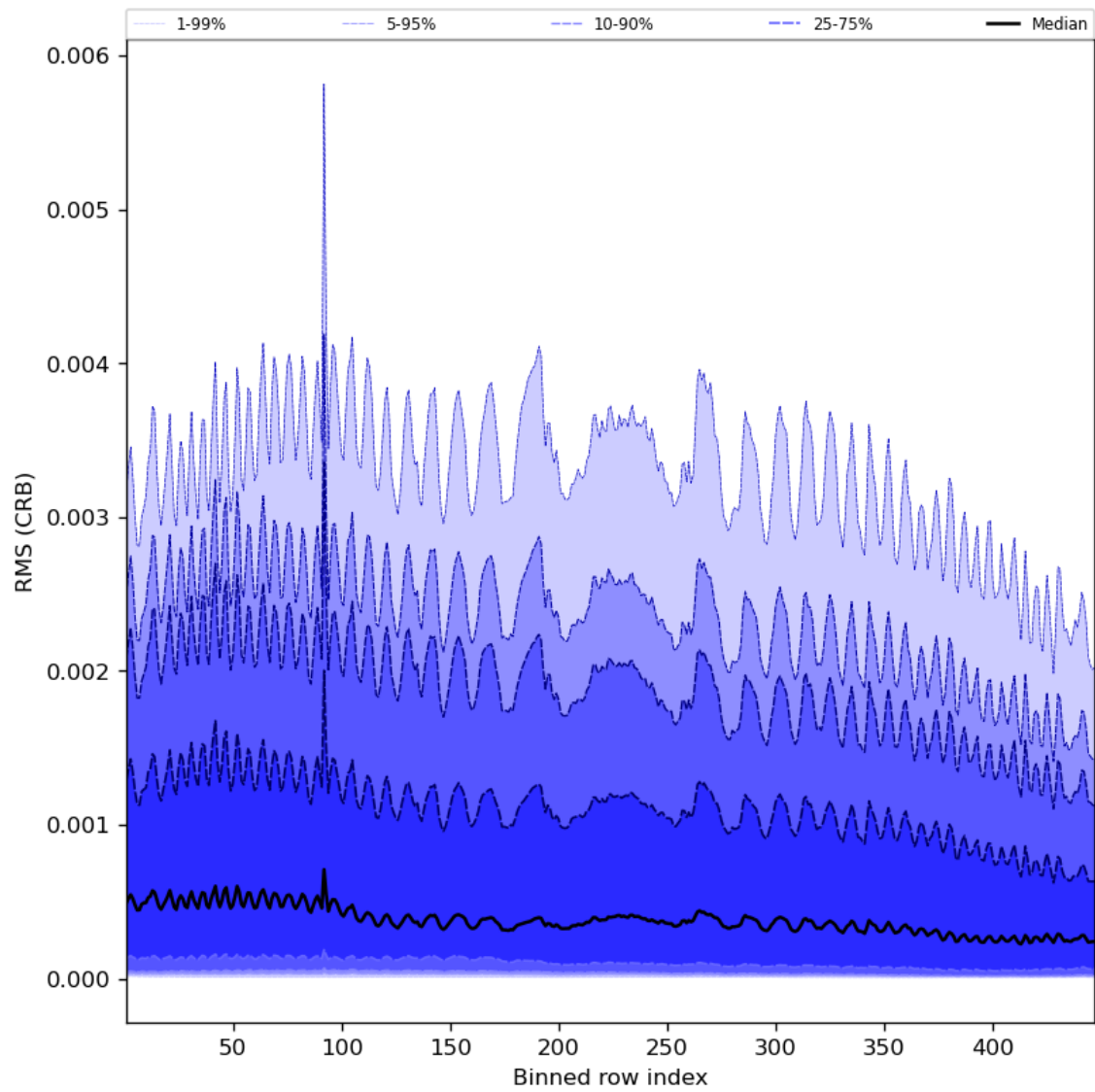
Figure 64: Along track statistics of “RMS (CRB)” for 2023-12-23 to 2023-12-25
