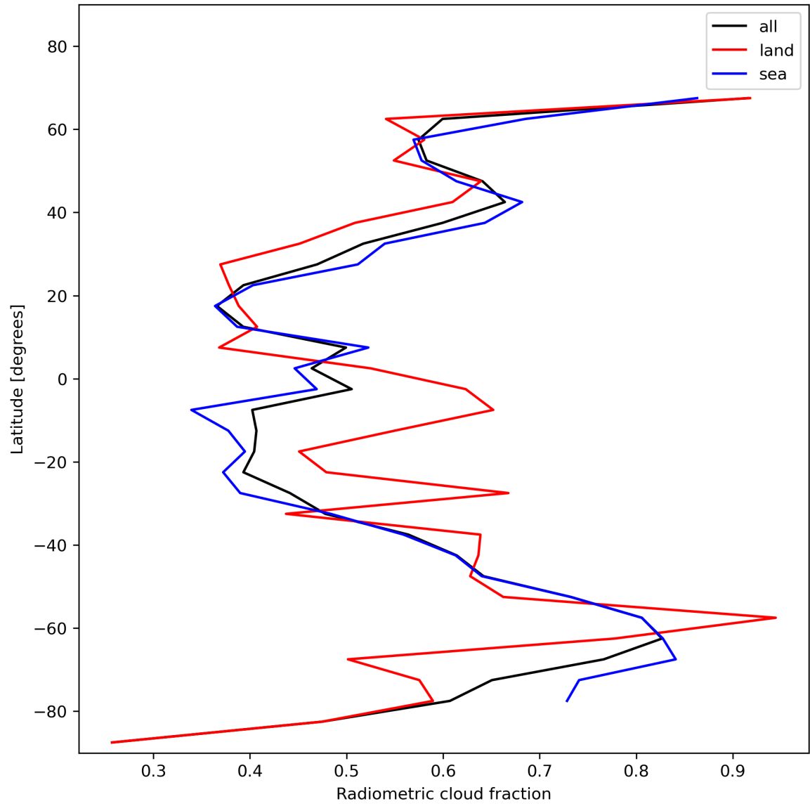
Figure 23: Zonal average of “Radiometric cloud fraction” for 2023-12-23 to 2023-12-25.
