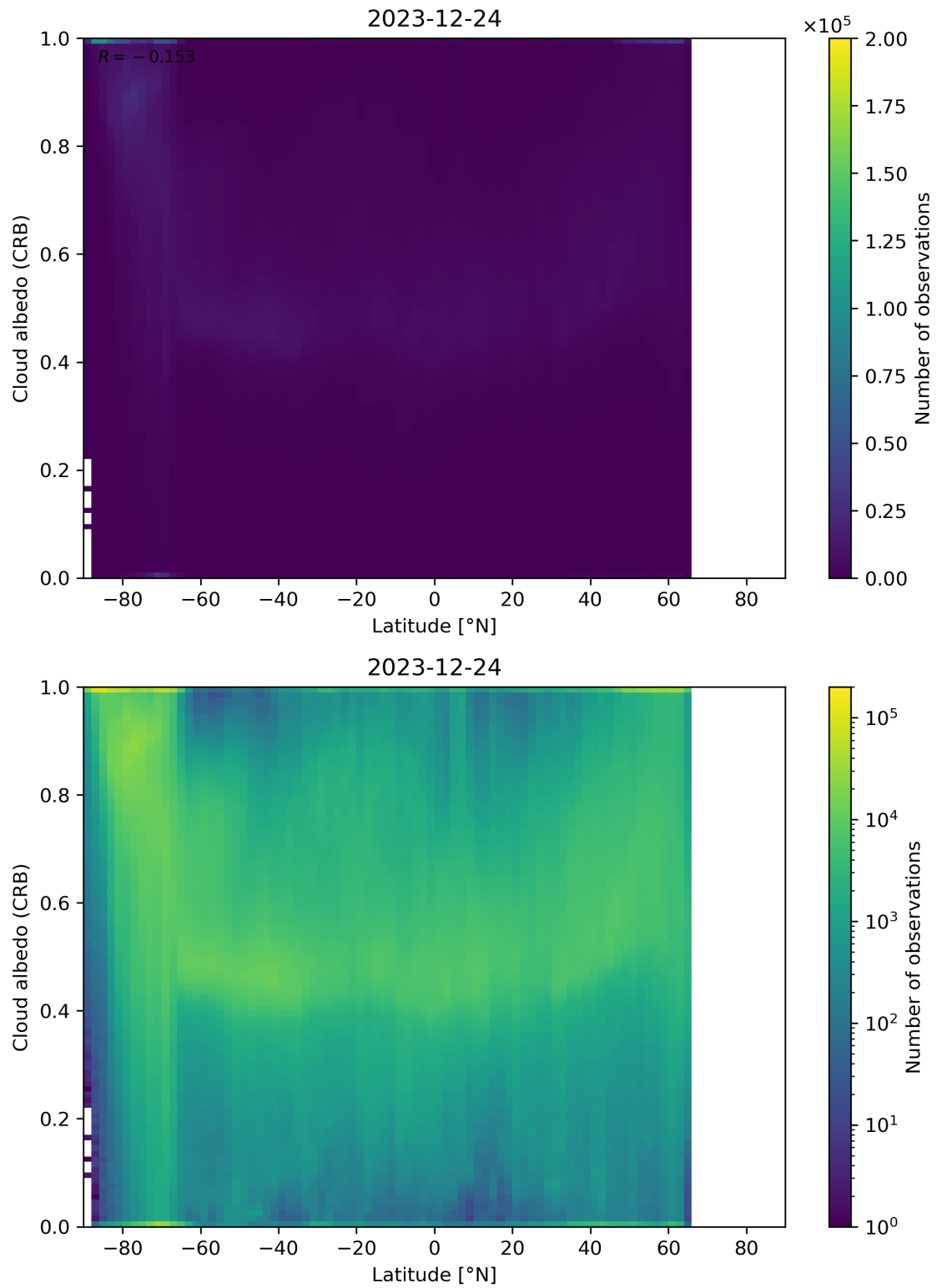
Figure 91: Scatter density plot of “Latitude” against “Cloud albedo (CRB)” for 2023-12-23 to 2023-12-25.
