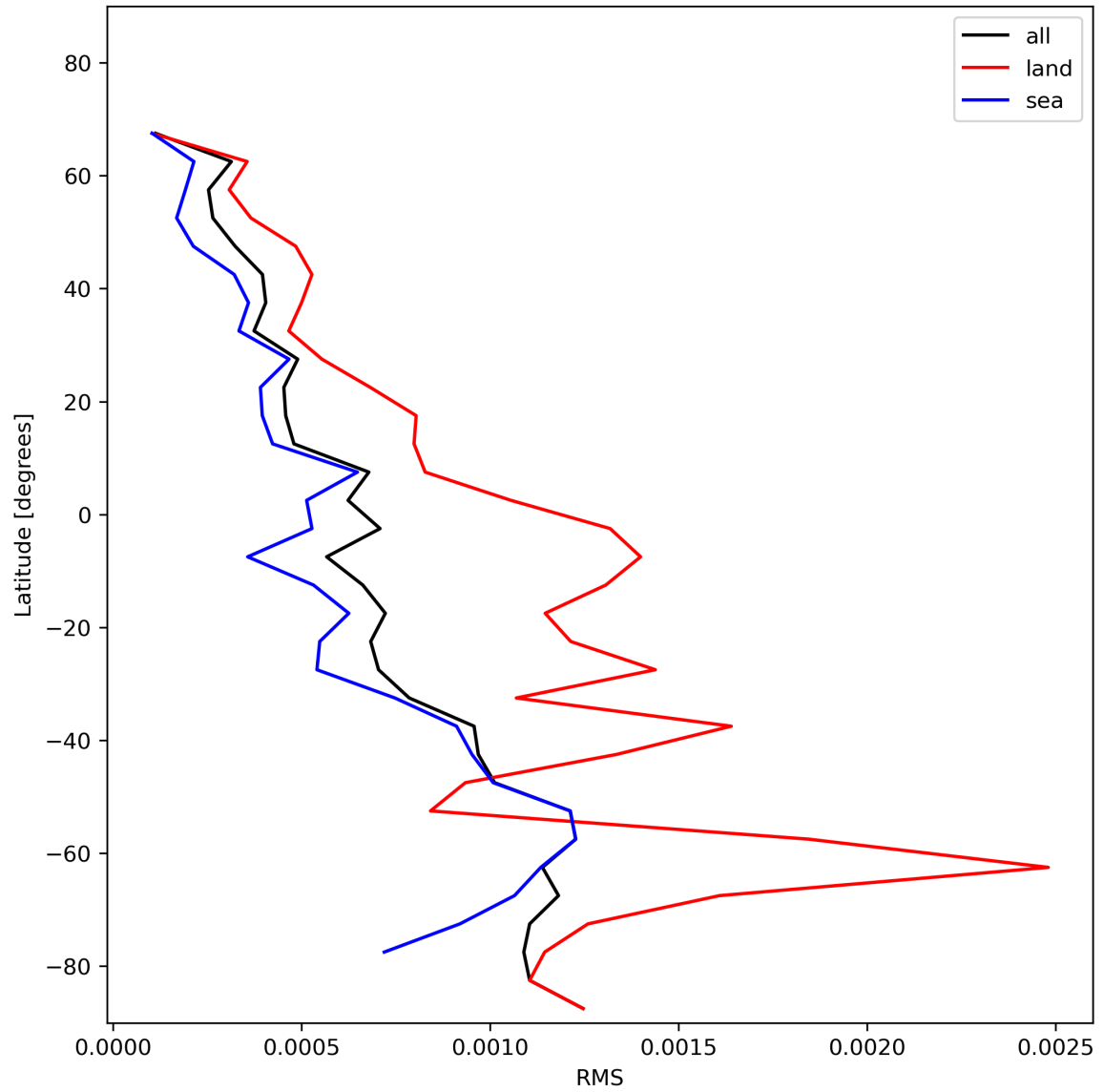
Figure 31: Zonal average of “RMS” for 2023-12-23 to 2023-12-25.
