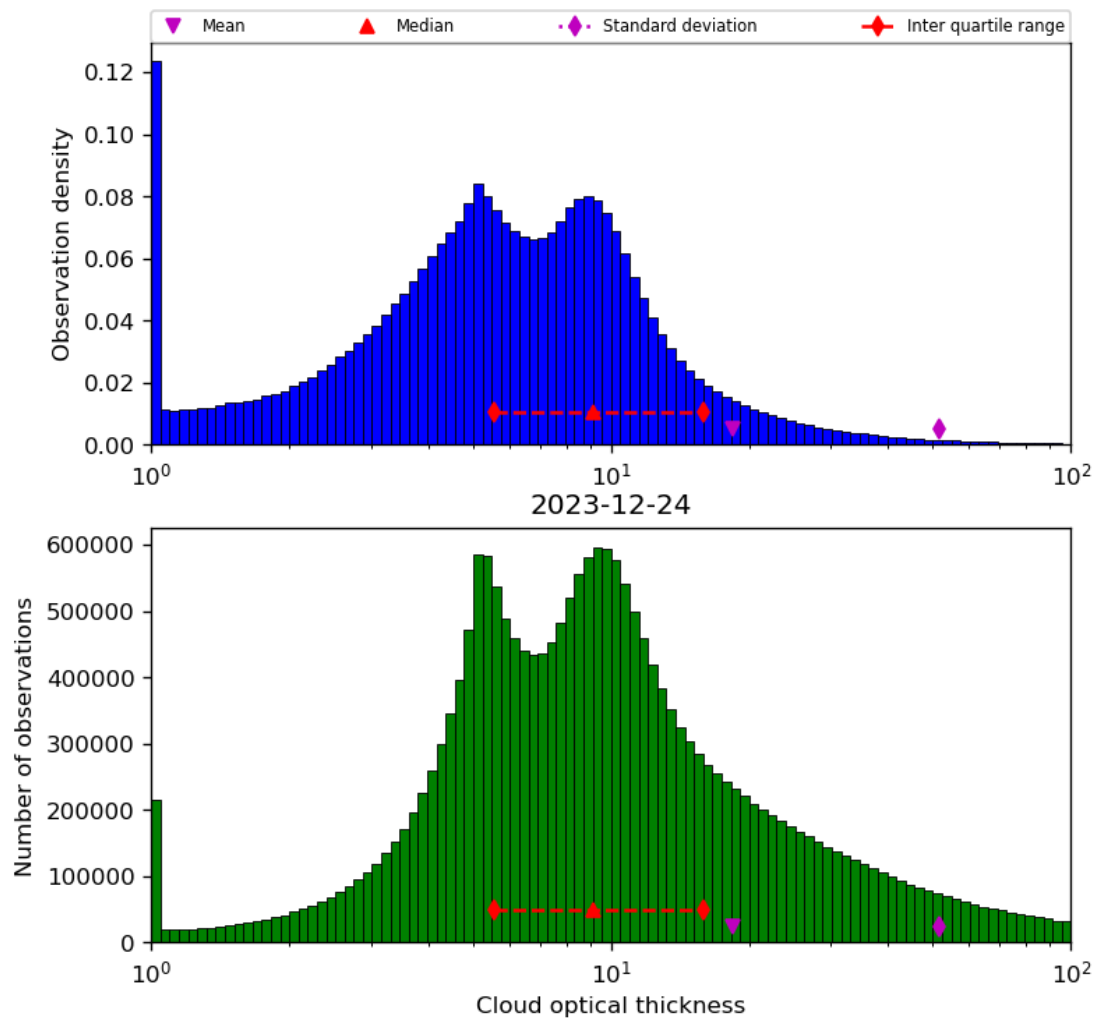
Figure 41: Histogram of “Cloud optical thickness” for 2023-12-23 to 2023-12-25
