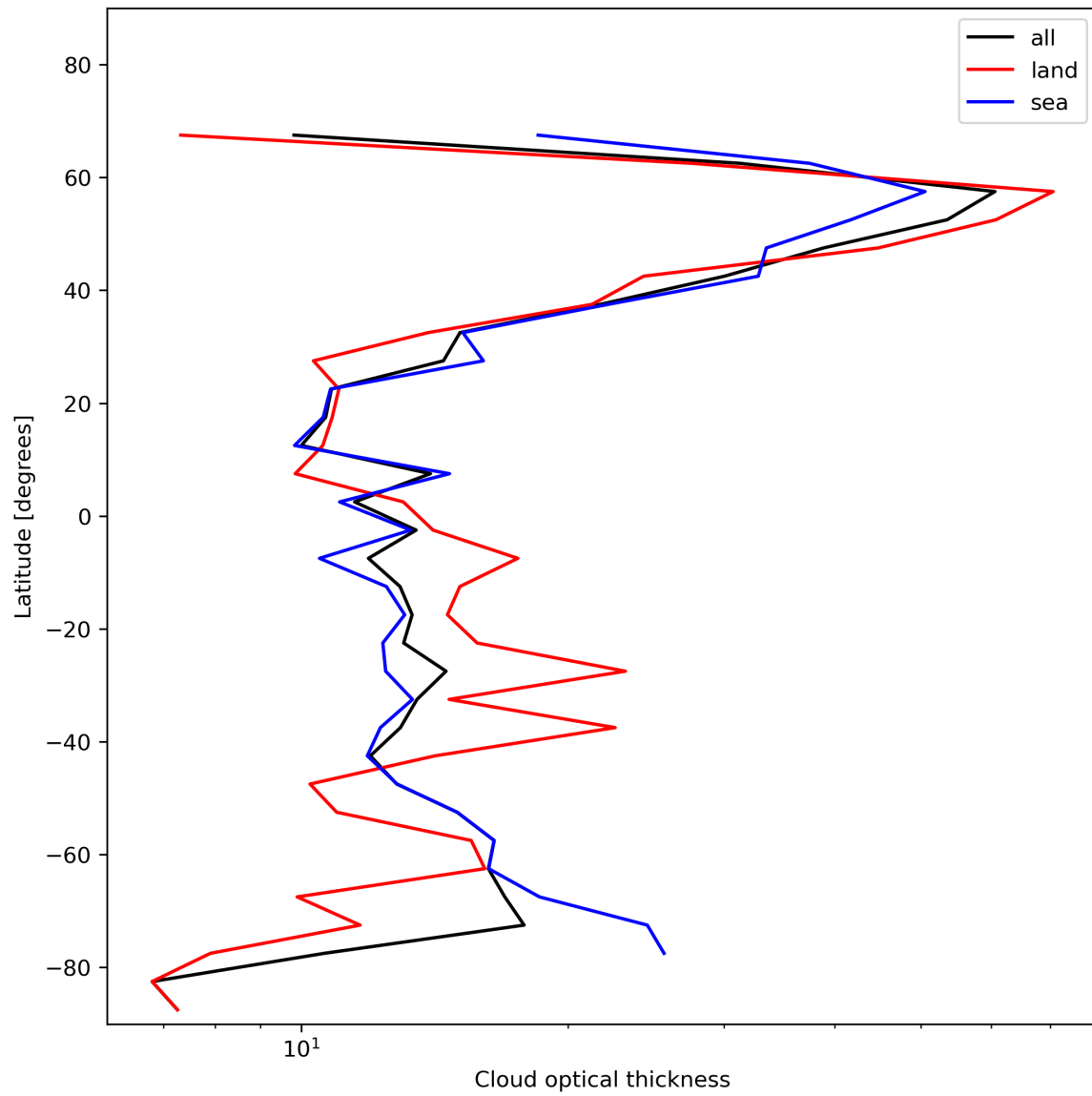
Figure 25: Zonal average of “Cloud optical thickness” for 2023-12-23 to 2023-12-25.
