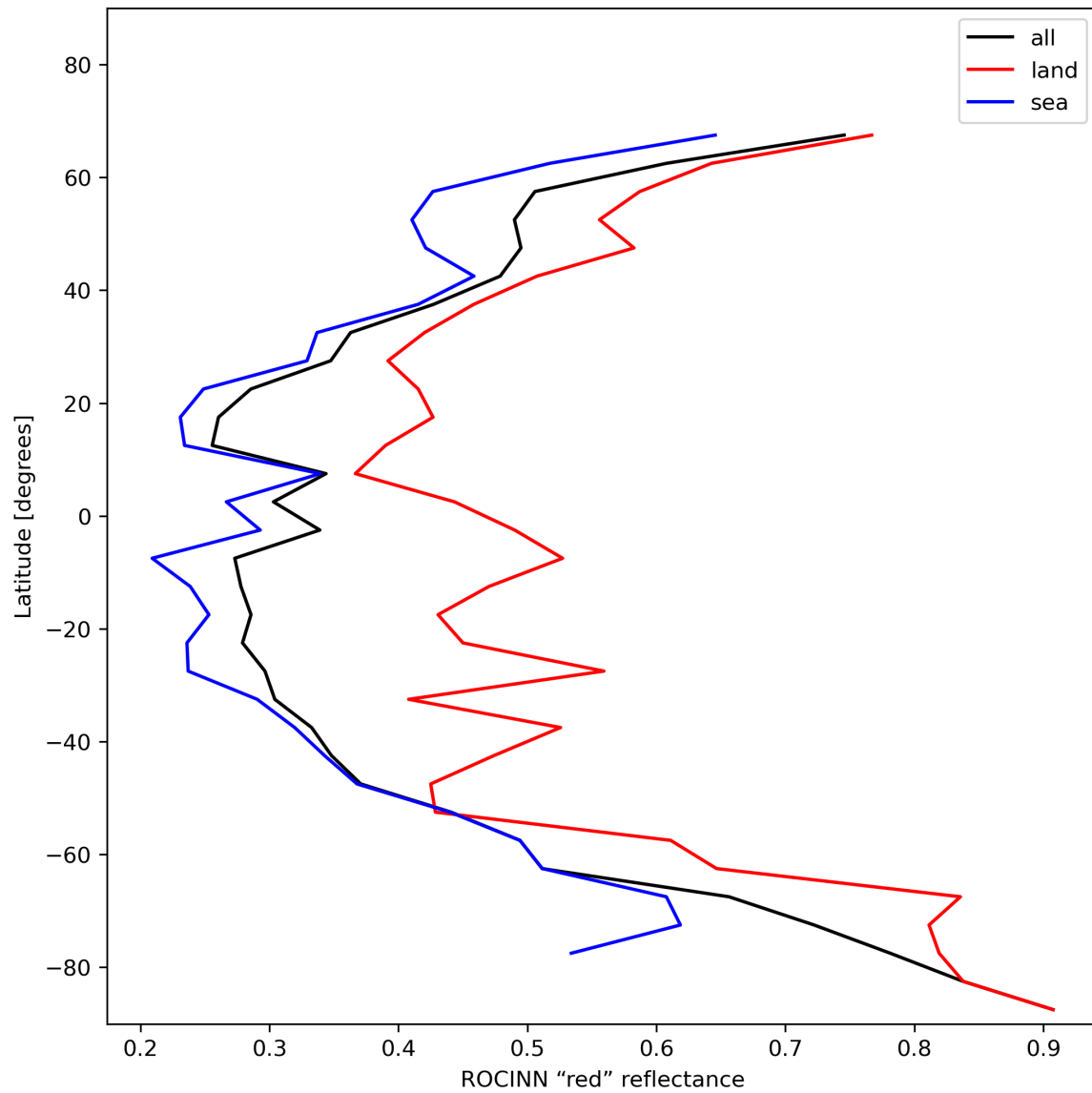
Figure 37: Zonal average of “ROCINN “red” reflectance” for 2023-12-23 to 2023-12-25.
