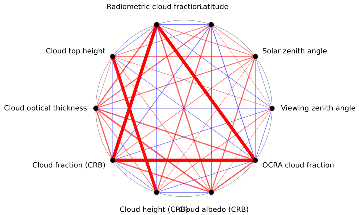
Figure 1: Map of correlation graph for 2023-12-23 to 2023-12-25.
