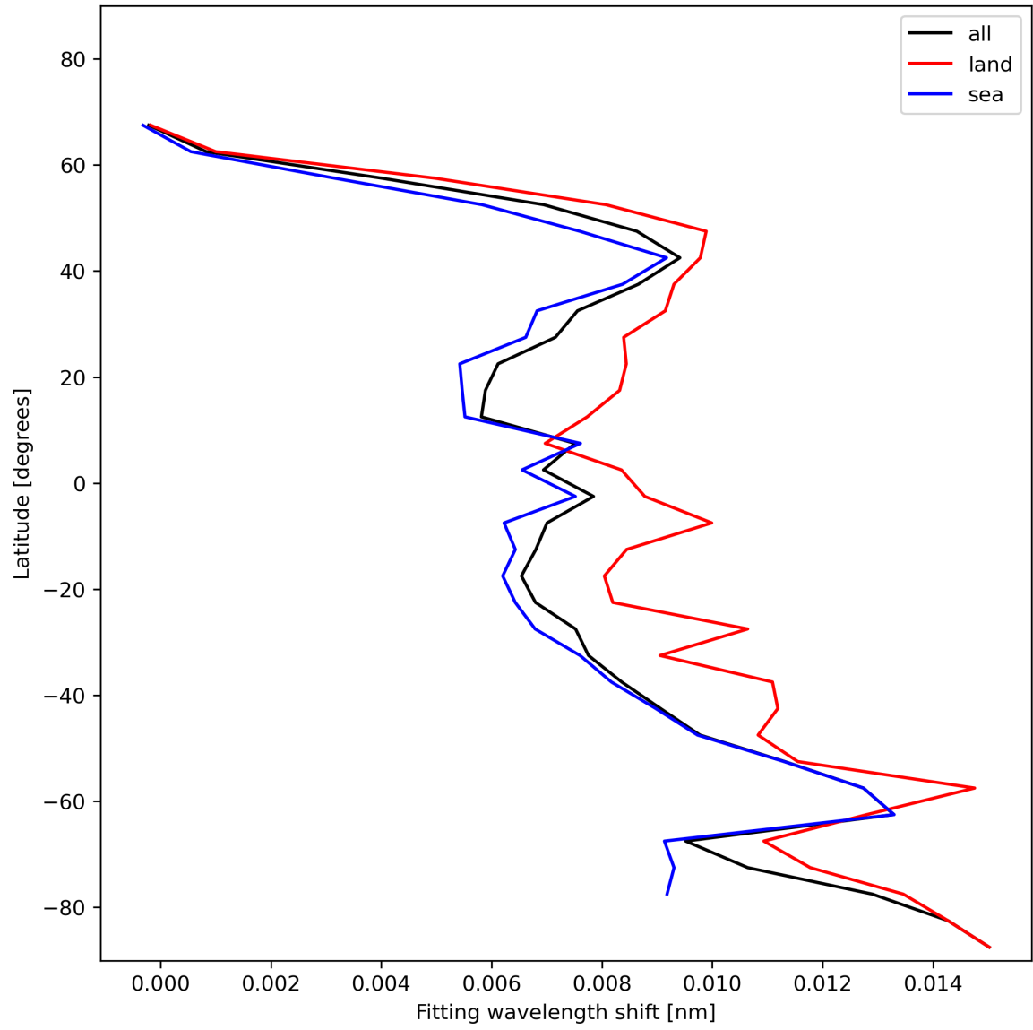
Figure 33: Zonal average of “Fitting wavelength shift” for 2023-12-23 to 2023-12-25.
