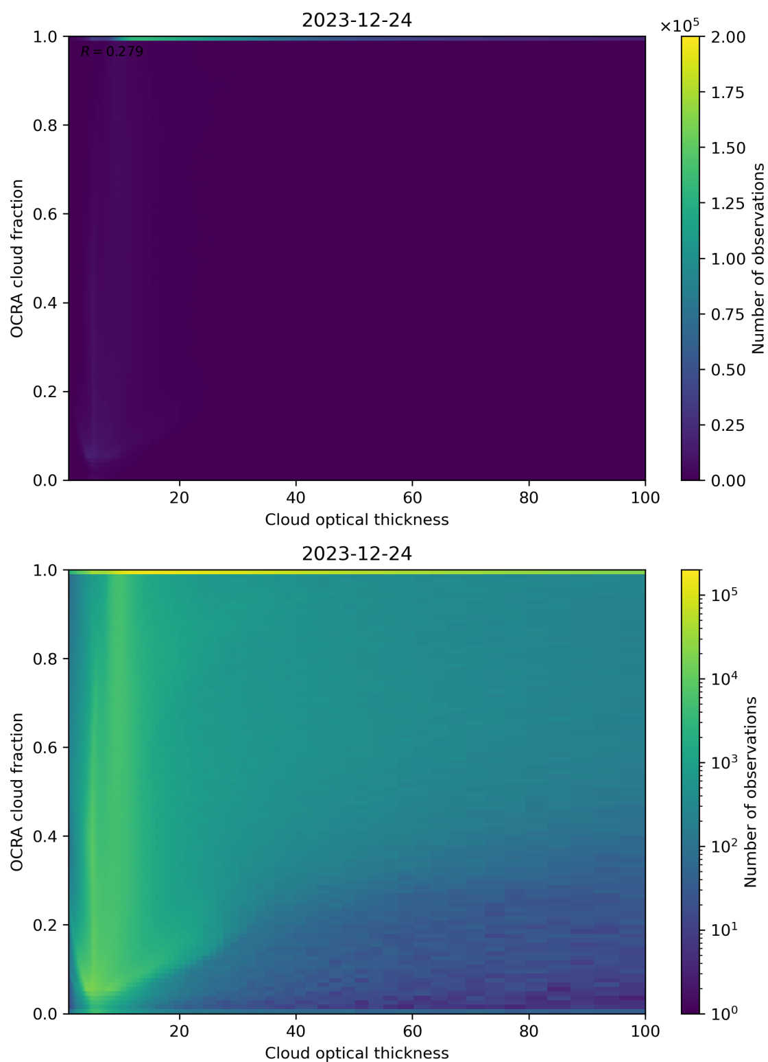
Figure 83: Scatter density plot of “Cloud optical thickness” against “OCRA cloud fraction” for 2023-12-23 to 2023-12-25.
