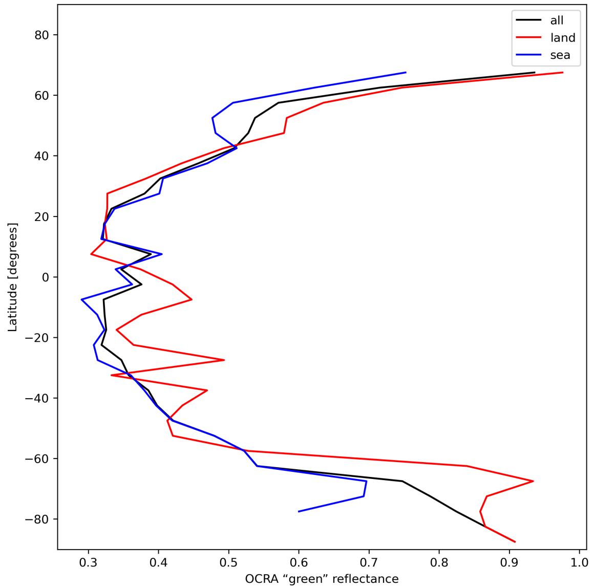
Figure 36: Zonal average of “OCRA “green” reflectance” for 2023-12-23 to 2023-12-25.
