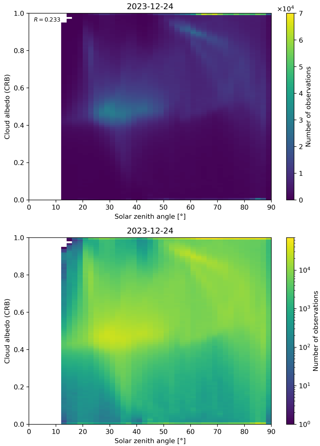
Figure 98: Scatter density plot of “Solar zenith angle” against “Cloud albedo (CRB)” for 2023-12-23 to 2023-12-25.
