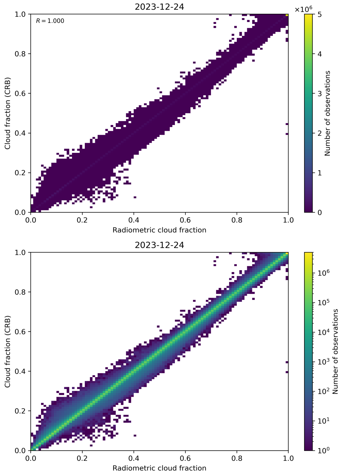
Figure 73: Scatter density plot of “Radiometric cloud fraction” against “Cloud fraction (CRB)” for 2023-12-23 to 2023-12-25.
