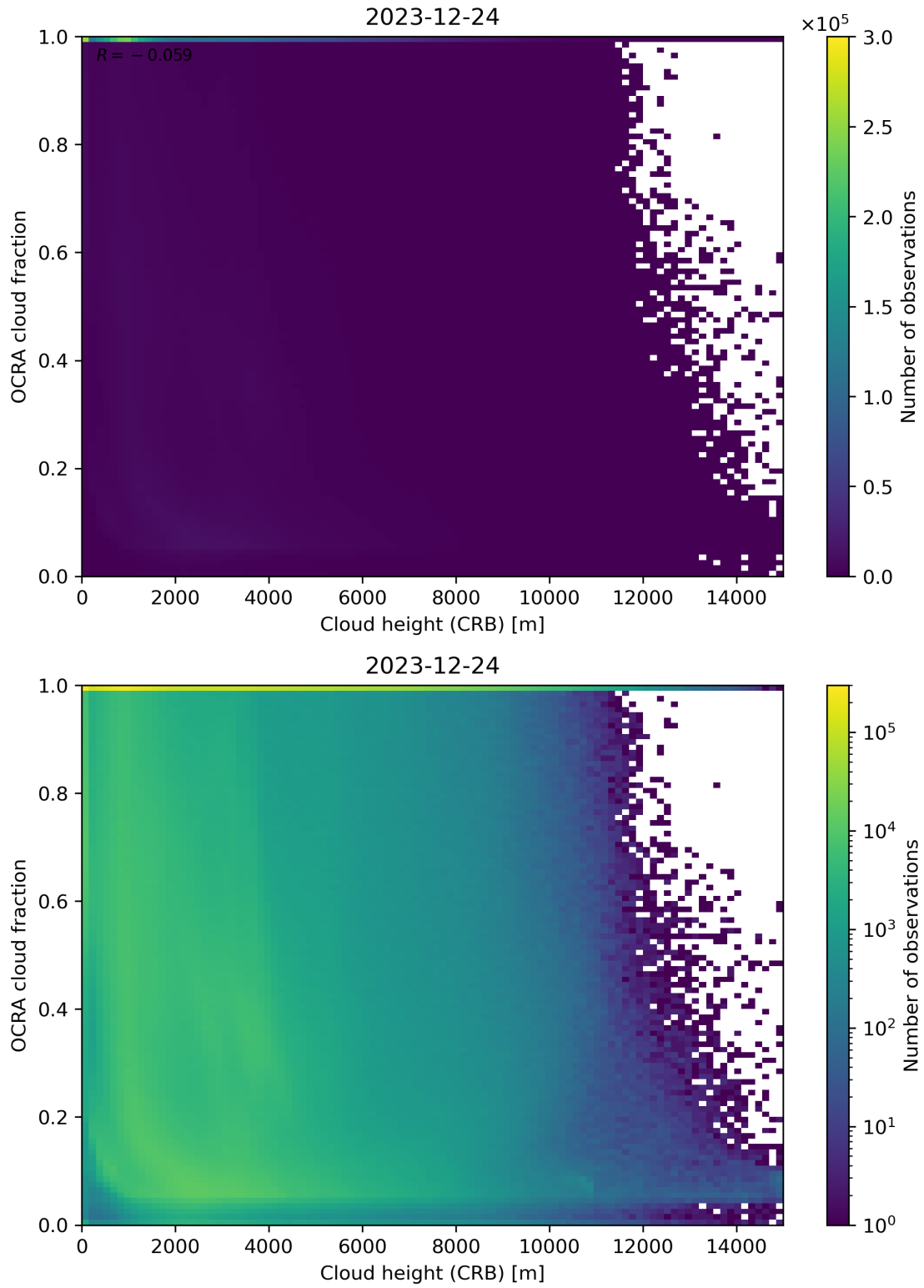
Figure 81: Scatter density plot of “Cloud height (CRB)” against “OCRA cloud fraction” for 2023-12-23 to 2023-12-25.
