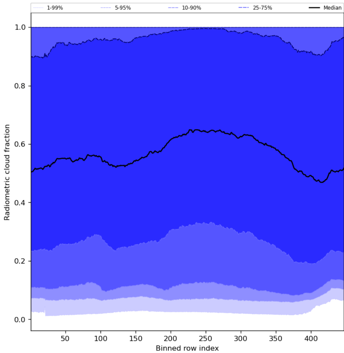
Figure 55: Along track statistics of “Radiometric cloud fraction” for 2023-12-23 to 2023-12-25
