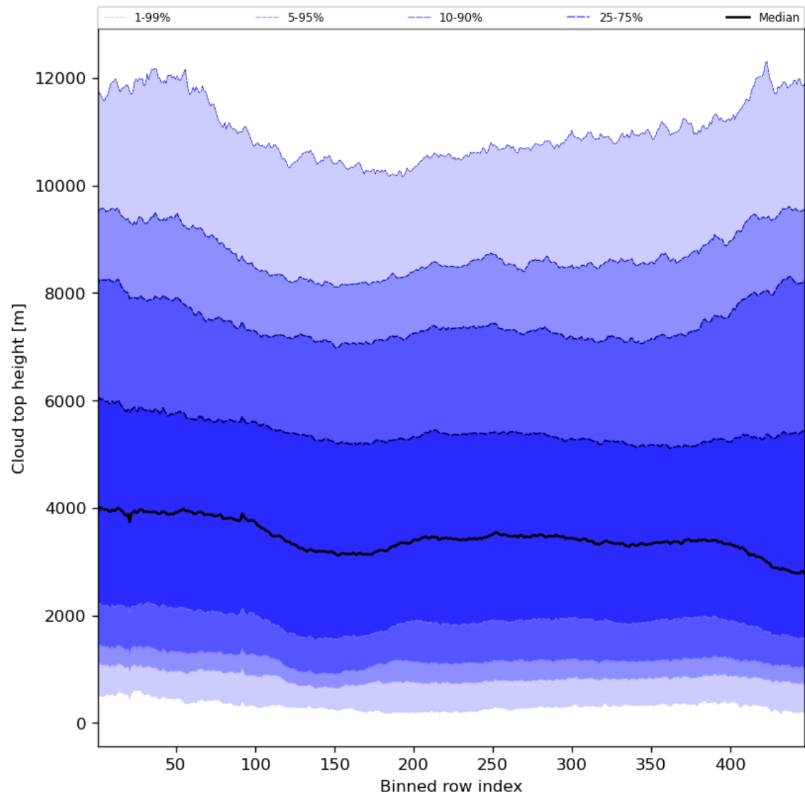
Figure 56: Along track statistics of “Cloud top height” for 2023-12-23 to 2023-12-25
