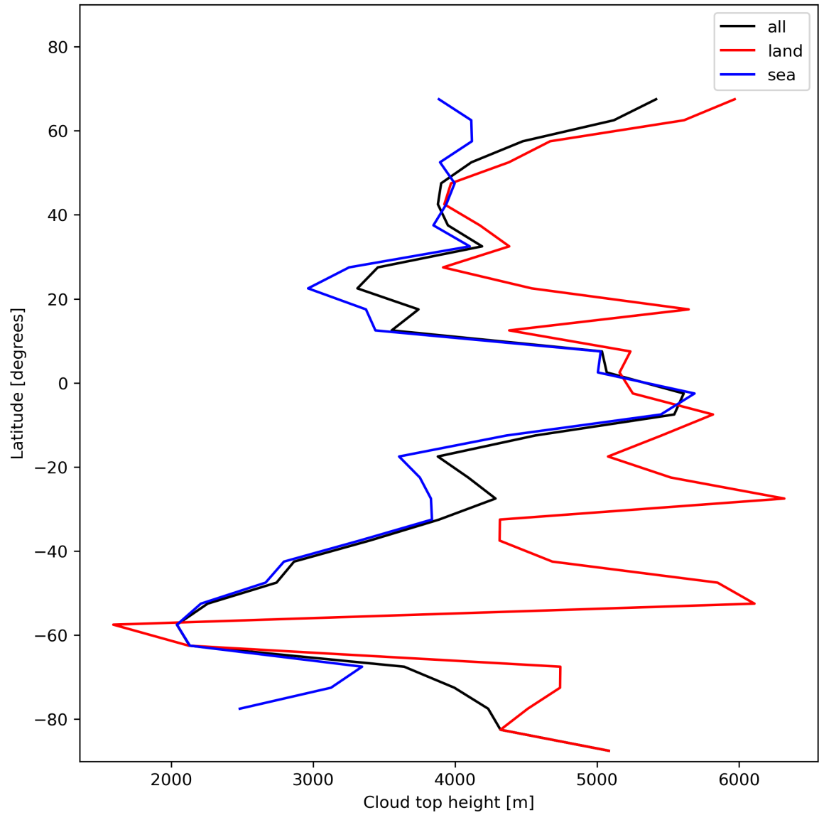
Figure 24: Zonal average of “Cloud top height” for 2023-12-23 to 2023-12-25.
