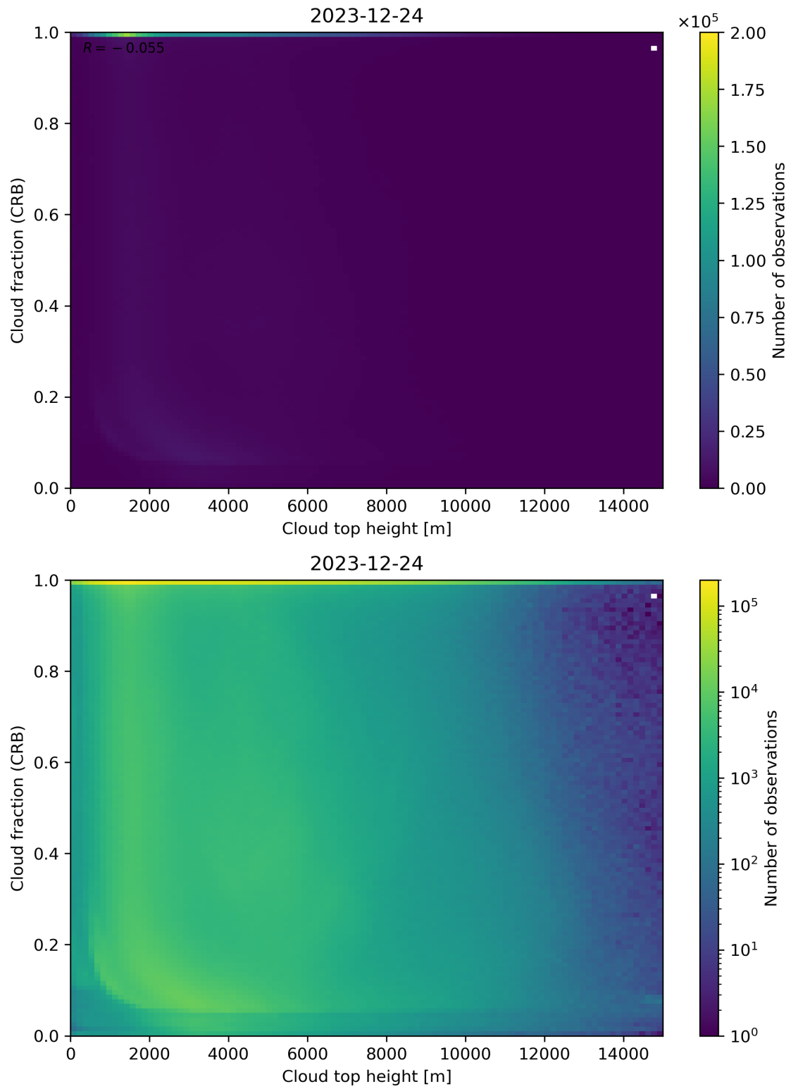
Figure 88: Scatter density plot of “Cloud top height” against “Cloud fraction (CRB)” for 2023-12-23 to 2023-12-25.
