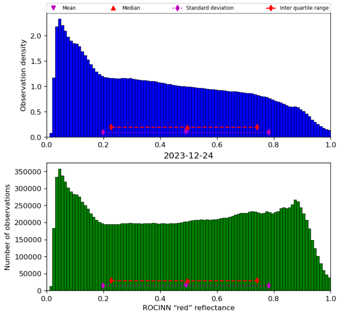
Figure 53: Histogram of “ROCINN “red” reflectance” for 2023-12-23 to 2023-12-25
