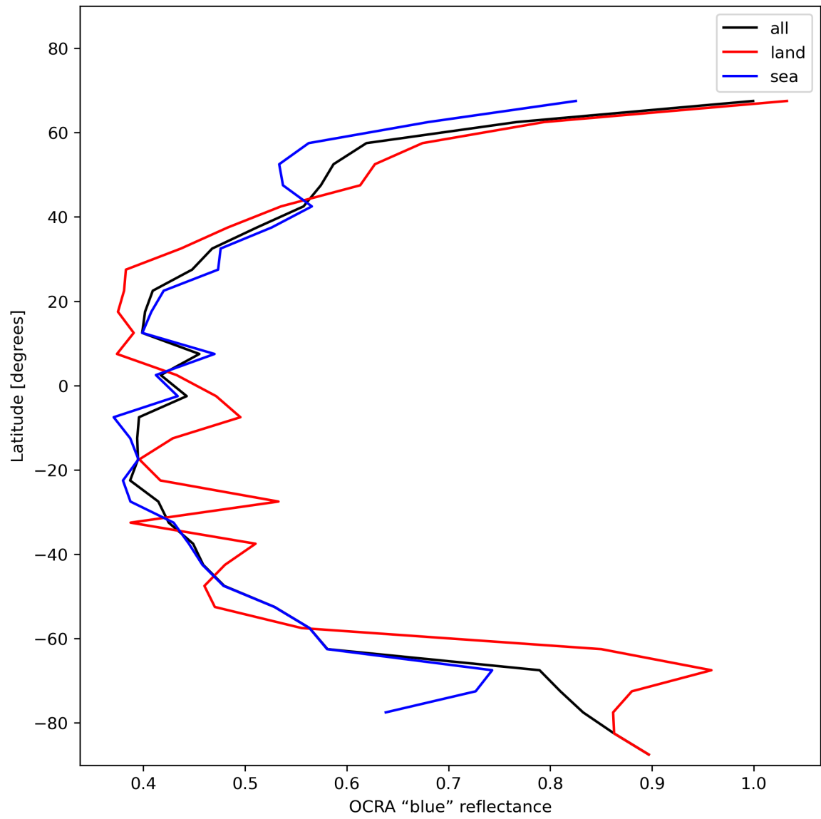
Figure 35: Zonal average of “OCRA “blue” reflectance” for 2023-12-23 to 2023-12-25.
