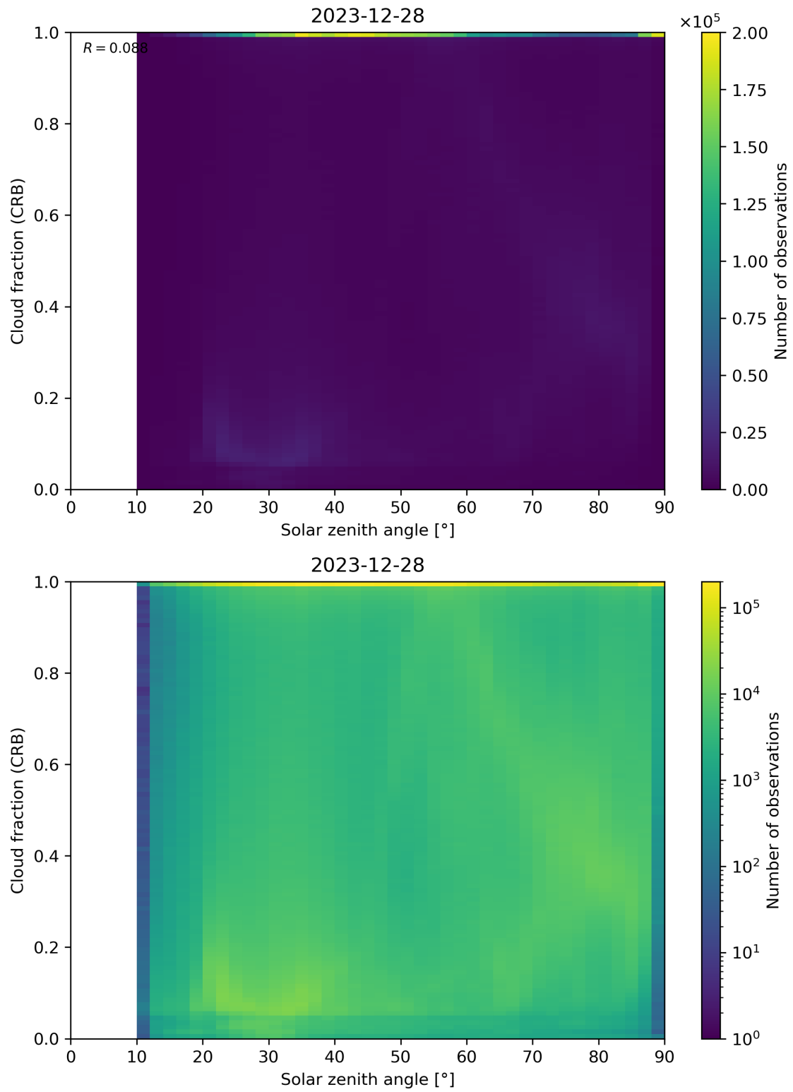
Figure 101: Scatter density plot of “Solar zenith angle” against “Cloud fraction (CRB)” for 2023-12-27 to 2023-12-29.
