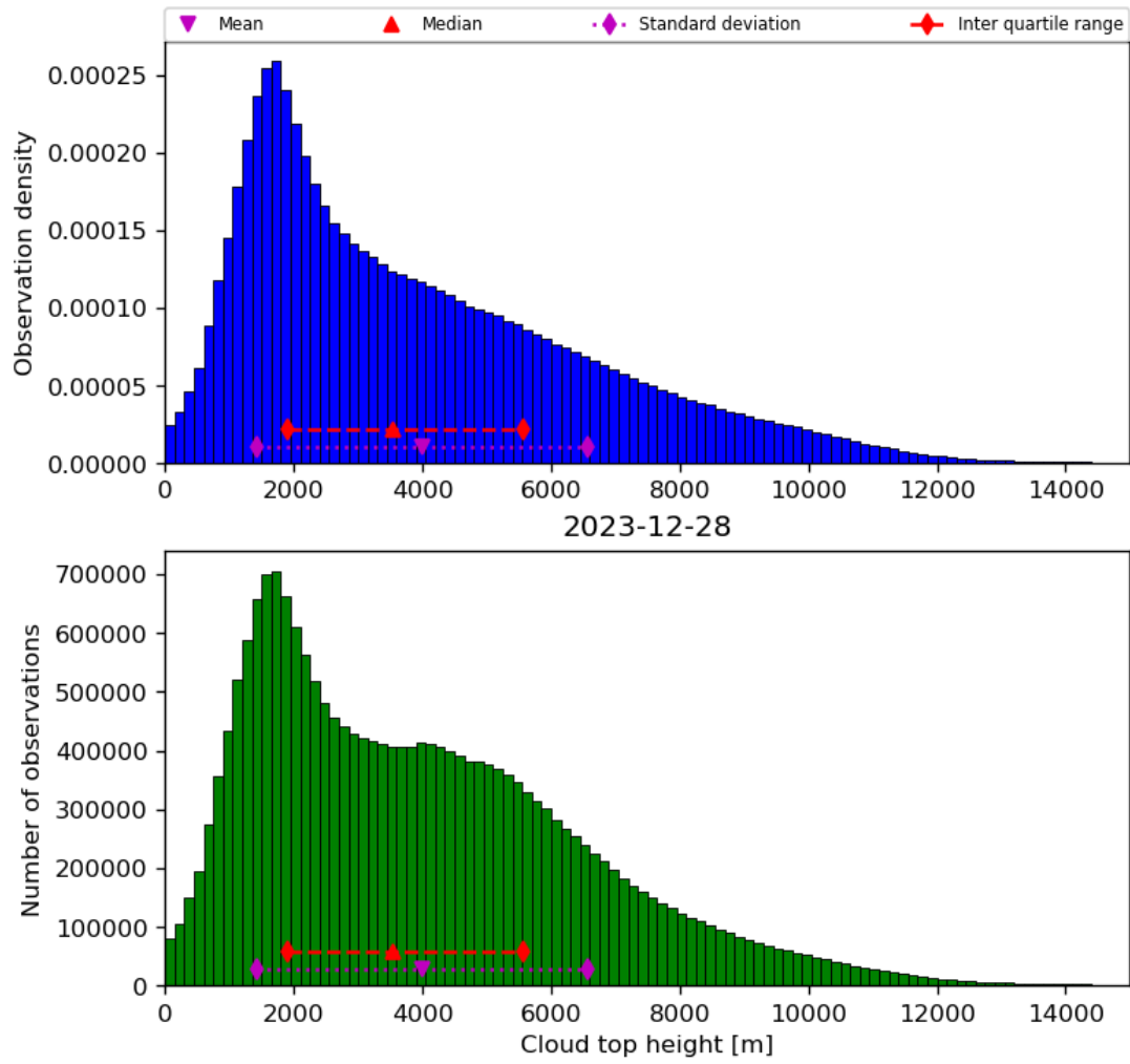
Figure 40: Histogram of “Cloud top height” for 2023-12-27 to 2023-12-29
