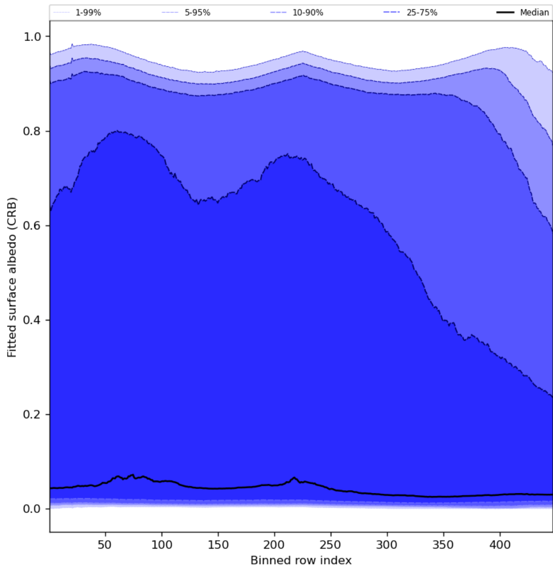
Figure 62: Along track statistics of “Fitted surface albedo (CRB)” for 2023-12-27 to 2023-12-29
