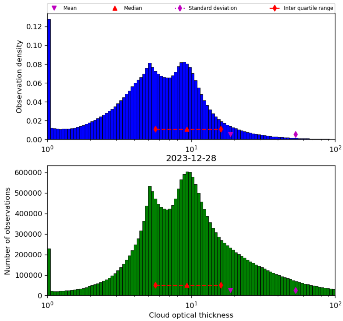
Figure 41: Histogram of “Cloud optical thickness” for 2023-12-27 to 2023-12-29
