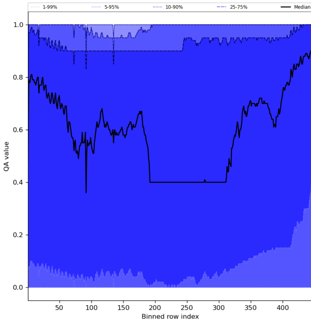
Figure 54: Along track statistics of “QA value” for 2023-12-27 to 2023-12-29
