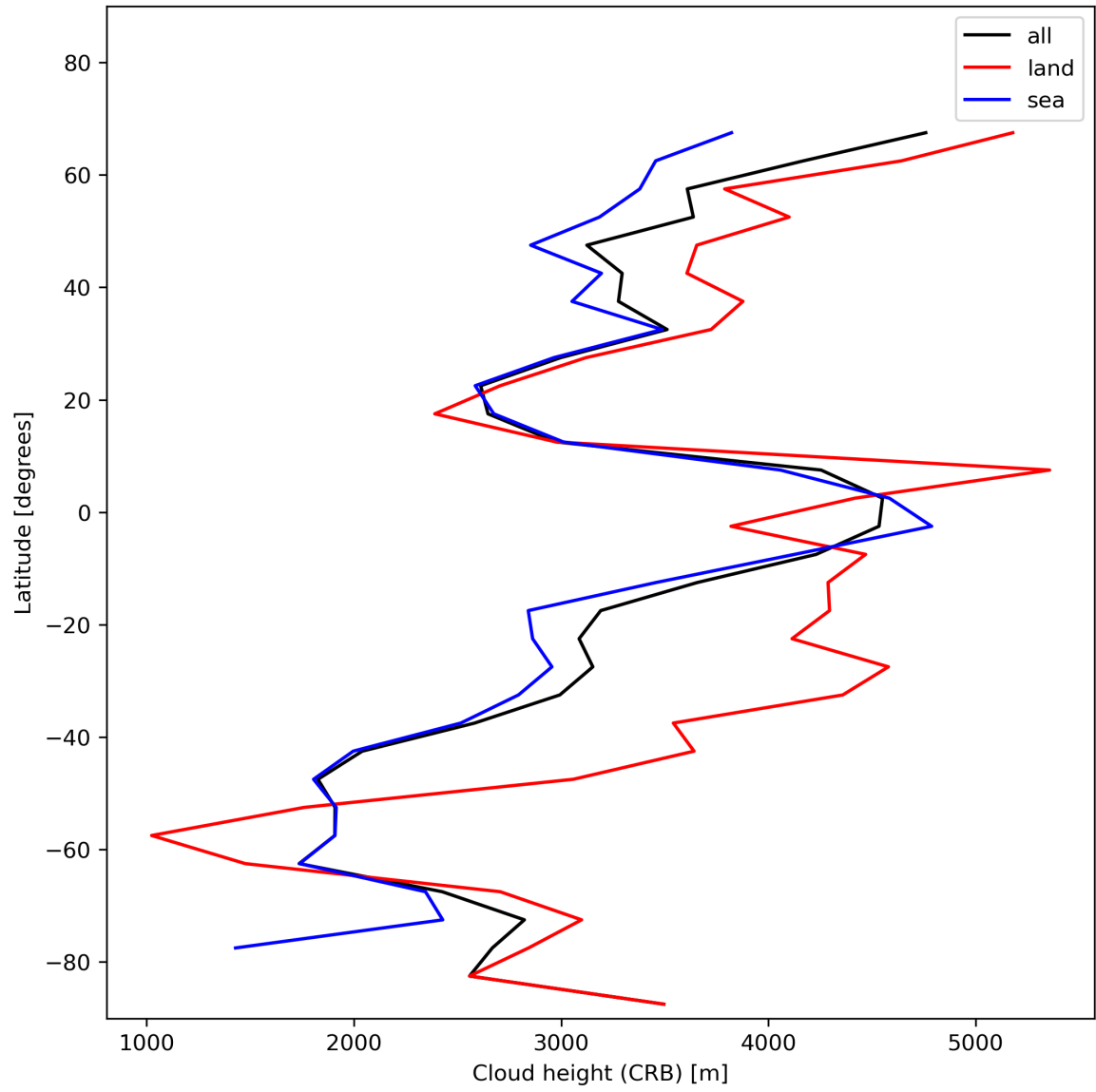
Figure 27: Zonal average of “Cloud height (CRB)” for 2023-12-27 to 2023-12-29.
