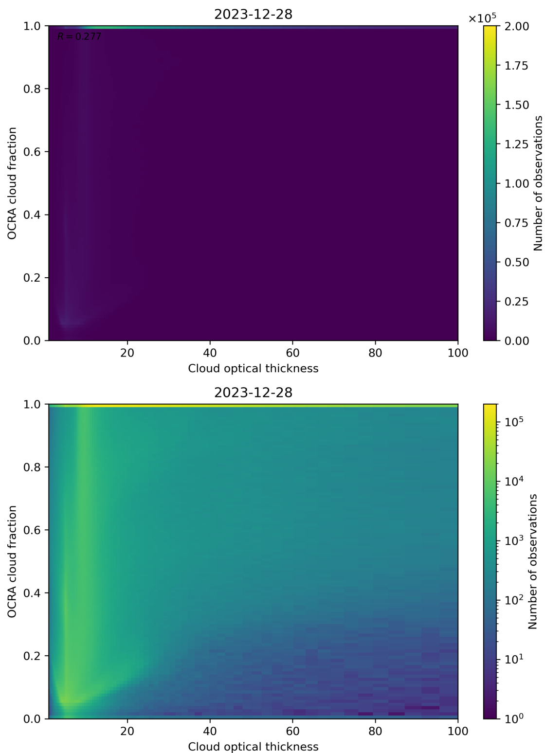
Figure 83: Scatter density plot of “Cloud optical thickness” against “OCRA cloud fraction” for 2023-12-27 to 2023-12-29.
