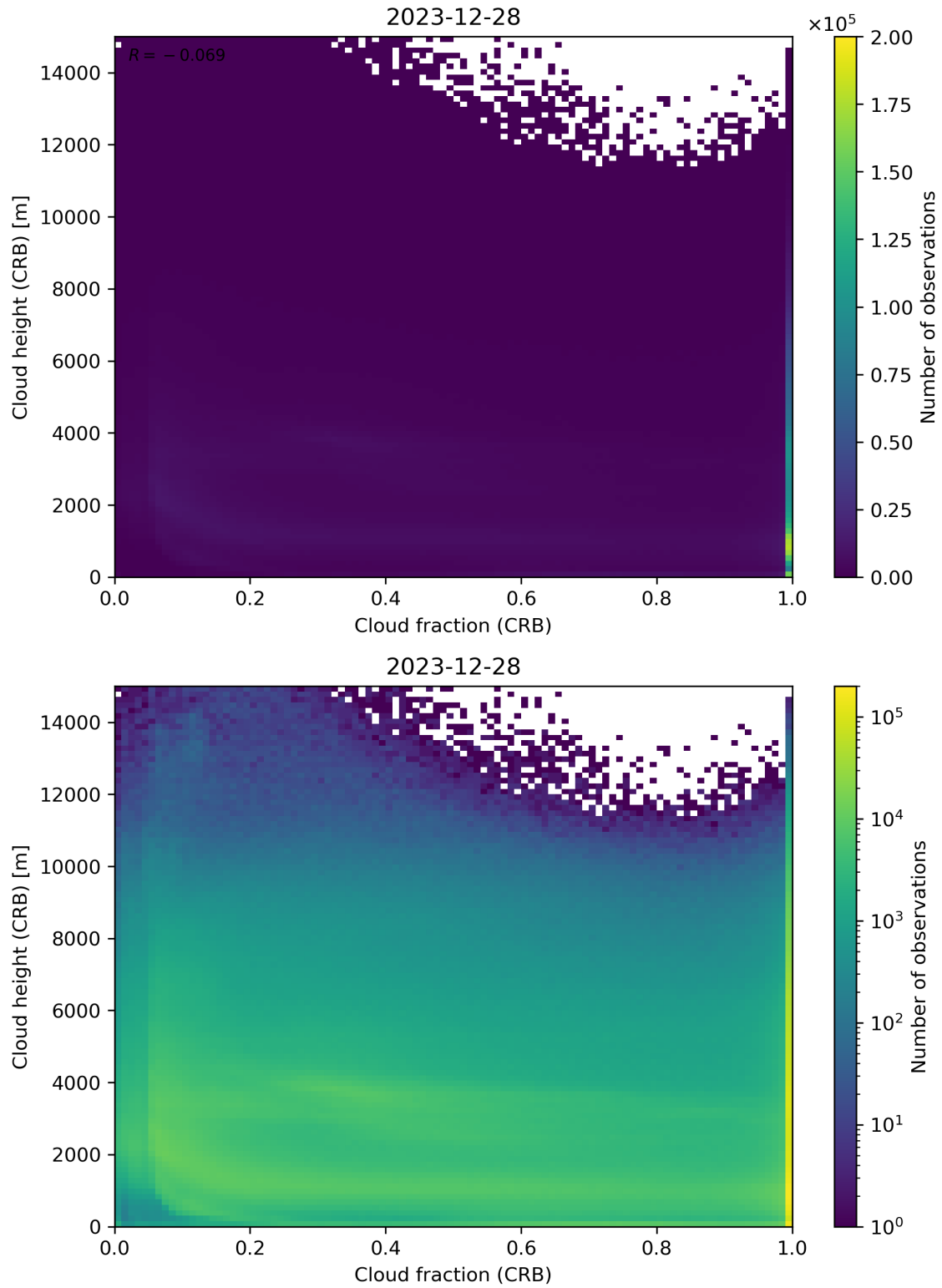
Figure 79: Scatter density plot of “Cloud fraction (CRB)” against “Cloud height (CRB)” for 2023-12-27 to 2023-12-29.
