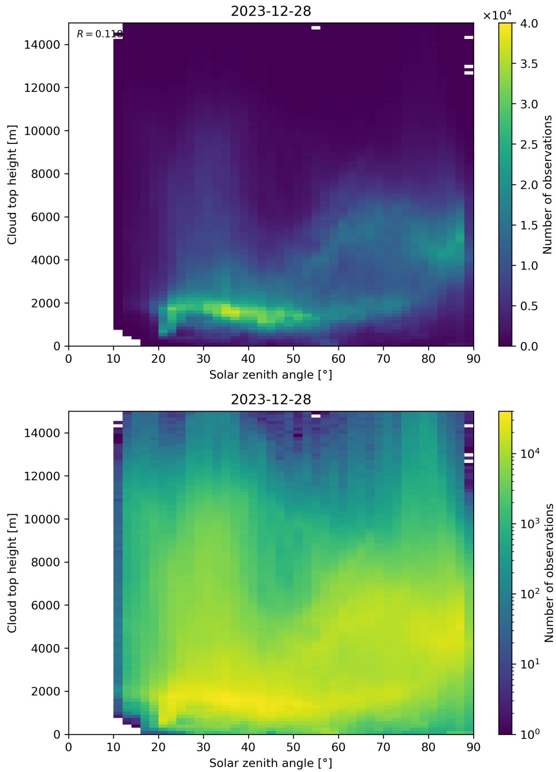
Figure 104: Scatter density plot of “Solar zenith angle” against “Cloud top height” for 2023-12-27 to 2023-12-29.
