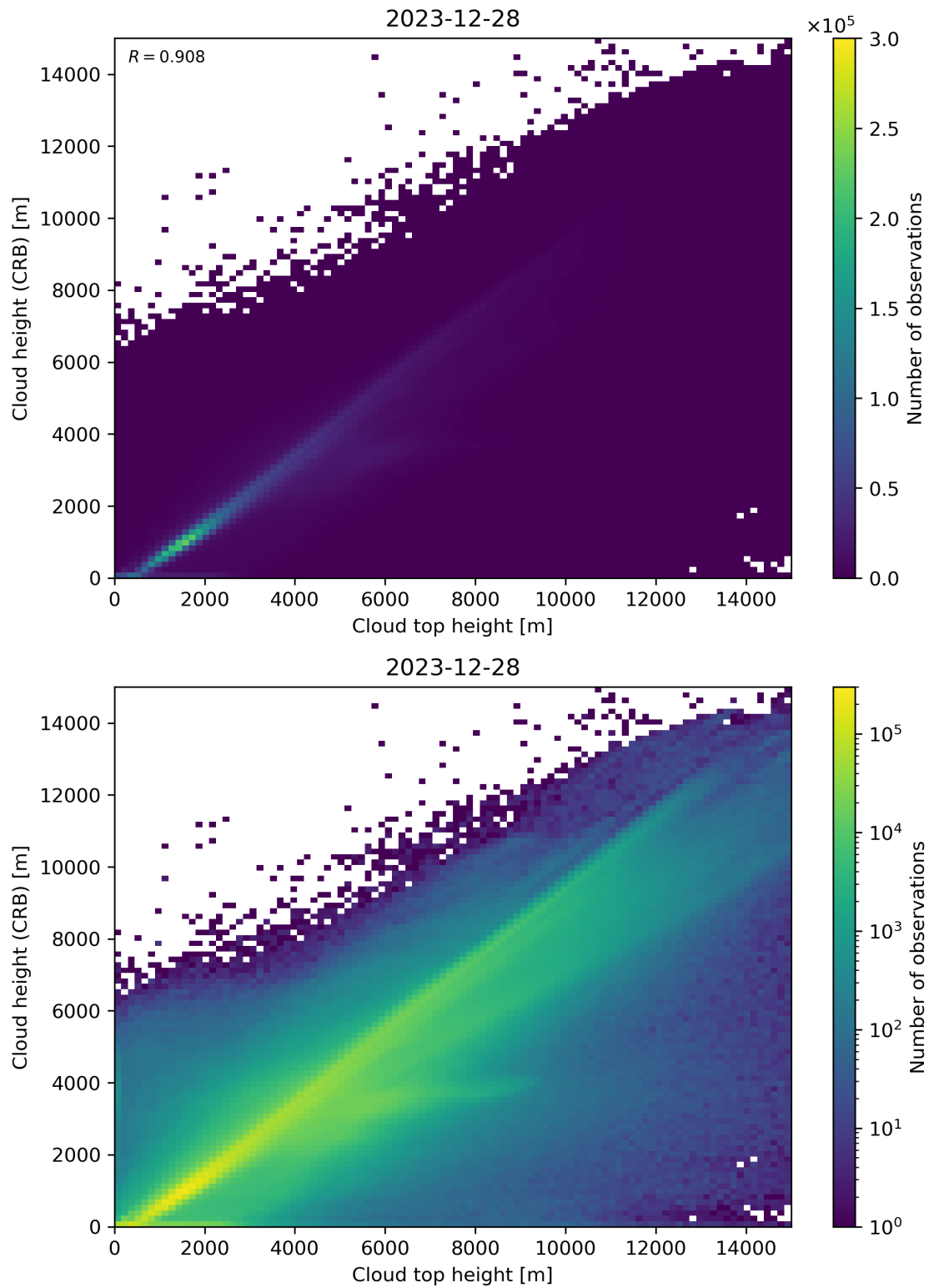
Figure 89: Scatter density plot of “Cloud top height” against “Cloud height (CRB)” for 2023-12-27 to 2023-12-29.
