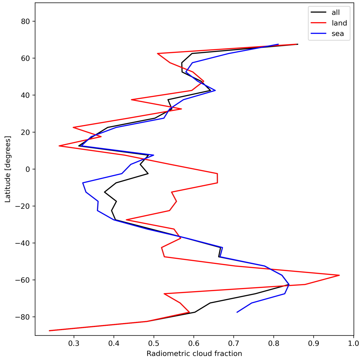
Figure 23: Zonal average of “Radiometric cloud fraction” for 2023-12-27 to 2023-12-29.
