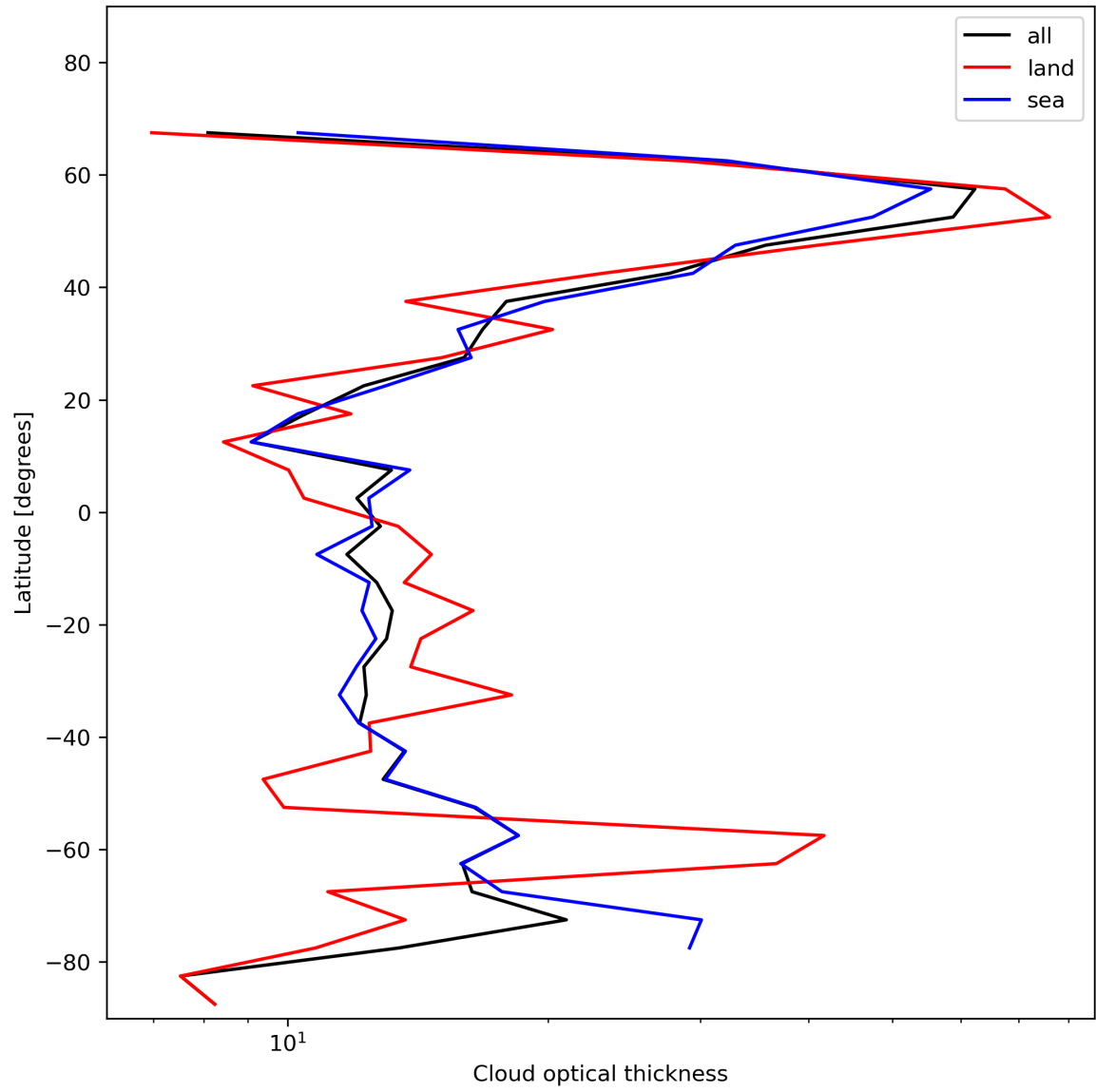
Figure 25: Zonal average of “Cloud optical thickness” for 2023-12-27 to 2023-12-29.
