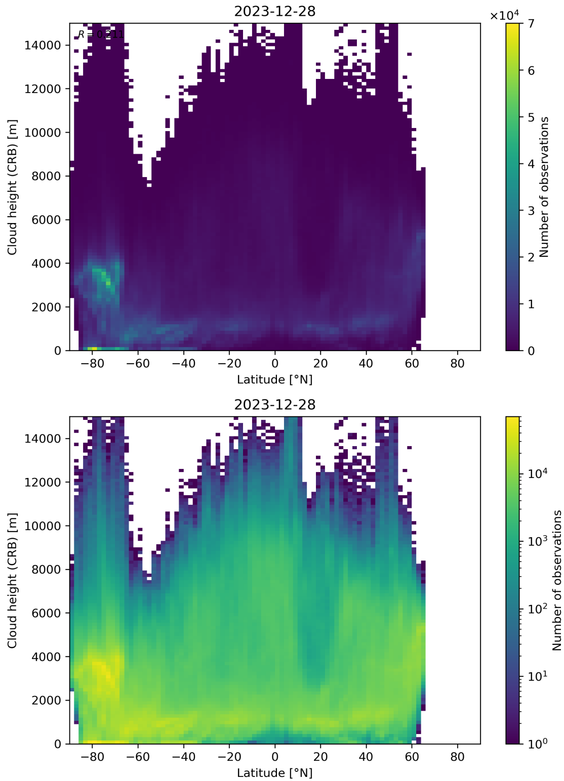
Figure 95: Scatter density plot of “Latitude” against “Cloud height (CRB)” for 2023-12-27 to 2023-12-29.
