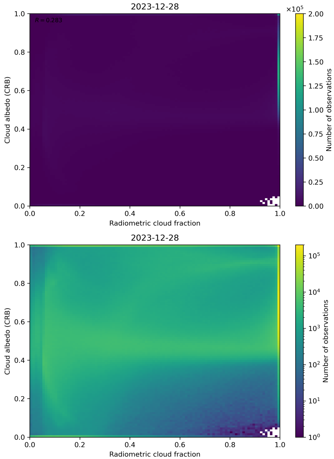
Figure 71: Scatter density plot of “Radiometric cloud fraction” against “Cloud albedo (CRB)” for 2023-12-27 to 2023-12-29.
