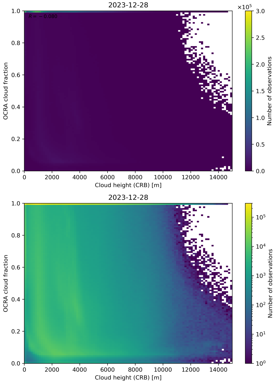
Figure 81: Scatter density plot of “Cloud height (CRB)” against “OCRA cloud fraction” for 2023-12-27 to 2023-12-29.
