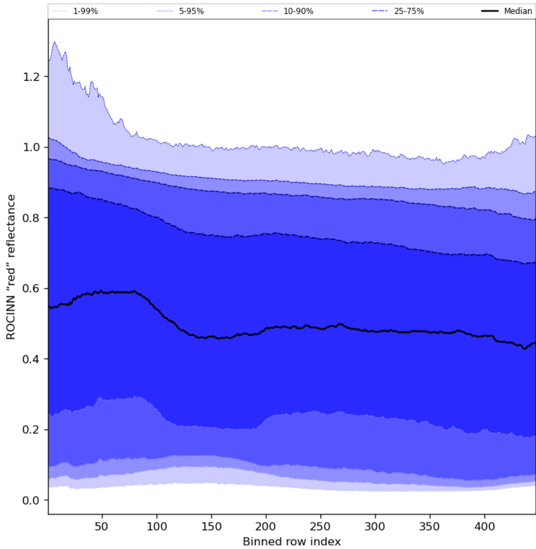
Figure 69: Along track statistics of “ROCINN “red” reflectance” for 2023-12-27 to 2023-12-29
