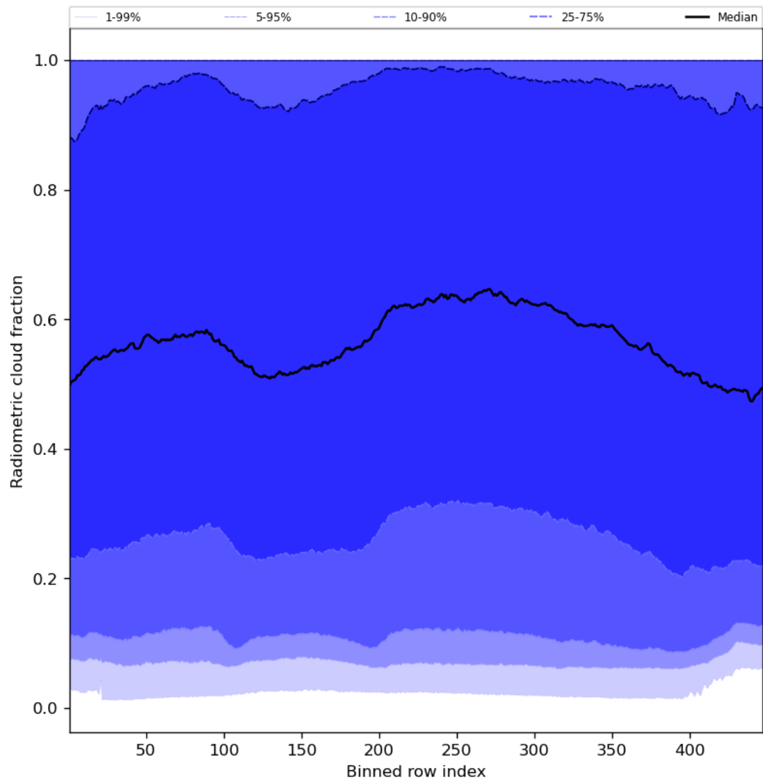
Figure 55: Along track statistics of “Radiometric cloud fraction” for 2023-12-27 to 2023-12-29
