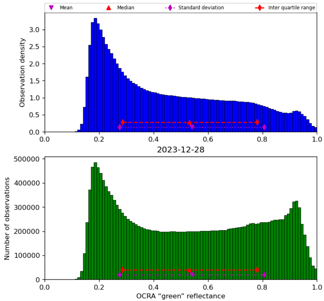
Figure 52: Histogram of “OCRA “green” reflectance” for 2023-12-27 to 2023-12-29
