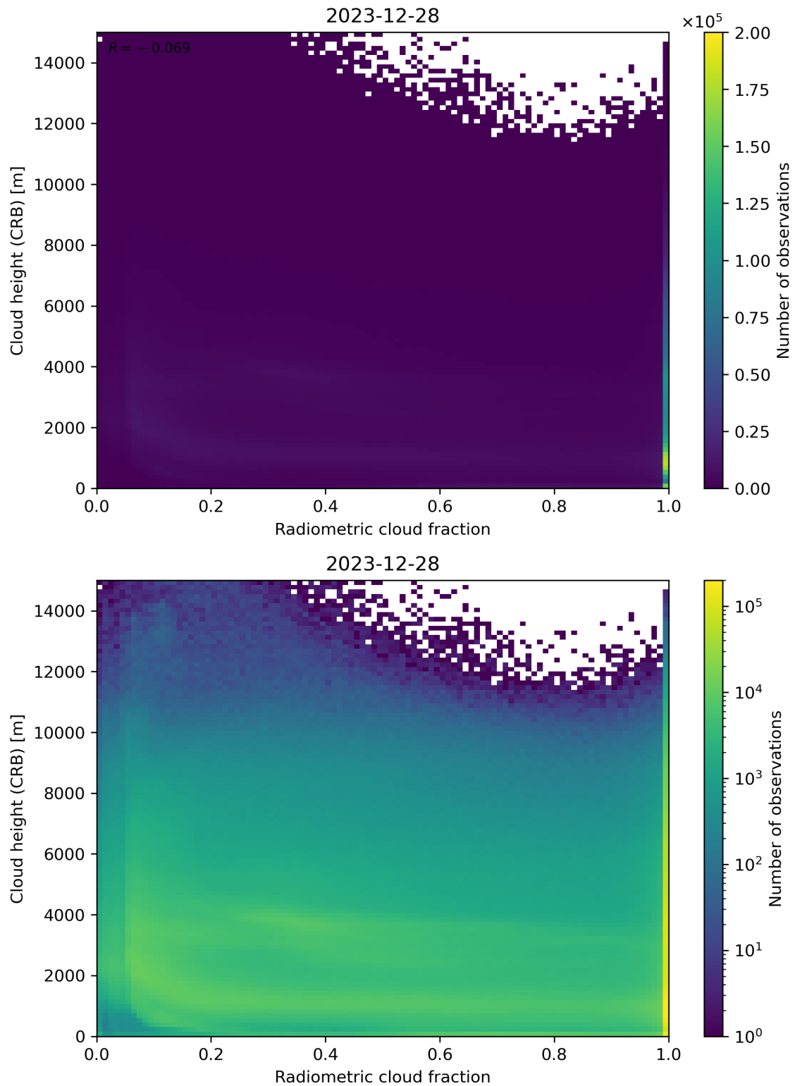
Figure 74: Scatter density plot of “Radiometric cloud fraction” against “Cloud height (CRB)” for 2023-12-27 to 2023-12-29.
