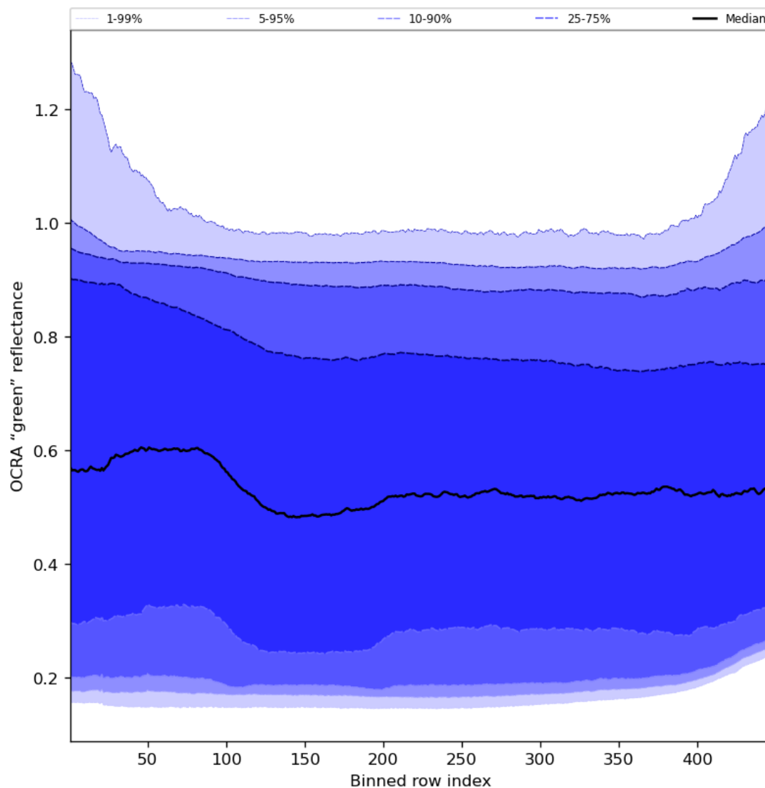
Figure 68: Along track statistics of “OCRA “green” reflectance” for 2023-12-27 to 2023-12-29
