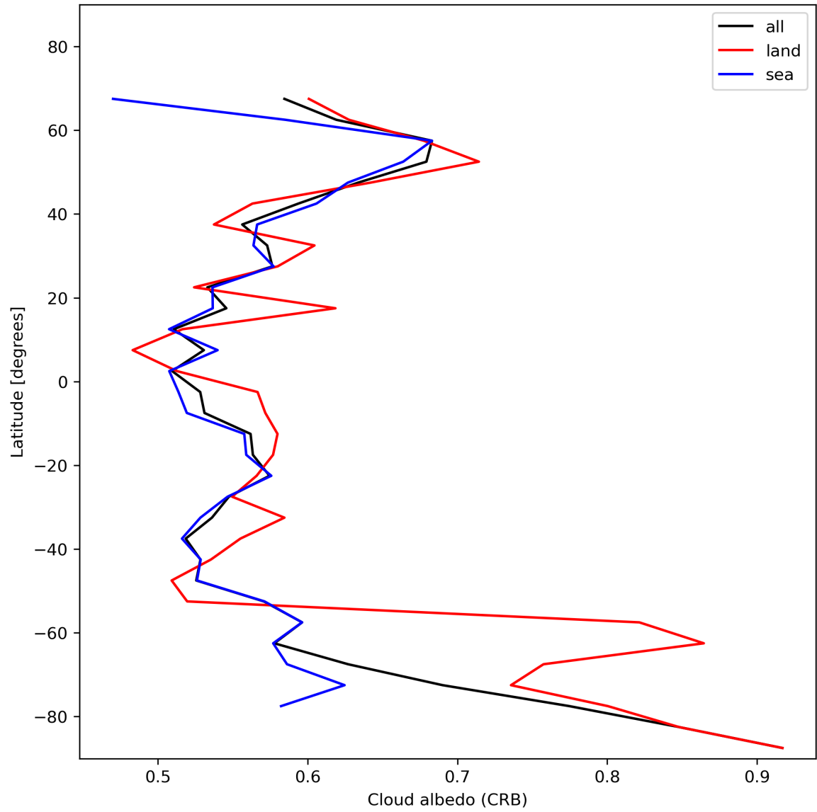
Figure 28: Zonal average of “Cloud albedo (CRB)” for 2023-12-27 to 2023-12-29.
