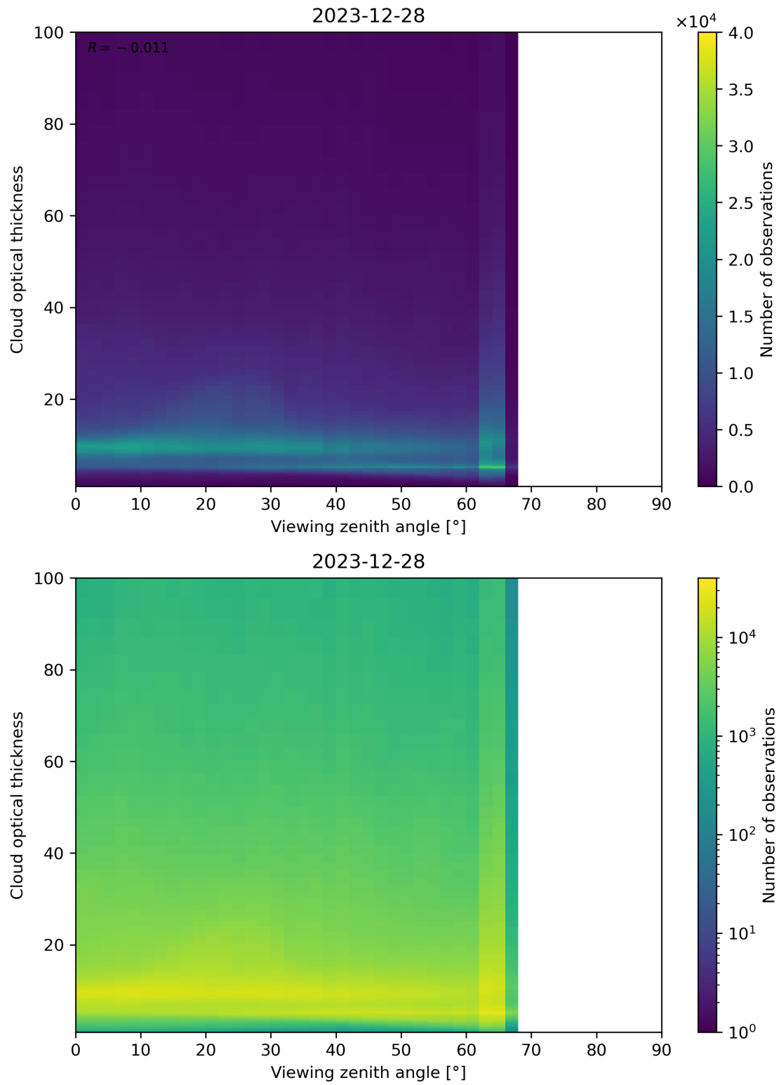
Figure 111: Scatter density plot of “Viewing zenith angle” against “Cloud optical thickness” for 2023-12-27 to 2023-12-29.
