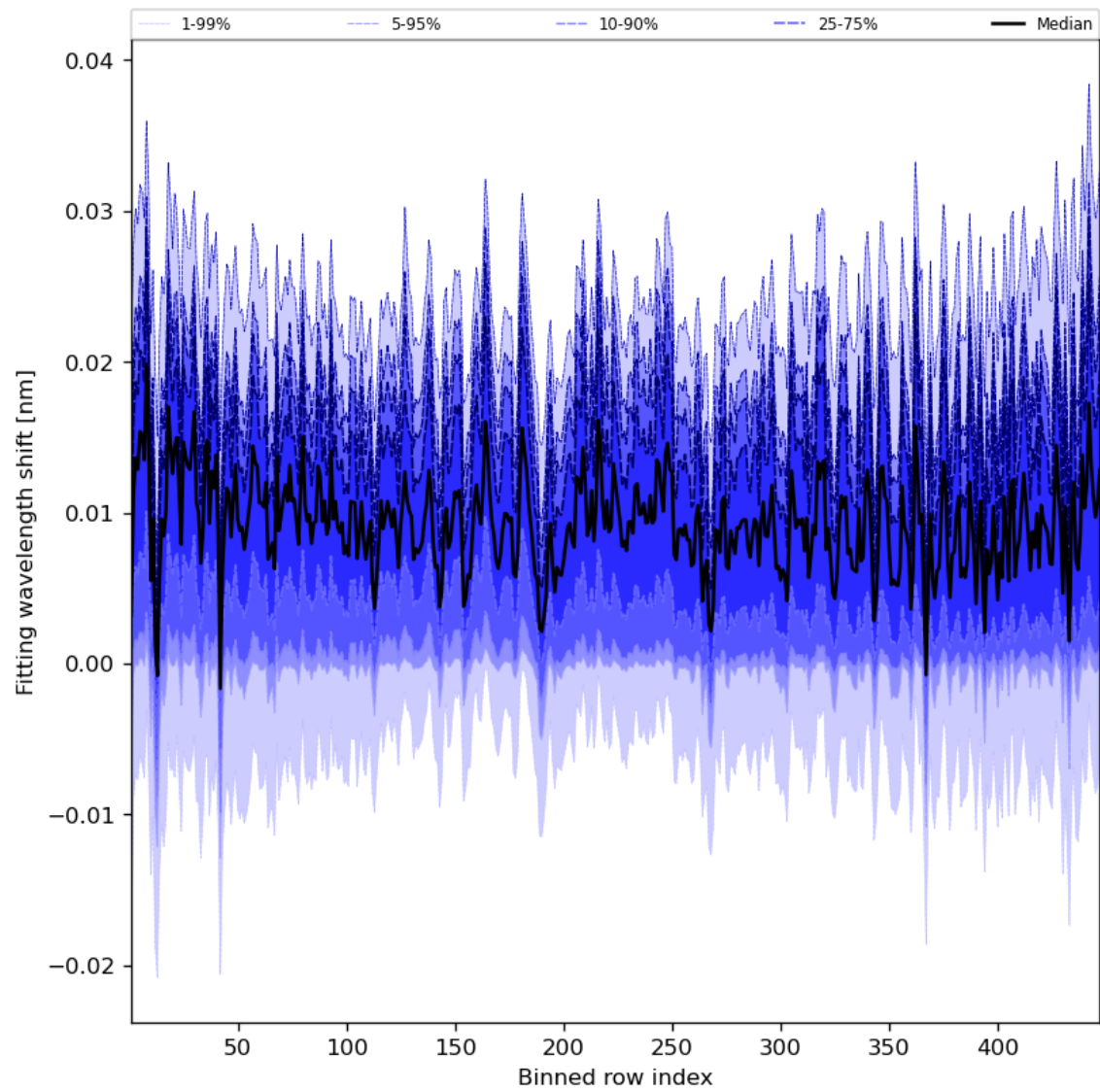
Figure 65: Along track statistics of “Fitting wavelength shift” for 2023-12-27 to 2023-12-29
