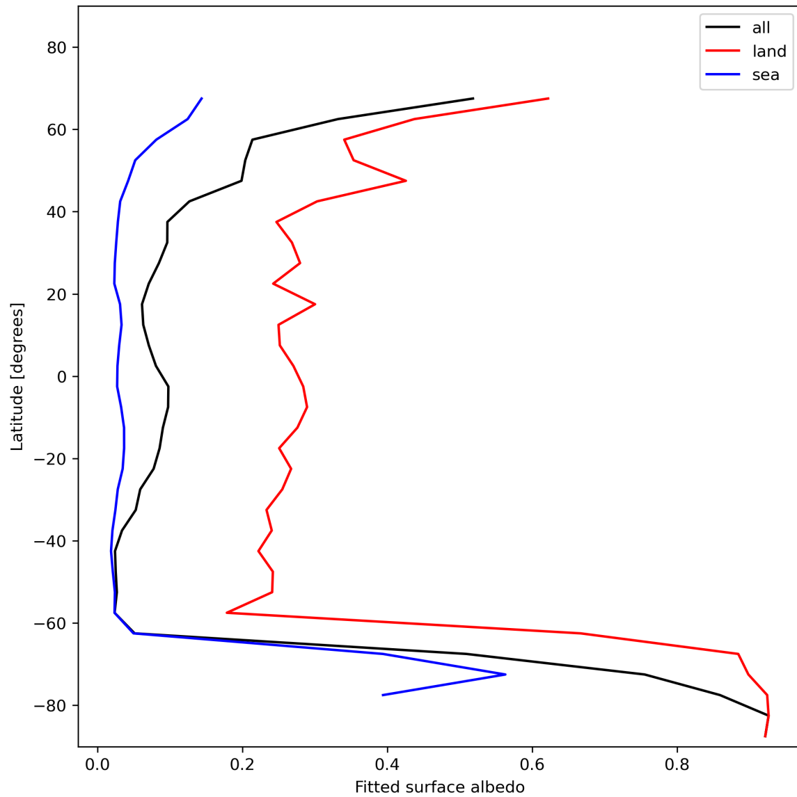
Figure 29: Zonal average of “Fitted surface albedo” for 2023-12-27 to 2023-12-29.
