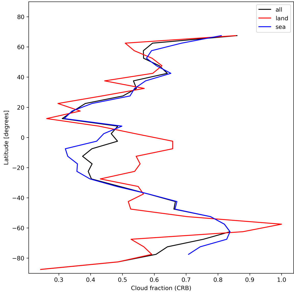
Figure 26: Zonal average of “Cloud fraction (CRB)” for 2023-12-27 to 2023-12-29.
