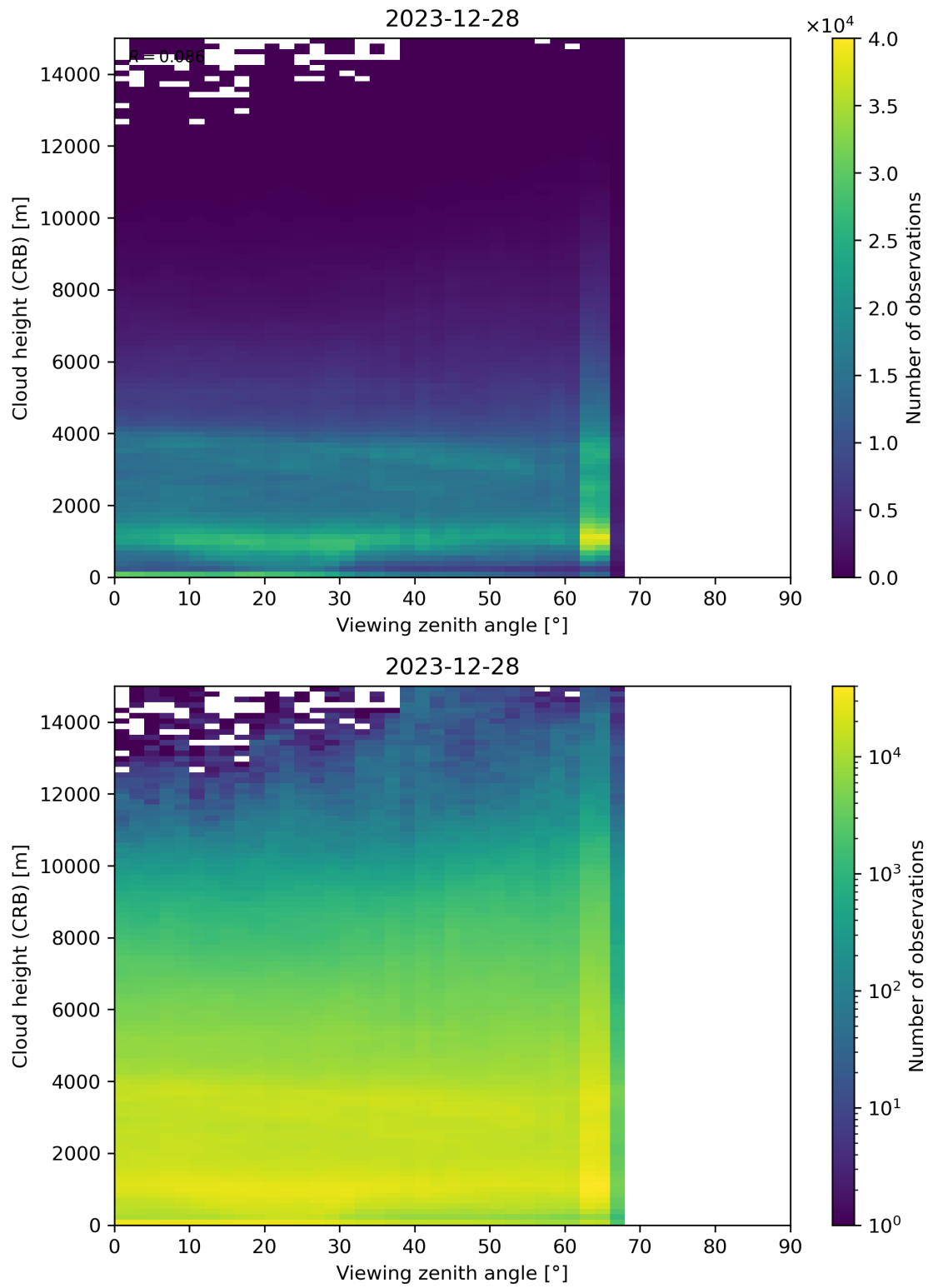
Figure 110: Scatter density plot of “Viewing zenith angle” against “Cloud height (CRB)” for 2023-12-27 to 2023-12-29.
