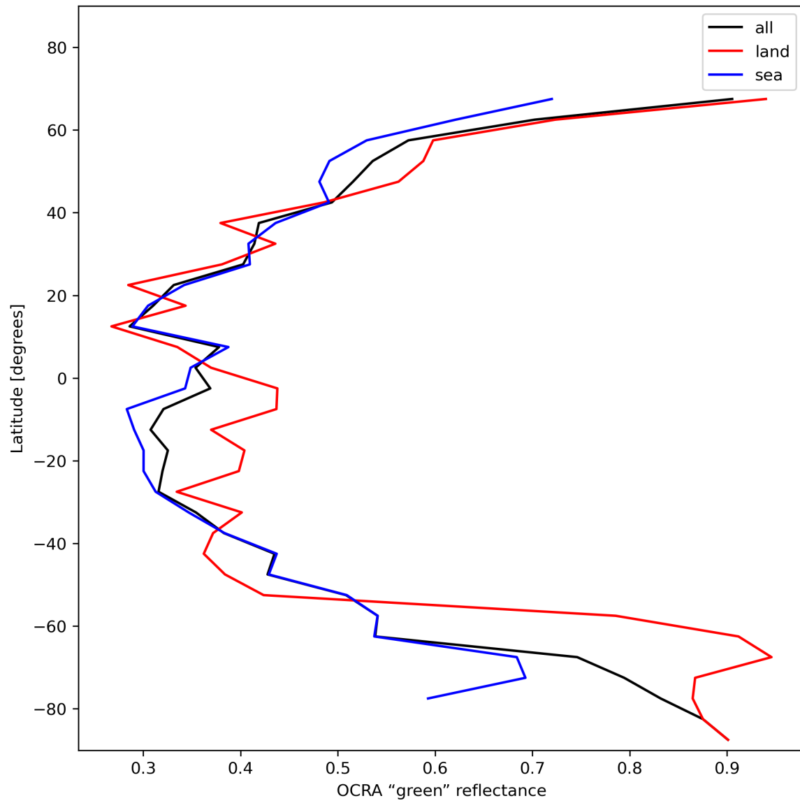
Figure 36: Zonal average of “OCRA “green” reflectance” for 2023-12-27 to 2023-12-29.
