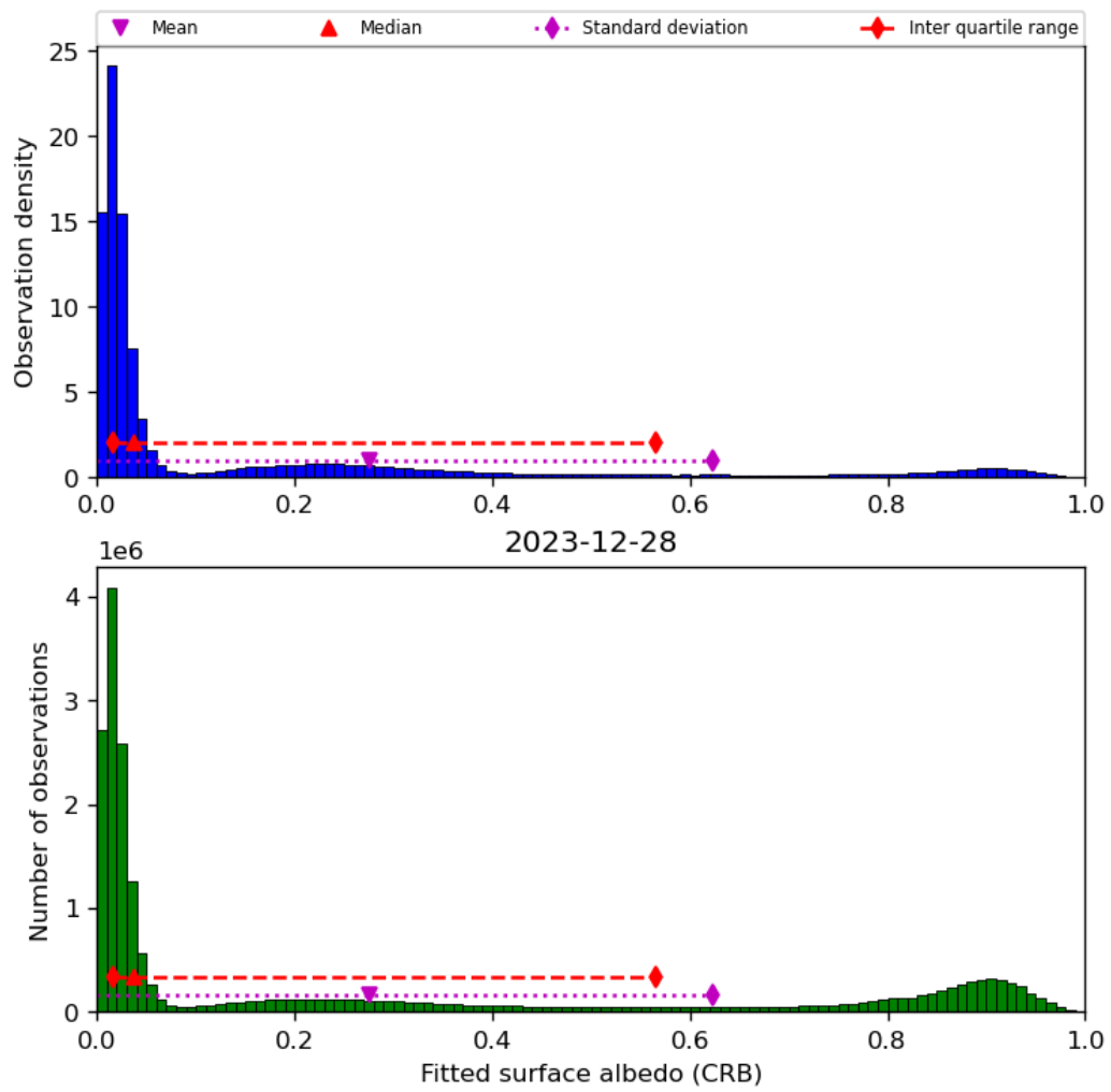
Figure 46: Histogram of “Fitted surface albedo (CRB)” for 2023-12-27 to 2023-12-29
