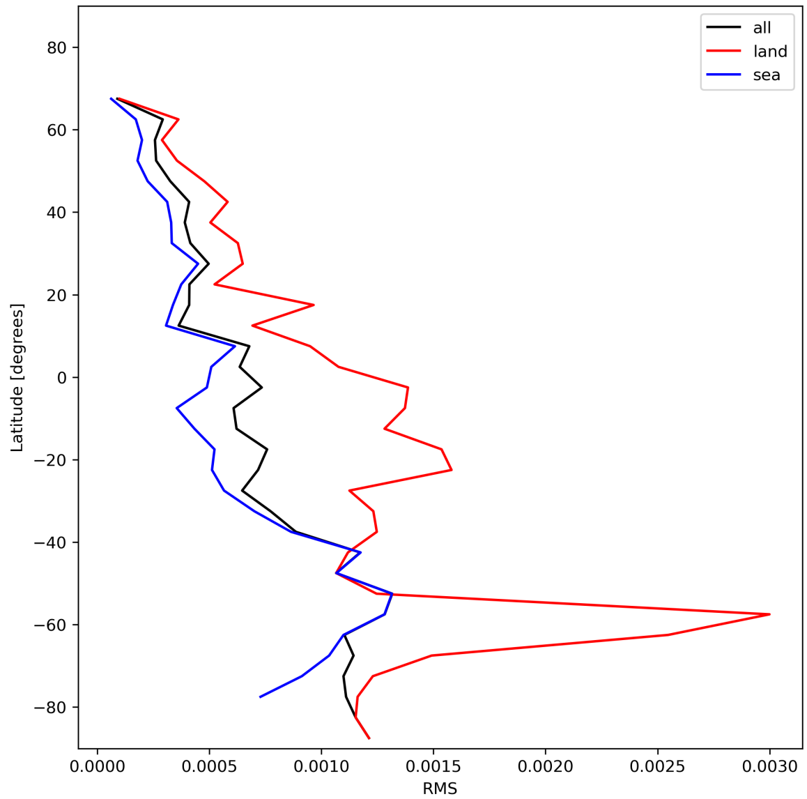
Figure 31: Zonal average of “RMS” for 2023-12-27 to 2023-12-29.
