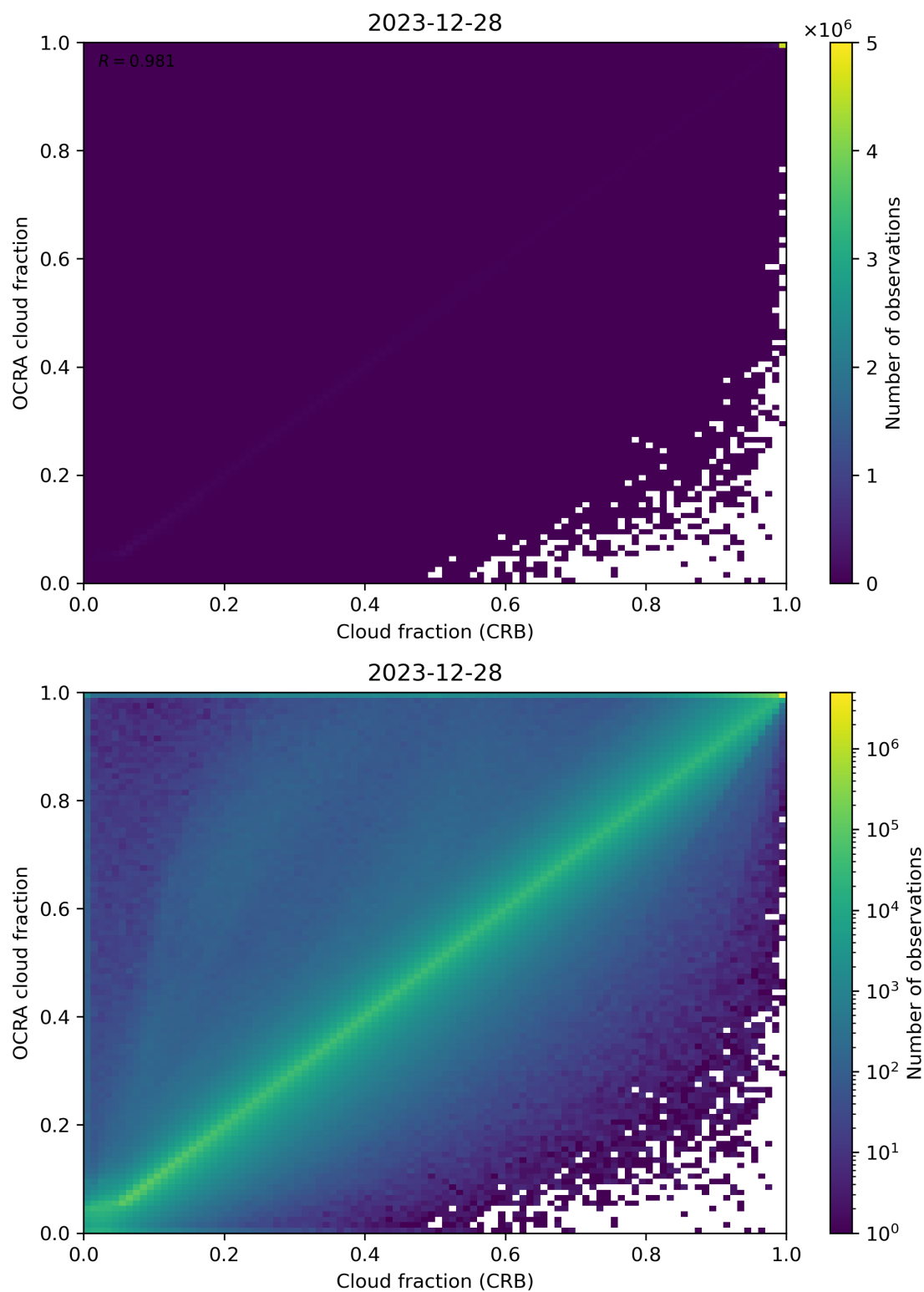
Figure 78: Scatter density plot of “Cloud fraction (CRB)” against “OCRA cloud fraction” for 2023-12-27 to 2023-12-29.
