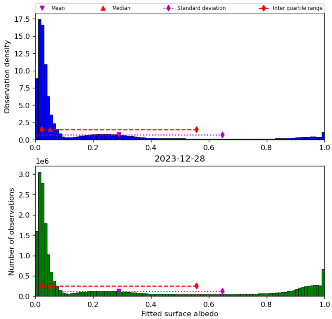
Figure 45: Histogram of “Fitted surface albedo” for 2023-12-27 to 2023-12-29
