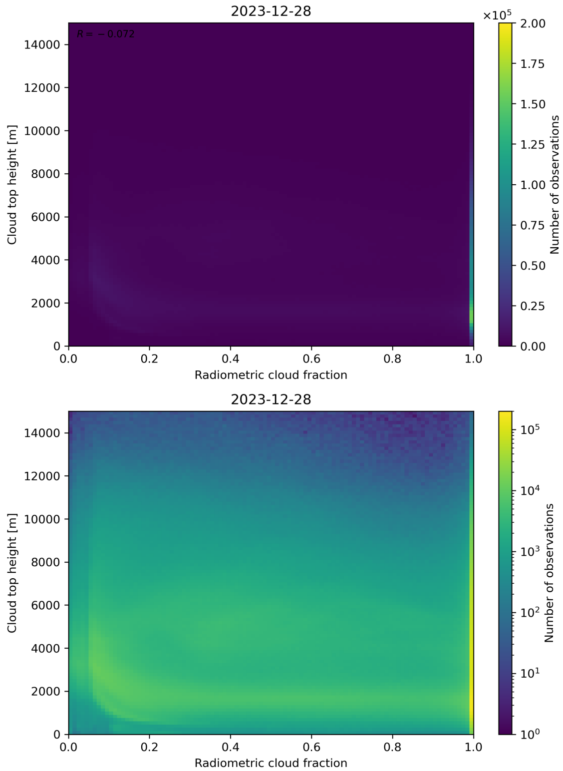
Figure 76: Scatter density plot of “Radiometric cloud fraction” against “Cloud top height” for 2023-12-27 to 2023-12-29.
