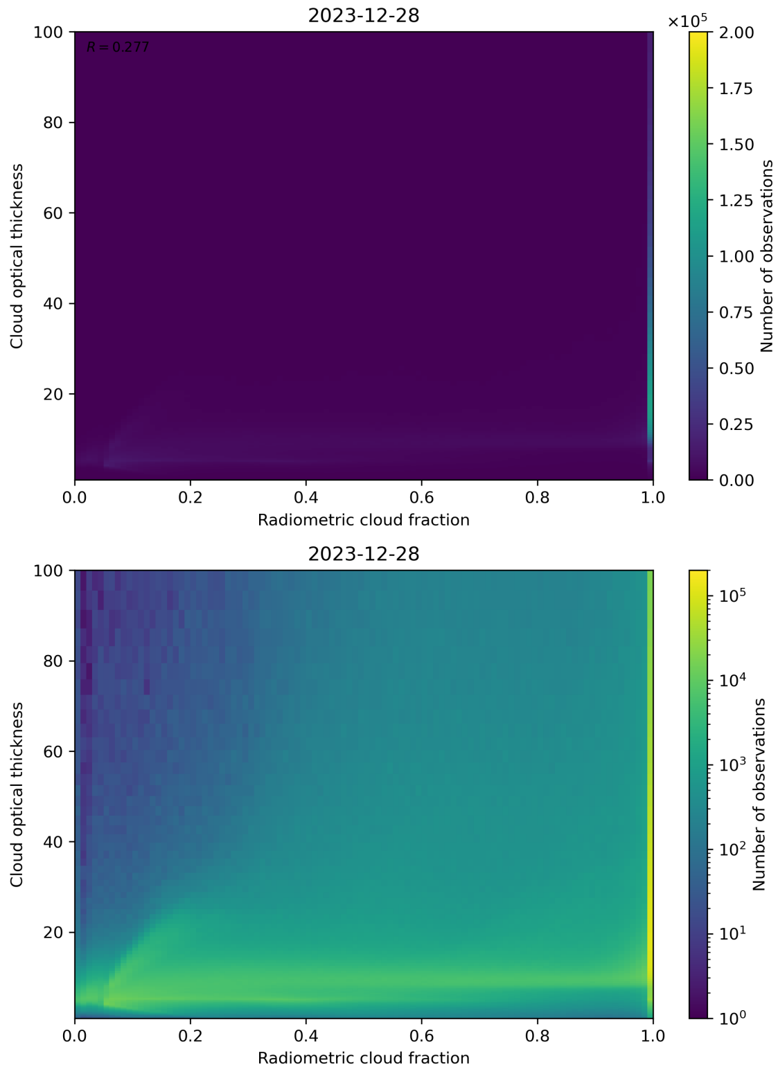
Figure 75: Scatter density plot of “Radiometric cloud fraction” against “Cloud optical thickness” for 2023-12-27 to 2023-12-29.
