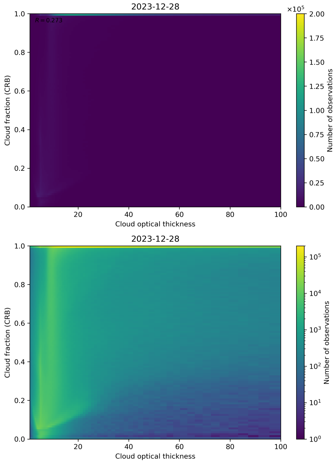
Figure 84: Scatter density plot of “Cloud optical thickness” against “Cloud fraction (CRB)” for 2023-12-27 to 2023-12-29.
