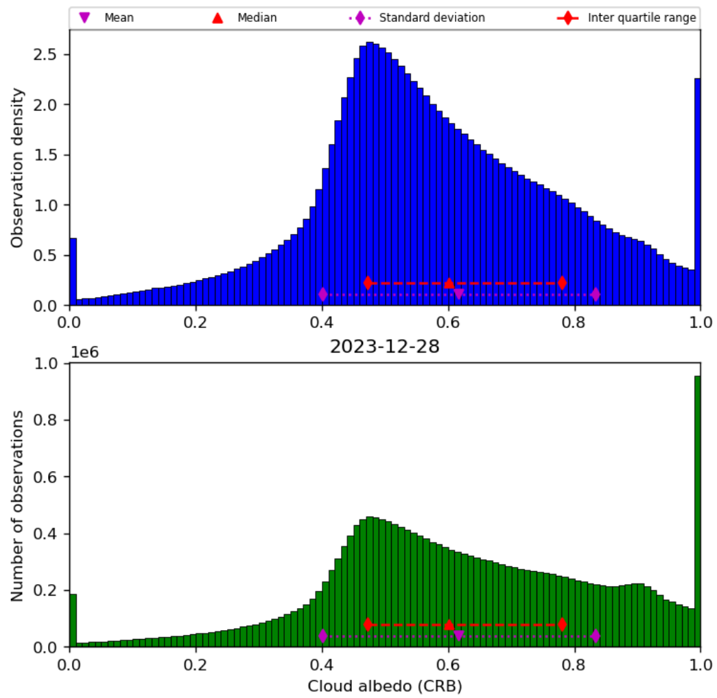
Figure 44: Histogram of “Cloud albedo (CRB)” for 2023-12-27 to 2023-12-29
