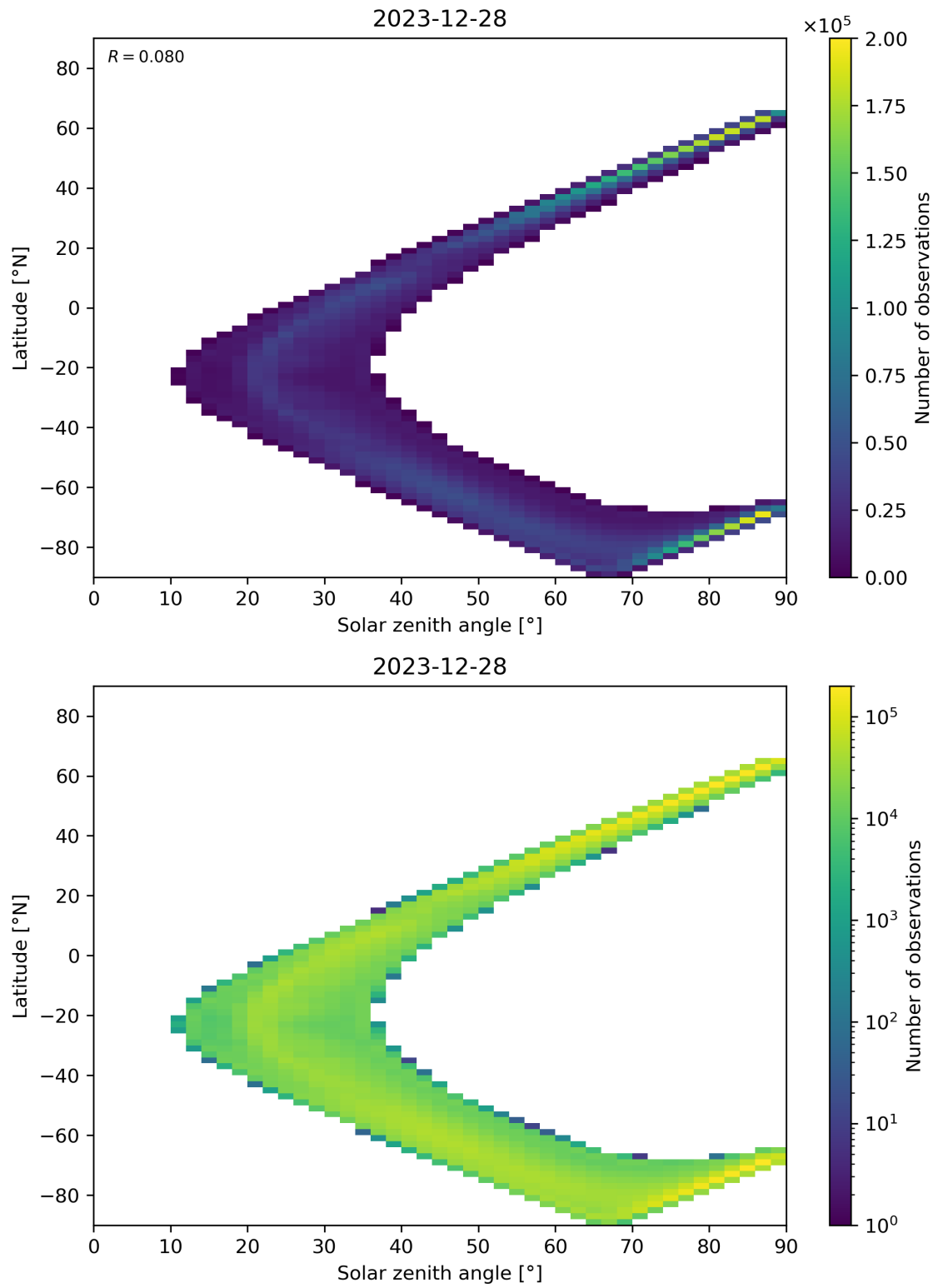
Figure 105: Scatter density plot of “Solar zenith angle” against “Latitude” for 2023-12-27 to 2023-12-29.
