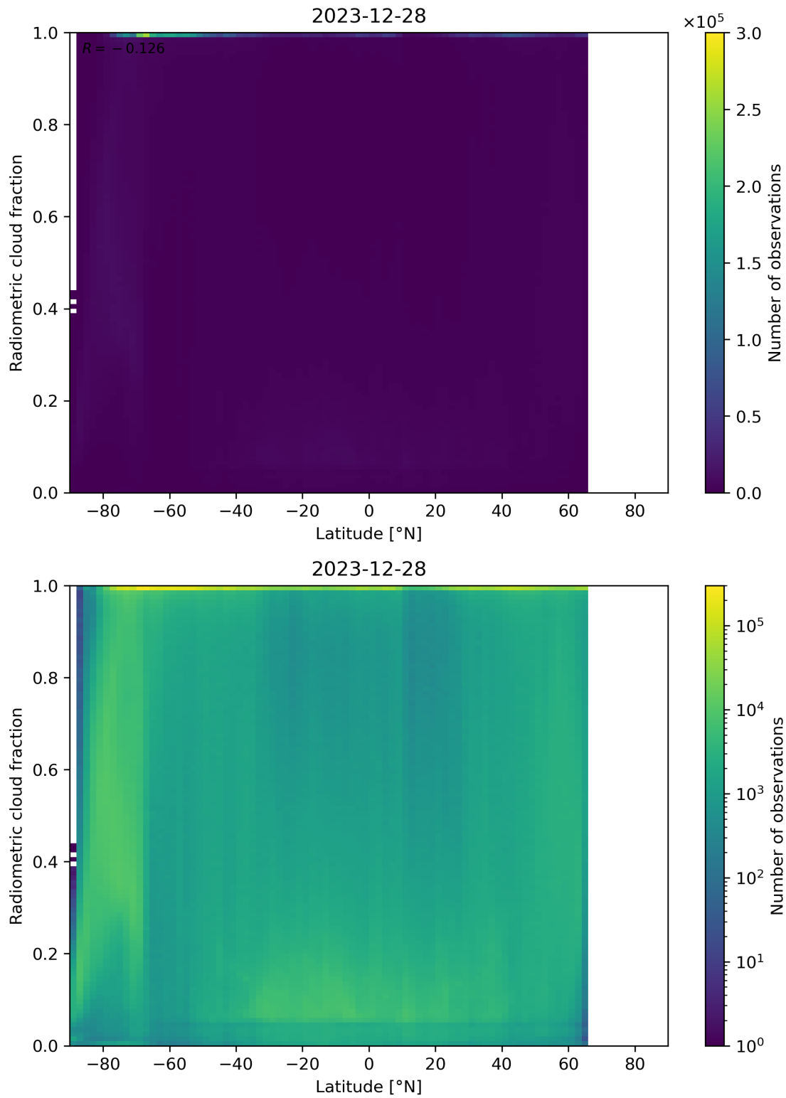
Figure 92: Scatter density plot of “Latitude” against “Radiometric cloud fraction” for 2023-12-27 to 2023-12-29.
