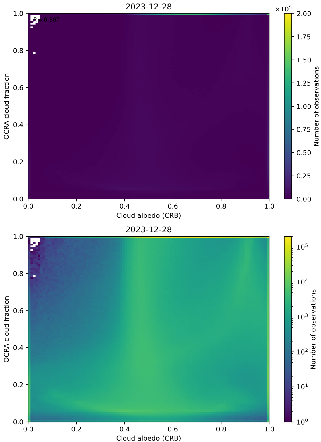
Figure 70: Scatter density plot of “Cloud albedo (CRB)” against “OCRA cloud fraction” for 2023-12-27 to 2023-12-29.
