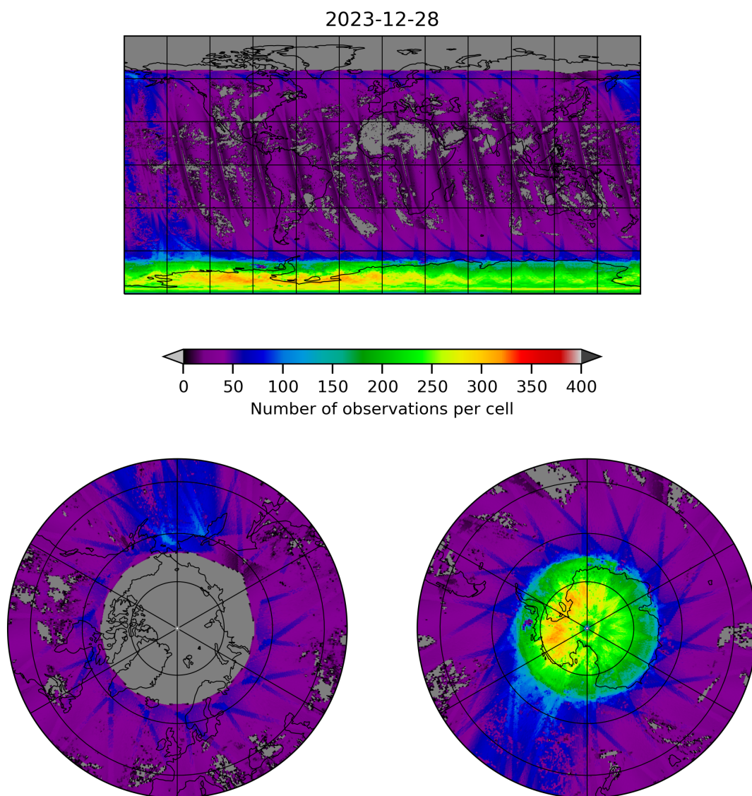
Figure 21: Map of the number of observations for 2023-12-27 to 2023-12-29
