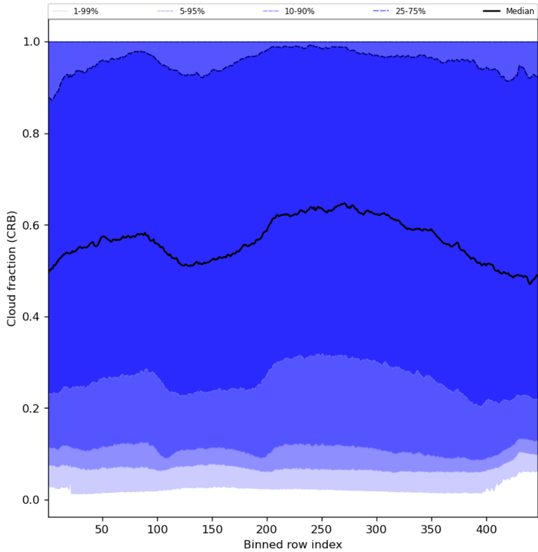
Figure 58: Along track statistics of “Cloud fraction (CRB)” for 2023-12-27 to 2023-12-29
