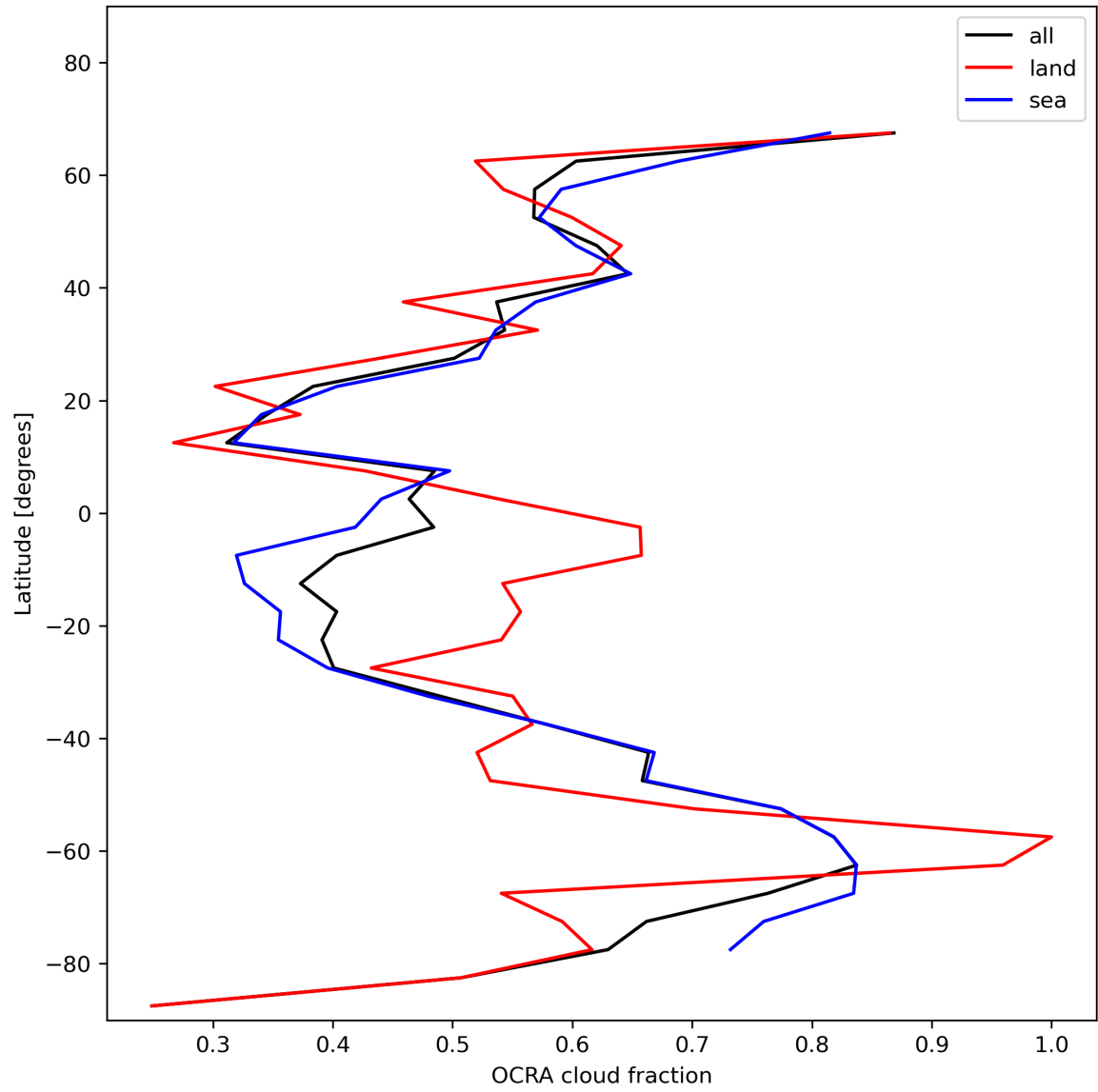
Figure 34: Zonal average of “OCRA cloud fraction” for 2023-12-27 to 2023-12-29.
