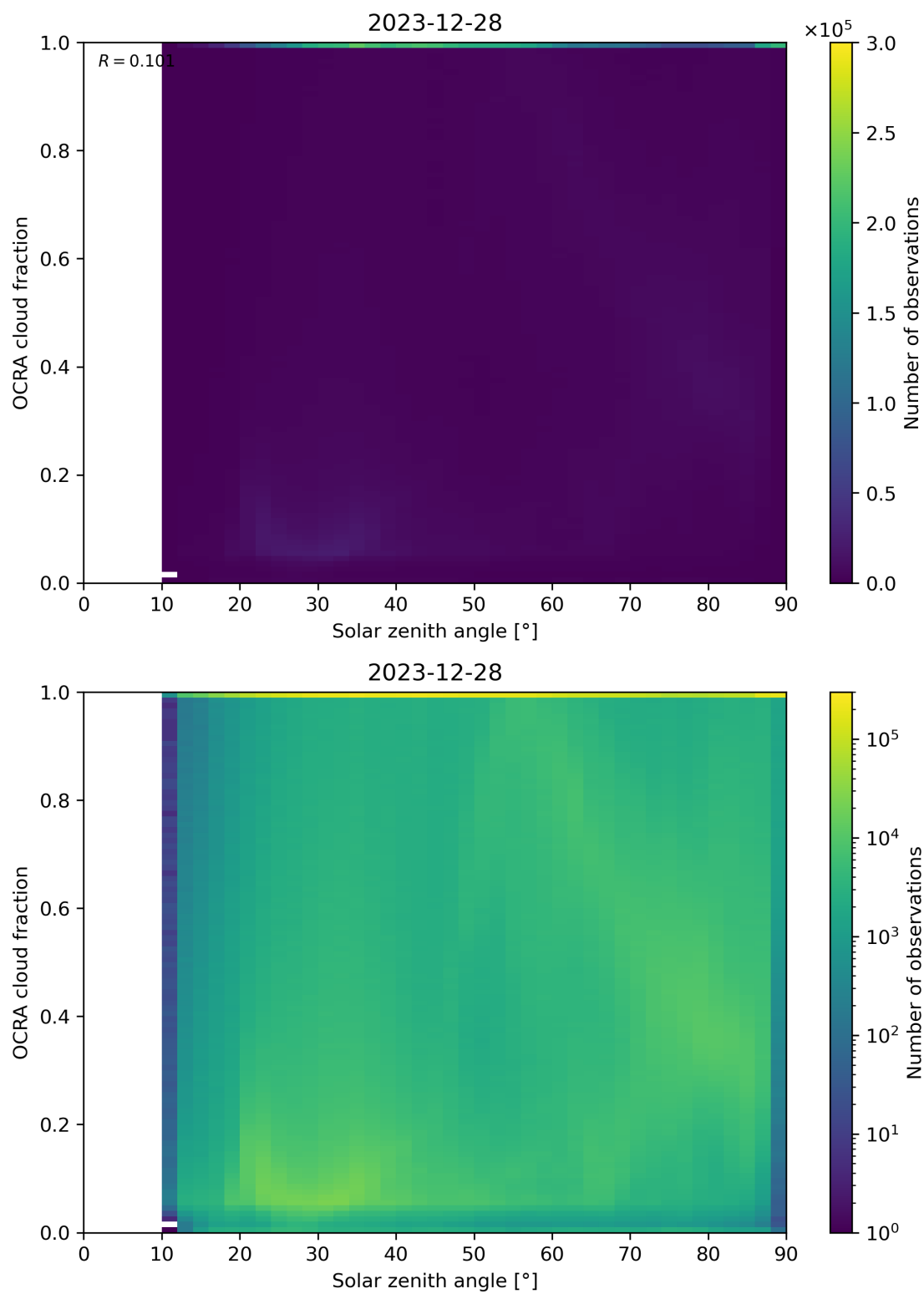
Figure 100: Scatter density plot of “Solar zenith angle” against “OCRA cloud fraction” for 2023-12-27 to 2023-12-29.
