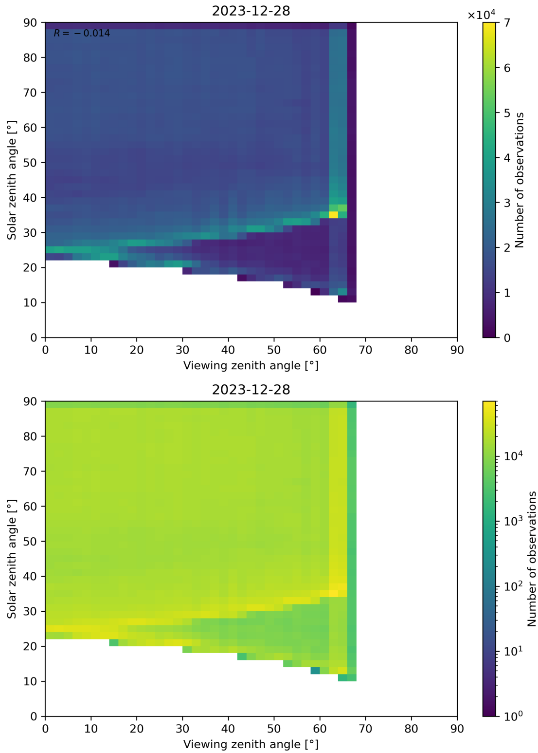
Figure 114: Scatter density plot of “Viewing zenith angle” against “Solar zenith angle” for 2023-12-27 to 2023-12-29.
