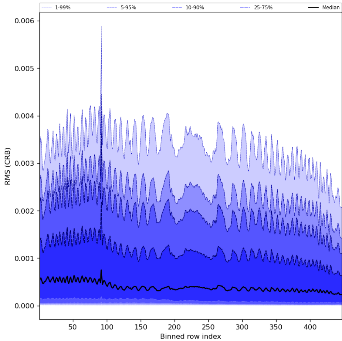
Figure 64: Along track statistics of “RMS (CRB)” for 2023-12-27 to 2023-12-29
