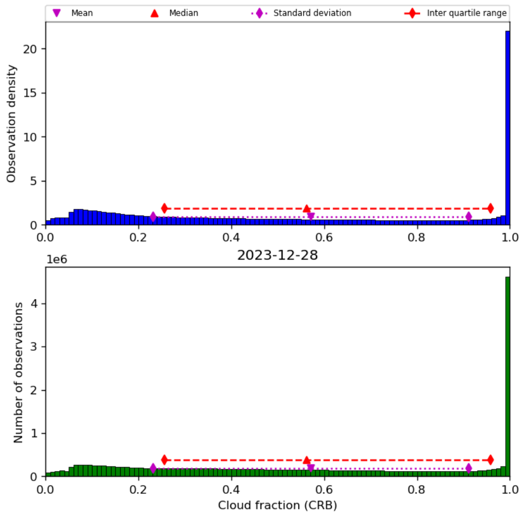
Figure 42: Histogram of “Cloud fraction (CRB)” for 2023-12-27 to 2023-12-29
