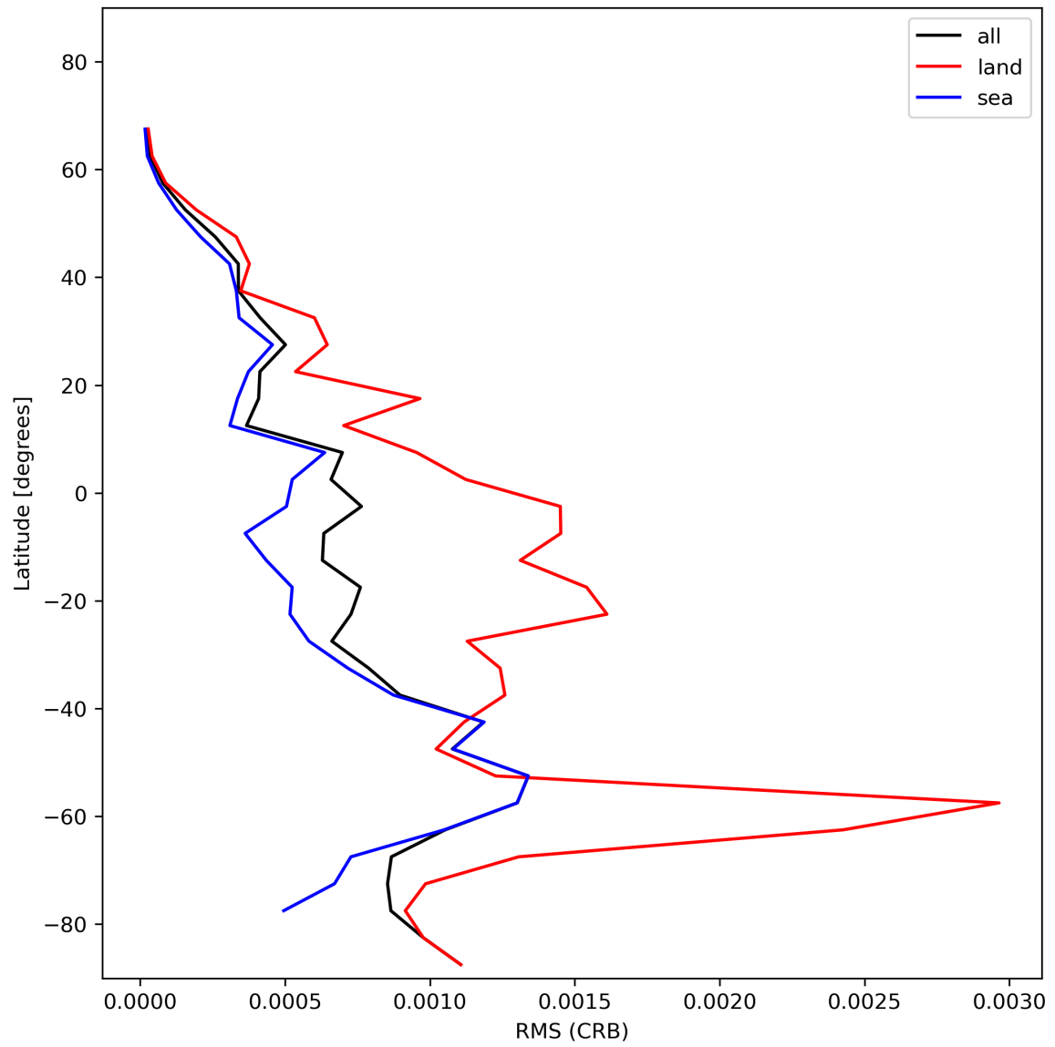
Figure 32: Zonal average of “RMS (CRB)” for 2023-12-27 to 2023-12-29.
