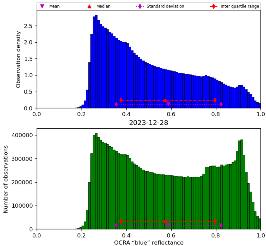
Figure 51: Histogram of “OCRA “blue” reflectance” for 2023-12-27 to 2023-12-29
