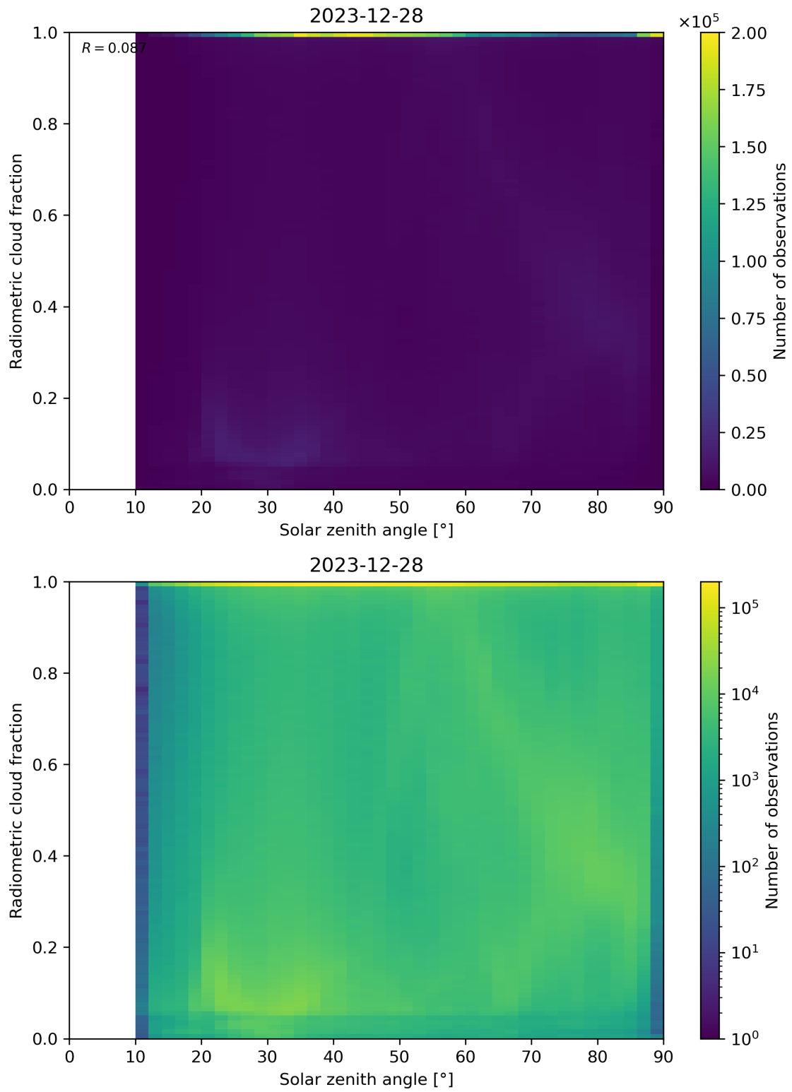
Figure 99: Scatter density plot of “Solar zenith angle” against “Radiometric cloud fraction” for 2023-12-27 to 2023-12-29.
