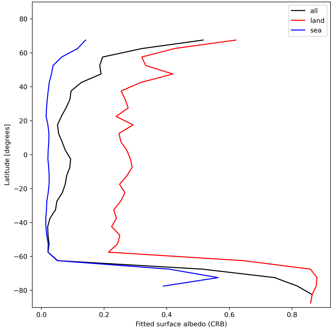
Figure 30: Zonal average of “Fitted surface albedo (CRB)” for 2023-12-27 to 2023-12-29.
