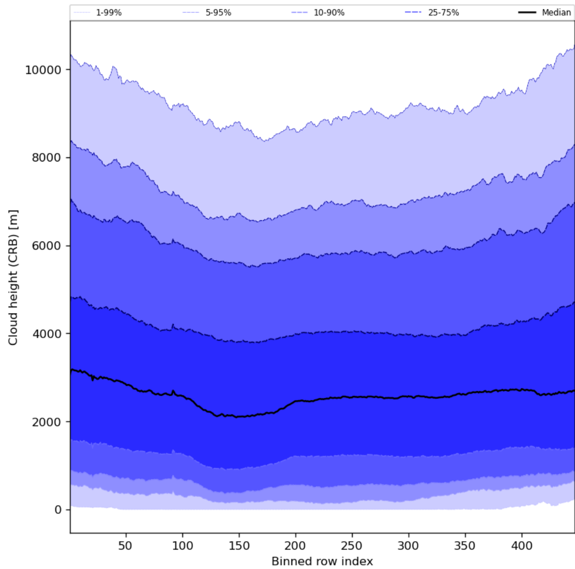
Figure 59: Along track statistics of “Cloud height (CRB)” for 2023-12-27 to 2023-12-29
