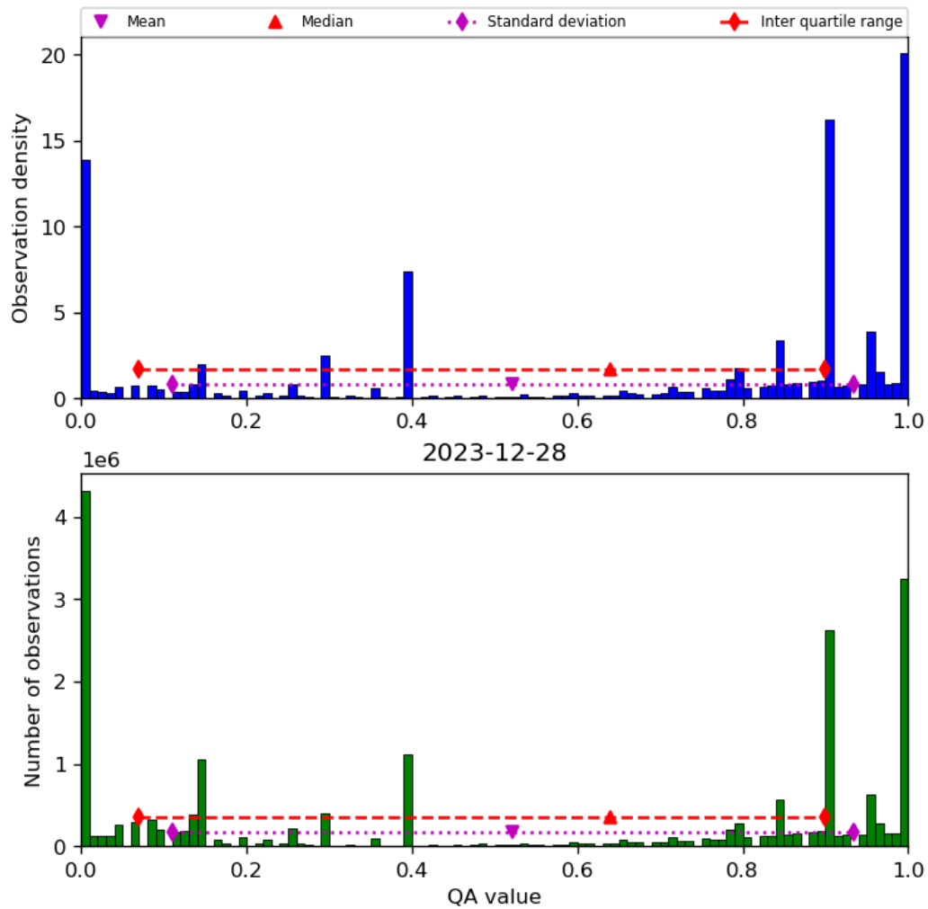
Figure 38: Histogram of “QA value” for 2023-12-27 to 2023-12-29
