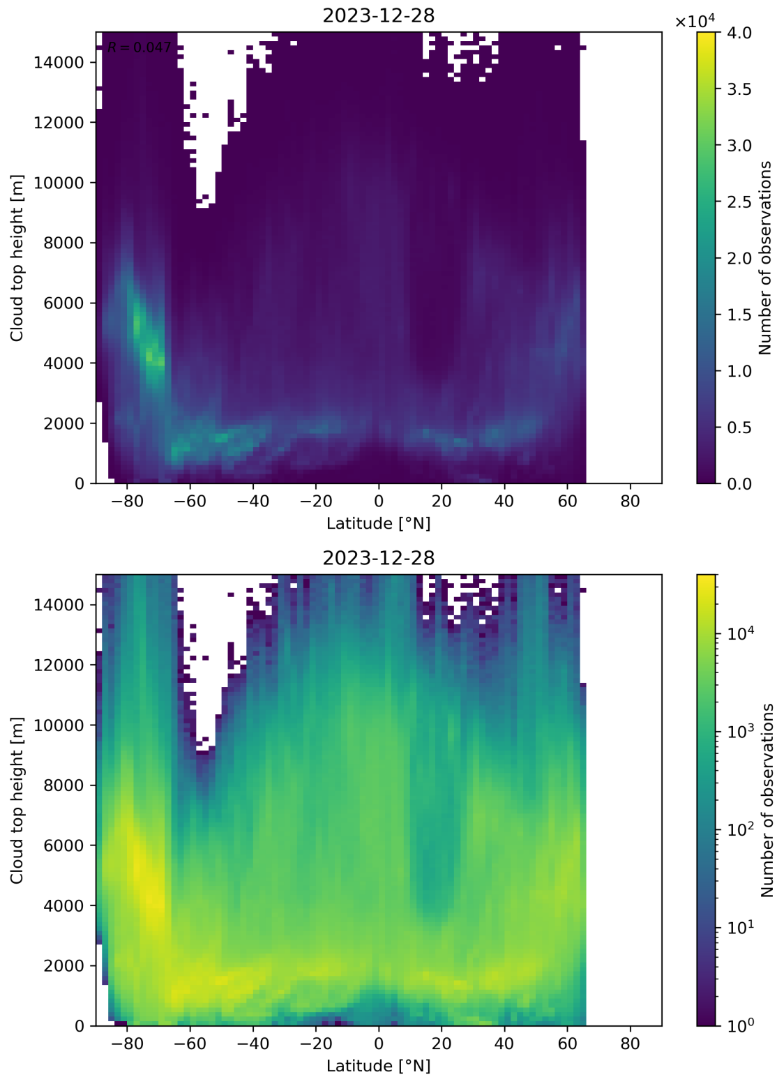
Figure 97: Scatter density plot of “Latitude” against “Cloud top height” for 2023-12-27 to 2023-12-29.
