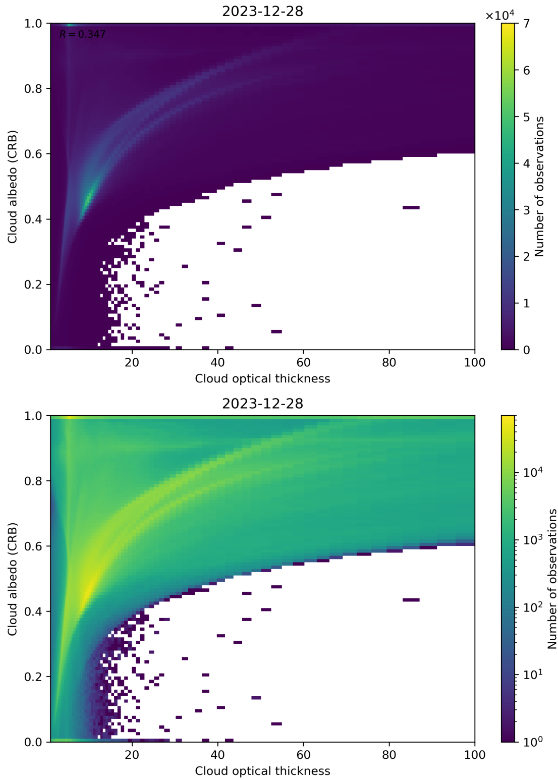
Figure 82: Scatter density plot of “Cloud optical thickness” against “Cloud albedo (CRB)” for 2023-12-27 to 2023-12-29.
