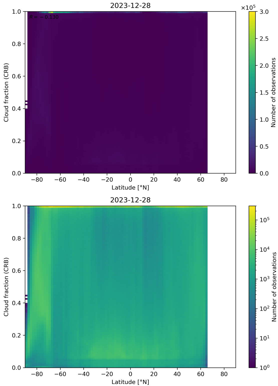
Figure 94: Scatter density plot of “Latitude” against “Cloud fraction (CRB)” for 2023-12-27 to 2023-12-29.
