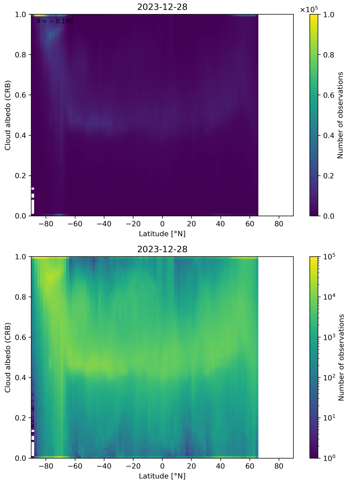
Figure 91: Scatter density plot of “Latitude” against “Cloud albedo (CRB)” for 2023-12-27 to 2023-12-29.
