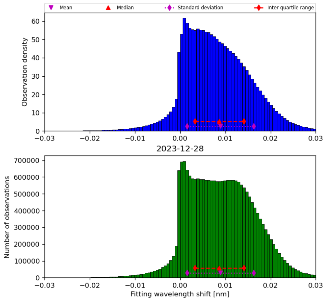
Figure 49: Histogram of “Fitting wavelength shift” for 2023-12-27 to 2023-12-29
