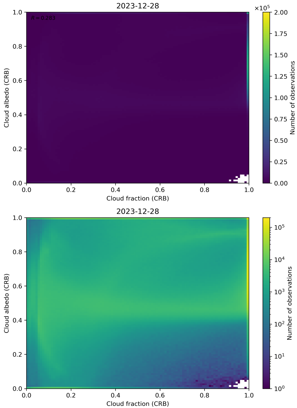
Figure 77: Scatter density plot of “Cloud fraction (CRB)” against “Cloud albedo (CRB)” for 2023-12-27 to 2023-12-29.
