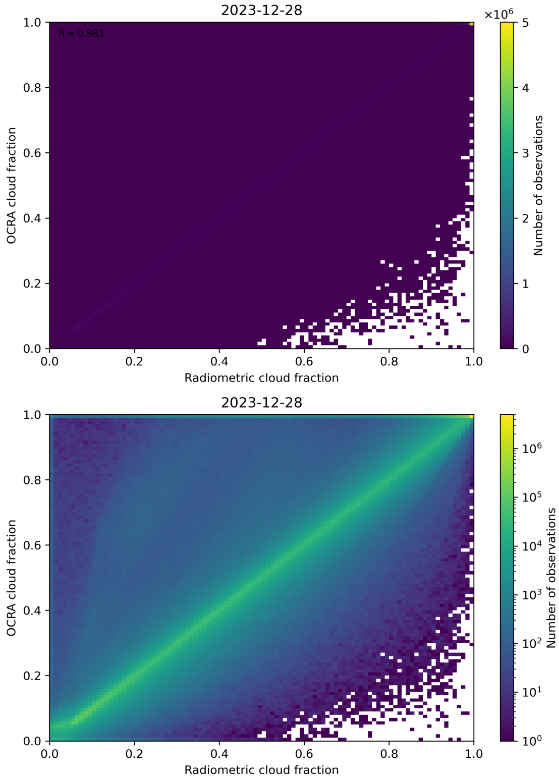
Figure 72: Scatter density plot of “Radiometric cloud fraction” against “OCRA cloud fraction” for 2023-12-27 to 2023-12-29.
