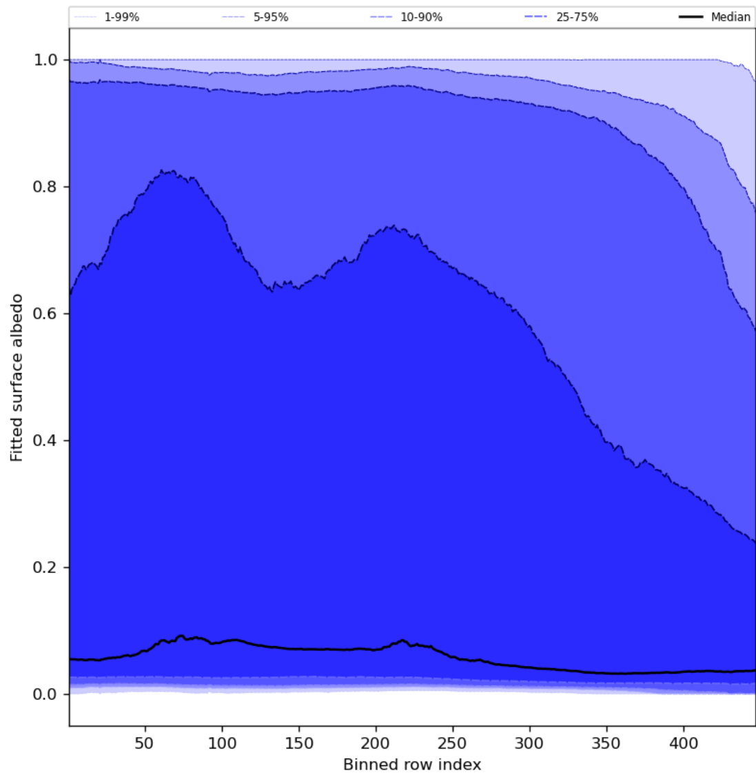
Figure 61: Along track statistics of “Fitted surface albedo” for 2023-12-27 to 2023-12-29
