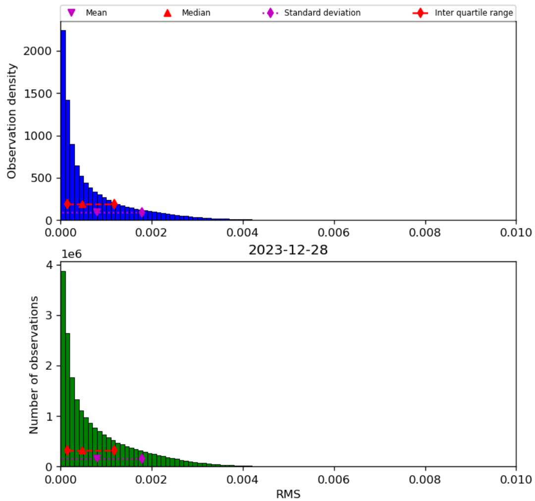
Figure 47: Histogram of “RMS” for 2023-12-27 to 2023-12-29
