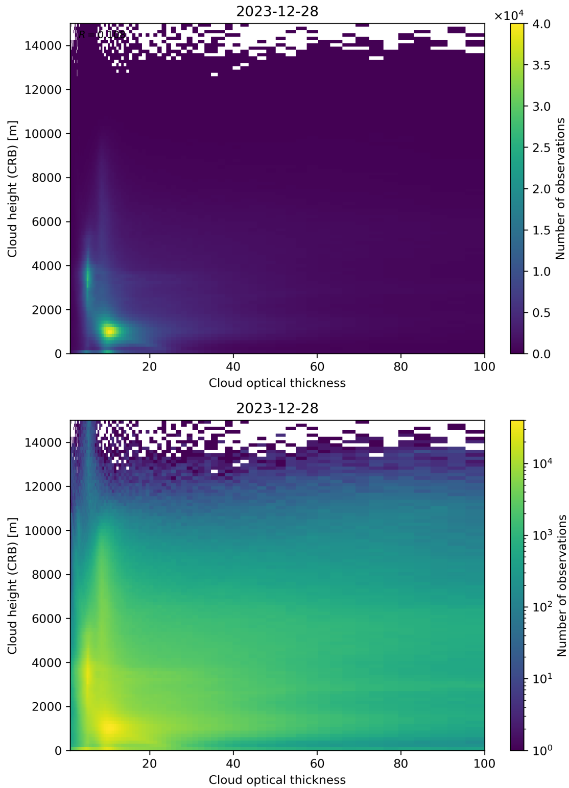
Figure 85: Scatter density plot of “Cloud optical thickness” against “Cloud height (CRB)” for 2023-12-27 to 2023-12-29.
