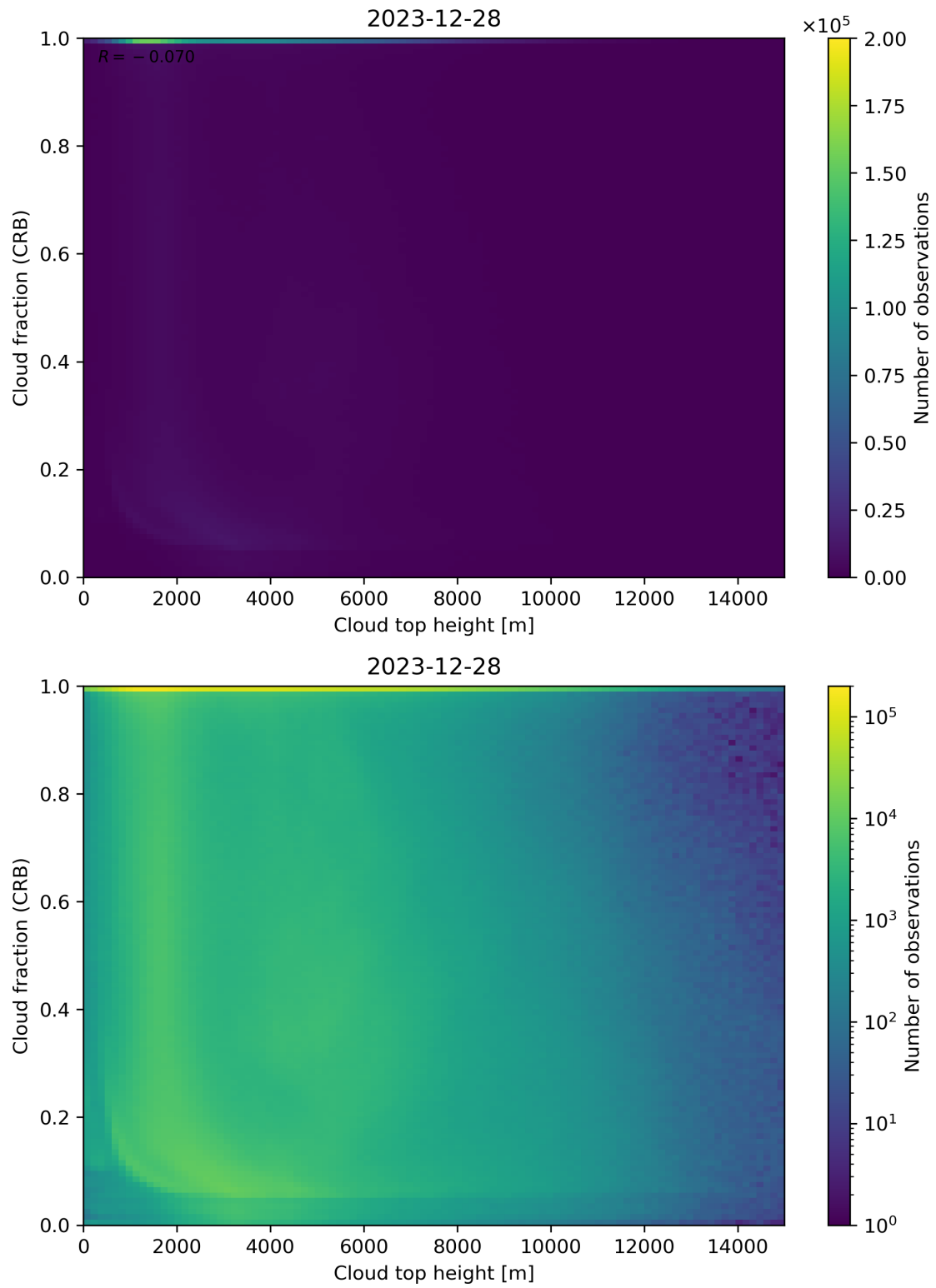
Figure 88: Scatter density plot of “Cloud top height” against “Cloud fraction (CRB)” for 2023-12-27 to 2023-12-29.
