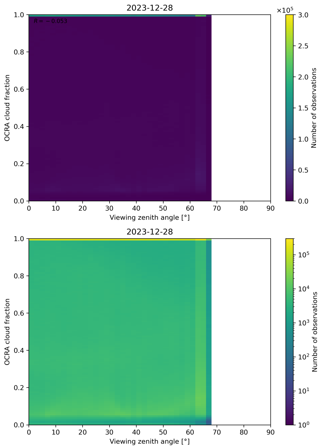
Figure 108: Scatter density plot of “Viewing zenith angle” against “OCRA cloud fraction” for 2023-12-27 to 2023-12-29.
