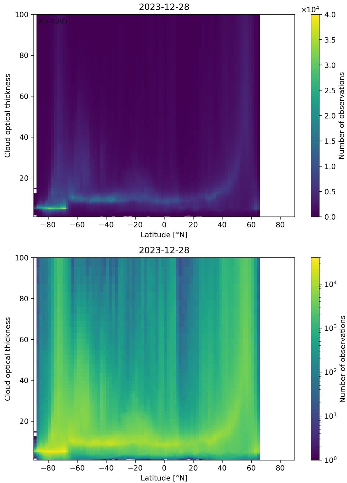
Figure 96: Scatter density plot of “Latitude” against “Cloud optical thickness” for 2023-12-27 to 2023-12-29.
