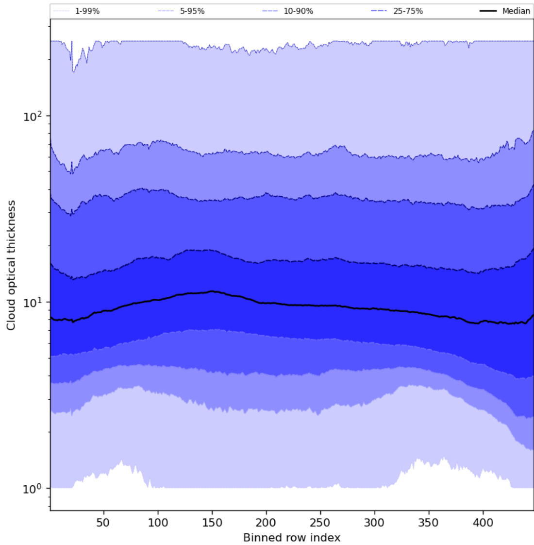
Figure 57: Along track statistics of “Cloud optical thickness” for 2023-12-27 to 2023-12-29
