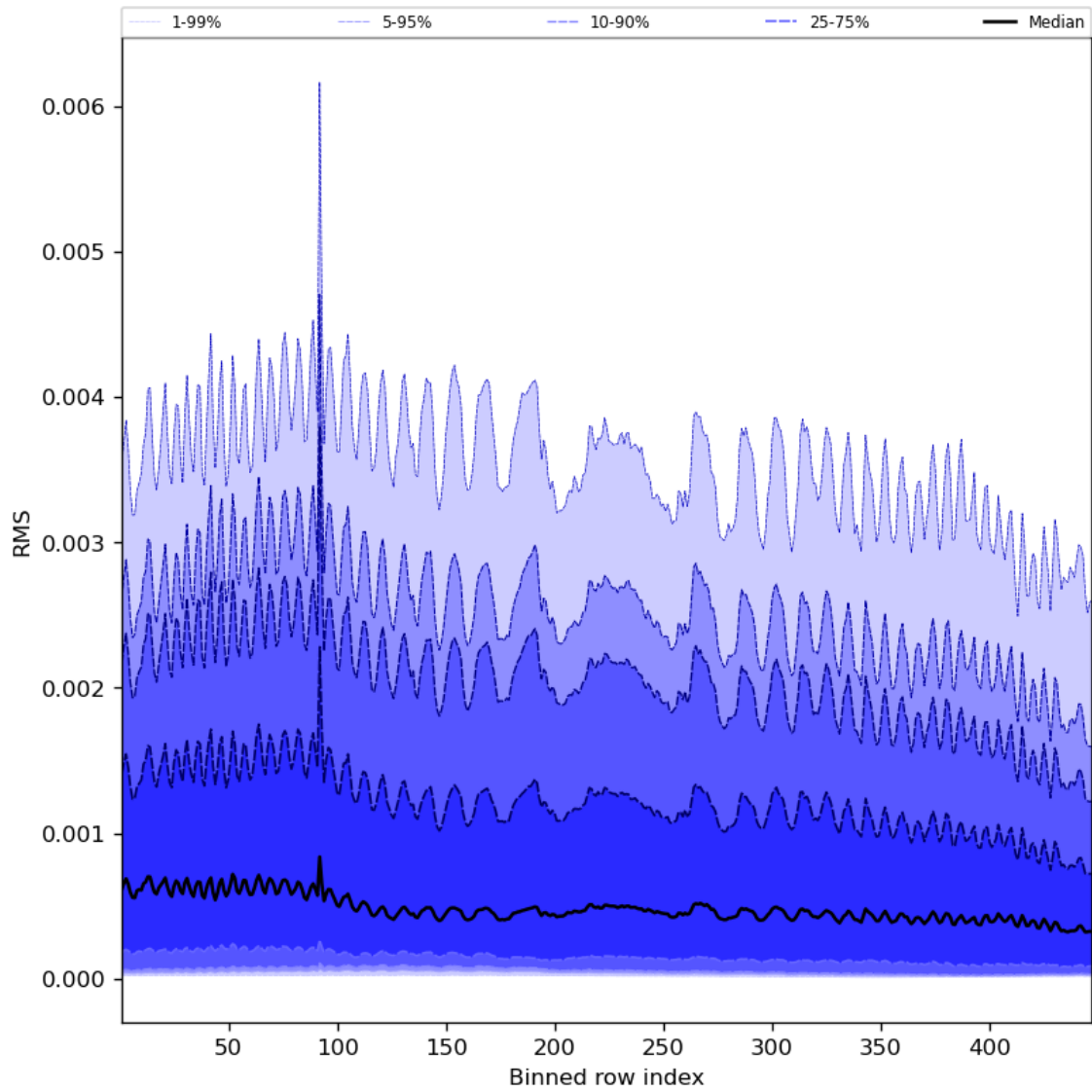
Figure 63: Along track statistics of “RMS” for 2023-12-27 to 2023-12-29
