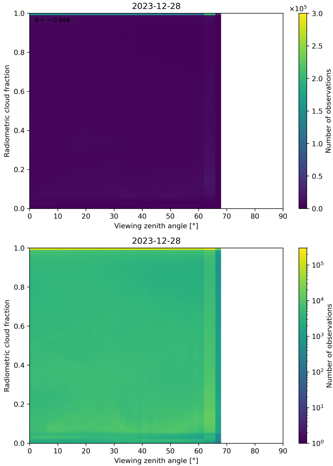
Figure 107: Scatter density plot of “Viewing zenith angle” against “Radiometric cloud fraction” for 2023-12-27 to 2023-12-29.
