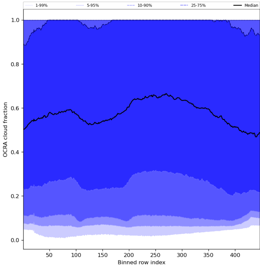
Figure 66: Along track statistics of “OCRA cloud fraction” for 2023-12-27 to 2023-12-29
