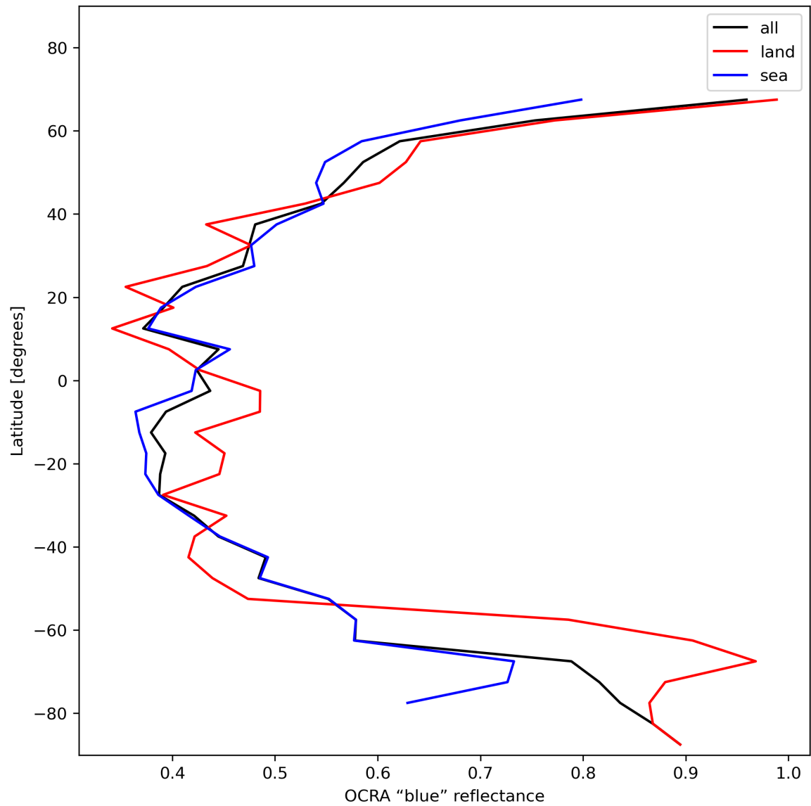
Figure 35: Zonal average of “OCRA “blue” reflectance” for 2023-12-27 to 2023-12-29.
