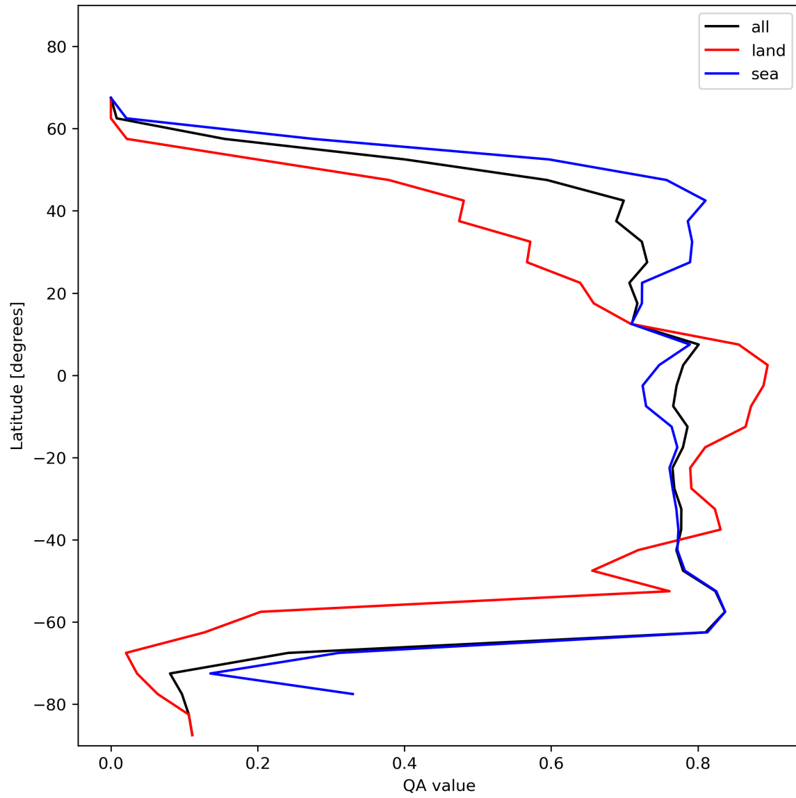
Figure 22: Zonal average of “QA value” for 2023-12-27 to 2023-12-29.
