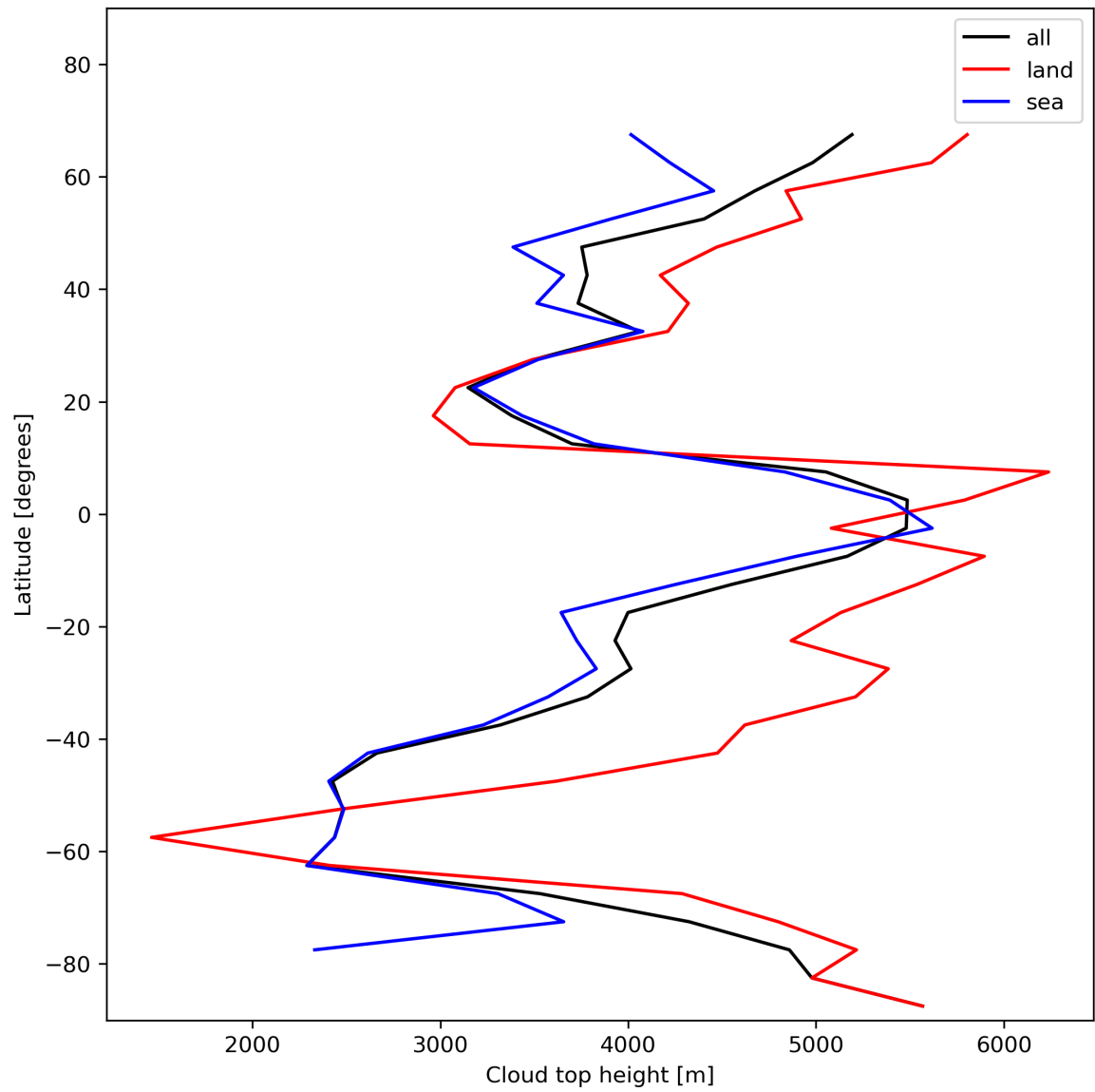
Figure 24: Zonal average of “Cloud top height” for 2023-12-27 to 2023-12-29.
