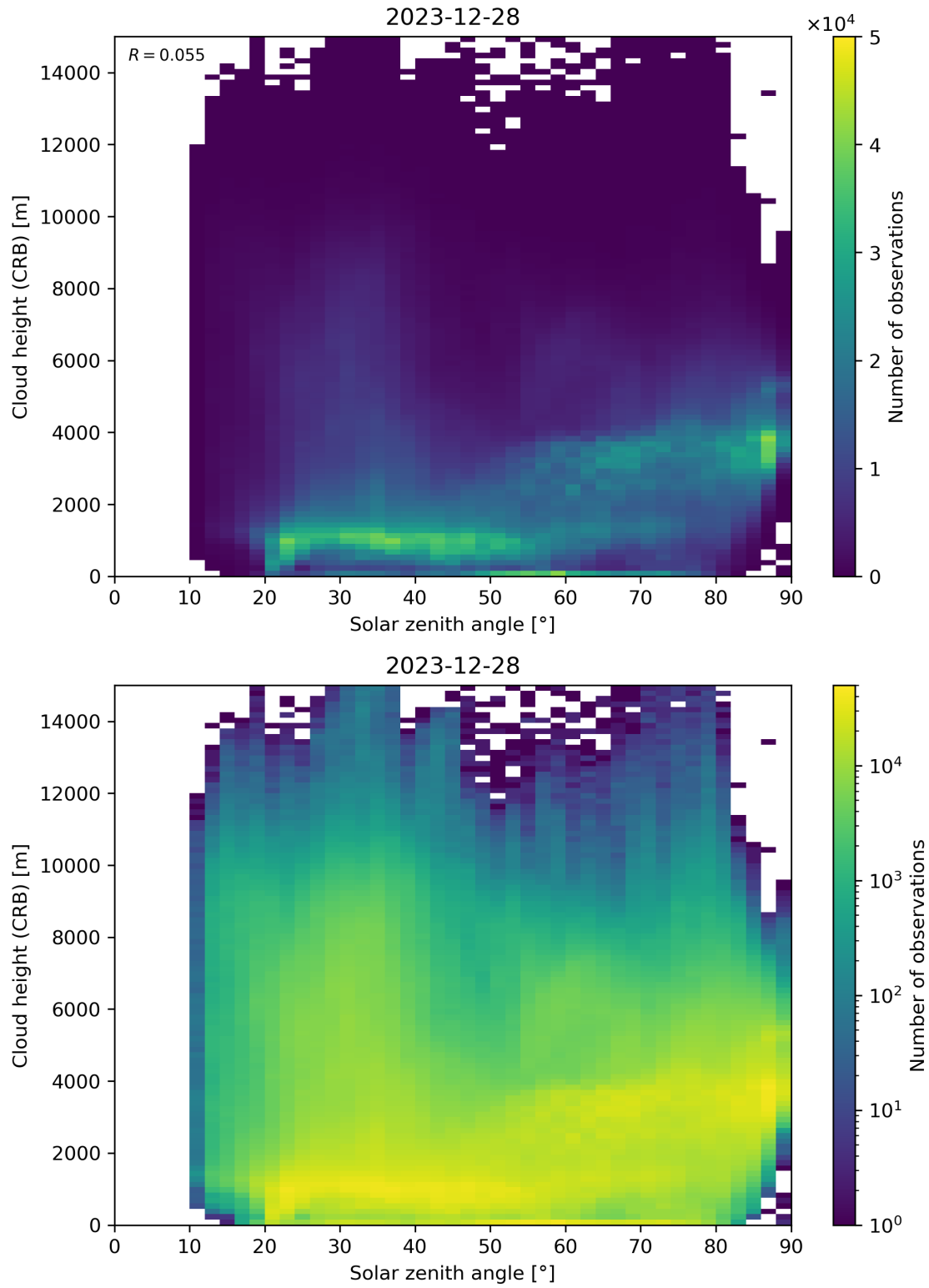
Figure 102: Scatter density plot of “Solar zenith angle” against “Cloud height (CRB)” for 2023-12-27 to 2023-12-29.
