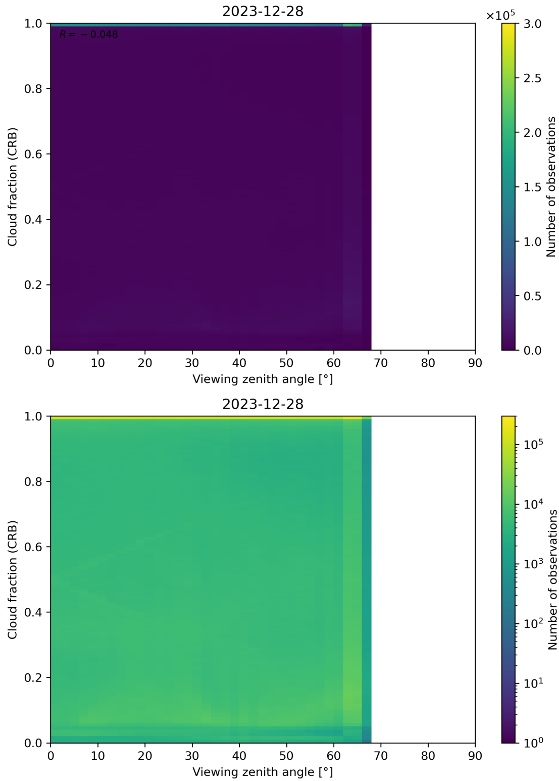
Figure 109: Scatter density plot of “Viewing zenith angle” against “Cloud fraction (CRB)” for 2023-12-27 to 2023-12-29.
