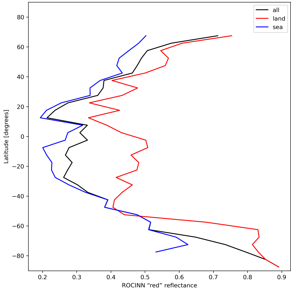
Figure 37: Zonal average of “ROCINN “red” reflectance” for 2023-12-27 to 2023-12-29.
