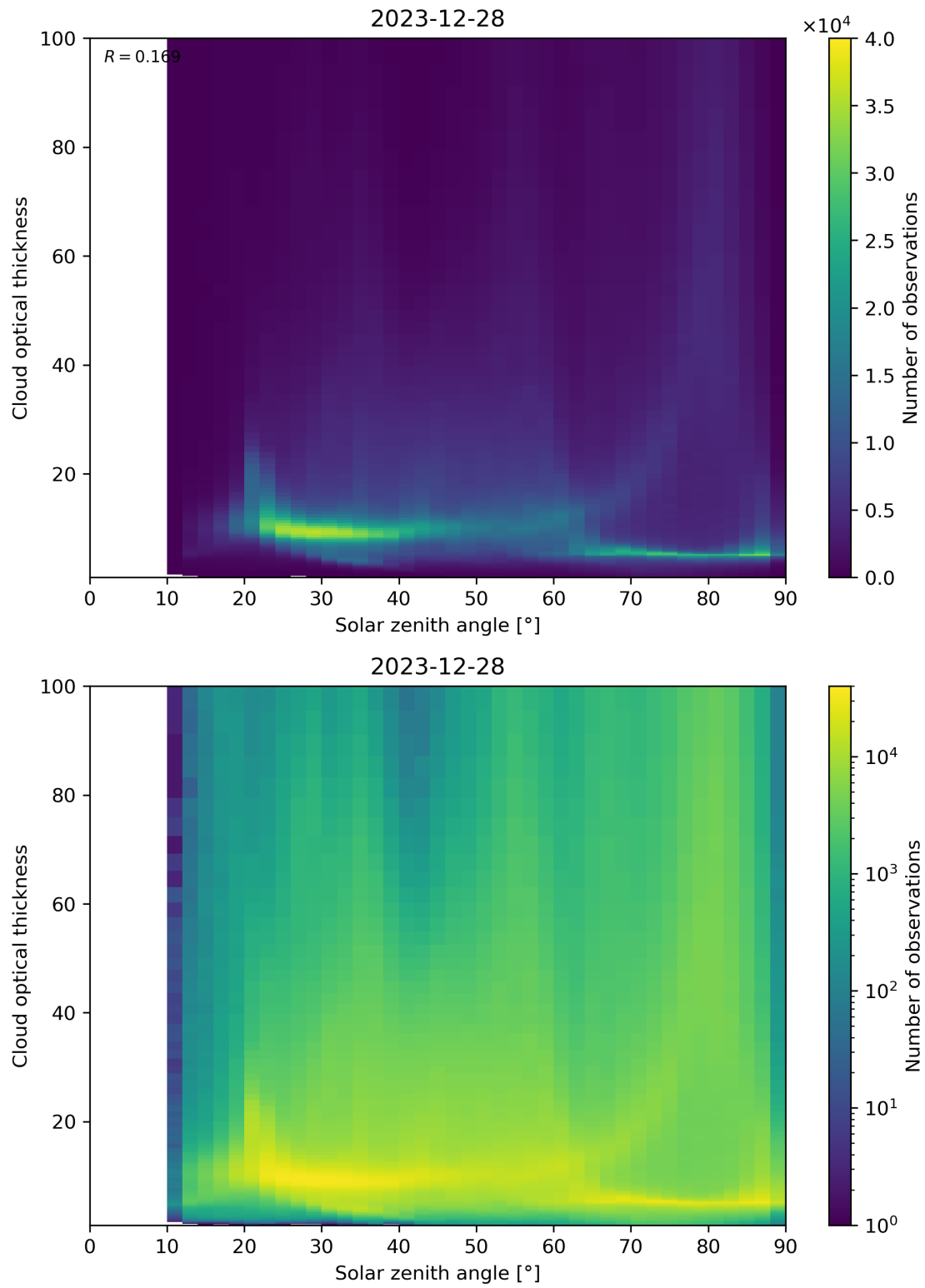
Figure 103: Scatter density plot of “Solar zenith angle” against “Cloud optical thickness” for 2023-12-27 to 2023-12-29.
