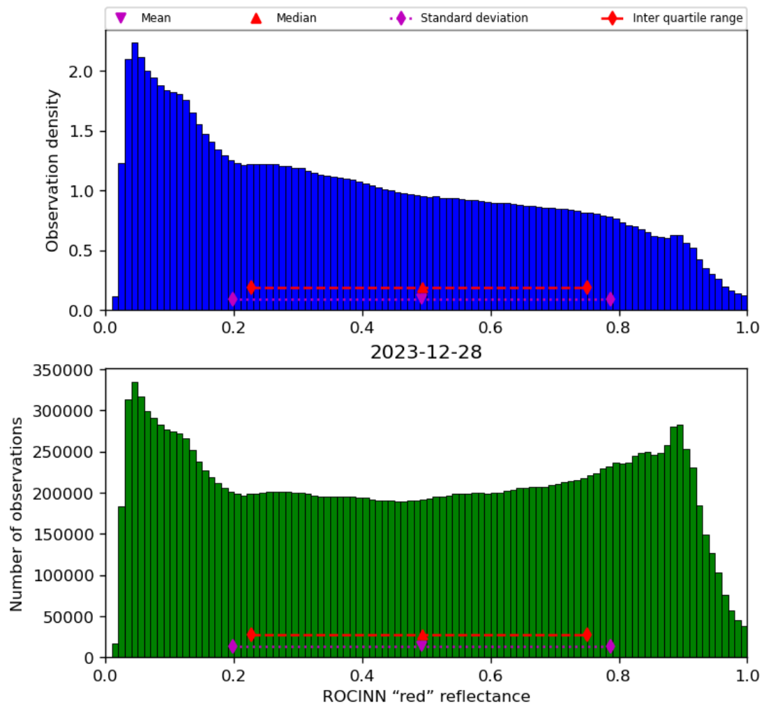
Figure 53: Histogram of “ROCINN “red” reflectance” for 2023-12-27 to 2023-12-29
