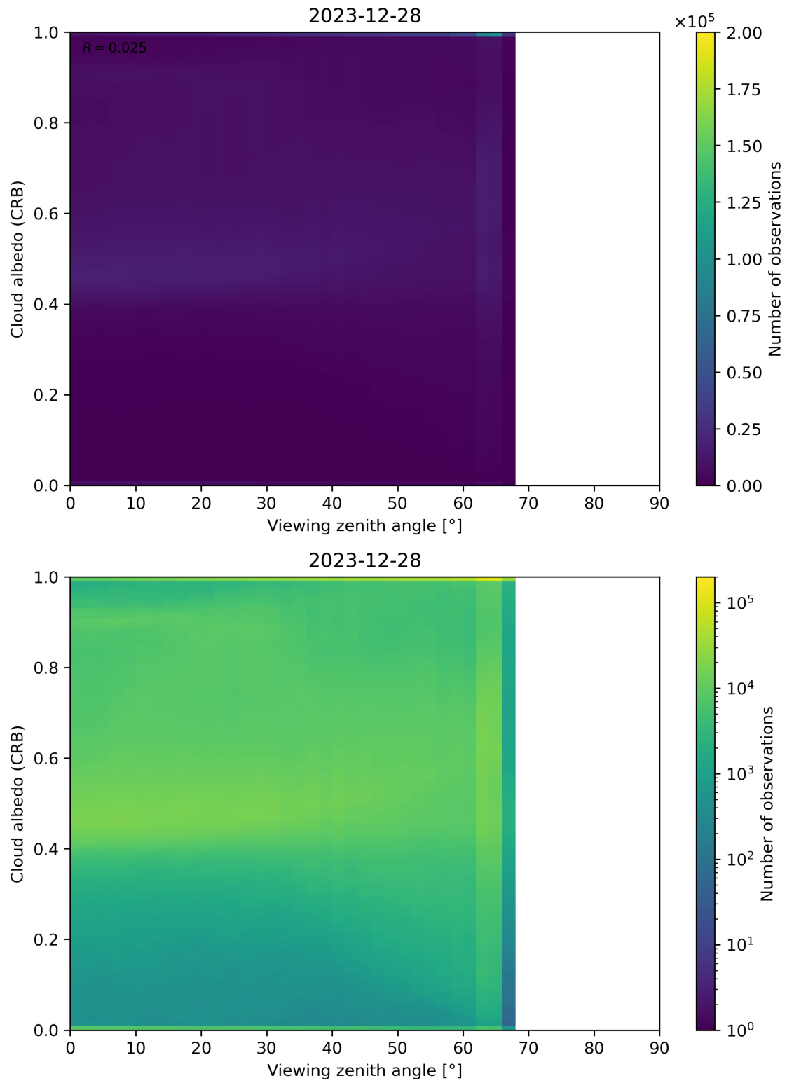
Figure 106: Scatter density plot of “Viewing zenith angle” against “Cloud albedo (CRB)” for 2023-12-27 to 2023-12-29.
