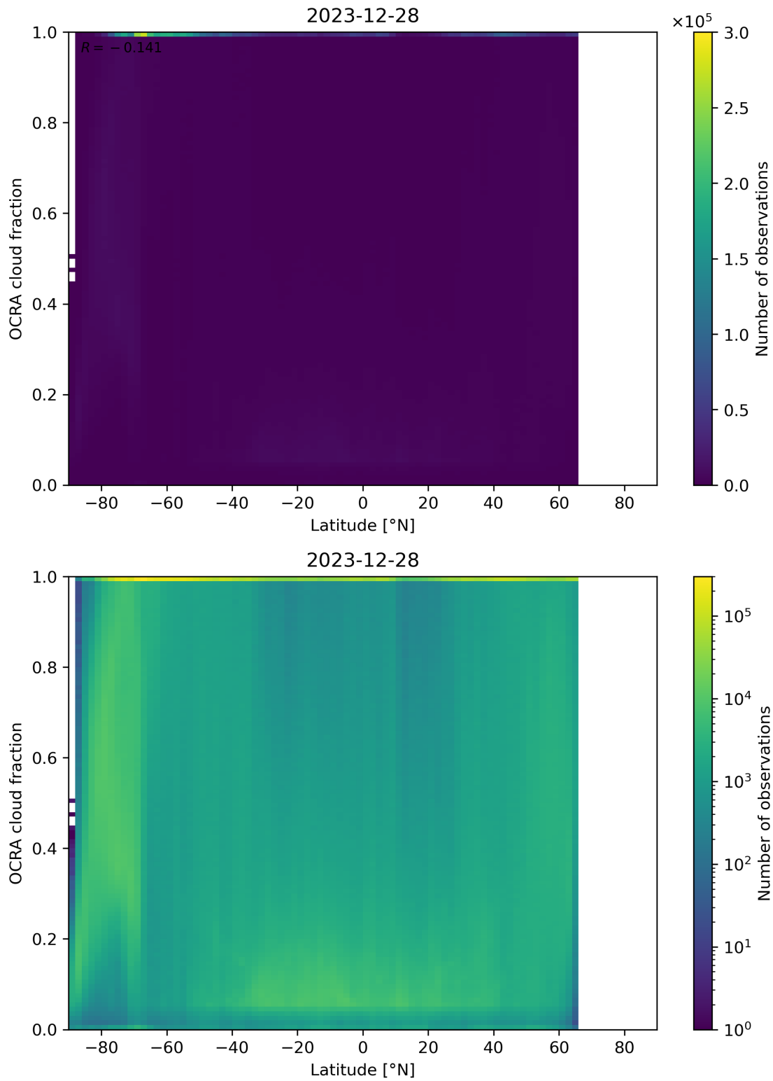
Figure 93: Scatter density plot of “Latitude” against “OCRA cloud fraction” for 2023-12-27 to 2023-12-29.
