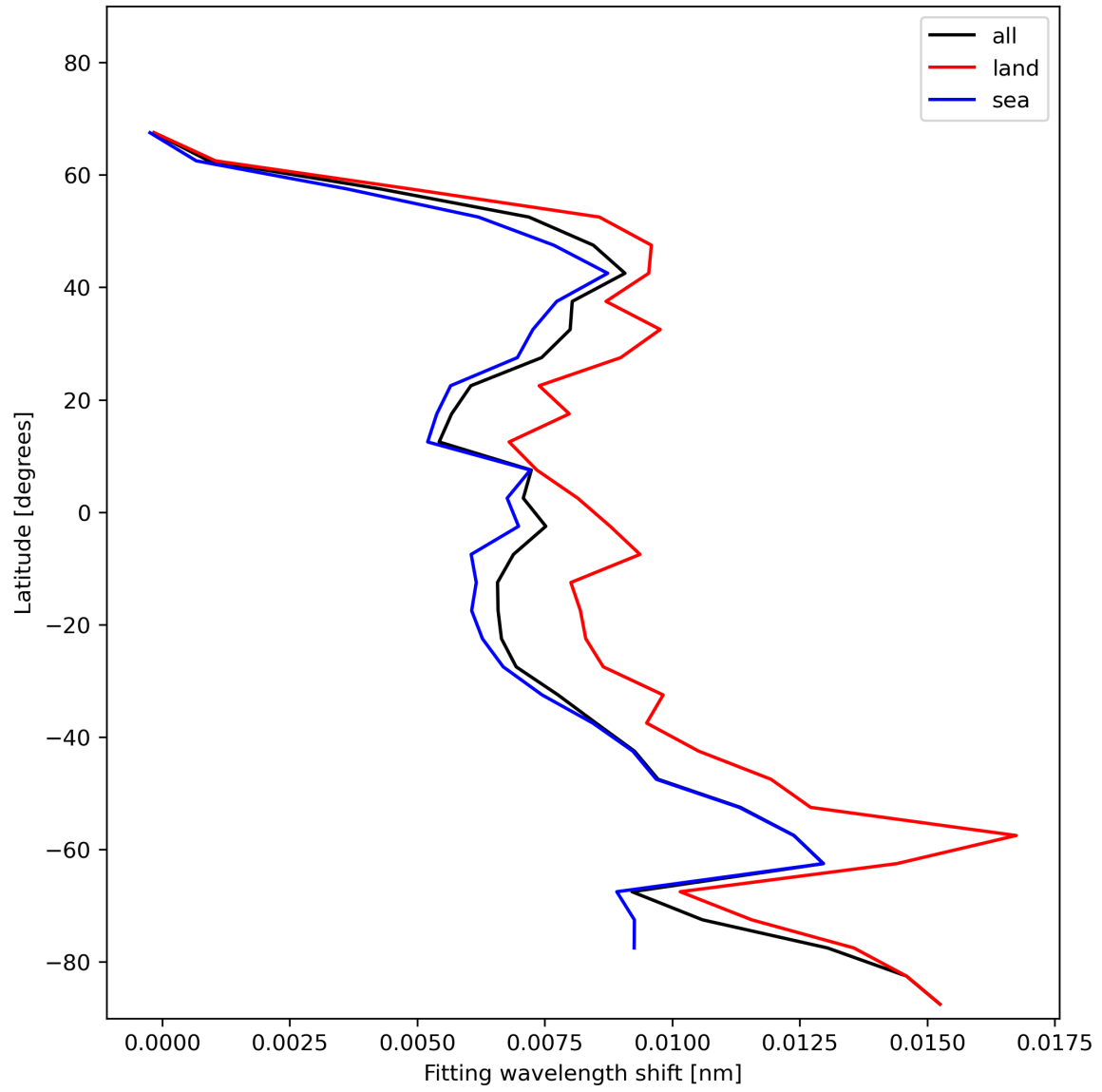
Figure 33: Zonal average of “Fitting wavelength shift” for 2023-12-27 to 2023-12-29.
