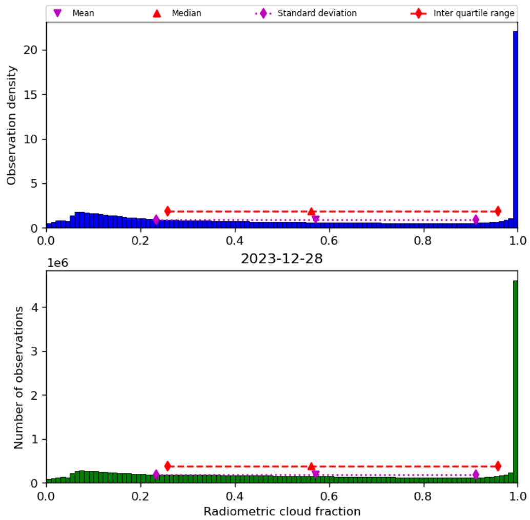
Figure 39: Histogram of “Radiometric cloud fraction” for 2023-12-27 to 2023-12-29
