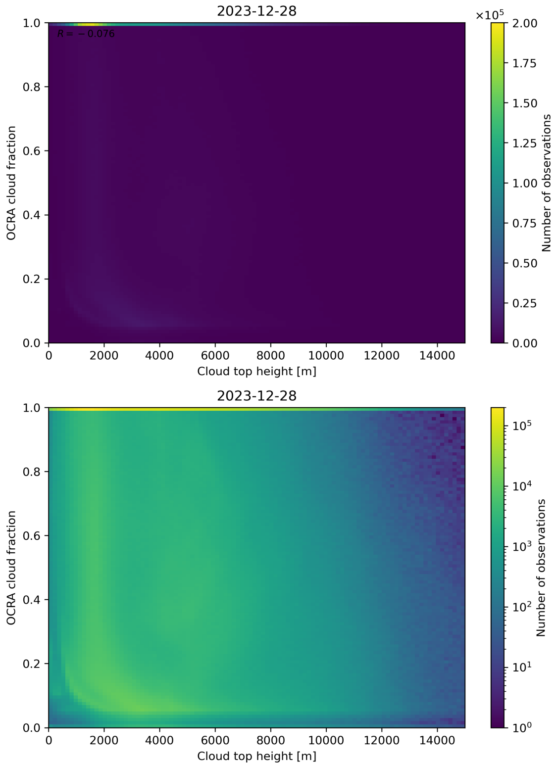
Figure 87: Scatter density plot of “Cloud top height” against “OCRA cloud fraction” for 2023-12-27 to 2023-12-29.
