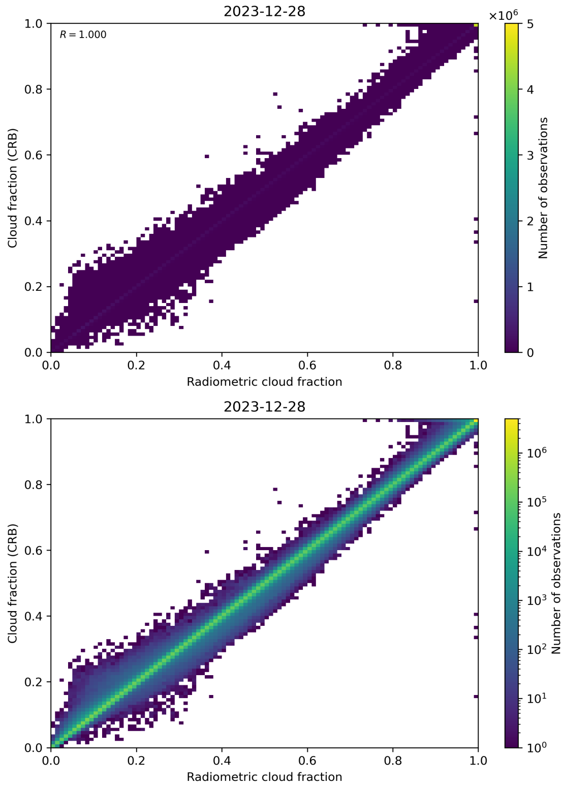
Figure 73: Scatter density plot of “Radiometric cloud fraction” against “Cloud fraction (CRB)” for 2023-12-27 to 2023-12-29.
