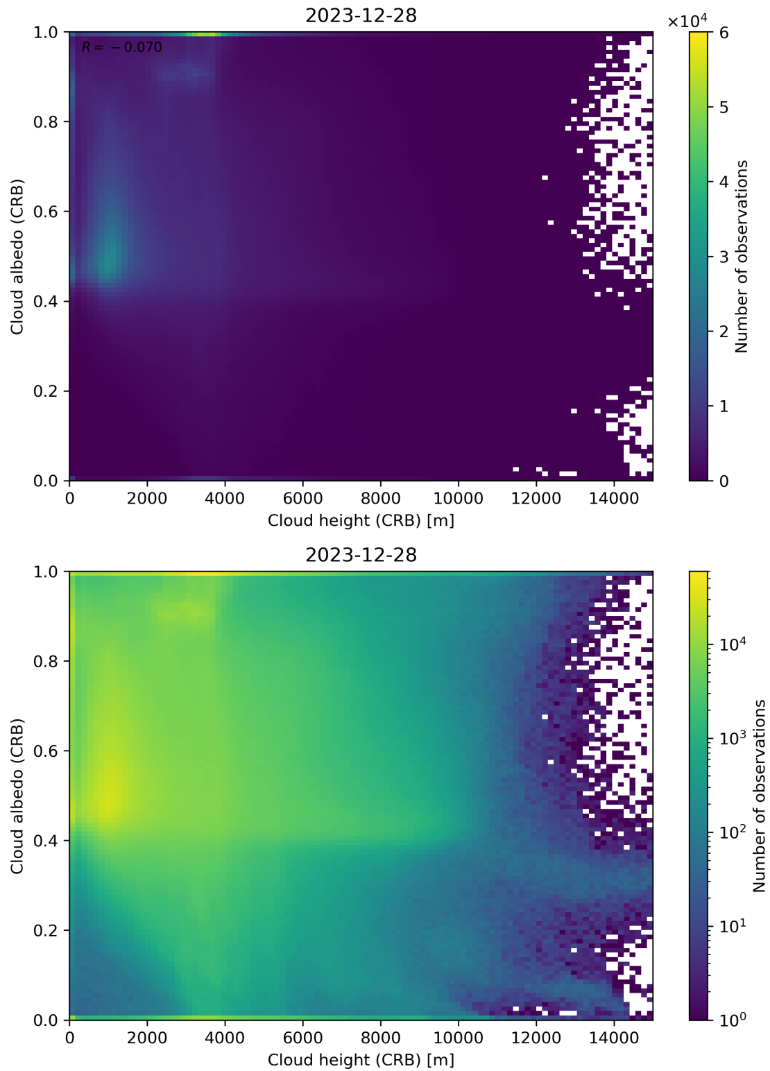
Figure 80: Scatter density plot of “Cloud height (CRB)” against “Cloud albedo (CRB)” for 2023-12-27 to 2023-12-29.
