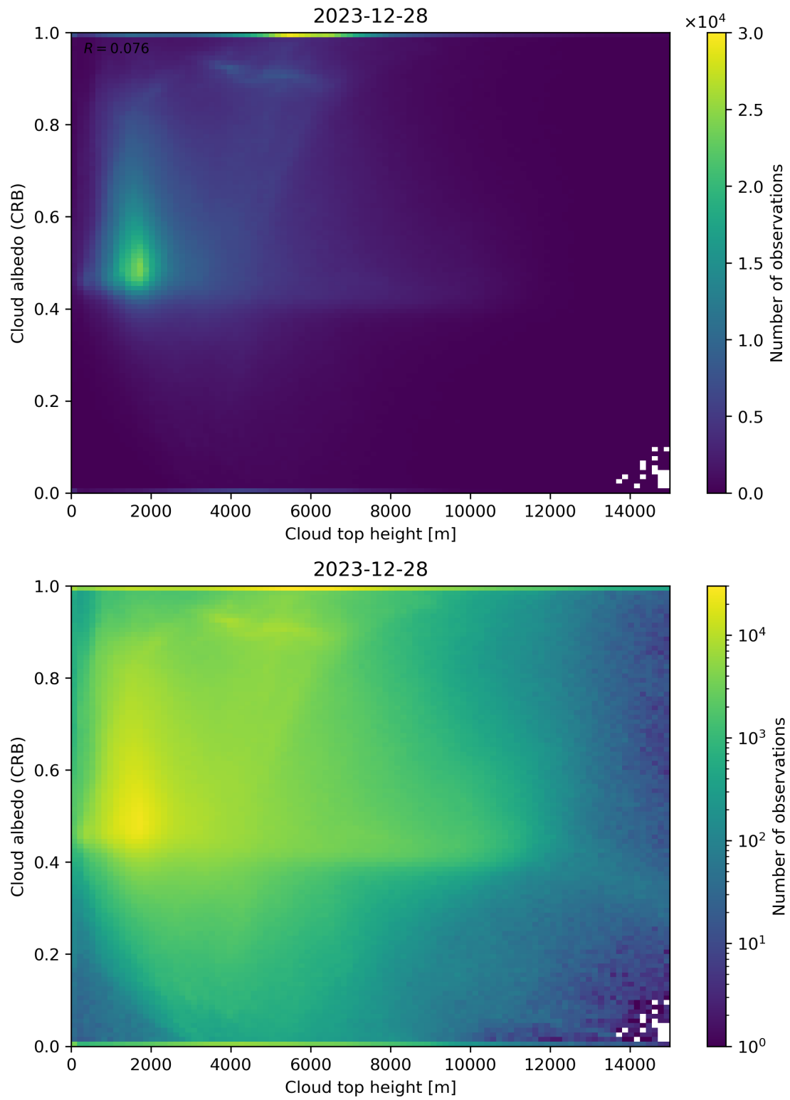
Figure 86: Scatter density plot of “Cloud top height” against “Cloud albedo (CRB)” for 2023-12-27 to 2023-12-29.
