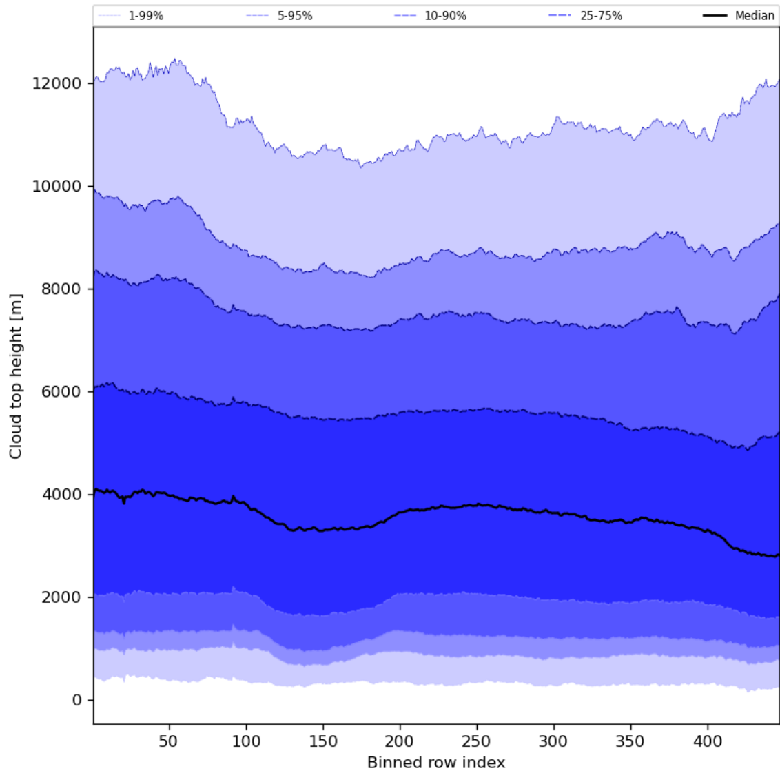
Figure 56: Along track statistics of “Cloud top height” for 2023-12-27 to 2023-12-29
