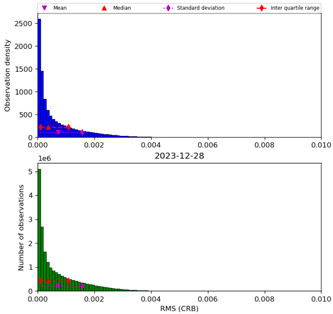
Figure 48: Histogram of “RMS (CRB)” for 2023-12-27 to 2023-12-29
