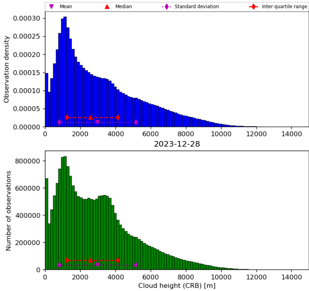
Figure 43: Histogram of “Cloud height (CRB)” for 2023-12-27 to 2023-12-29
