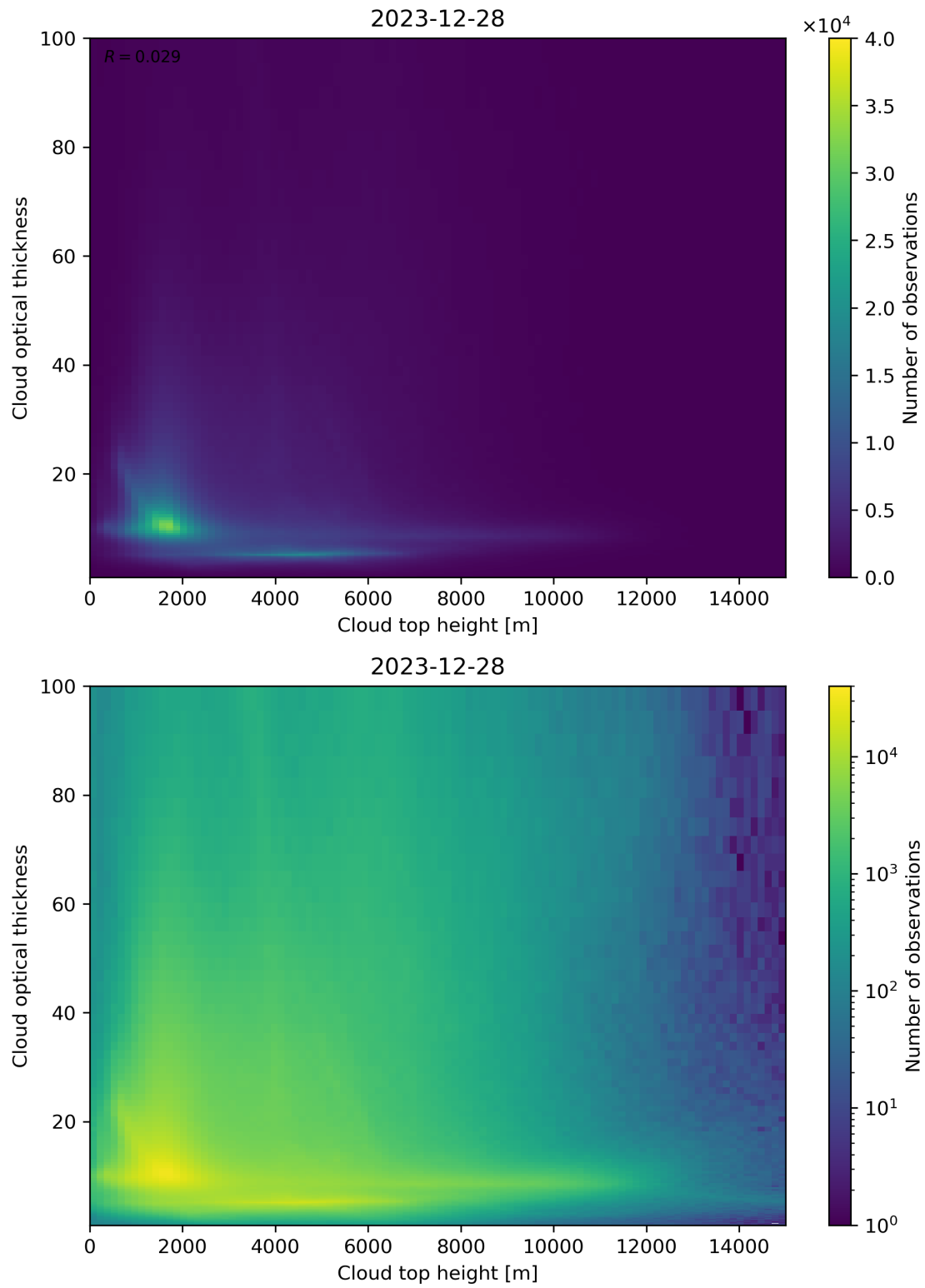
Figure 90: Scatter density plot of “Cloud top height” against “Cloud optical thickness” for 2023-12-27 to 2023-12-29.
