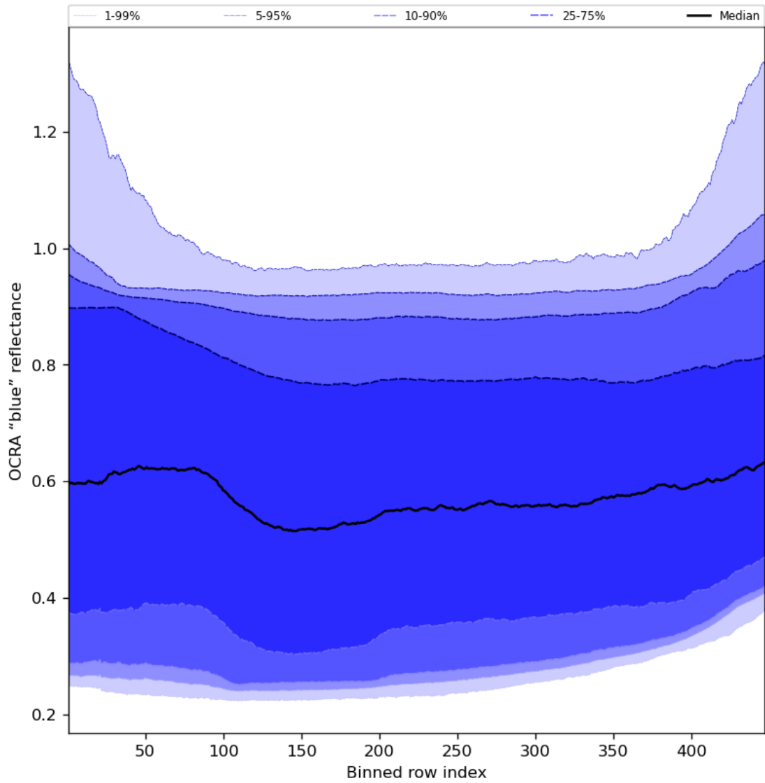
Figure 67: Along track statistics of “OCRA “blue” reflectance” for 2023-12-27 to 2023-12-29
