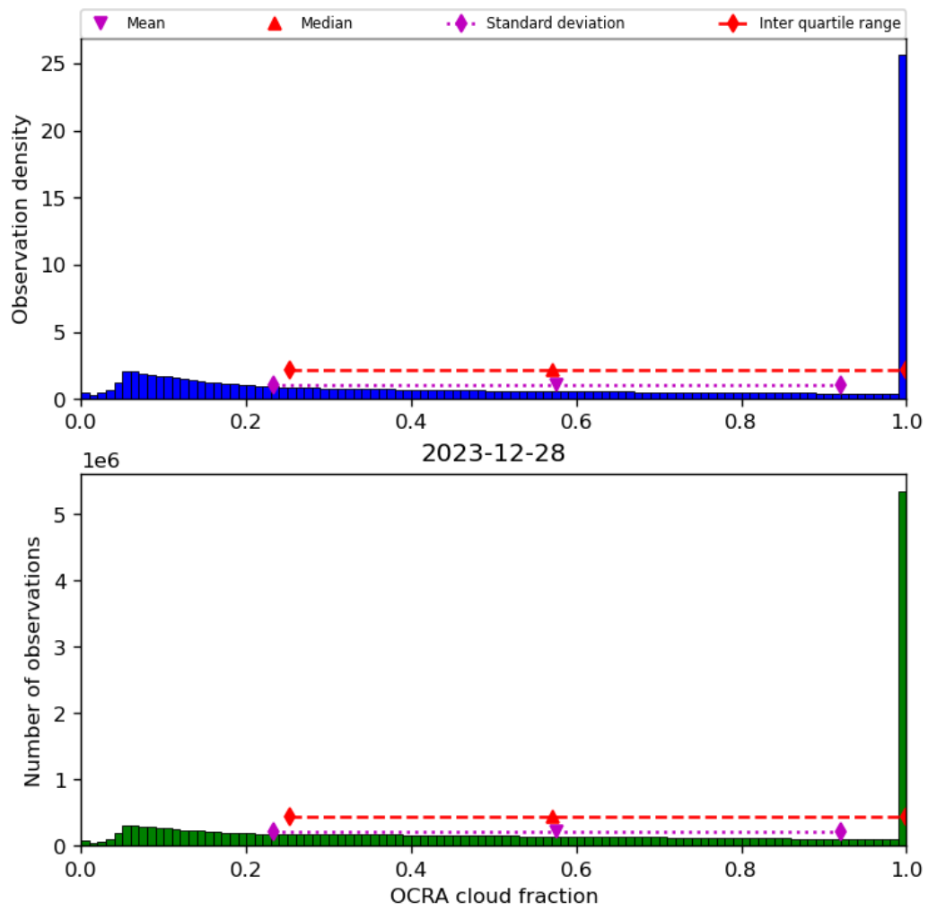
Figure 50: Histogram of “OCRA cloud fraction” for 2023-12-27 to 2023-12-29
