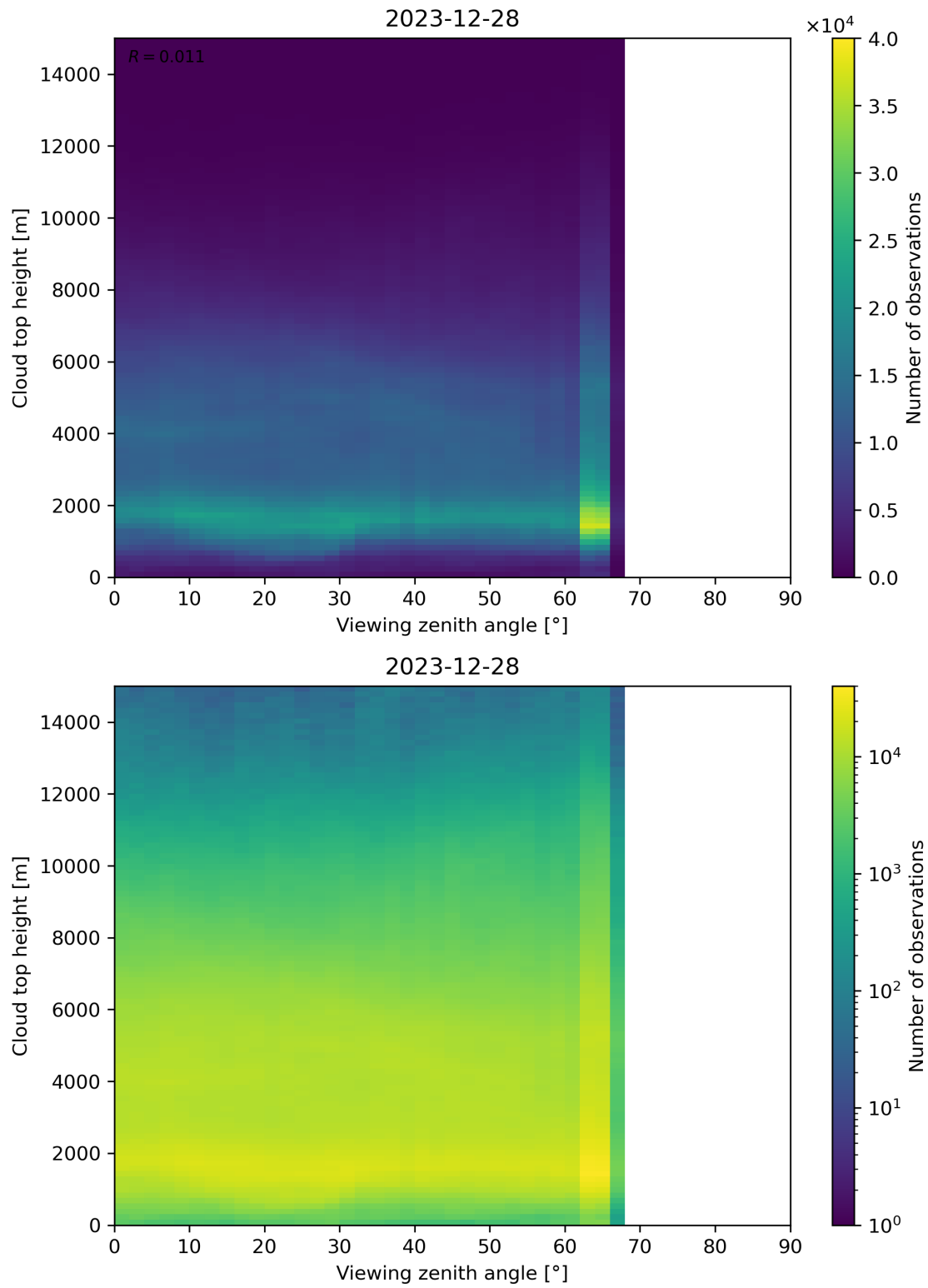
Figure 112: Scatter density plot of “Viewing zenith angle” against “Cloud top height” for 2023-12-27 to 2023-12-29.
