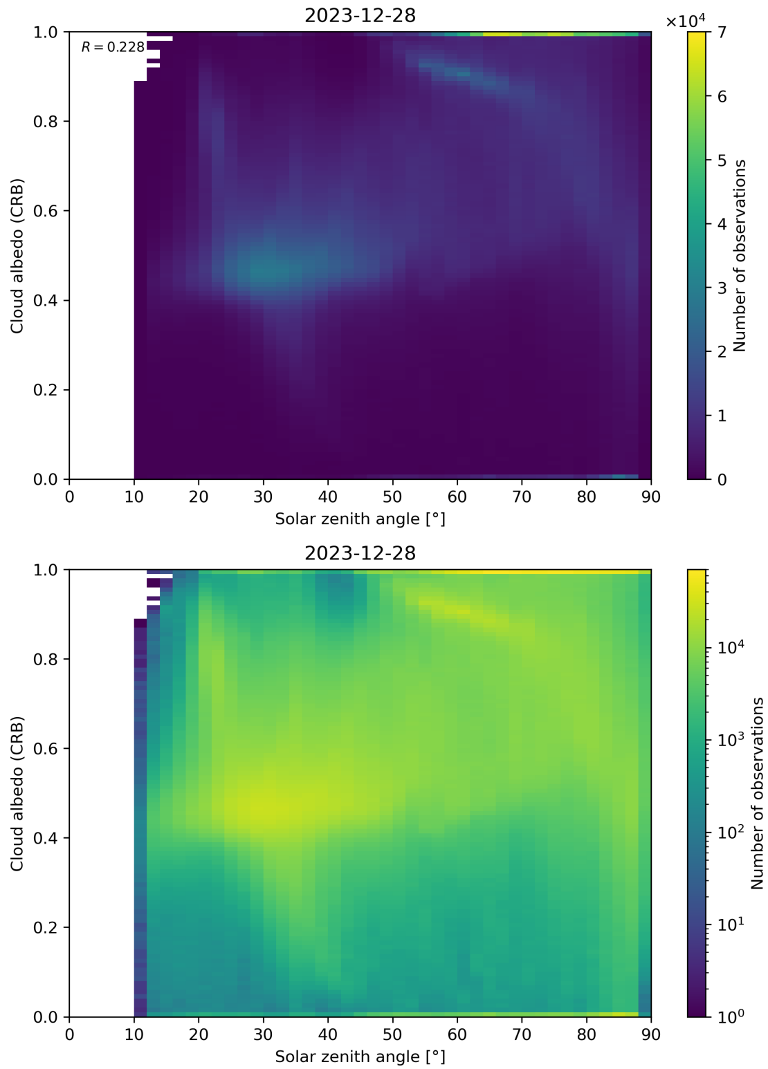
Figure 98: Scatter density plot of “Solar zenith angle” against “Cloud albedo (CRB)” for 2023-12-27 to 2023-12-29.
