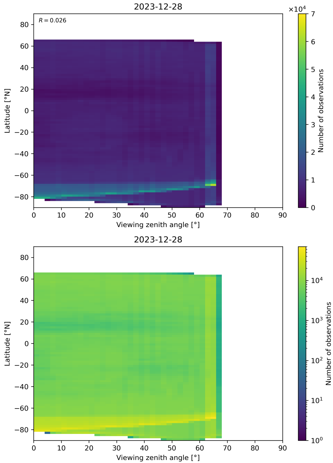
Figure 113: Scatter density plot of “Viewing zenith angle” against “Latitude” for 2023-12-27 to 2023-12-29.
