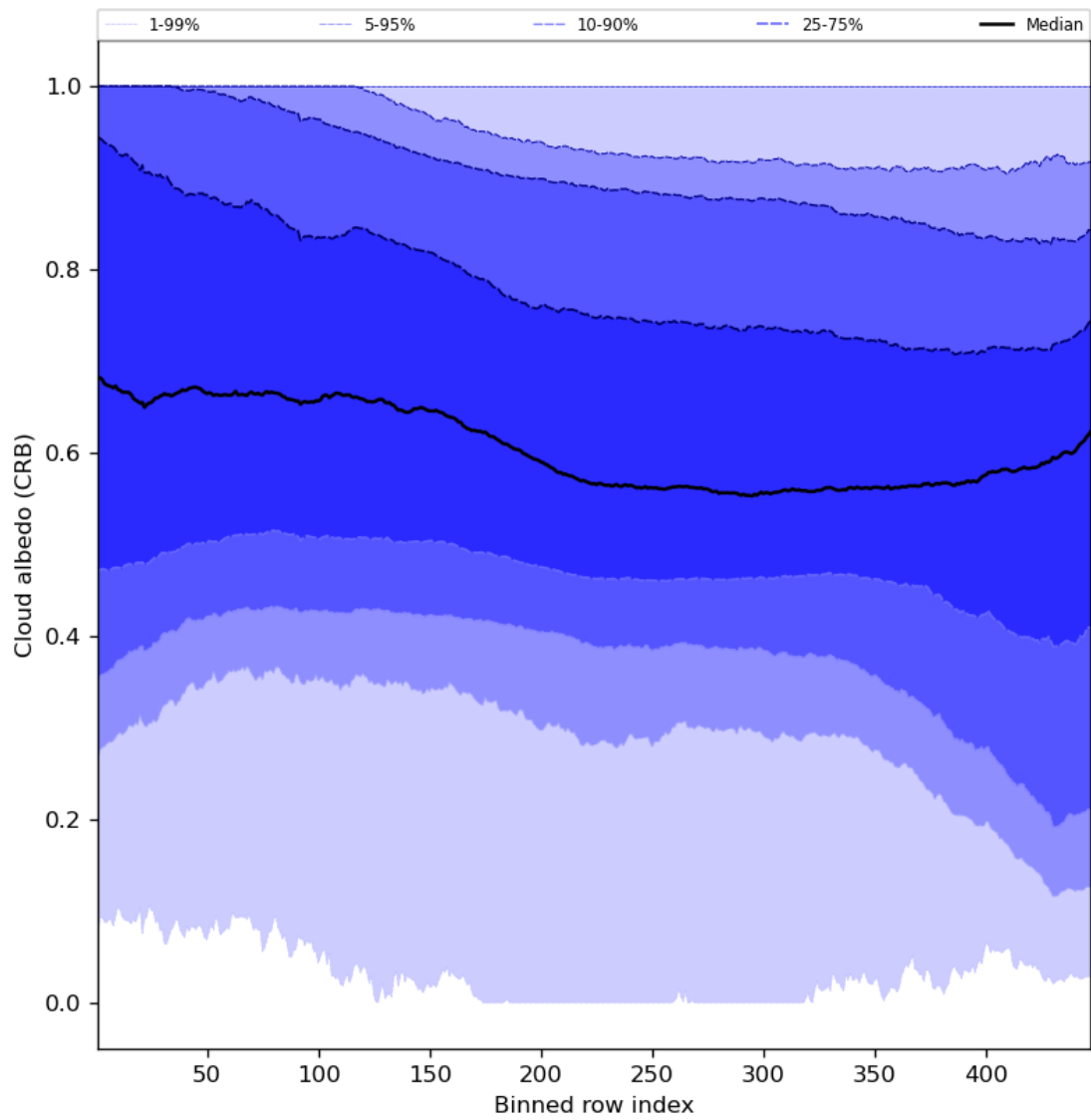
Figure 60: Along track statistics of “Cloud albedo (CRB)” for 2023-12-27 to 2023-12-29
