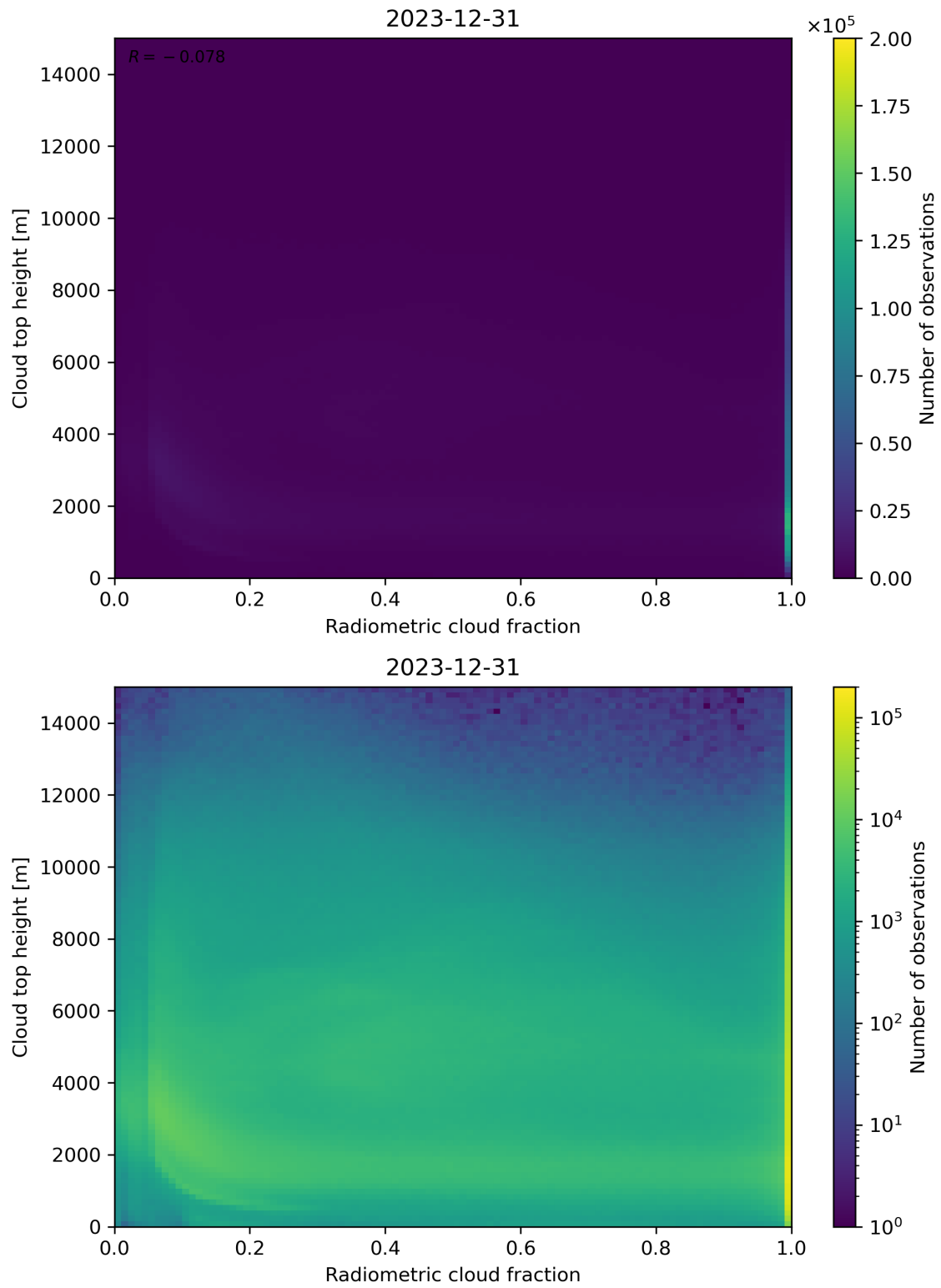
Figure 76: Scatter density plot of “Radiometric cloud fraction” against “Cloud top height” for 2023-12-30 to 2023-12-31.
