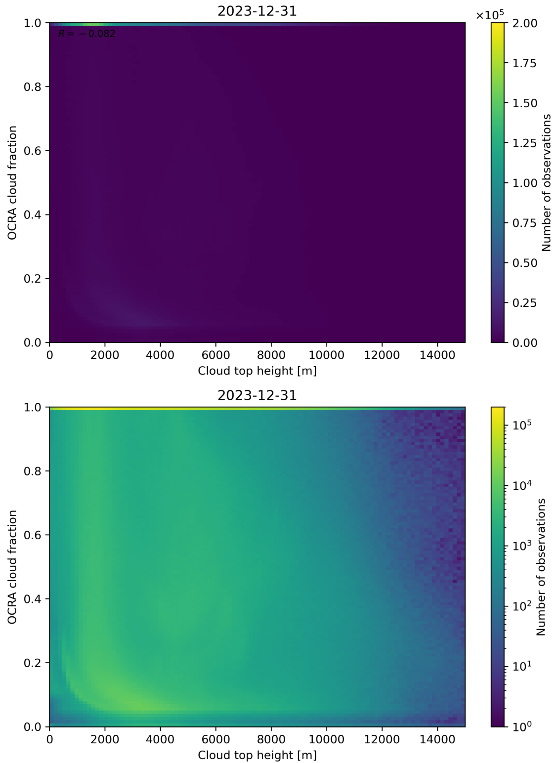
Figure 87: Scatter density plot of “Cloud top height” against “OCRA cloud fraction” for 2023-12-30 to 2023-12-31.
