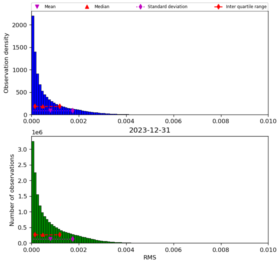
Figure 47: Histogram of “RMS” for 2023-12-30 to 2023-12-31
