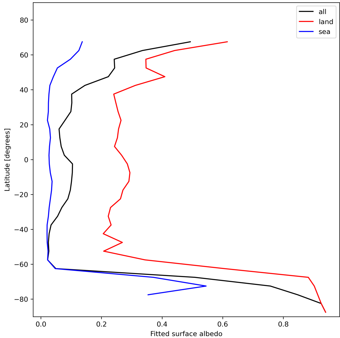
Figure 29: Zonal average of “Fitted surface albedo” for 2023-12-30 to 2023-12-31.
