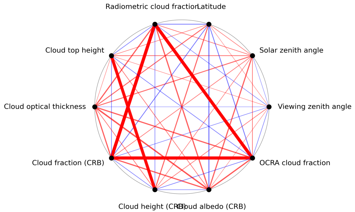
Figure 1: Map of correlation graph for 2023-12-30 to 2023-12-31.
