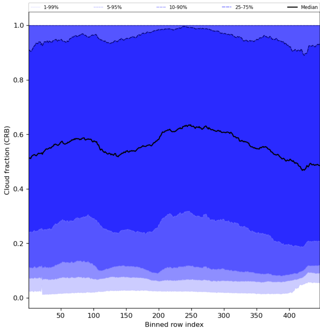
Figure 58: Along track statistics of “Cloud fraction (CRB)” for 2023-12-30 to 2023-12-31
