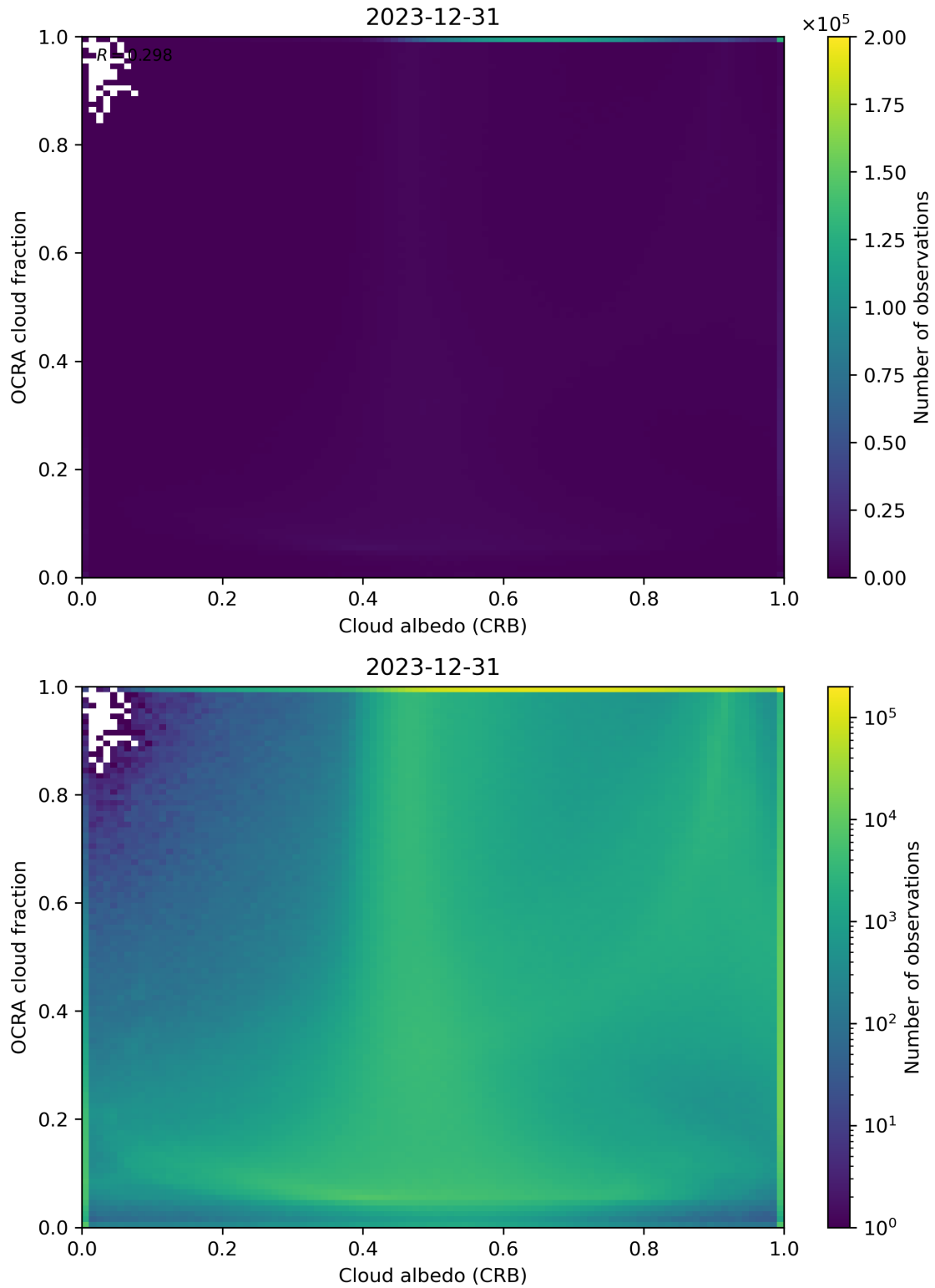
Figure 70: Scatter density plot of “Cloud albedo (CRB)” against “OCRA cloud fraction” for 2023-12-30 to 2023-12-31.
