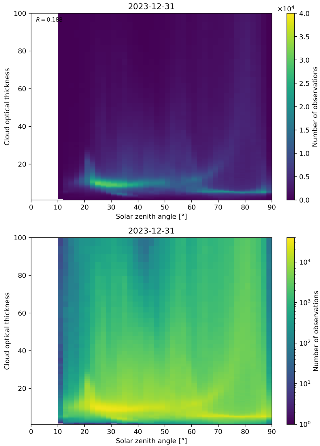
Figure 103: Scatter density plot of “Solar zenith angle” against “Cloud optical thickness” for 2023-12-30 to 2023-12-31.
