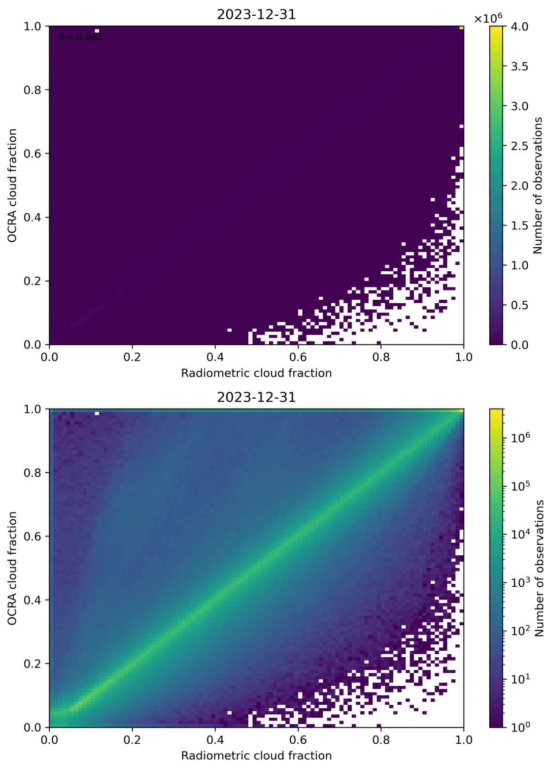
Figure 72: Scatter density plot of “Radiometric cloud fraction” against “OCRA cloud fraction” for 2023-12-30 to 2023-12-31.
