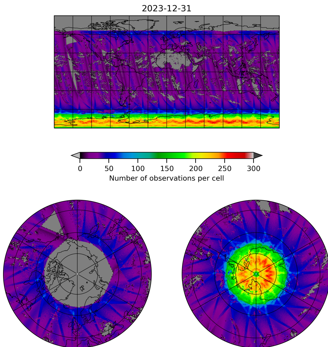
Figure 21: Map of the number of observations for 2023-12-30 to 2023-12-31
