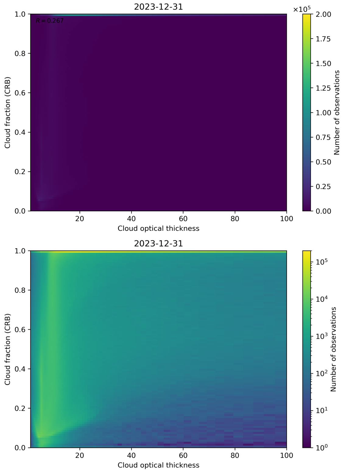
Figure 84: Scatter density plot of “Cloud optical thickness” against “Cloud fraction (CRB)” for 2023-12-30 to 2023-12-31.
