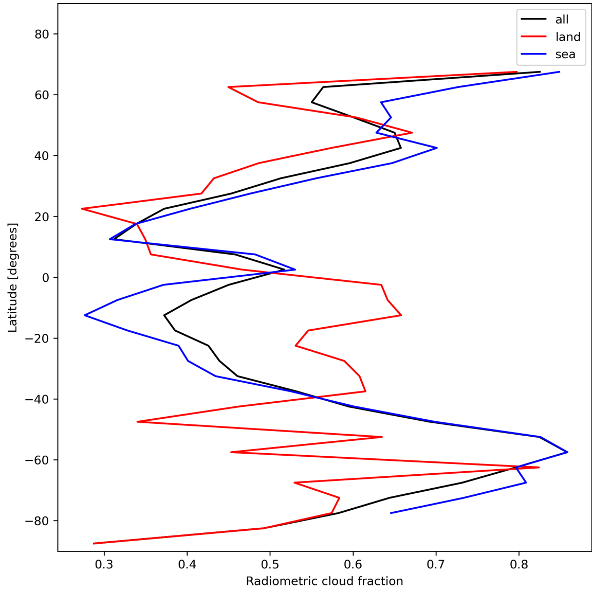
Figure 23: Zonal average of “Radiometric cloud fraction” for 2023-12-30 to 2023-12-31.
