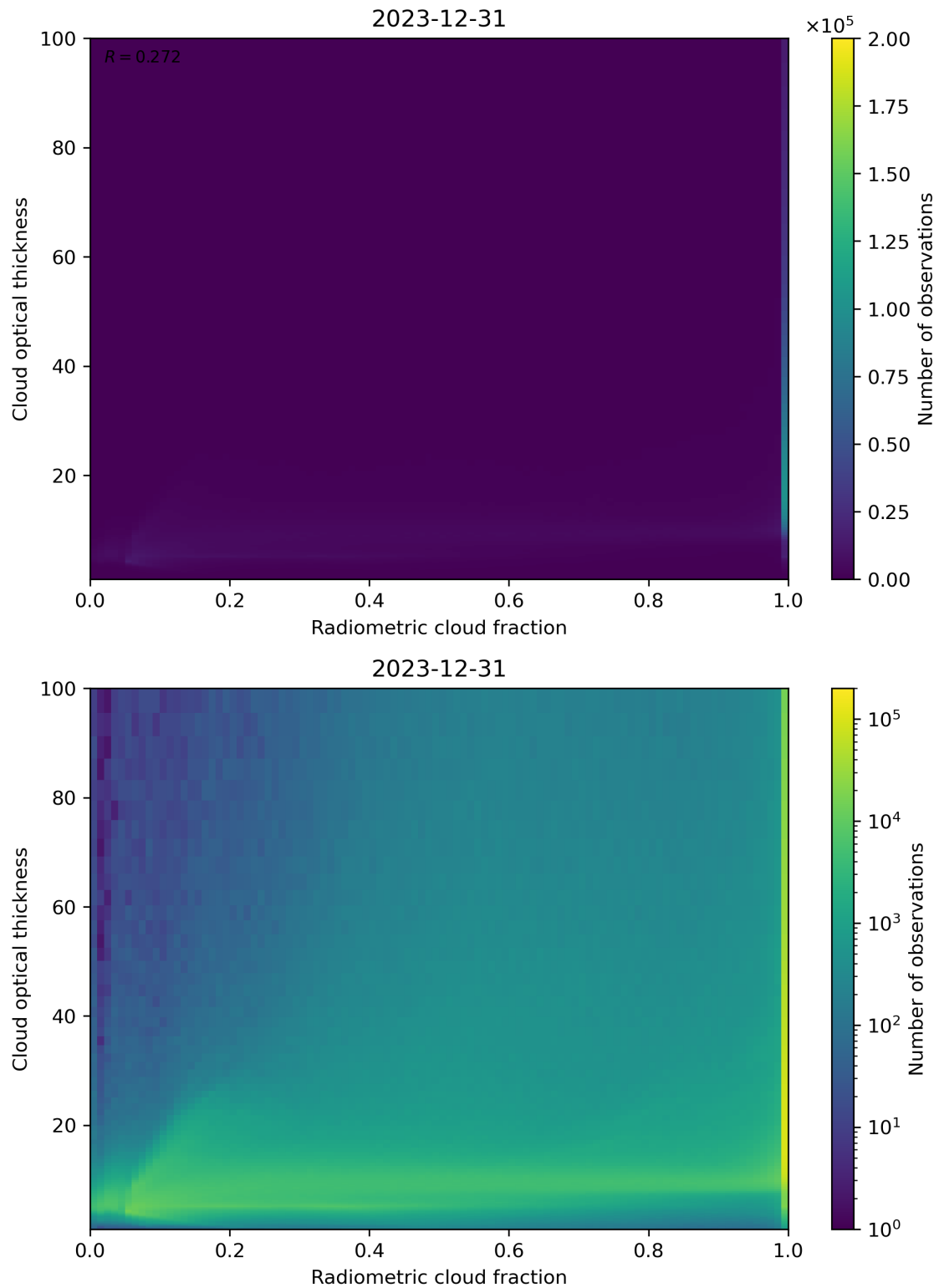
Figure 75: Scatter density plot of “Radiometric cloud fraction” against “Cloud optical thickness” for 2023-12-30 to 2023-12-31.
