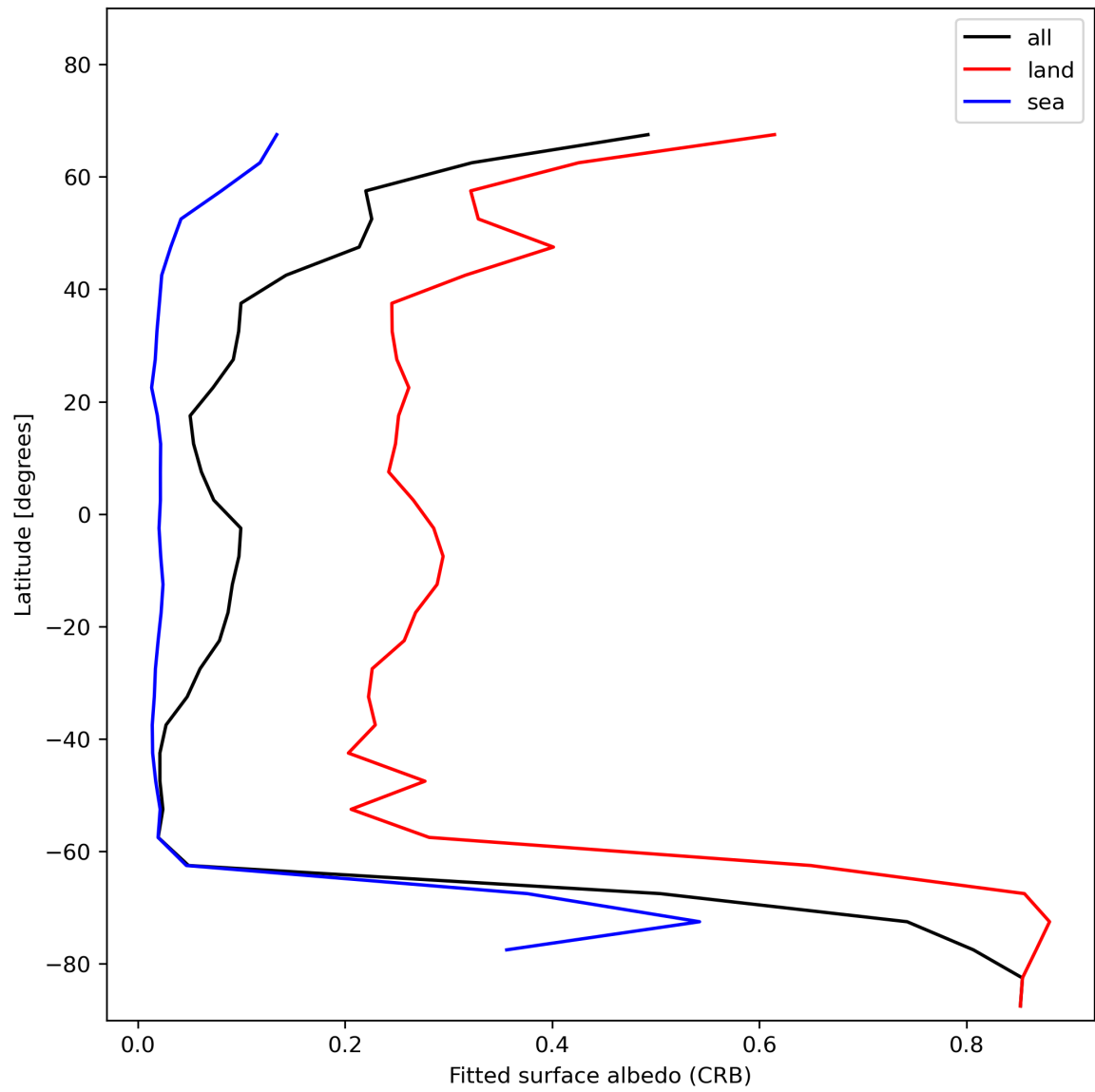
Figure 30: Zonal average of “Fitted surface albedo (CRB)” for 2023-12-30 to 2023-12-31.
