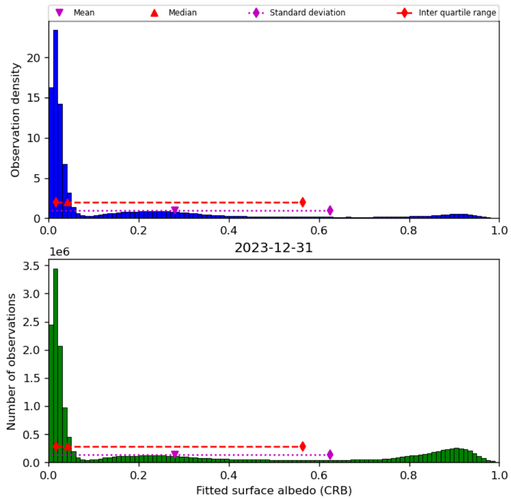
Figure 46: Histogram of “Fitted surface albedo (CRB)” for 2023-12-30 to 2023-12-31
