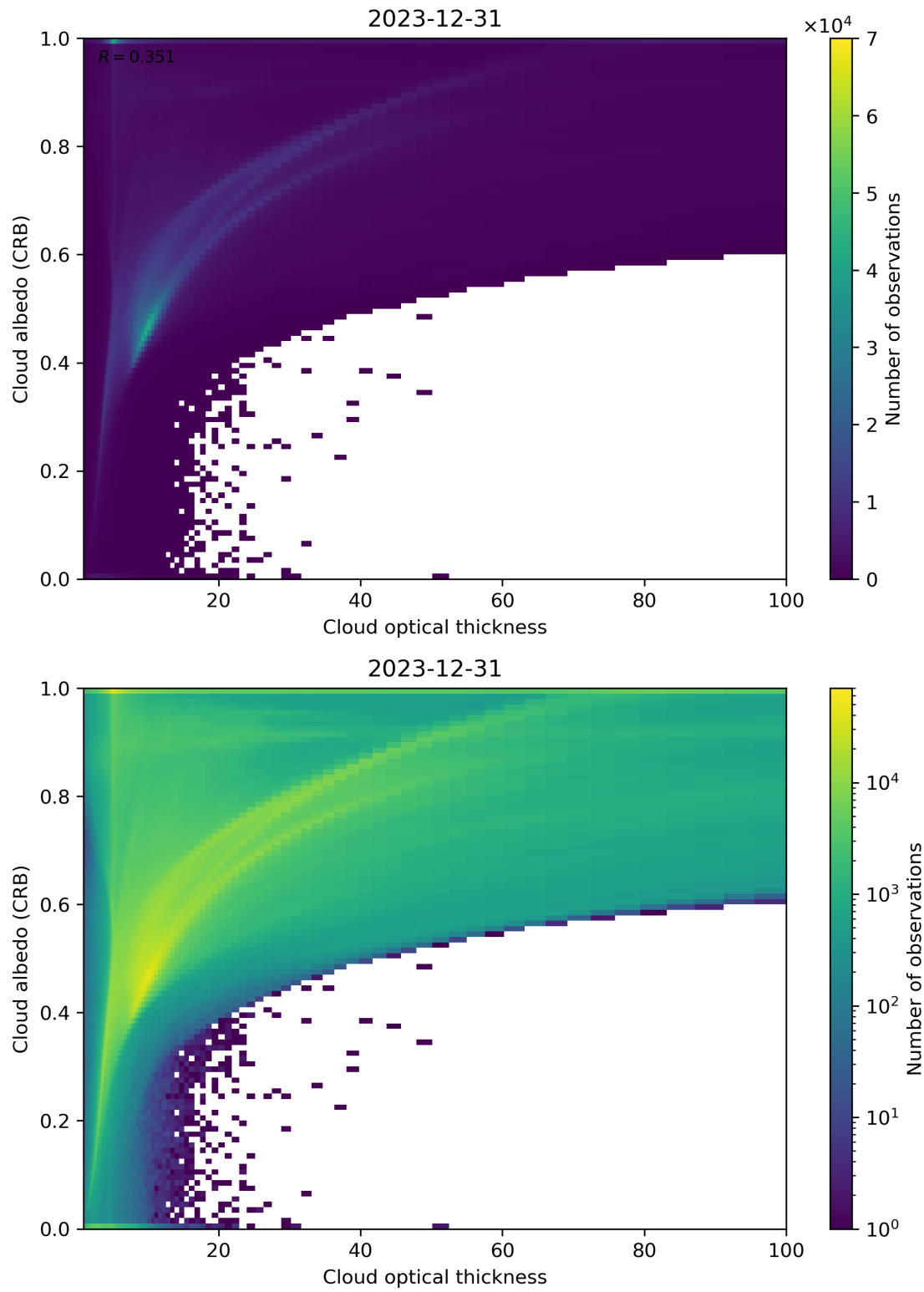
Figure 82: Scatter density plot of “Cloud optical thickness” against “Cloud albedo (CRB)” for 2023-12-30 to 2023-12-31.
