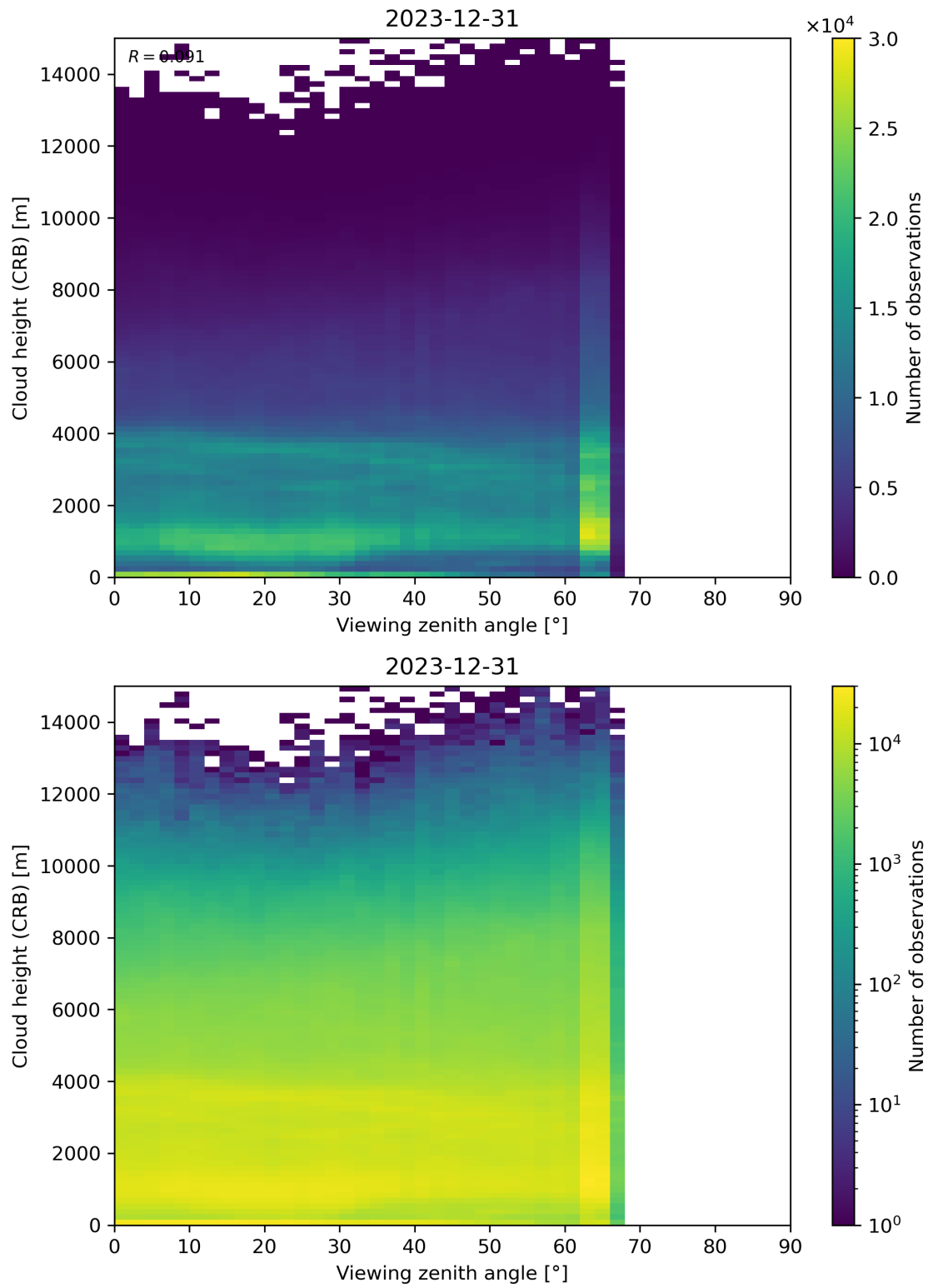
Figure 110: Scatter density plot of “Viewing zenith angle” against “Cloud height (CRB)” for 2023-12-30 to 2023-12-31.
