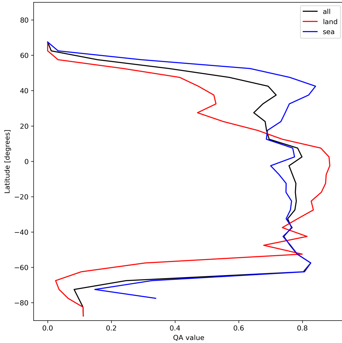
Figure 22: Zonal average of “QA value” for 2023-12-30 to 2023-12-31.
