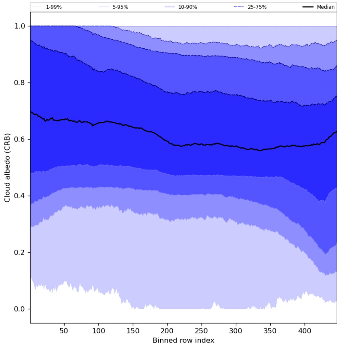
Figure 60: Along track statistics of “Cloud albedo (CRB)” for 2023-12-30 to 2023-12-31
