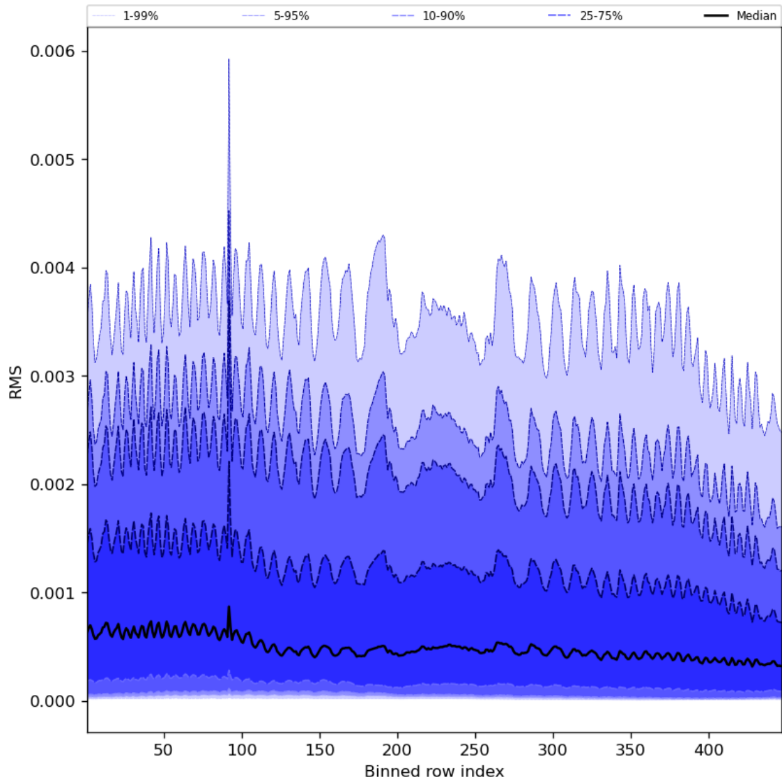
Figure 63: Along track statistics of “RMS” for 2023-12-30 to 2023-12-31
