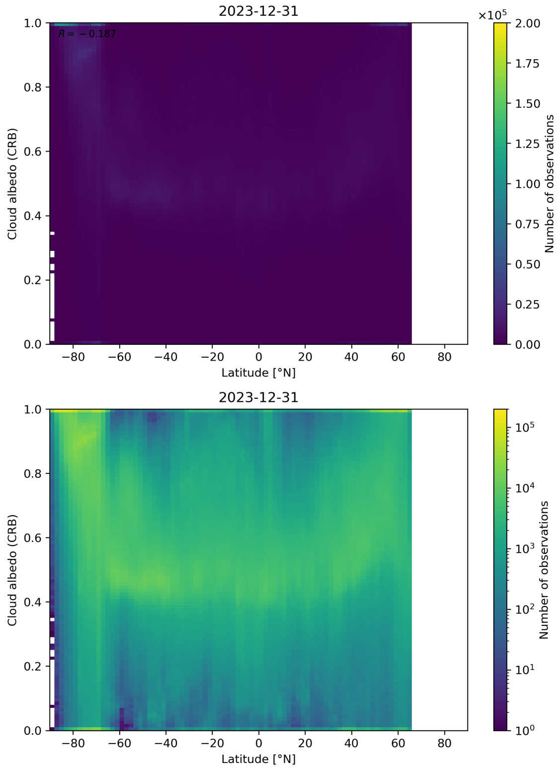
Figure 91: Scatter density plot of “Latitude” against “Cloud albedo (CRB)” for 2023-12-30 to 2023-12-31.
