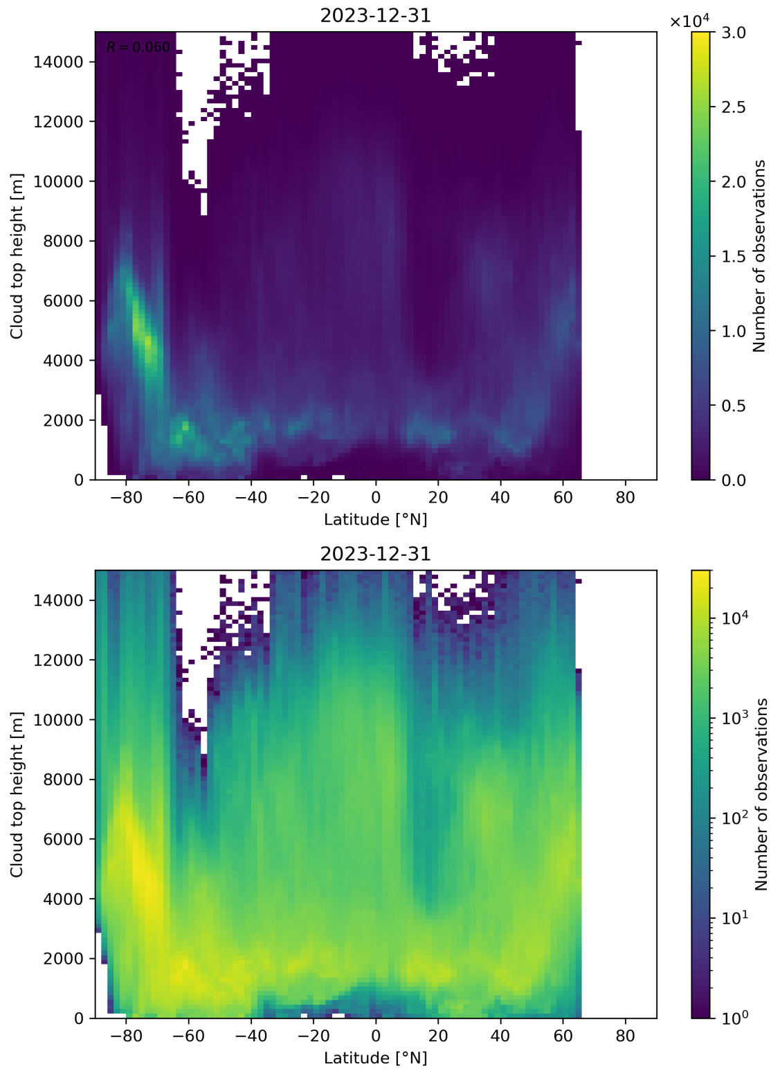
Figure 97: Scatter density plot of “Latitude” against “Cloud top height” for 2023-12-30 to 2023-12-31.
