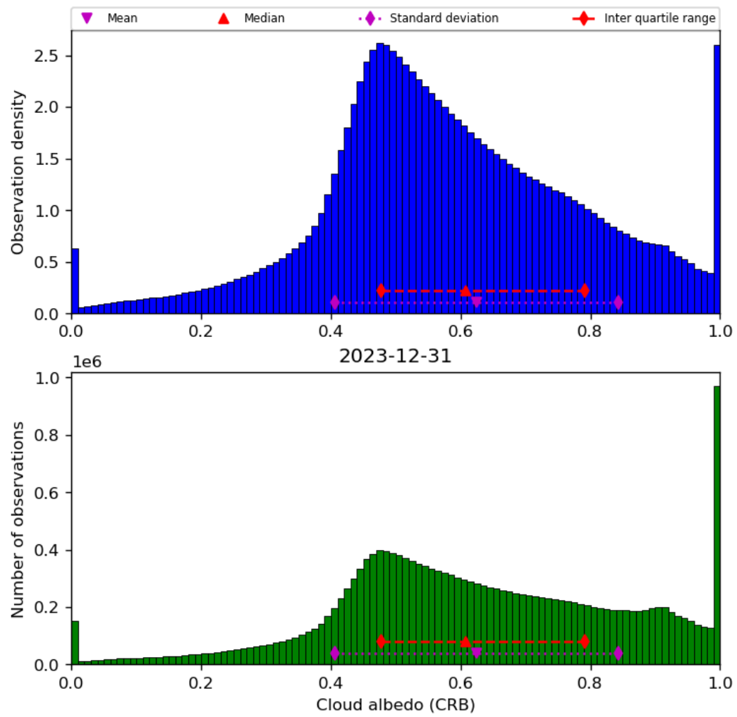
Figure 44: Histogram of “Cloud albedo (CRB)” for 2023-12-30 to 2023-12-31
