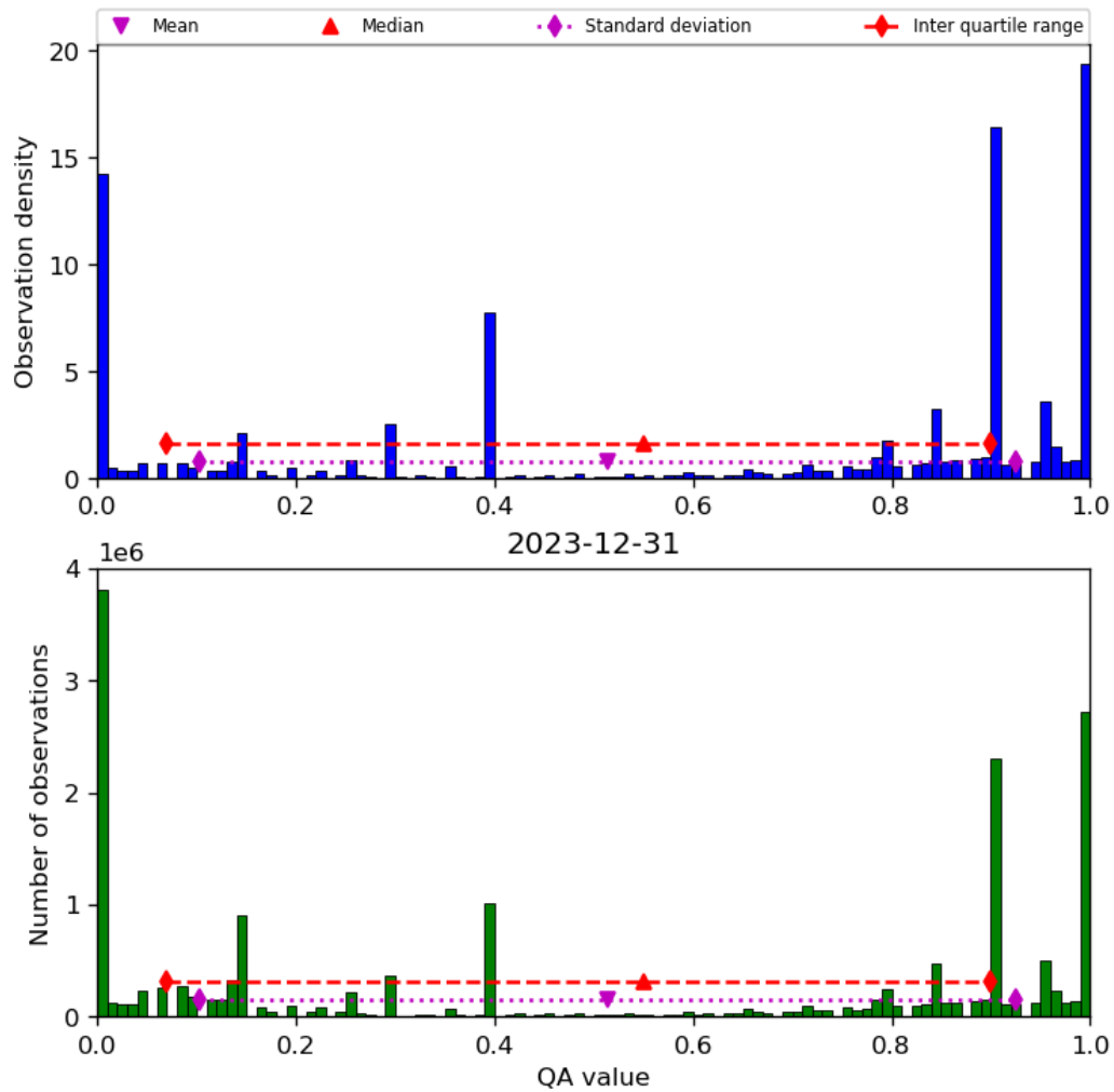
Figure 38: Histogram of “QA value” for 2023-12-30 to 2023-12-31
