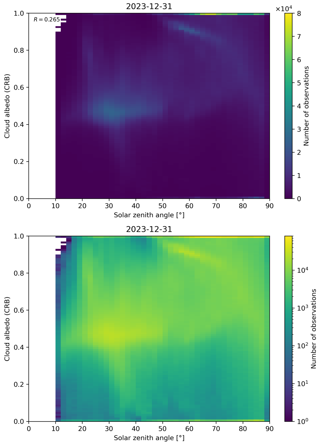
Figure 98: Scatter density plot of “Solar zenith angle” against “Cloud albedo (CRB)” for 2023-12-30 to 2023-12-31.
