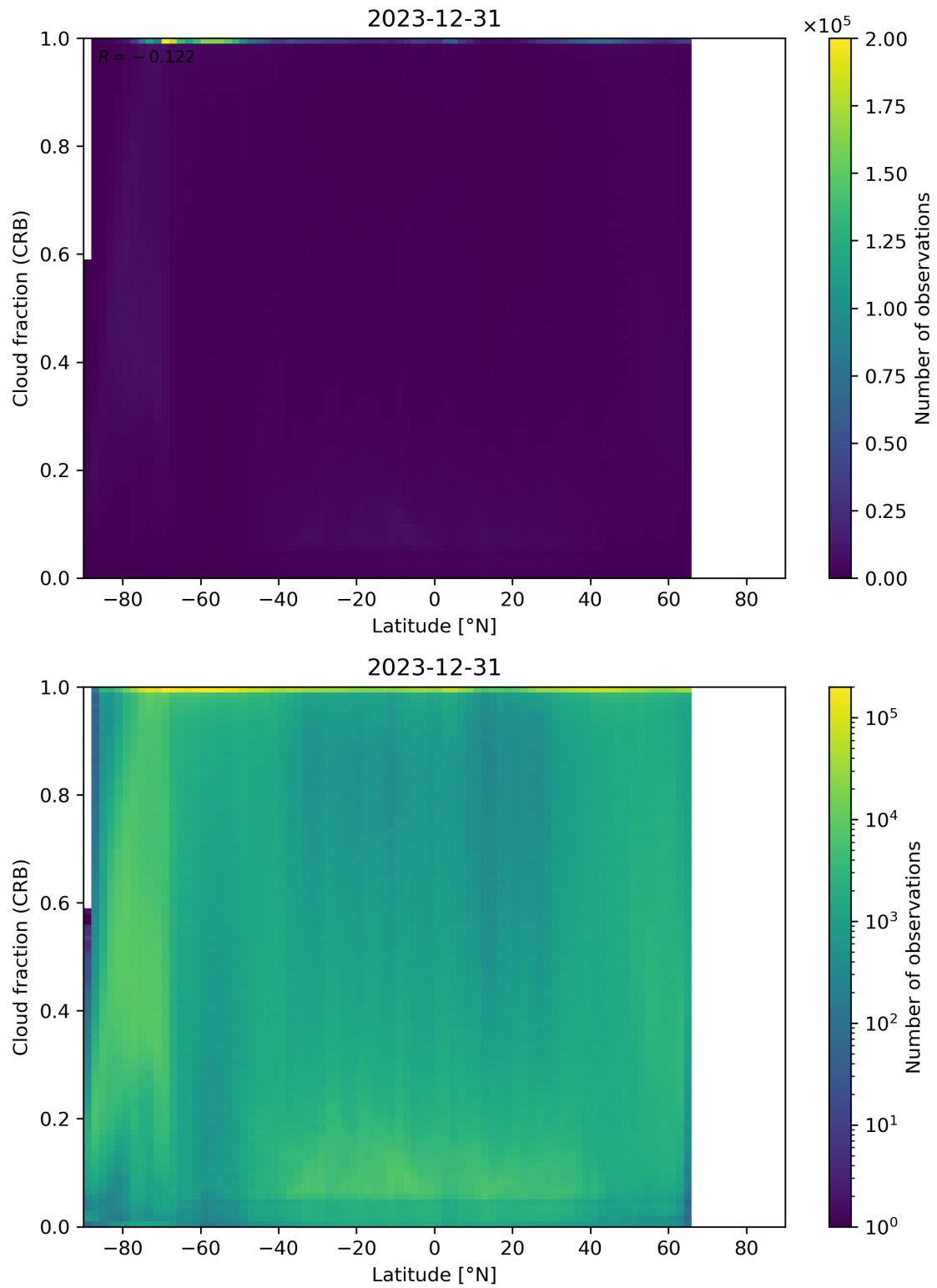
Figure 94: Scatter density plot of “Latitude” against “Cloud fraction (CRB)” for 2023-12-30 to 2023-12-31.
