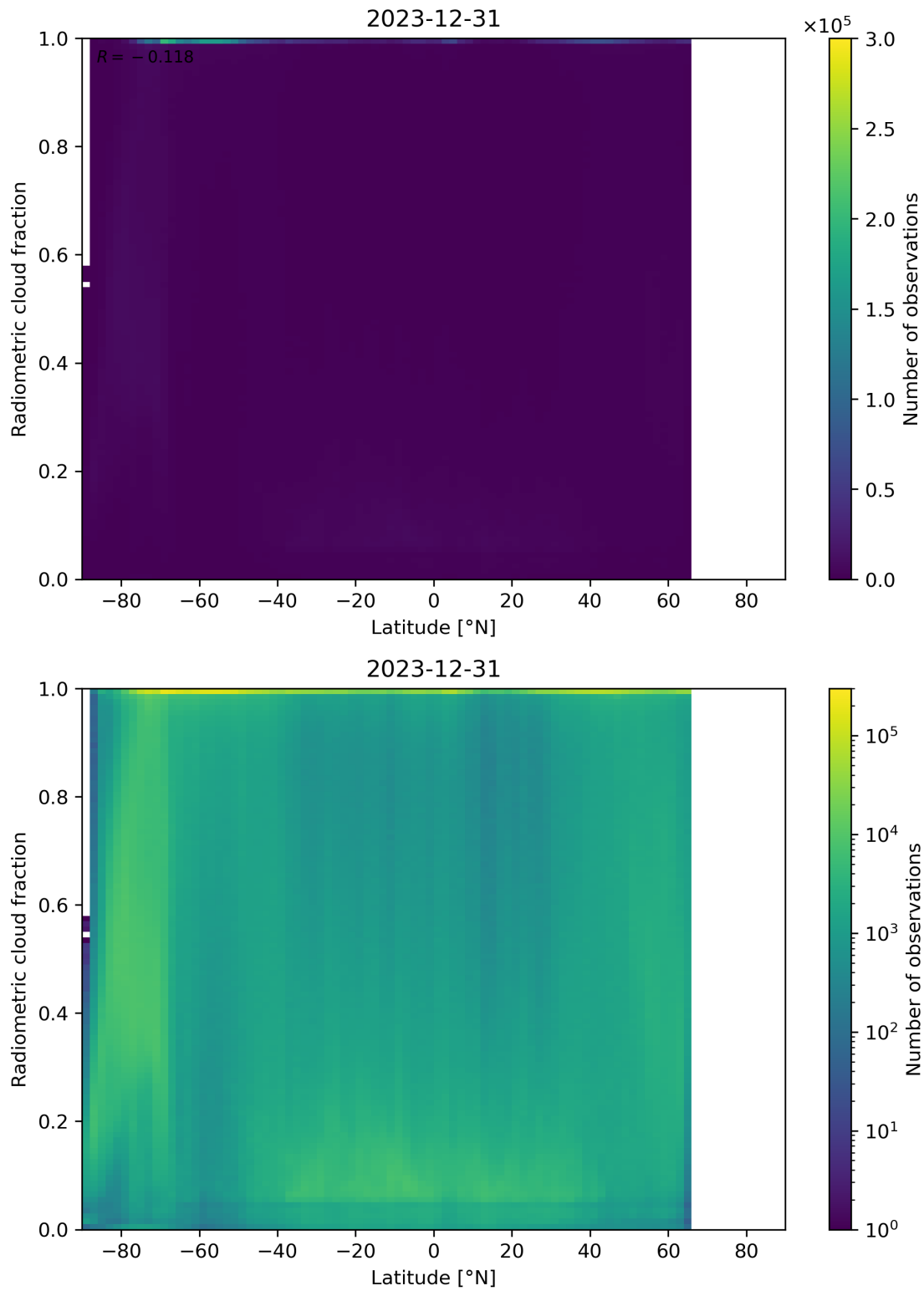
Figure 92: Scatter density plot of “Latitude” against “Radiometric cloud fraction” for 2023-12-30 to 2023-12-31.
