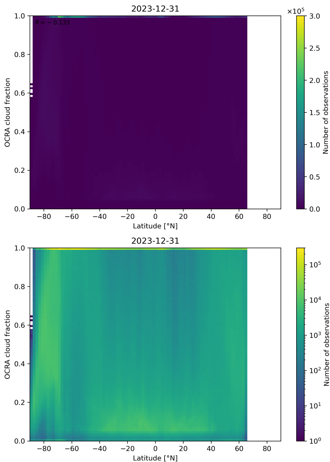
Figure 93: Scatter density plot of “Latitude” against “OCRA cloud fraction” for 2023-12-30 to 2023-12-31.
