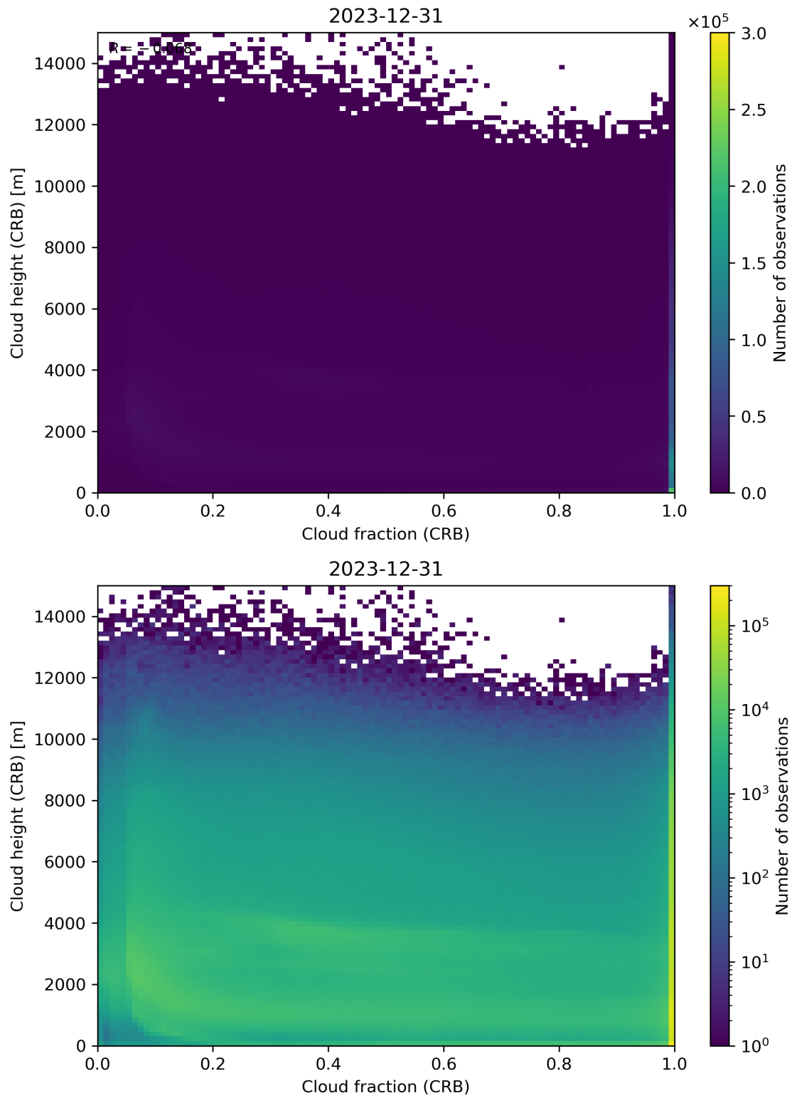
Figure 79: Scatter density plot of “Cloud fraction (CRB)” against “Cloud height (CRB)” for 2023-12-30 to 2023-12-31.
