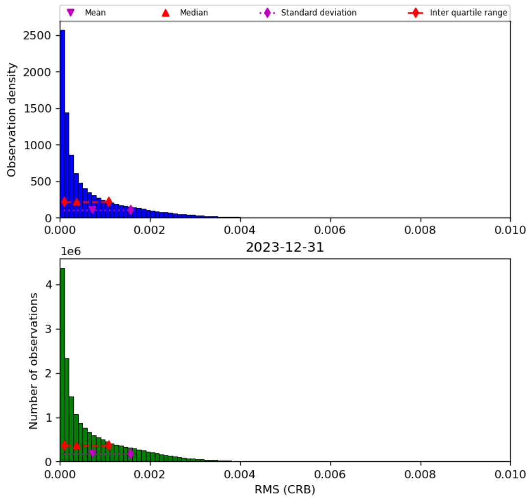
Figure 48: Histogram of “RMS (CRB)” for 2023-12-30 to 2023-12-31
