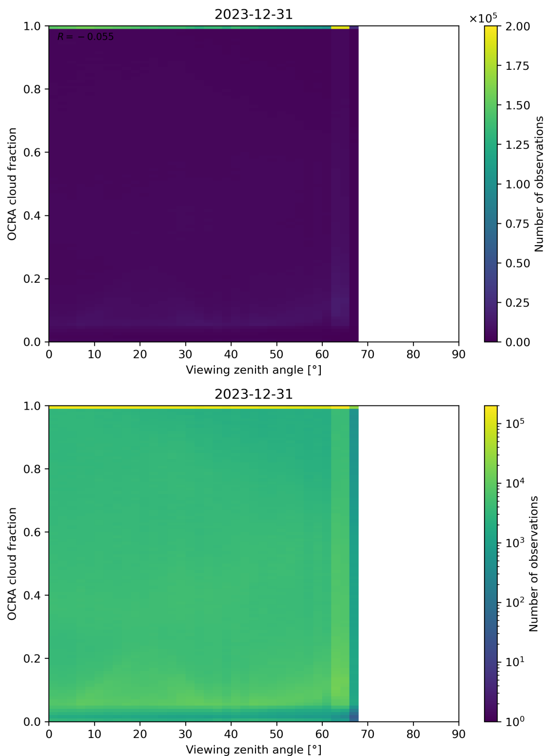
Figure 108: Scatter density plot of “Viewing zenith angle” against “OCRA cloud fraction” for 2023-12-30 to 2023-12-31.
