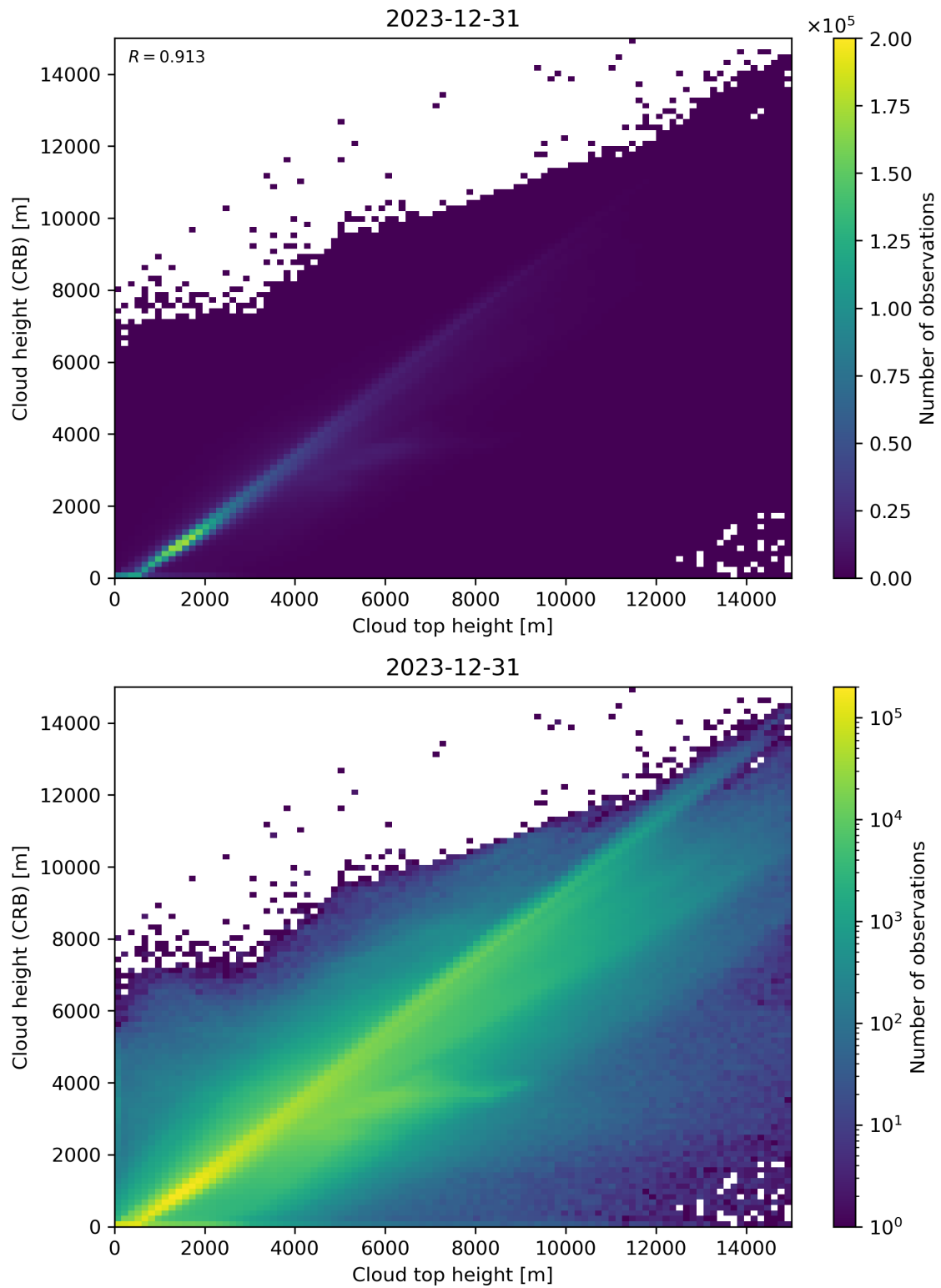
Figure 89: Scatter density plot of “Cloud top height” against “Cloud height (CRB)” for 2023-12-30 to 2023-12-31.
