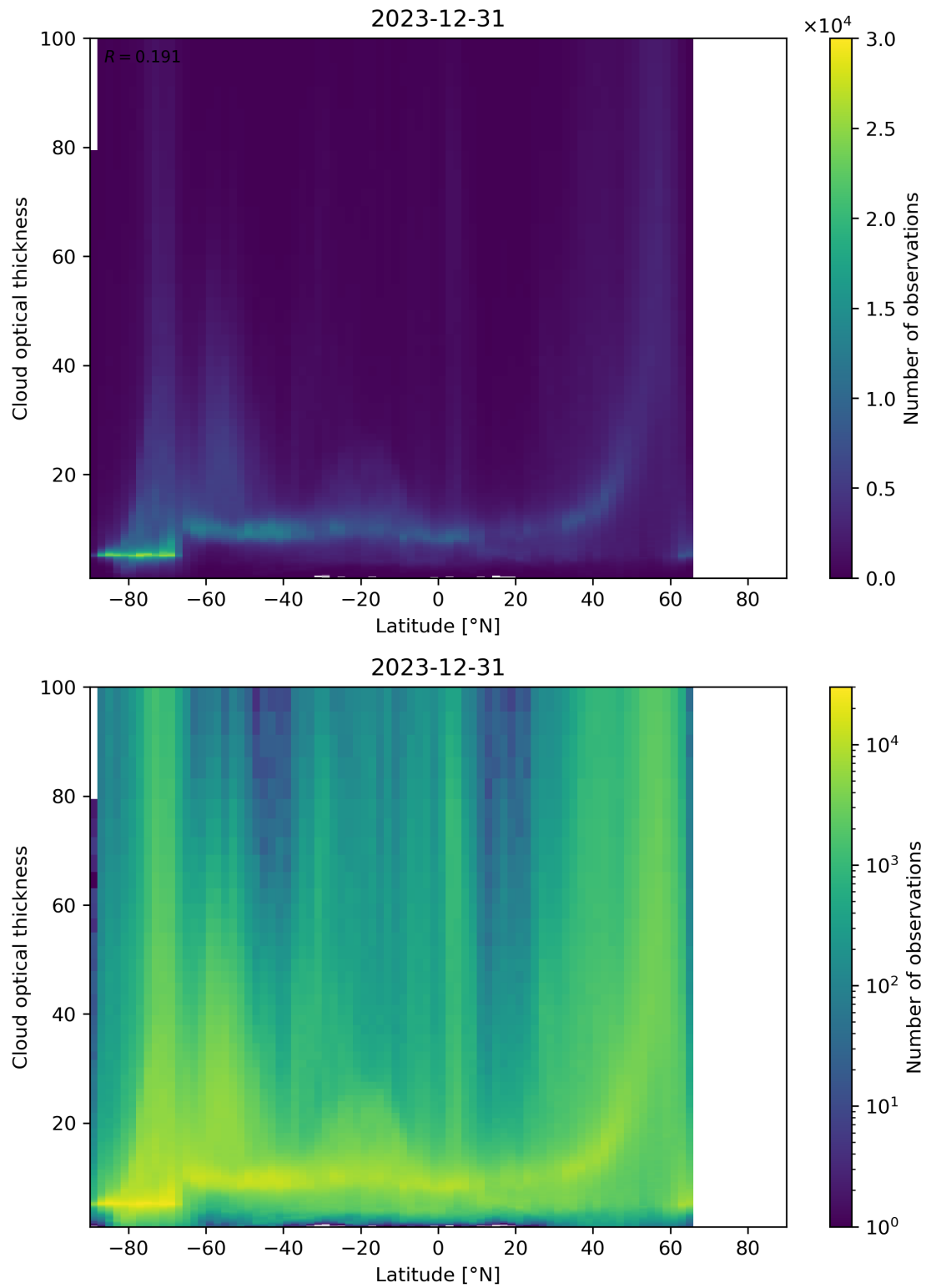
Figure 96: Scatter density plot of “Latitude” against “Cloud optical thickness” for 2023-12-30 to 2023-12-31.
