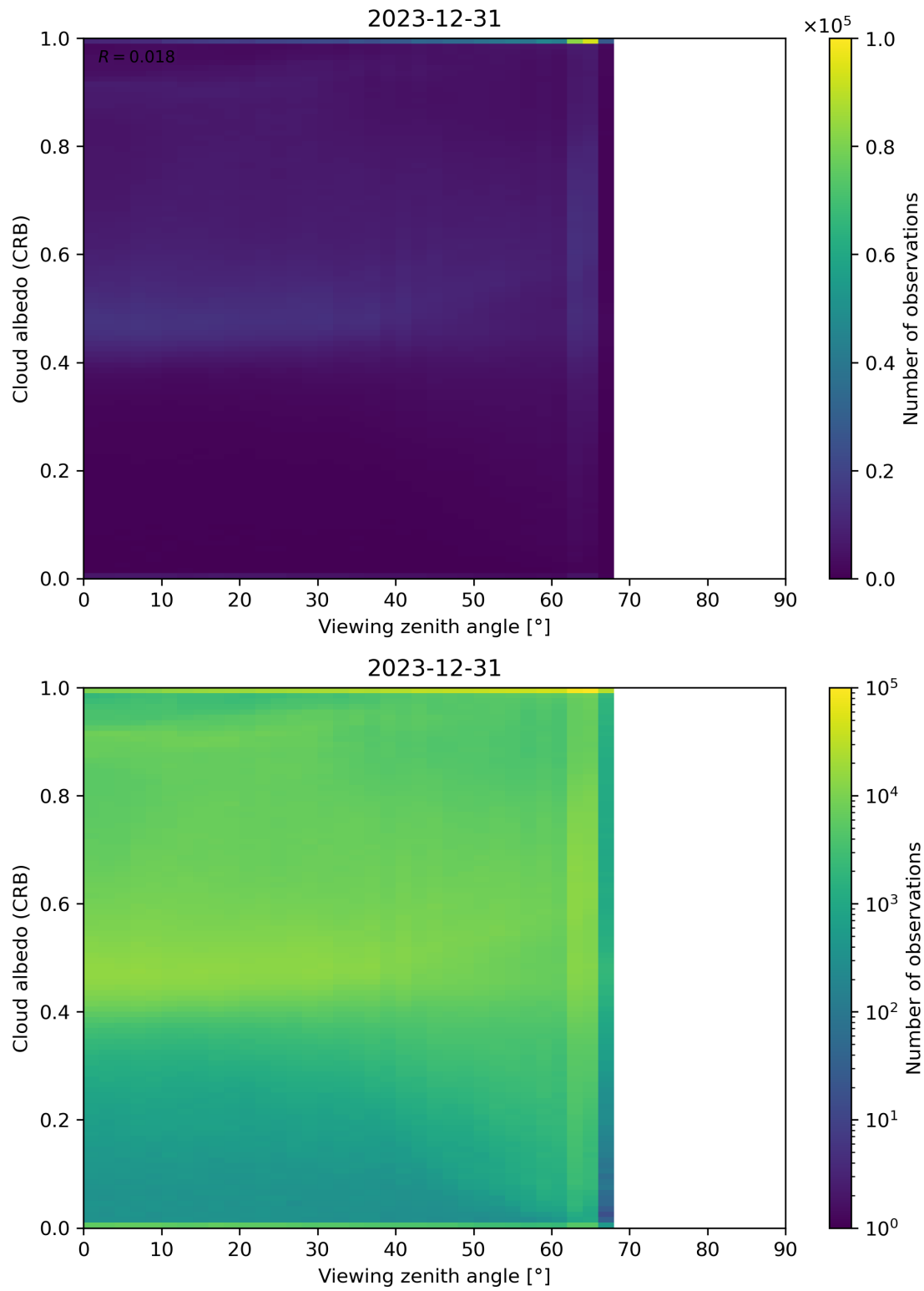
Figure 106: Scatter density plot of “Viewing zenith angle” against “Cloud albedo (CRB)” for 2023-12-30 to 2023-12-31.
