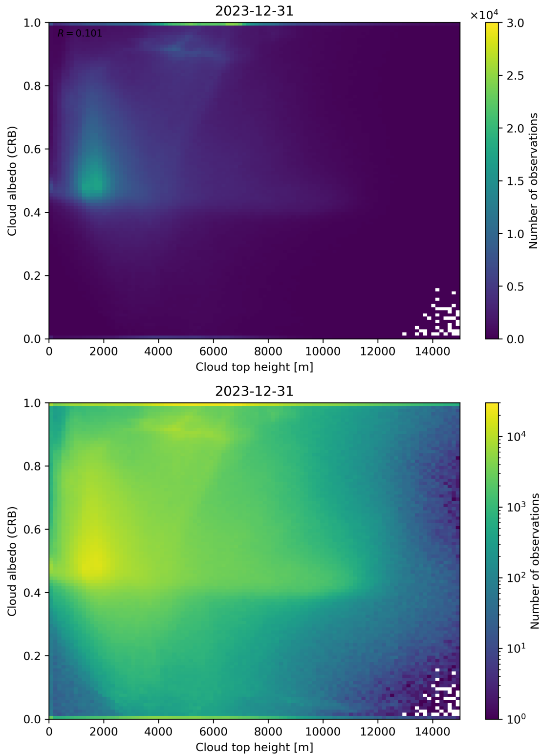
Figure 86: Scatter density plot of “Cloud top height” against “Cloud albedo (CRB)” for 2023-12-30 to 2023-12-31.
