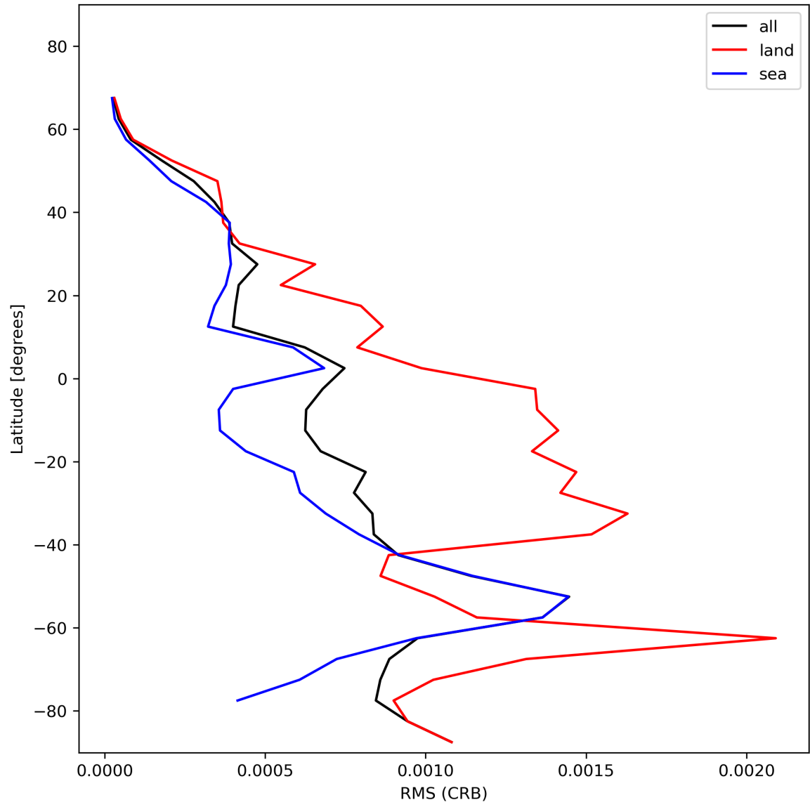
Figure 32: Zonal average of “RMS (CRB)” for 2023-12-30 to 2023-12-31.
