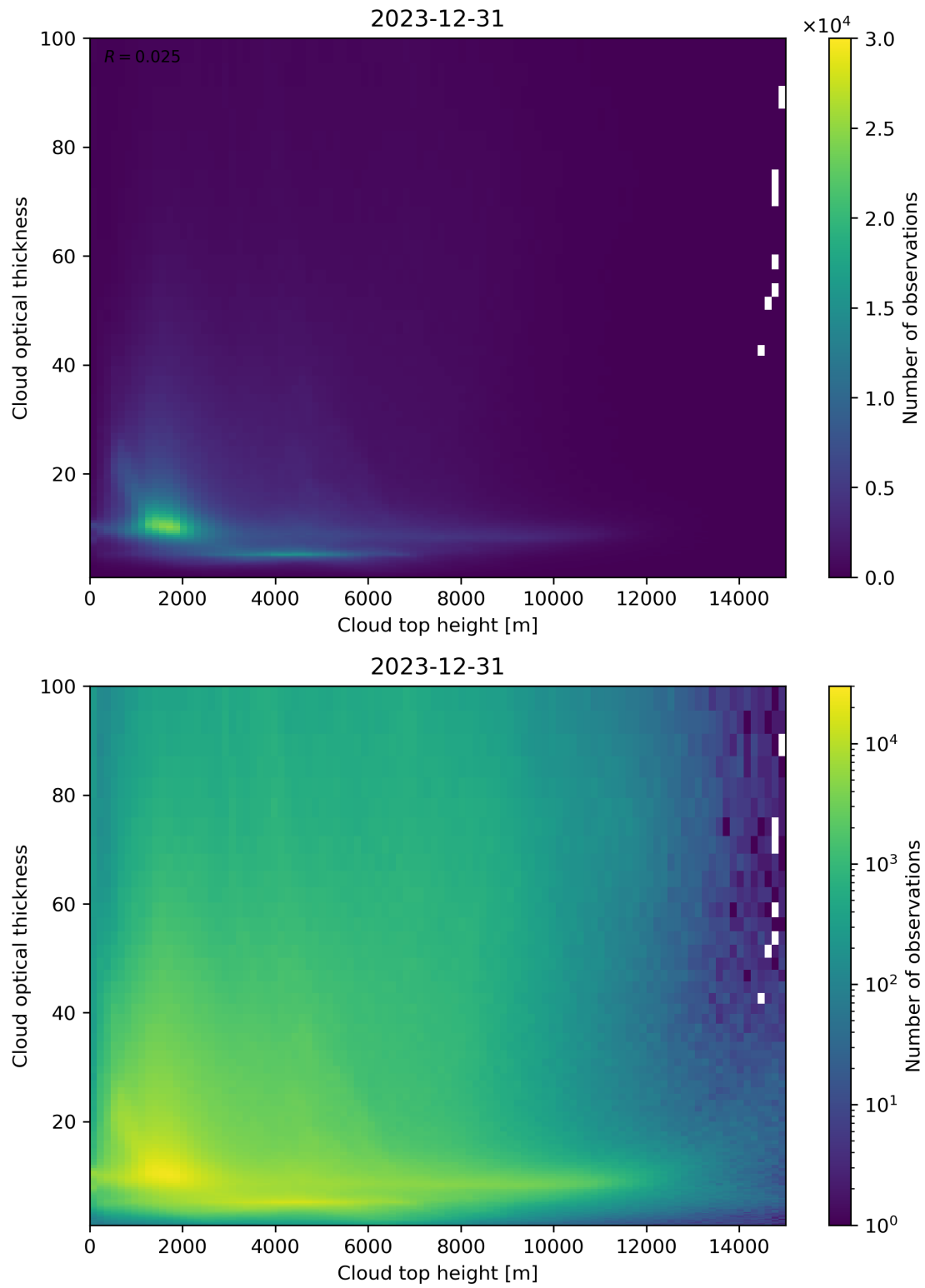
Figure 90: Scatter density plot of “Cloud top height” against “Cloud optical thickness” for 2023-12-30 to 2023-12-31.
