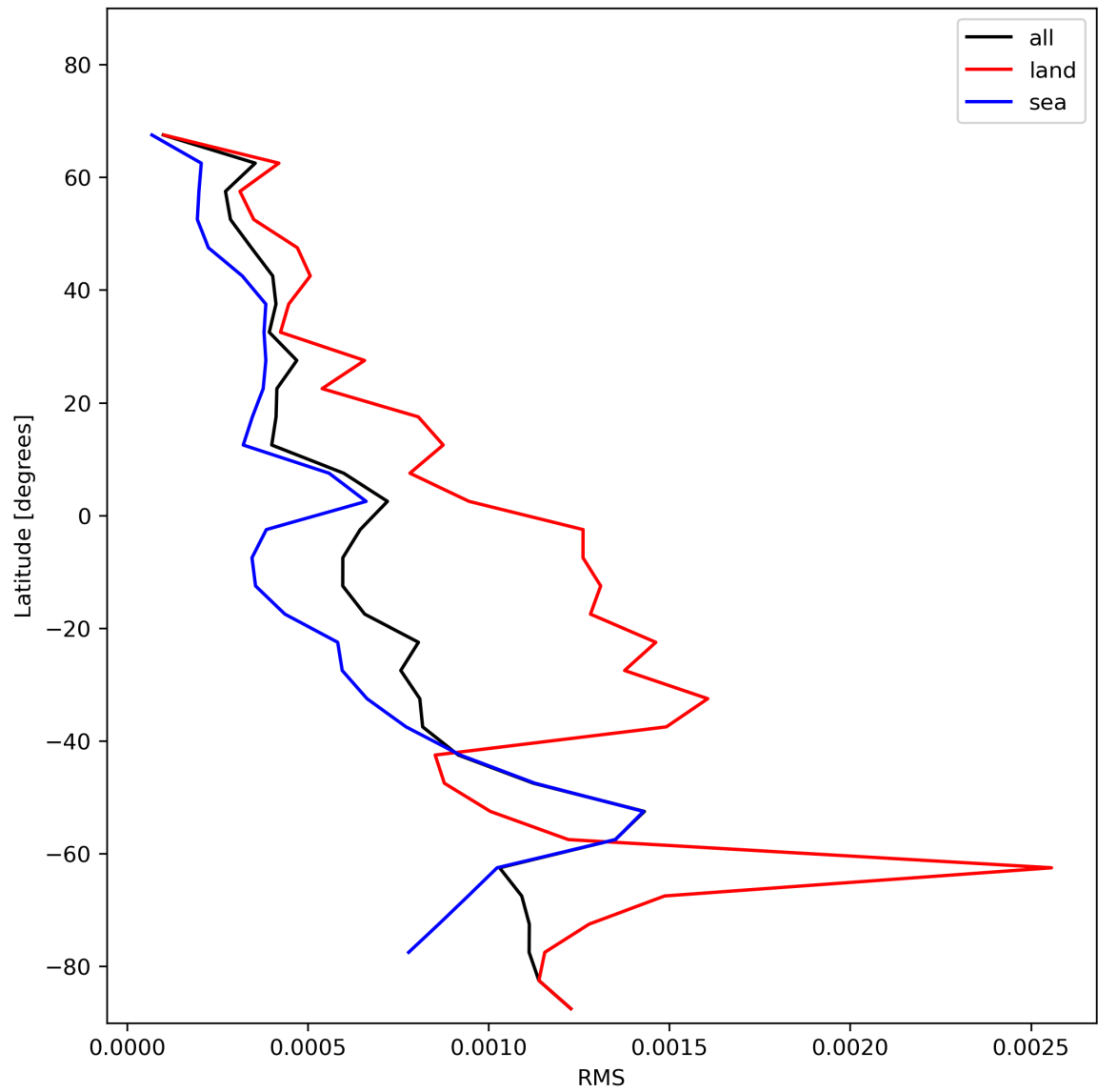
Figure 31: Zonal average of “RMS” for 2023-12-30 to 2023-12-31.
