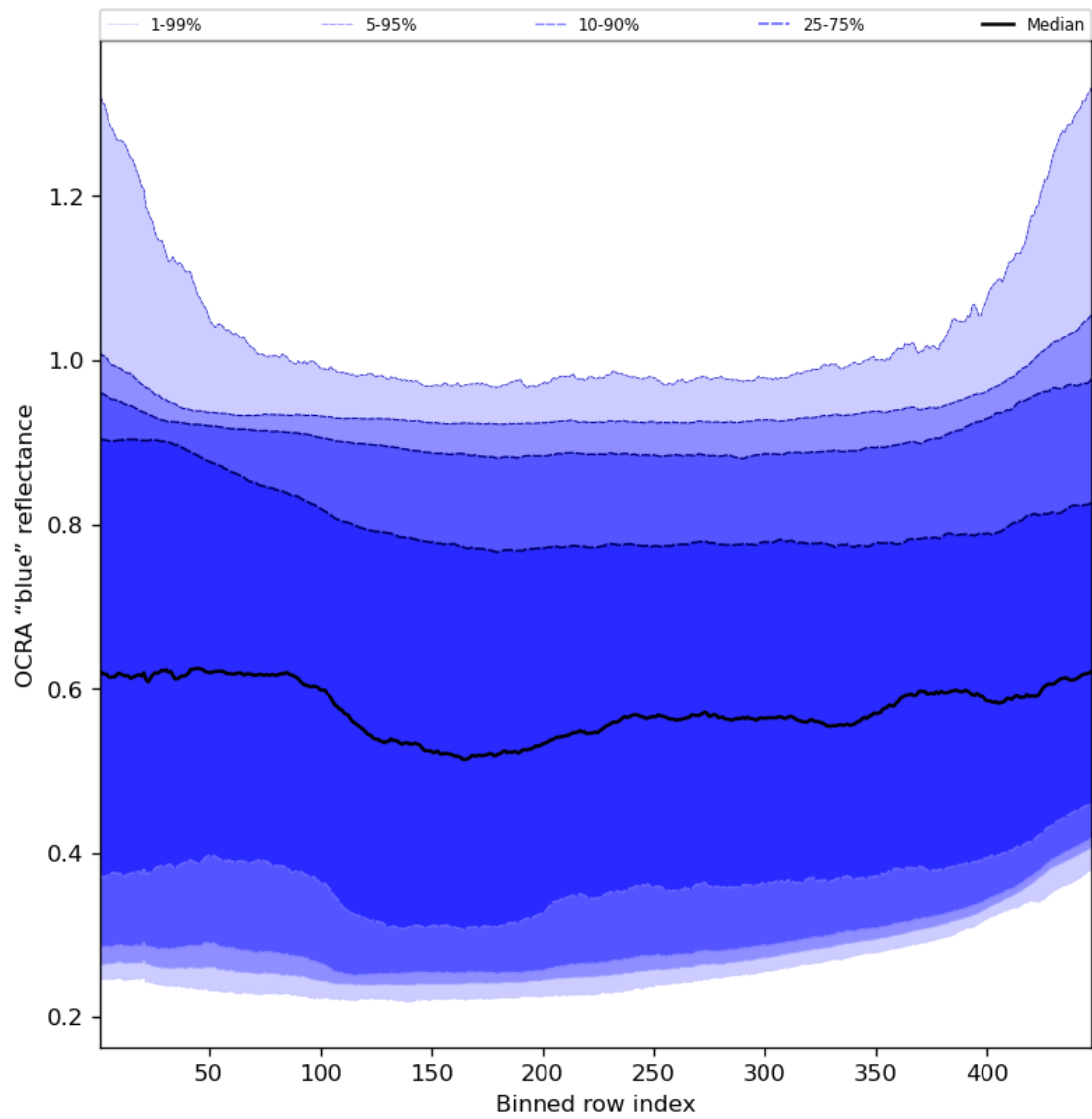
Figure 67: Along track statistics of “OCRA “blue” reflectance” for 2023-12-30 to 2023-12-31
