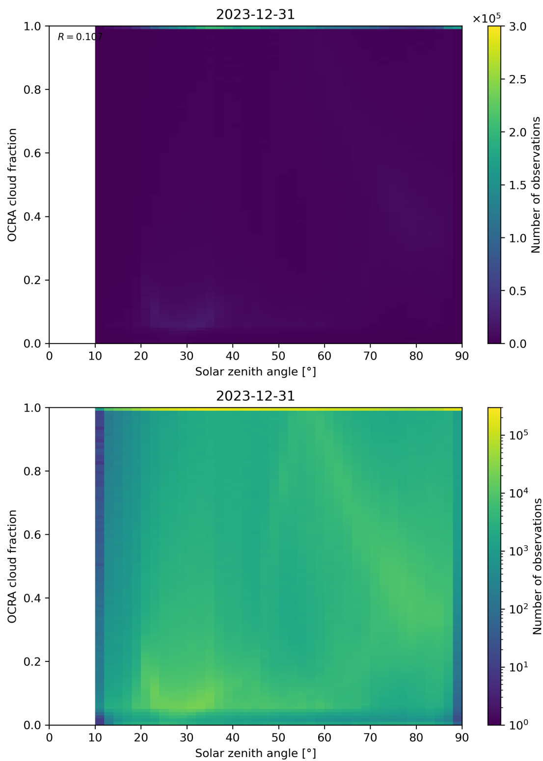
Figure 100: Scatter density plot of “Solar zenith angle” against “OCRA cloud fraction” for 2023-12-30 to 2023-12-31.
