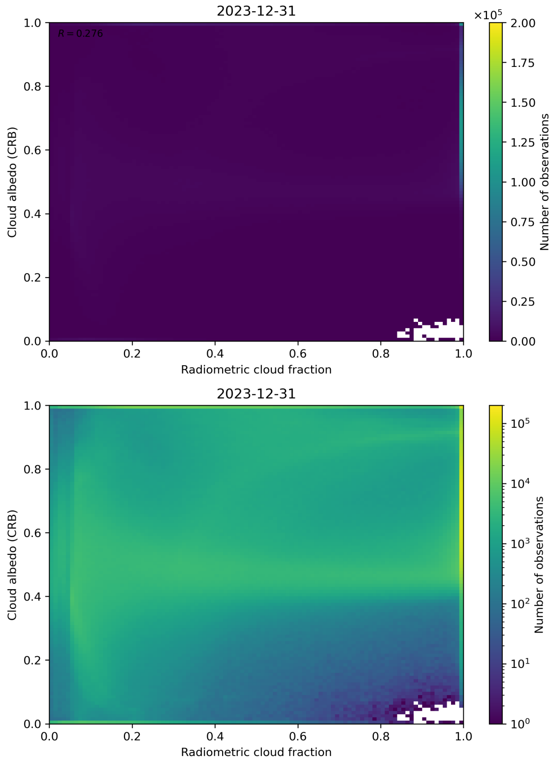
Figure 71: Scatter density plot of “Radiometric cloud fraction” against “Cloud albedo (CRB)” for 2023-12-30 to 2023-12-31.
