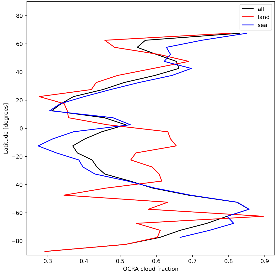
Figure 34: Zonal average of “OCRA cloud fraction” for 2023-12-30 to 2023-12-31.
