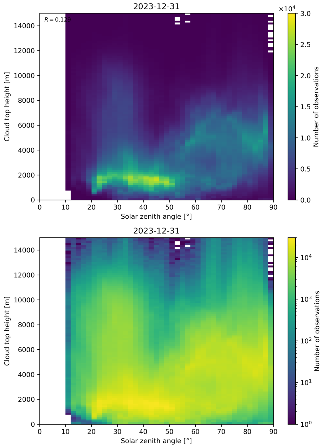
Figure 104: Scatter density plot of “Solar zenith angle” against “Cloud top height” for 2023-12-30 to 2023-12-31.
