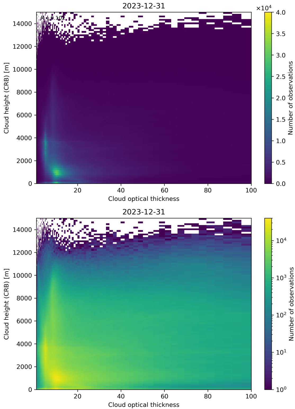
Figure 85: Scatter density plot of “Cloud optical thickness” against “Cloud height (CRB)” for 2023-12-30 to 2023-12-31.
