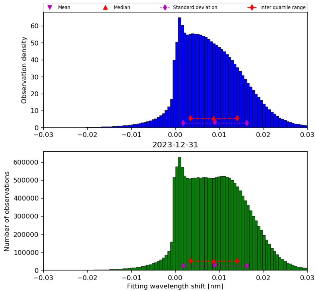
Figure 49: Histogram of “Fitting wavelength shift” for 2023-12-30 to 2023-12-31
