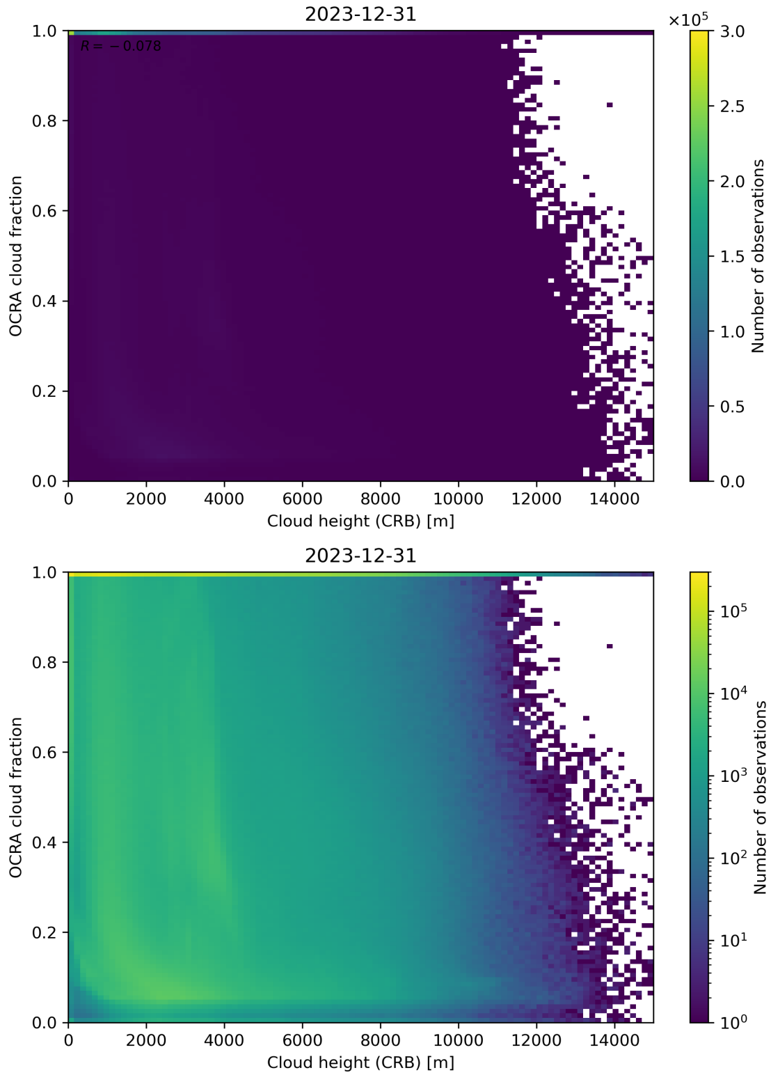
Figure 81: Scatter density plot of “Cloud height (CRB)” against “OCRA cloud fraction” for 2023-12-30 to 2023-12-31.
