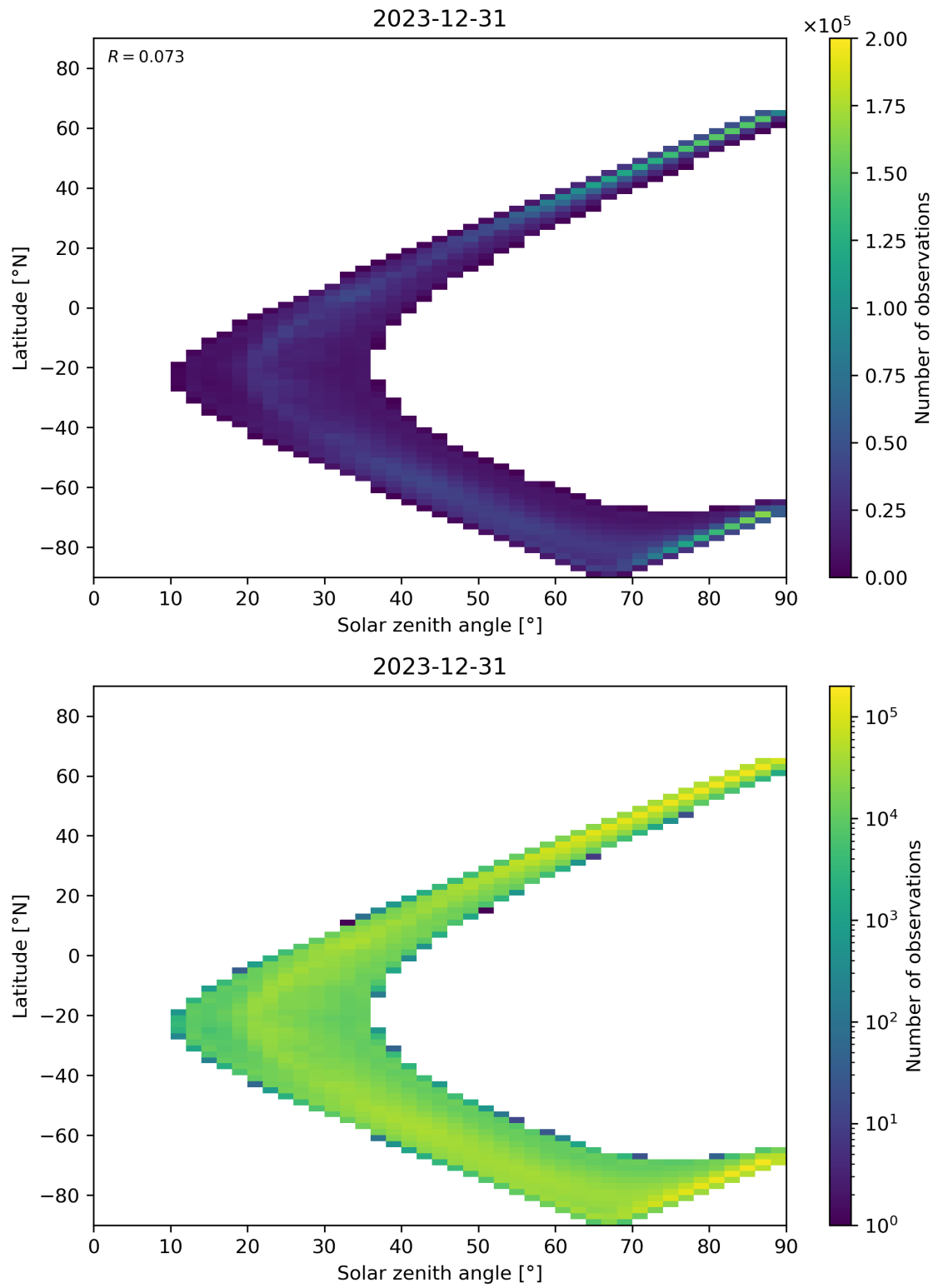
Figure 105: Scatter density plot of “Solar zenith angle” against “Latitude” for 2023-12-30 to 2023-12-31.
