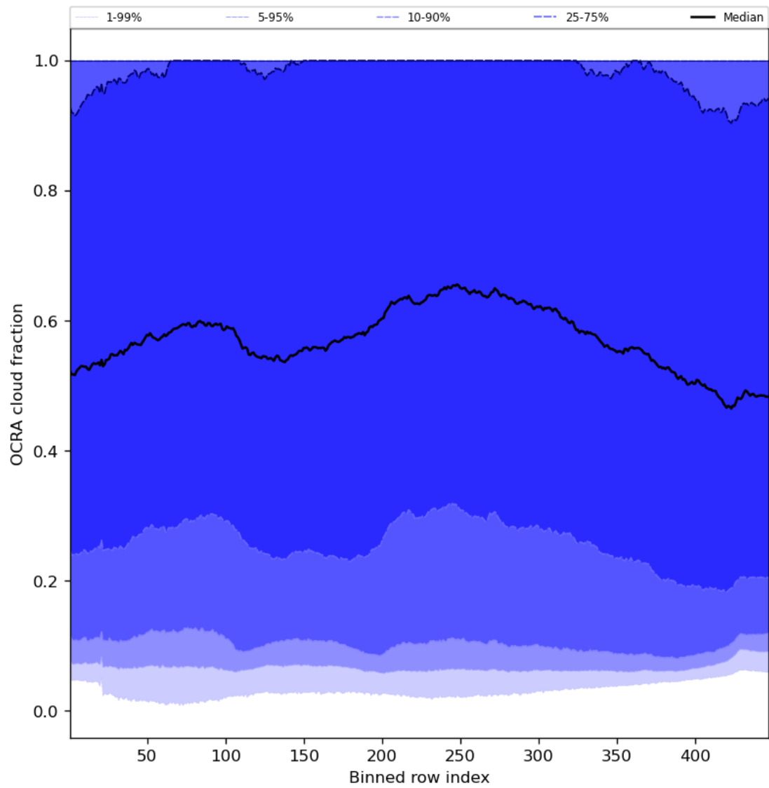
Figure 66: Along track statistics of “OCRA cloud fraction” for 2023-12-30 to 2023-12-31
