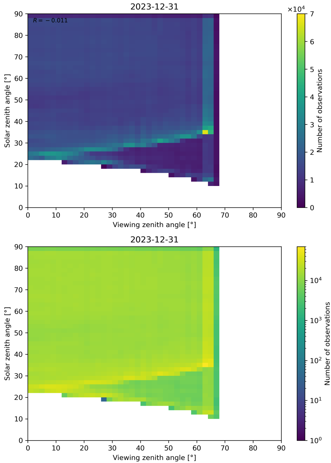
Figure 114: Scatter density plot of “Viewing zenith angle” against “Solar zenith angle” for 2023-12-30 to 2023-12-31.
