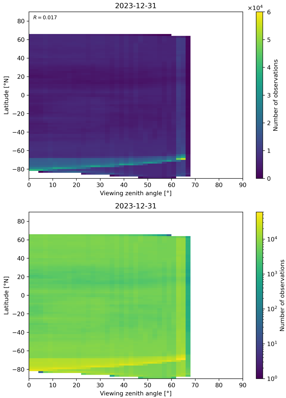
Figure 113: Scatter density plot of “Viewing zenith angle” against “Latitude” for 2023-12-30 to 2023-12-31.
