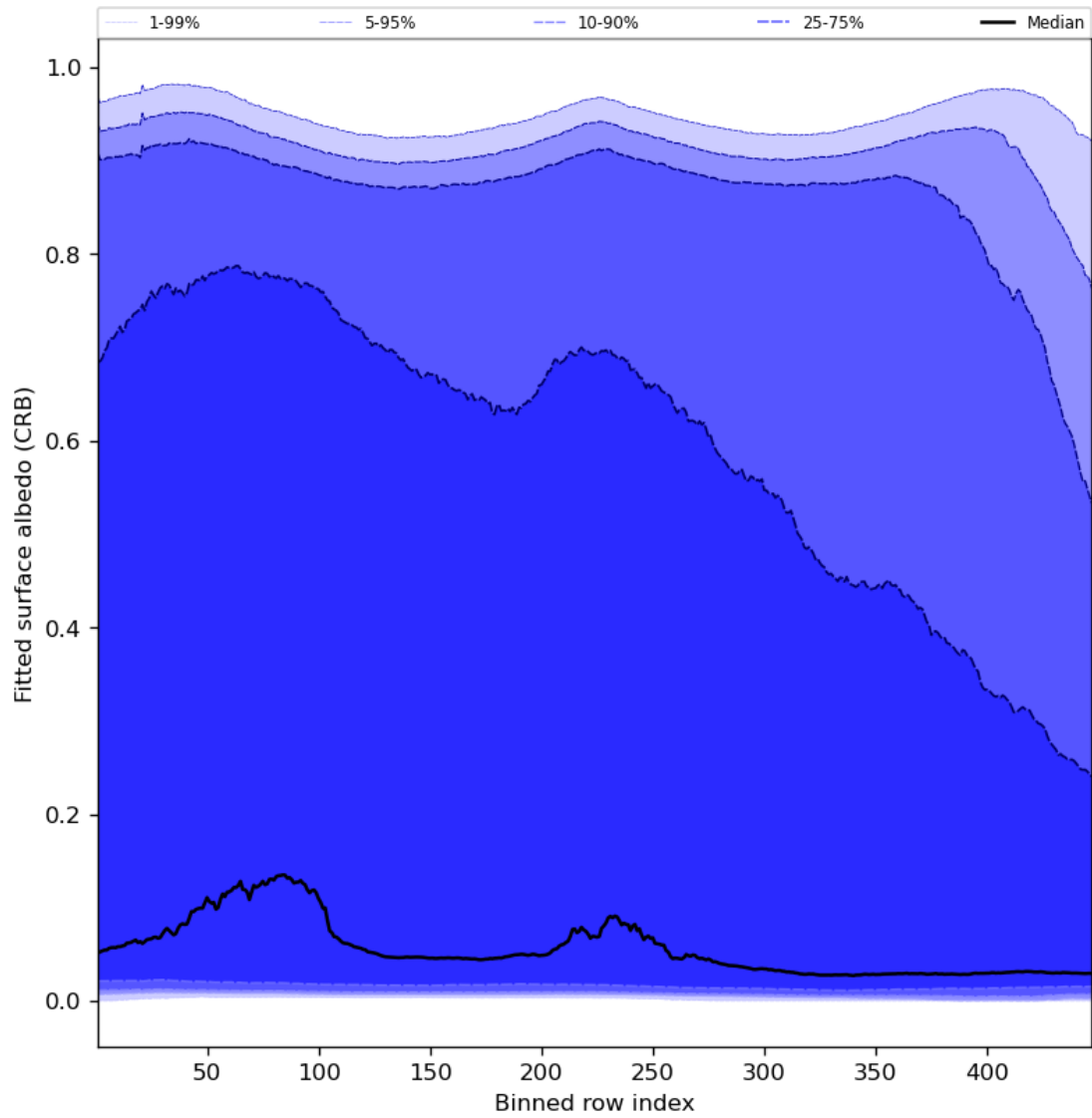
Figure 62: Along track statistics of “Fitted surface albedo (CRB)” for 2023-12-30 to 2023-12-31
