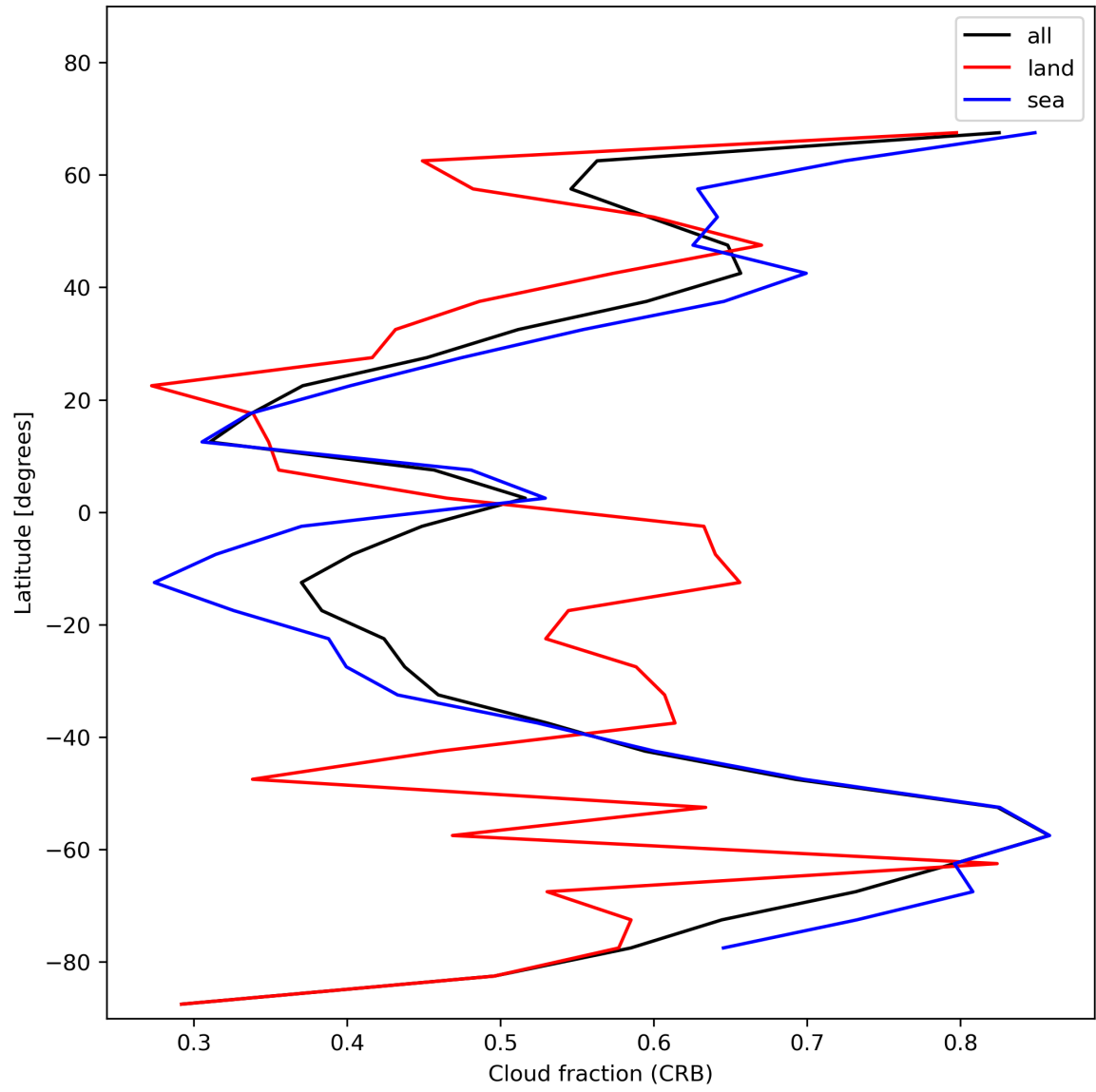
Figure 26: Zonal average of “Cloud fraction (CRB)” for 2023-12-30 to 2023-12-31.
