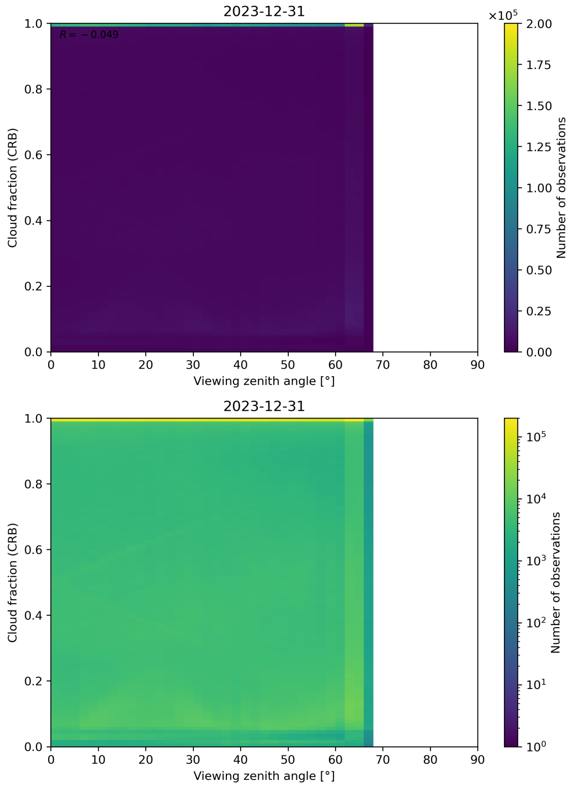
Figure 109: Scatter density plot of “Viewing zenith angle” against “Cloud fraction (CRB)” for 2023-12-30 to 2023-12-31.
