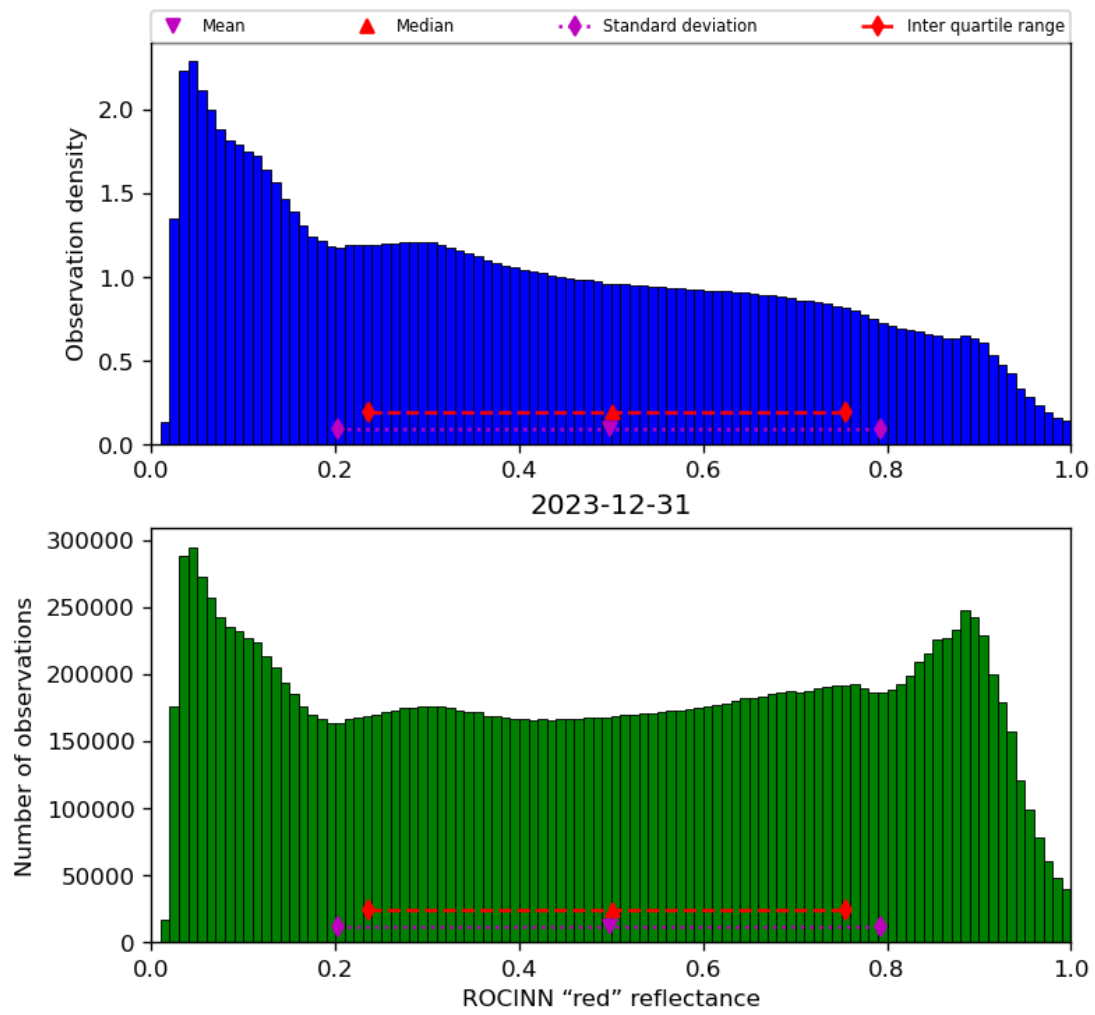
Figure 53: Histogram of “ROCINN “red” reflectance” for 2023-12-30 to 2023-12-31
