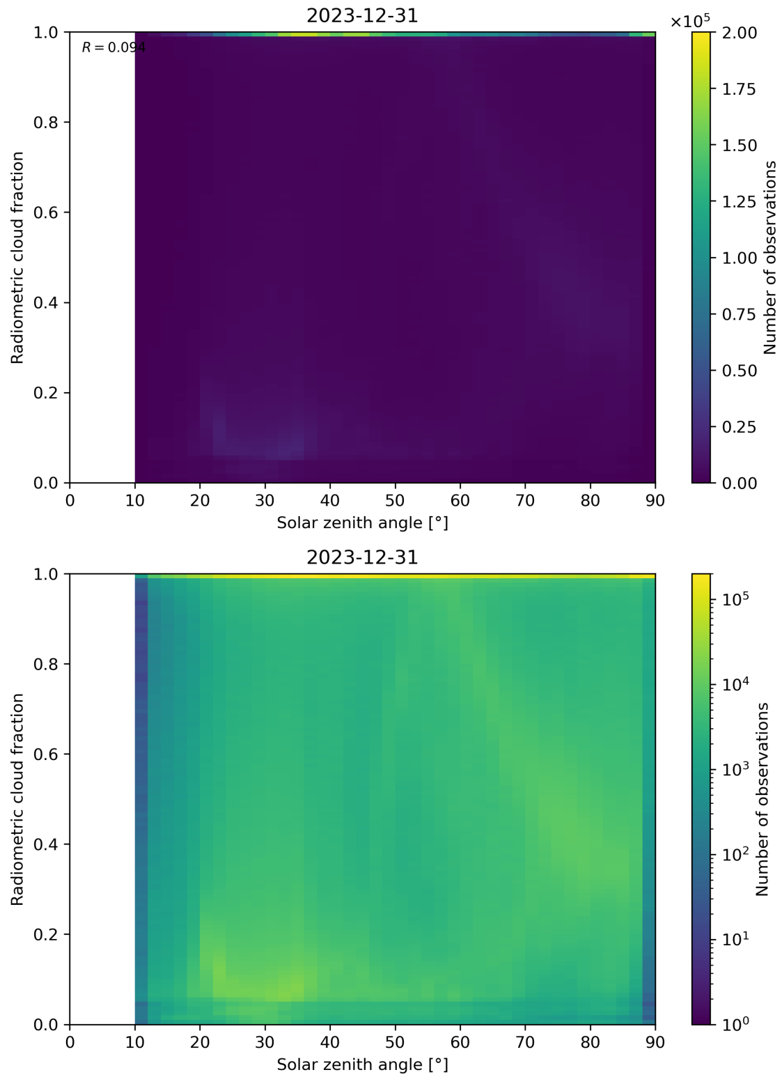
Figure 99: Scatter density plot of “Solar zenith angle” against “Radiometric cloud fraction” for 2023-12-30 to 2023-12-31.
