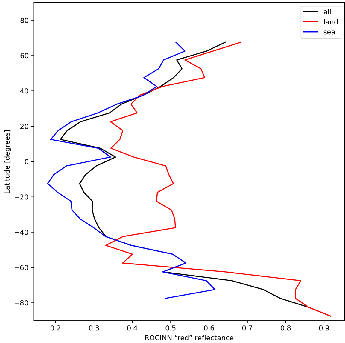
Figure 37: Zonal average of “ROCINN “red” reflectance” for 2023-12-30 to 2023-12-31.
