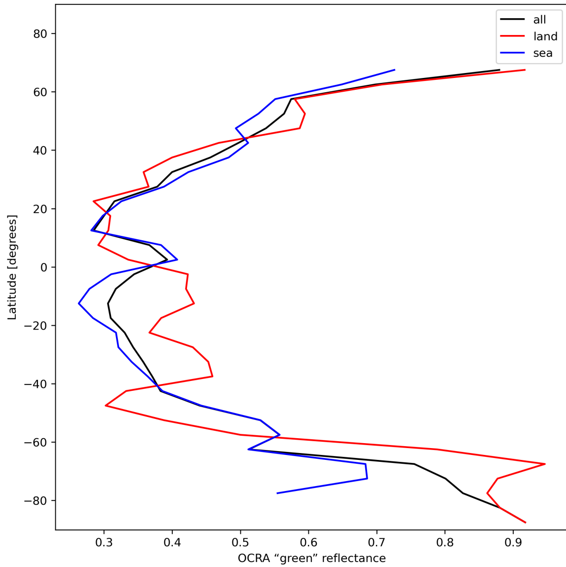
Figure 36: Zonal average of “OCRA “green” reflectance” for 2023-12-30 to 2023-12-31.
