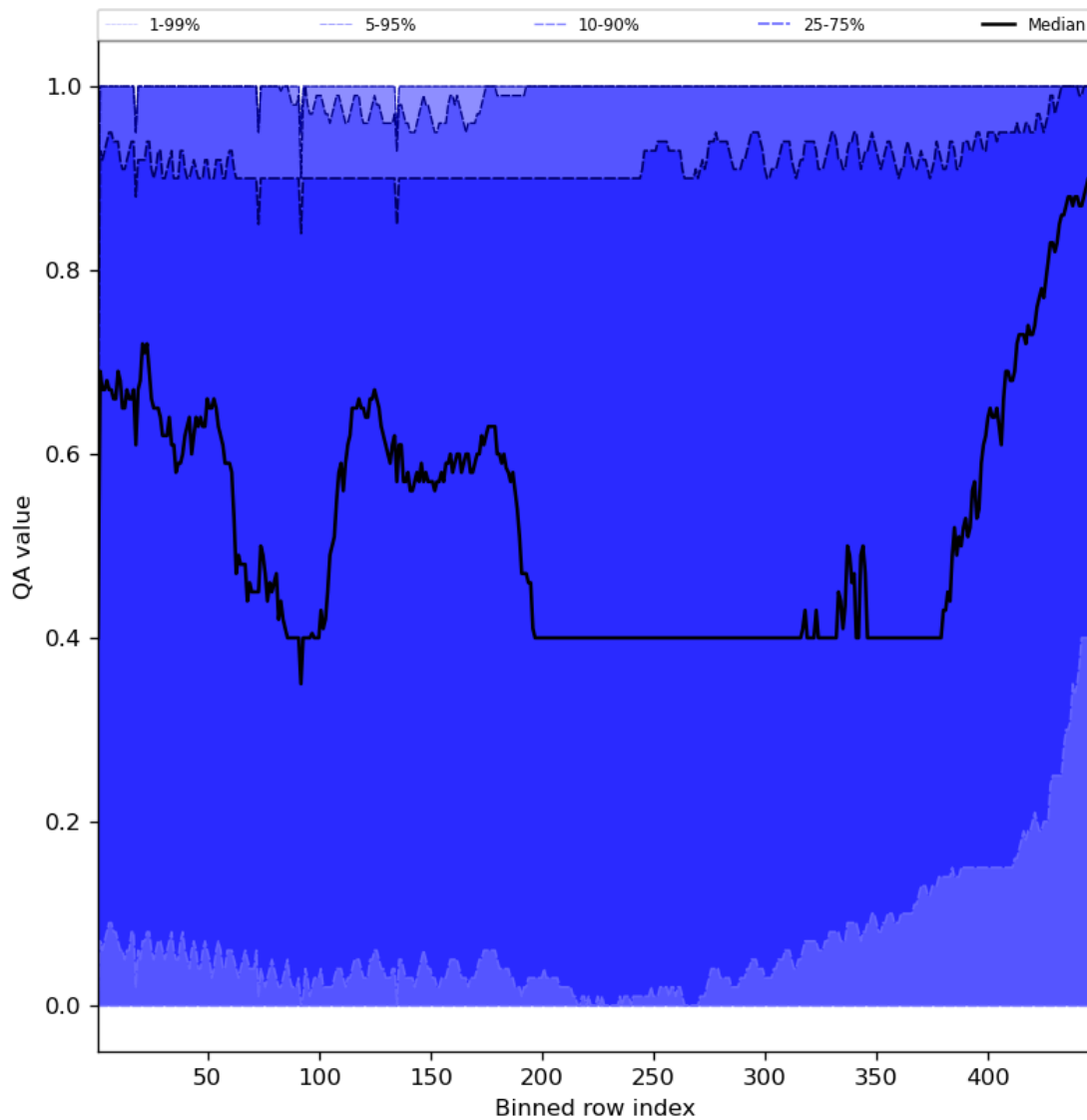
Figure 54: Along track statistics of “QA value” for 2023-12-30 to 2023-12-31
