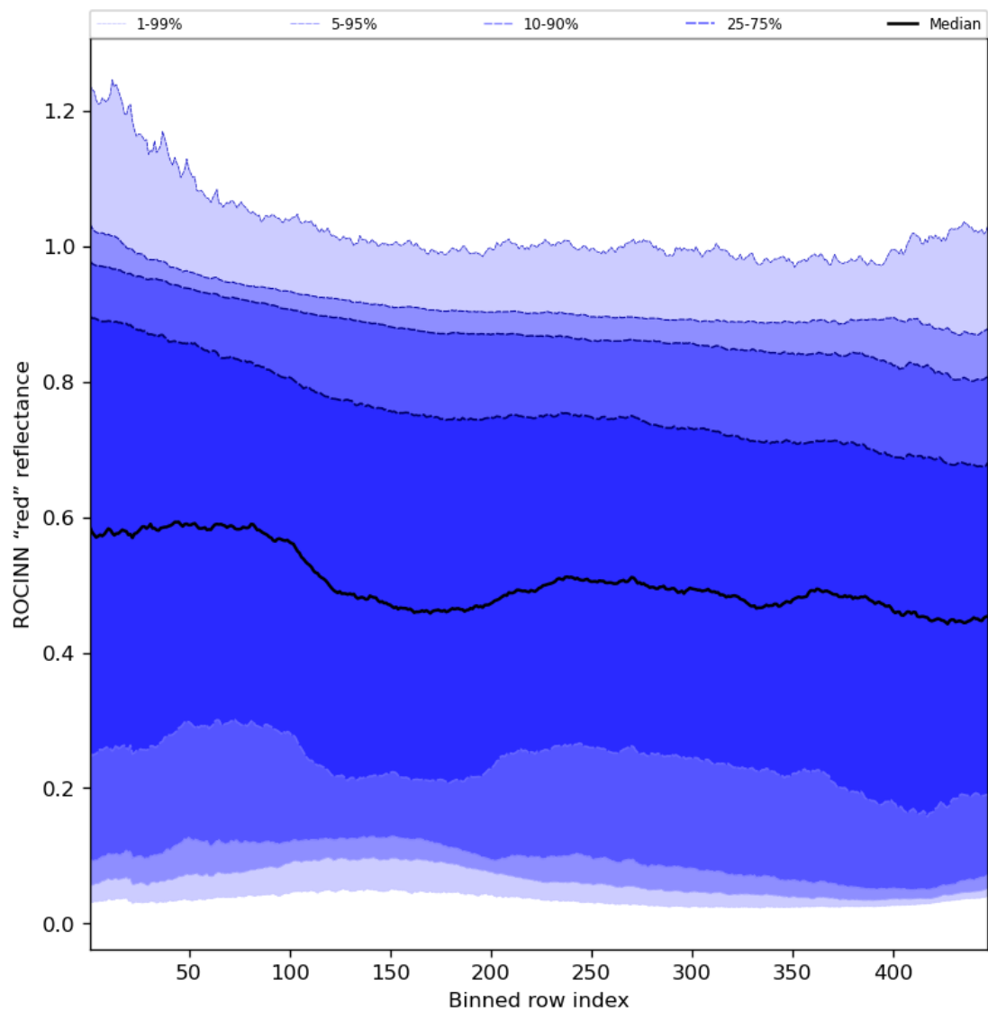
Figure 69: Along track statistics of “ROCINN “red” reflectance” for 2023-12-30 to 2023-12-31
