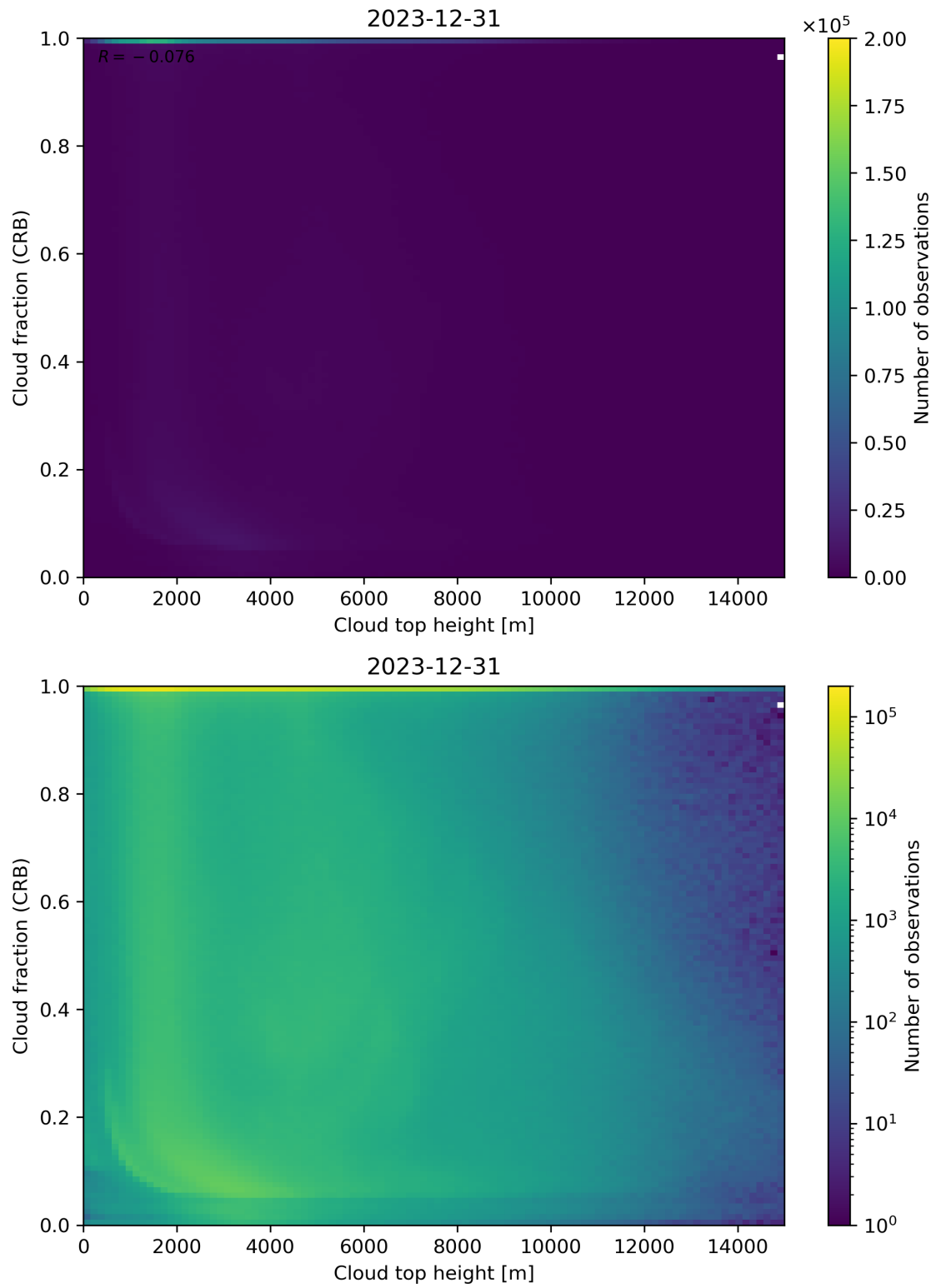
Figure 88: Scatter density plot of “Cloud top height” against “Cloud fraction (CRB)” for 2023-12-30 to 2023-12-31.
