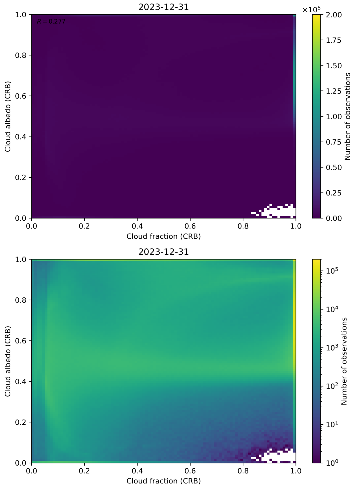
Figure 77: Scatter density plot of “Cloud fraction (CRB)” against “Cloud albedo (CRB)” for 2023-12-30 to 2023-12-31.
