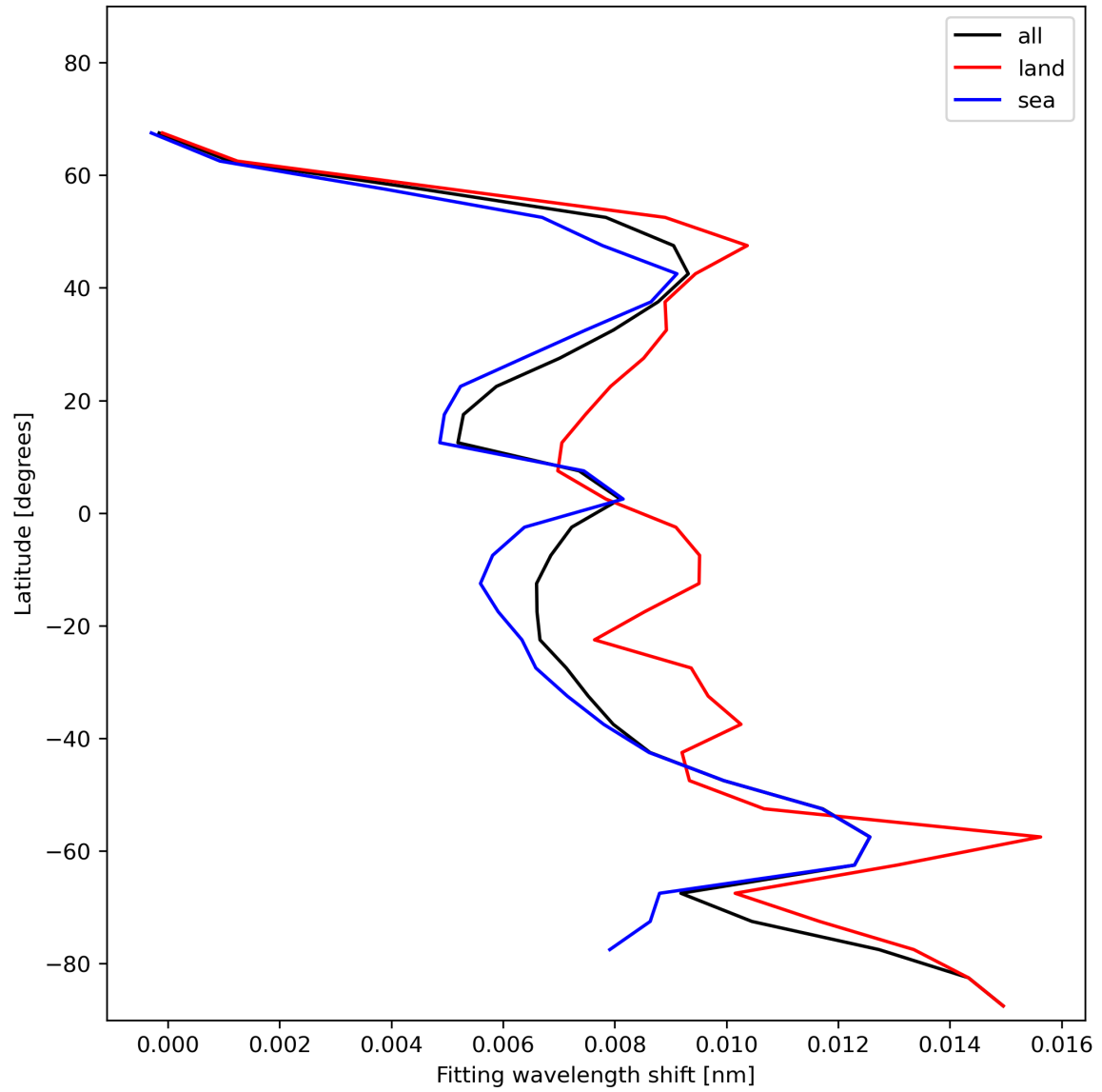
Figure 33: Zonal average of “Fitting wavelength shift” for 2023-12-30 to 2023-12-31.
