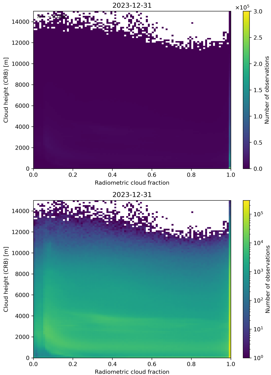
Figure 74: Scatter density plot of “Radiometric cloud fraction” against “Cloud height (CRB)” for 2023-12-30 to 2023-12-31.
