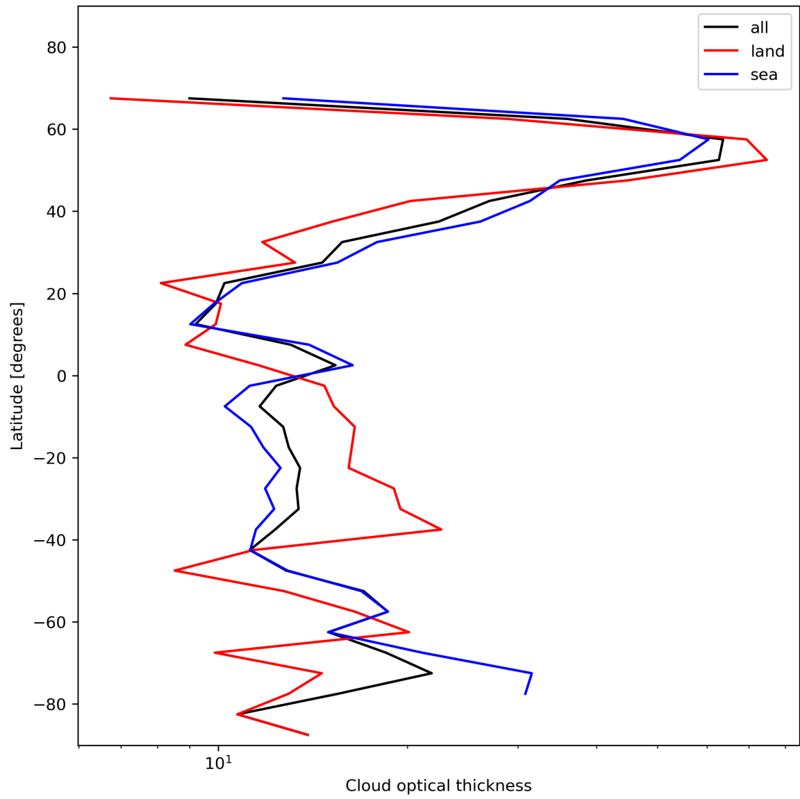
Figure 25: Zonal average of “Cloud optical thickness” for 2023-12-30 to 2023-12-31.
