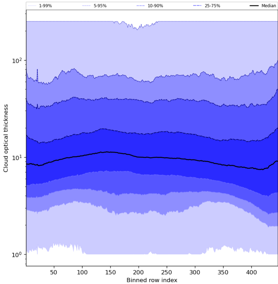
Figure 57: Along track statistics of “Cloud optical thickness” for 2023-12-30 to 2023-12-31
