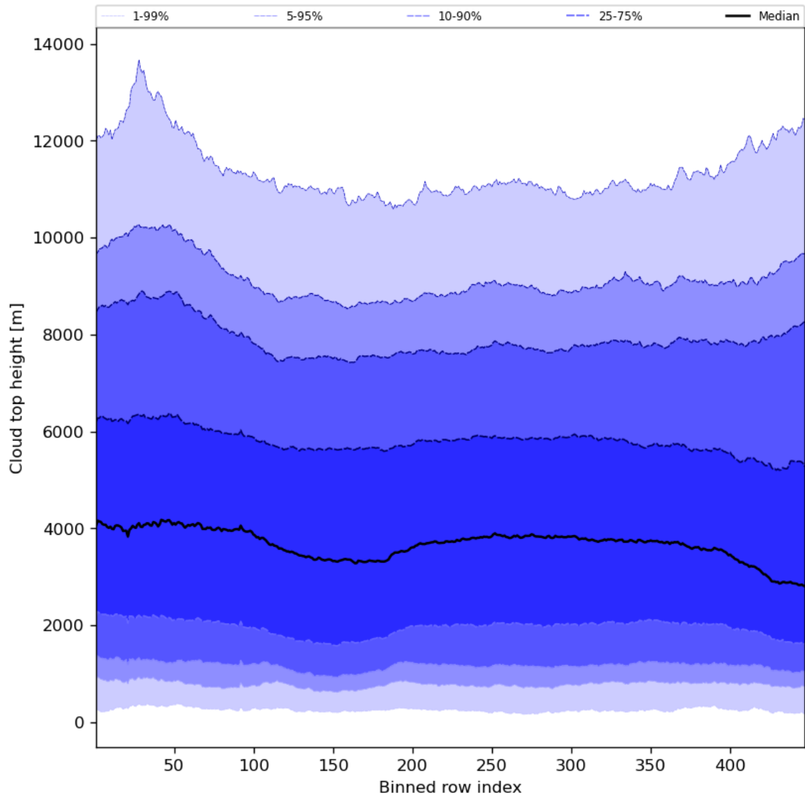
Figure 56: Along track statistics of “Cloud top height” for 2023-12-30 to 2023-12-31
