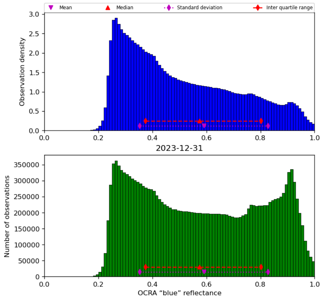
Figure 51: Histogram of "OCRA "blue" reflectance" for 2023-12-30 to 2023-12-31
