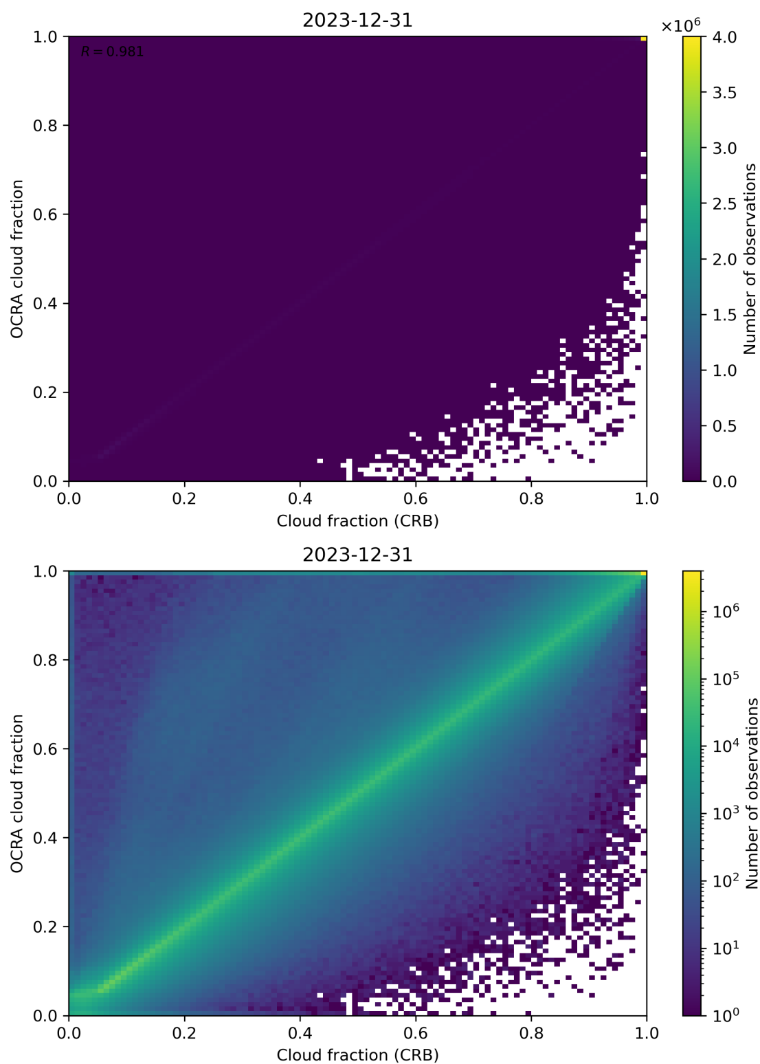
Figure 78: Scatter density plot of “Cloud fraction (CRB)” against “OCRA cloud fraction” for 2023-12-30 to 2023-12-31.
