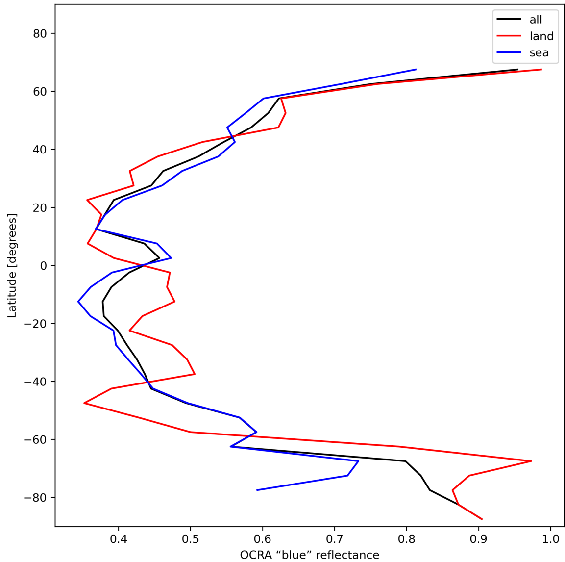
Figure 35: Zonal average of “OCRA “blue” reflectance” for 2023-12-30 to 2023-12-31.
