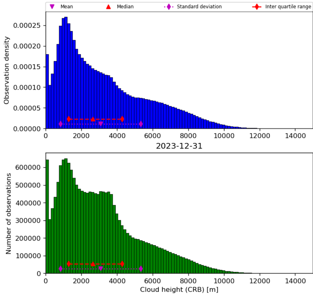
Figure 43: Histogram of “Cloud height (CRB)” for 2023-12-30 to 2023-12-31
