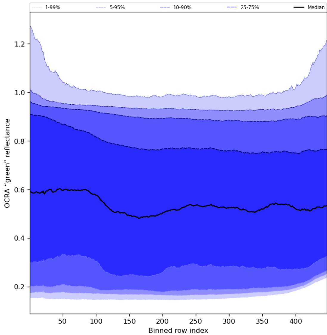
Figure 68: Along track statistics of "OCRA "green" reflectance" for 2023-12-30 to 2023-12-31
