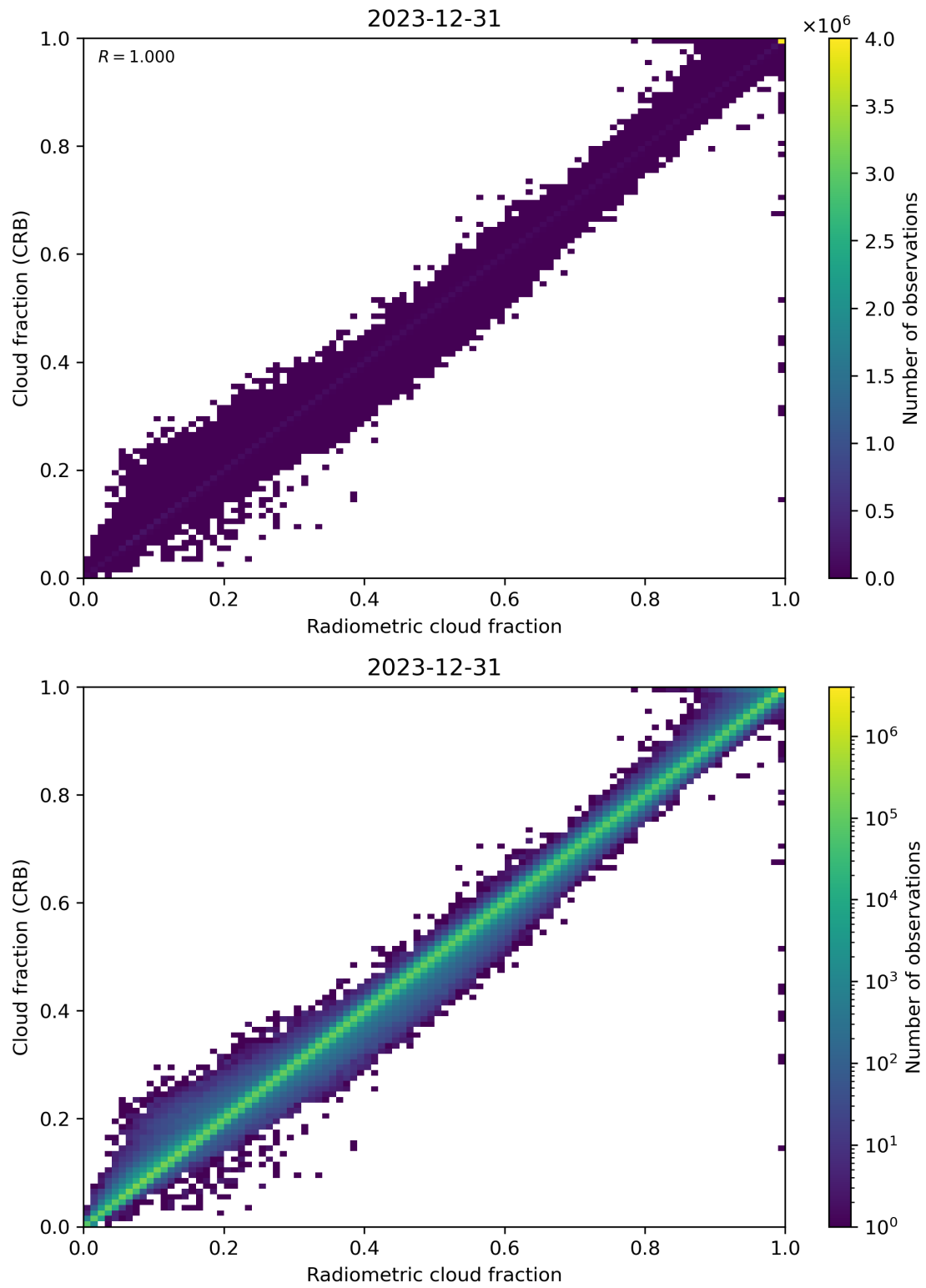
Figure 73: Scatter density plot of “Radiometric cloud fraction” against “Cloud fraction (CRB)” for 2023-12-30 to 2023-12-31.
