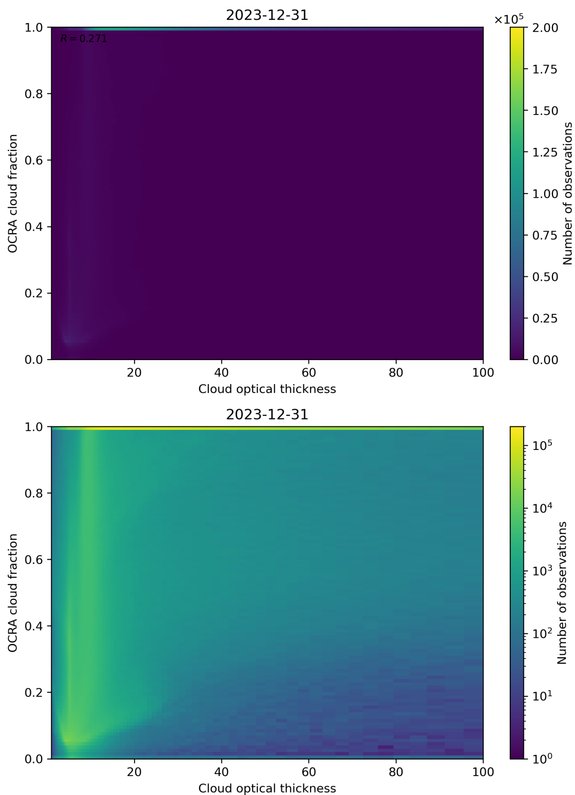
Figure 83: Scatter density plot of “Cloud optical thickness” against “OCRA cloud fraction” for 2023-12-30 to 2023-12-31.
