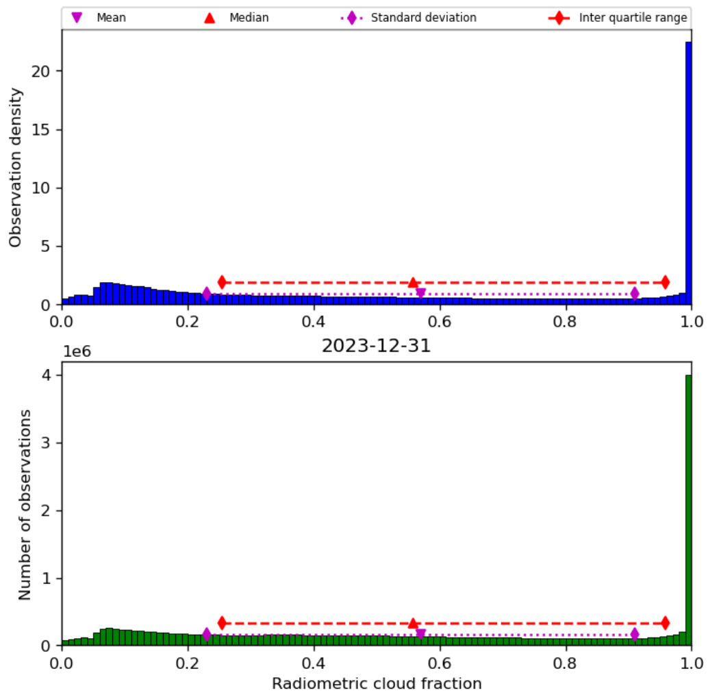
Figure 39: Histogram of “Radiometric cloud fraction” for 2023-12-30 to 2023-12-31
