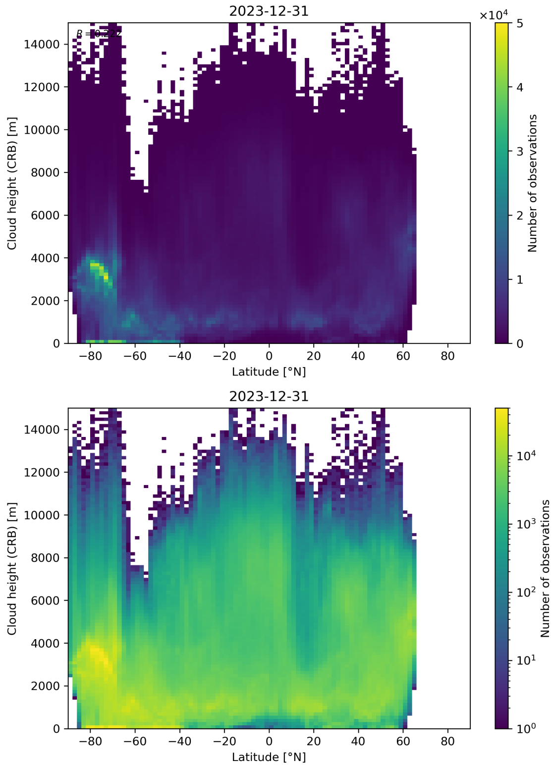
Figure 95: Scatter density plot of “Latitude” against “Cloud height (CRB)” for 2023-12-30 to 2023-12-31.
