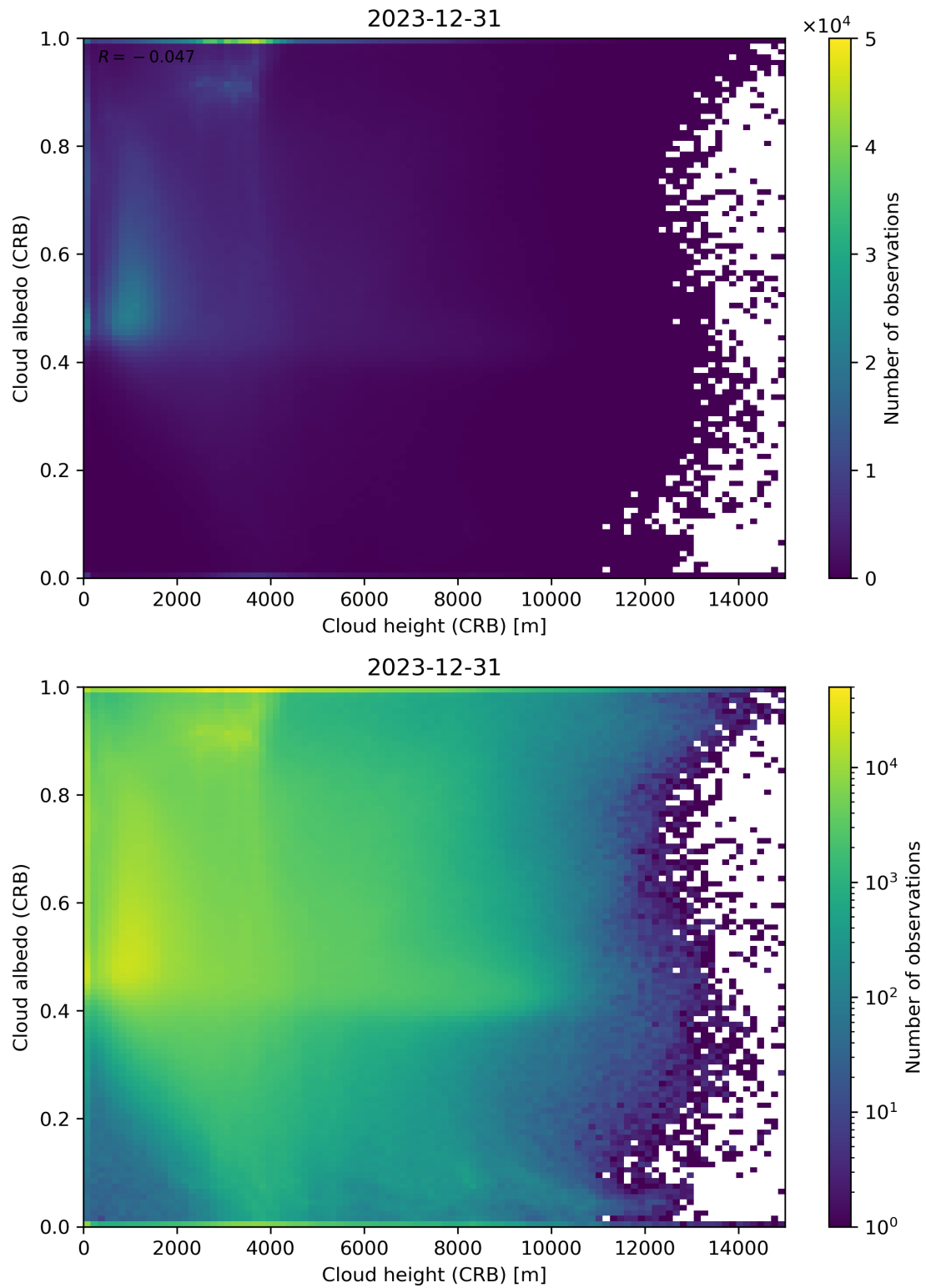
Figure 80: Scatter density plot of “Cloud height (CRB)” against “Cloud albedo (CRB)” for 2023-12-30 to 2023-12-31.
