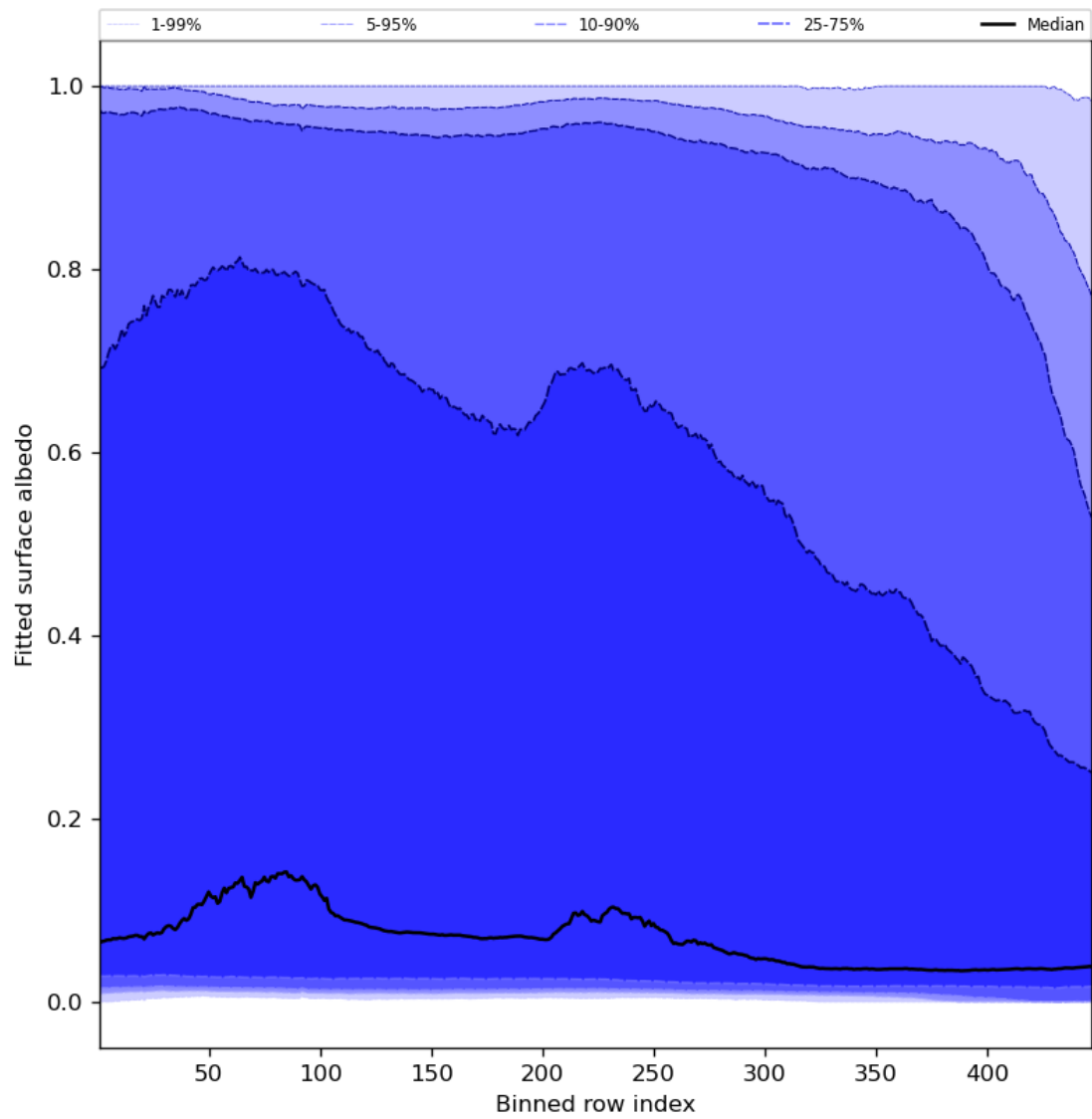
Figure 61: Along track statistics of “Fitted surface albedo” for 2023-12-30 to 2023-12-31
