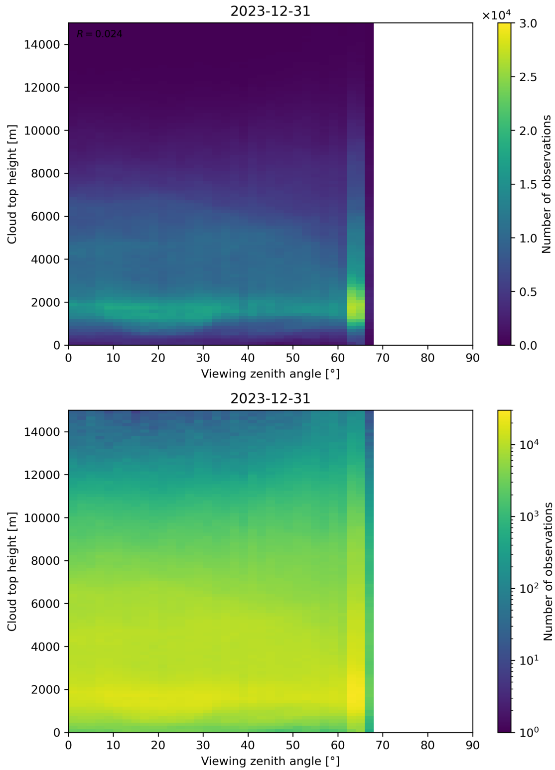
Figure 112: Scatter density plot of “Viewing zenith angle” against “Cloud top height” for 2023-12-30 to 2023-12-31.
