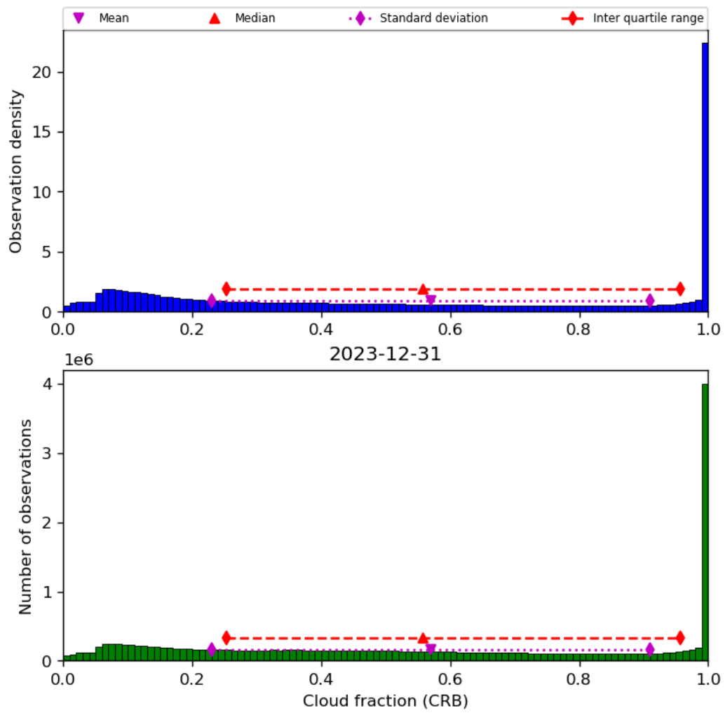
Figure 42: Histogram of “Cloud fraction (CRB)” for 2023-12-30 to 2023-12-31
