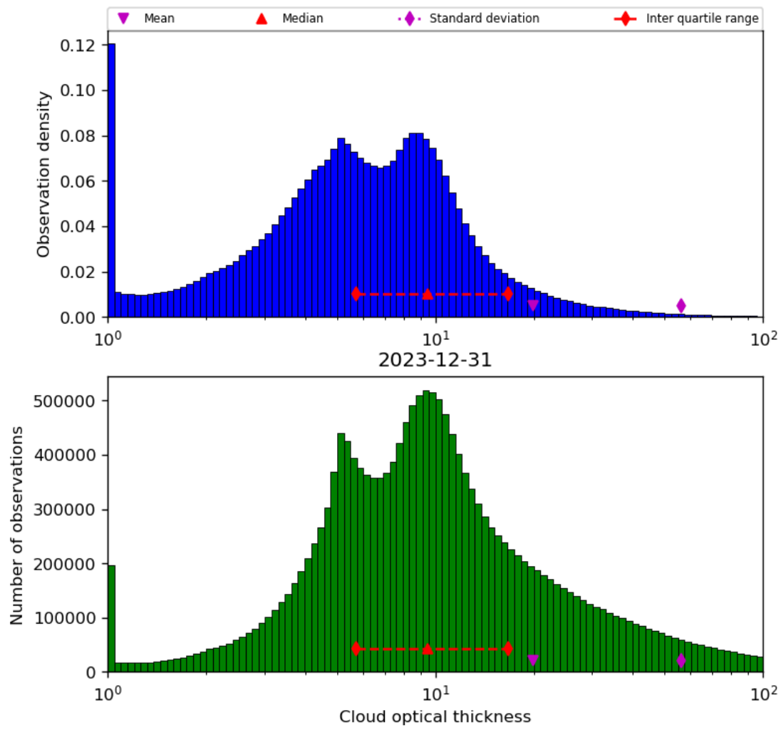
Figure 41: Histogram of “Cloud optical thickness” for 2023-12-30 to 2023-12-31
