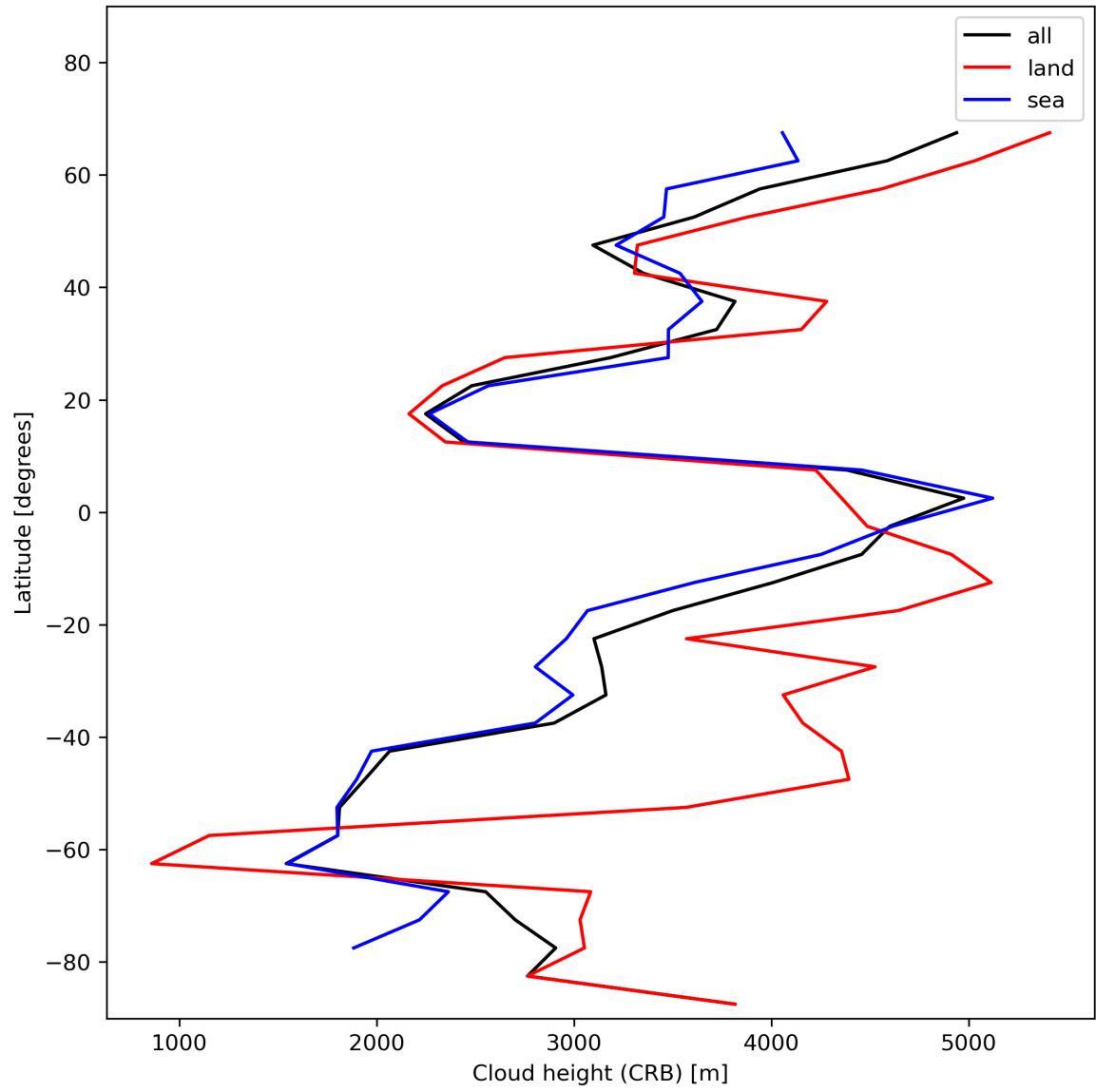
Figure 27: Zonal average of “Cloud height (CRB)” for 2023-12-30 to 2023-12-31.
