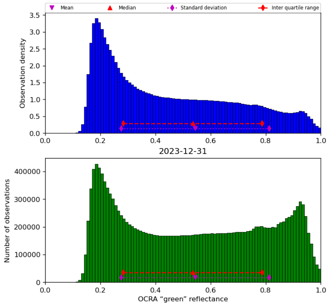
Figure 52: Histogram of “OCRA “green” reflectance” for 2023-12-30 to 2023-12-31
