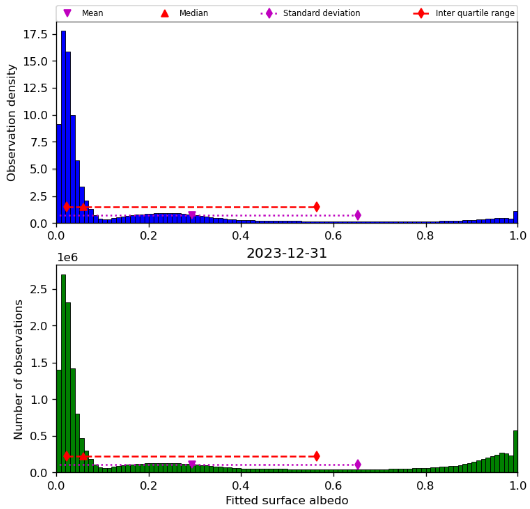
Figure 45: Histogram of “Fitted surface albedo” for 2023-12-30 to 2023-12-31
