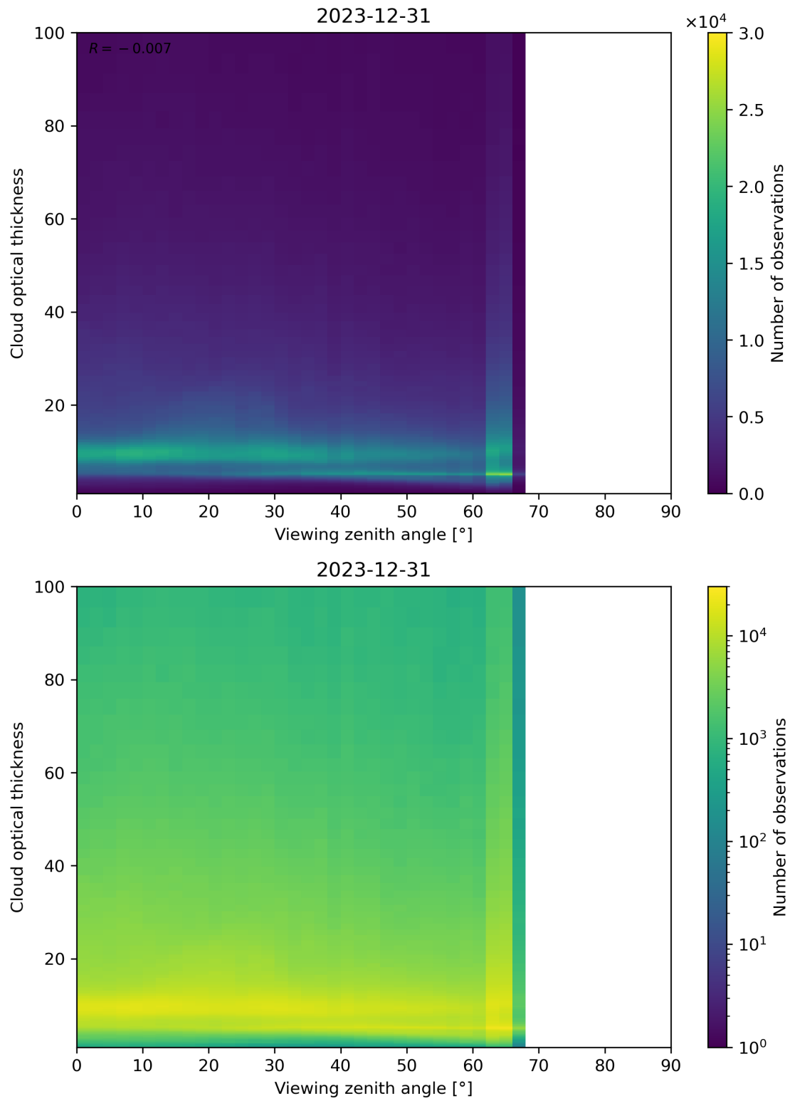
Figure 111: Scatter density plot of “Viewing zenith angle” against “Cloud optical thickness” for 2023-12-30 to 2023-12-31.
