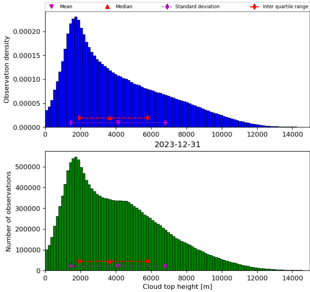
Figure 40: Histogram of “Cloud top height” for 2023-12-30 to 2023-12-31
