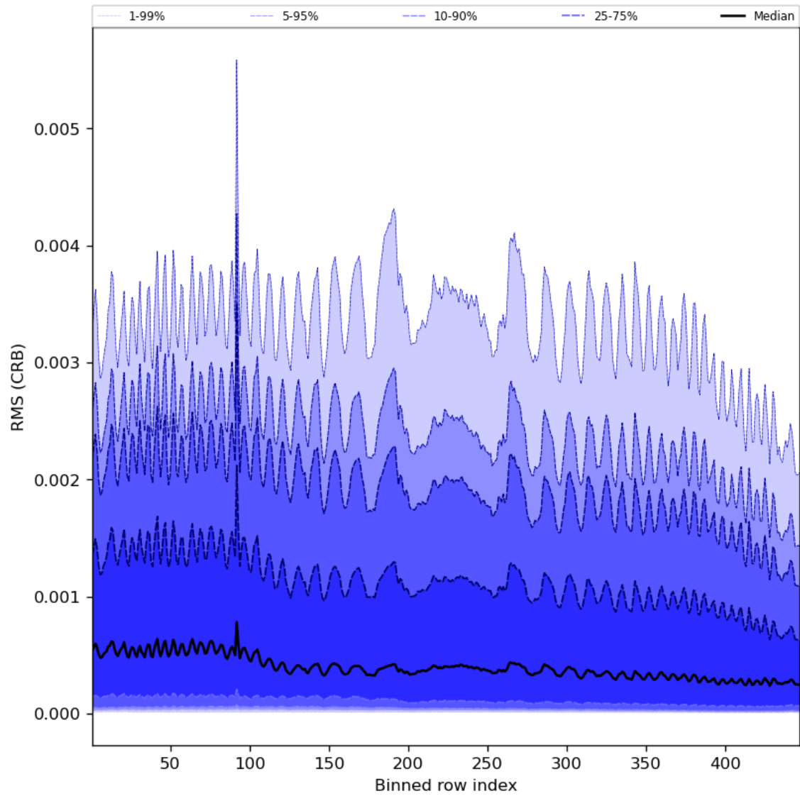
Figure 64: Along track statistics of “RMS (CRB)” for 2023-12-30 to 2023-12-31
