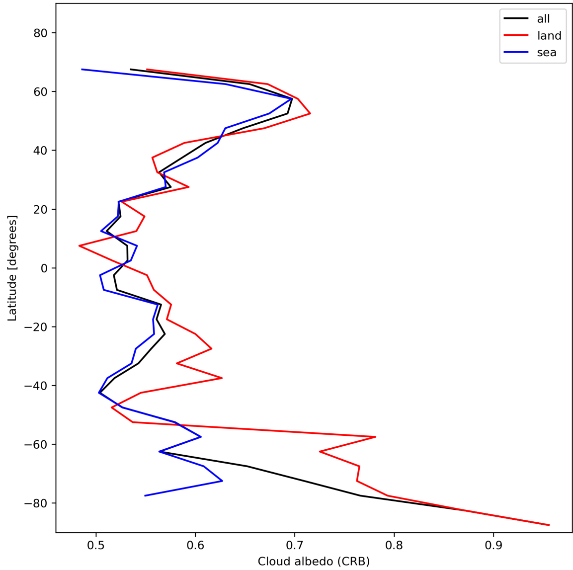
Figure 28: Zonal average of “Cloud albedo (CRB)” for 2023-12-30 to 2023-12-31.
