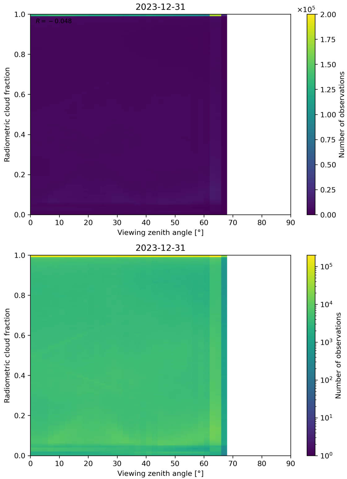
Figure 107: Scatter density plot of “Viewing zenith angle” against “Radiometric cloud fraction” for 2023-12-30 to 2023-12-31.
