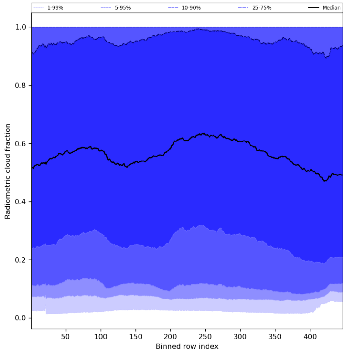
Figure 55: Along track statistics of “Radiometric cloud fraction” for 2023-12-30 to 2023-12-31
