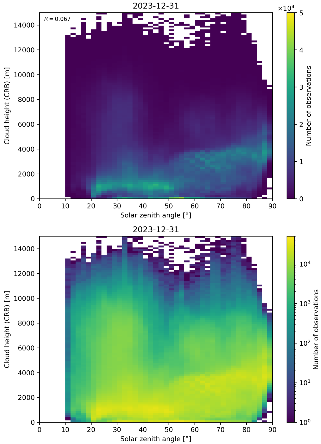
Figure 102: Scatter density plot of “Solar zenith angle” against “Cloud height (CRB)” for 2023-12-30 to 2023-12-31.
