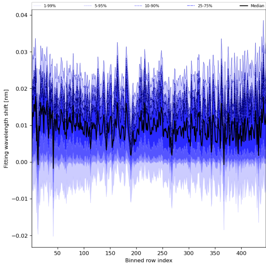
Figure 65: Along track statistics of “Fitting wavelength shift” for 2023-12-30 to 2023-12-31
