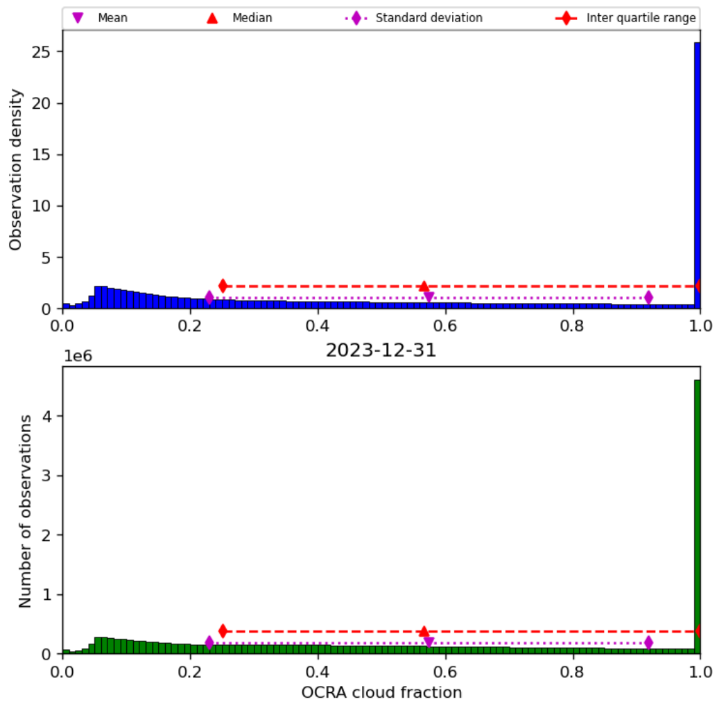
Figure 50: Histogram of “OCRA cloud fraction” for 2023-12-30 to 2023-12-31
