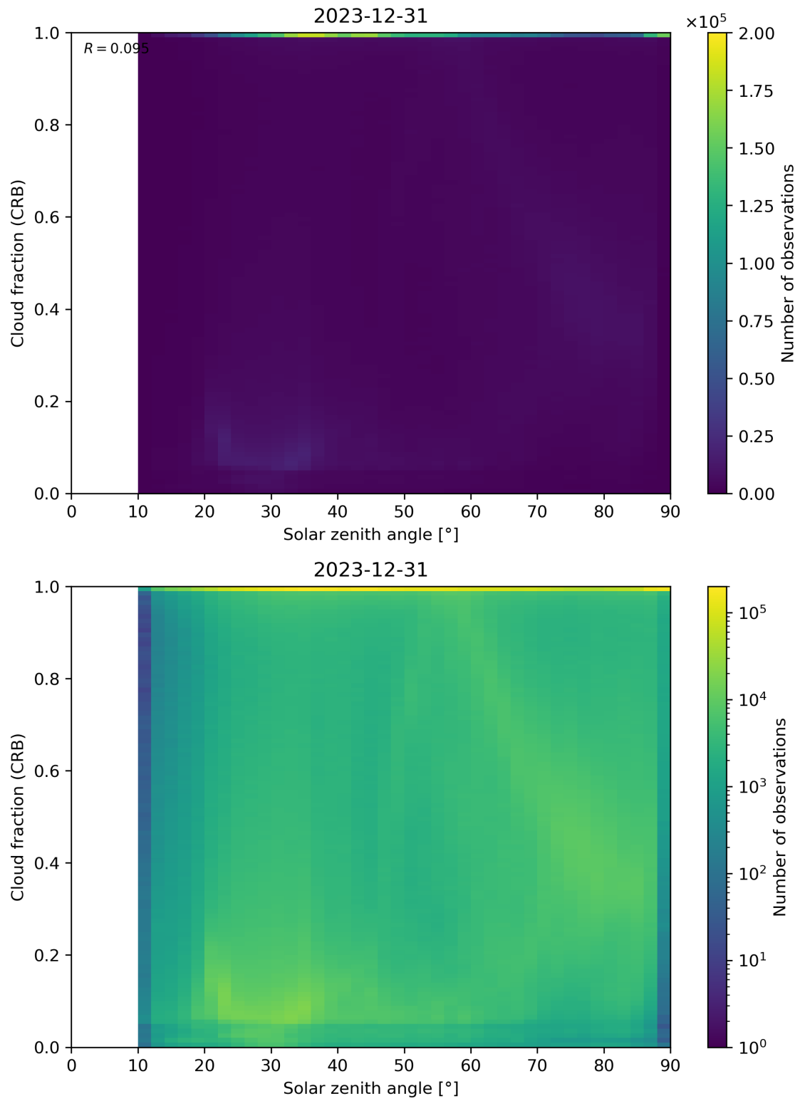
Figure 101: Scatter density plot of “Solar zenith angle” against “Cloud fraction (CRB)” for 2023-12-30 to 2023-12-31.
