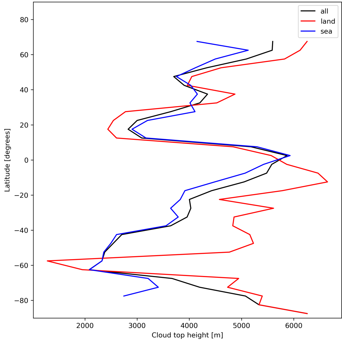
Figure 24: Zonal average of “Cloud top height” for 2023-12-30 to 2023-12-31.
