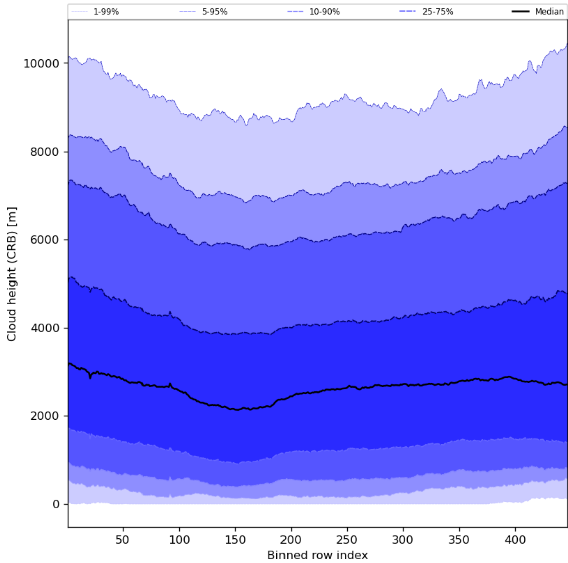
Figure 59: Along track statistics of “Cloud height (CRB)” for 2023-12-30 to 2023-12-31
