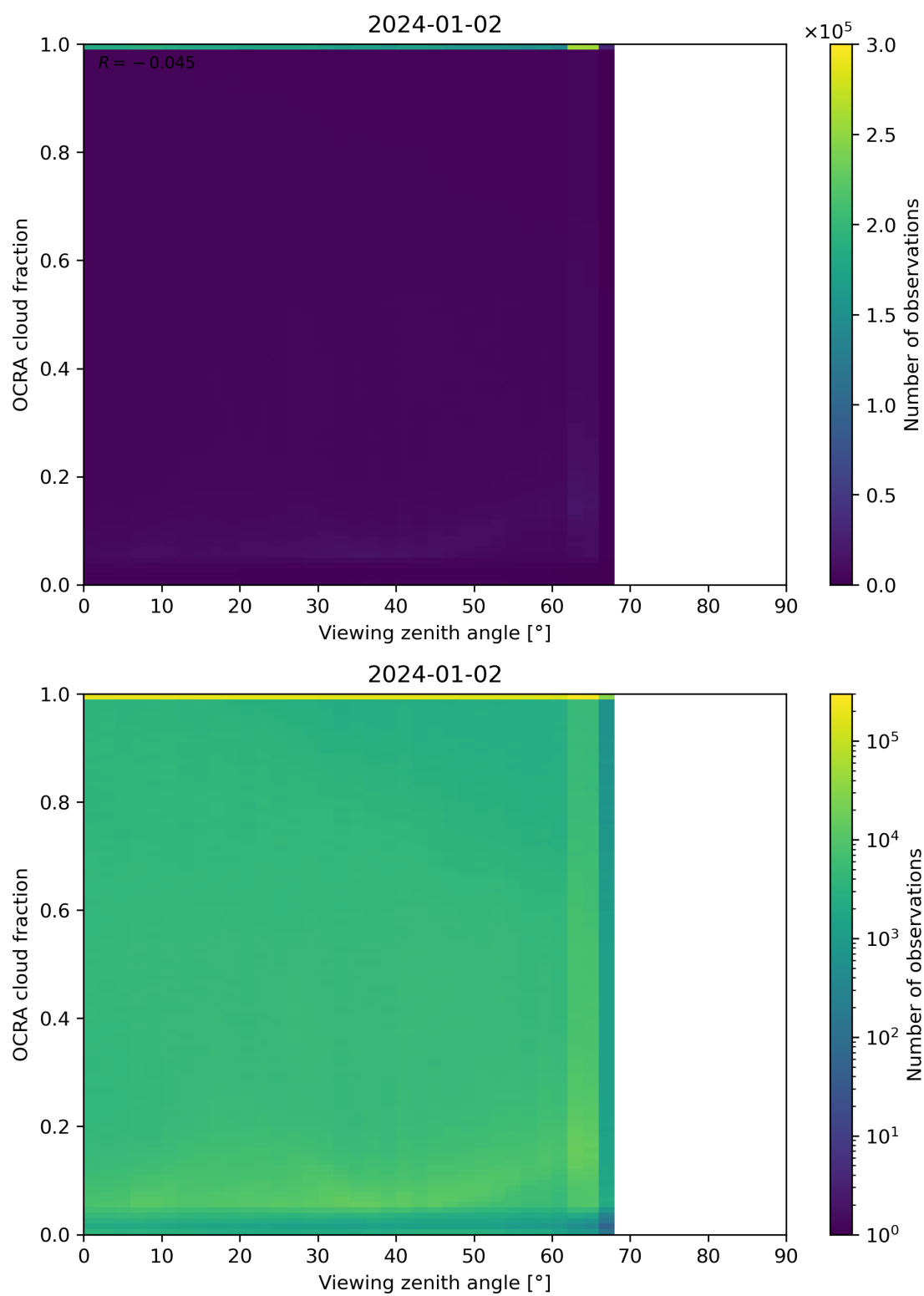
Figure 108: Scatter density plot of “Viewing zenith angle” against “OCRA cloud fraction” for 2024-01-01 to 2024-01-03.
