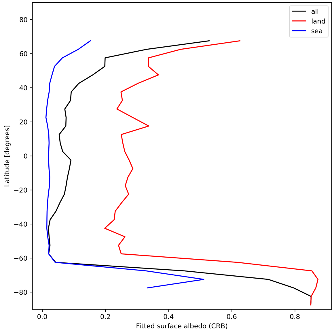
Figure 30: Zonal average of “Fitted surface albedo (CRB)” for 2024-01-01 to 2024-01-03.
