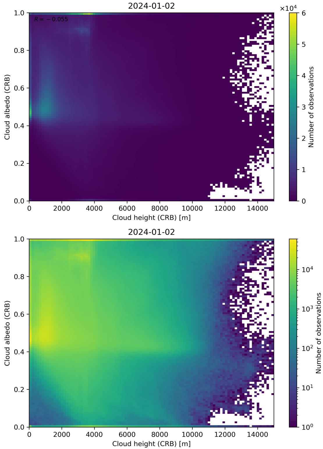
Figure 80: Scatter density plot of “Cloud height (CRB)” against “Cloud albedo (CRB)” for 2024-01-01 to 2024-01-03.
