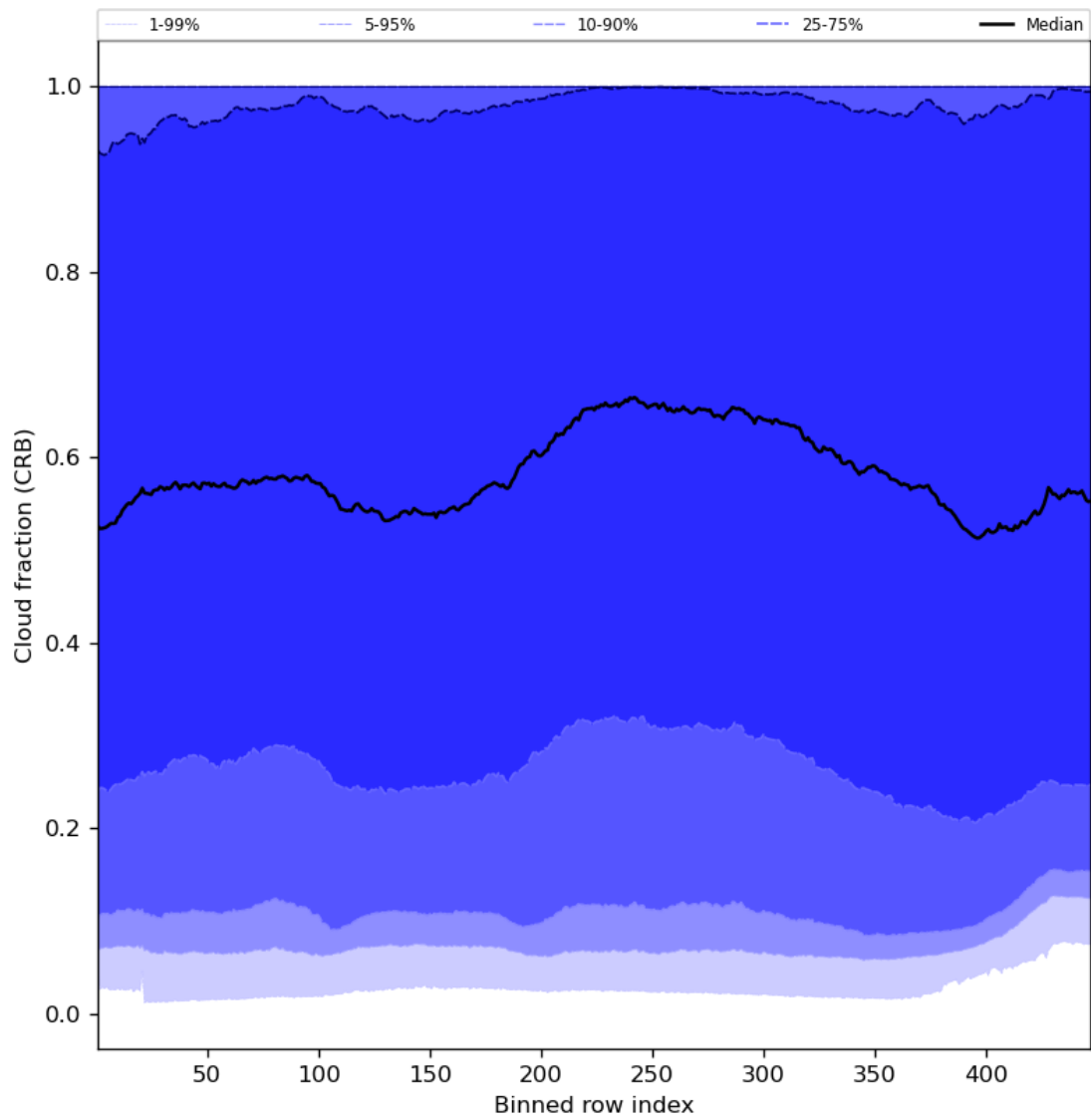
Figure 58: Along track statistics of “Cloud fraction (CRB)” for 2024-01-01 to 2024-01-03
