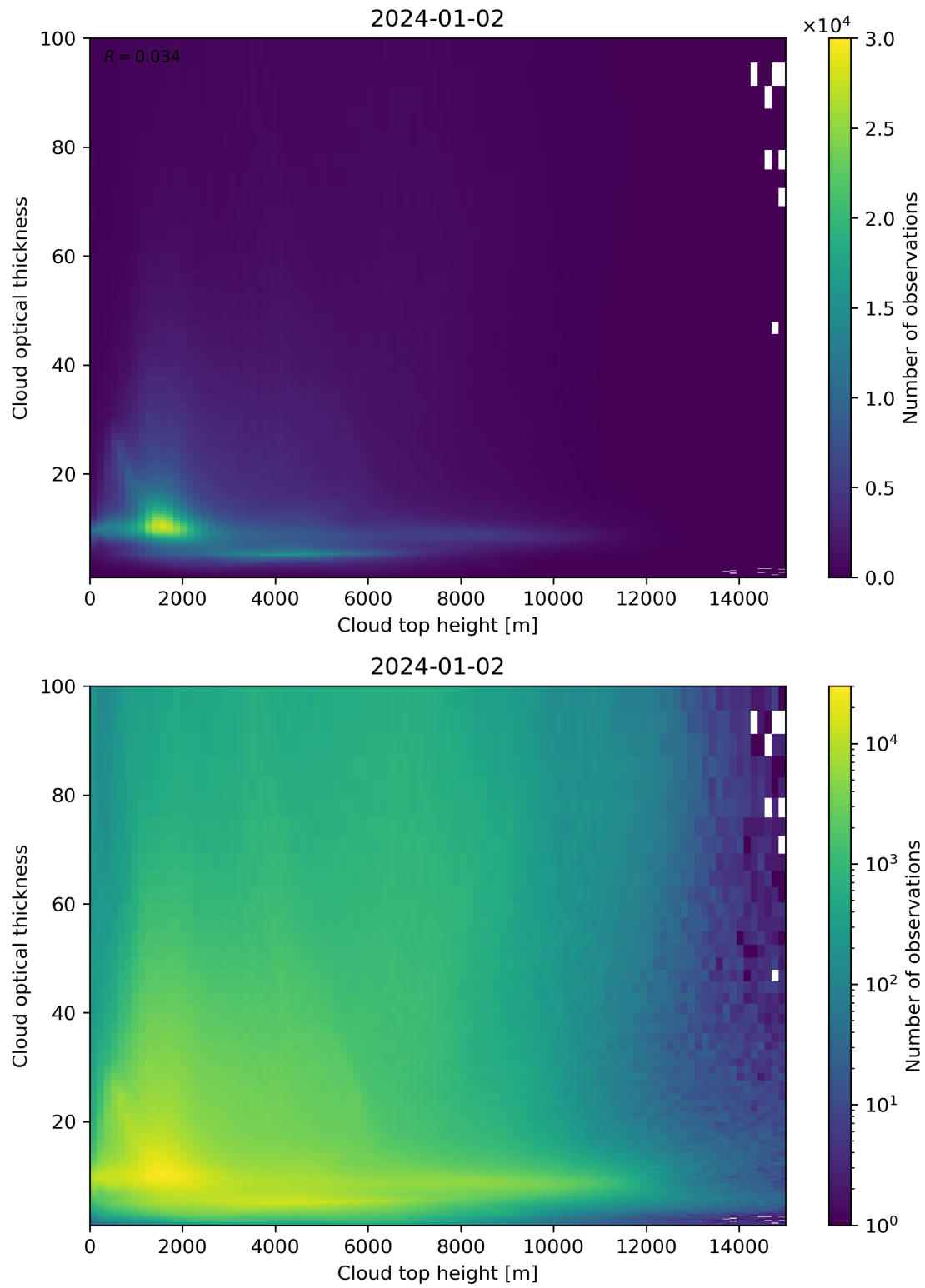
Figure 90: Scatter density plot of “Cloud top height” against “Cloud optical thickness” for 2024-01-01 to 2024-01-03.
