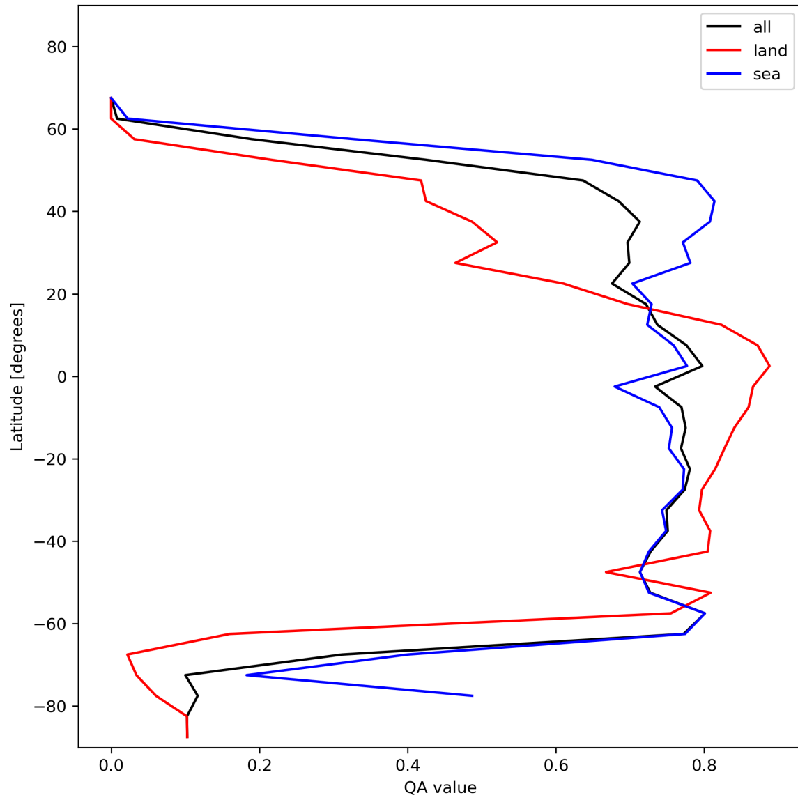
Figure 22: Zonal average of “QA value” for 2024-01-01 to 2024-01-03.
