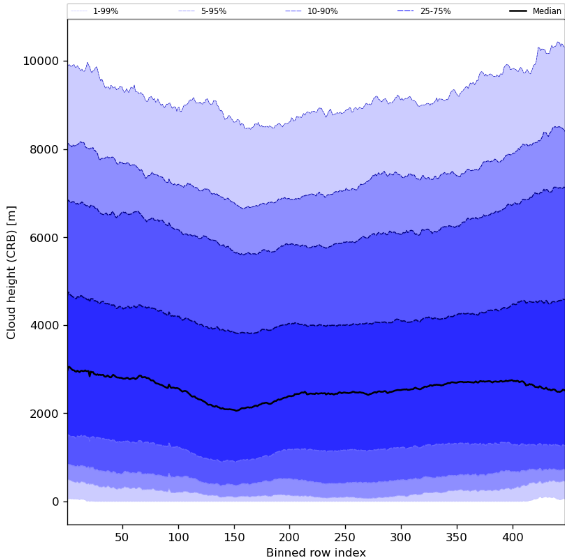
Figure 59: Along track statistics of “Cloud height (CRB)” for 2024-01-01 to 2024-01-03
