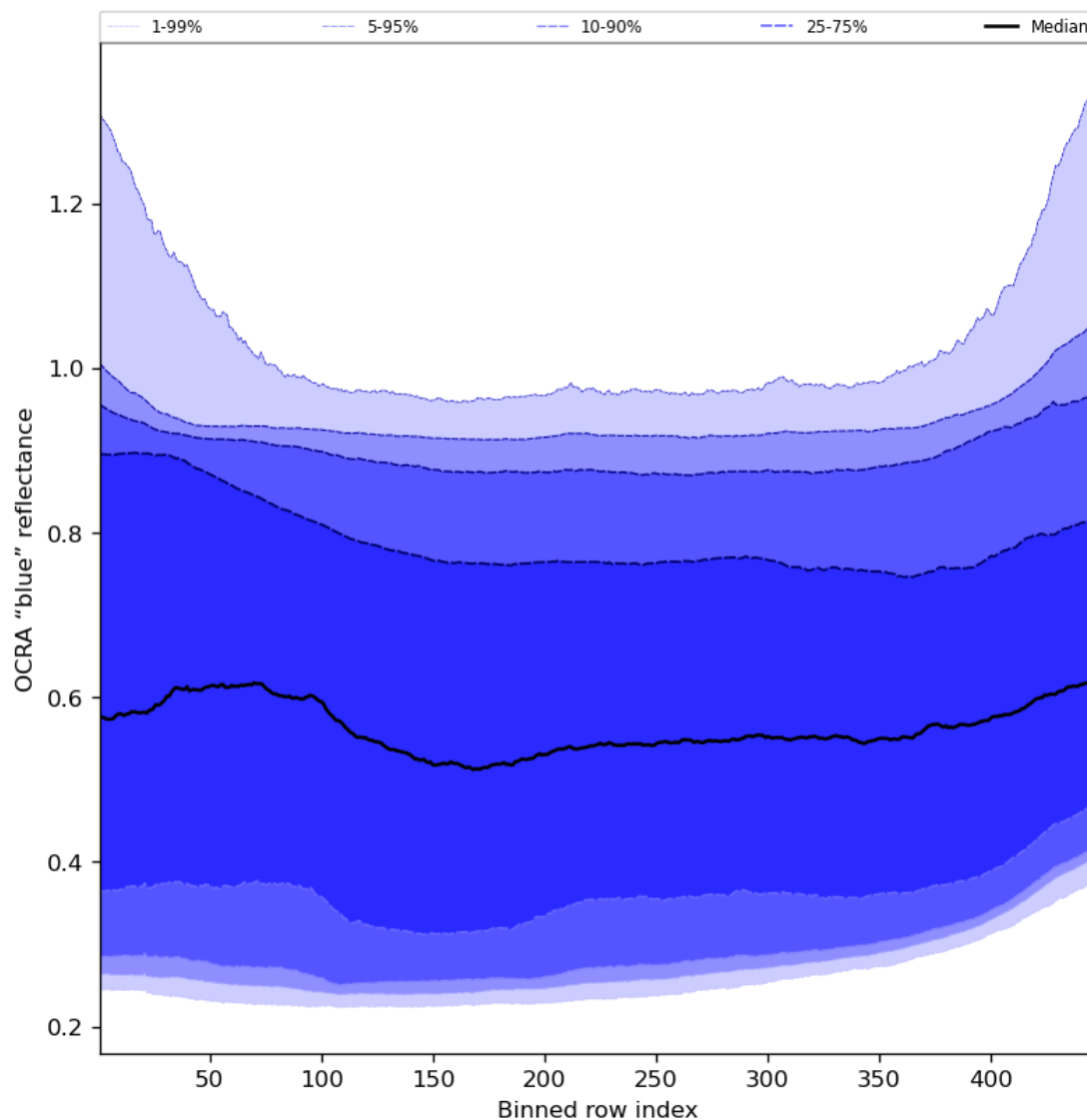
Figure 67: Along track statistics of “OCRA “blue” reflectance” for 2024-01-01 to 2024-01-03
