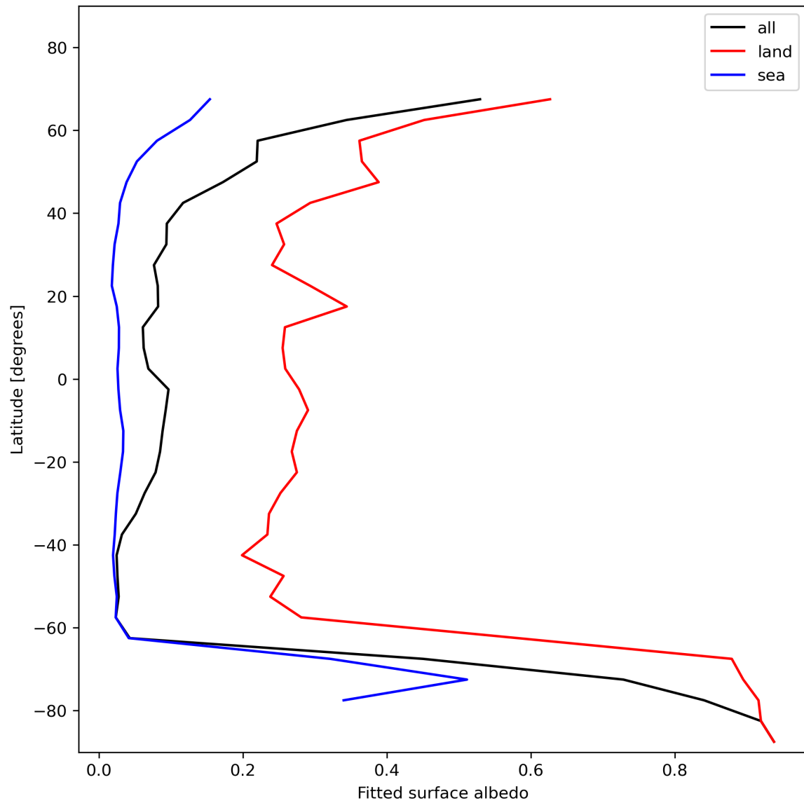
Figure 29: Zonal average of “Fitted surface albedo” for 2024-01-01 to 2024-01-03.
