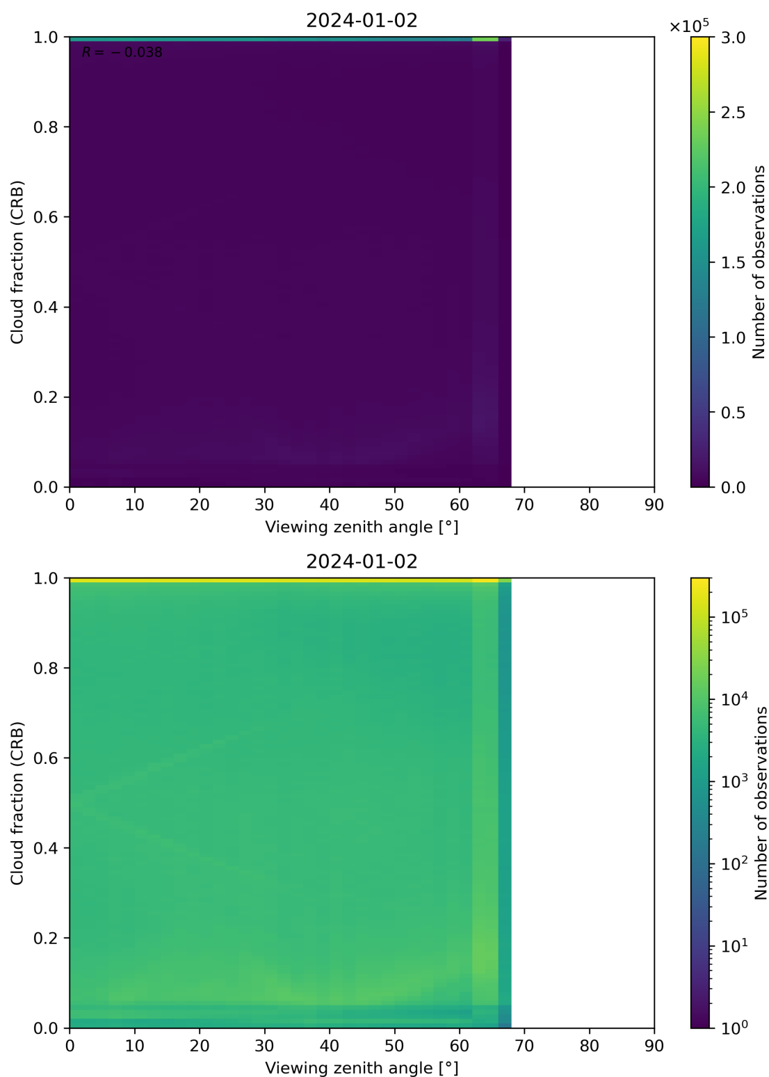
Figure 109: Scatter density plot of “Viewing zenith angle” against “Cloud fraction (CRB)” for 2024-01-01 to 2024-01-03.
