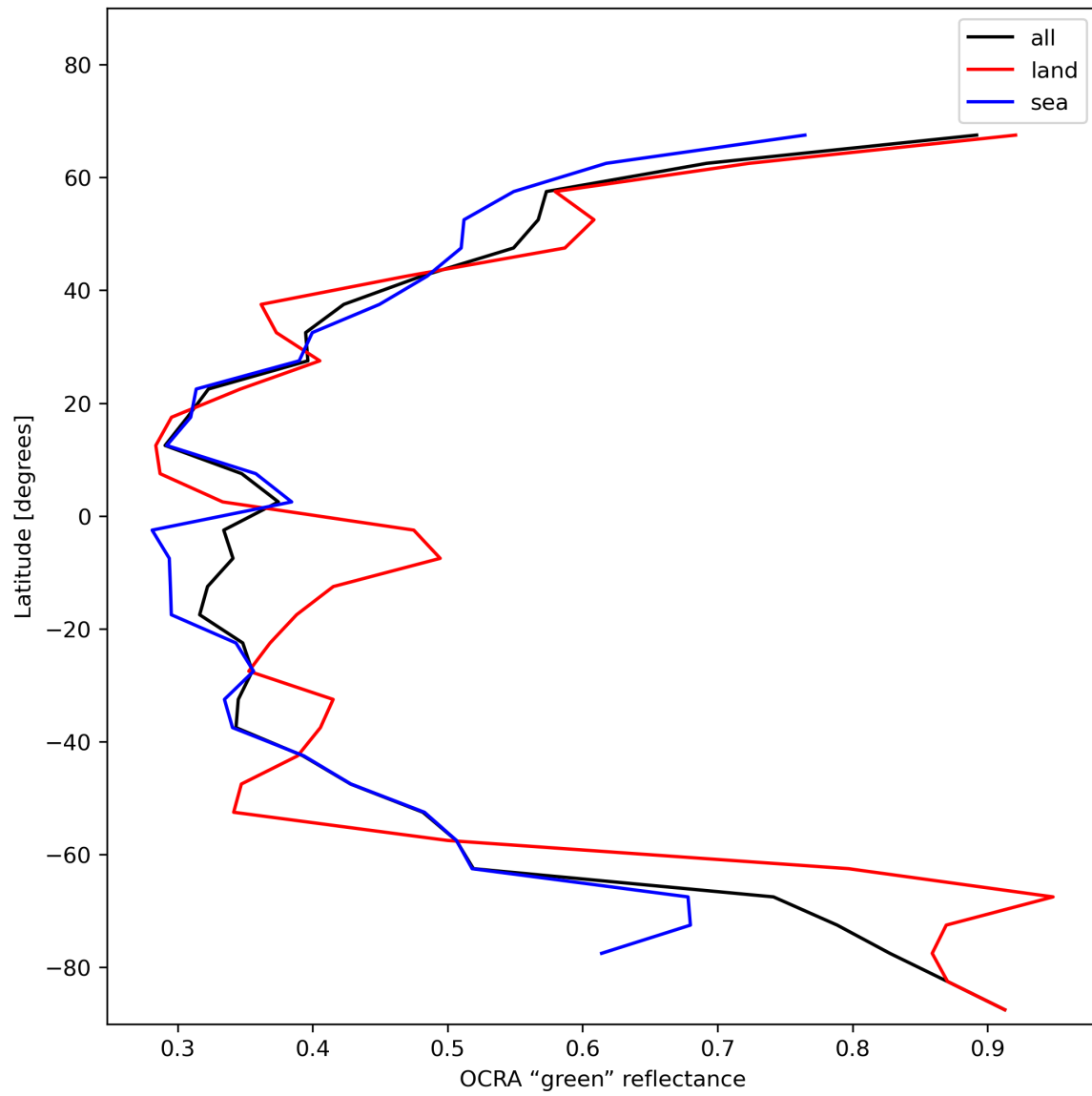
Figure 36: Zonal average of “OCRA “green” reflectance” for 2024-01-01 to 2024-01-03.
