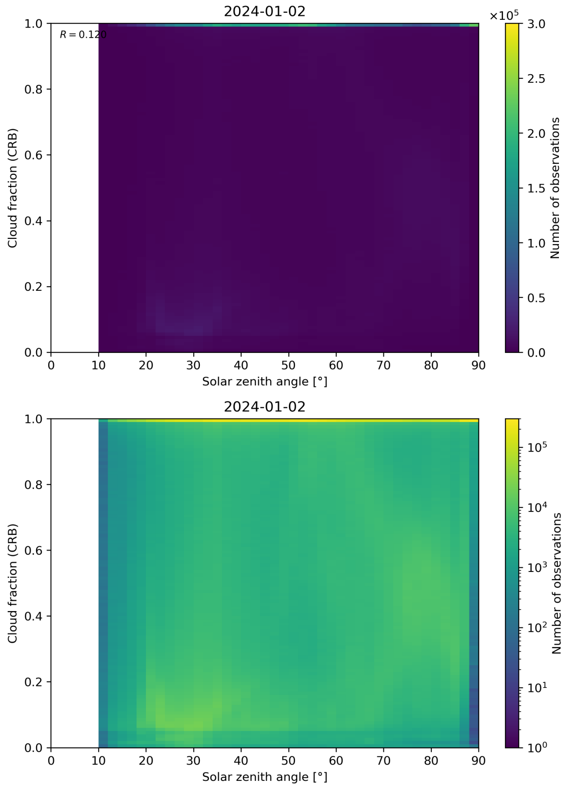
Figure 101: Scatter density plot of “Solar zenith angle” against “Cloud fraction (CRB)” for 2024-01-01 to 2024-01-03.
