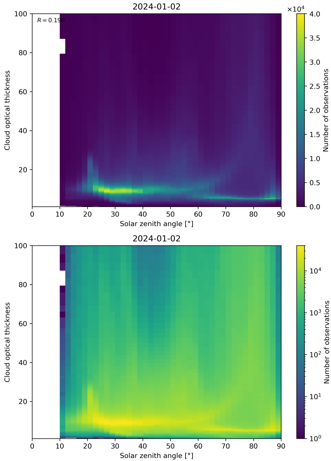
Figure 103: Scatter density plot of “Solar zenith angle” against “Cloud optical thickness” for 2024-01-01 to 2024-01-03.
