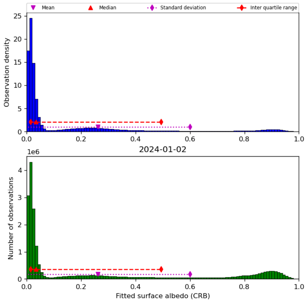
Figure 46: Histogram of “Fitted surface albedo (CRB)” for 2024-01-01 to 2024-01-03
