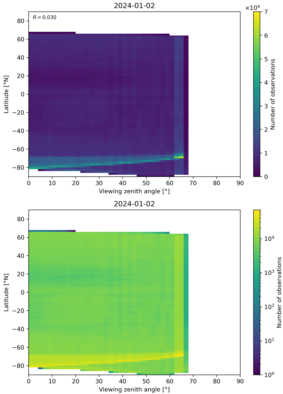
Figure 113: Scatter density plot of “Viewing zenith angle” against “Latitude” for 2024-01-01 to 2024-01-03.
