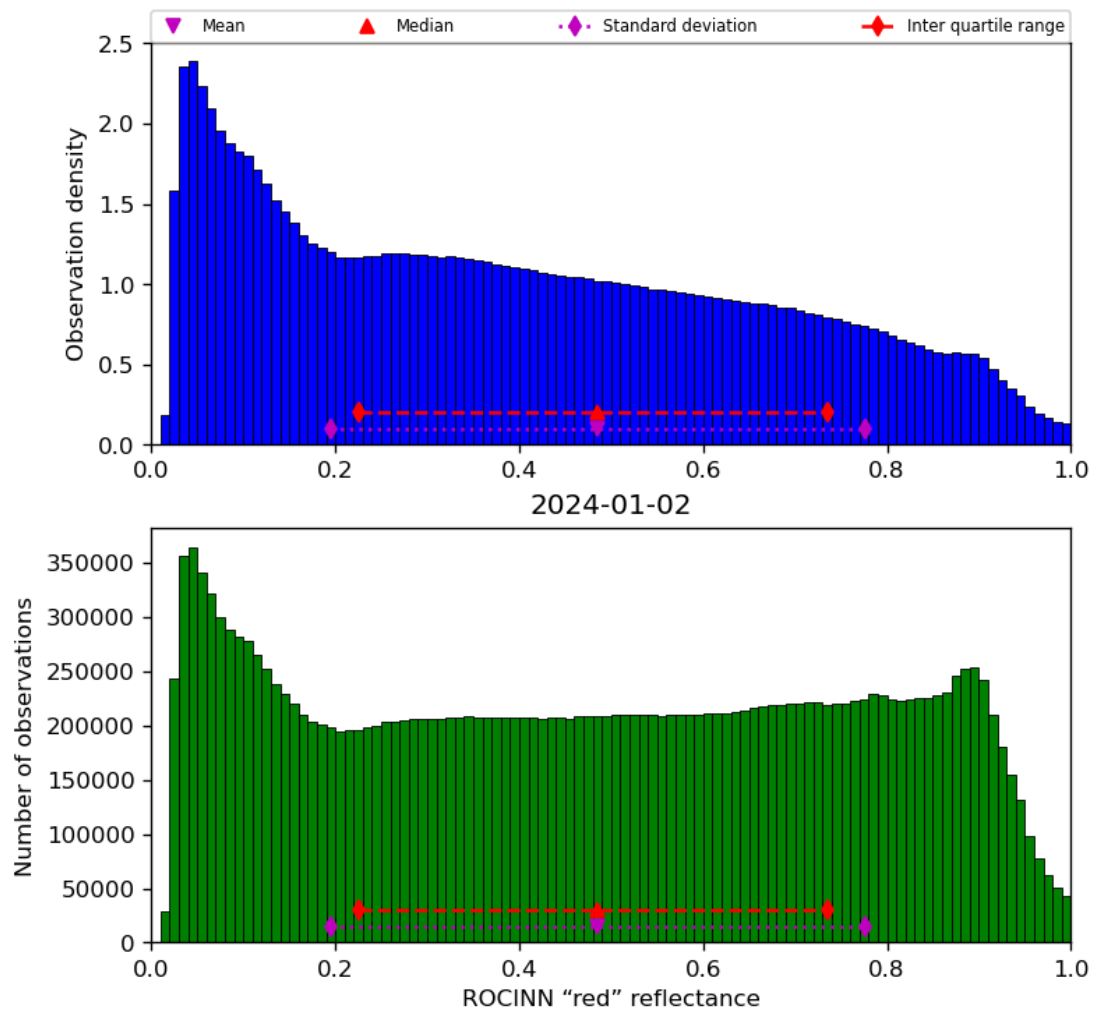
Figure 53: Histogram of “ROCINN “red” reflectance” for 2024-01-01 to 2024-01-03
