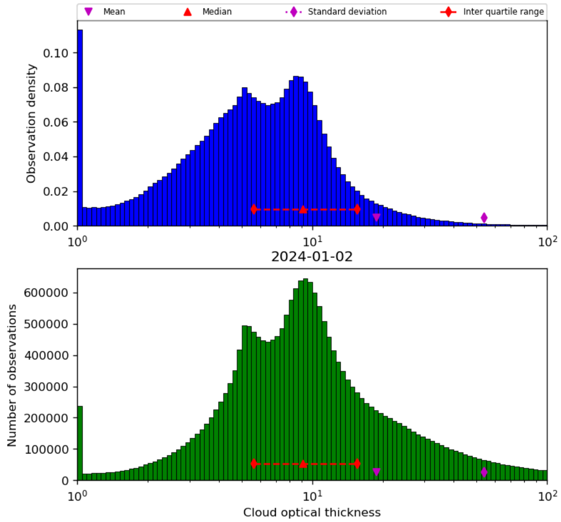
Figure 41: Histogram of “Cloud optical thickness” for 2024-01-01 to 2024-01-03
