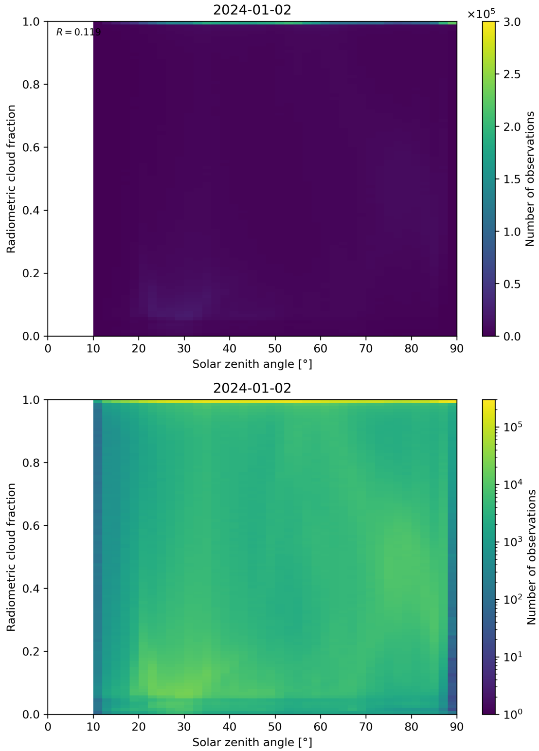
Figure 99: Scatter density plot of “Solar zenith angle” against “Radiometric cloud fraction” for 2024-01-01 to 2024-01-03.
