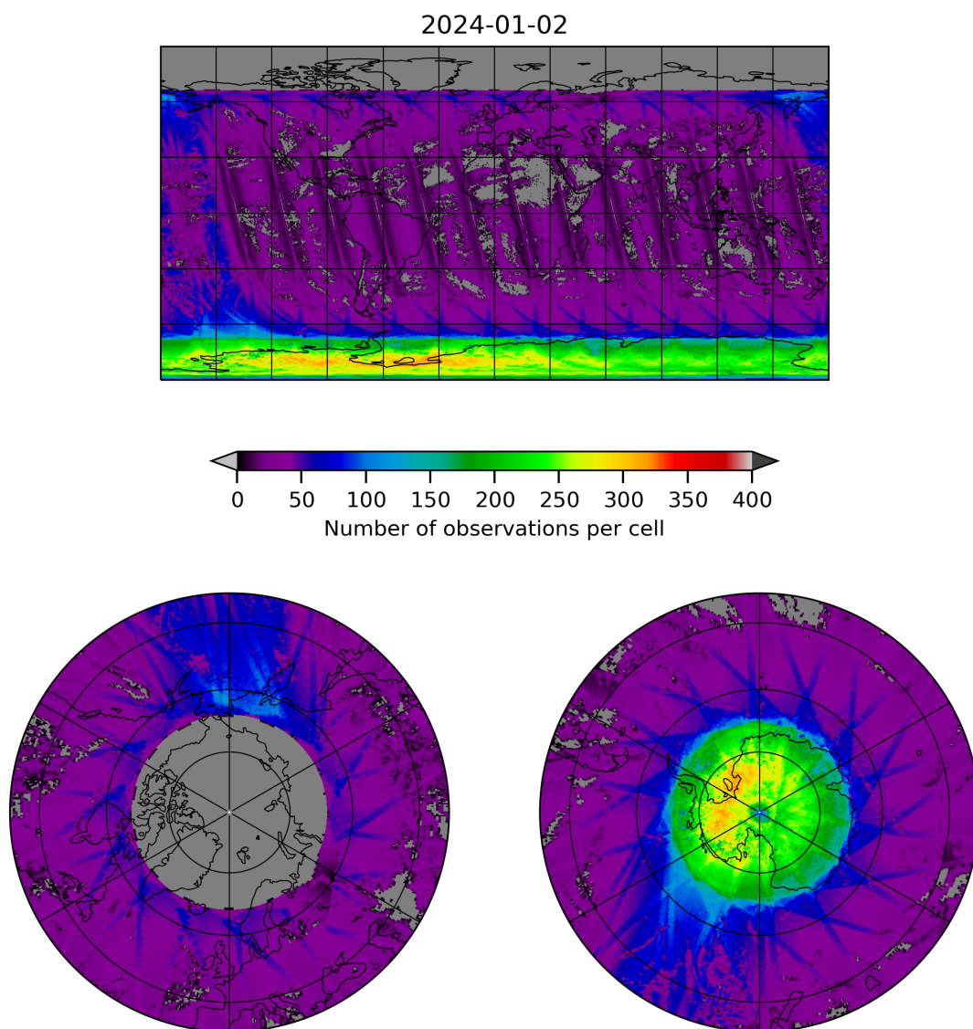
Figure 21: Map of the number of observations for 2024-01-01 to 2024-01-03
