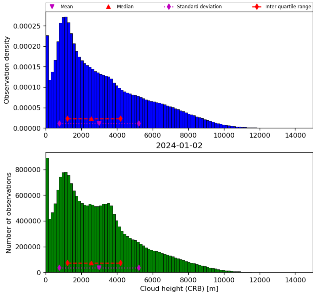
Figure 43: Histogram of “Cloud height (CRB)” for 2024-01-01 to 2024-01-03
