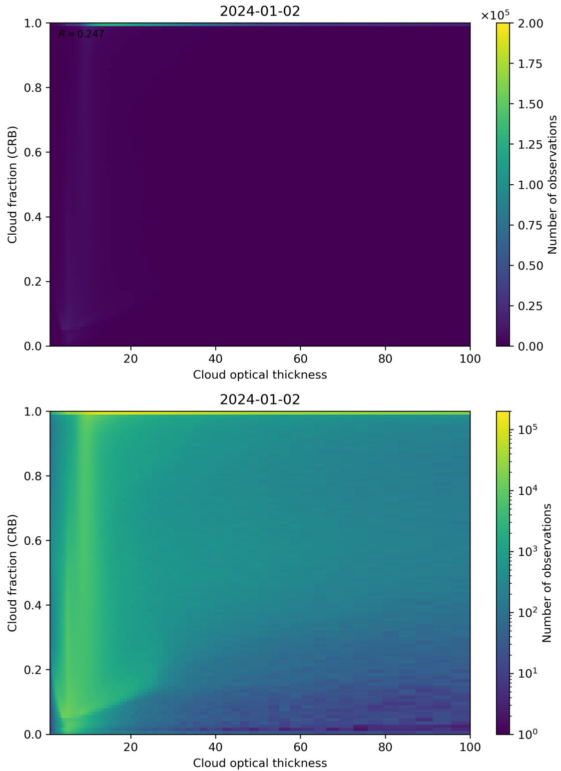
Figure 84: Scatter density plot of “Cloud optical thickness” against “Cloud fraction (CRB)” for 2024-01-01 to 2024-01-03.
