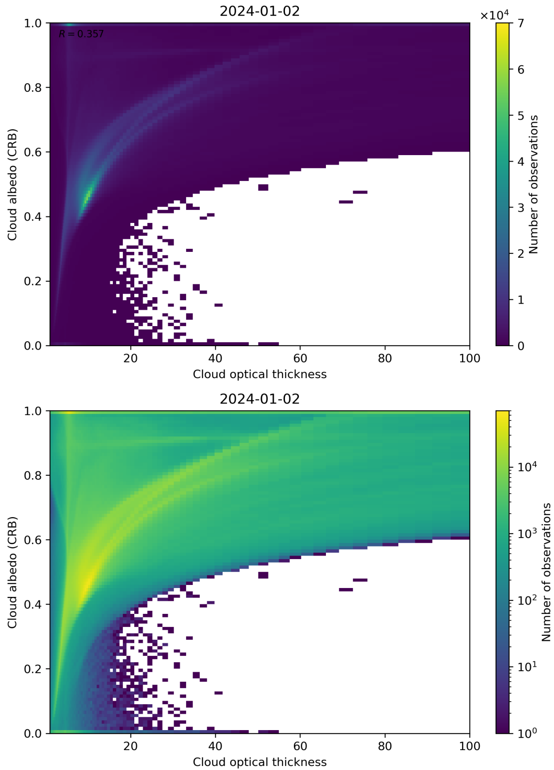
Figure 82: Scatter density plot of “Cloud optical thickness” against “Cloud albedo (CRB)” for 2024-01-01 to 2024-01-03.
