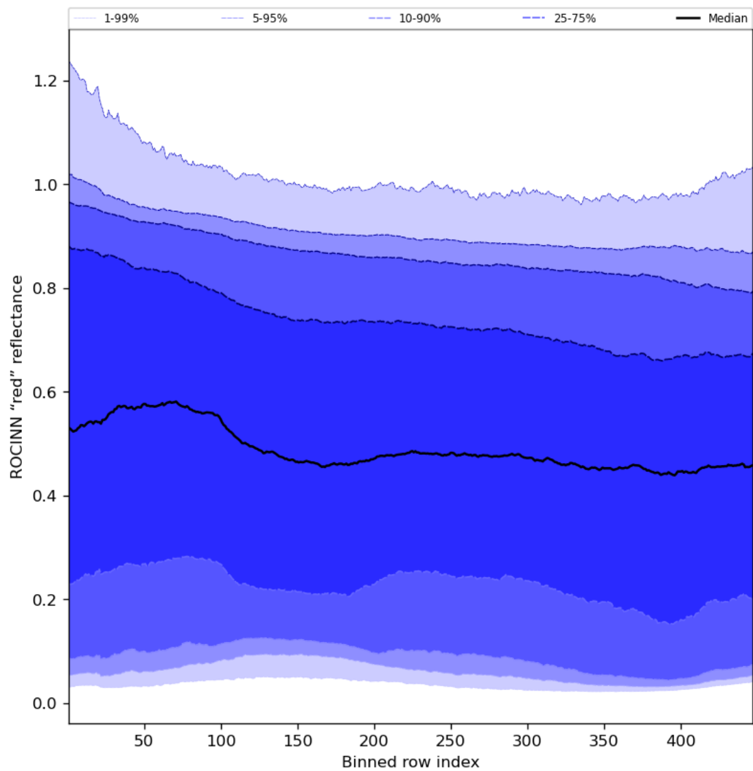
Figure 69: Along track statistics of “ROCINN “red” reflectance” for 2024-01-01 to 2024-01-03
