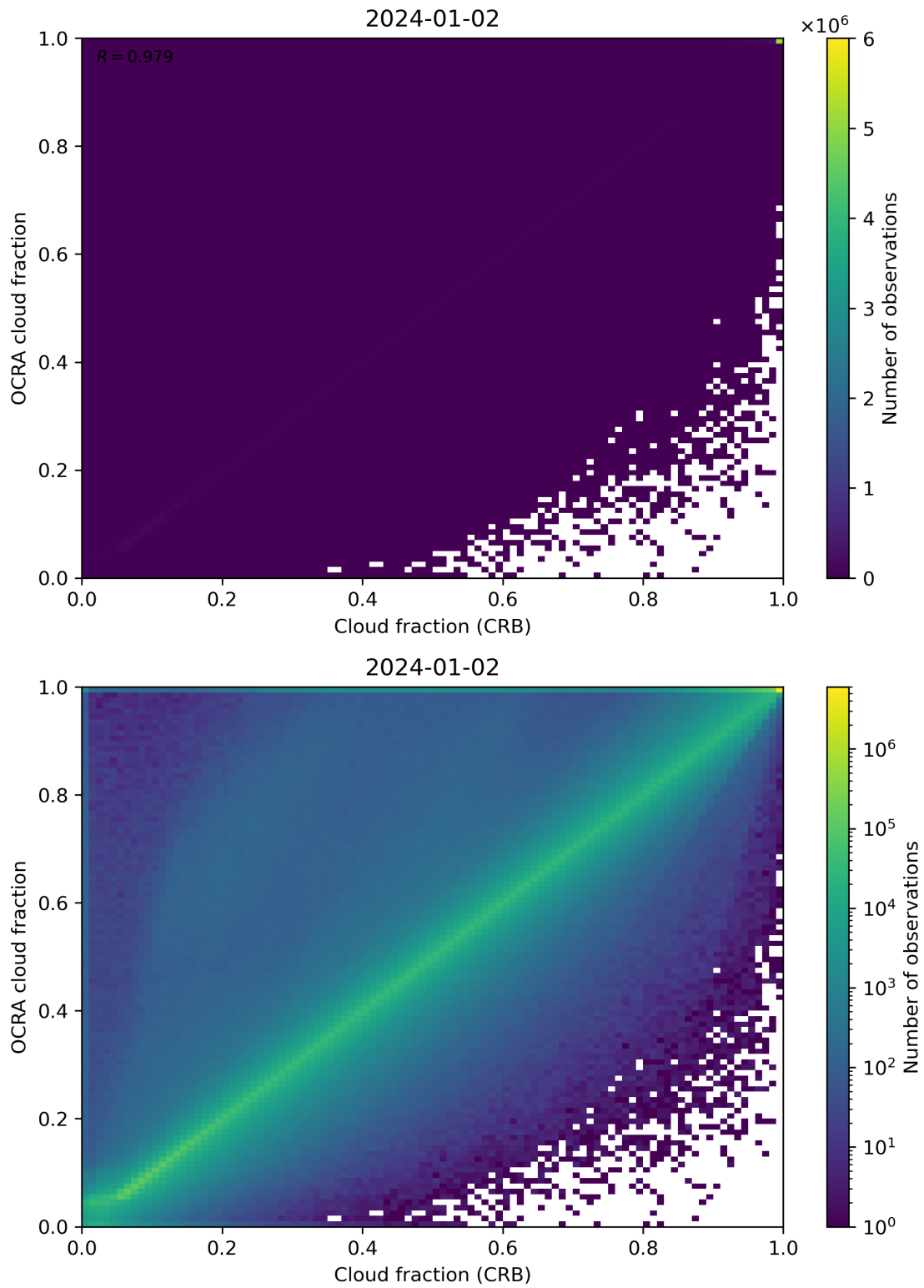
Figure 78: Scatter density plot of “Cloud fraction (CRB)” against “OCRA cloud fraction” for 2024-01-01 to 2024-01-03.
