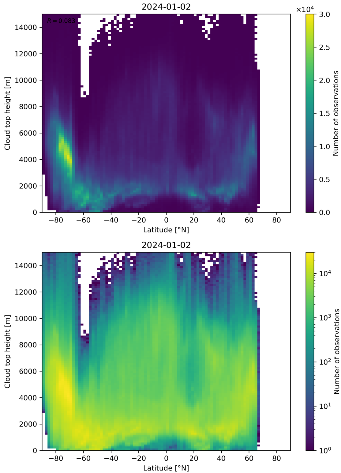
Figure 97: Scatter density plot of “Latitude” against “Cloud top height” for 2024-01-01 to 2024-01-03.
