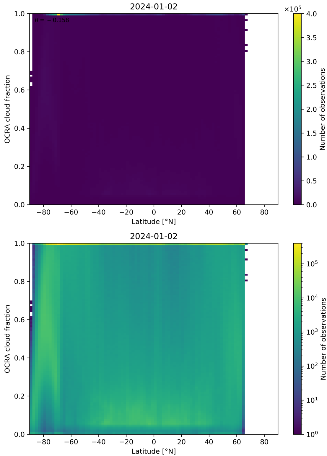
Figure 93: Scatter density plot of “Latitude” against “OCRA cloud fraction” for 2024-01-01 to 2024-01-03.
