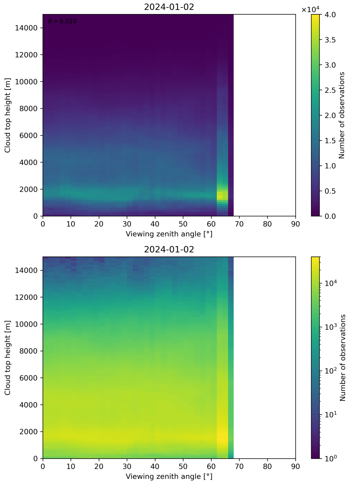
Figure 112: Scatter density plot of “Viewing zenith angle” against “Cloud top height” for 2024-01-01 to 2024-01-03.
