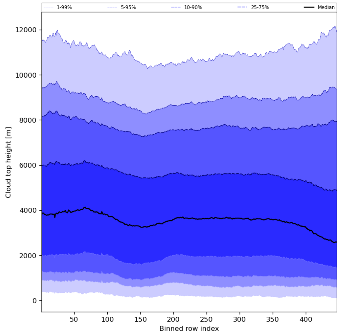
Figure 56: Along track statistics of “Cloud top height” for 2024-01-01 to 2024-01-03
