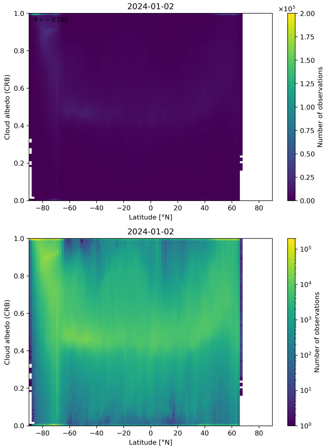
Figure 91: Scatter density plot of “Latitude” against “Cloud albedo (CRB)” for 2024-01-01 to 2024-01-03.
