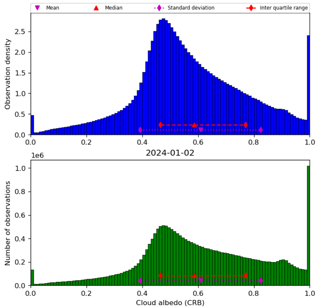
Figure 44: Histogram of “Cloud albedo (CRB)” for 2024-01-01 to 2024-01-03
