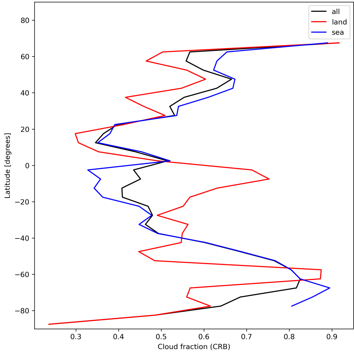
Figure 26: Zonal average of “Cloud fraction (CRB)” for 2024-01-01 to 2024-01-03.
