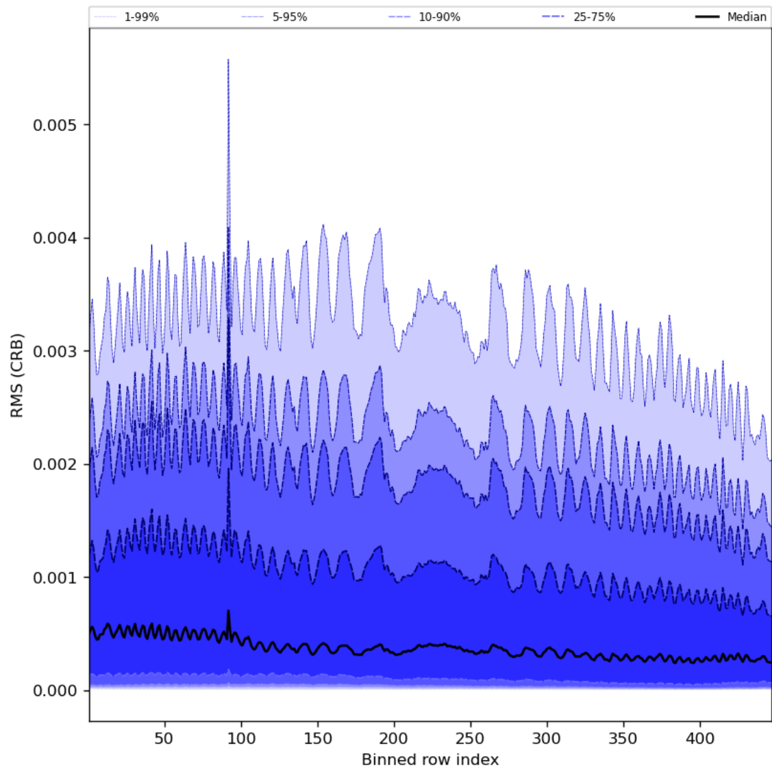
Figure 64: Along track statistics of “RMS (CRB)” for 2024-01-01 to 2024-01-03
