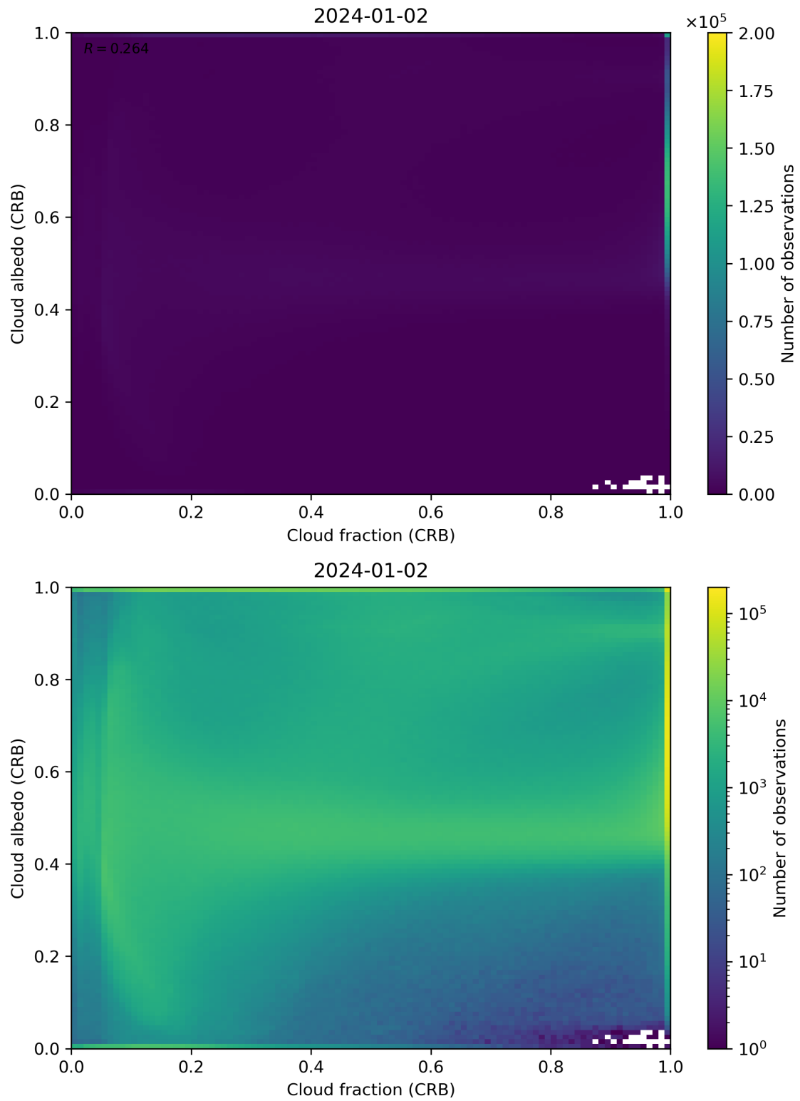
Figure 77: Scatter density plot of “Cloud fraction (CRB)” against “Cloud albedo (CRB)” for 2024-01-01 to 2024-01-03.
