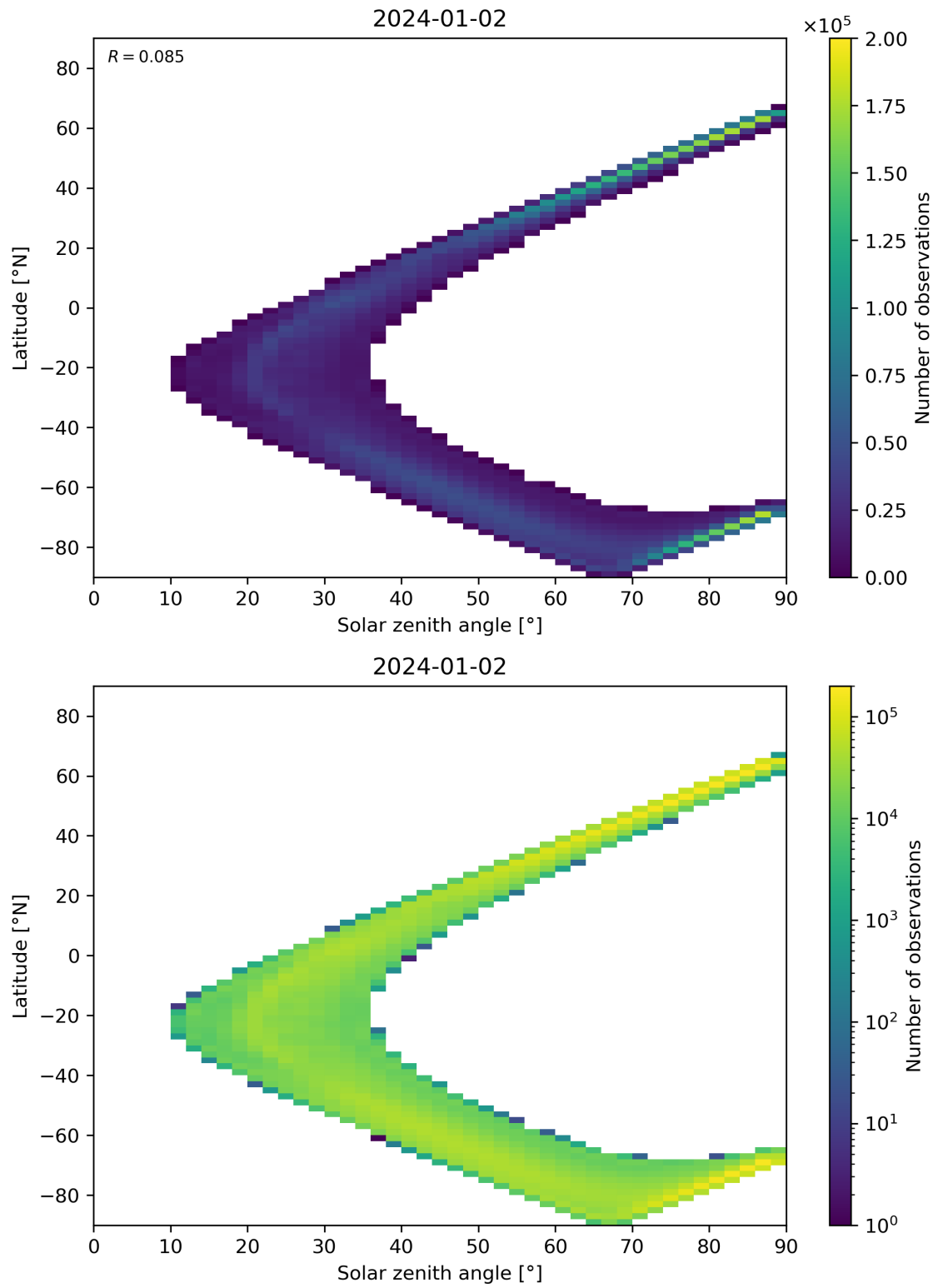
Figure 105: Scatter density plot of “Solar zenith angle” against “Latitude” for 2024-01-01 to 2024-01-03.
