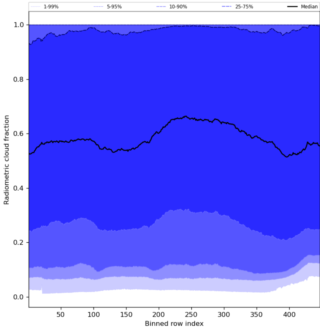
Figure 55: Along track statistics of “Radiometric cloud fraction” for 2024-01-01 to 2024-01-03
