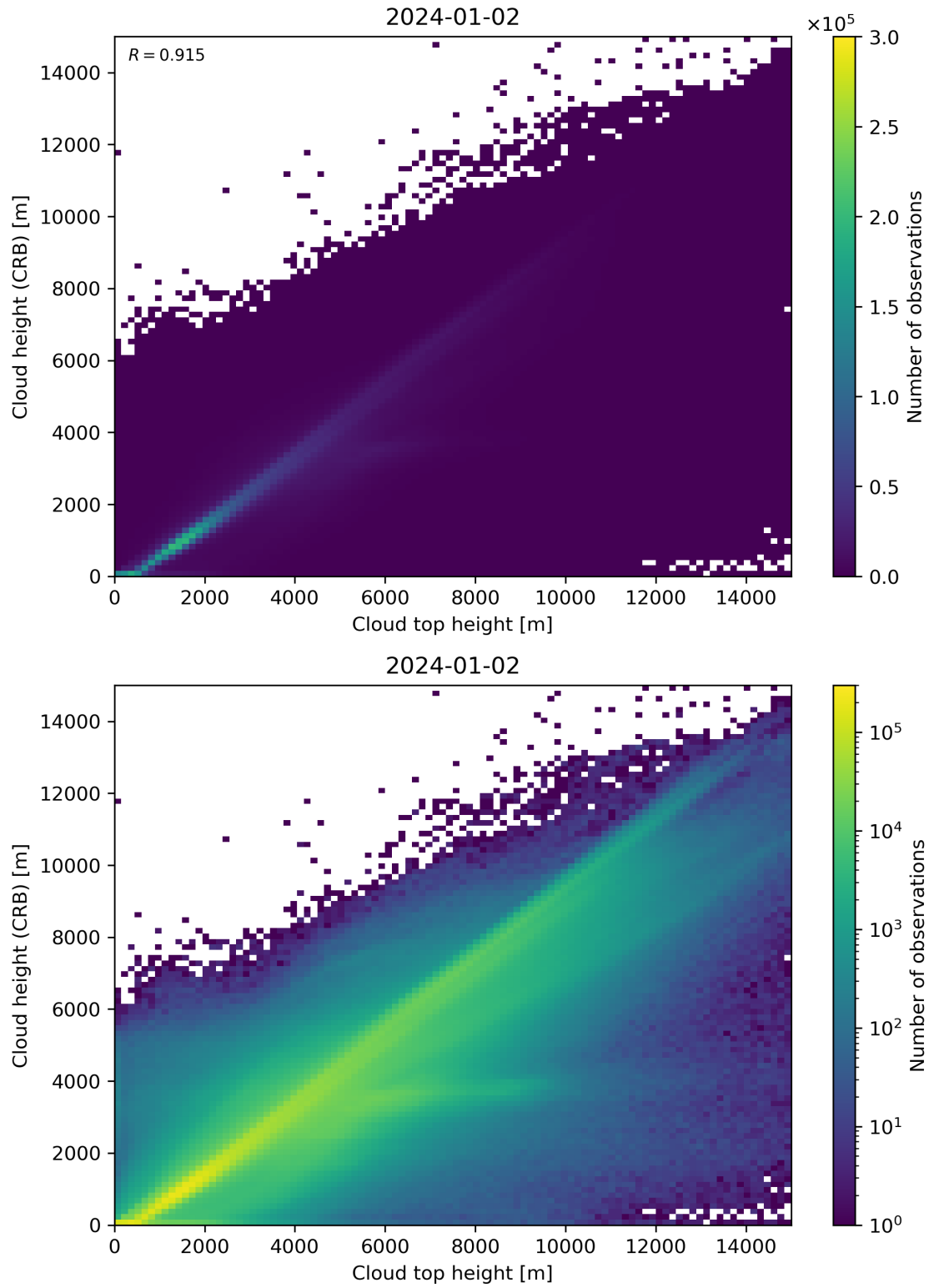
Figure 89: Scatter density plot of “Cloud top height” against “Cloud height (CRB)” for 2024-01-01 to 2024-01-03.
