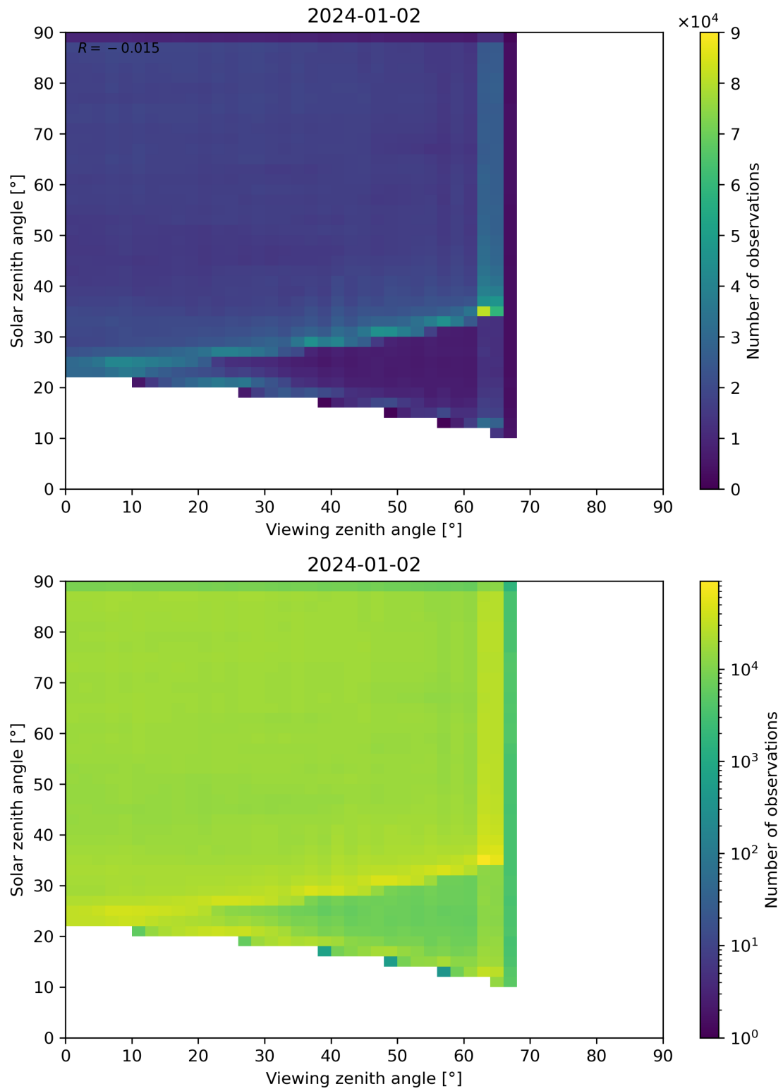
Figure 114: Scatter density plot of “Viewing zenith angle” against “Solar zenith angle” for 2024-01-01 to 2024-01-03.
