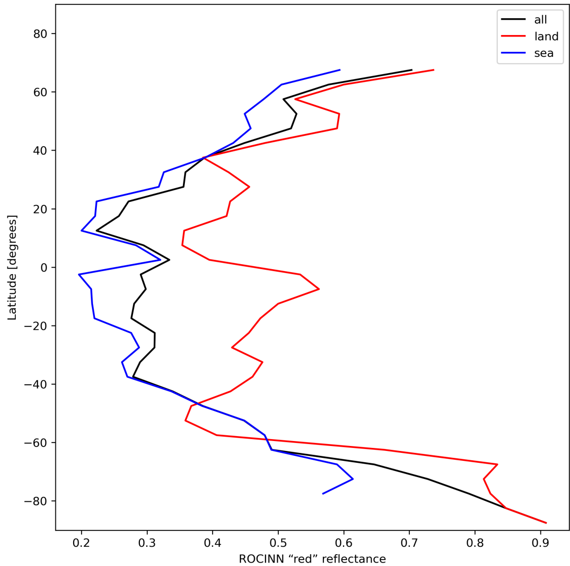
Figure 37: Zonal average of “ROCINN “red” reflectance” for 2024-01-01 to 2024-01-03.
