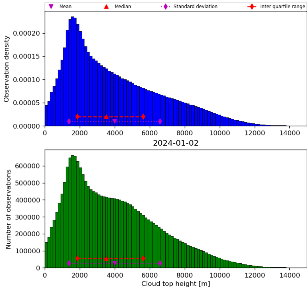
Figure 40: Histogram of “Cloud top height” for 2024-01-01 to 2024-01-03
