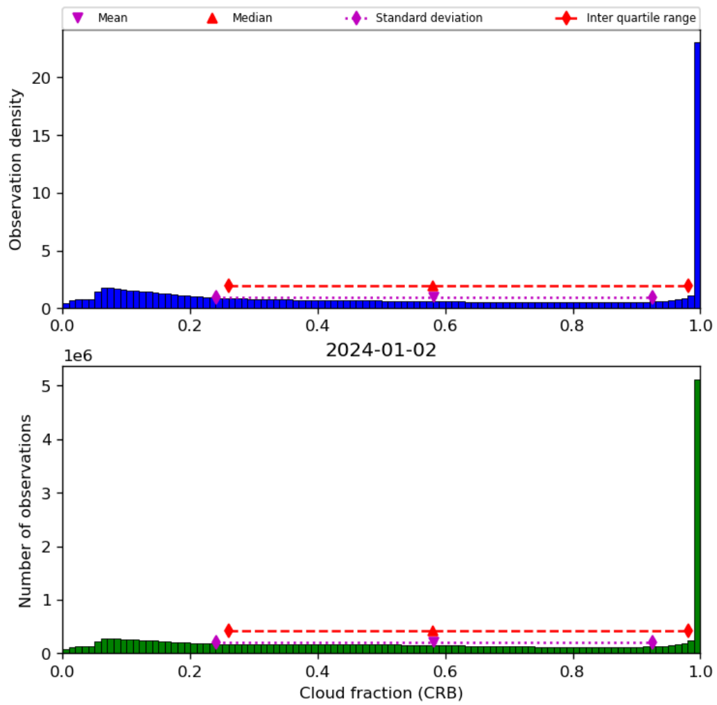
Figure 42: Histogram of “Cloud fraction (CRB)” for 2024-01-01 to 2024-01-03
