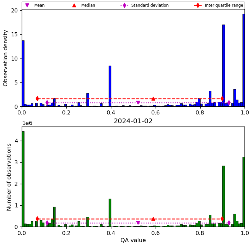
Figure 38: Histogram of “QA value” for 2024-01-01 to 2024-01-03
