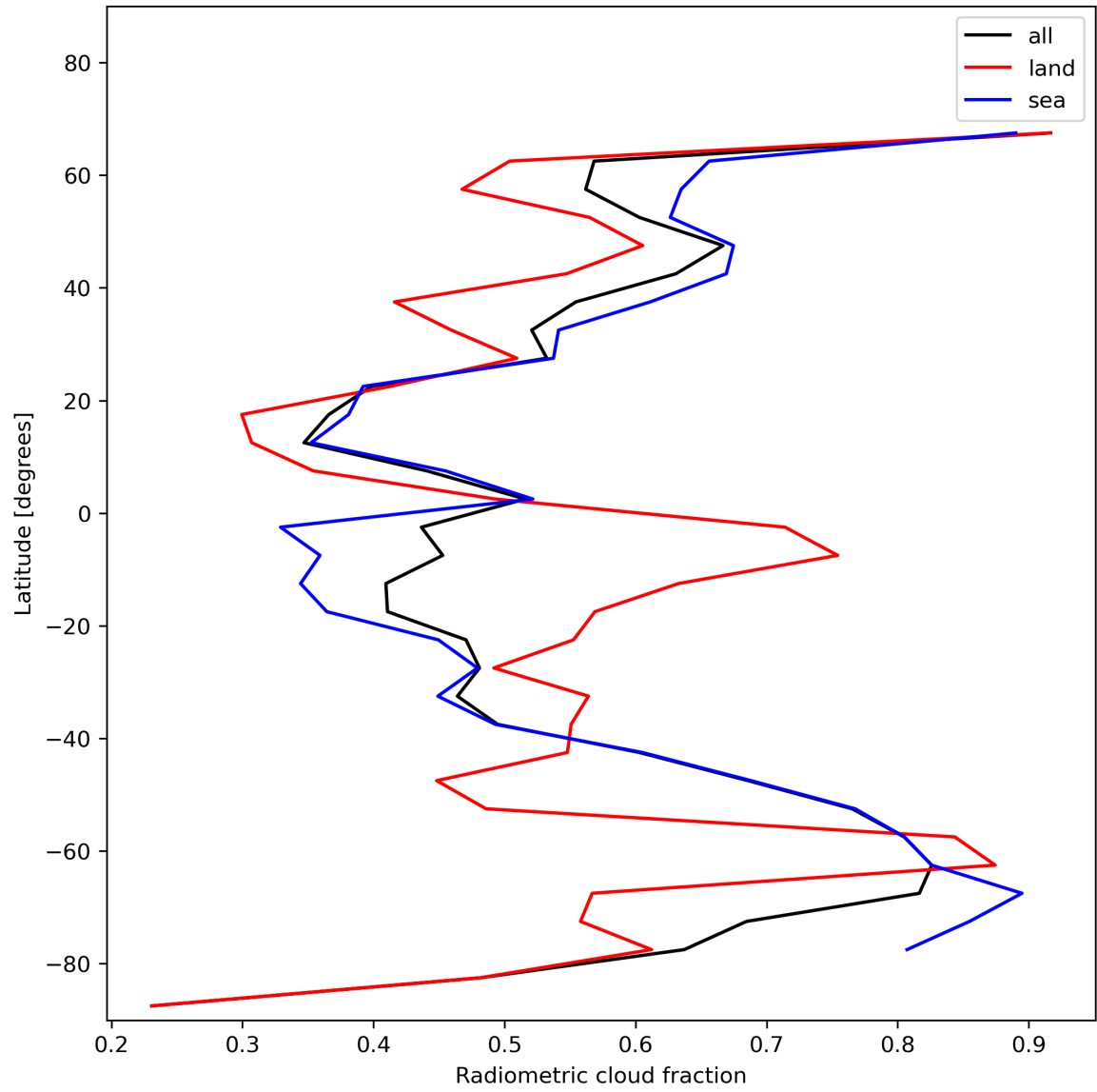
Figure 23: Zonal average of “Radiometric cloud fraction” for 2024-01-01 to 2024-01-03.
