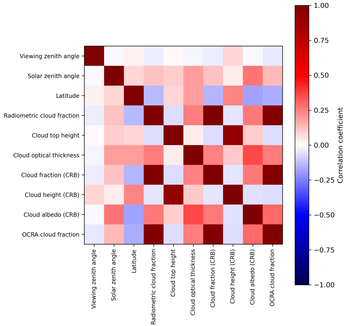
Figure 2: Map of correlation matrix for 2024-01-01 to 2024-01-03.
