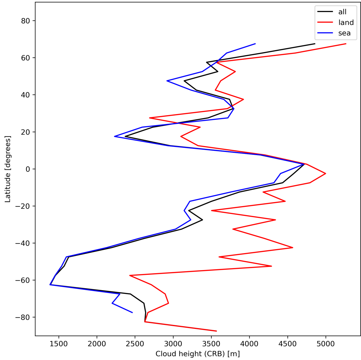
Figure 27: Zonal average of “Cloud height (CRB)” for 2024-01-01 to 2024-01-03.
