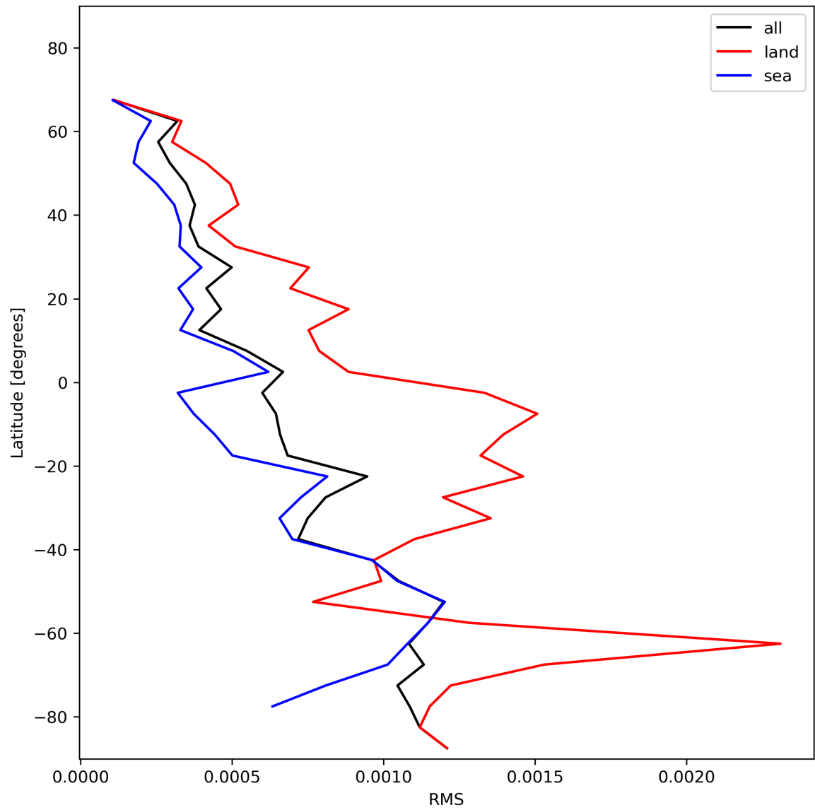
Figure 31: Zonal average of “RMS” for 2024-01-01 to 2024-01-03.
