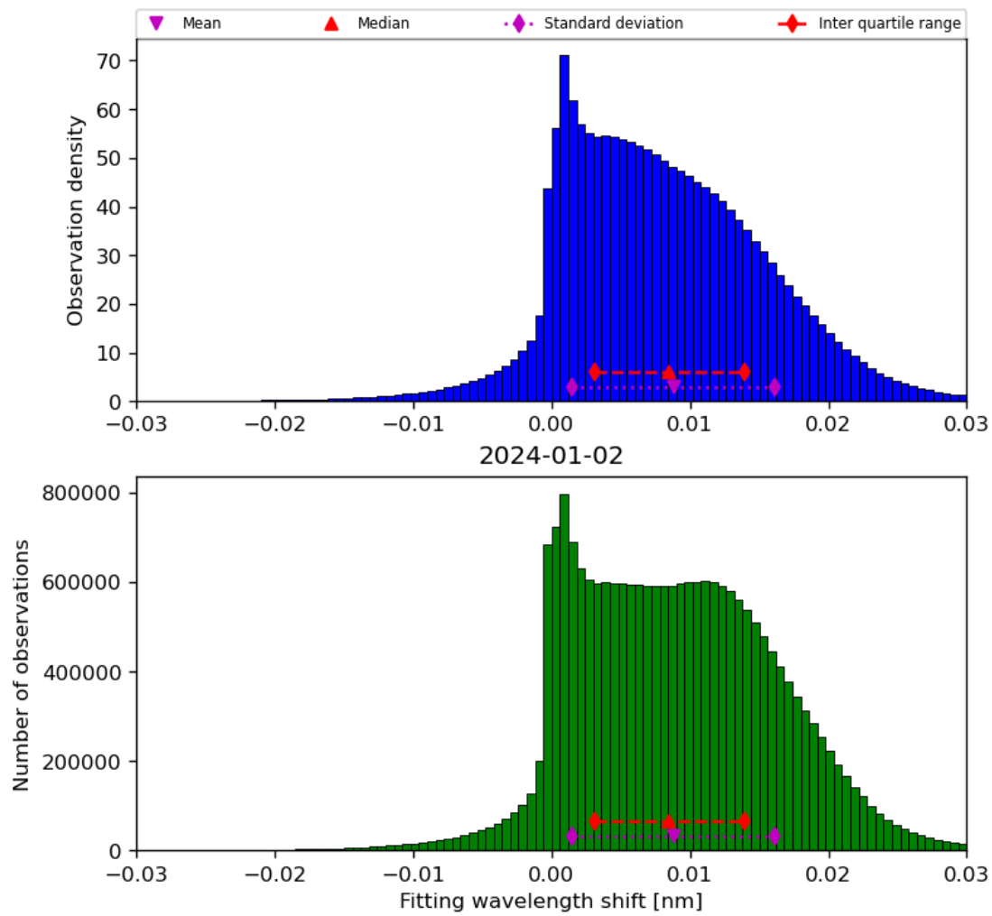
Figure 49: Histogram of “Fitting wavelength shift” for 2024-01-01 to 2024-01-03
