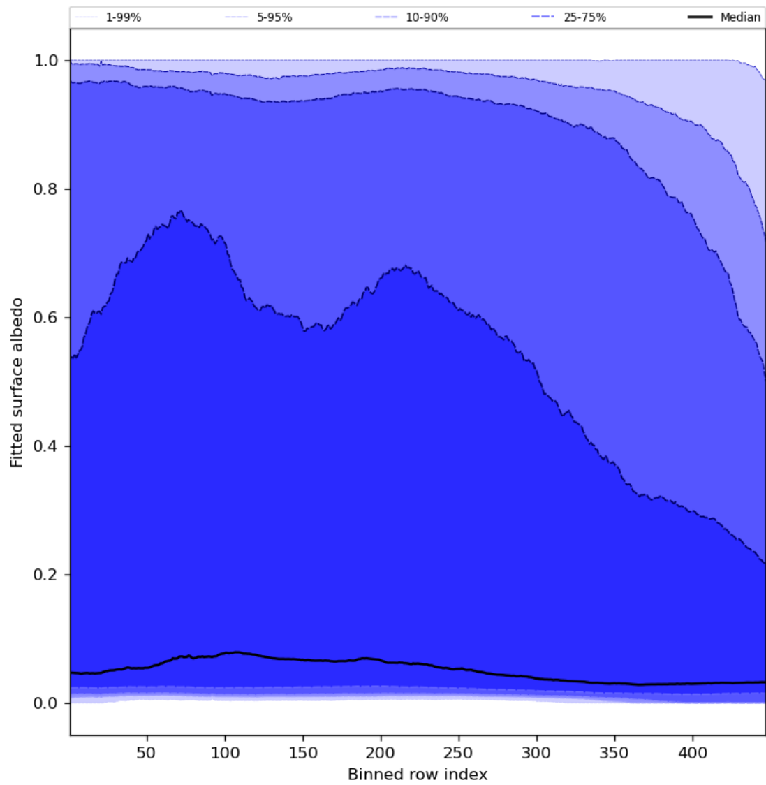
Figure 61: Along track statistics of “Fitted surface albedo” for 2024-01-01 to 2024-01-03
