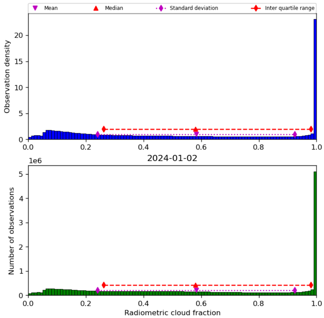
Figure 39: Histogram of “Radiometric cloud fraction” for 2024-01-01 to 2024-01-03
