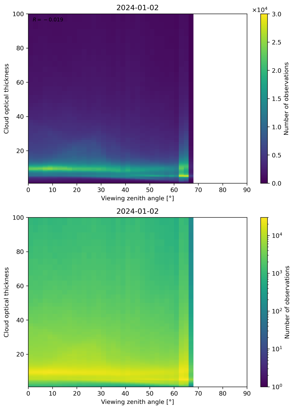
Figure 111: Scatter density plot of “Viewing zenith angle” against “Cloud optical thickness” for 2024-01-01 to 2024-01-03.
