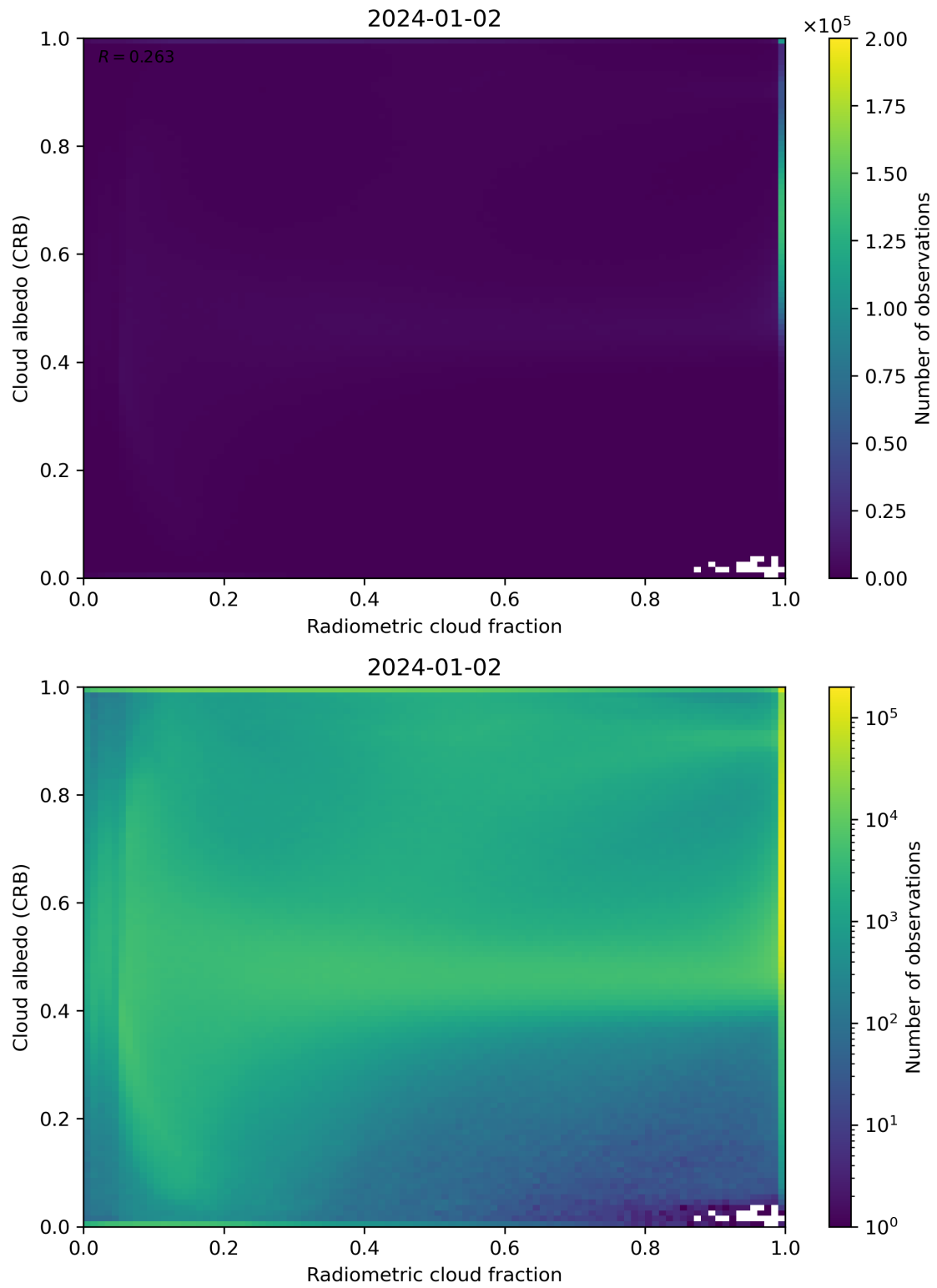
Figure 71: Scatter density plot of “Radiometric cloud fraction” against “Cloud albedo (CRB)” for 2024-01-01 to 2024-01-03.
