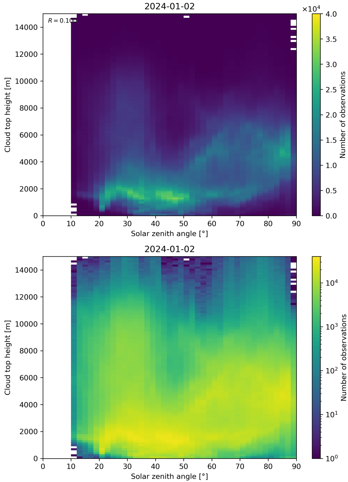
Figure 104: Scatter density plot of “Solar zenith angle” against “Cloud top height” for 2024-01-01 to 2024-01-03.
