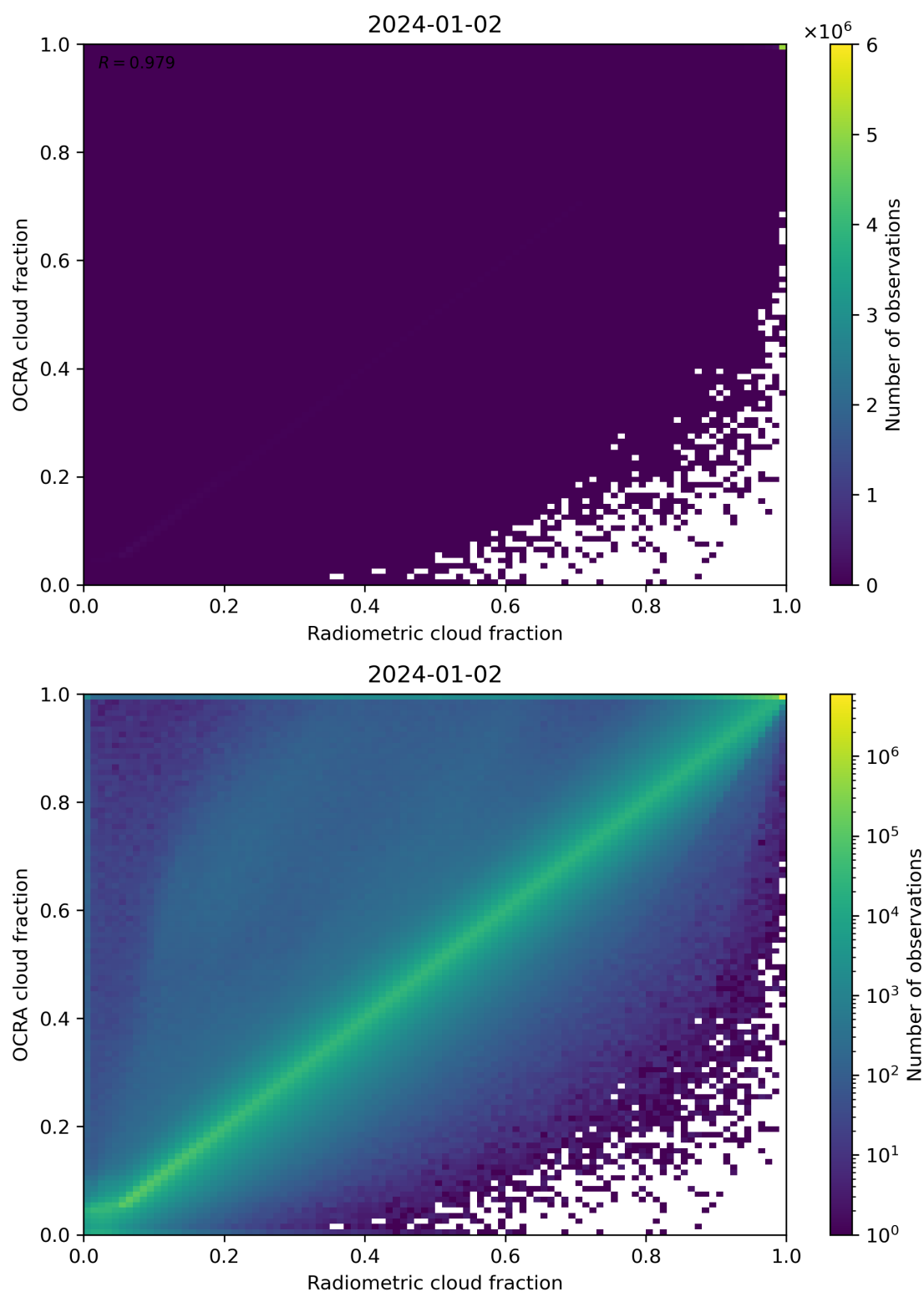
Figure 72: Scatter density plot of “Radiometric cloud fraction” against “OCRA cloud fraction” for 2024-01-01 to 2024-01-03.
