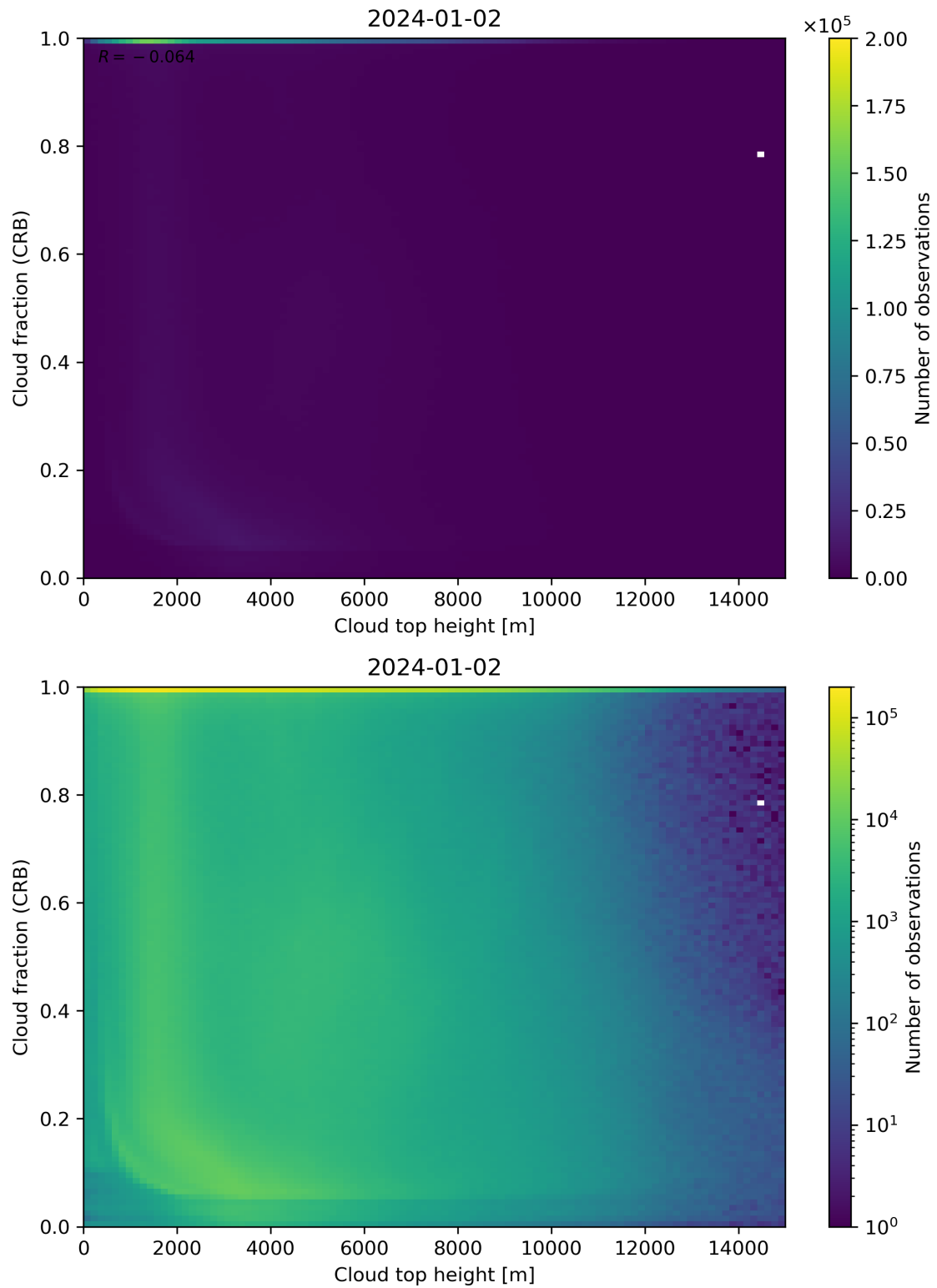
Figure 88: Scatter density plot of “Cloud top height” against “Cloud fraction (CRB)” for 2024-01-01 to 2024-01-03.
