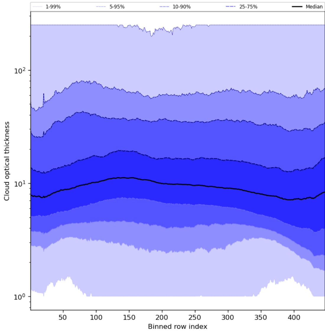
Figure 57: Along track statistics of “Cloud optical thickness” for 2024-01-01 to 2024-01-03
