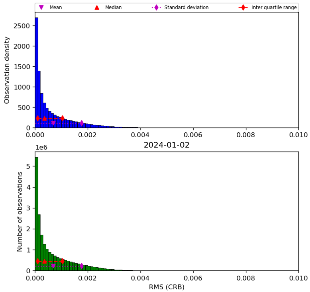
Figure 48: Histogram of “RMS (CRB)” for 2024-01-01 to 2024-01-03
