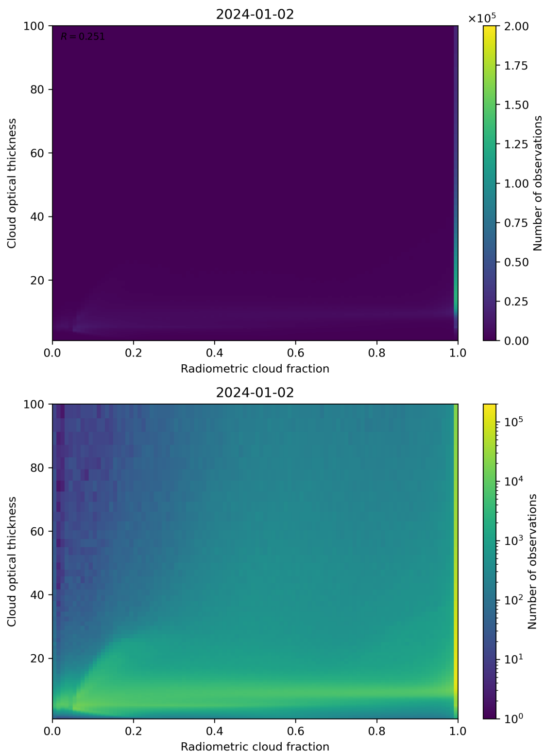
Figure 75: Scatter density plot of “Radiometric cloud fraction” against “Cloud optical thickness” for 2024-01-01 to 2024-01-03.
