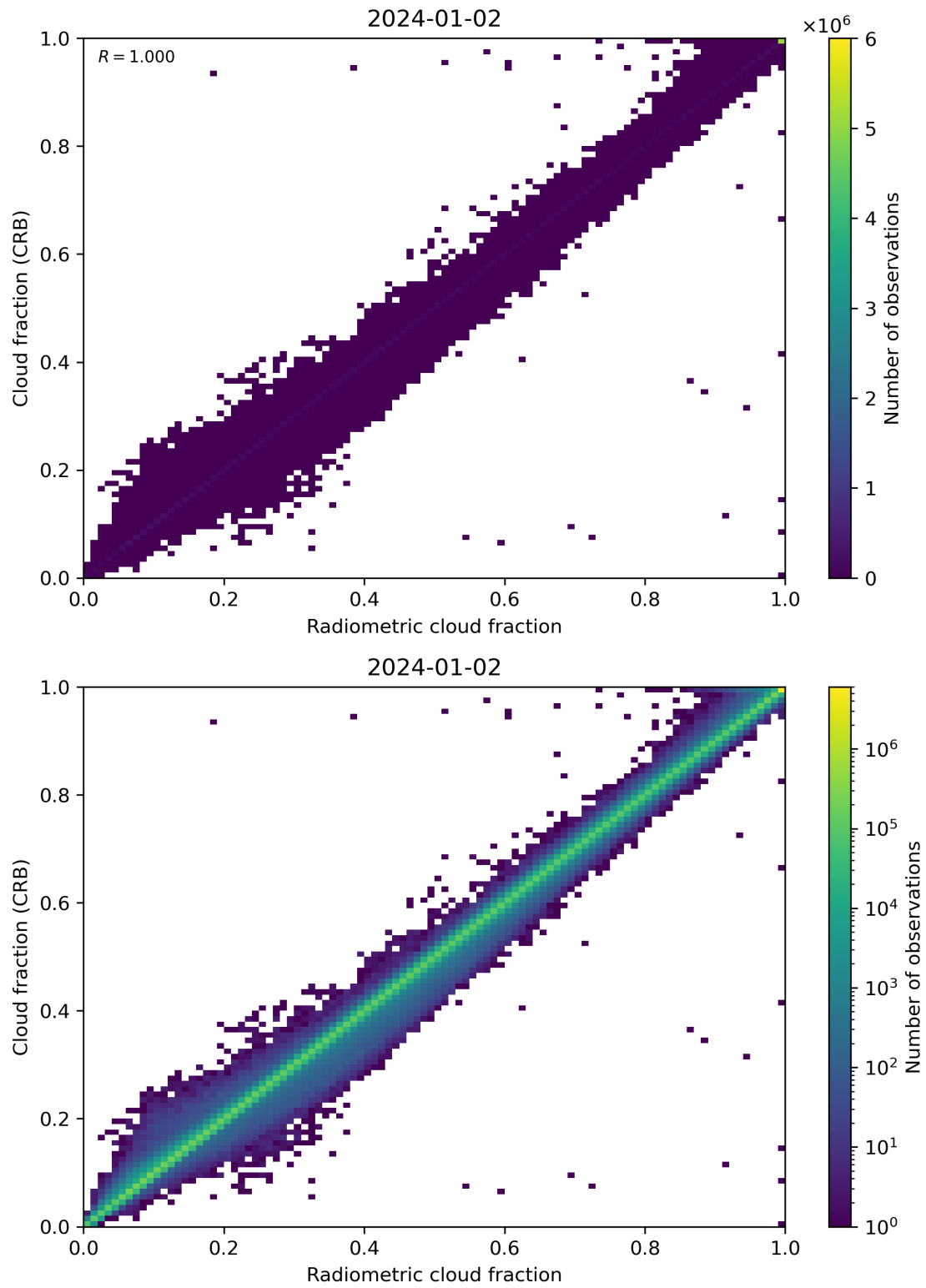
Figure 73: Scatter density plot of “Radiometric cloud fraction” against “Cloud fraction (CRB)” for 2024-01-01 to 2024-01-03.
