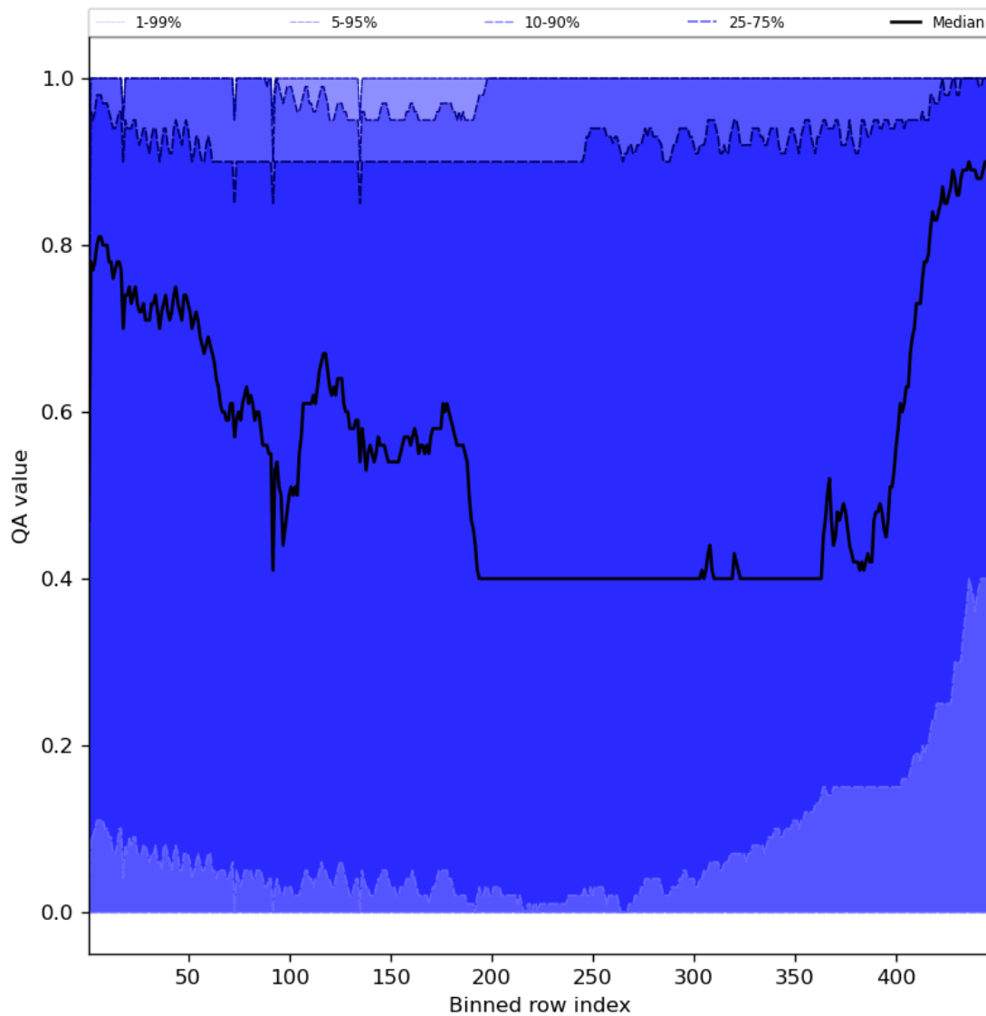
Figure 54: Along track statistics of “QA value” for 2024-01-01 to 2024-01-03
