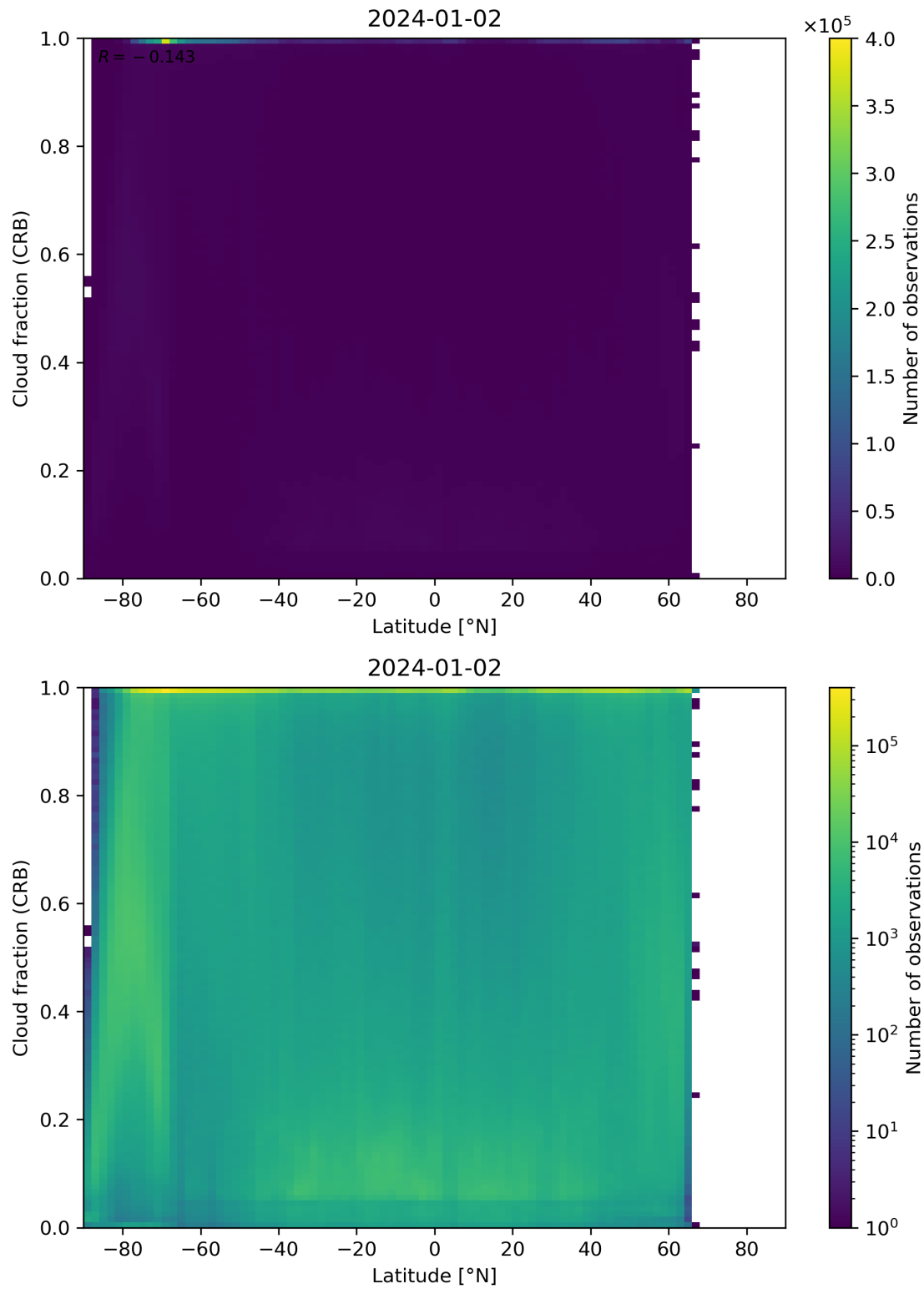
Figure 94: Scatter density plot of “Latitude” against “Cloud fraction (CRB)” for 2024-01-01 to 2024-01-03.
