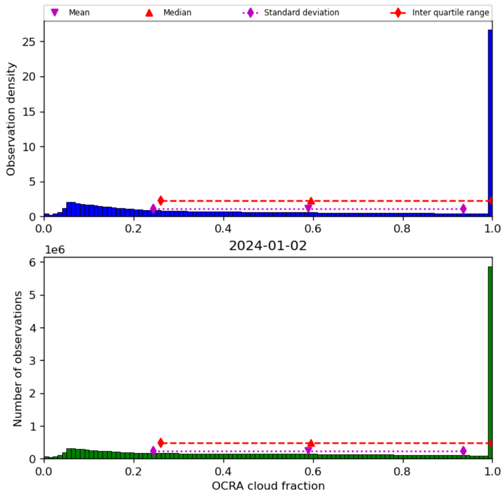
Figure 50: Histogram of “OCRA cloud fraction” for 2024-01-01 to 2024-01-03
