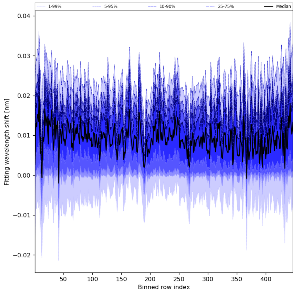
Figure 65: Along track statistics of “Fitting wavelength shift” for 2024-01-01 to 2024-01-03
