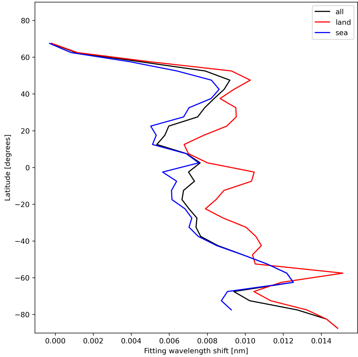
Figure 33: Zonal average of “Fitting wavelength shift” for 2024-01-01 to 2024-01-03.
