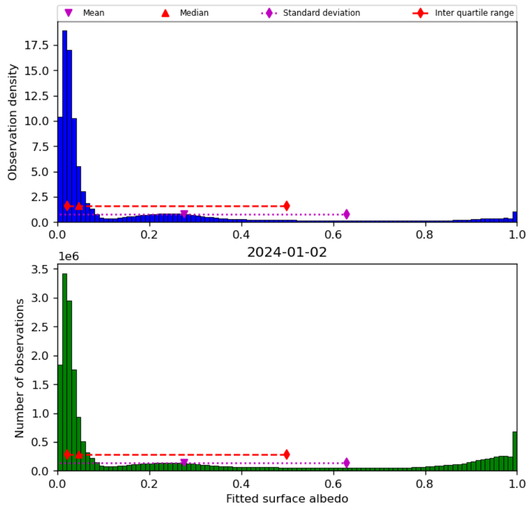
Figure 45: Histogram of “Fitted surface albedo” for 2024-01-01 to 2024-01-03
