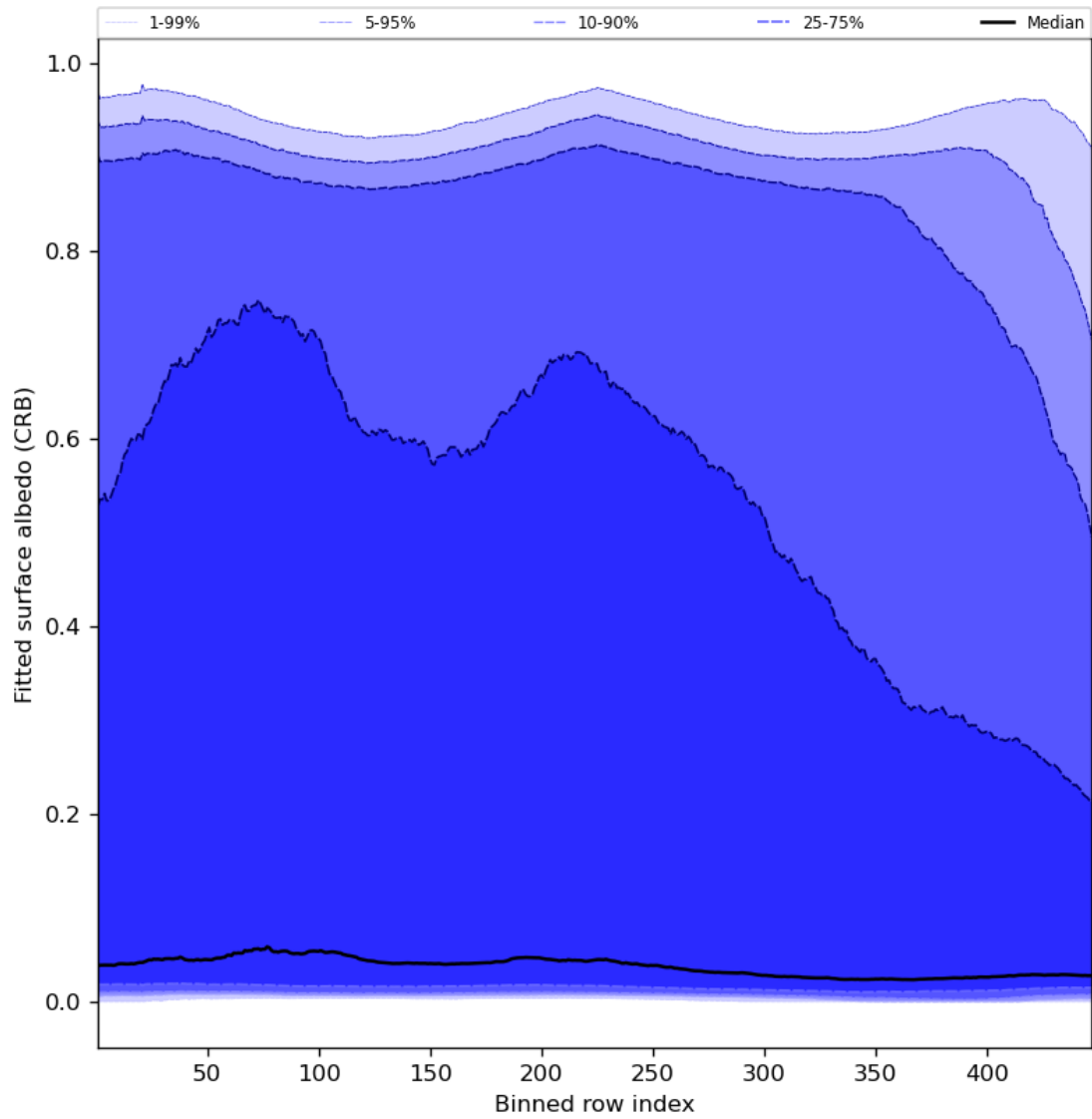
Figure 62: Along track statistics of “Fitted surface albedo (CRB)” for 2024-01-01 to 2024-01-03
