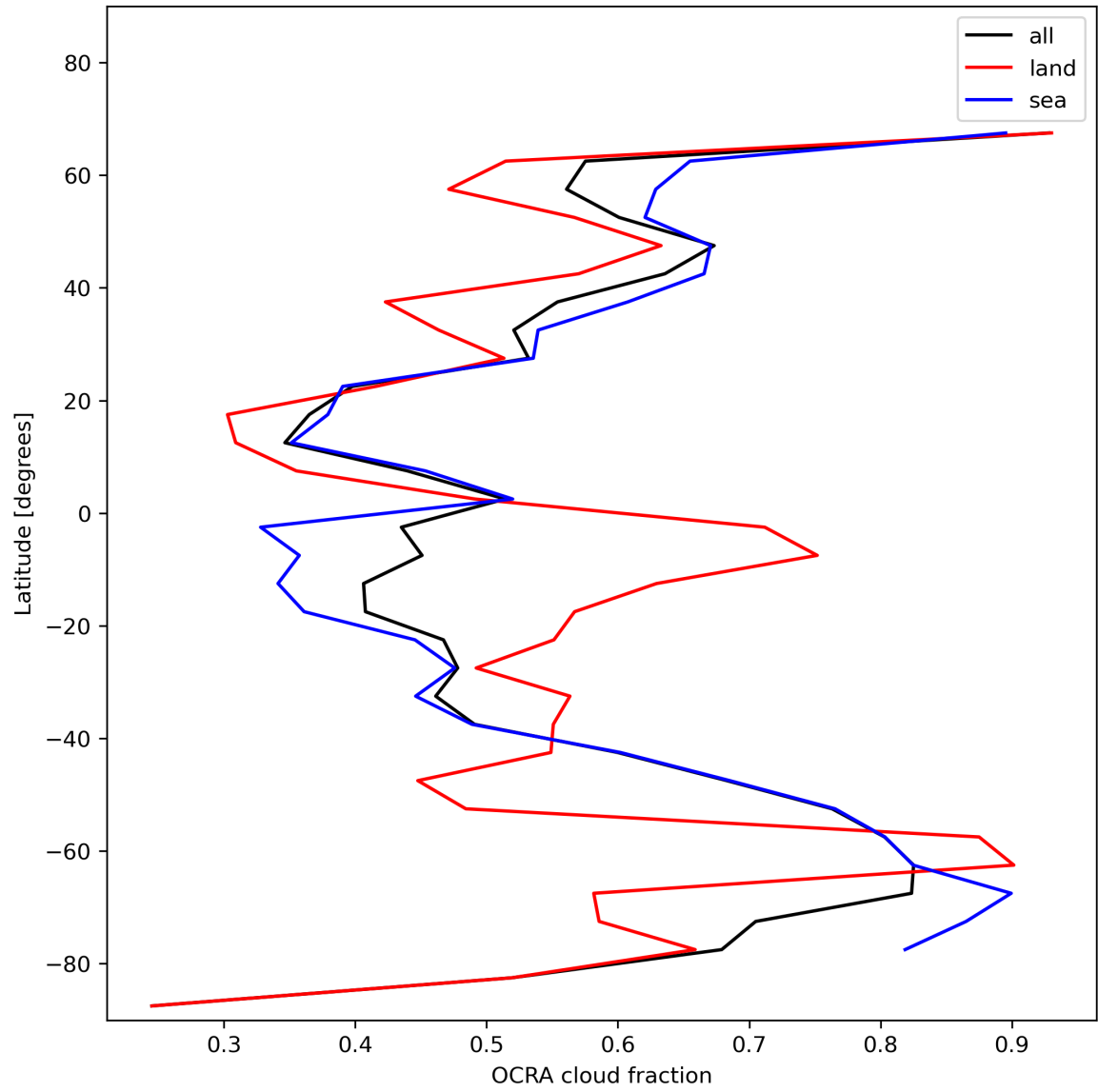
Figure 34: Zonal average of “OCRA cloud fraction” for 2024-01-01 to 2024-01-03.
