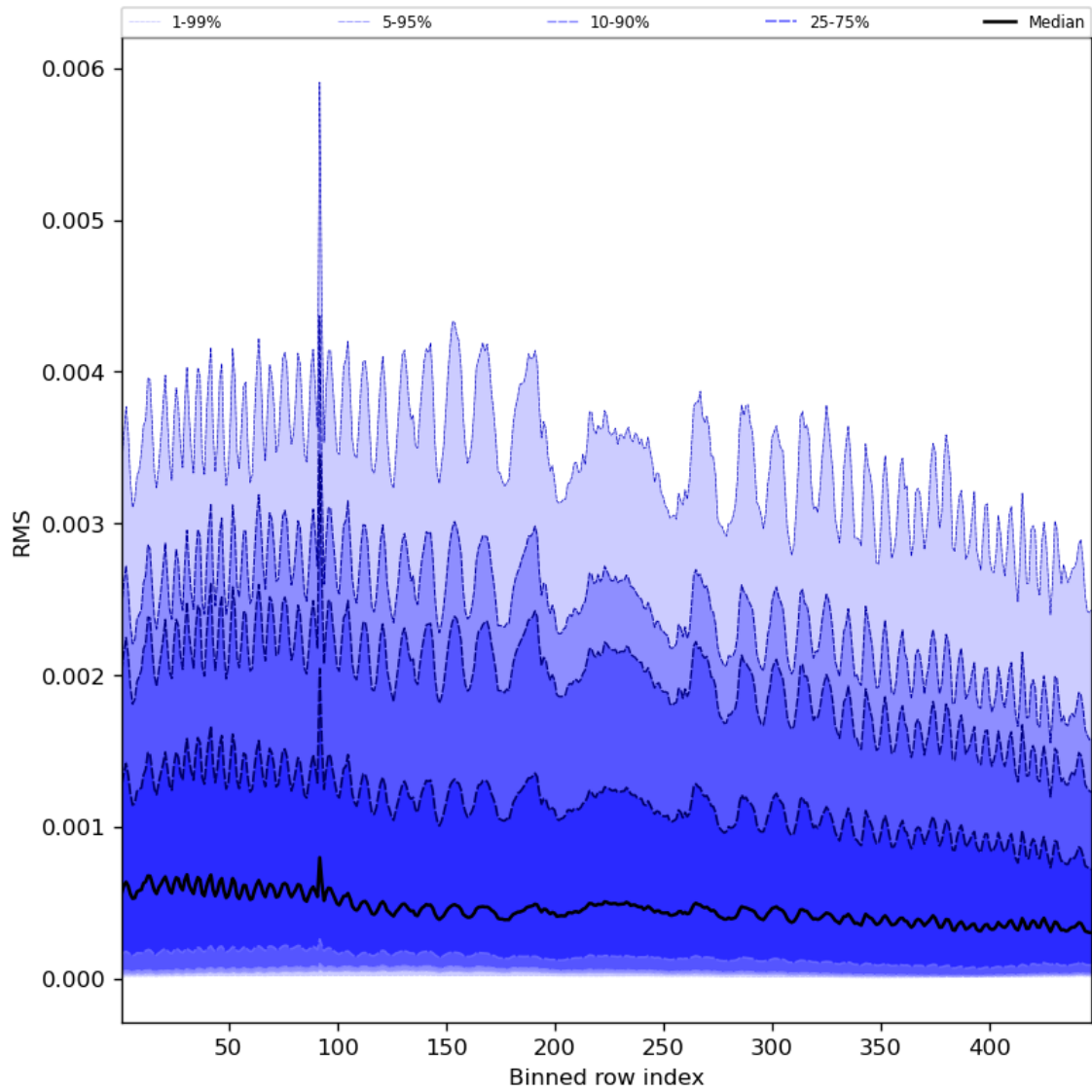
Figure 63: Along track statistics of “RMS” for 2024-01-01 to 2024-01-03
