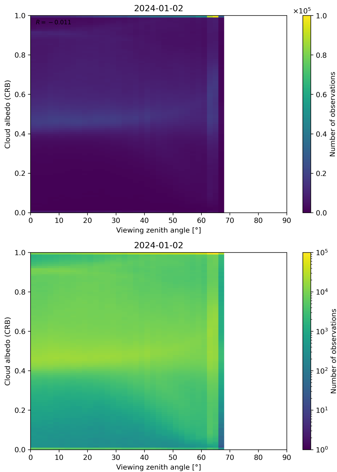
Figure 106: Scatter density plot of “Viewing zenith angle” against “Cloud albedo (CRB)” for 2024-01-01 to 2024-01-03.
