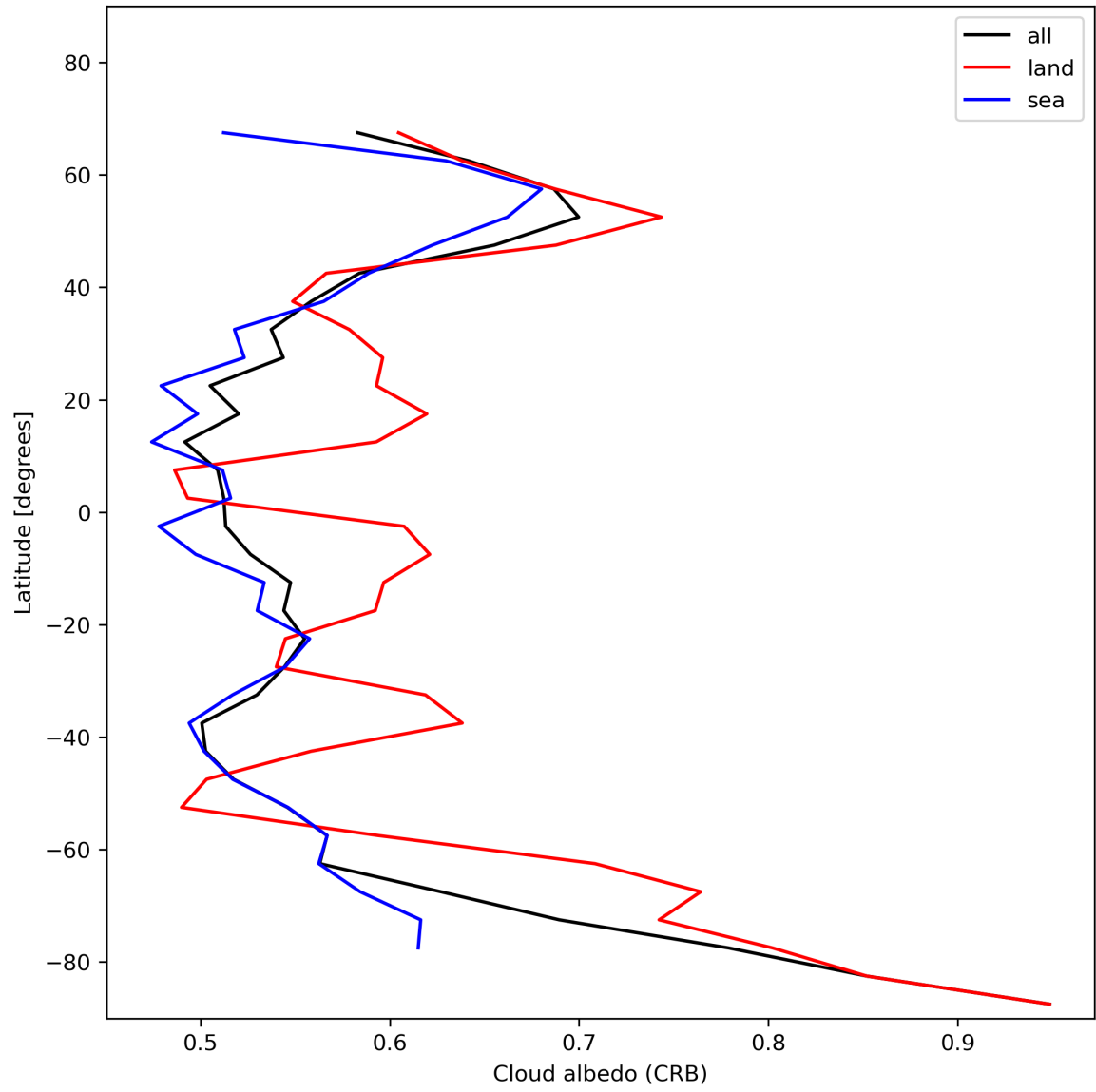
Figure 28: Zonal average of “Cloud albedo (CRB)” for 2024-01-01 to 2024-01-03.
