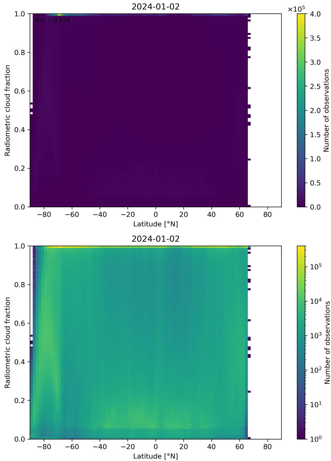
Figure 92: Scatter density plot of “Latitude” against “Radiometric cloud fraction” for 2024-01-01 to 2024-01-03.
