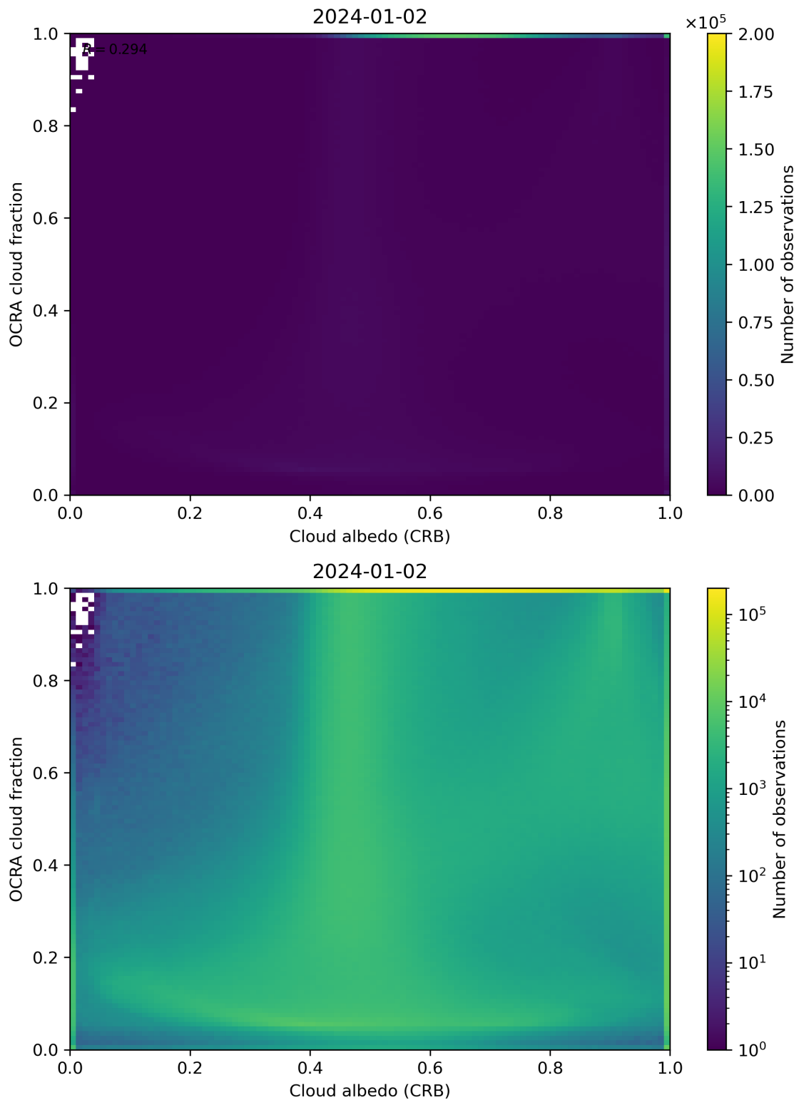
Figure 70: Scatter density plot of “Cloud albedo (CRB)” against “OCRA cloud fraction” for 2024-01-01 to 2024-01-03.
