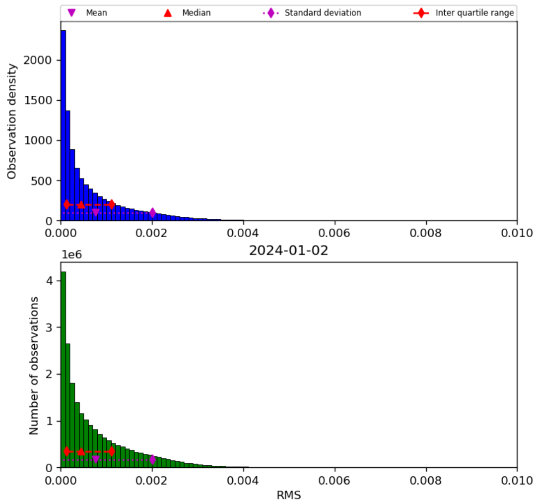
Figure 47: Histogram of “RMS” for 2024-01-01 to 2024-01-03
