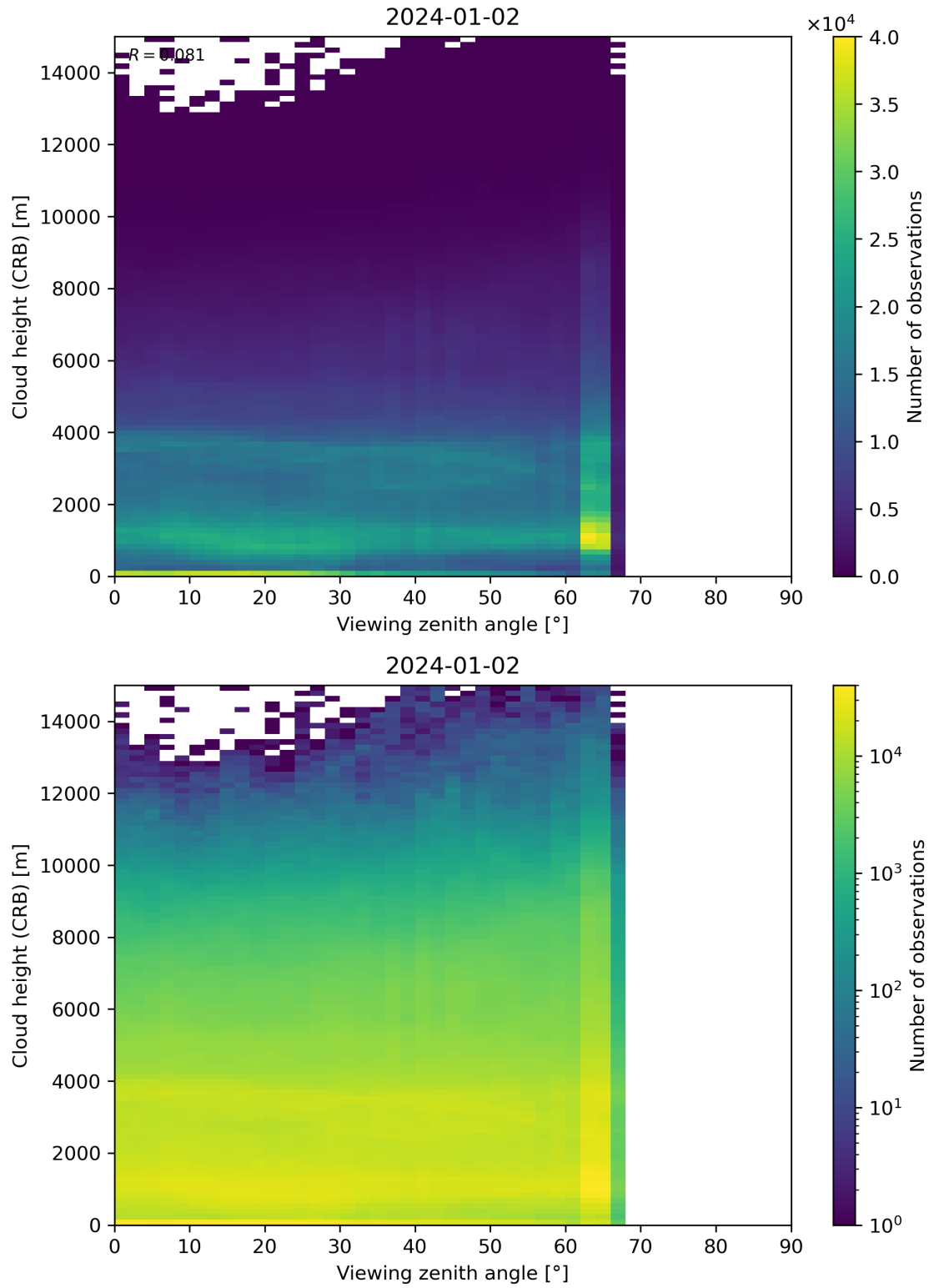
Figure 110: Scatter density plot of “Viewing zenith angle” against “Cloud height (CRB)” for 2024-01-01 to 2024-01-03.
