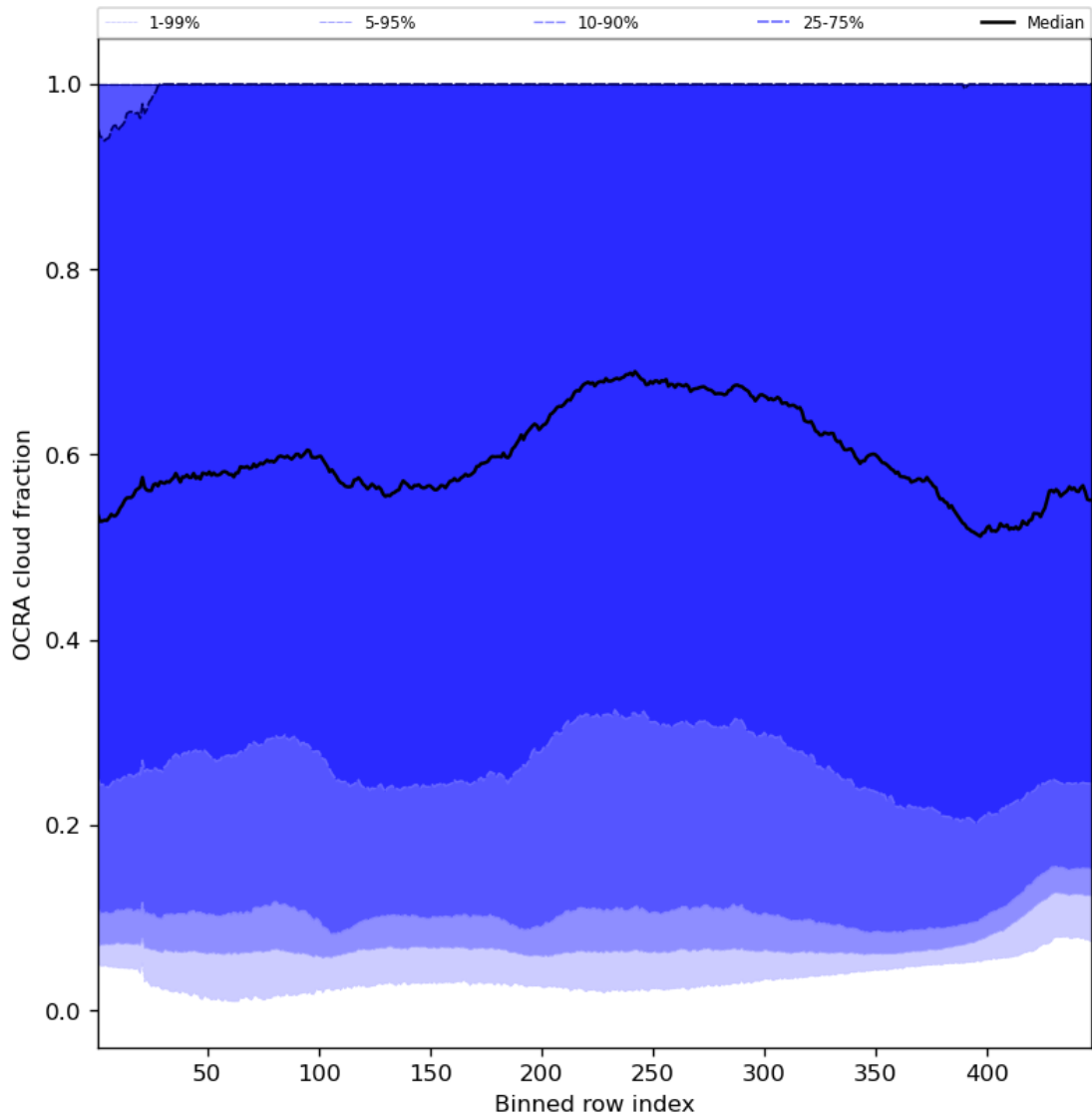
Figure 66: Along track statistics of “OCRA cloud fraction” for 2024-01-01 to 2024-01-03
