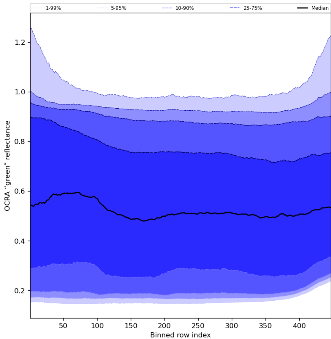
Figure 68: Along track statistics of “OCRA “green” reflectance” for 2024-01-01 to 2024-01-03
