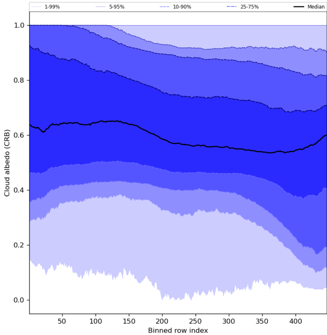
Figure 60: Along track statistics of “Cloud albedo (CRB)” for 2024-01-01 to 2024-01-03
