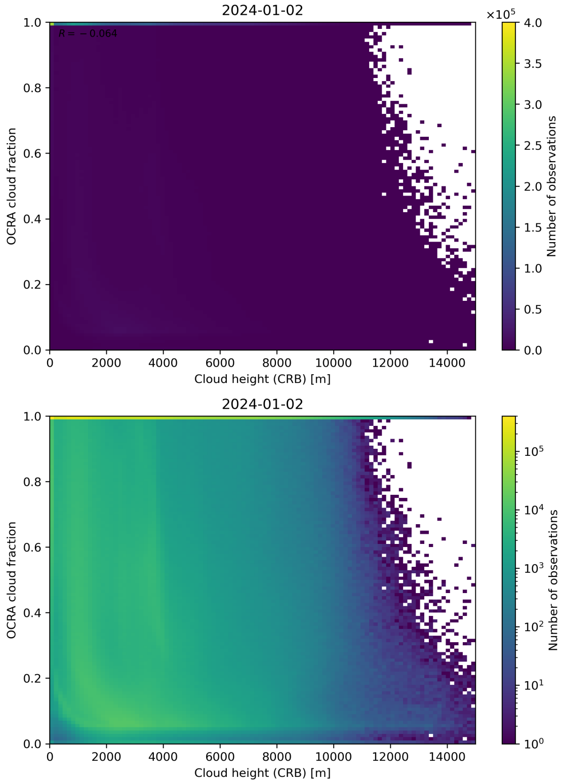
Figure 81: Scatter density plot of “Cloud height (CRB)” against “OCRA cloud fraction” for 2024-01-01 to 2024-01-03.
