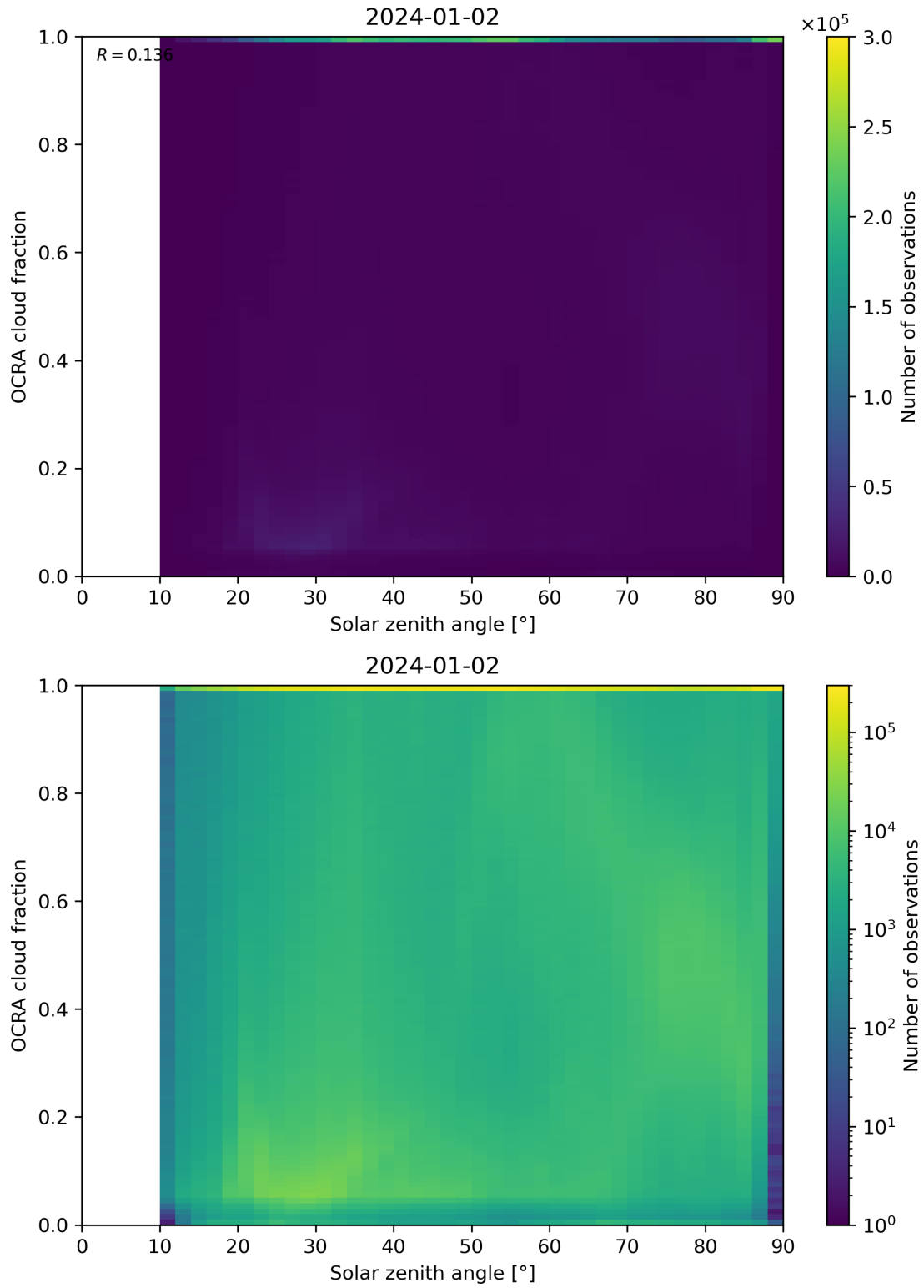
Figure 100: Scatter density plot of “Solar zenith angle” against “OCRA cloud fraction” for 2024-01-01 to 2024-01-03.
