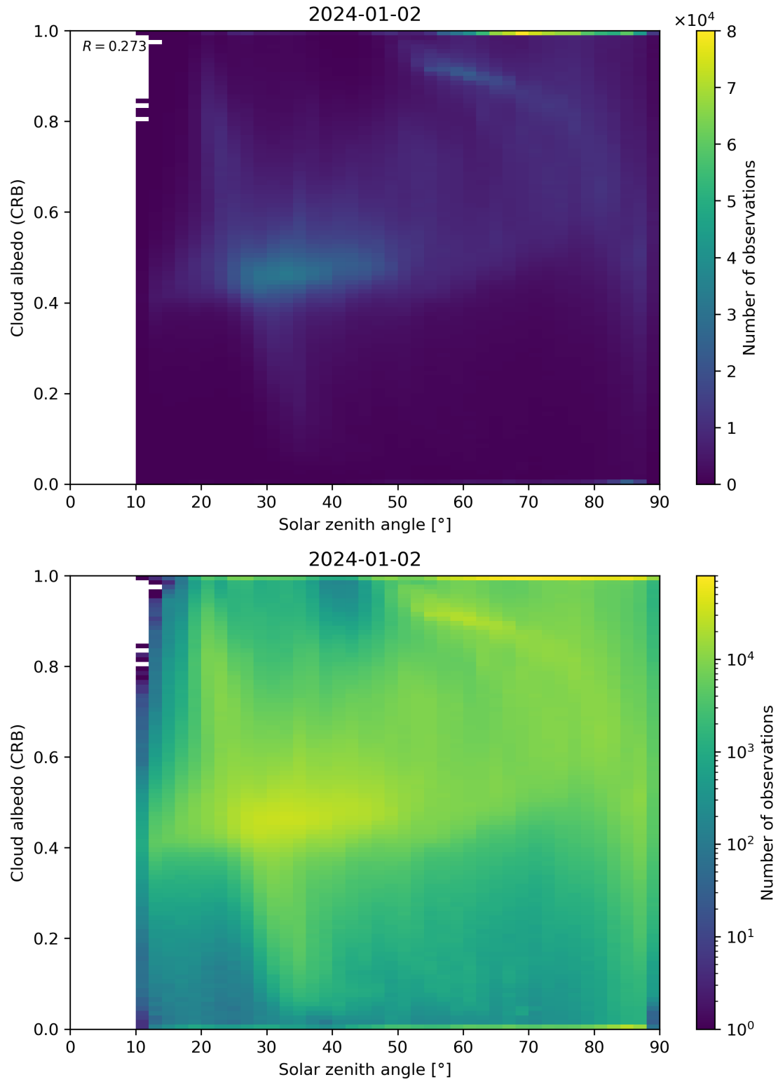
Figure 98: Scatter density plot of “Solar zenith angle” against “Cloud albedo (CRB)” for 2024-01-01 to 2024-01-03.
