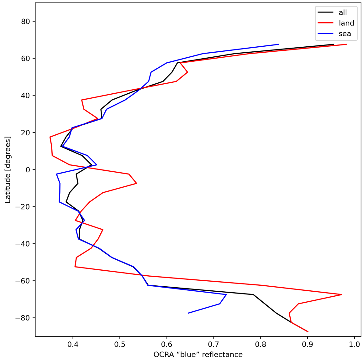
Figure 35: Zonal average of “OCRA “blue” reflectance” for 2024-01-01 to 2024-01-03.
