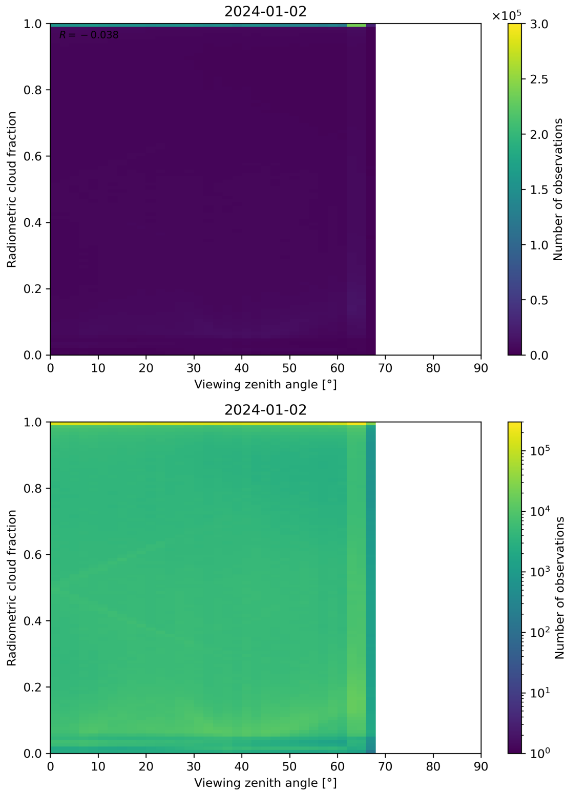
Figure 107: Scatter density plot of “Viewing zenith angle” against “Radiometric cloud fraction” for 2024-01-01 to 2024-01-03.
