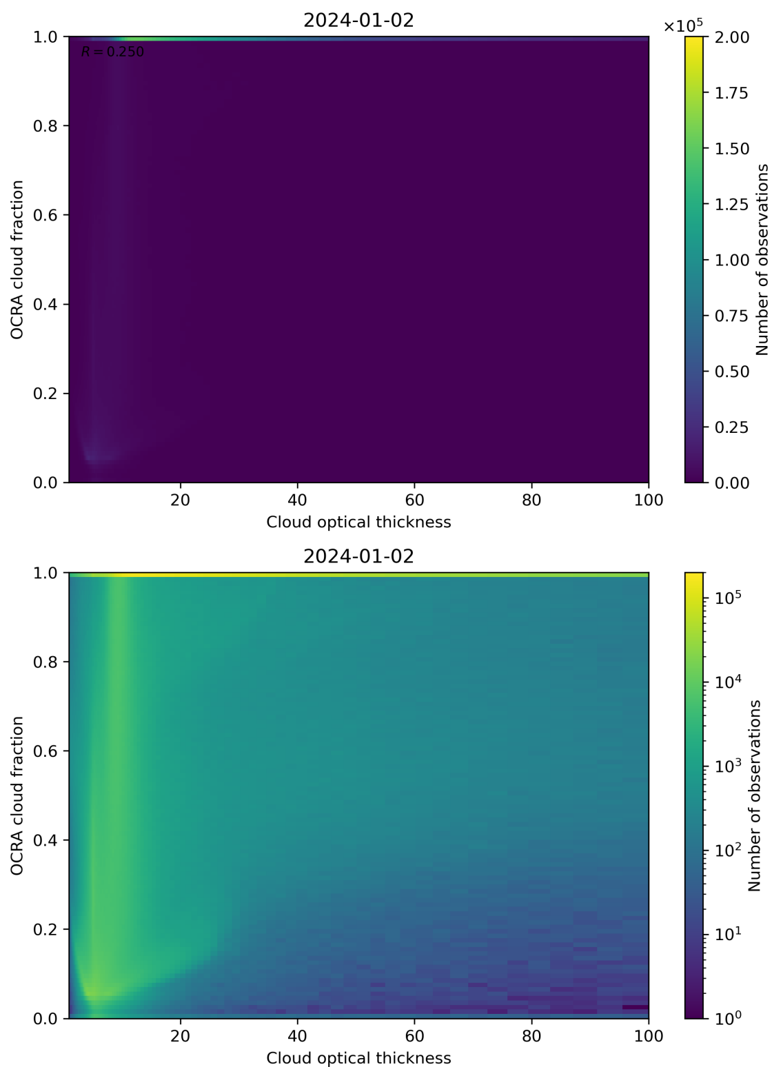
Figure 83: Scatter density plot of “Cloud optical thickness” against “OCRA cloud fraction” for 2024-01-01 to 2024-01-03.
