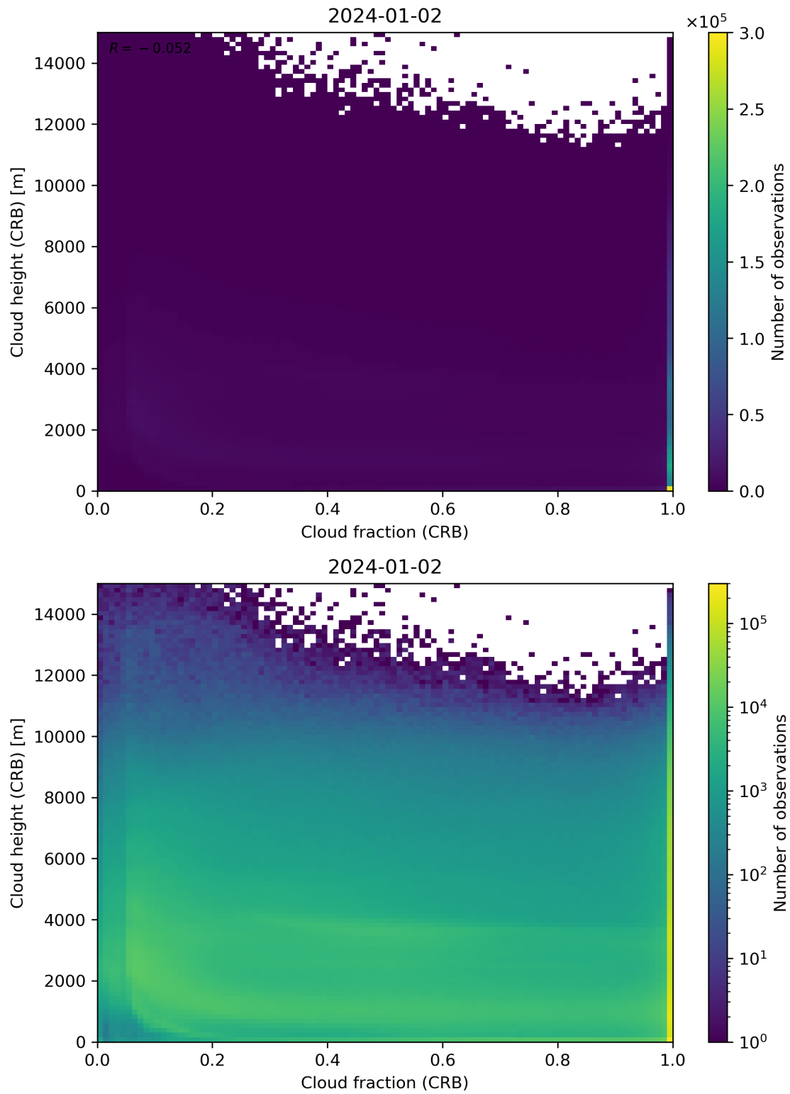
Figure 79: Scatter density plot of “Cloud fraction (CRB)” against “Cloud height (CRB)” for 2024-01-01 to 2024-01-03.
