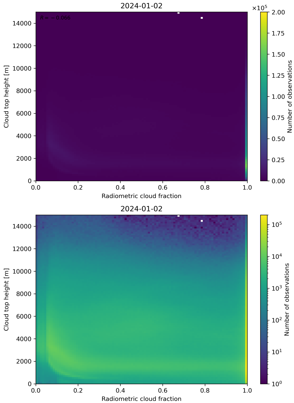
Figure 76: Scatter density plot of “Radiometric cloud fraction” against “Cloud top height” for 2024-01-01 to 2024-01-03.
