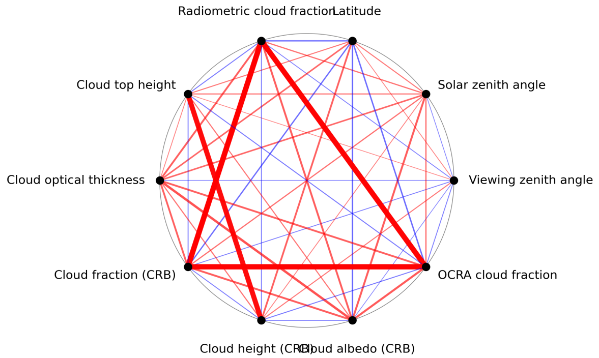
Figure 1: Map of correlation graph for 2024-01-01 to 2024-01-03.
