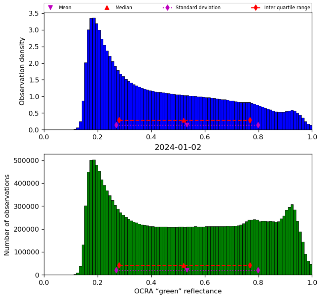
Figure 52: Histogram of “OCRA “green” reflectance” for 2024-01-01 to 2024-01-03
