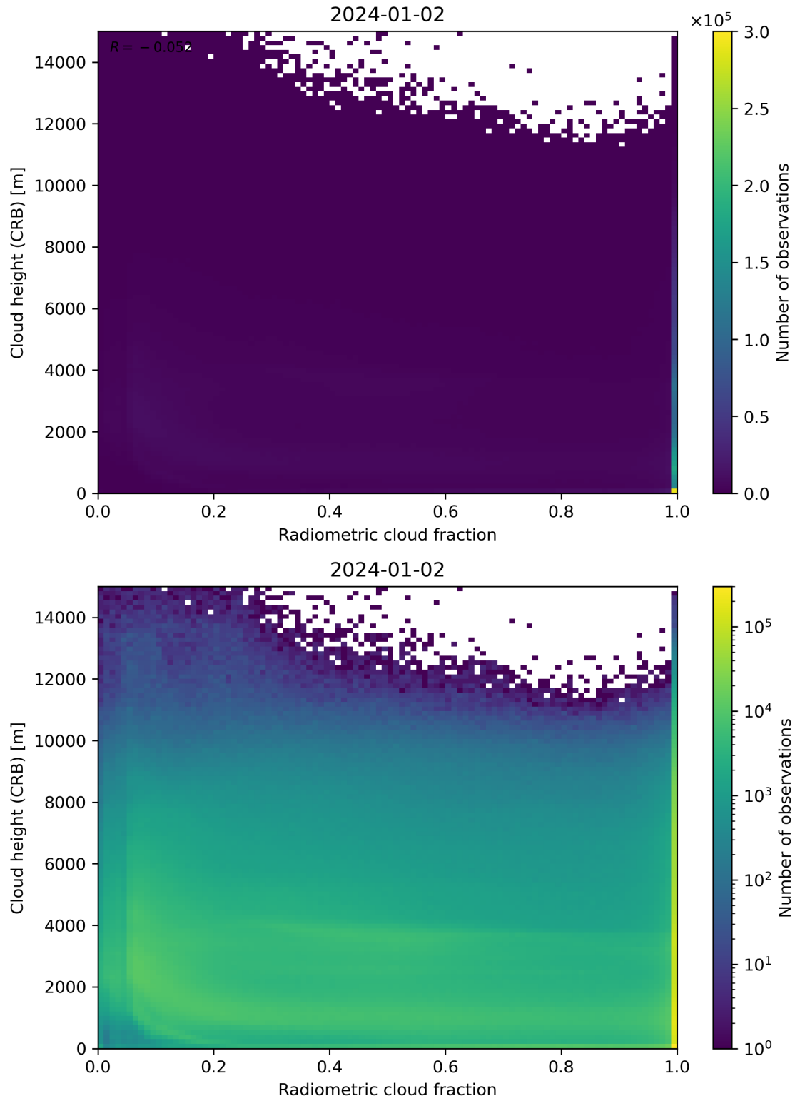
Figure 74: Scatter density plot of “Radiometric cloud fraction” against “Cloud height (CRB)” for 2024-01-01 to 2024-01-03.
