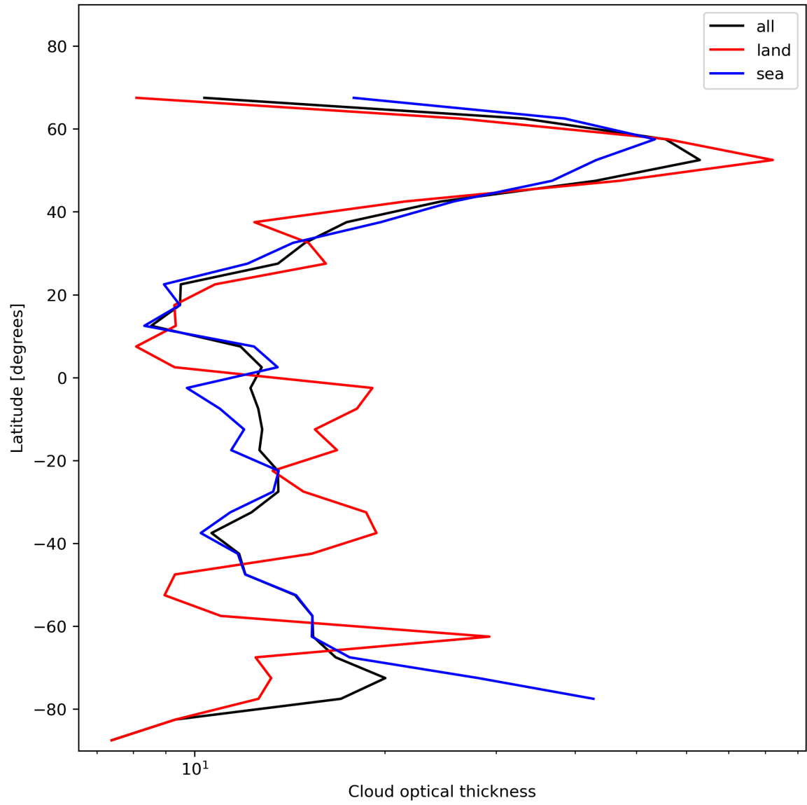
Figure 25: Zonal average of “Cloud optical thickness” for 2024-01-01 to 2024-01-03.
