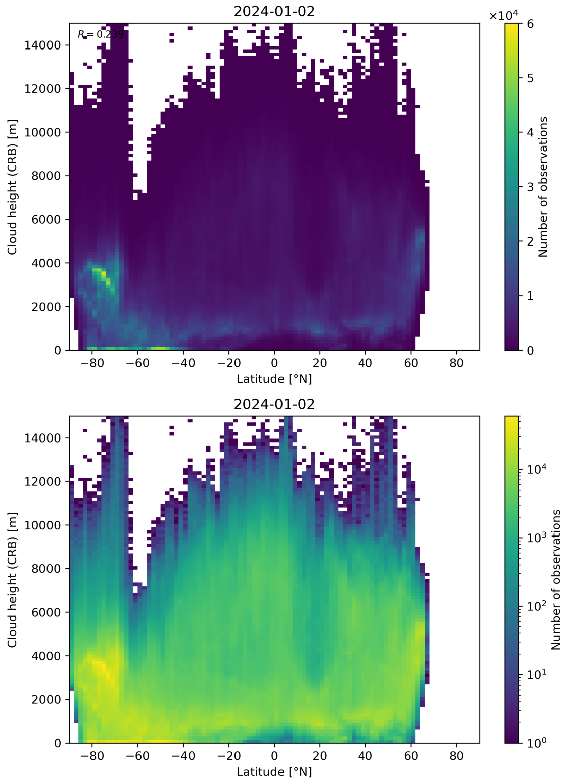
Figure 95: Scatter density plot of “Latitude” against “Cloud height (CRB)” for 2024-01-01 to 2024-01-03.
