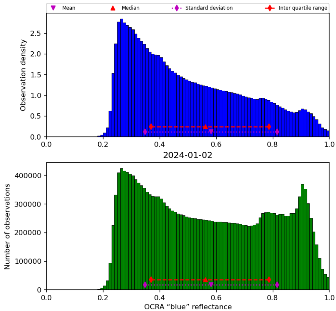
Figure 51: Histogram of “OCRA “blue” reflectance” for 2024-01-01 to 2024-01-03
