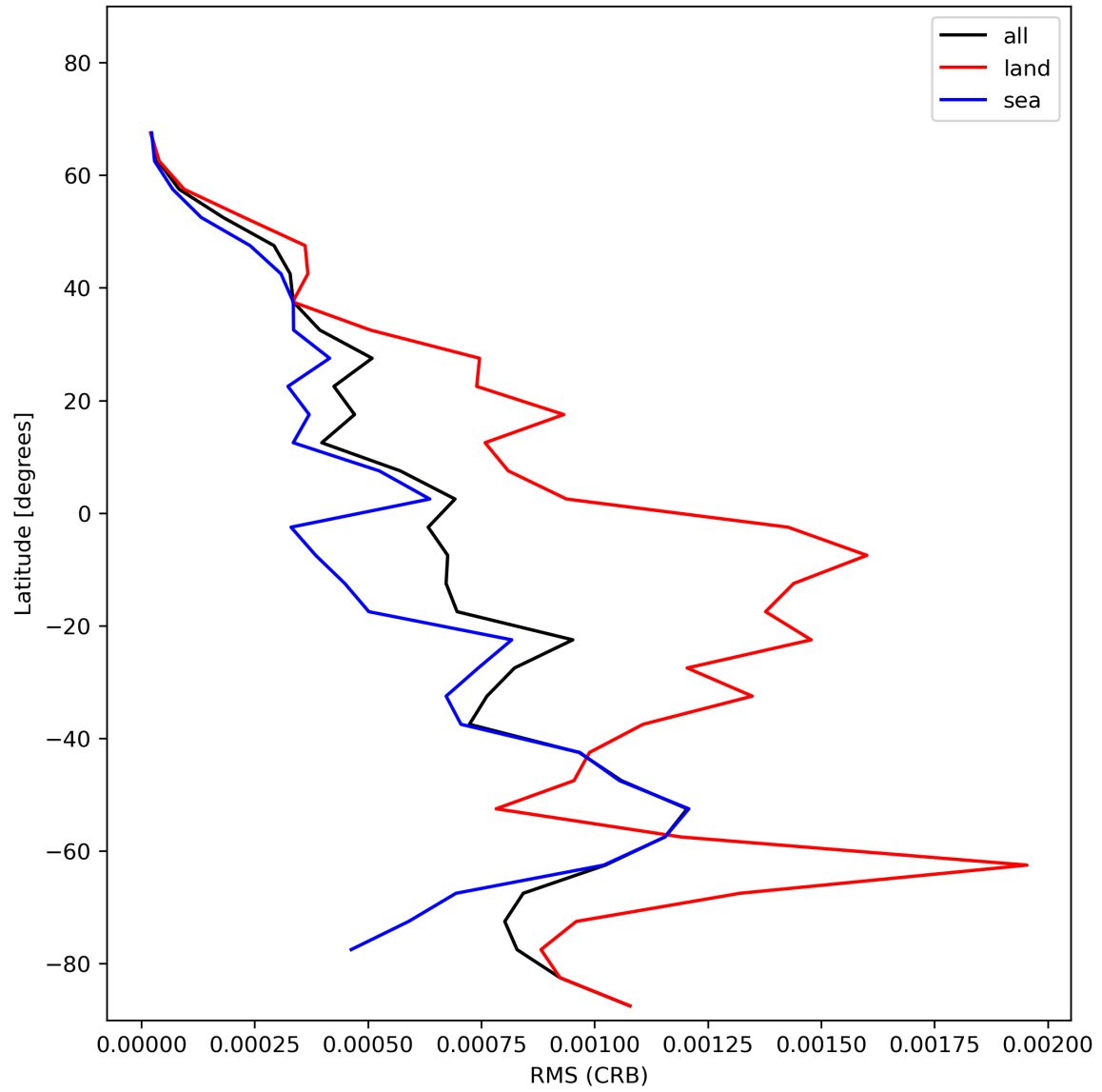
Figure 32: Zonal average of “RMS (CRB)” for 2024-01-01 to 2024-01-03.
