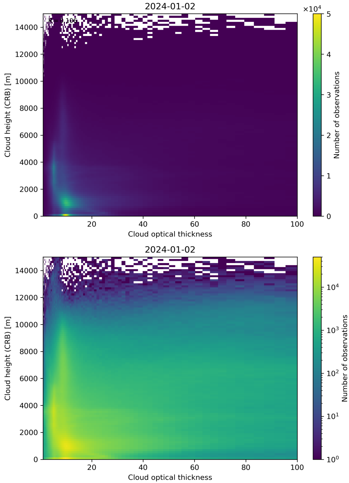
Figure 85: Scatter density plot of “Cloud optical thickness” against “Cloud height (CRB)” for 2024-01-01 to 2024-01-03.
