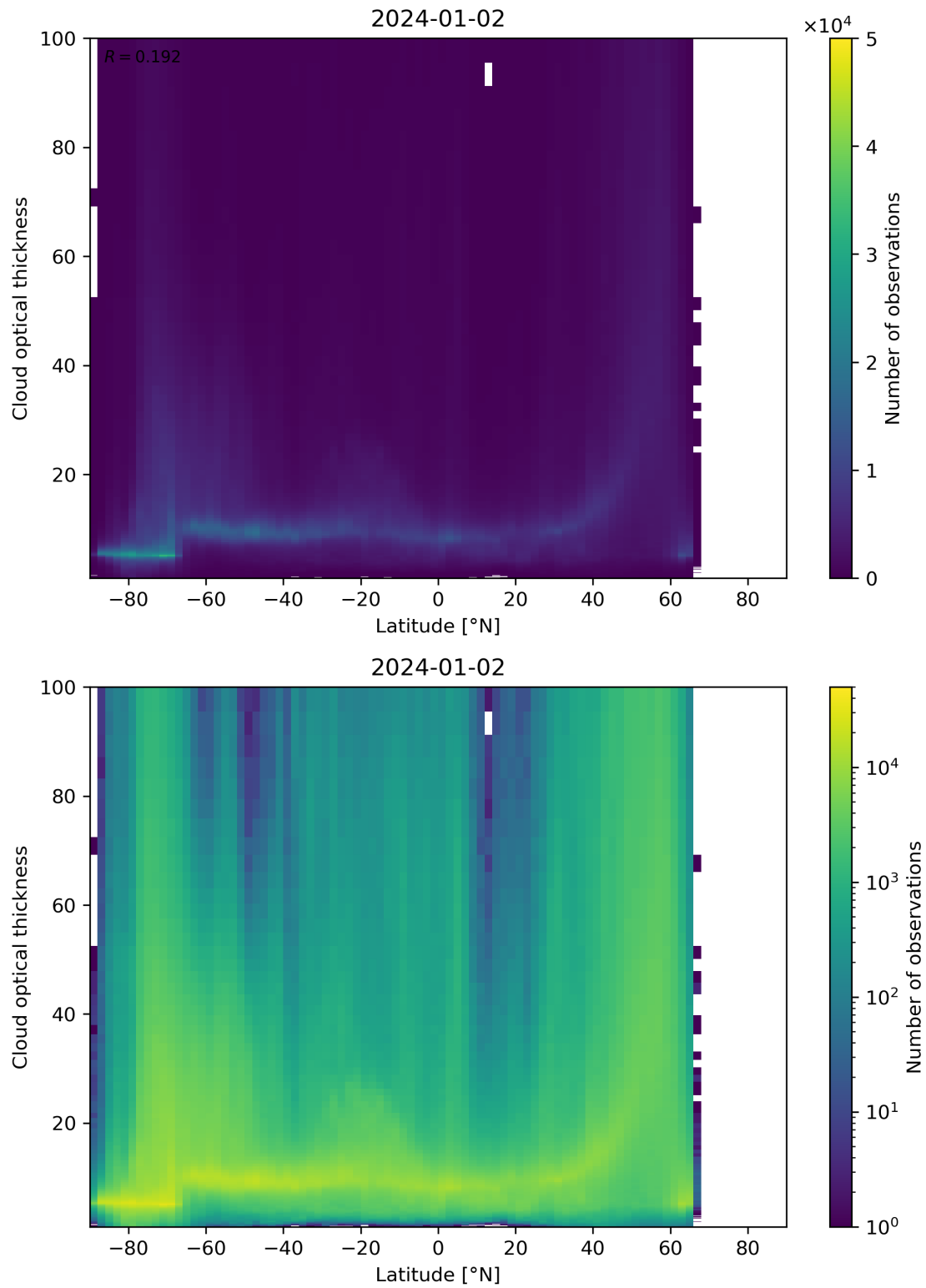
Figure 96: Scatter density plot of “Latitude” against “Cloud optical thickness” for 2024-01-01 to 2024-01-03.
