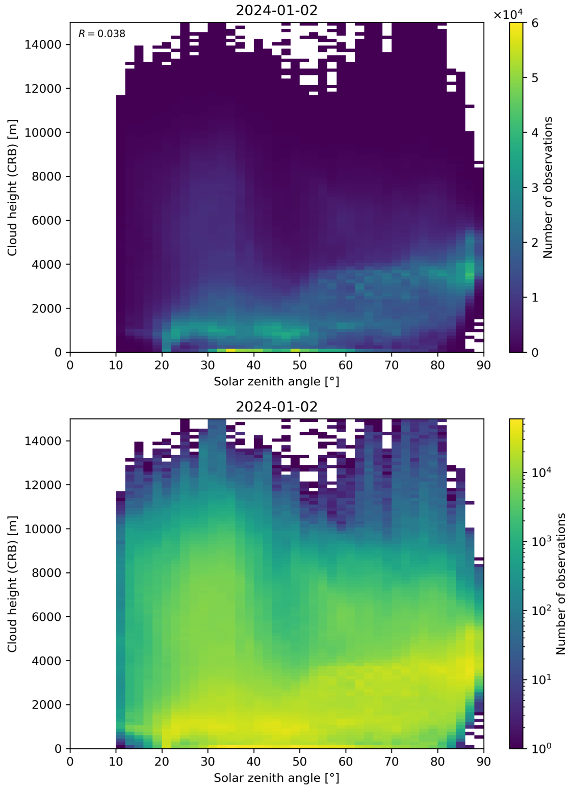
Figure 102: Scatter density plot of “Solar zenith angle” against “Cloud height (CRB)” for 2024-01-01 to 2024-01-03.
