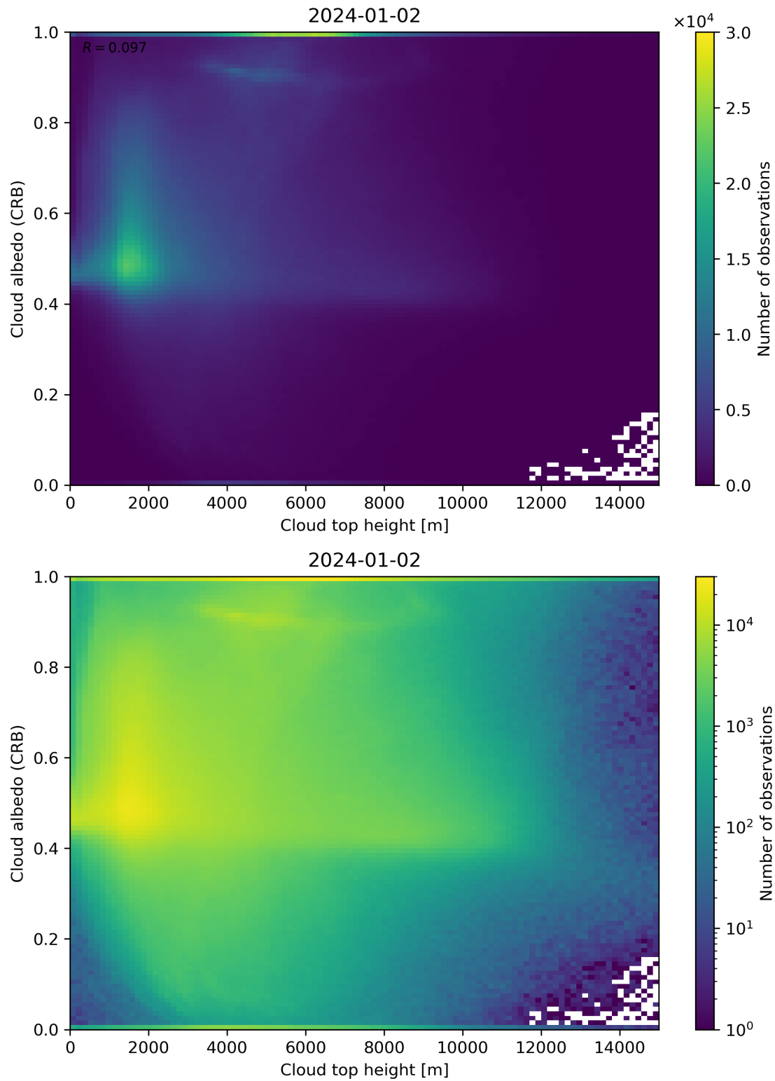
Figure 86: Scatter density plot of “Cloud top height” against “Cloud albedo (CRB)” for 2024-01-01 to 2024-01-03.
