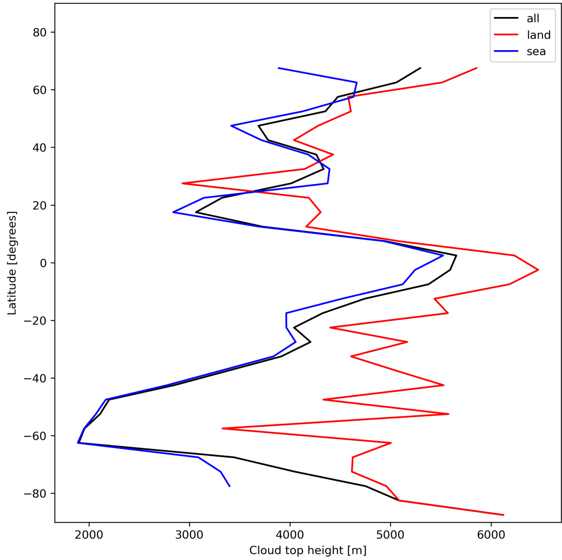
Figure 24: Zonal average of “Cloud top height” for 2024-01-01 to 2024-01-03.
