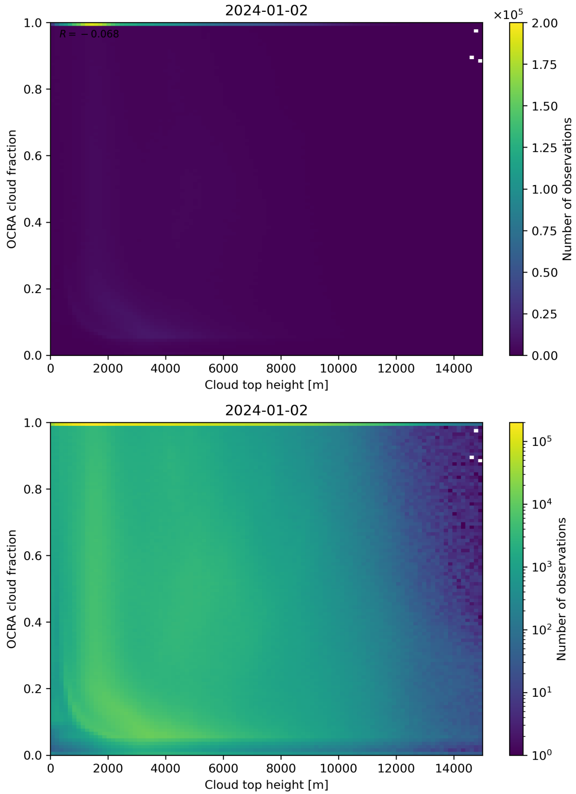
Figure 87: Scatter density plot of “Cloud top height” against “OCRA cloud fraction” for 2024-01-01 to 2024-01-03.
