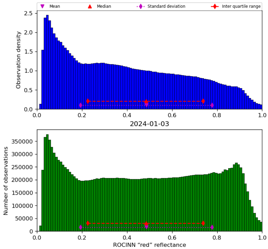
Figure 53: Histogram of “ROCINN “red” reflectance” for 2024-01-02 to 2024-01-04
