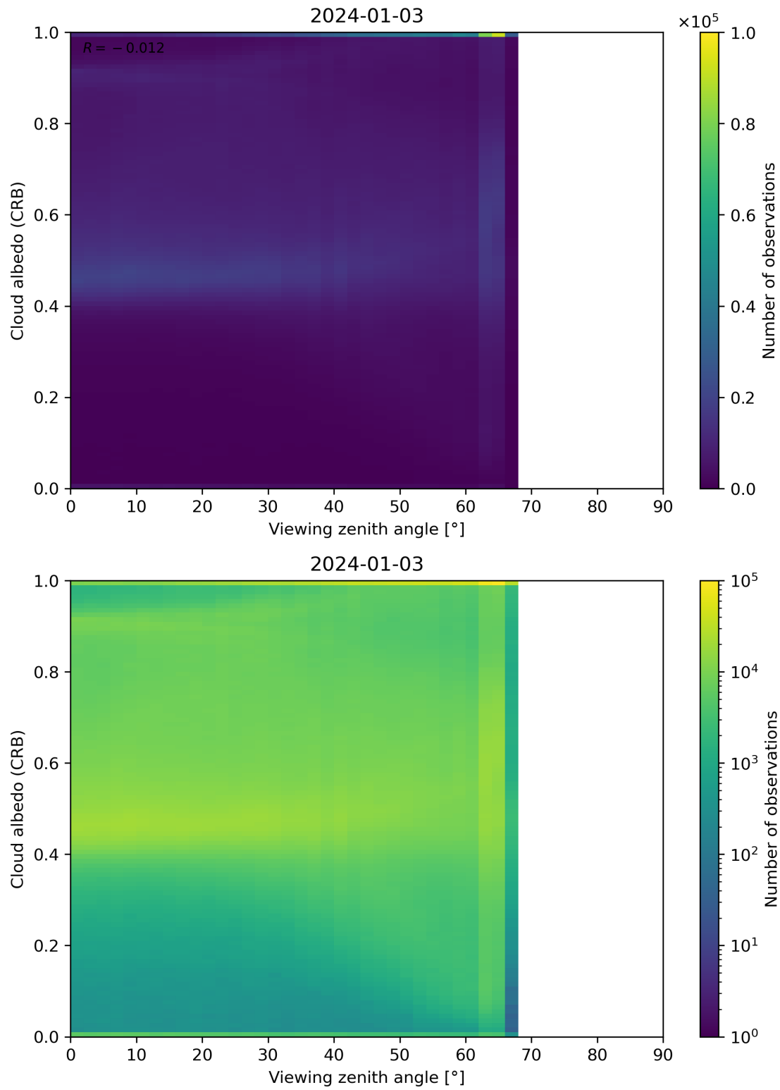
Figure 106: Scatter density plot of “Viewing zenith angle” against “Cloud albedo (CRB)” for 2024-01-02 to 2024-01-04.
