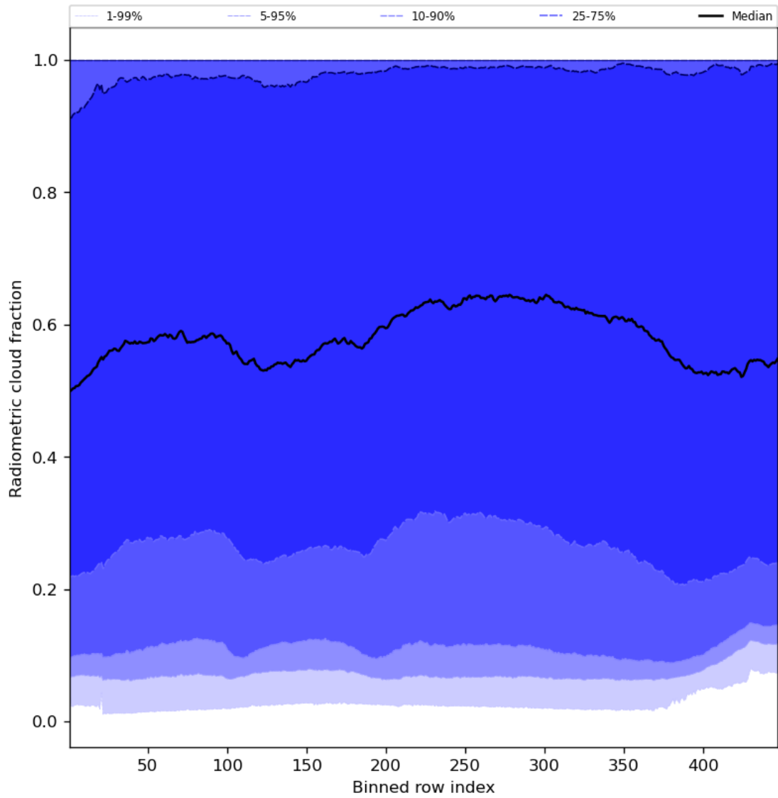
Figure 55: Along track statistics of “Radiometric cloud fraction” for 2024-01-02 to 2024-01-04
