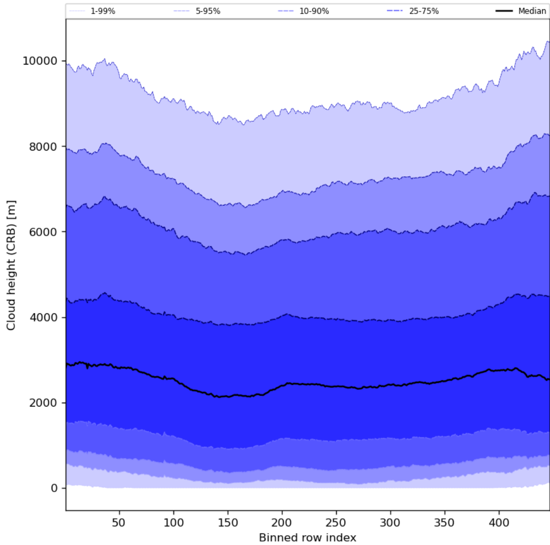
Figure 59: Along track statistics of “Cloud height (CRB)” for 2024-01-02 to 2024-01-04
