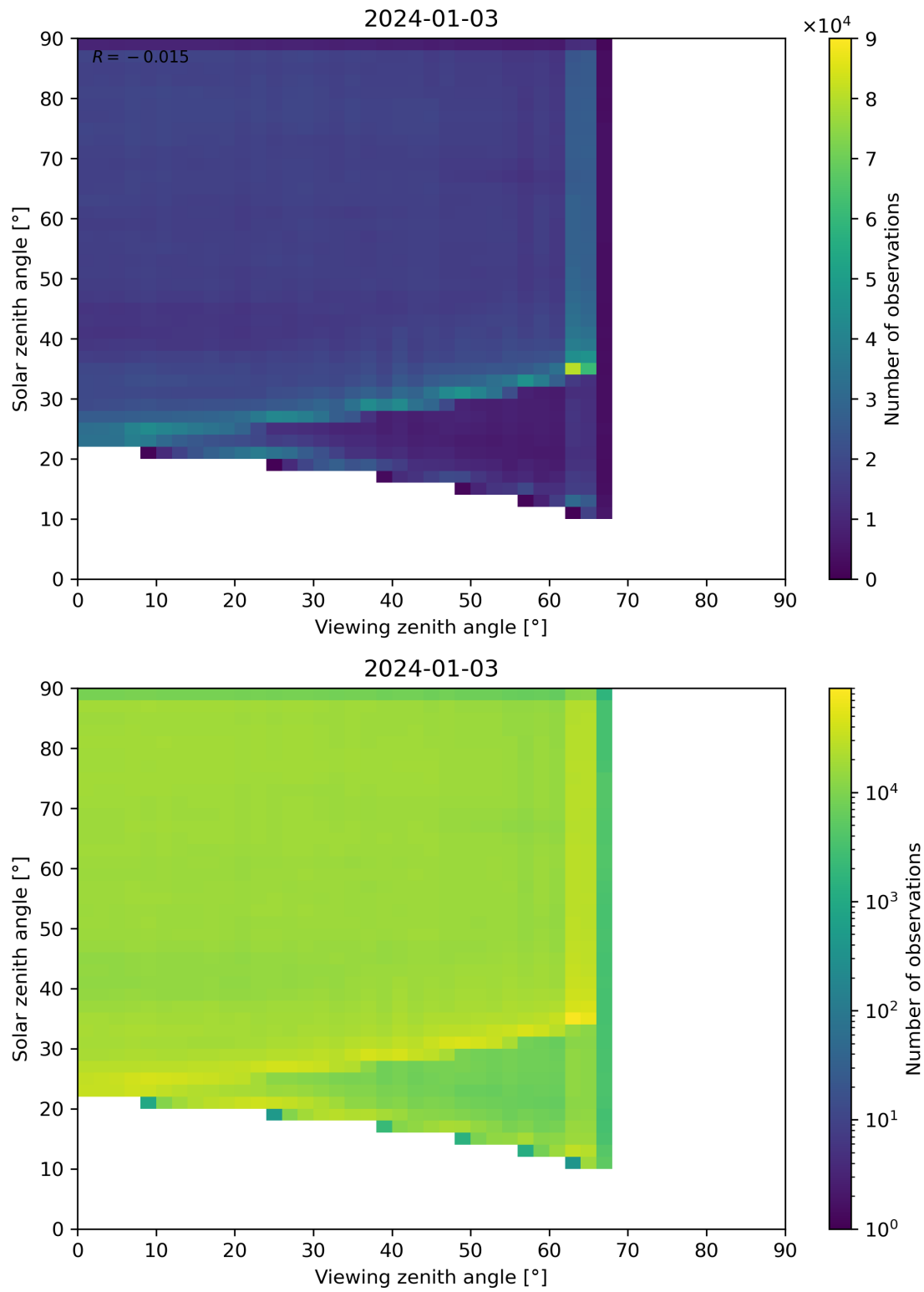
Figure 114: Scatter density plot of “Viewing zenith angle” against “Solar zenith angle” for 2024-01-02 to 2024-01-04.
