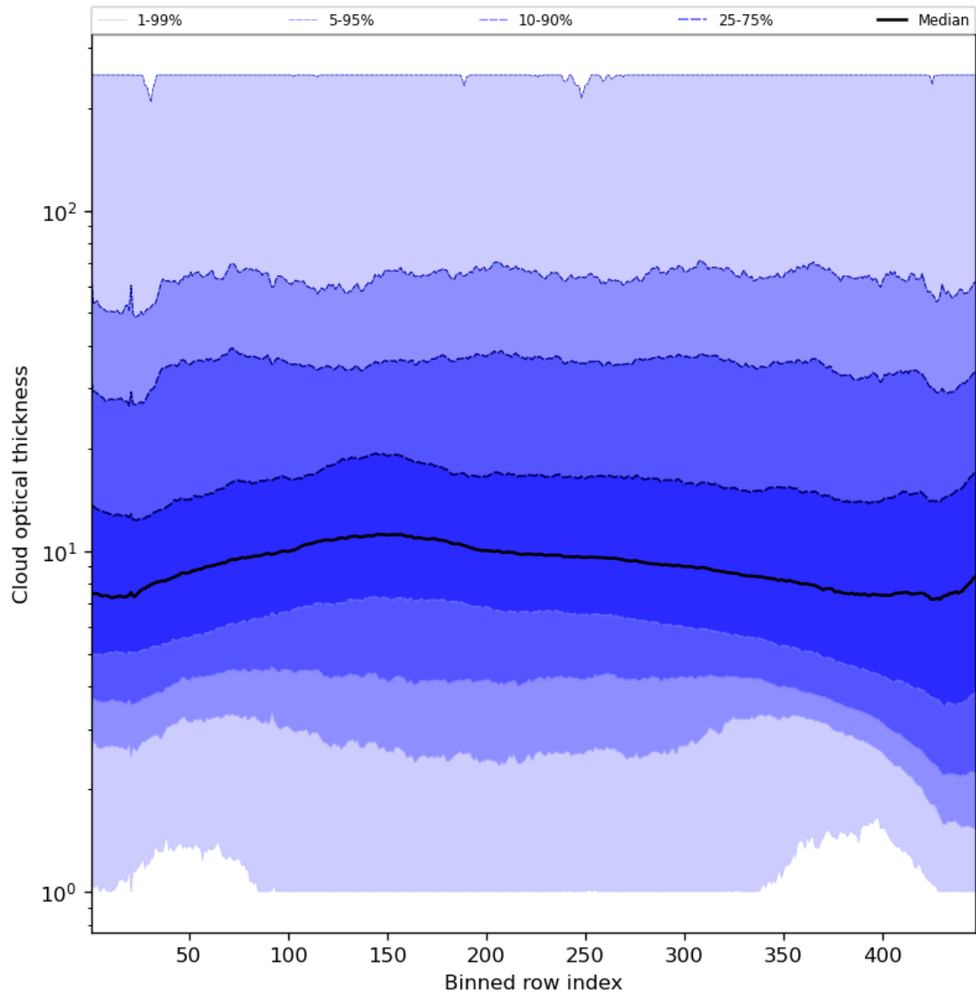
Figure 57: Along track statistics of “Cloud optical thickness” for 2024-01-02 to 2024-01-04
