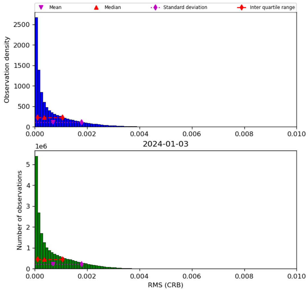
Figure 48: Histogram of “RMS (CRB)” for 2024-01-02 to 2024-01-04
