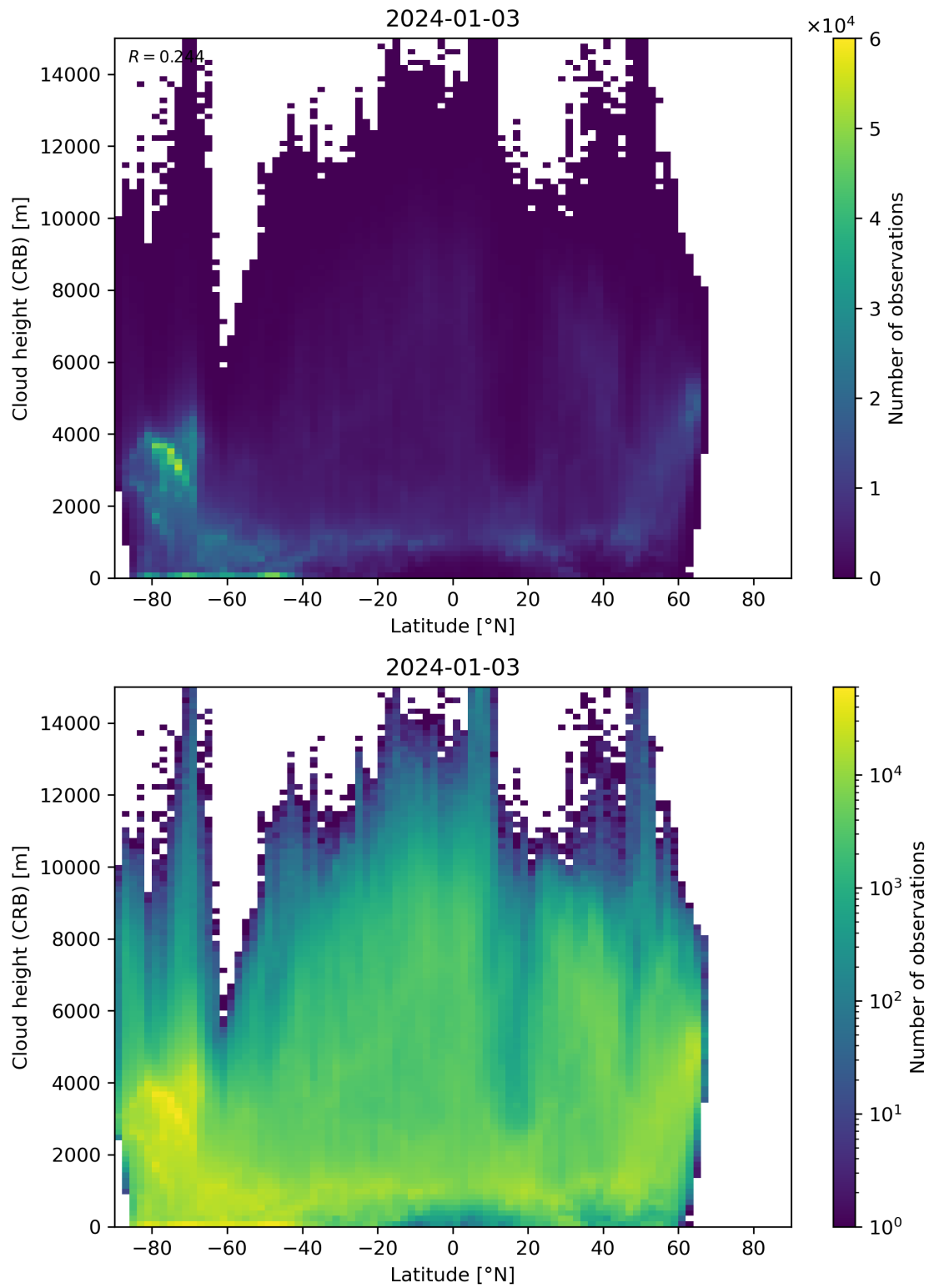
Figure 95: Scatter density plot of “Latitude” against “Cloud height (CRB)” for 2024-01-02 to 2024-01-04.
