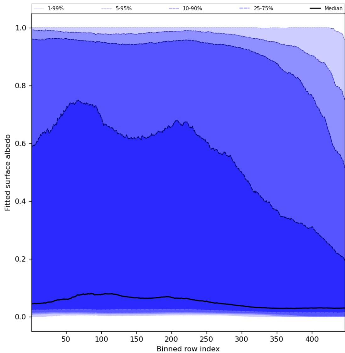
Figure 61: Along track statistics of “Fitted surface albedo” for 2024-01-02 to 2024-01-04
