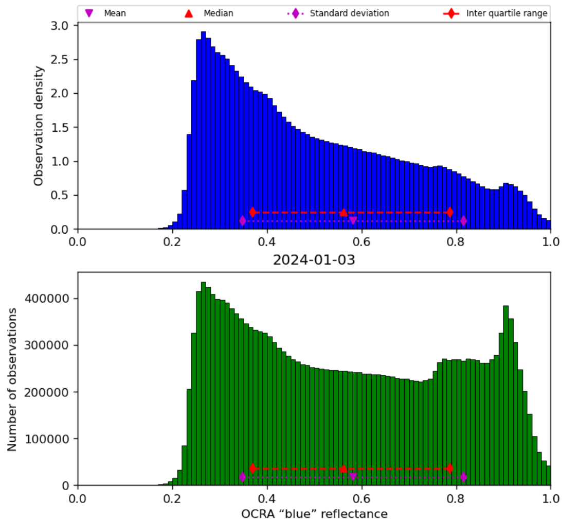
Figure 51: Histogram of “OCRA “blue” reflectance” for 2024-01-02 to 2024-01-04
