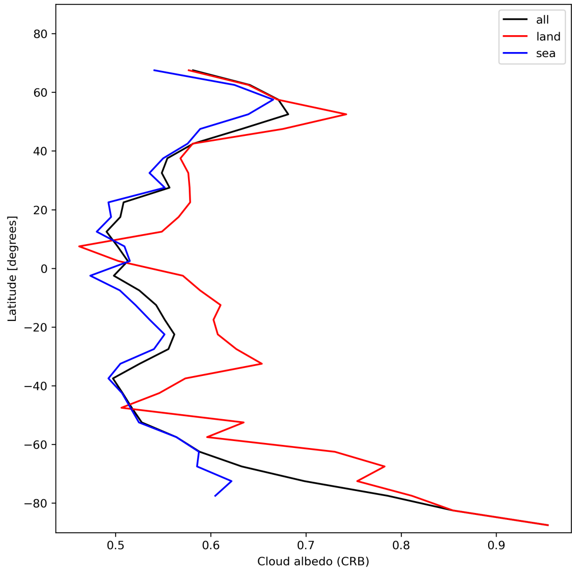
Figure 28: Zonal average of “Cloud albedo (CRB)” for 2024-01-02 to 2024-01-04.
