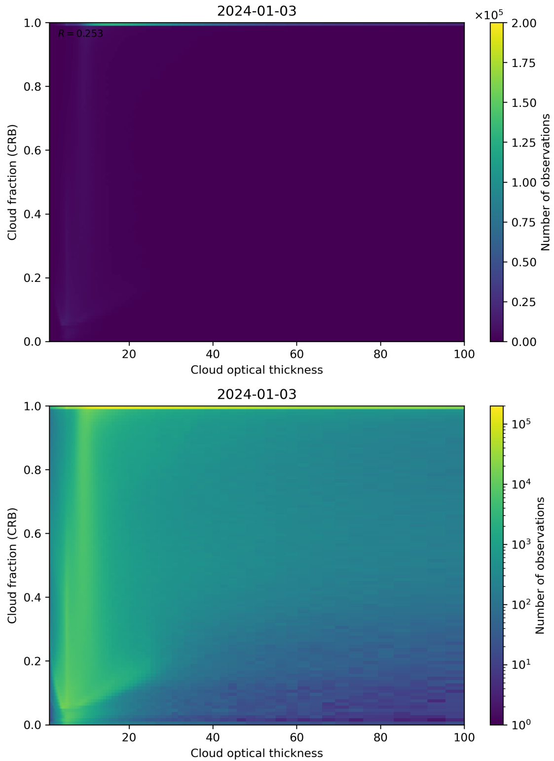
Figure 84: Scatter density plot of “Cloud optical thickness” against “Cloud fraction (CRB)” for 2024-01-02 to 2024-01-04.
