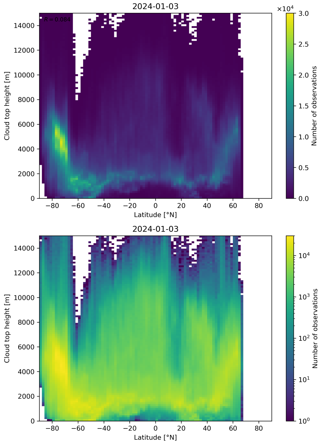
Figure 97: Scatter density plot of “Latitude” against “Cloud top height” for 2024-01-02 to 2024-01-04.
