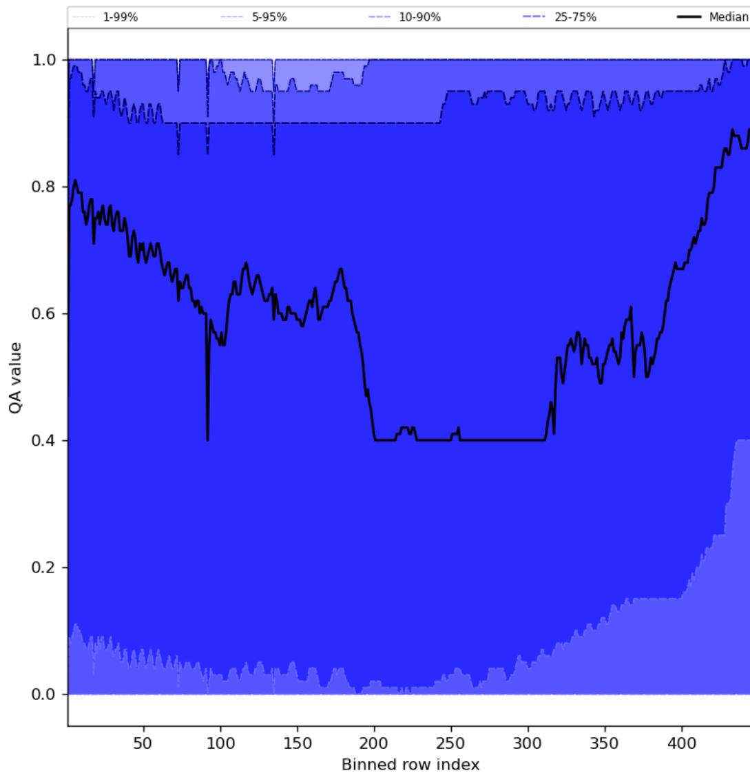
Figure 54: Along track statistics of “QA value” for 2024-01-02 to 2024-01-04
