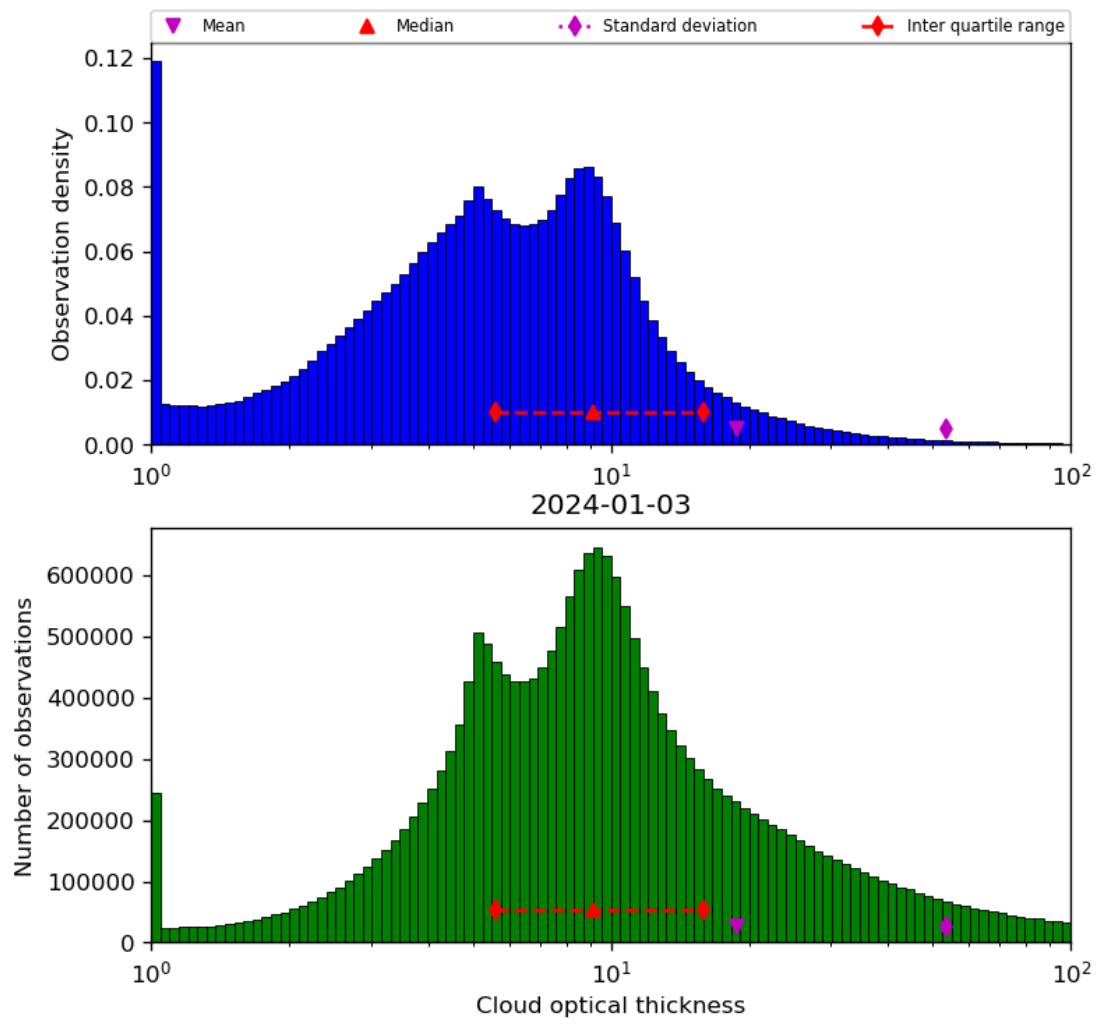
Figure 41: Histogram of “Cloud optical thickness” for 2024-01-02 to 2024-01-04
