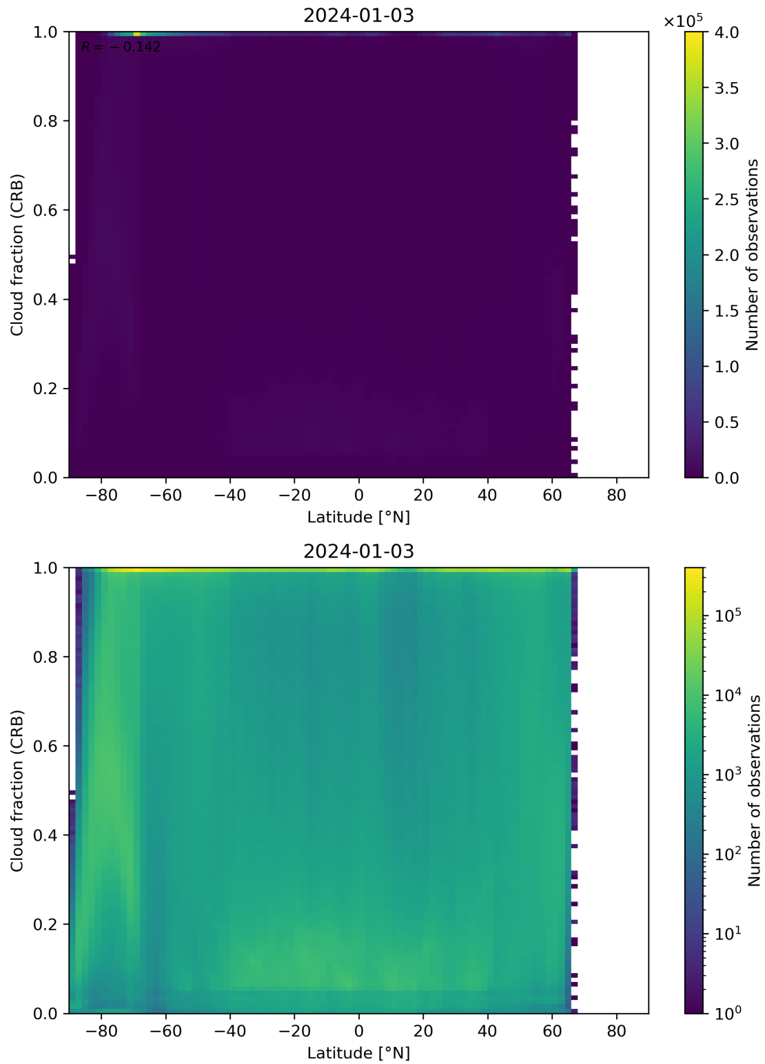
Figure 94: Scatter density plot of “Latitude” against “Cloud fraction (CRB)” for 2024-01-02 to 2024-01-04.
