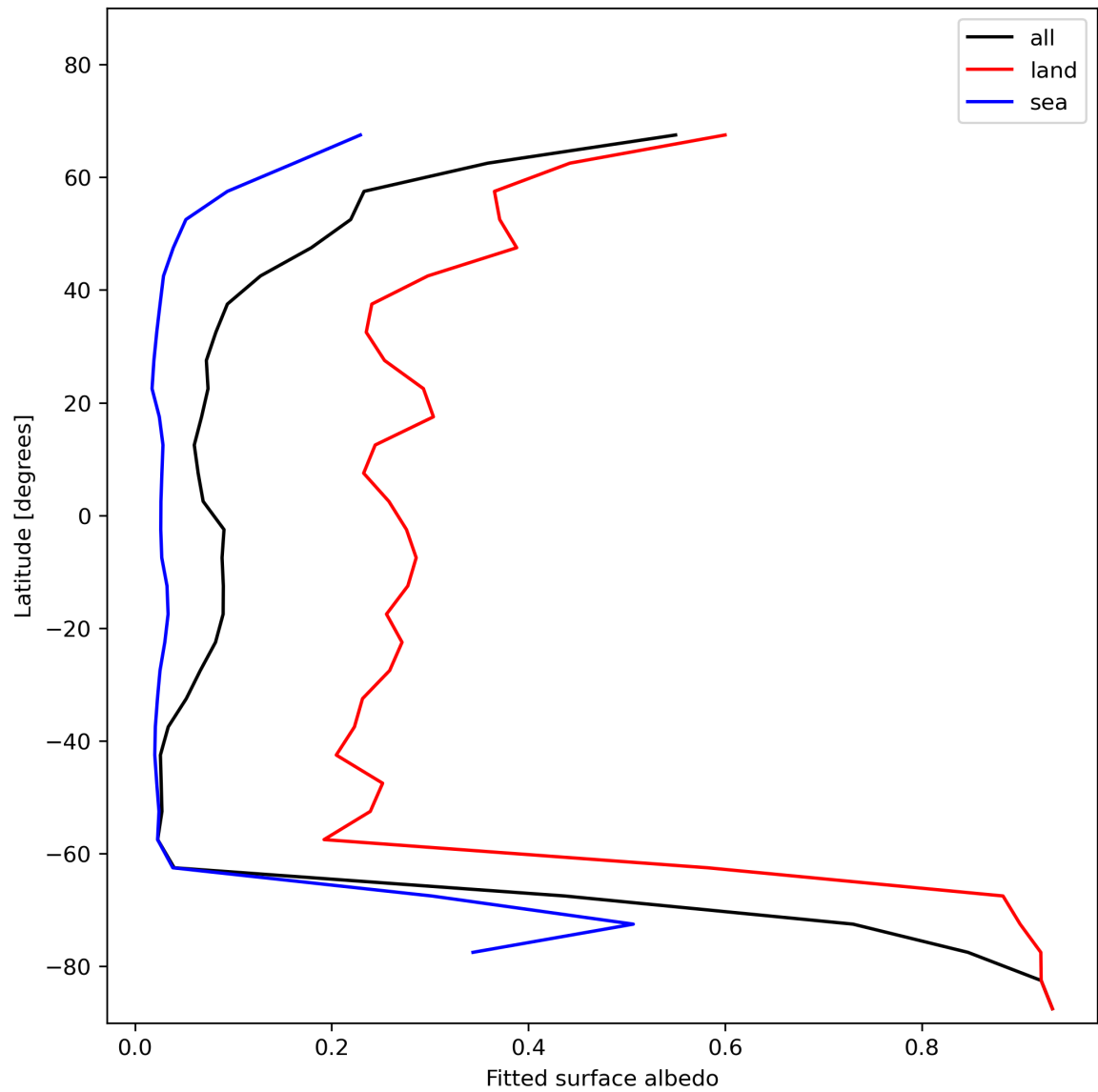
Figure 29: Zonal average of “Fitted surface albedo” for 2024-01-02 to 2024-01-04.
