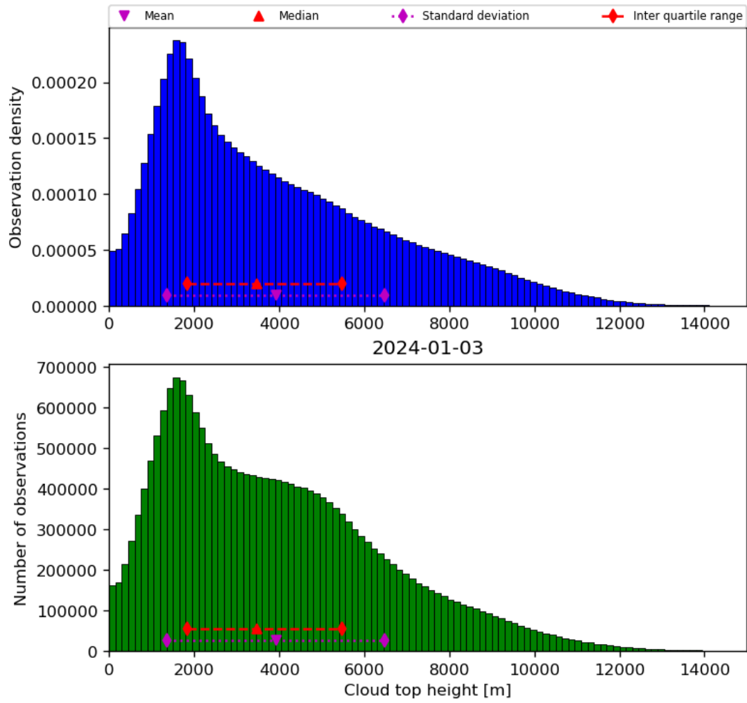
Figure 40: Histogram of “Cloud top height” for 2024-01-02 to 2024-01-04
