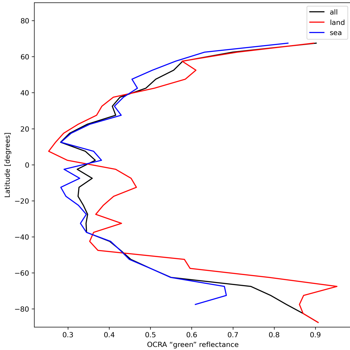
Figure 36: Zonal average of “OCRA “green” reflectance” for 2024-01-02 to 2024-01-04.
