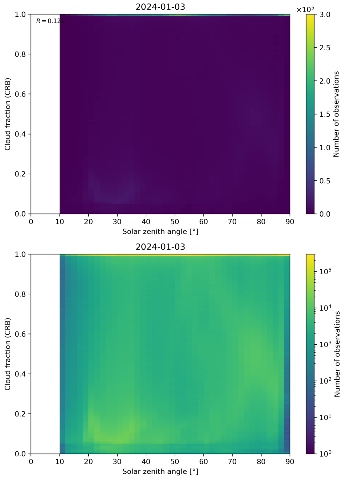
Figure 101: Scatter density plot of “Solar zenith angle” against “Cloud fraction (CRB)” for 2024-01-02 to 2024-01-04.
