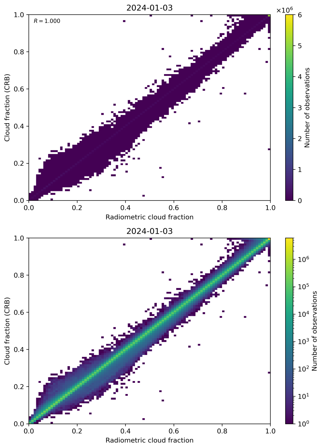
Figure 73: Scatter density plot of “Radiometric cloud fraction” against “Cloud fraction (CRB)” for 2024-01-02 to 2024-01-04.
