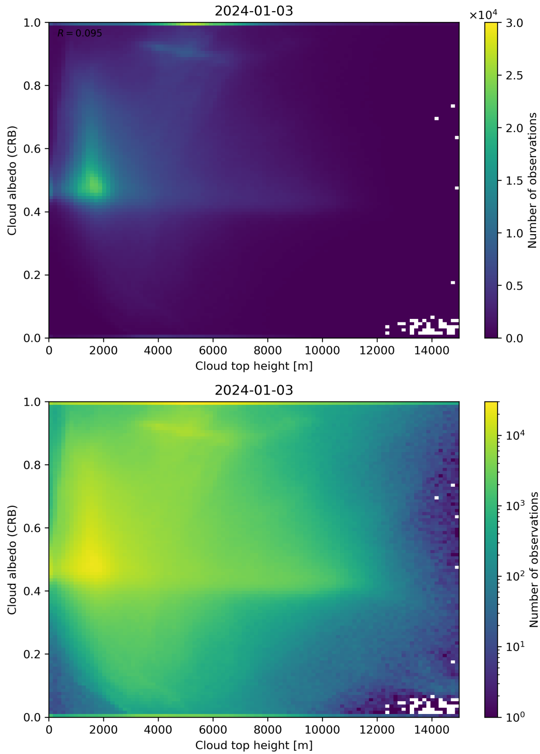
Figure 86: Scatter density plot of “Cloud top height” against “Cloud albedo (CRB)” for 2024-01-02 to 2024-01-04.
