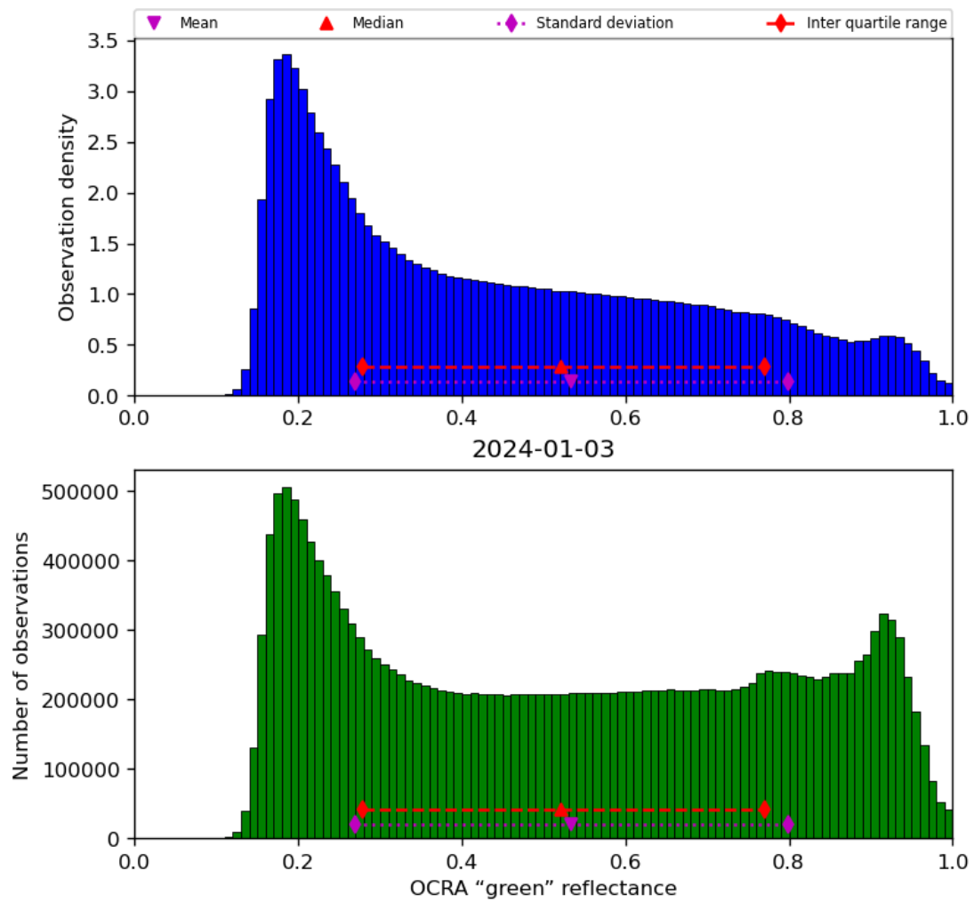
Figure 52: Histogram of “OCRA “green” reflectance” for 2024-01-02 to 2024-01-04
