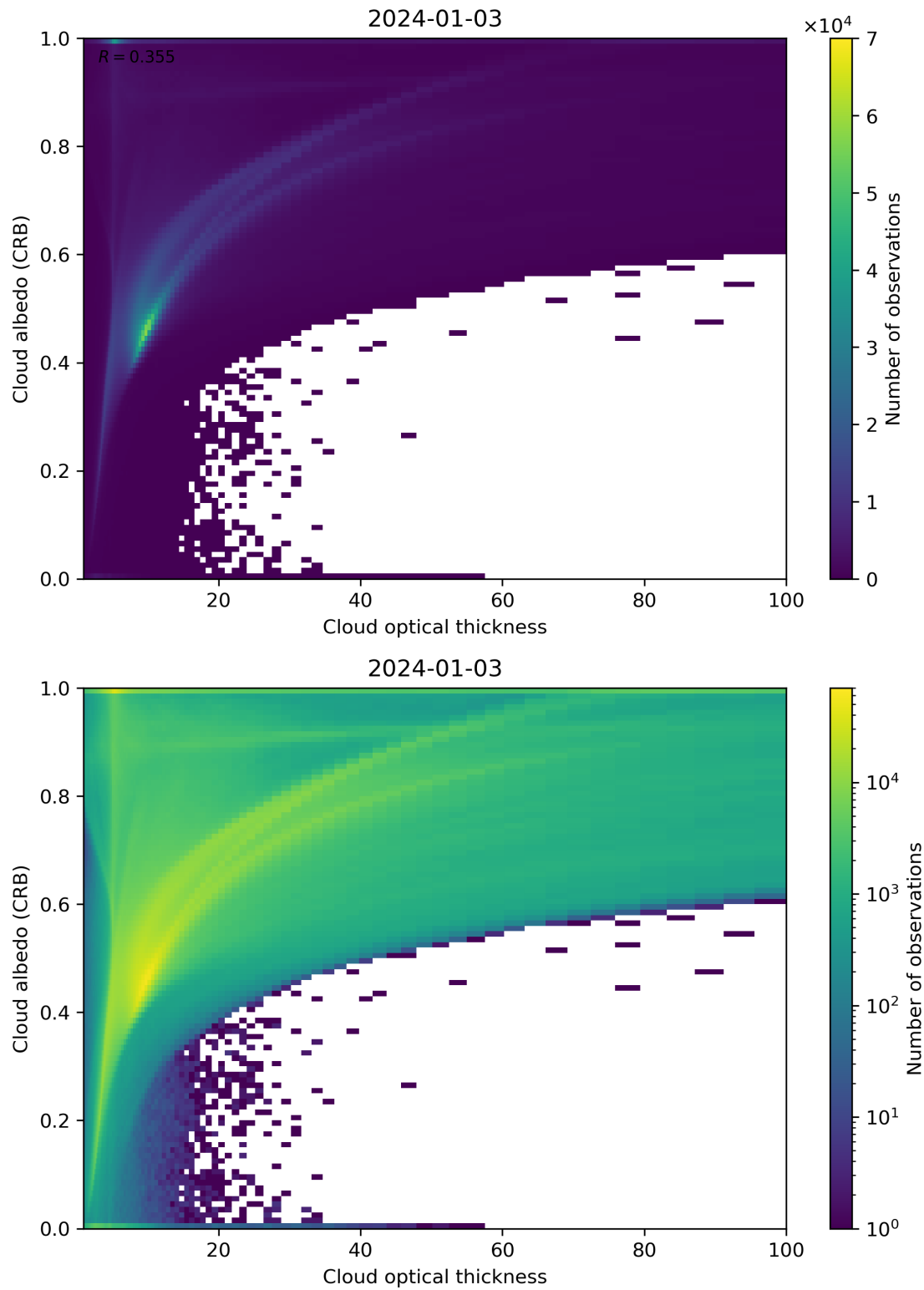
Figure 82: Scatter density plot of “Cloud optical thickness” against “Cloud albedo (CRB)” for 2024-01-02 to 2024-01-04.
