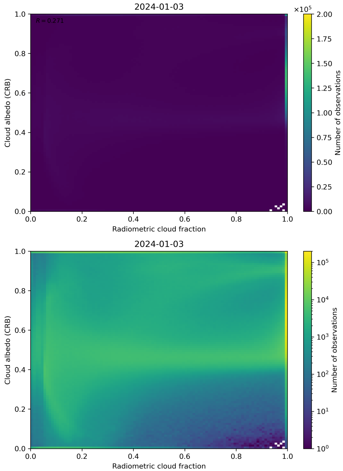
Figure 71: Scatter density plot of “Radiometric cloud fraction” against “Cloud albedo (CRB)” for 2024-01-02 to 2024-01-04.
