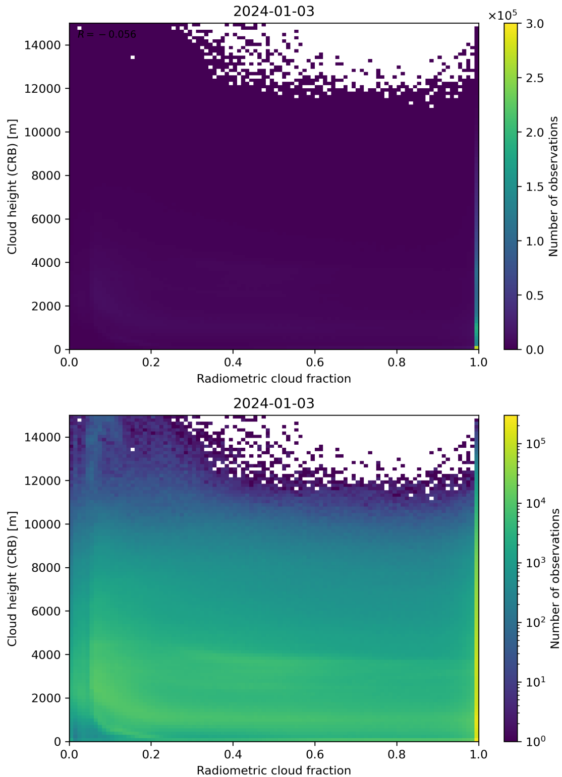
Figure 74: Scatter density plot of “Radiometric cloud fraction” against “Cloud height (CRB)” for 2024-01-02 to 2024-01-04.
