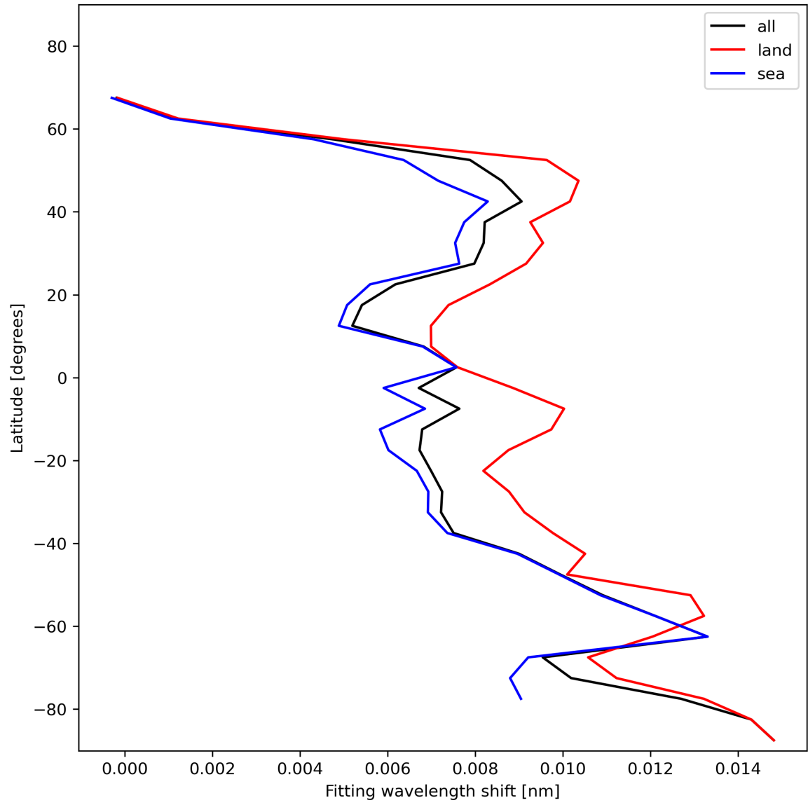
Figure 33: Zonal average of “Fitting wavelength shift” for 2024-01-02 to 2024-01-04.
