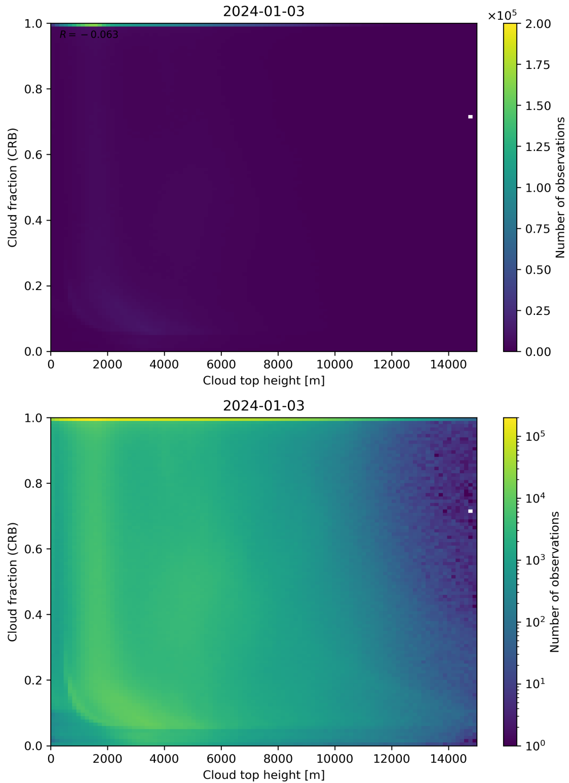
Figure 88: Scatter density plot of “Cloud top height” against “Cloud fraction (CRB)” for 2024-01-02 to 2024-01-04.
