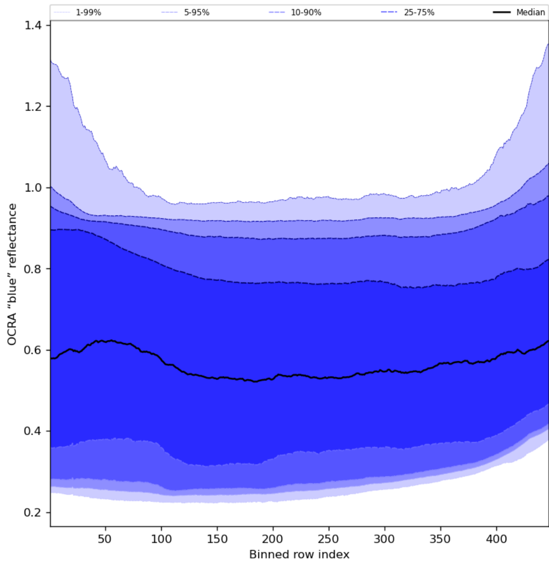
Figure 67: Along track statistics of “OCRA “blue” reflectance” for 2024-01-02 to 2024-01-04
