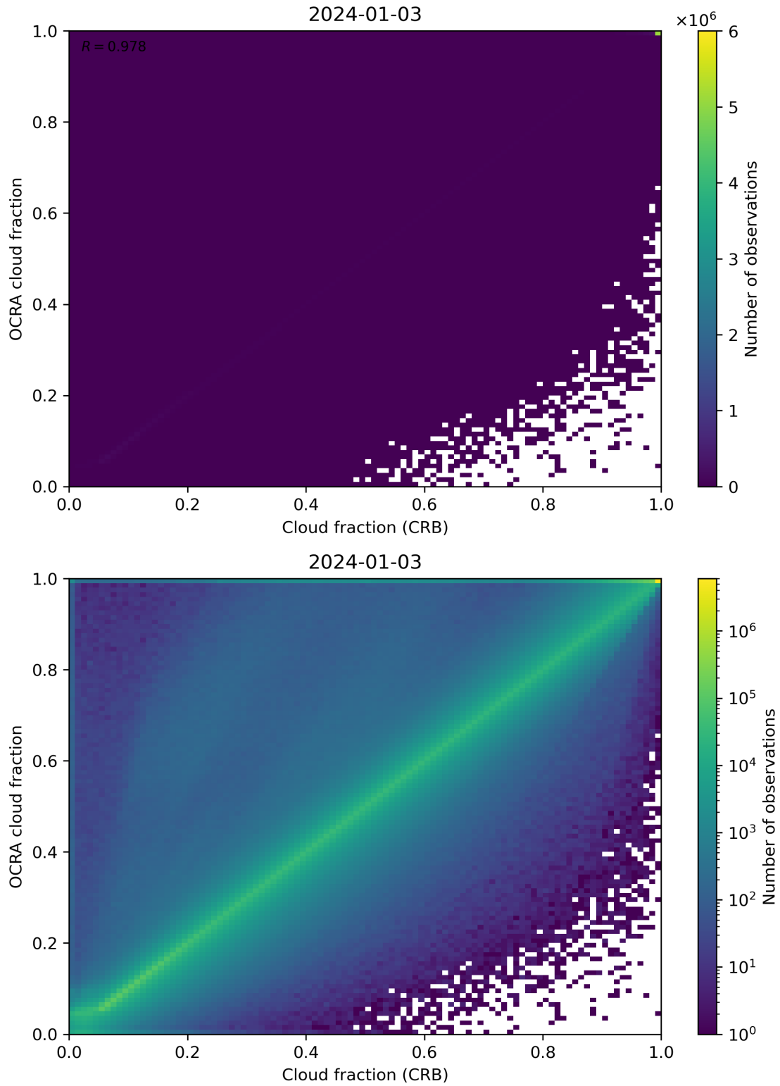
Figure 78: Scatter density plot of “Cloud fraction (CRB)” against “OCRA cloud fraction” for 2024-01-02 to 2024-01-04.
