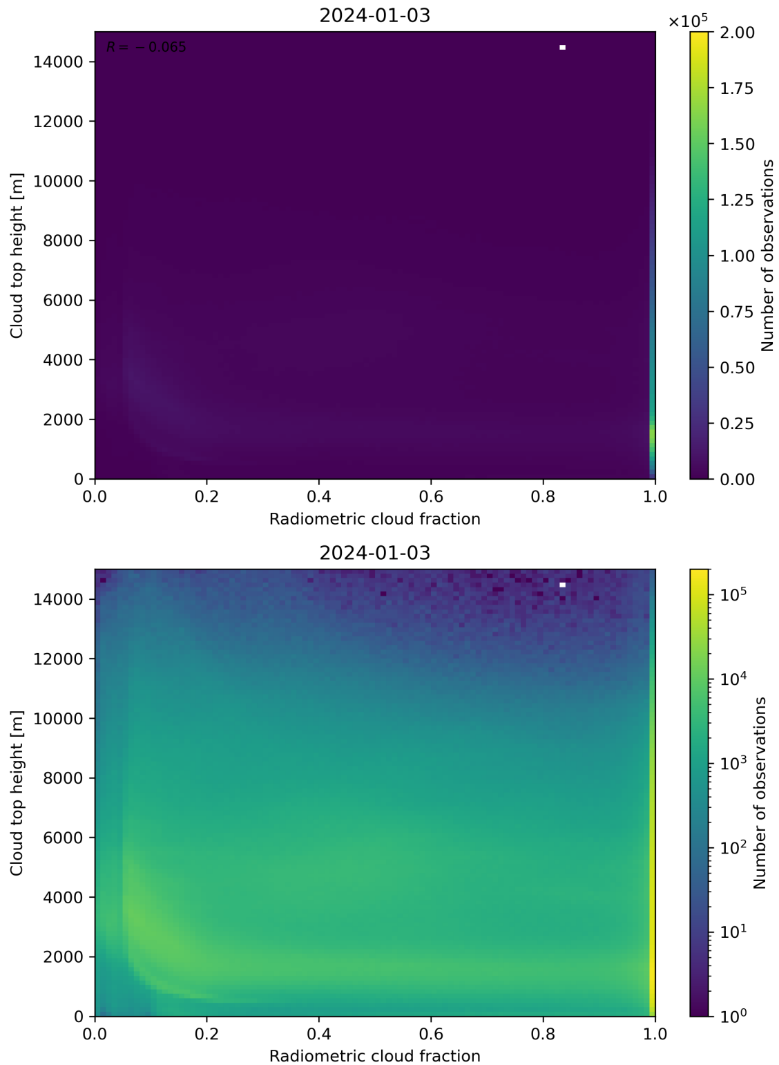
Figure 76: Scatter density plot of “Radiometric cloud fraction” against “Cloud top height” for 2024-01-02 to 2024-01-04.
