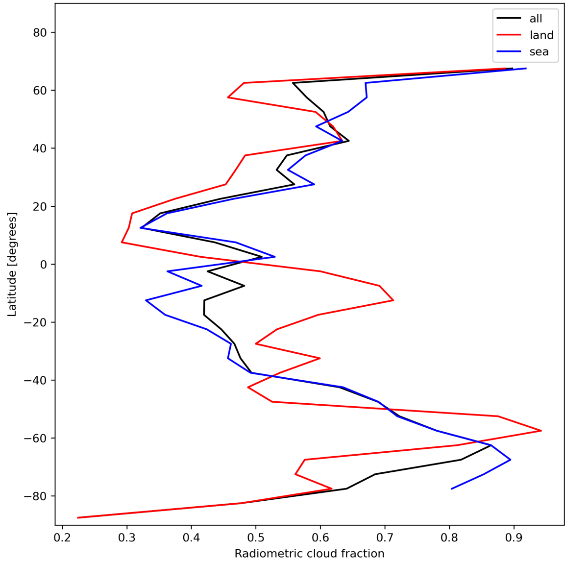
Figure 23: Zonal average of “Radiometric cloud fraction” for 2024-01-02 to 2024-01-04.
