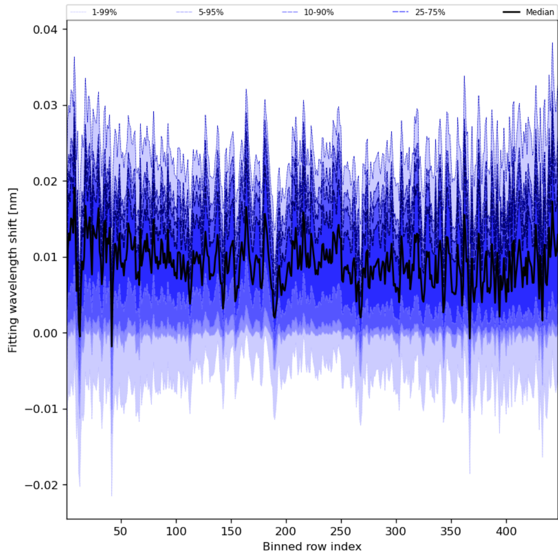
Figure 65: Along track statistics of “Fitting wavelength shift” for 2024-01-02 to 2024-01-04
