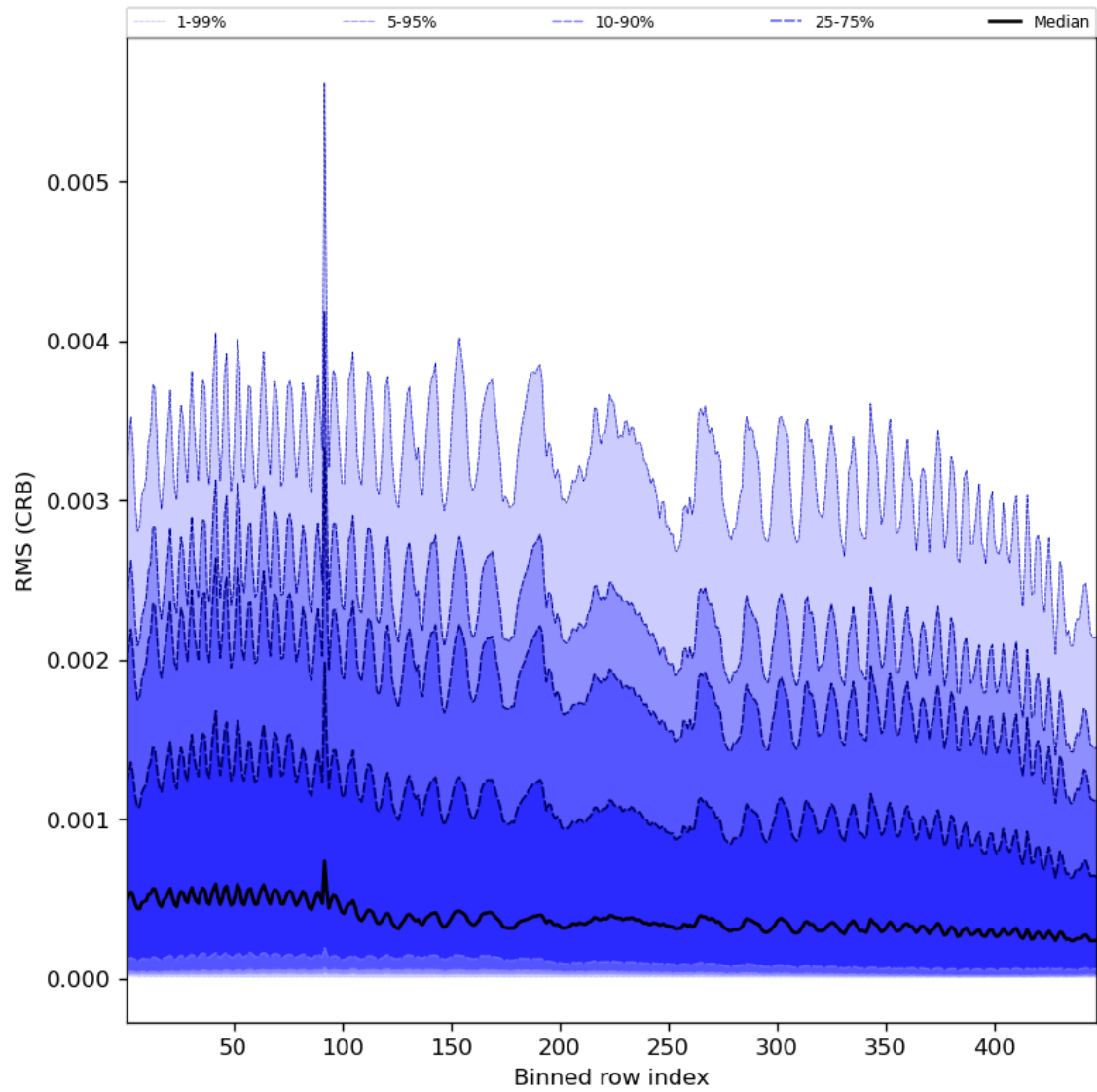
Figure 64: Along track statistics of “RMS (CRB)” for 2024-01-02 to 2024-01-04
