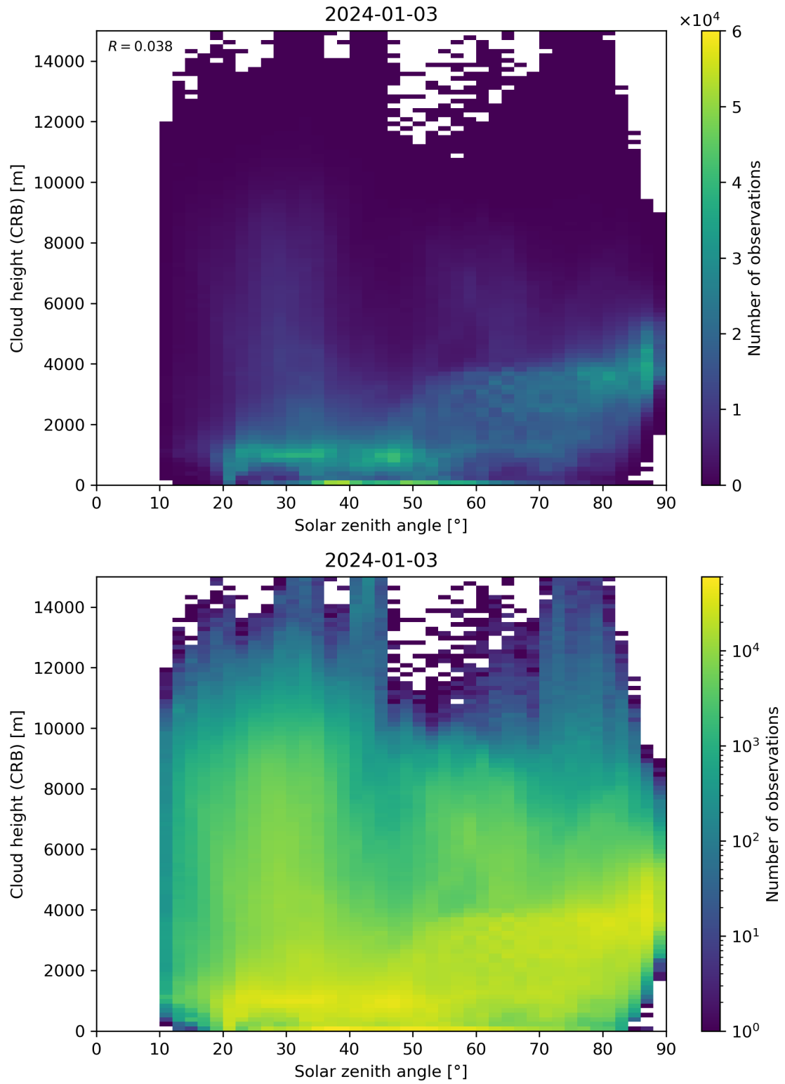
Figure 102: Scatter density plot of “Solar zenith angle” against “Cloud height (CRB)” for 2024-01-02 to 2024-01-04.
