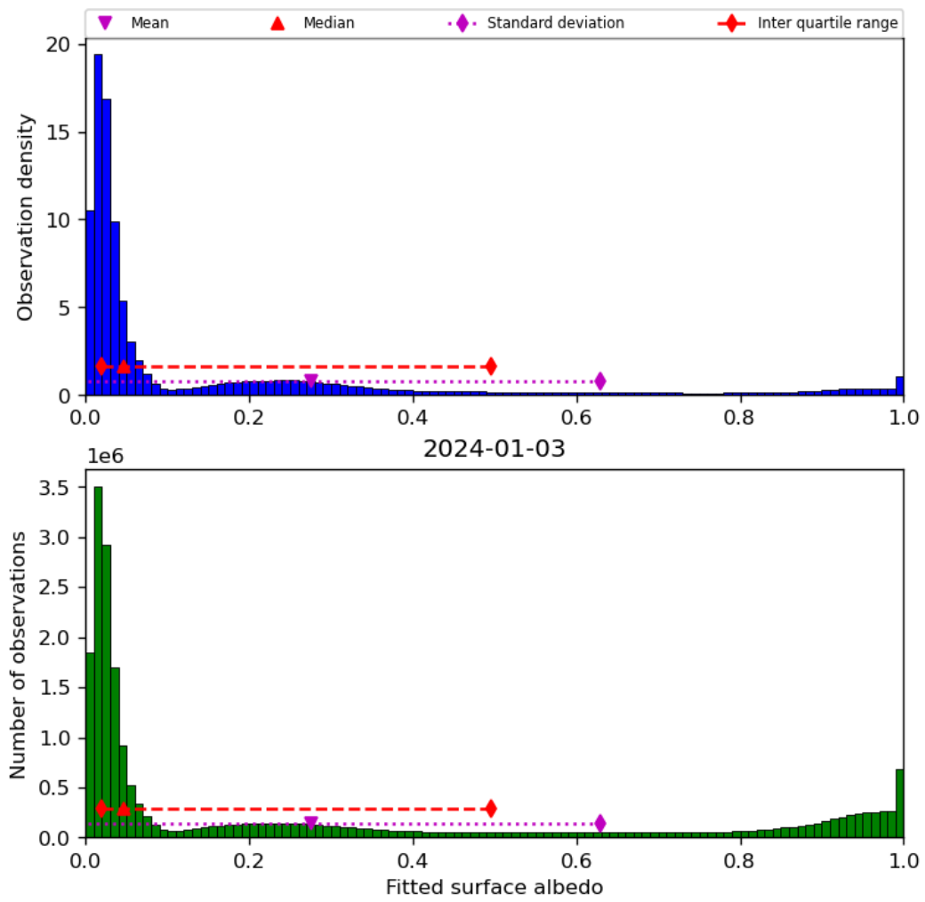
Figure 45: Histogram of “Fitted surface albedo” for 2024-01-02 to 2024-01-04
