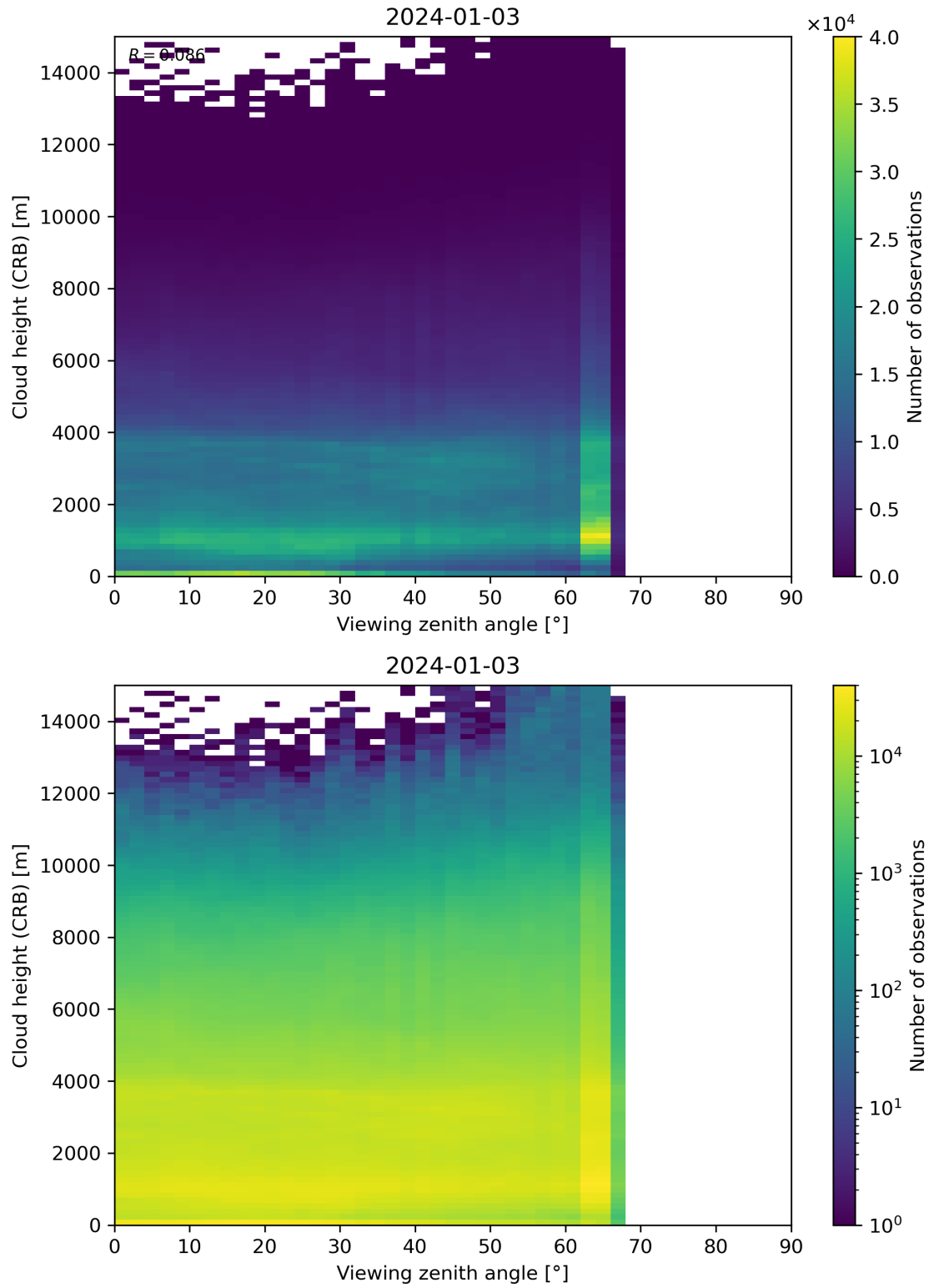
Figure 110: Scatter density plot of “Viewing zenith angle” against “Cloud height (CRB)” for 2024-01-02 to 2024-01-04.
