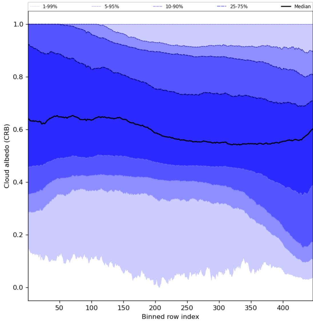
Figure 60: Along track statistics of “Cloud albedo (CRB)” for 2024-01-02 to 2024-01-04
