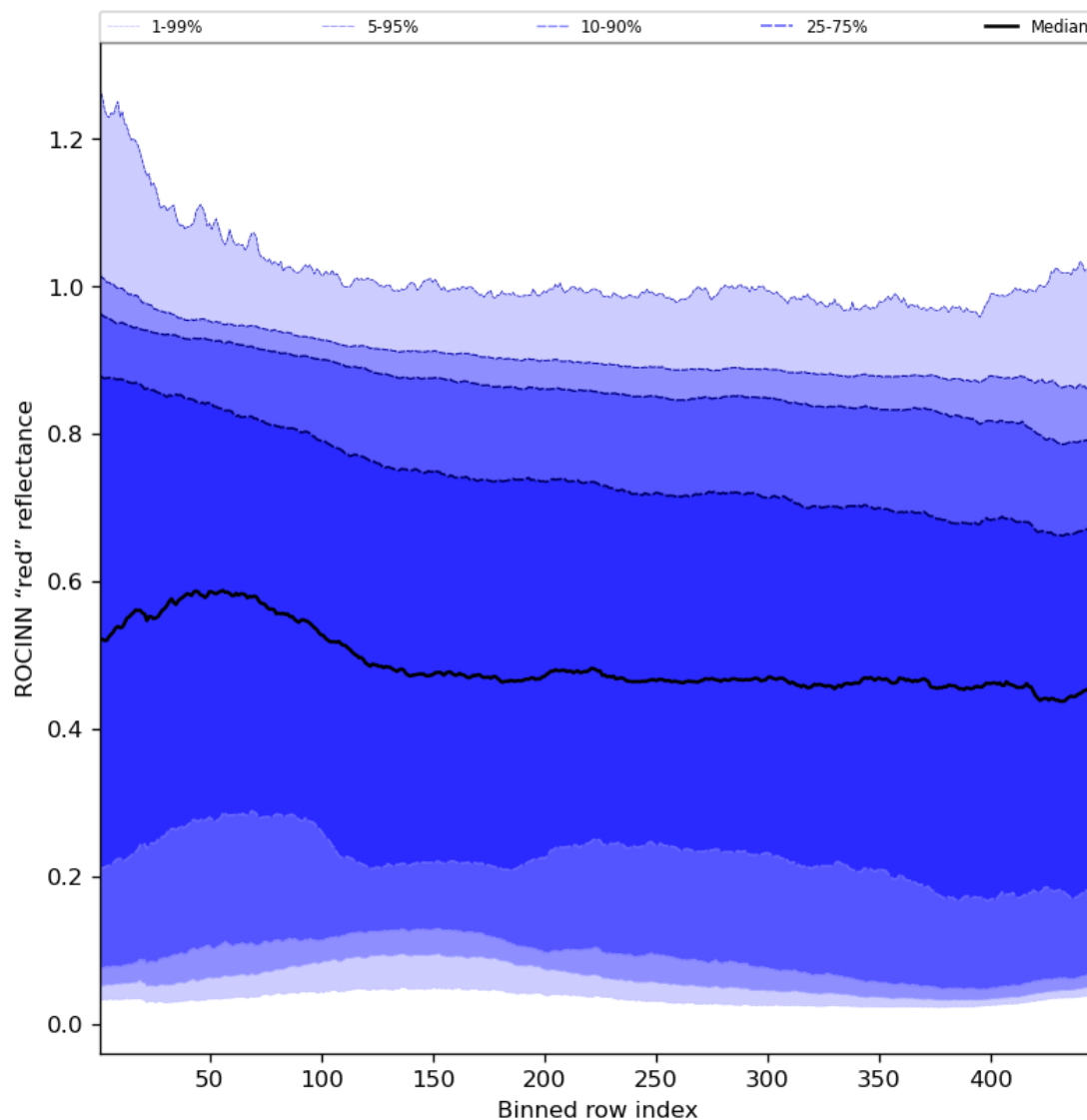
Figure 69: Along track statistics of “ROCINN “red” reflectance” for 2024-01-02 to 2024-01-04
