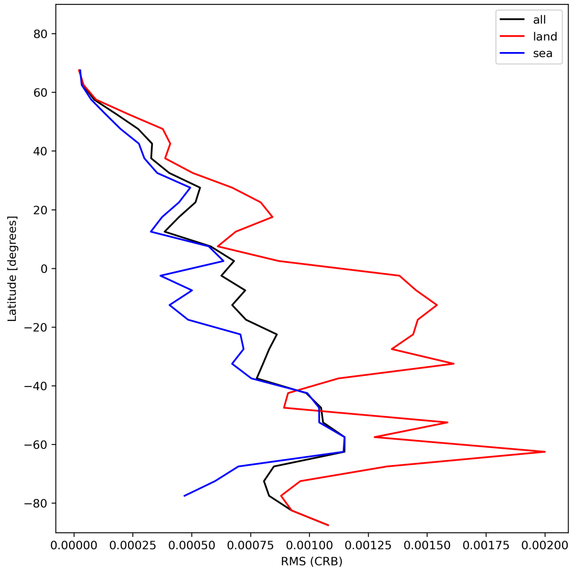
Figure 32: Zonal average of “RMS (CRB)” for 2024-01-02 to 2024-01-04.
