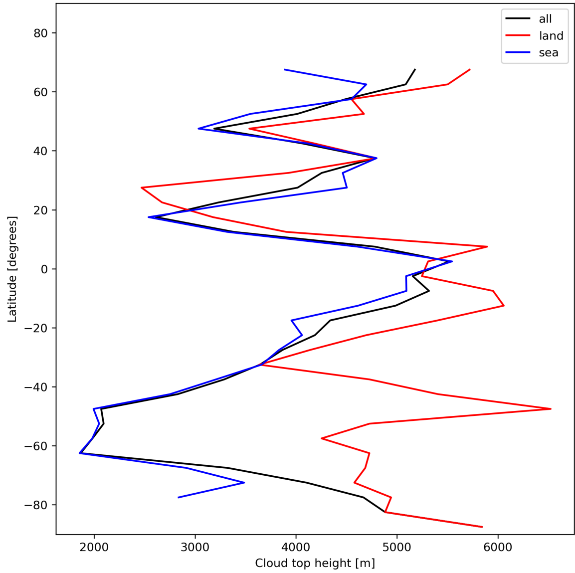
Figure 24: Zonal average of “Cloud top height” for 2024-01-02 to 2024-01-04.
