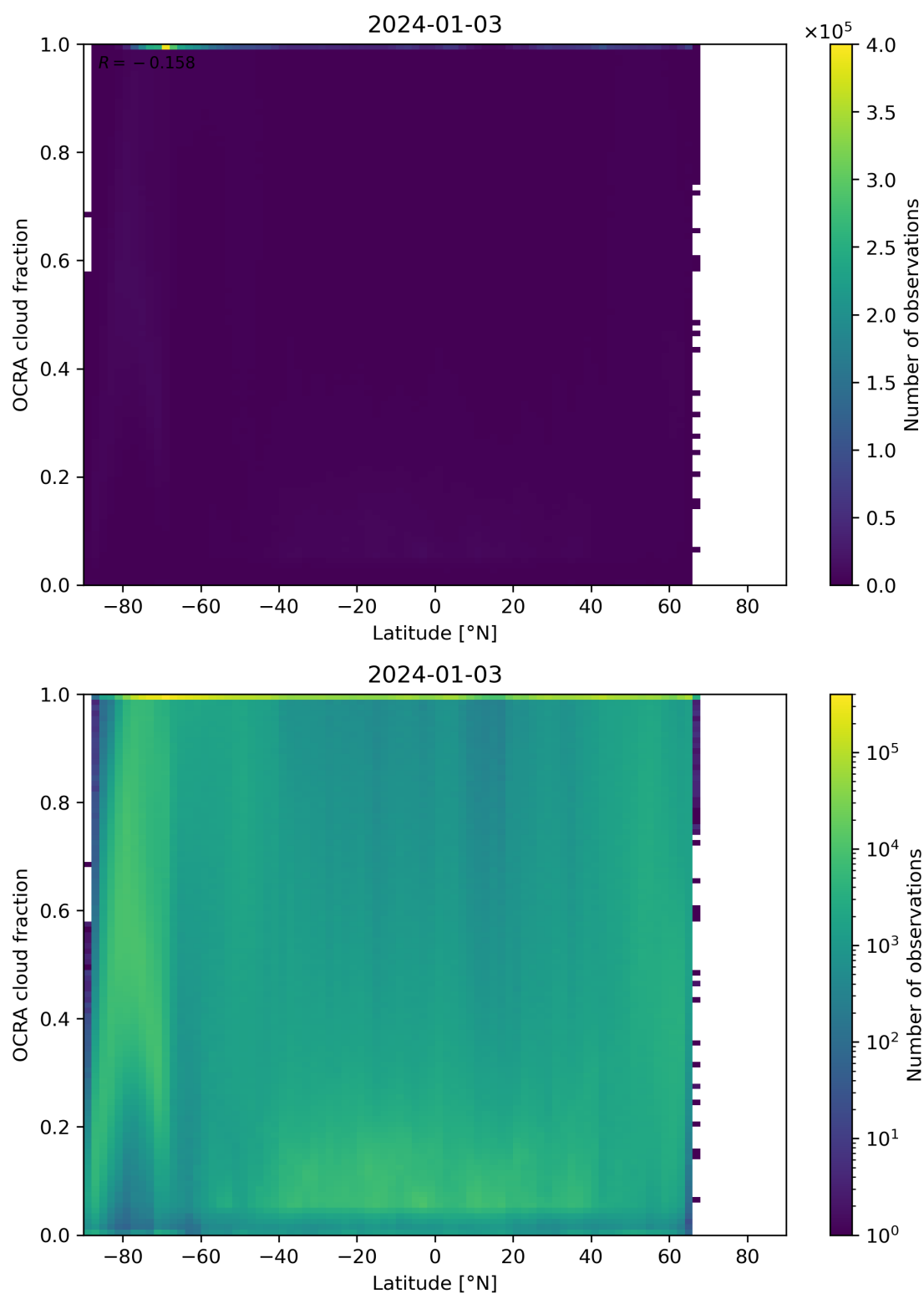
Figure 93: Scatter density plot of “Latitude” against “OCRA cloud fraction” for 2024-01-02 to 2024-01-04.
