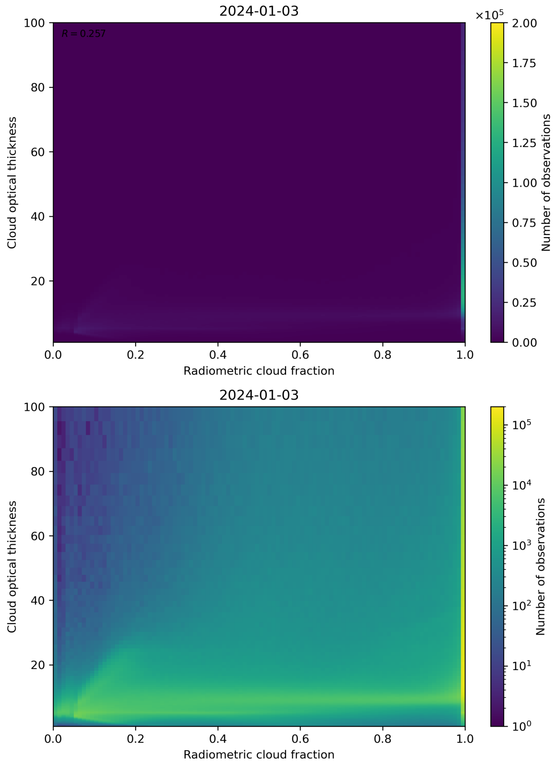
Figure 75: Scatter density plot of “Radiometric cloud fraction” against “Cloud optical thickness” for 2024-01-02 to 2024-01-04.
