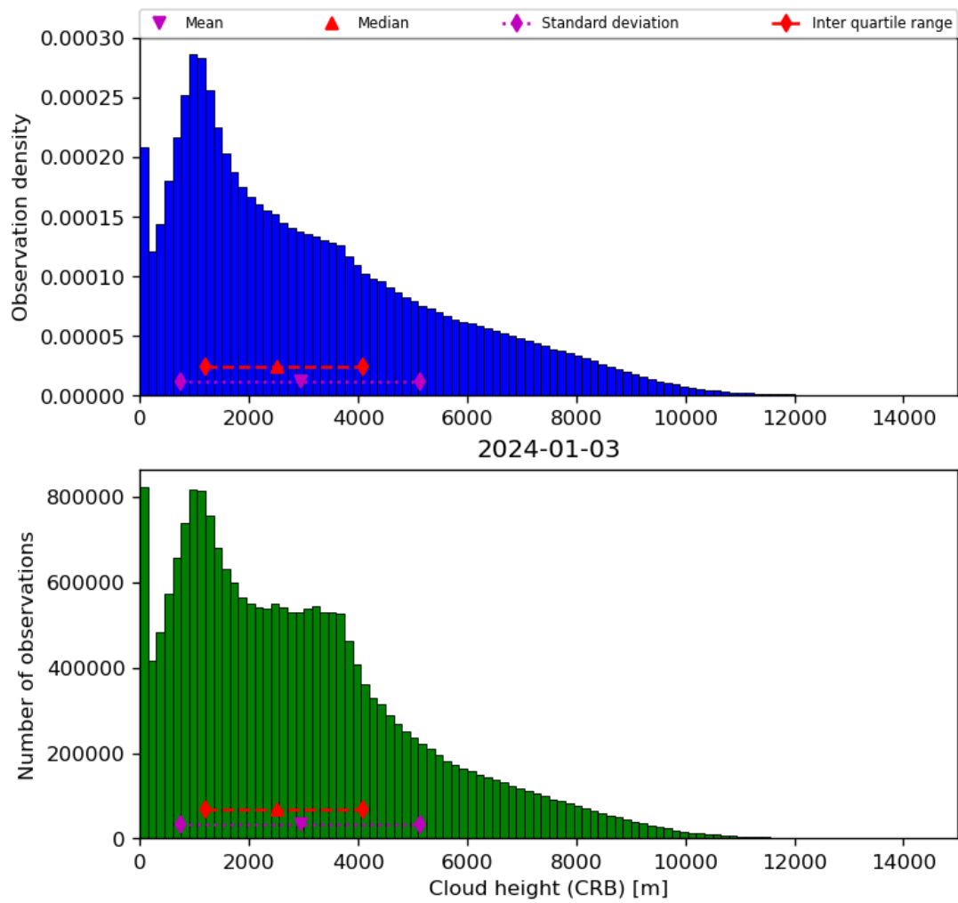
Figure 43: Histogram of “Cloud height (CRB)” for 2024-01-02 to 2024-01-04
