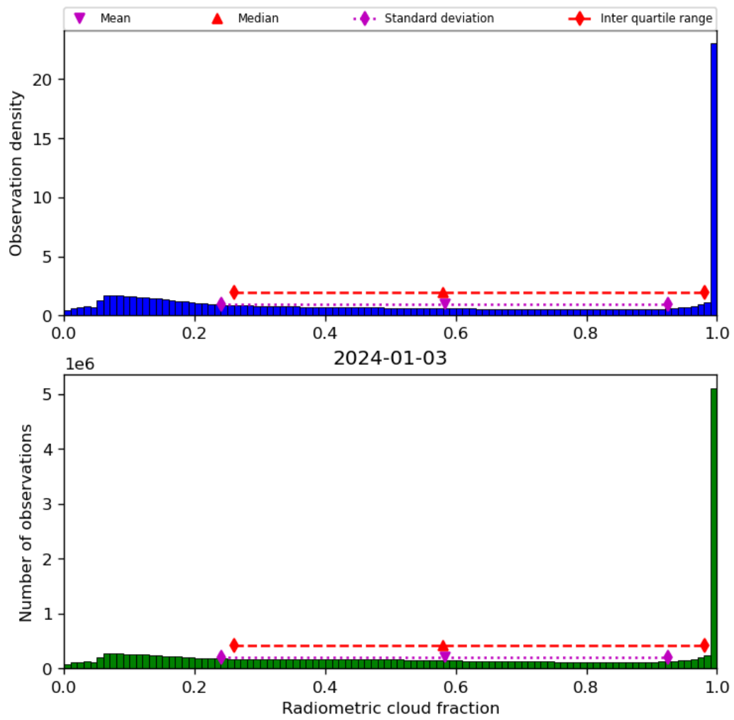
Figure 39: Histogram of “Radiometric cloud fraction” for 2024-01-02 to 2024-01-04
