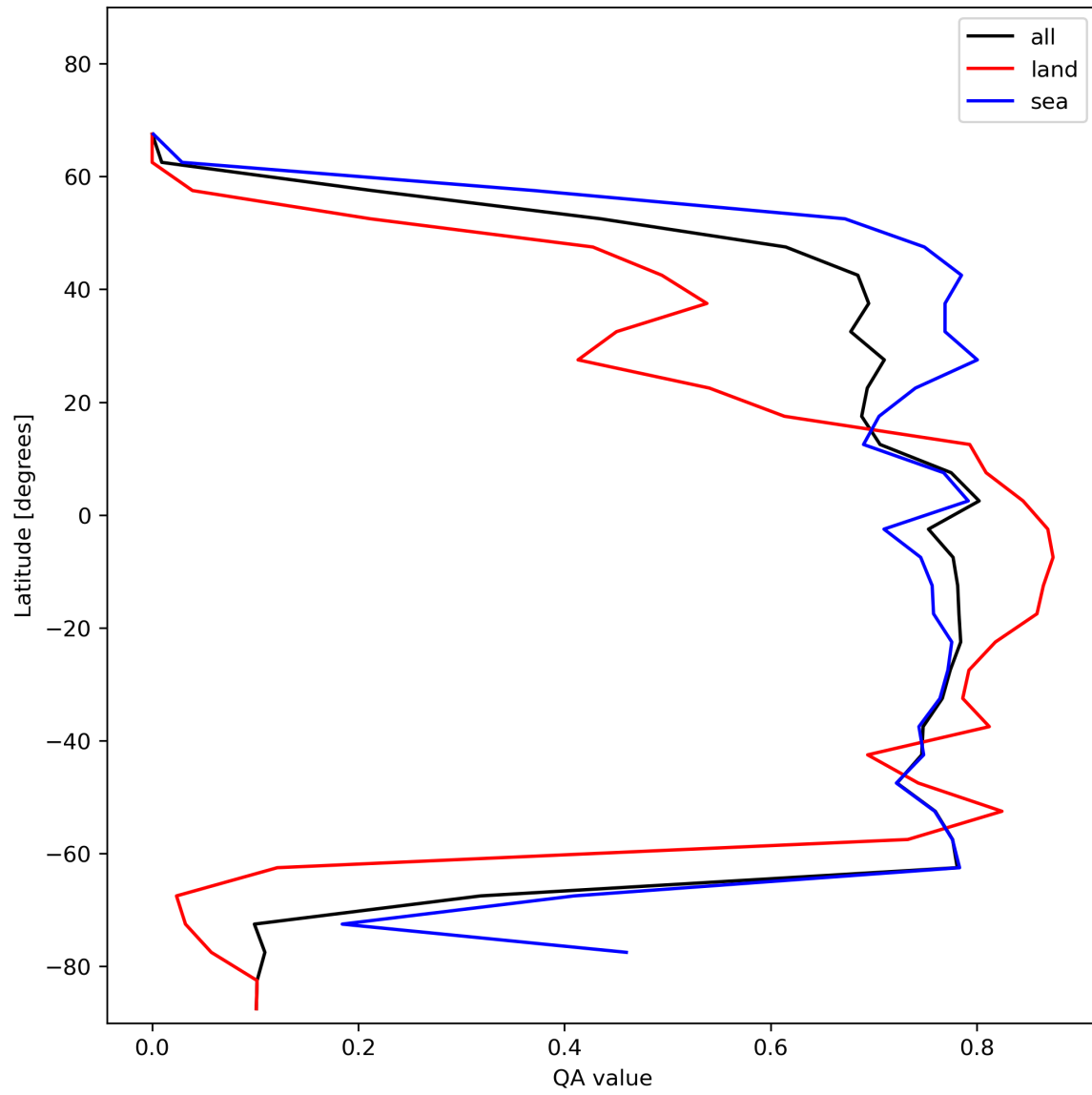
Figure 22: Zonal average of “QA value” for 2024-01-02 to 2024-01-04.
