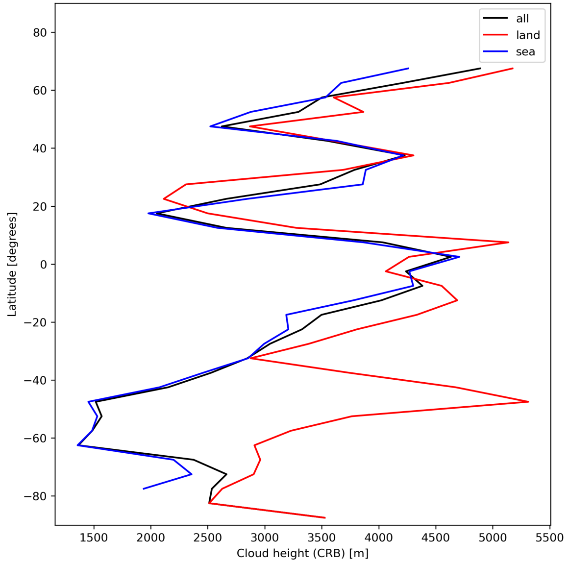
Figure 27: Zonal average of “Cloud height (CRB)” for 2024-01-02 to 2024-01-04.
