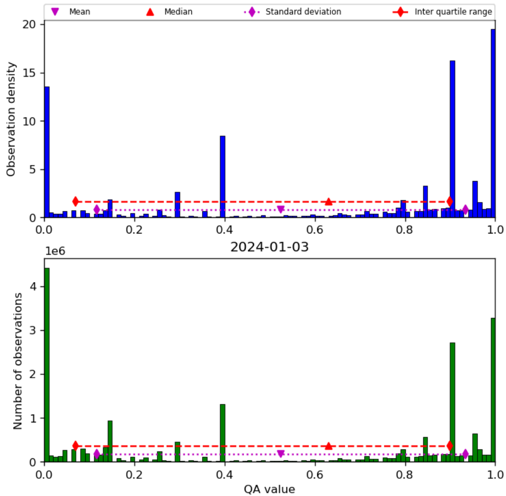
Figure 38: Histogram of “QA value” for 2024-01-02 to 2024-01-04
