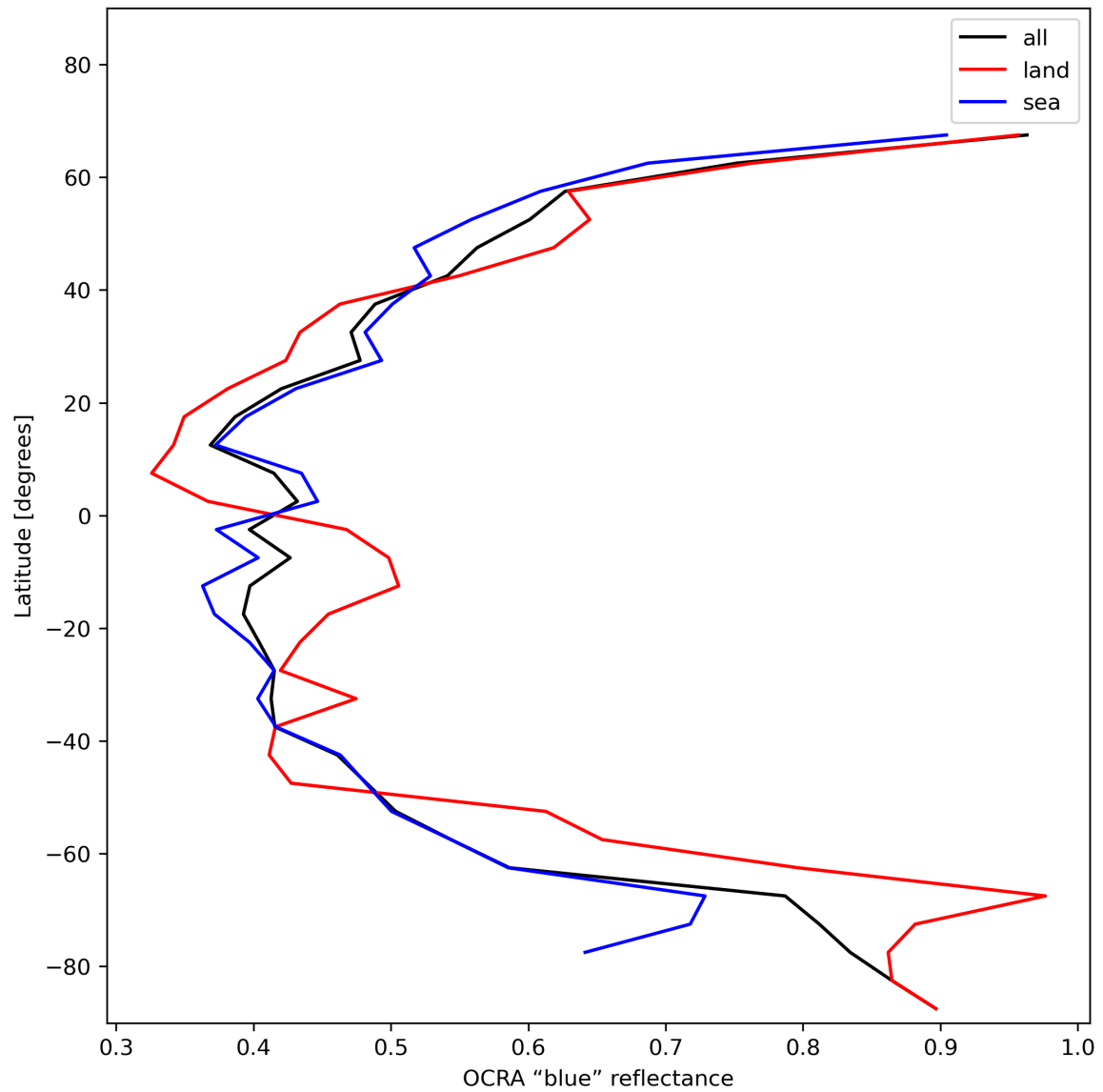
Figure 35: Zonal average of "OCRA "blue" reflectance" for 2024-01-02 to 2024-01-04.
