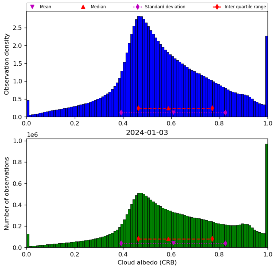
Figure 44: Histogram of “Cloud albedo (CRB)” for 2024-01-02 to 2024-01-04
