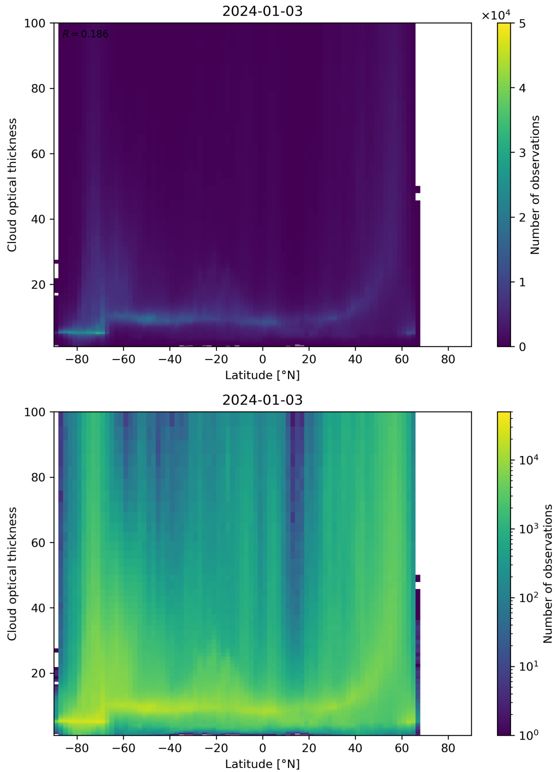
Figure 96: Scatter density plot of “Latitude” against “Cloud optical thickness” for 2024-01-02 to 2024-01-04.
