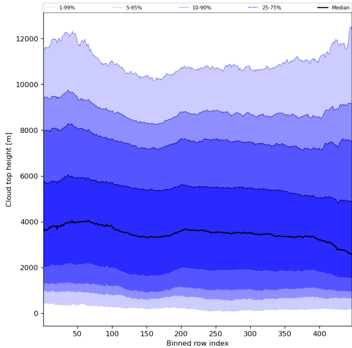
Figure 56: Along track statistics of “Cloud top height” for 2024-01-02 to 2024-01-04
