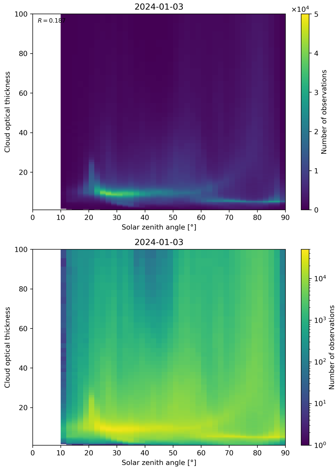
Figure 103: Scatter density plot of “Solar zenith angle” against “Cloud optical thickness” for 2024-01-02 to 2024-01-04.
