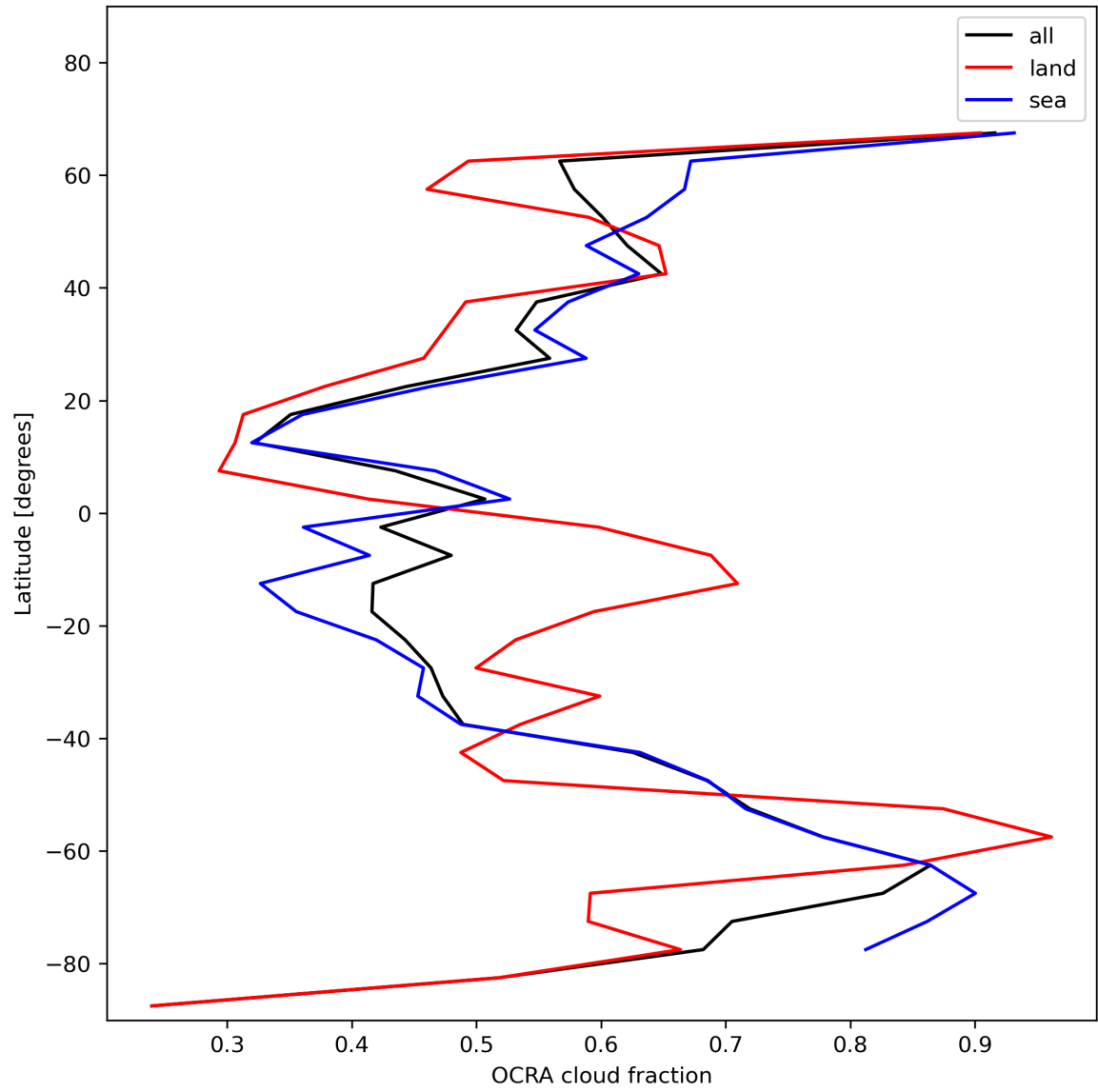
Figure 34: Zonal average of “OCRA cloud fraction” for 2024-01-02 to 2024-01-04.
