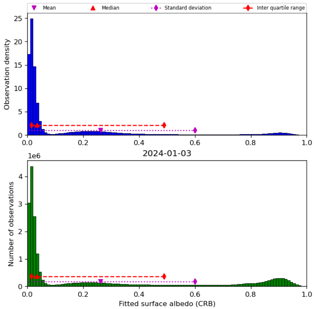
Figure 46: Histogram of “Fitted surface albedo (CRB)” for 2024-01-02 to 2024-01-04
