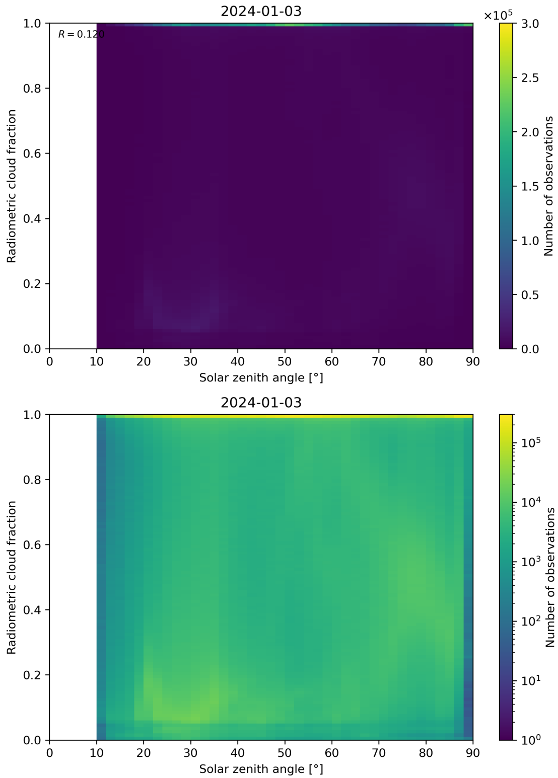
Figure 99: Scatter density plot of “Solar zenith angle” against “Radiometric cloud fraction” for 2024-01-02 to 2024-01-04.
