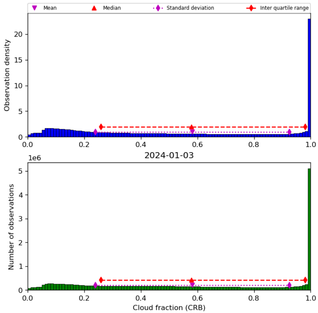
Figure 42: Histogram of “Cloud fraction (CRB)” for 2024-01-02 to 2024-01-04
