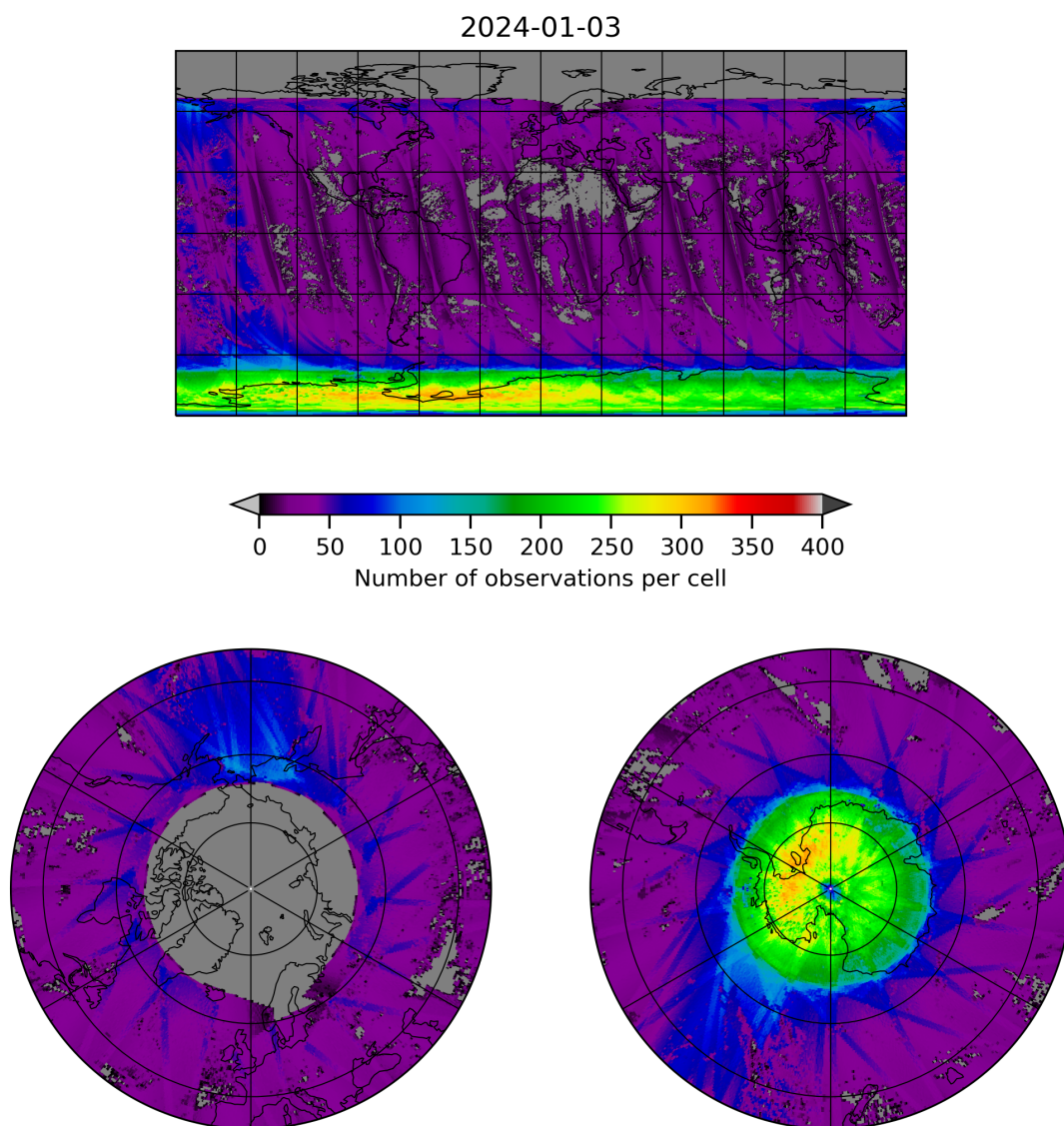
Figure 21: Map of the number of observations for 2024-01-02 to 2024-01-04
