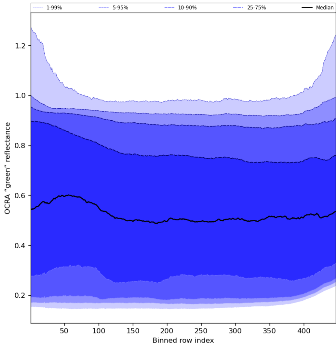
Figure 68: Along track statistics of “OCRA “green” reflectance” for 2024-01-02 to 2024-01-04
