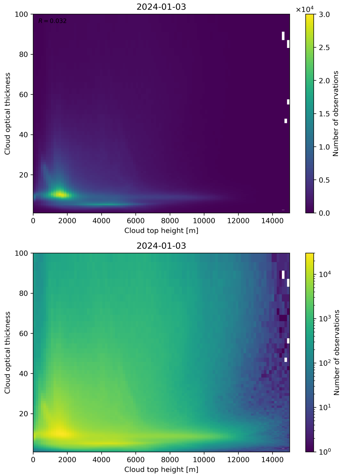
Figure 90: Scatter density plot of “Cloud top height” against “Cloud optical thickness” for 2024-01-02 to 2024-01-04.
