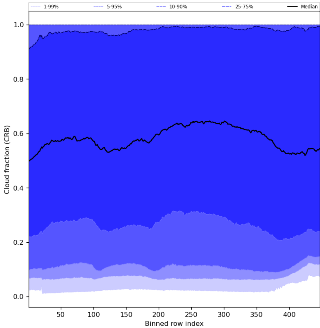
Figure 58: Along track statistics of “Cloud fraction (CRB)” for 2024-01-02 to 2024-01-04
