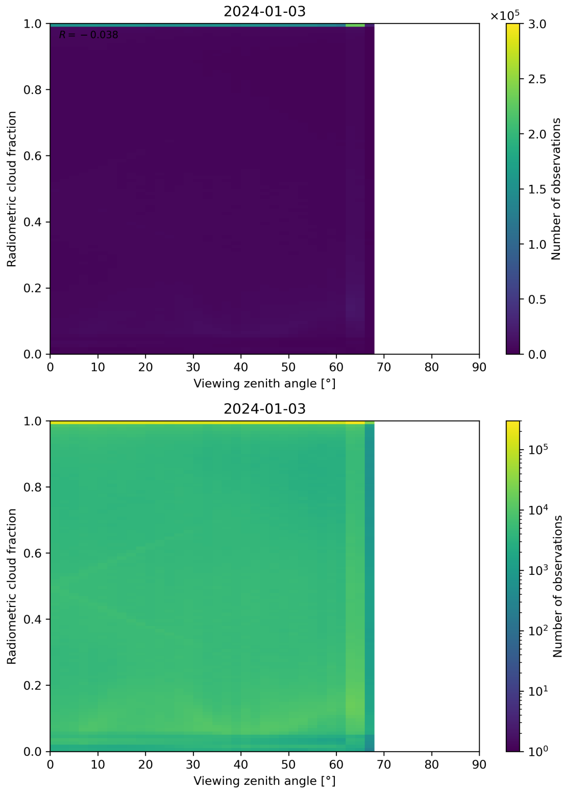
Figure 107: Scatter density plot of “Viewing zenith angle” against “Radiometric cloud fraction” for 2024-01-02 to 2024-01-04.
