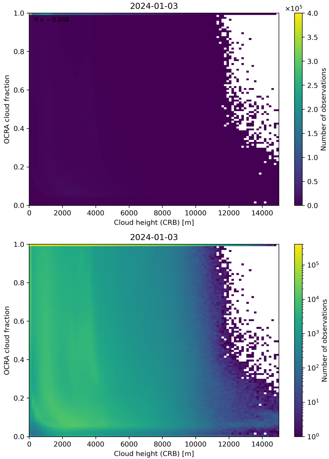
Figure 81: Scatter density plot of “Cloud height (CRB)” against “OCRA cloud fraction” for 2024-01-02 to 2024-01-04.
