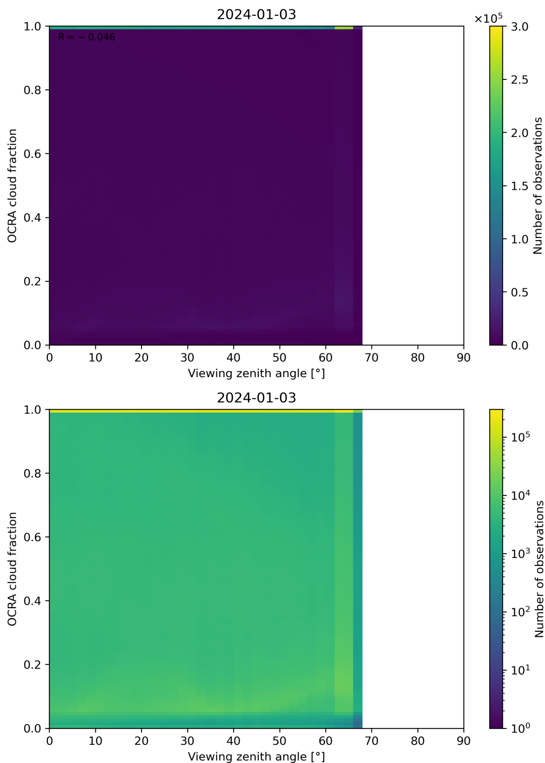
Figure 108: Scatter density plot of “Viewing zenith angle” against “OCRA cloud fraction” for 2024-01-02 to 2024-01-04.
