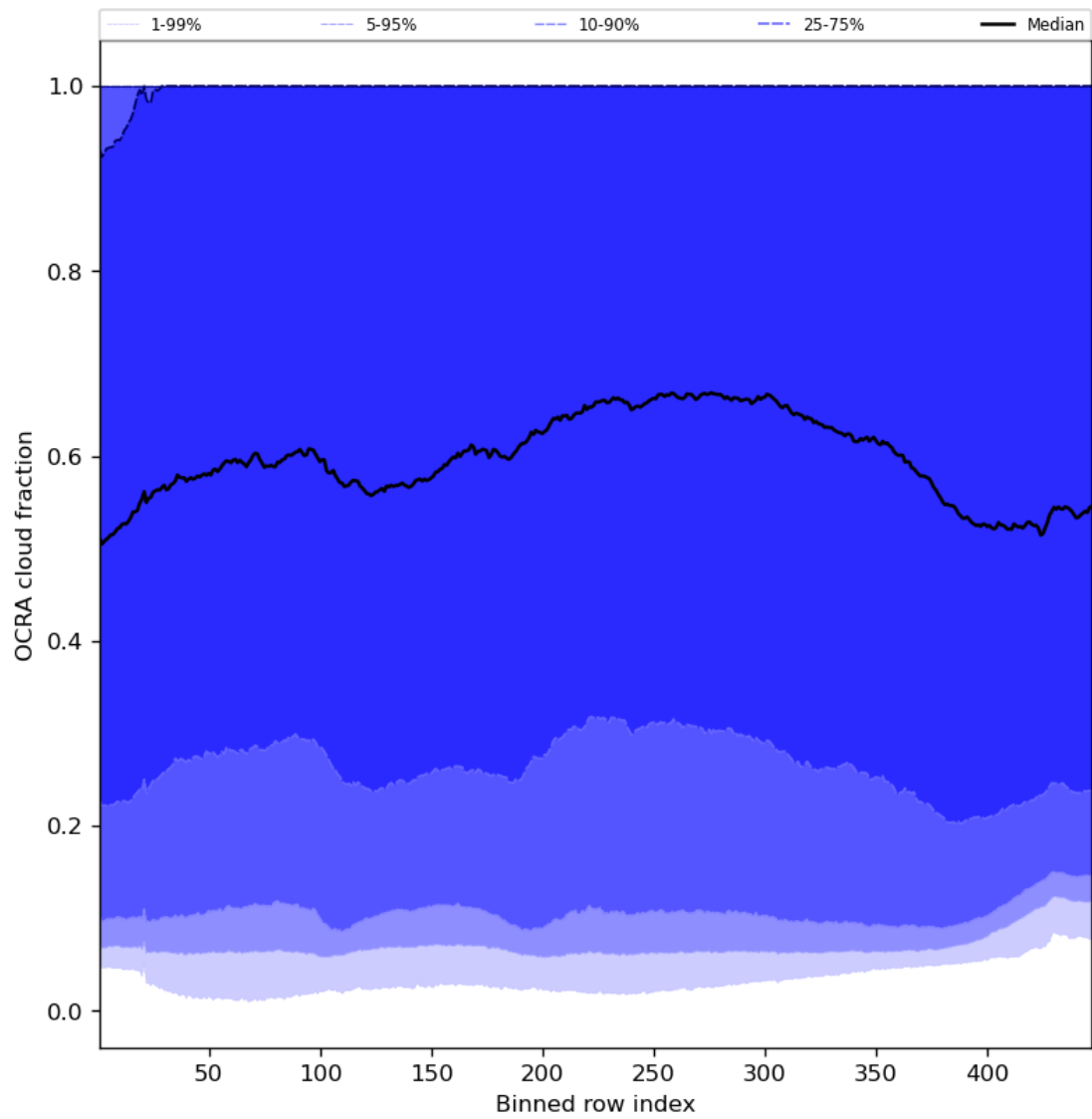
Figure 66: Along track statistics of “OCRA cloud fraction” for 2024-01-02 to 2024-01-04
