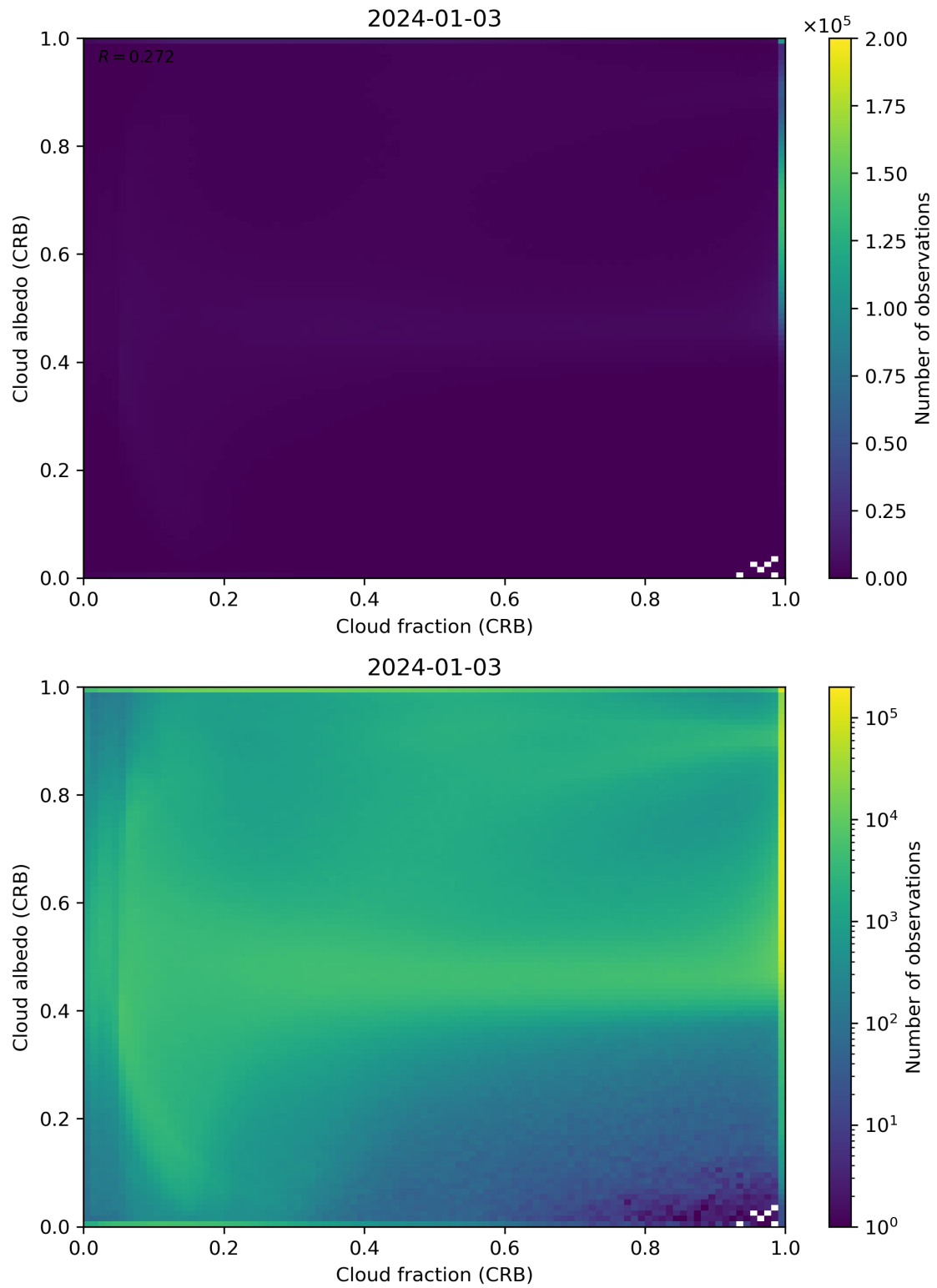
Figure 77: Scatter density plot of “Cloud fraction (CRB)” against “Cloud albedo (CRB)” for 2024-01-02 to 2024-01-04.
