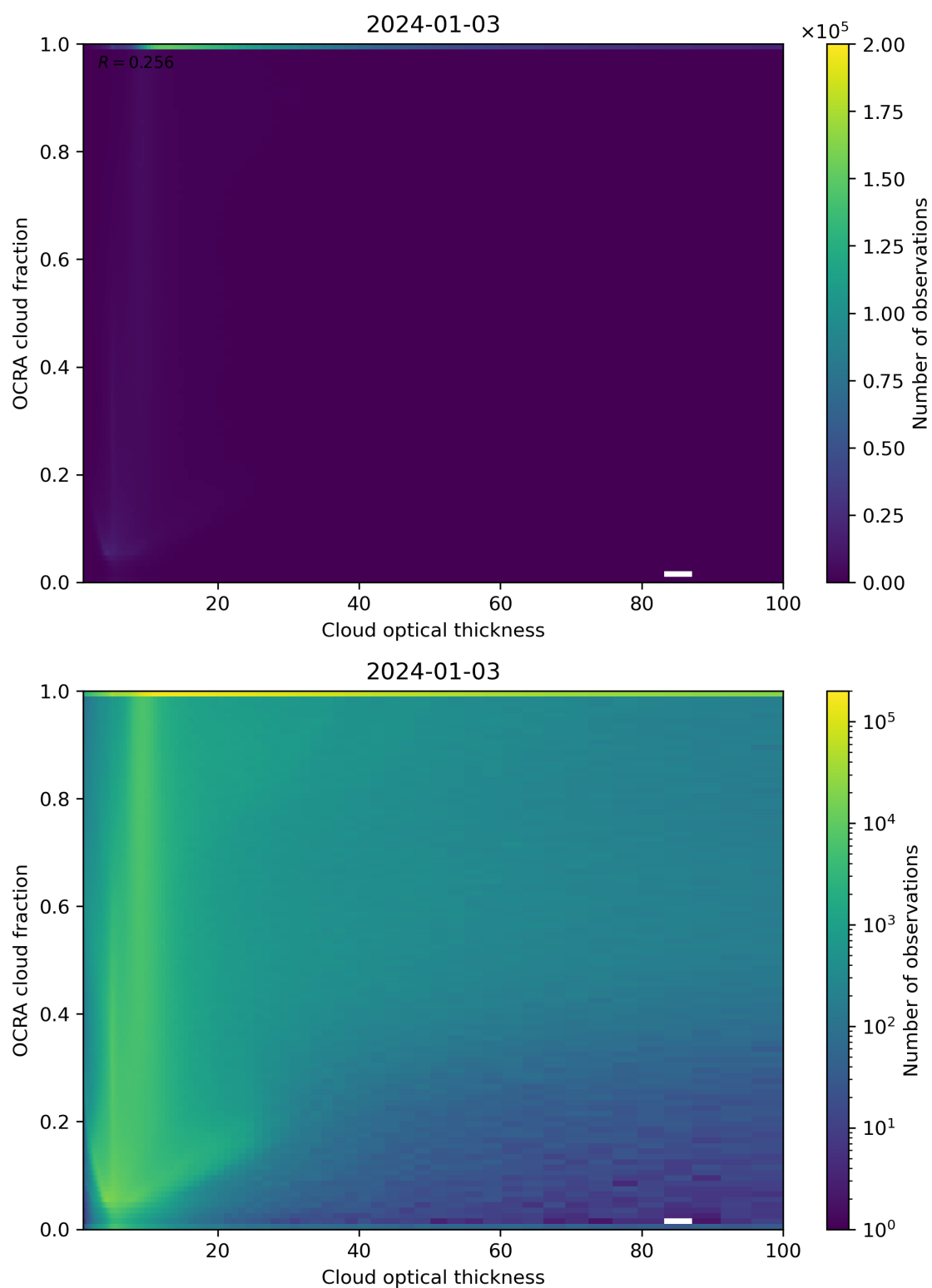
Figure 83: Scatter density plot of “Cloud optical thickness” against “OCRA cloud fraction” for 2024-01-02 to 2024-01-04.
