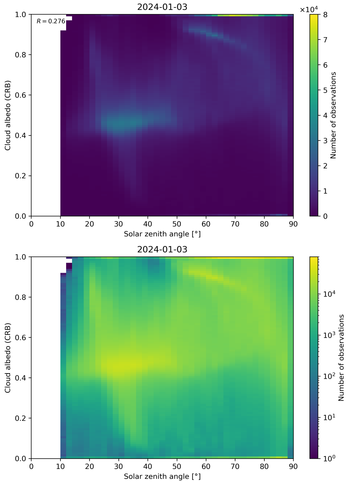
Figure 98: Scatter density plot of “Solar zenith angle” against “Cloud albedo (CRB)” for 2024-01-02 to 2024-01-04.
