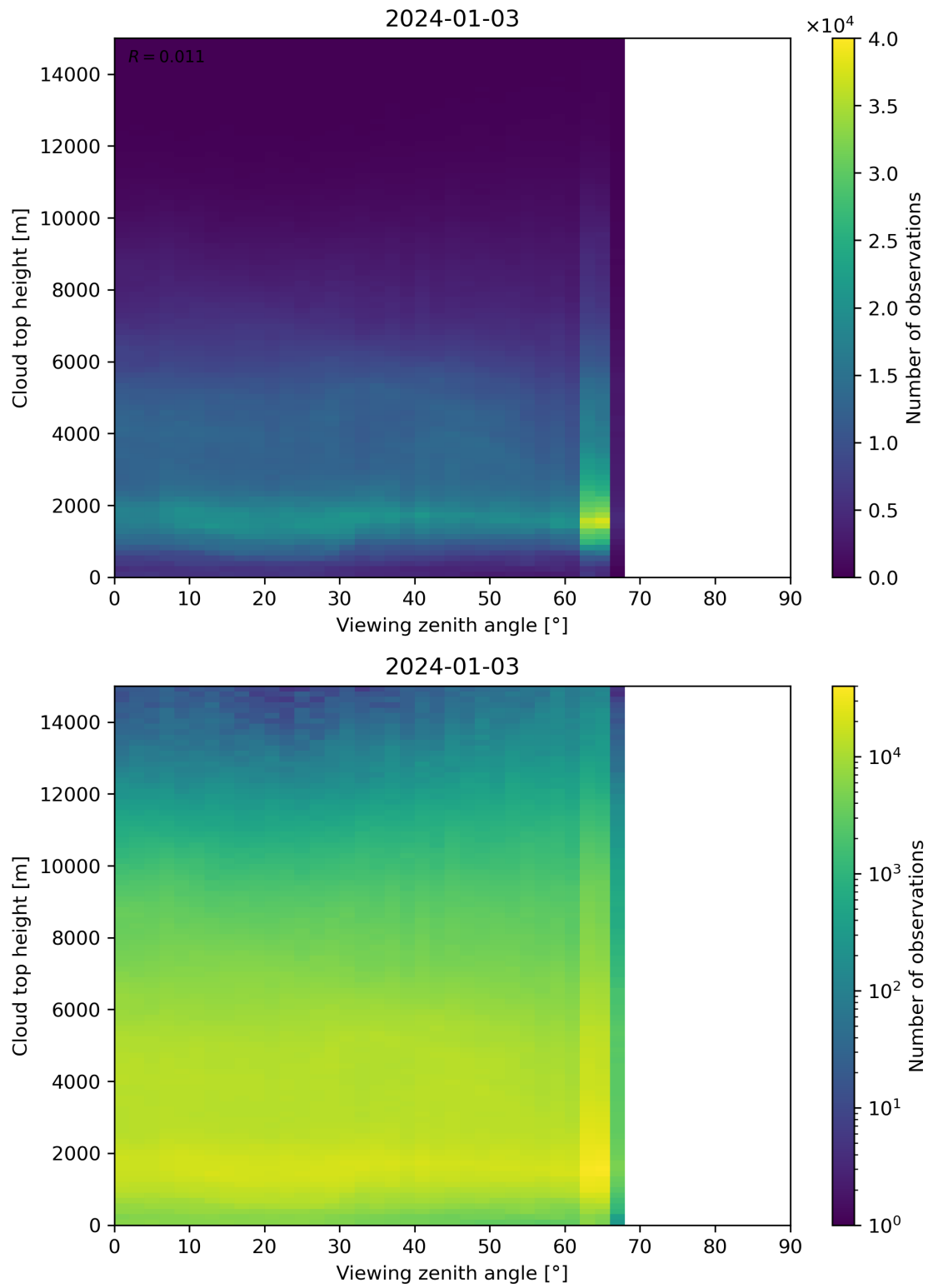
Figure 112: Scatter density plot of “Viewing zenith angle” against “Cloud top height” for 2024-01-02 to 2024-01-04.
