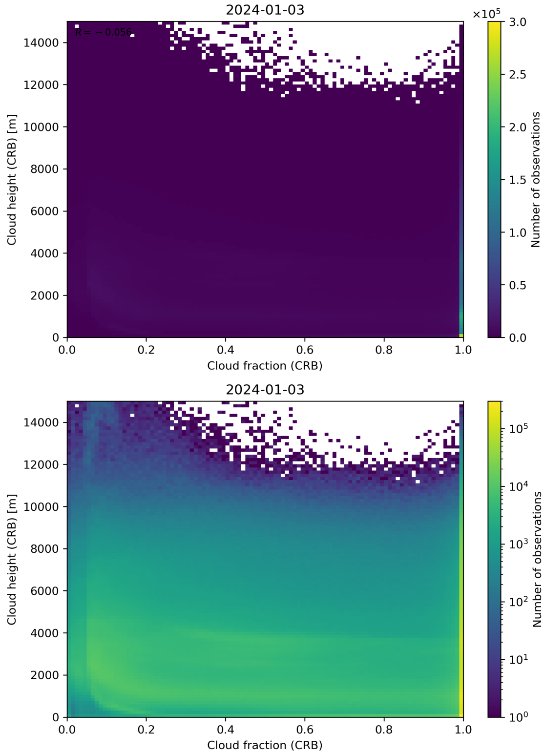
Figure 79: Scatter density plot of “Cloud fraction (CRB)” against “Cloud height (CRB)” for 2024-01-02 to 2024-01-04.
