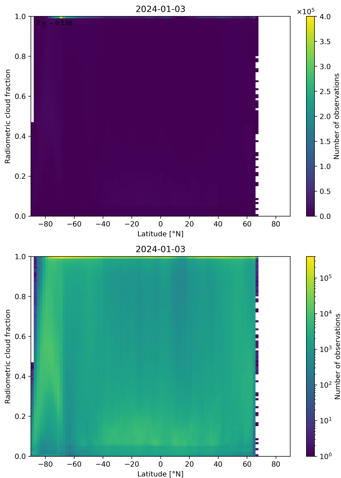
Figure 92: Scatter density plot of “Latitude” against “Radiometric cloud fraction” for 2024-01-02 to 2024-01-04.
