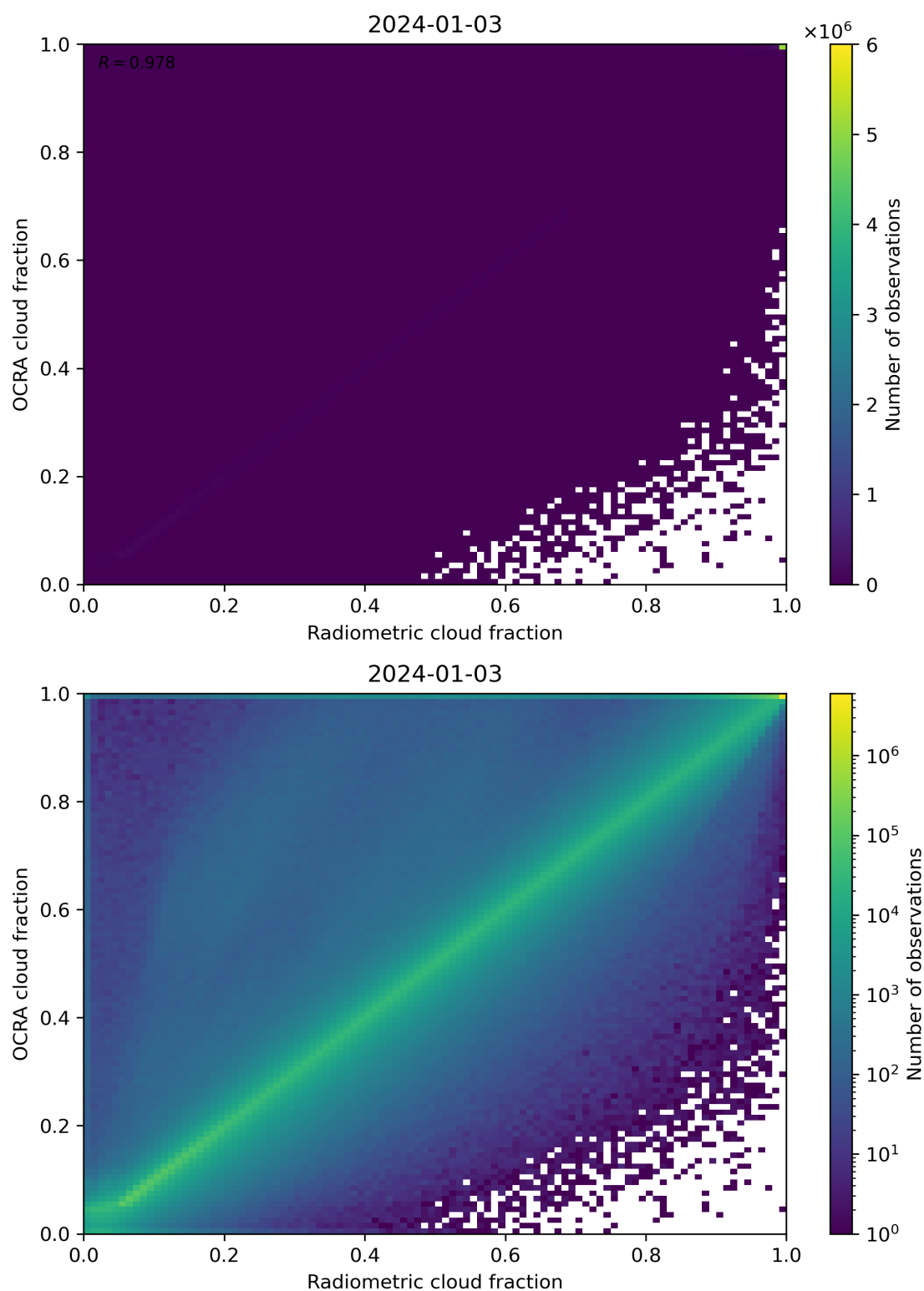
Figure 72: Scatter density plot of “Radiometric cloud fraction” against “OCRA cloud fraction” for 2024-01-02 to 2024-01-04.
