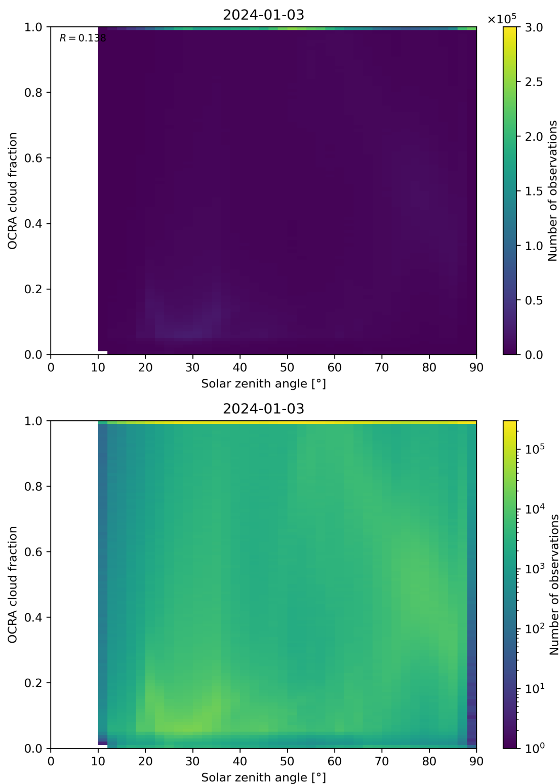
Figure 100: Scatter density plot of “Solar zenith angle” against “OCRA cloud fraction” for 2024-01-02 to 2024-01-04.
