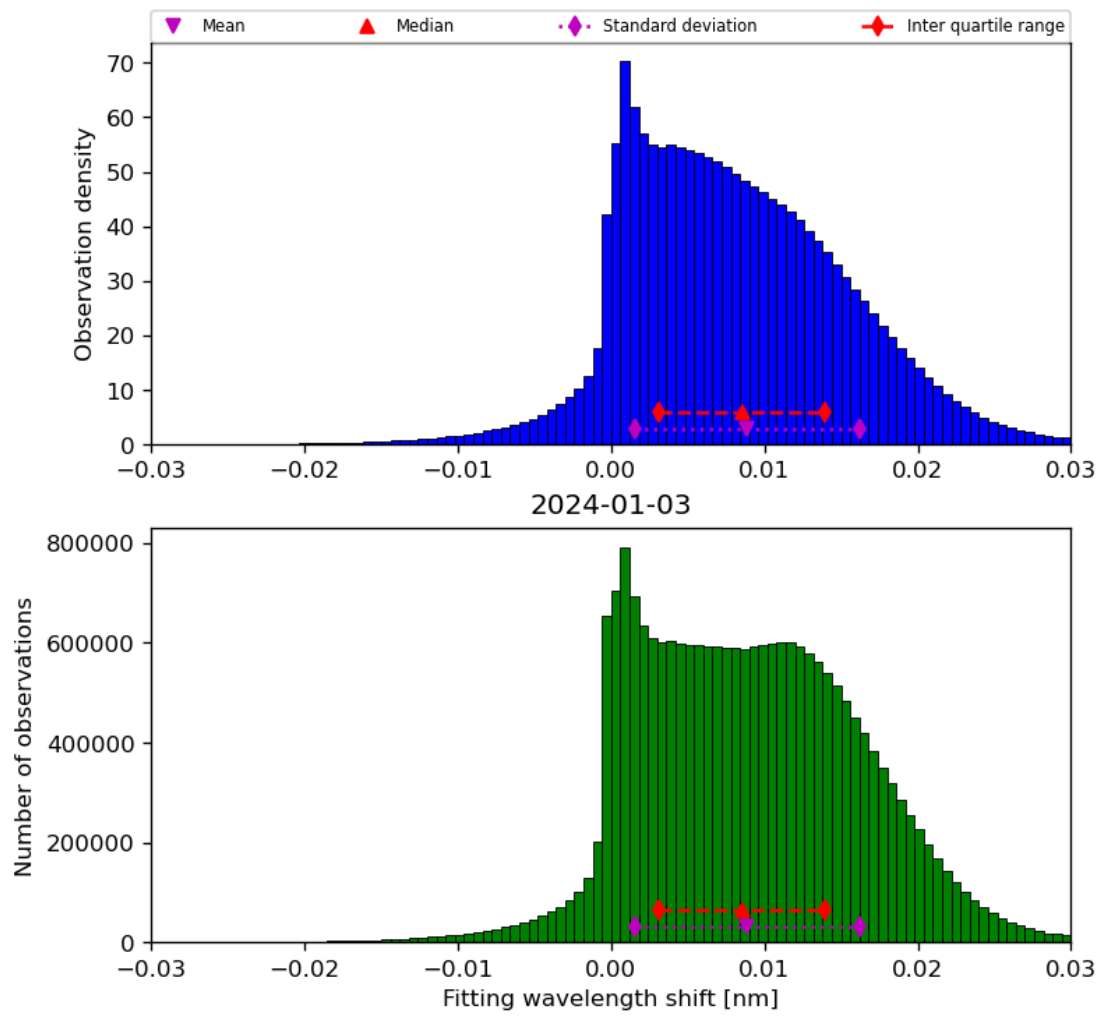
Figure 49: Histogram of “Fitting wavelength shift” for 2024-01-02 to 2024-01-04
