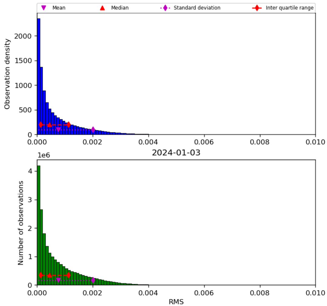
Figure 47: Histogram of “RMS” for 2024-01-02 to 2024-01-04
