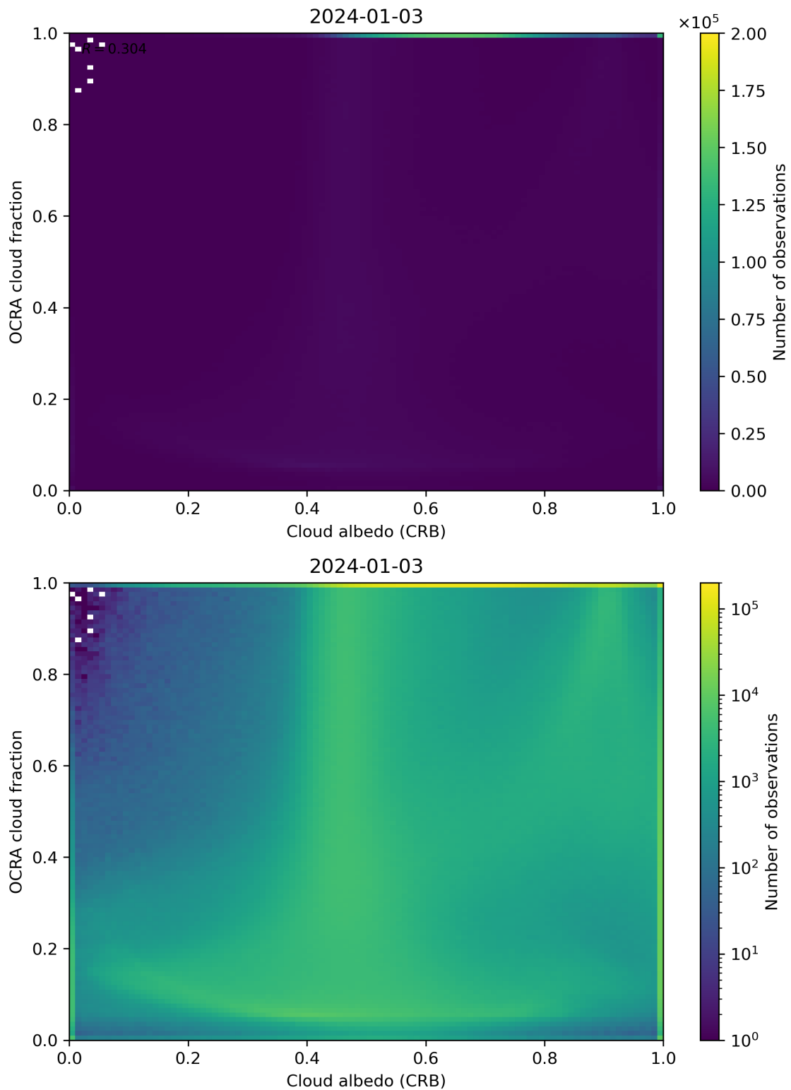
Figure 70: Scatter density plot of “Cloud albedo (CRB)” against “OCRA cloud fraction” for 2024-01-02 to 2024-01-04.
