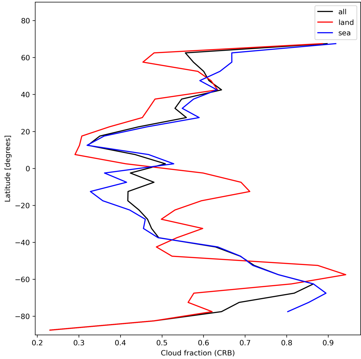
Figure 26: Zonal average of “Cloud fraction (CRB)” for 2024-01-02 to 2024-01-04.
