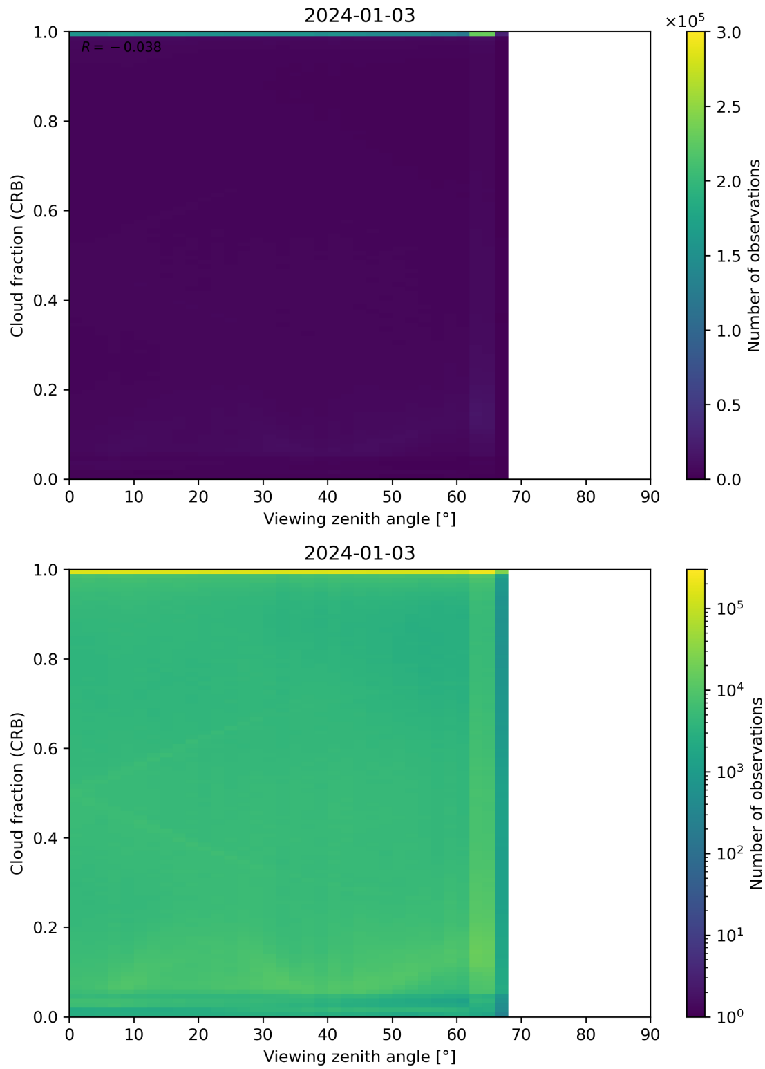
Figure 109: Scatter density plot of “Viewing zenith angle” against “Cloud fraction (CRB)” for 2024-01-02 to 2024-01-04.
