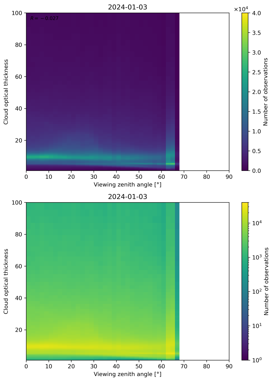
Figure 111: Scatter density plot of “Viewing zenith angle” against “Cloud optical thickness” for 2024-01-02 to 2024-01-04.
