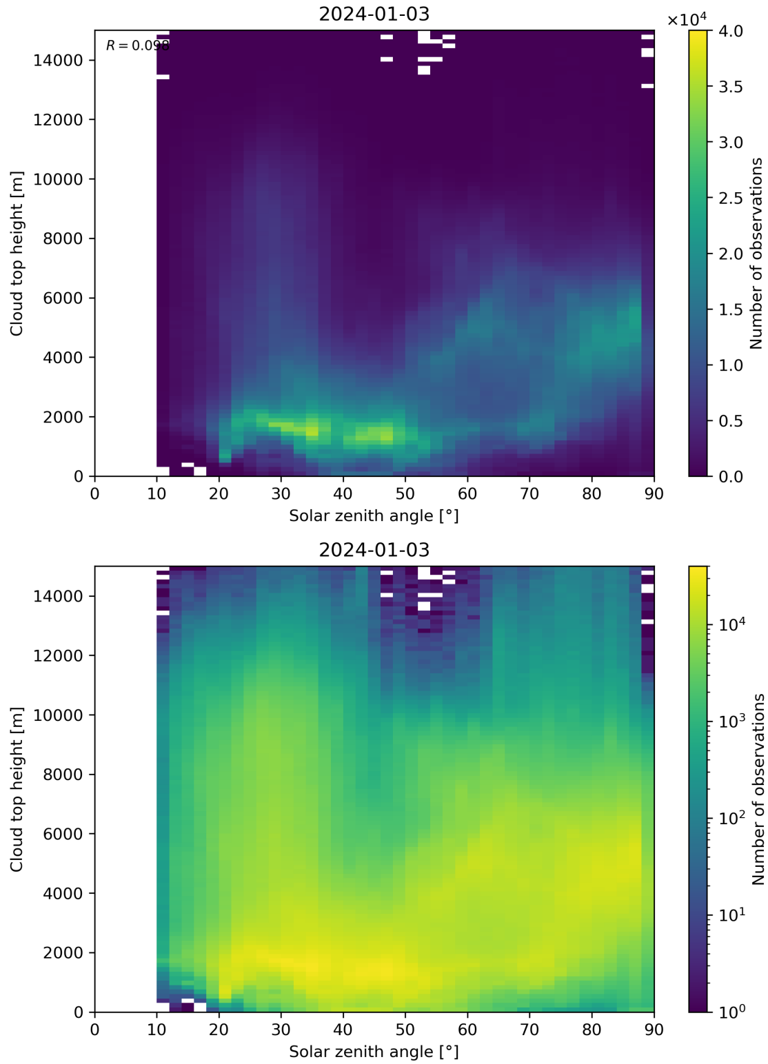
Figure 104: Scatter density plot of “Solar zenith angle” against “Cloud top height” for 2024-01-02 to 2024-01-04.
