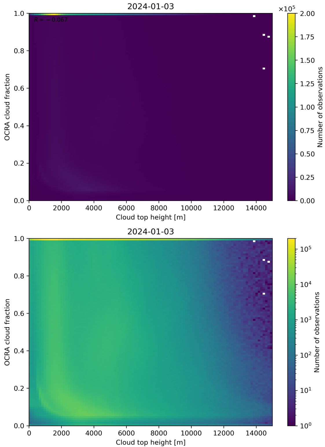
Figure 87: Scatter density plot of “Cloud top height” against “OCRA cloud fraction” for 2024-01-02 to 2024-01-04.
