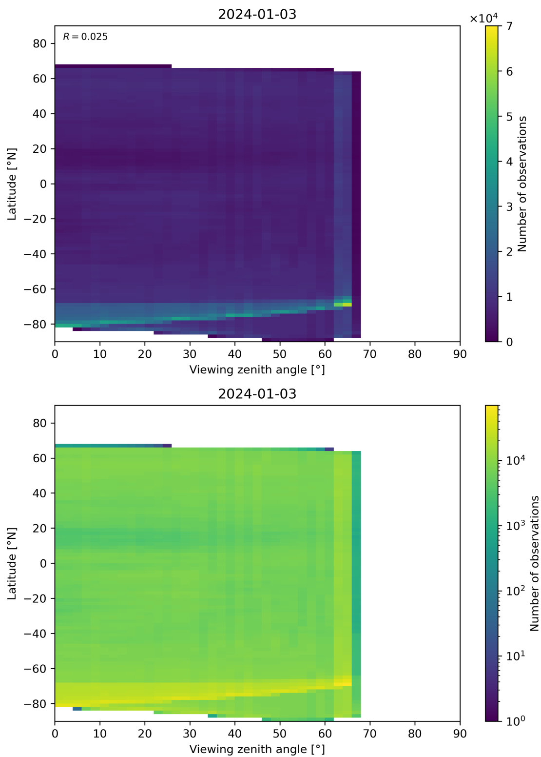
Figure 113: Scatter density plot of “Viewing zenith angle” against “Latitude” for 2024-01-02 to 2024-01-04.
