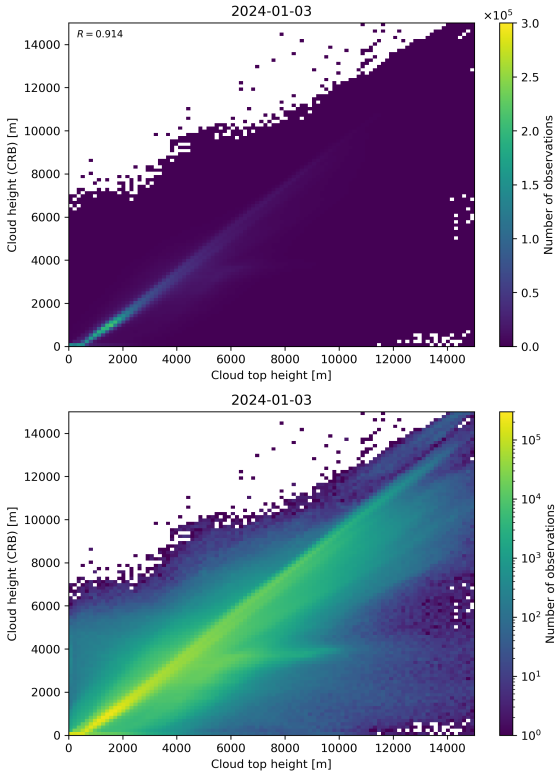
Figure 89: Scatter density plot of “Cloud top height” against “Cloud height (CRB)” for 2024-01-02 to 2024-01-04.
