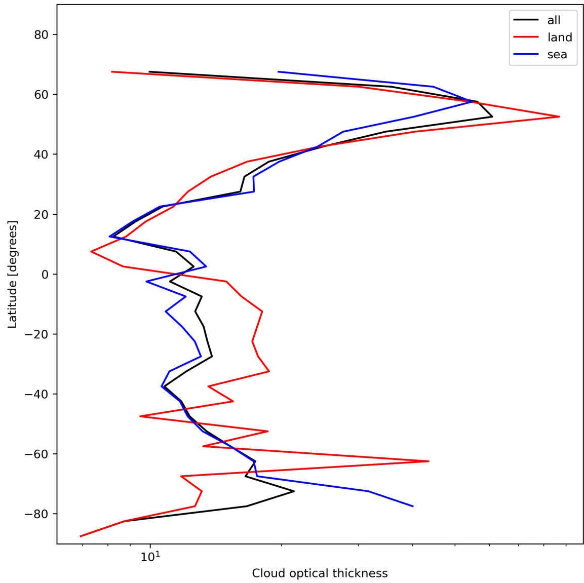
Figure 25: Zonal average of “Cloud optical thickness” for 2024-01-02 to 2024-01-04.
