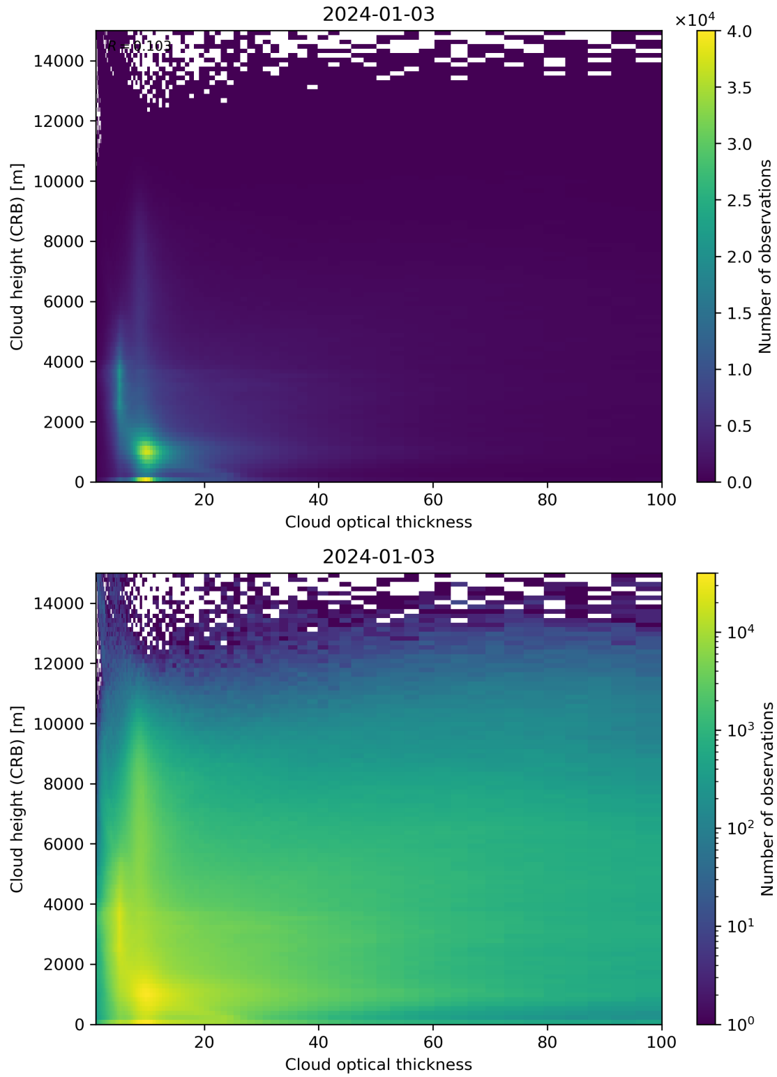
Figure 85: Scatter density plot of “Cloud optical thickness” against “Cloud height (CRB)” for 2024-01-02 to 2024-01-04.
