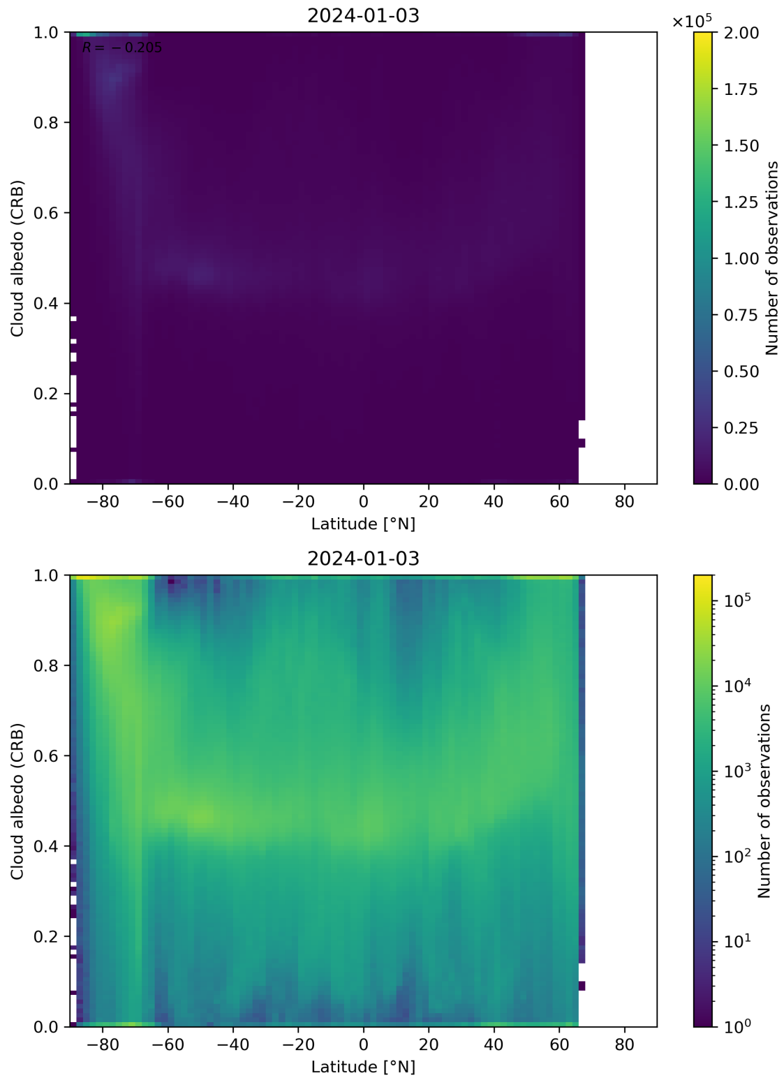
Figure 91: Scatter density plot of “Latitude” against “Cloud albedo (CRB)” for 2024-01-02 to 2024-01-04.
