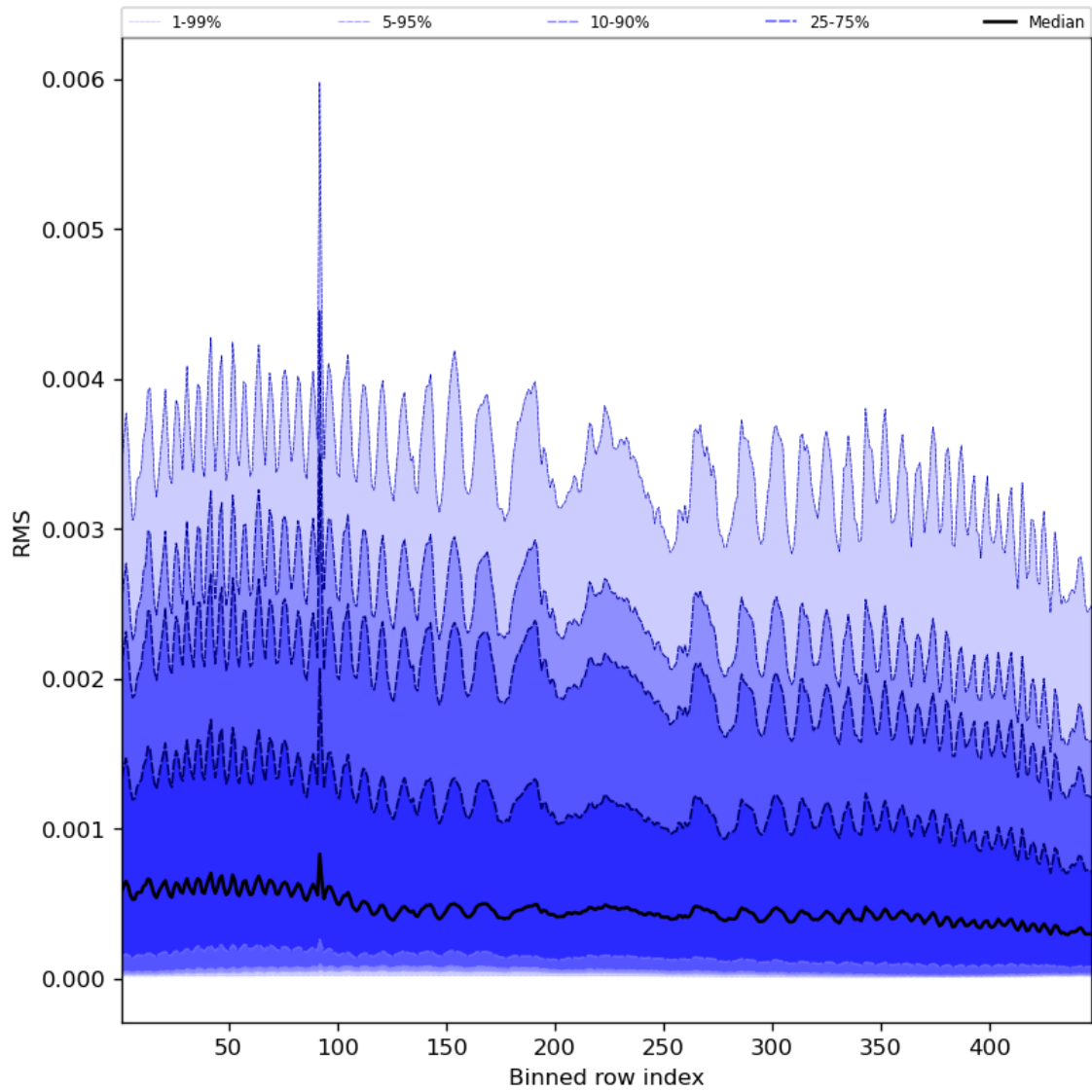
Figure 63: Along track statistics of “RMS” for 2024-01-02 to 2024-01-04
