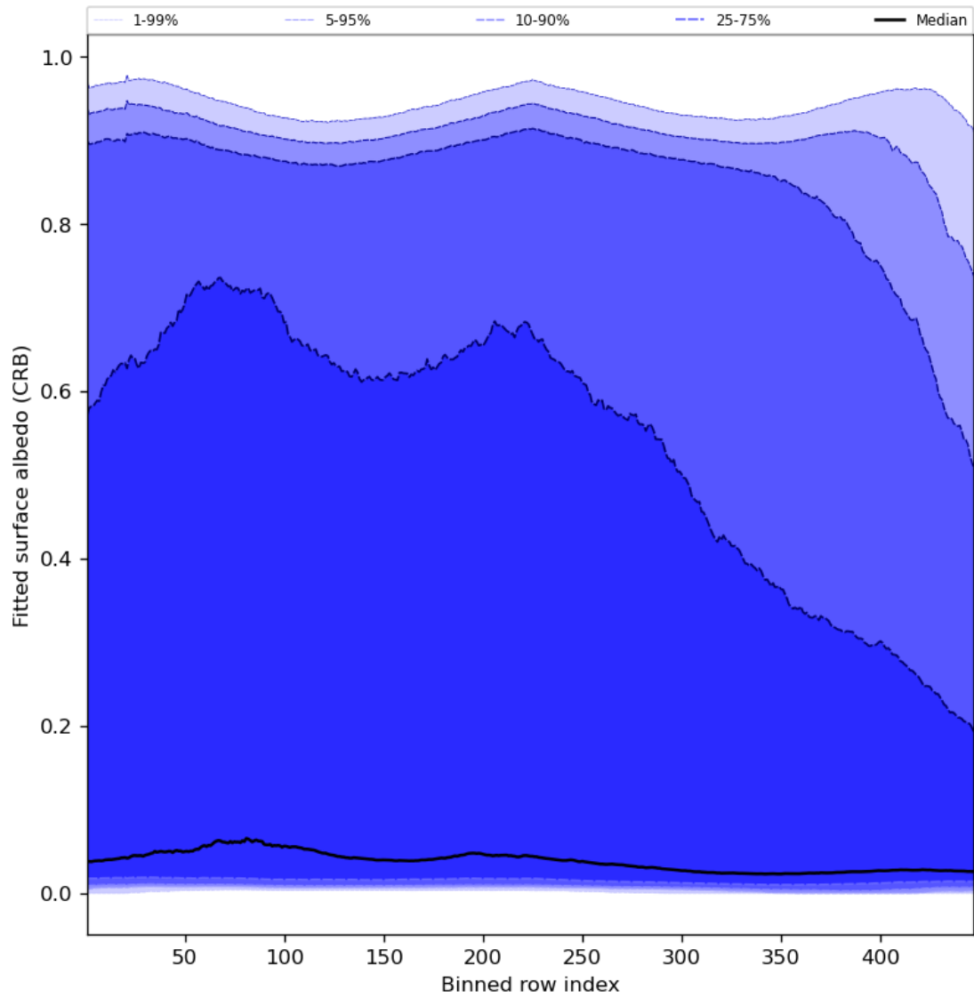
Figure 62: Along track statistics of “Fitted surface albedo (CRB)” for 2024-01-02 to 2024-01-04
