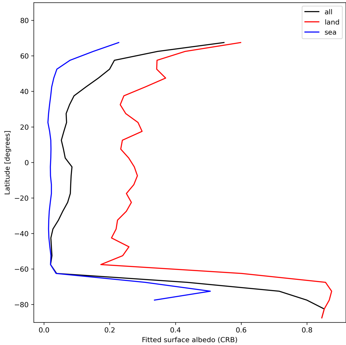
Figure 30: Zonal average of “Fitted surface albedo (CRB)” for 2024-01-02 to 2024-01-04.
