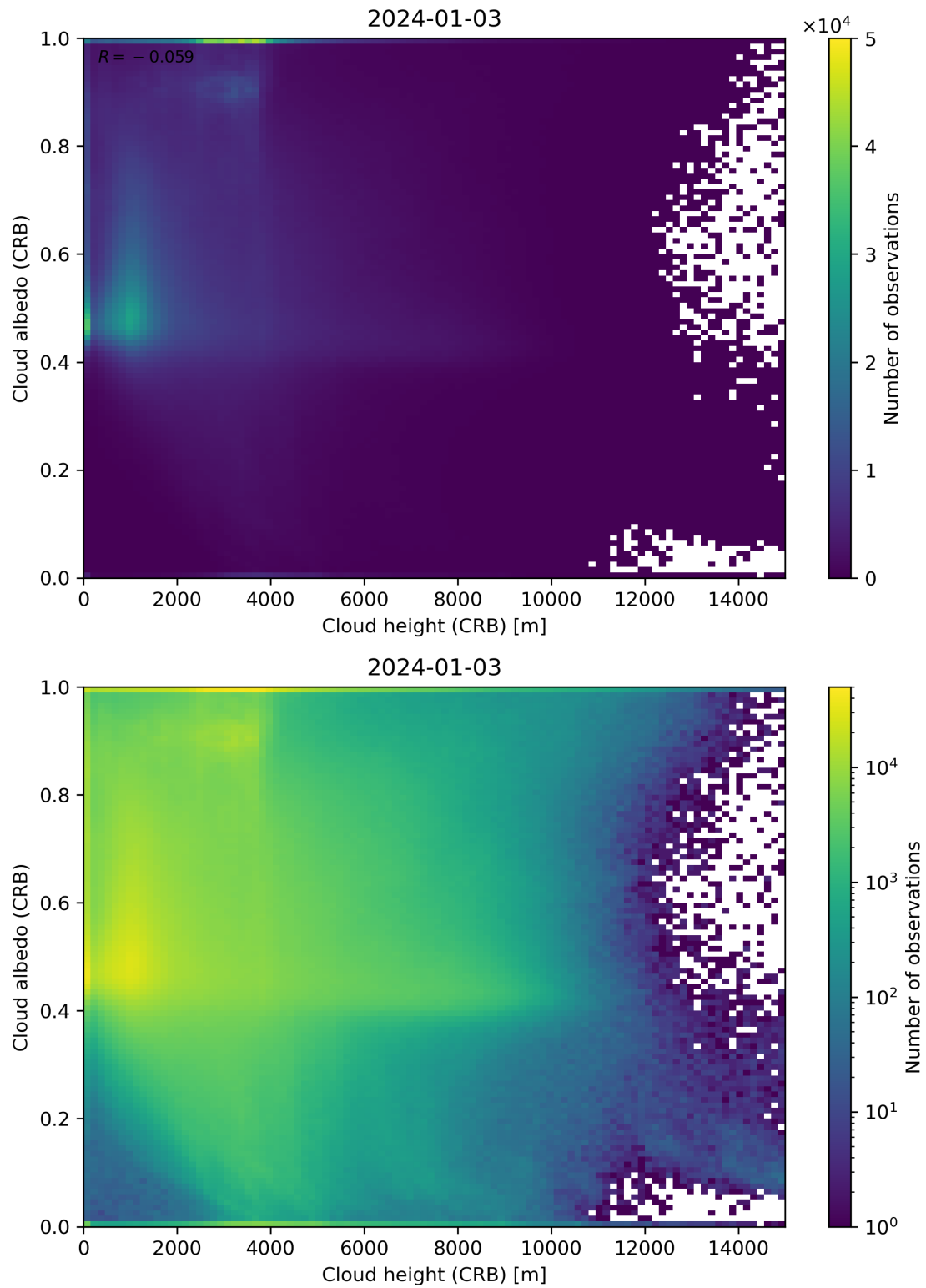
Figure 80: Scatter density plot of “Cloud height (CRB)” against “Cloud albedo (CRB)” for 2024-01-02 to 2024-01-04.
