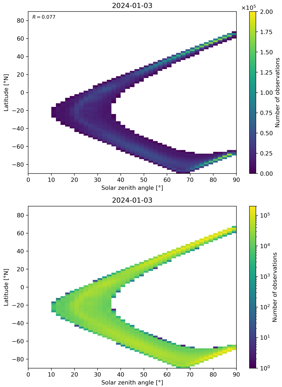
Figure 105: Scatter density plot of “Solar zenith angle” against “Latitude” for 2024-01-02 to 2024-01-04.
