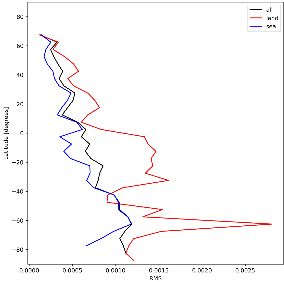
Figure 31: Zonal average of “RMS” for 2024-01-02 to 2024-01-04.
