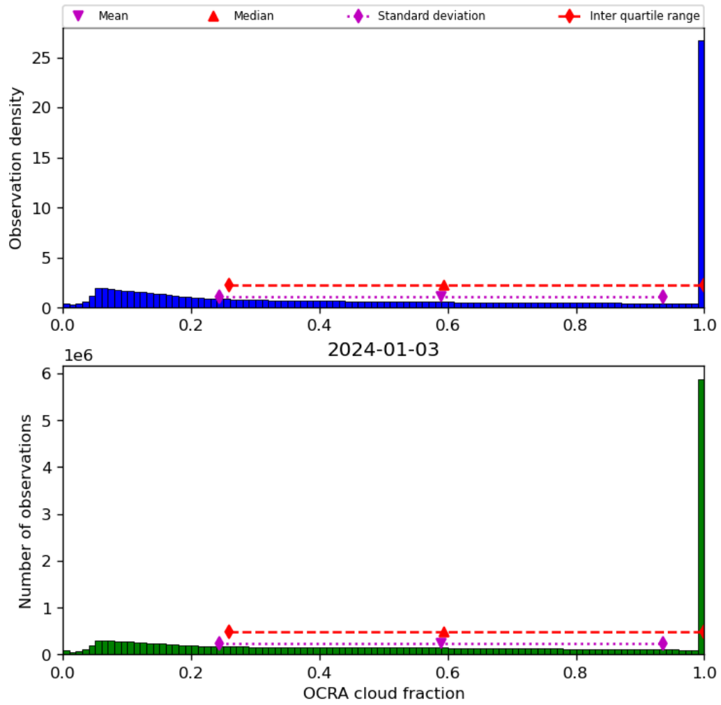
Figure 50: Histogram of “OCRA cloud fraction” for 2024-01-02 to 2024-01-04
