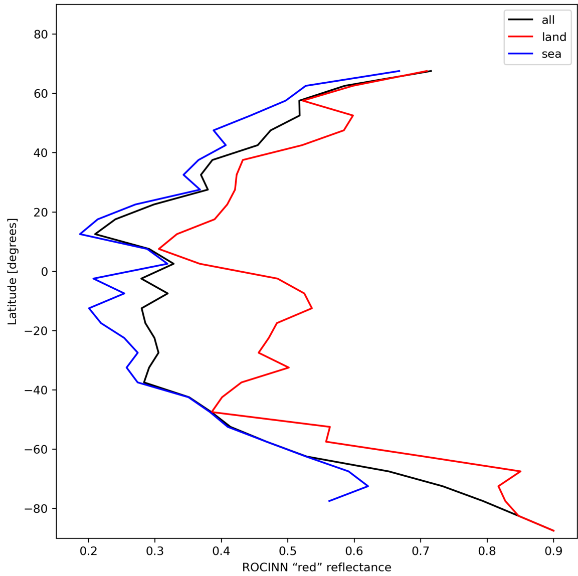
Figure 37: Zonal average of “ROCINN “red” reflectance” for 2024-01-02 to 2024-01-04.
