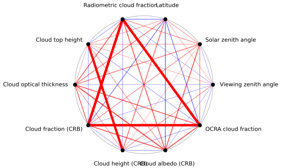
Figure 1: Map of correlation graph for 2024-01-03 to 2024-01-05.
