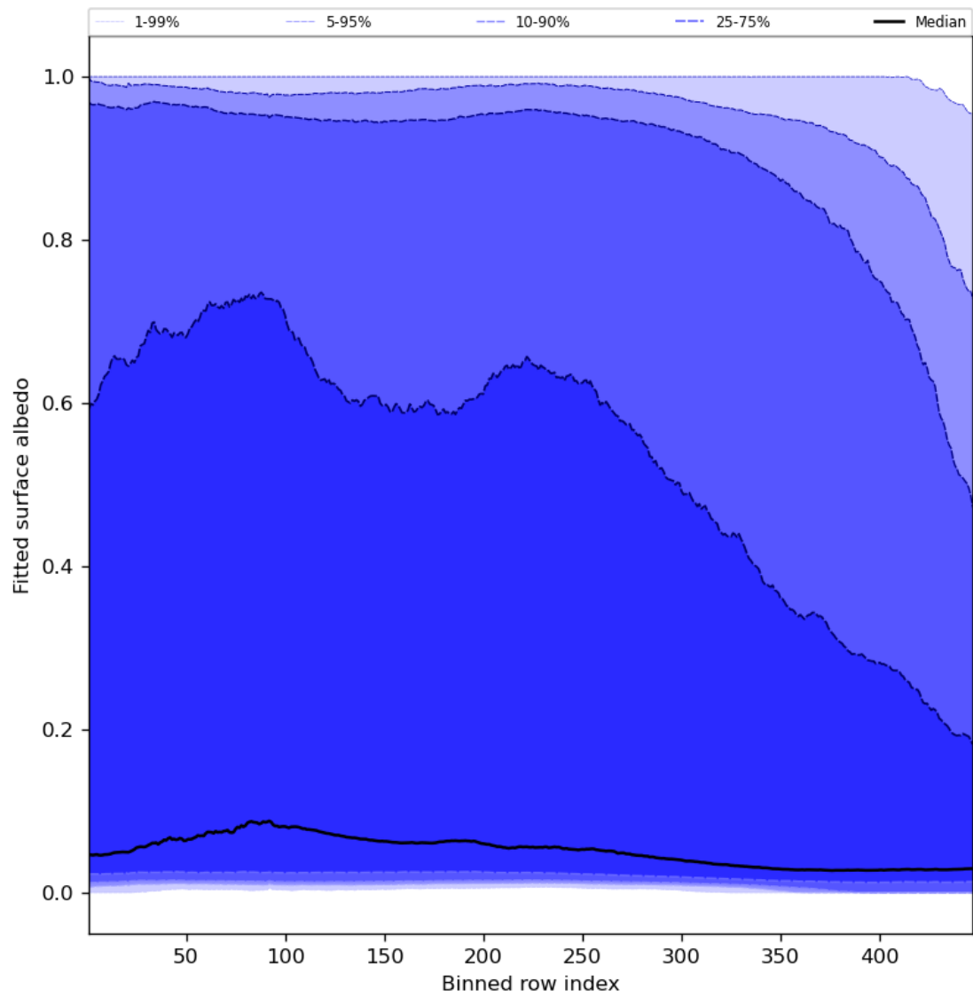
Figure 61: Along track statistics of “Fitted surface albedo” for 2024-01-03 to 2024-01-05
