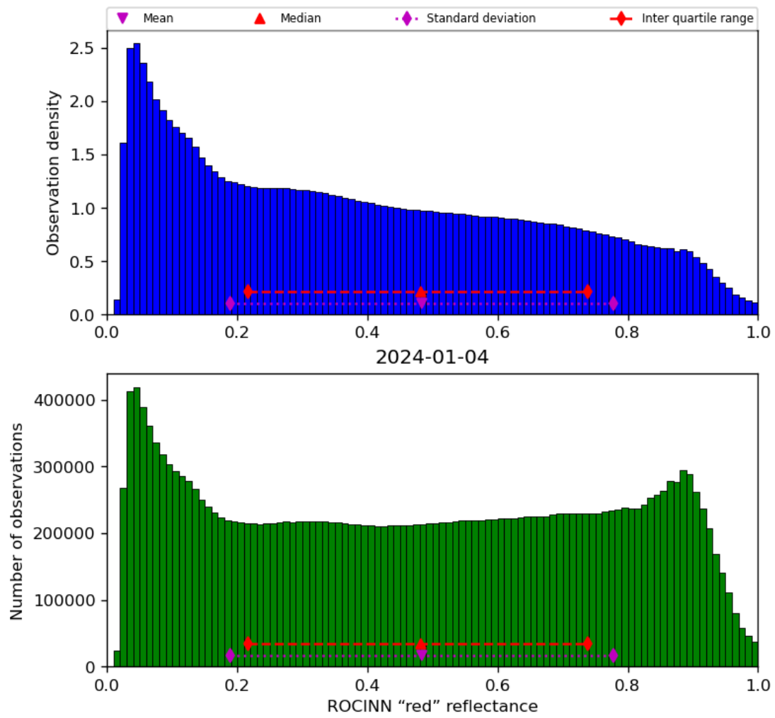
Figure 53: Histogram of "ROCINN "red" reflectance" for 2024-01-03 to 2024-01-05
