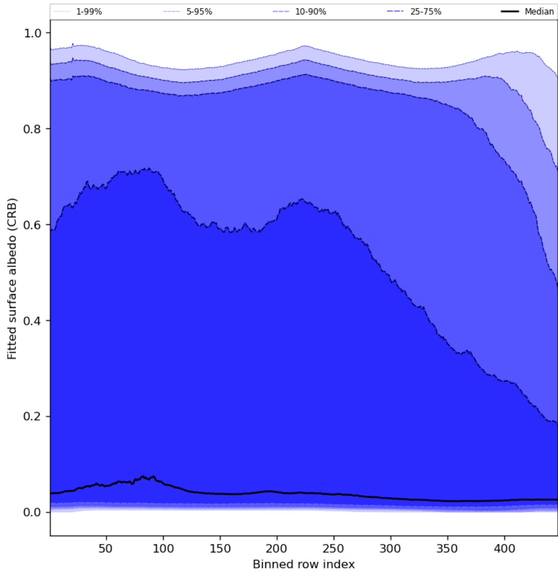
Figure 62: Along track statistics of “Fitted surface albedo (CRB)” for 2024-01-03 to 2024-01-05
