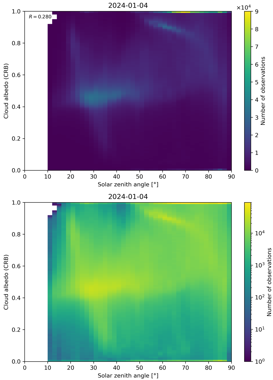
Figure 98: Scatter density plot of “Solar zenith angle” against “Cloud albedo (CRB)” for 2024-01-03 to 2024-01-05.
