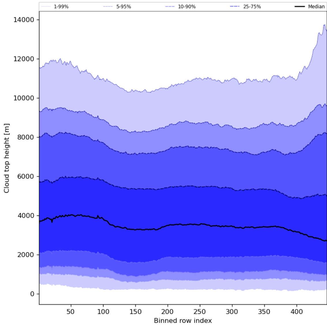
Figure 56: Along track statistics of “Cloud top height” for 2024-01-03 to 2024-01-05
