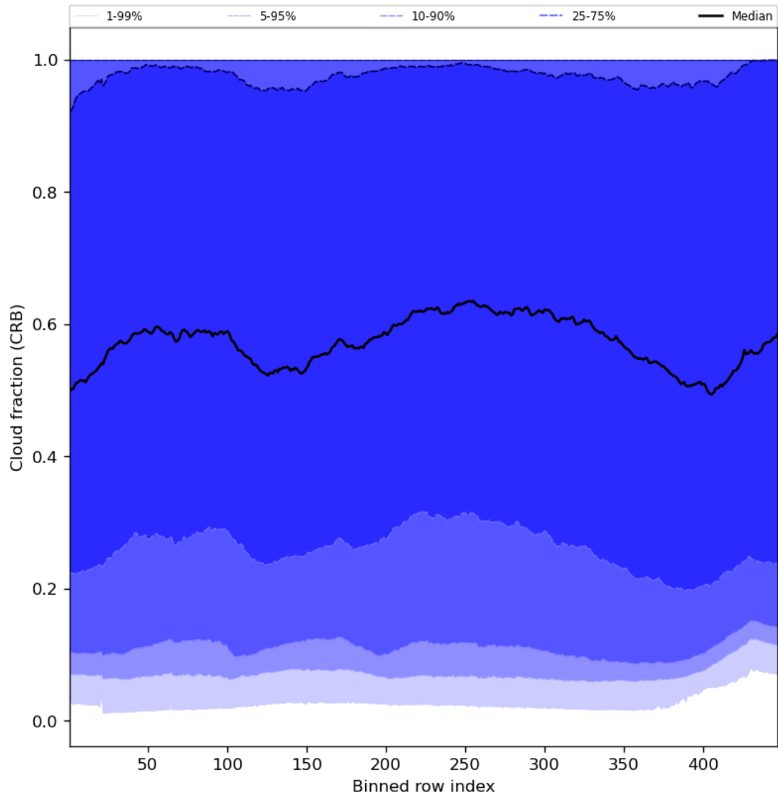
Figure 58: Along track statistics of “Cloud fraction (CRB)” for 2024-01-03 to 2024-01-05
