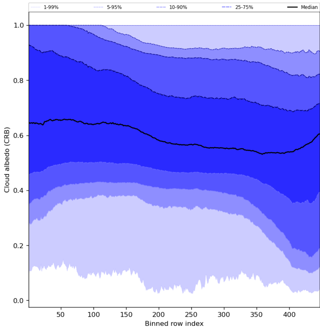
Figure 60: Along track statistics of “Cloud albedo (CRB)” for 2024-01-03 to 2024-01-05
