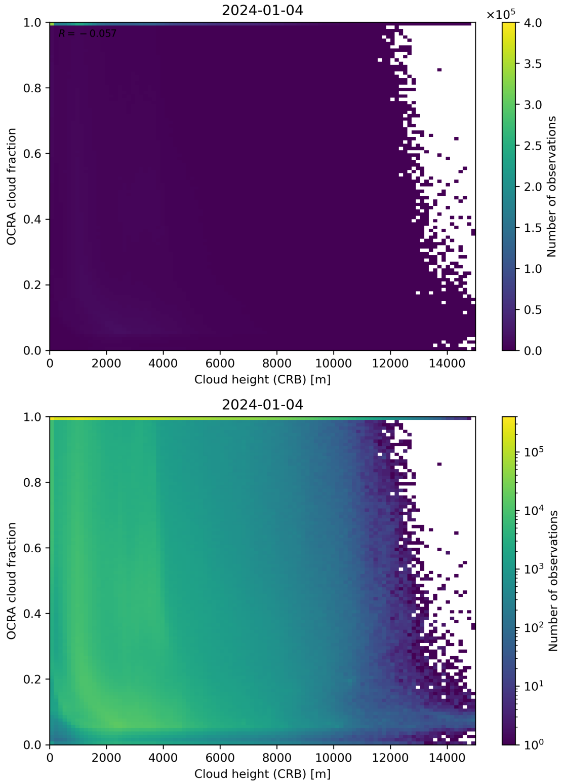
Figure 81: Scatter density plot of “Cloud height (CRB)” against “OCRA cloud fraction” for 2024-01-03 to 2024-01-05.
