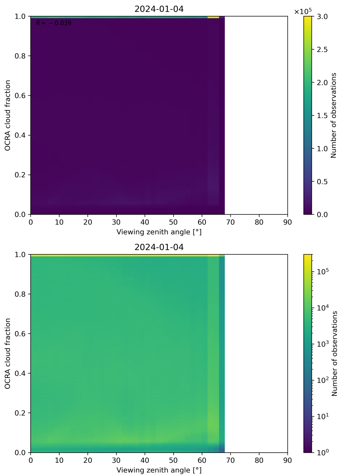
Figure 108: Scatter density plot of “Viewing zenith angle” against “OCRA cloud fraction” for 2024-01-03 to 2024-01-05.
