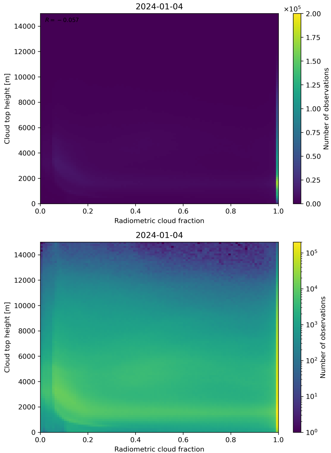
Figure 76: Scatter density plot of “Radiometric cloud fraction” against “Cloud top height” for 2024-01-03 to 2024-01-05.
