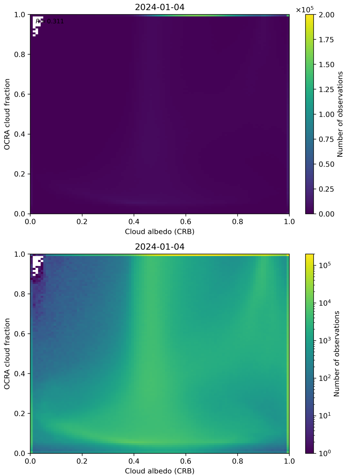
Figure 70: Scatter density plot of “Cloud albedo (CRB)” against “OCRA cloud fraction” for 2024-01-03 to 2024-01-05.
