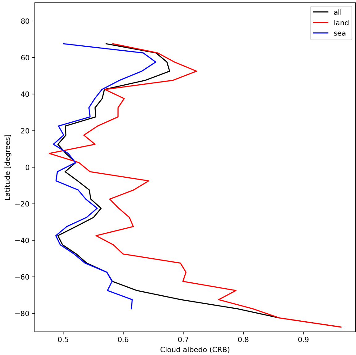
Figure 28: Zonal average of “Cloud albedo (CRB)” for 2024-01-03 to 2024-01-05.
