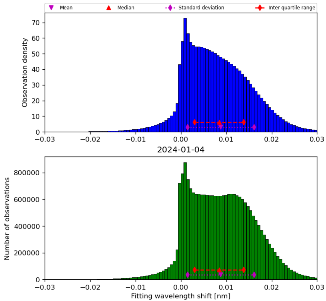
Figure 49: Histogram of “Fitting wavelength shift” for 2024-01-03 to 2024-01-05
