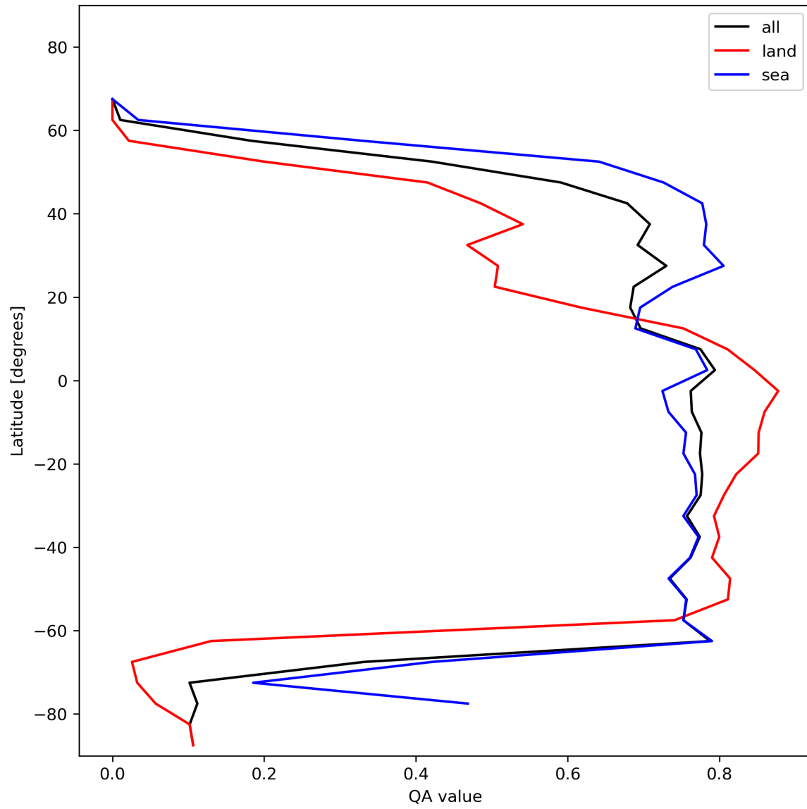
Figure 22: Zonal average of “QA value” for 2024-01-03 to 2024-01-05.
