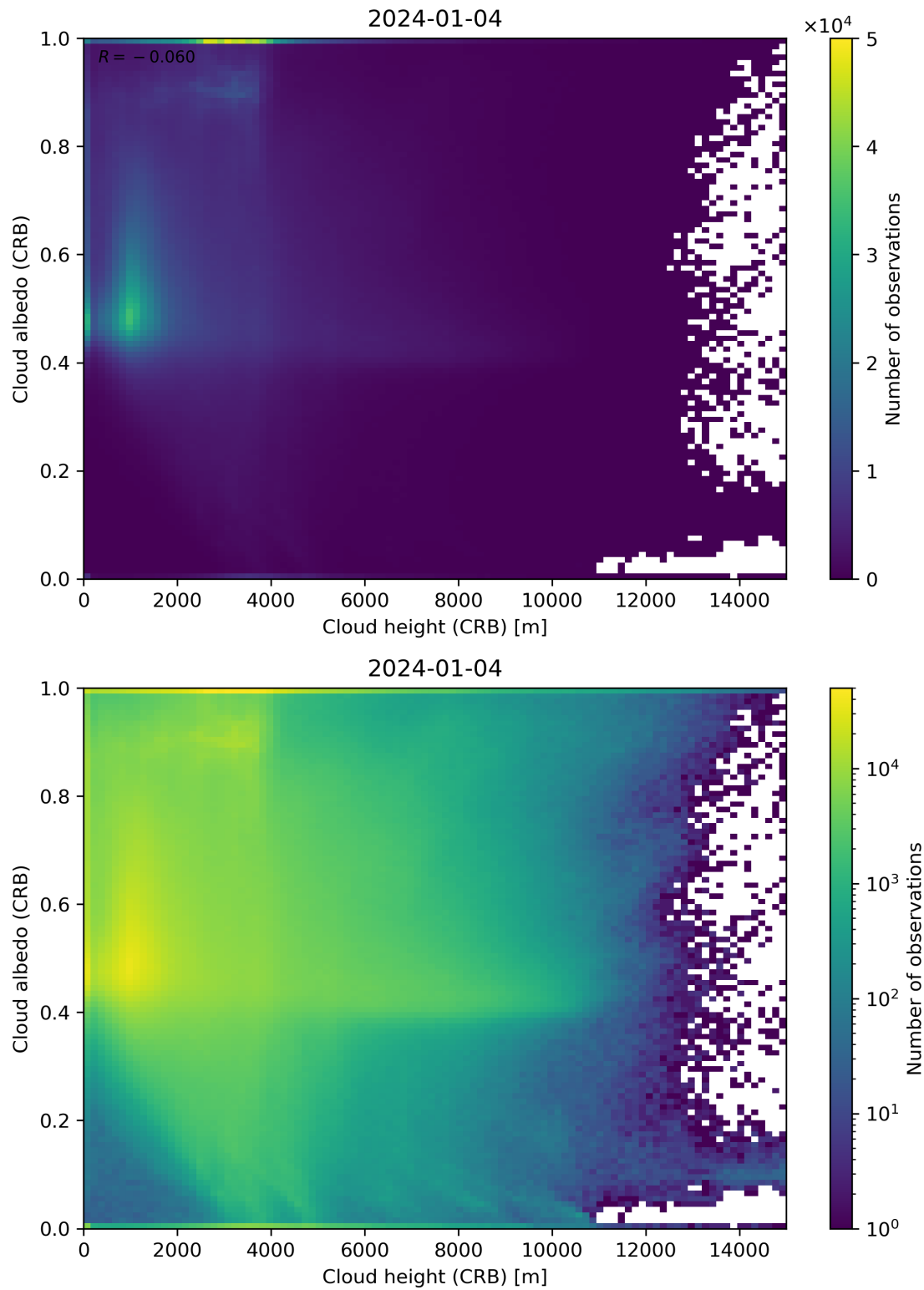
Figure 80: Scatter density plot of “Cloud height (CRB)” against “Cloud albedo (CRB)” for 2024-01-03 to 2024-01-05.
