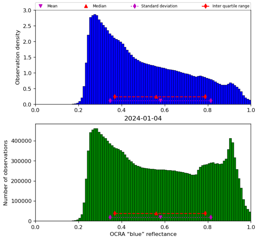
Figure 51: Histogram of “OCRA “blue” reflectance” for 2024-01-03 to 2024-01-05
