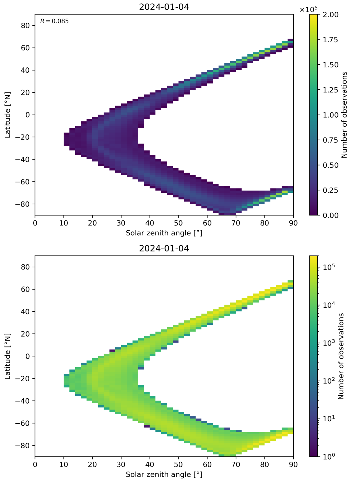
Figure 105: Scatter density plot of “Solar zenith angle” against “Latitude” for 2024-01-03 to 2024-01-05.
