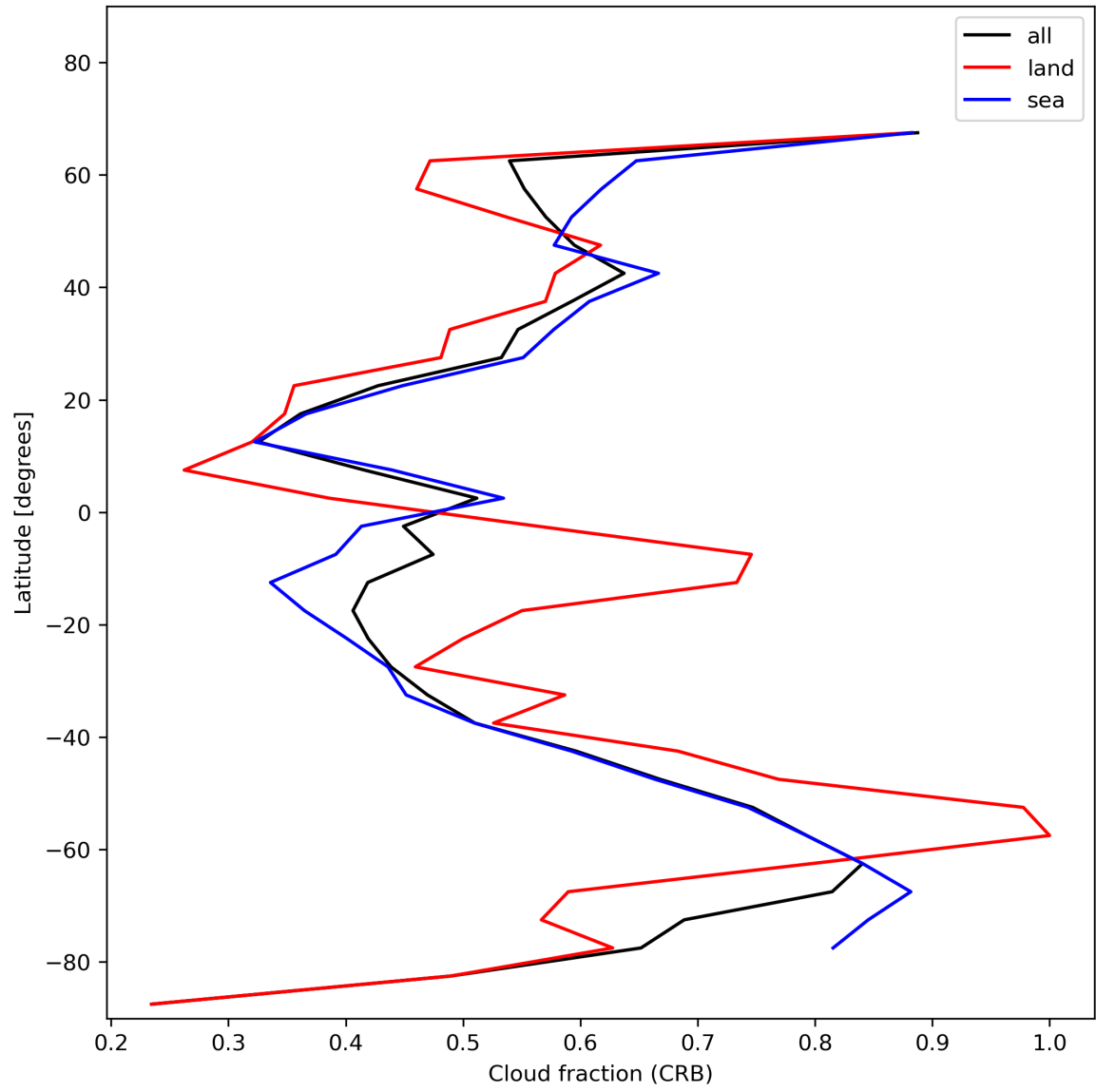
Figure 26: Zonal average of “Cloud fraction (CRB)” for 2024-01-03 to 2024-01-05.
