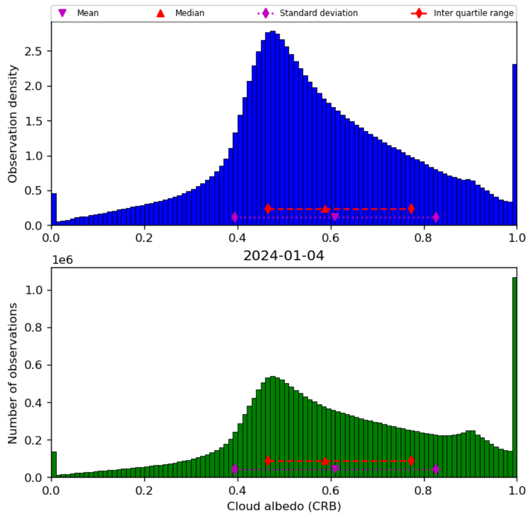
Figure 44: Histogram of “Cloud albedo (CRB)” for 2024-01-03 to 2024-01-05
