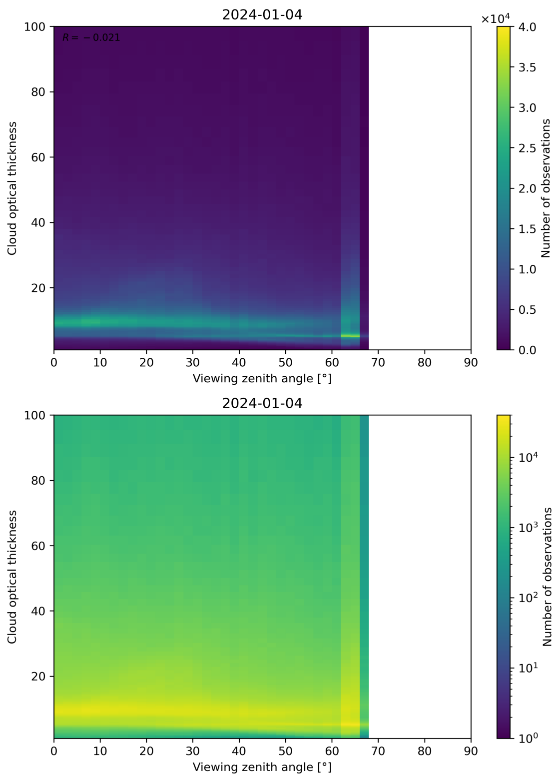
Figure 111: Scatter density plot of “Viewing zenith angle” against “Cloud optical thickness” for 2024-01-03 to 2024-01-05.
