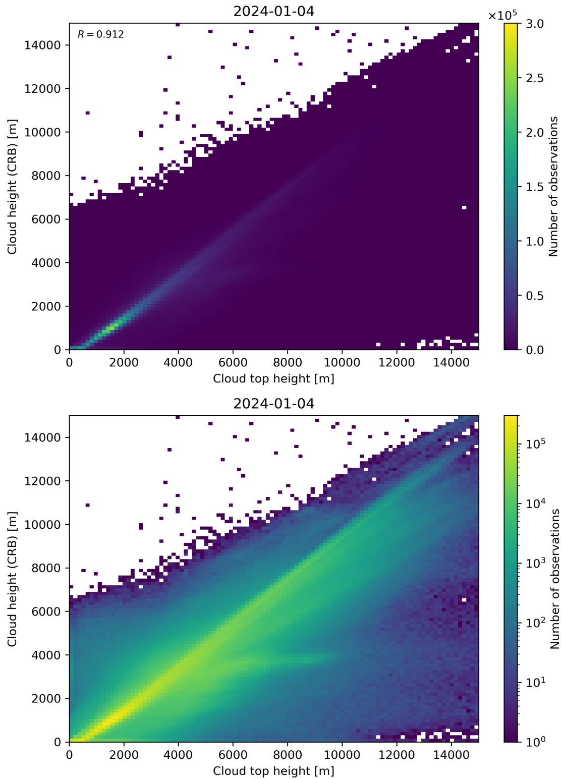
Figure 89: Scatter density plot of “Cloud top height” against “Cloud height (CRB)” for 2024-01-03 to 2024-01-05.
