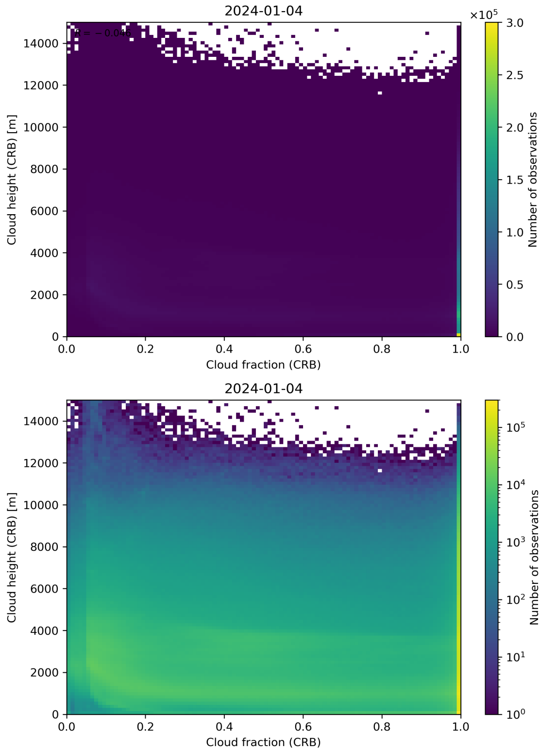
Figure 79: Scatter density plot of “Cloud fraction (CRB)” against “Cloud height (CRB)” for 2024-01-03 to 2024-01-05.
