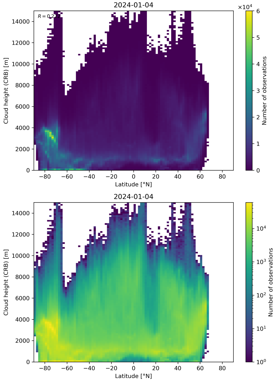
Figure 95: Scatter density plot of “Latitude” against “Cloud height (CRB)” for 2024-01-03 to 2024-01-05.
