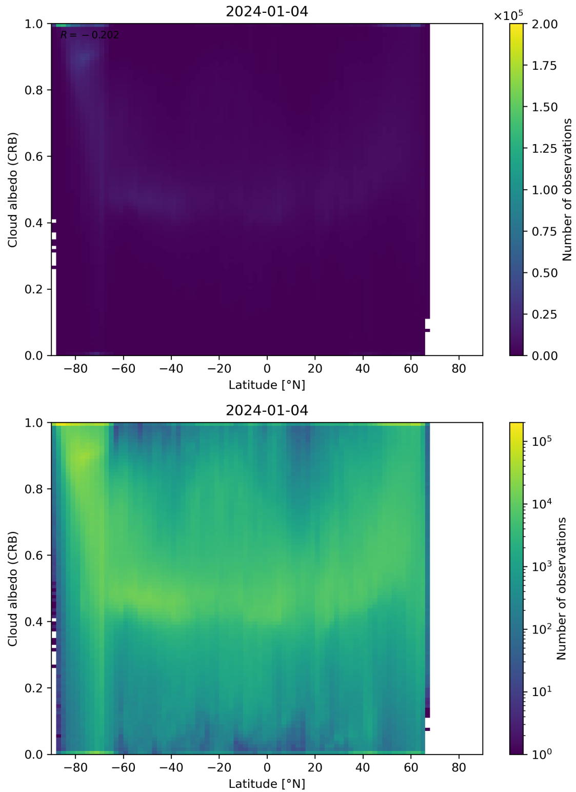
Figure 91: Scatter density plot of “Latitude” against “Cloud albedo (CRB)” for 2024-01-03 to 2024-01-05.
