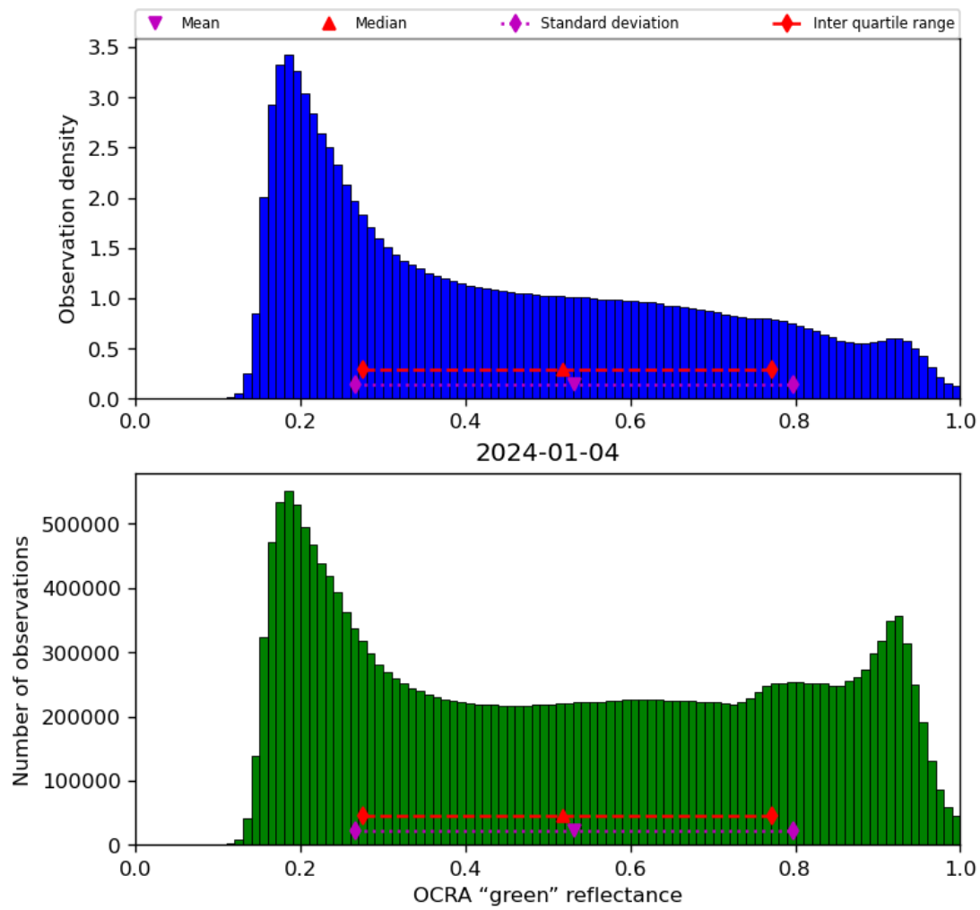
Figure 52: Histogram of “OCRA “green” reflectance” for 2024-01-03 to 2024-01-05
