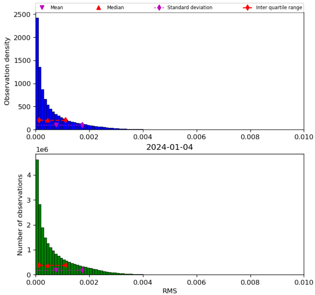
Figure 47: Histogram of “RMS” for 2024-01-03 to 2024-01-05
