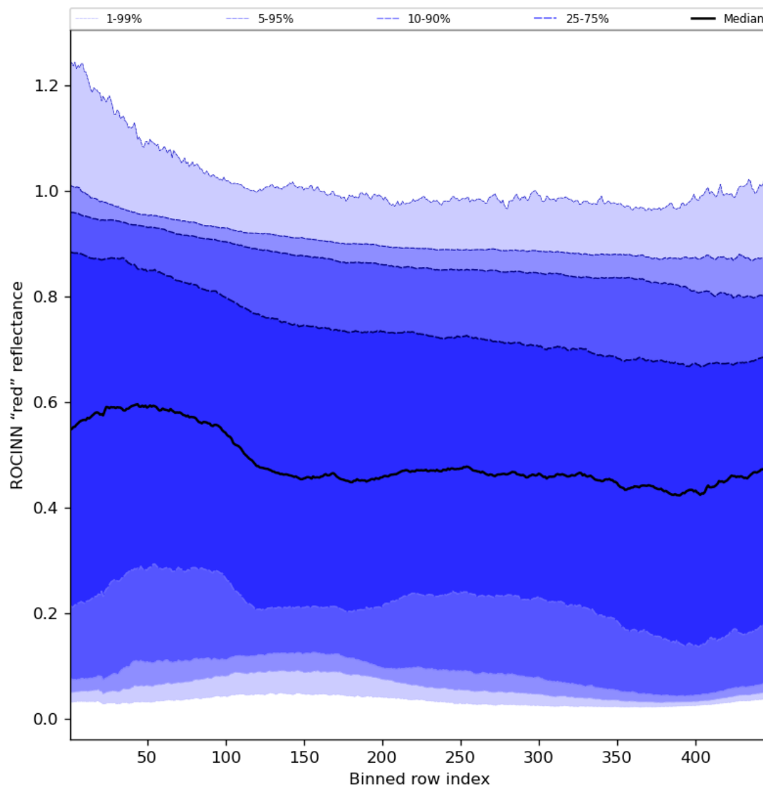
Figure 69: Along track statistics of “ROCINN “red” reflectance” for 2024-01-03 to 2024-01-05
