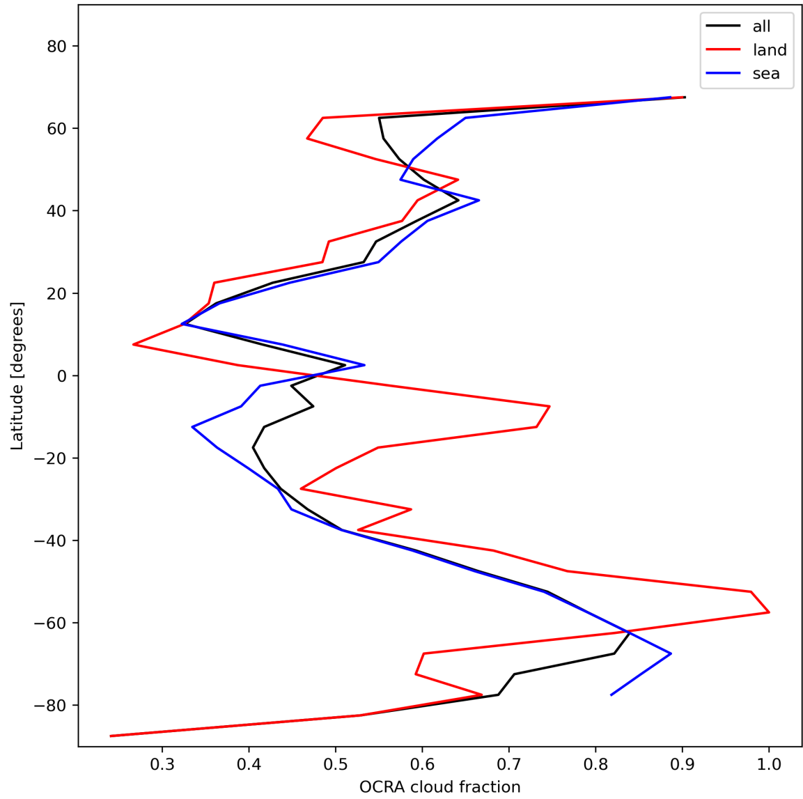
Figure 34: Zonal average of “OCRA cloud fraction” for 2024-01-03 to 2024-01-05.
