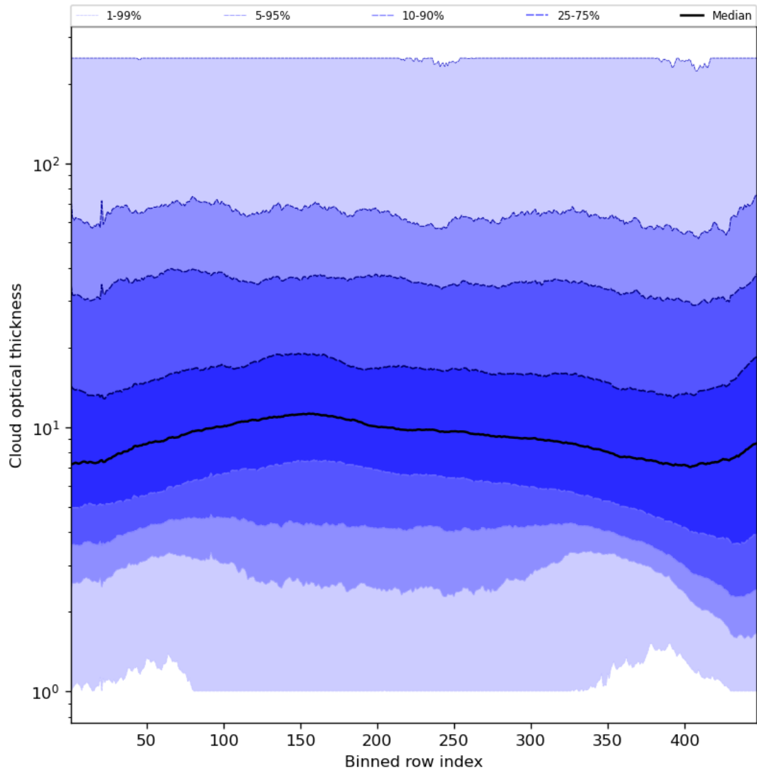
Figure 57: Along track statistics of “Cloud optical thickness” for 2024-01-03 to 2024-01-05
