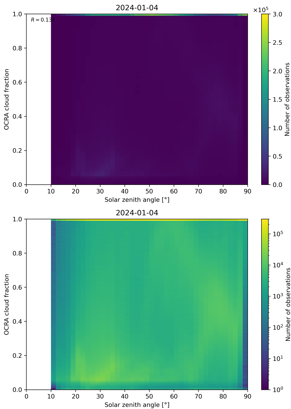
Figure 100: Scatter density plot of “Solar zenith angle” against “OCRA cloud fraction” for 2024-01-03 to 2024-01-05.
