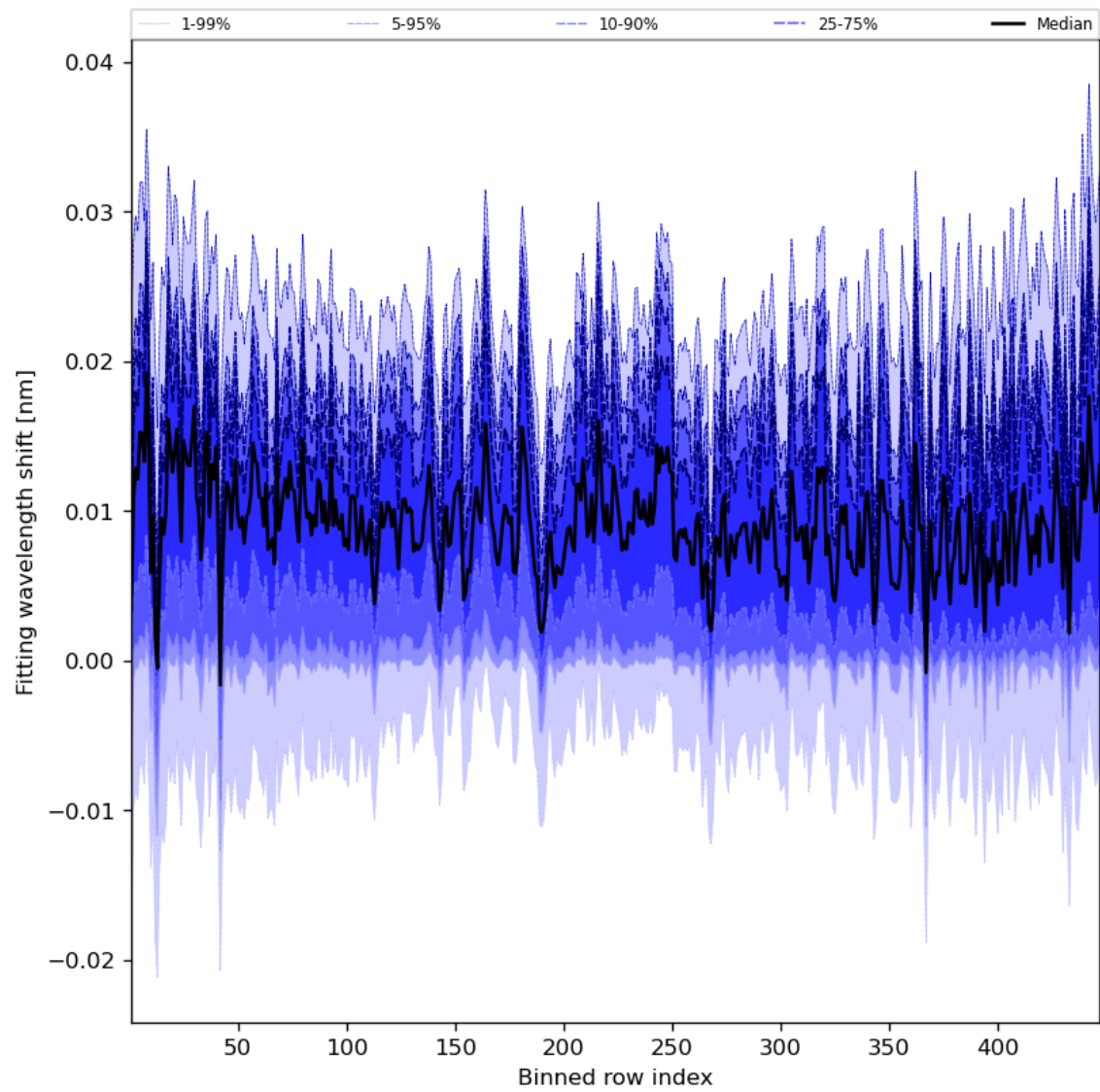
Figure 65: Along track statistics of “Fitting wavelength shift” for 2024-01-03 to 2024-01-05
