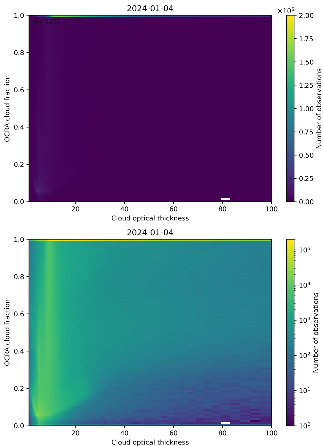
Figure 83: Scatter density plot of “Cloud optical thickness” against “OCRA cloud fraction” for 2024-01-03 to 2024-01-05.
