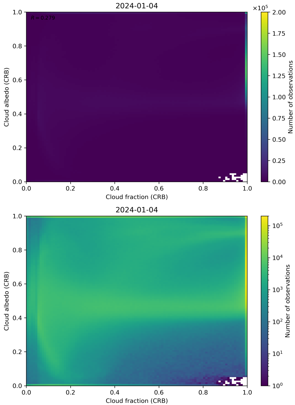
Figure 77: Scatter density plot of “Cloud fraction (CRB)” against “Cloud albedo (CRB)” for 2024-01-03 to 2024-01-05.
