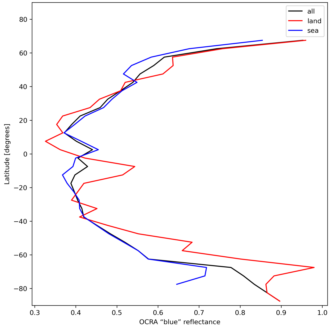
Figure 35: Zonal average of “OCRA “blue” reflectance” for 2024-01-03 to 2024-01-05.
