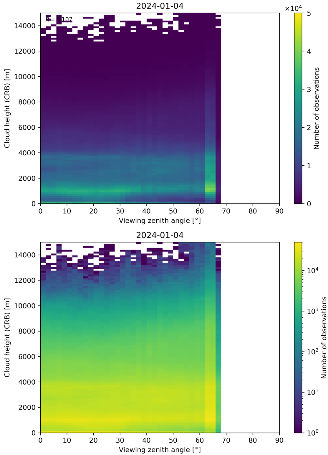
Figure 110: Scatter density plot of “Viewing zenith angle” against “Cloud height (CRB)” for 2024-01-03 to 2024-01-05.
