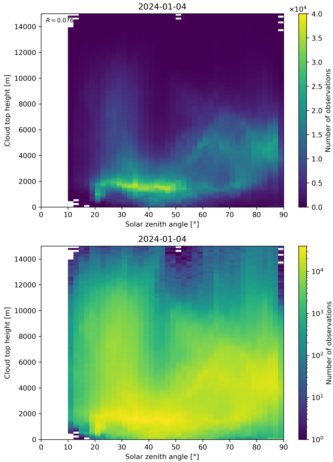
Figure 104: Scatter density plot of “Solar zenith angle” against “Cloud top height” for 2024-01-03 to 2024-01-05.
