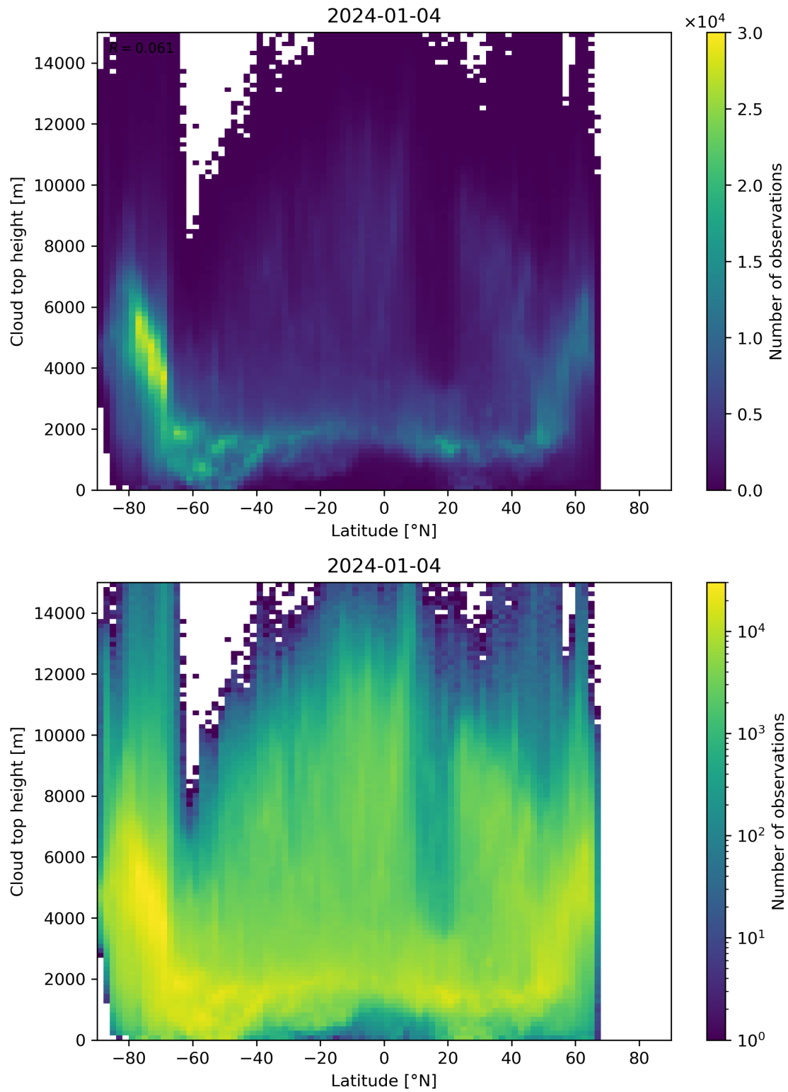
Figure 97: Scatter density plot of “Latitude” against “Cloud top height” for 2024-01-03 to 2024-01-05.
