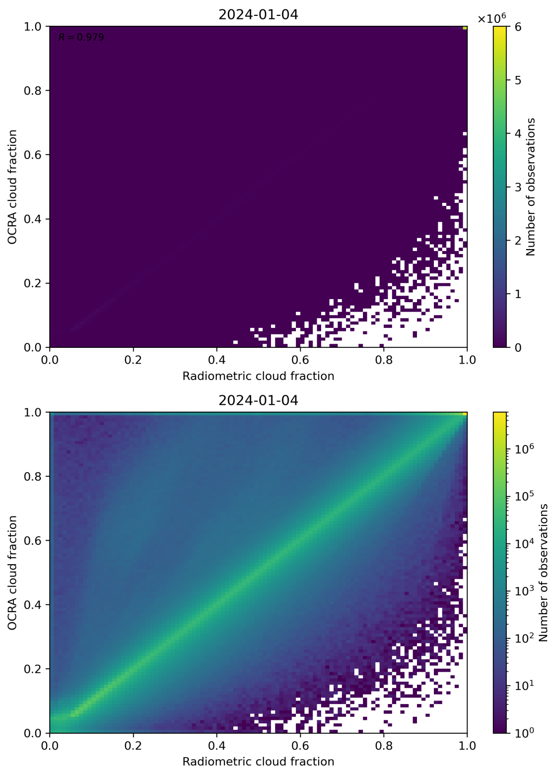
Figure 72: Scatter density plot of “Radiometric cloud fraction” against “OCRA cloud fraction” for 2024-01-03 to 2024-01-05.
