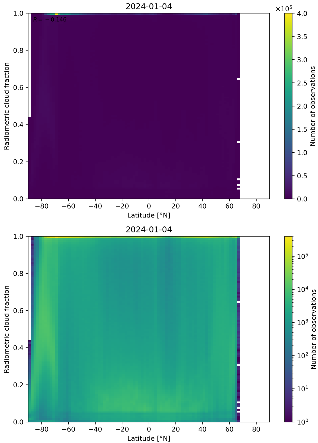
Figure 92: Scatter density plot of “Latitude” against “Radiometric cloud fraction” for 2024-01-03 to 2024-01-05.
