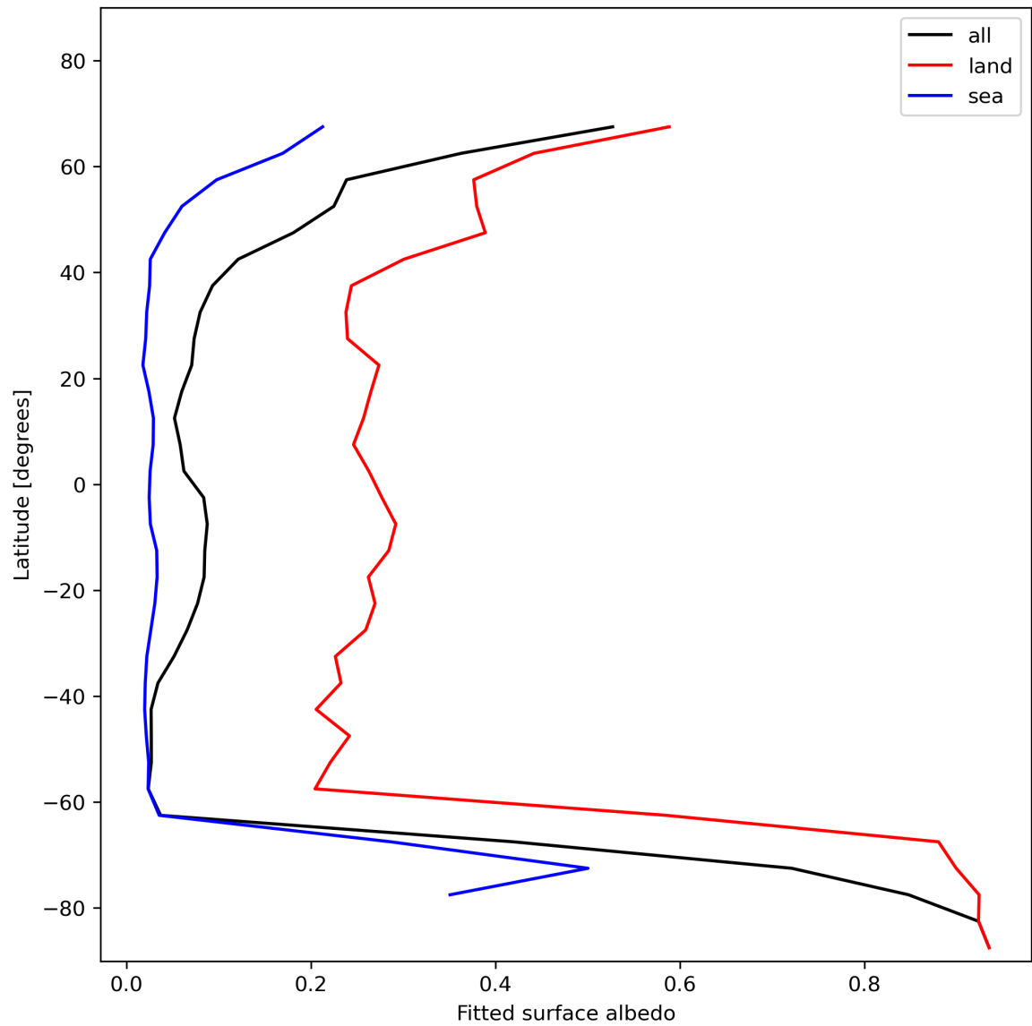
Figure 29: Zonal average of “Fitted surface albedo” for 2024-01-03 to 2024-01-05.
