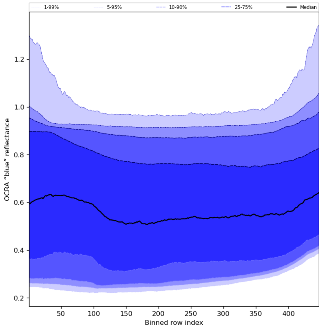
Figure 67: Along track statistics of “OCRA “blue” reflectance” for 2024-01-03 to 2024-01-05
