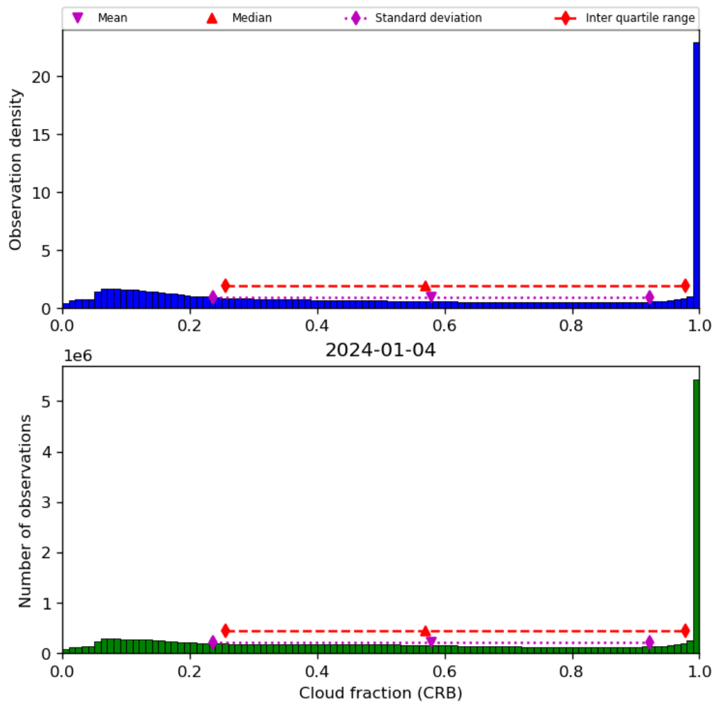
Figure 42: Histogram of “Cloud fraction (CRB)” for 2024-01-03 to 2024-01-05
