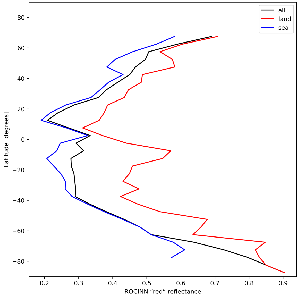
Figure 37: Zonal average of “ROCINN “red” reflectance” for 2024-01-03 to 2024-01-05.
