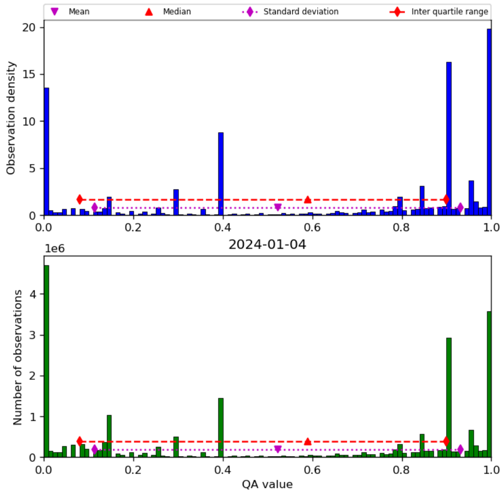
Figure 38: Histogram of “QA value” for 2024-01-03 to 2024-01-05
