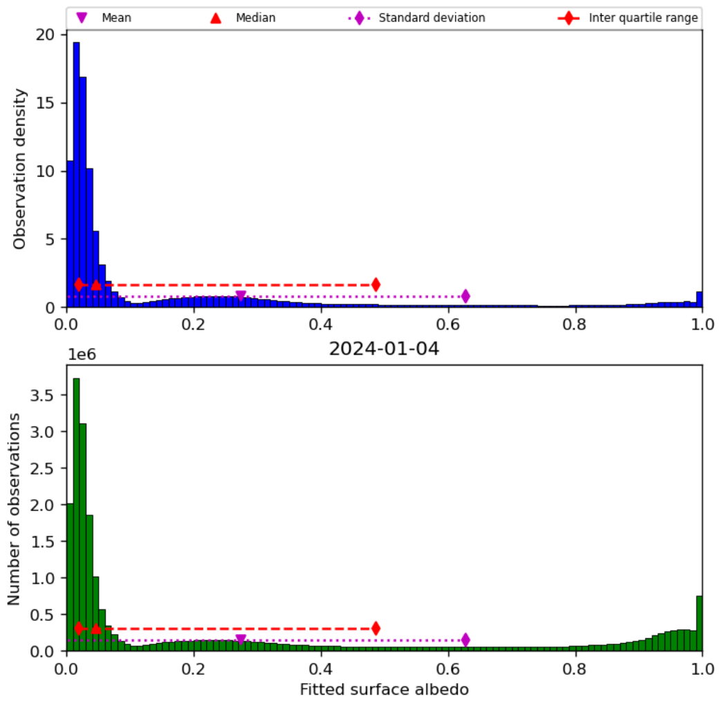
Figure 45: Histogram of “Fitted surface albedo” for 2024-01-03 to 2024-01-05
