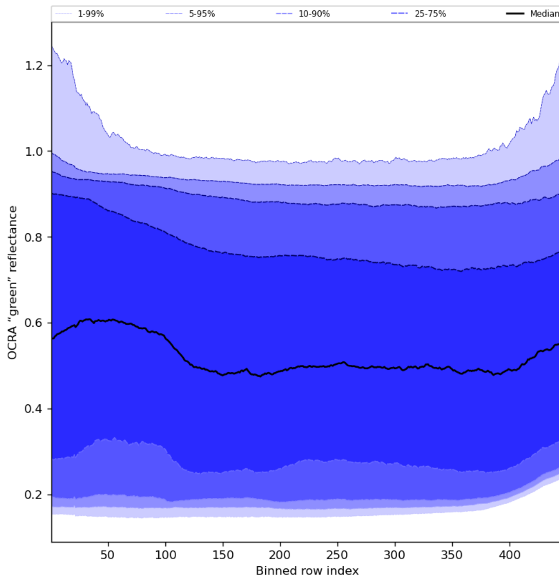
Figure 68: Along track statistics of “OCRA “green” reflectance” for 2024-01-03 to 2024-01-05
