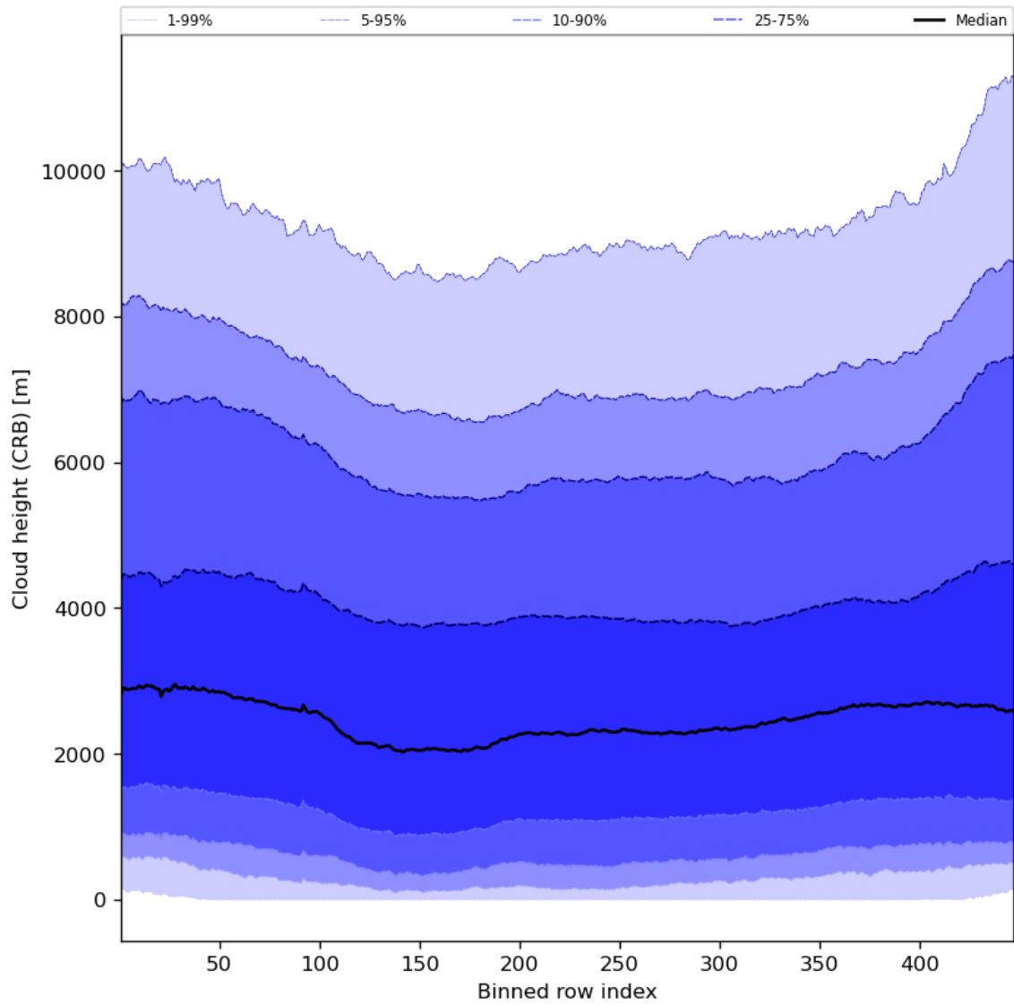
Figure 59: Along track statistics of “Cloud height (CRB)” for 2024-01-03 to 2024-01-05
