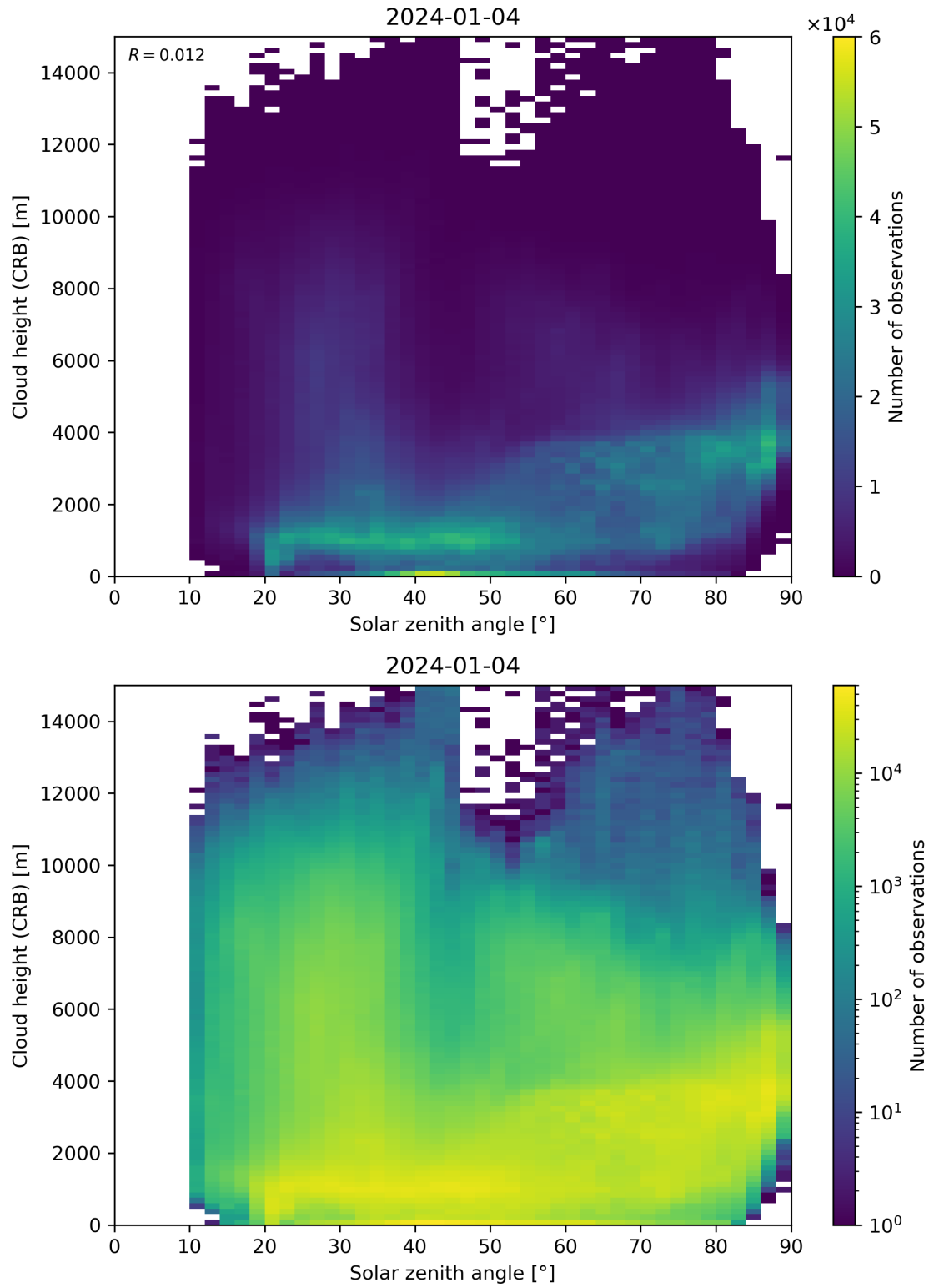
Figure 102: Scatter density plot of “Solar zenith angle” against “Cloud height (CRB)” for 2024-01-03 to 2024-01-05.
