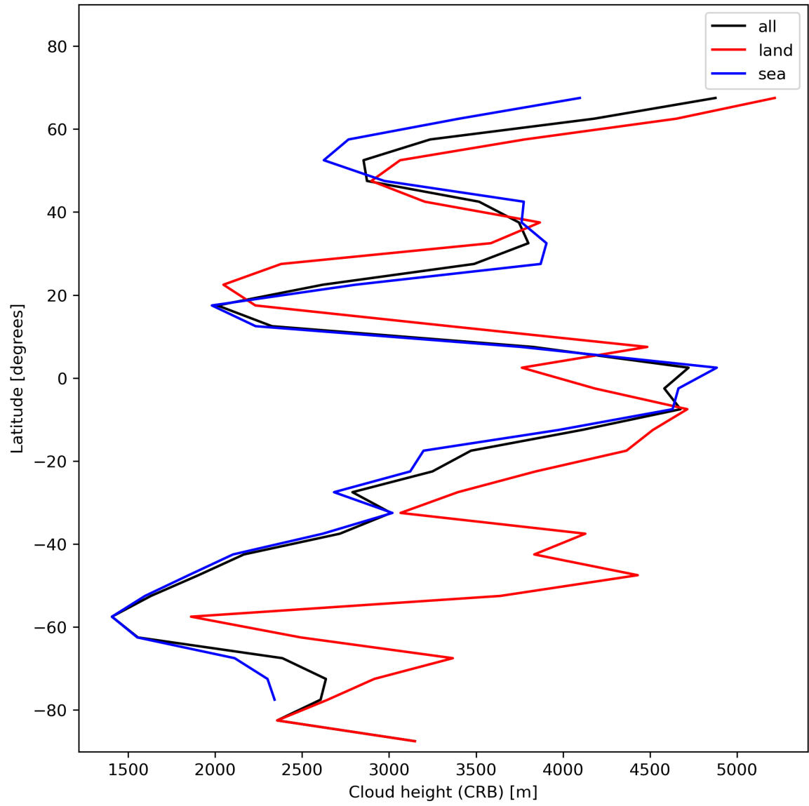
Figure 27: Zonal average of “Cloud height (CRB)” for 2024-01-03 to 2024-01-05.
