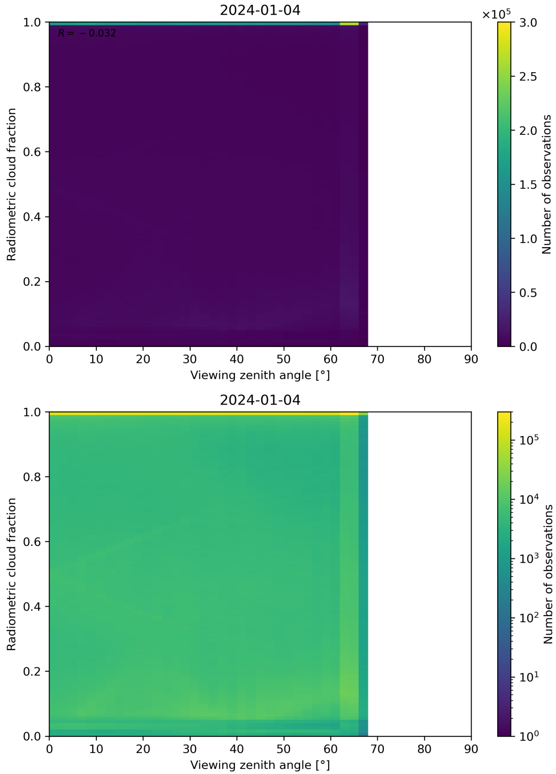
Figure 107: Scatter density plot of “Viewing zenith angle” against “Radiometric cloud fraction” for 2024-01-03 to 2024-01-05.
