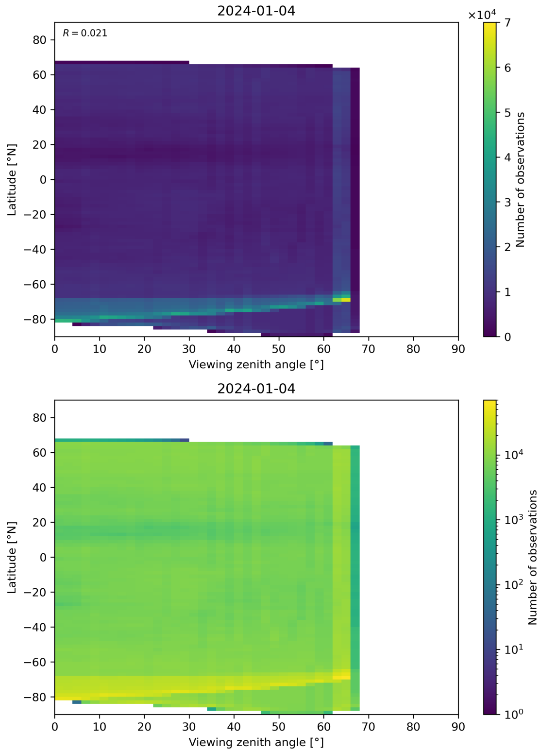
Figure 113: Scatter density plot of “Viewing zenith angle” against “Latitude” for 2024-01-03 to 2024-01-05.
