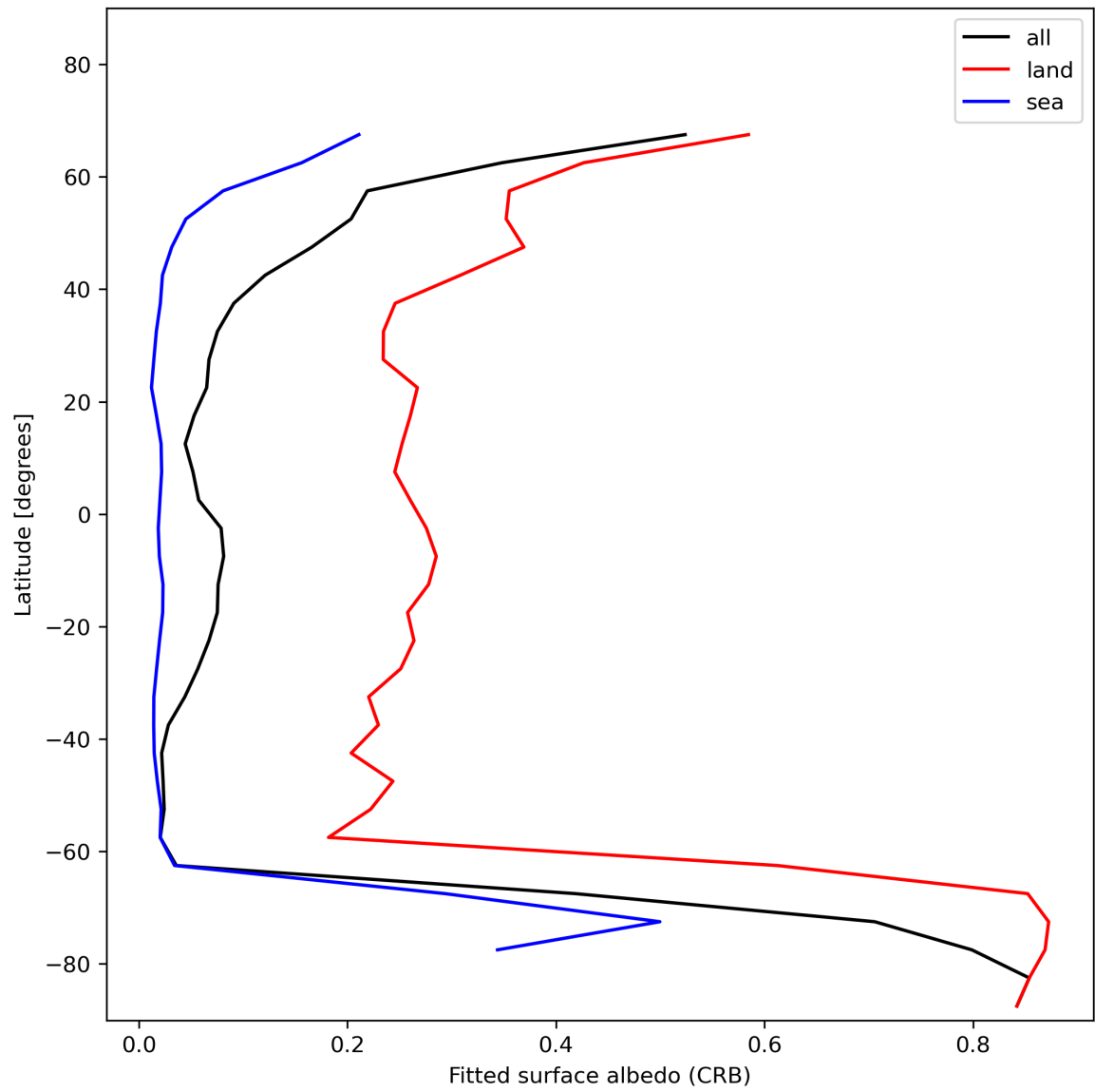
Figure 30: Zonal average of “Fitted surface albedo (CRB)” for 2024-01-03 to 2024-01-05.
