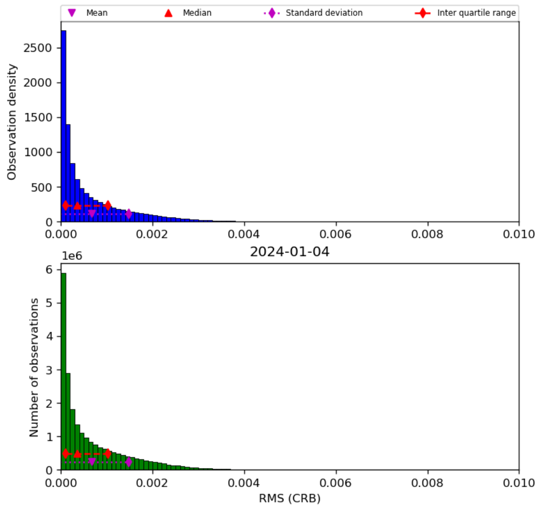
Figure 48: Histogram of “RMS (CRB)” for 2024-01-03 to 2024-01-05
