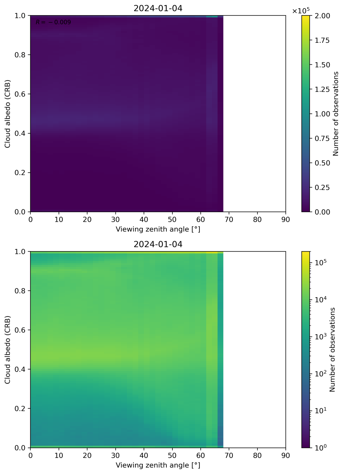
Figure 106: Scatter density plot of “Viewing zenith angle” against “Cloud albedo (CRB)” for 2024-01-03 to 2024-01-05.
