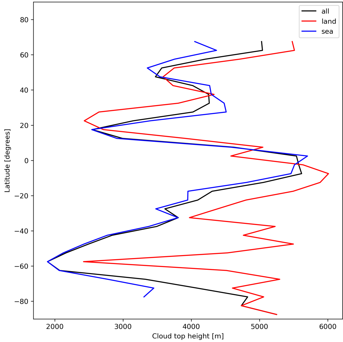
Figure 24: Zonal average of “Cloud top height” for 2024-01-03 to 2024-01-05.
