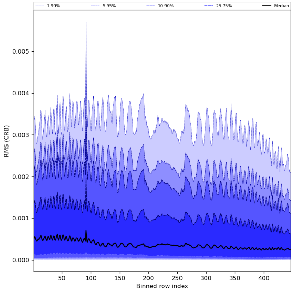
Figure 64: Along track statistics of “RMS (CRB)” for 2024-01-03 to 2024-01-05
