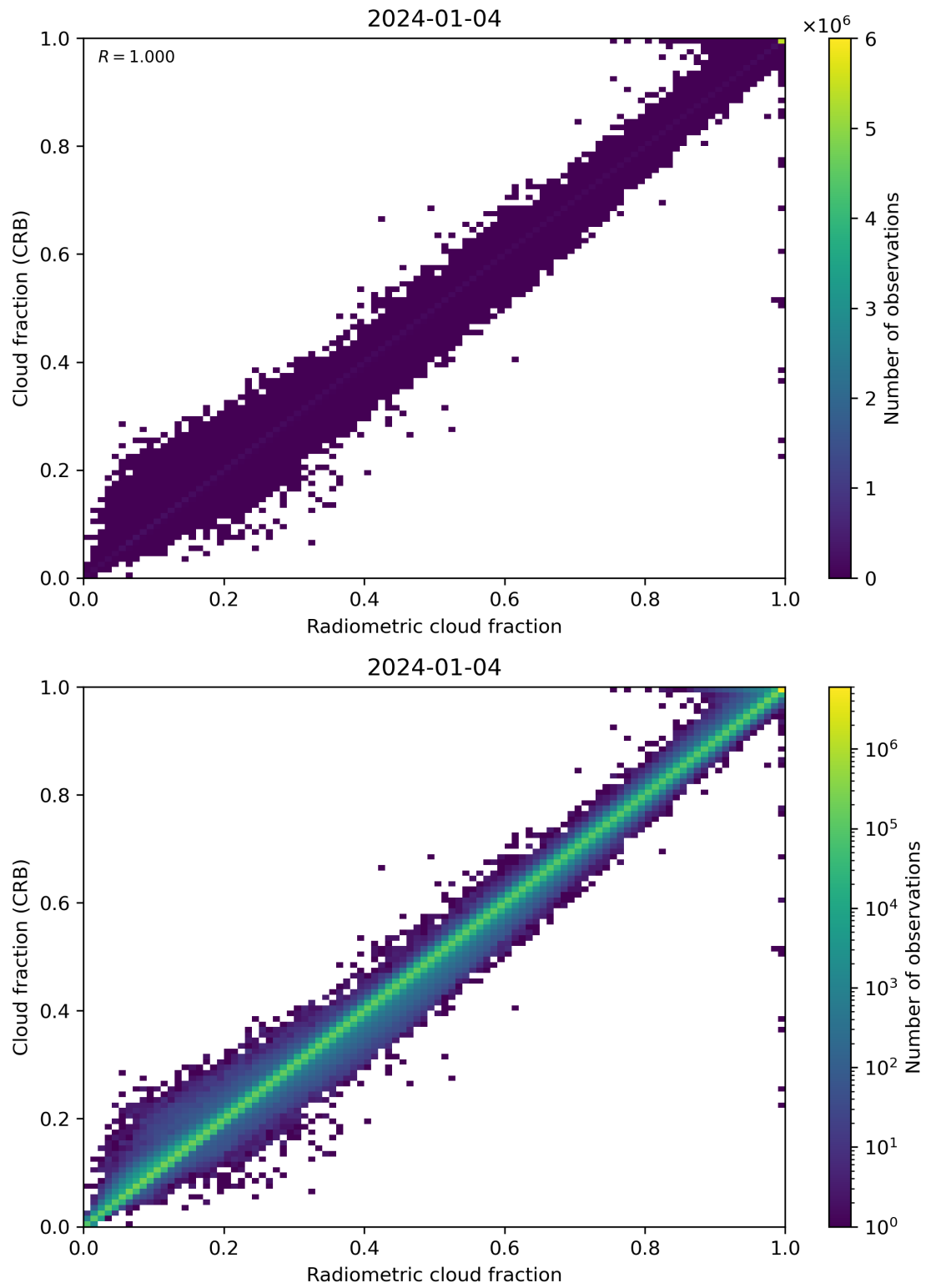
Figure 73: Scatter density plot of “Radiometric cloud fraction” against “Cloud fraction (CRB)” for 2024-01-03 to 2024-01-05.
