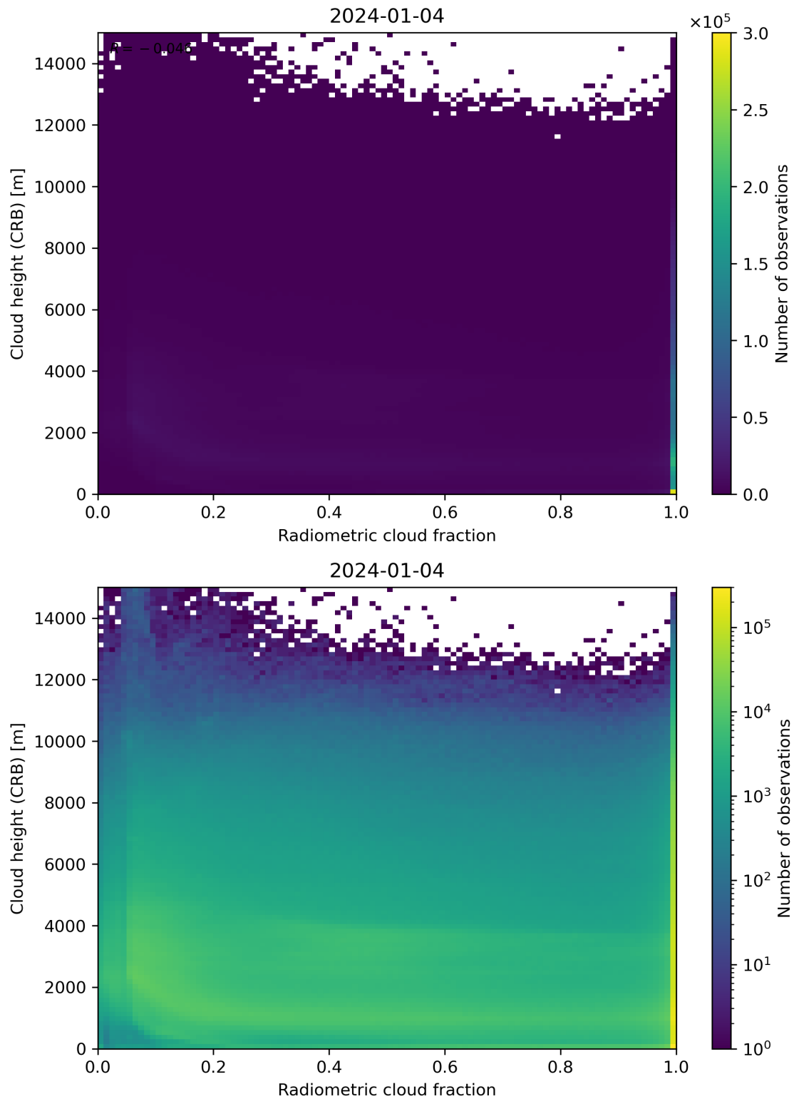
Figure 74: Scatter density plot of “Radiometric cloud fraction” against “Cloud height (CRB)” for 2024-01-03 to 2024-01-05.
