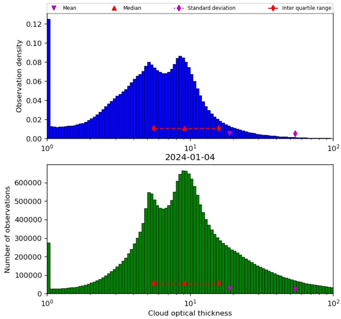
Figure 41: Histogram of “Cloud optical thickness” for 2024-01-03 to 2024-01-05
