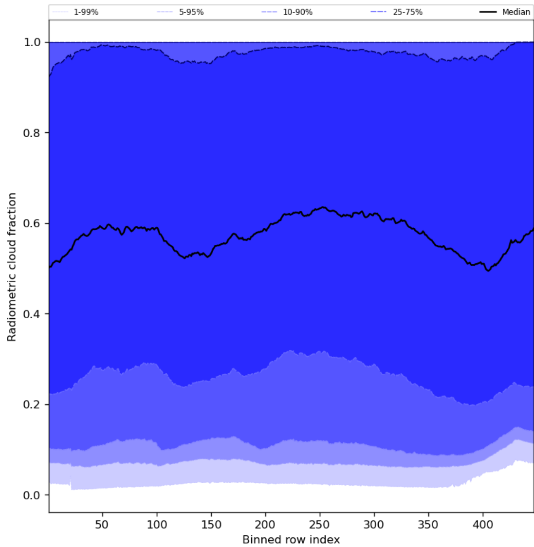
Figure 55: Along track statistics of “Radiometric cloud fraction” for 2024-01-03 to 2024-01-05
