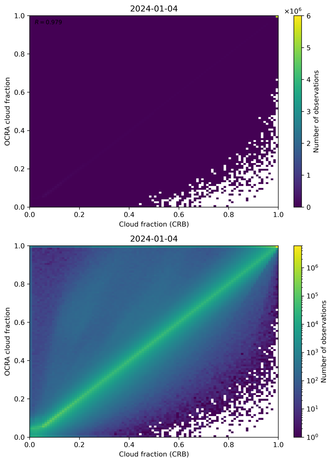
Figure 78: Scatter density plot of “Cloud fraction (CRB)” against “OCRA cloud fraction” for 2024-01-03 to 2024-01-05.
