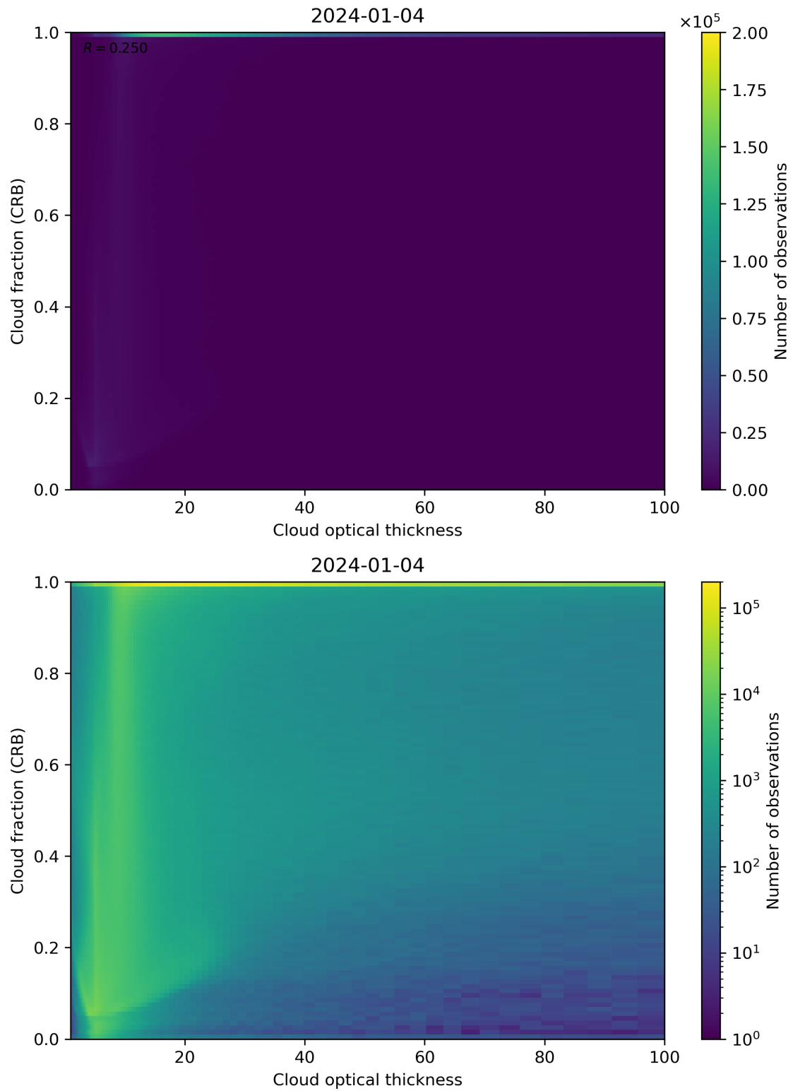
Figure 84: Scatter density plot of “Cloud optical thickness” against “Cloud fraction (CRB)” for 2024-01-03 to 2024-01-05.
