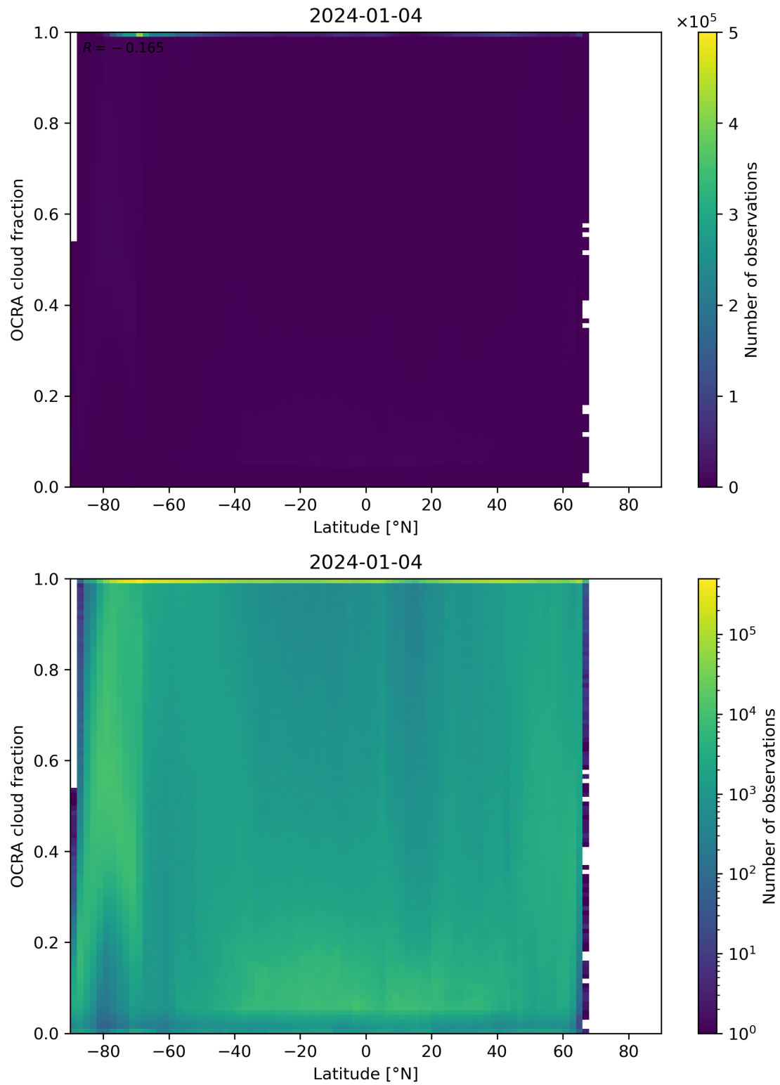
Figure 93: Scatter density plot of “Latitude” against “OCRA cloud fraction” for 2024-01-03 to 2024-01-05.
