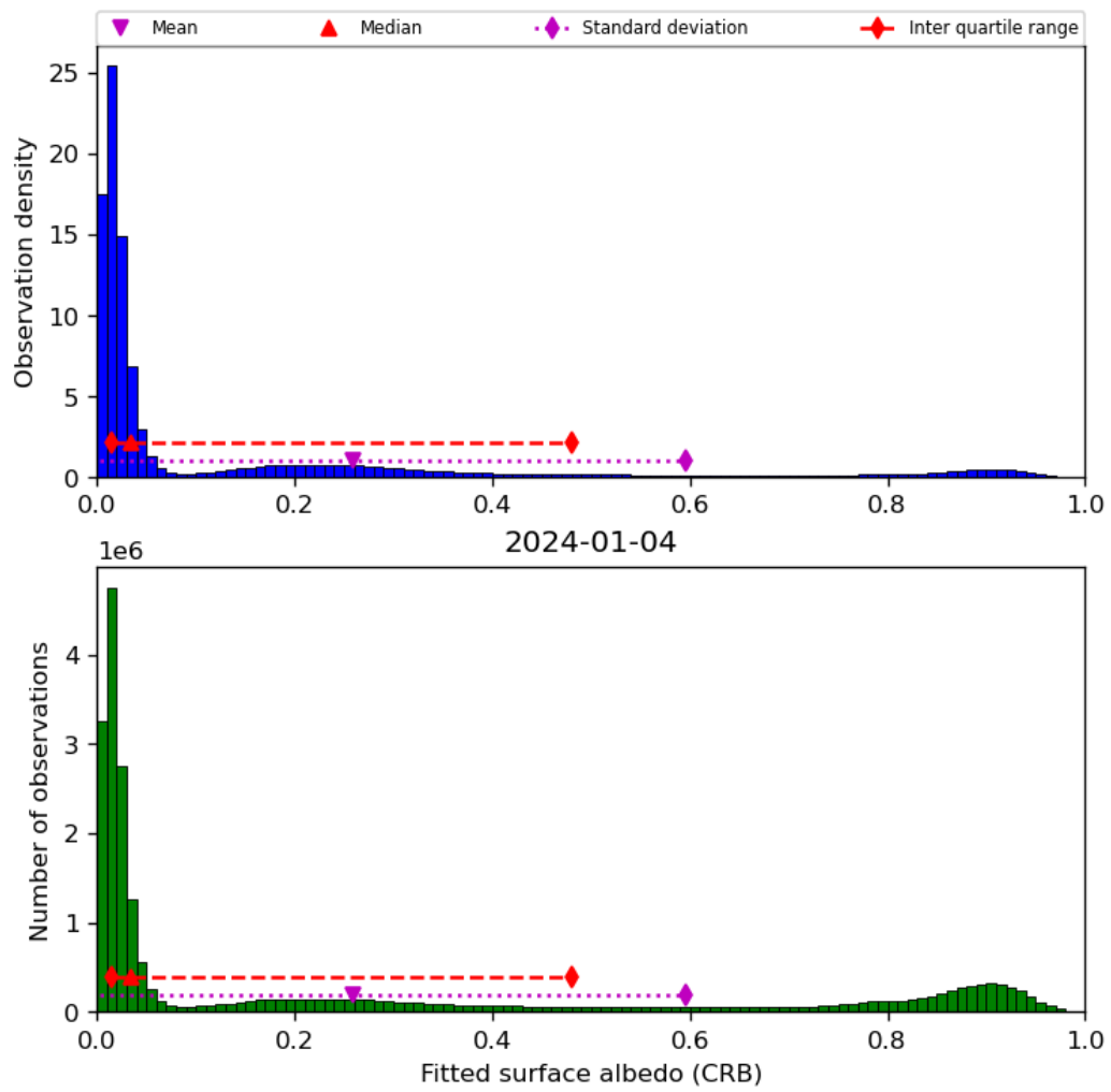
Figure 46: Histogram of “Fitted surface albedo (CRB)” for 2024-01-03 to 2024-01-05
