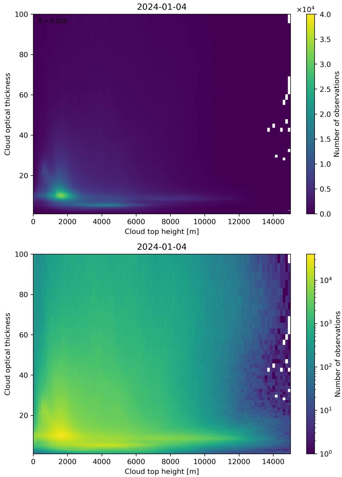
Figure 90: Scatter density plot of “Cloud top height” against “Cloud optical thickness” for 2024-01-03 to 2024-01-05.
