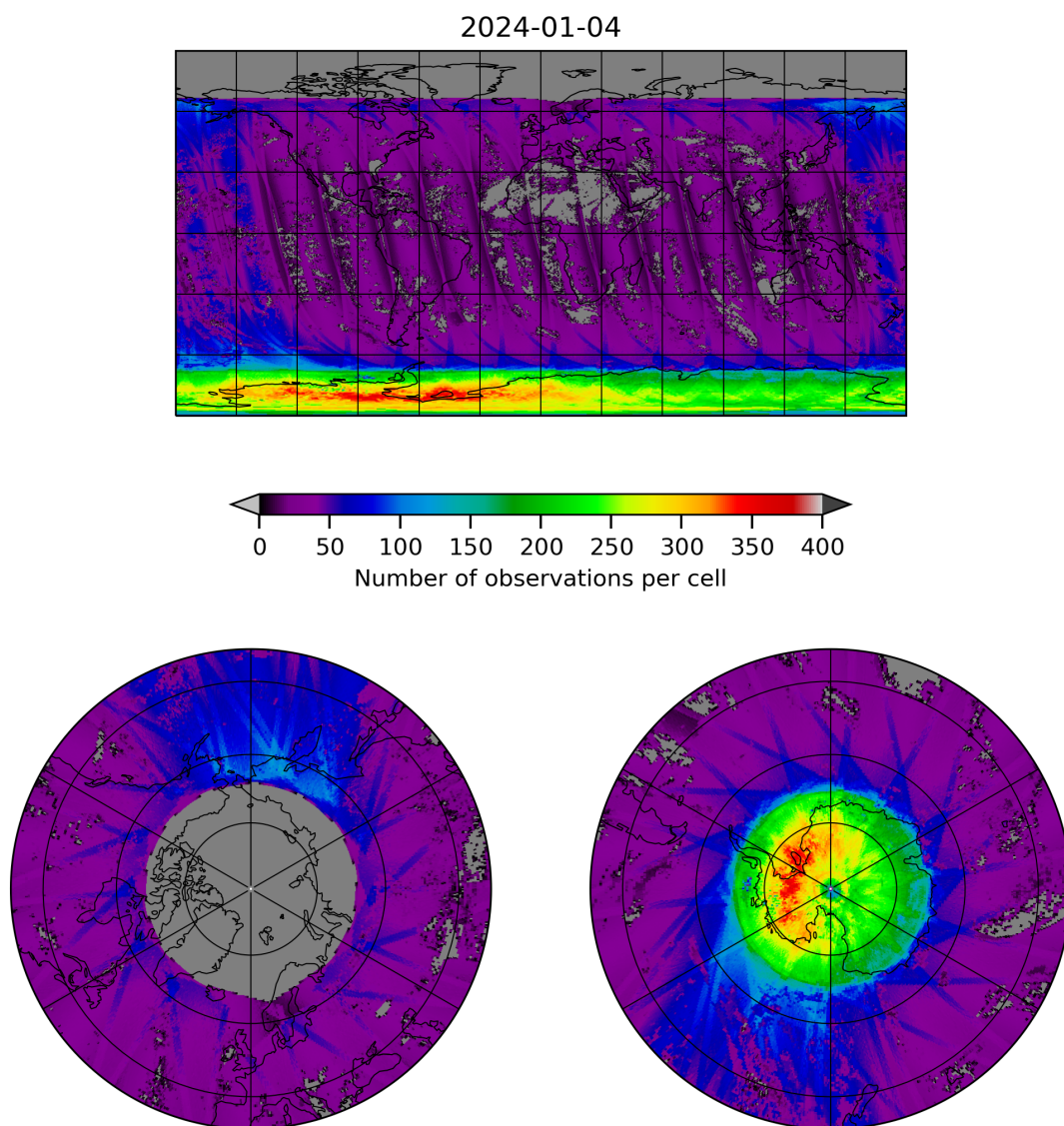
Figure 21: Map of the number of observations for 2024-01-03 to 2024-01-05
