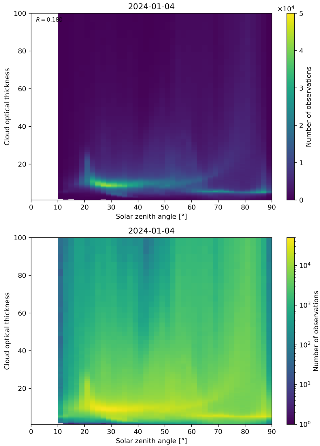
Figure 103: Scatter density plot of “Solar zenith angle” against “Cloud optical thickness” for 2024-01-03 to 2024-01-05.
