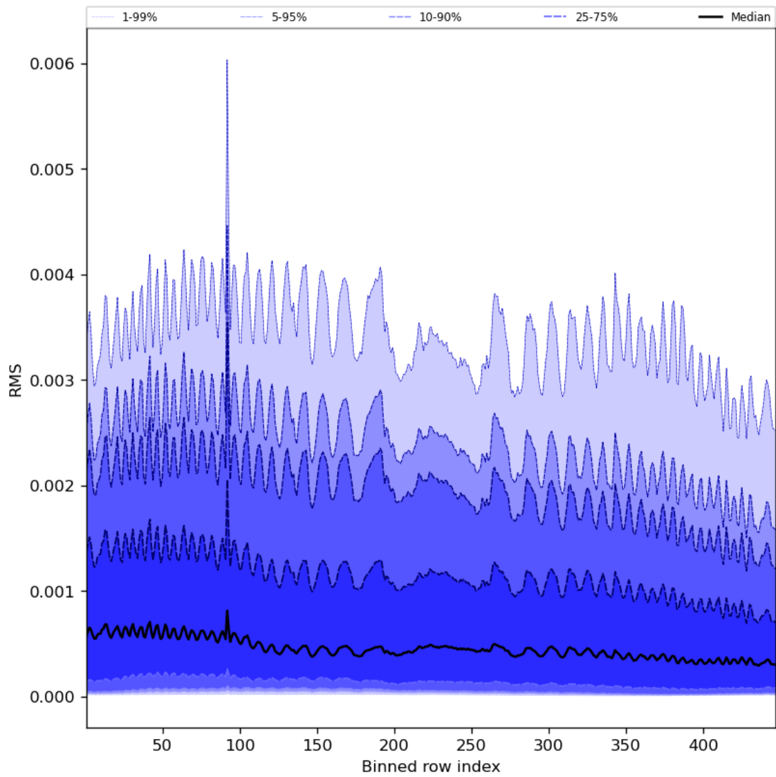
Figure 63: Along track statistics of “RMS” for 2024-01-03 to 2024-01-05
