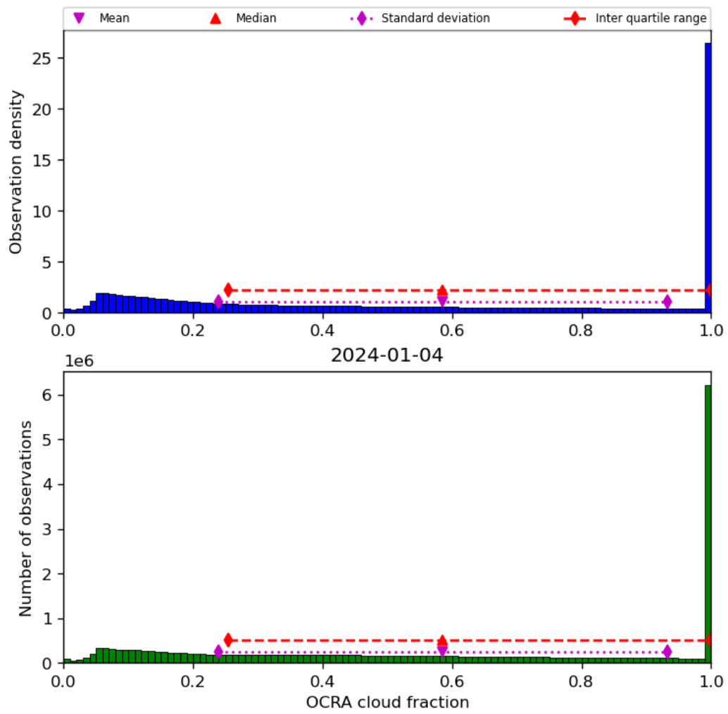
Figure 50: Histogram of “OCRA cloud fraction” for 2024-01-03 to 2024-01-05
