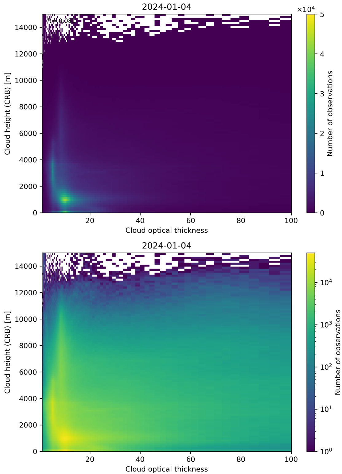
Figure 85: Scatter density plot of “Cloud optical thickness” against “Cloud height (CRB)” for 2024-01-03 to 2024-01-05.
