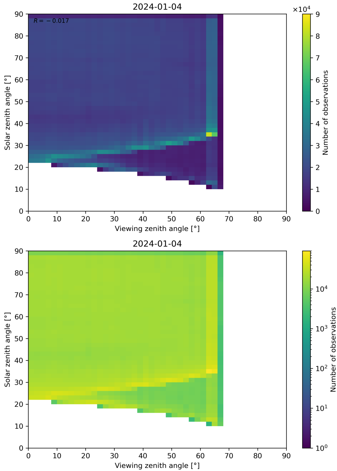
Figure 114: Scatter density plot of “Viewing zenith angle” against “Solar zenith angle” for 2024-01-03 to 2024-01-05.
