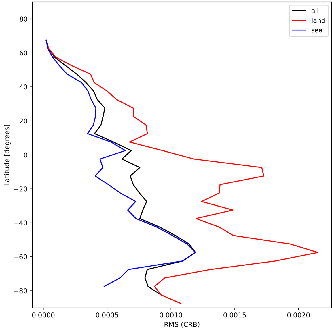
Figure 32: Zonal average of “RMS (CRB)” for 2024-01-03 to 2024-01-05.
