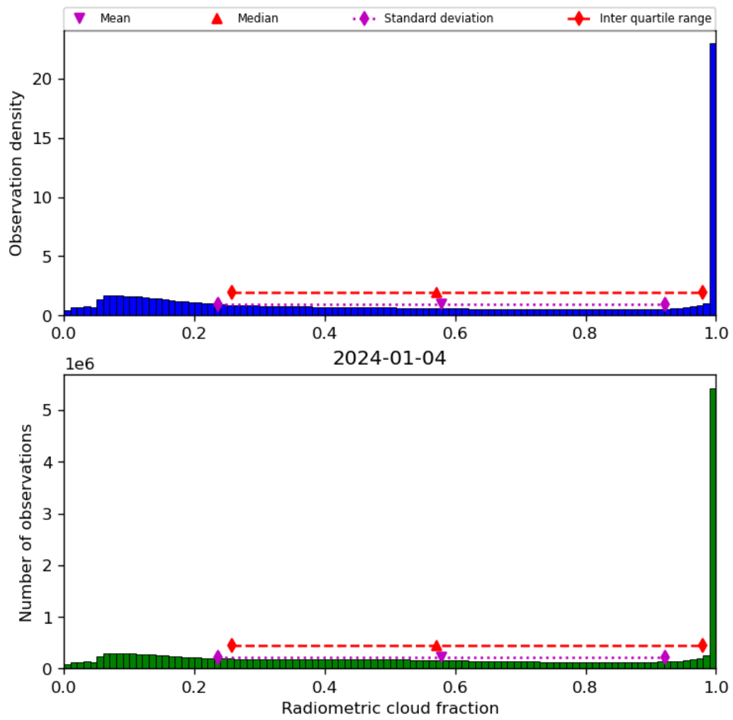
Figure 39: Histogram of “Radiometric cloud fraction” for 2024-01-03 to 2024-01-05
