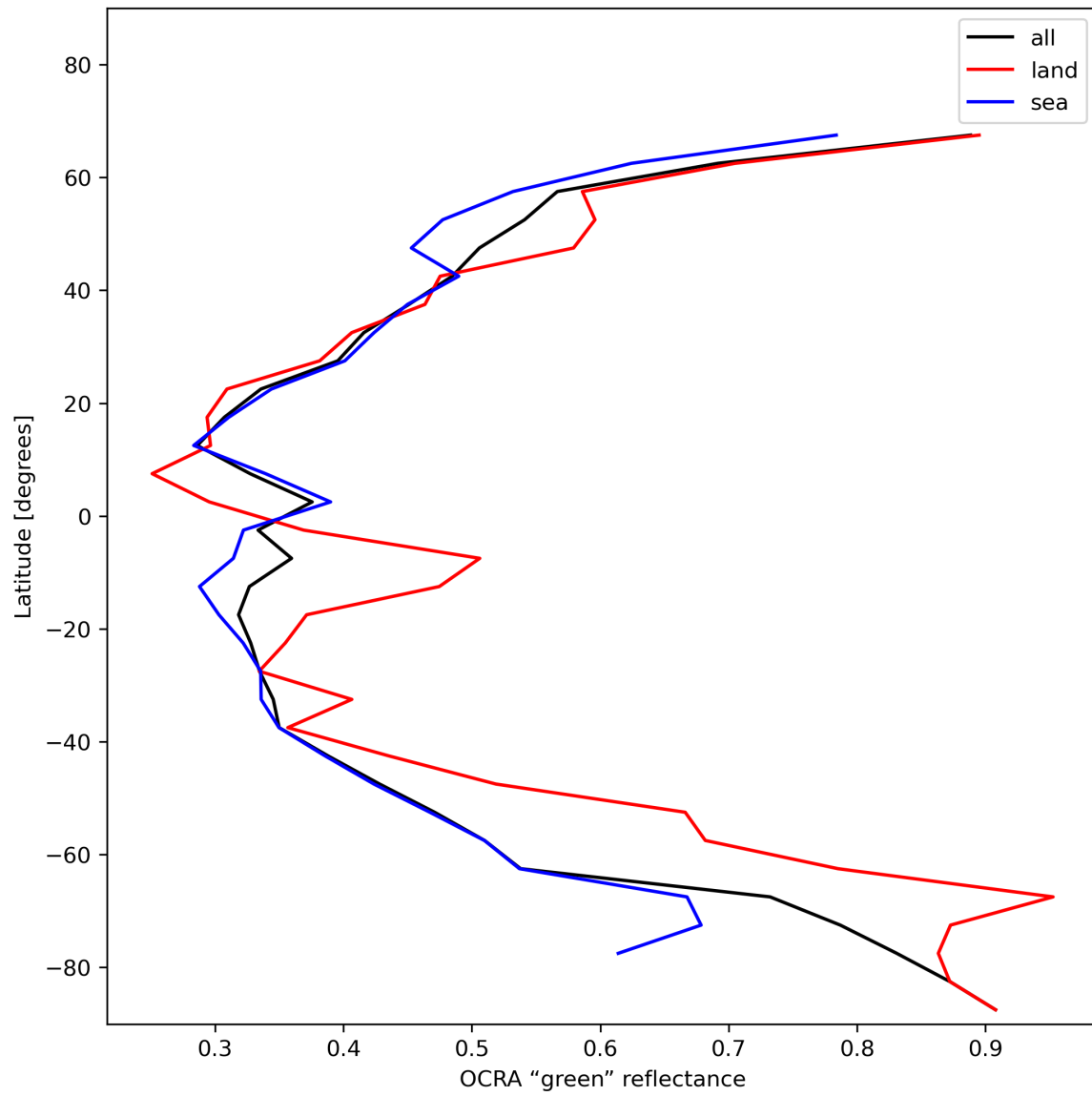
Figure 36: Zonal average of “OCRA “green” reflectance” for 2024-01-03 to 2024-01-05.
