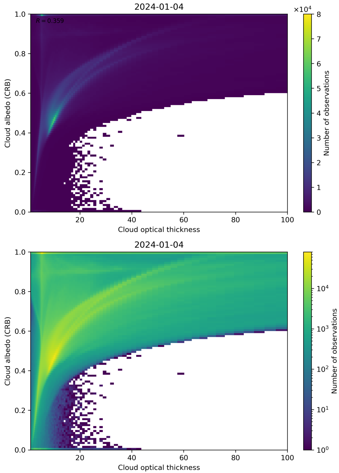
Figure 82: Scatter density plot of “Cloud optical thickness” against “Cloud albedo (CRB)” for 2024-01-03 to 2024-01-05.
