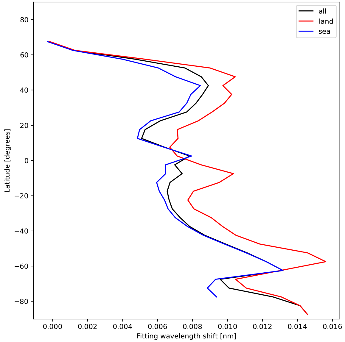
Figure 33: Zonal average of “Fitting wavelength shift” for 2024-01-03 to 2024-01-05.
