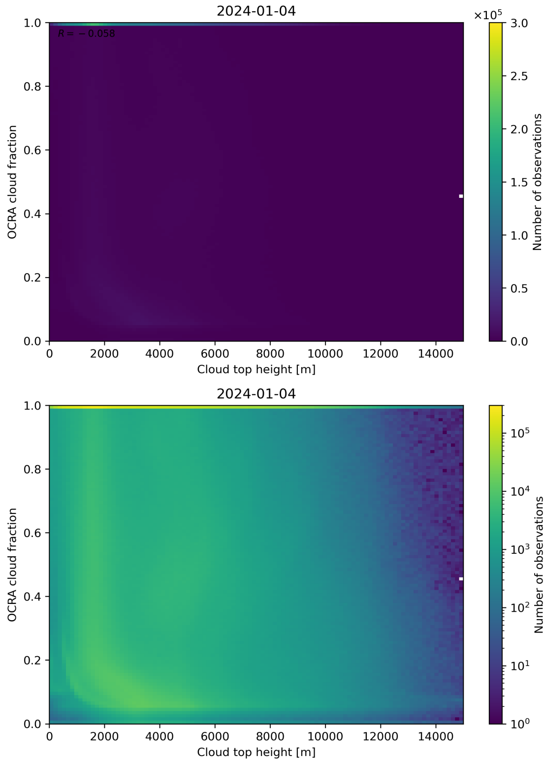
Figure 87: Scatter density plot of “Cloud top height” against “OCRA cloud fraction” for 2024-01-03 to 2024-01-05.
