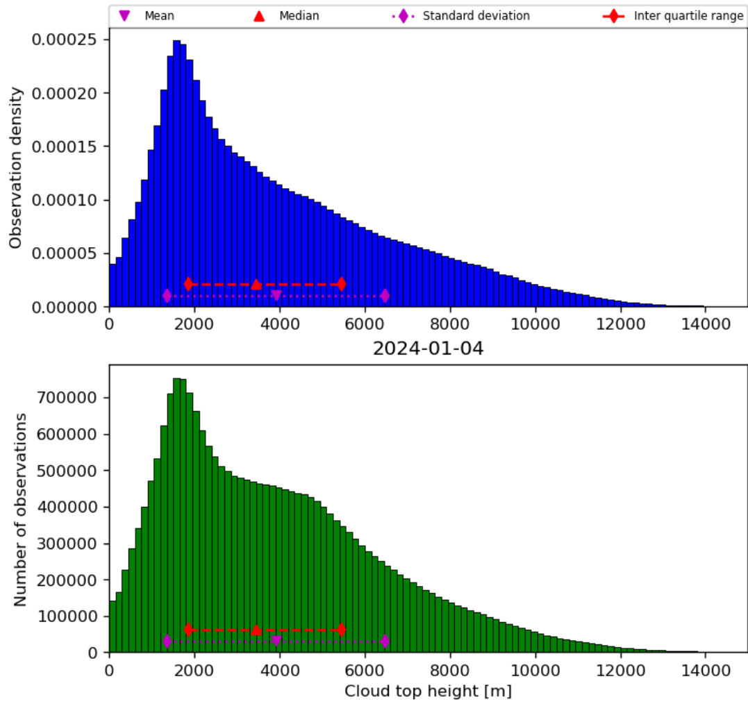
Figure 40: Histogram of “Cloud top height” for 2024-01-03 to 2024-01-05
