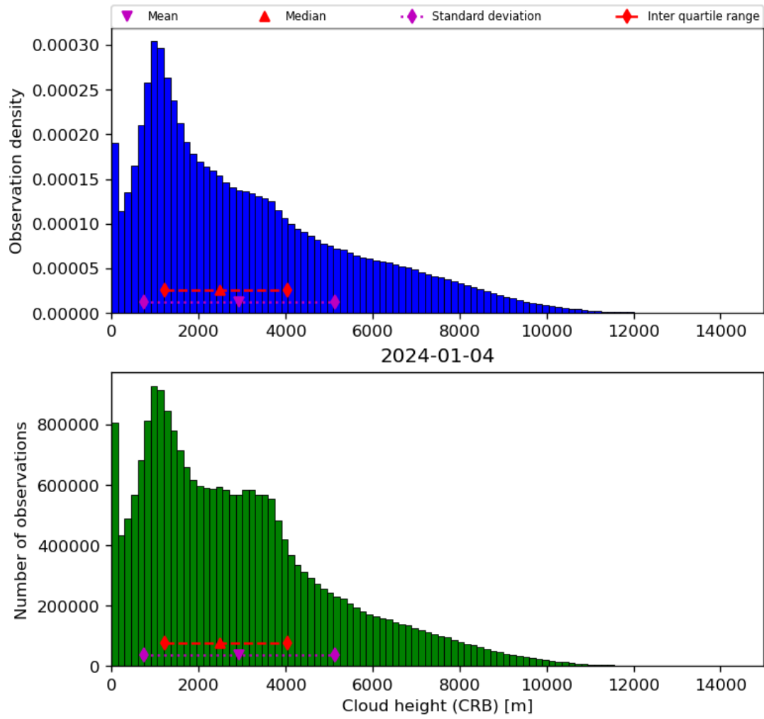
Figure 43: Histogram of “Cloud height (CRB)” for 2024-01-03 to 2024-01-05
