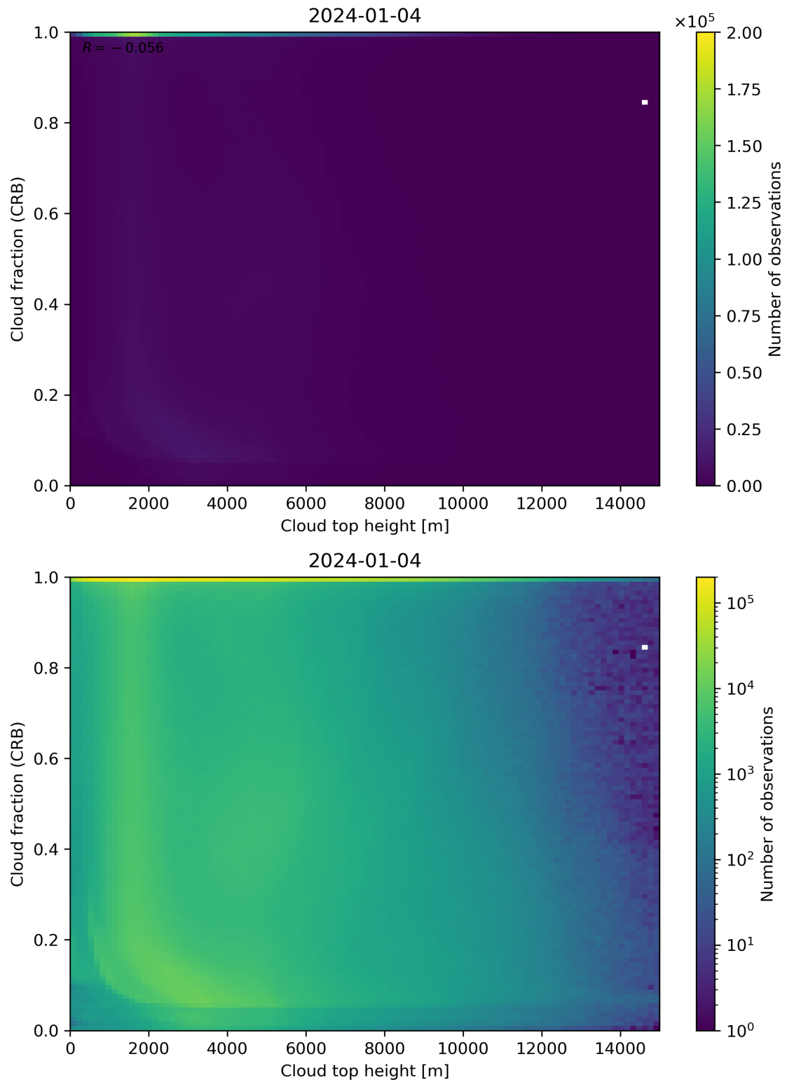
Figure 88: Scatter density plot of “Cloud top height” against “Cloud fraction (CRB)” for 2024-01-03 to 2024-01-05.
