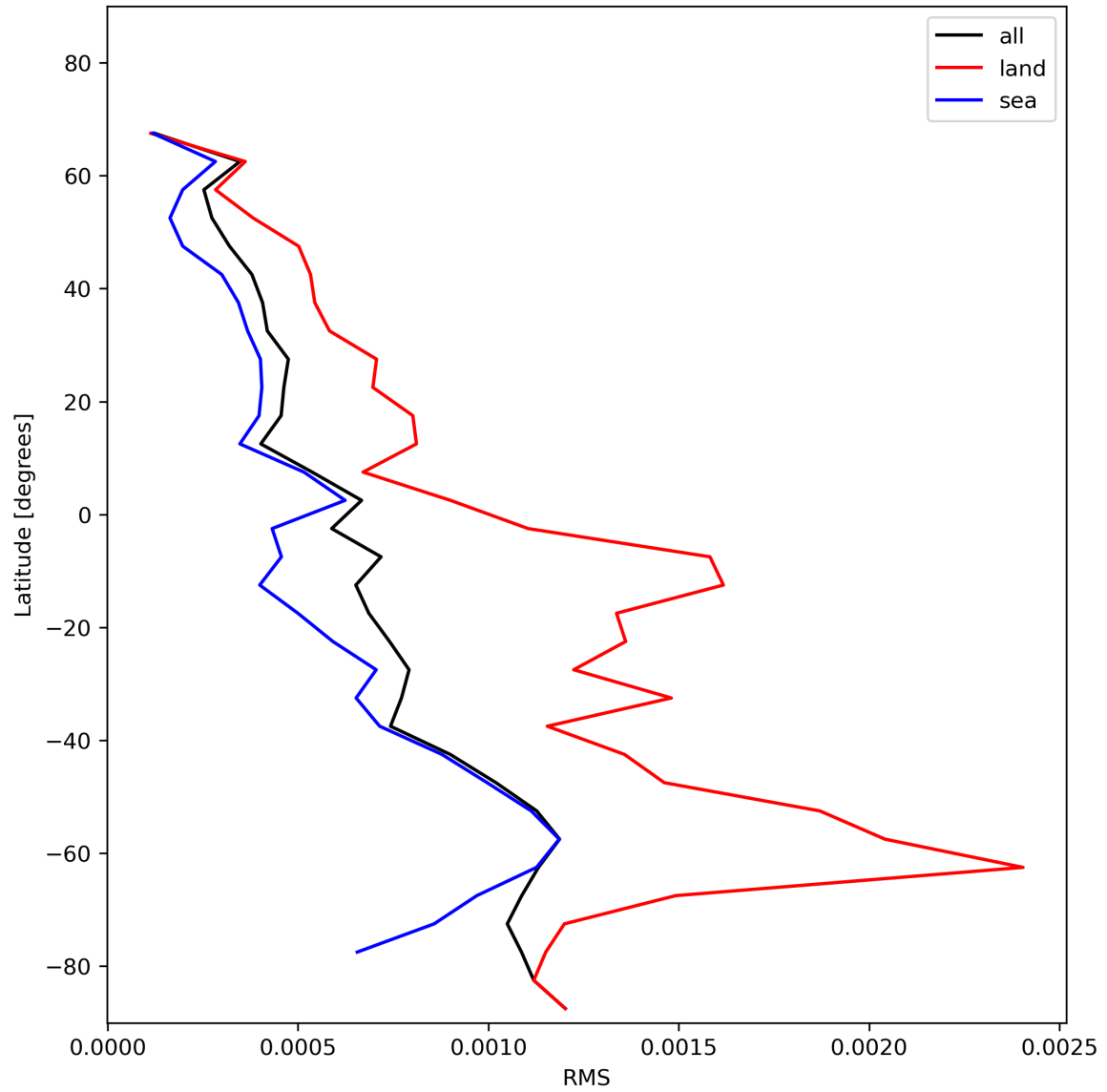
Figure 31: Zonal average of “RMS” for 2024-01-03 to 2024-01-05.
