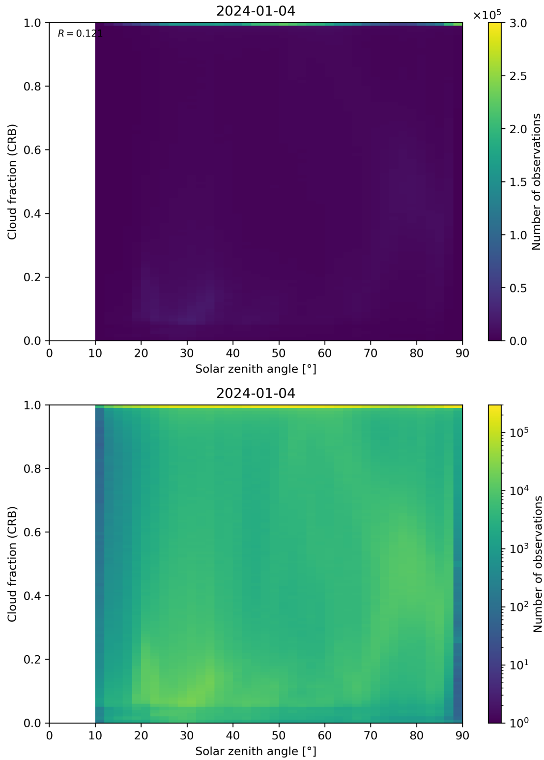
Figure 101: Scatter density plot of “Solar zenith angle” against “Cloud fraction (CRB)” for 2024-01-03 to 2024-01-05.
