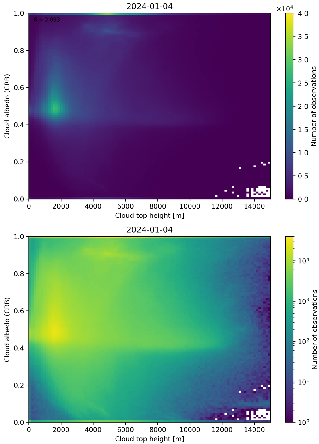
Figure 86: Scatter density plot of “Cloud top height” against “Cloud albedo (CRB)” for 2024-01-03 to 2024-01-05.
