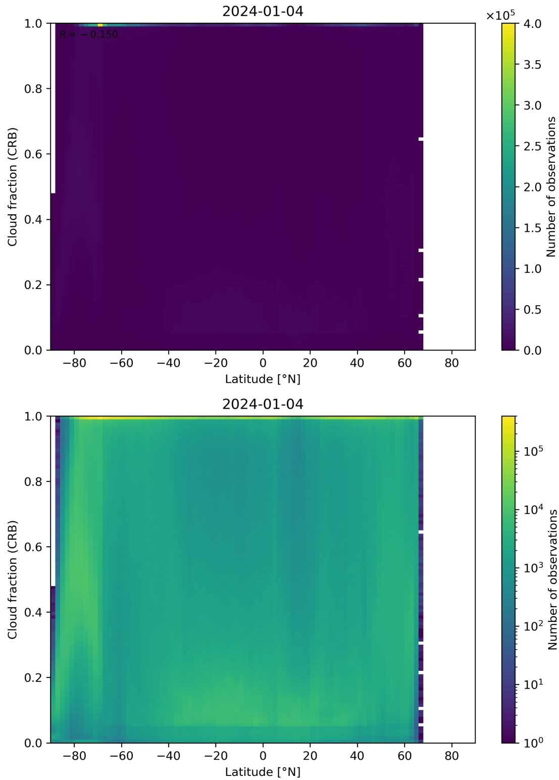
Figure 94: Scatter density plot of “Latitude” against “Cloud fraction (CRB)” for 2024-01-03 to 2024-01-05.
