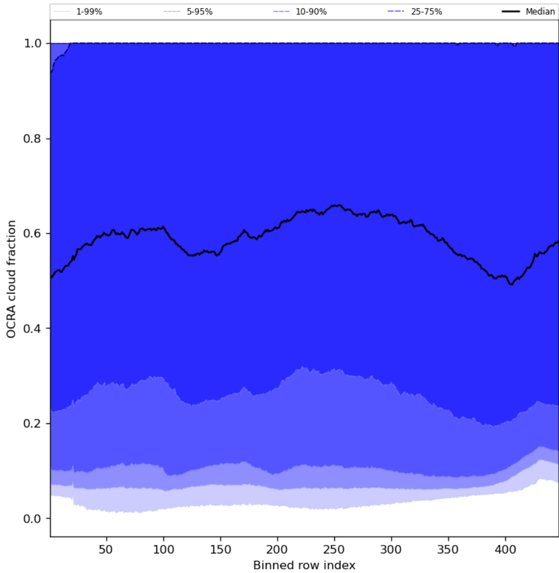
Figure 66: Along track statistics of “OCRA cloud fraction” for 2024-01-03 to 2024-01-05
