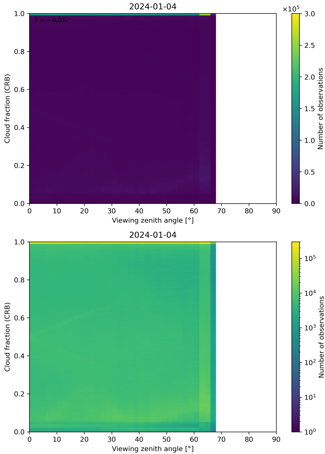
Figure 109: Scatter density plot of “Viewing zenith angle” against “Cloud fraction (CRB)” for 2024-01-03 to 2024-01-05.
