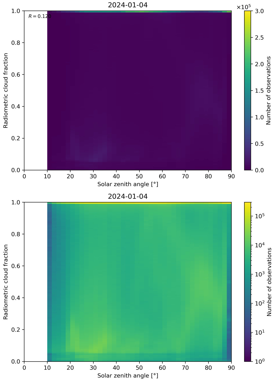
Figure 99: Scatter density plot of “Solar zenith angle” against “Radiometric cloud fraction” for 2024-01-03 to 2024-01-05.
