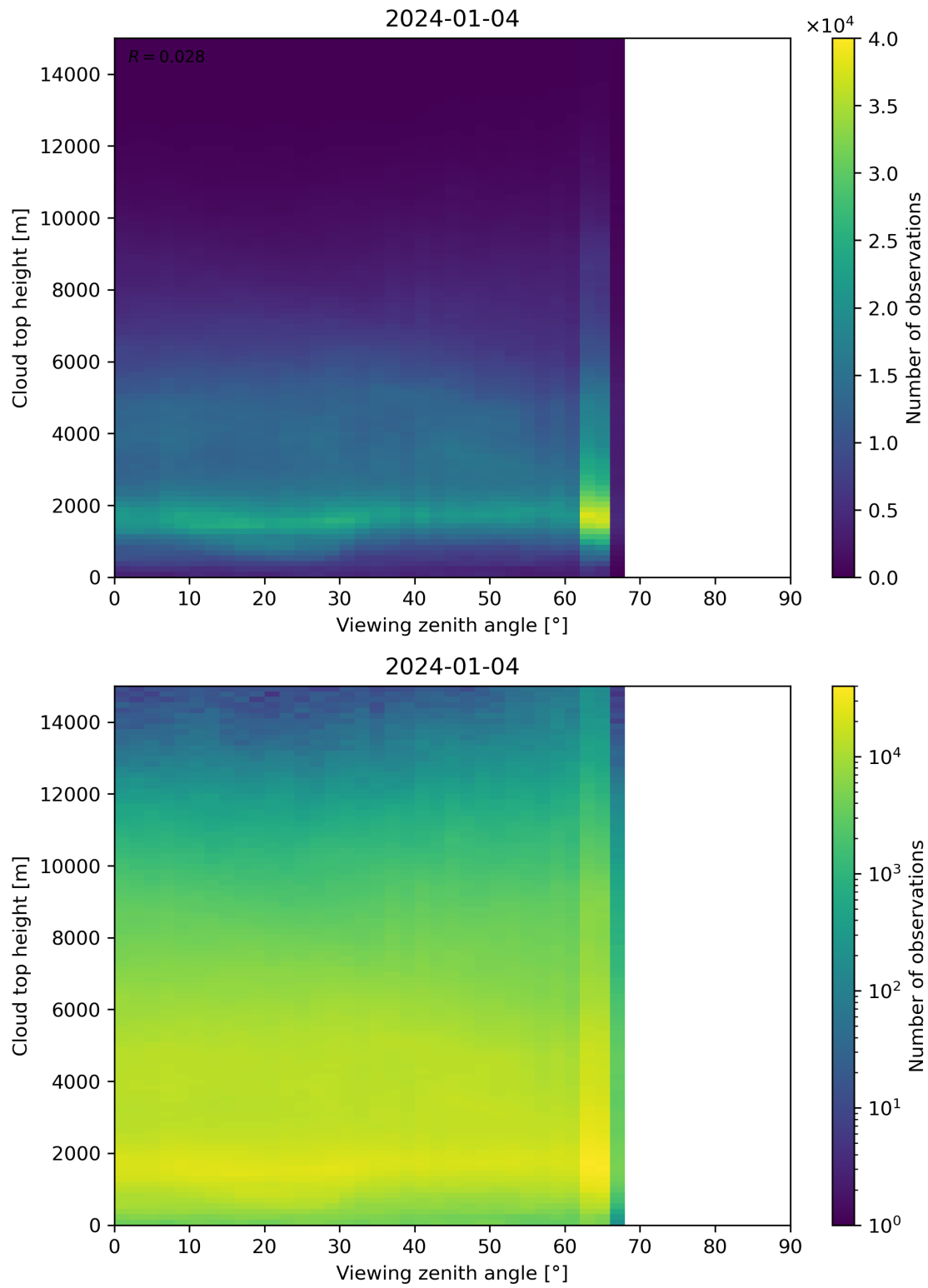
Figure 112: Scatter density plot of “Viewing zenith angle” against “Cloud top height” for 2024-01-03 to 2024-01-05.
