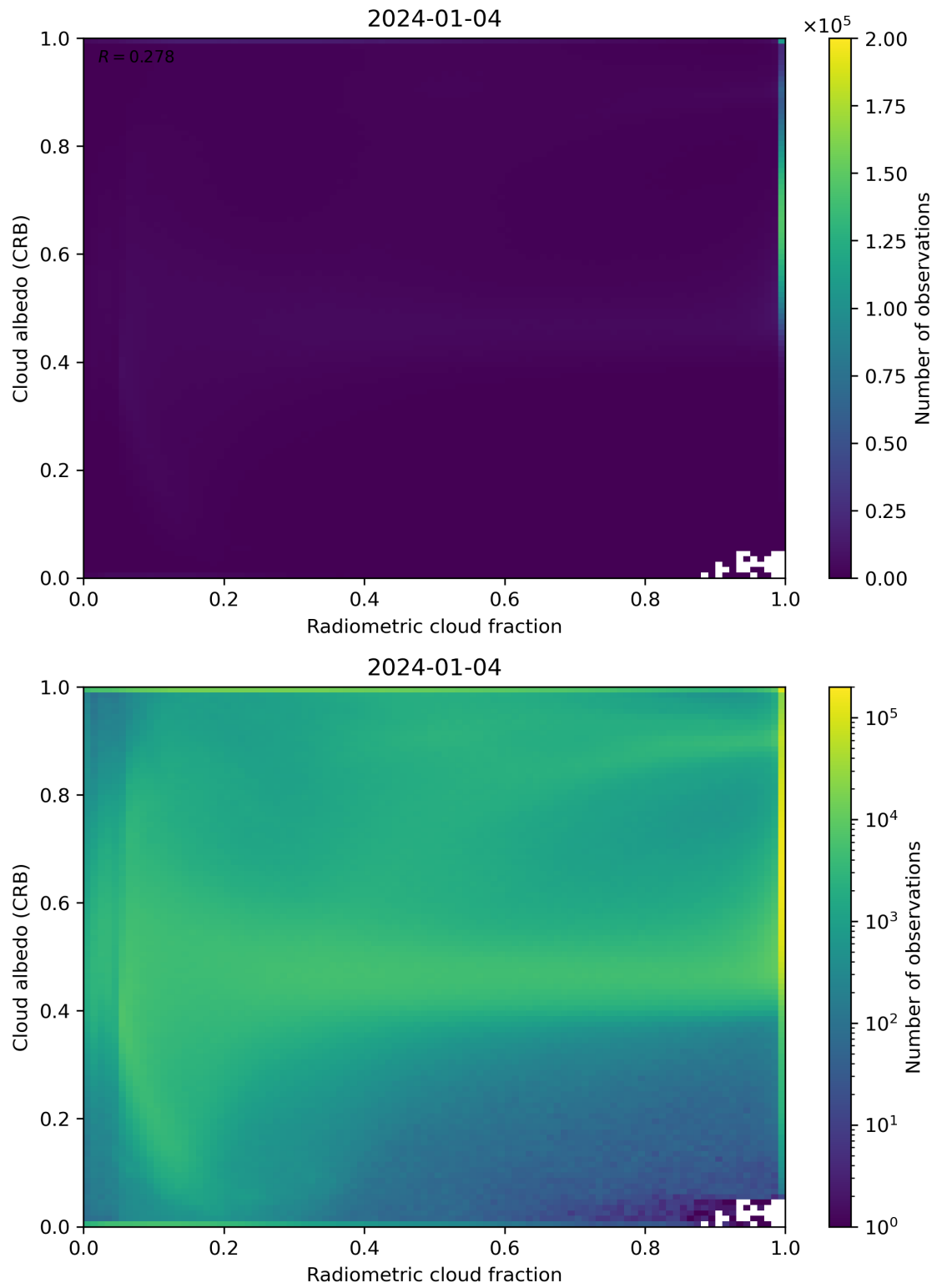
Figure 71: Scatter density plot of “Radiometric cloud fraction” against “Cloud albedo (CRB)” for 2024-01-03 to 2024-01-05.
