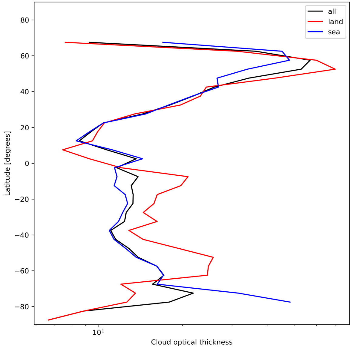
Figure 25: Zonal average of “Cloud optical thickness” for 2024-01-03 to 2024-01-05.
