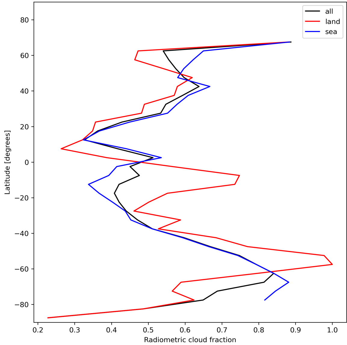
Figure 23: Zonal average of “Radiometric cloud fraction” for 2024-01-03 to 2024-01-05.
