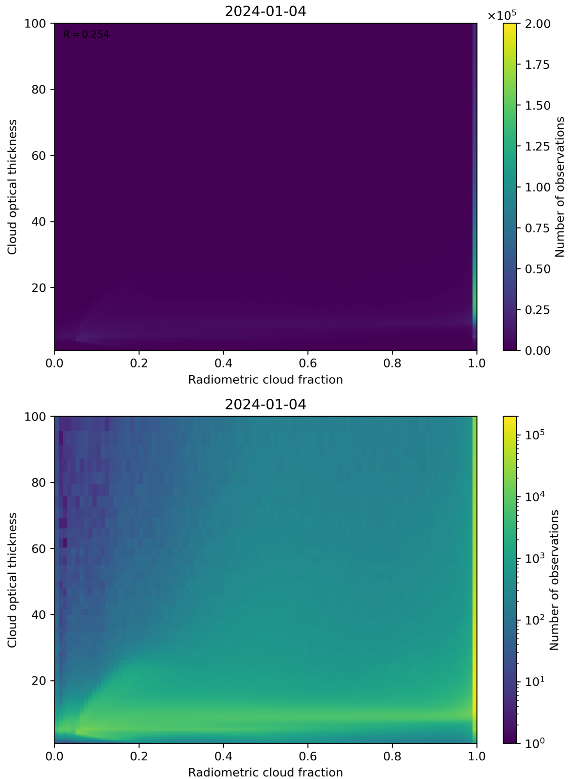
Figure 75: Scatter density plot of “Radiometric cloud fraction” against “Cloud optical thickness” for 2024-01-03 to 2024-01-05.
