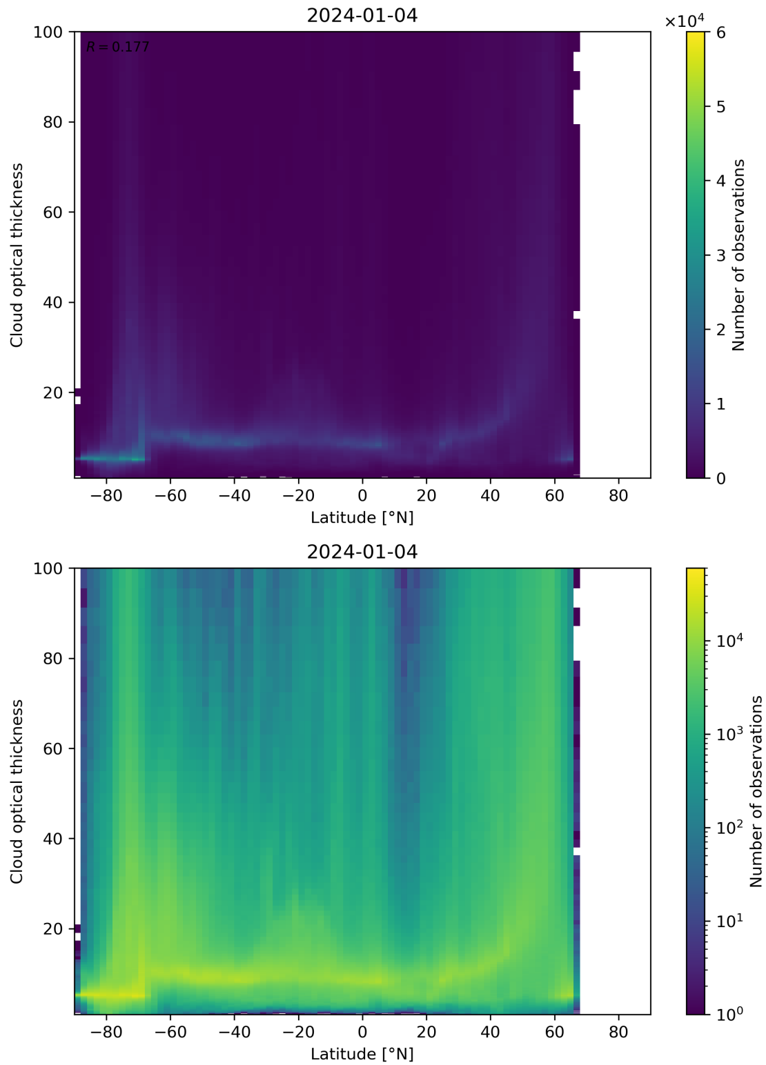
Figure 96: Scatter density plot of “Latitude” against “Cloud optical thickness” for 2024-01-03 to 2024-01-05.
