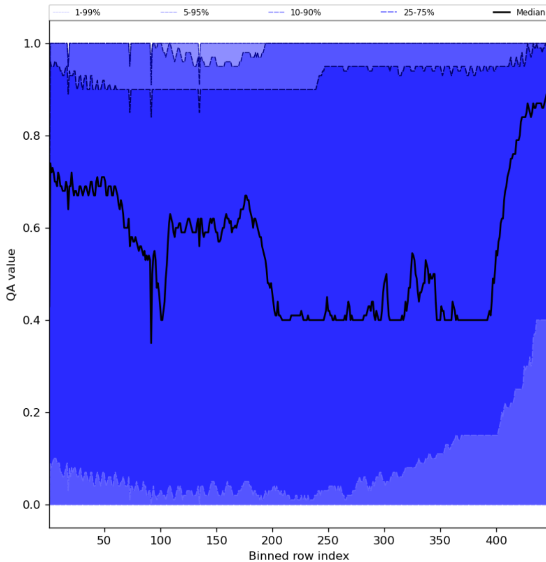
Figure 54: Along track statistics of “QA value” for 2024-01-03 to 2024-01-05
